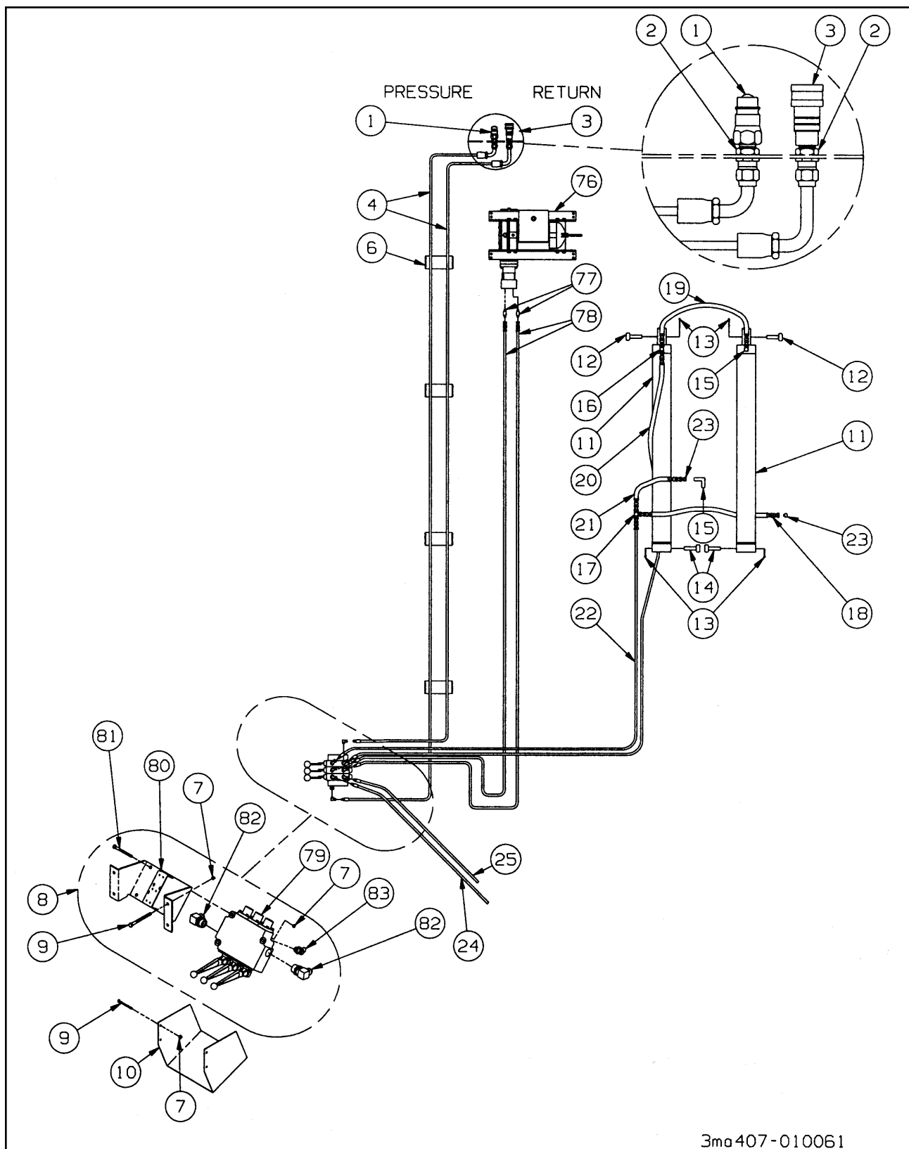
Figure 1-3 Hydraulic System
