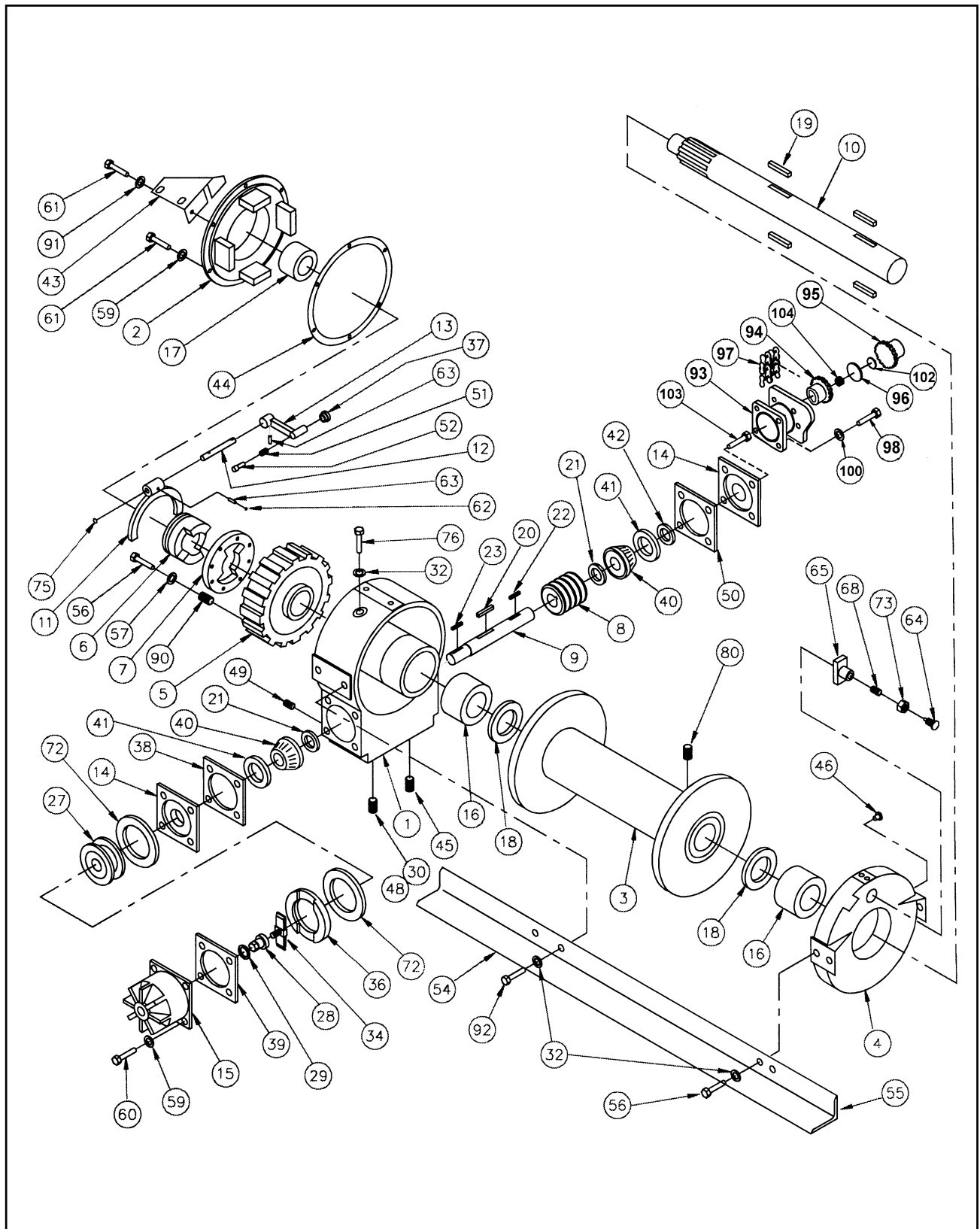
Figure 1-32 20,000# Winch Assembly
