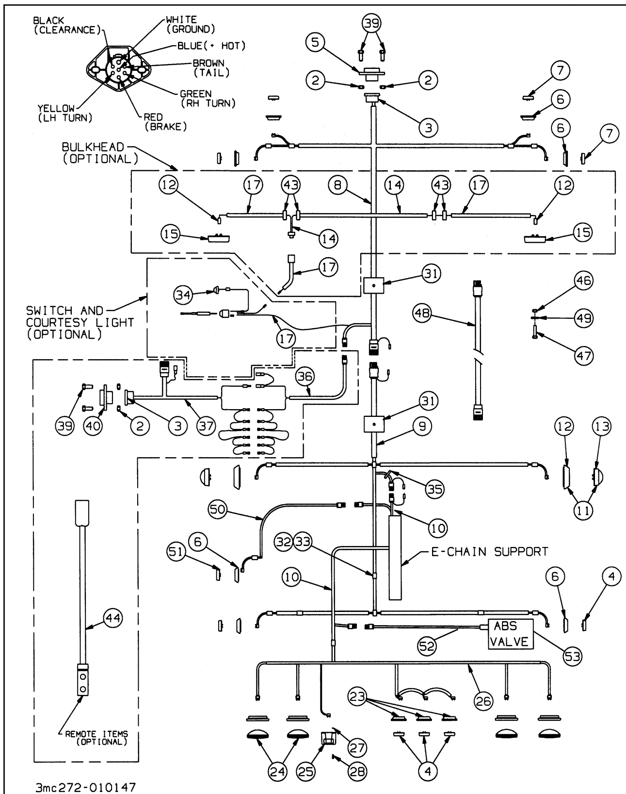
Figure 1-13 Electrical System
