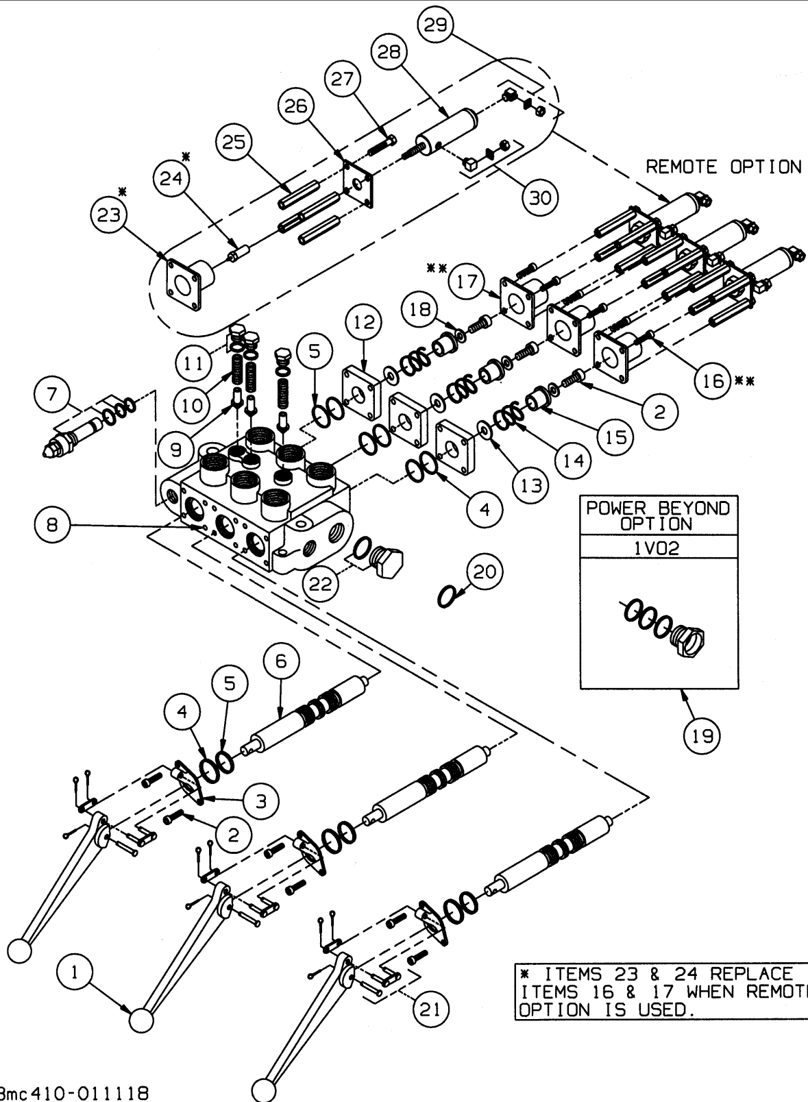
Figure 1-12 Three Spool Valve
