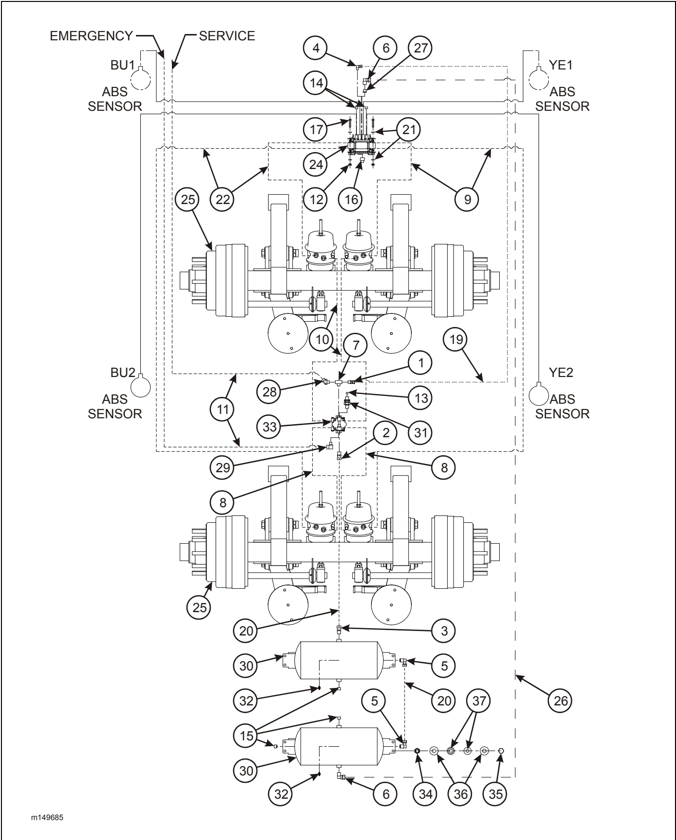
Figure 2-19: Air Brake System, Tandem Axle
