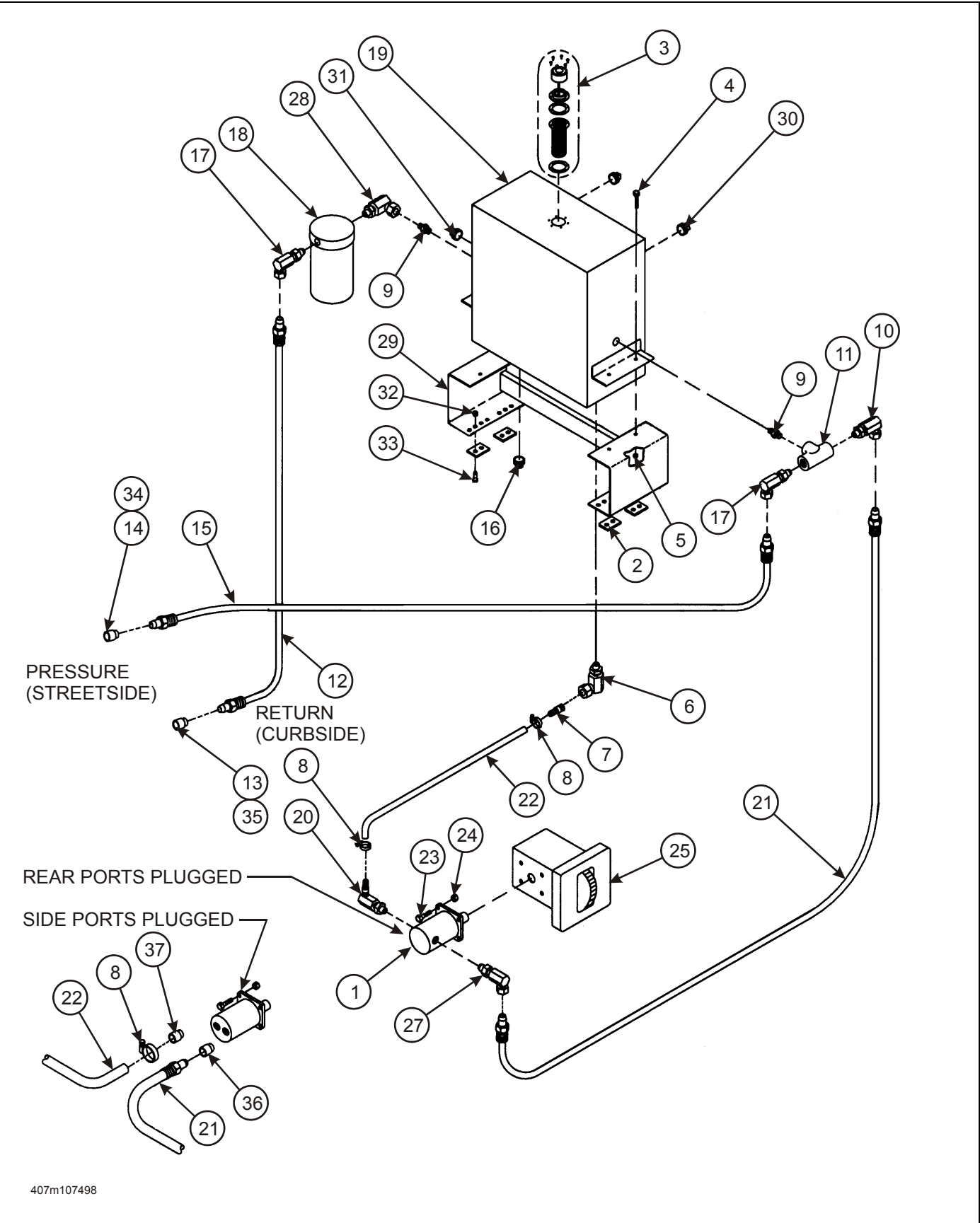
Figure 2-56: Hydraulic Wet Kit Assembly (Option)
