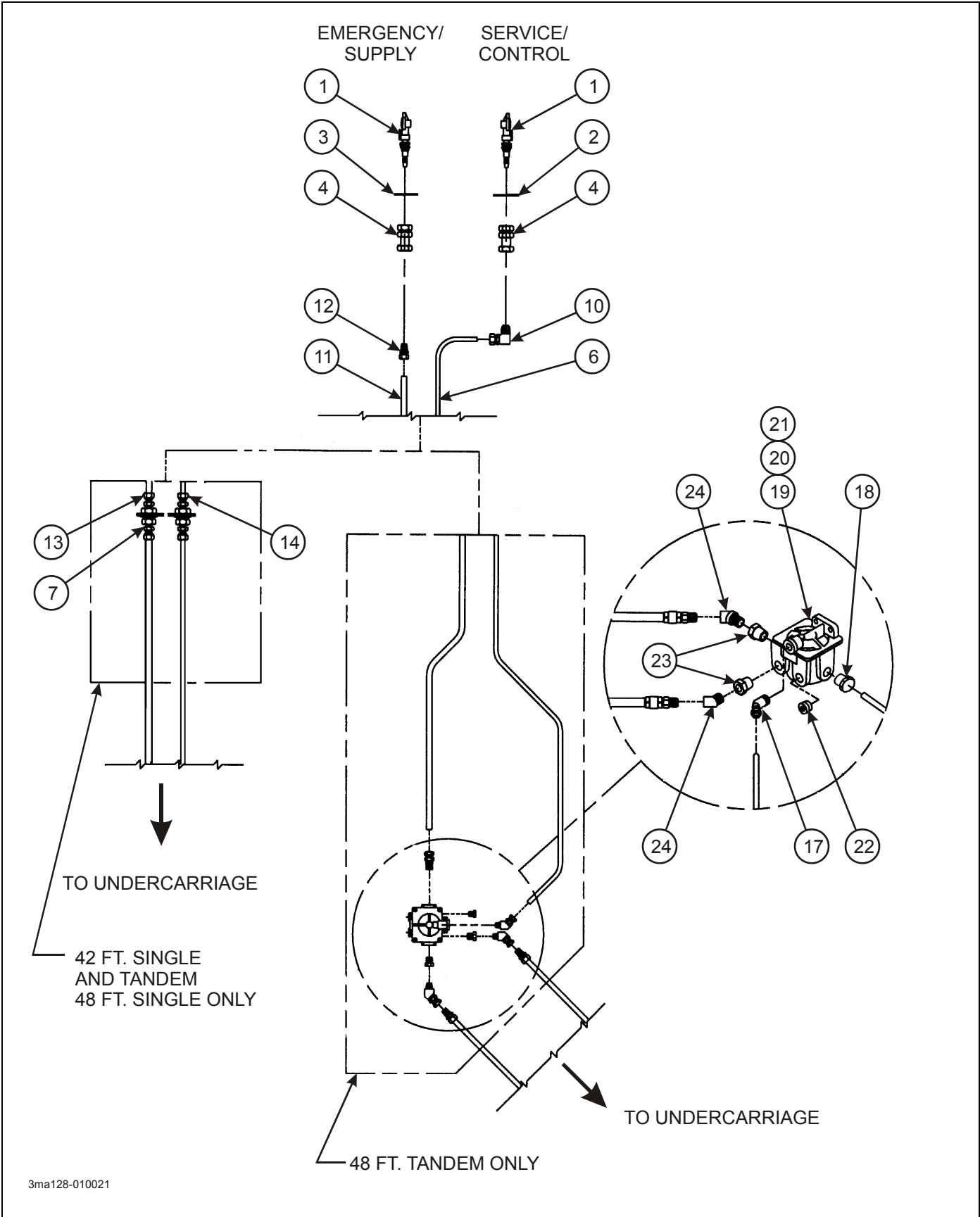
Figure 2-16: Air System
