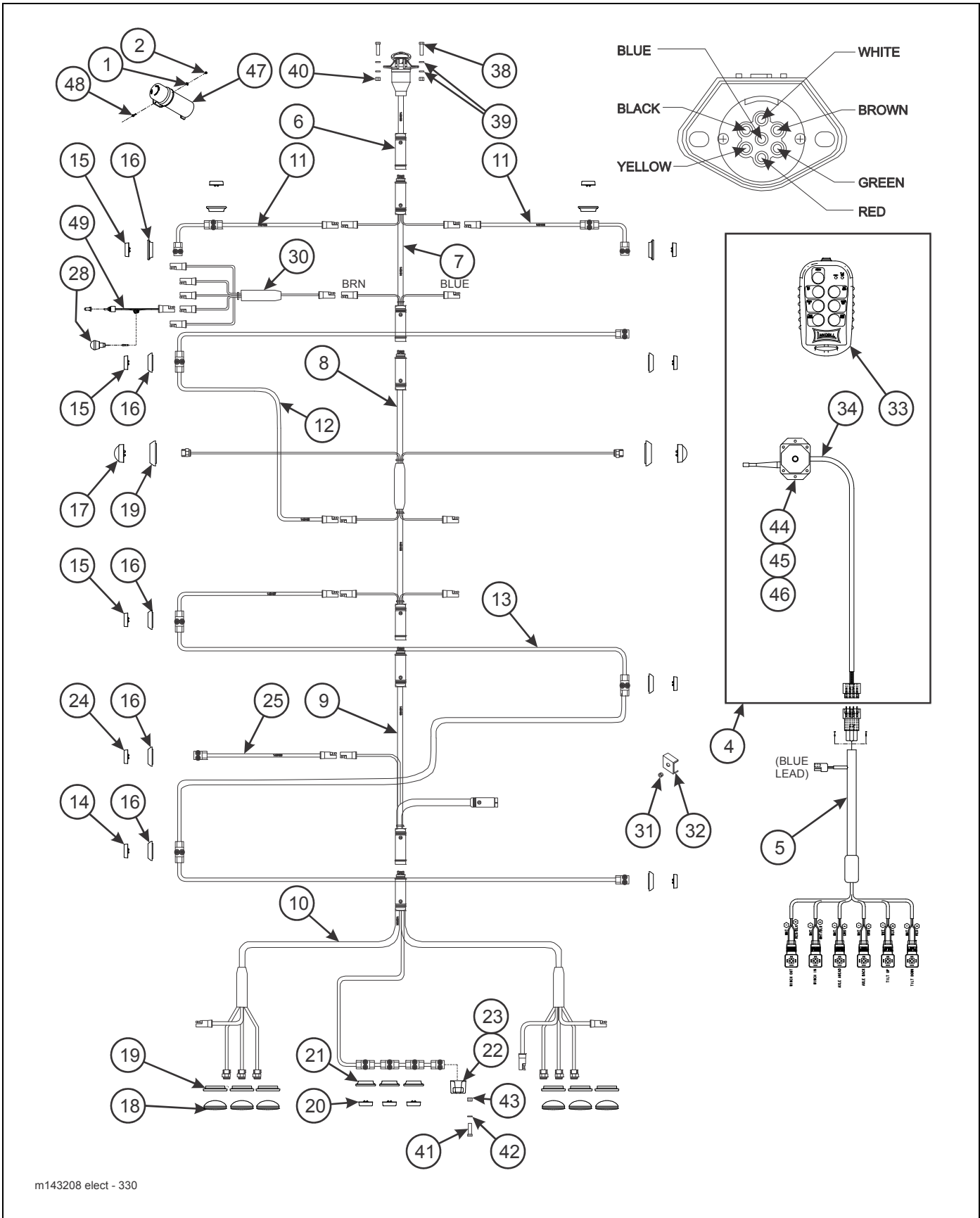
Figure 2-13: Electrical System
