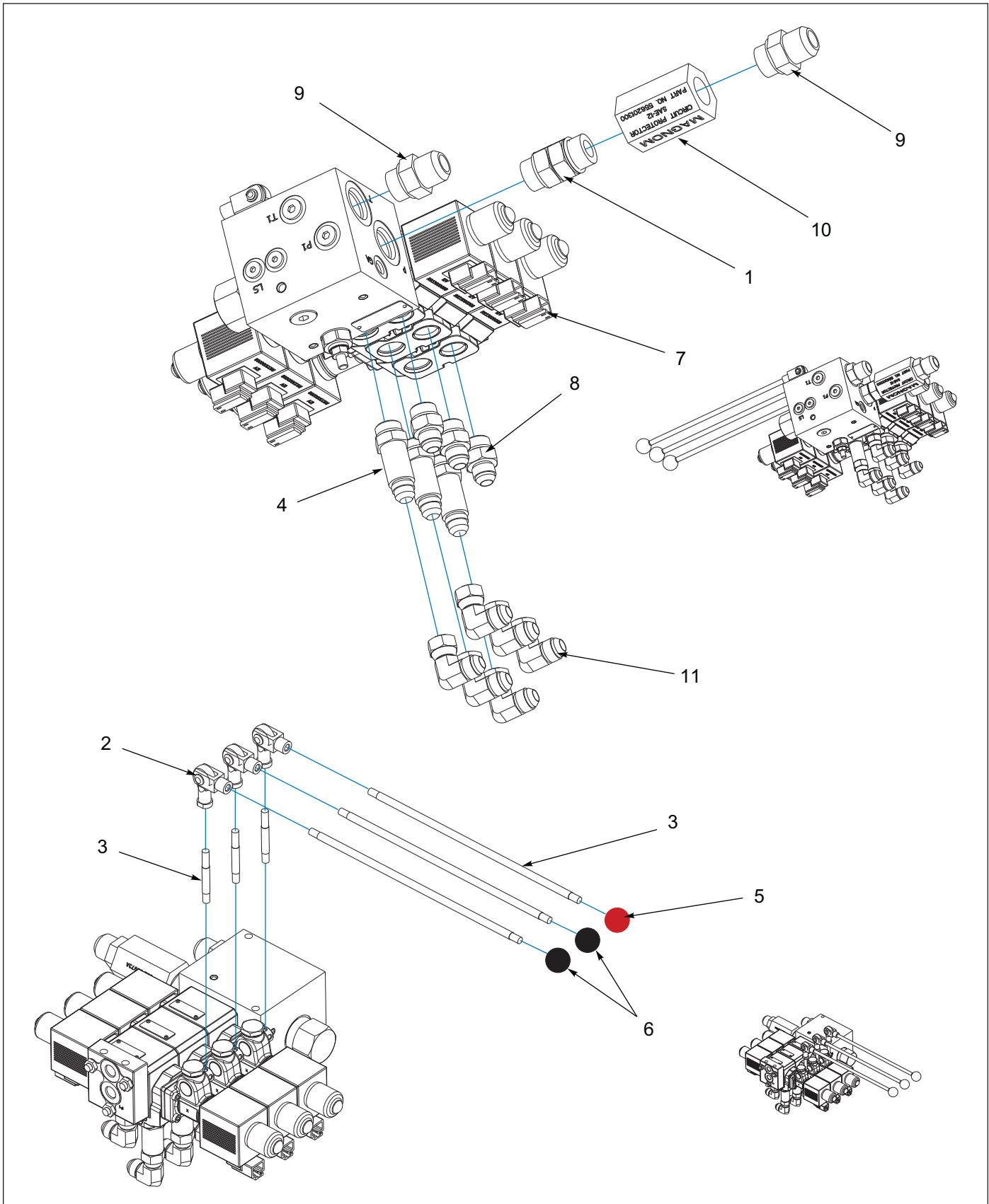
Figure 10-9: Valve Assembly
