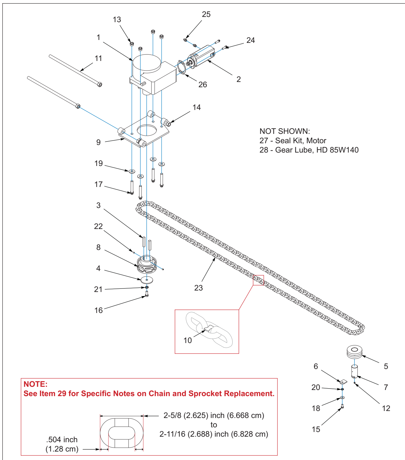
Figure 11-1: Chain Drive Installation, Braden
