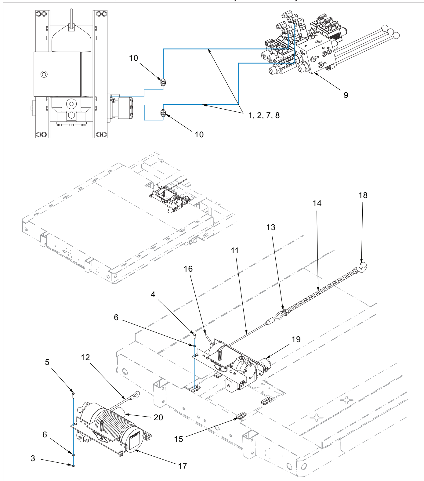
Figure 11-3: Winch Installation, Braden 12K / 20K (Options)
