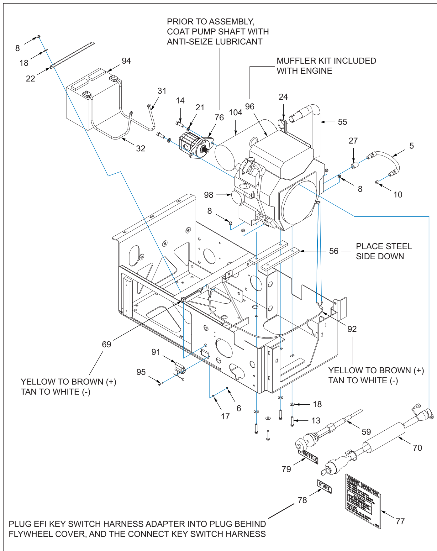
Figure 12-8: Engine Assembly, Kohler 25HP EFI, Gasoline, 30 Gallon (OPTION) (3 of 5)
