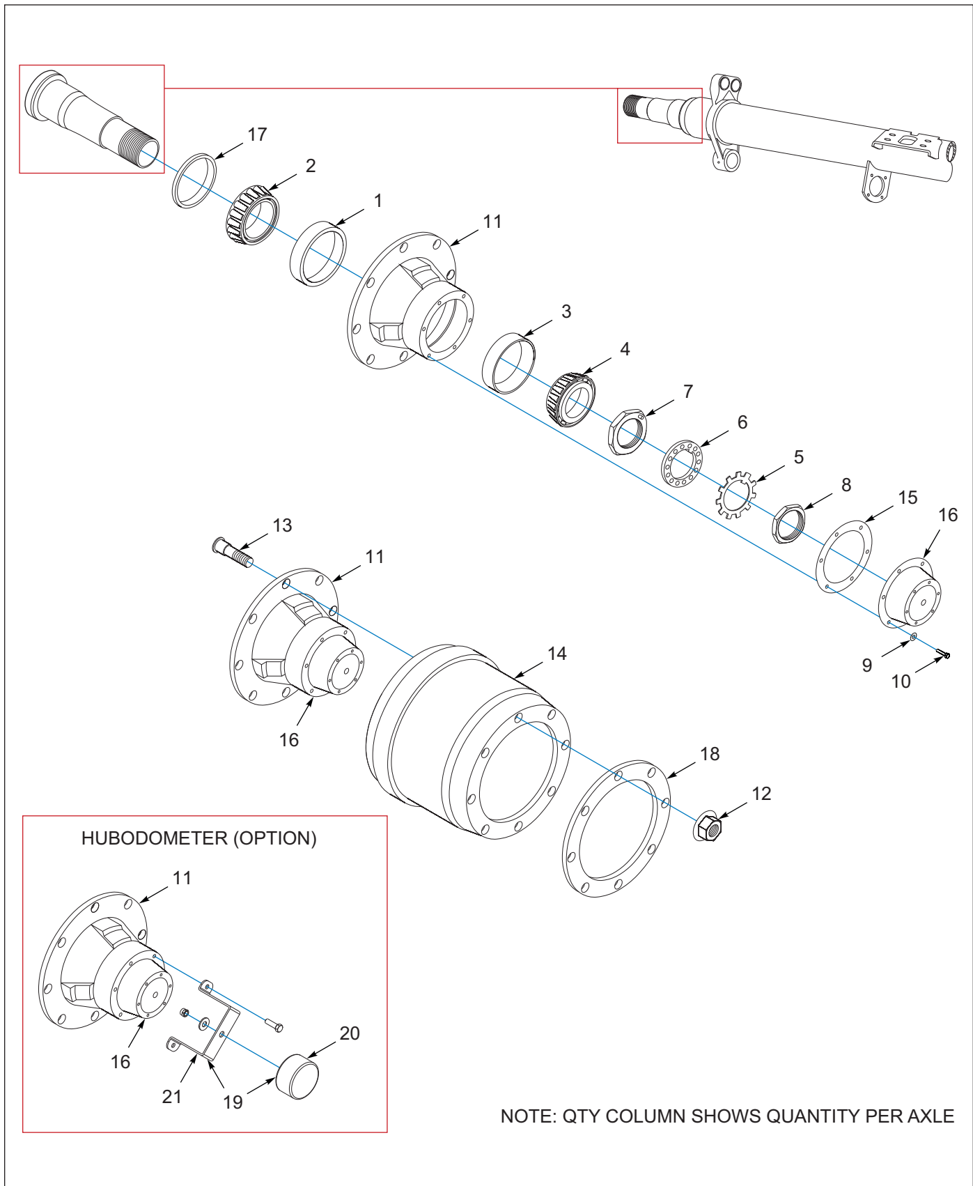
Figure 3-8: Axle 12.25 x 7.5 Drum & Hub Assembly
