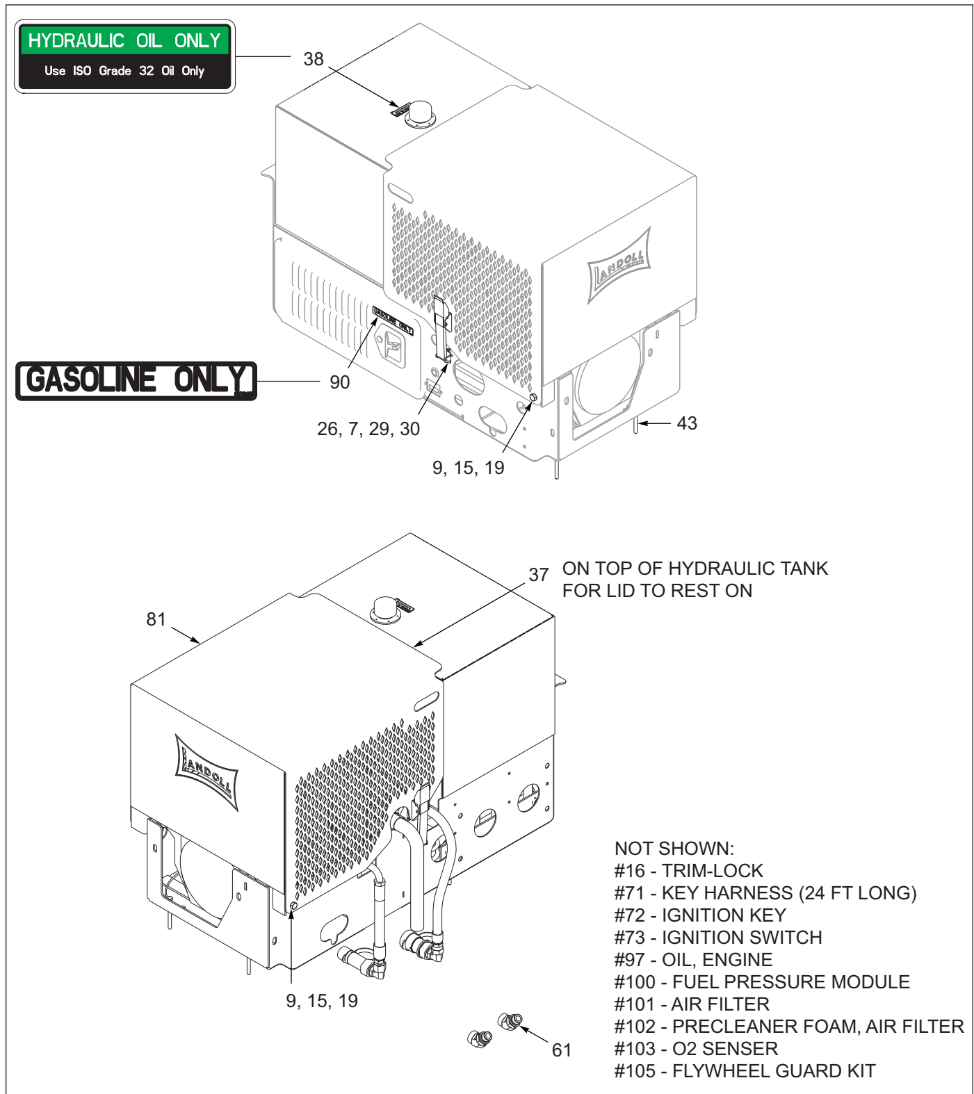
Figure 12-6: Engine Assembly, Kohler 25HP EFI, Gasoline, 30 Gallon (OPTION) (1 of 5)
