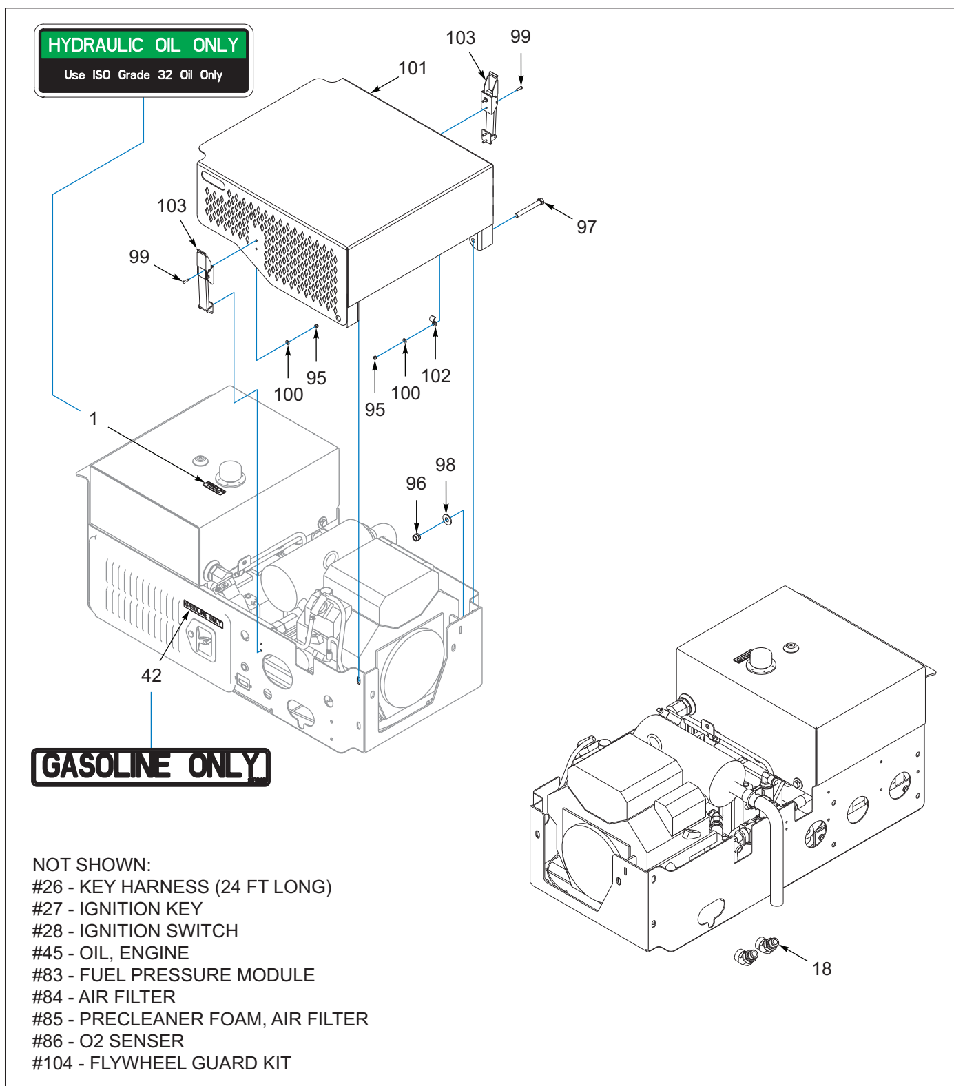
Figure 12-1: Engine Assembly, Kohler 25HP EFI, Gasoline, 15 Gallon (OPTION) (1 of 5)
