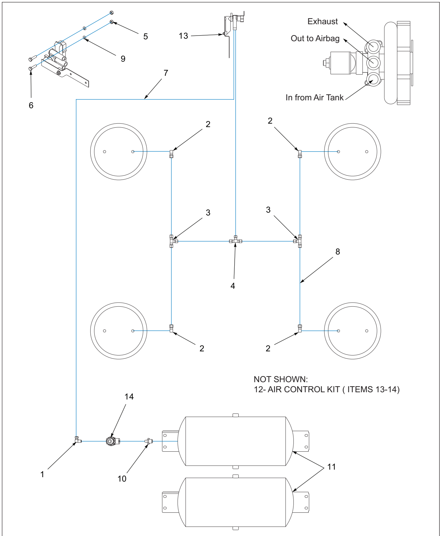
Figure 7-6: Control, Air Suspension Height, Tandem Axle
