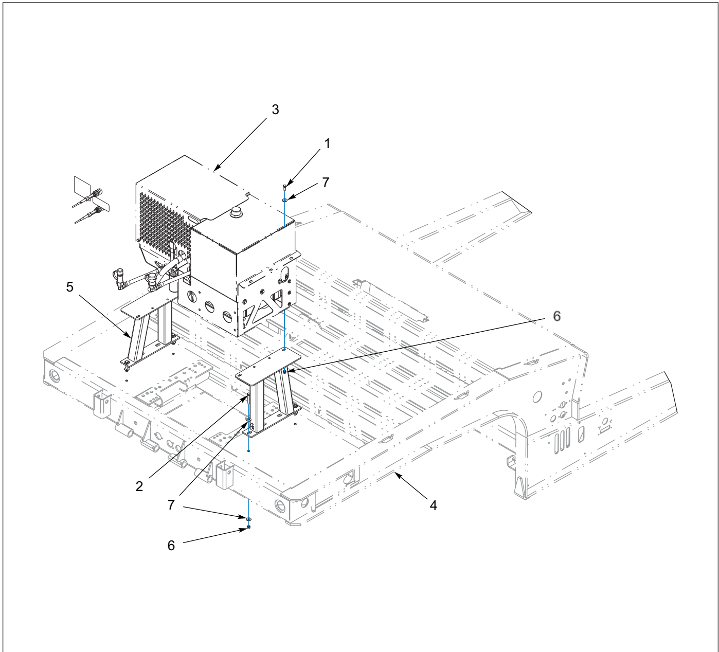
FIGURE 12-11: Engine, Mount, Upper Deck Stand Assembly (OPTION)
