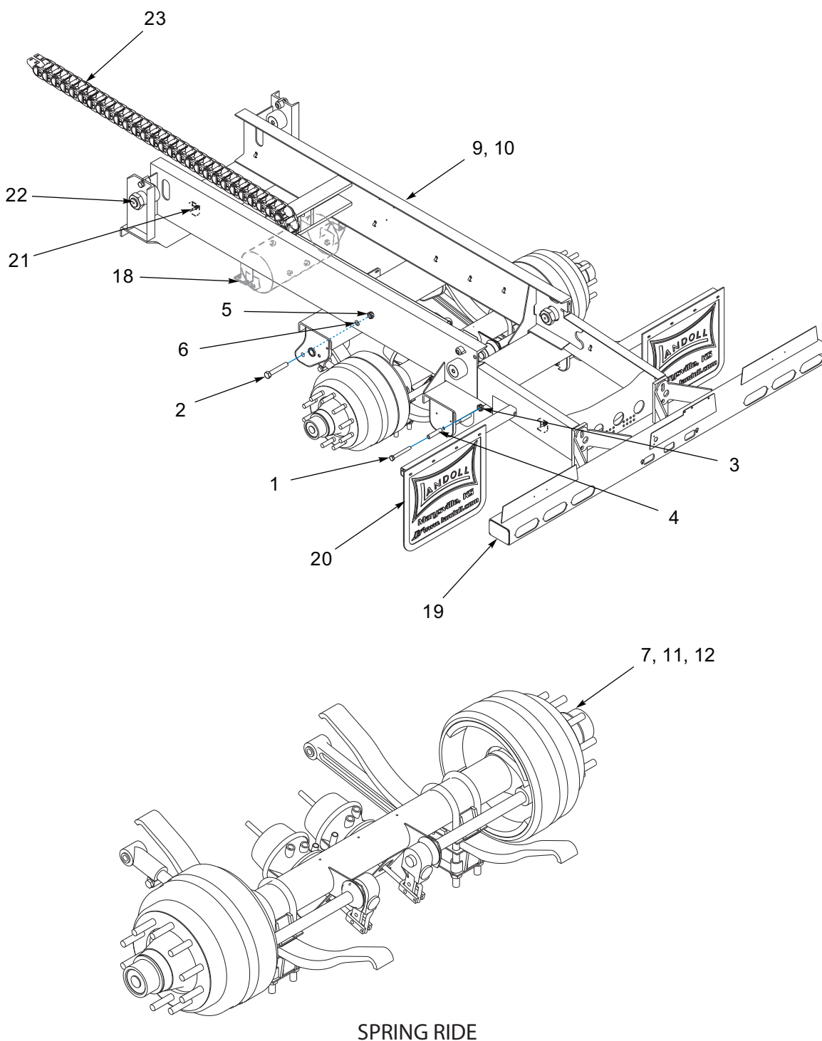
Figure 3-1: General Assembly, Single Axle (1 of 2)
