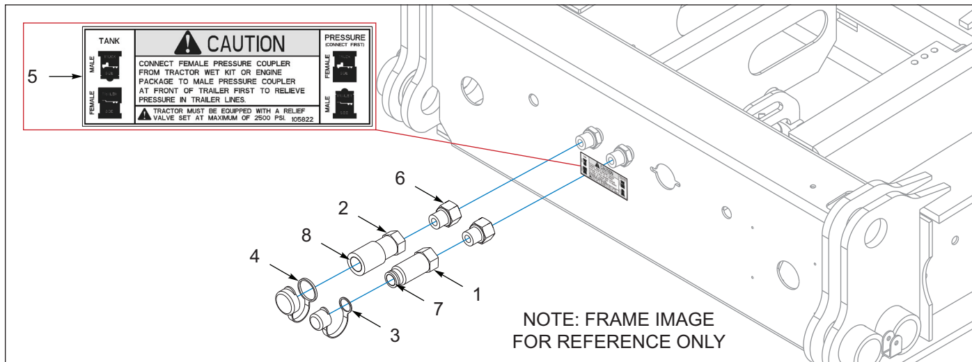
Figure 10-11: Kit, Conversion & Repair, Quick Coupler, Ball to Flat
