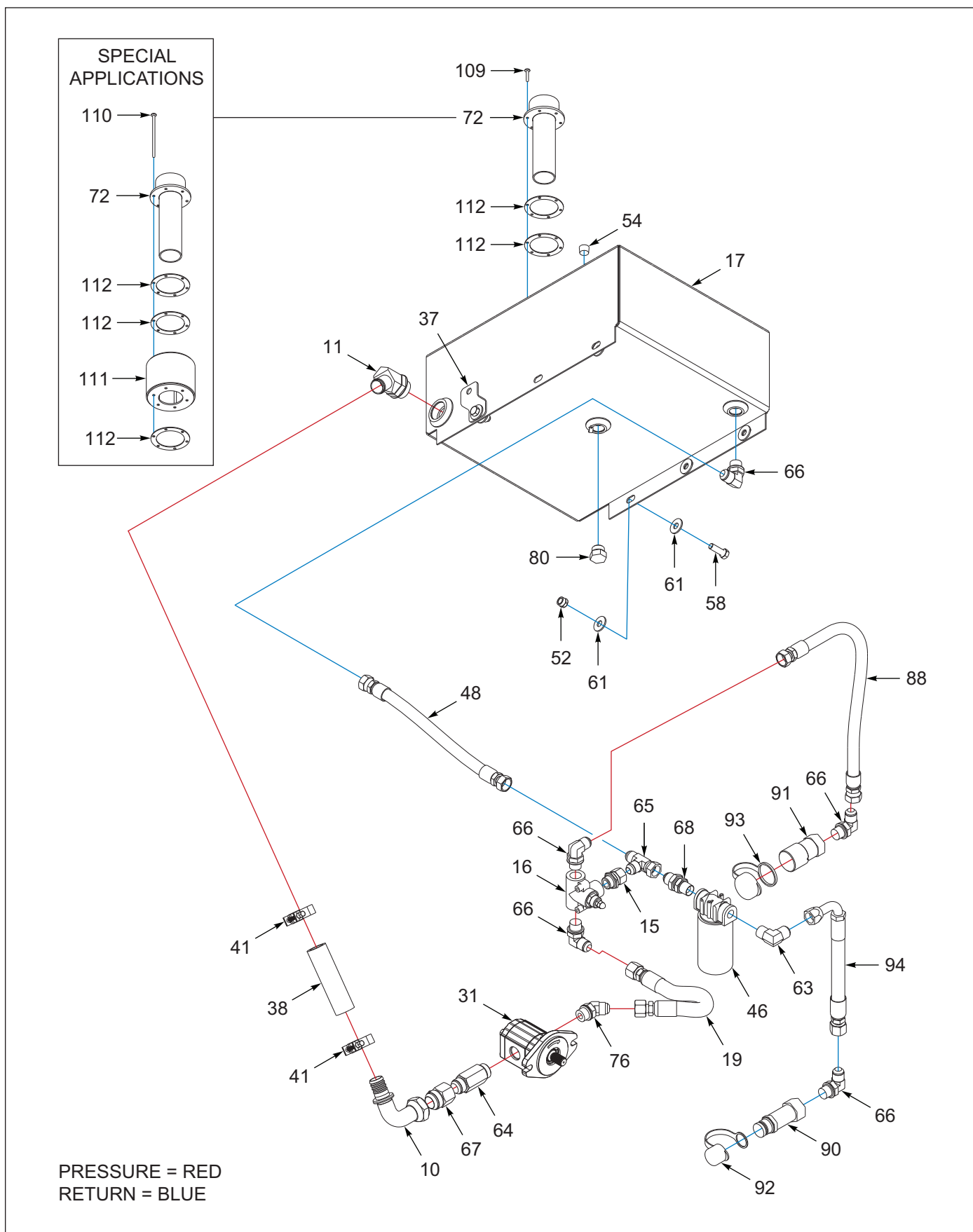
Figure 12-5: Engine Assembly, Kohler 25HP EFI, Gasoline, 15 Gallon (OPTION) (5 of 5)
