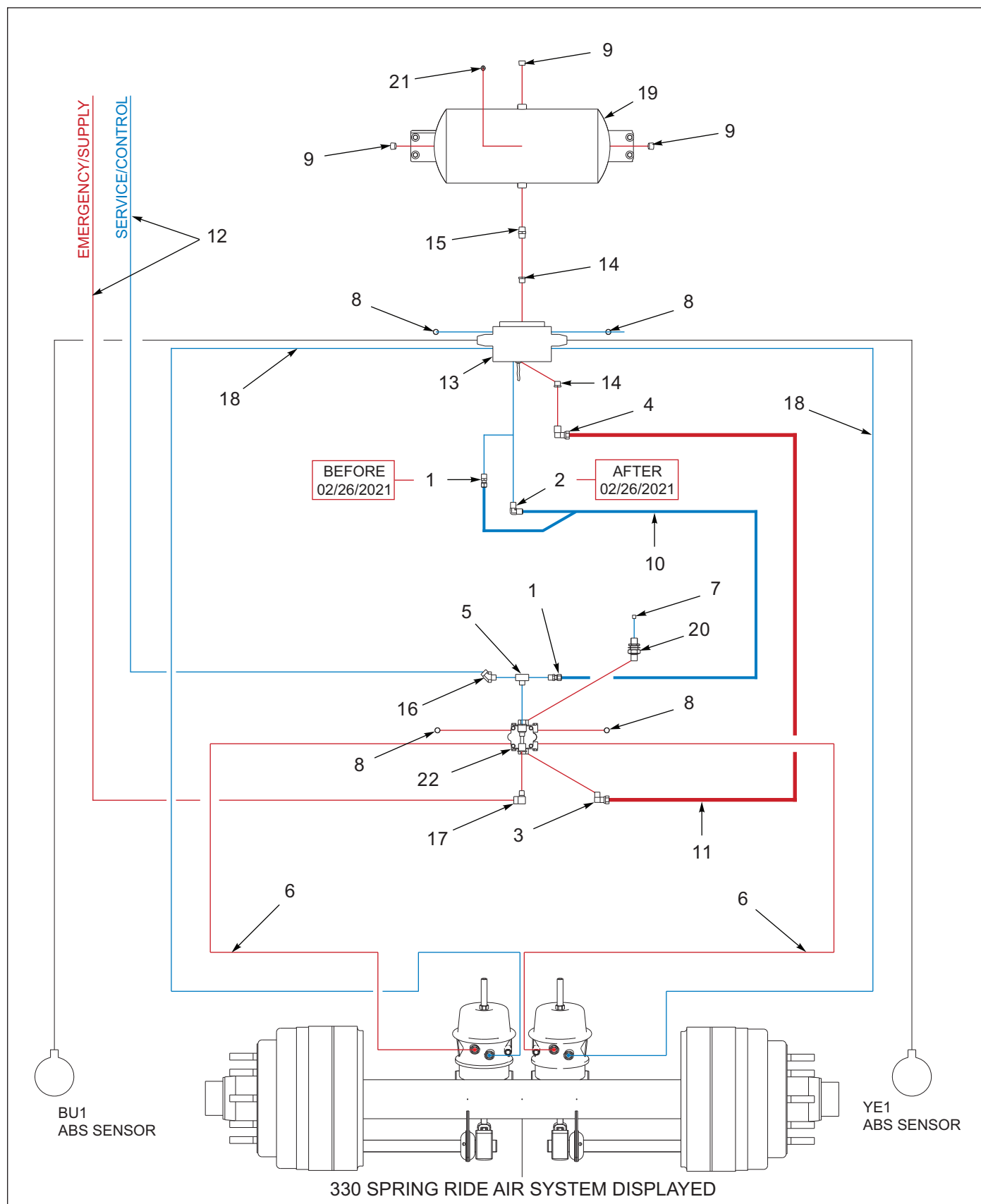
Figure 7-2: Anti-Lock Brake System, Single Axle
