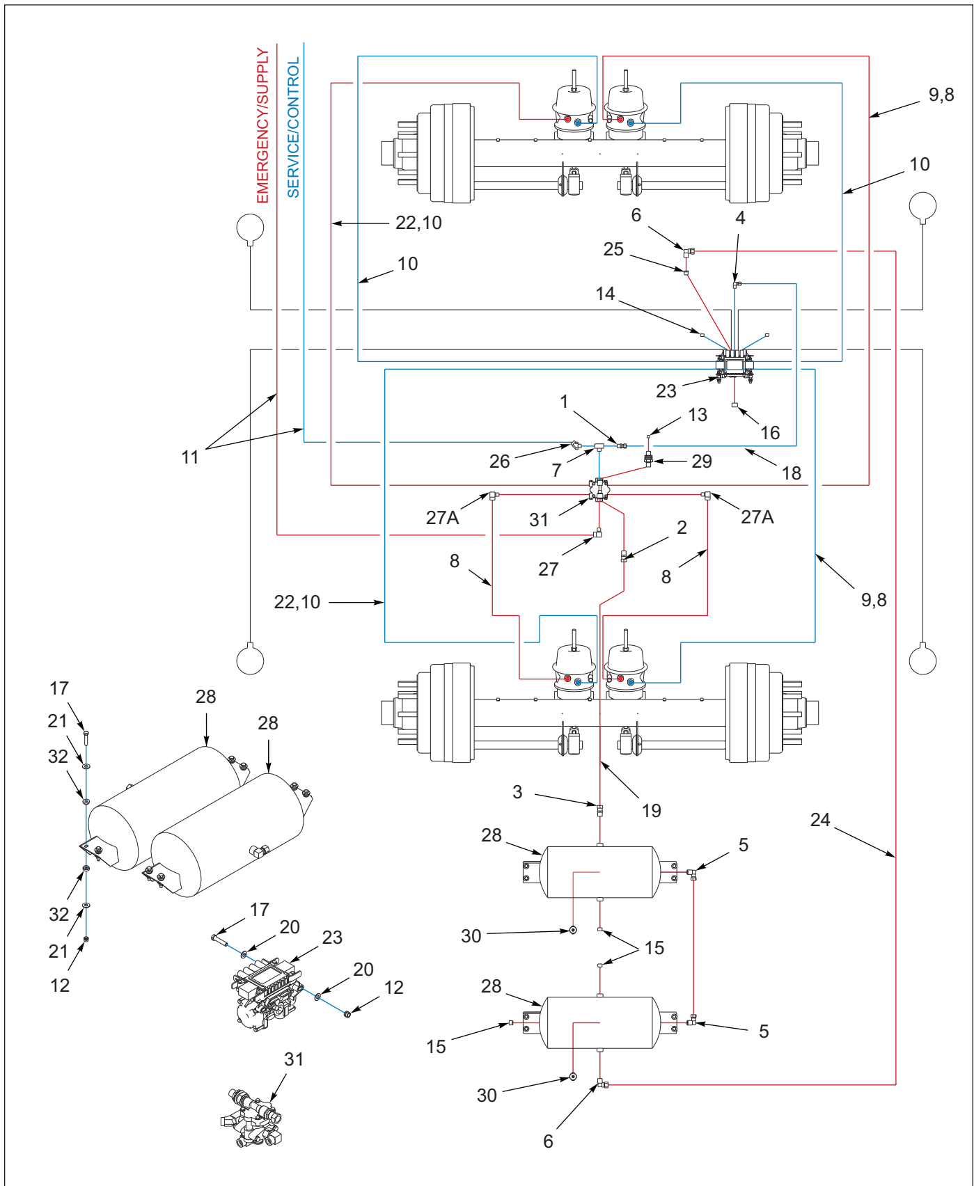
Figure 7-3: Anti-Lock Brake System, Tandem Axle
