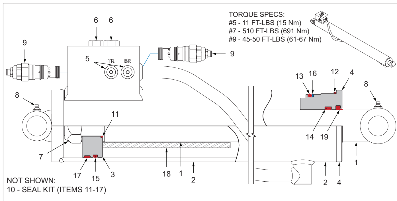
Figure 10-8: Cylinder, Hydraulic, 4 x 42 W/Counterbalance Valve
