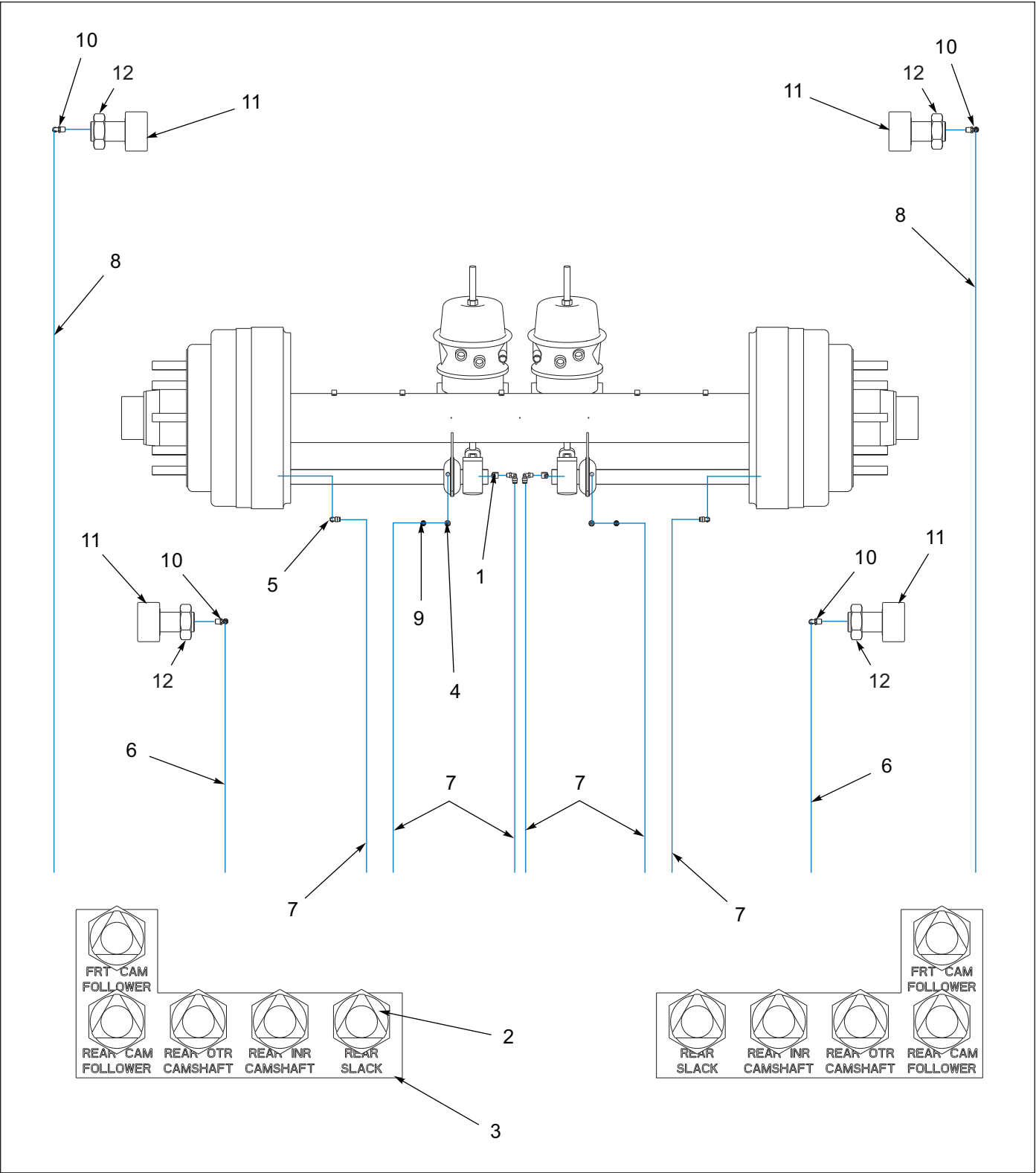
Figure 9-1: Frame, Single Axle Assembly
