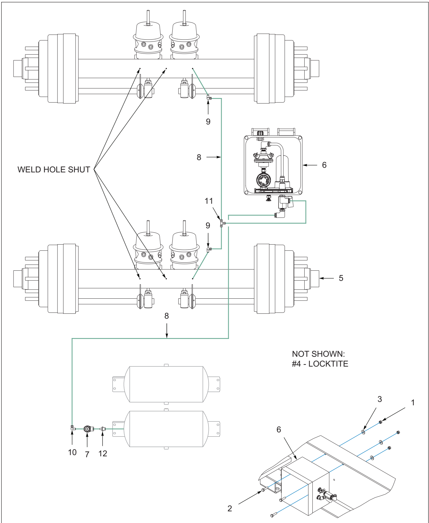
Figure 7-9: Tire Inflation System, Tandem Axle (OPTION)
