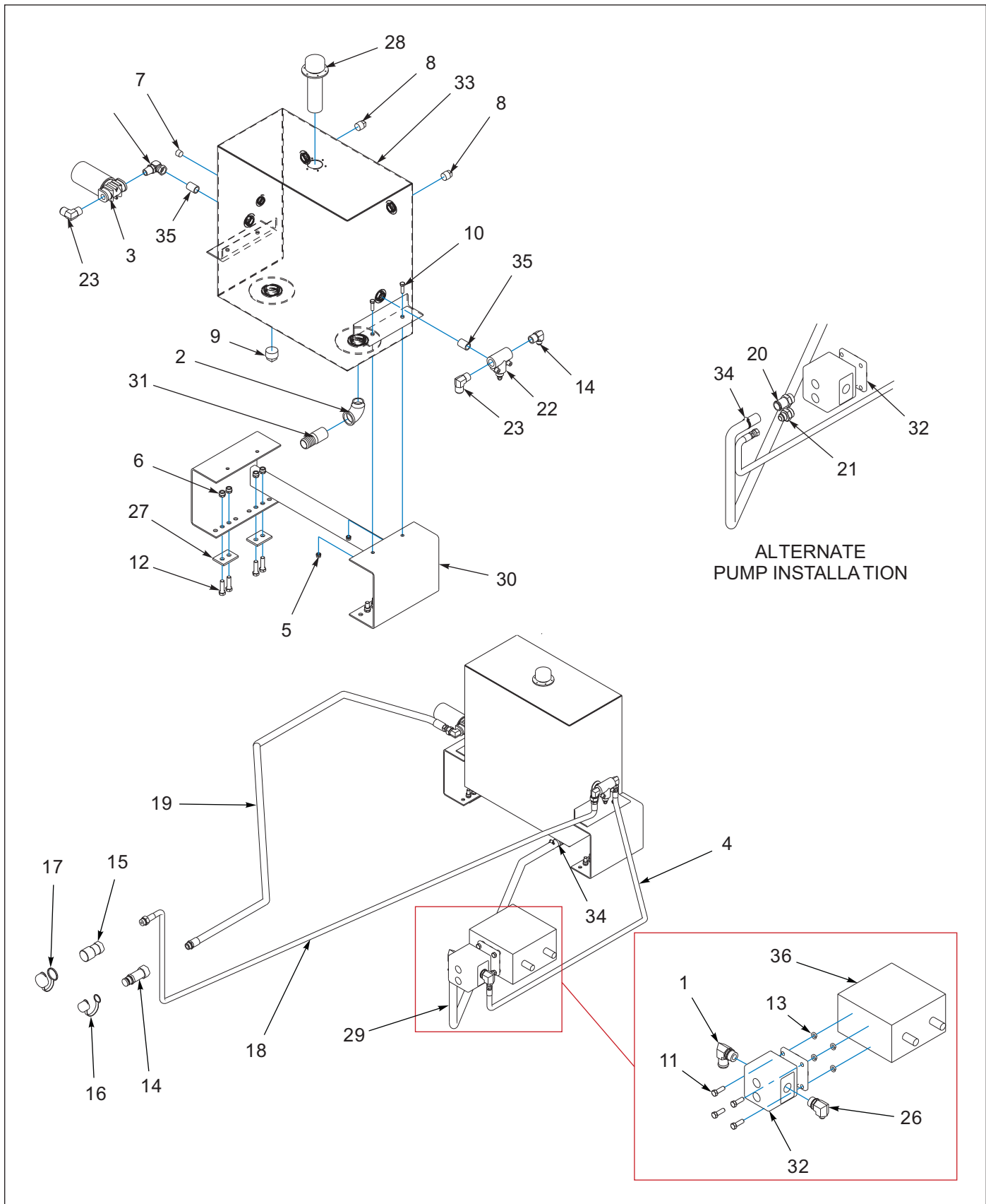
Figure 10-12: Kit, Wet, Hydraulic (OPTION) (BEFORE 02/21/2019)
