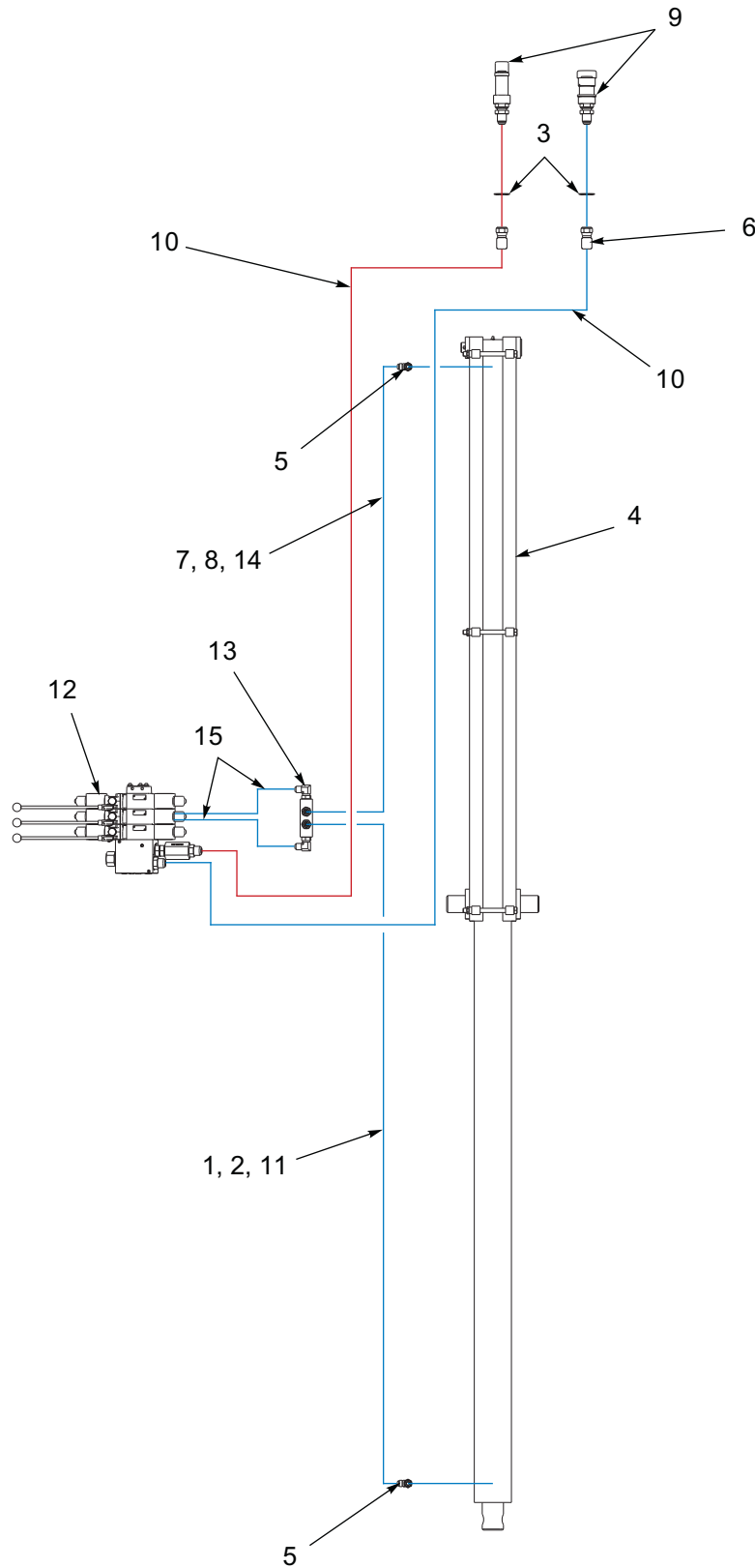
Figure 10-4: Chain Drive System
