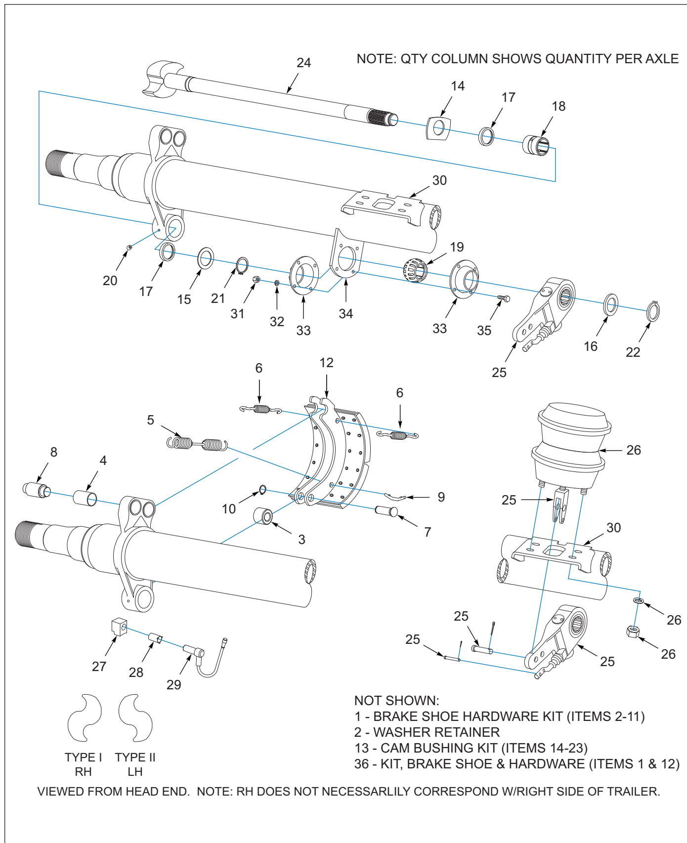
Figure 3-7: Axle 12.25 x 7.5 Drum Brakes
