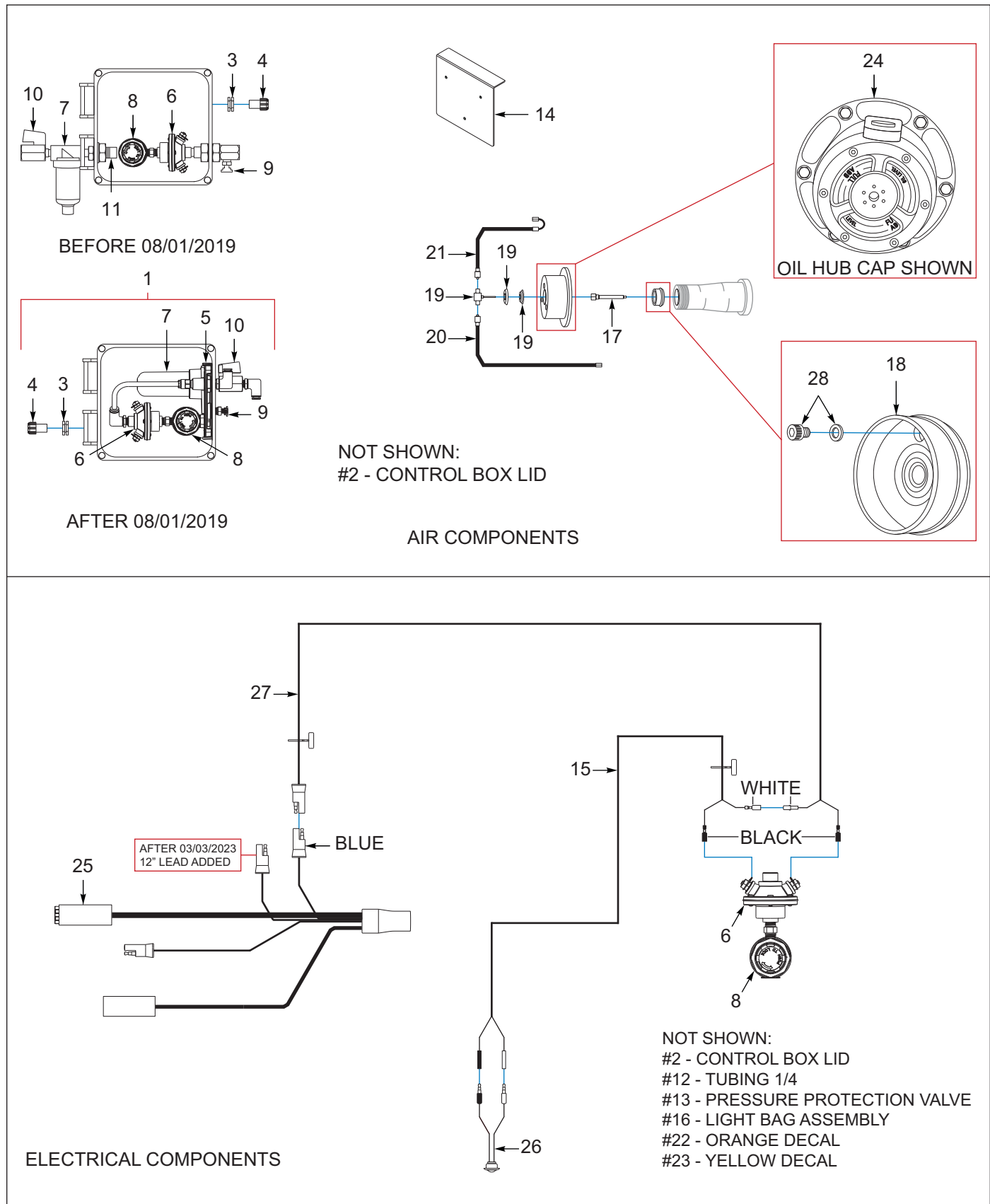
Figure 7-10: Tire Inflation System, Air & Electrical Components (OPTION)
