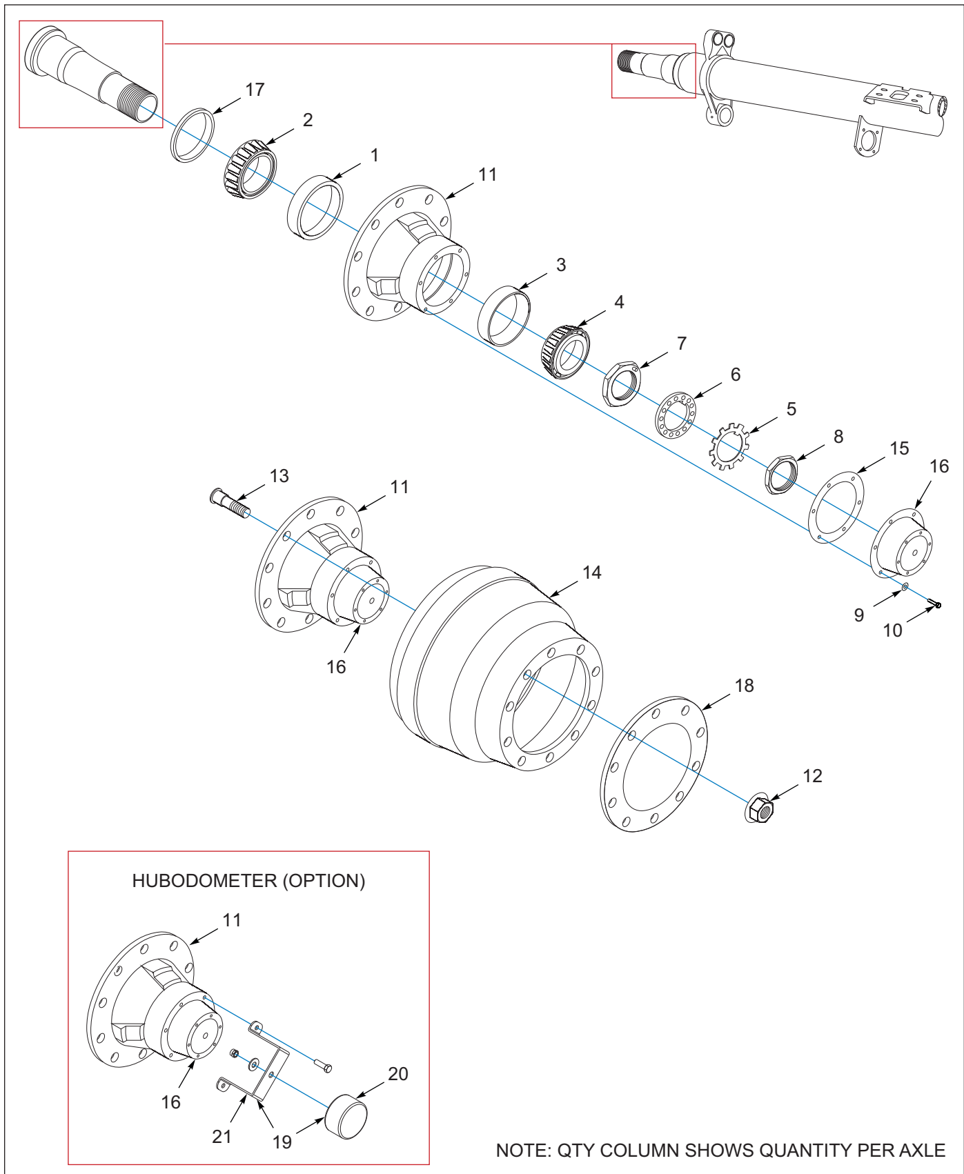
Figure 3-12: Axle 16.5 x 7 Drum & Hub Assembly, Dexter
