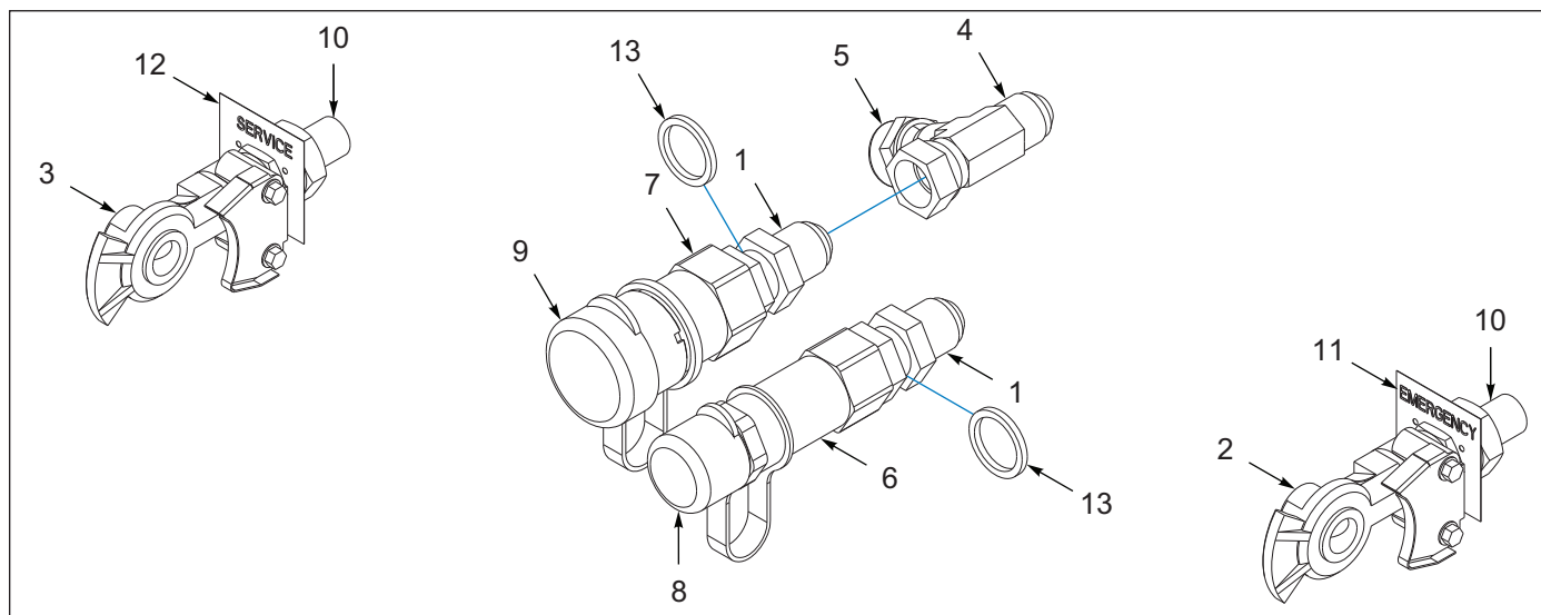
Figure 10-1: Connectors, Front Sub Assembly, Air & Hydraulic
