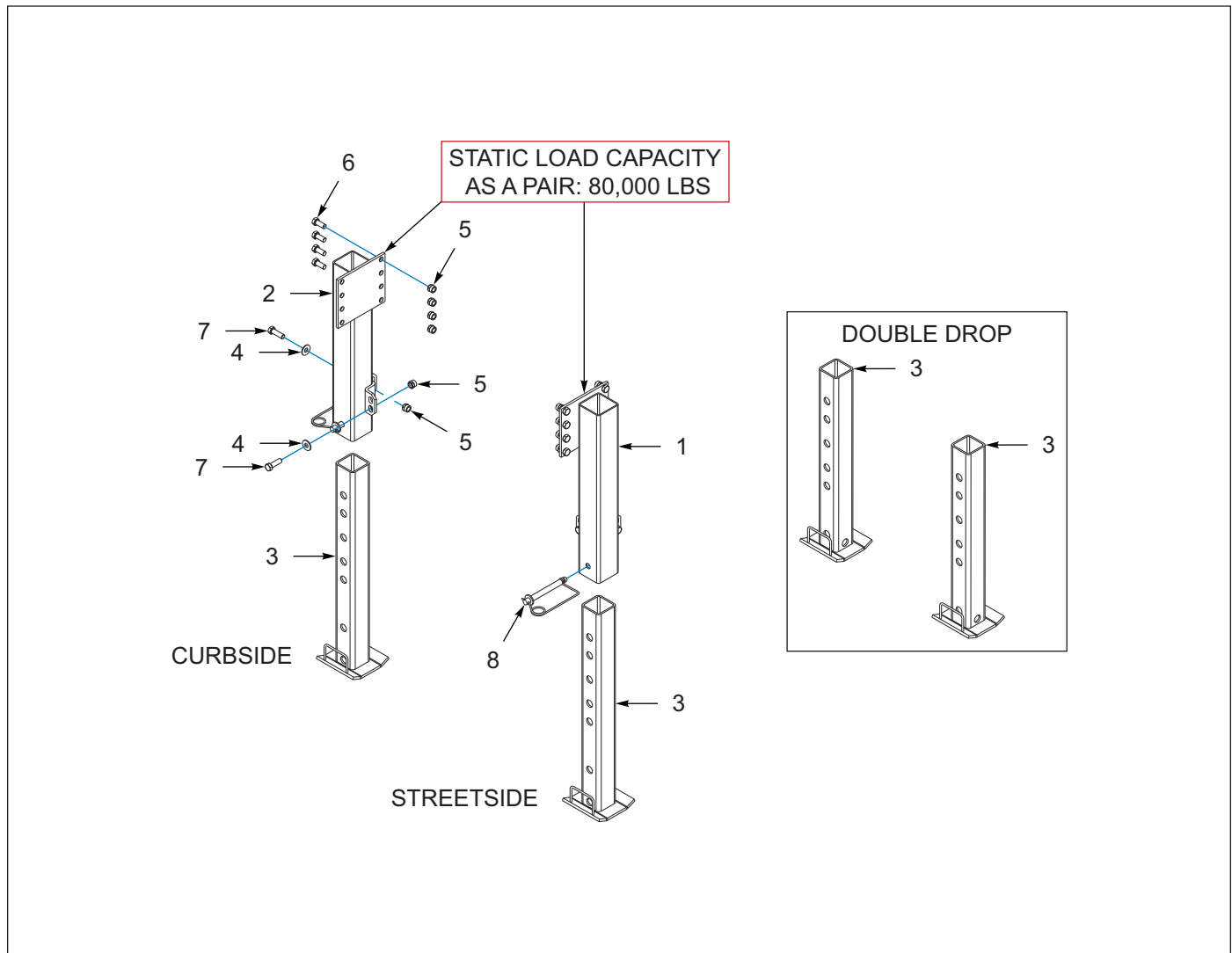
Figure 5-5: Landing Legs, Pinned
