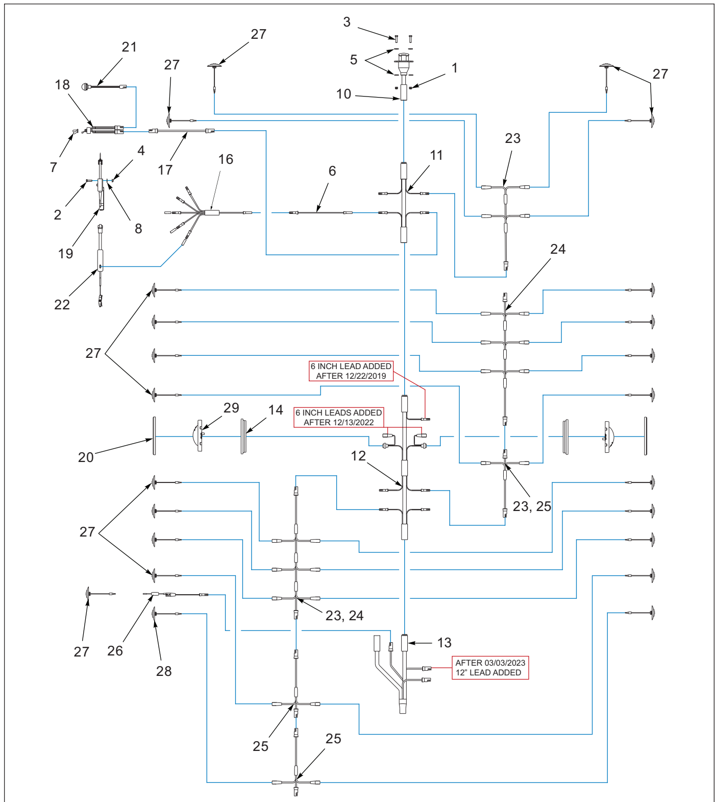
Figure 8-1: Frame, Harness & Lights
