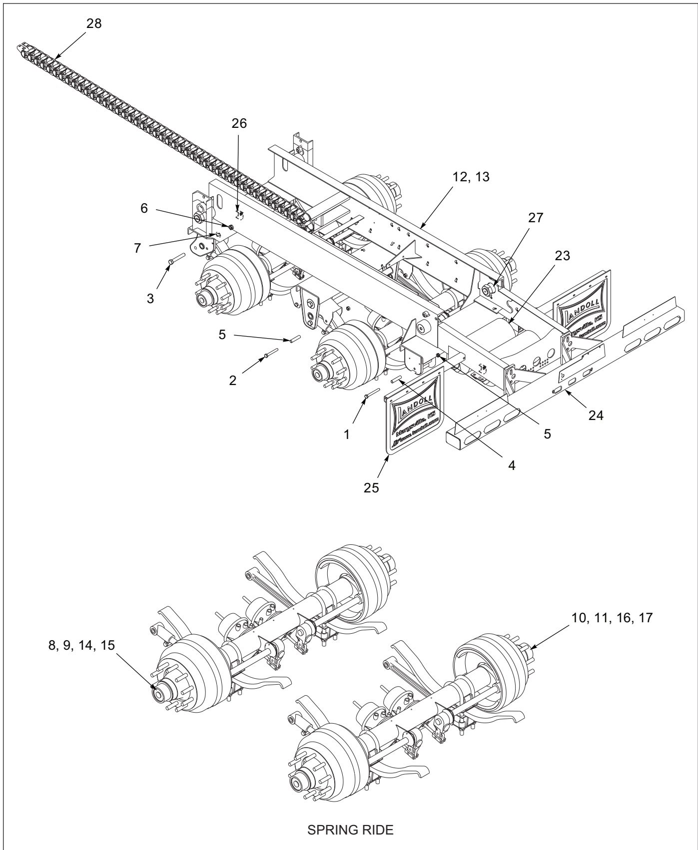
Figure 3-3: General Assembly, Tandem Axle (1 of 2)
