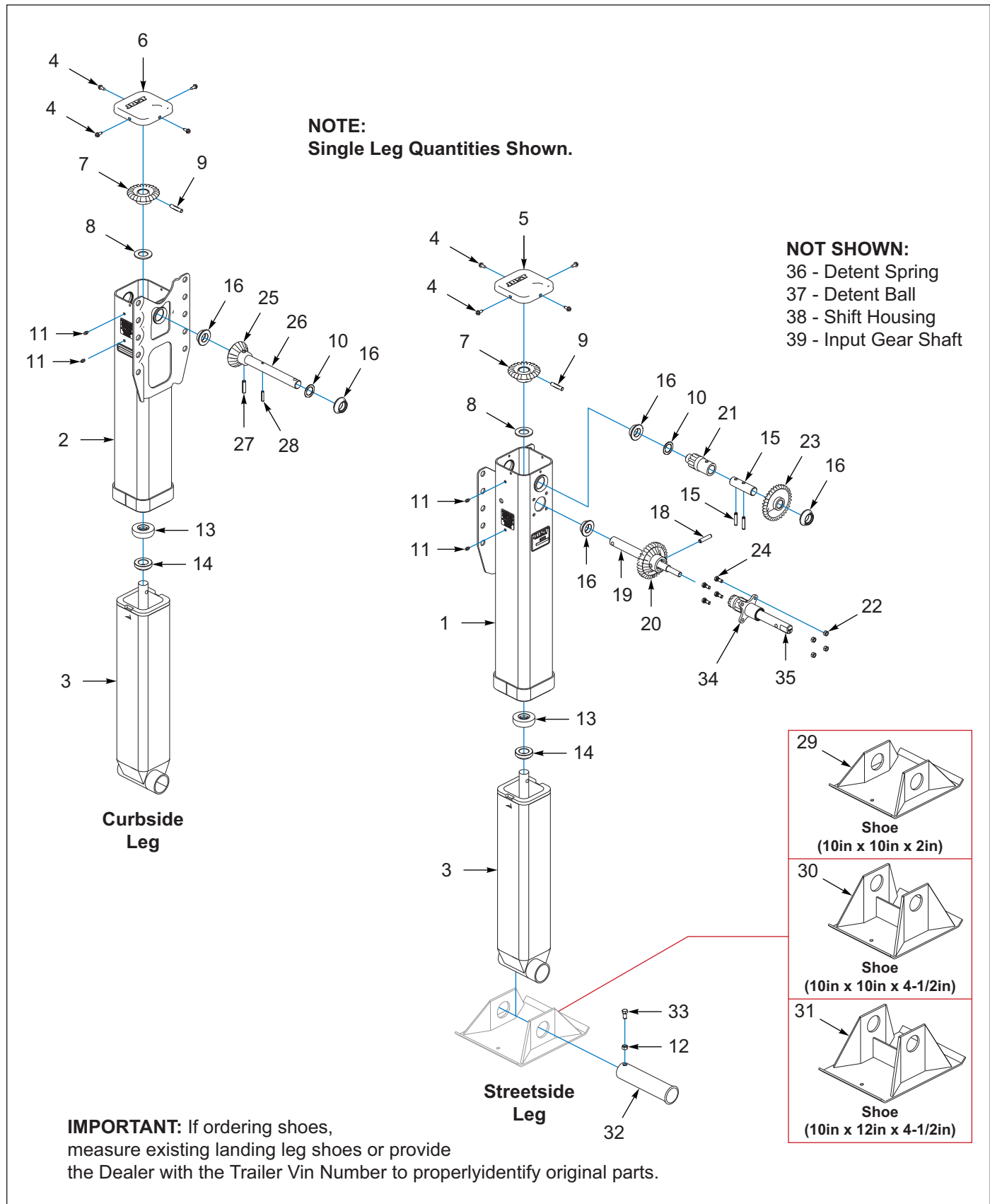
Figure 5-6: Landing Legs Components, Gear, 2 Spd
