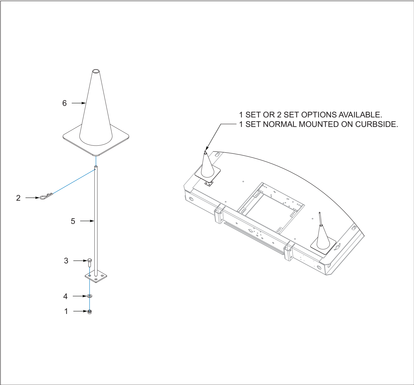
Figure 6-7: Storage, Emergency Cone (OPTION)
