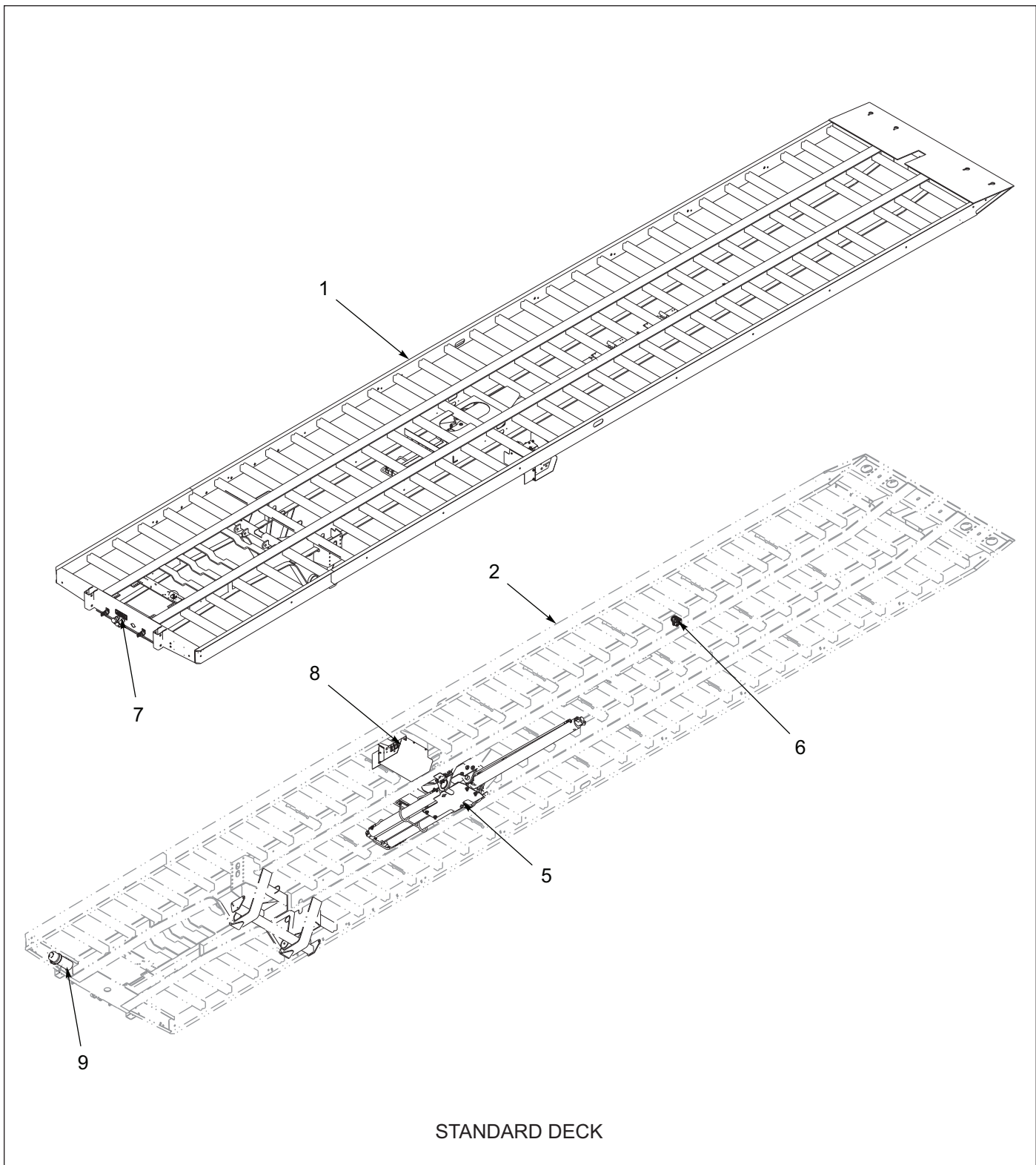
Figure 2-1: Deck Assembly (1 of 3)
