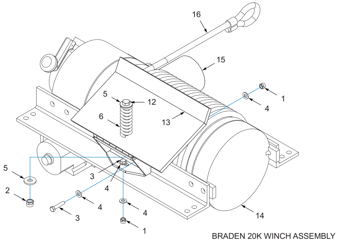
Figure 11-4: Winch Assembly, Braden 12K / 20K
