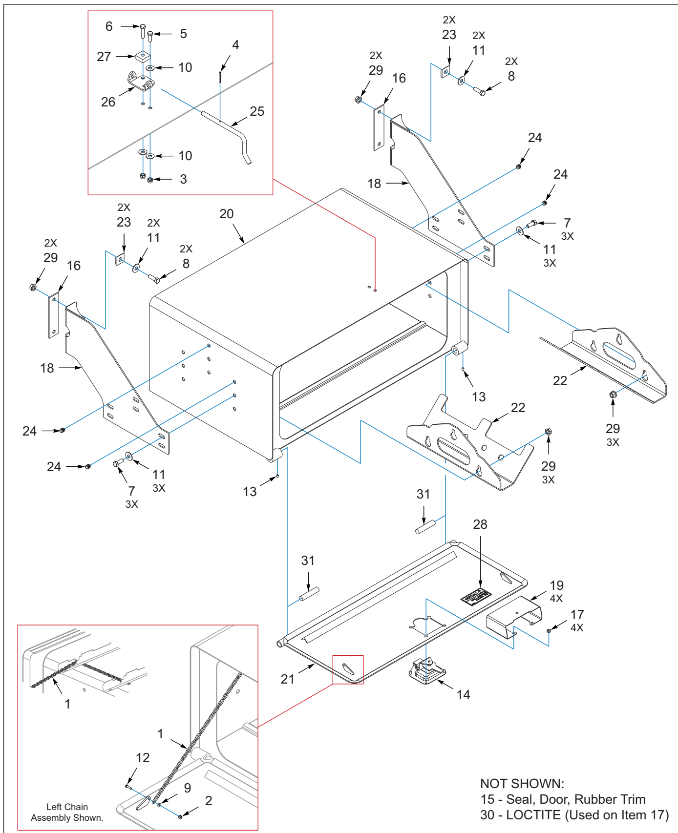
Figure 6-9: Toolbox, Bolt-On, 42"W X 28"D X 17"H (OPTION)
