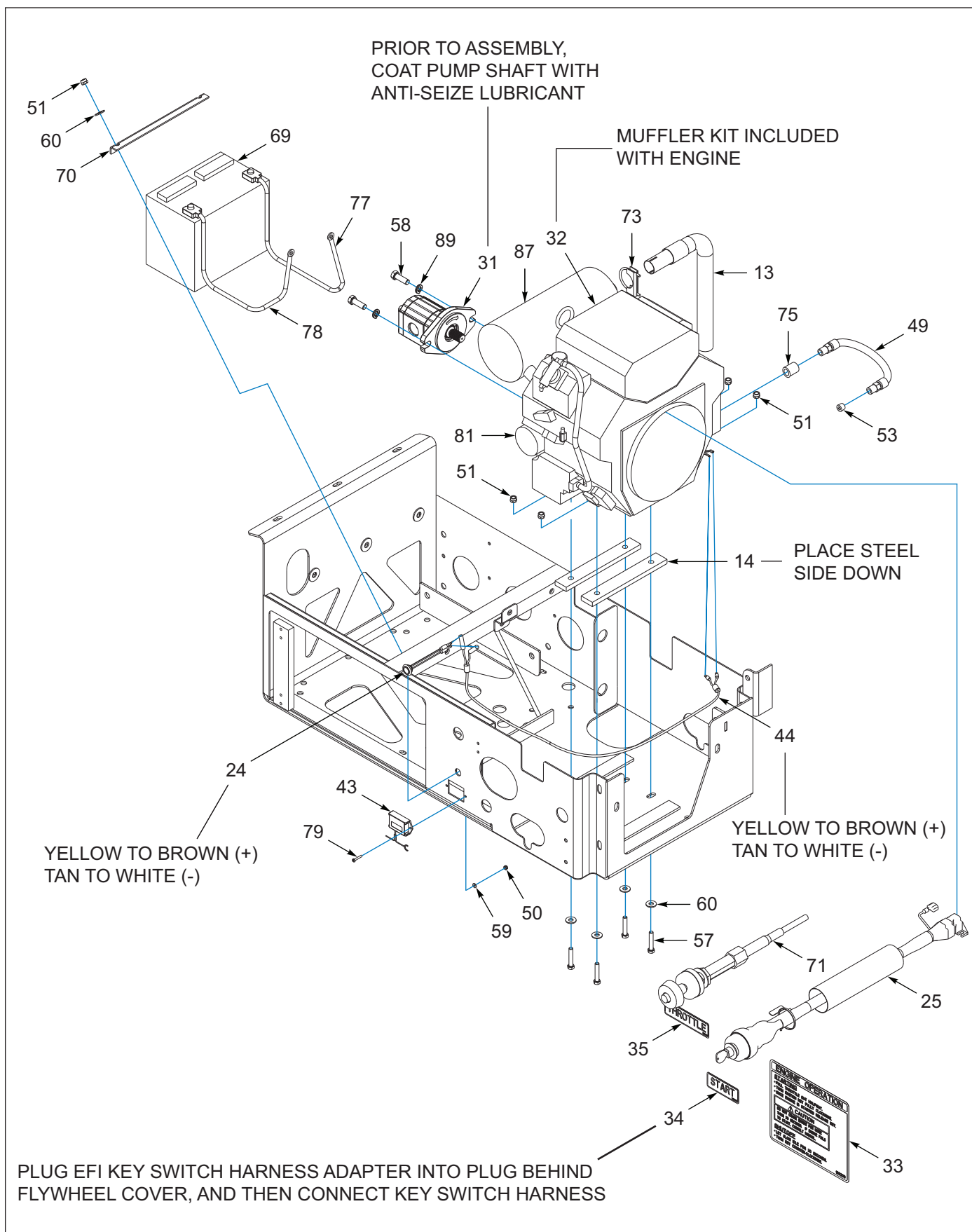
Figure 12-3: Engine Assembly, Kohler 25HP EFI, Gasoline, 15 Gallon (OPTION) (3 of 5)
