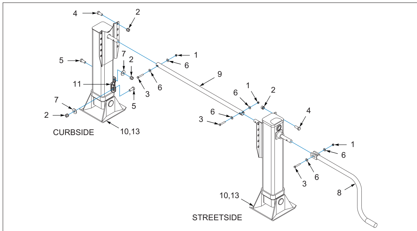
Figure 5-2: Landing Legs, Gear, 2 Spd, Flip Crank, Rear Low Mt Bkt
