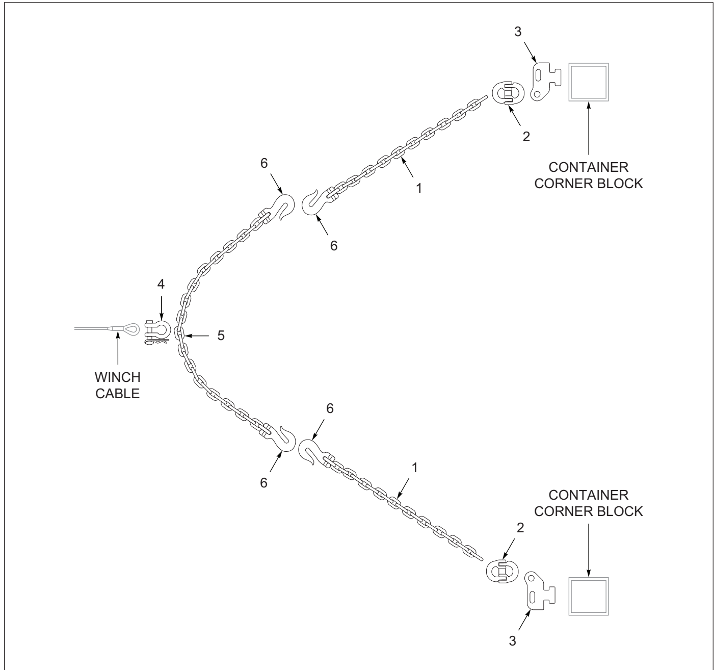
Figure 6-2: Chain Assembly, Container Loading, 3 Chain (OPTION)
