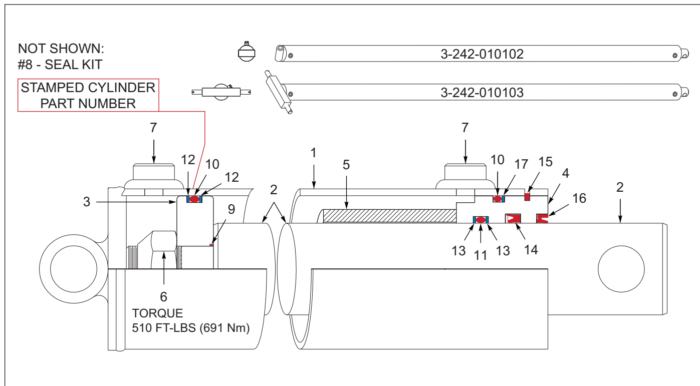
Figure 10-7: Cylinder, Hydraulic, 4 x 126
