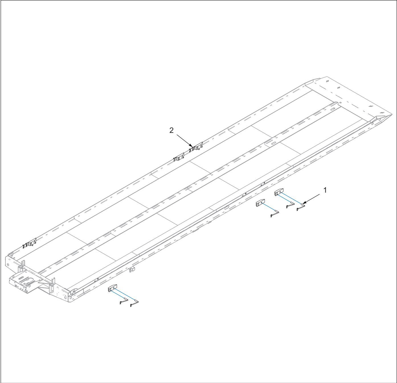
Figure 6-6: Container, Stop / Lock Pin Assembly
