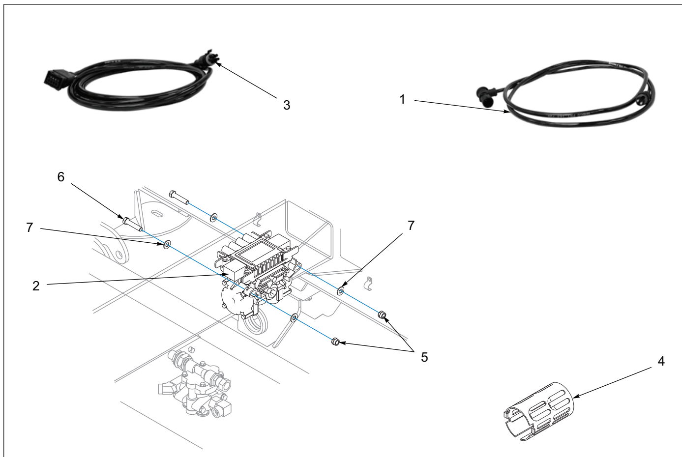
Figure 7-4: Anti-Lock Brake Kit, Components
