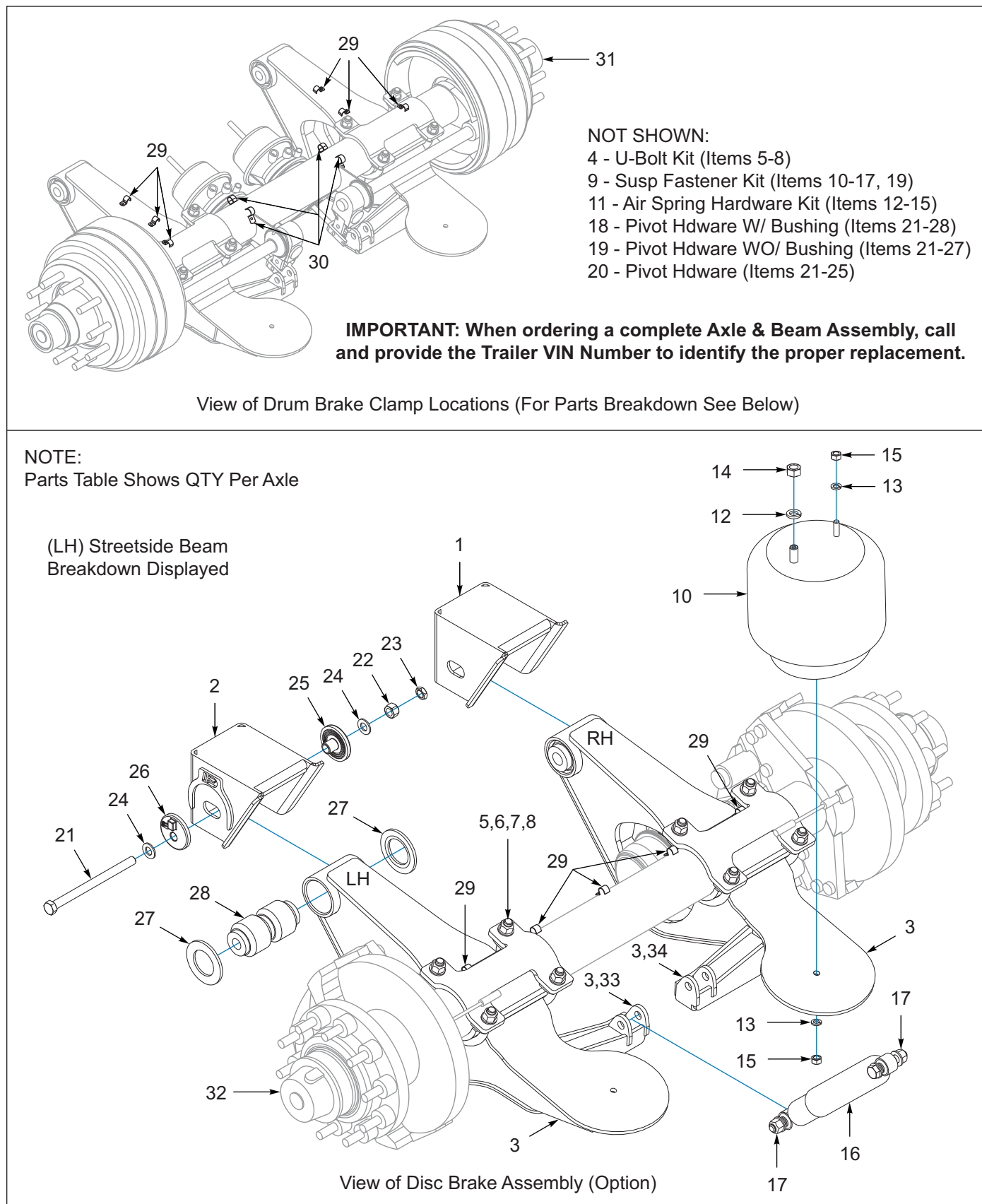
Figure 3-16: Axle Suspension, LSS-25K-5.5RLU, 16.5
