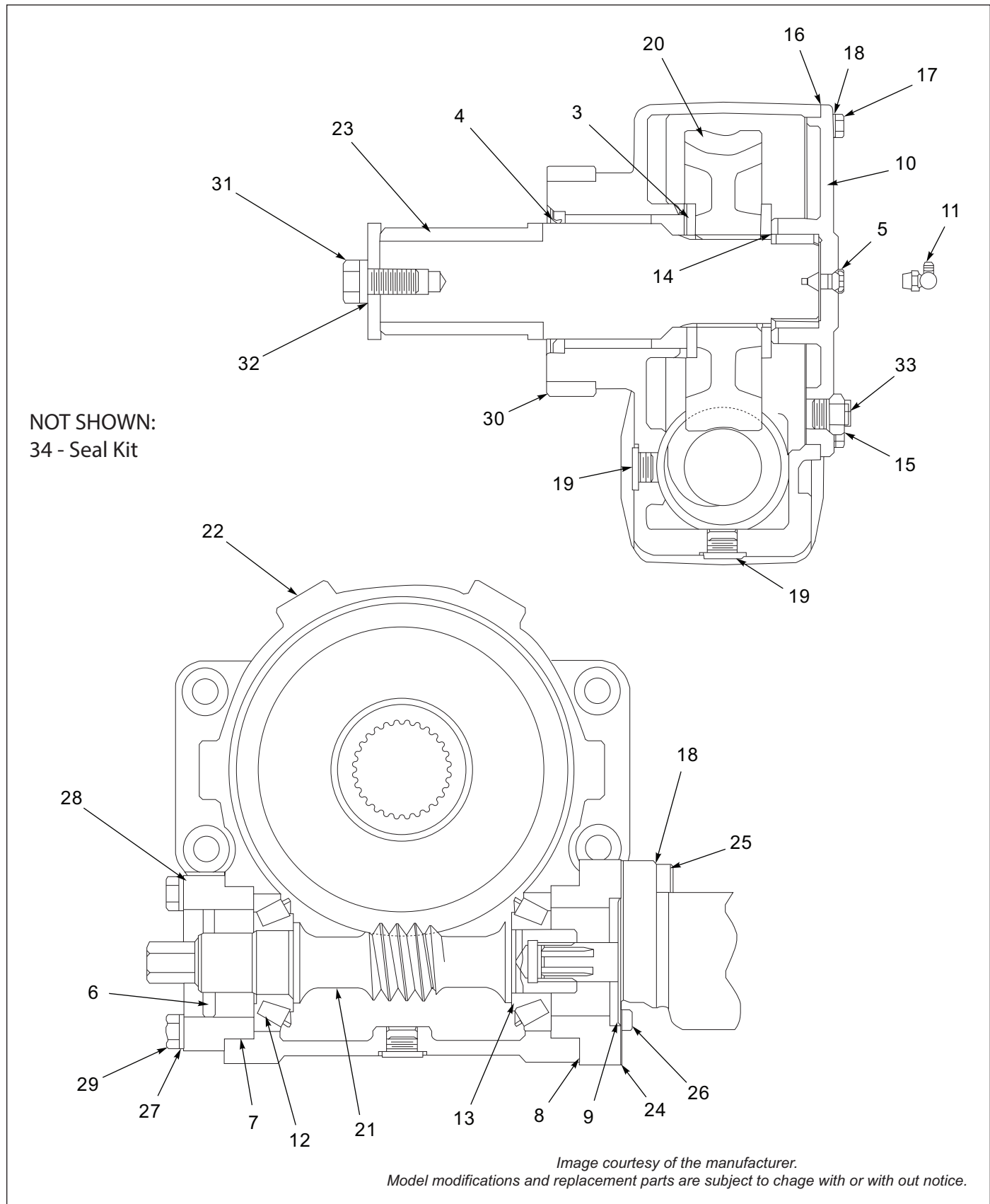
Figure 11-2: Chain Drive Components, Gearbox
