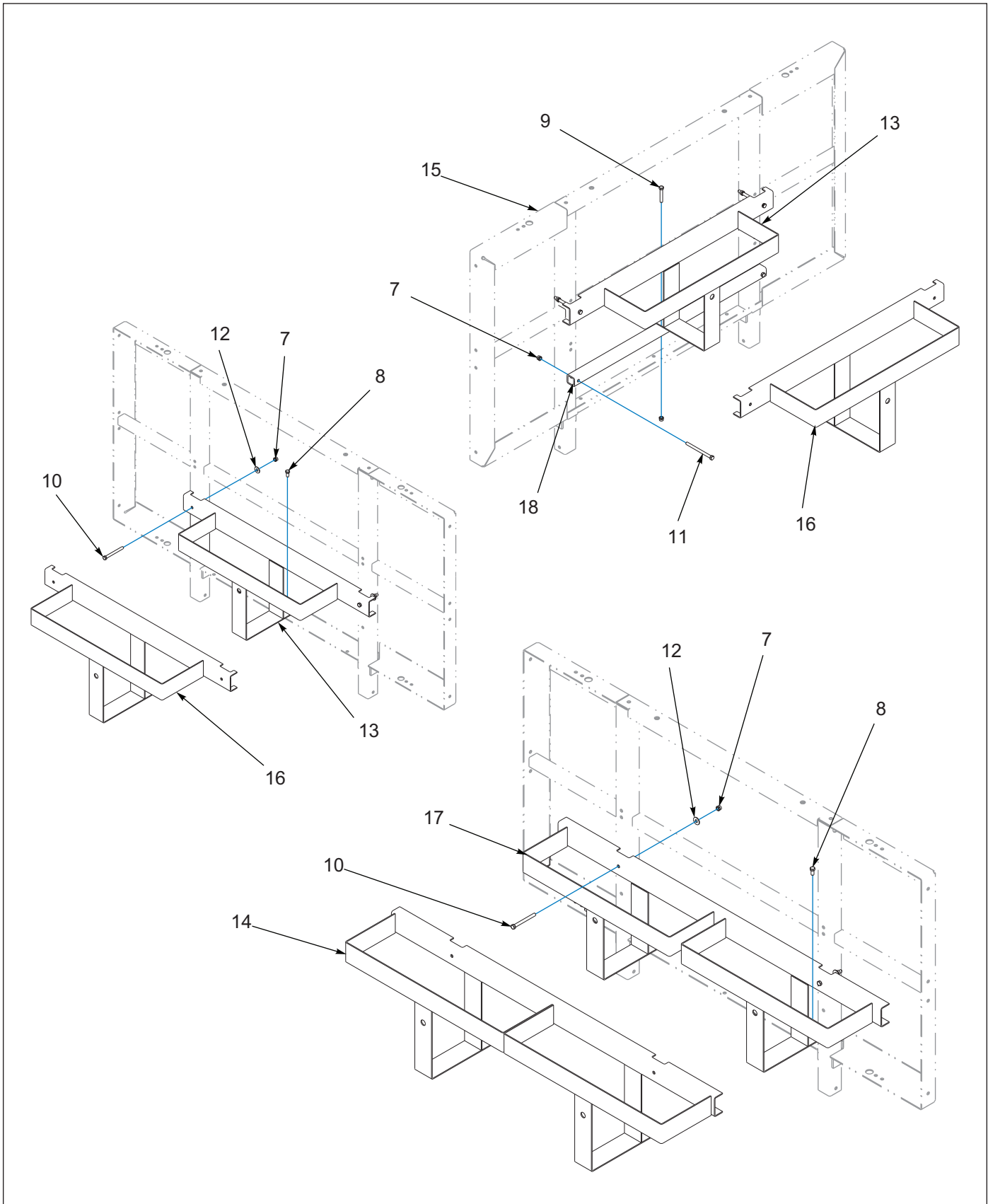
Figure 4-2: Rack, Spare Tire (OPTION)
