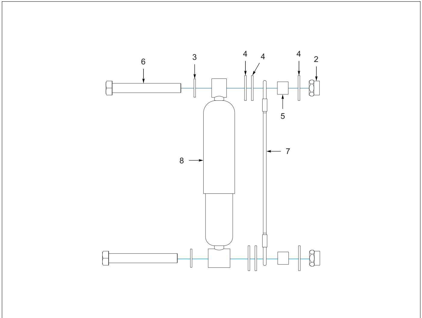
Figure 3-20: Shock Strap, Limit, RLU 228-5.5 (OPTION)
