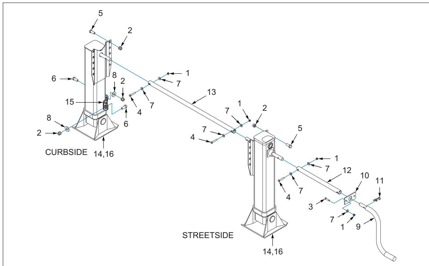
Figure 5-4: Landing Legs, Gear, 2 Spd, Pin Crank, Rear Low Mt Bkt
