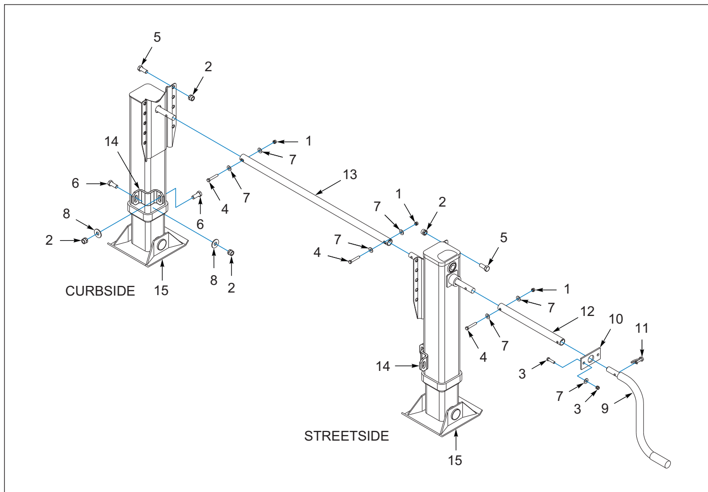
Figure 5-3: Landing Legs, Gear, 2 Spd, Pin Crank, Front Low Mt Bkt
