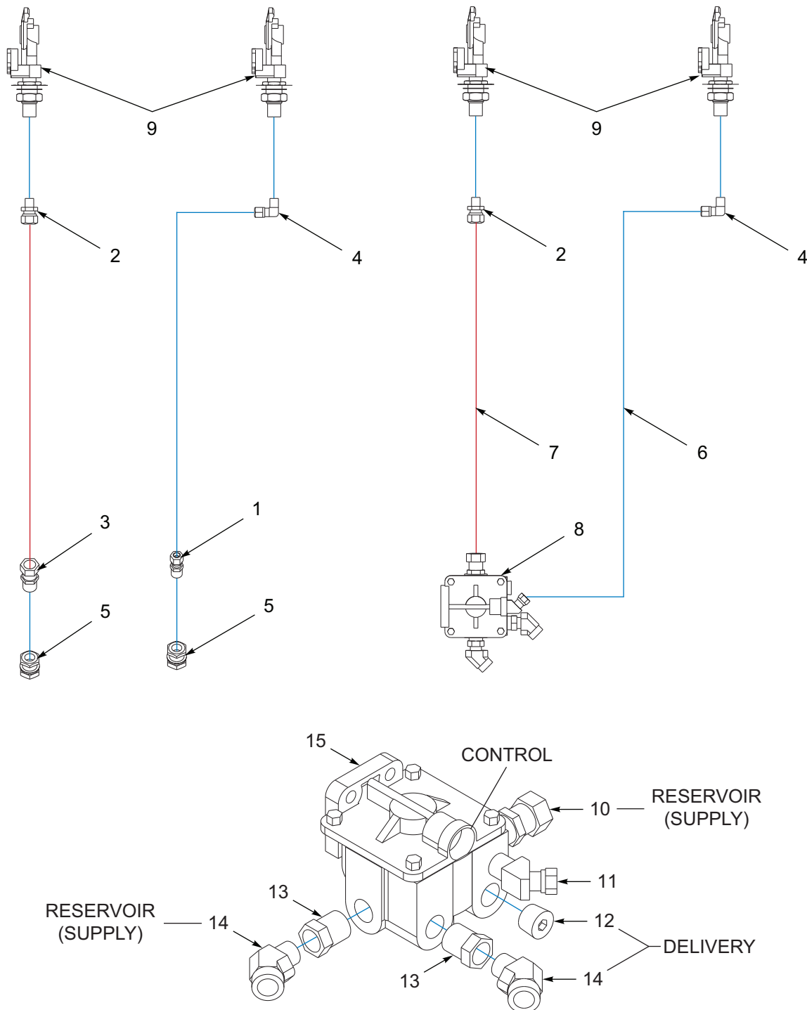
Figure 7-1: Air System - Standard & Low Load Angle
