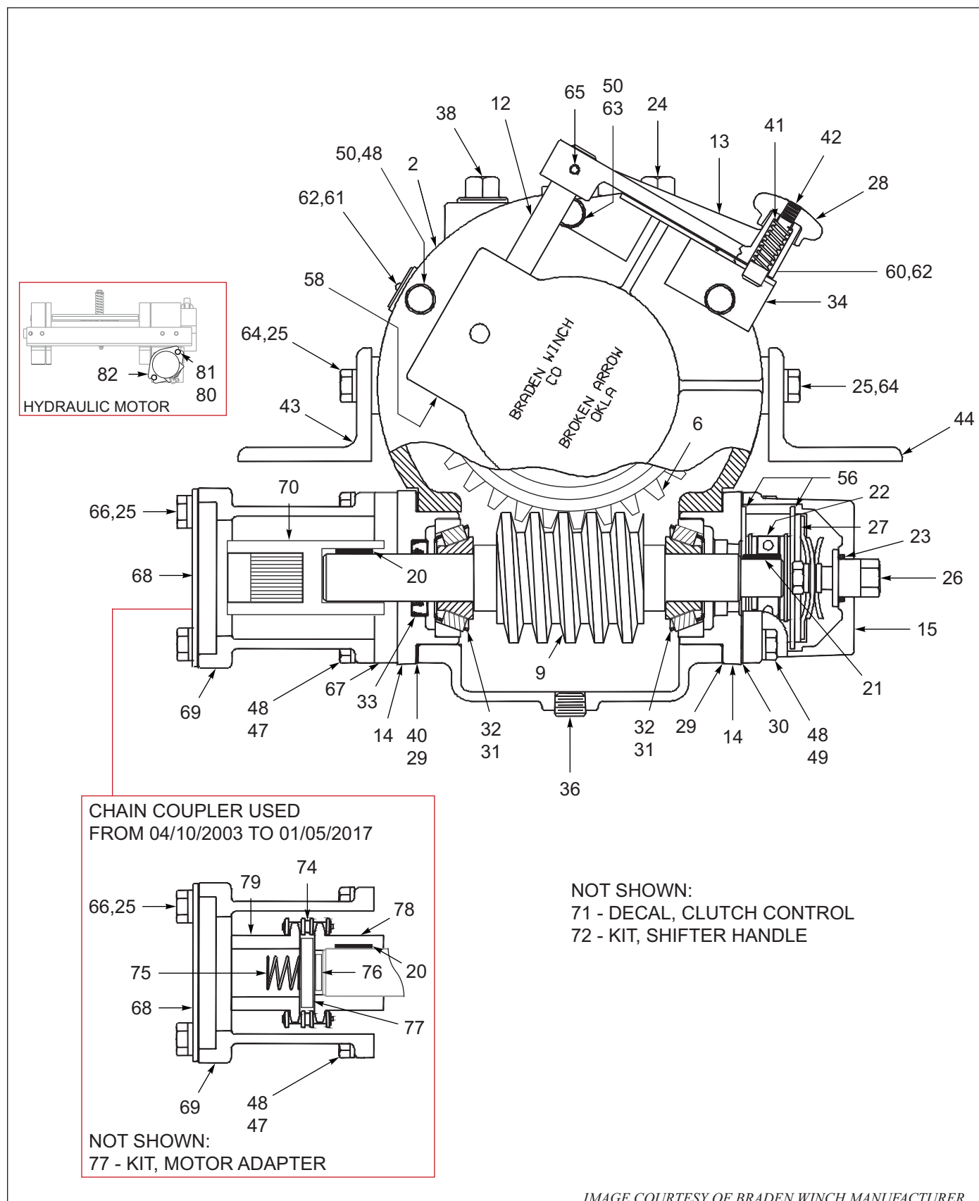
Figure 11-7: Winch Components, Braden 20K (OPTION) (1 of 2)
