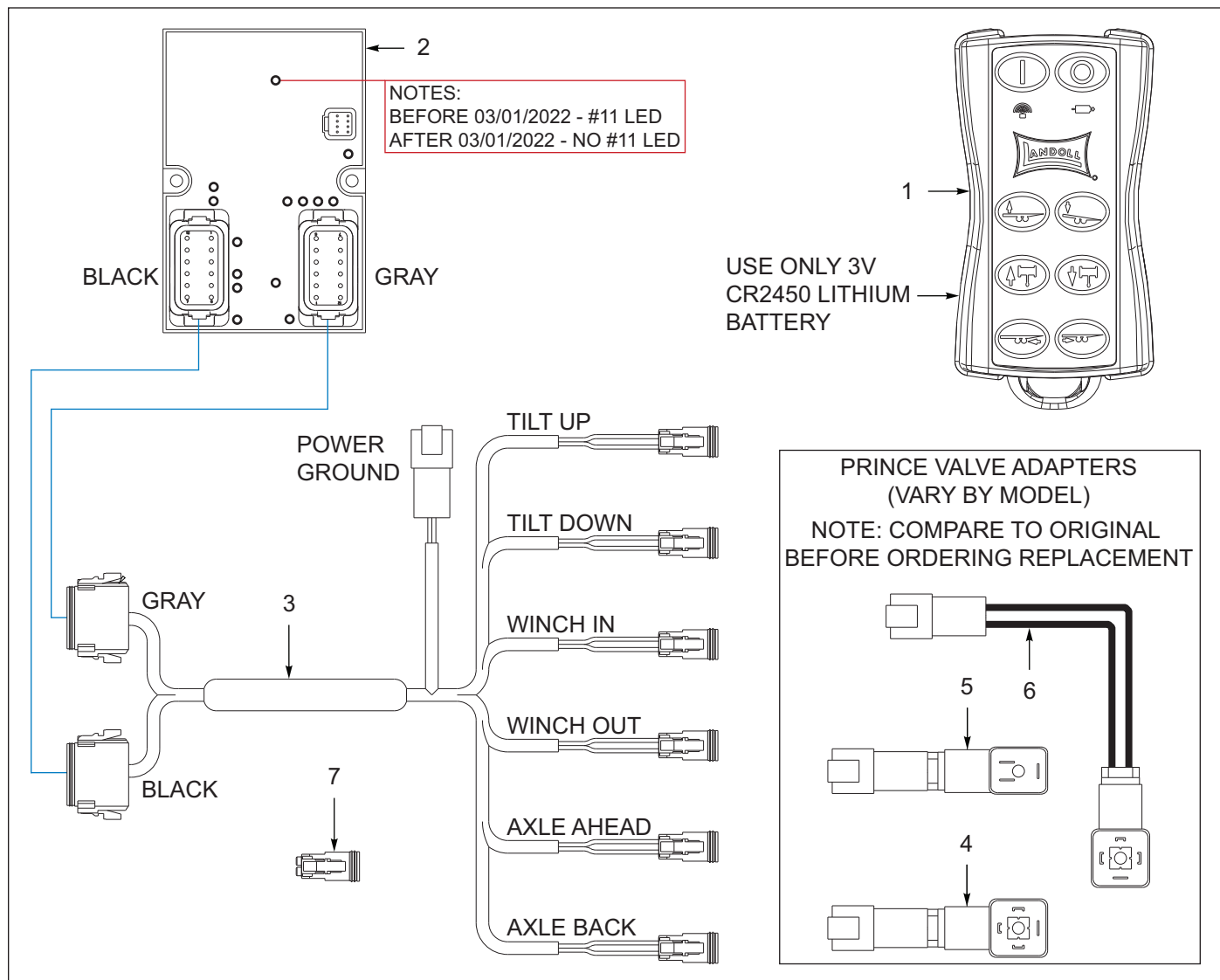
Figure 8-4: Wireless Remote Assembly, Brand (AFTER 08/01/2019)
