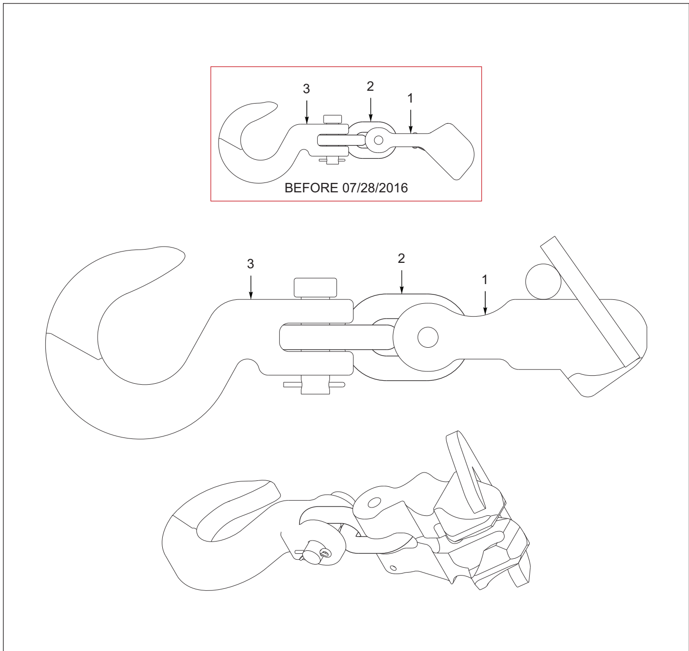
Figure 6-5: Container, Hook Assembly
