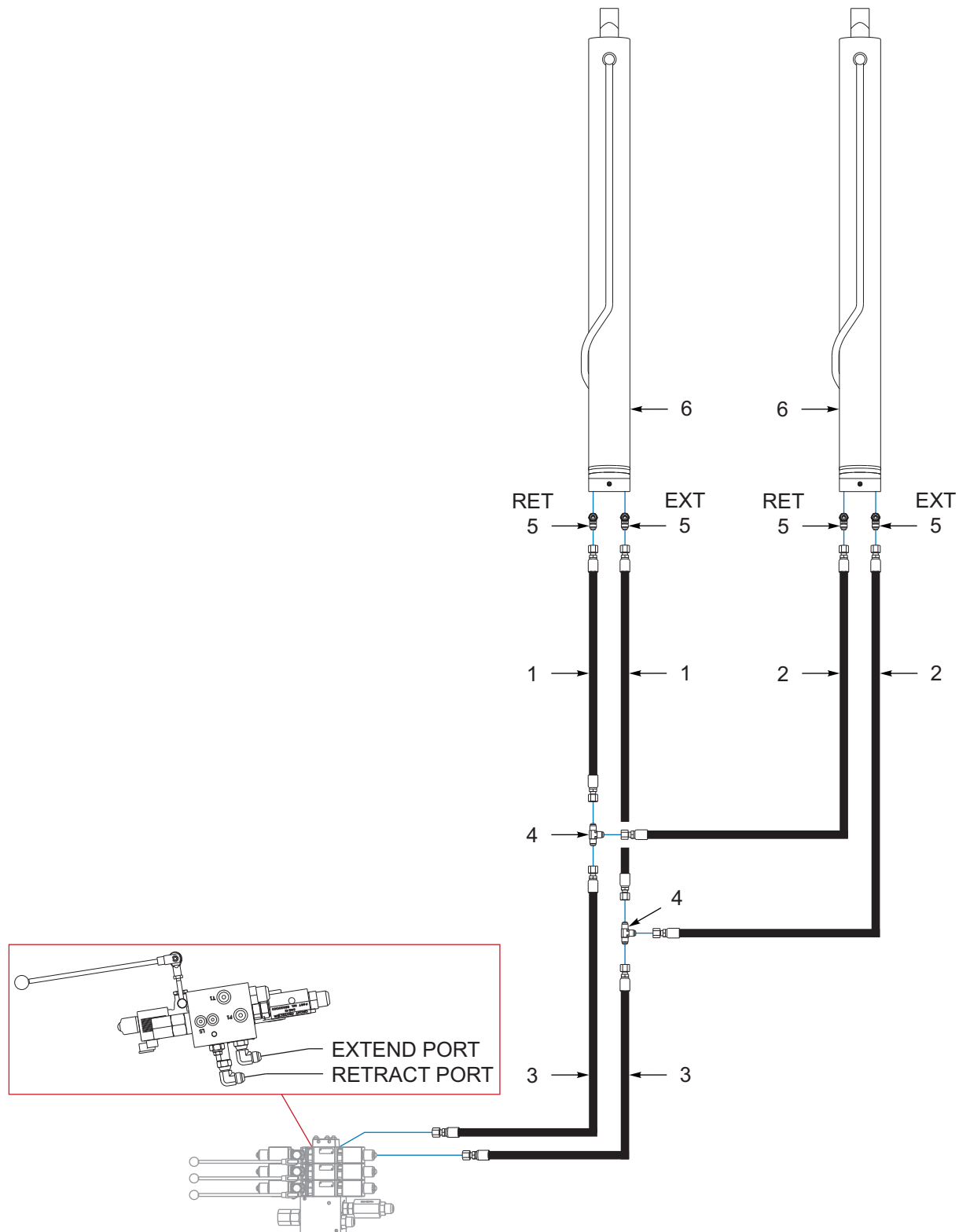
Figure 10-2: Fifth Wheel
