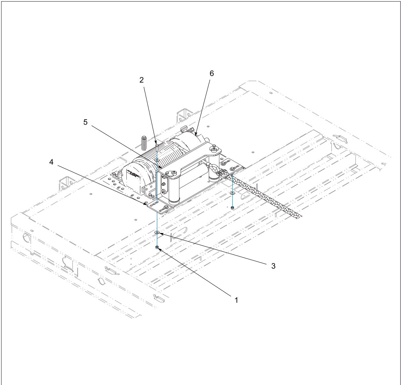
Figure 11-10: Winch Guide, Braden 20K, 4-Roller (OPTION)
