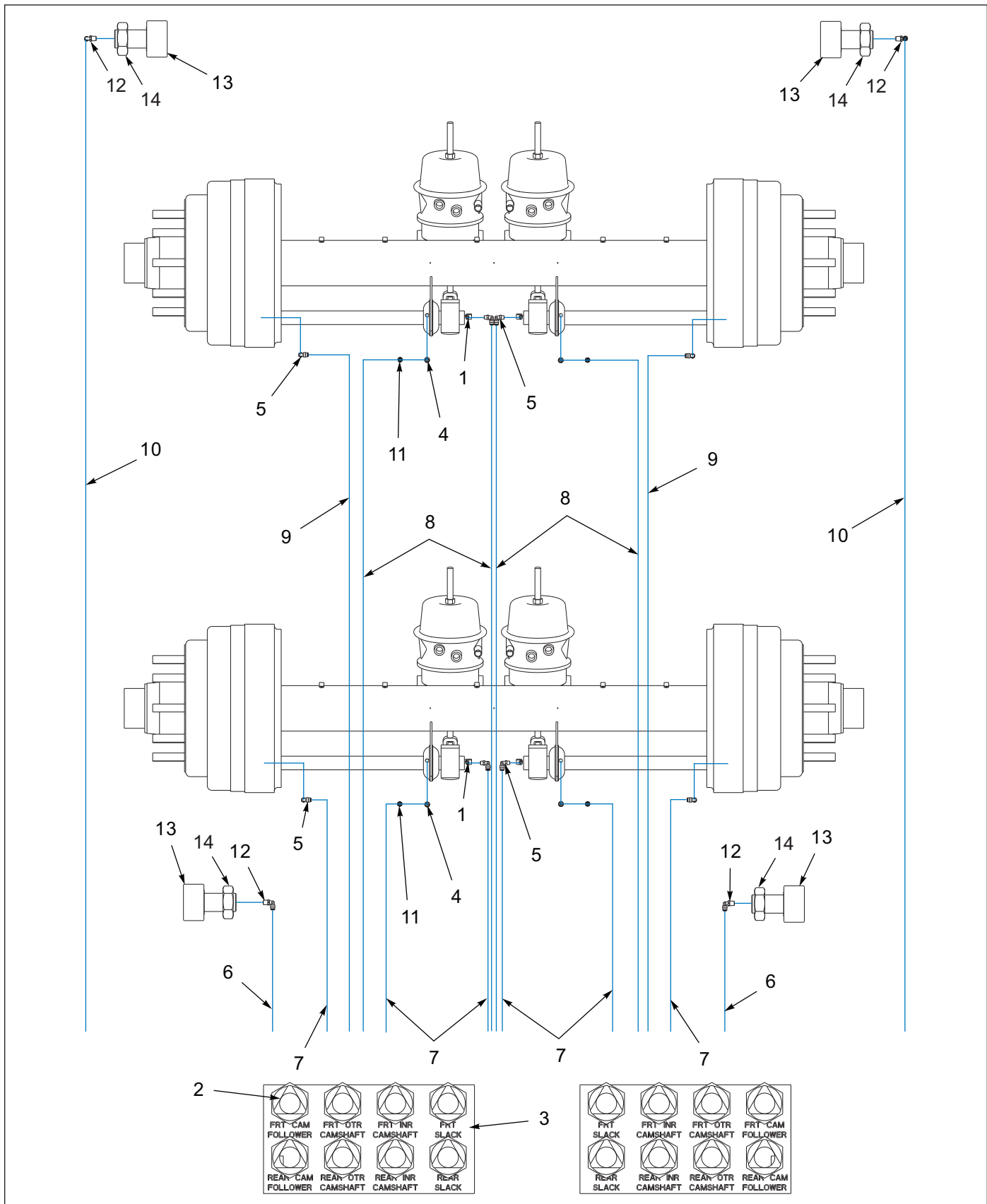
Figure 9-2: Frame, Tandem Axle Assembly
