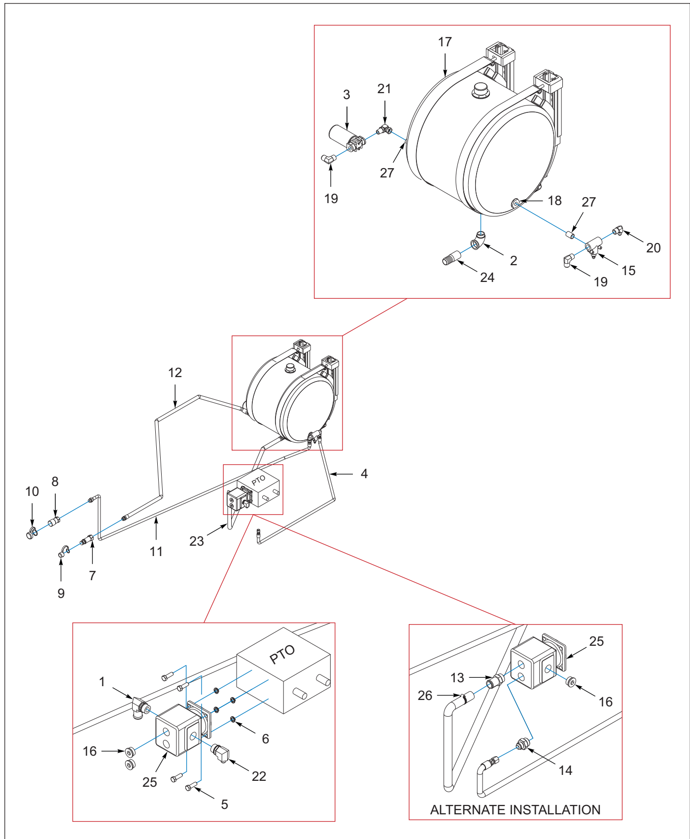
Figure 10-13: Kit, Wet, Hydraulic (OPTION) (AFTER 02/21/2019)
