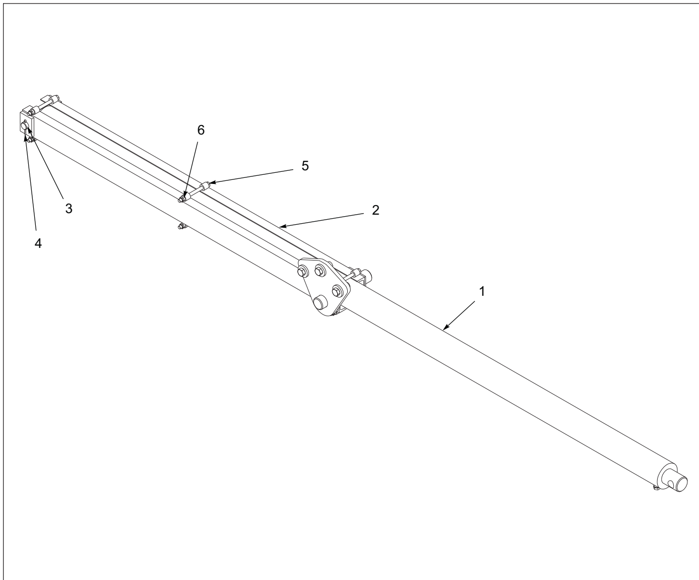
Figure 10-5: Cylinder Assembly, Standard Load Angle
