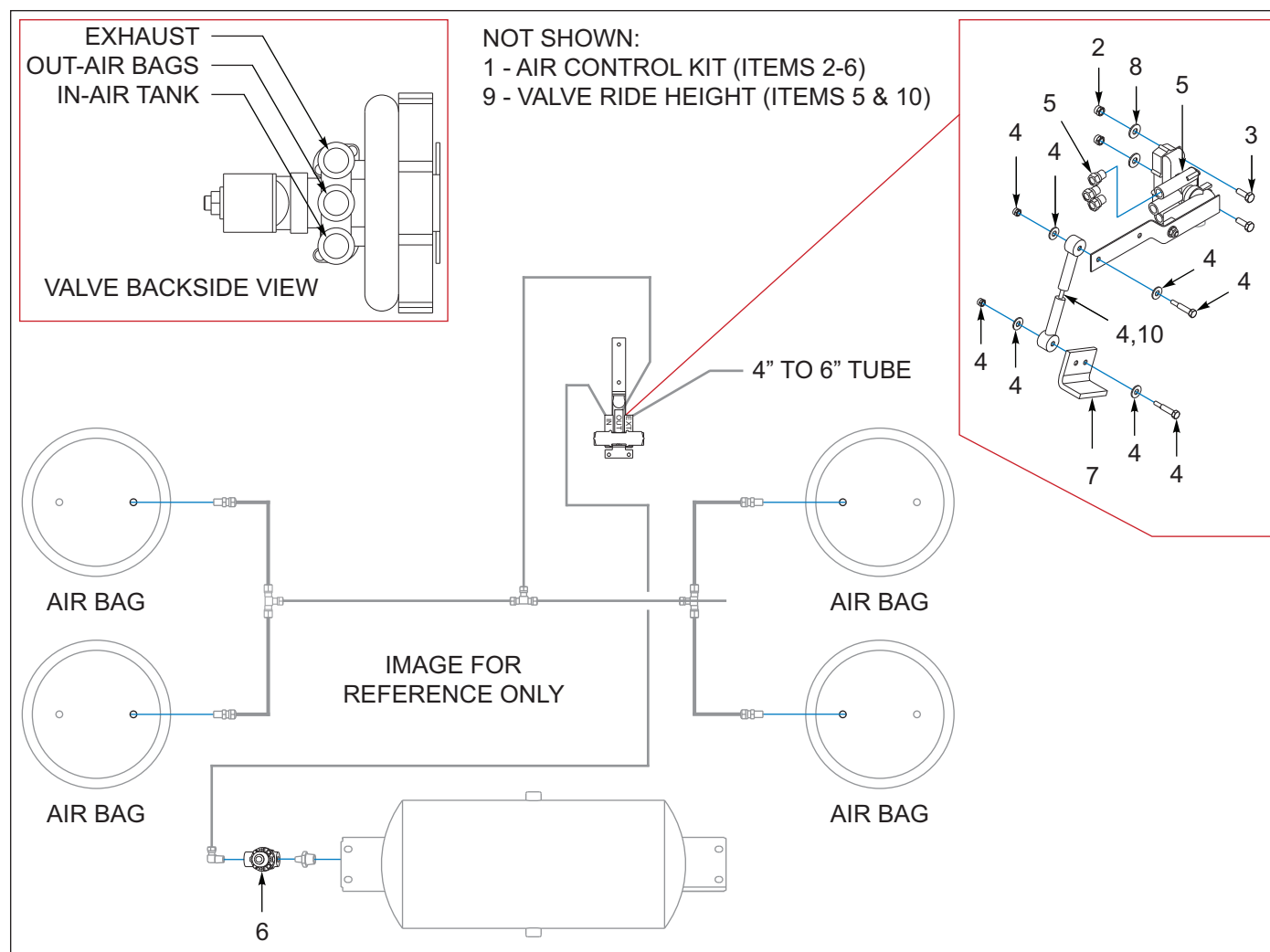
Figure 7-7: Air Control Kit
