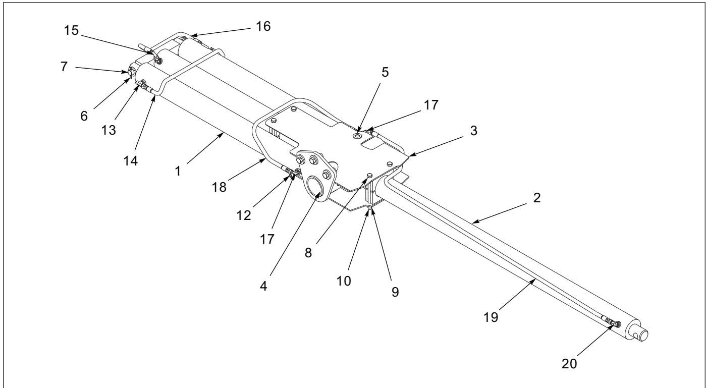
Figure 10-6: Cylinder Assembly, Low Load Angle (317 / 318)
