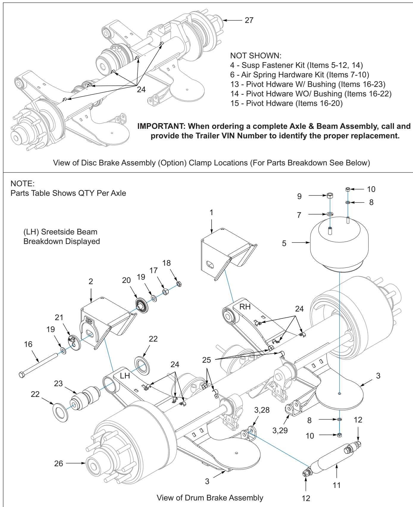
Figure 3-15: Axle Suspension, LSS-25K-3.5RLU, 12.25
