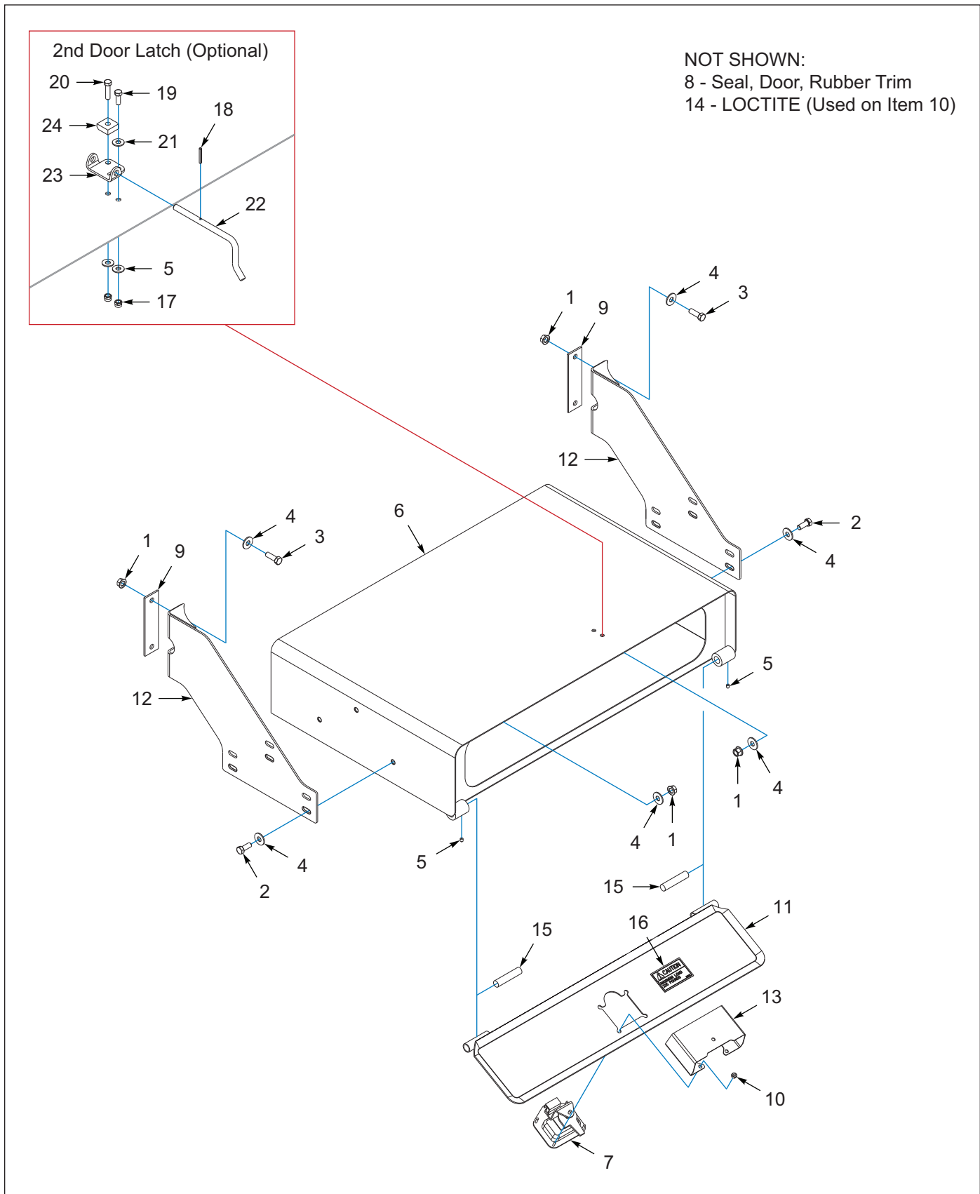
Figure 6-8: Toolbox, Bolt-On, 42"W X 28"D X 9"H (OPTIONS)
