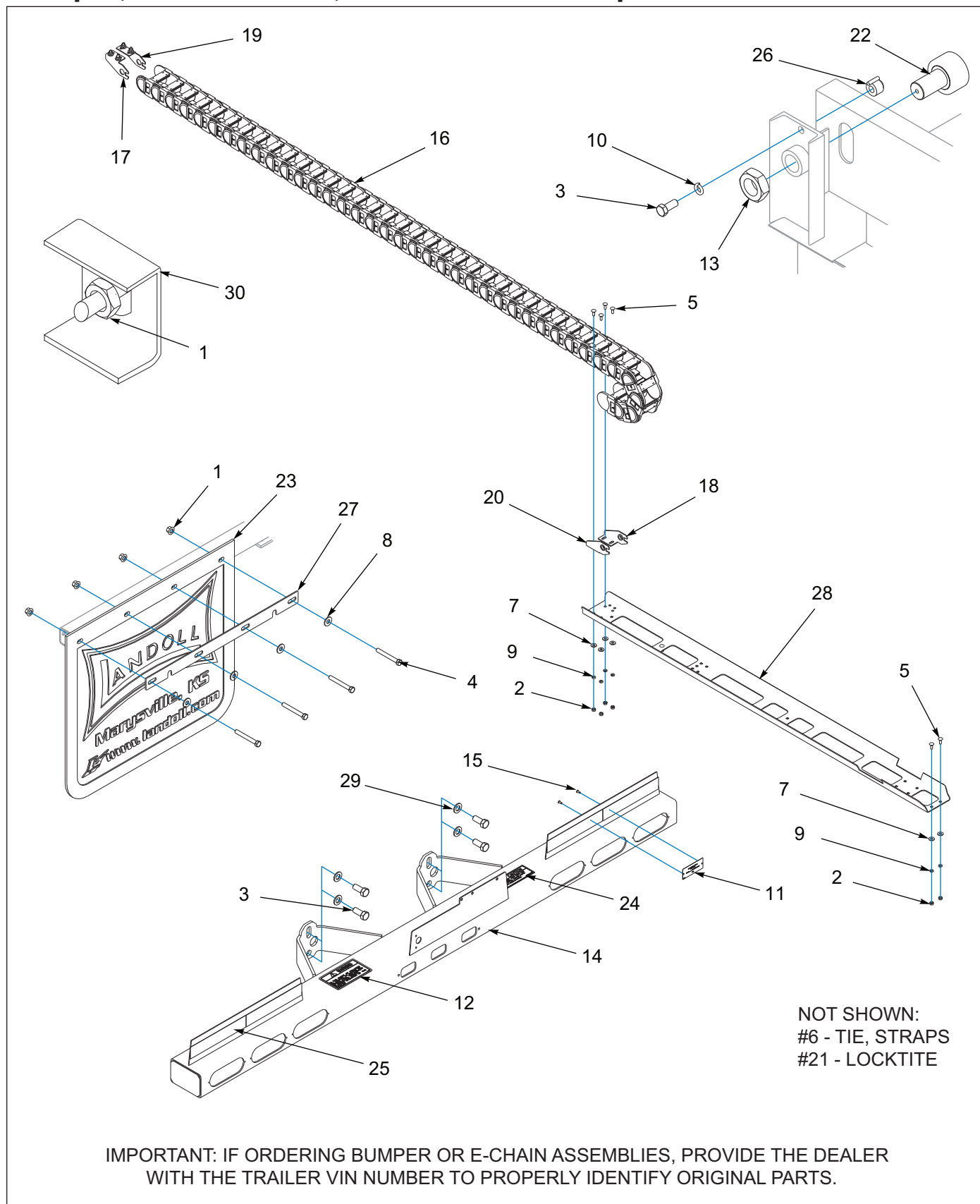
Figure 3-21: Bumper, Cam Follower, E-Chain & Mud Flap
