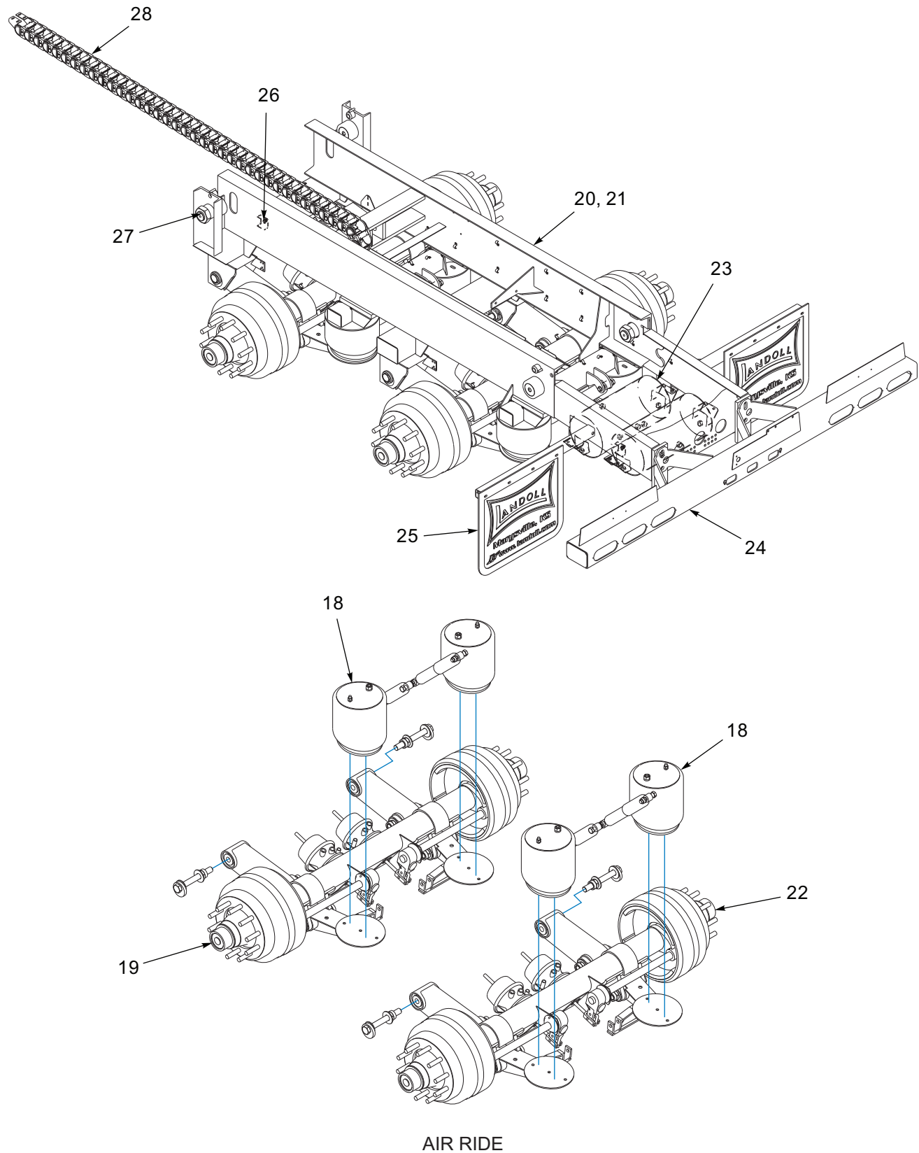
Figure 3-4: General Assembly, Tandem Axle (2 of 2)
