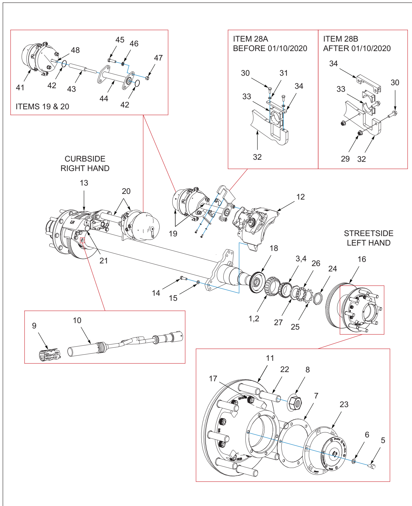
Figure 3-5: Axle 12.25 Disc Brakes & Hub Assembly (OPTION) (1 of 2)
