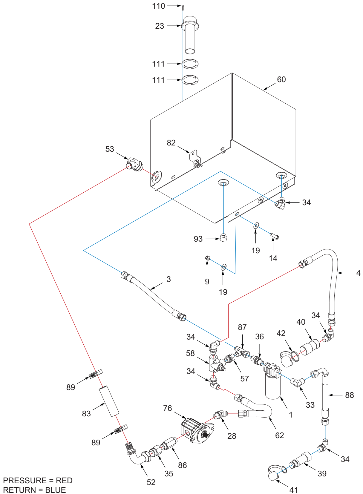
Figure 12-10: Engine Assembly, Kohler 25HP EFI, Gasoline, 30 Gallon (OPTION) (5 of 5)
