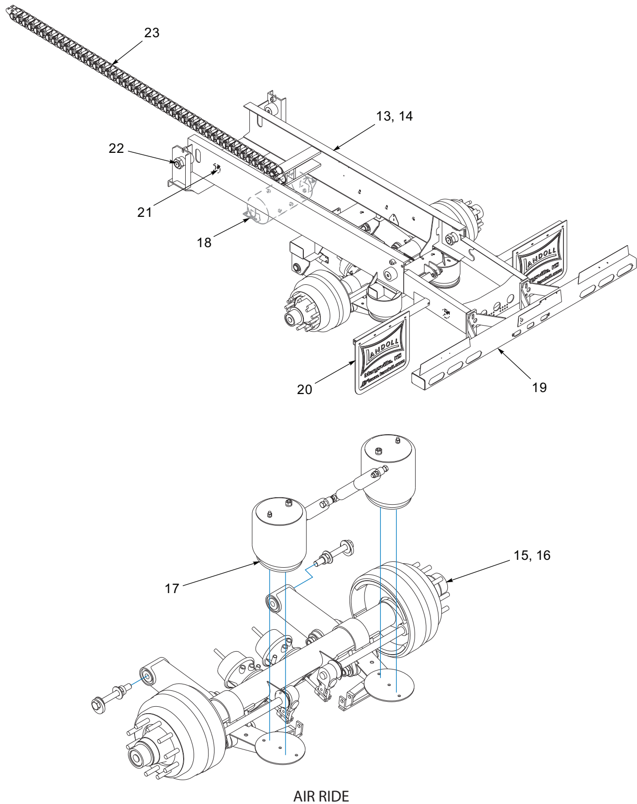
Figure 3-2: General Assembly, Single Axle (2 of 2)
