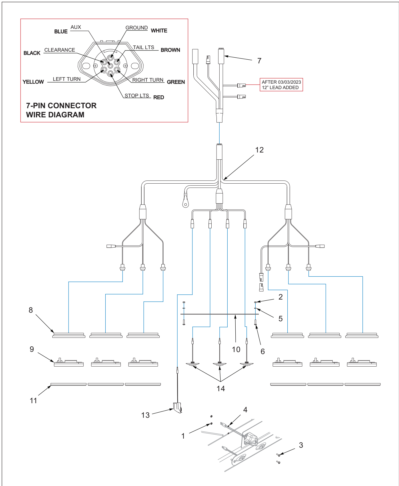
Figure 8-2: Frame, Harness, Rear Bumper
