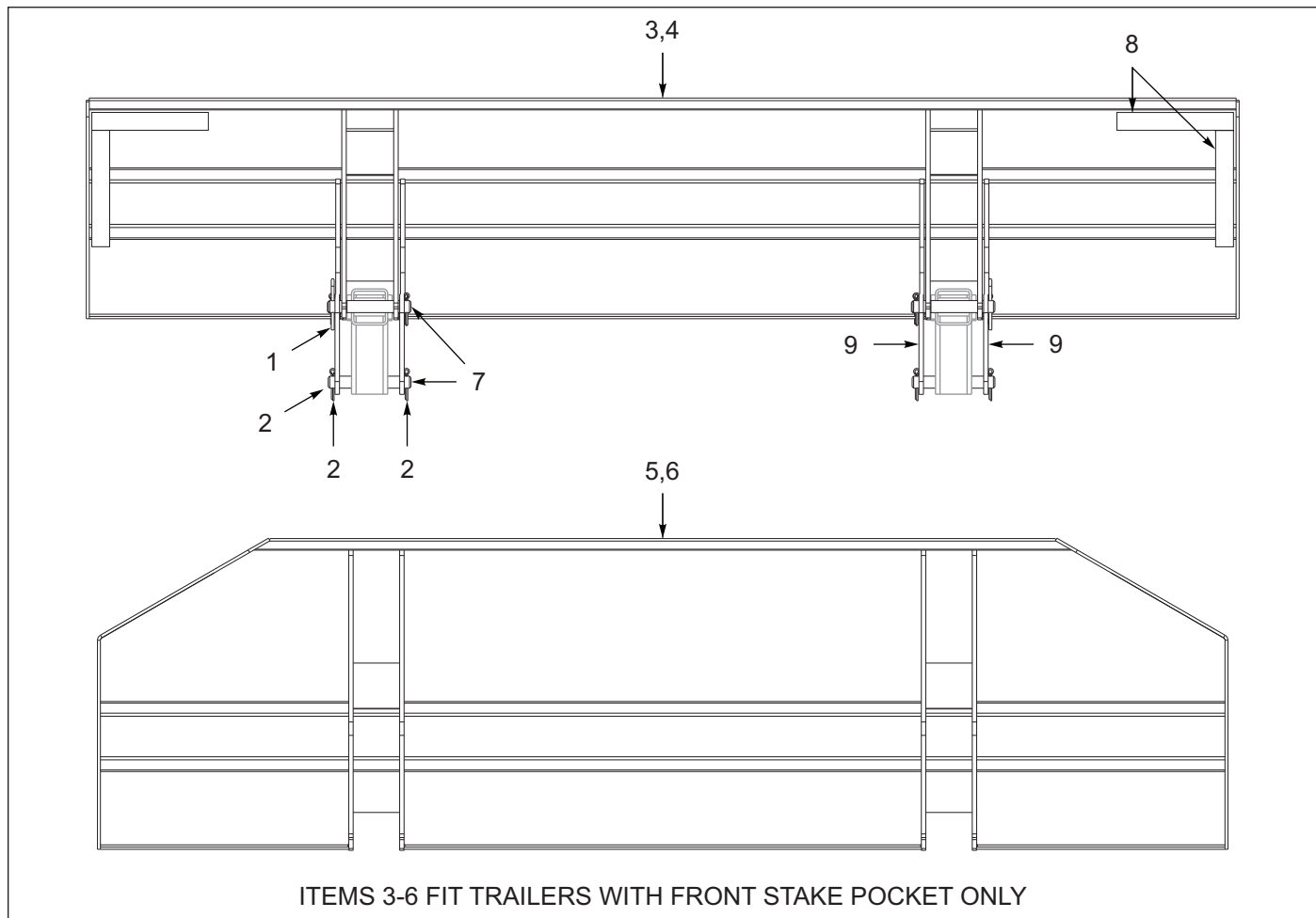
Figure 4-1: Bulkhead, 2 Position (OPTION)
