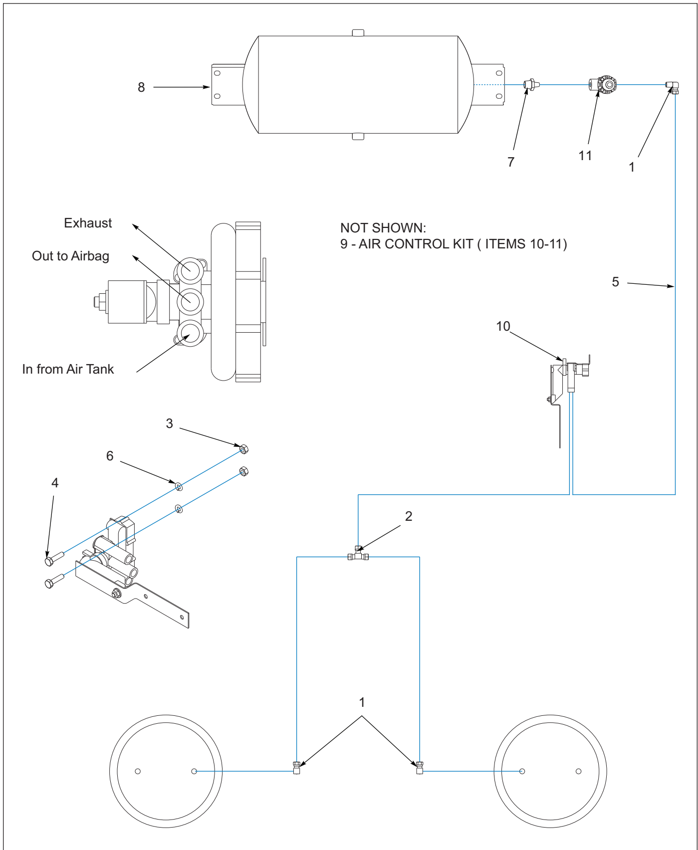
Figure 7-5: Control, Air Suspension Height, Single Axle
