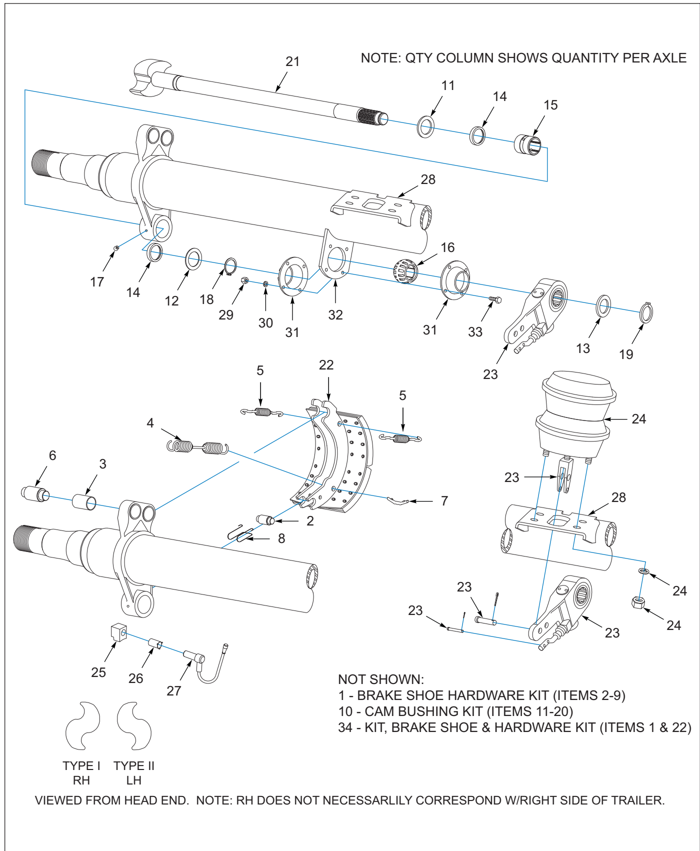
Figure 3-11: Axle 16.5 x 7 Drum Brakes, Dexter
