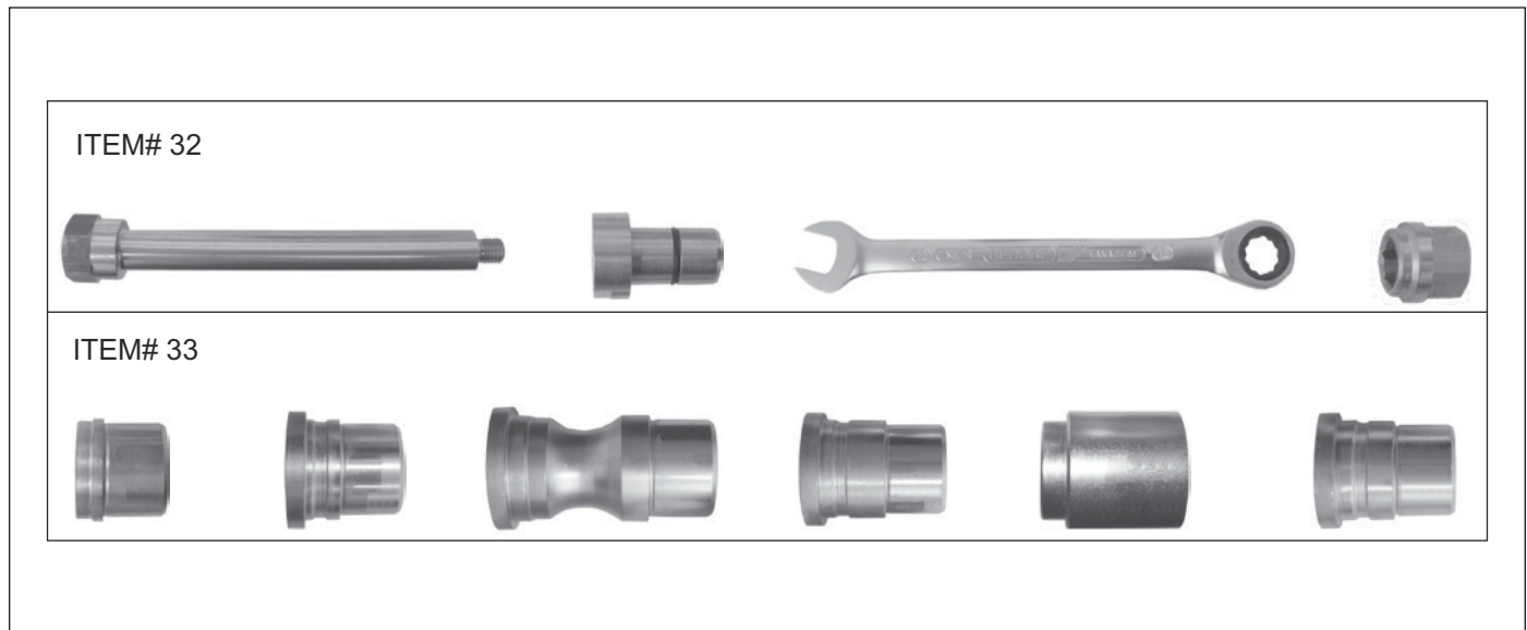
Figure 3-10: Axle 16.5 Disc Brakes &amp; Hub Assembly (OPTION) (2 of 2)
