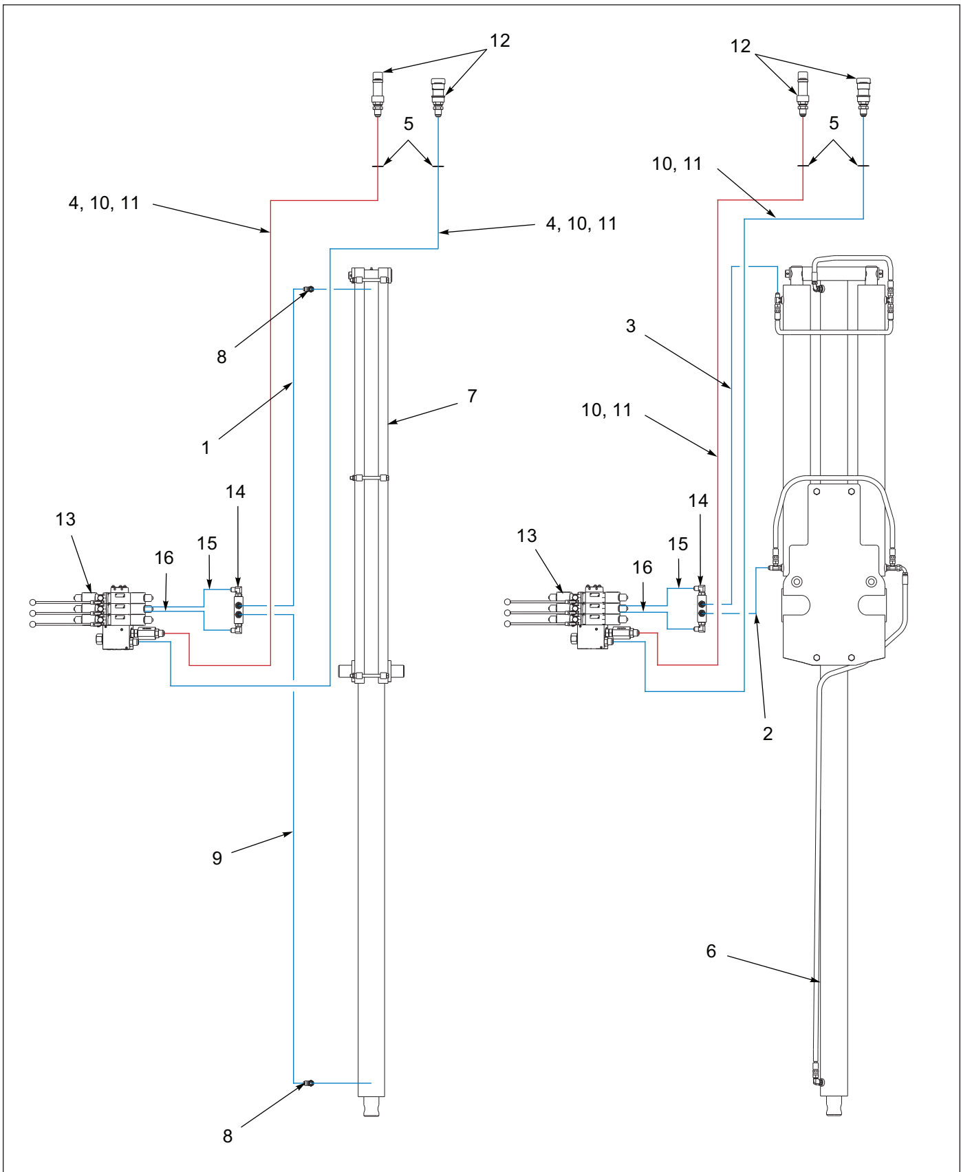
Figure 10-3: Standard & Low Load Angle Cylinder Assembly
