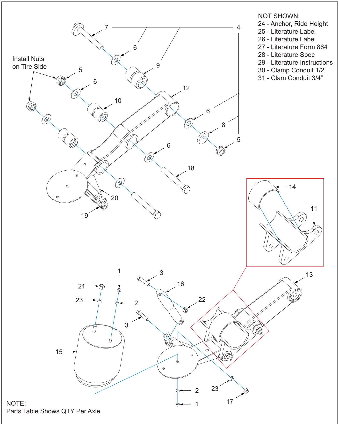
Figure 3-14: Axle Suspension, RLU-228, 12.25 & 16.5 (2 of 2)
