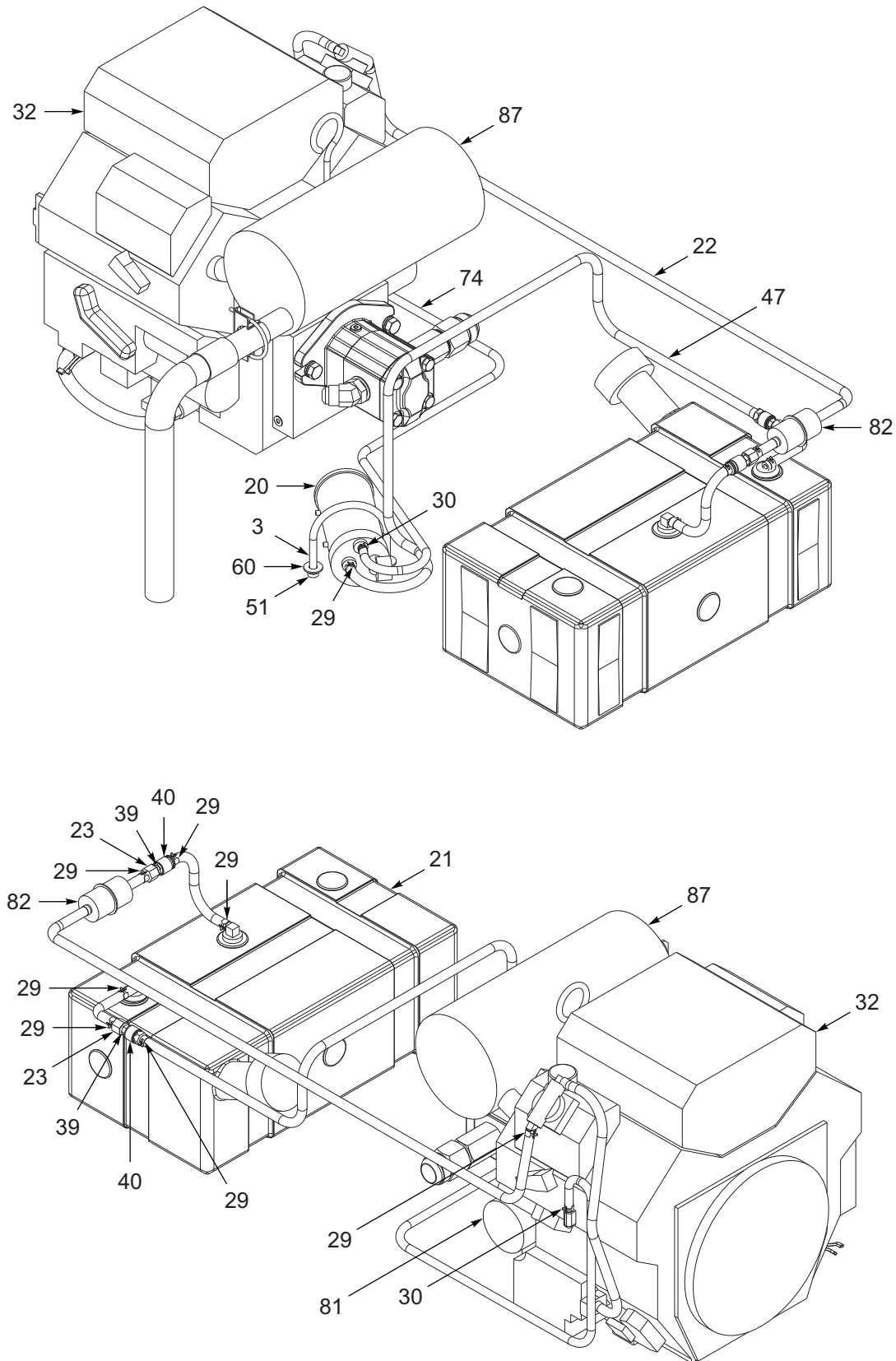
Figure 12-4: Engine Assembly, Kohler 25HP EFI, Gasoline, 15 Gallon (OPTION) (4 of 5)
