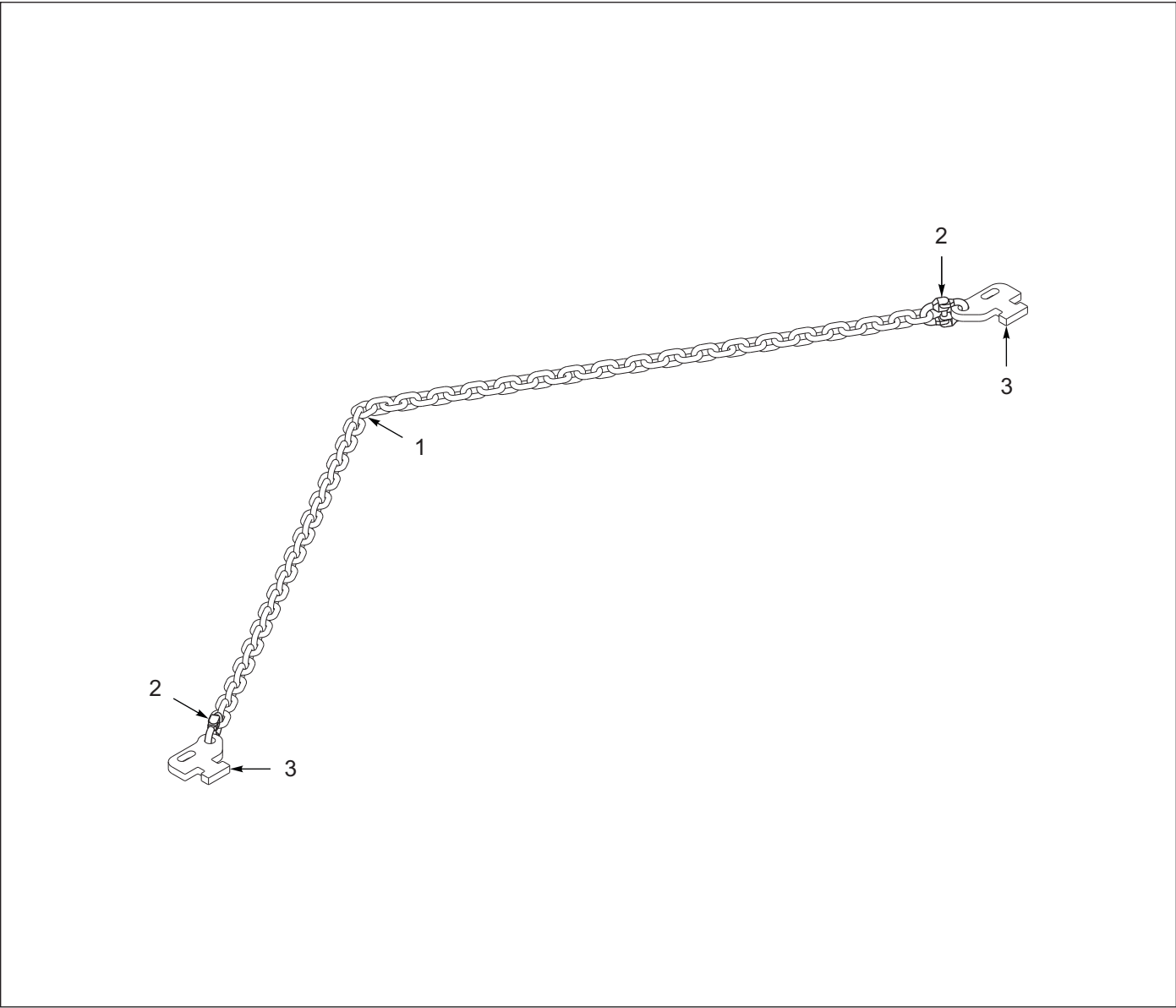
Figure 6-1: Chain Assembly, Container Loading, 1 Chain
