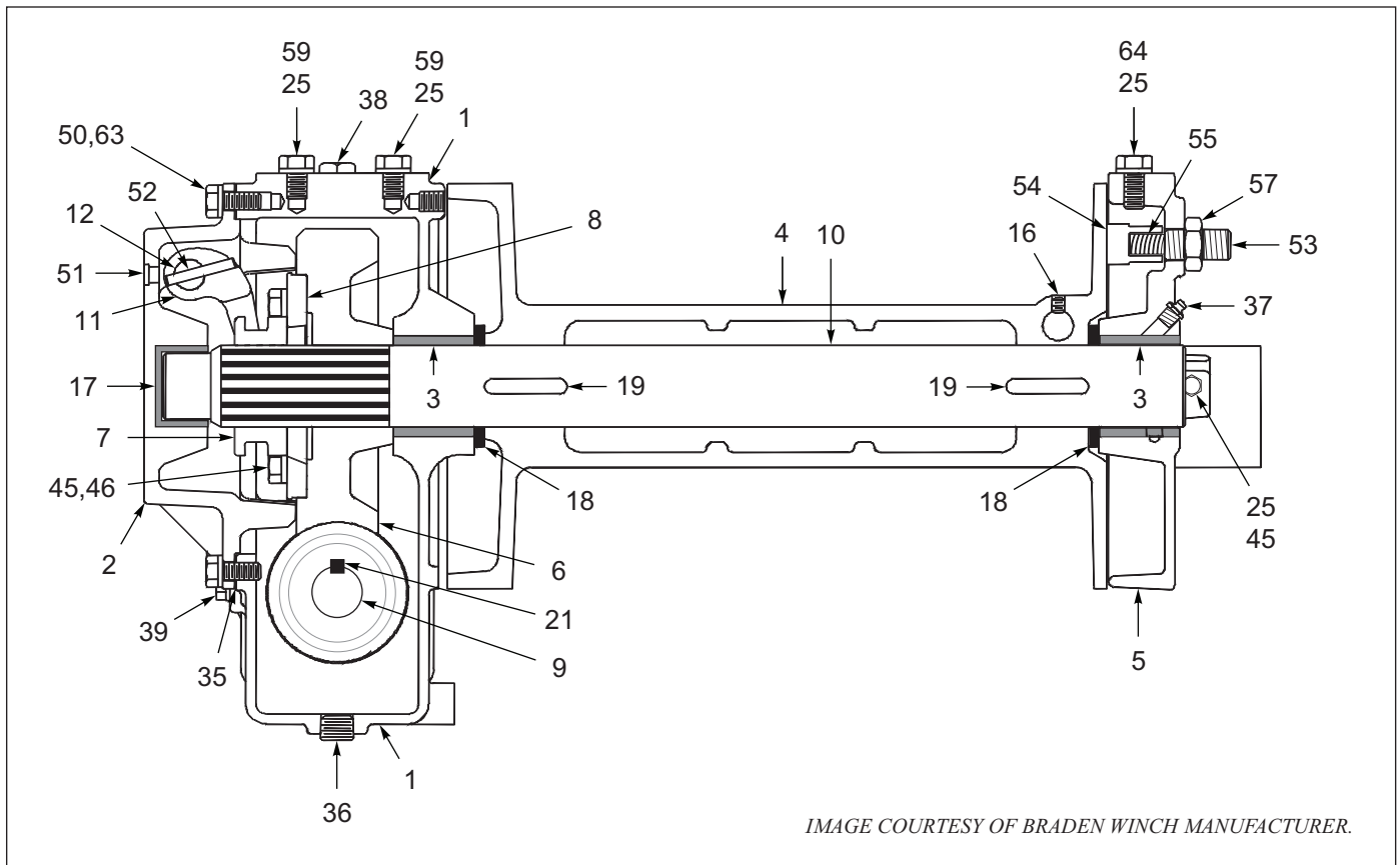
Figure 11-8: Winch Components, Braden 20K (OPTION) (2 of 2)
