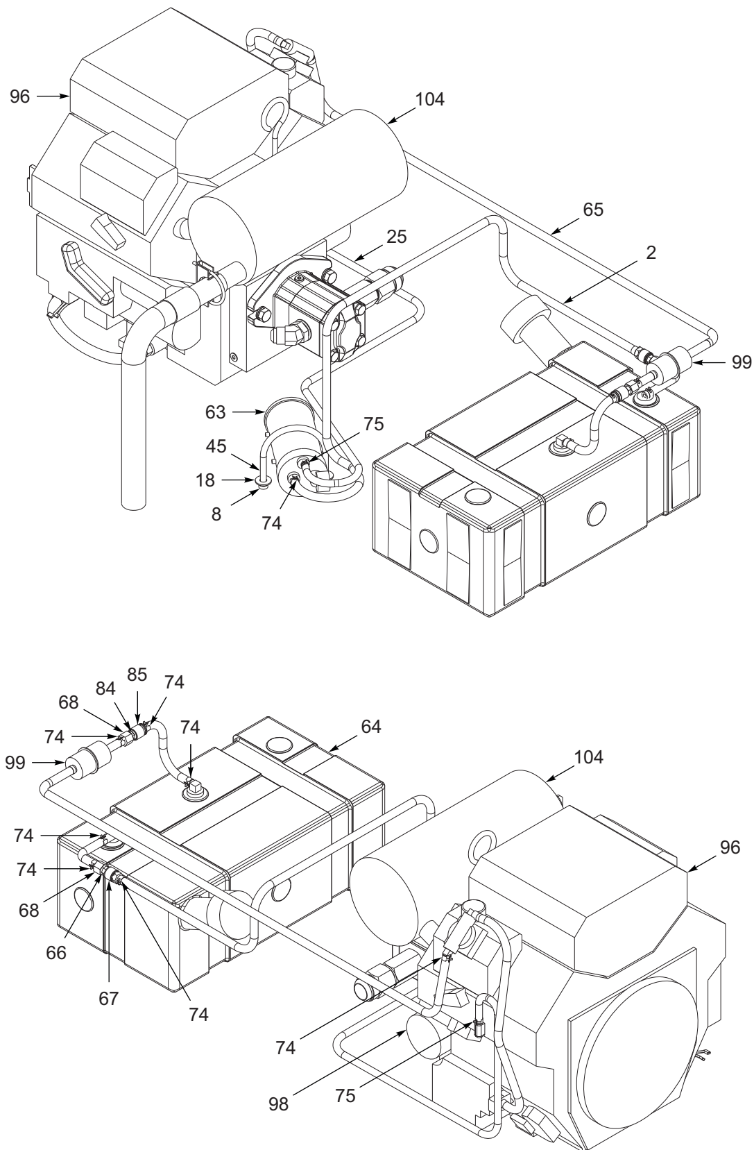
Figure 12-9: Engine Assembly, Kohler 25HP EFI, Gasoline, 30 Gallon (OPTION) (4 of 5)
