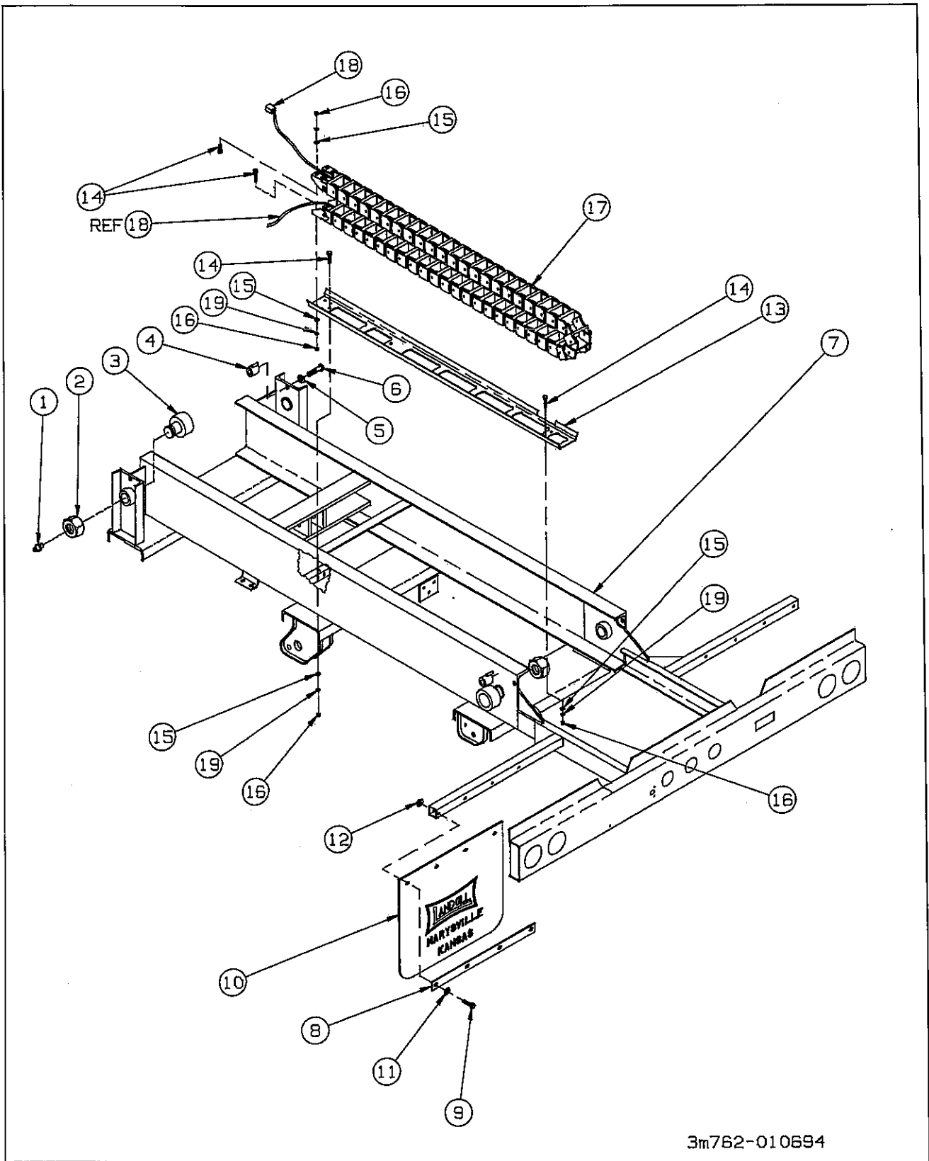
Figure 1-10 Undercarriage Assembly
