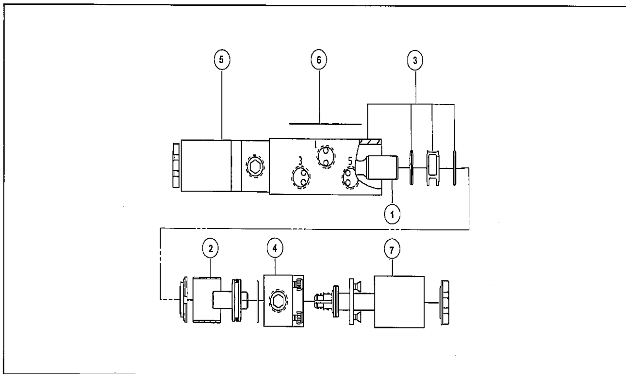
Figure 1-37 Pneumatic Valve
