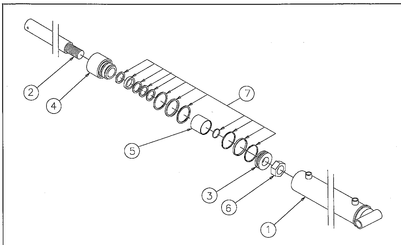
Figure 1-7 Undercarriage Slide Cylinder Assembly
