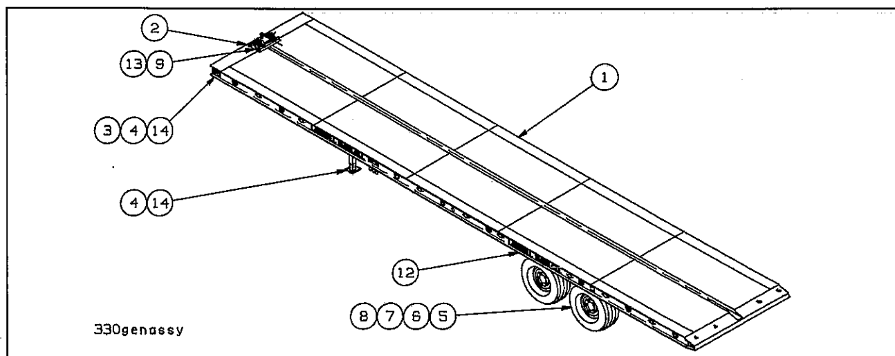
Figure 1-1 General Assembly
