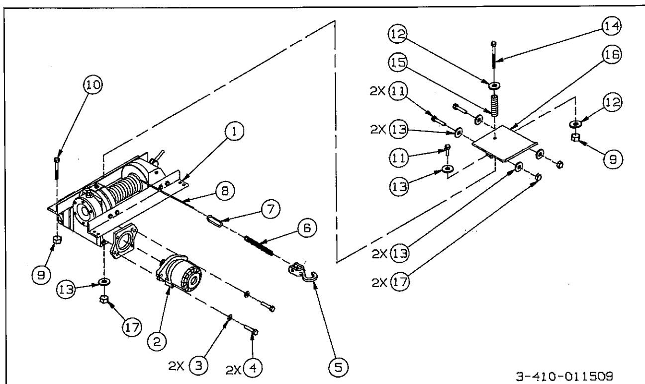
Figure 1-22 Winch Installation
