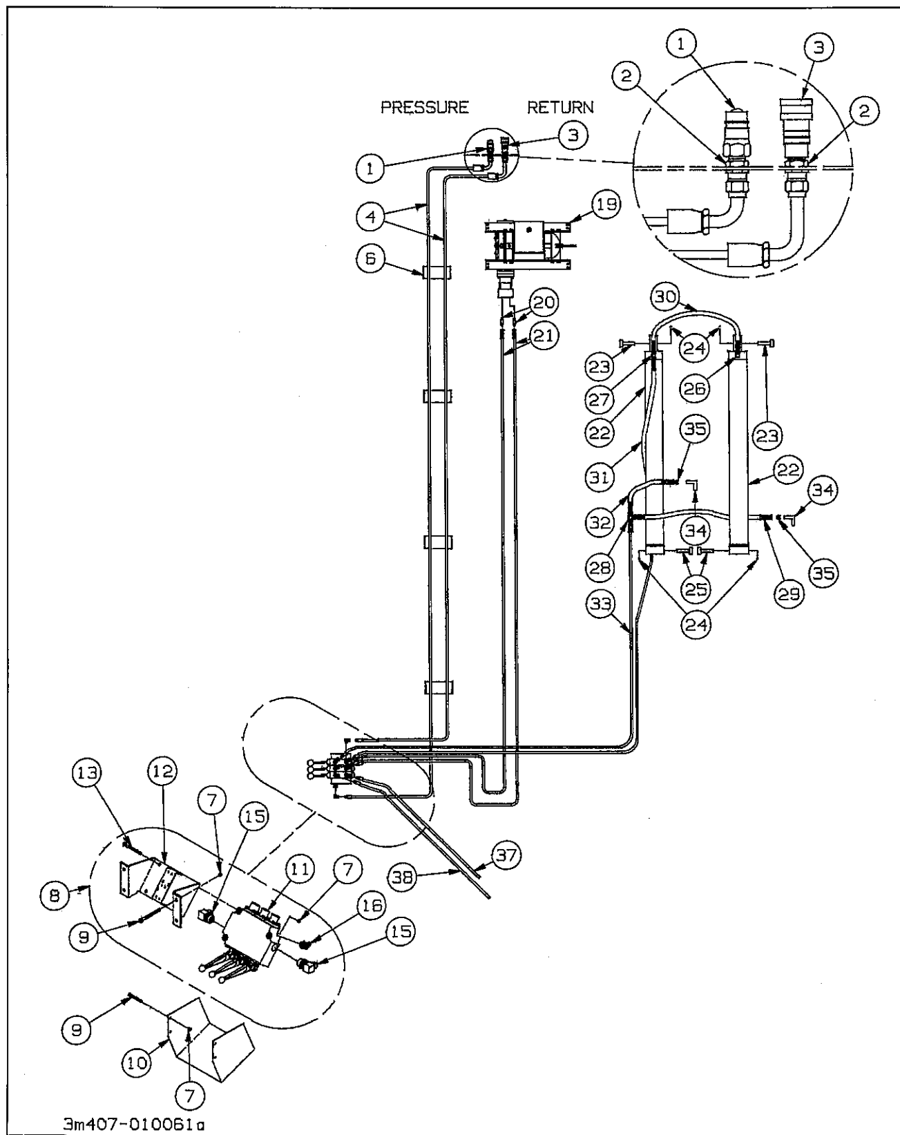
Figure 1-3 Hydraulic System
