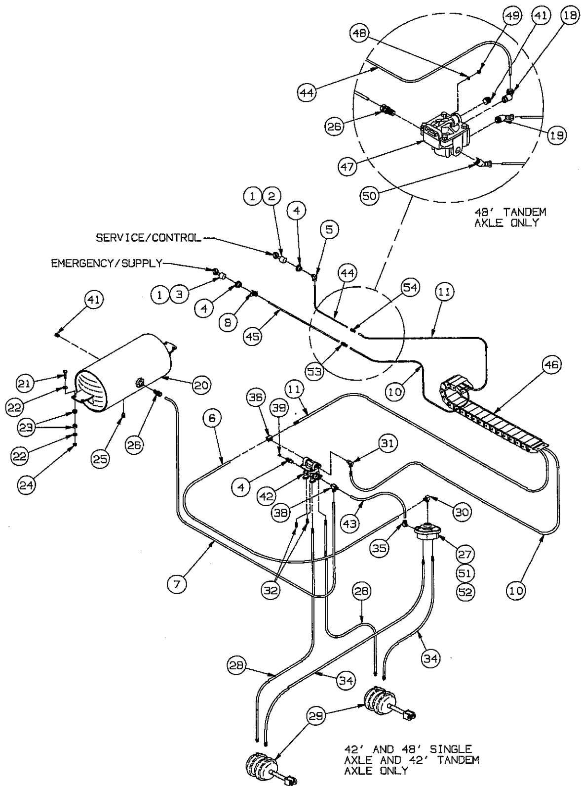
Figure 1-17 Air Brake System, Single Axle
