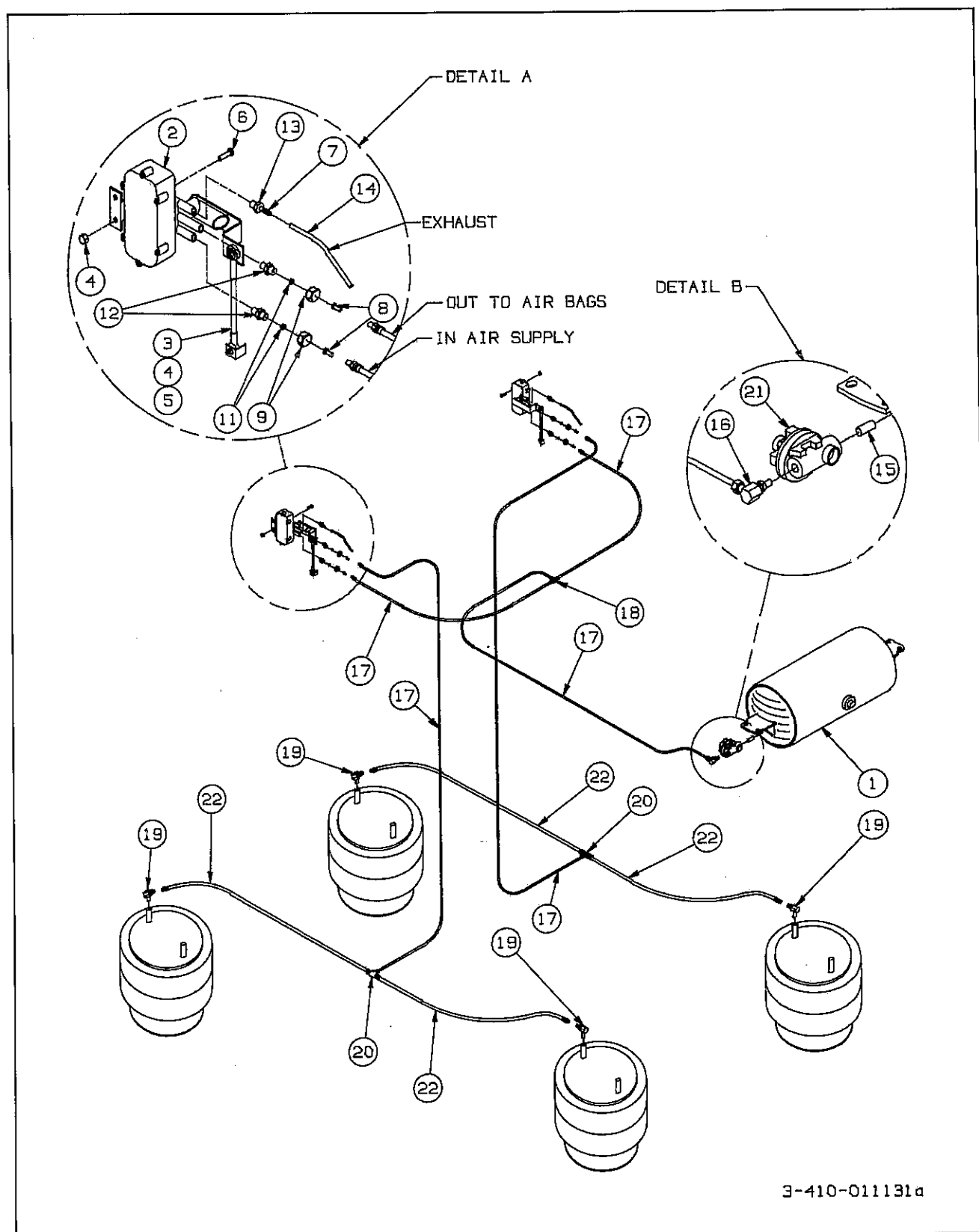
Figure 1-15 Air Ride Suspension System (Tandem)
