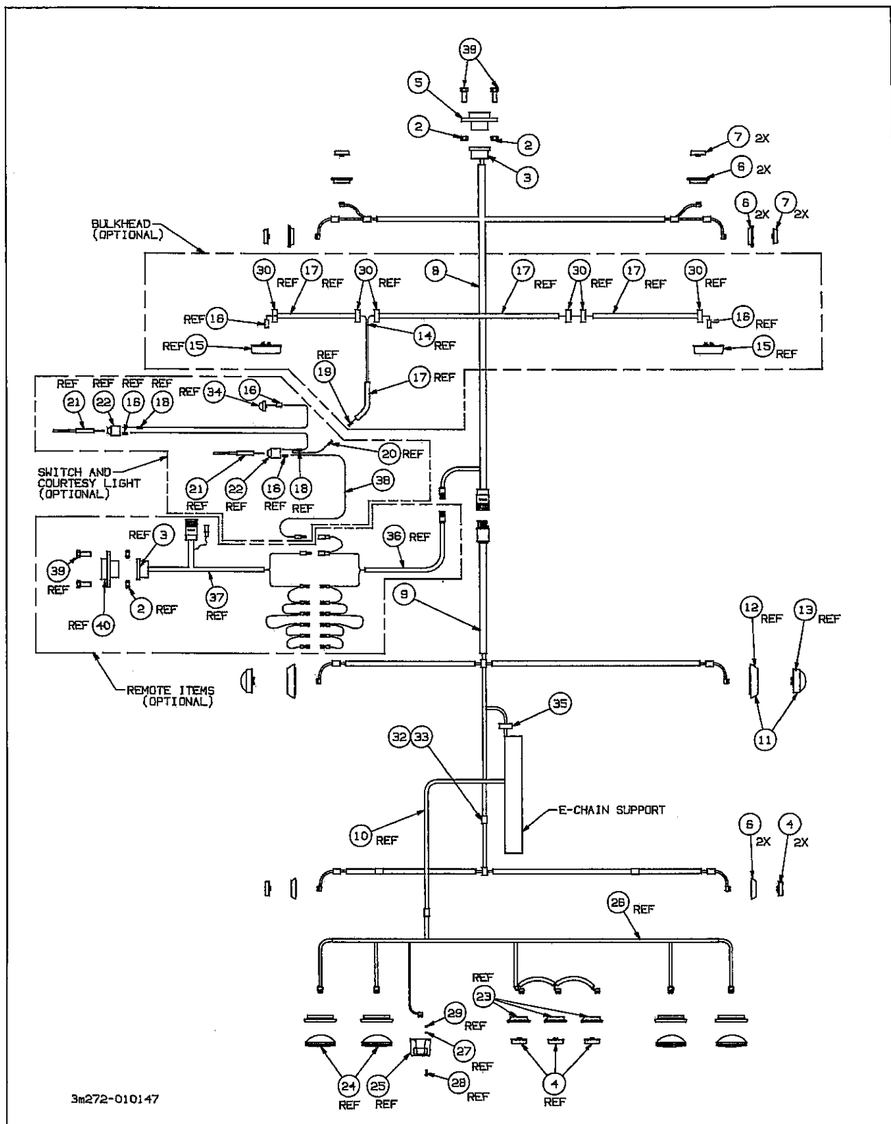
Figure 1-9 Electrical System
