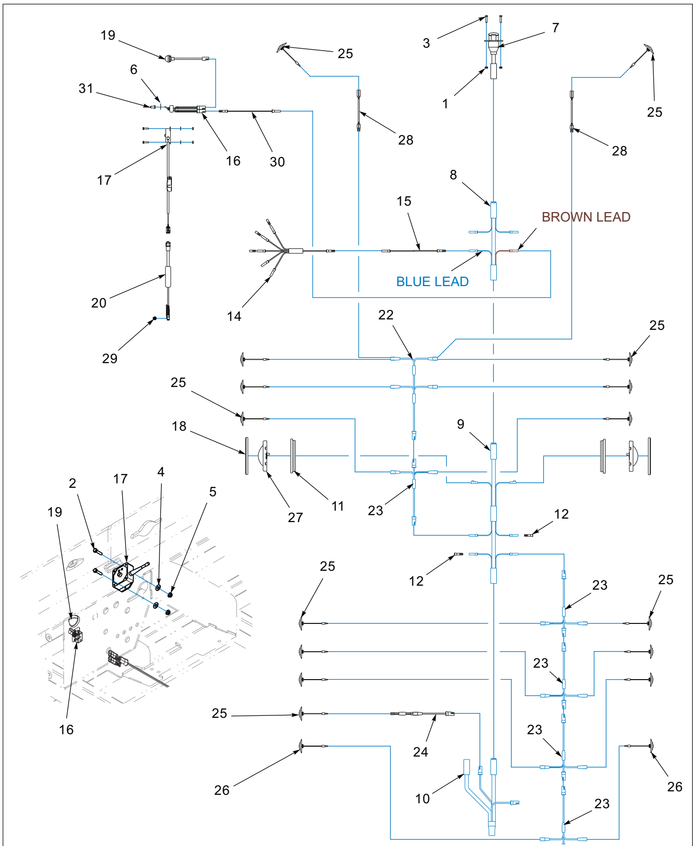
Figure 1-11: Electrical System
