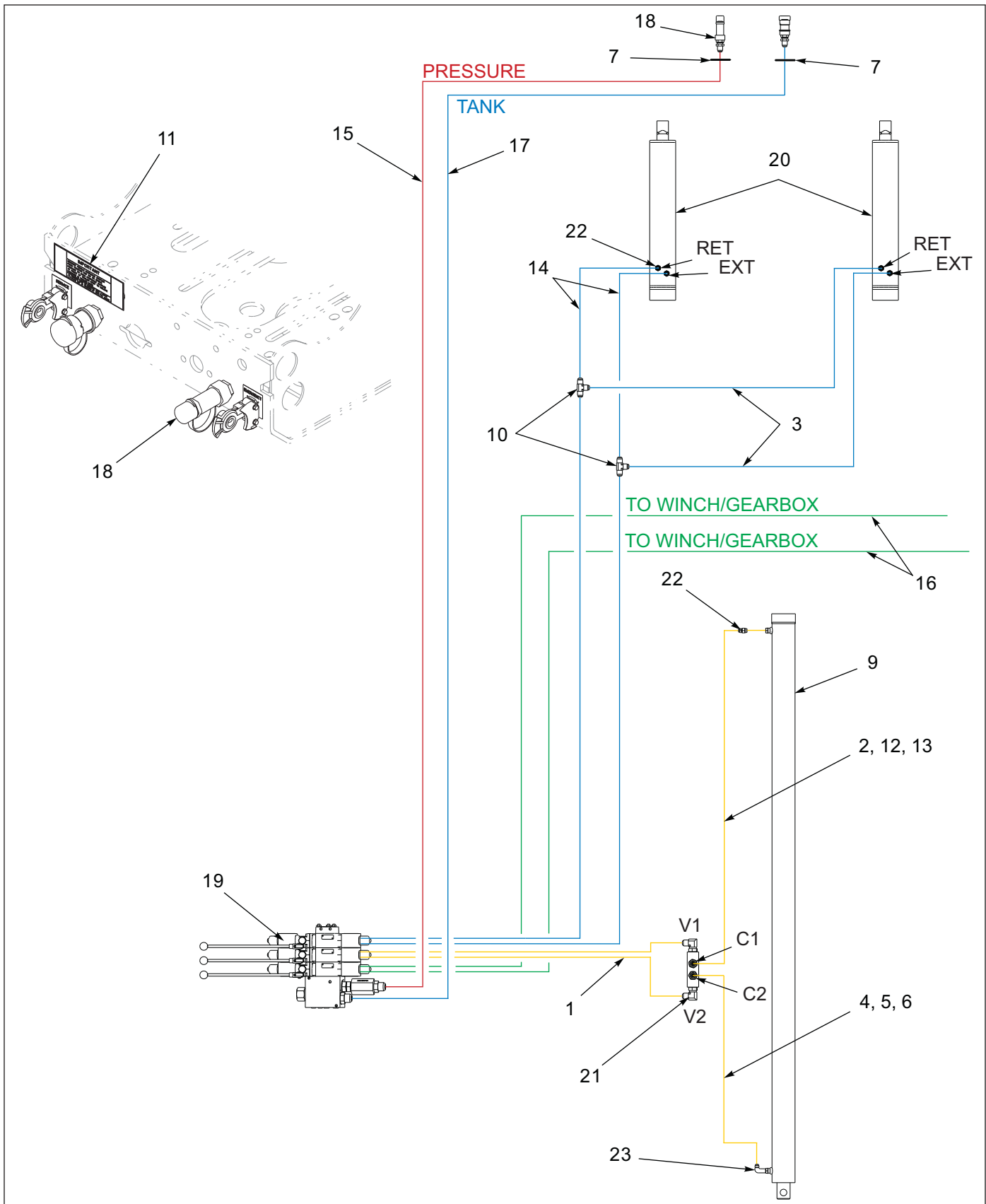
Figure 1-6: Hydraulic Assembly
