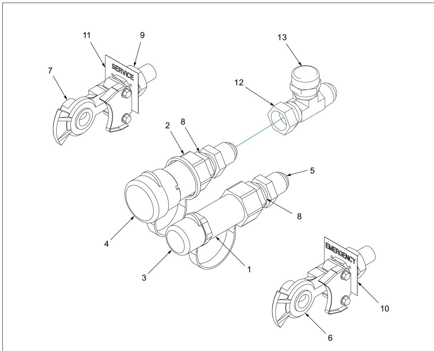
Figure 1-8: Connectors - Front Sub Assembly
