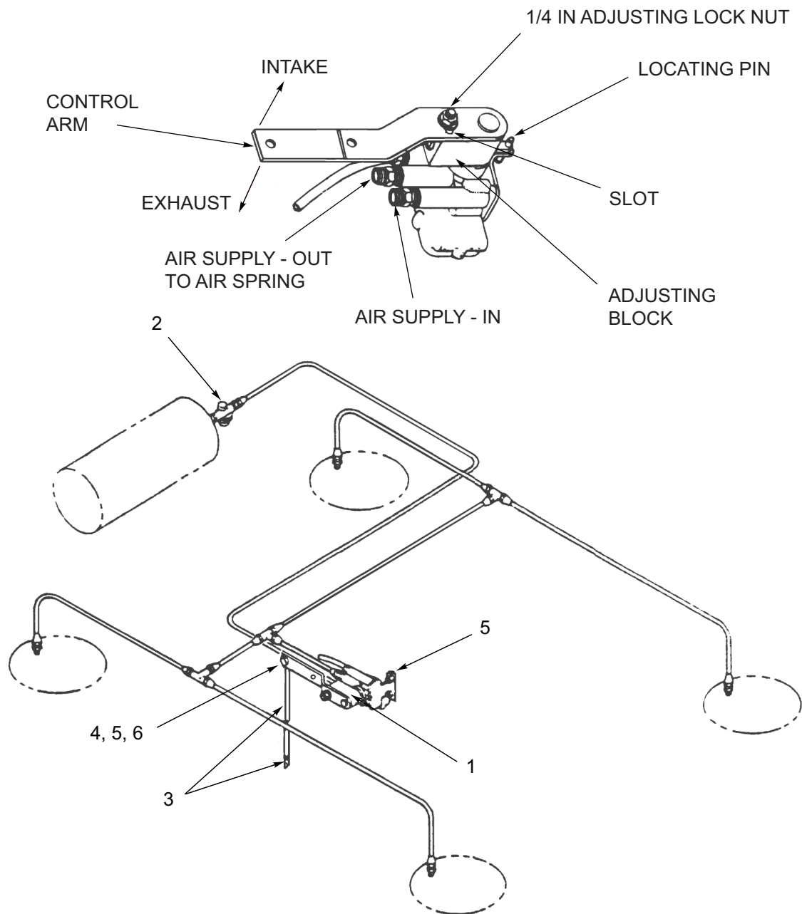
Figure 1-18: Air Control Kit
