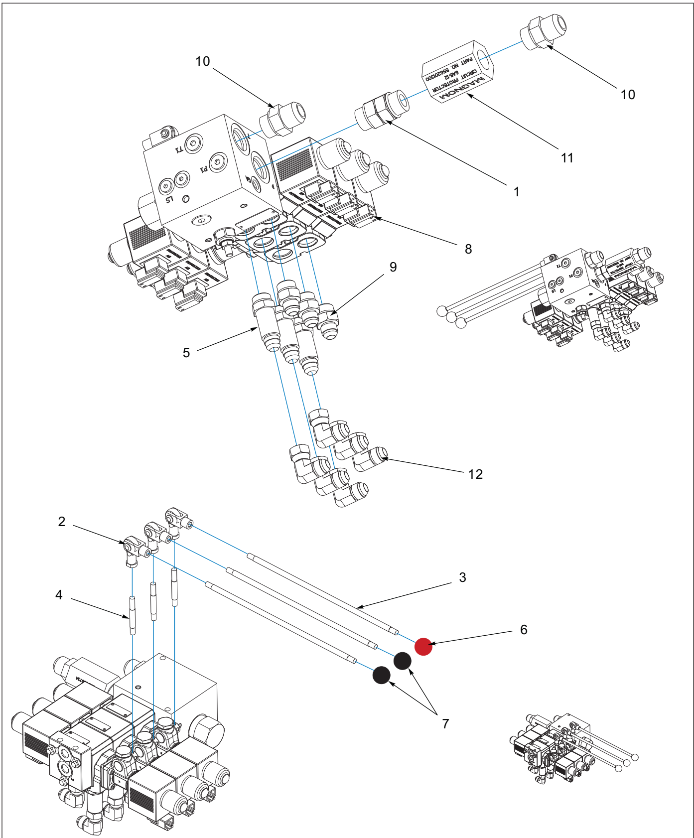
Figure 1-9: Valve Assembly - Three Spool
