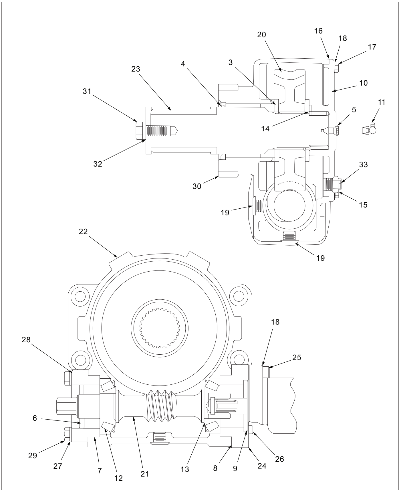
Figure 1-29: Gearbox Items
