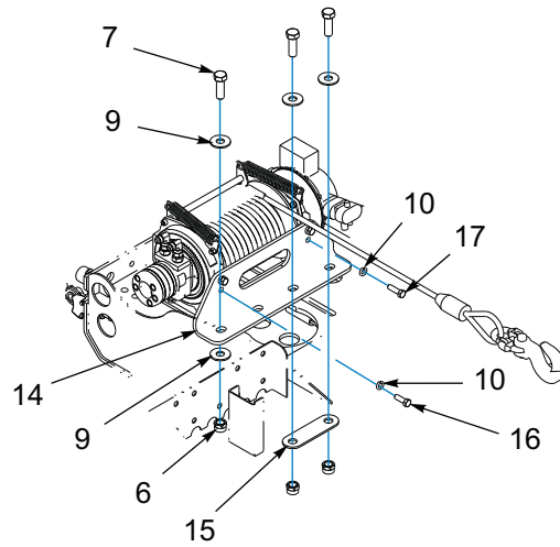
GENERAL ASSEMBLY
