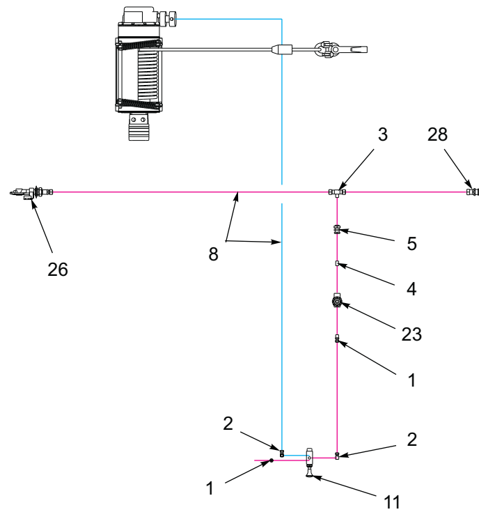
AIR SYSTEM
