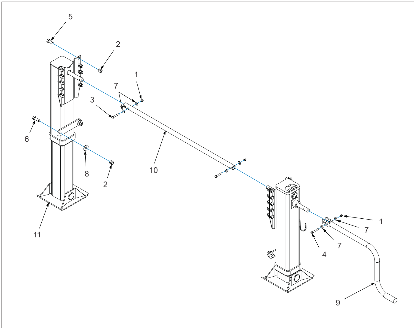
Figure 1-47: Landing Gear Installation - Jost 343
