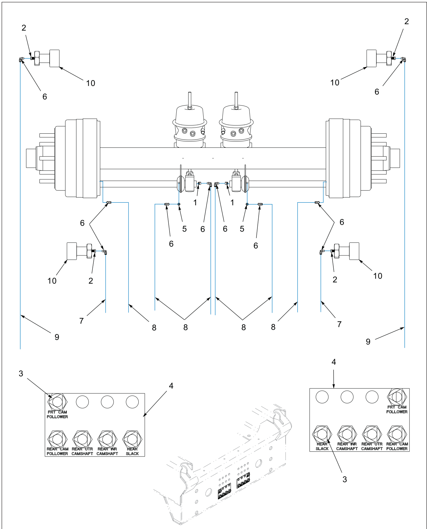
Figure 1-16: Grease System
