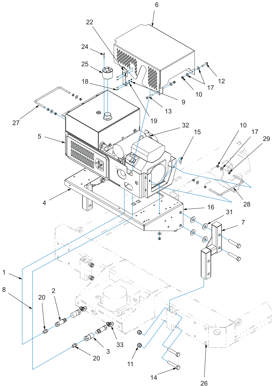
Figure 1-53: Engine - 25 HP Drive Installation
