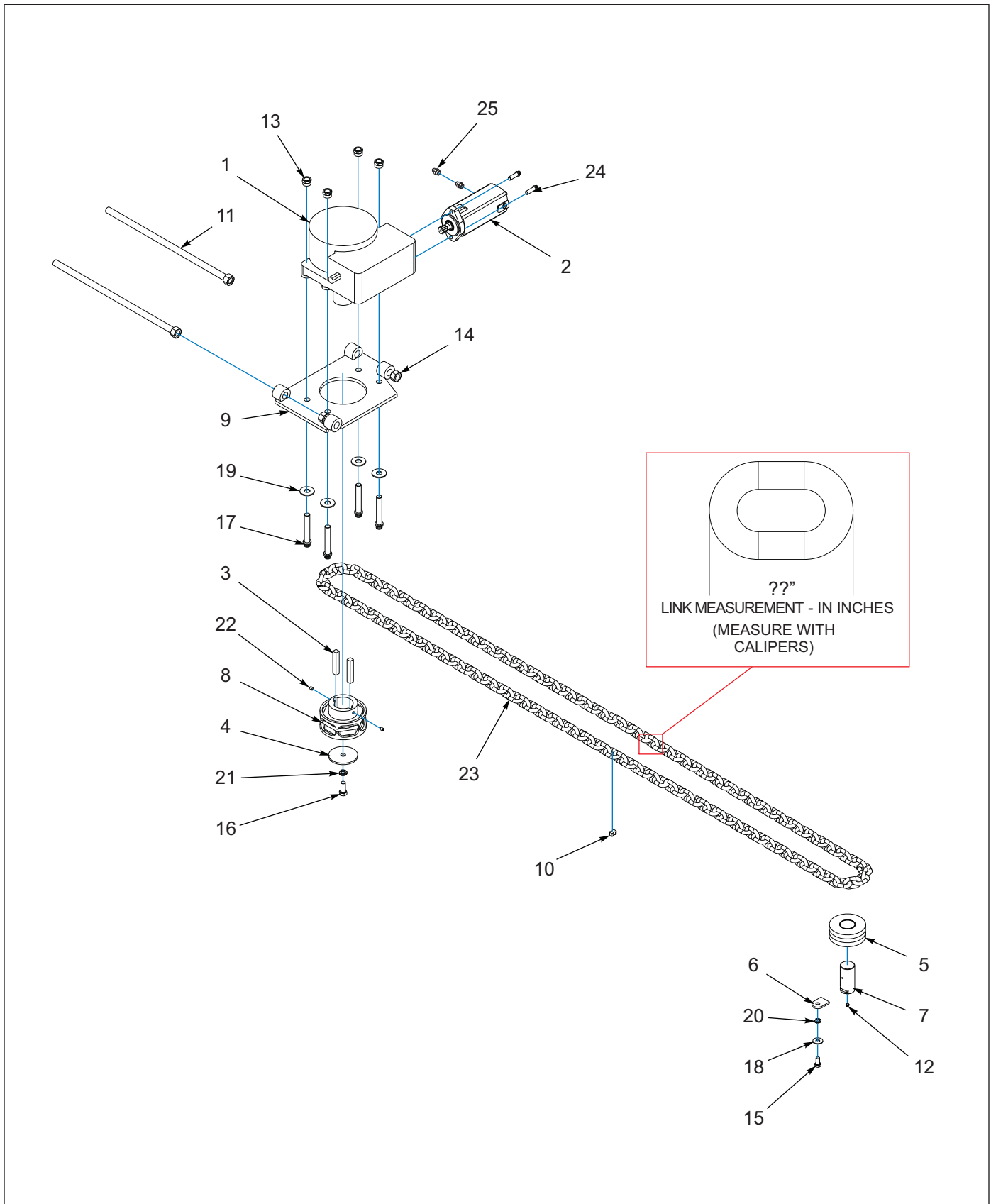
Figure 1-28: Gearbox Assembly
