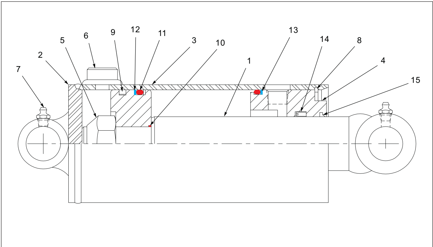
Figure 1-7: Hydraulic Cylinder - 4 x 20
