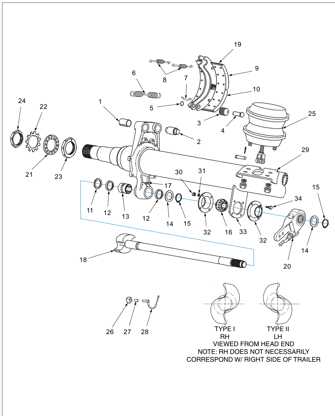
Figure 1-23: Axle and Brake Assembly - Dexter (12-1/4" X 7-1/2")
