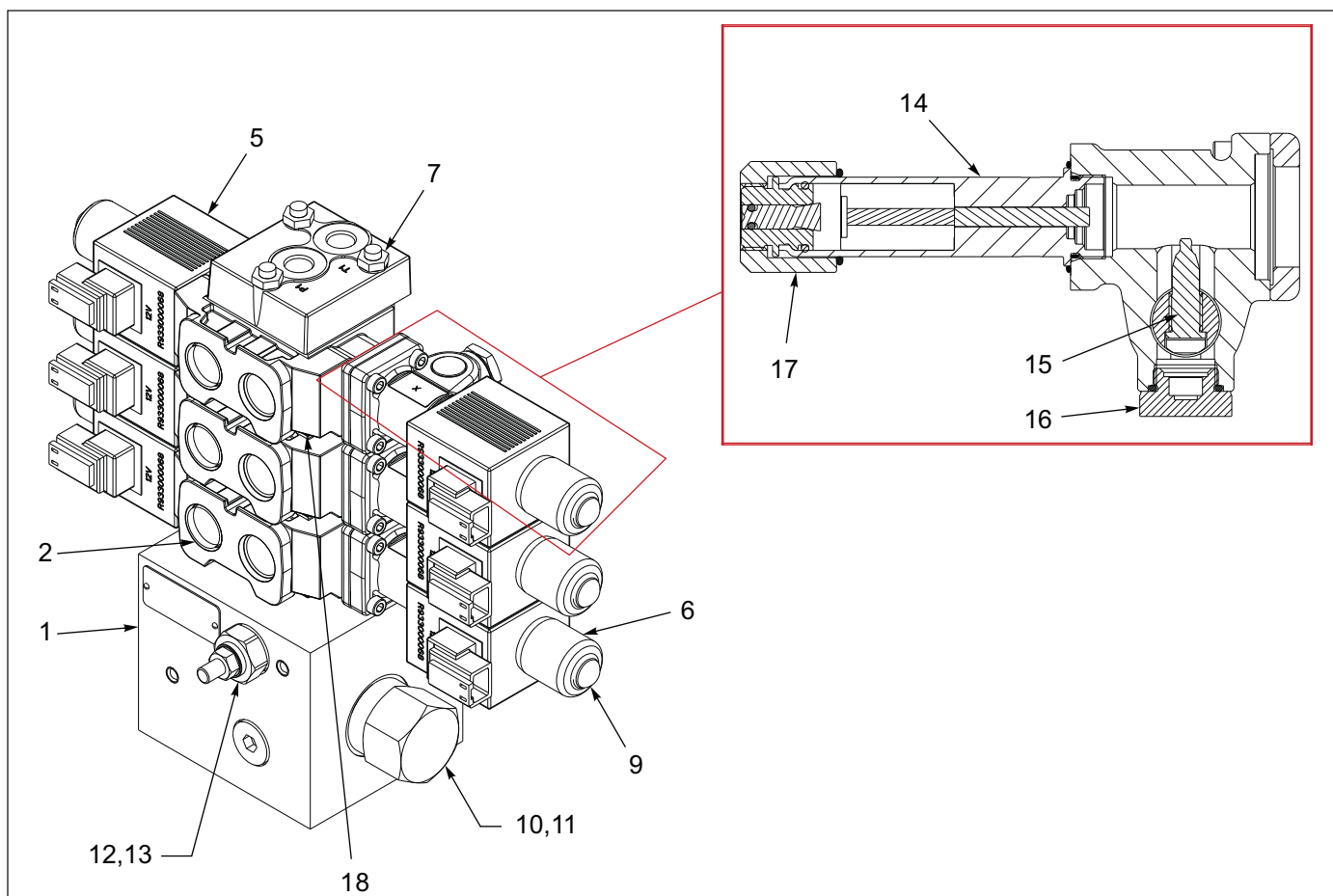
Figure 1-10: Three Spool Valve
