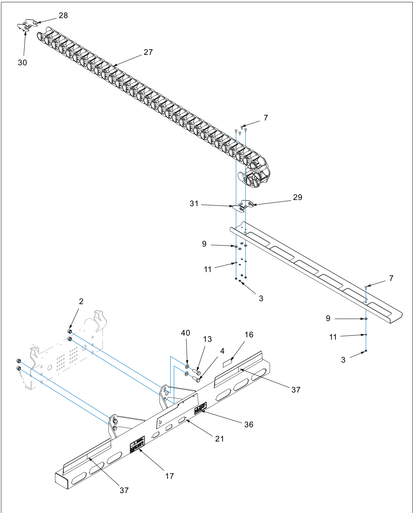
Figure 1-15: General Items (3 of 3)
