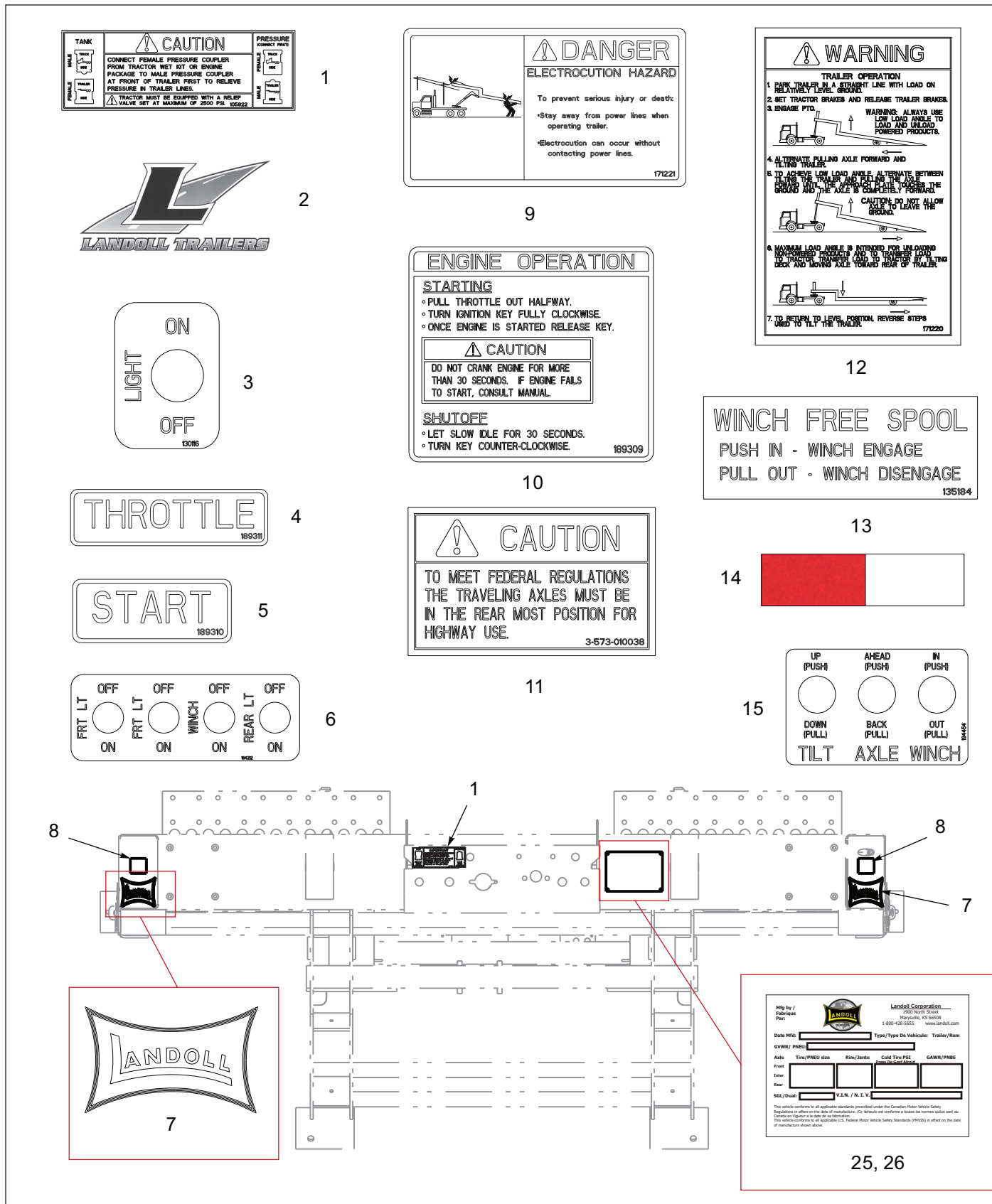
Figure 1-3: Decals (1 of 2)
