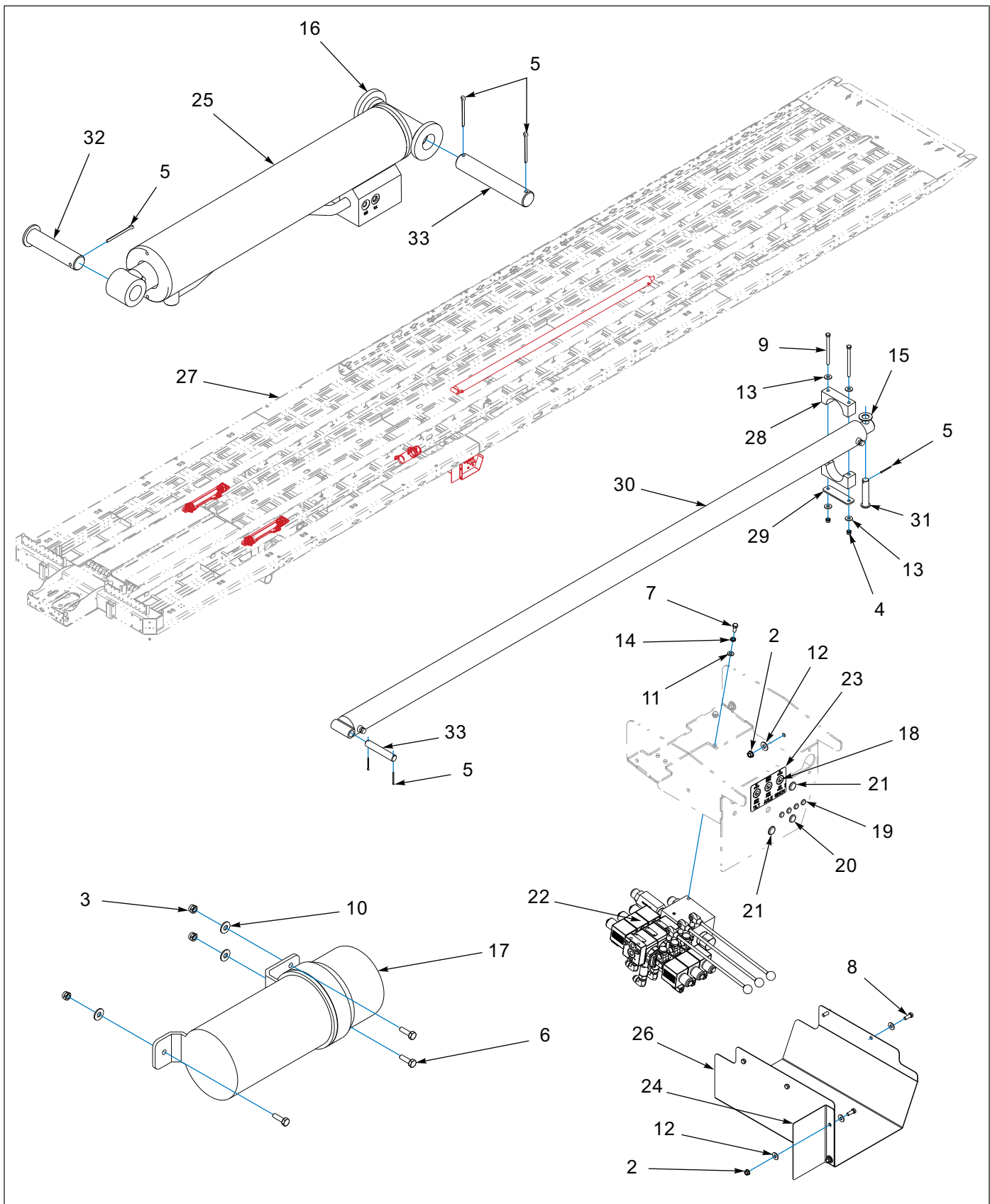
Figure 1-5: Hydraulic Electric Air - General Assembly
