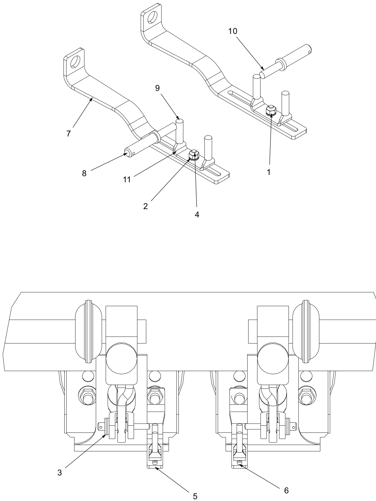
Figure 1-25: Brake Indicator - Long Brakesafe
