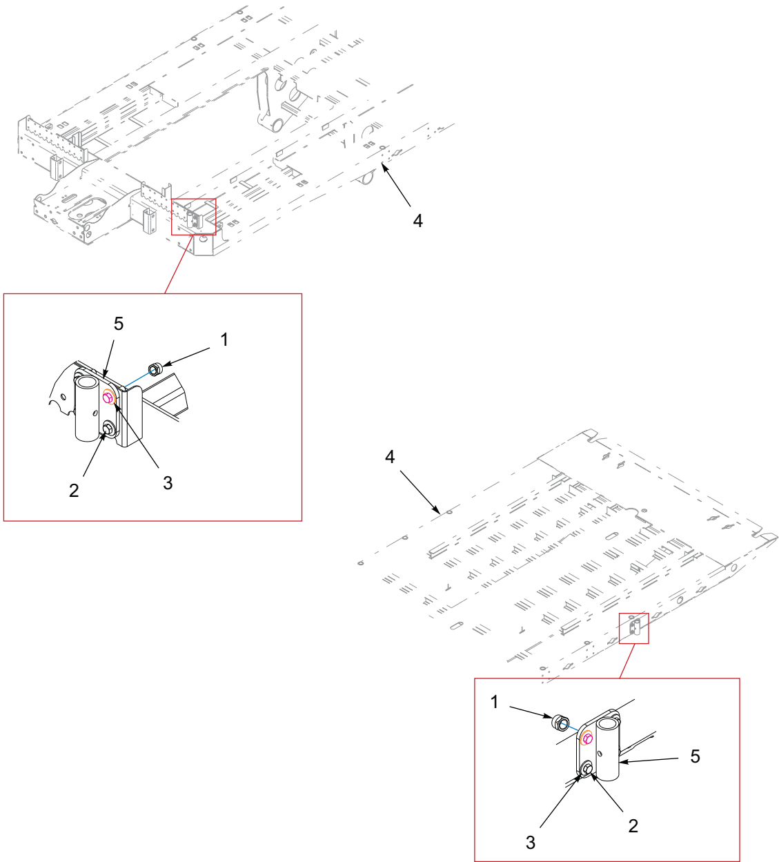
Figure 1-60: Side Guide - Anchor Pair
