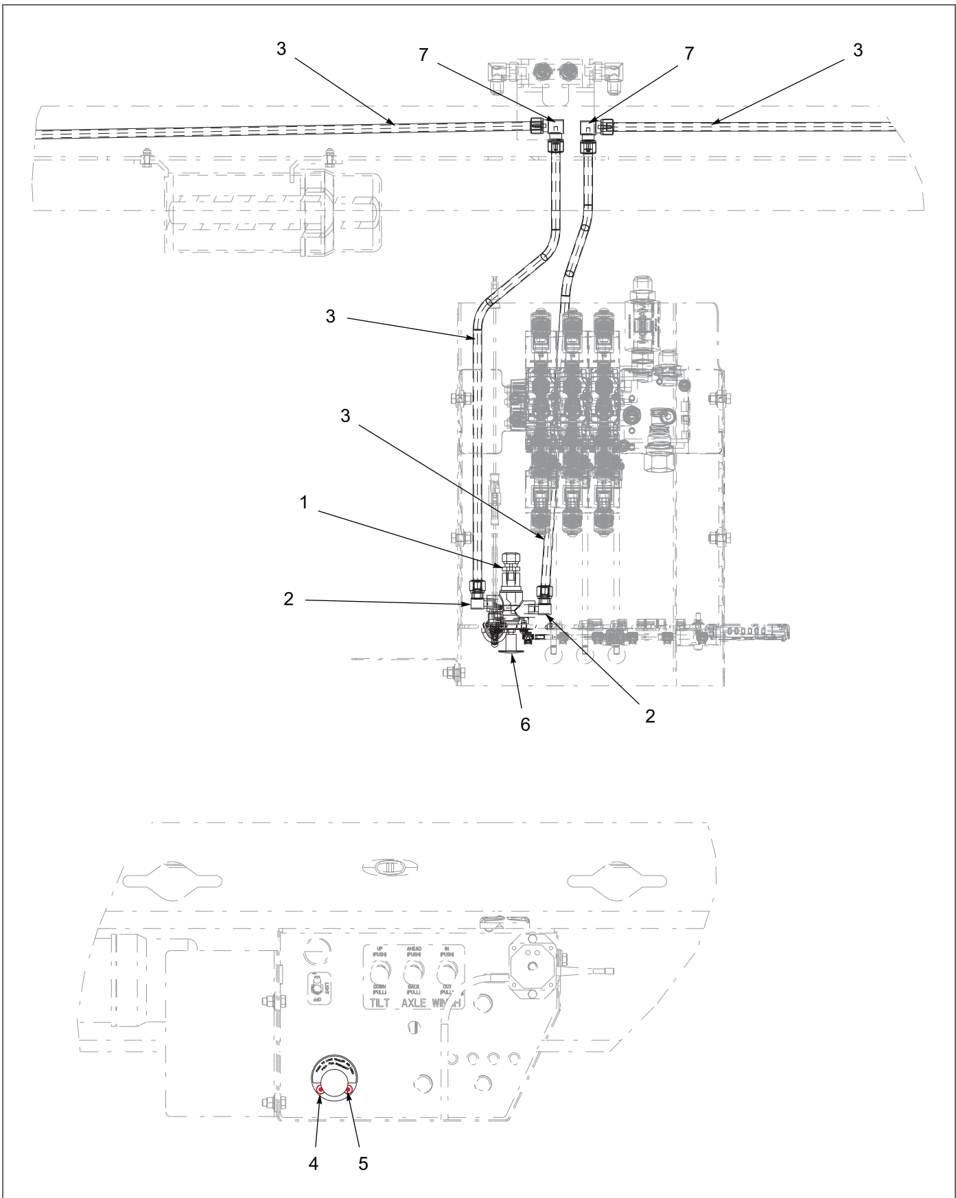
Figure 1-67: Brake Lock - 343A
