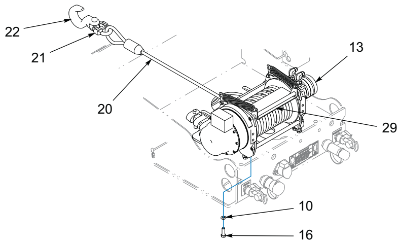
GENERAL ASSEMBLY
