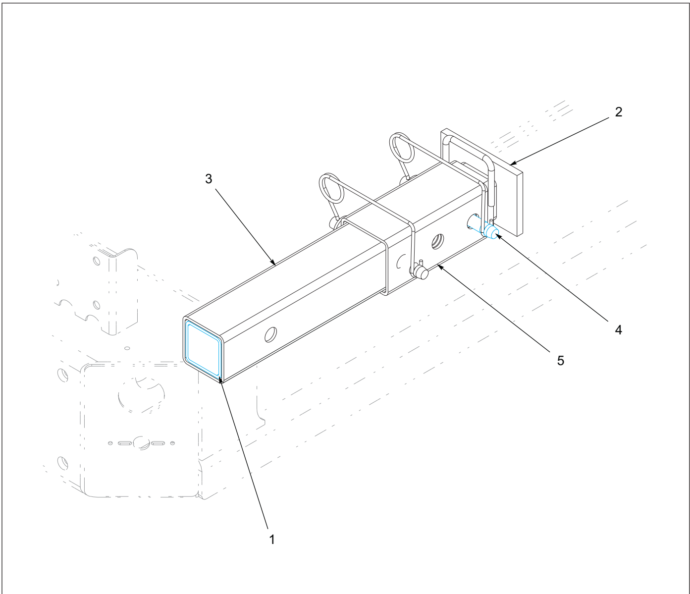
Figure 1-30: Adjustable Stop Assembly
