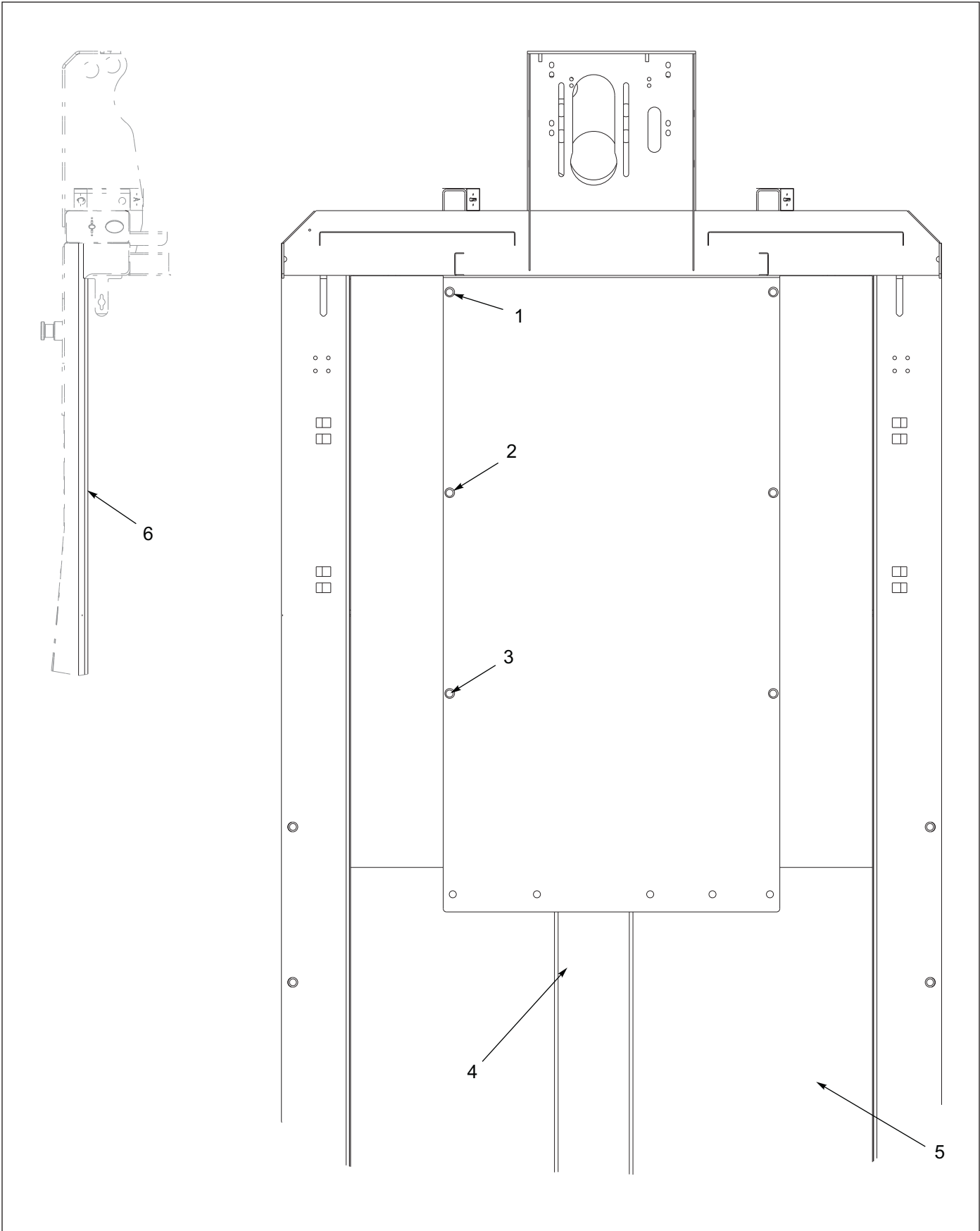
Figure 1-82: Hitch Cover
