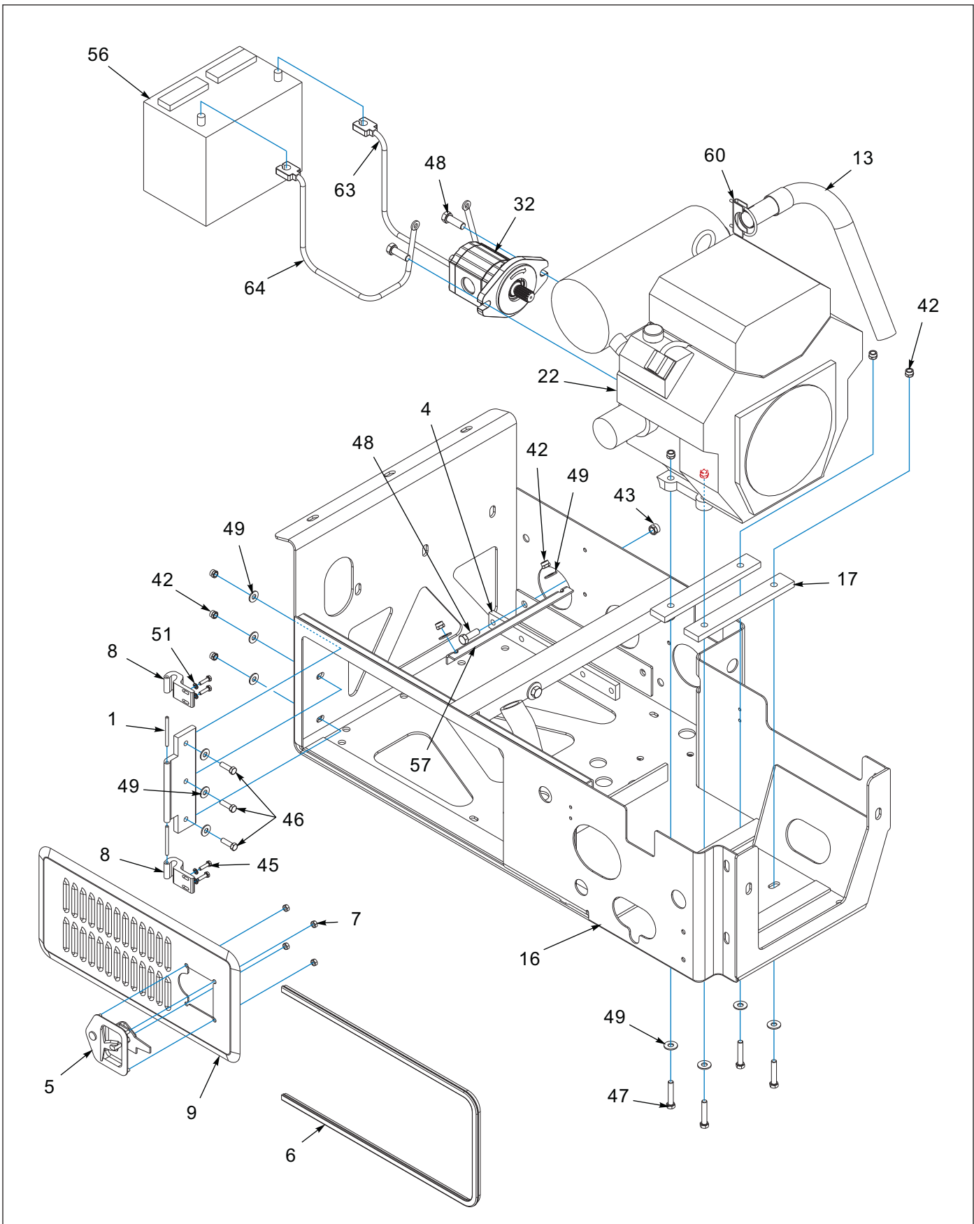
Figure 1-69: Engine - 25 HP Gas Package (1 of 2)
