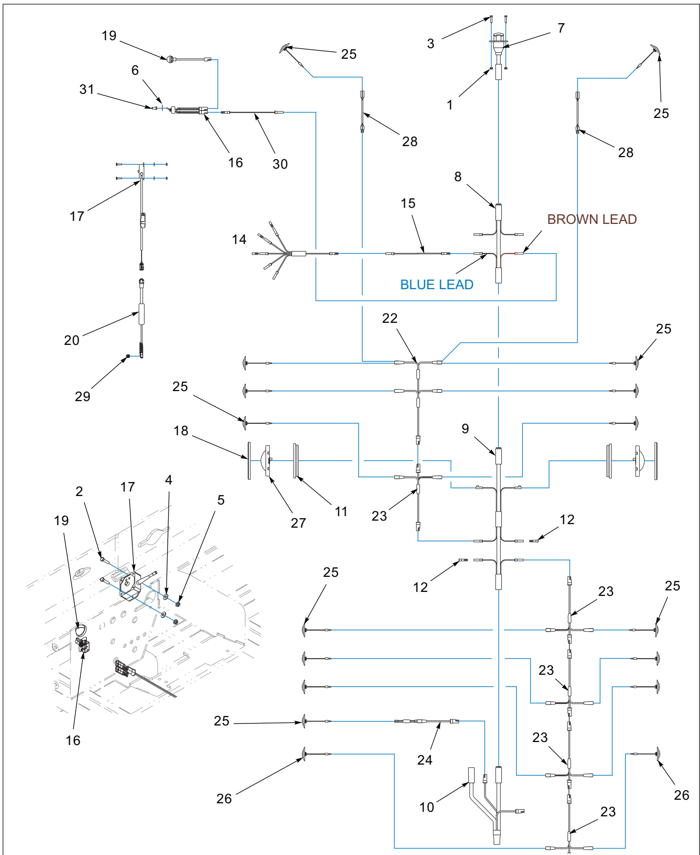
Figure 1-10: Electrical System (Before 08/01/2019)
