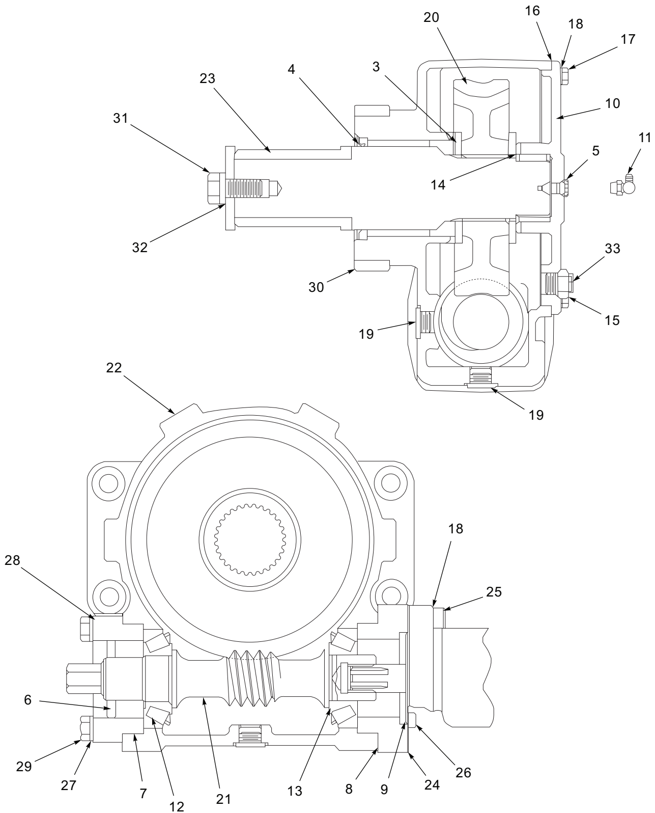
Figure 1-44: Gearbox Items
