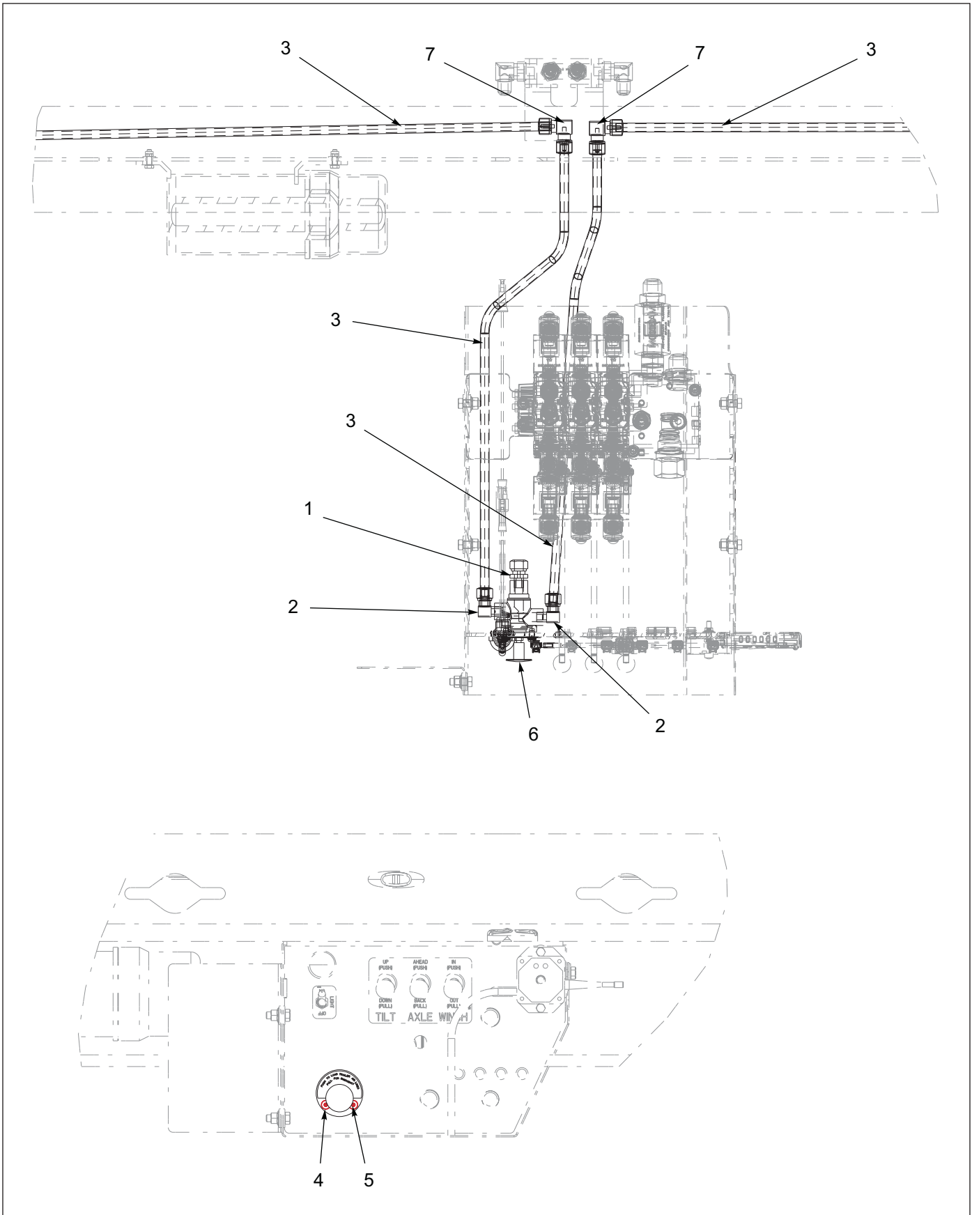
Figure 1-83: Brake Lock - 343A
