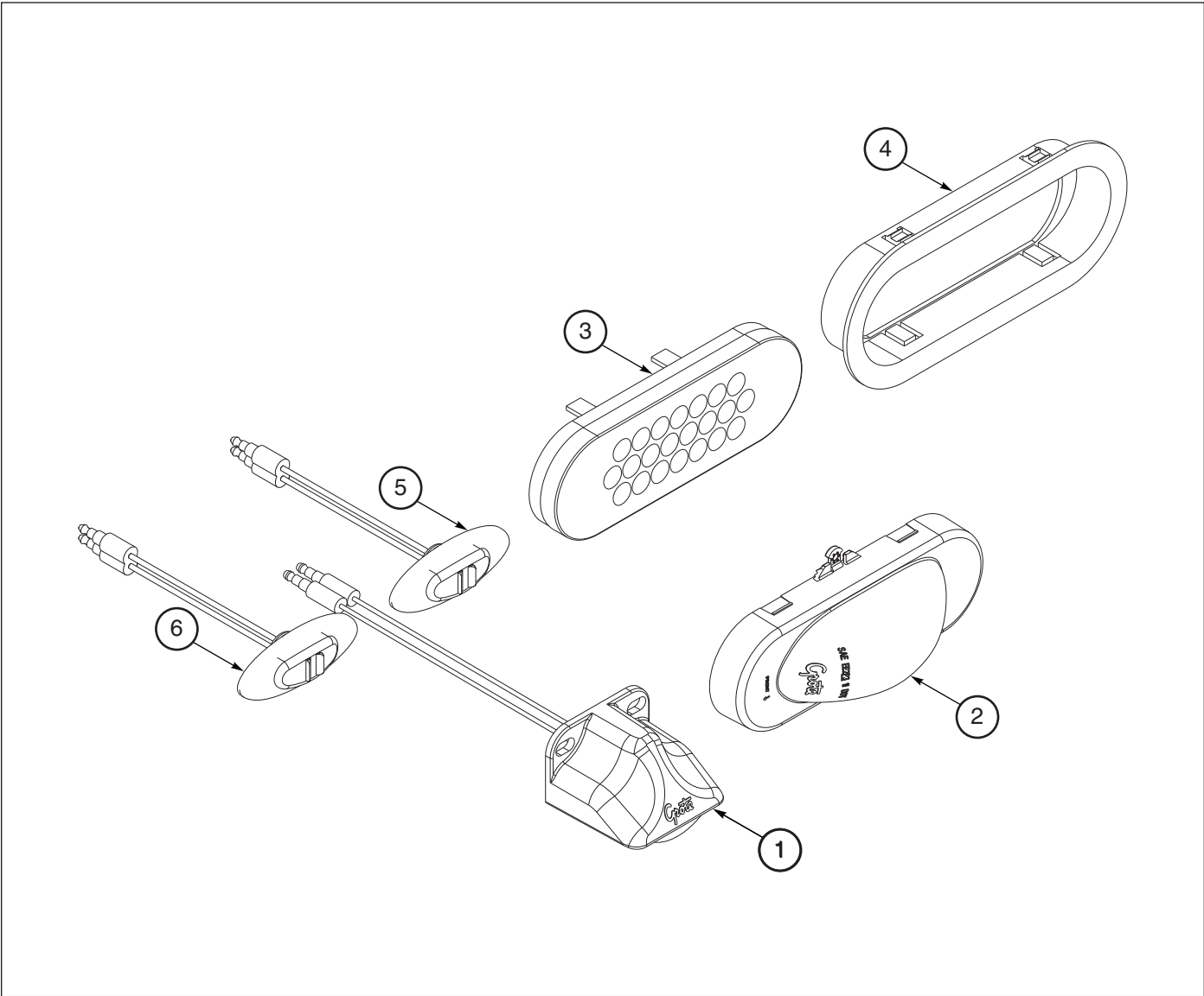
Figure 1-75: Spare Light Kit 343A LED-196586
