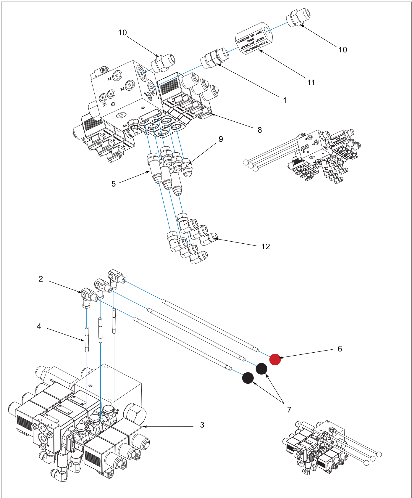
Figure 1-8: Valve Assembly - Three Spool
