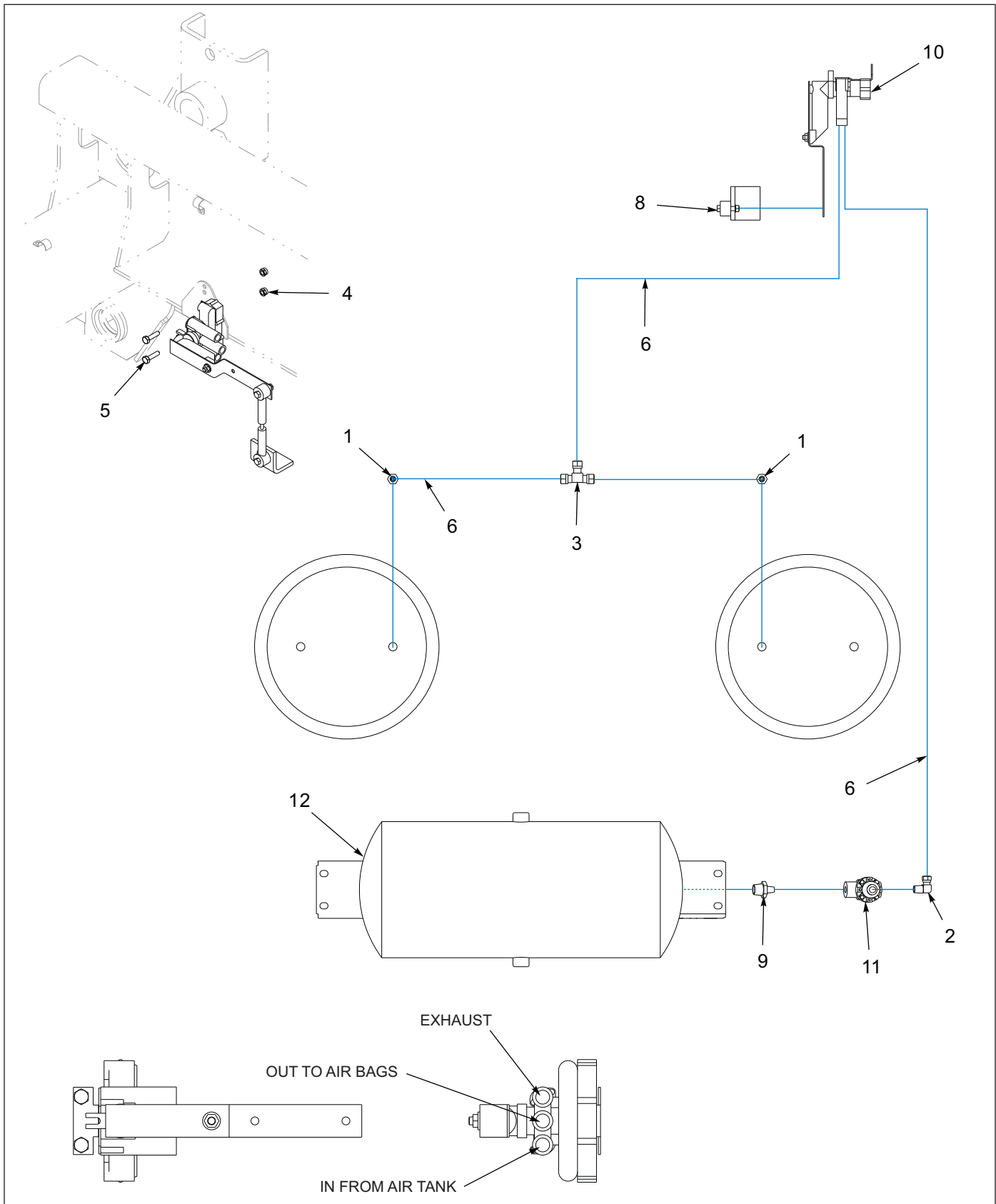
Figure 1-21: Air Ride Suspension
