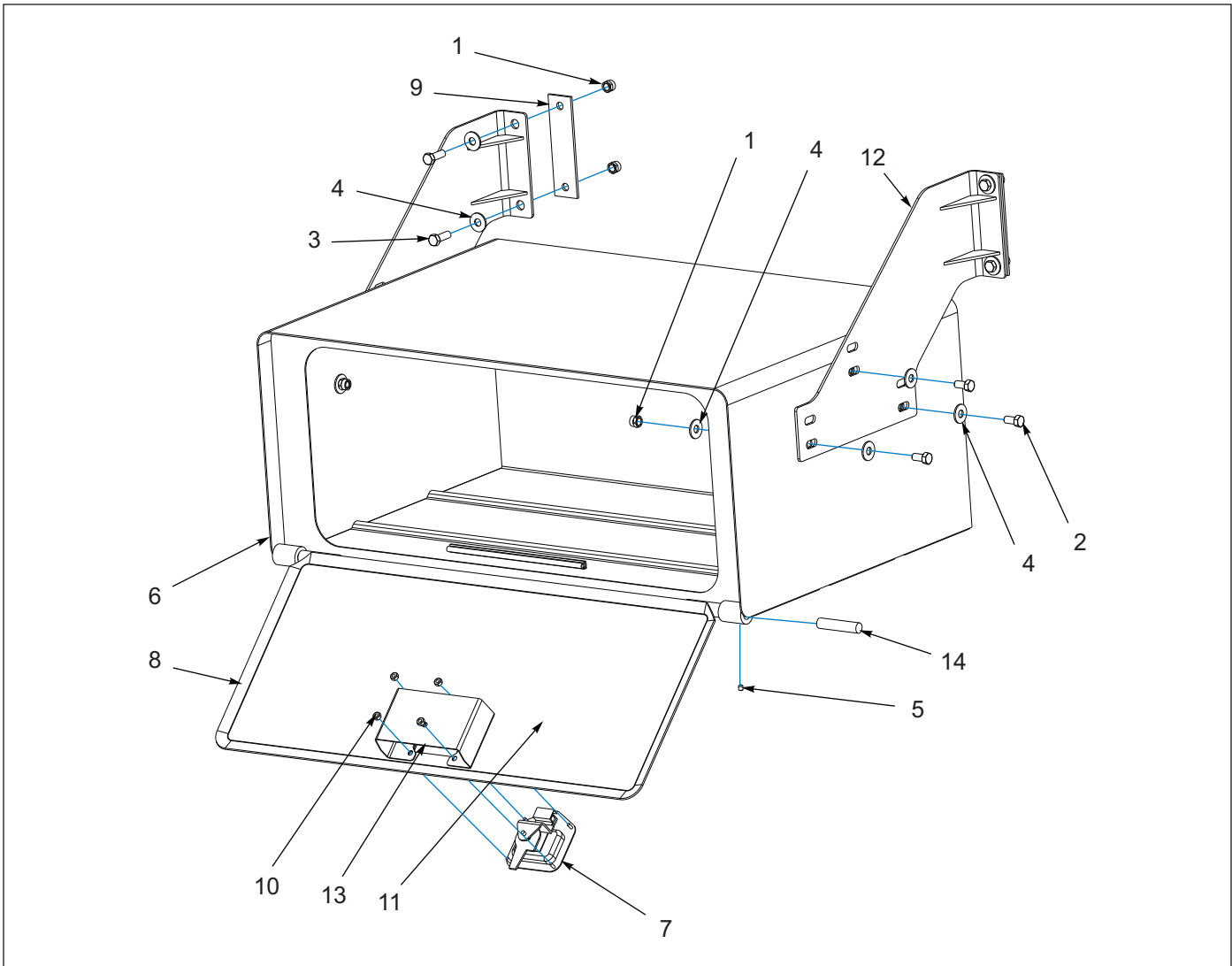
Figure 1-81: Tool Box Installation
