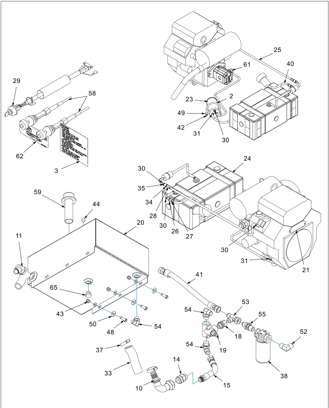
Figure 1-70: Engine - 25 HP Gas Package (2 of 2)
