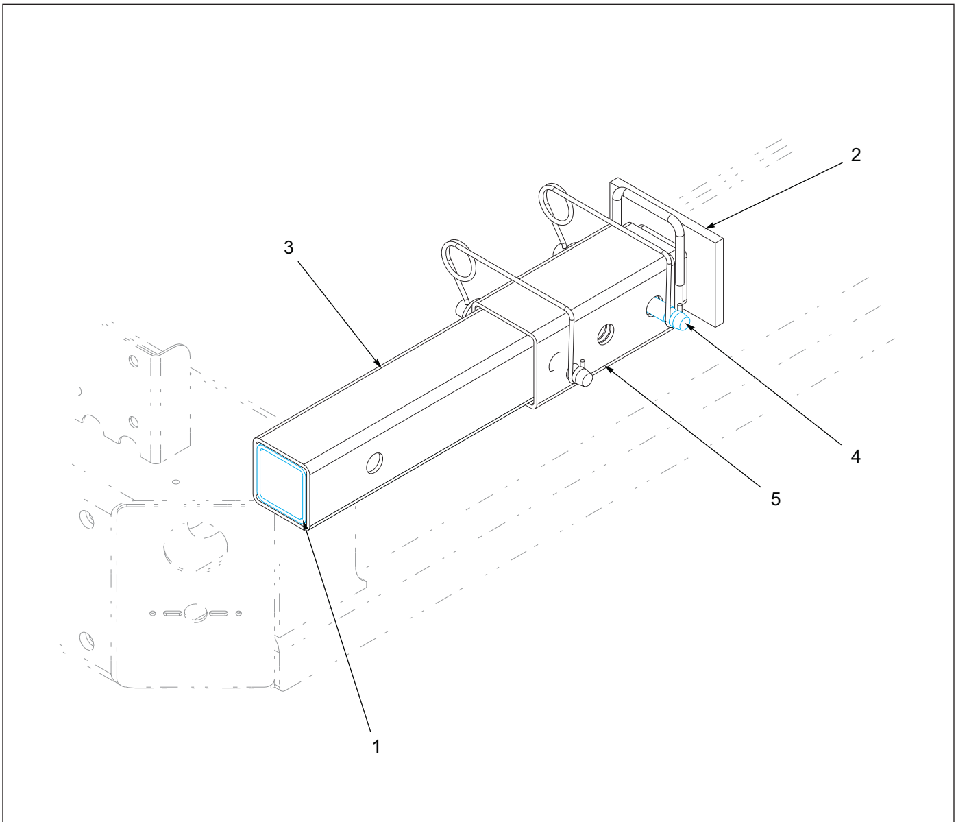
Figure 1-45: Adjustable Stop Assembly
