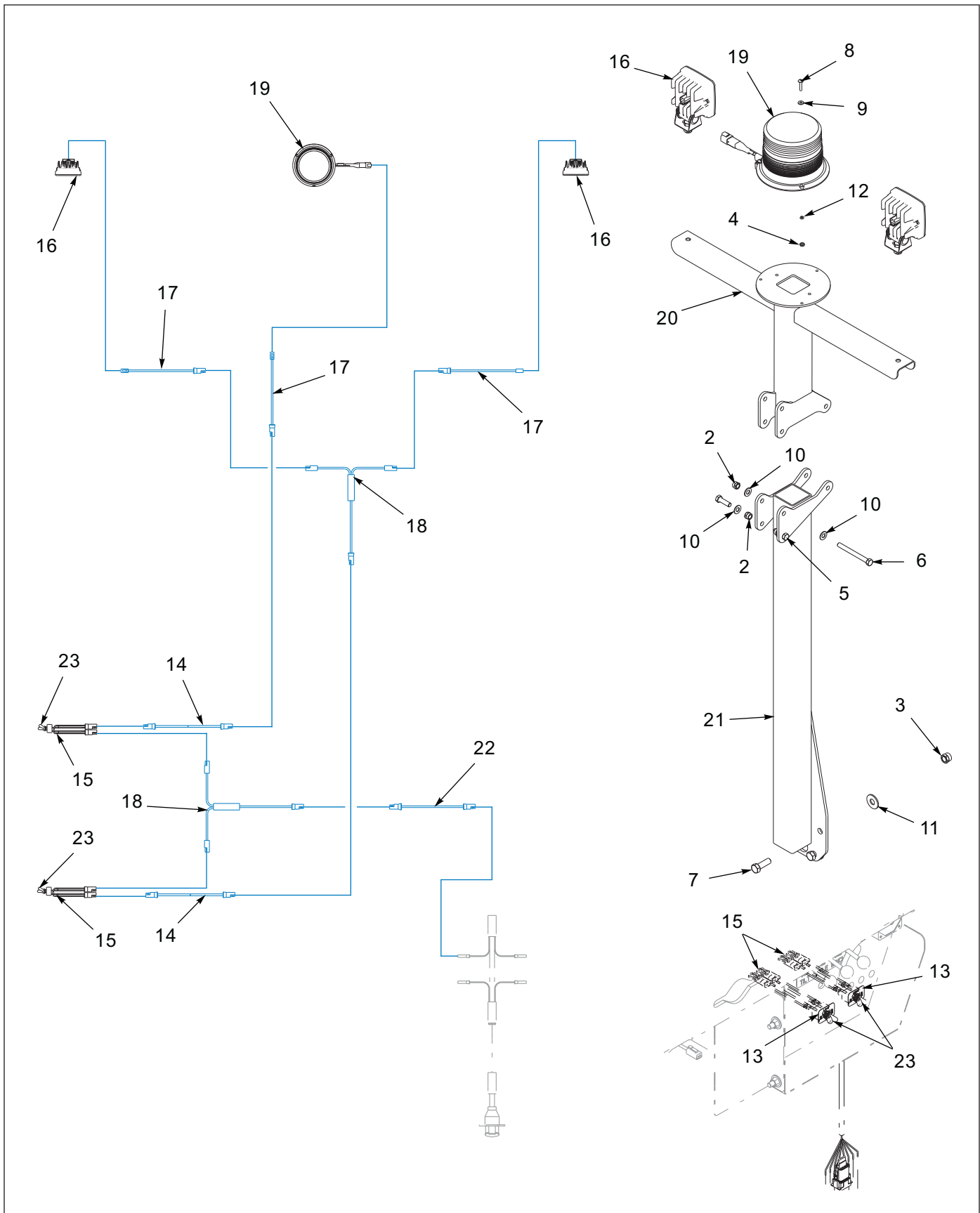
Figure 1-74: Strobe Beacon and Work Light Installation
