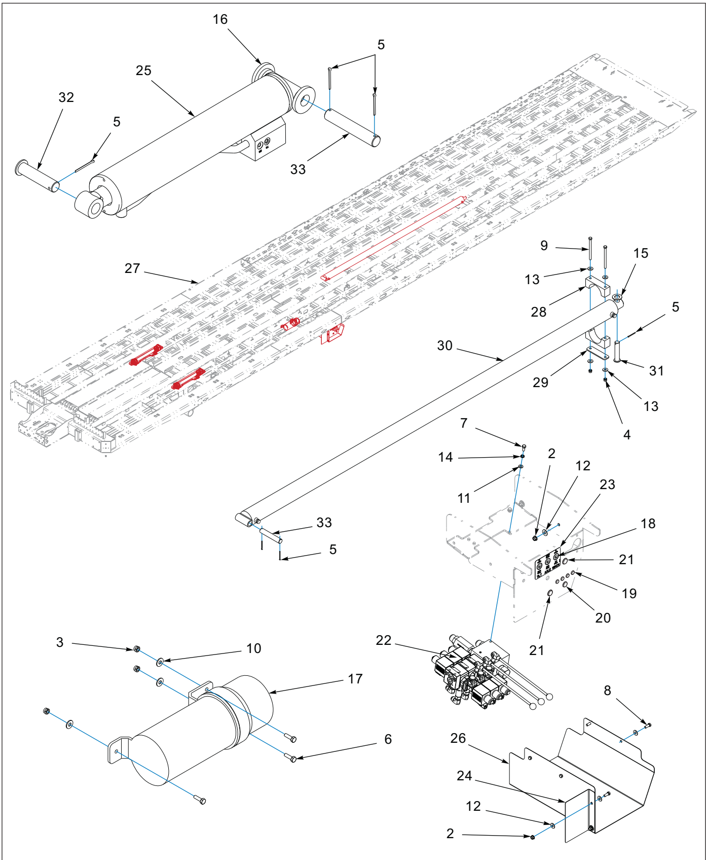
Figure 1-4: General Assembly
