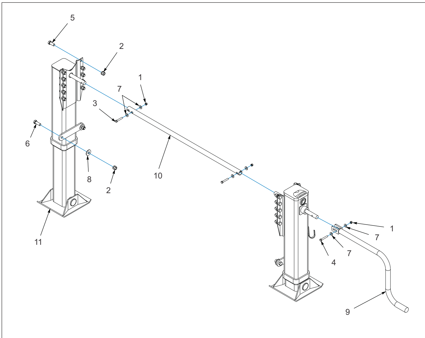
Figure 1-62: Landing Gear Installation - Jost 343
