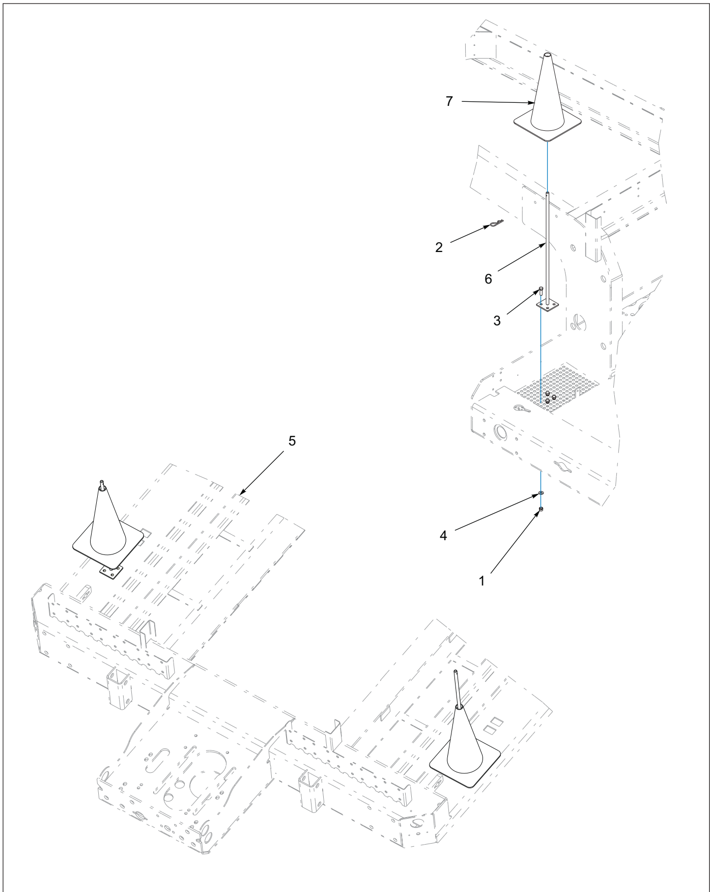
Figure 1-84: Cone Holder Assembly
