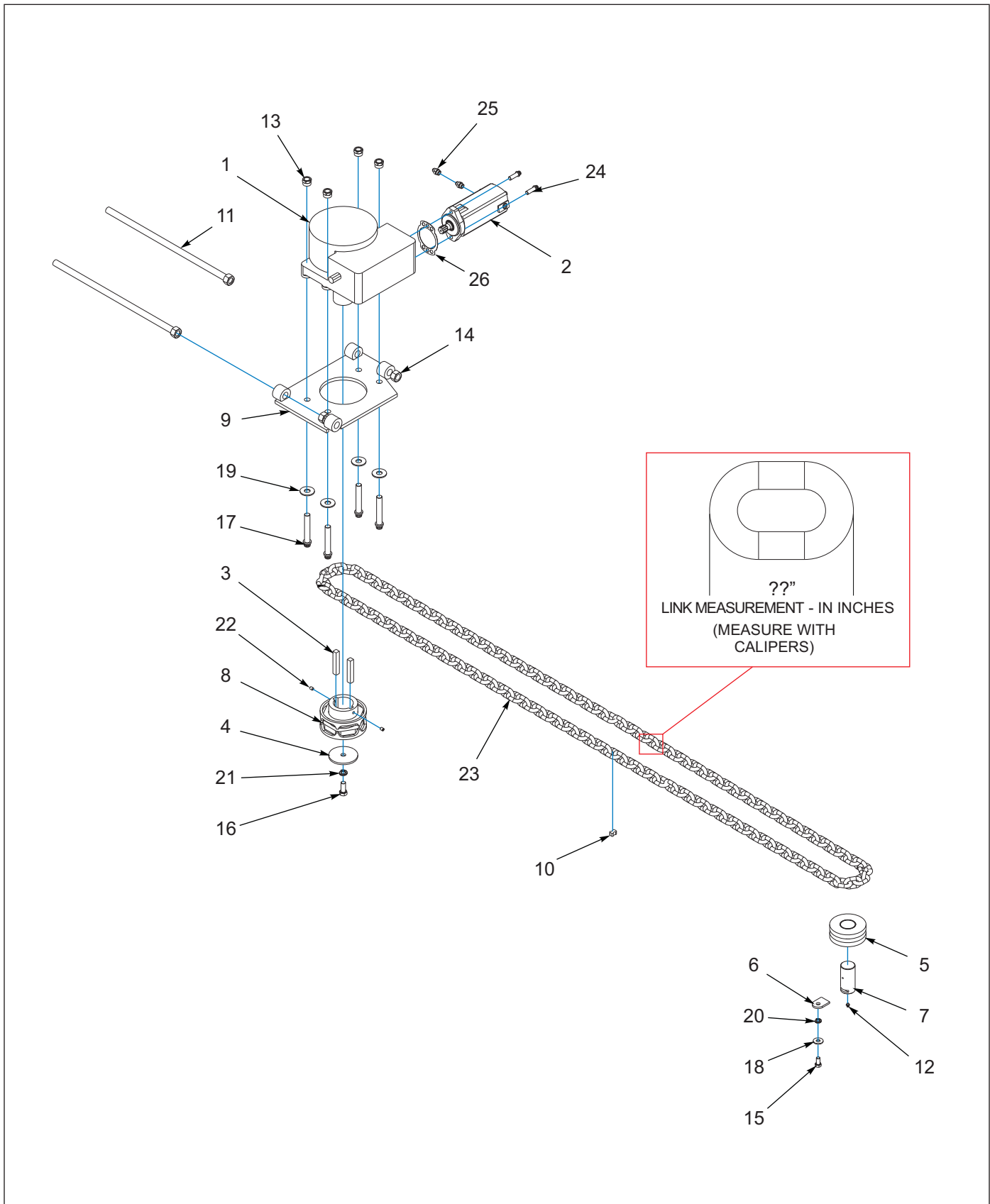
Figure 1-43: Gearbox Assembly
