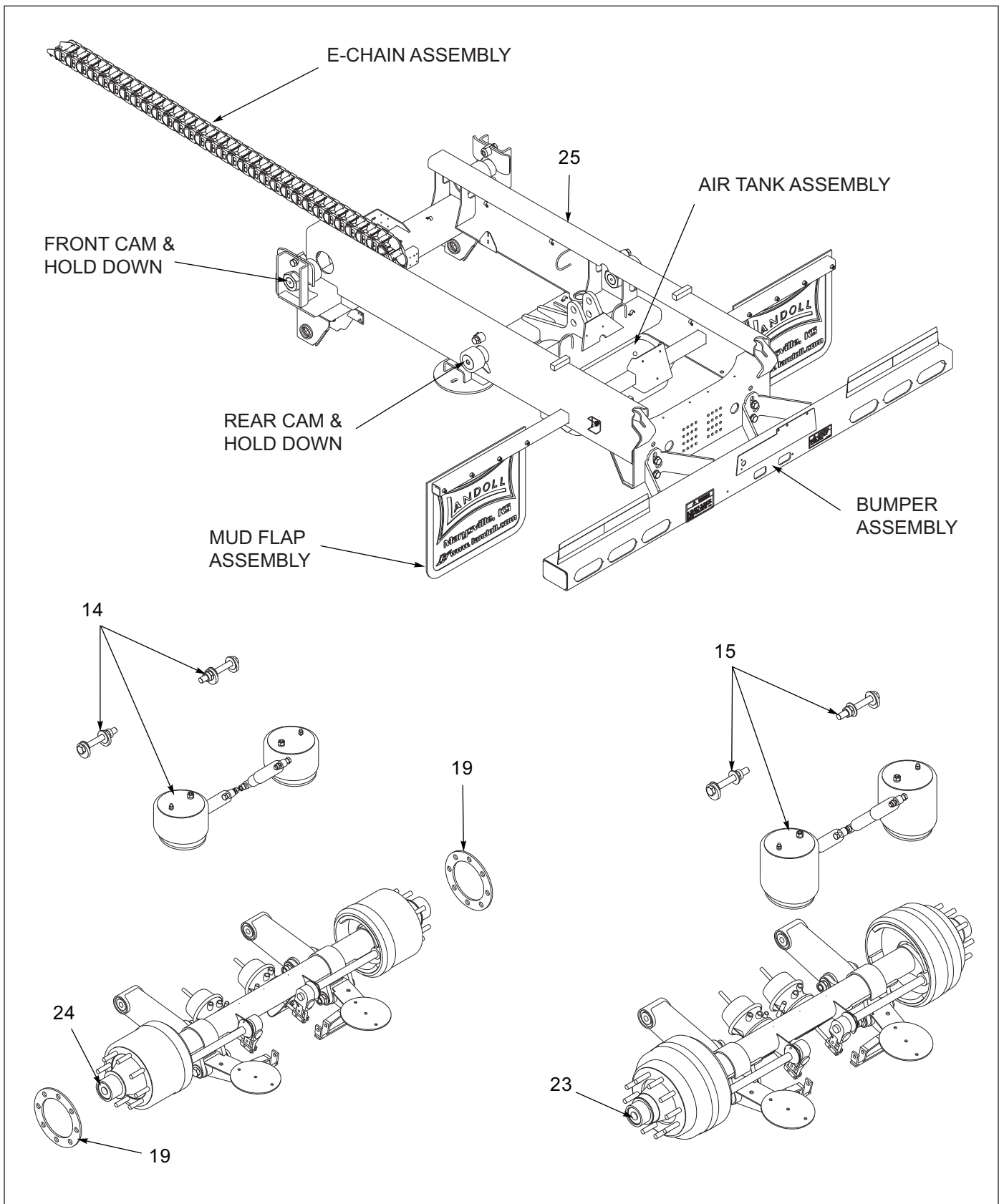
Figure 1-16: General Items (1 of 3)
