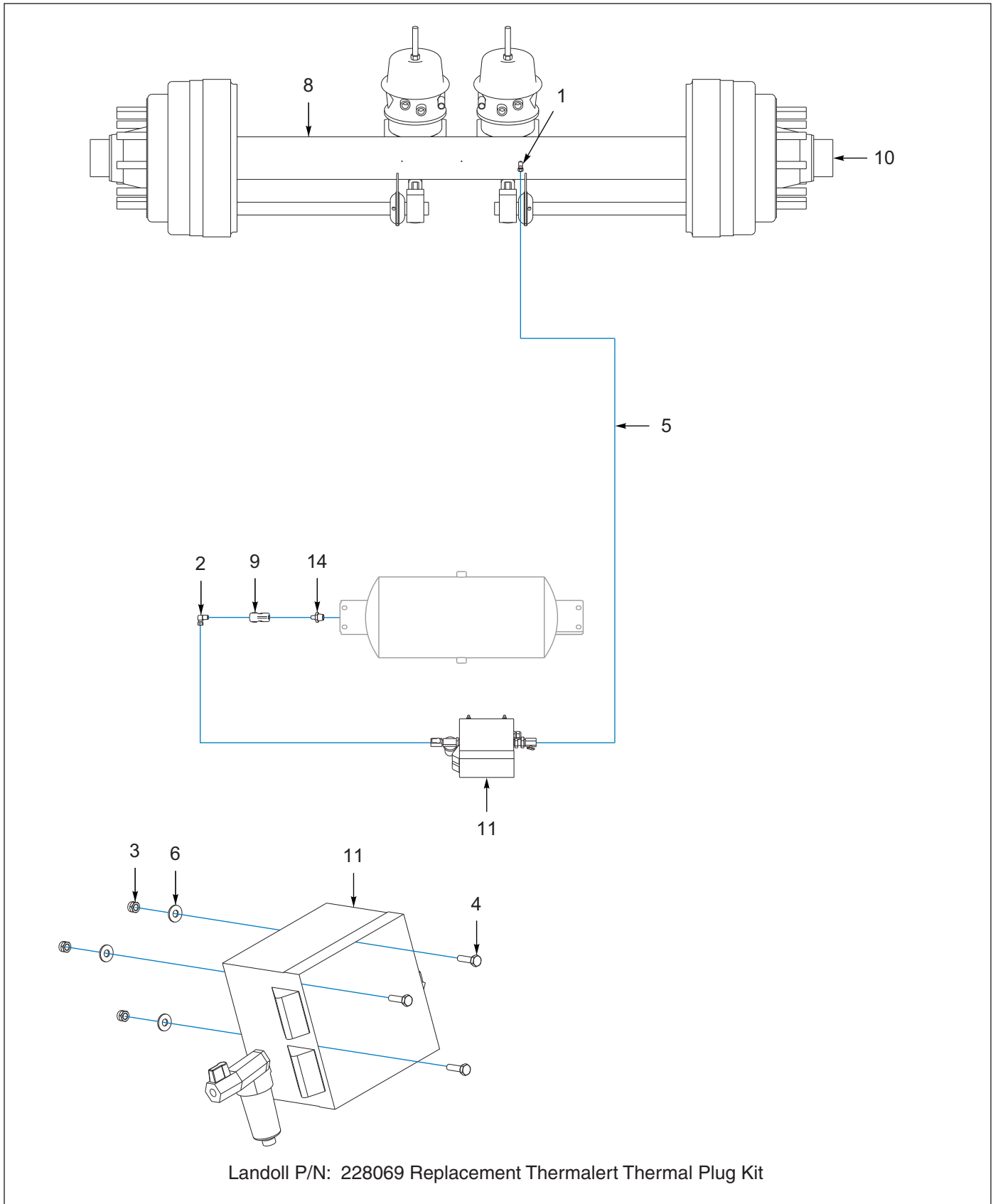
Figure 1-40: Thermalert, 1 Axle Air System (OPTION)
