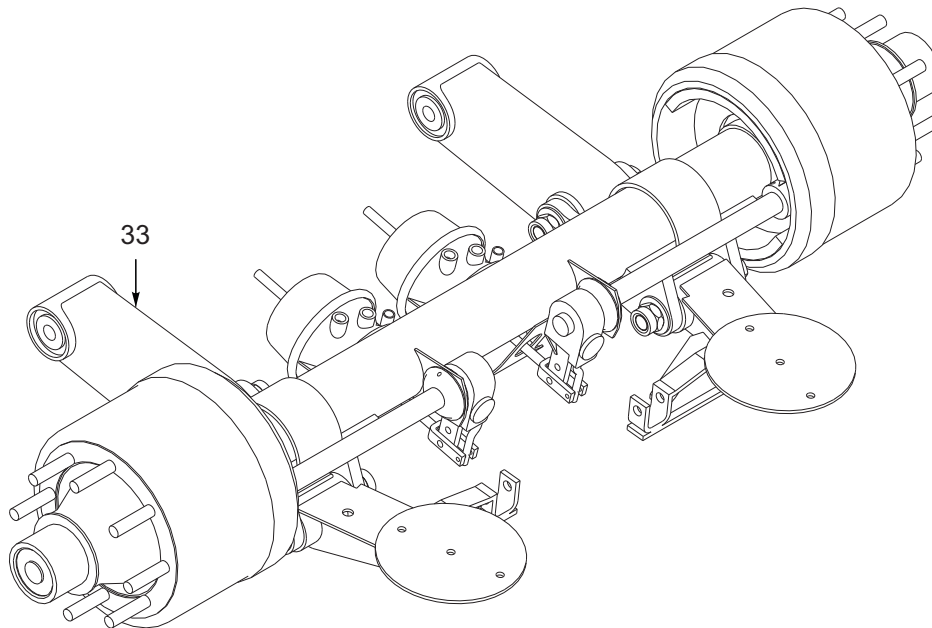
VIEW OF RLU-228-3.5, 12.25 X 7.5 DRUM BRAKES
