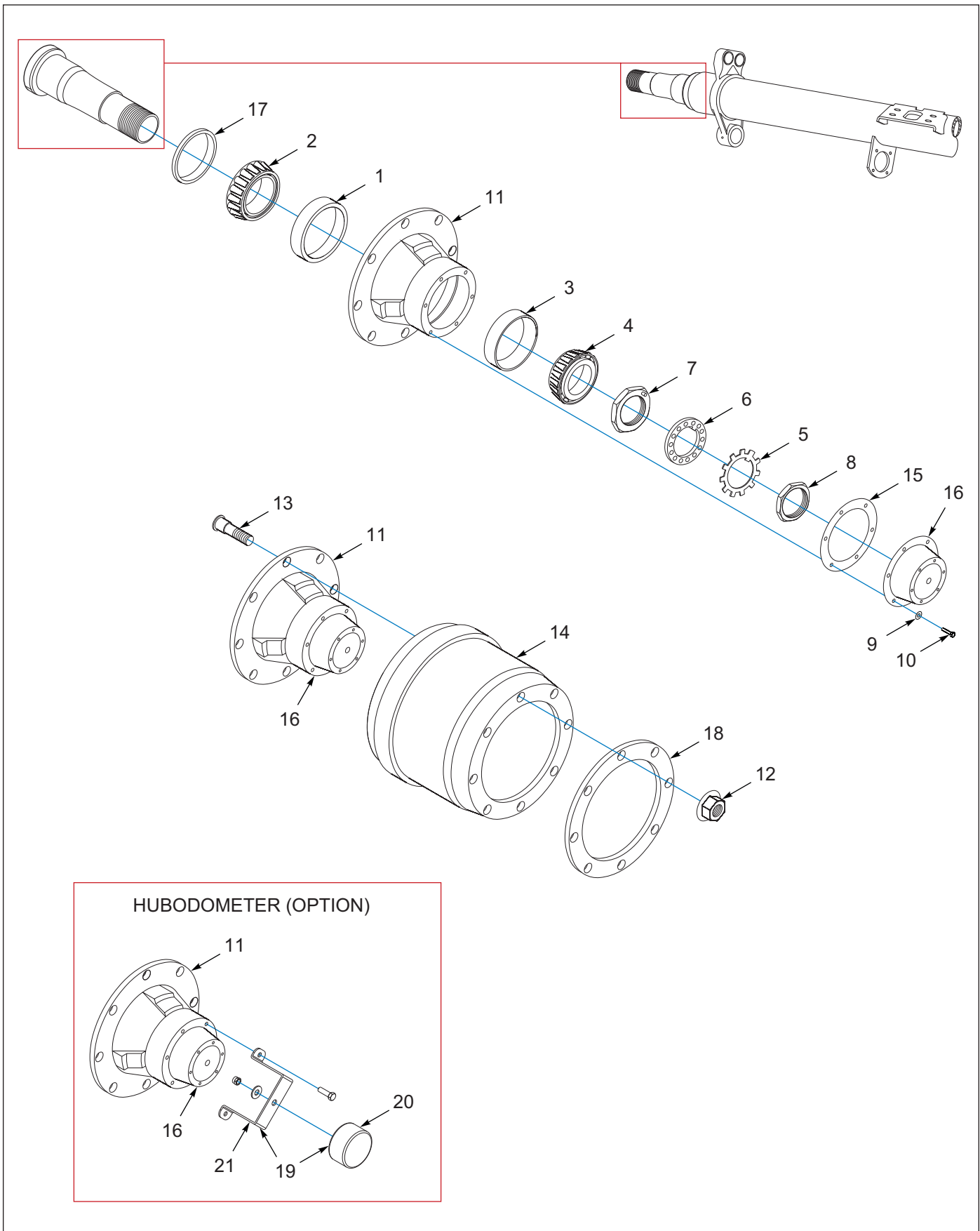
Figure 1-33: Axle 12.25 x 7.5 Drum and Hub Assembly
