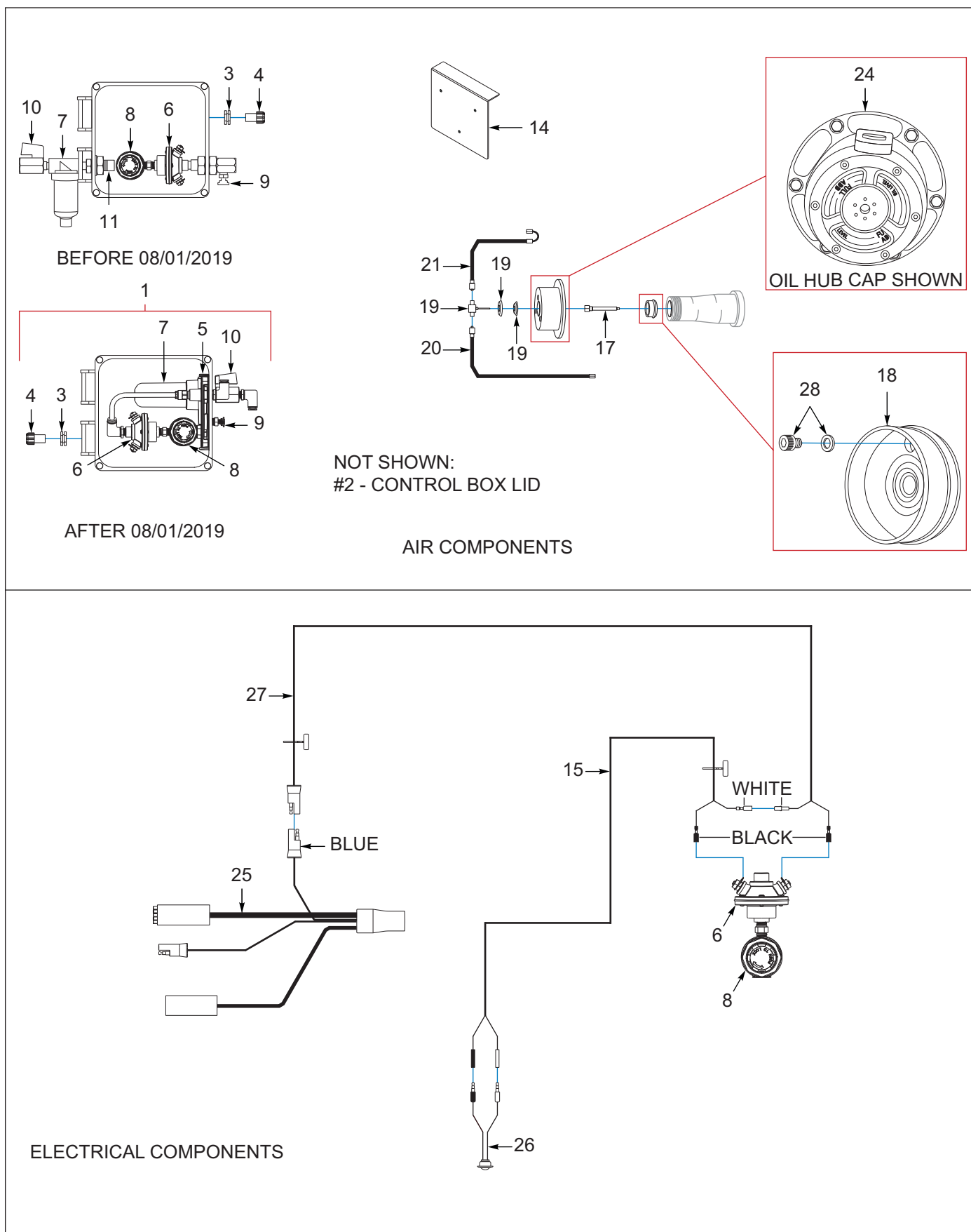
Figure 1-41: Thermalert Electrical System &amp; Components (OPTION)
