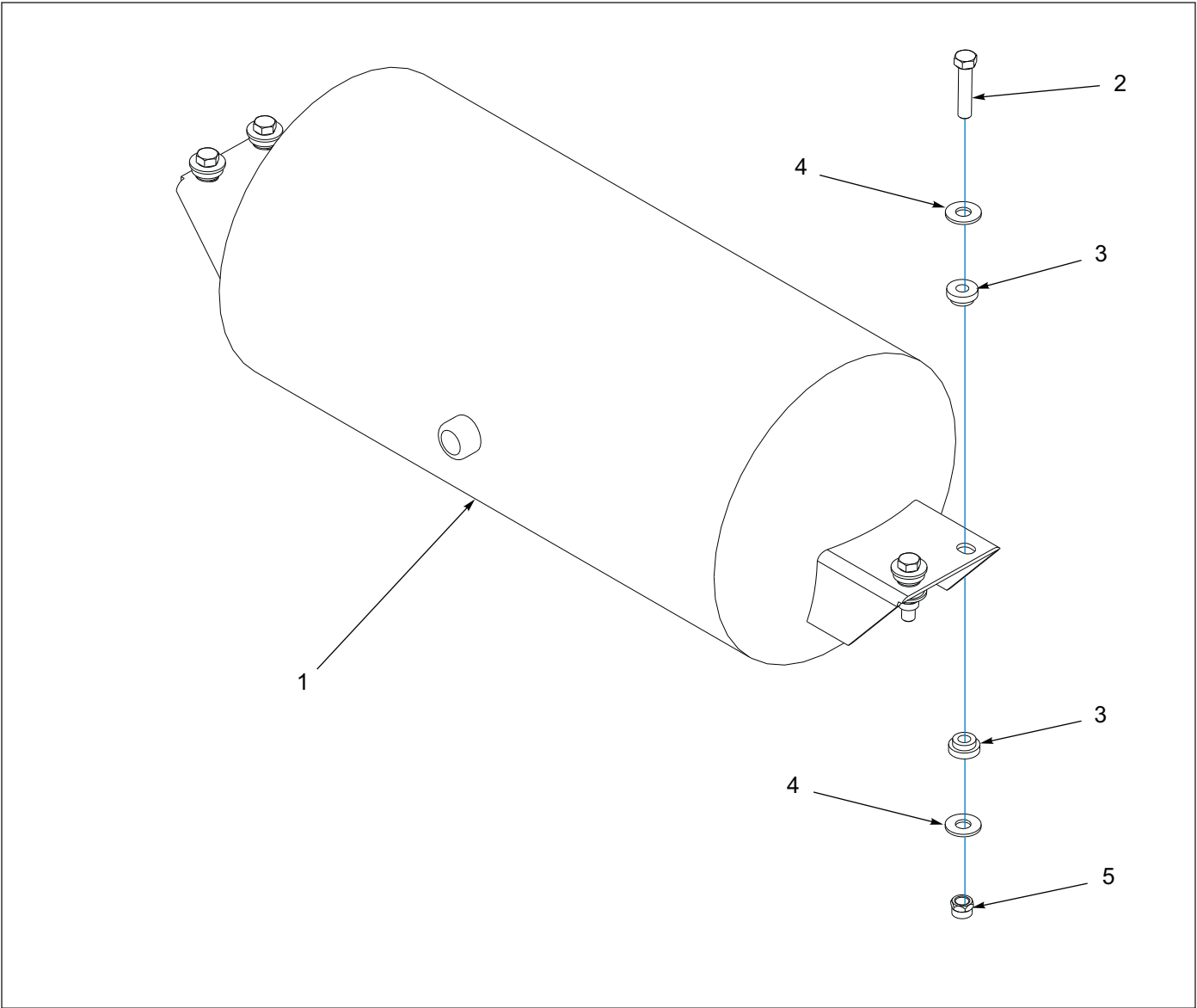
Figure 1-23: Air Tank Assembly
