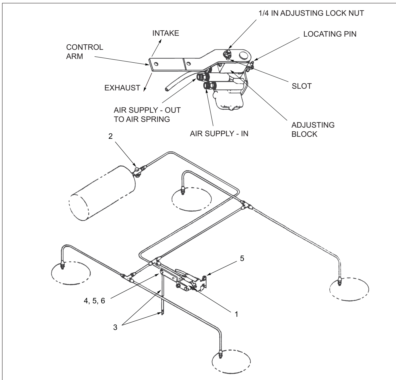
Figure 1-22: Air Control Kit
