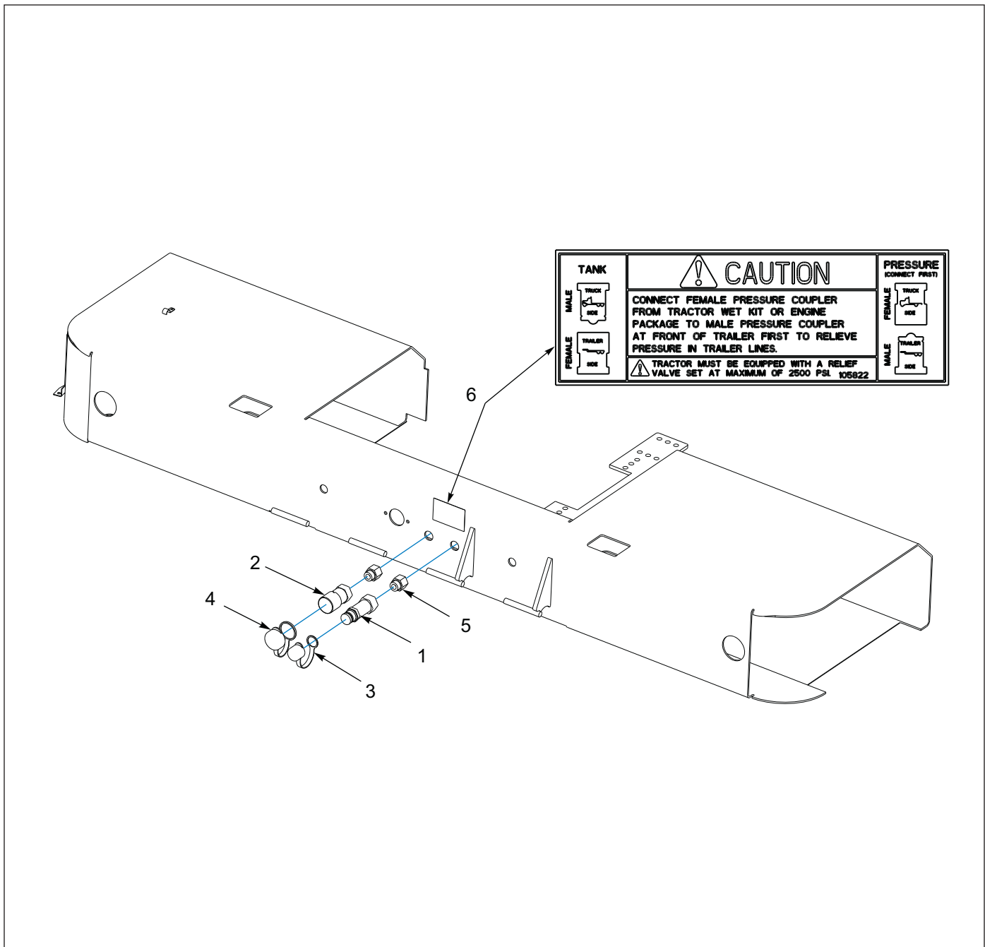
Figure 1-73: Hydraulic Conversion Kit - Ball to Flat
