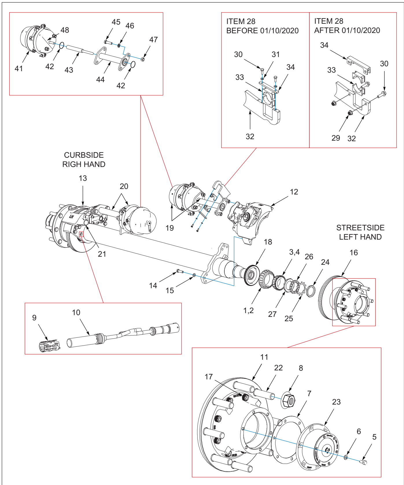
Figure 1-30: Axle 12.25 Disc Brakes & Hub Assembly, Dexter (OPTION) (1 of 2)
