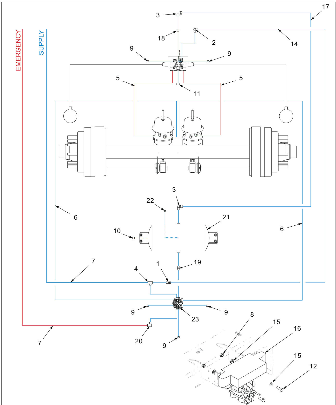
Figure 1-28: Air Brake System
