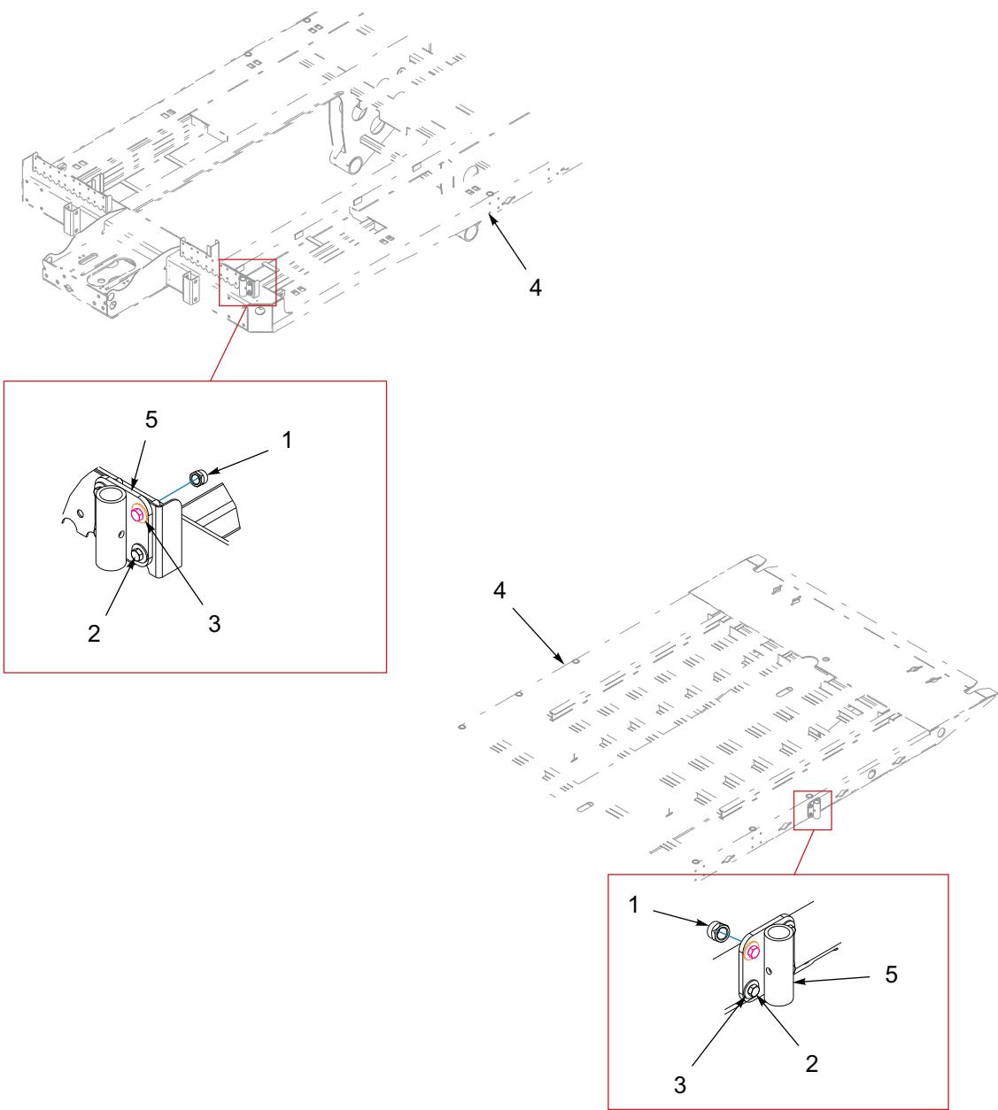
Figure 1-76: Side Guide - Anchor Pair
