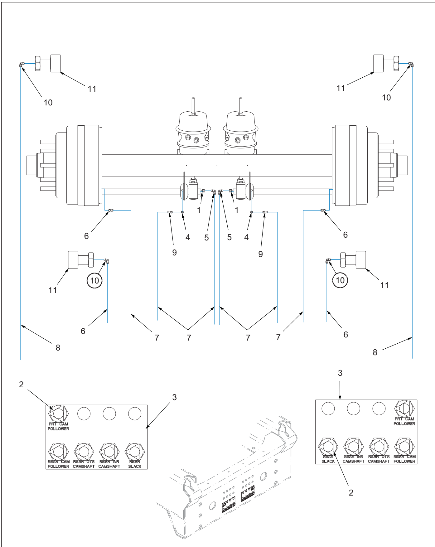
Figure 1-20: Grease System (After 11/07/2018)
