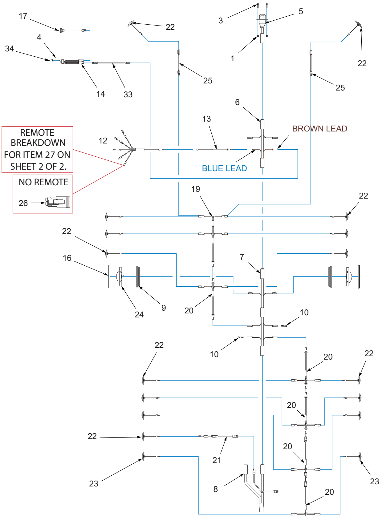
Figure 1-12: Electrical System (After 08/01/2019) (1 of 2)
