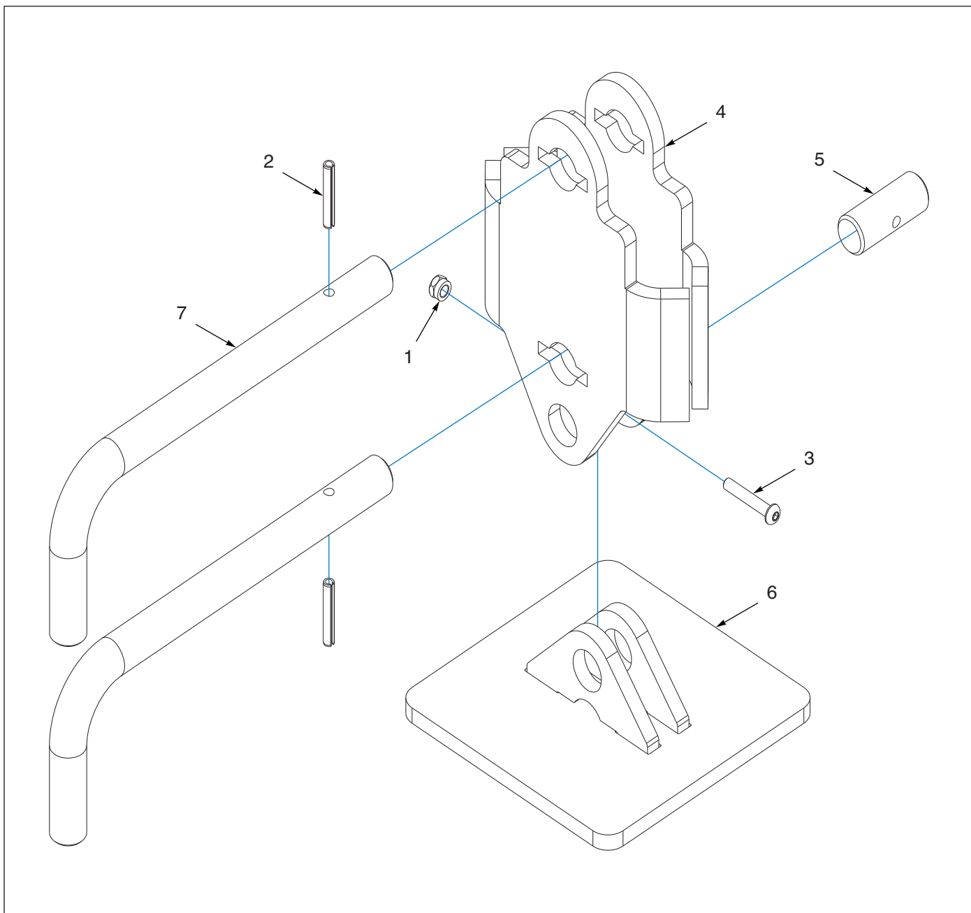
Figure 1-79: Shoe Lock Tiedown Assembly-128469
