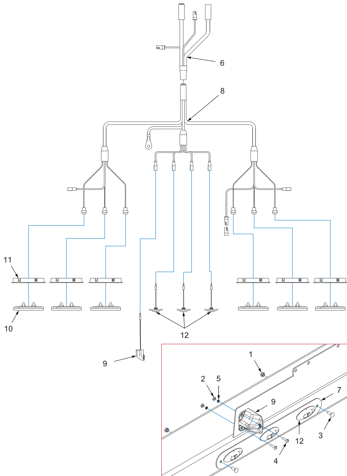
Figure 1-15: Bumper Electrical (After 01/02/2020)
