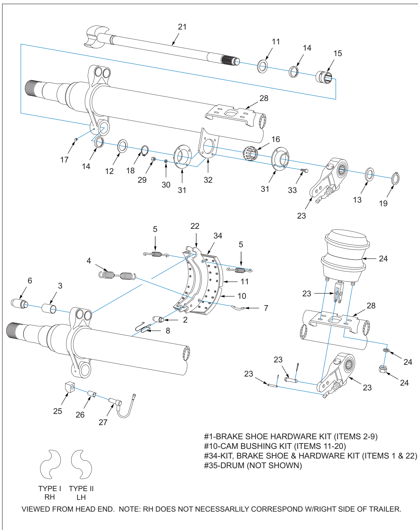
Figure 1-36: Axle 16.5 x 7 Drum Brakes, Dexter
