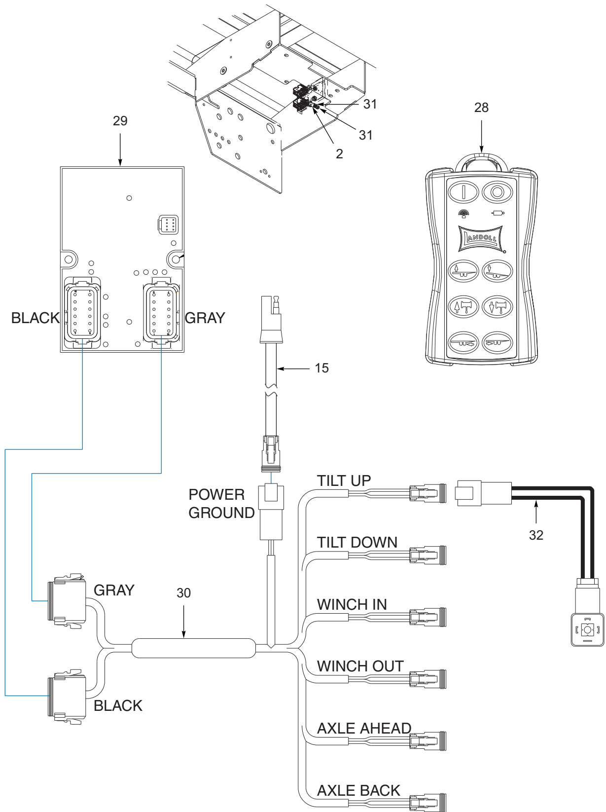
Figure 1-13: Electrical System (After 08/01/2019) (2 of 2)
