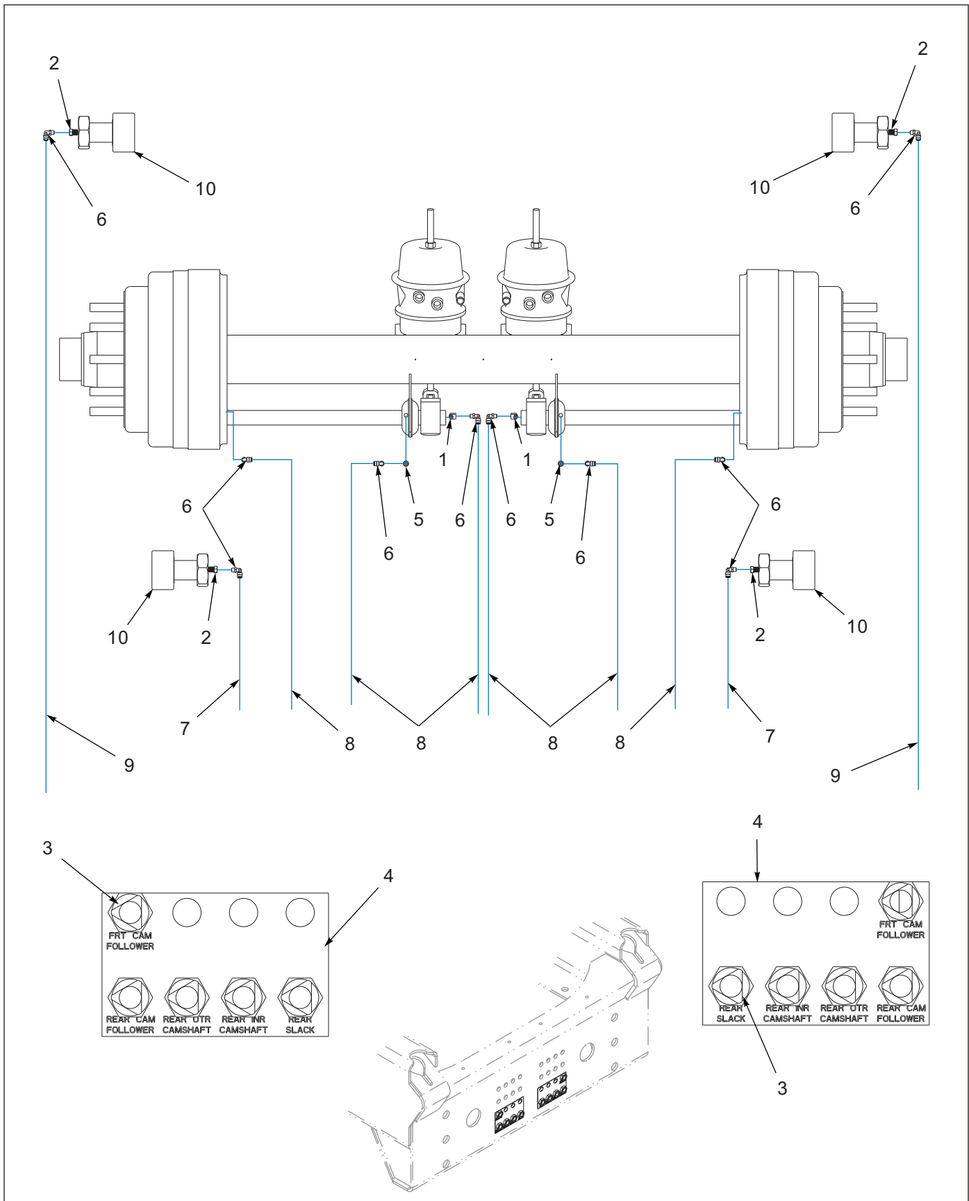
Figure 1-19: Grease System (Before 11/07/2018)
