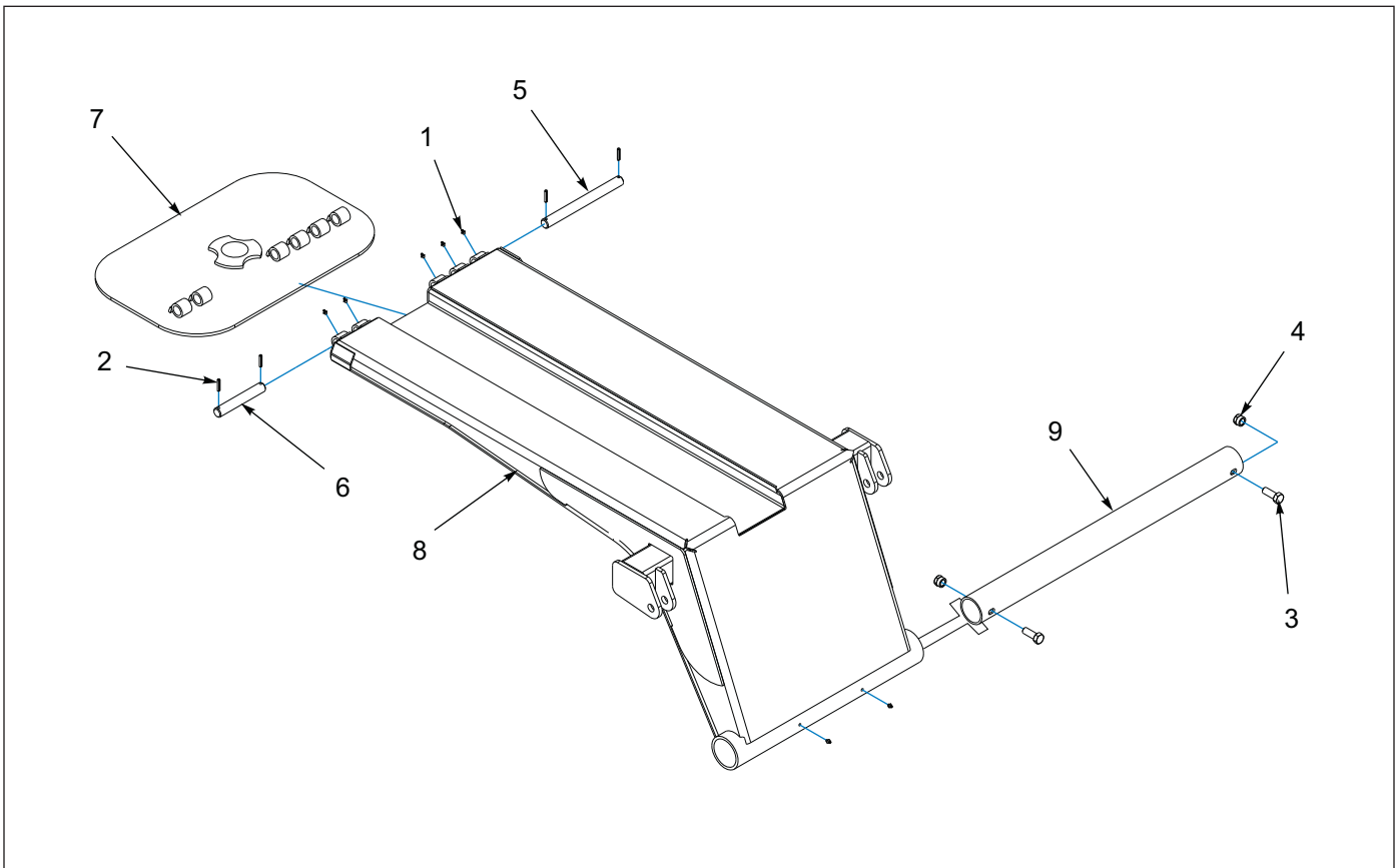
Figure 1-65: Hitch
