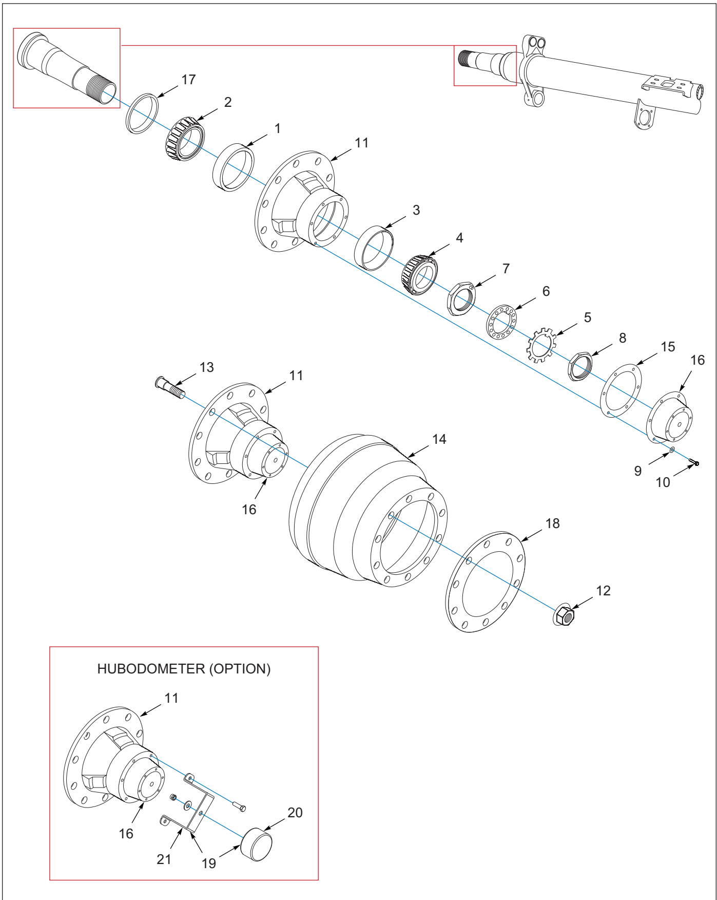
Figure 1-37: Axle 16.5 x 7 Drum and Hub Assembly, Dexter
