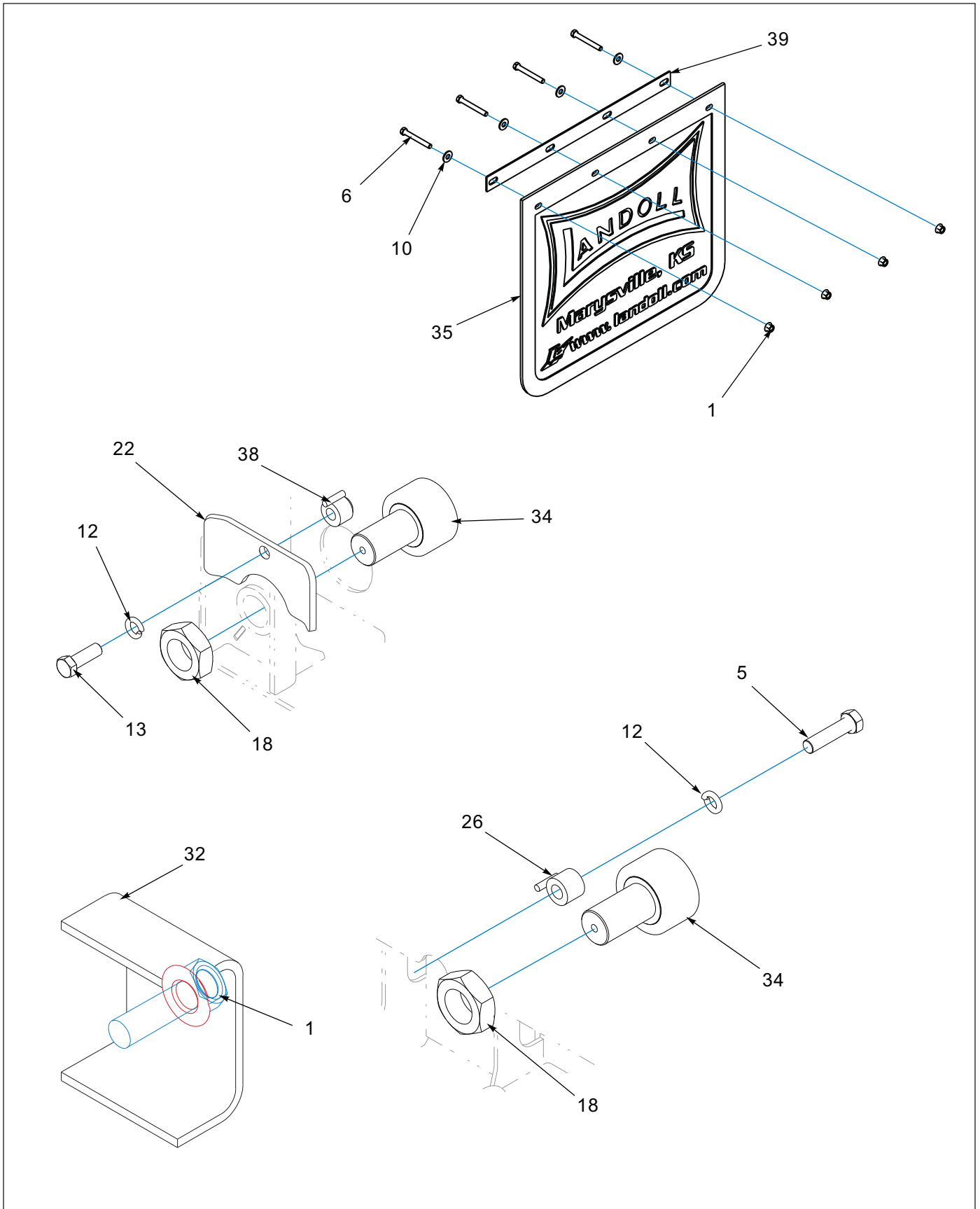
Figure 1-17: General Items (2 of 3)
