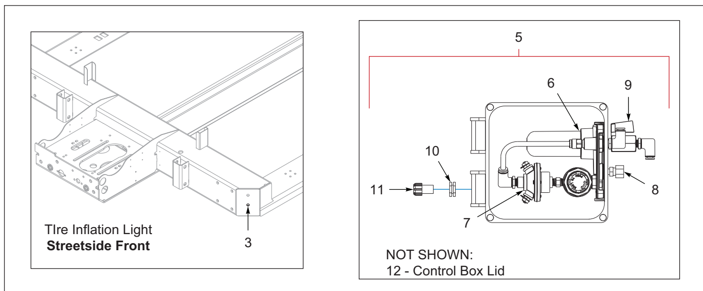
Figure 9-17: Tire Inflation, 1 Axle (2 of 2)
