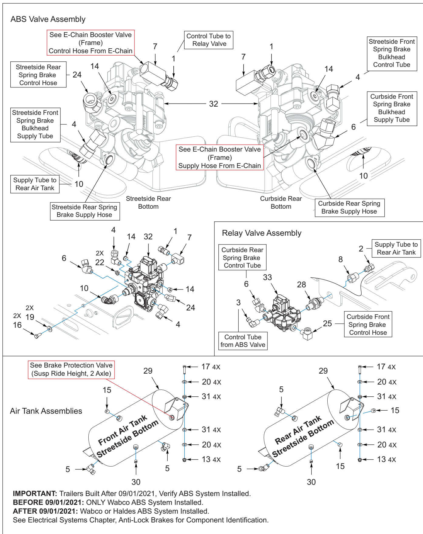
Figure 8-6: Anti-Lock Brakes, 2 Axle, Haldex (2 of 3)
