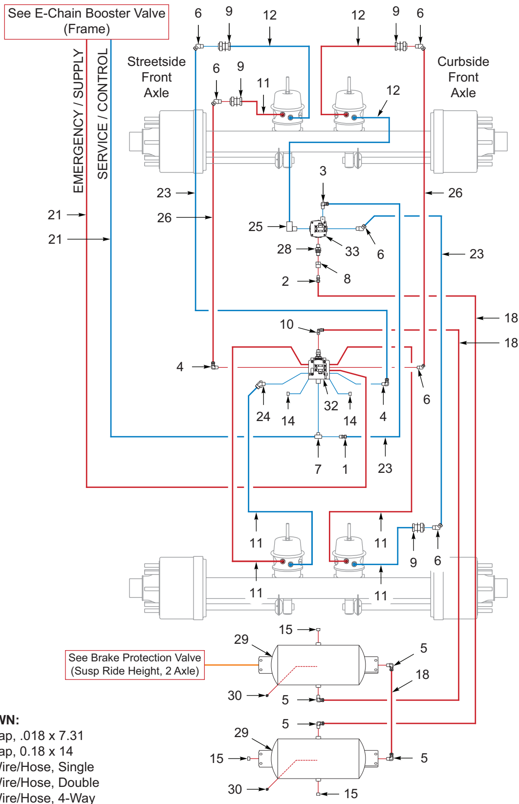
Figure 8-7: Anti-Lock Brakes, 2 Axle, Haldex (3 of 3)
