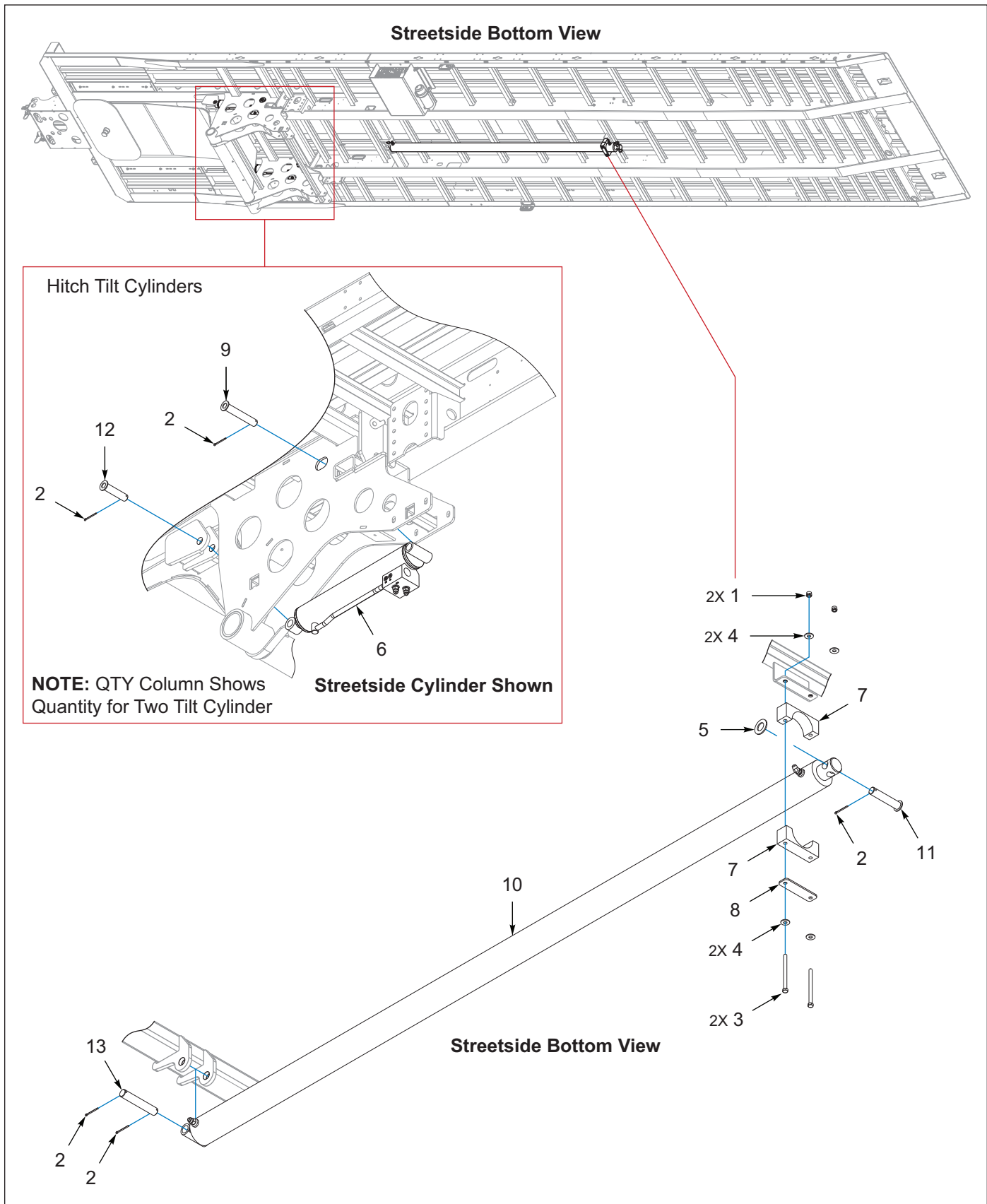
Figure 2-12: Hydraulic Cylinders, Hitch Tilt & Travel Axle
