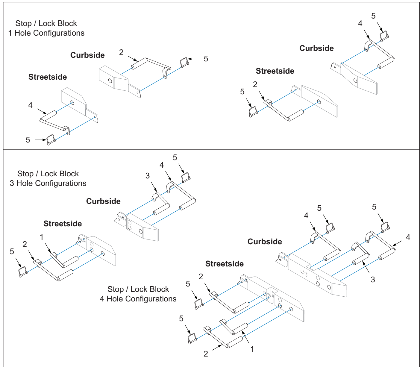
Figure 7-12: Container Stop & Lock Block, Stop / Lock Pins
