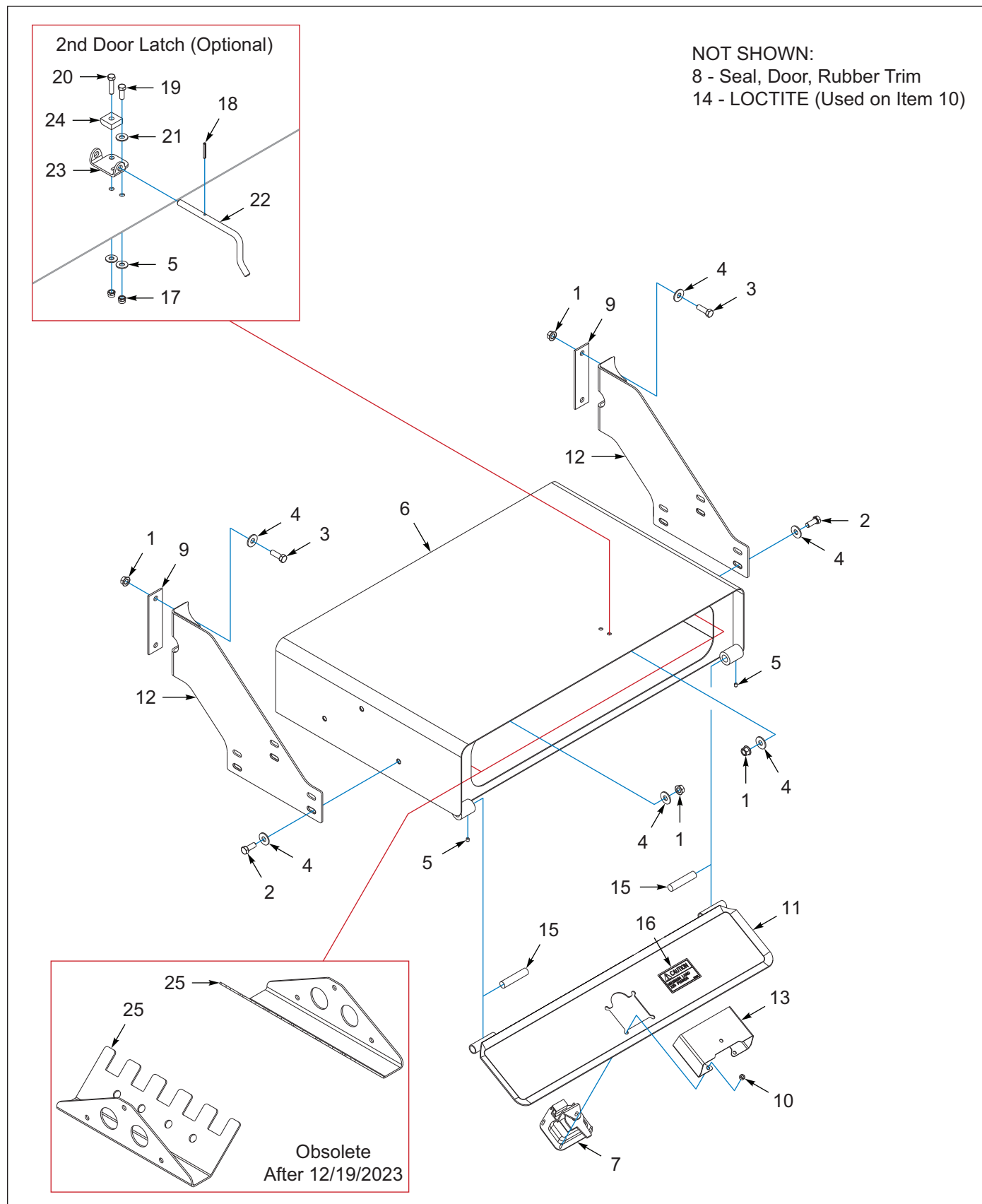
Figure 4-8: Toolbox, Bolt-On, 42"W X 28"D X 9"H
