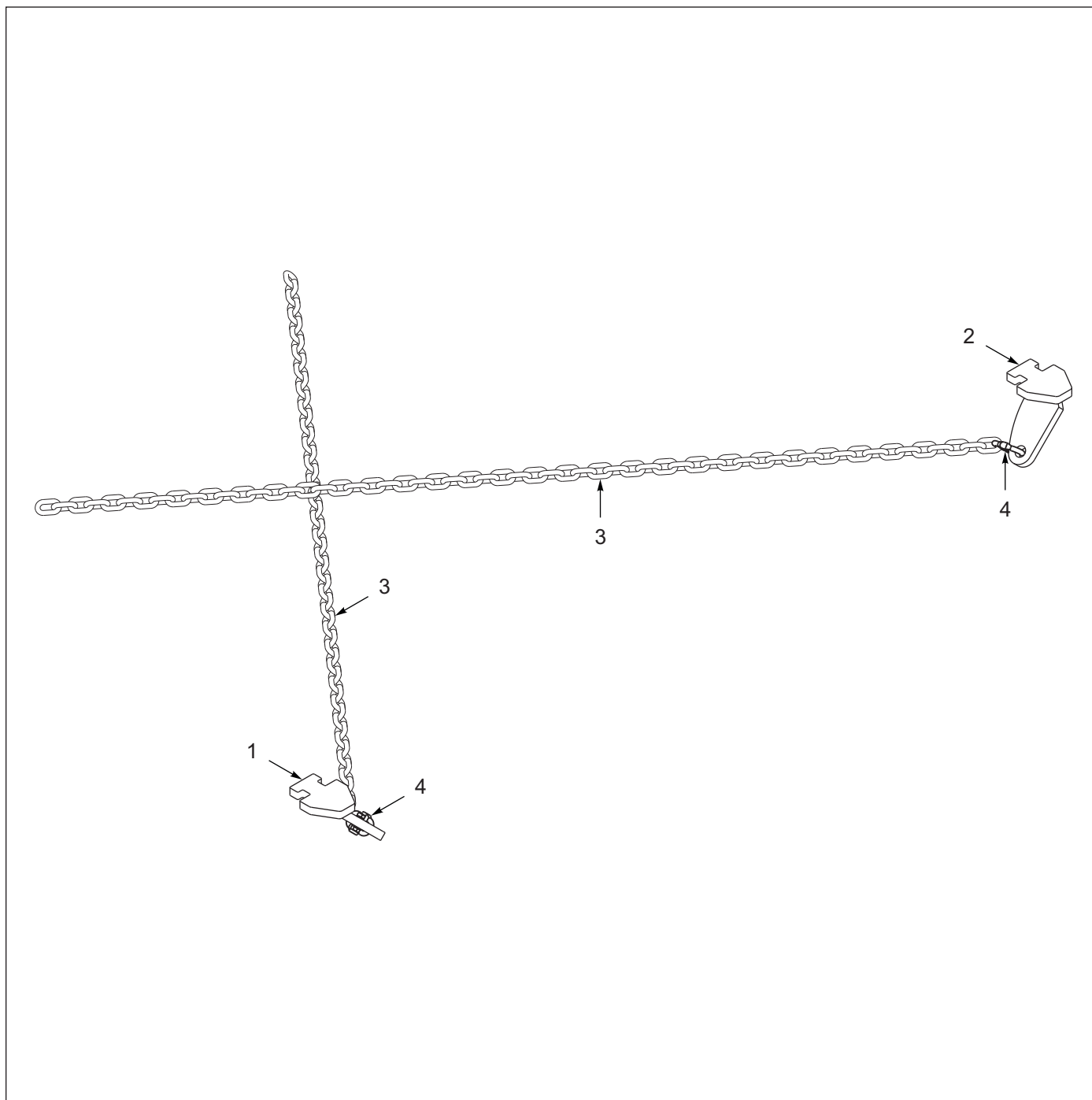
Figure 7-3: Chain Assembly, Container Loading, Rear
