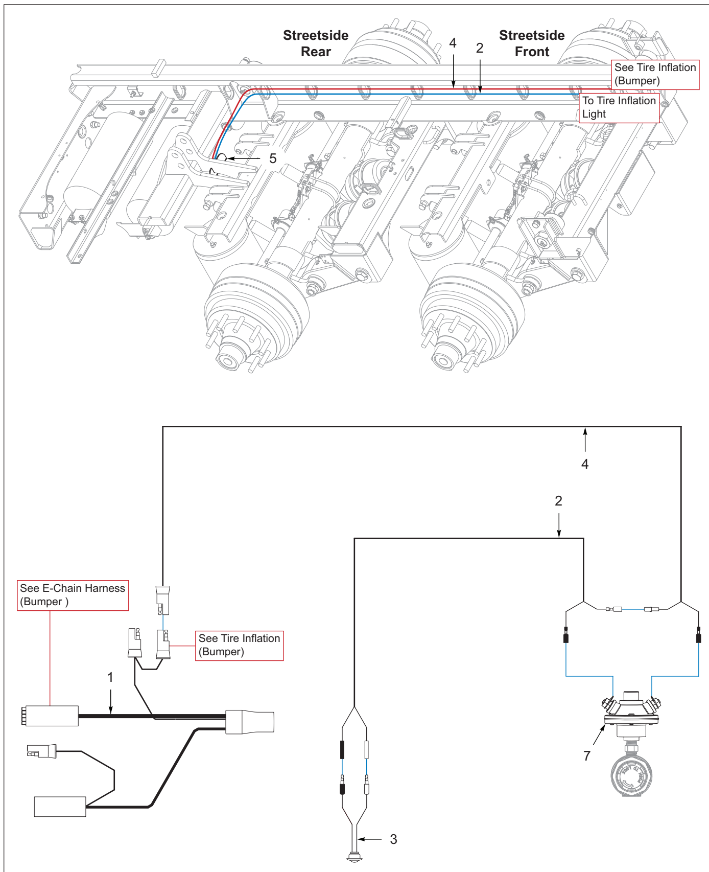
Figure 9-18: Tire Inflation, 2 Axle (1 of 2)
