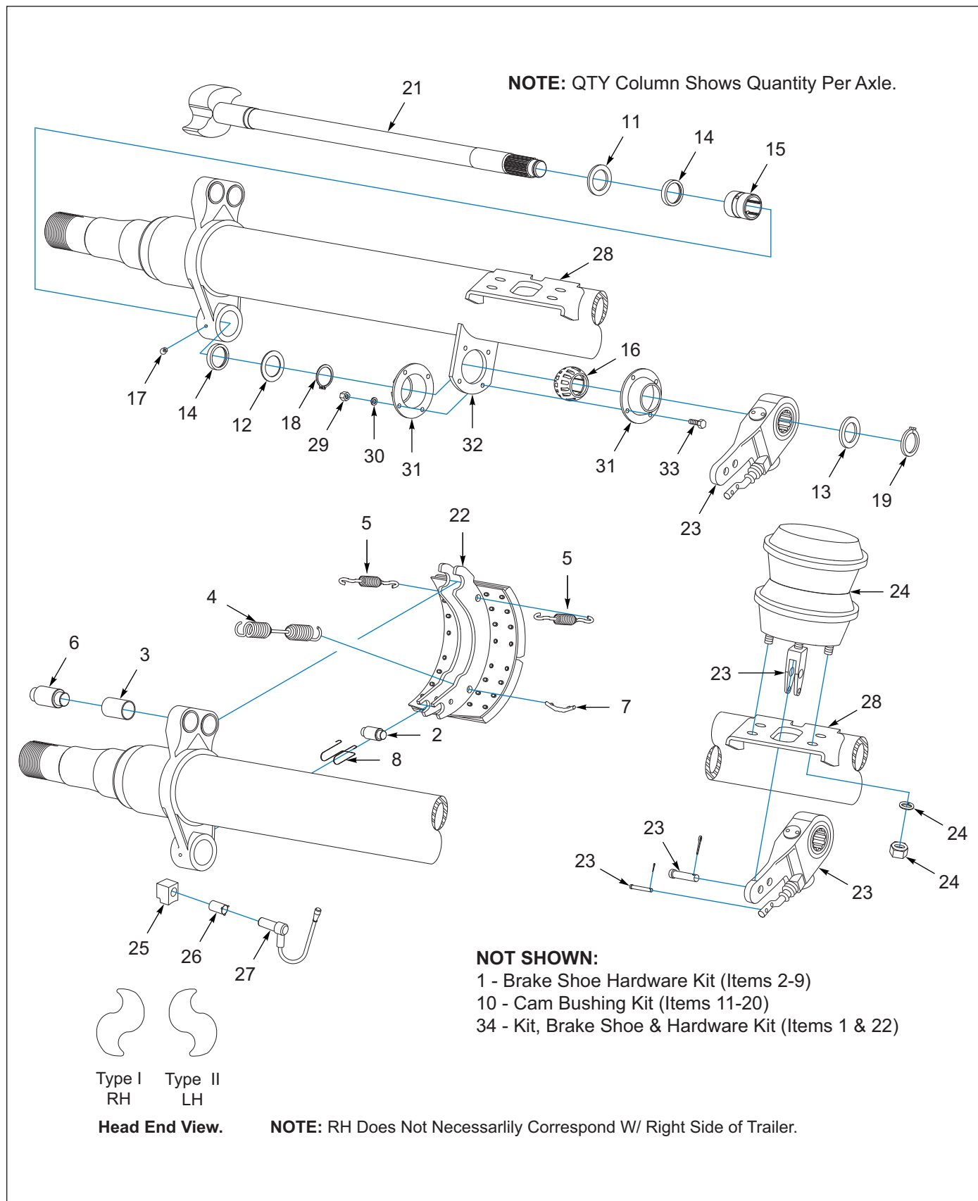
Figure 3-5: Axle 16.50 x 7.00 Drum Brake Components
