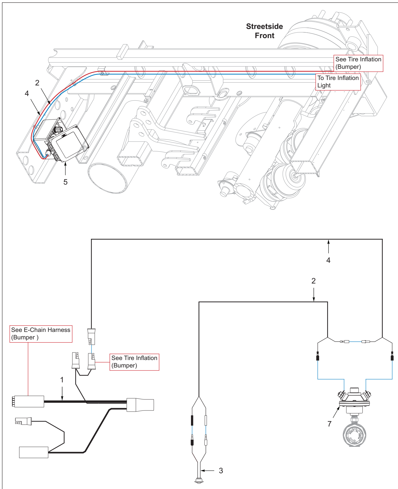
Figure 9-16: Tire Inflation, 1 Axle (1 of 2)
