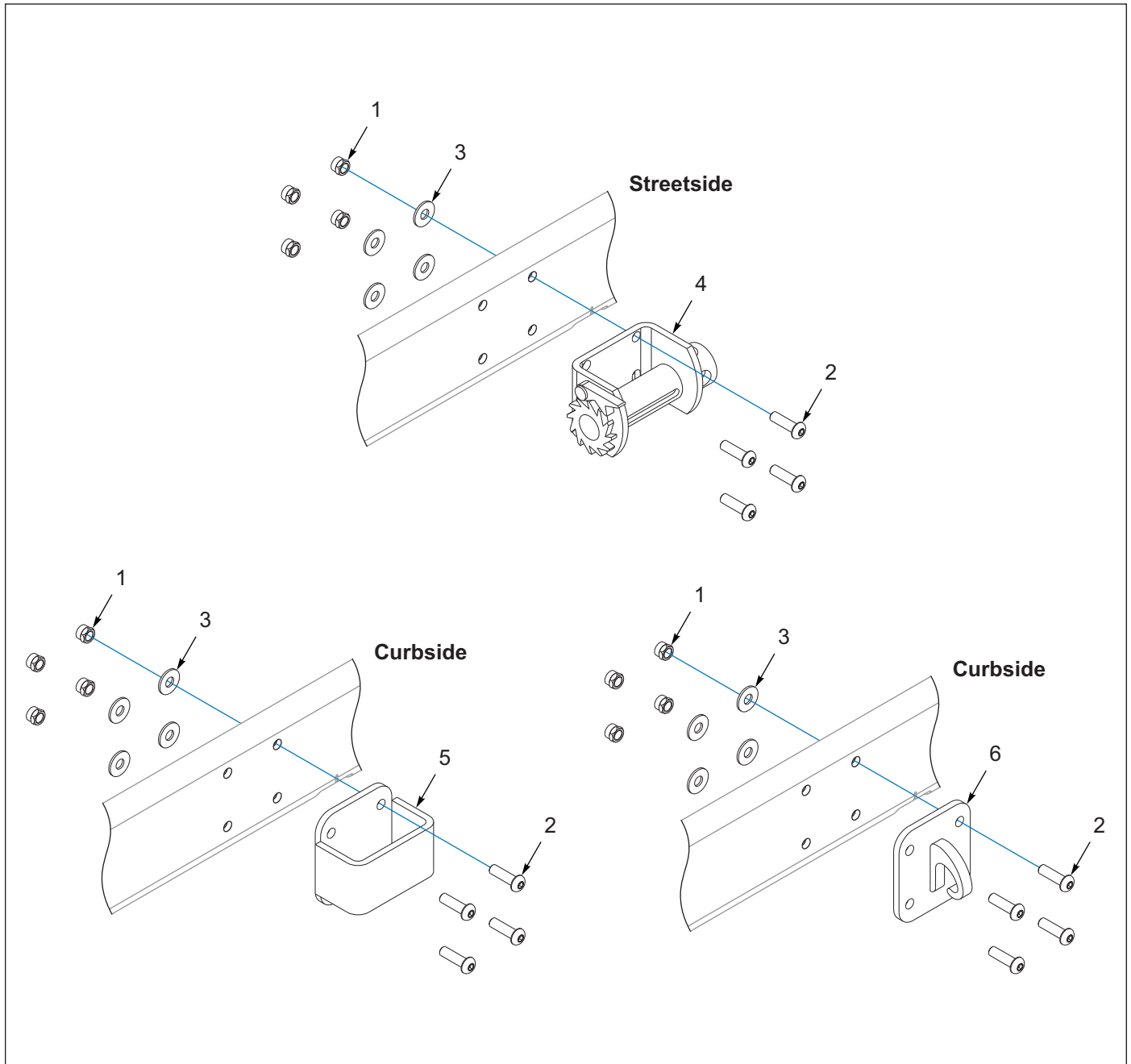
Figure 7-18: Tie Down, Strap Ratchet, Lo-Pro, Strap Pocket / J-Hook, Bolt On
