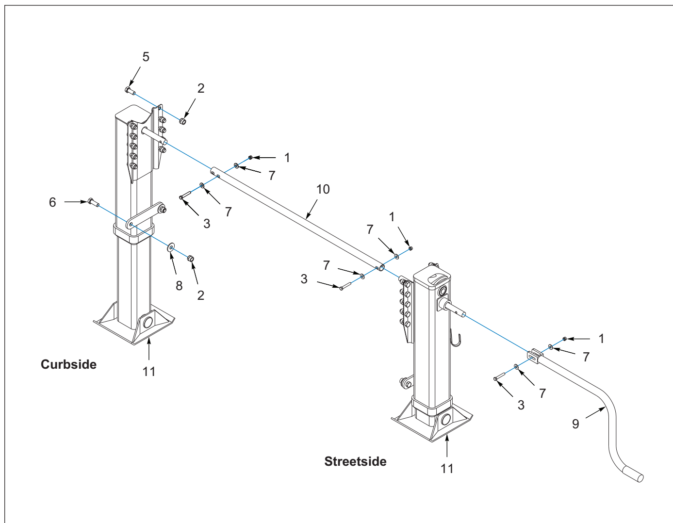
Figure 2-14: Landing Legs, Gear, 2 Spd, Flip Crank
