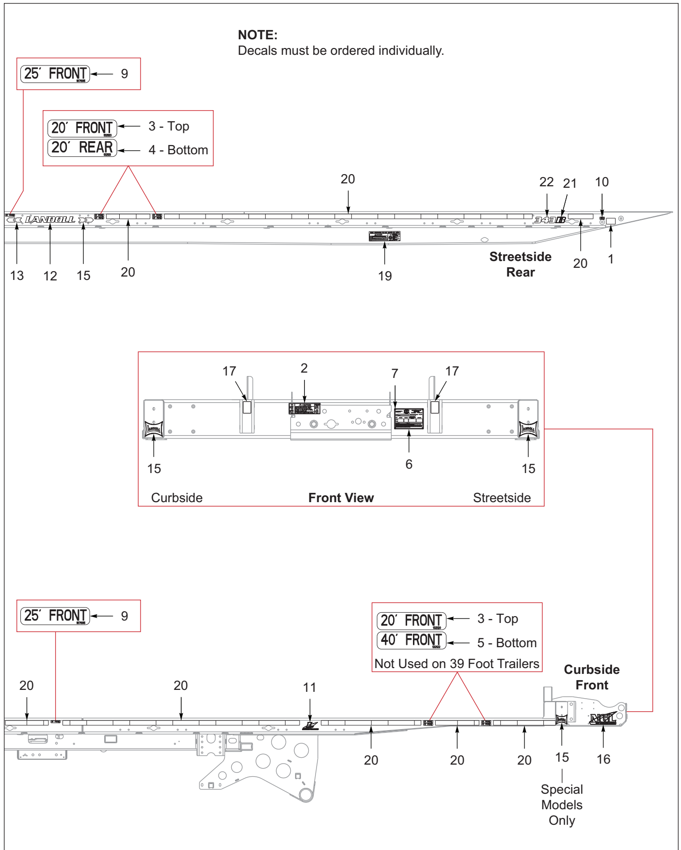
Figure 1-2: Frame Assembly (2 of 3)
