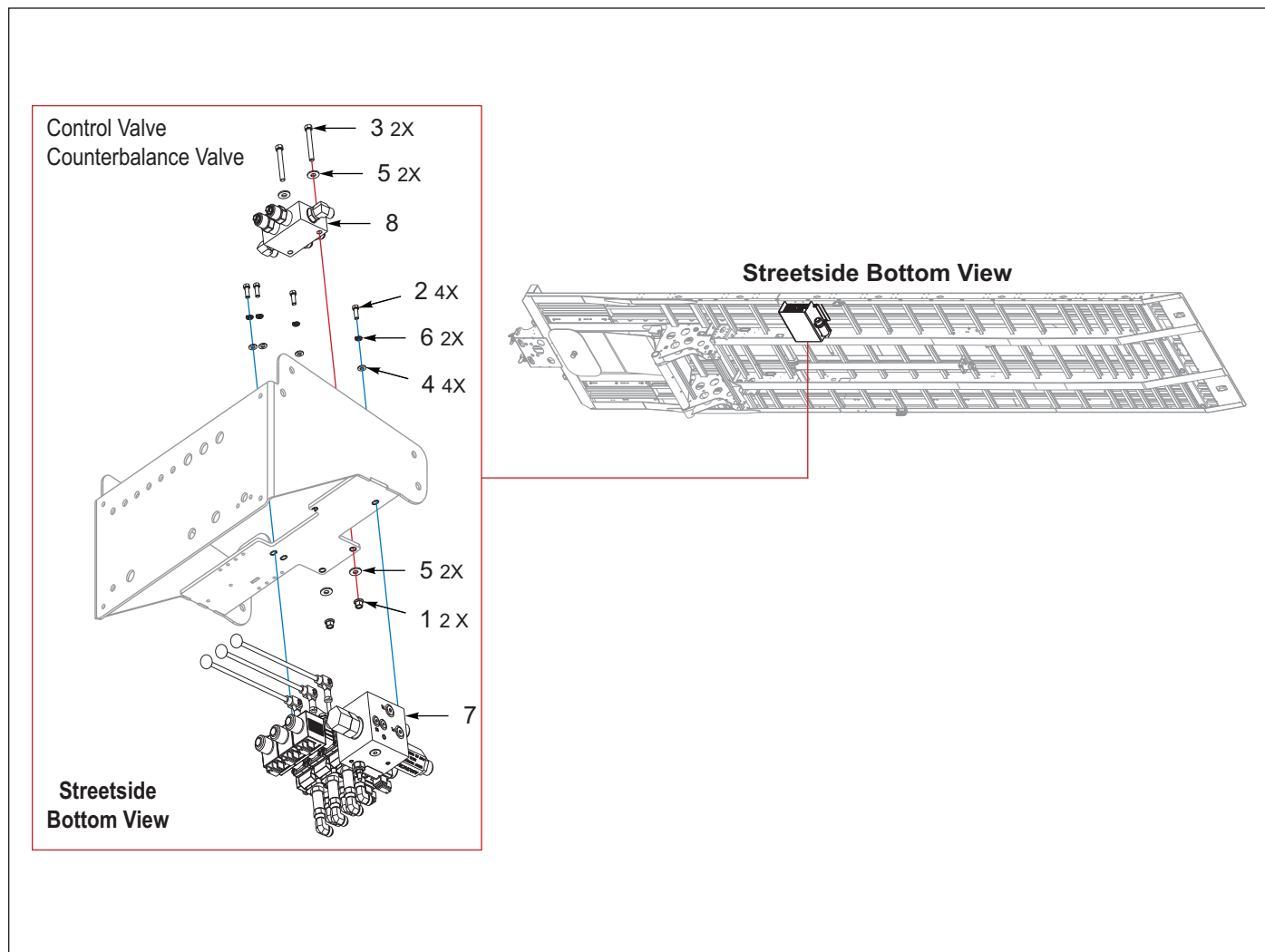
Figure 2-13: Hydraulic Valve, Control & Counterbalance
