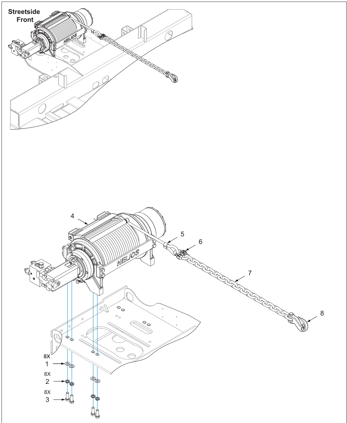
Figure 6-5: Winch Install, Ramsey 20K, 2 Speed, Spring Tension
