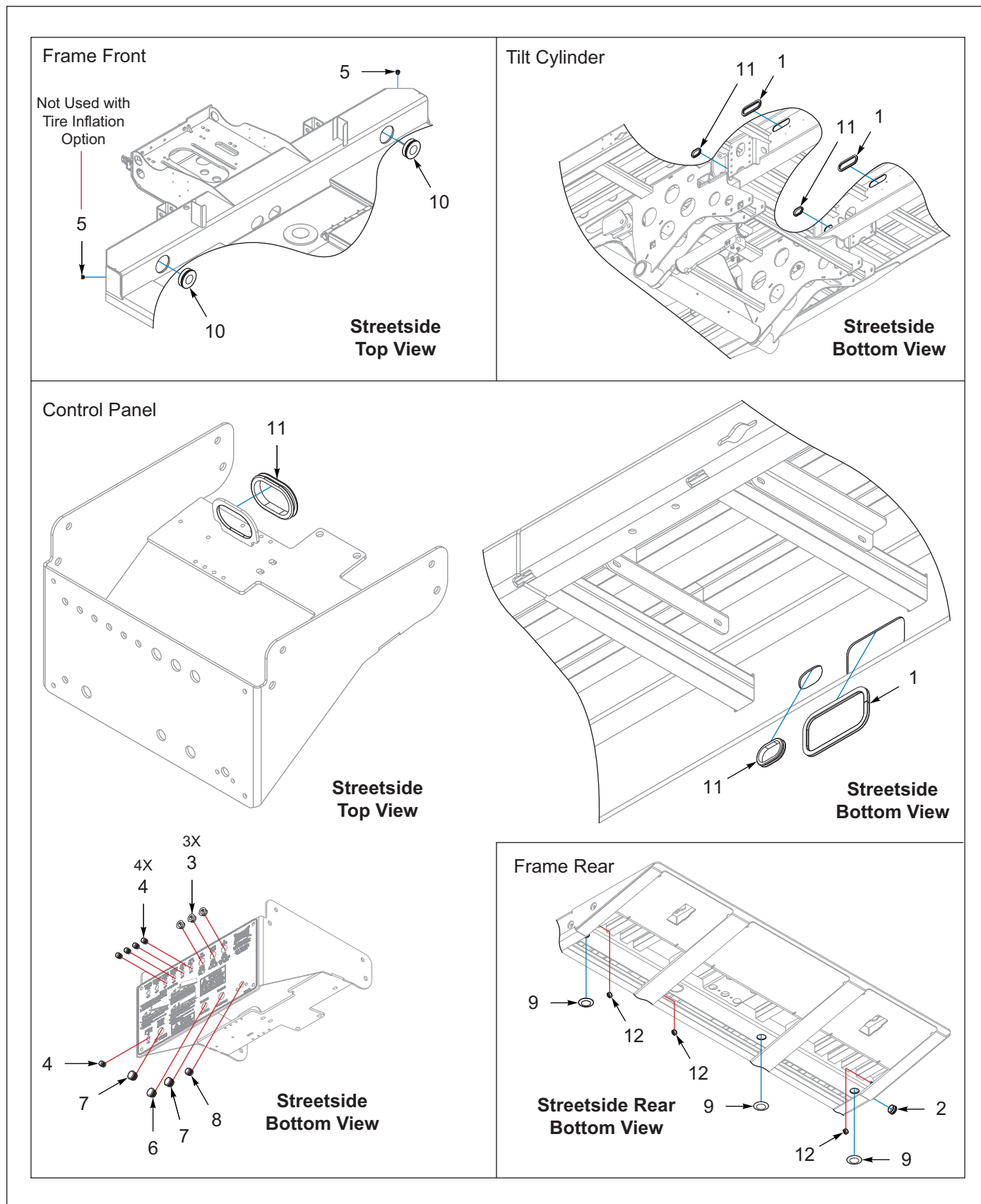
Figure 2-8: Grommets & Plugs, Frame Assembly
