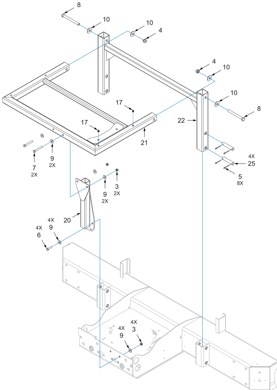
Figure 5-8: Mount, Front, Stand (1 of 2)
