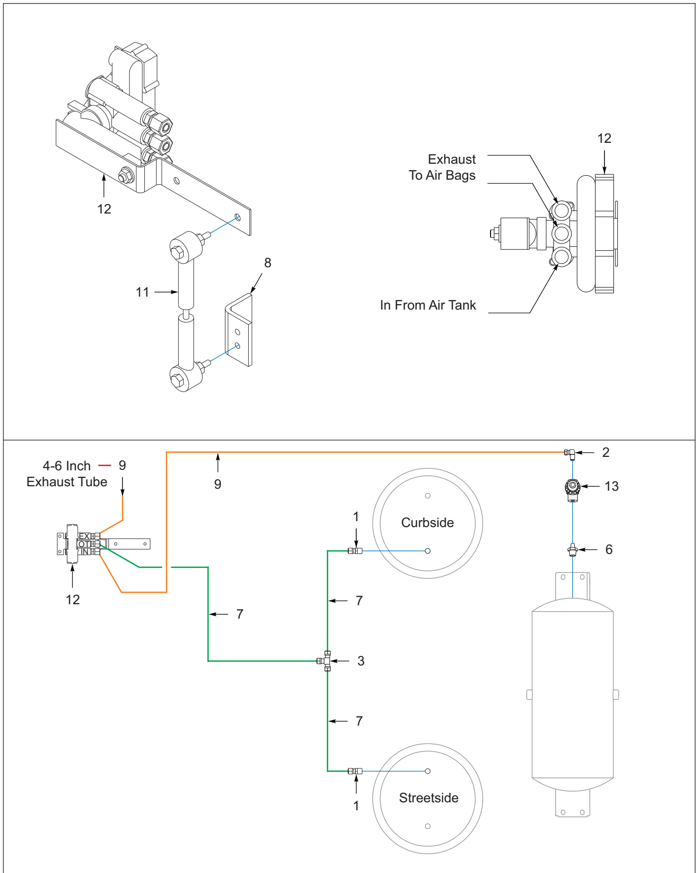
Figure 8-9: Suspension, Ride Height, 1 Axle (2 of 2)
