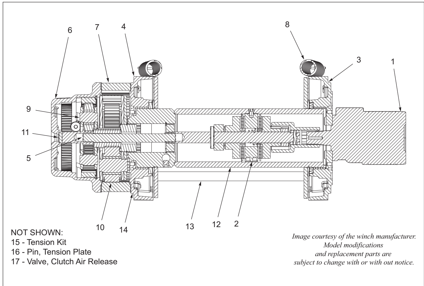
Figure 6-10: Winch Components, Warn 12K, 1 Speed, Spring Tension
