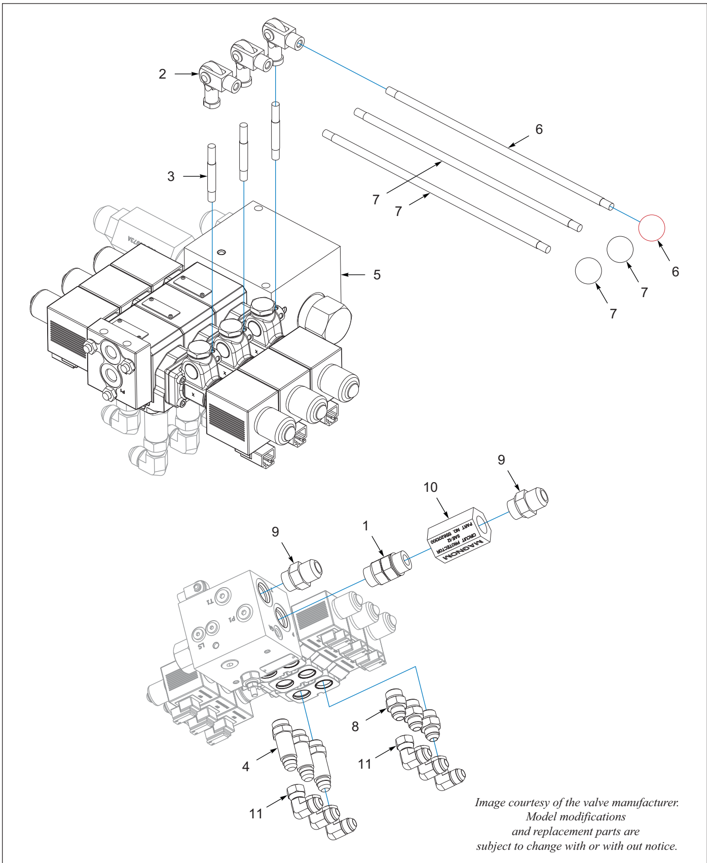
Figure 11-11: Valve Assembly, 3 Spool Solenoid
