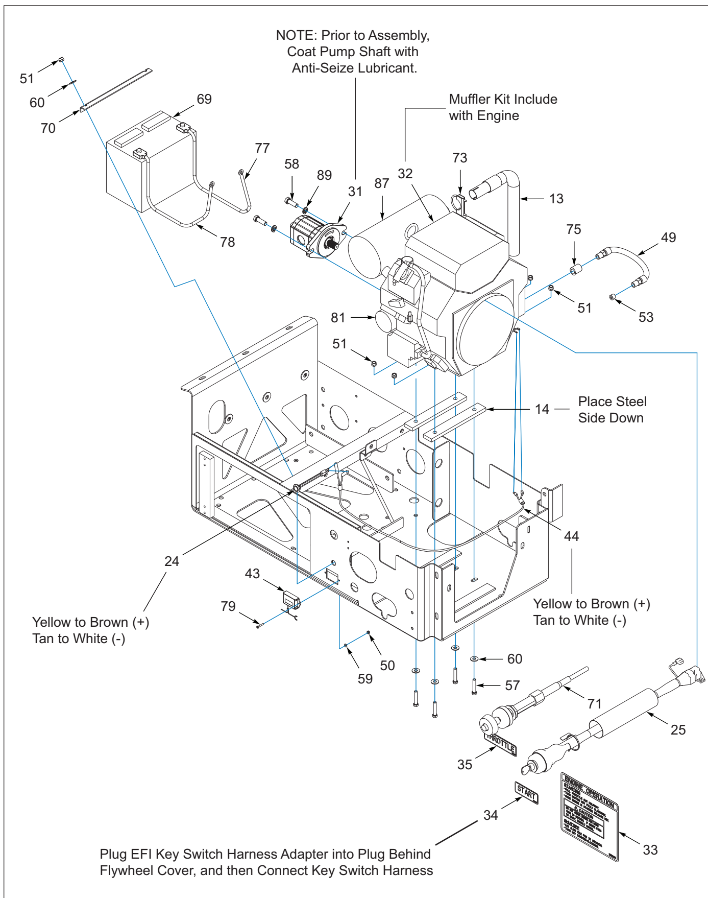
Figure 5-3: Engine Package, 25 HP, Upper Deck Assembly (3 of 5)
