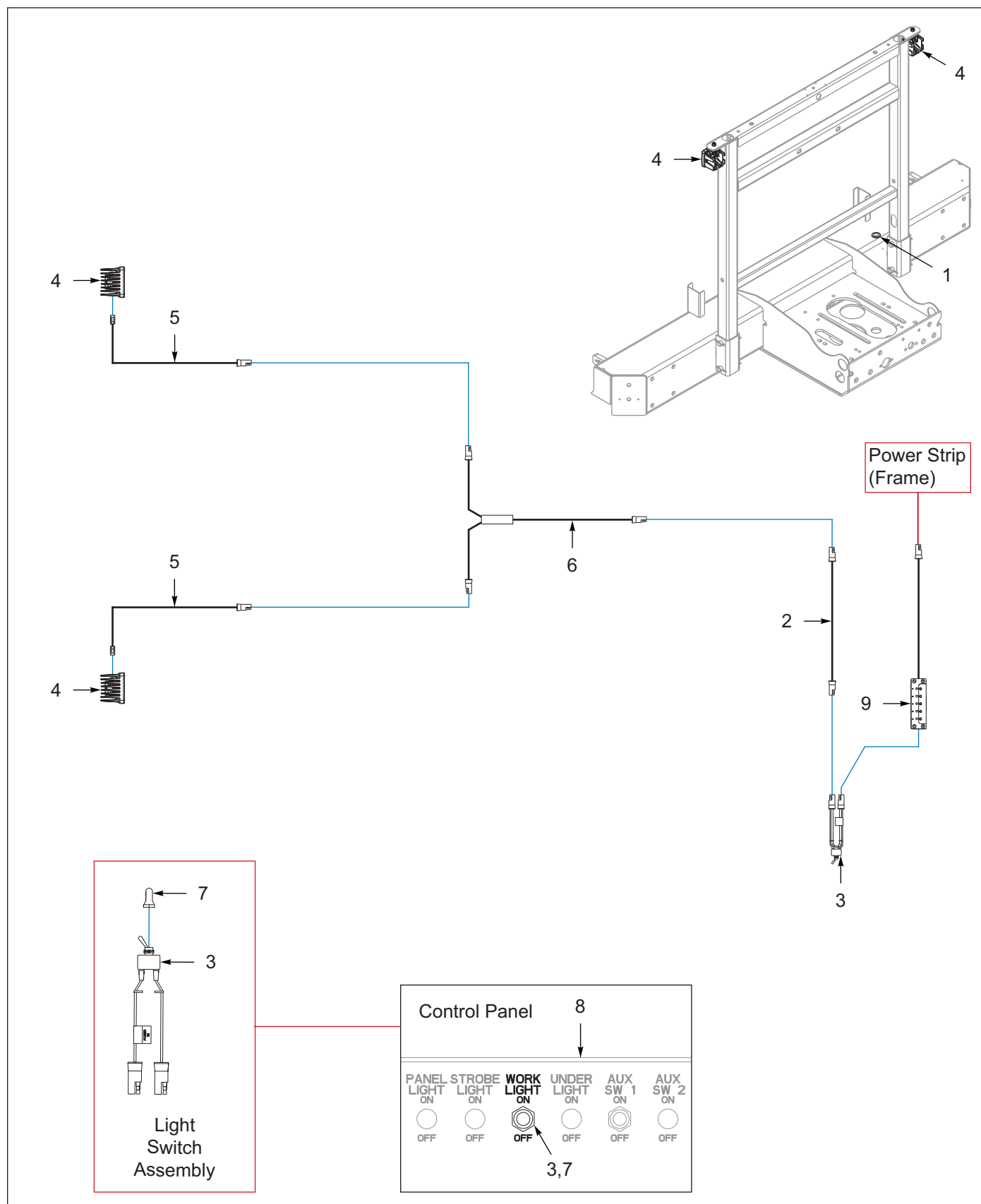
Figure 9-13: Lights, Work, Bulkhead, Accessory Rack (Option)
