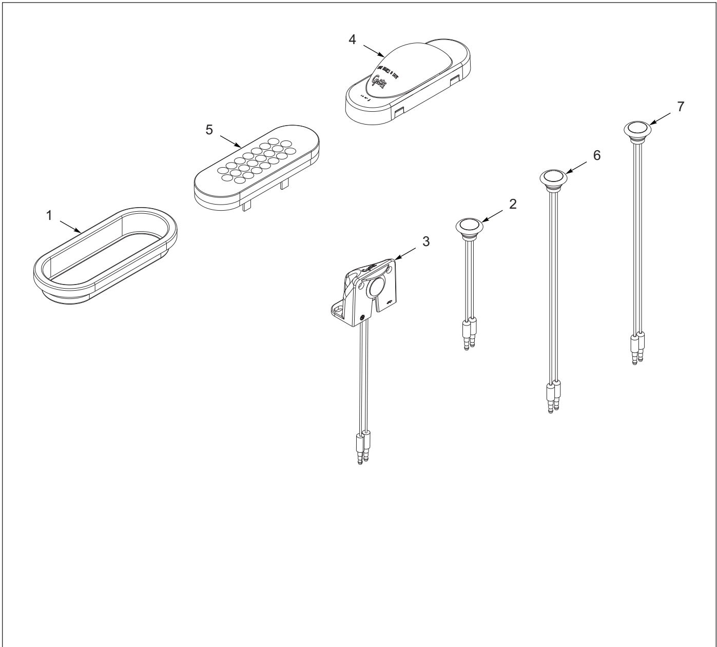
Figure 9-10: Light Kit, Spare (Option)
