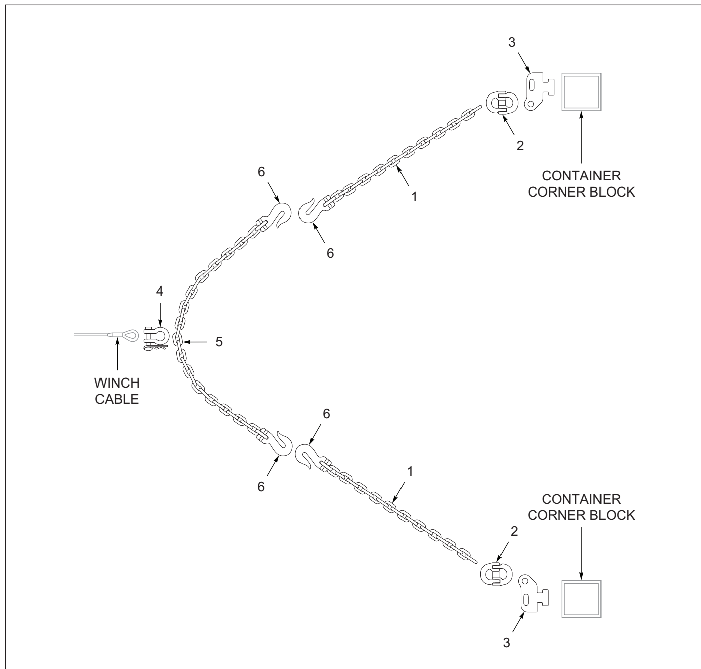
Figure 7-2: Chain Assembly, Container Loading, Front, Chain / Bridle
