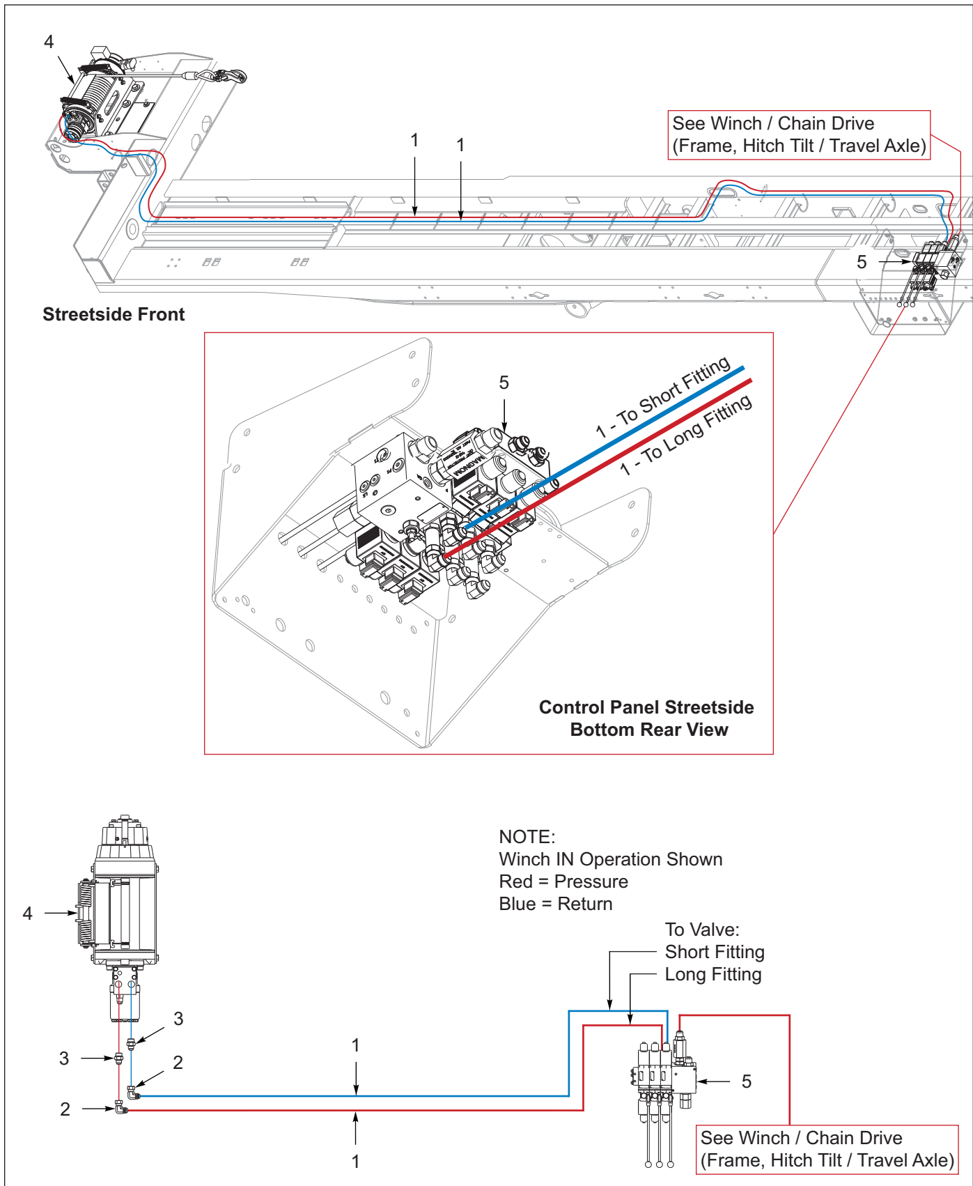
Figure 11-4: Winch Install, Ramsey 12K, 1 Speed, Spring Tension
