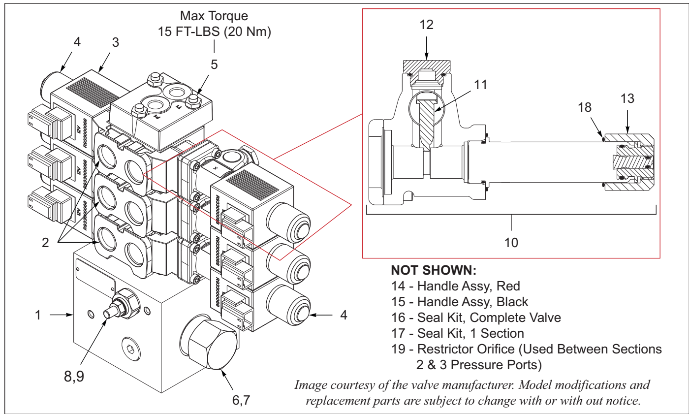
Figure 11-12: Valve Components, 3 Spool Solenoid
