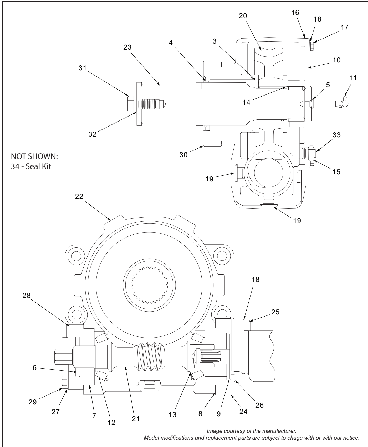
Figure 6-3: Chain Drive Components, Gearbox
