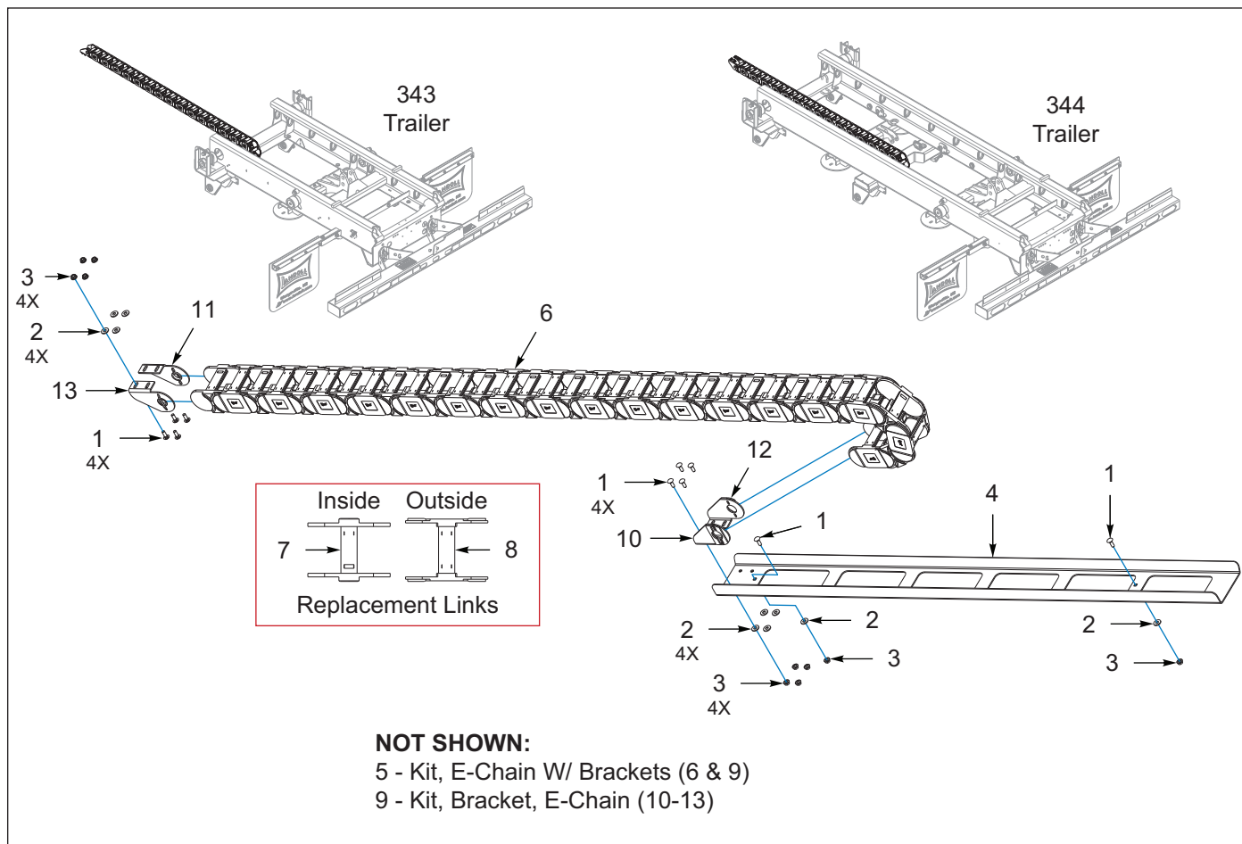
Figure 2-6: E-Chain & E-Chain Tray
