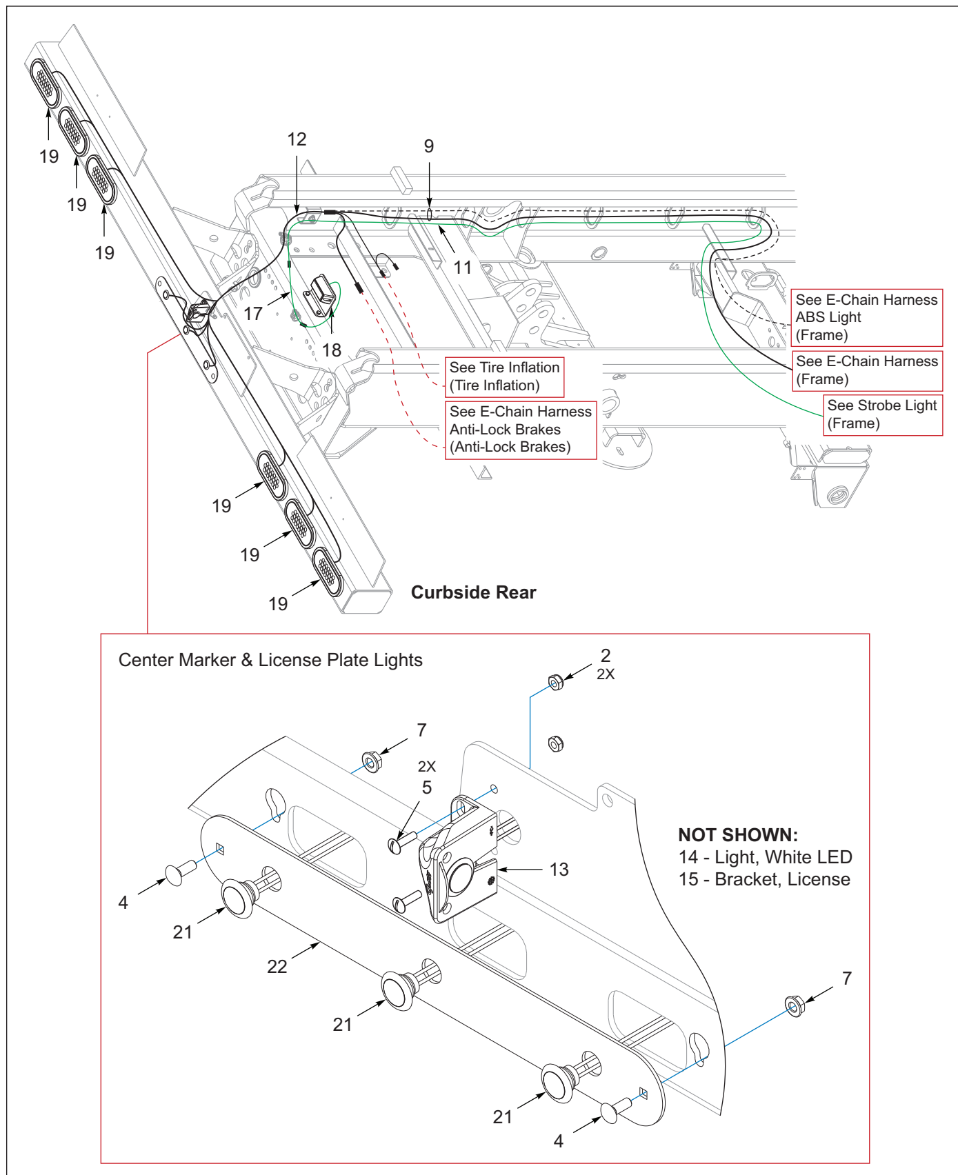
Figure 9-3: Bumper Assembly (1 of 2)
