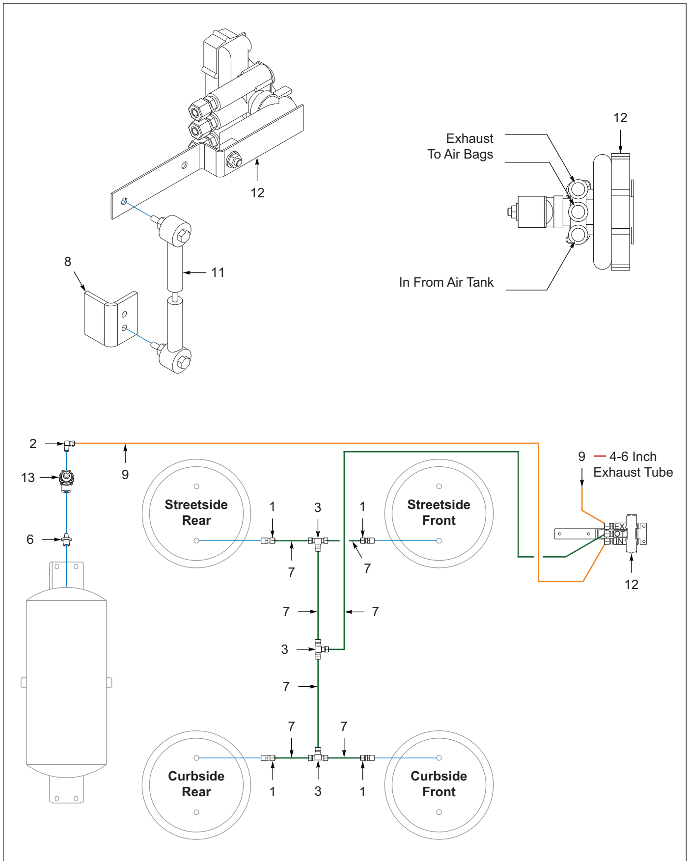
Figure 8-11: Suspension, Ride Height, 2 Axle (2 of 2)
