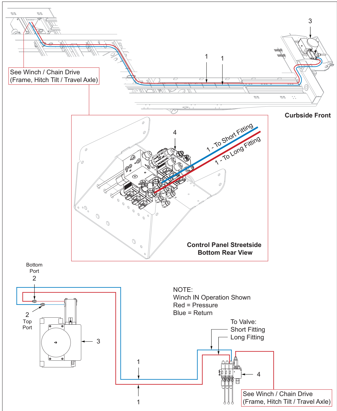
Figure 11-3: Chain Drive Install, 1 Speed
