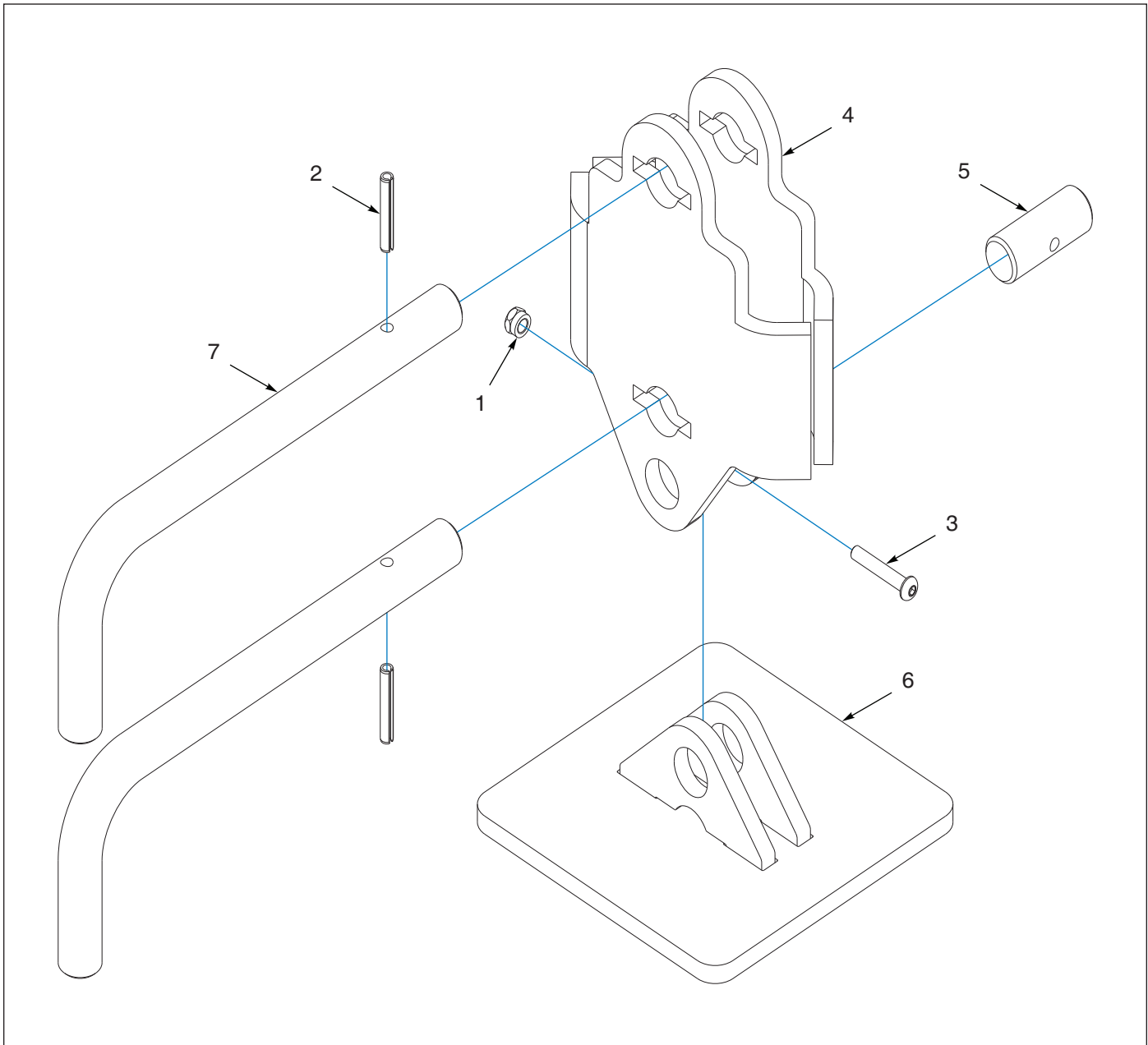
Figure 7-13: Container Stop & Hold Down, Shoe Lock Assembly
