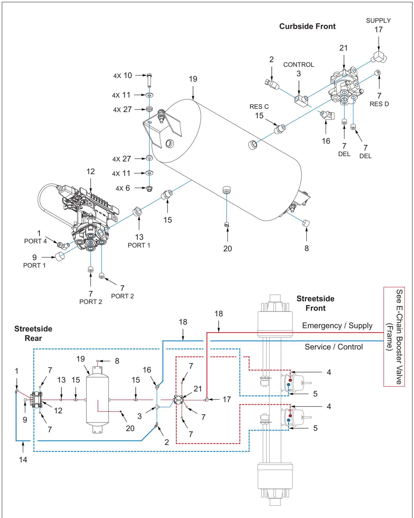
Figure 8-4: Anti-Lock Brakes, 1 Axle, Wabco (2 of 2)
