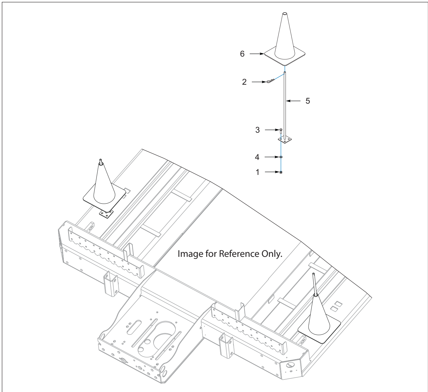
Figure 4-10: Traffic Cone Holder
