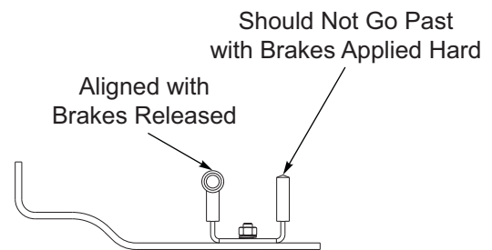
Figure 3-13: Brake Stroke Indicator, Drum Brakes Only (Option)
