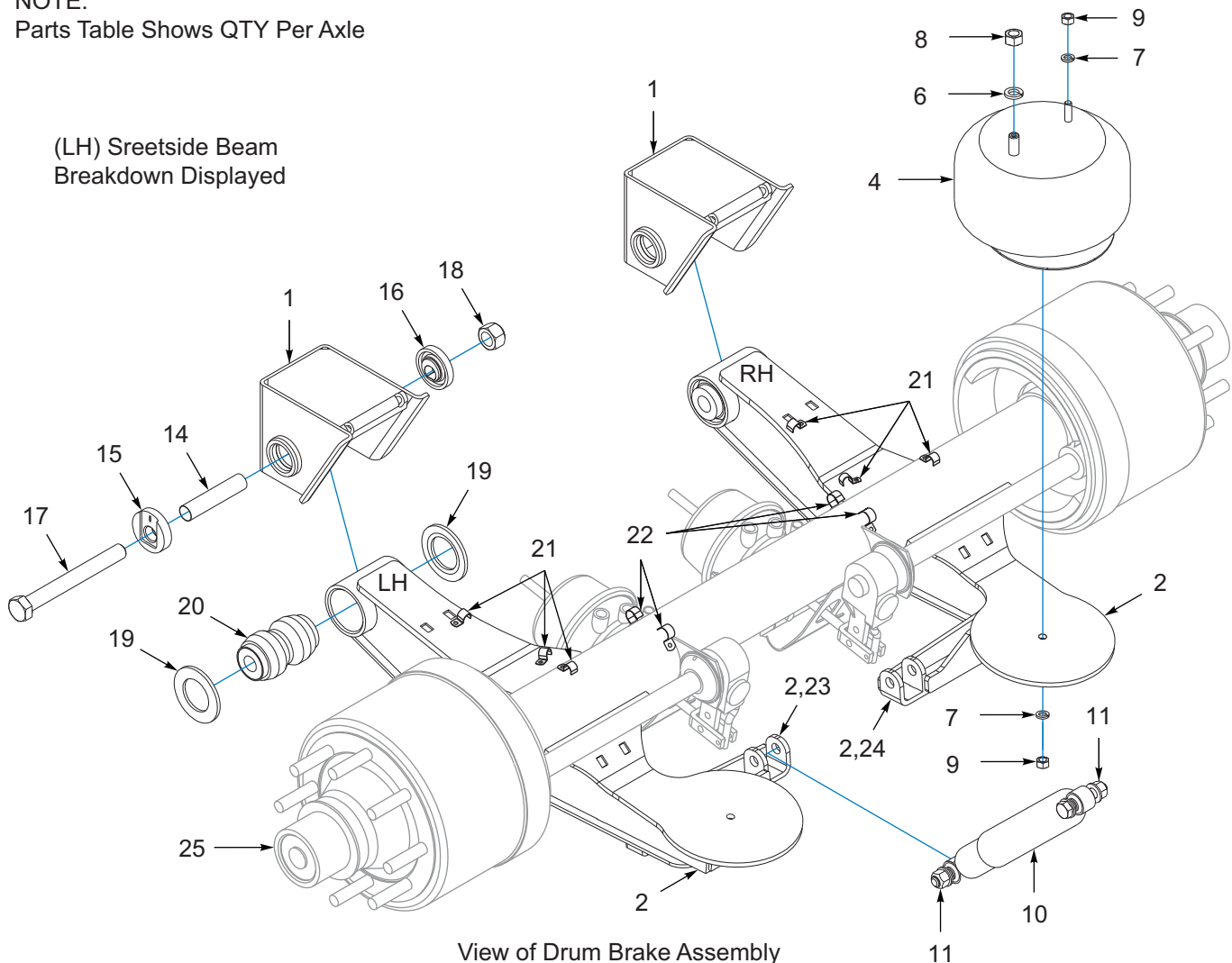
Figure 3-11: Axle Suspension, LSS-25K-3.5 RLU CC, 12.25
