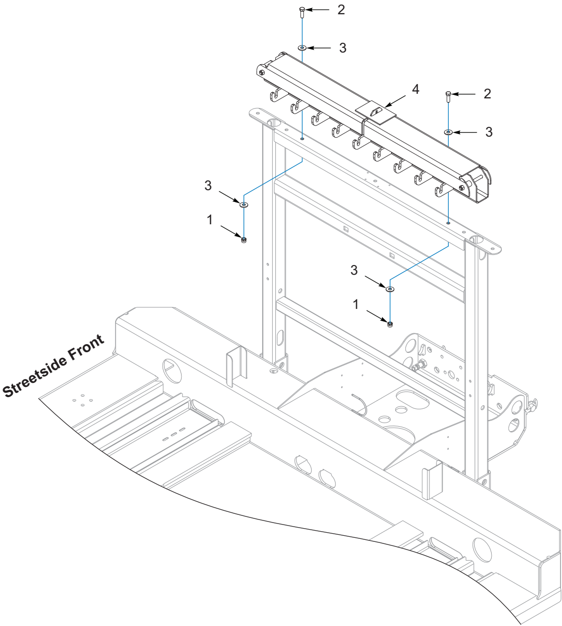
Figure 4-2: Bulkhead, Accessory Rack, Chain Rack, Lockable
