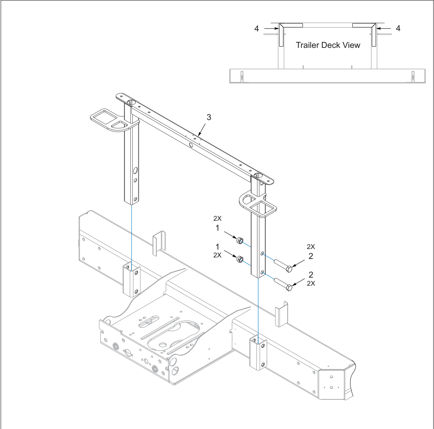
Figure 4-4: Bulkhead, Grab Handle, Stand
