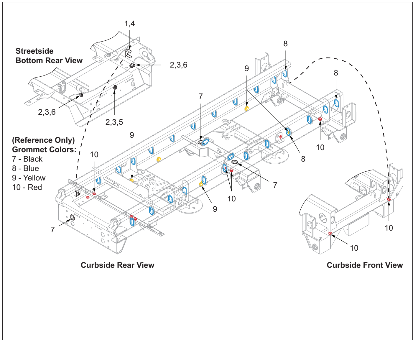
Figure 2-10: Grommets, Hose Clamps, & P-Clamps, Undercarriage, 344
