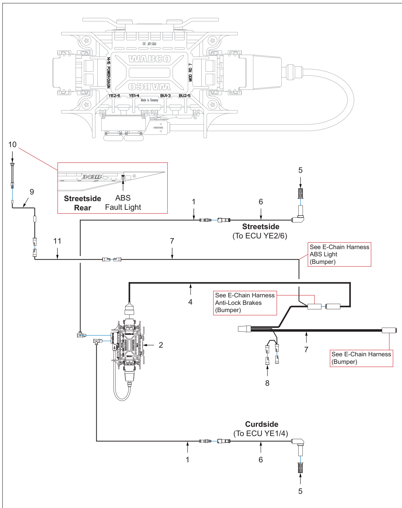
Figure 9-6: Anti-Lock Brakes, 1 Axle, Wabco (2 of 2)
