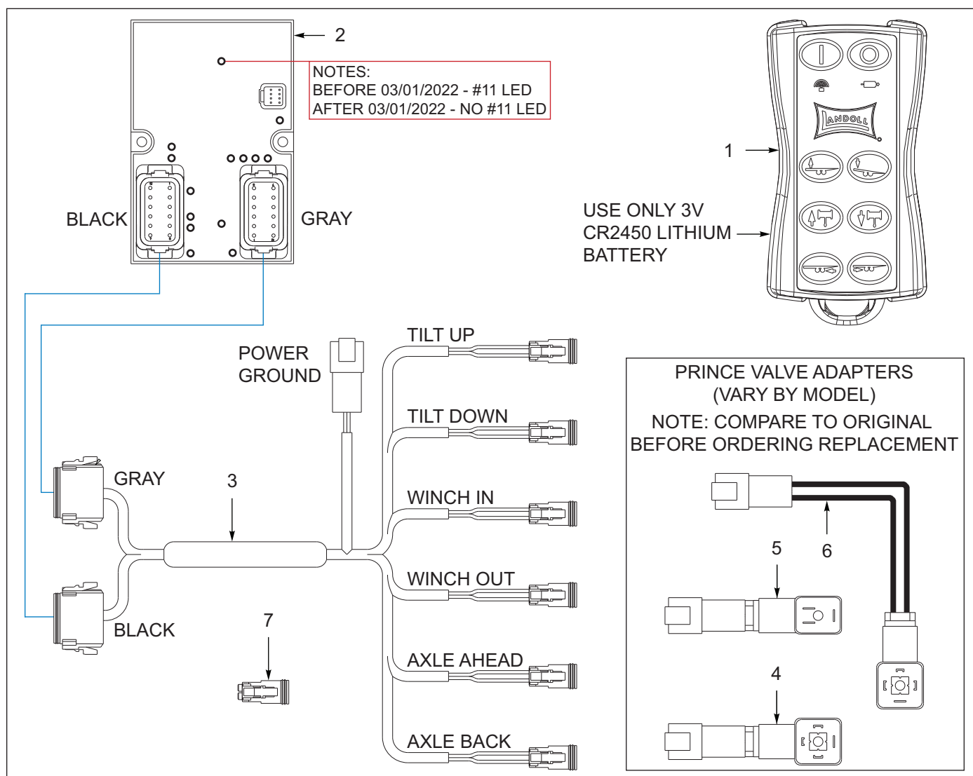
Figure 9-15: Remote Control Assembly, Wireless, Brand (Options)
