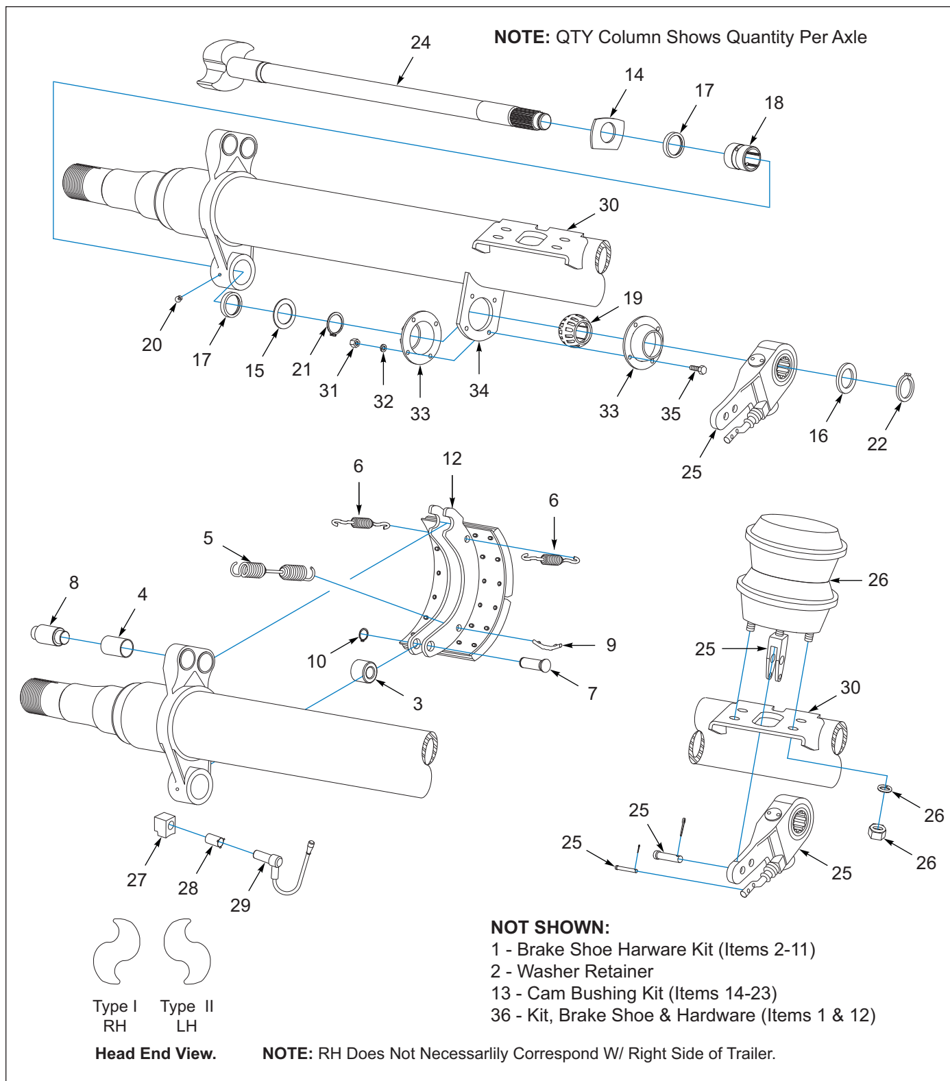
Figure 3-1: Axle 12.25 x 7.50 Drum Brake Components
