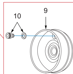
Figure 8-13: Tire Inflation, 1 Axle (2 of 2)
