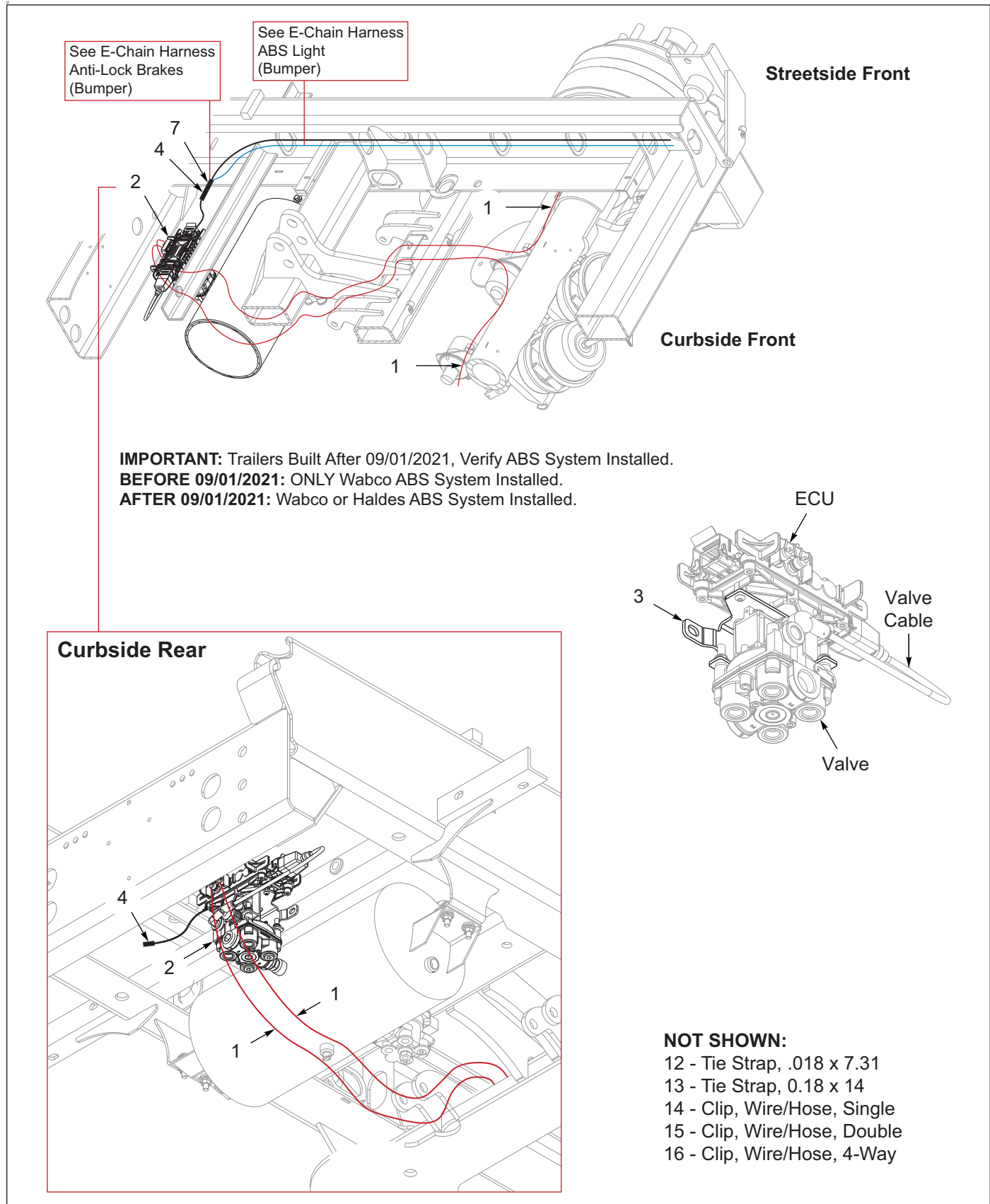
Figure 9-5: Anti-Lock Brakes, 1 Axle, Wabco (1 of 2)
