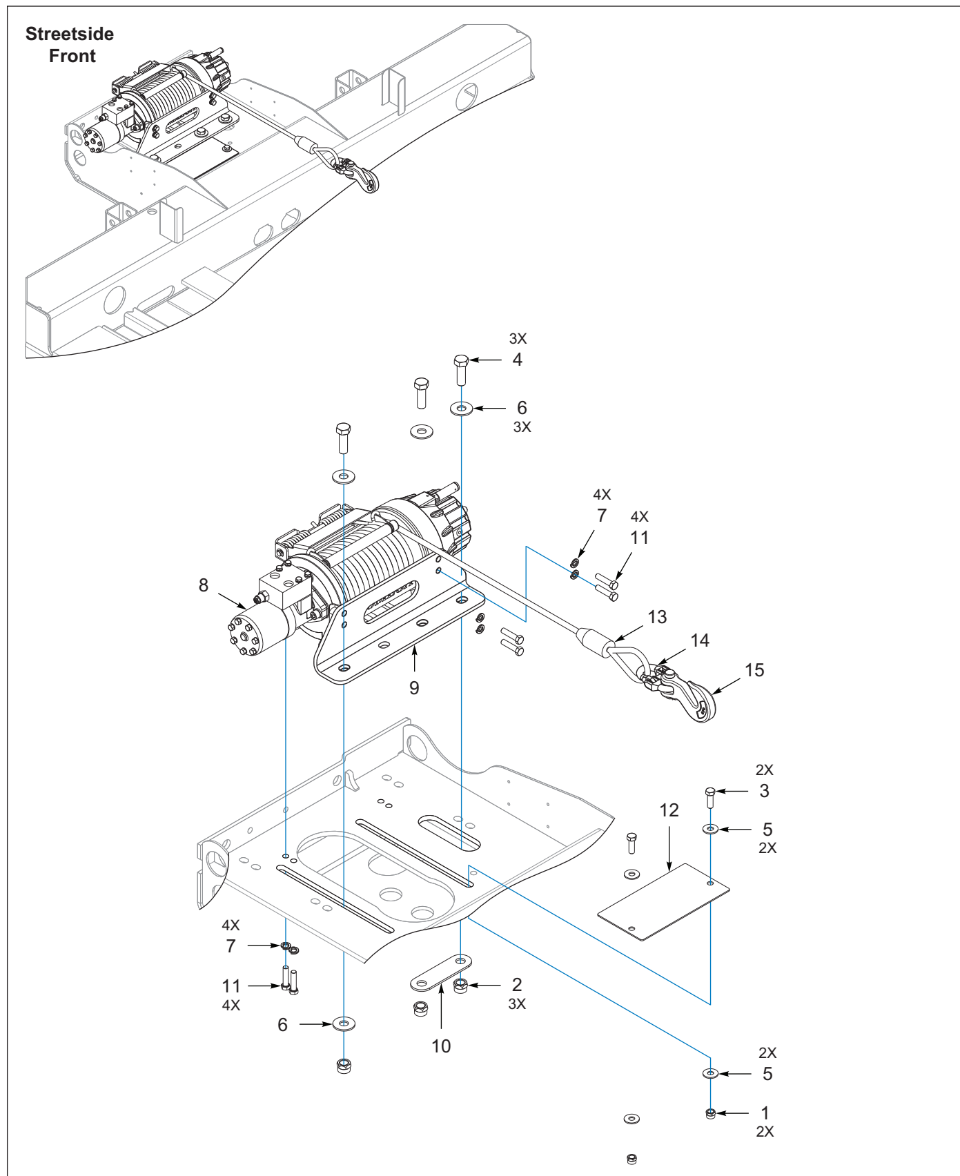
Figure 6-4: Winch Install, Ramsey 12K, 1 Speed, Spring Tension
