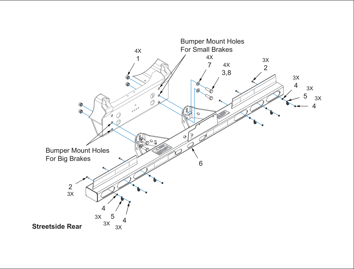
Figure 2-2: Bumper, Rear
