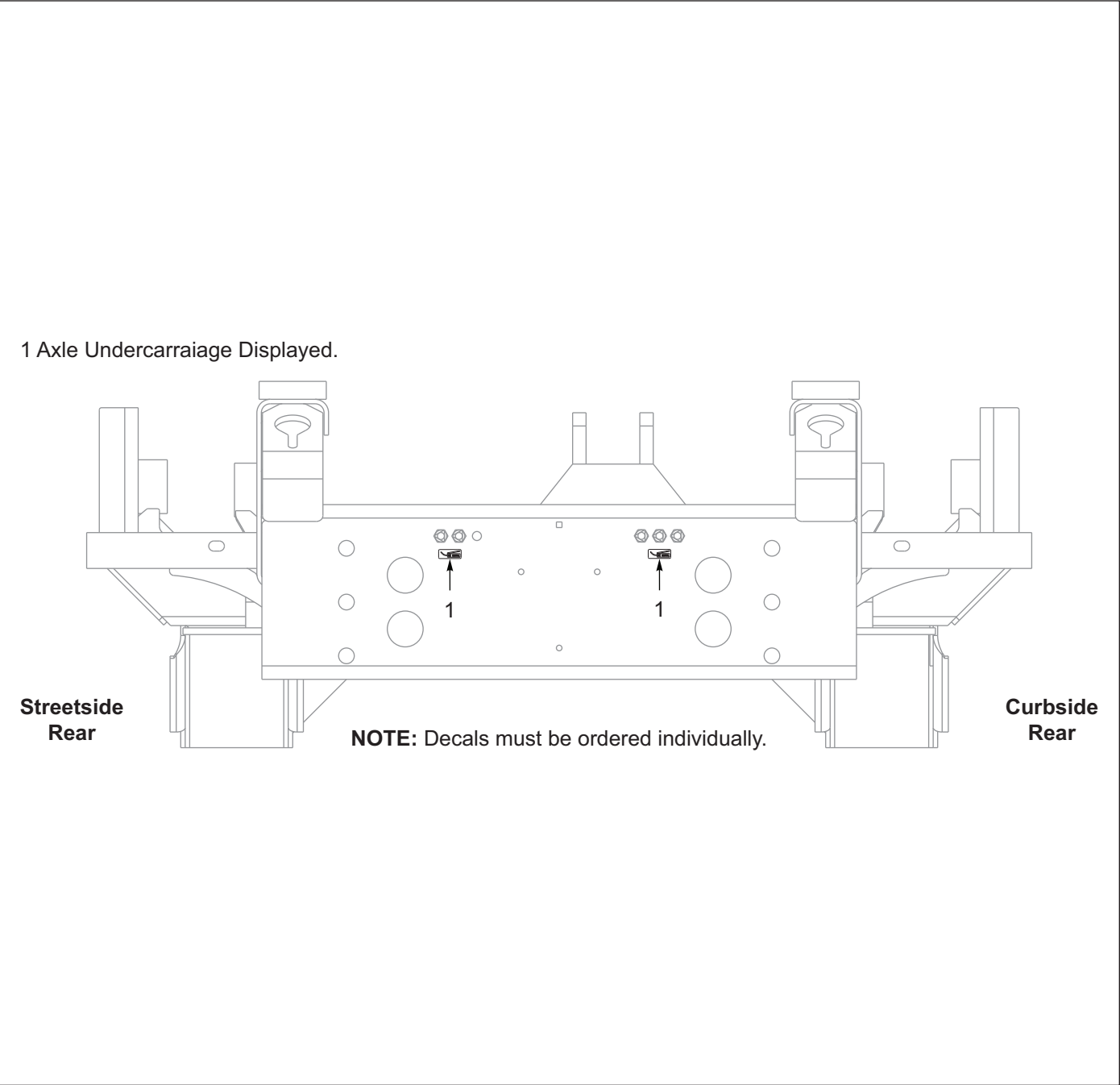
Figure 1-5: Undercarriage Assembly
