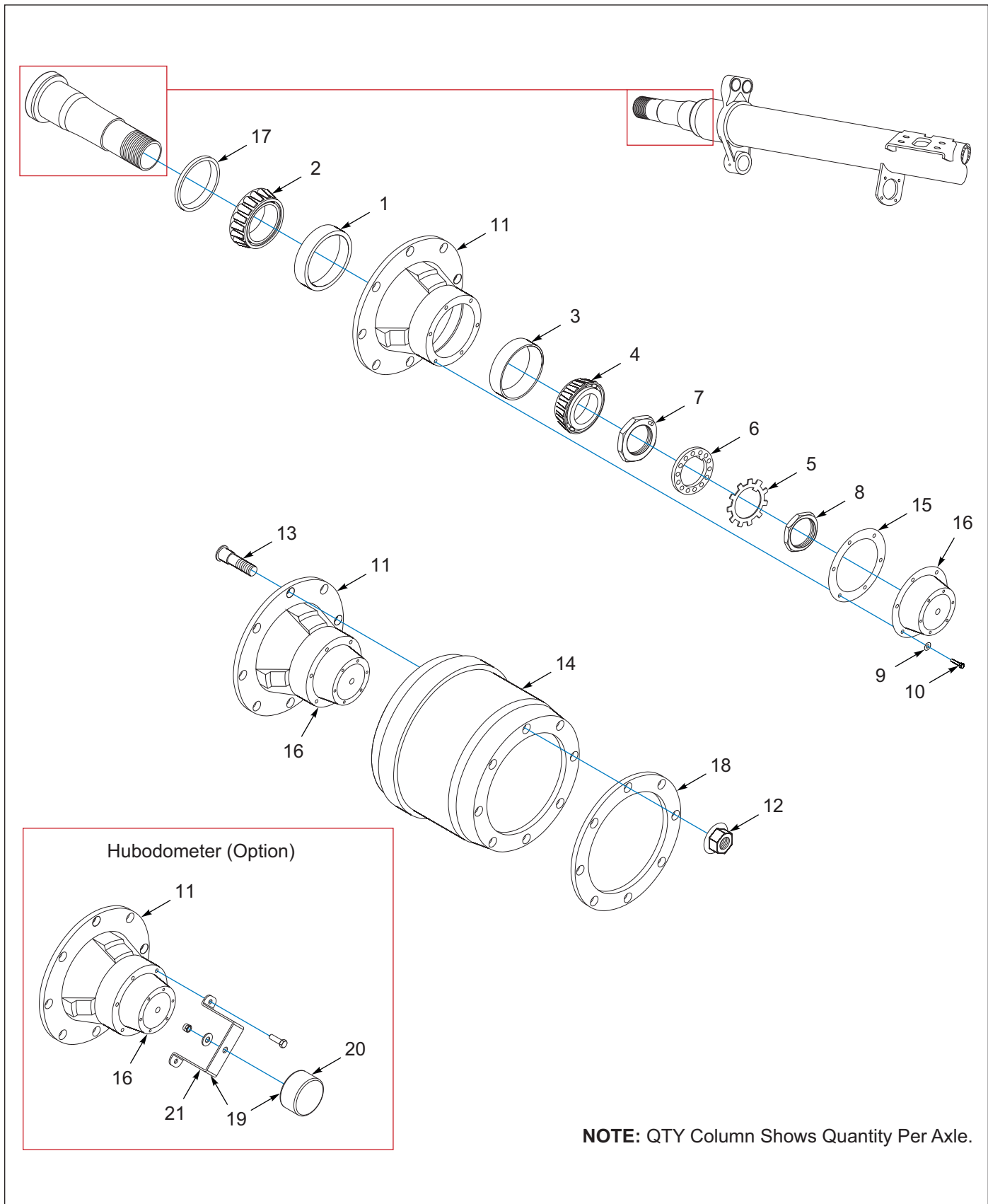
Figure 3-2: Axle 12.25 x 7.50 Drum & Hub Components
