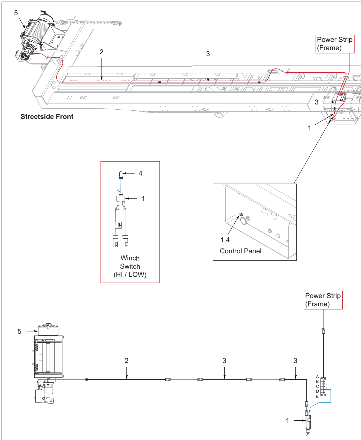
Figure 9-21: Winch Install, Warn 20K, 2 Speed, Spring Tension
