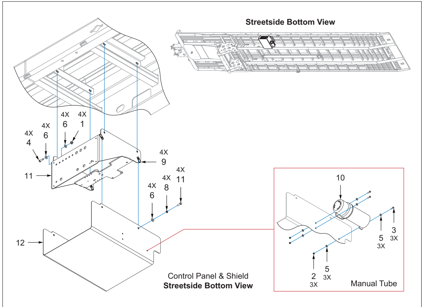
Figure 2-4: Control Panel, Shield & Manual Tube
