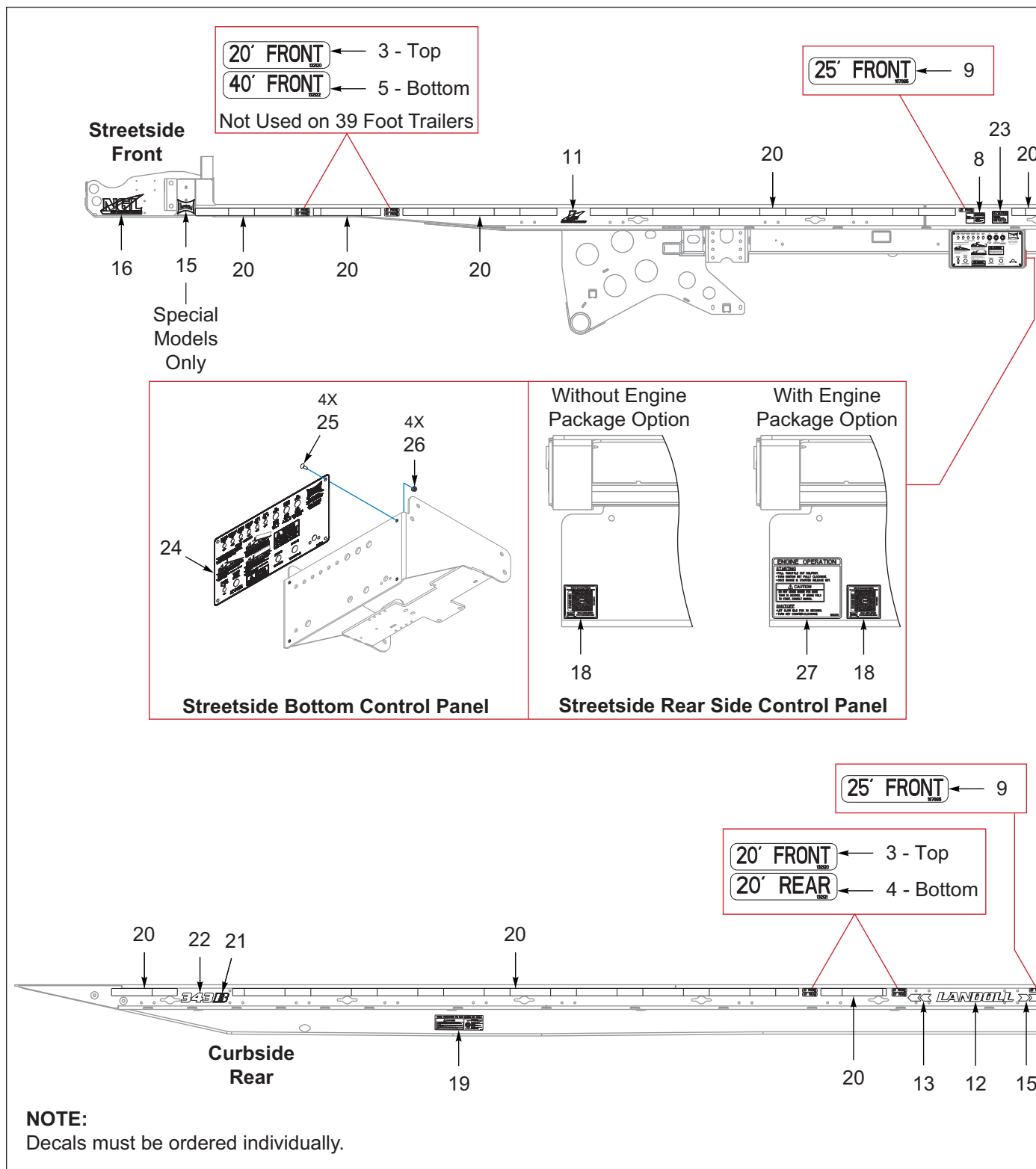
Figure 1-1: Frame Assembly (1 of 3)
