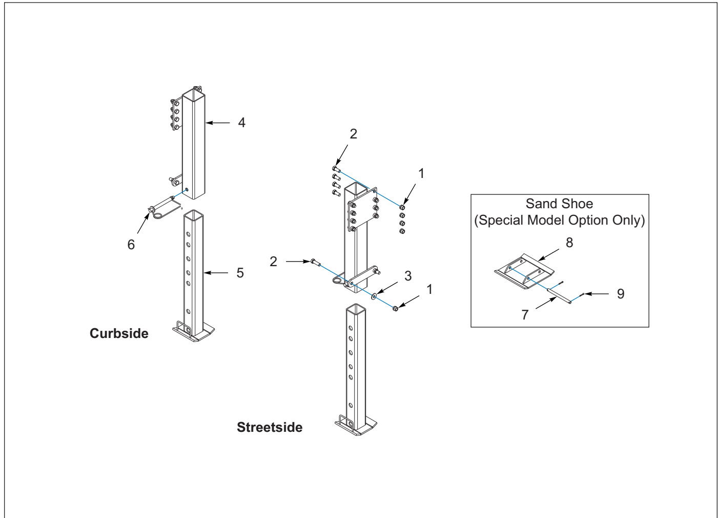
Figure 2-15: Landing Legs, Pinned (Option)
