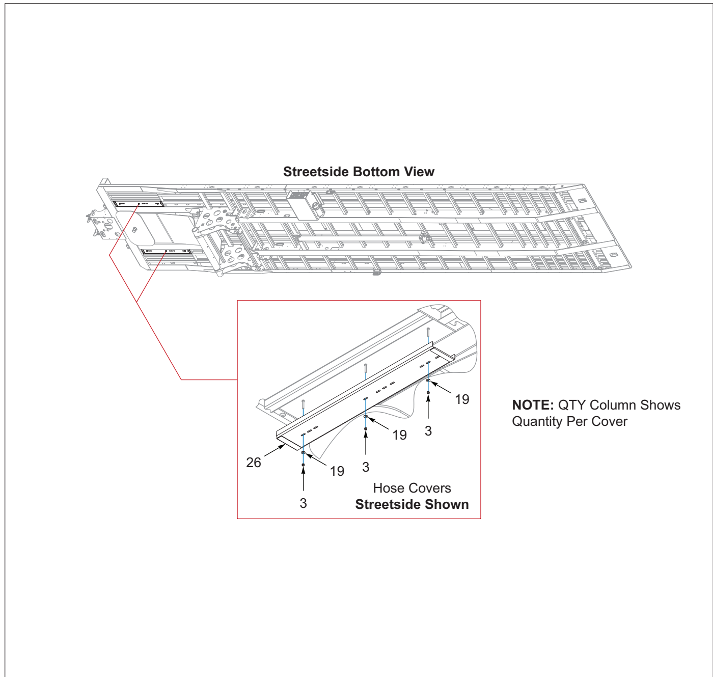
Figure 2-5: Covers, Hose
