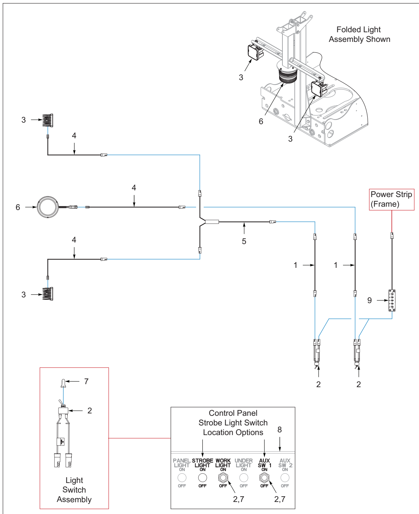
Figure 9-11: Light Stand, Folding, Strobe Beacon & Work Lights (Option)
