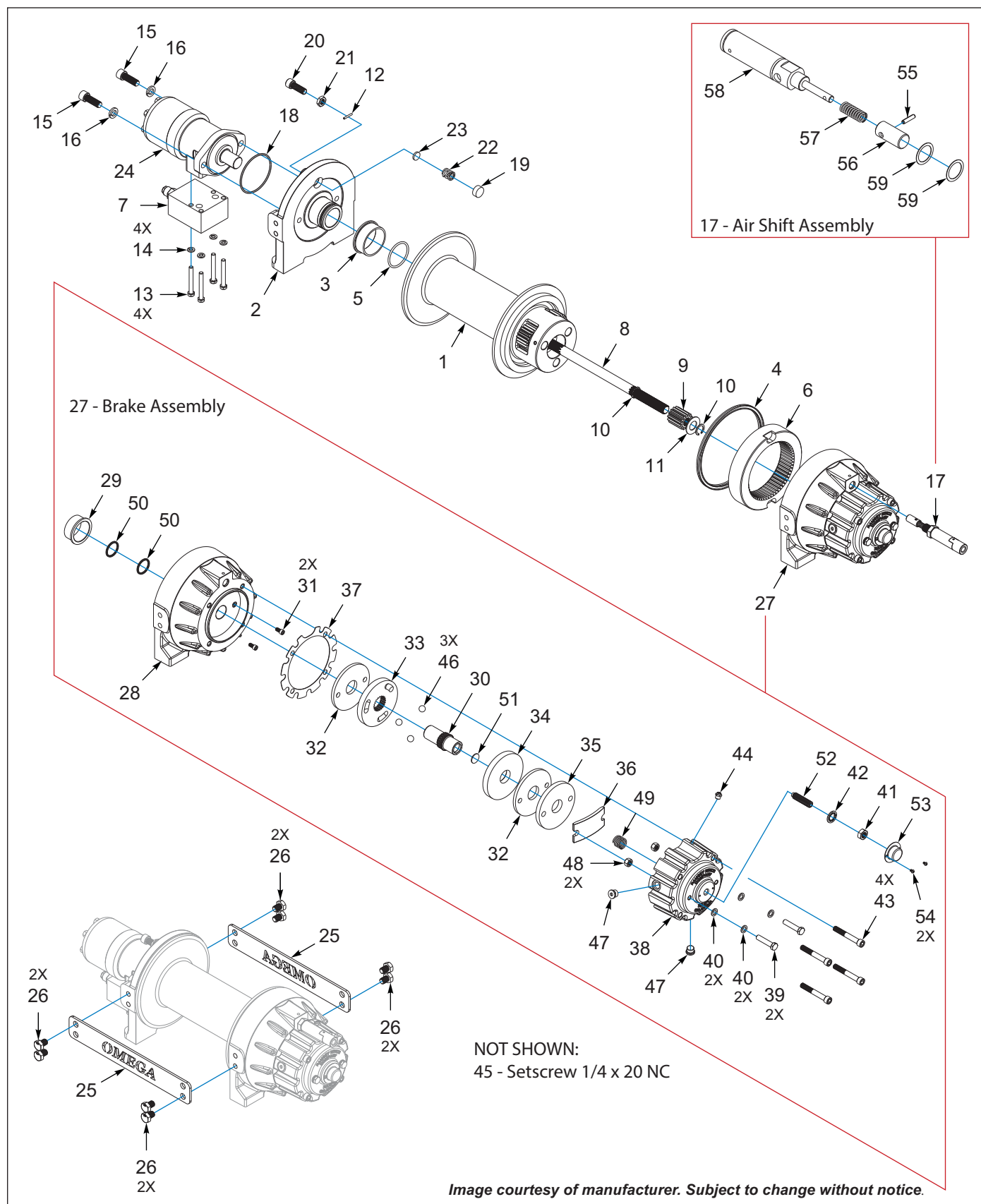
Figure 6-8: Winch Components, Ramsey 12K, 1 Speed, Spring Tension
