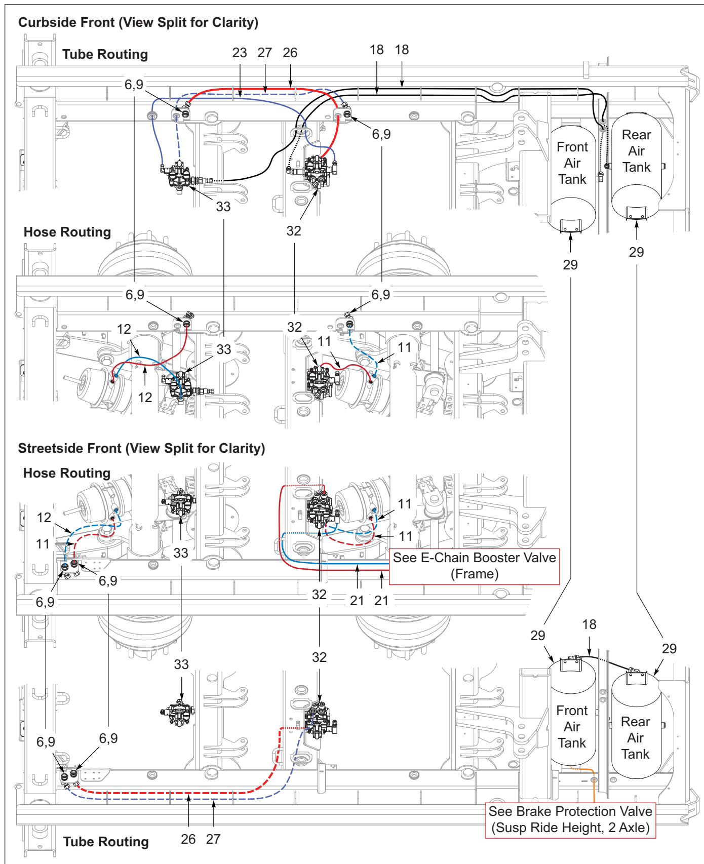
Figure 8-5: Anti-Lock Brakes, 2 Axle, Haldex (1 of 3)
