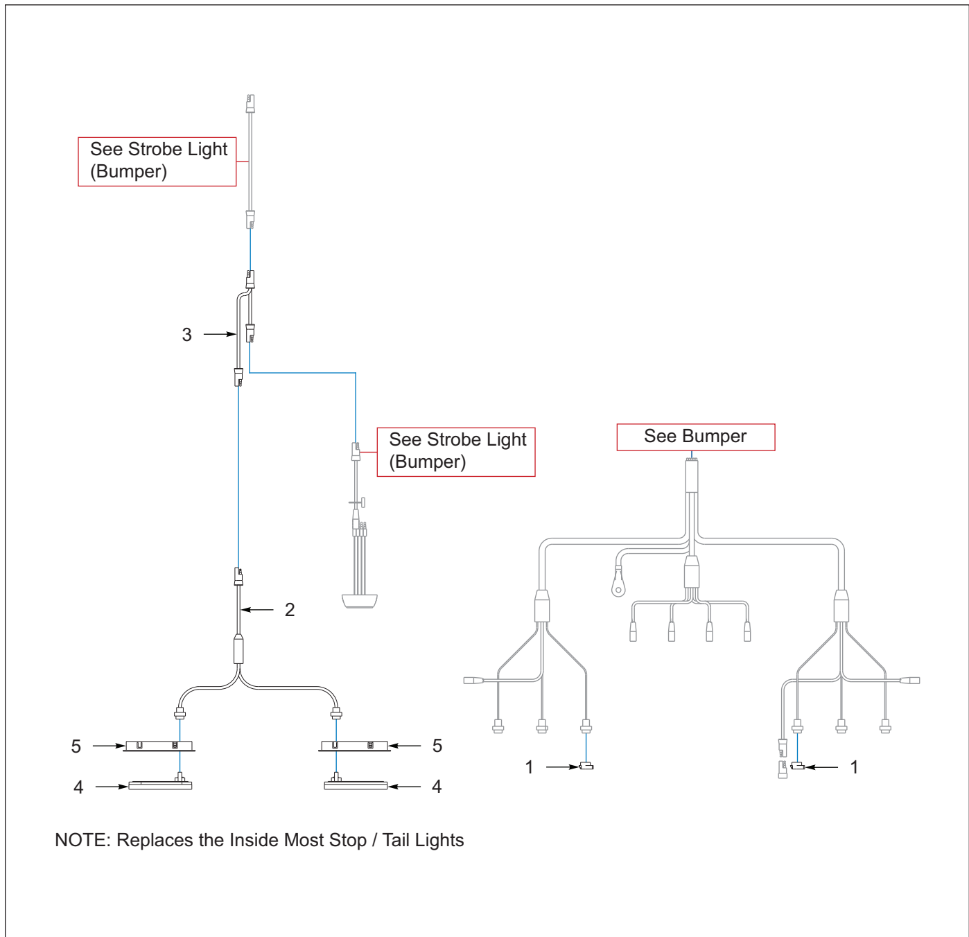
Figure 9-12: Lights, Strobe, Bumper (Option)
