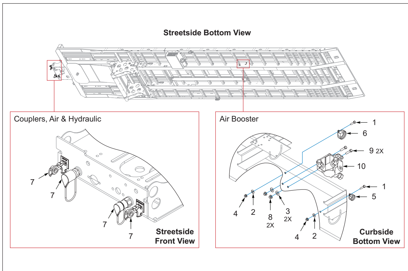
Figure 2-1: Air Booster, Air / Hydraulic Coupler
