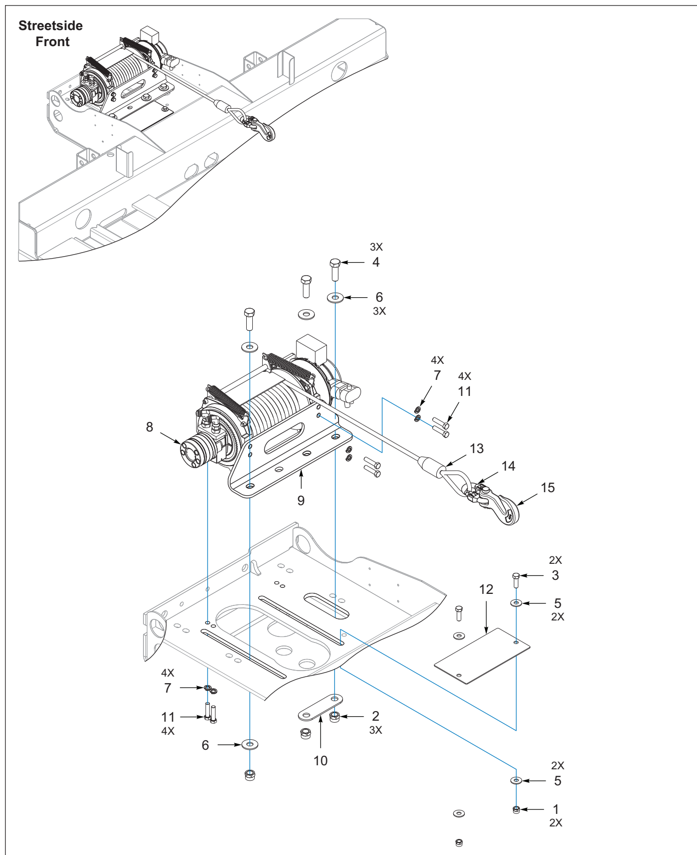
Figure 6-6: Winch Install, Warn 12K, 1 Speed, Spring Tension
