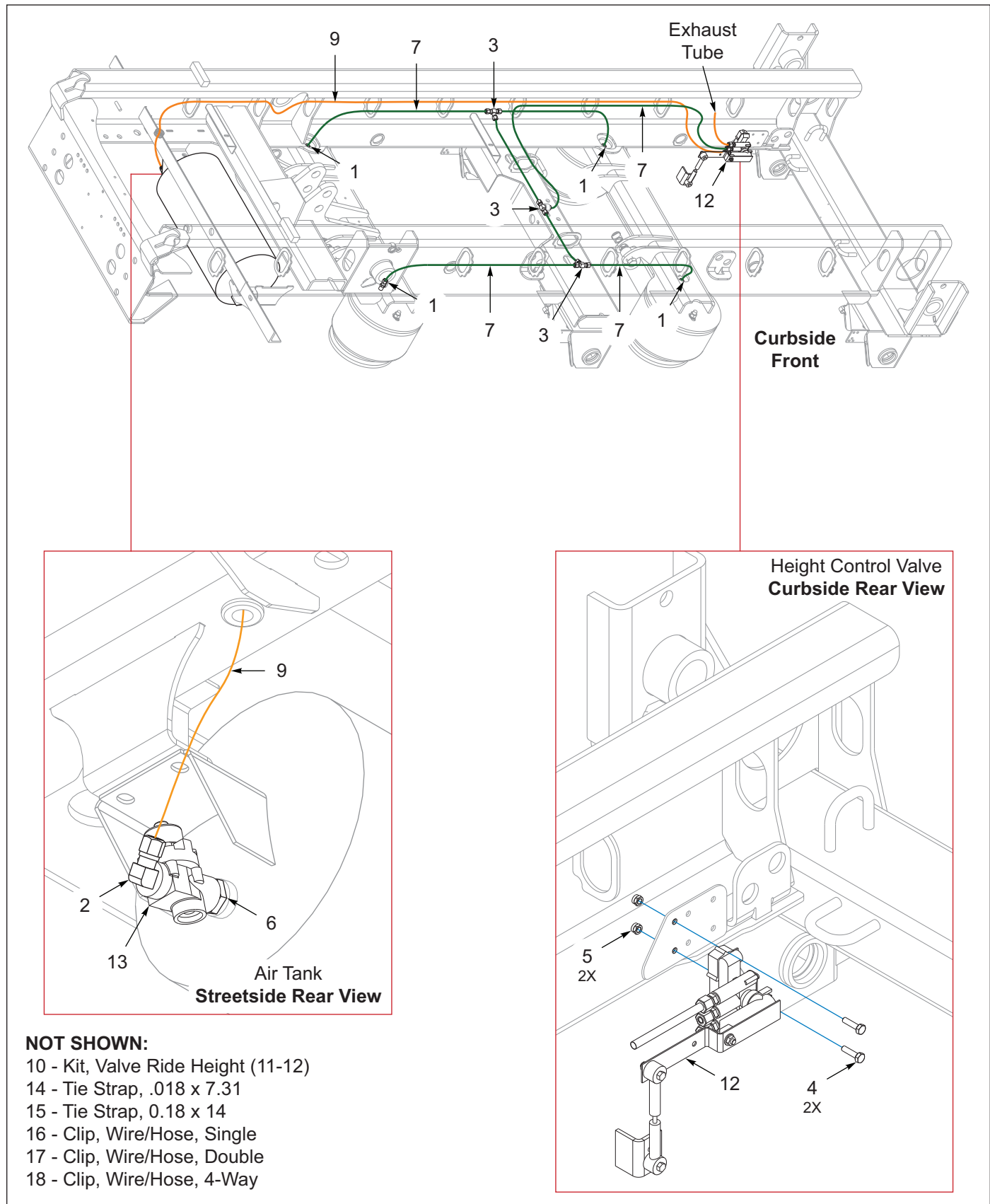
Figure 8-10: Suspension, Ride Height, 2 Axle (1 of 2)
