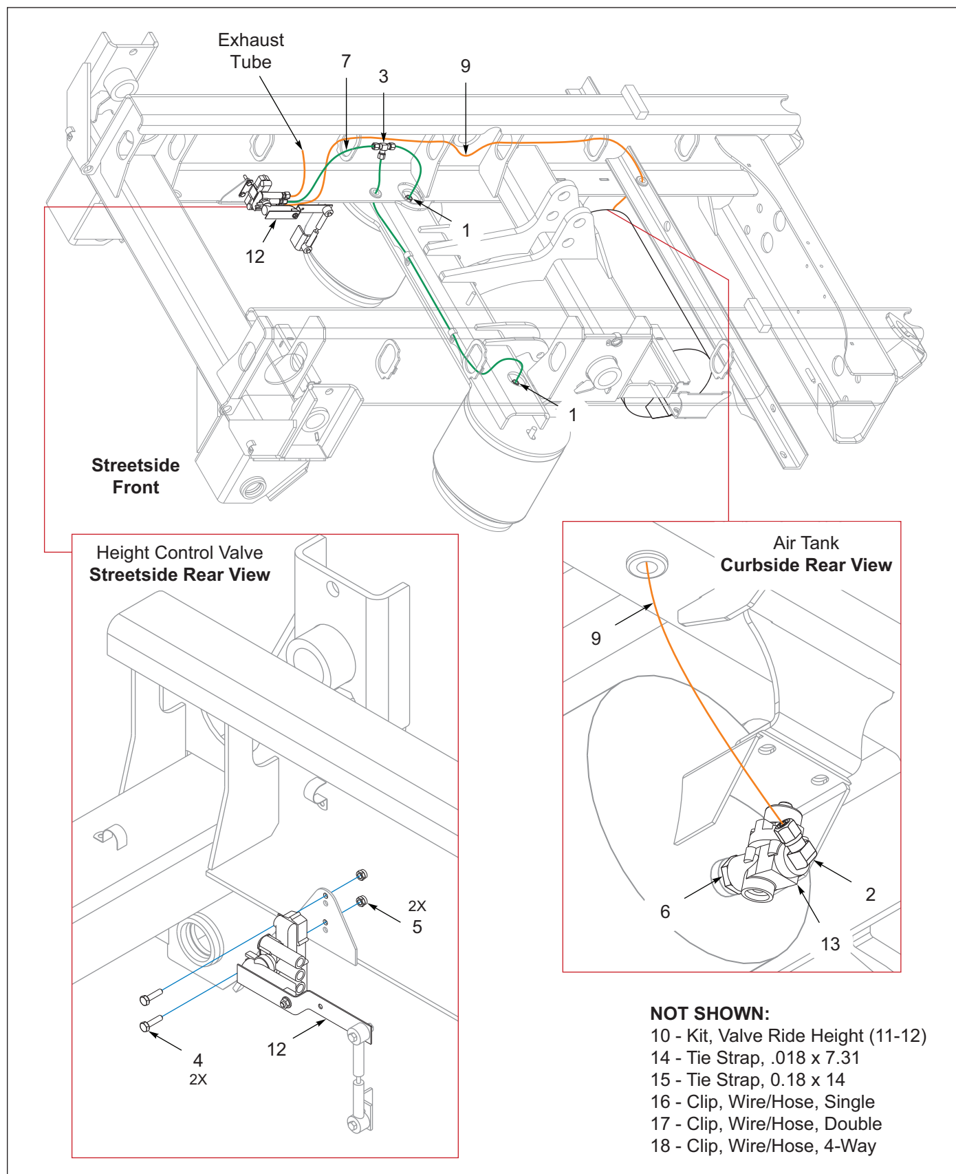
Figure 8-8: Suspension, Ride Height, 1 Axle (1 of 2)
