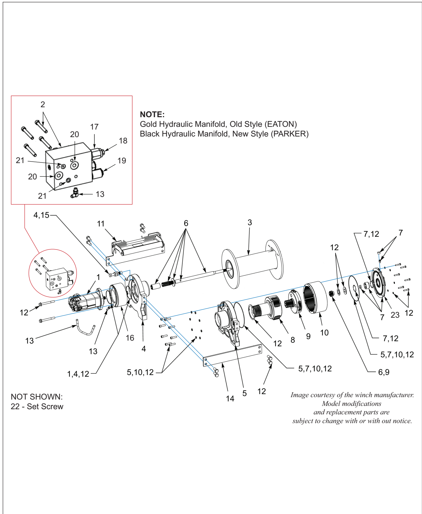
Figure 6-11: Winch Components, Warn 20K, 2 Speed, Spring Tension
