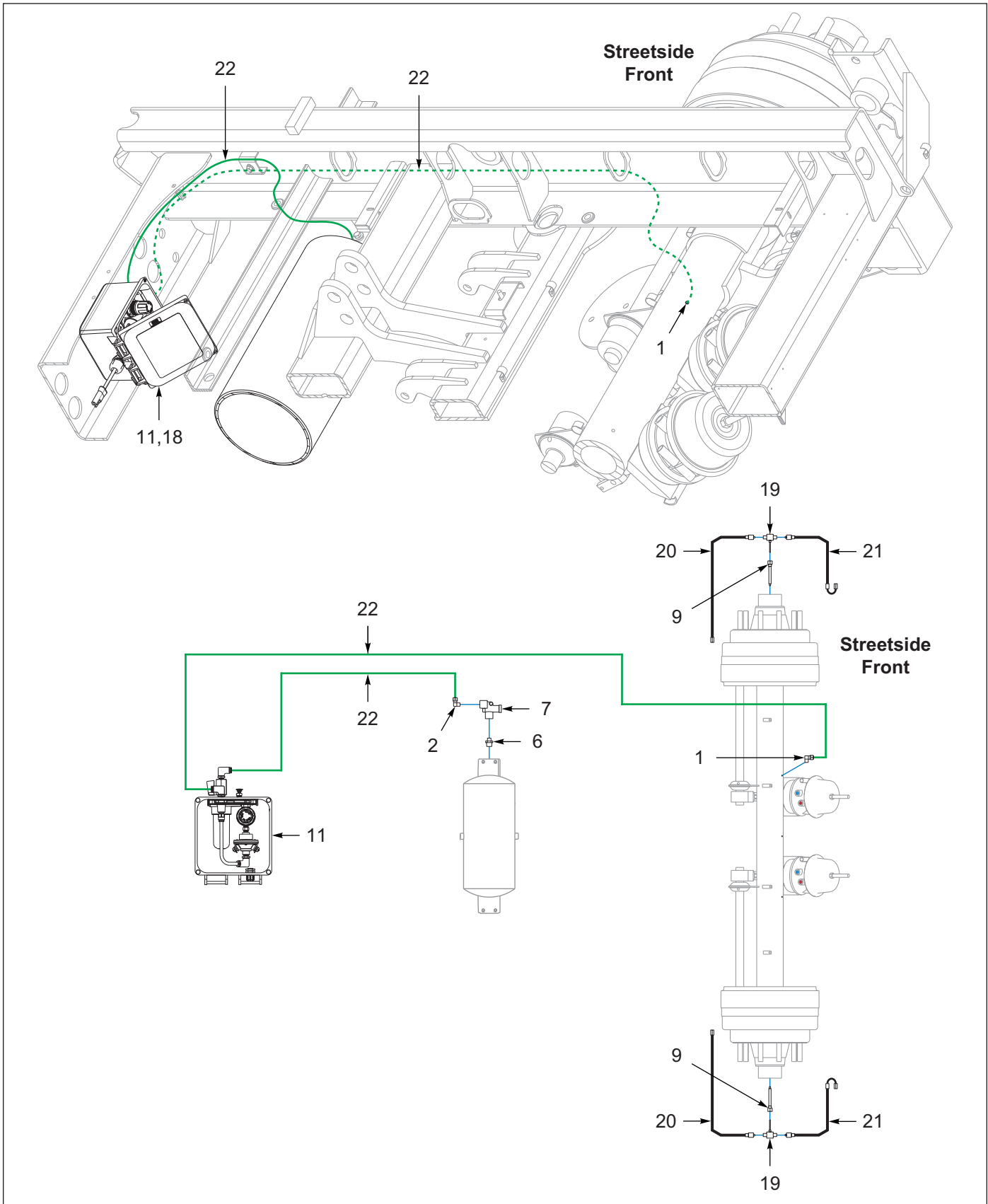
Figure 8-12: Tire Inflation, 1 Axle (1 of 2)
