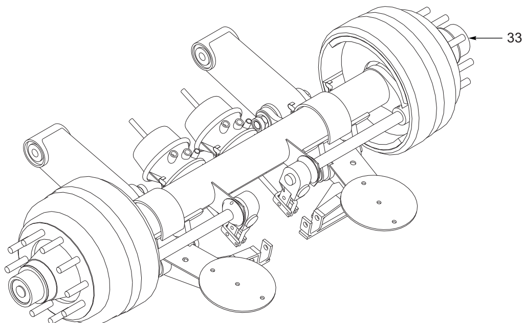
View of RLU-228-5.5, 16.5 x 7 Drum Brakes
