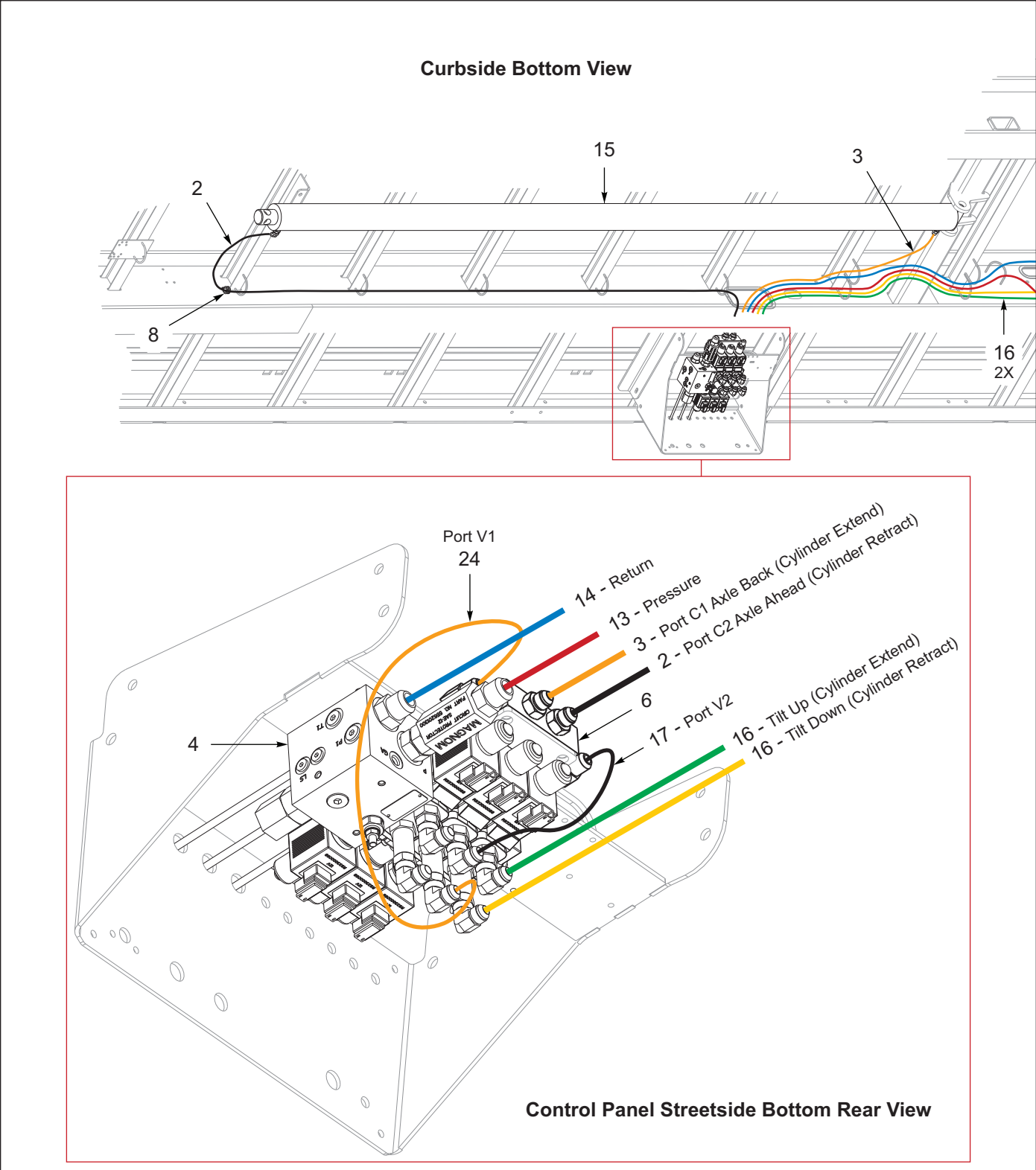
Figure 11-1: Frame, Hitch Tilt / Travel Axle (1 of 2)
