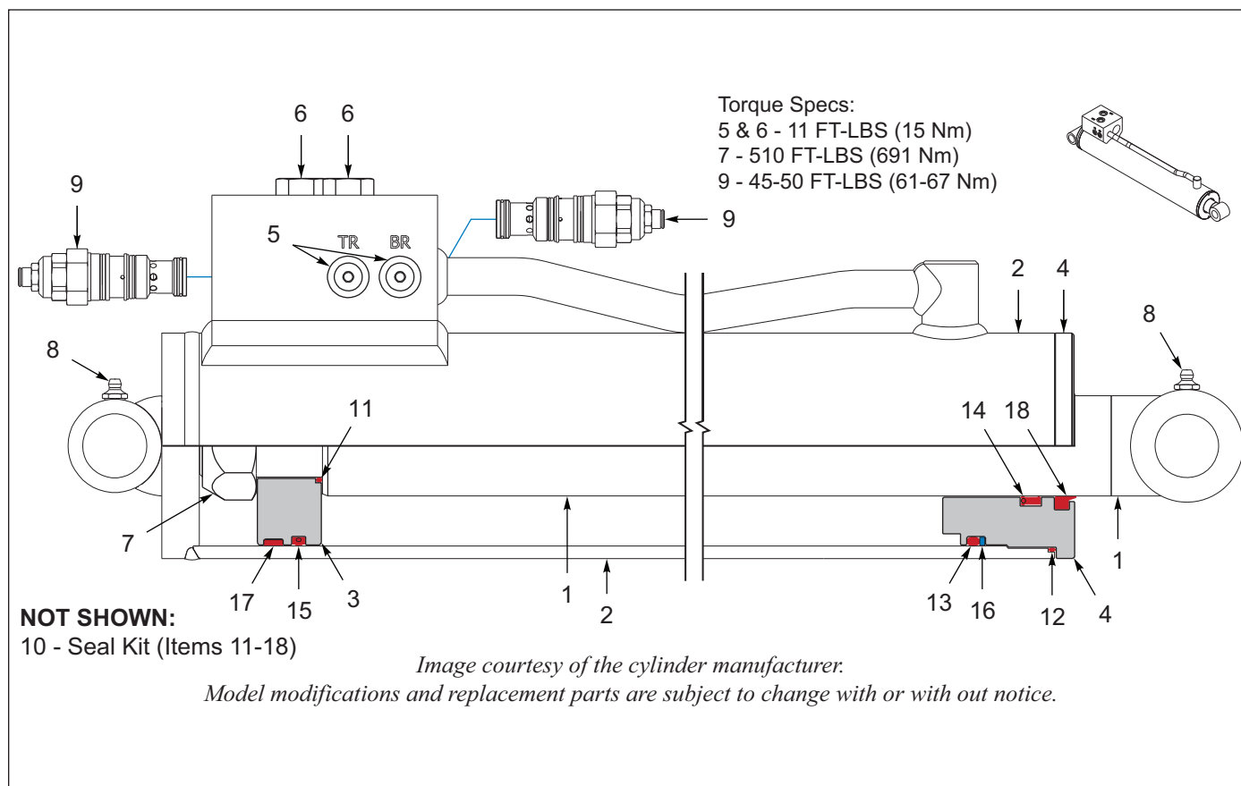
Figure 11-9: Cylinder Components, 4 x 20
