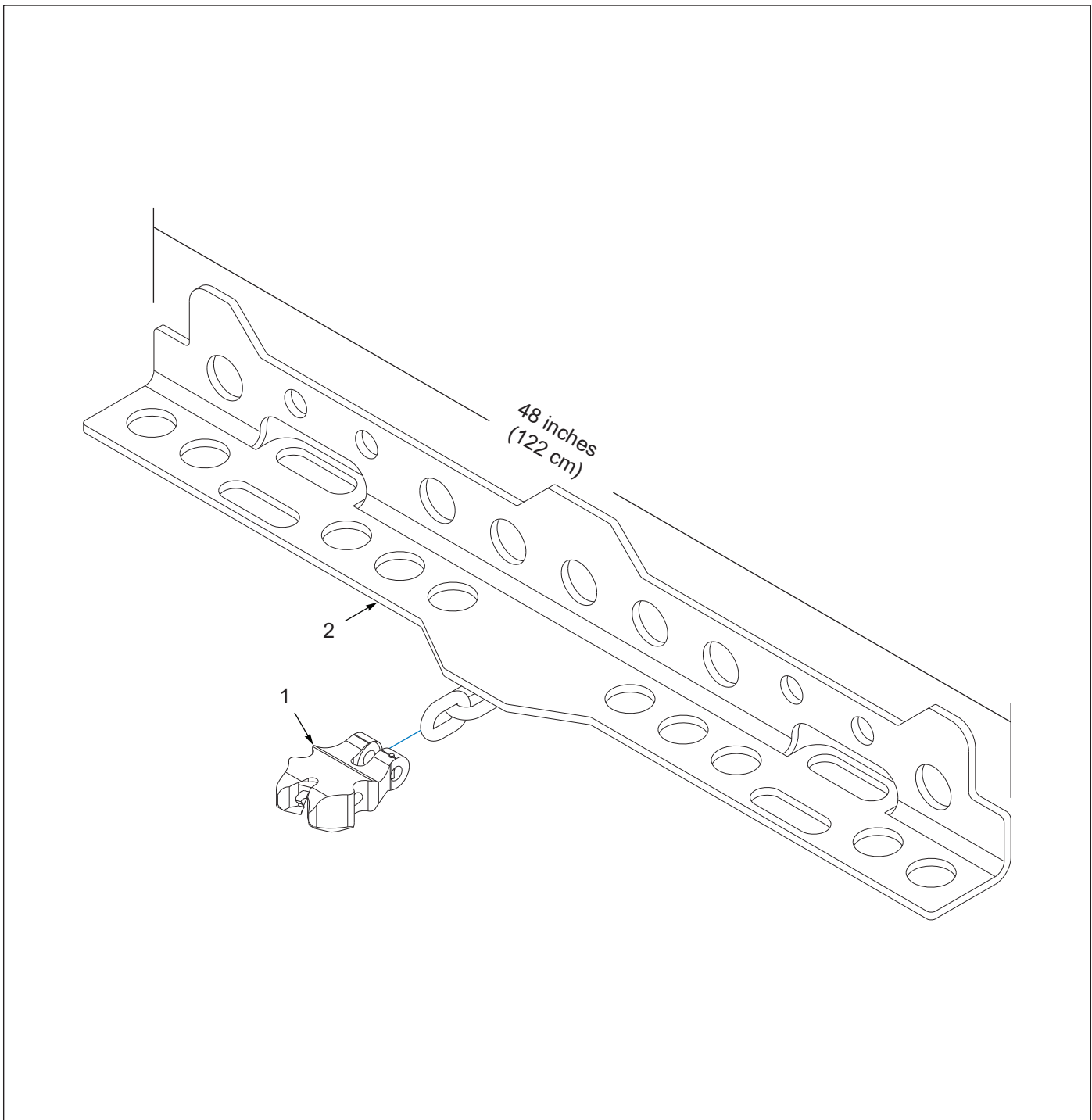
Figure 7-5: Container Pusher
