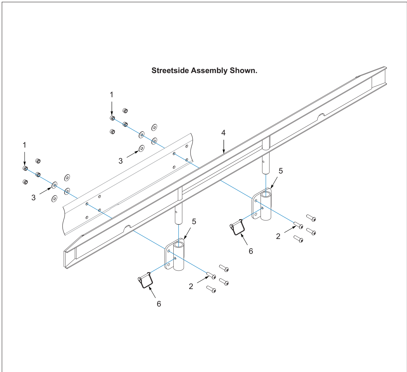
Figure 7-7: Container Side Guide, 88 Inch, Bolt On
