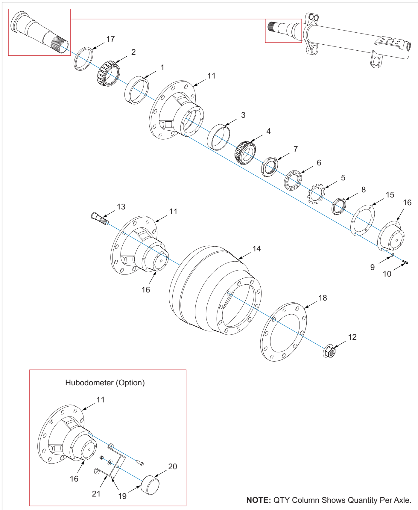
Figure 3-6: Axle 16.50 x 7.00 Drum & Hub Components
