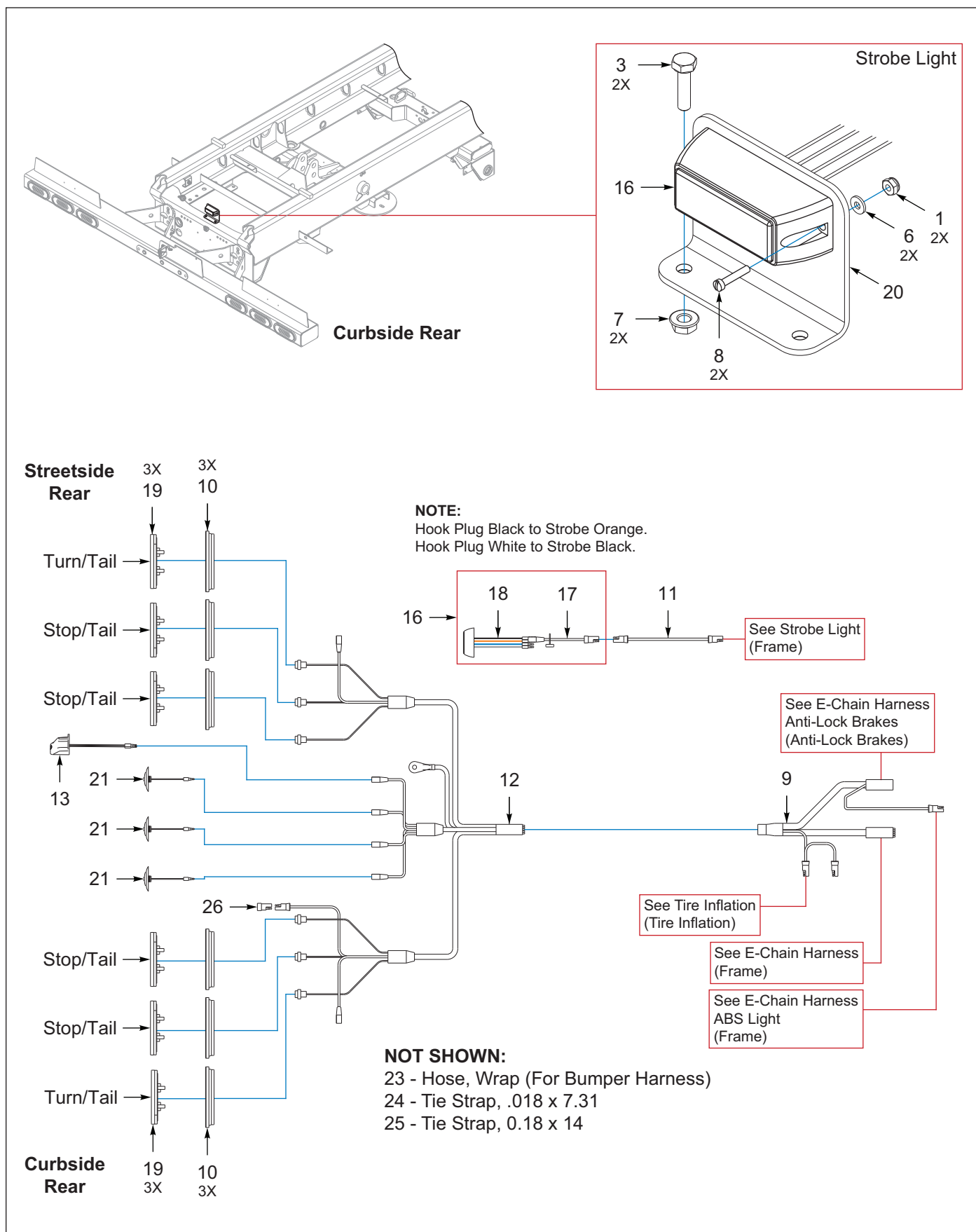
Figure 9-4: Bumper Assembly (2 of 2)
