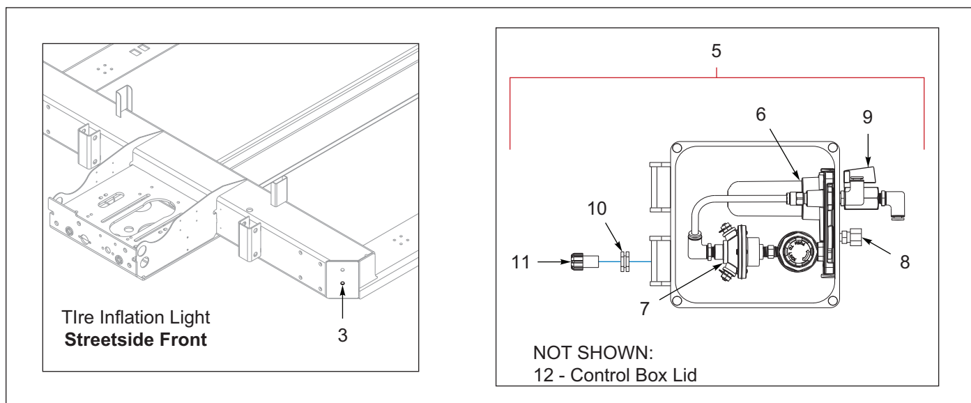
Figure 9-19: Tire Inflation, 2 Axle (2 of 2)
