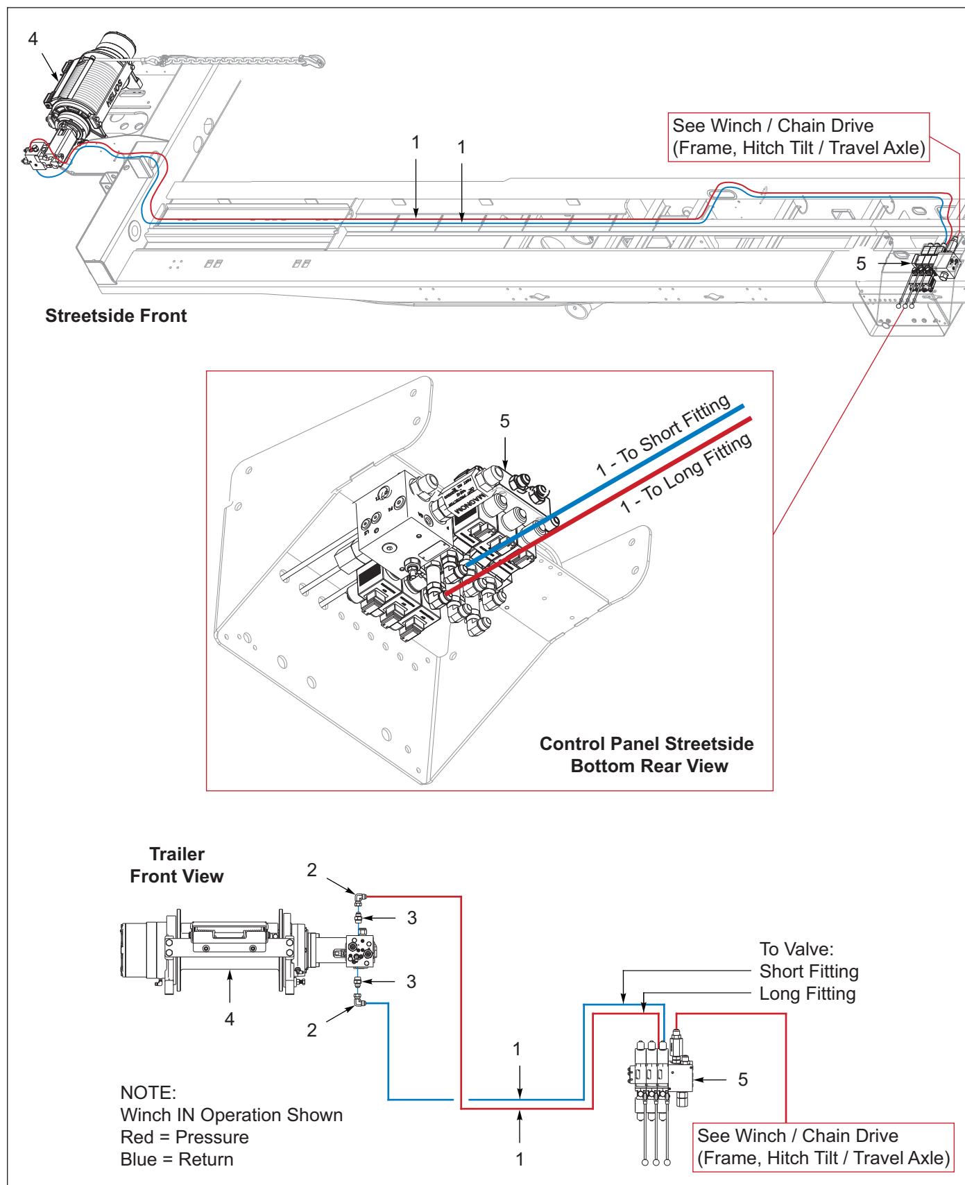
Figure 11-5: Winch Install, Ramsey 20K, 2 Speed, Spring Tension
