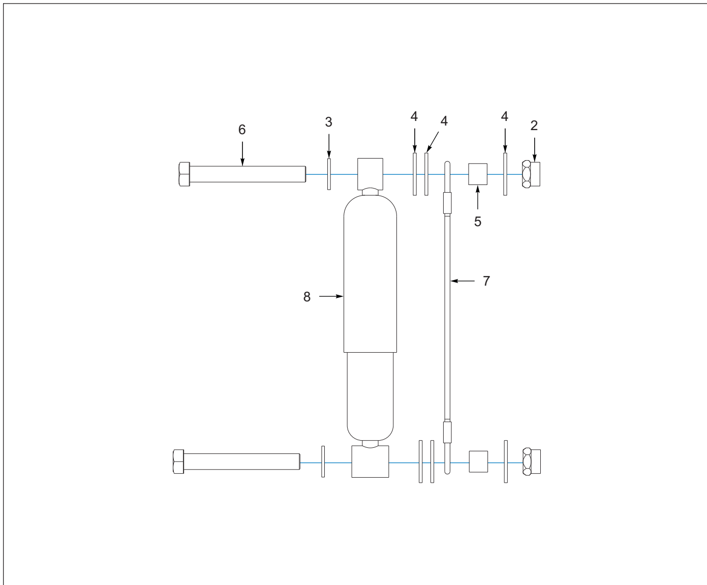
Figure 3-17: Shock Strap, Limit, LSS-25K-5.5 (Option)
