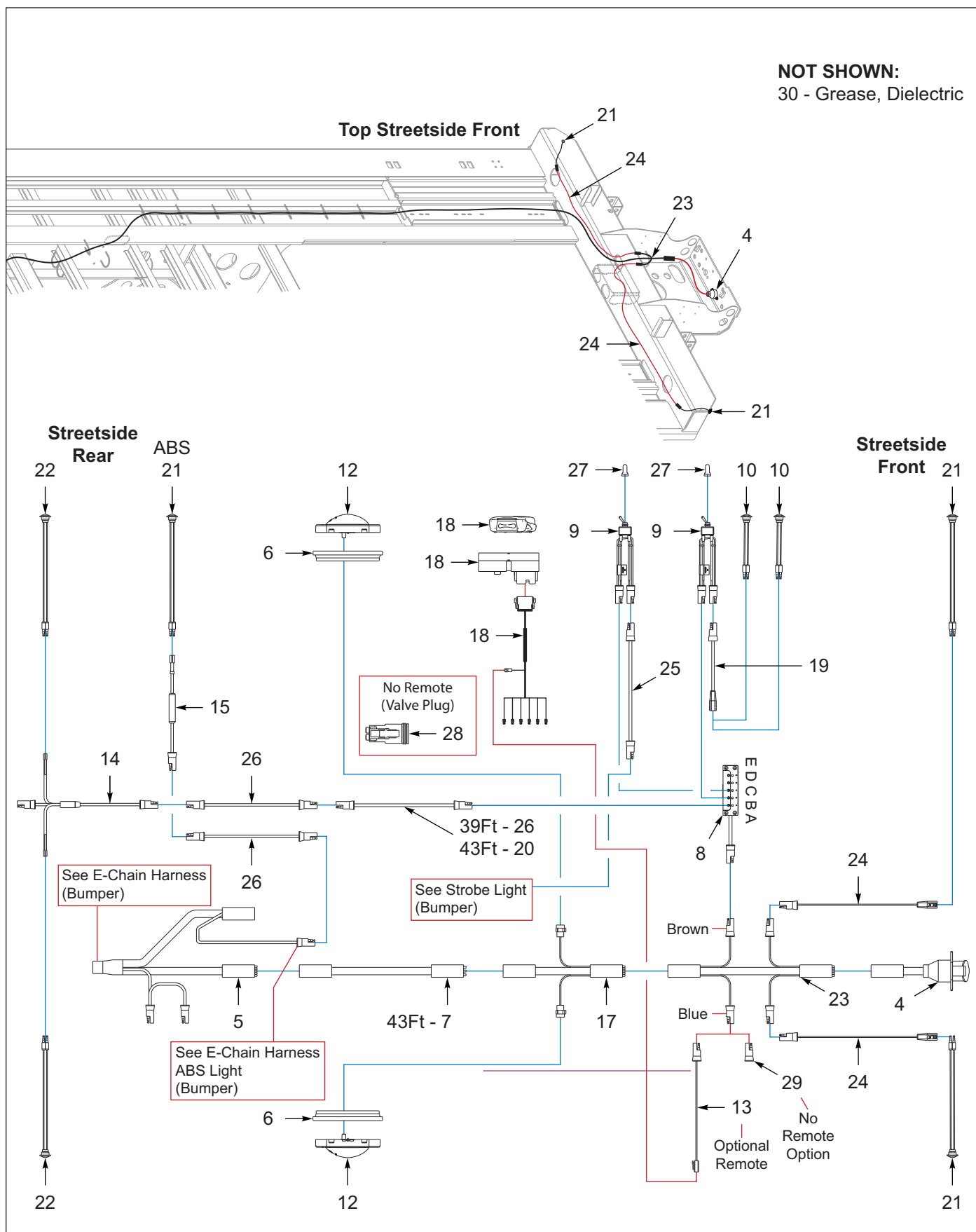
Figure 9-2: Frame, Control Panel & Marker Lights (2 of 2)
