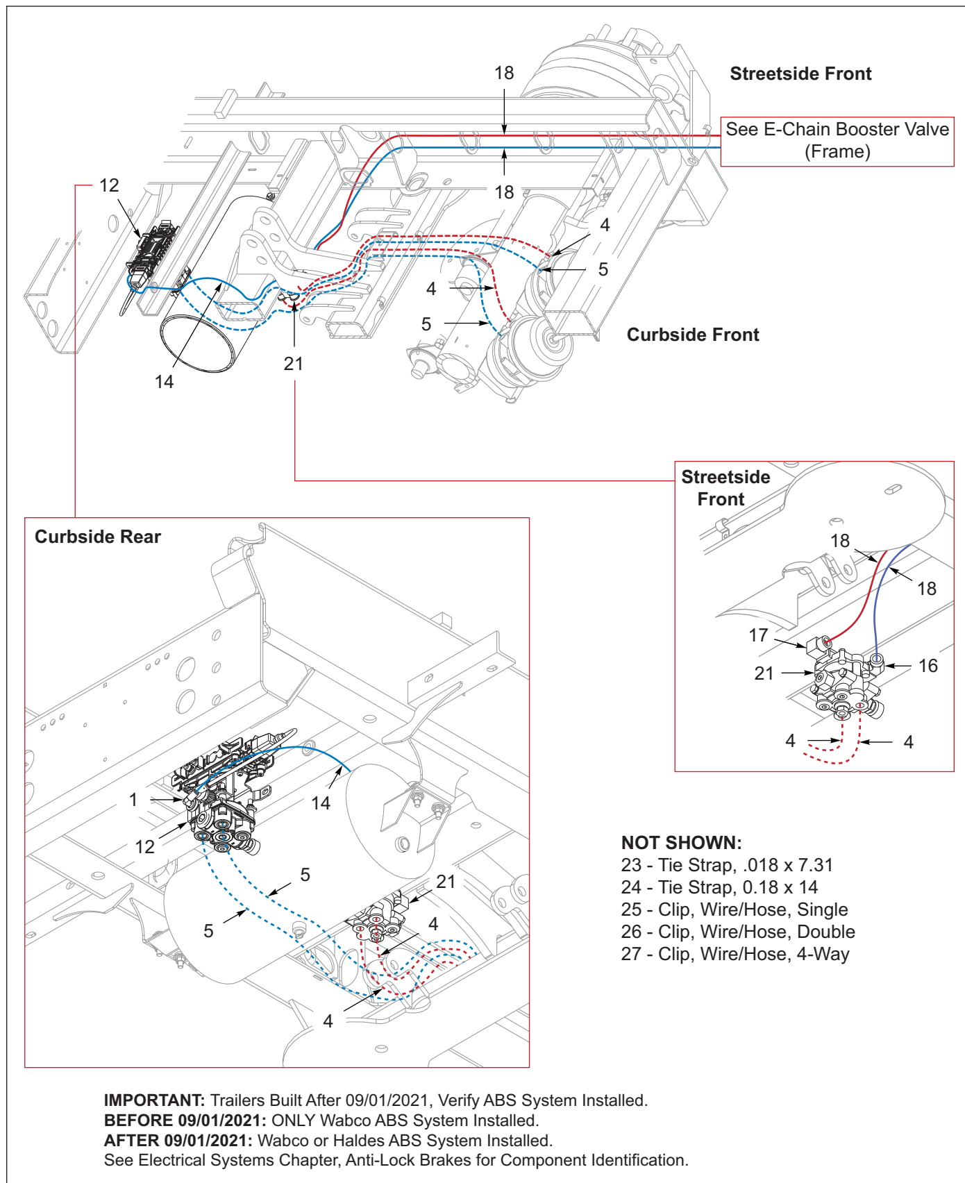
Figure 8-3: Anti-Lock Brakes, 1 Axle, Wabco (1 of 2)
