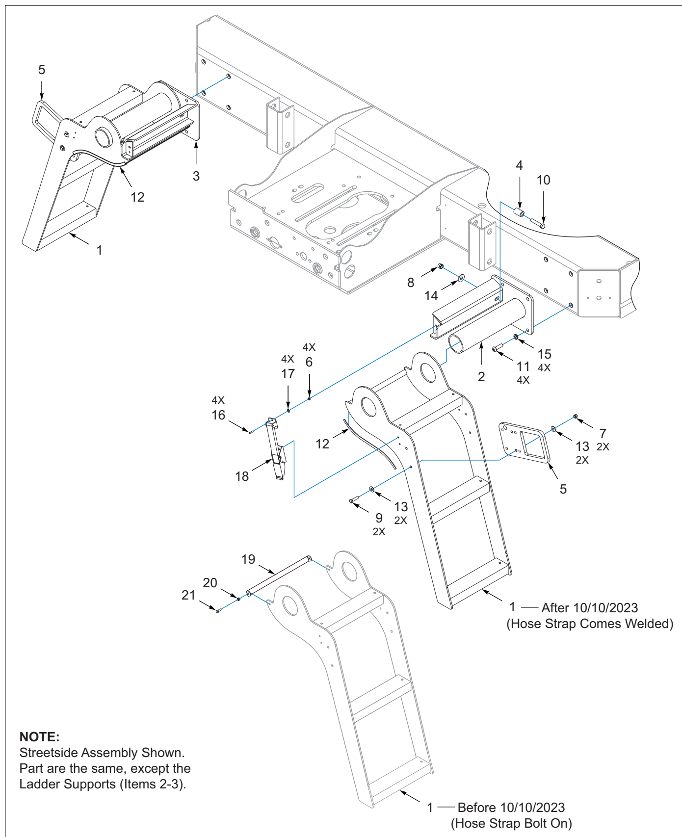
Figure 4-5: Ladder Assembly, Pivoting
