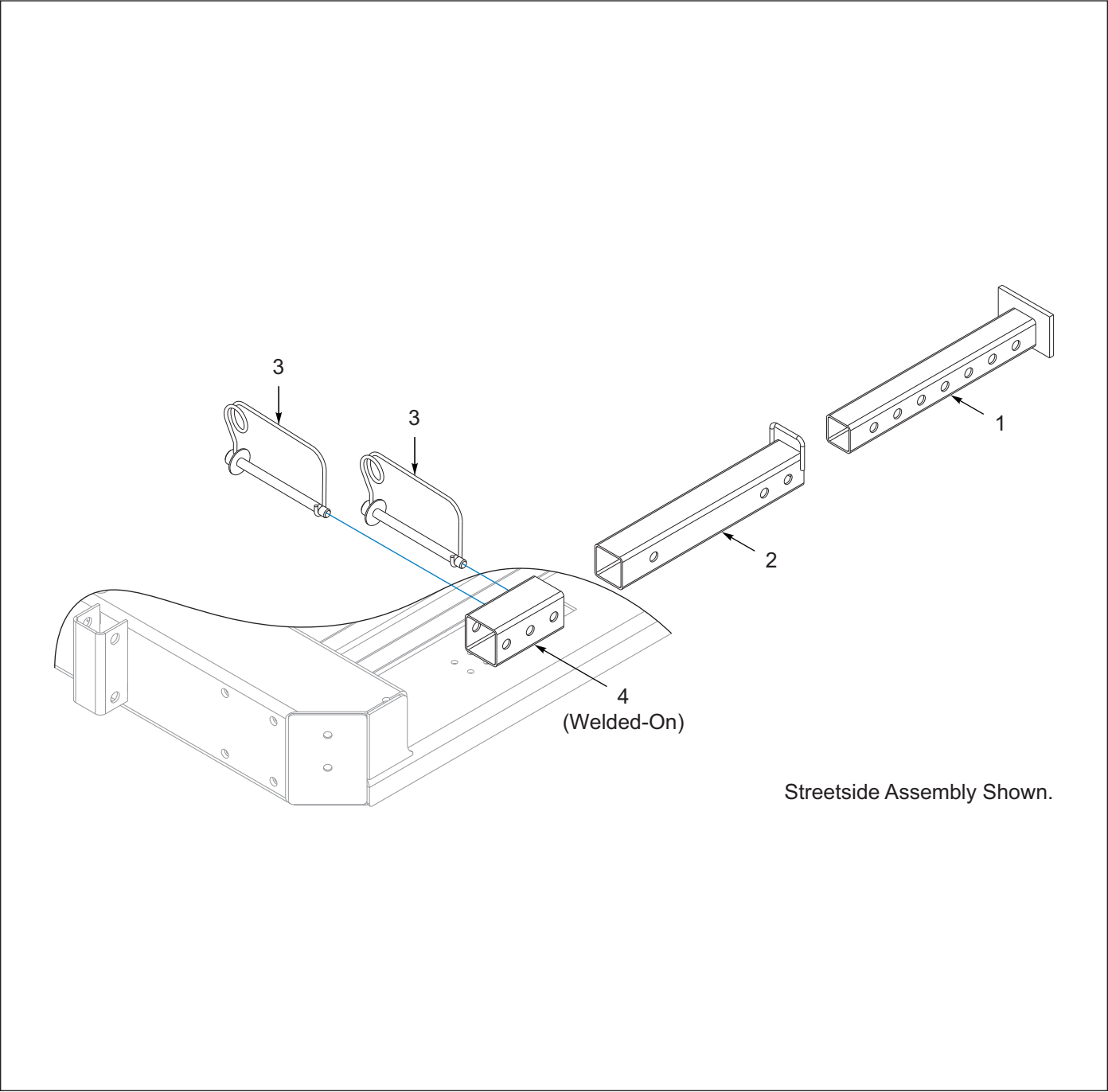
Figure 7-8: Container Stop, Front, Adjustable
