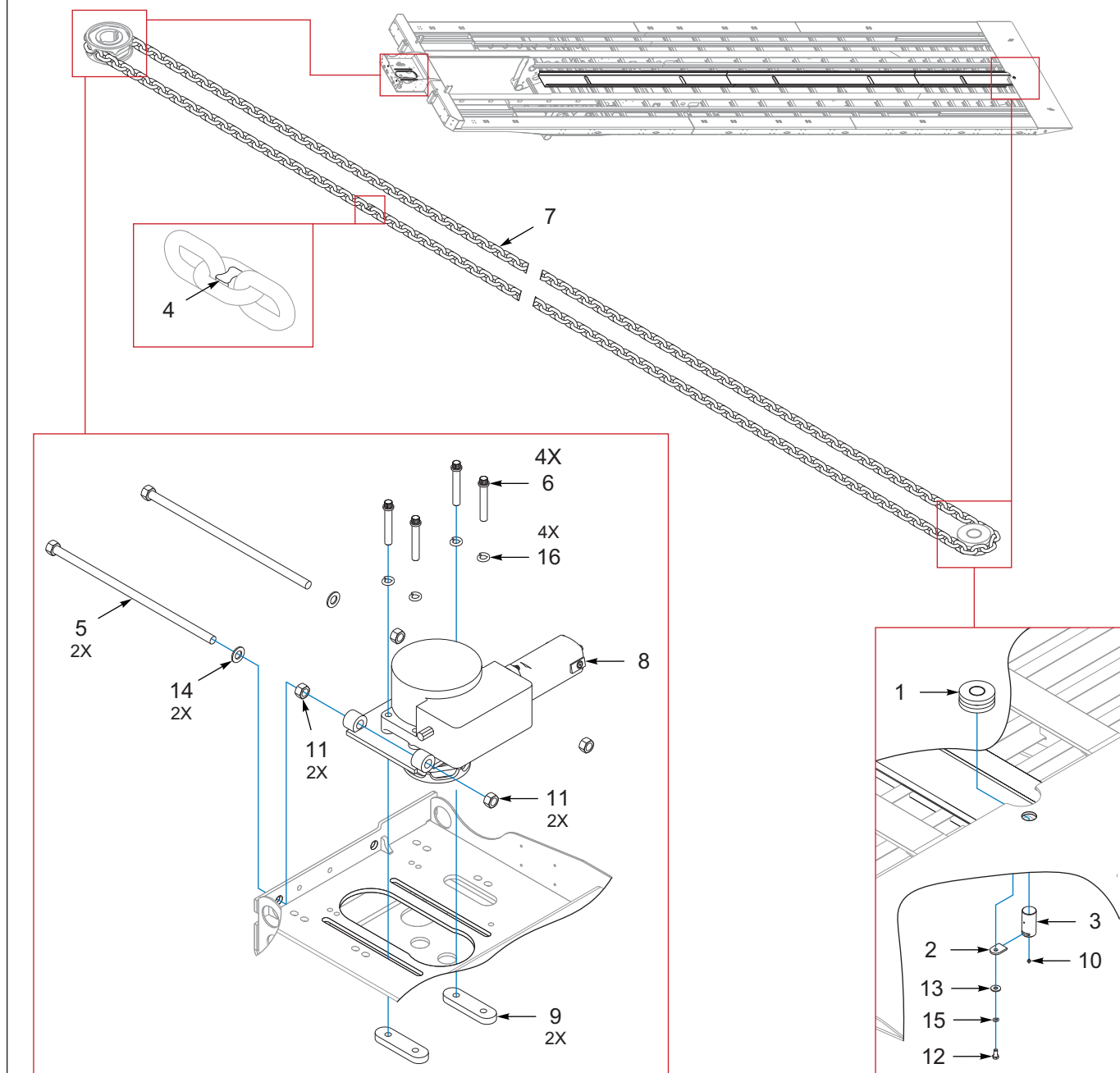
Figure 6-1: Chain Drive Install, 1 Speed
