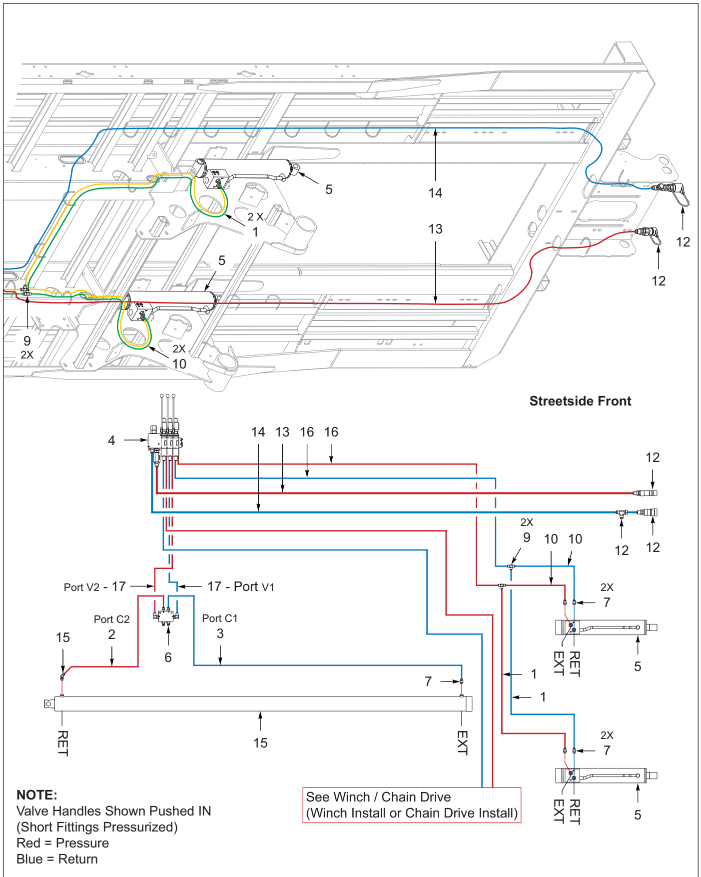
Figure 11-2: Frame, Hitch Tilt / Travel Axle (2 of 2)
