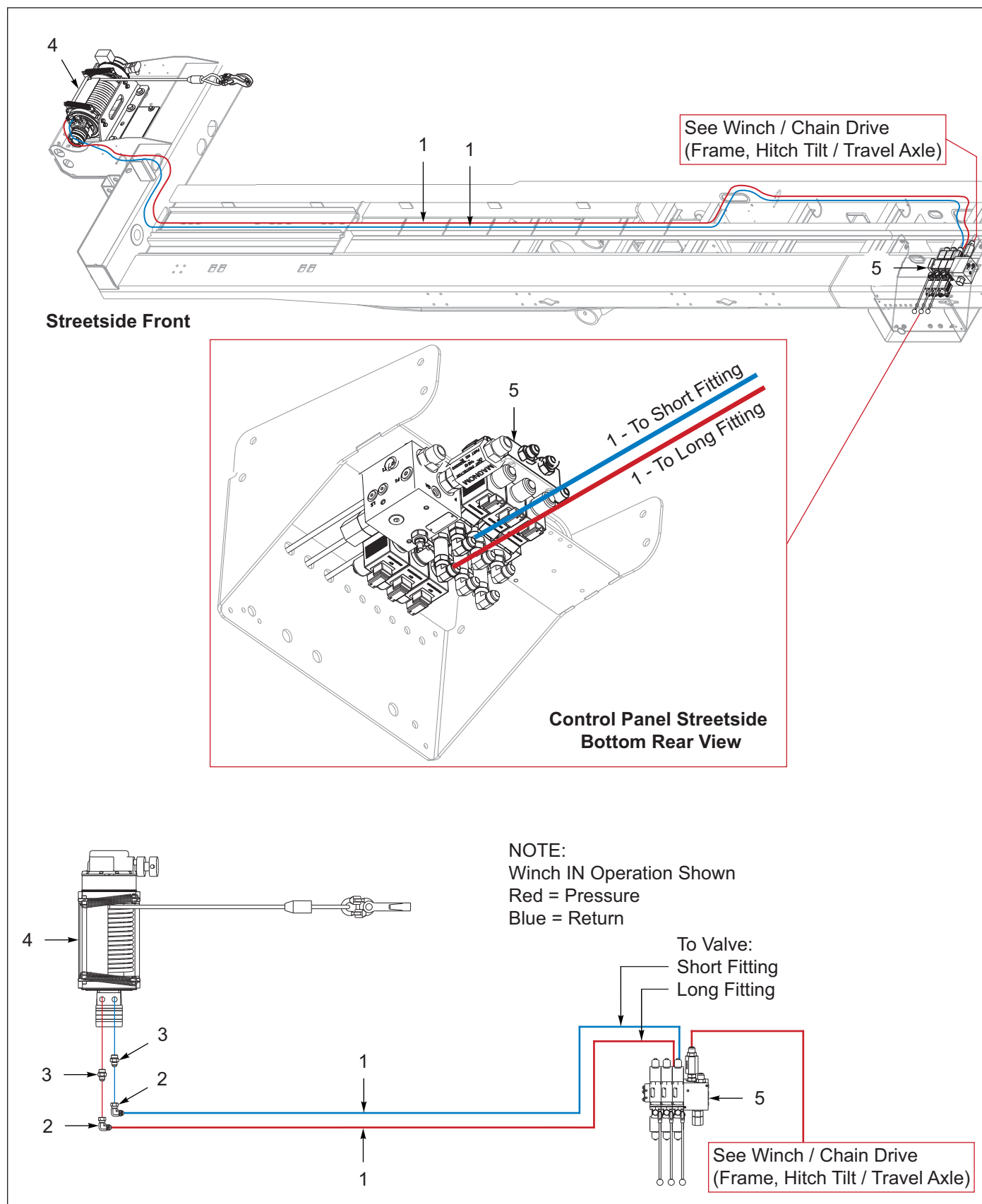
Figure 11-6: Winch Install, Warn 12K, 1 Speed, Spring Tension
