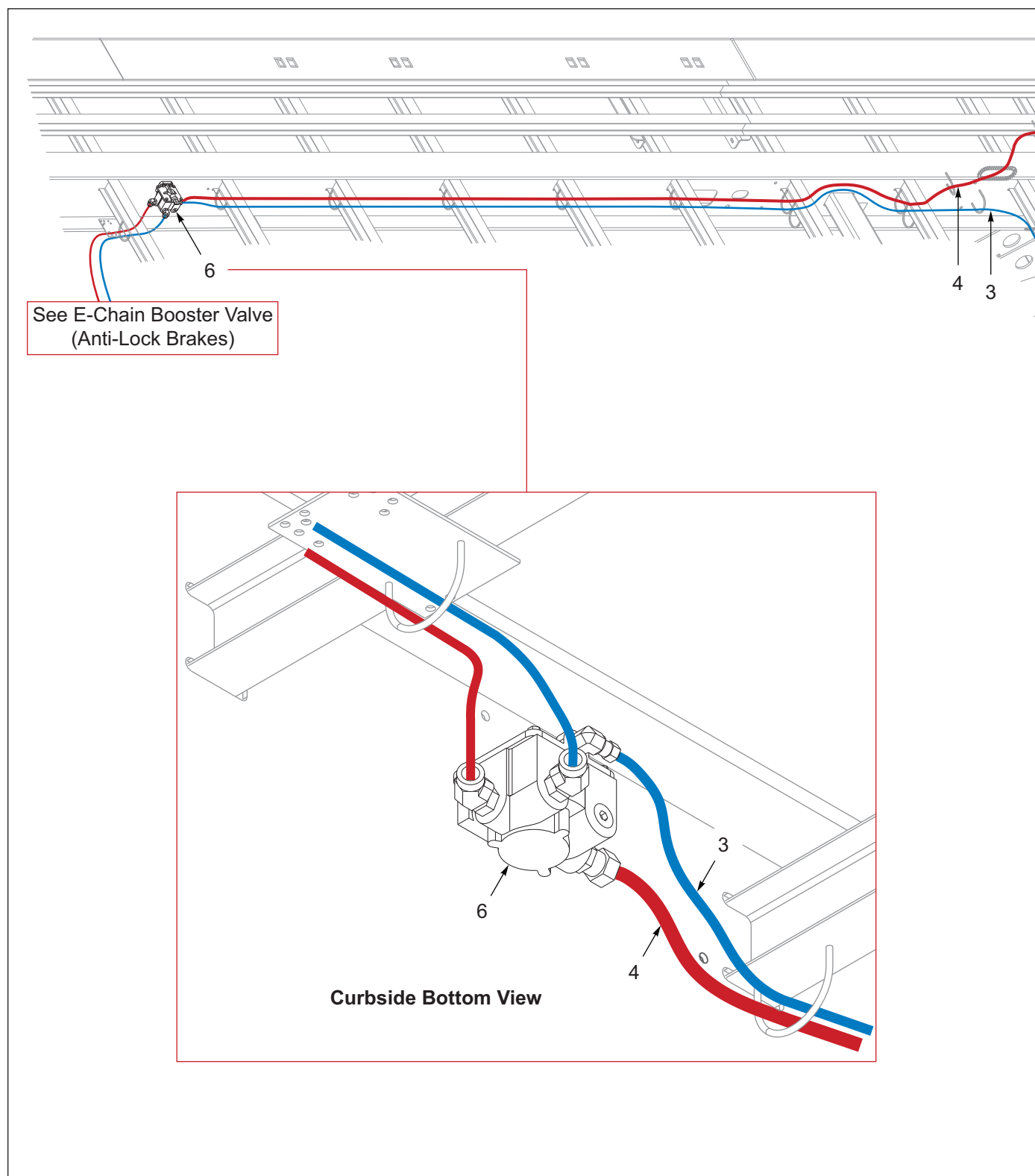
Figure 8-1: Frame, Service & Emergency (1 of 2)
