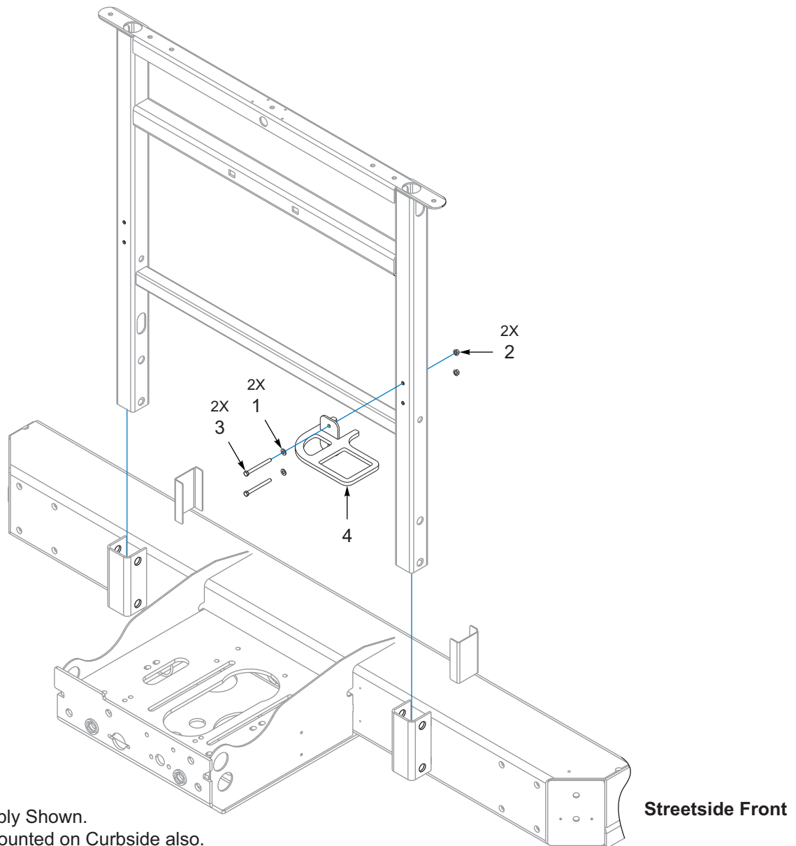
Figure 4-3: Bulkhead, Grab Handle, Accessory Rack
