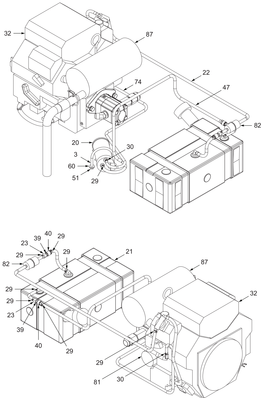
Figure 5-4: Engine Package, 25 HP, Upper Deck Assembly (4 of 5)
