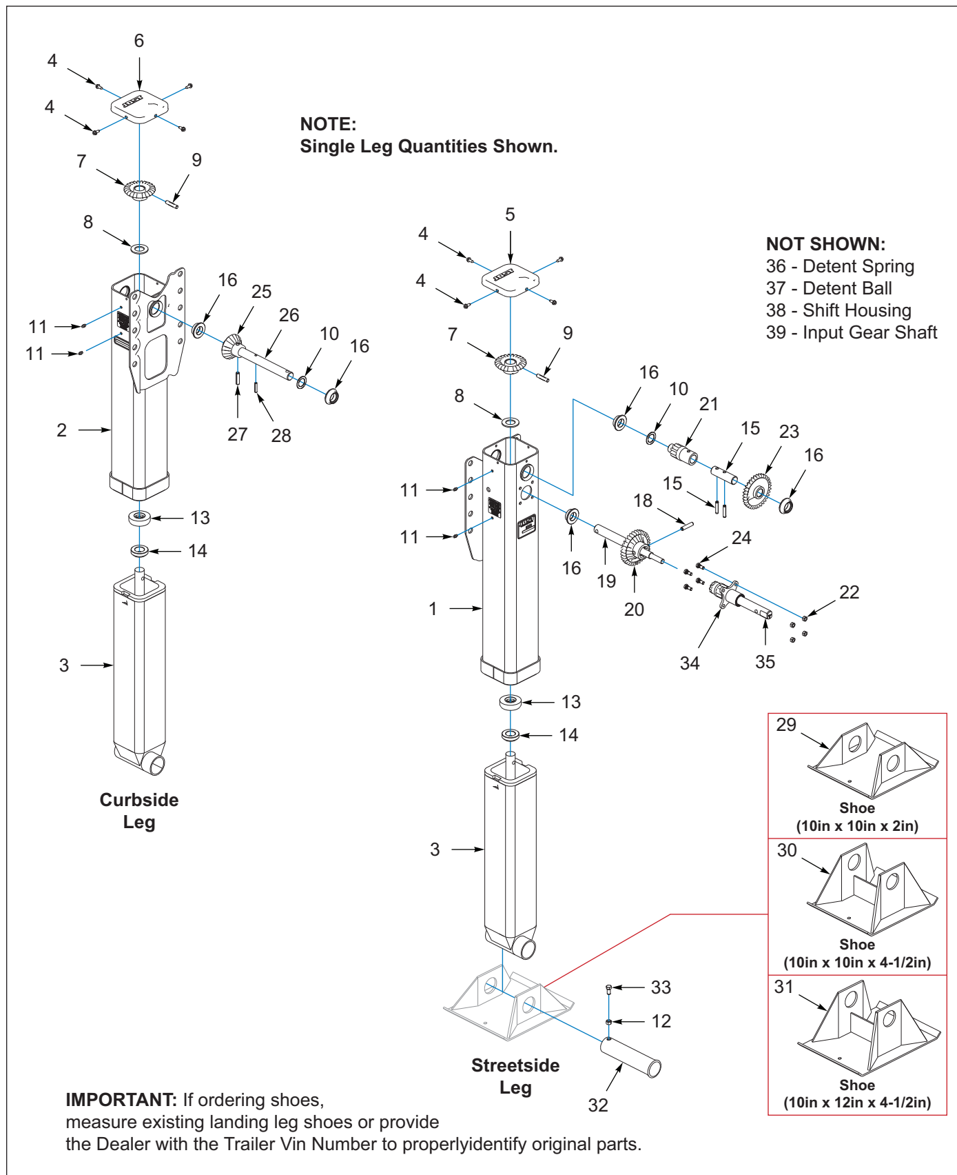
Figure 2-16: Landing Leg Components, Gear, 2 Spd
