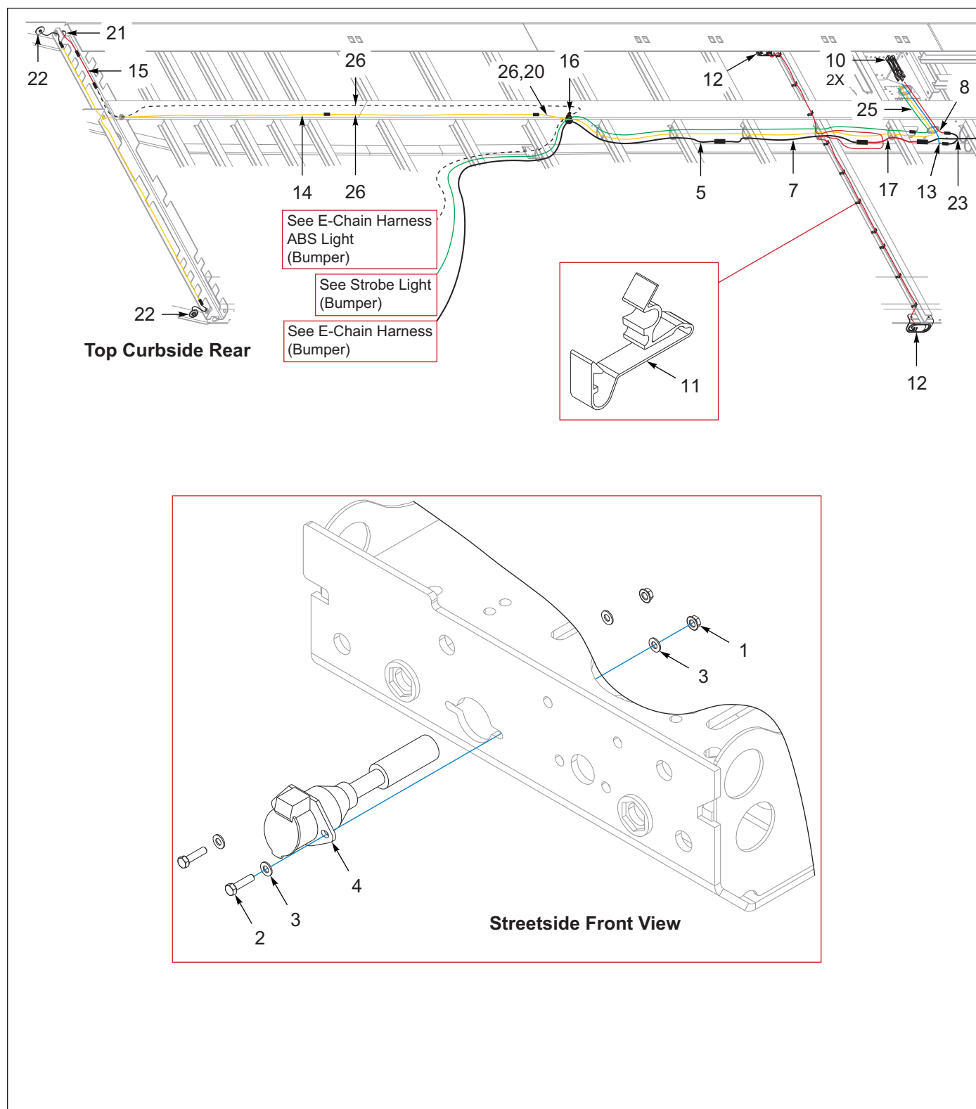
Figure 9-1: Frame, Control Panel & Marker Lights (1 of 2)
