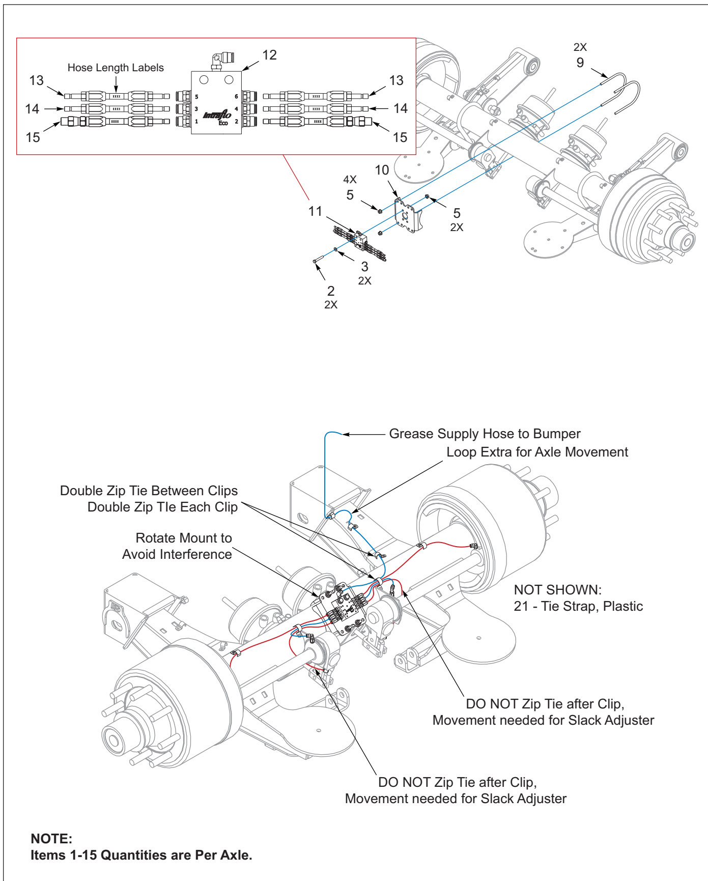
Figure 10-2: Axle Drum Brakes, 1 Axle (2 of 2)
