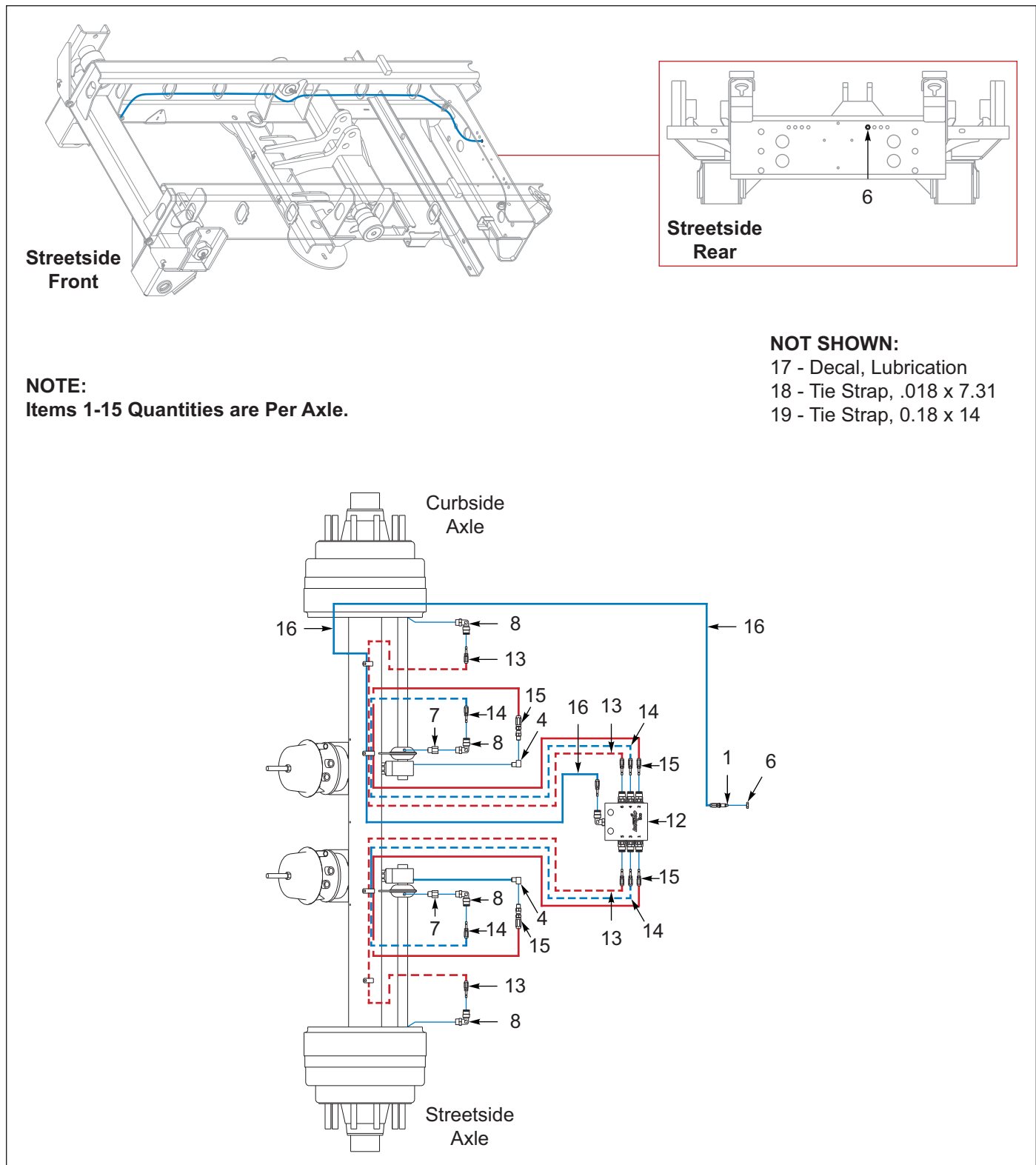
Figure 10-1: Axle Drum Brakes, 1 Axle (1 of 2)
