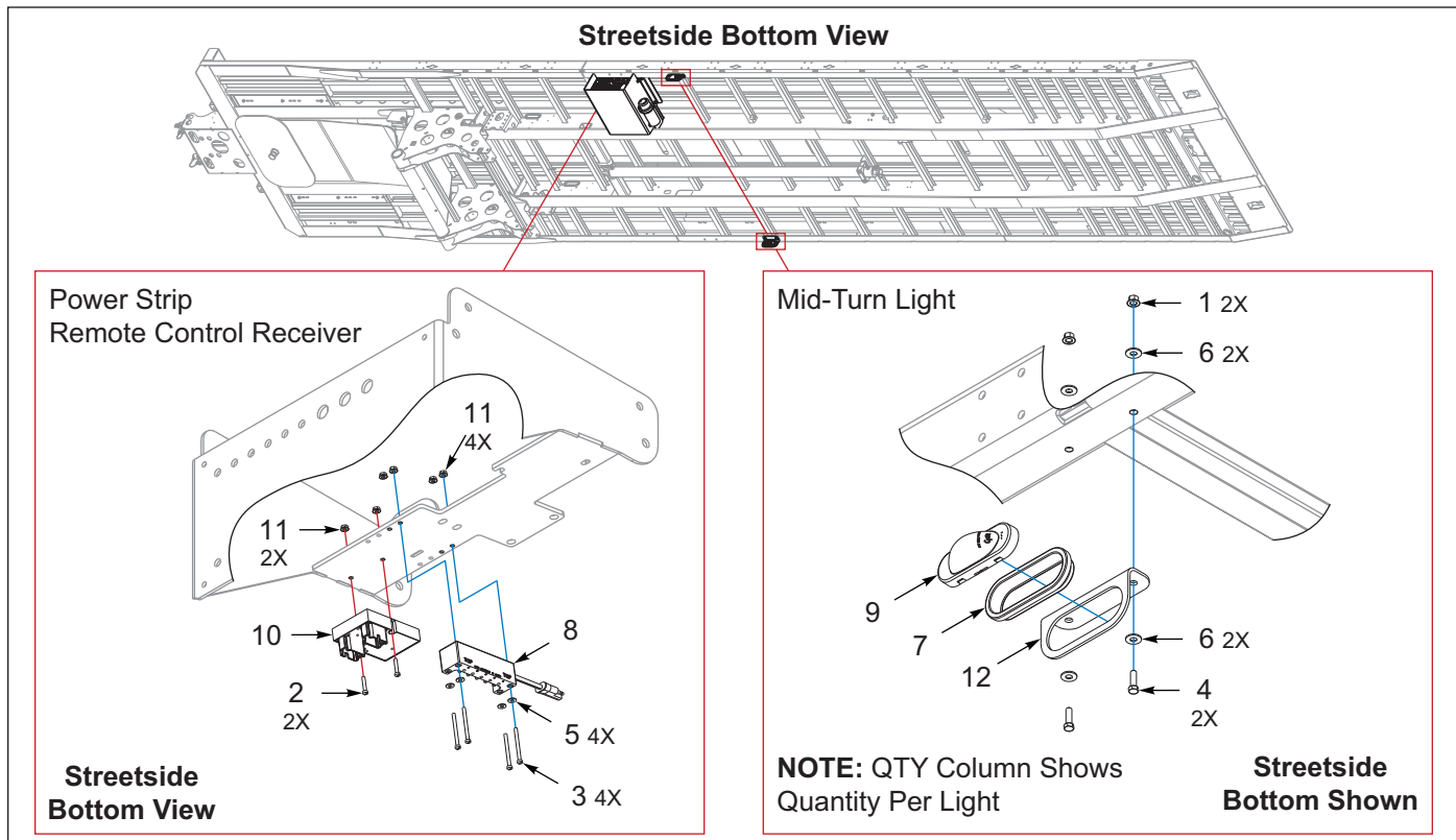
Figure 2-7: Electrical Power Strip, Remote Control Receiver, Mid-Turn Light
