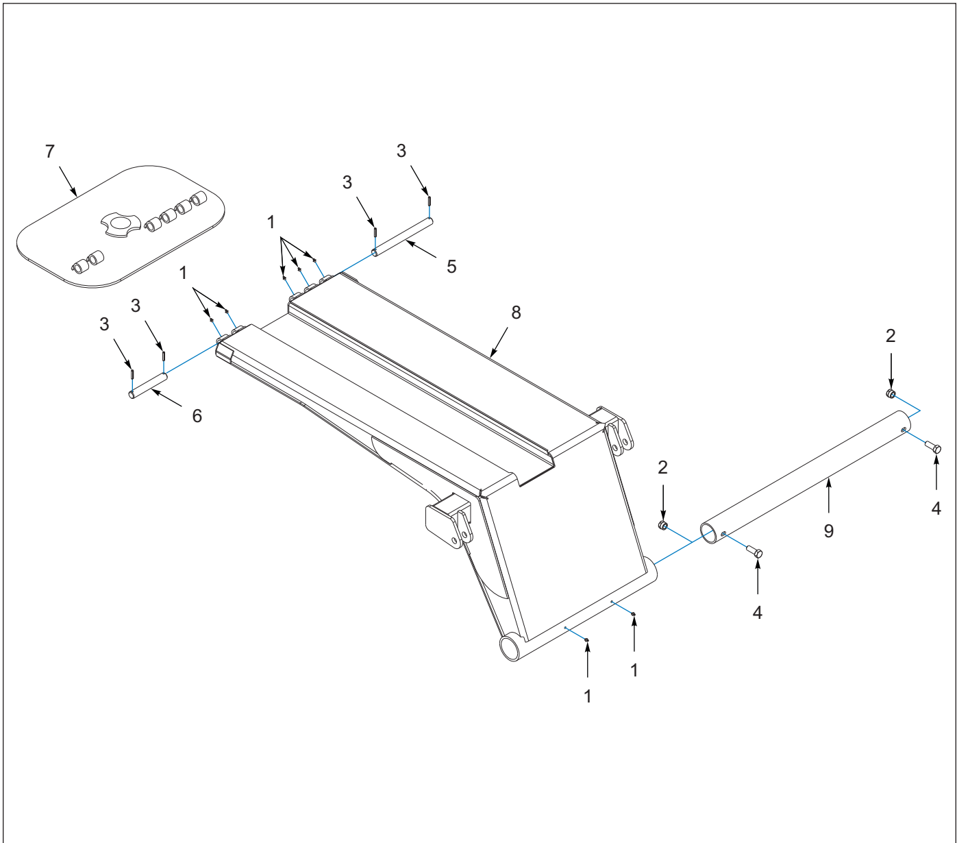
Figure 2-11: Hitch
