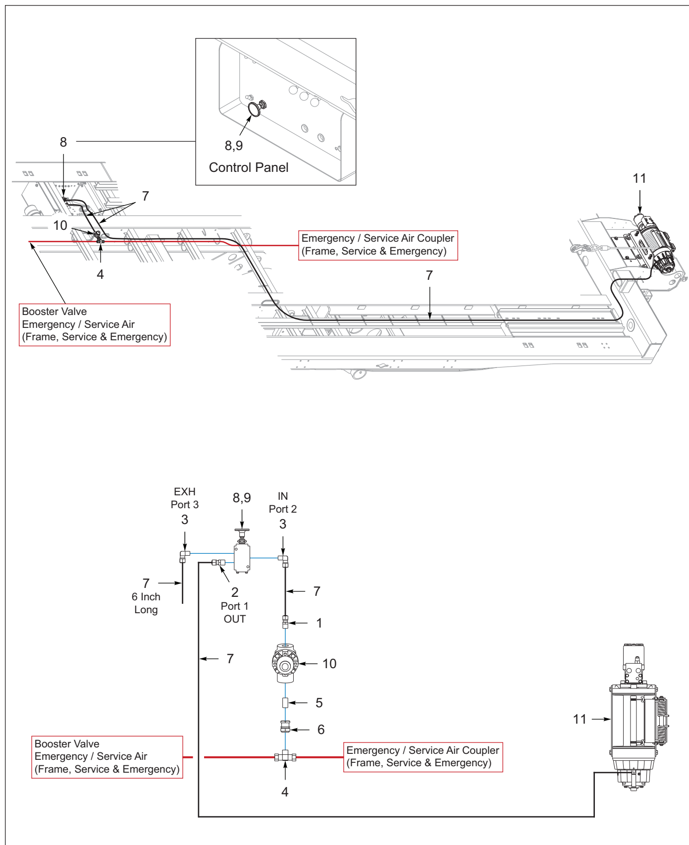
Figure 8-17: Winch Install, Ramsey 12K, 1 Speed, Spring Tension
