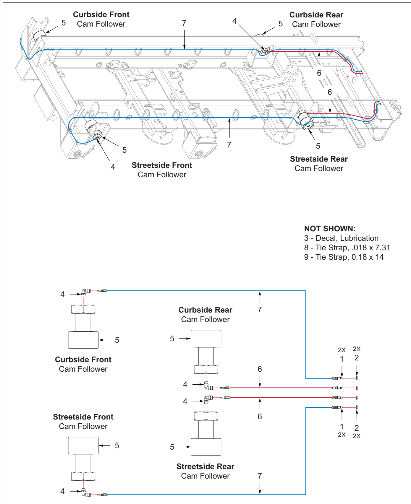
Figure 10-7: Cam Followers, 2 Axle (1 of 2)
