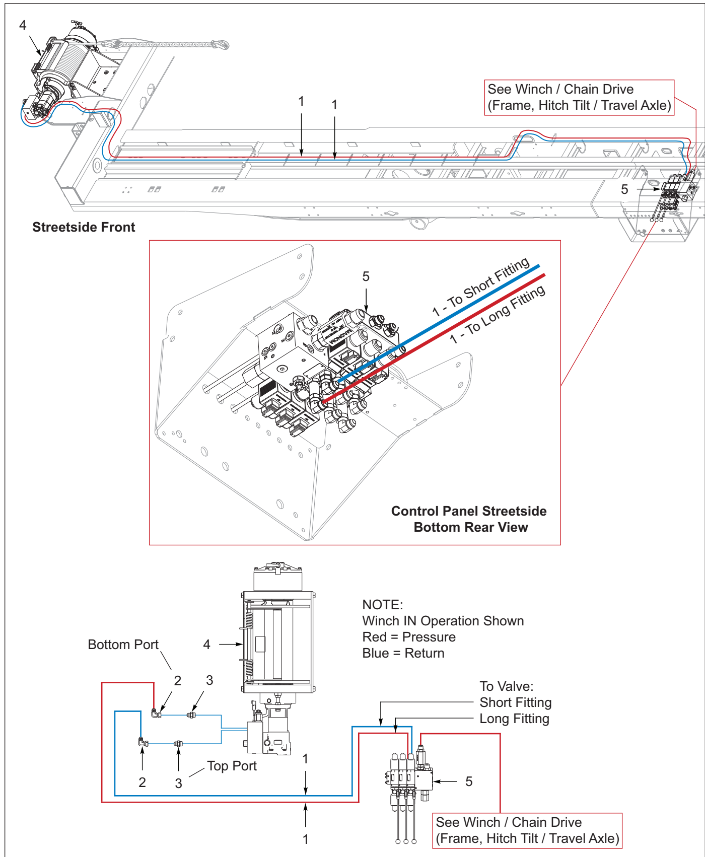
Figure 11-7: Winch Install, Warn 20K, 2 Speed, Spring Tension
