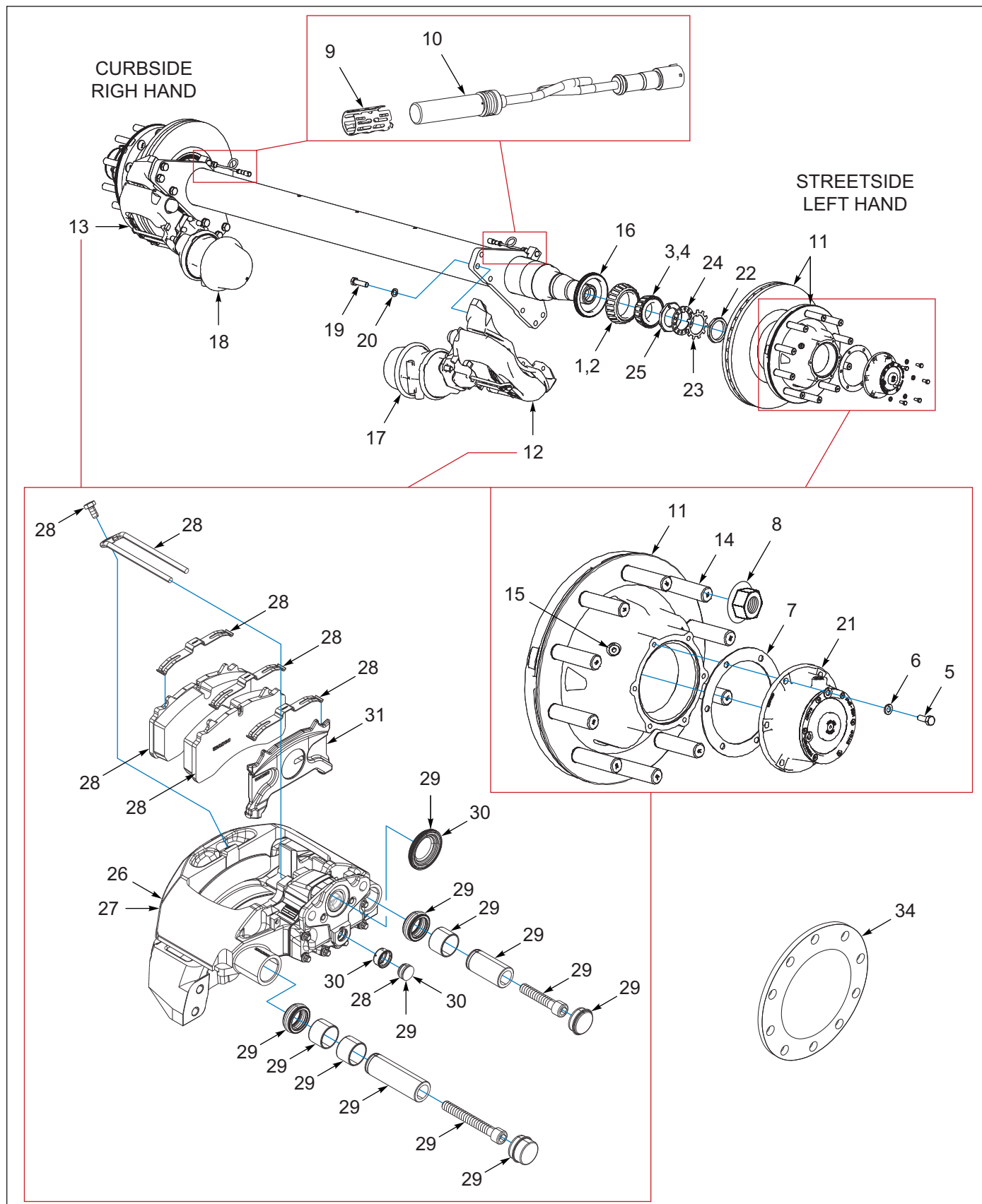
Figure 3-7: Axle 16.50 Disc Brake & Hub Components (Option) (1 of 2)
