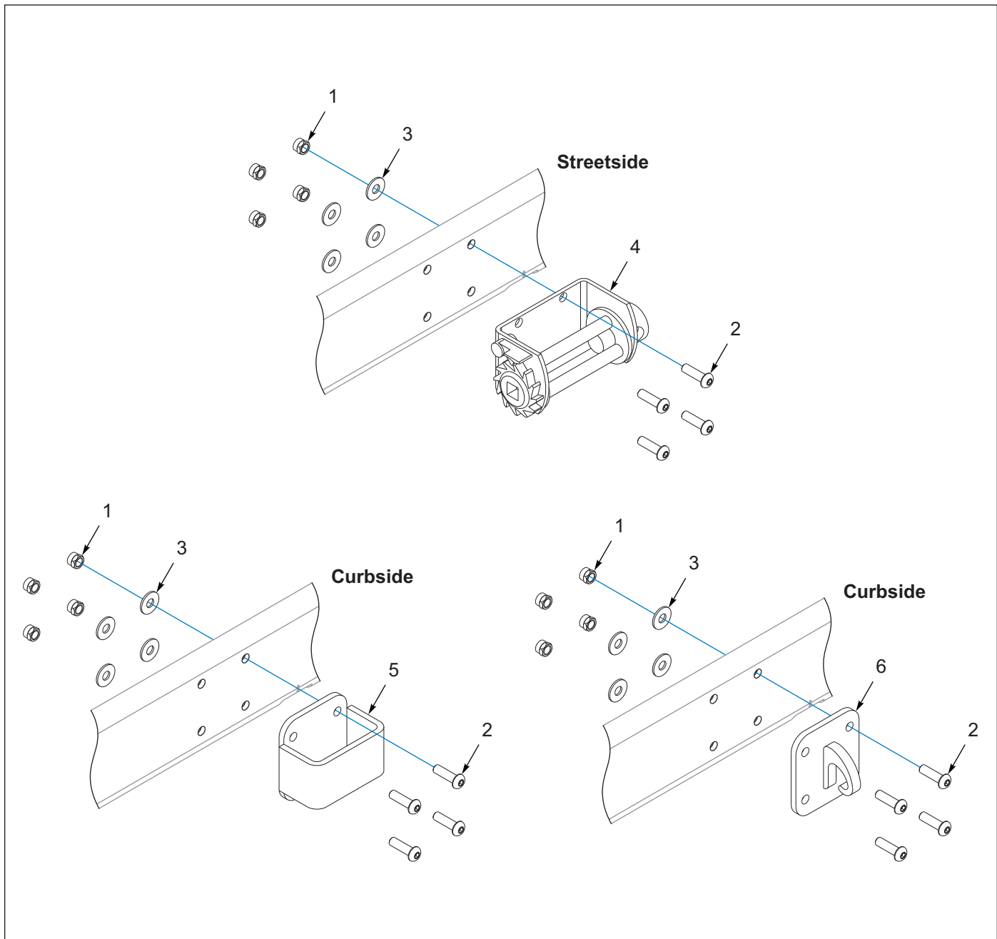
Figure 7-17: Tie Down, Strap Ratchet, 3-Bar, Strap Pocket / J-Hook, Bolt On
