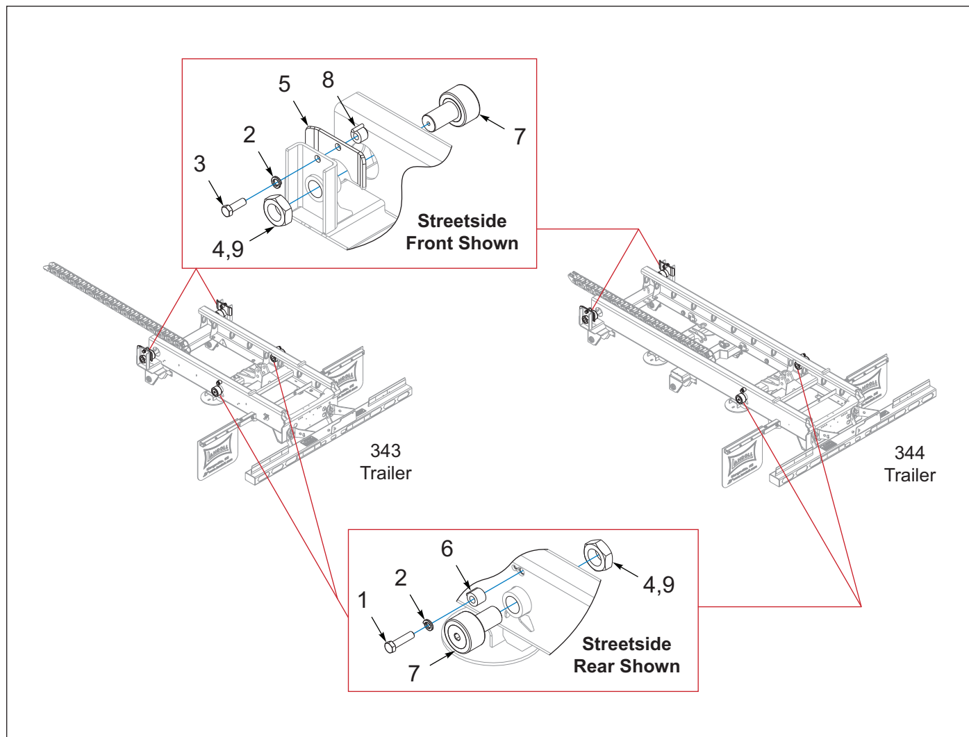
Figure 2-3: Cam Followers & Hold Downs
