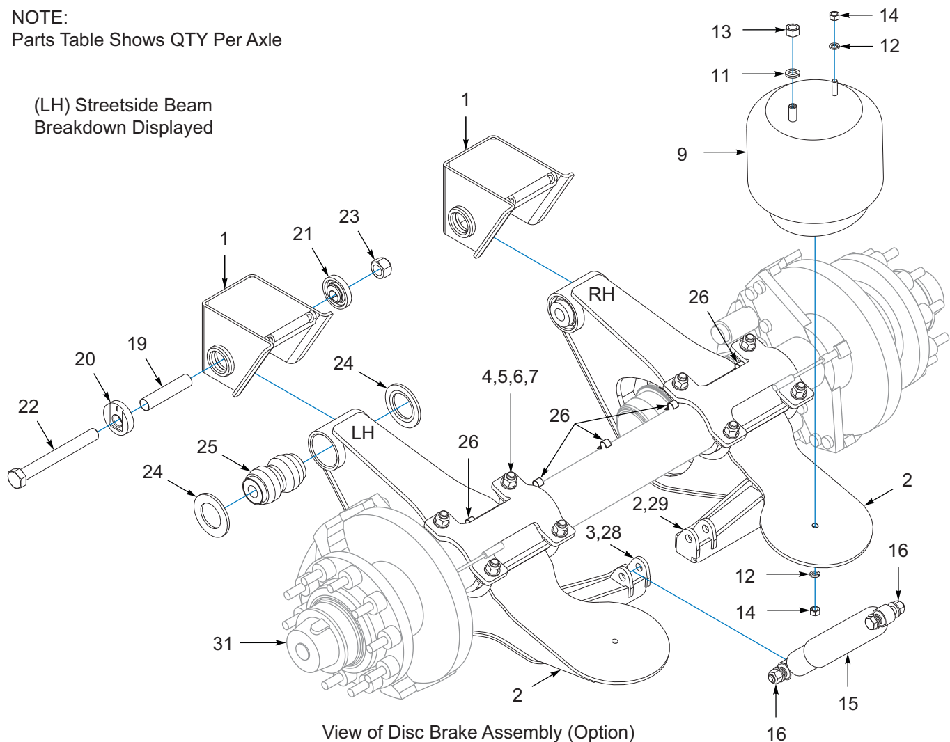
Figure 3-12: Axle Suspension, LSS-25K-5.5 RLU, 16.50
