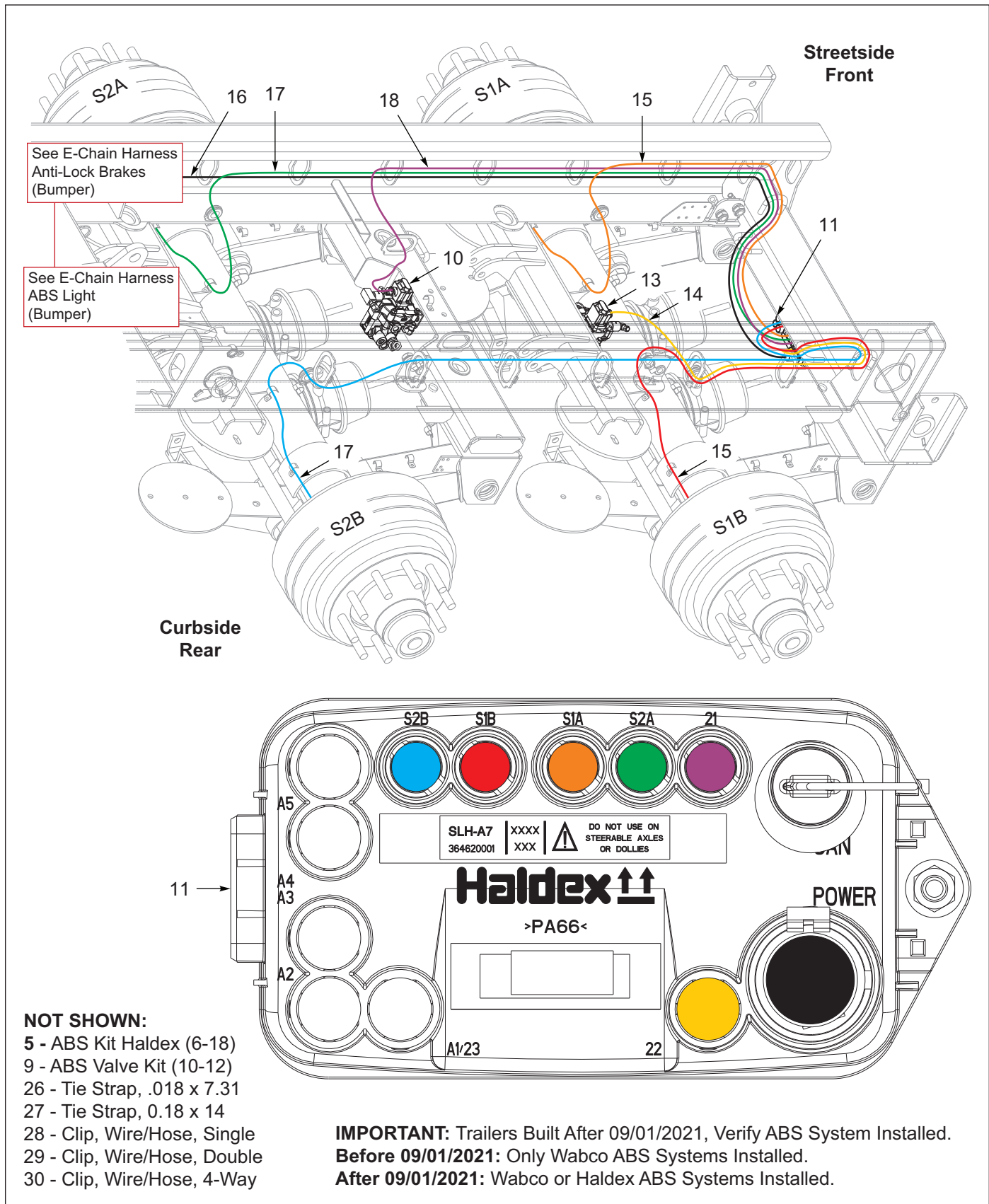
Figure 9-7: Anti-Lock Brakes, 2 Axle, Haldex (1 of 3)
