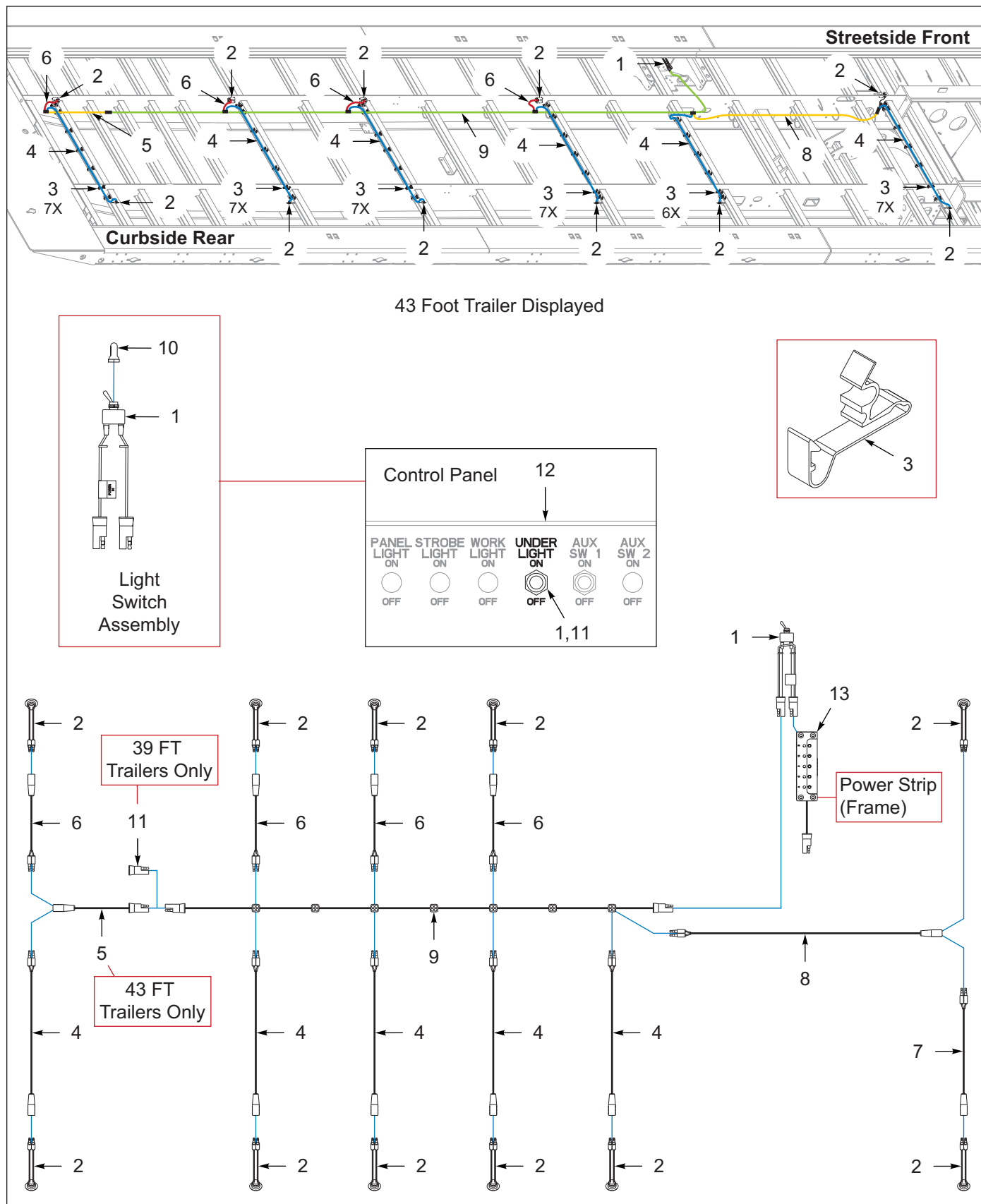
Figure 9-14: Lights, Work Zone, Underdeck (Option)
