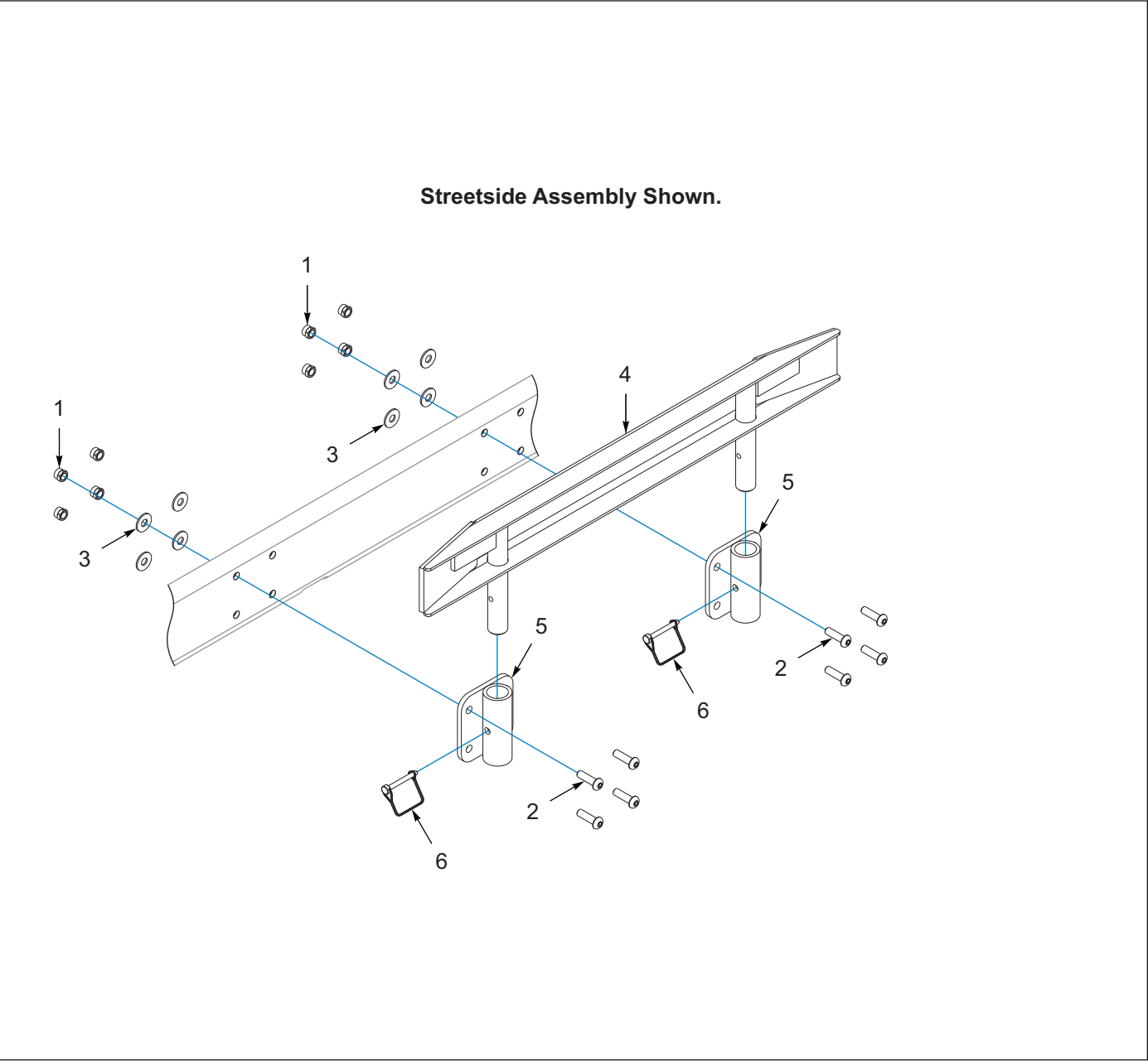
Figure 7-6: Container Side Guide, 40 Inch, Bolt On
