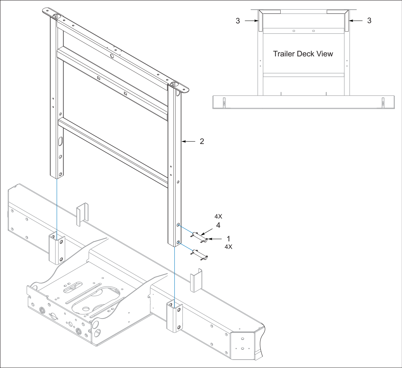
Figure 4-1: Bulkhead, Accessory Rack
