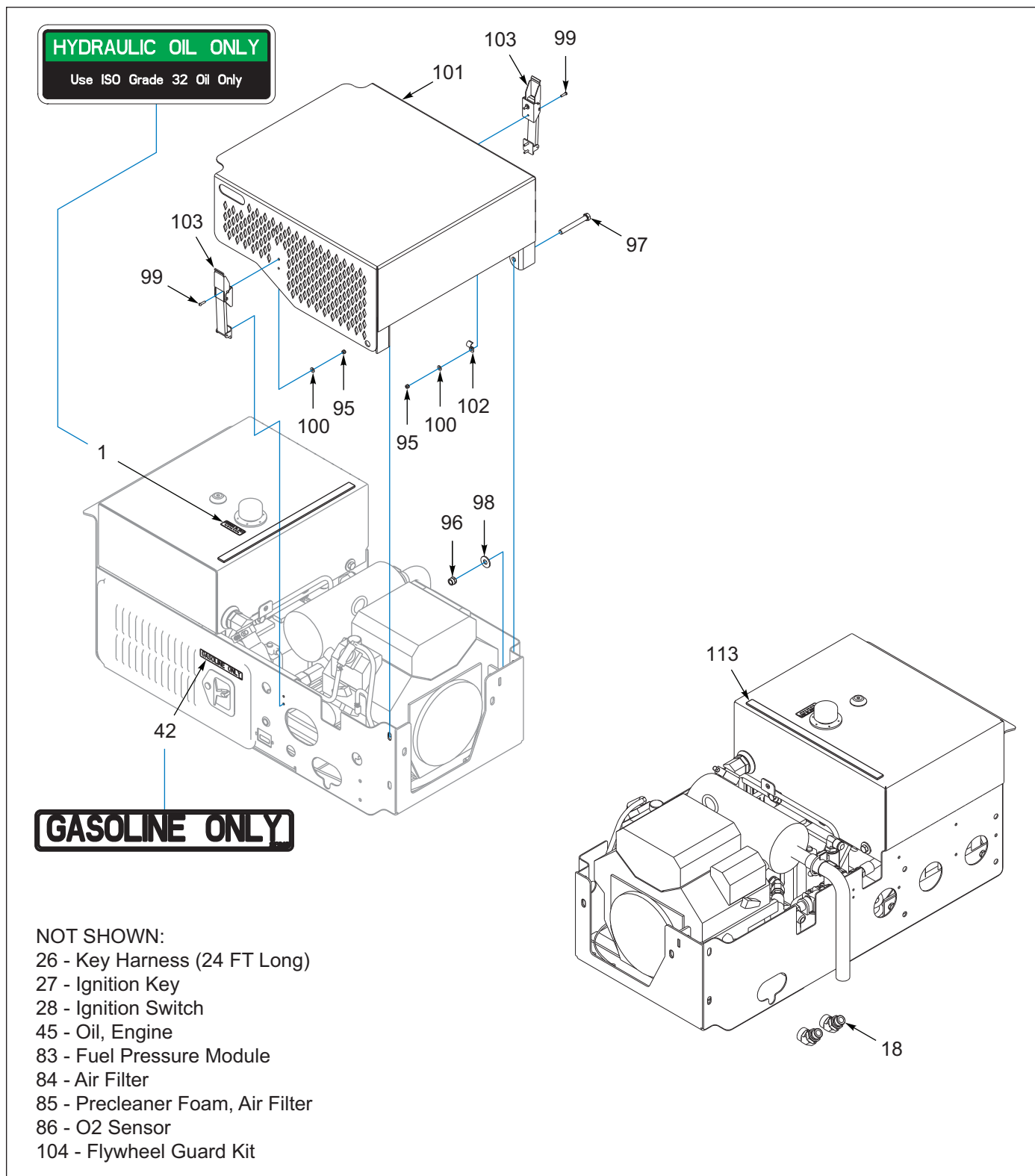
Figure 5-1: Engine Package, 25 HP, Upper Deck Assembly (1 of 5)
