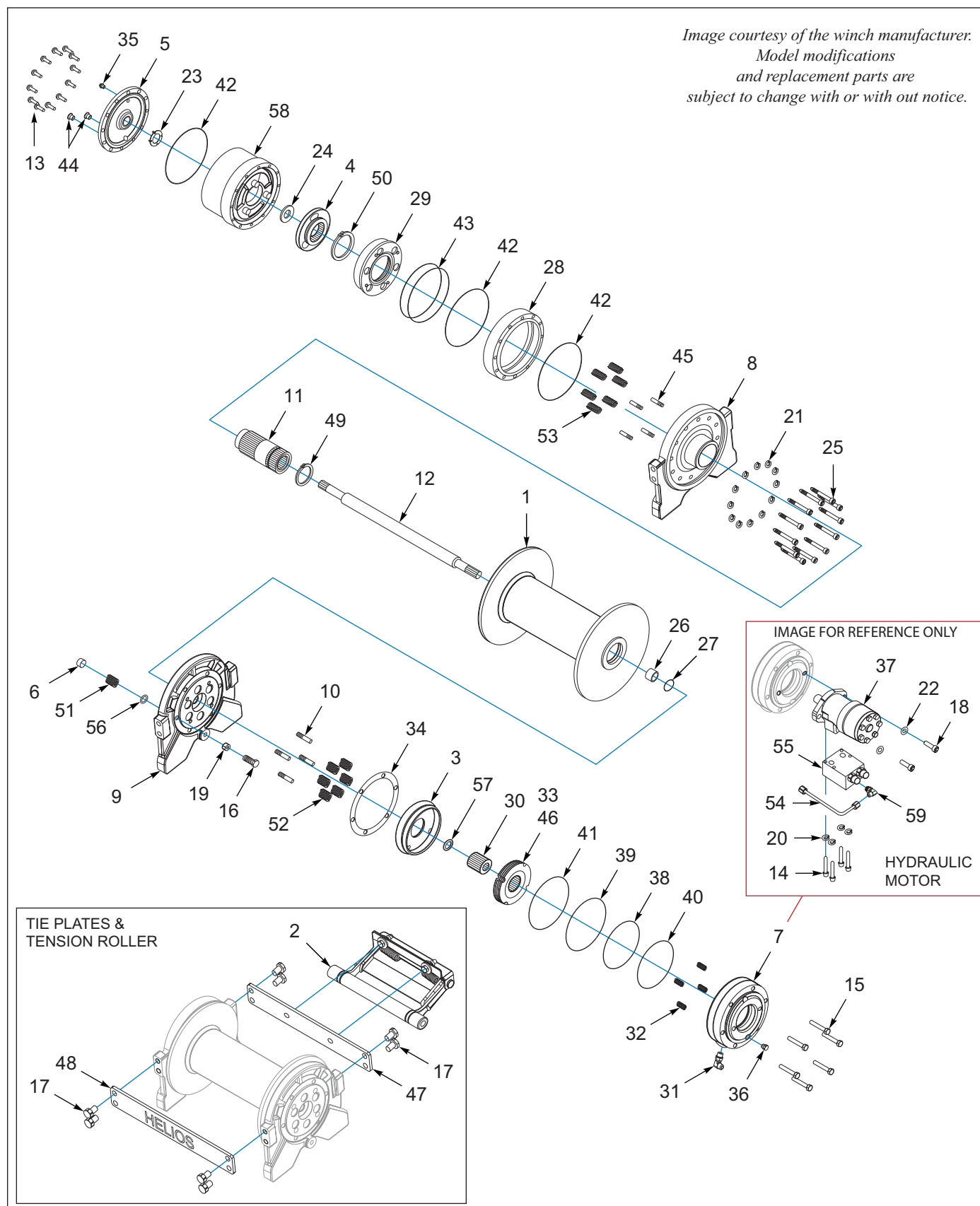
Figure 6-9: Winch Components, Ramsey 20K, 2 Speed, Spring Tension
