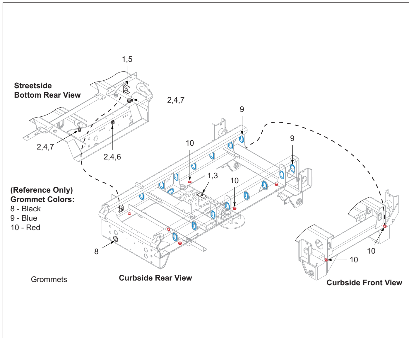
Figure 2-9: Grommets, Hose Clamps, & P-Clamps, Undercarriage, 343
