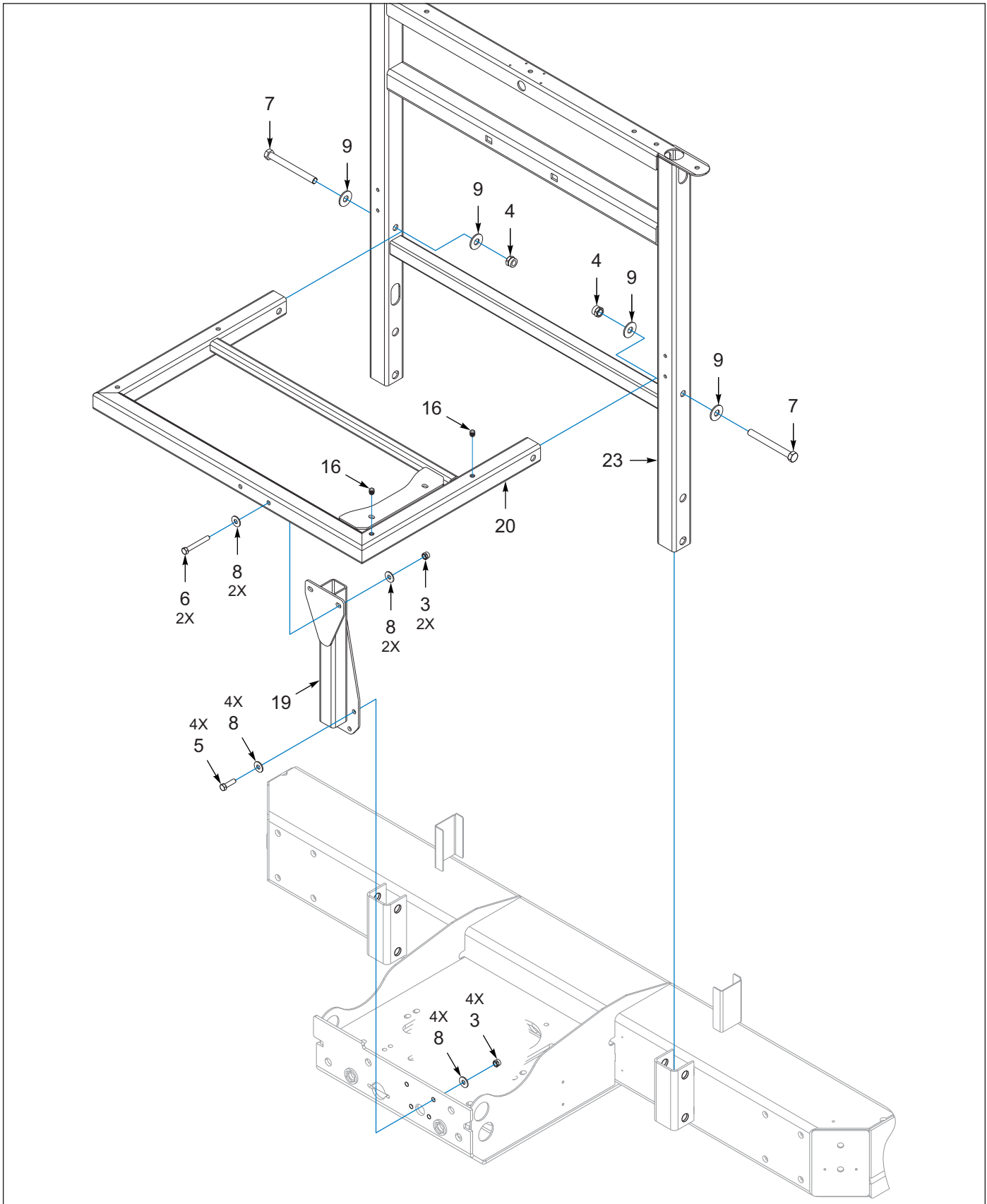
Figure 5-6: Mount, Front, Accessory Rack (1 of 2)
