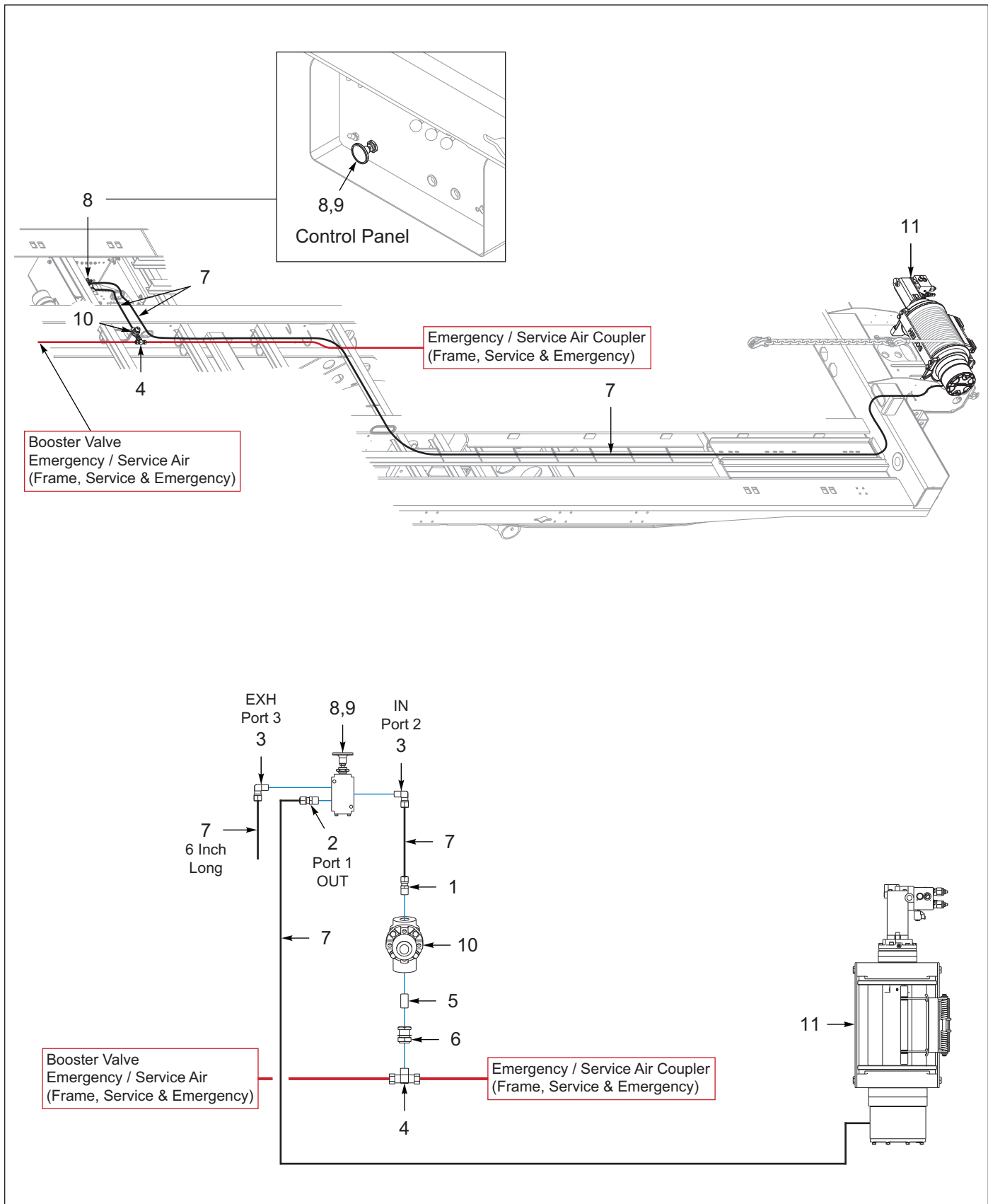
Figure 8-18: Winch Install, Ramsey 20K, 2 Speed, Spring Tension
