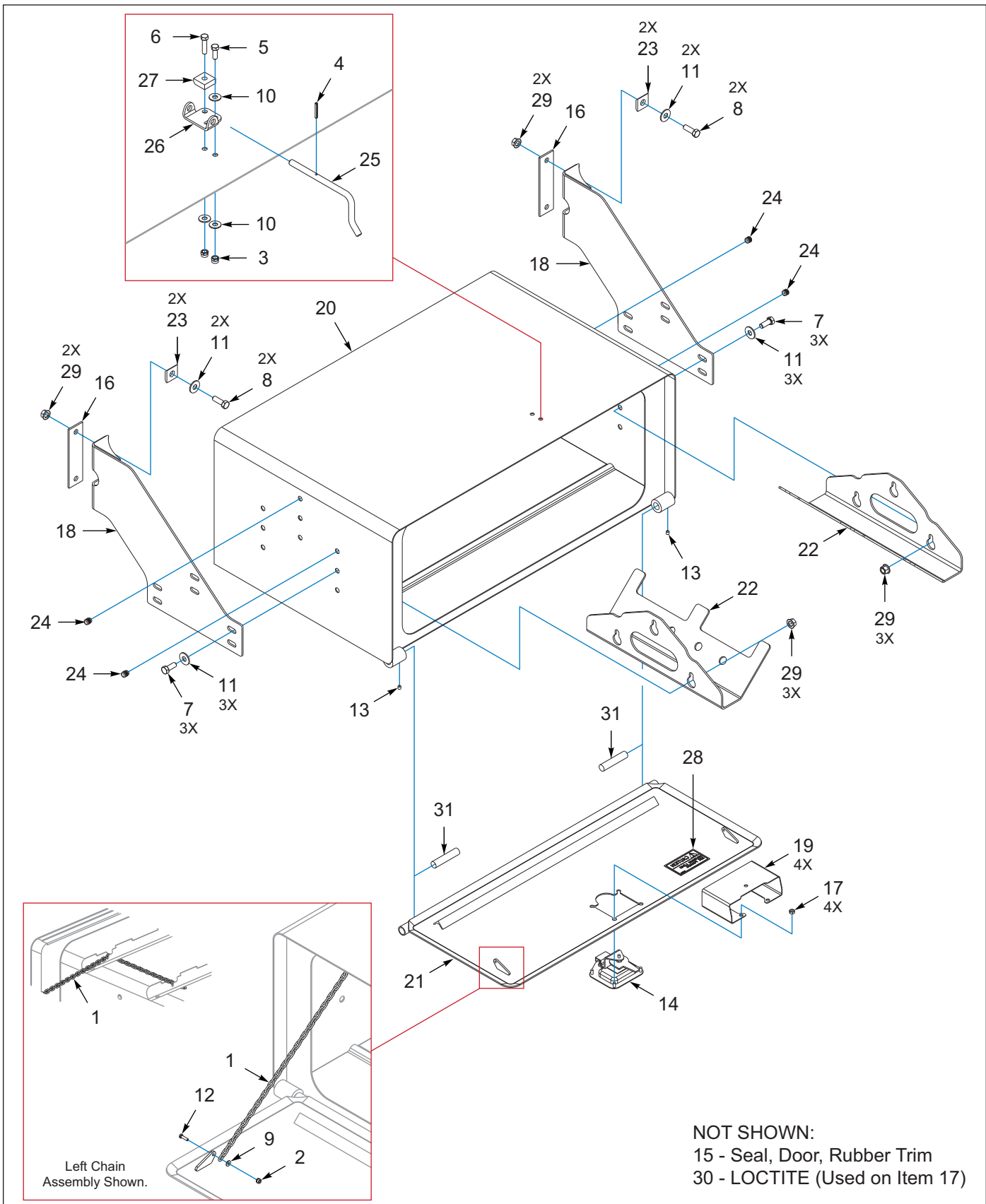
Figure 4-9: Toolbox, Bolt-On, 42"W X 28"D X 17"H
