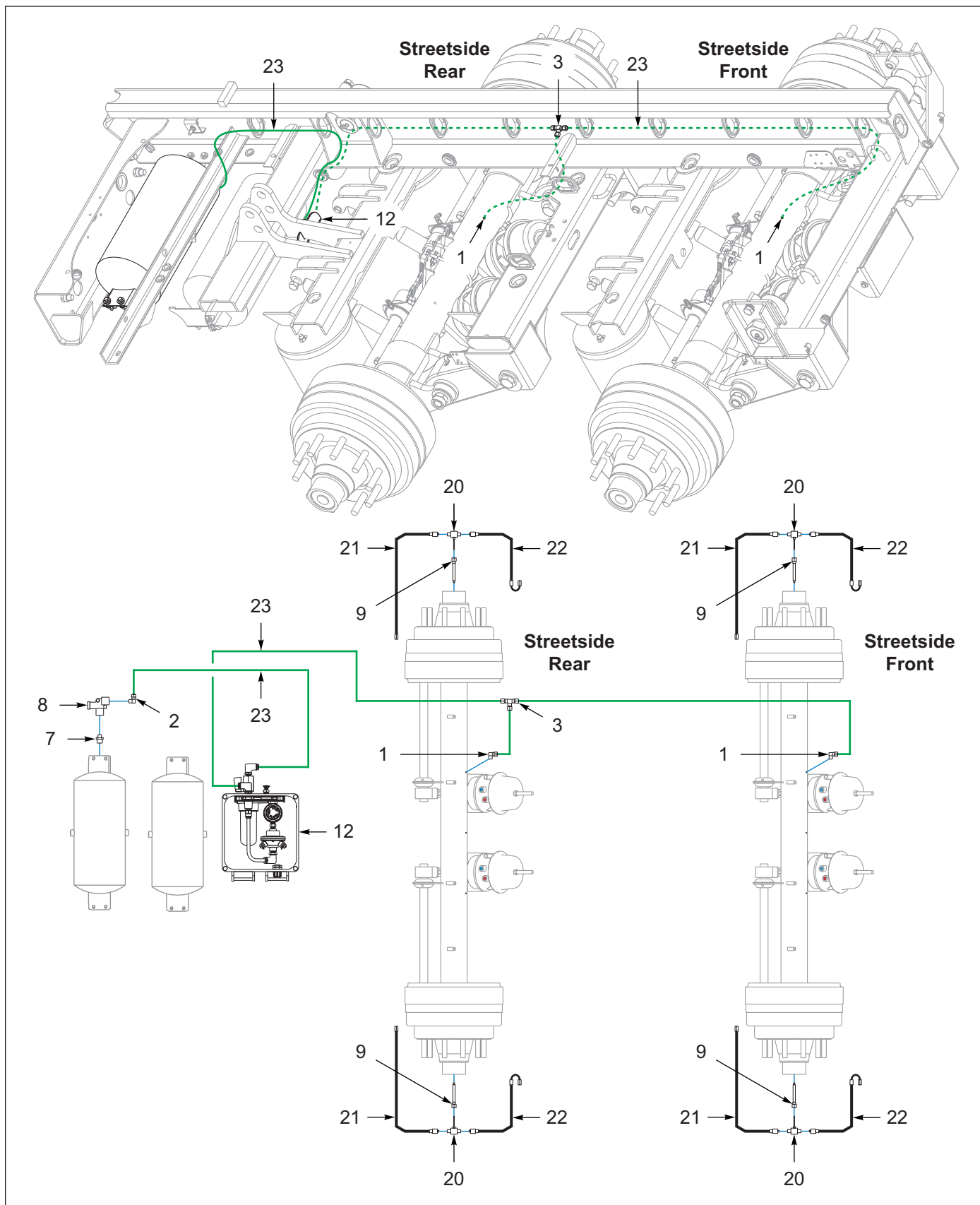
Figure 8-14: Tire Inflation, 2 Axle (1 of 2)
