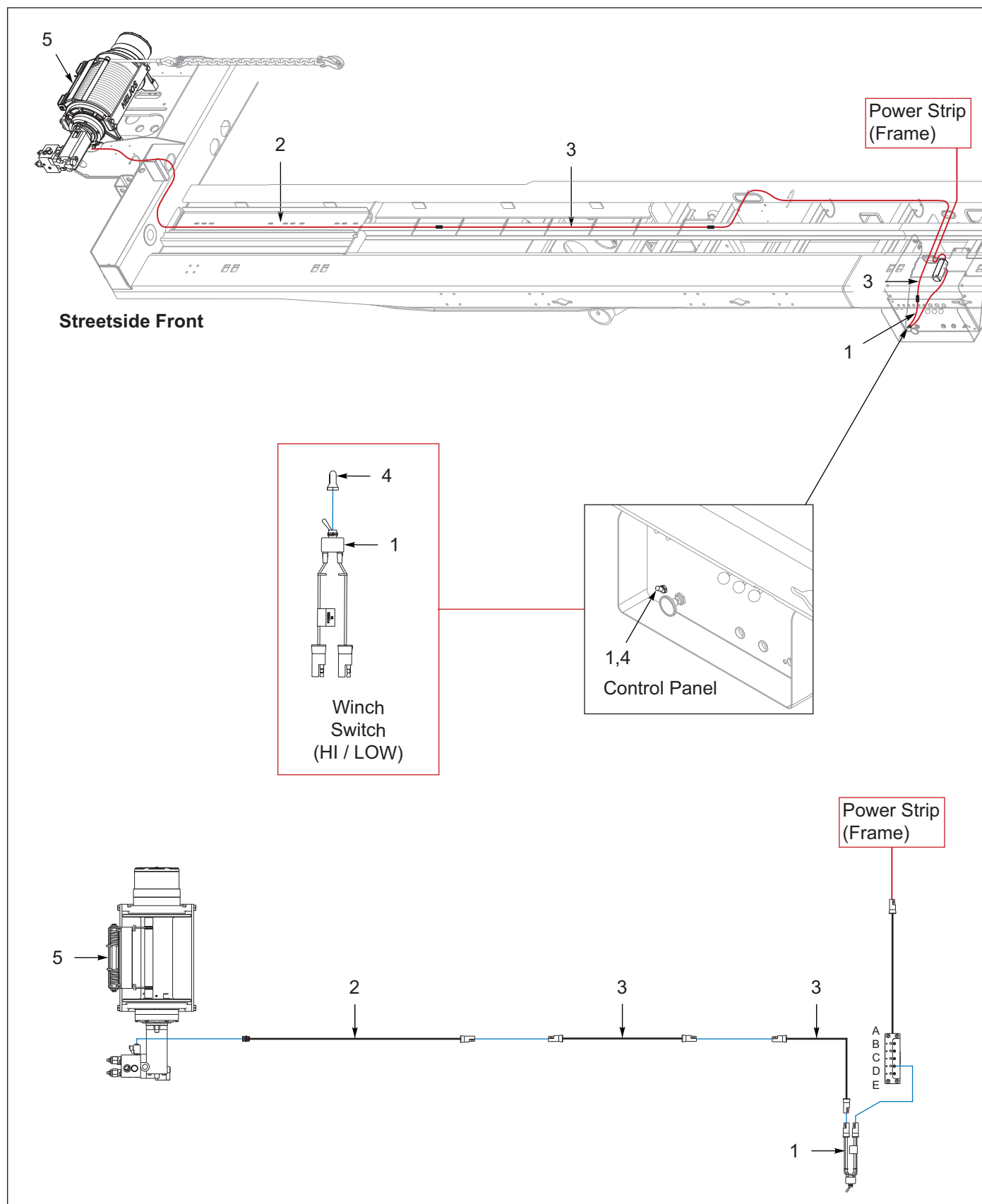
Figure 9-20: Winch Install, Ramsey 20K, 2 Speed, Spring Tension
