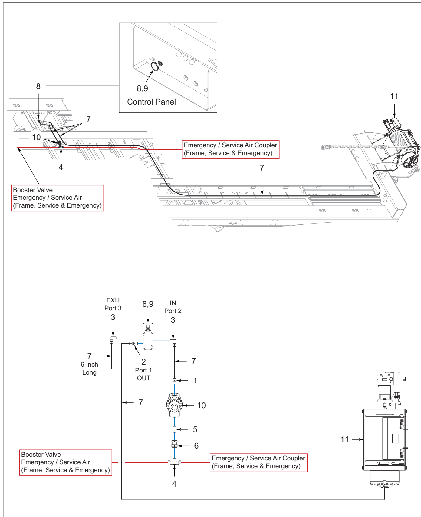
Figure 8-20: Winch Install, Warn 20K, 2 Speed, Spring Tension
