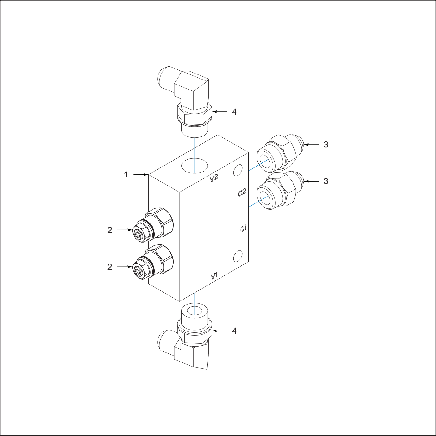
Figure 11-13: Valve Components, Counter Balance, Dual
