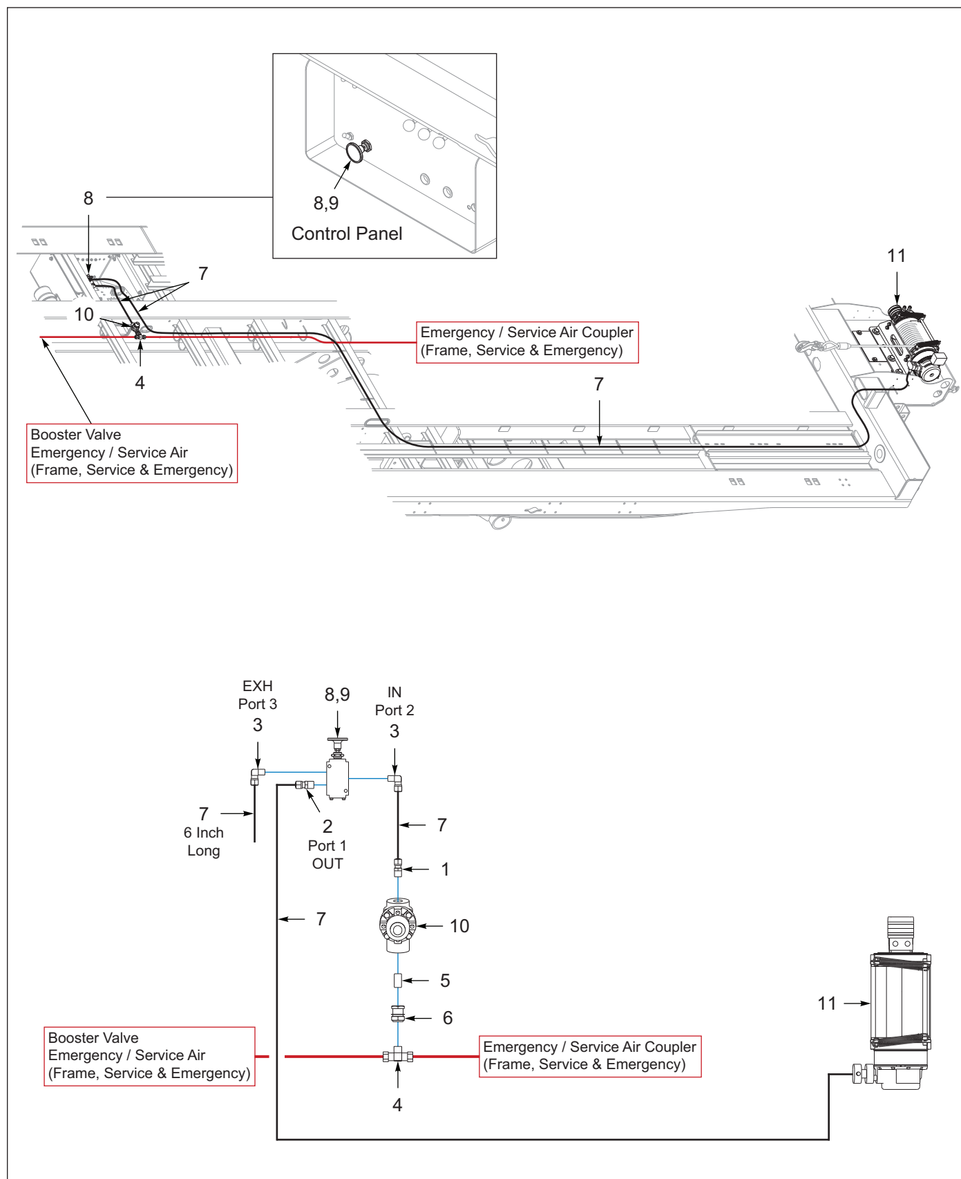
Figure 8-19: Winch Install, Warn 12K, 1 Speed, Spring Tension
