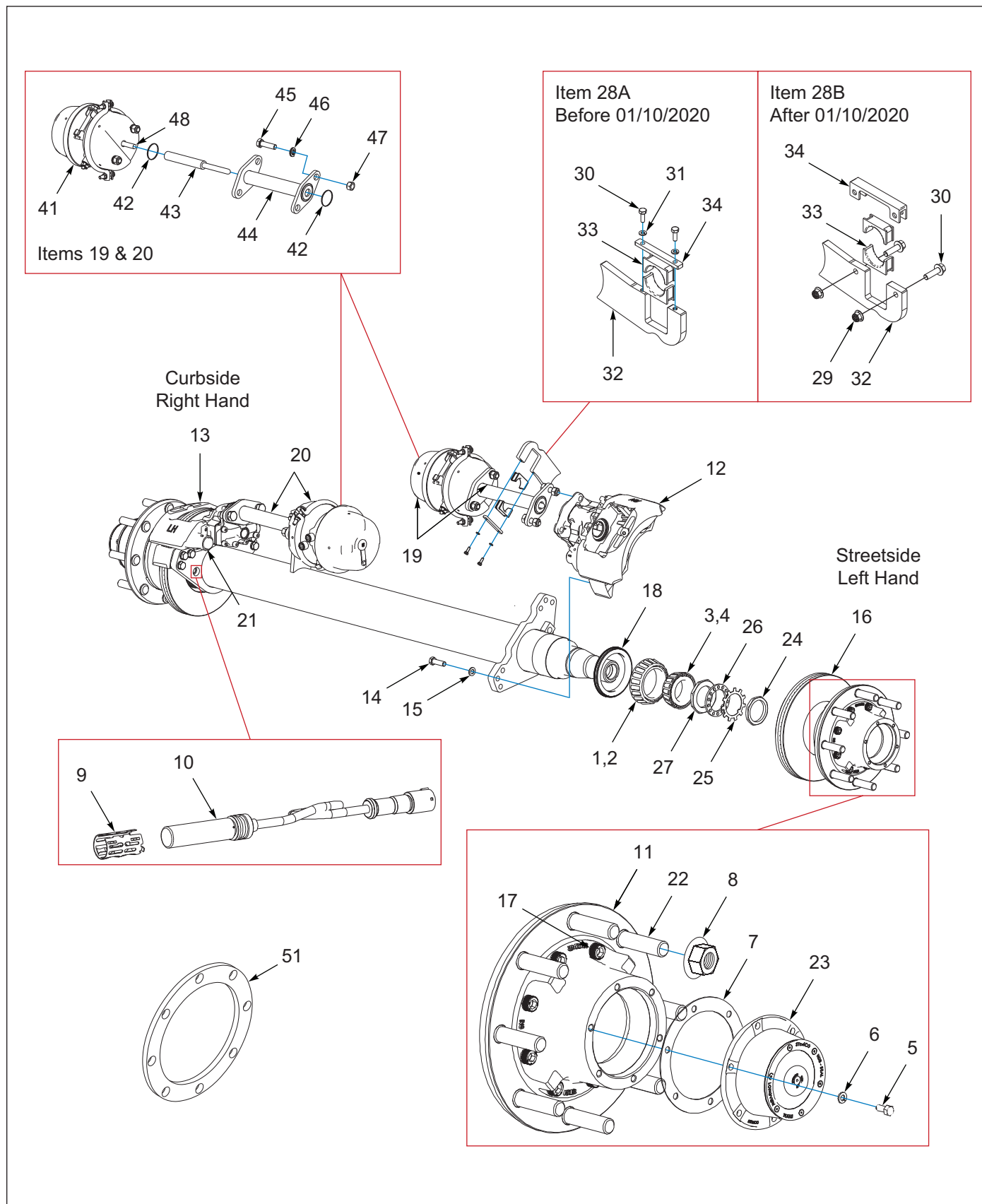
Figure 3-3: Axle 12.25 Disc Brake & Hub Components (Option) (1 of 2)
