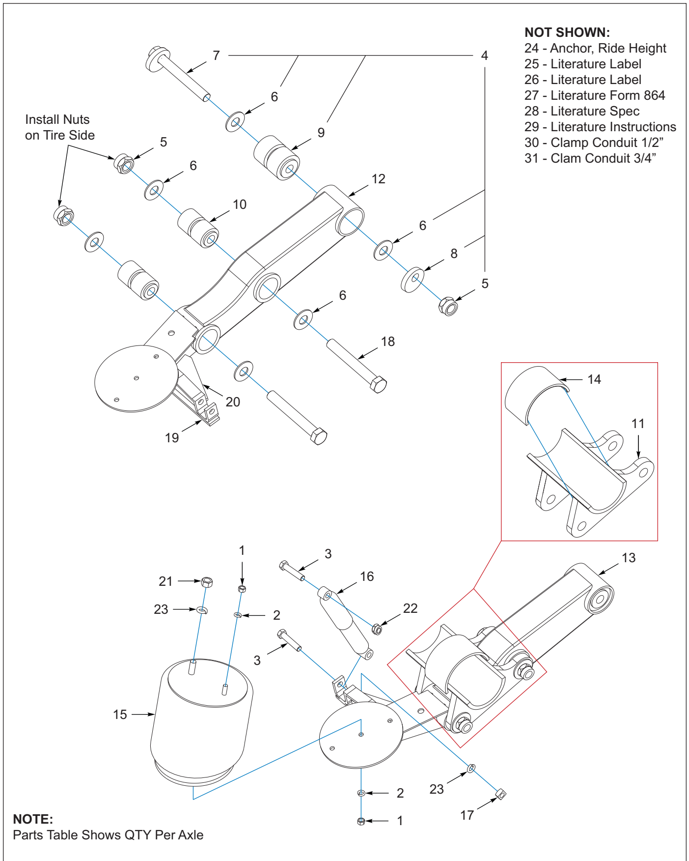
Figure 3-10: Axle Suspension, RLU-228, 12.25 & 16.50 (2 of 2)
