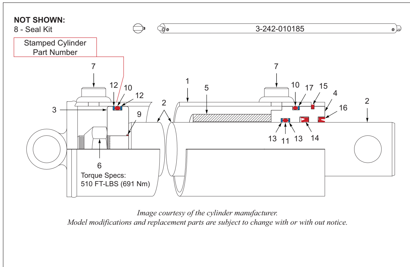
Figure 11-10: Cylinder Components, 4 x 126
