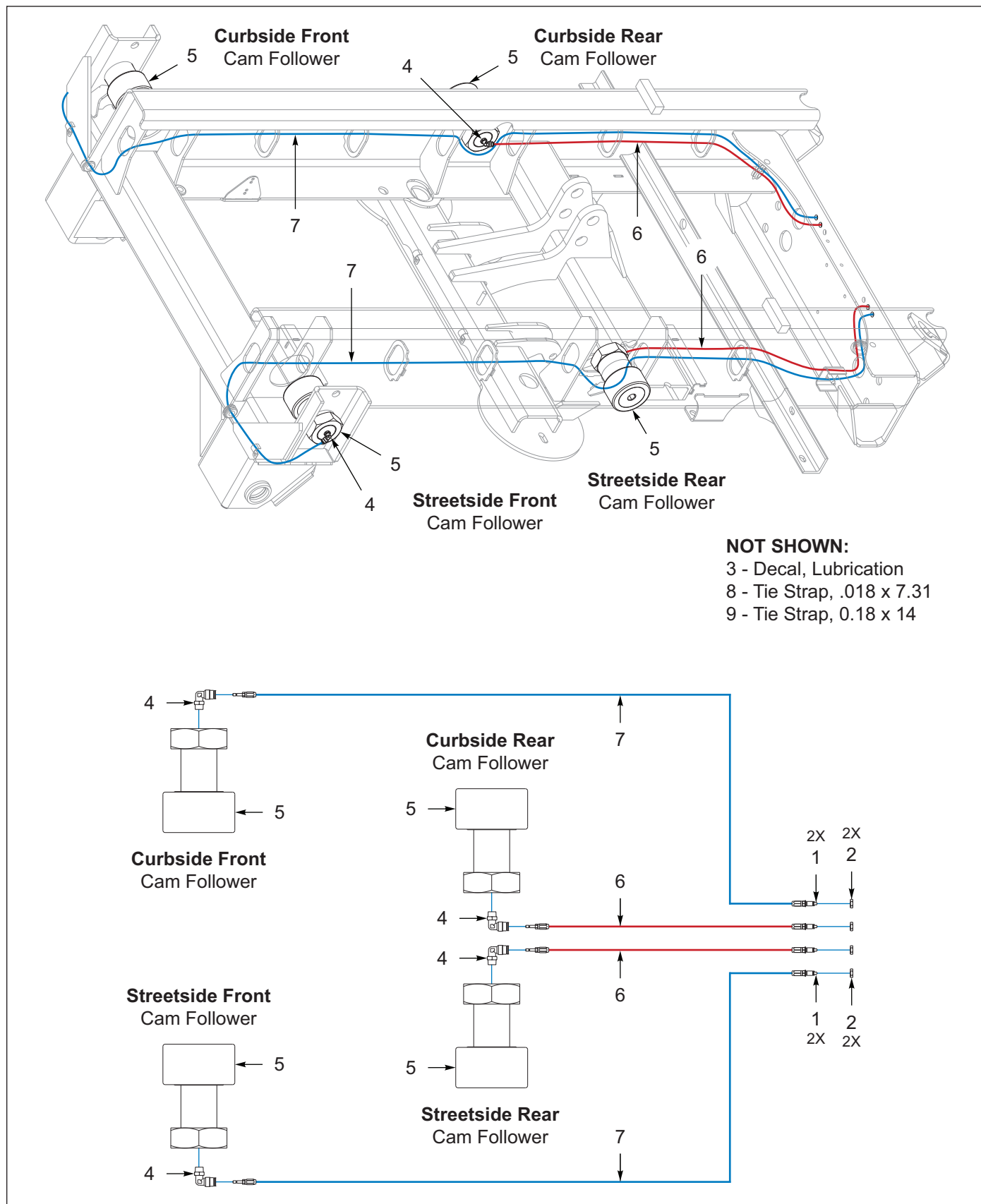
Figure 10-5: Cam Followers, 1 Axle (1 of 2)
