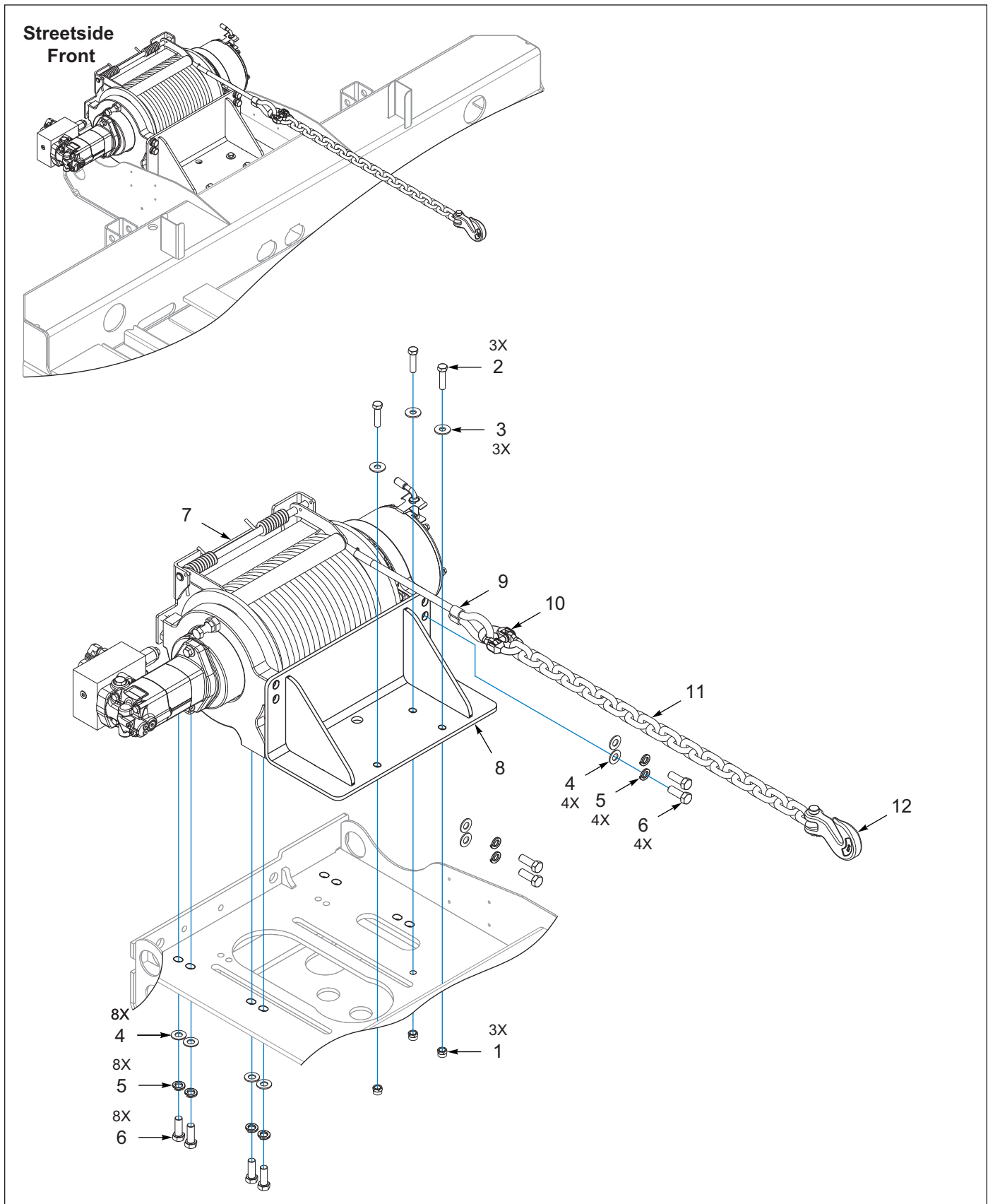
Figure 6-7: Winch Install, Warn 20K, 2 Speed, Spring Tension
