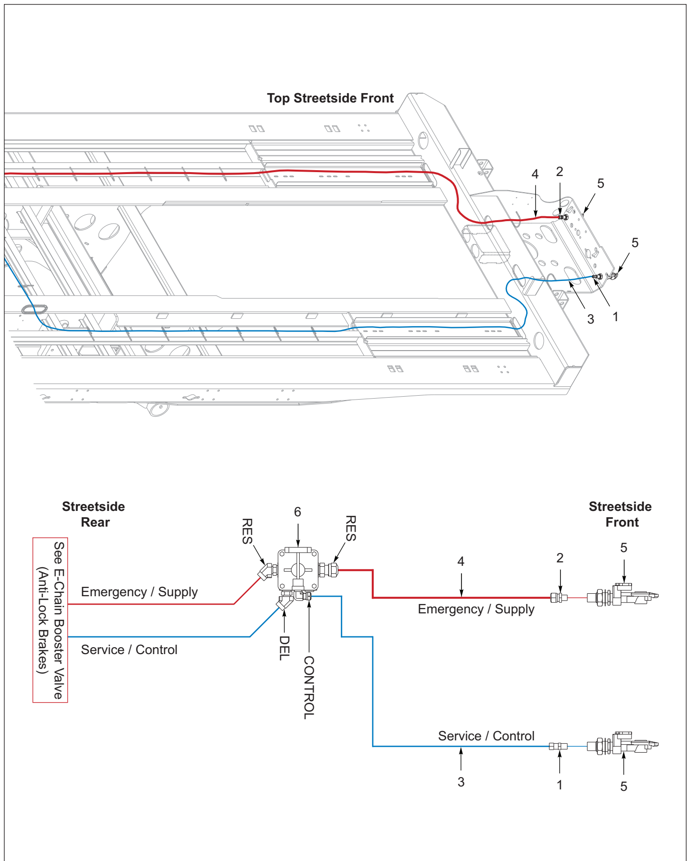
Figure 8-2: Frame, Service &amp; Emergency (2 of 2)
