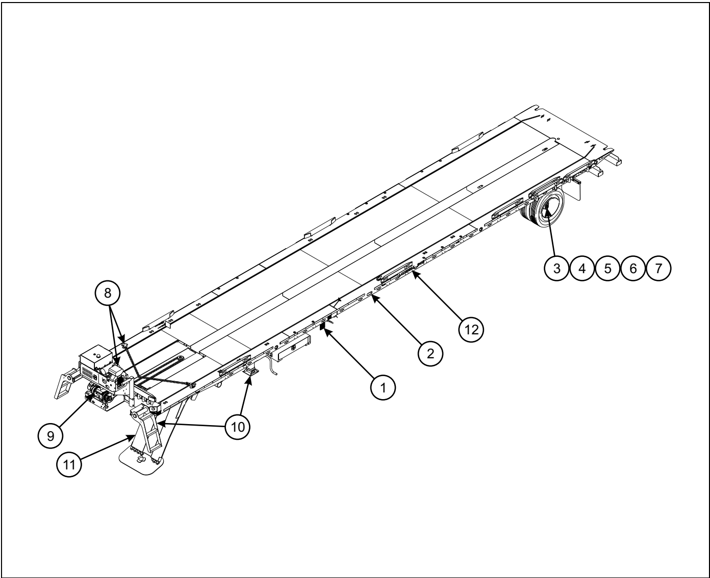
Figure 1-2: General Assembly
