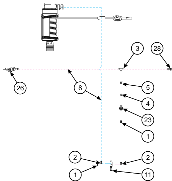
HYDRAULIC SYSTEM
