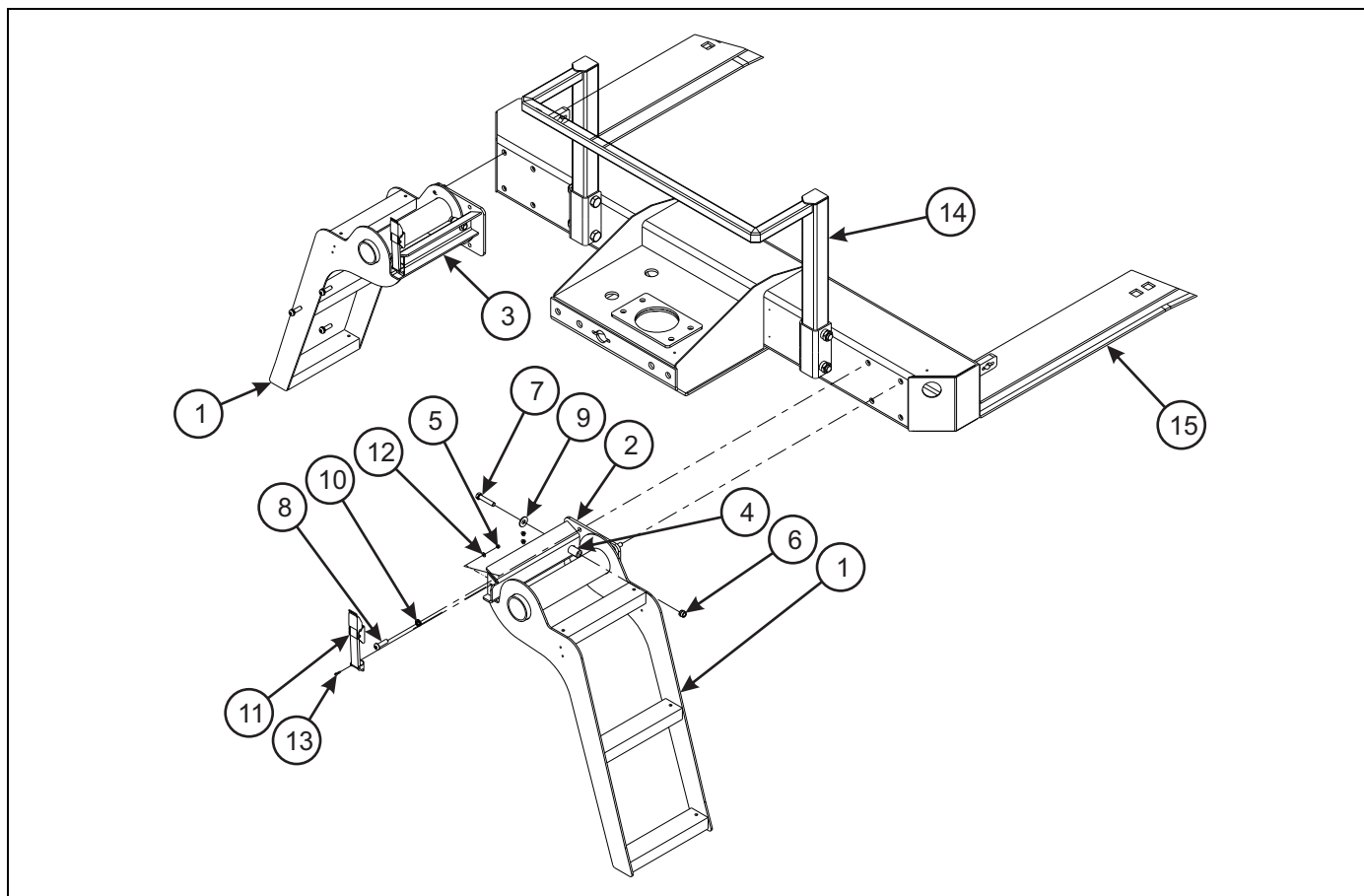
Figure 1-51: Ladder Assembly
