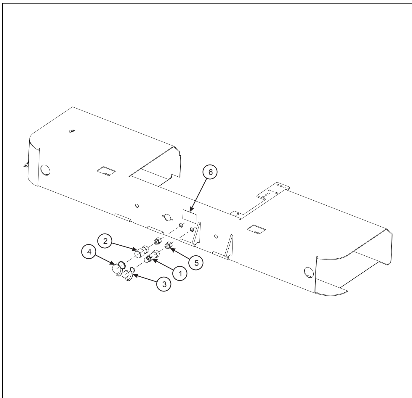
Figure 1-64: Hydraulic Conversion Kit - Ball to Flat
