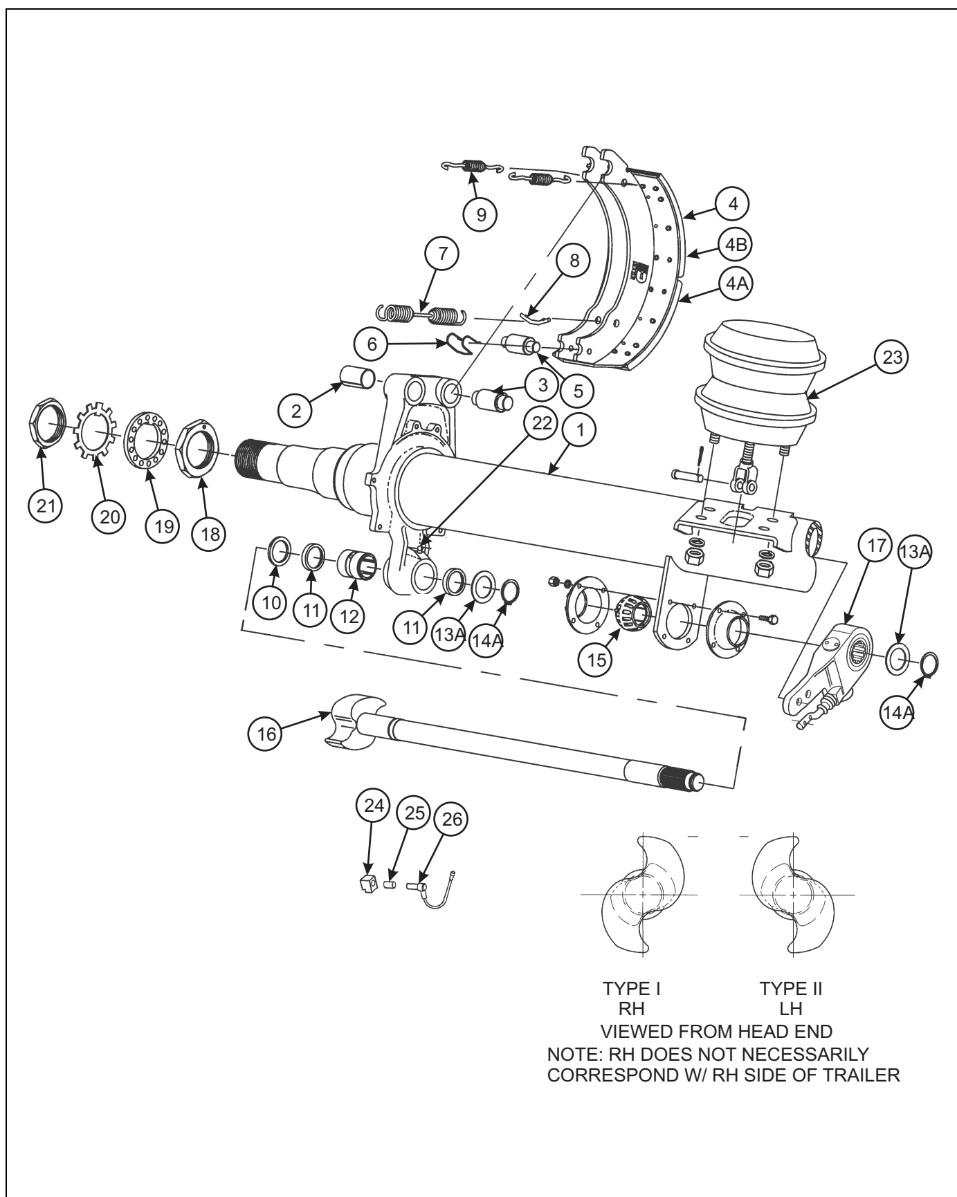
Figure 1-24: Axle and Brake Assembly - Dexter (16-1/2" X 7")
