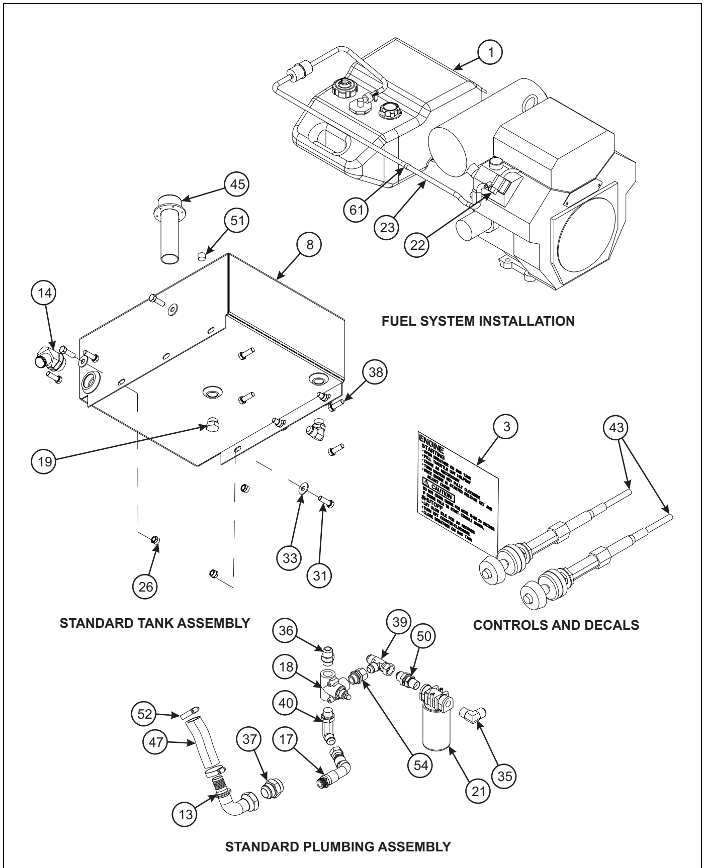
Figure 1-60: Engine - 27 HP Gas Package (2 of 2)
