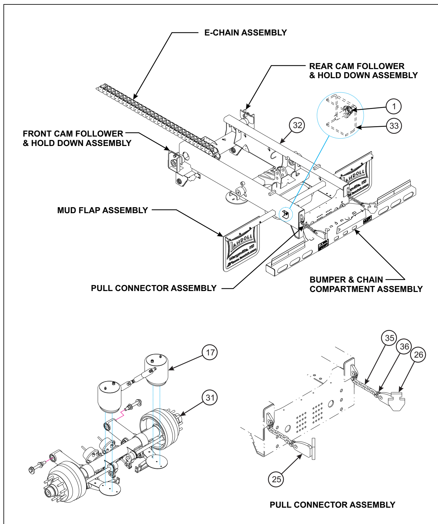
Figure 1-14: General Items (1 of 3)
