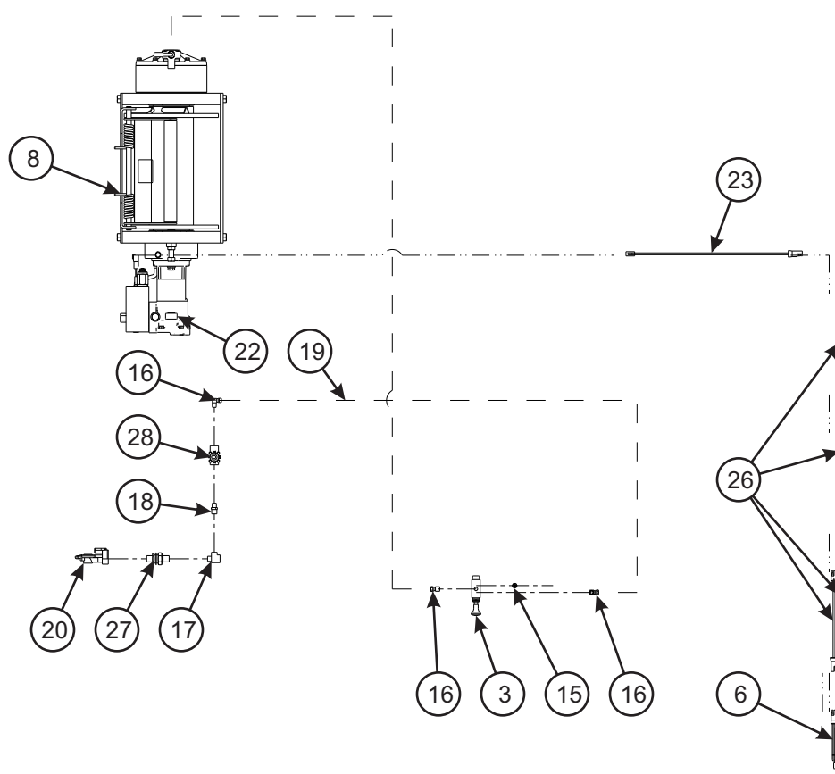
ELECTRICAL AND AIR SYSTEM
