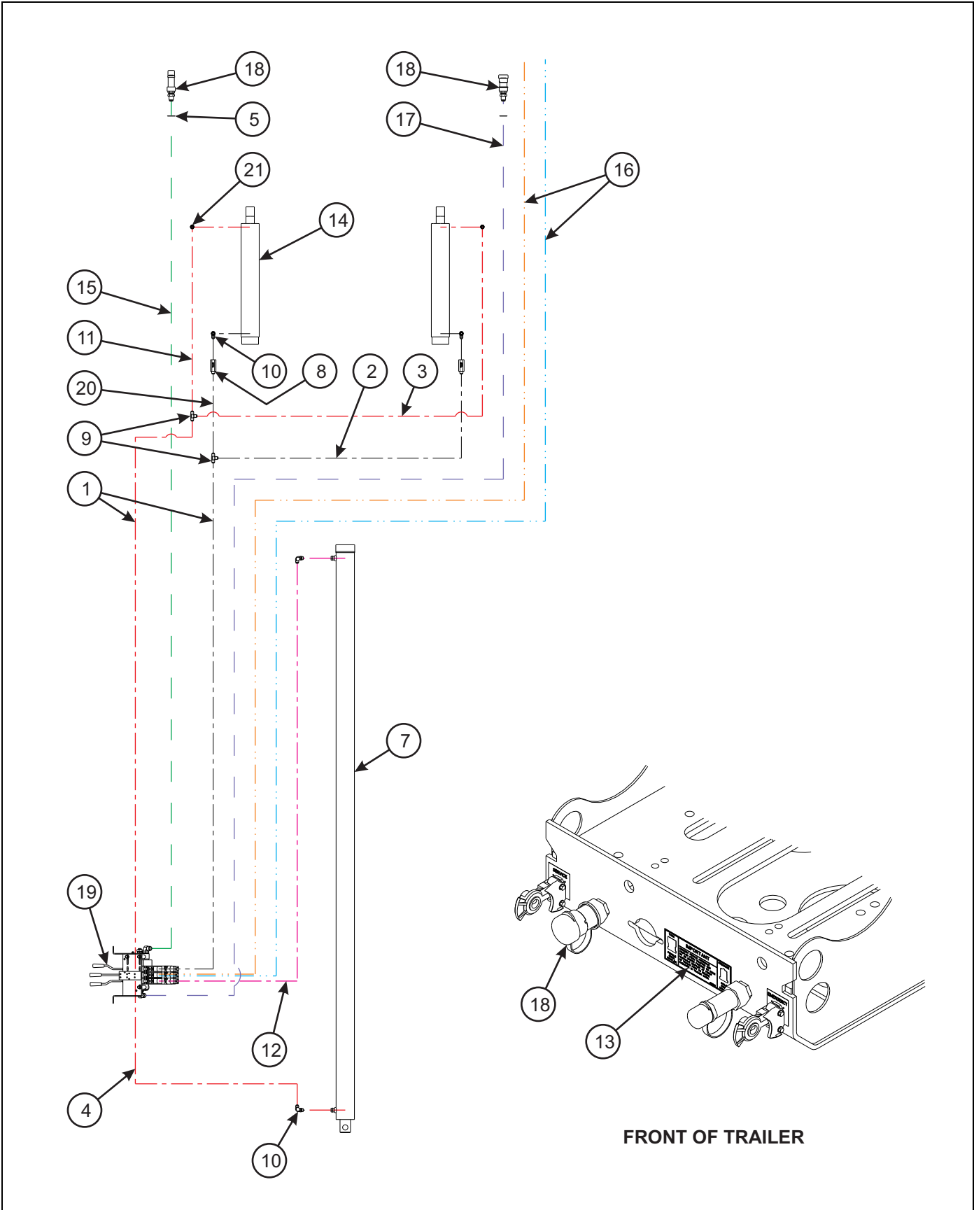
Figure 1-5: Hydraulic System
