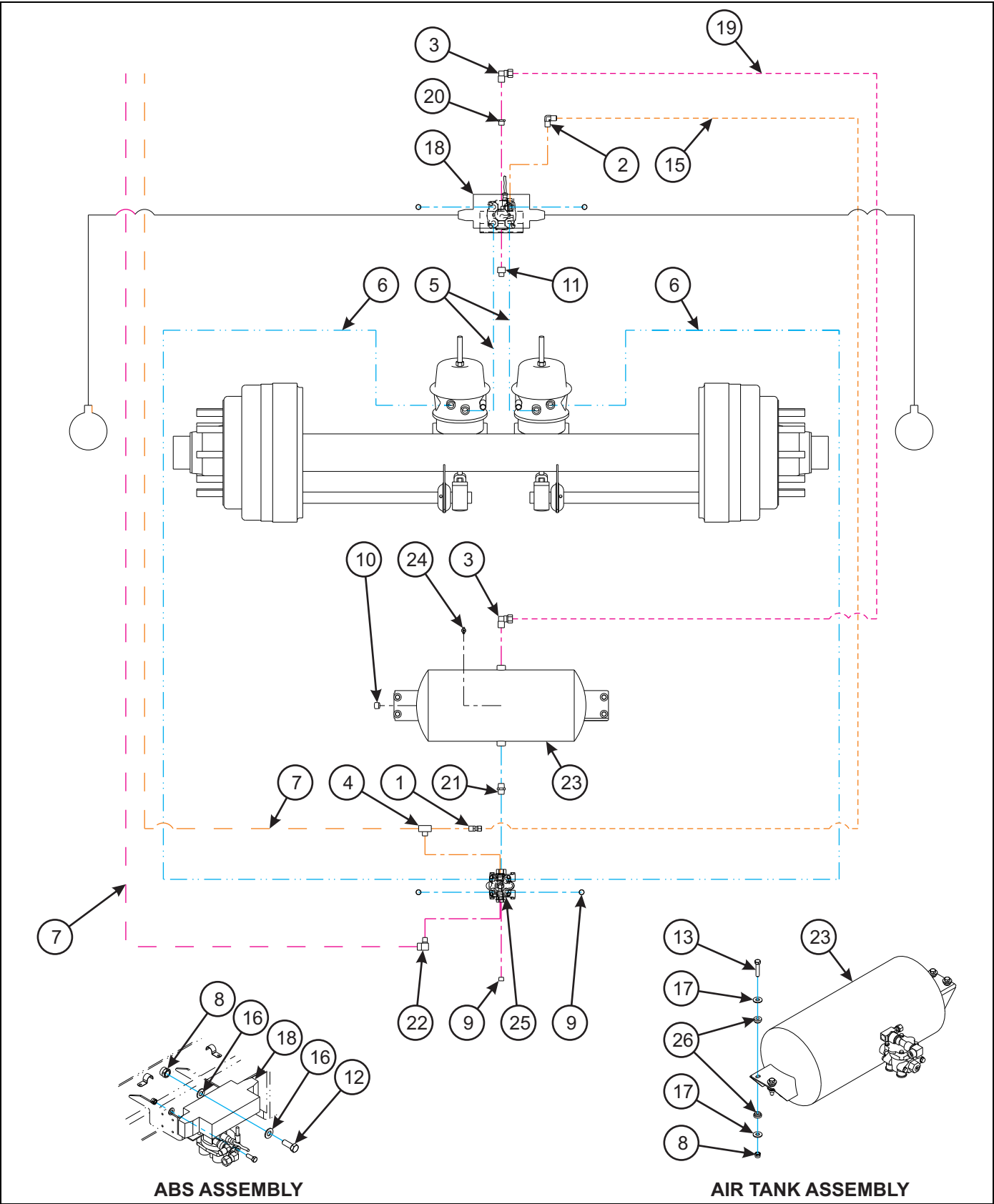
Figure 1-21: Air Brake System
