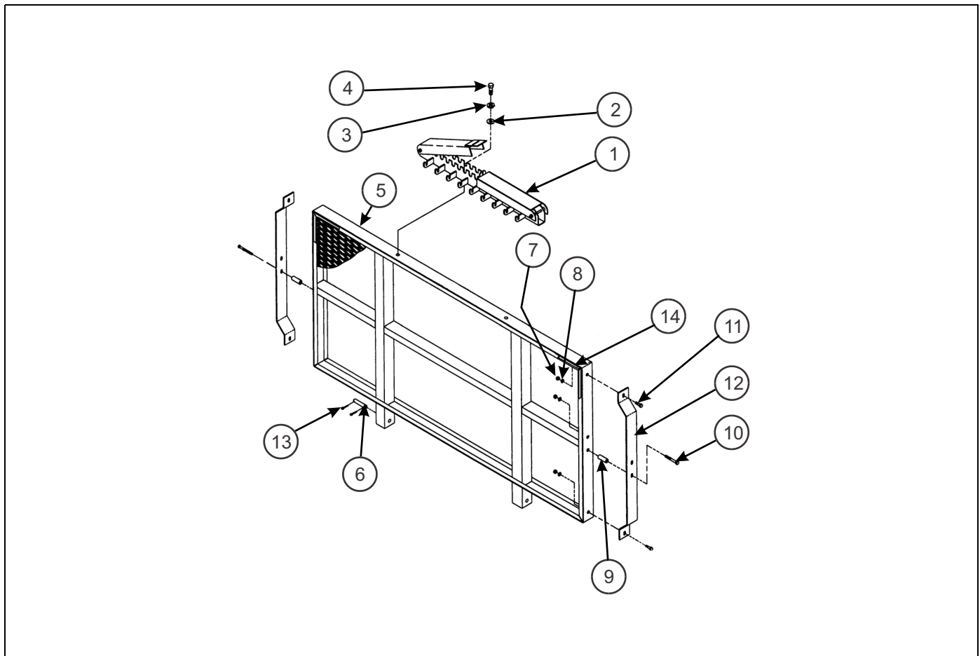
Figure 1-55: Bulkhead Assembly
