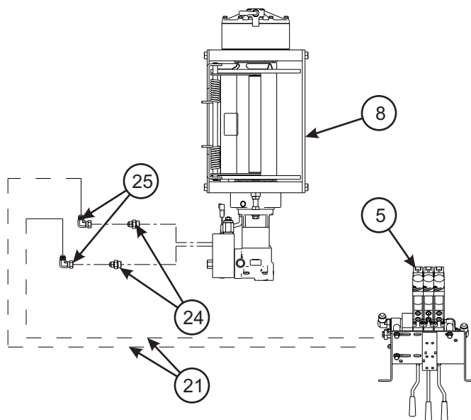
HYDRAULIC SYSTEM
