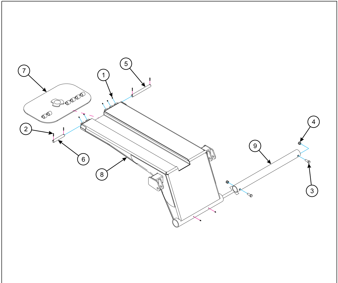
Figure 1-52: Hitch Installation
