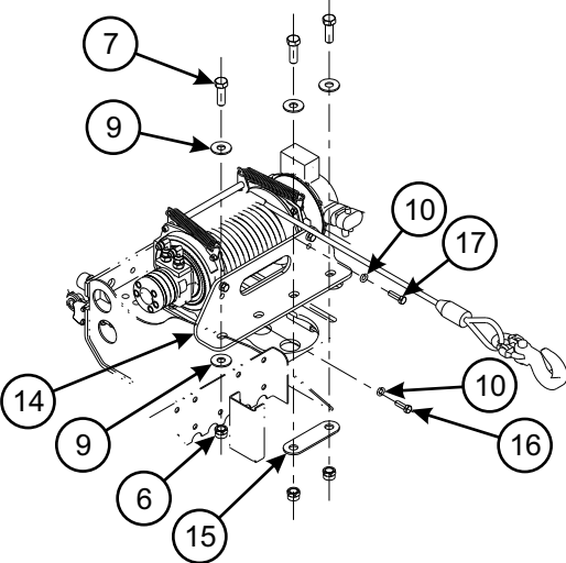
GENERAL ASSEMBLY
