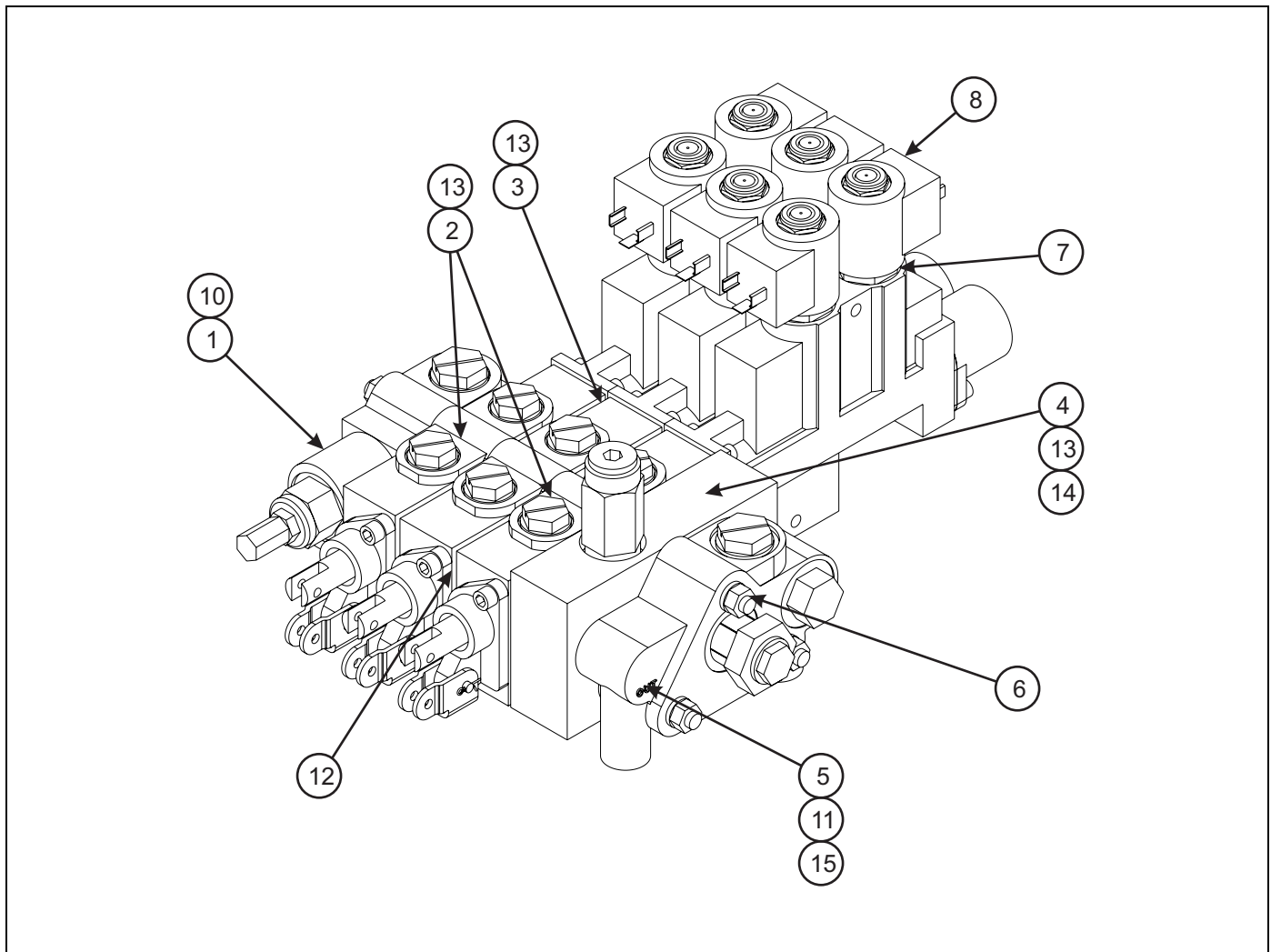
Figure 1-11: Three Stack Valve
