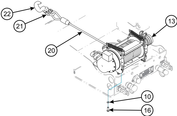
GENERAL ASSEMBLY
