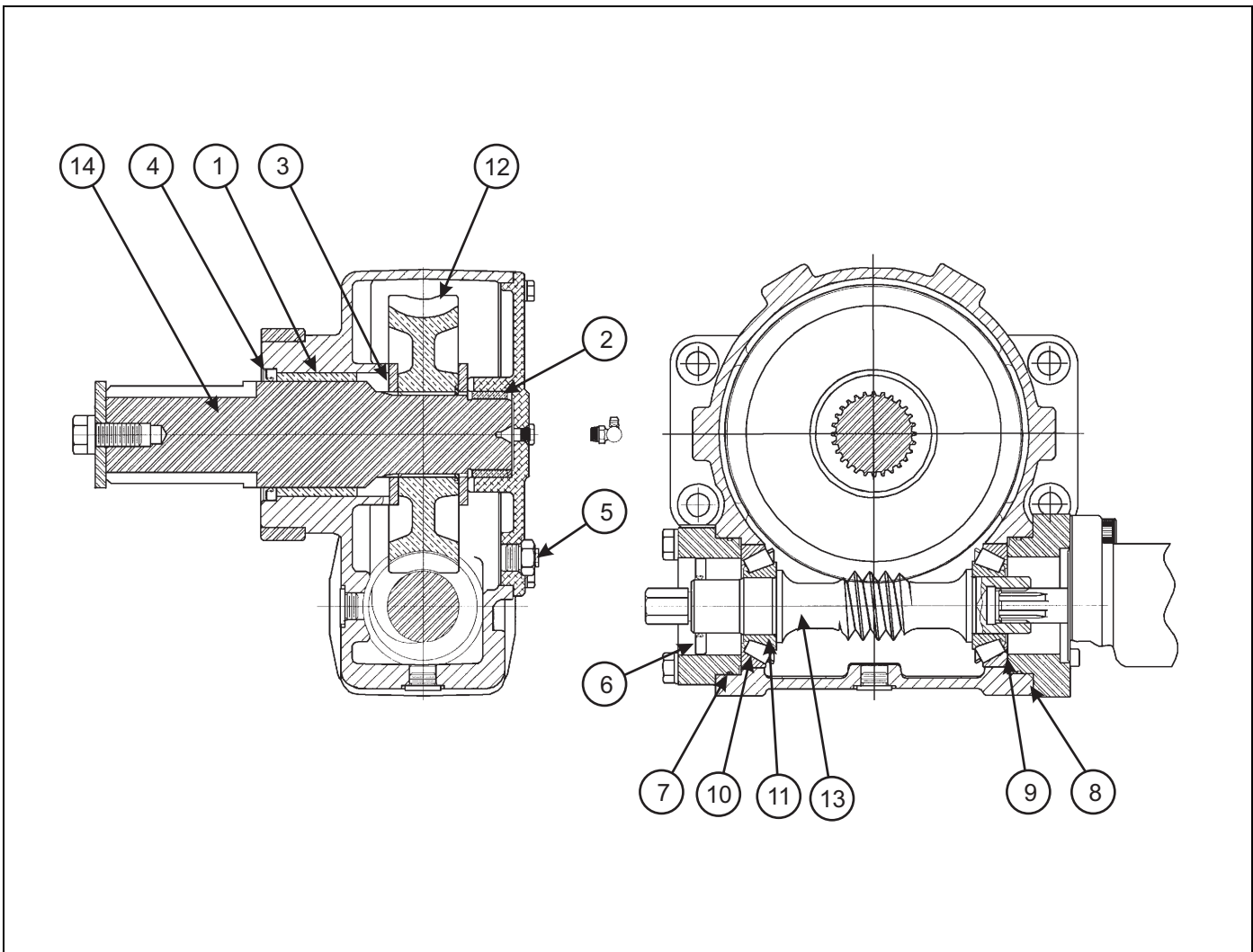
Figure 1-31: Gearbox Items
