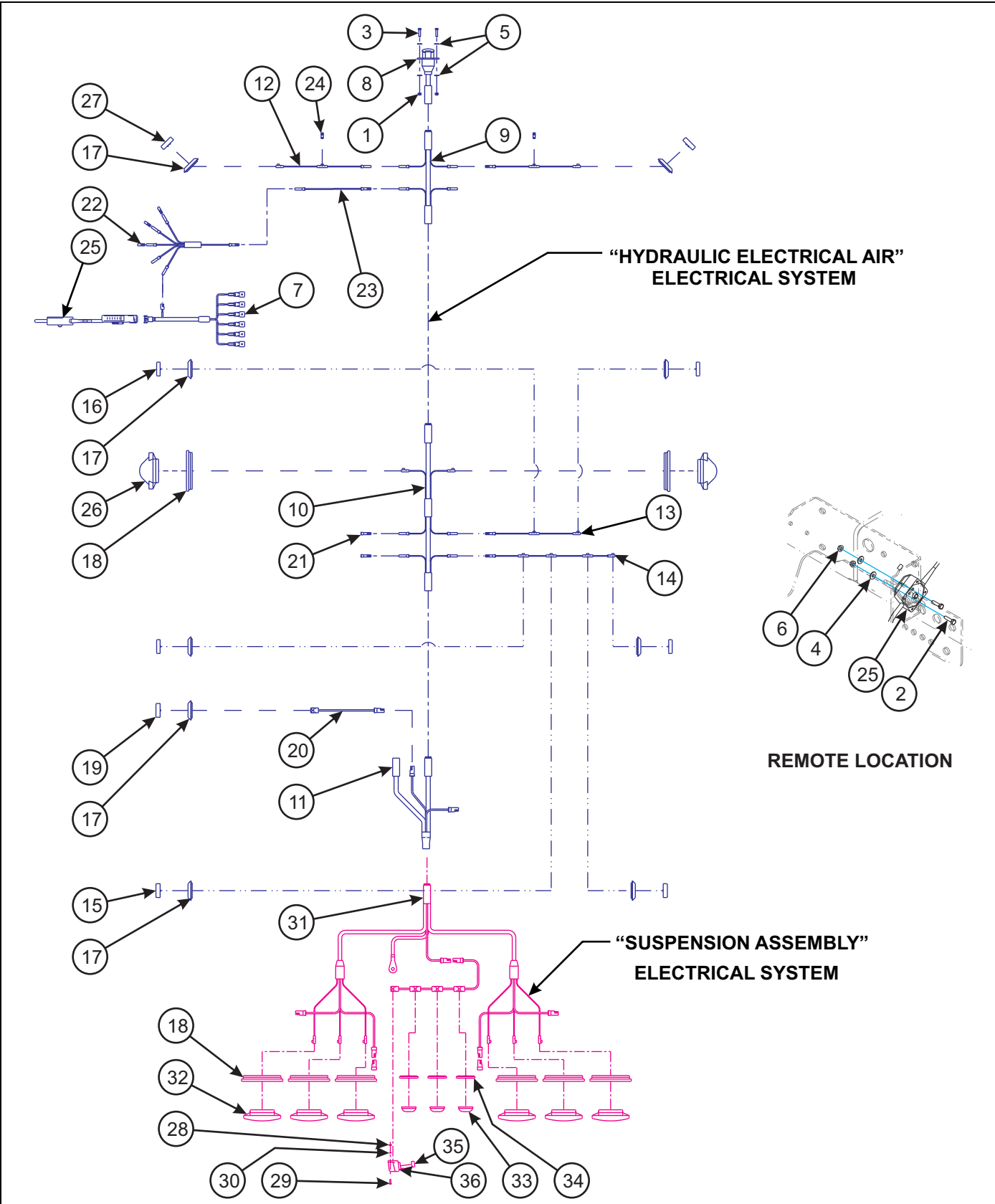
Figure 1-12: Electrical System
