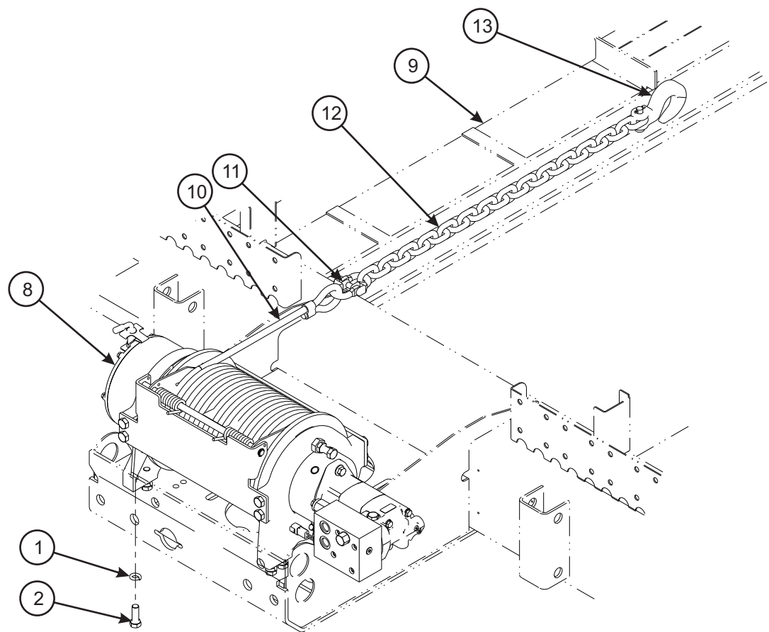
WINCH ASSEMBLY
