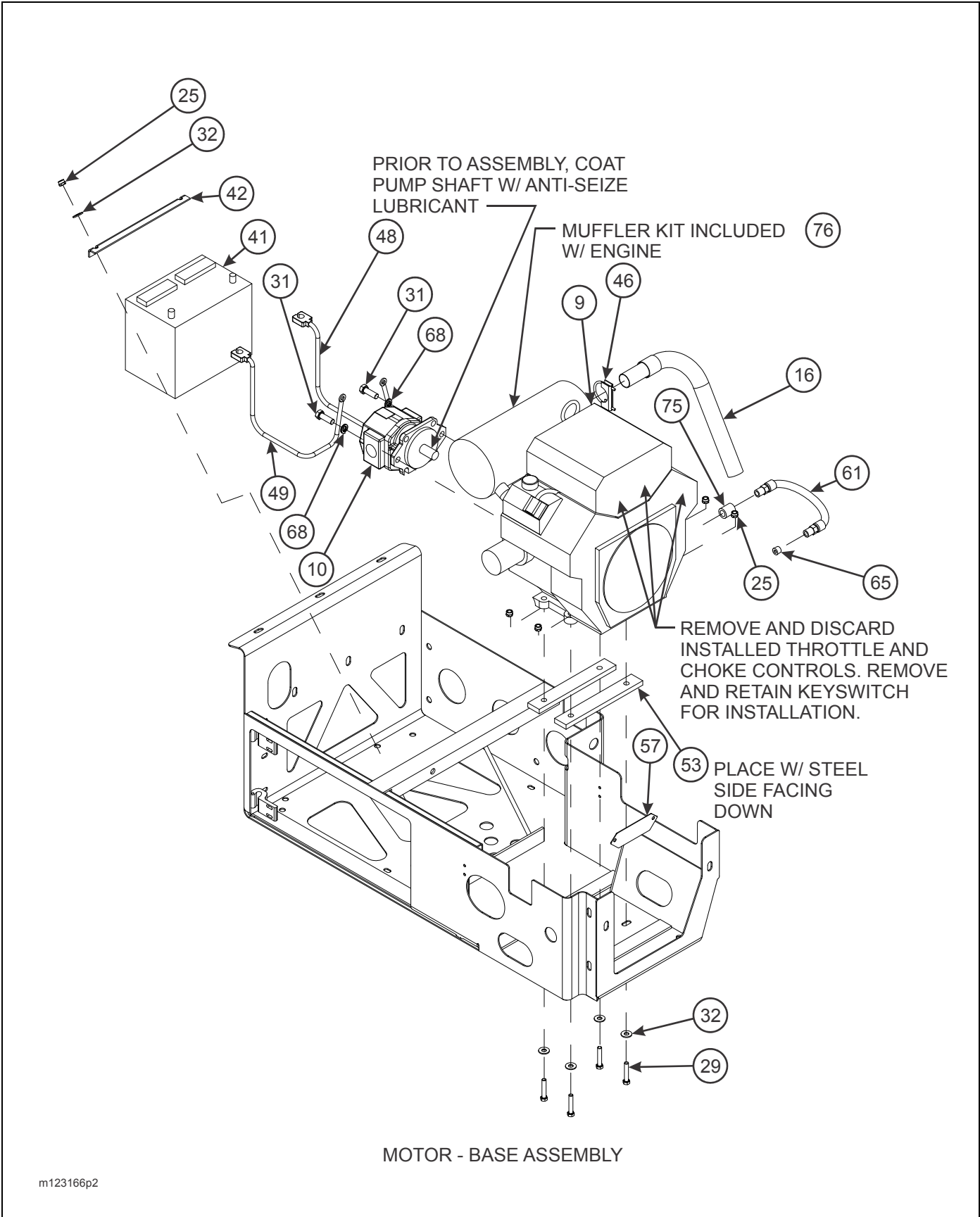
Figure 2-78: Upper Deck Engine Installation (2 of 4)
