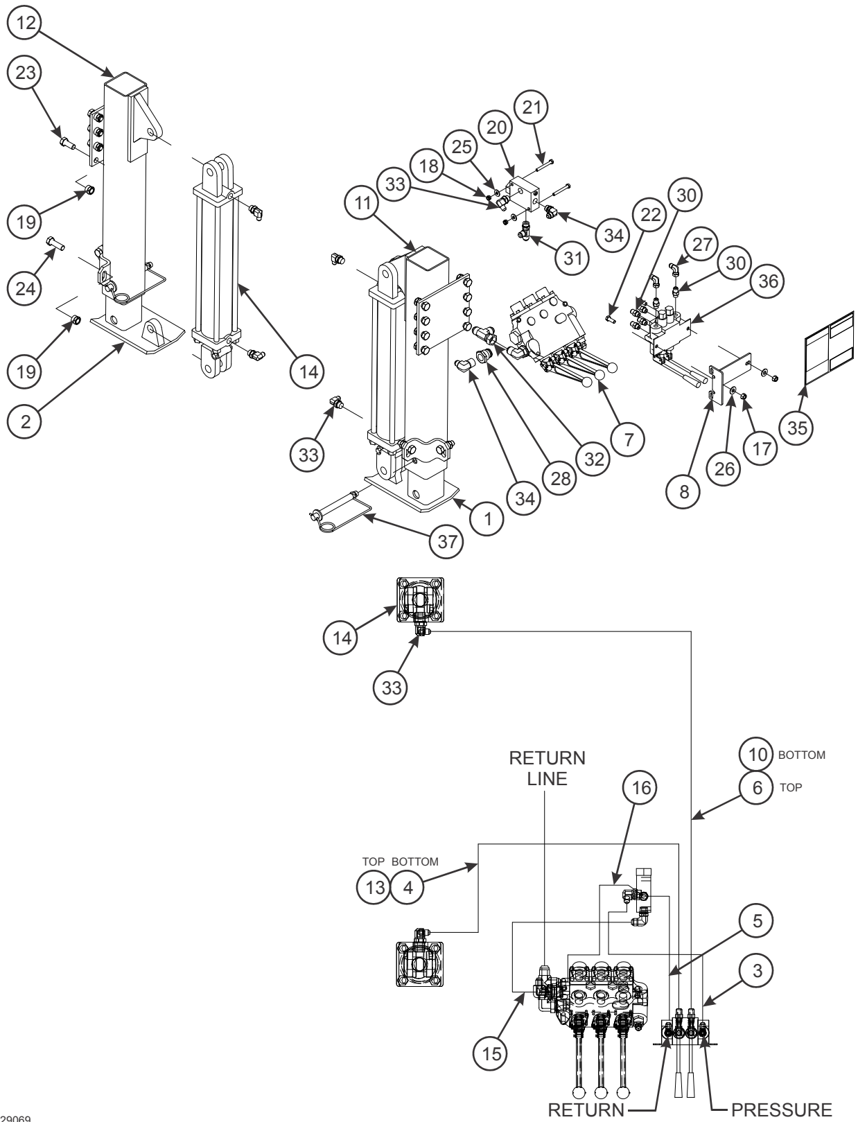
Figure 2-74: Hydraulic Park Stand Installation
