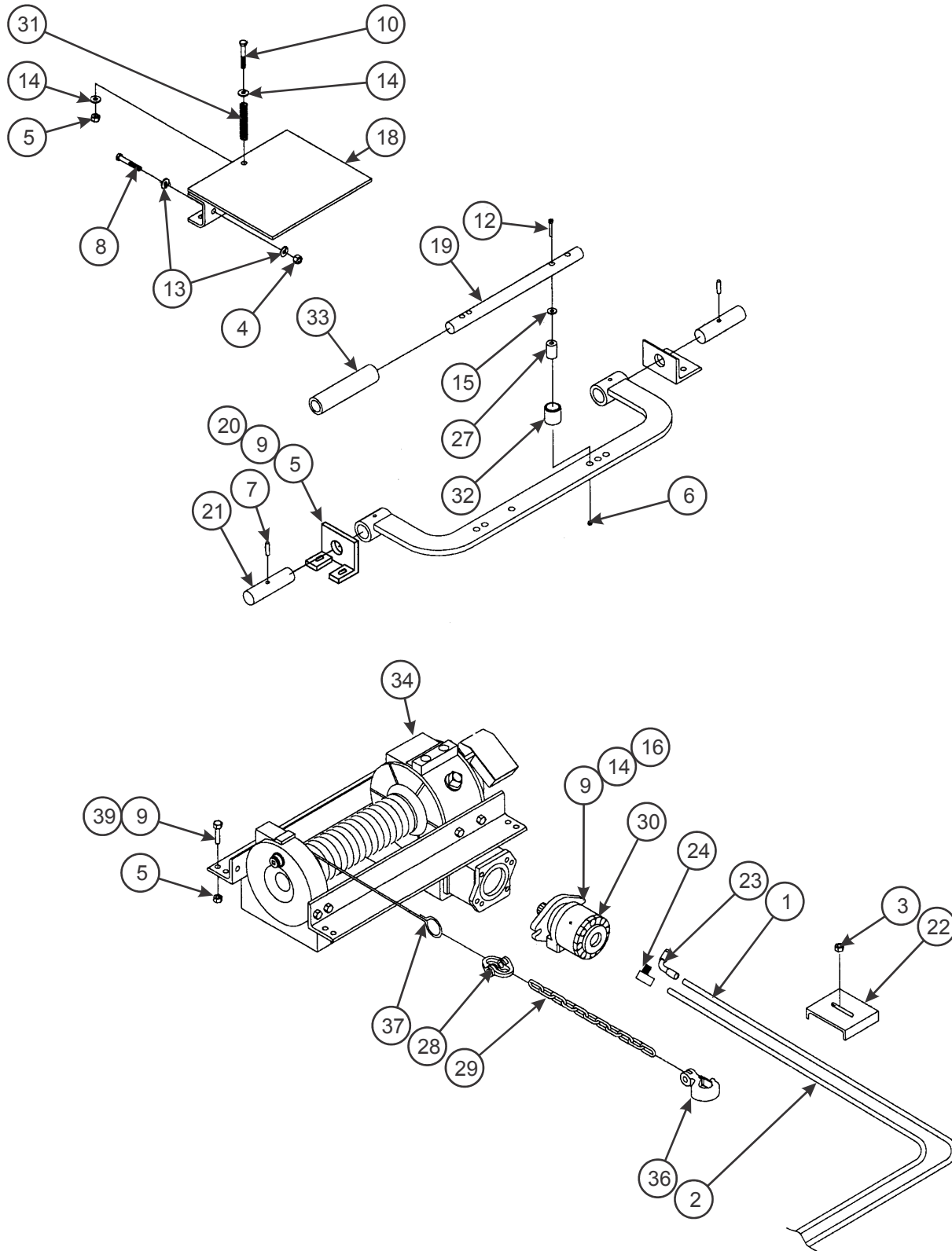
Figure 2-44: Winch Installation, Spring Tension Cable Roller
