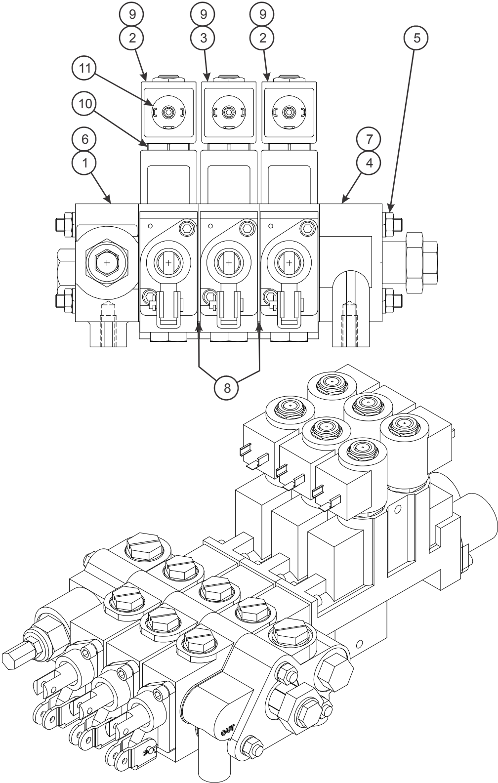
Figure 2-10: Three Spool Valve
