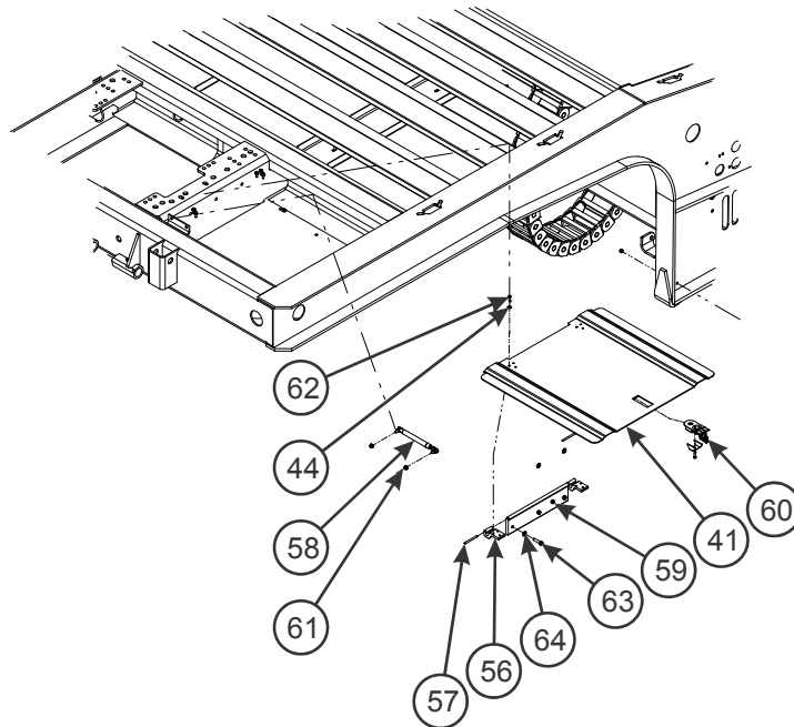
GALVANIZED FLIP-UP TOOLBOX OPTION
