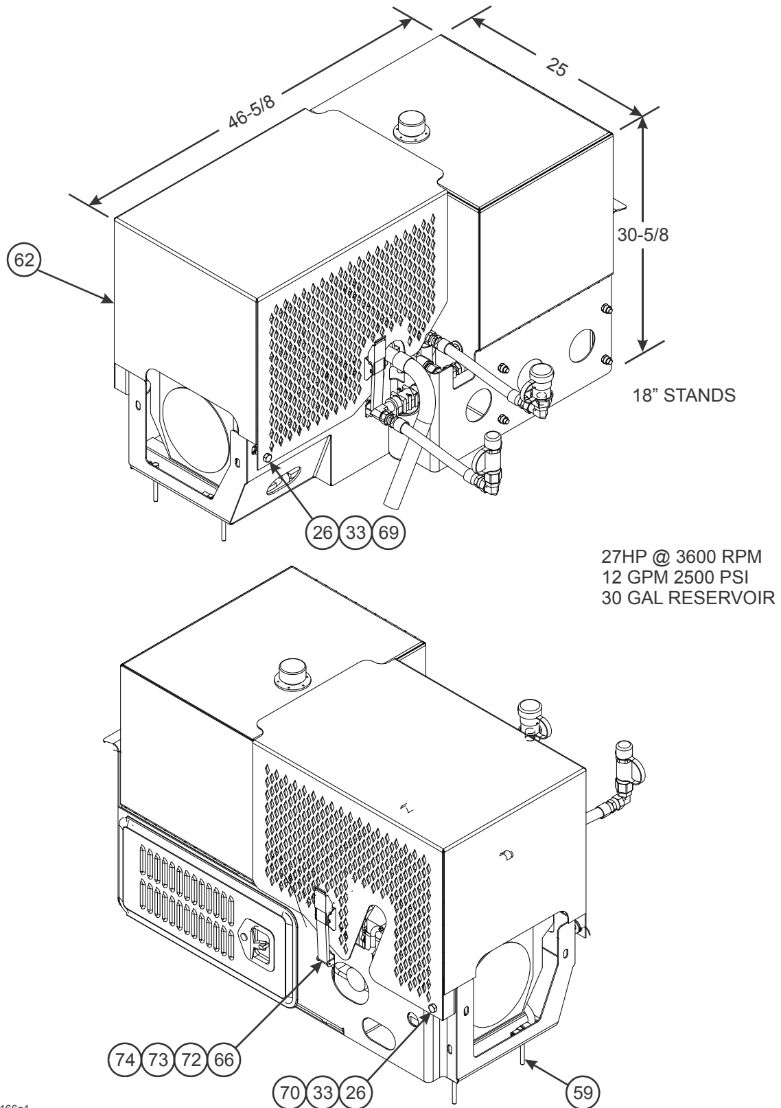
Figure 2-77: Upper Deck Engine Installation (1 of 4)
