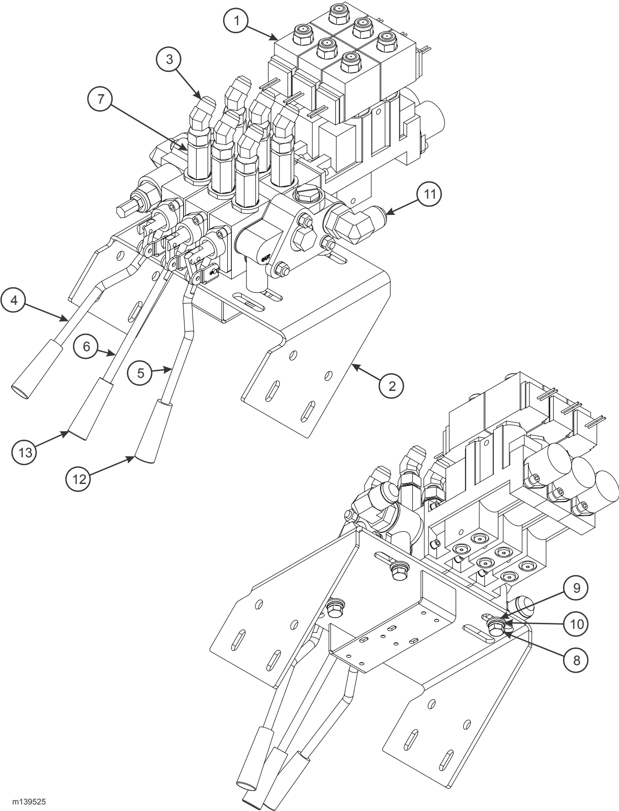
Figure 2-9: Three Spool Valve Assembly
