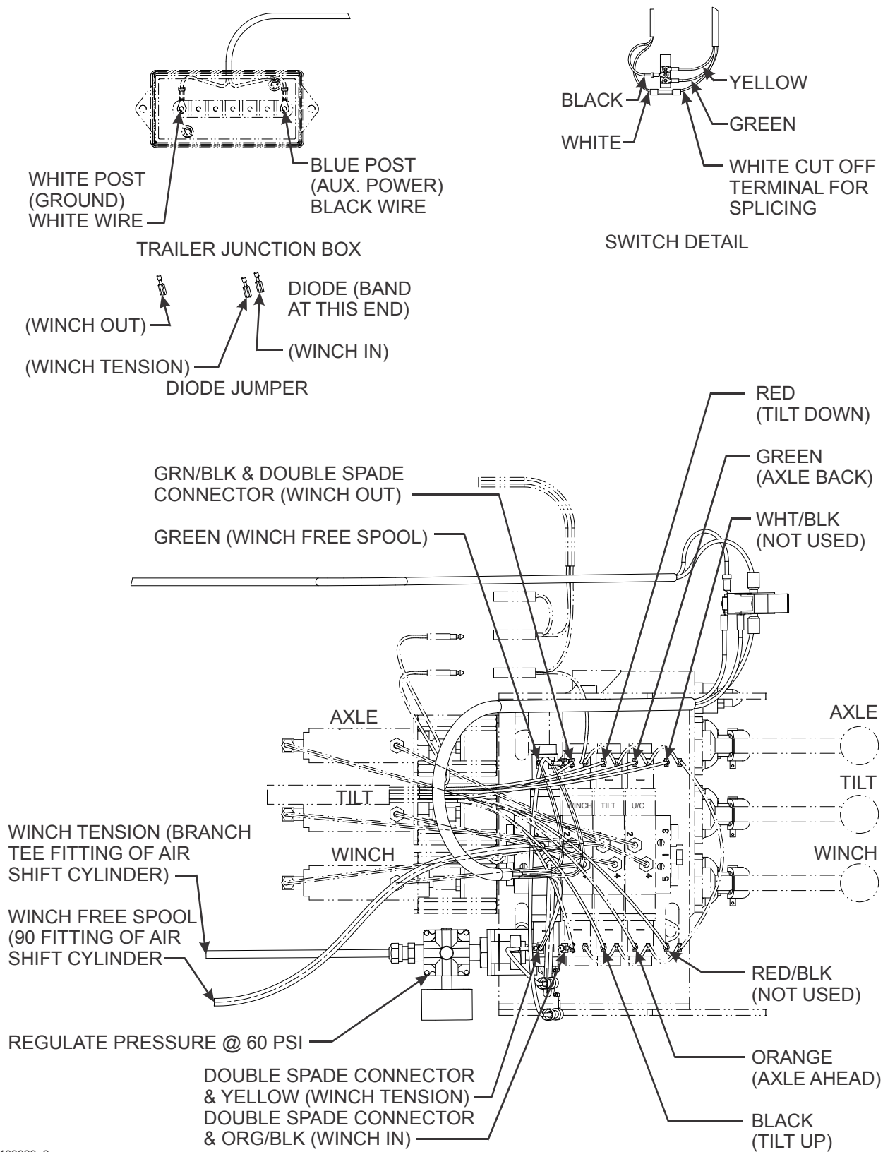
Figure 2-43: Winch Installation (2 of 2)
