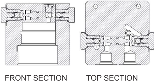
STABILIZER LEG CHECK VALVE (PRIOR TO 03/19/2010)
