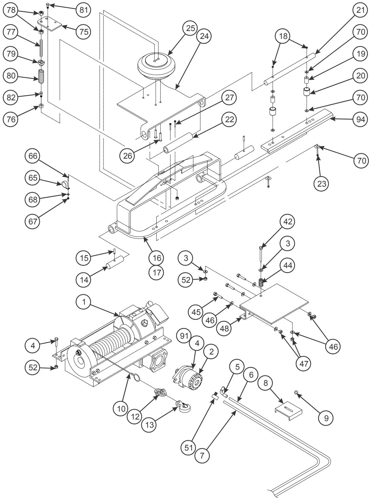
Figure 2-40: Winch Installation (1 of 2)
