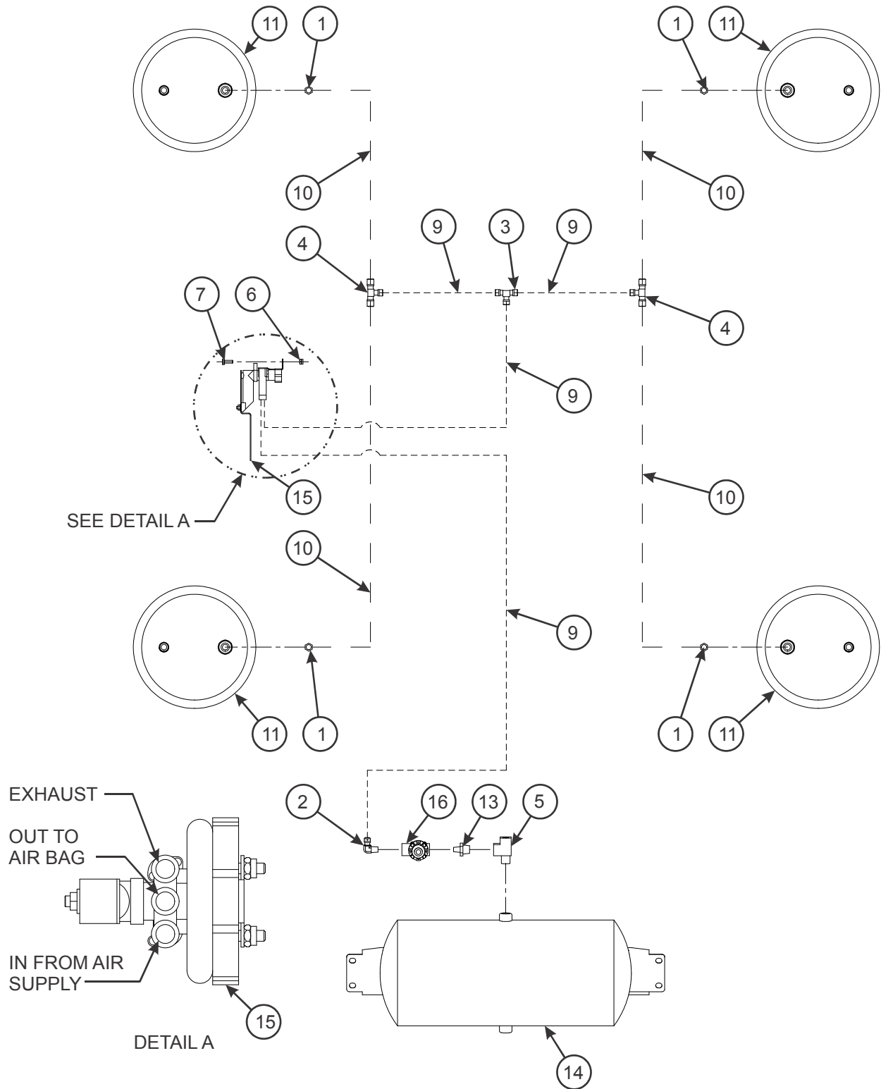
Figure 2-30: Air Ride Suspension, Air System (Tandem)
