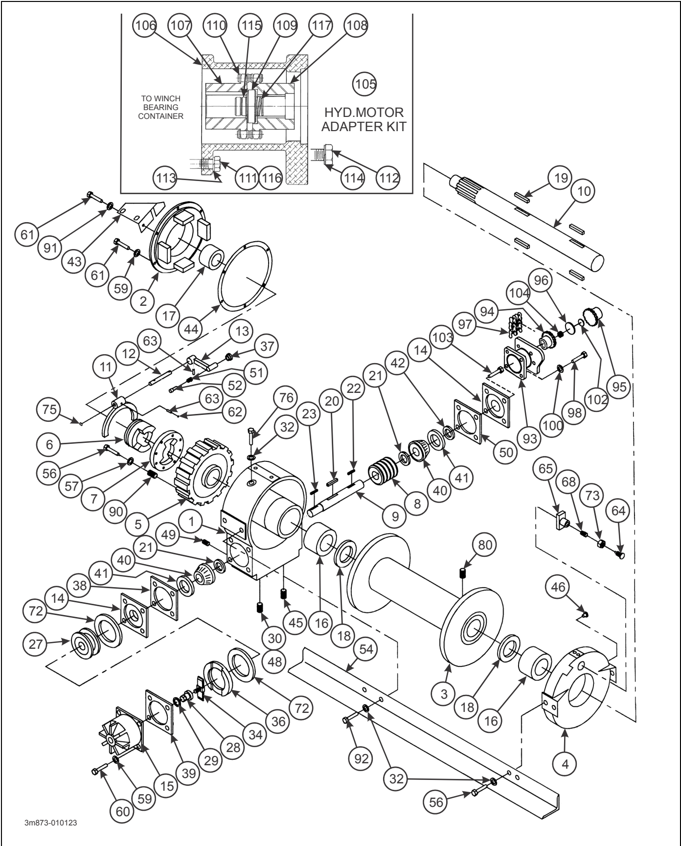
Figure 2-46: 20,000 Lb. Winch Items
