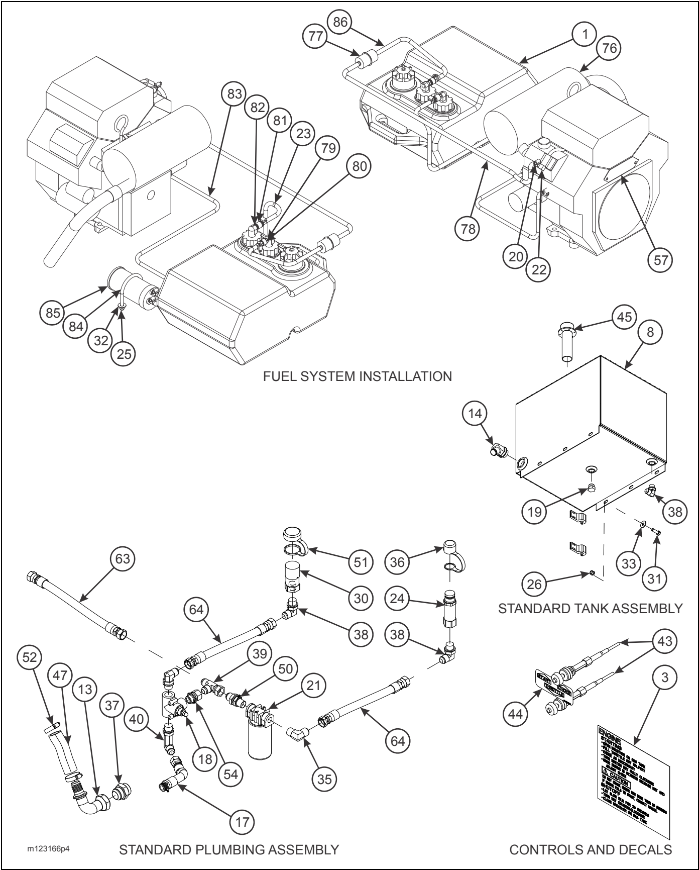
Figure 2-80: Upper Deck Engine Installation (4 of 4)
