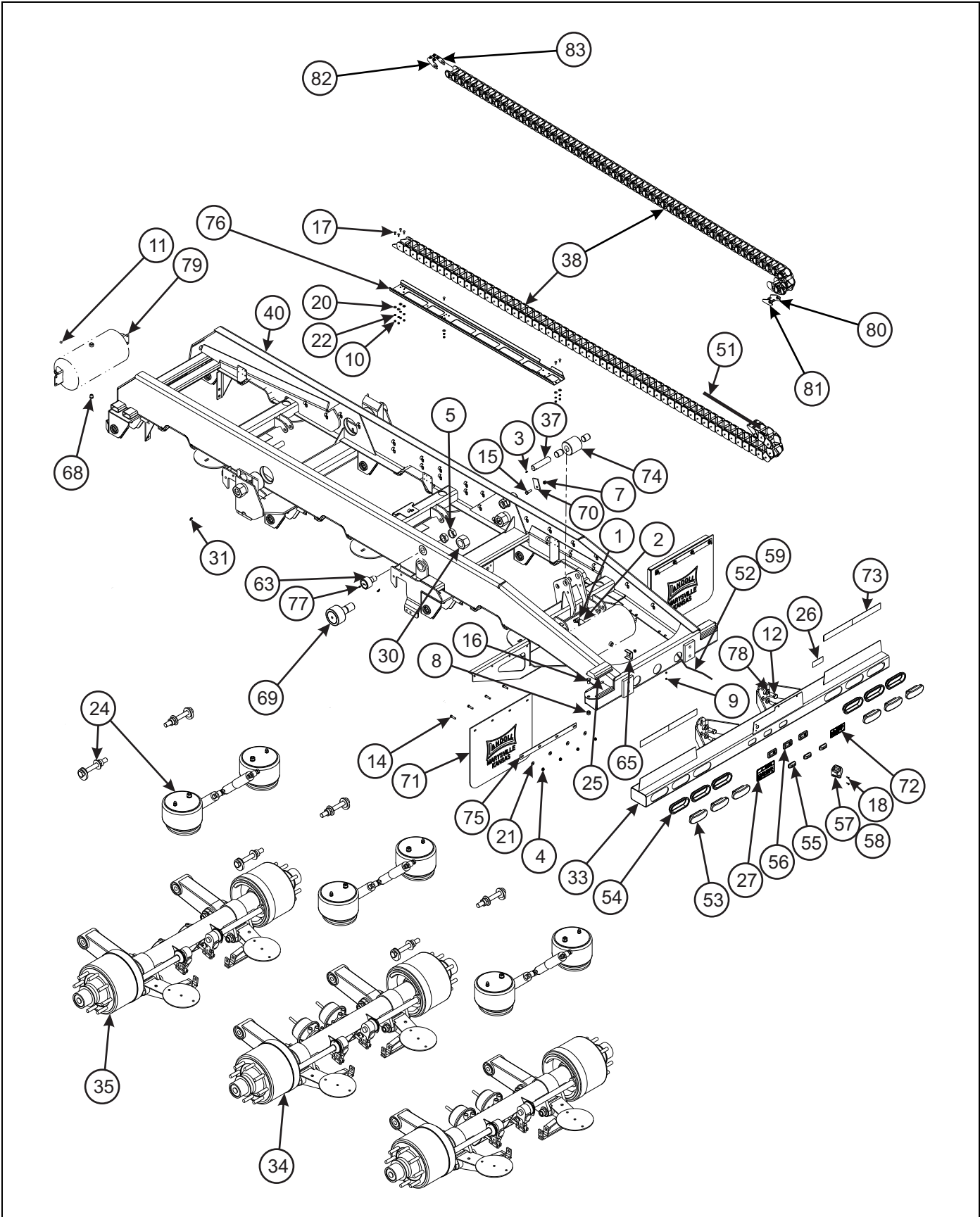
Figure 2-22: U/C Assembly, Air Ride Suspension (410) (1 of 4)
