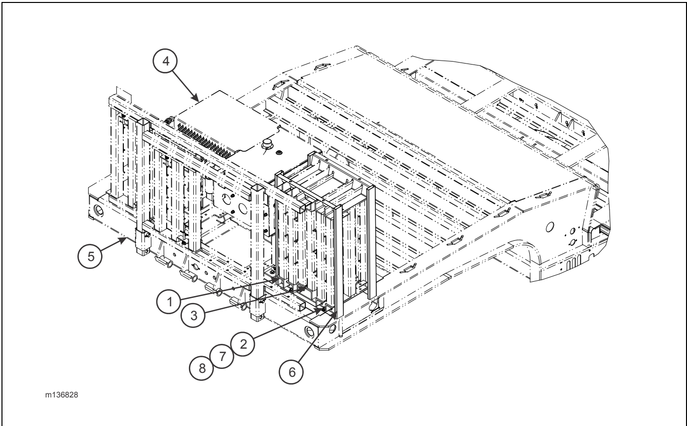
Figure 2-90: Upper Deck Extension Bridge Storage Rack (Option)
