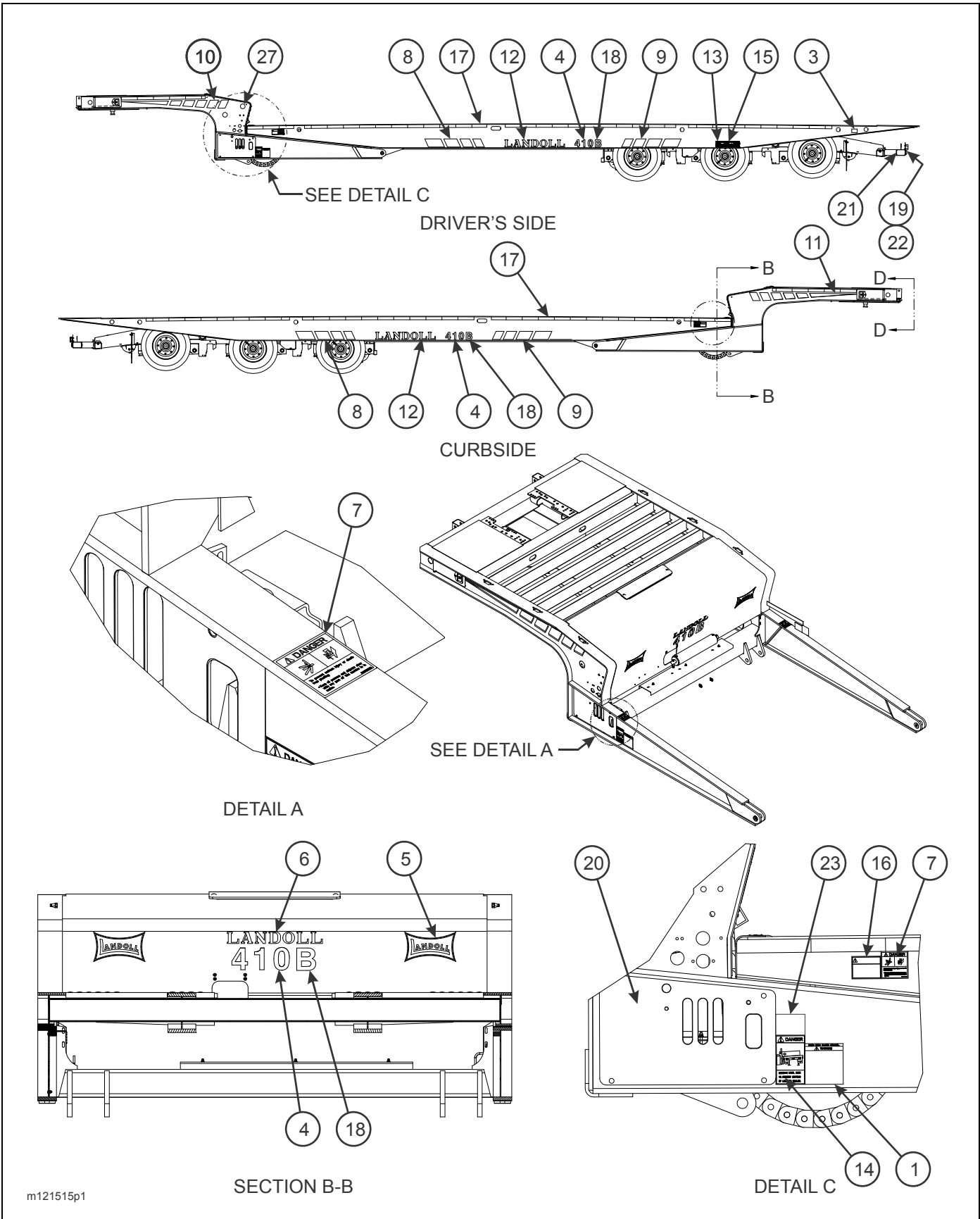
Figure 2-70: Decal Installation (1 of 2)
