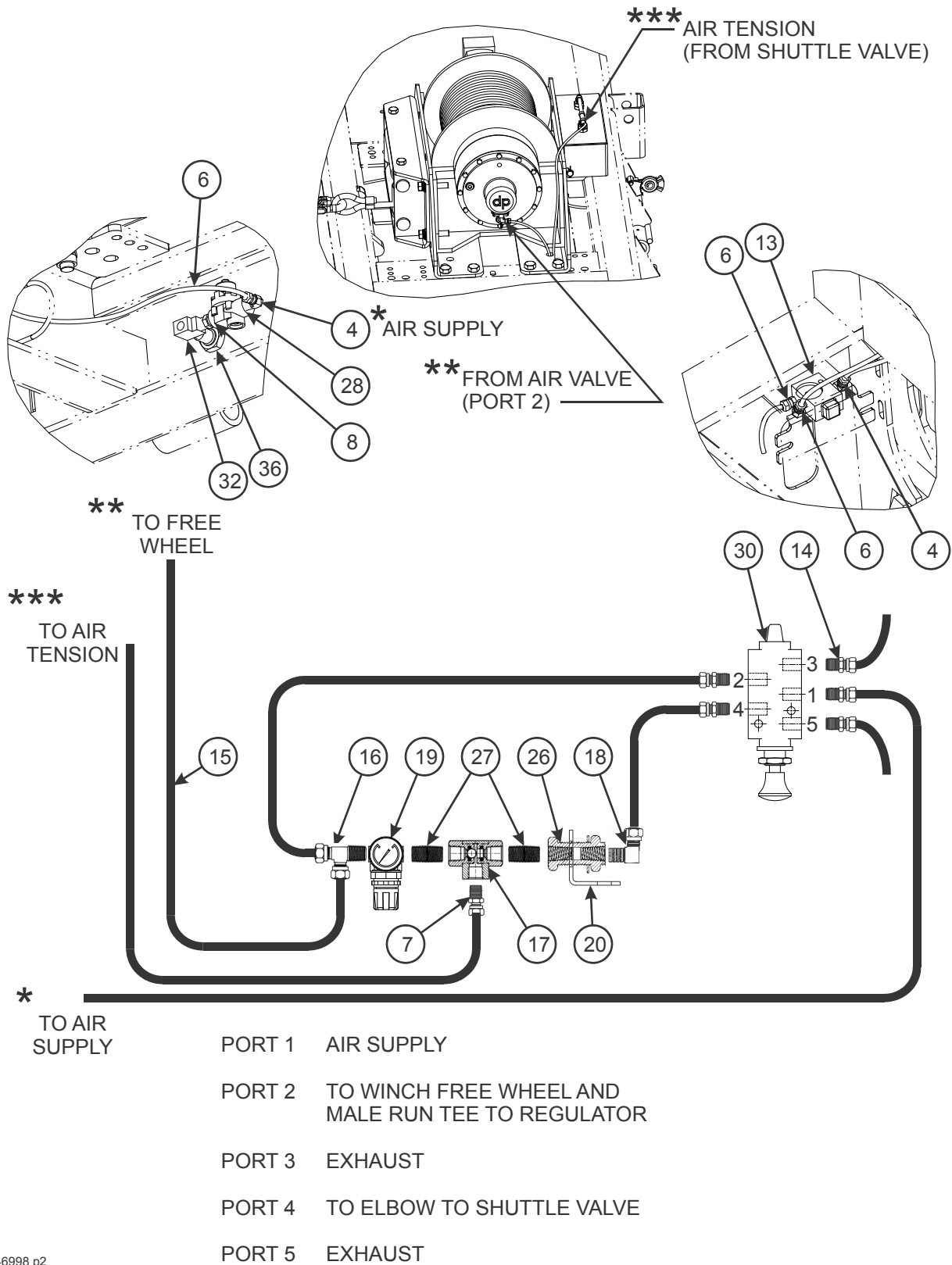
Figure 2-51: 30,000 Lb. Upper Deck Winch Installation (3 of 3)
