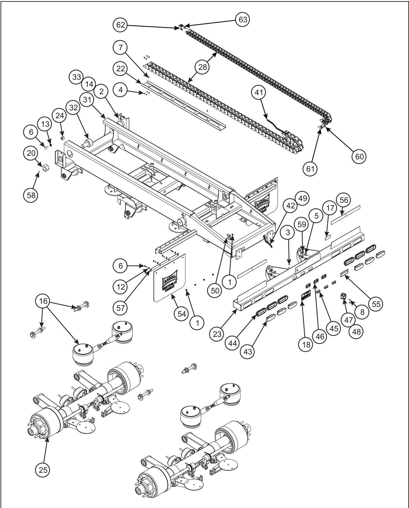
Figure 2-26: U/C Assembly, Air Ride Suspension (425 & 435) (1 of 4)
