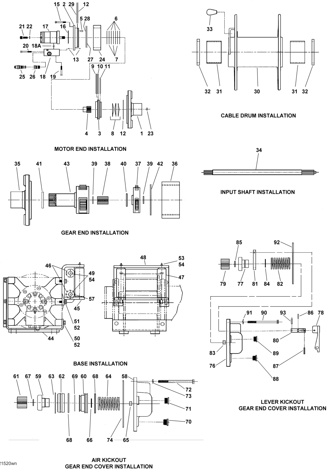
Figure 2-59: 12K, 15K, & 20K Winch Items (DP Planetary)
