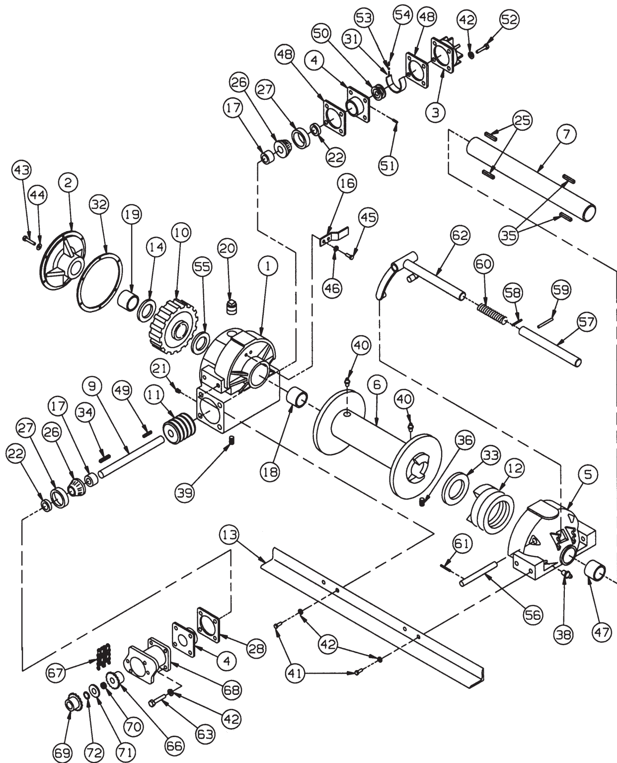
Figure 1-34 12,000# Winch Items
