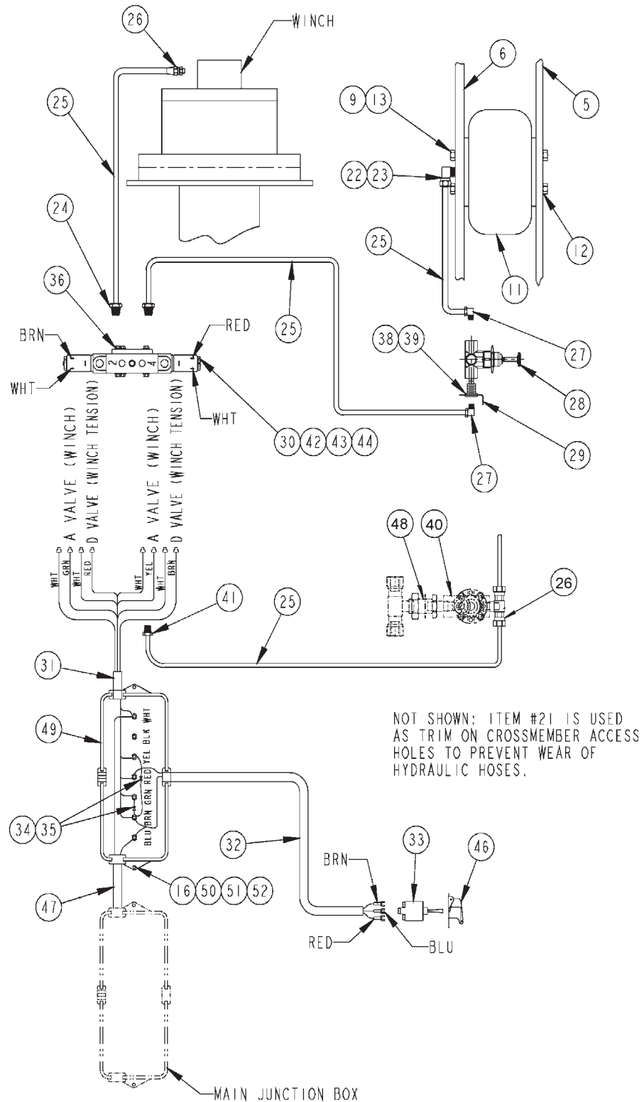
Figure 1-46 12K, 15K, & 20K Upper Deck Winch (DP) (2 of 2)
