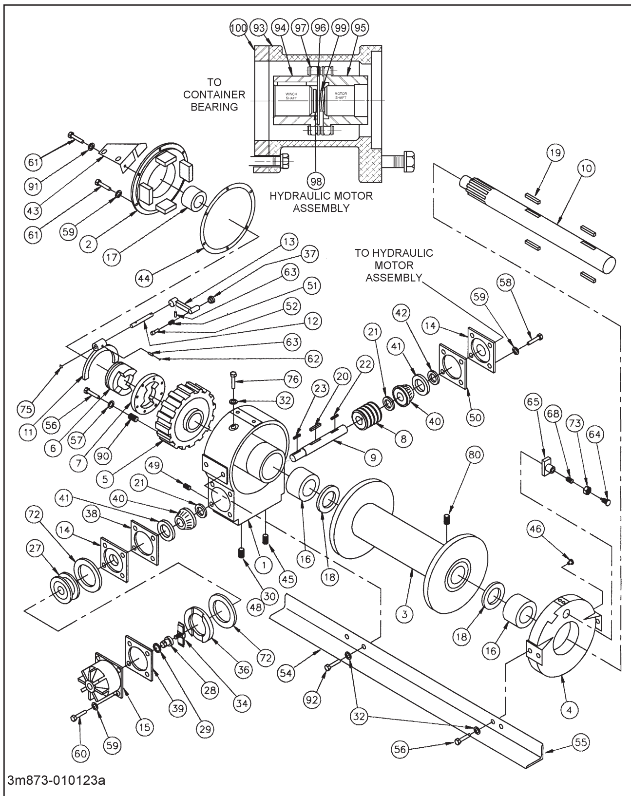
Figure 1-35 20,000# Winch Items
