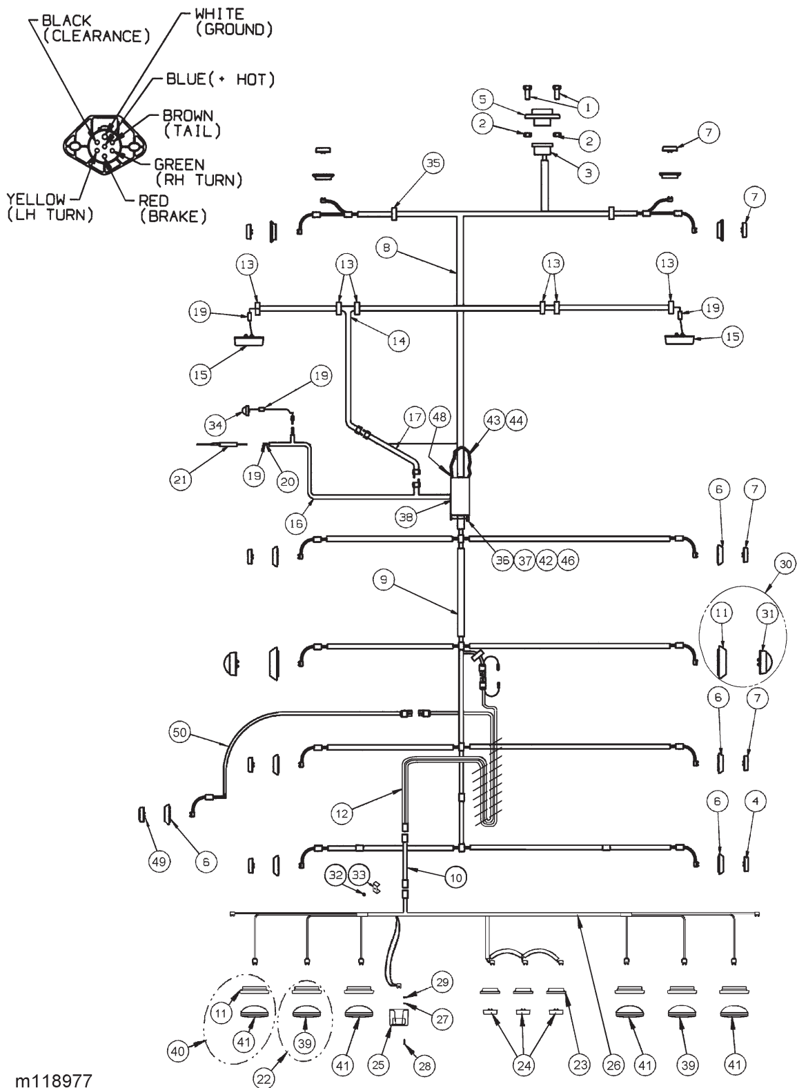
Figure 1-18 Electrical System Schematic
