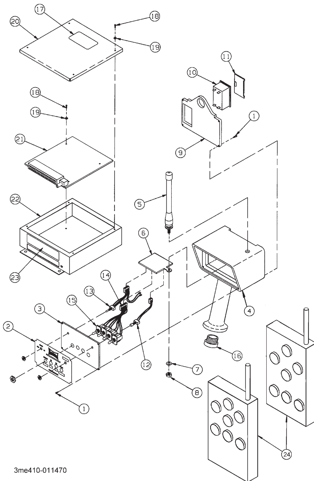
Figure 1-53 Wireless Remote Control
