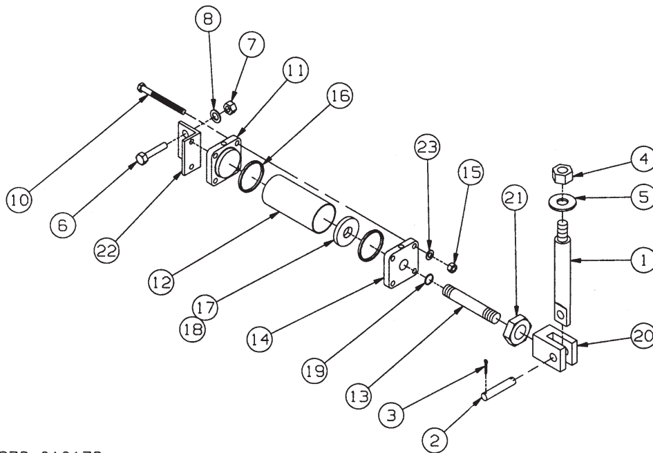
Figure 1-36 Winch Air Shift Cylinder for 20,000# Winch
