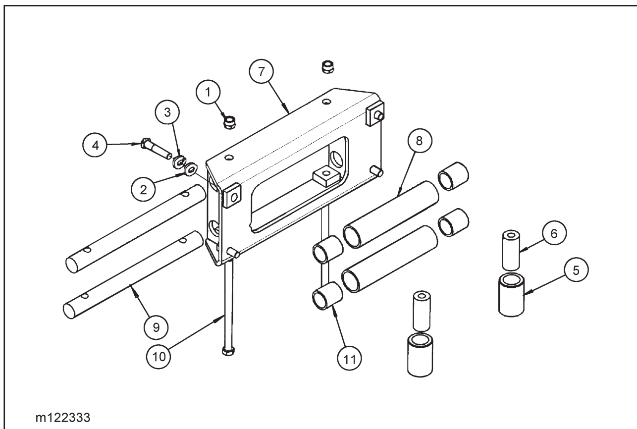
Figure 1-43 Winch Roller Guide - 30K
