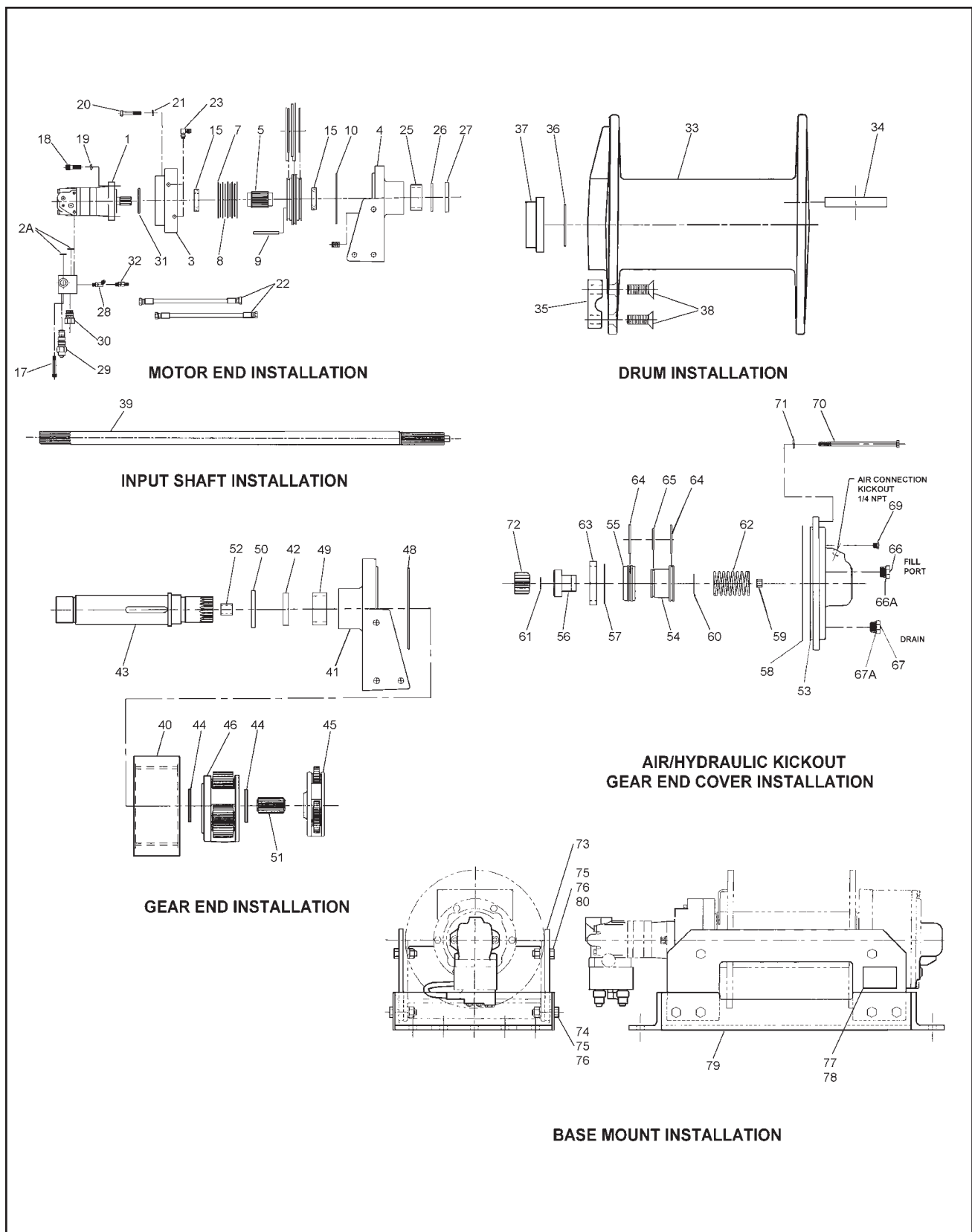
Figure 1-40 30,000# Winch Items
