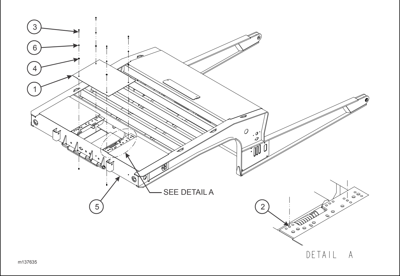
Figure 2-109: Upper Deck Cover Assembly (Option)
