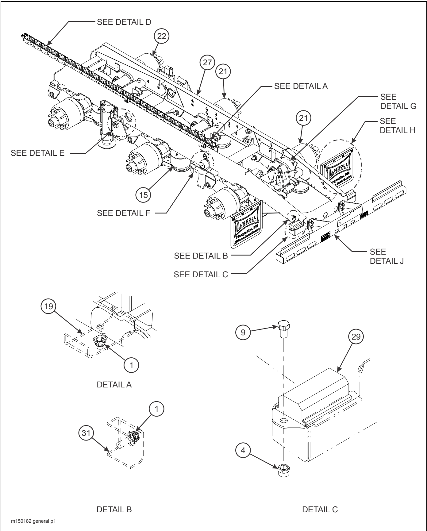
Figure 2-33: Suspension Assembly, General Items (455) (1 of 2)
