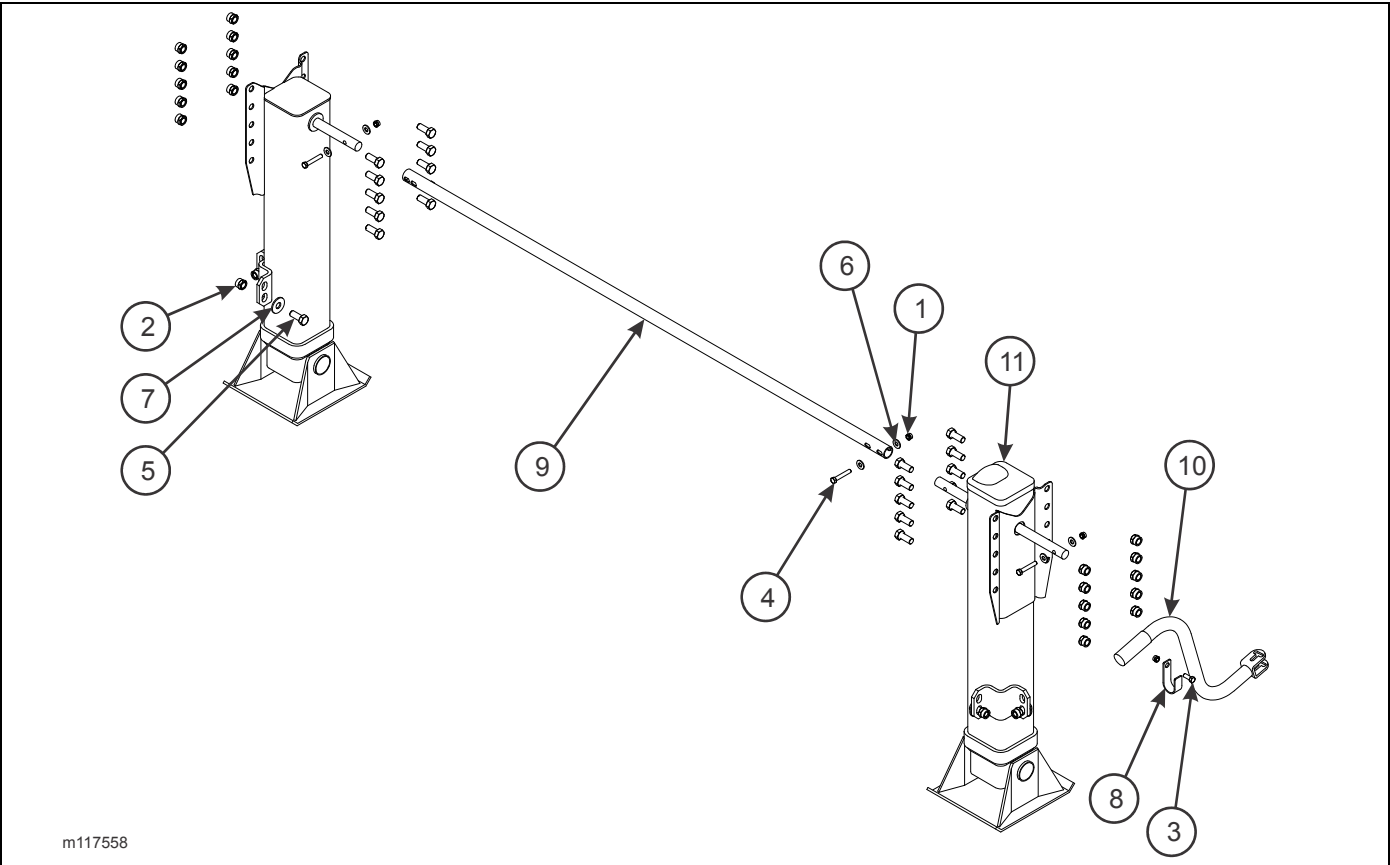
Figure 2-135: Landing Gear Installation
