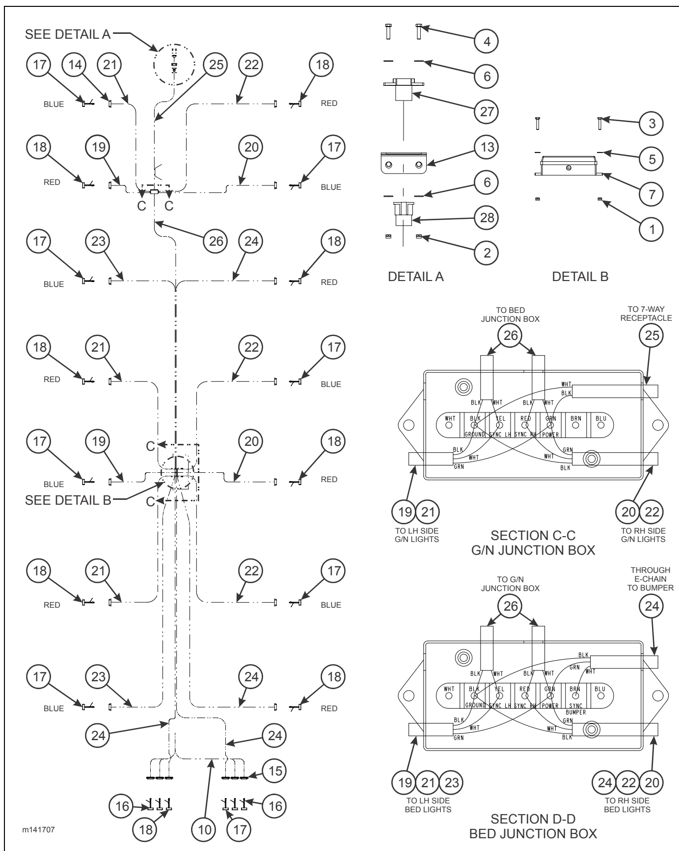
Figure 2-171: Strobe Installation (Option)
