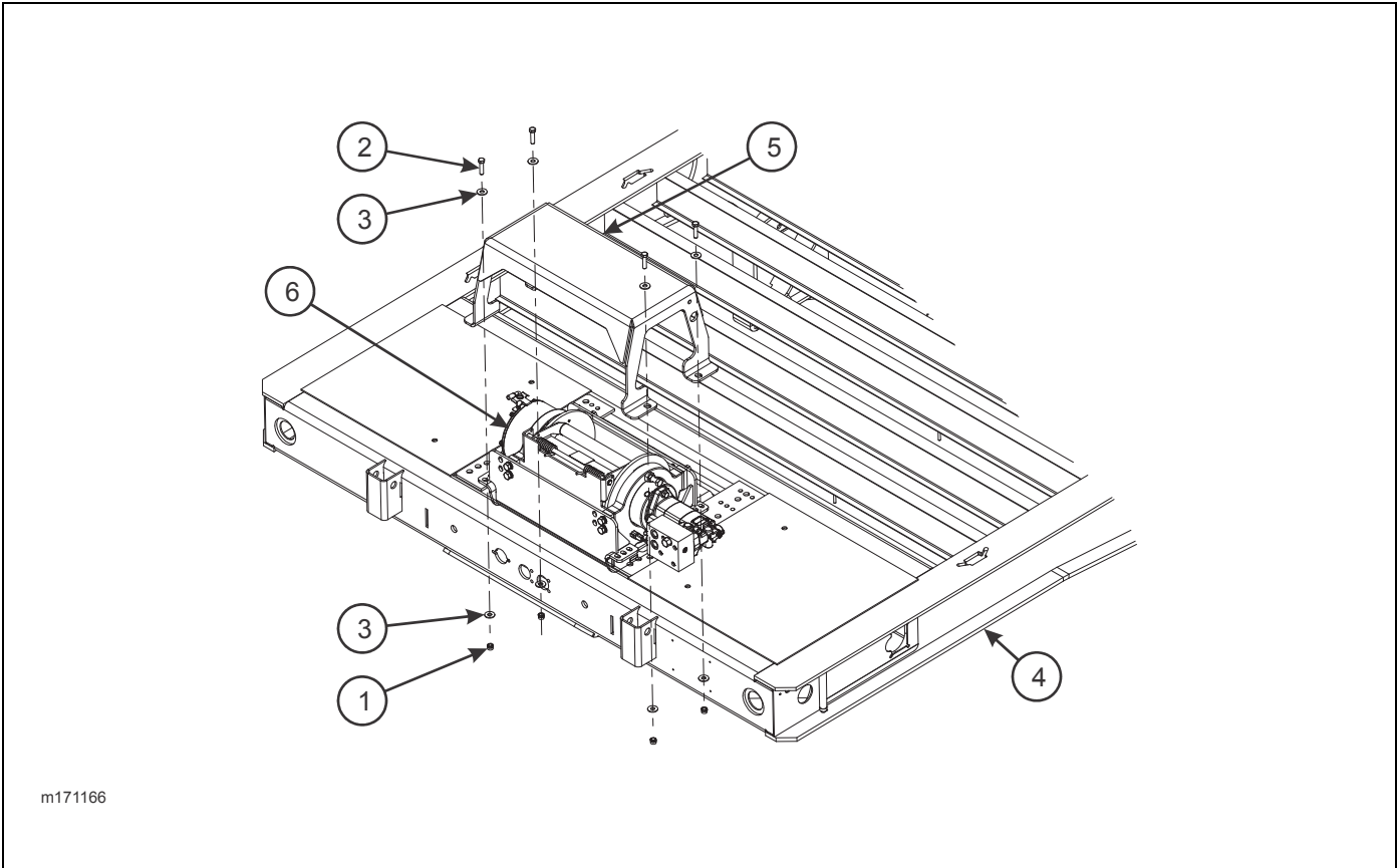
Figure 2-121: Winch Guard Installation for 20K/30K Warn Winch (Option)
