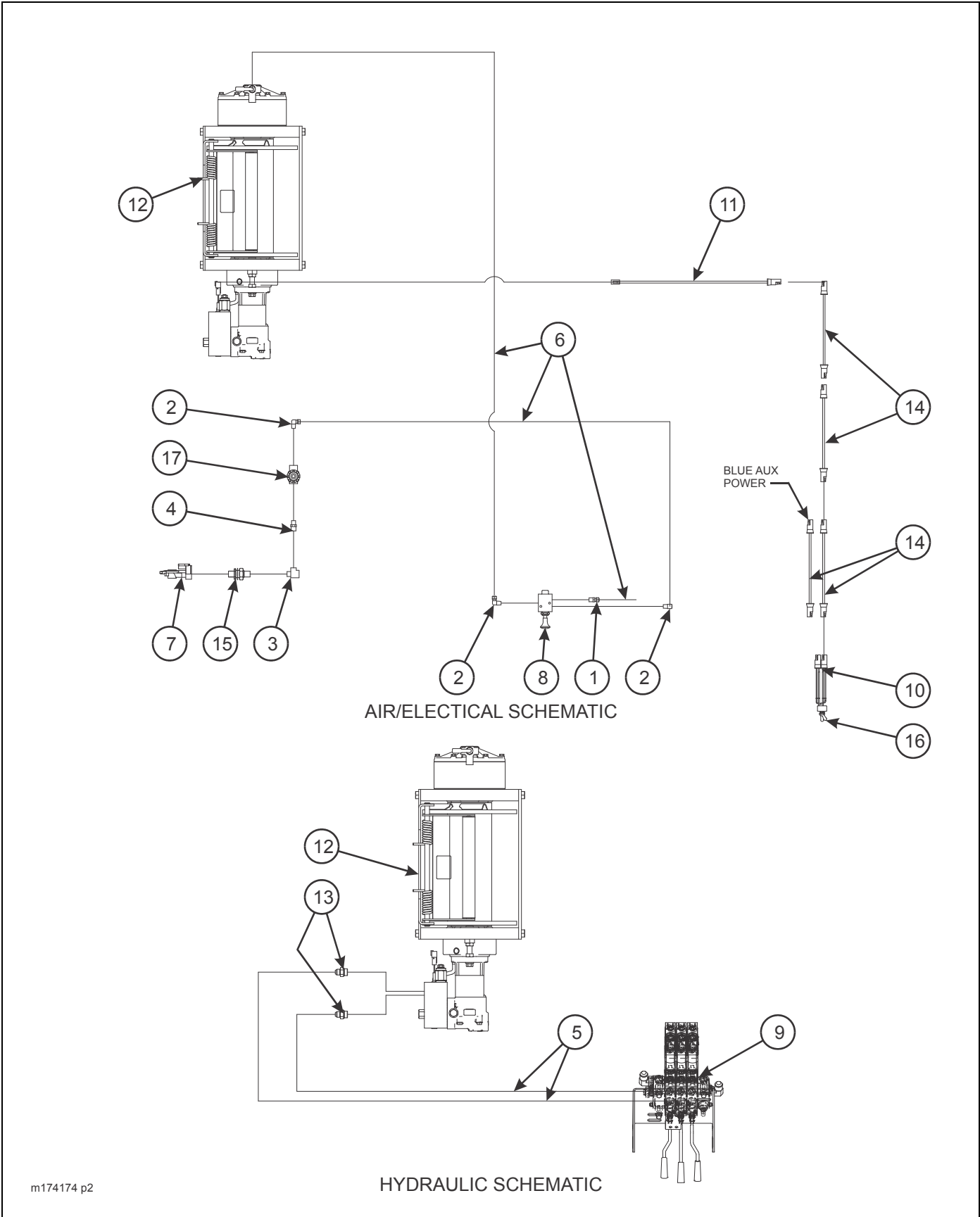
Figure 2-77: Winch Installation, 20K 2 Speed General Items (Warn)
