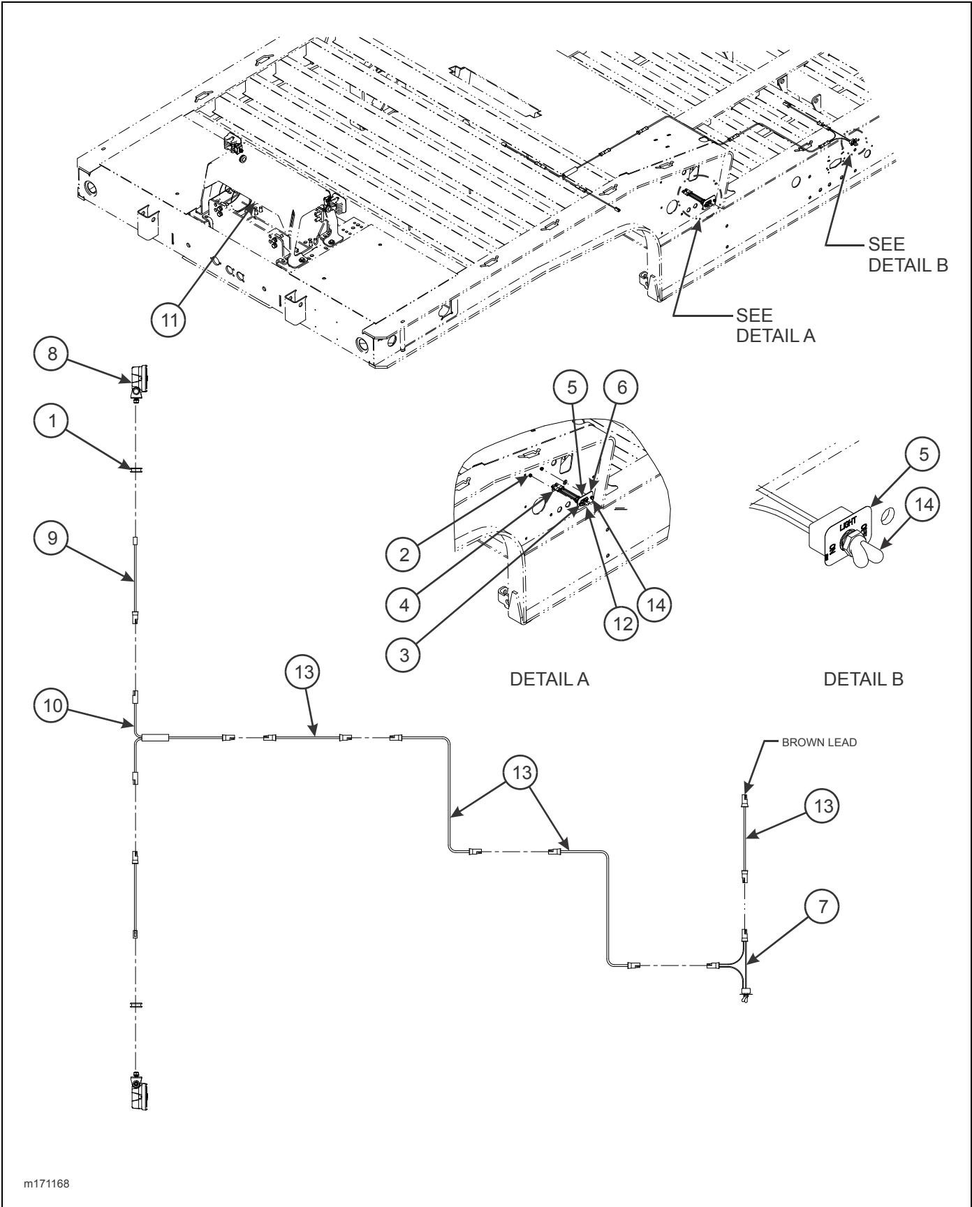
Figure 2-159: Work Light Installation, Winch (Option)
