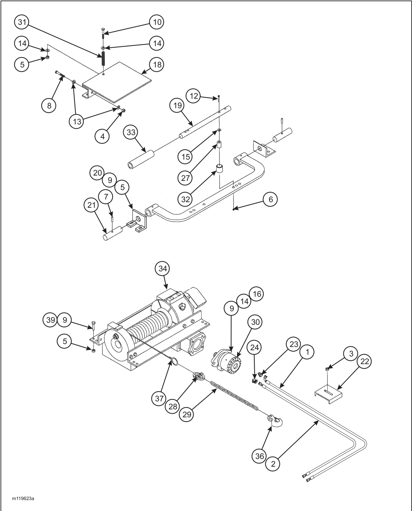
Figure 2-94: Winch Installation, Spring Tension Cable Roller
