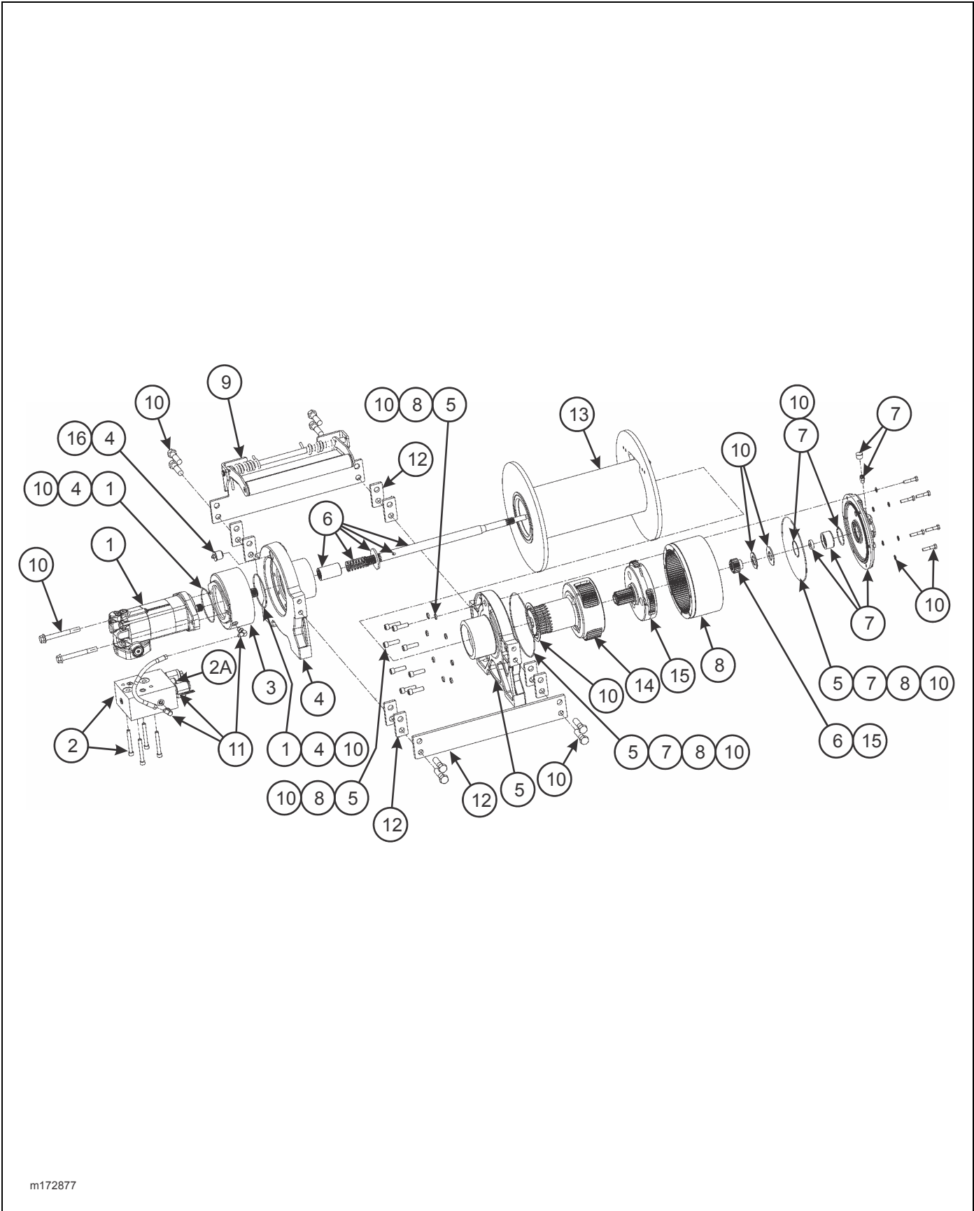
Figure 2-87: 30K Winch Installation, Hydraulic/Air Items (Warn)
