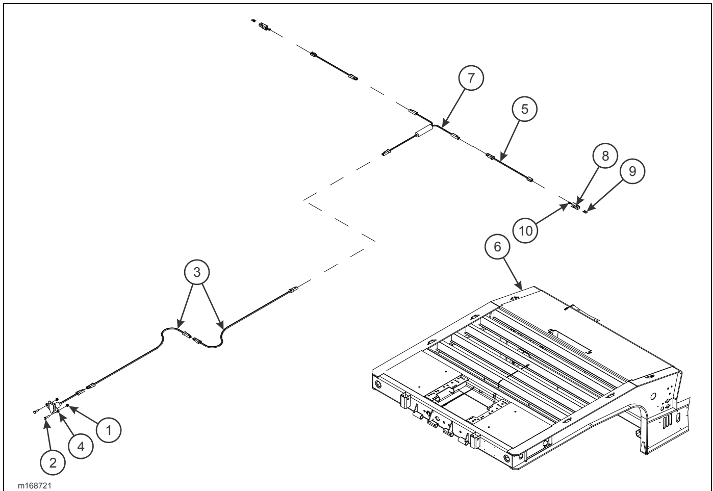
Figure 2-176: Front/Rear Harness Installation (Option)
