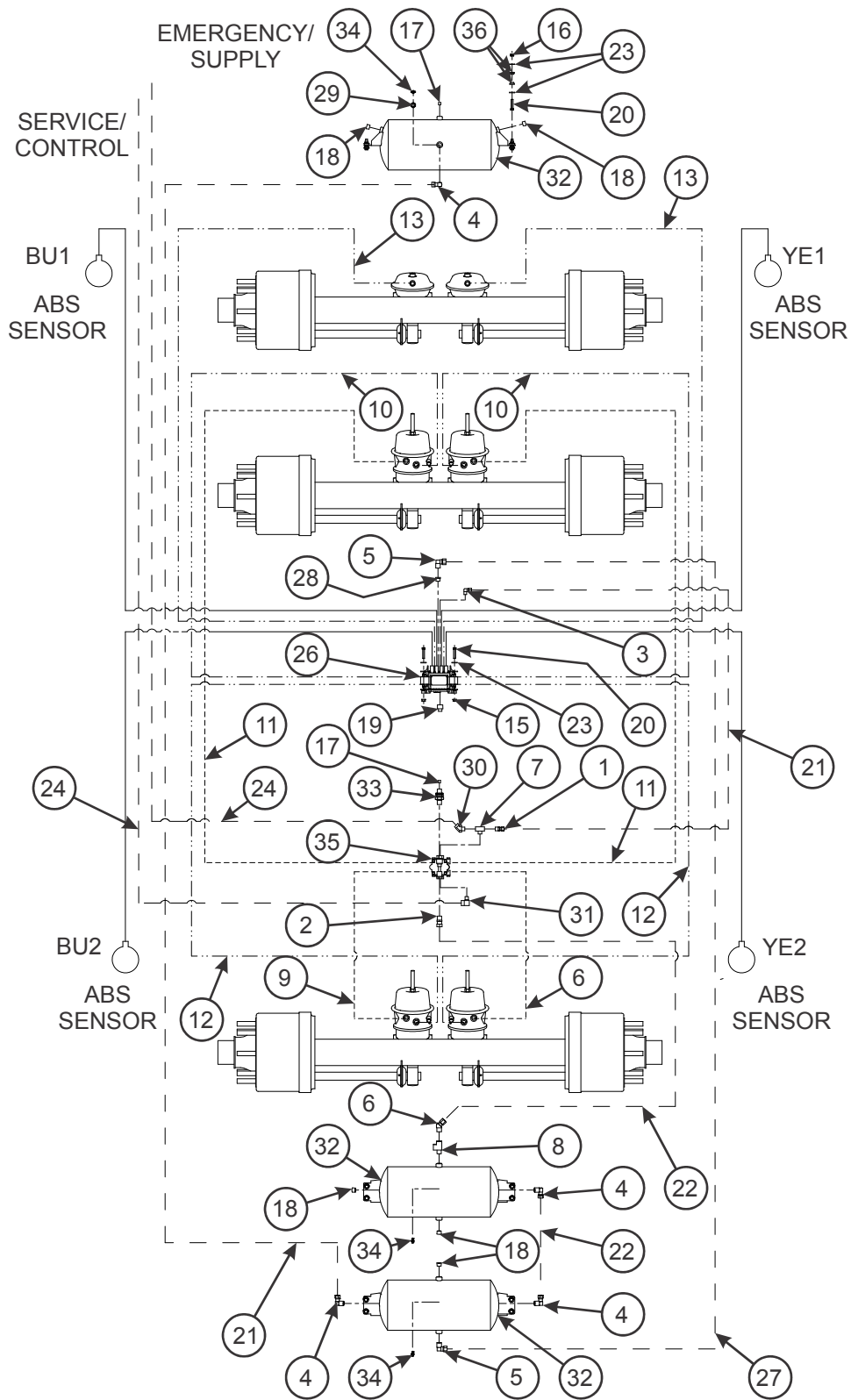
Figure 2-41: Spring Air Brake System w/ ABS (455)
