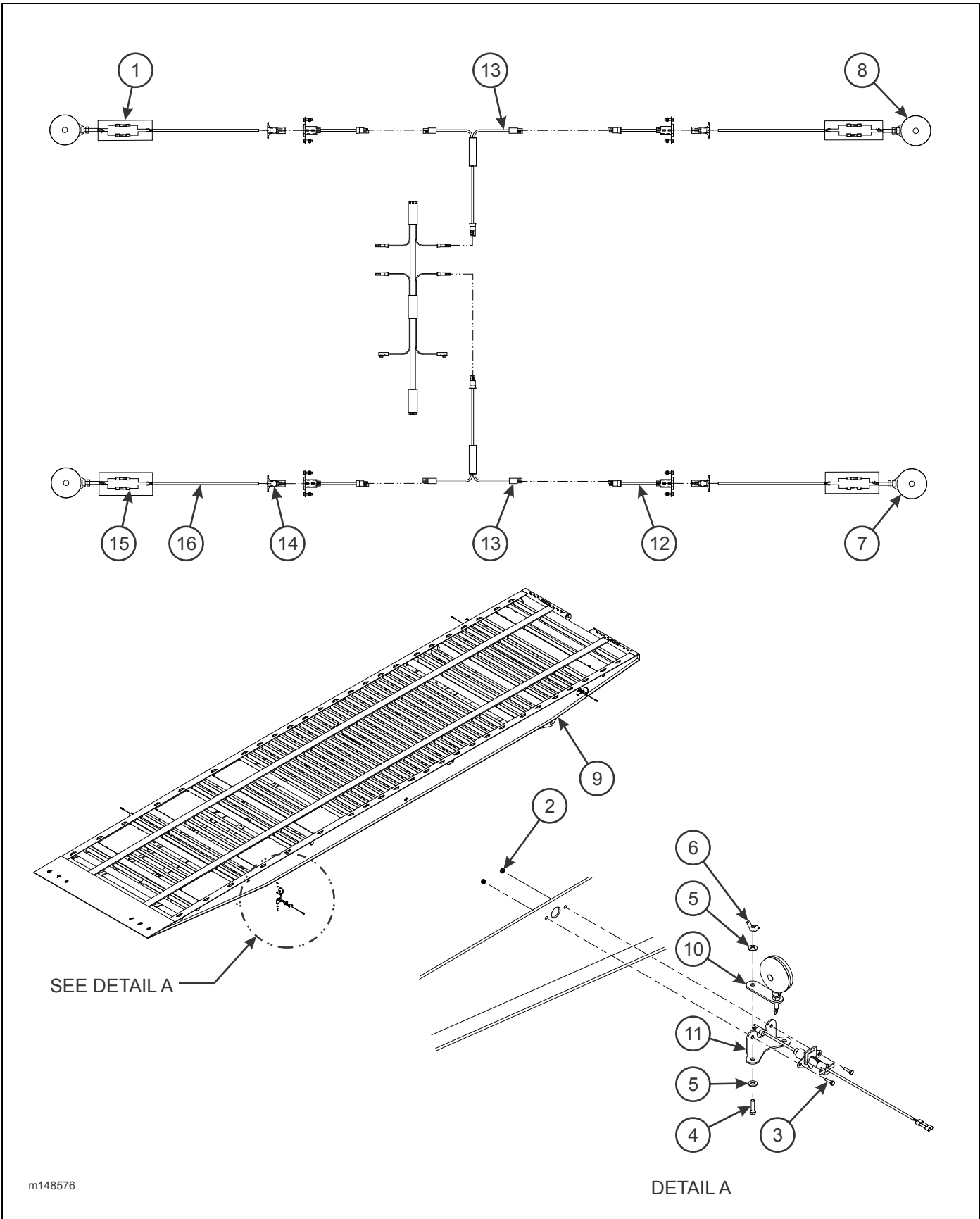
Figure 2-168: Four Corner Light Installation (Option)
