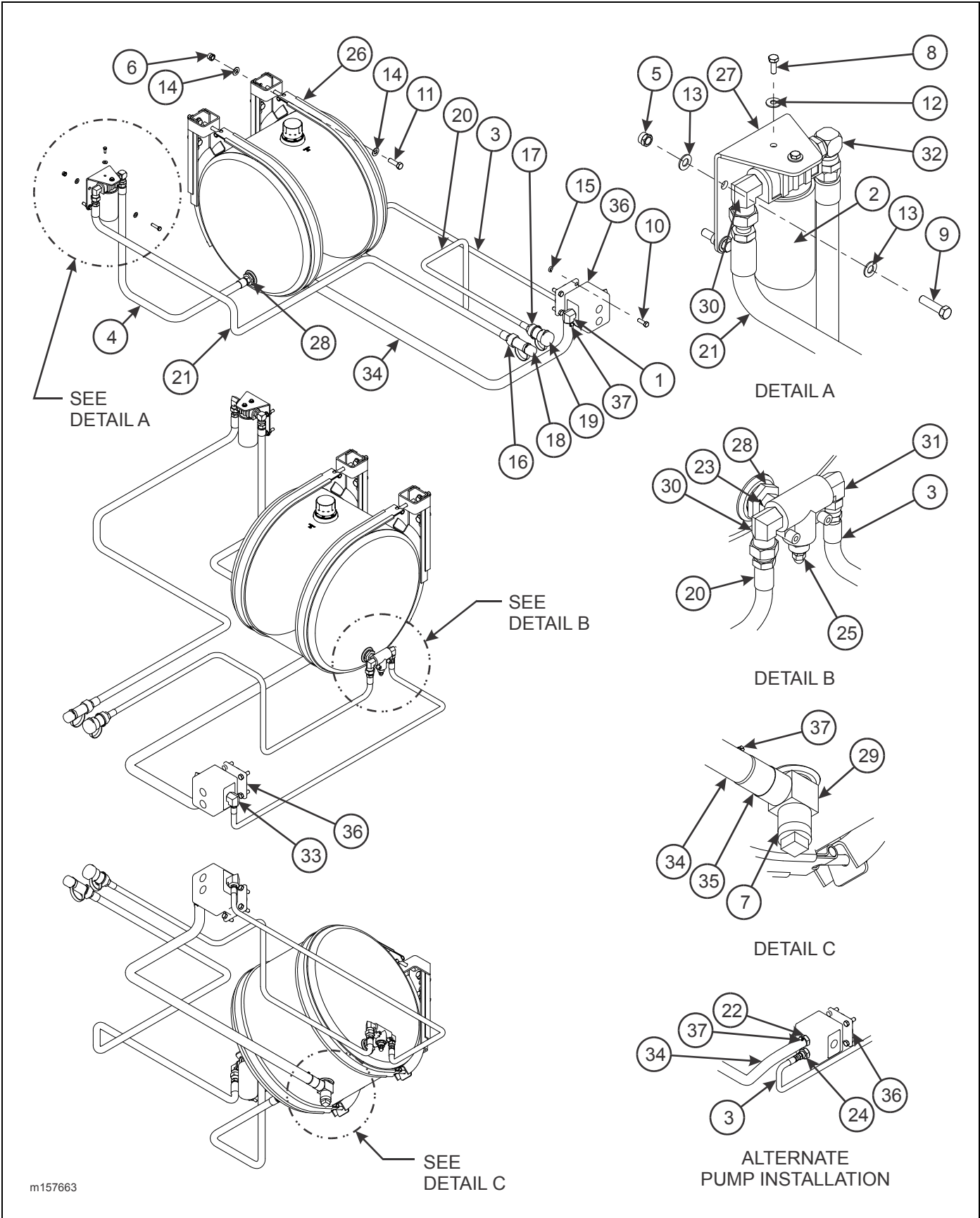
Figure 2-24: 35 Gallon Aluminum Wet Kit Items
