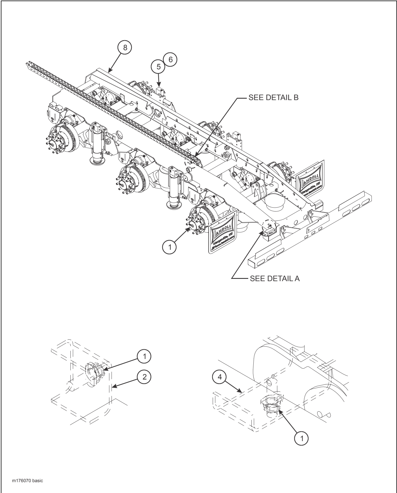
Figure 2-53: Disk Brake Suspension, Basic Assembly
