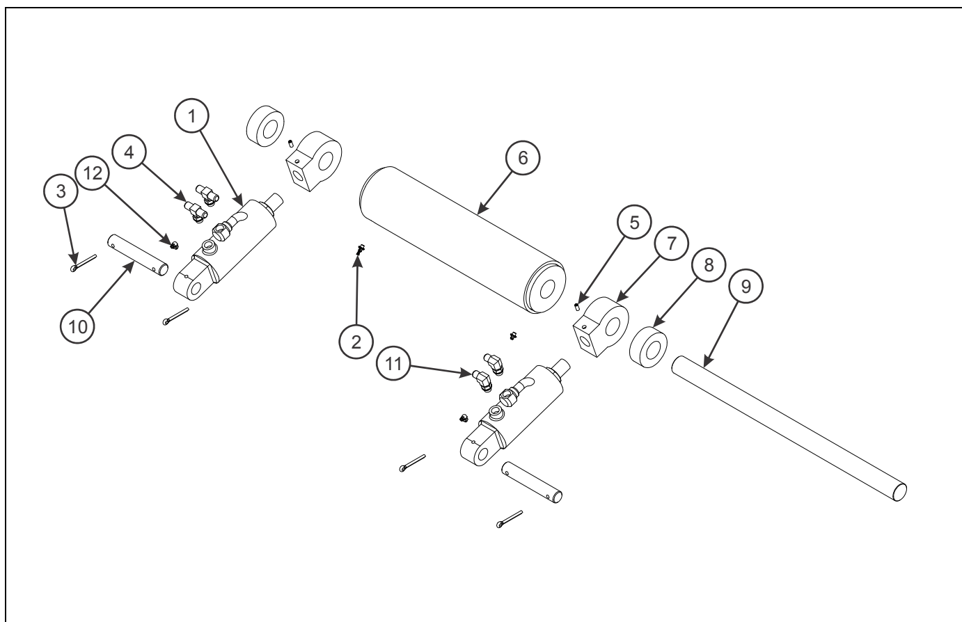
Figure 2-119: Pop-Up Roller Installation (Option)
