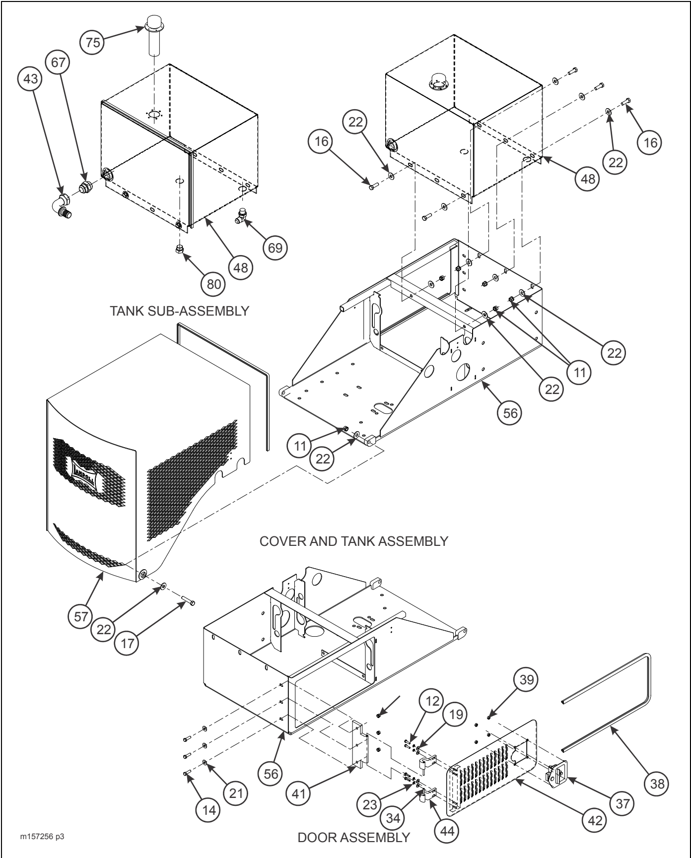
Figure 2-147: 25HP Diesel Engine Installation (3 of 4)
