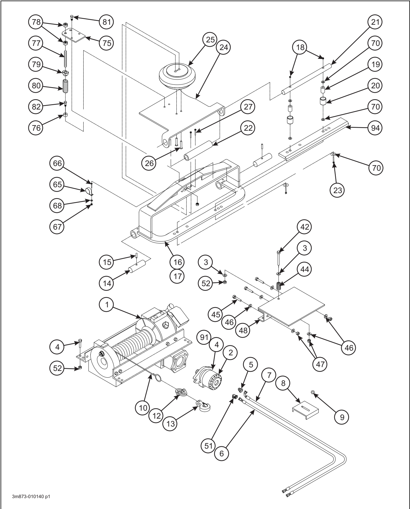
Figure 2-88: Winch Installation (1 of 2)
