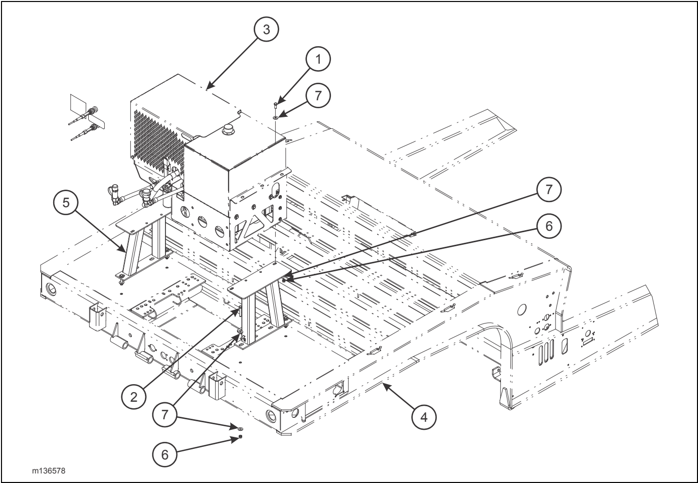
Figure 2-149: Upper Deck Engine Stand Installation
