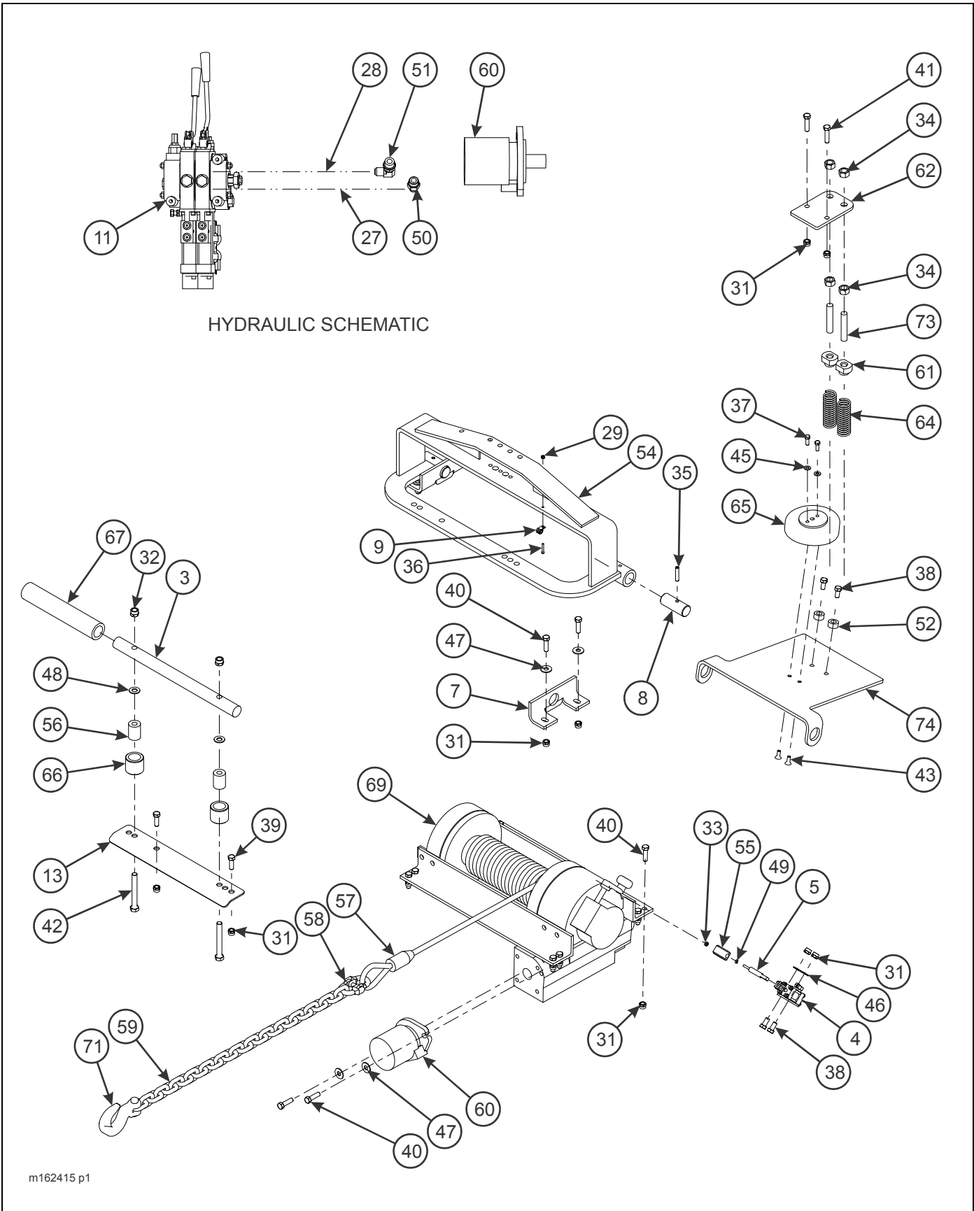
Figure 2-92: 20K Air Tension/Release Winch Installation (1 of 2)
