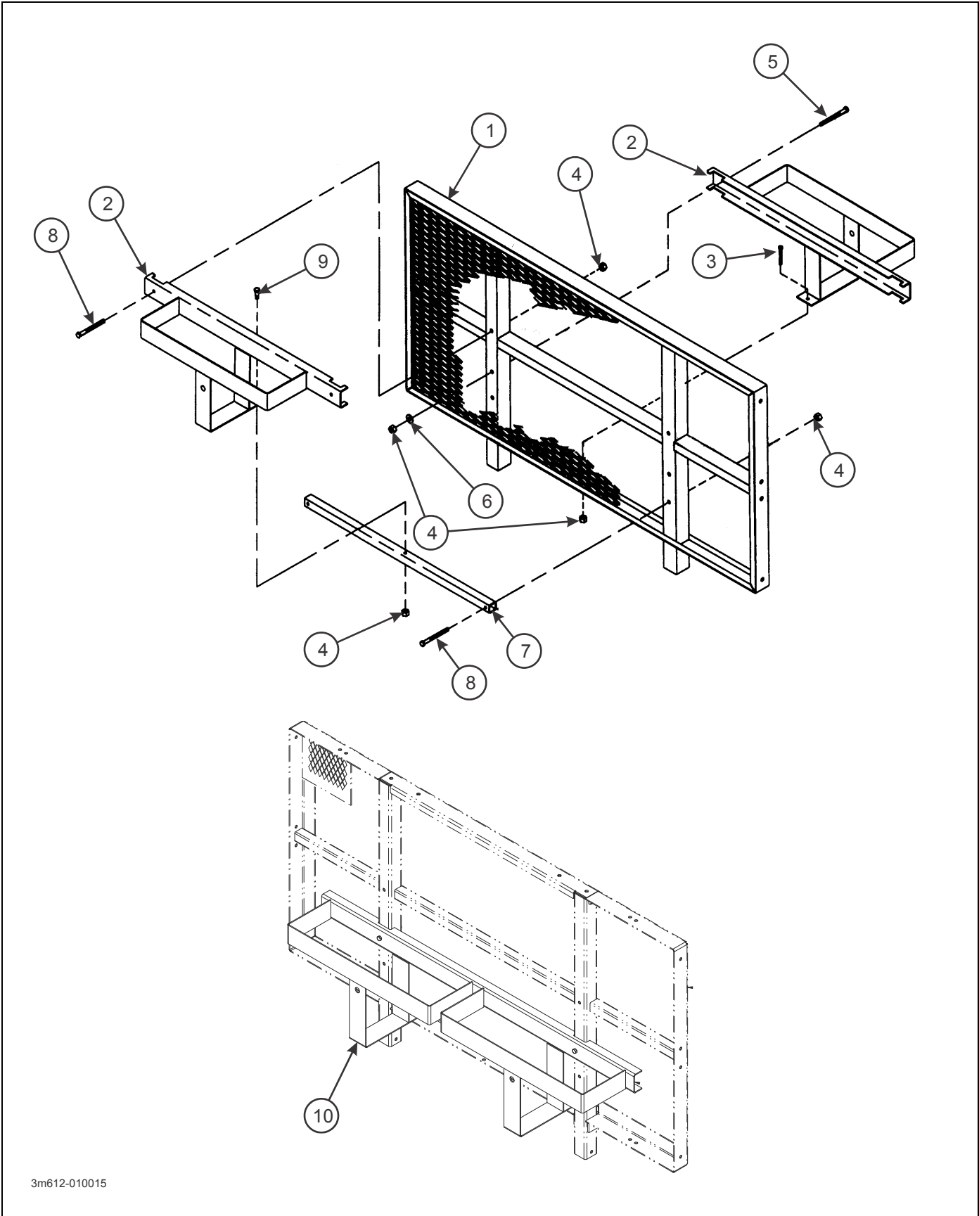
Figure 2-191: Spare Tire Carrier (Option)
