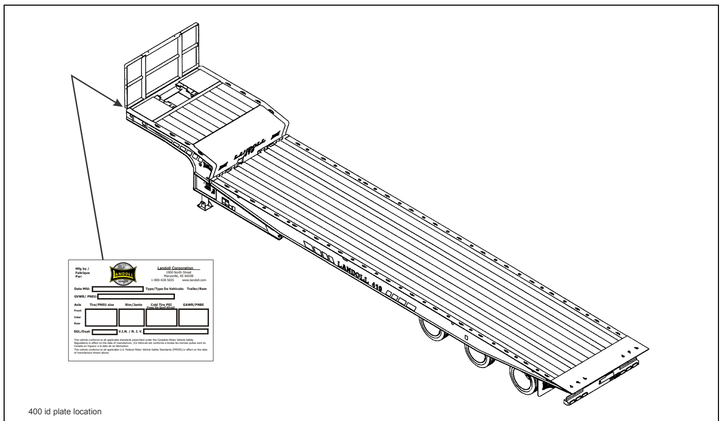
Figure 1-1: Identification Plate and Location
