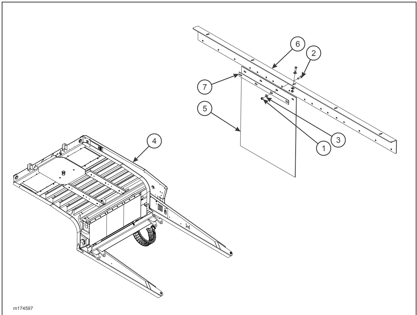
Figure 2-195: Mud Flap Installation
