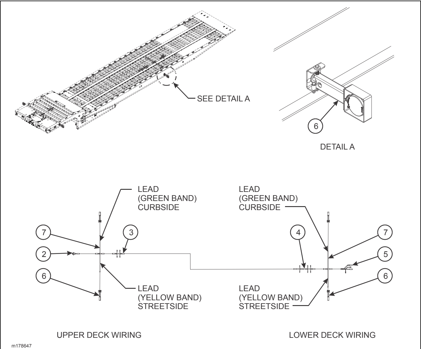
Figure 2-169: Swingout Light Installation (Option)
