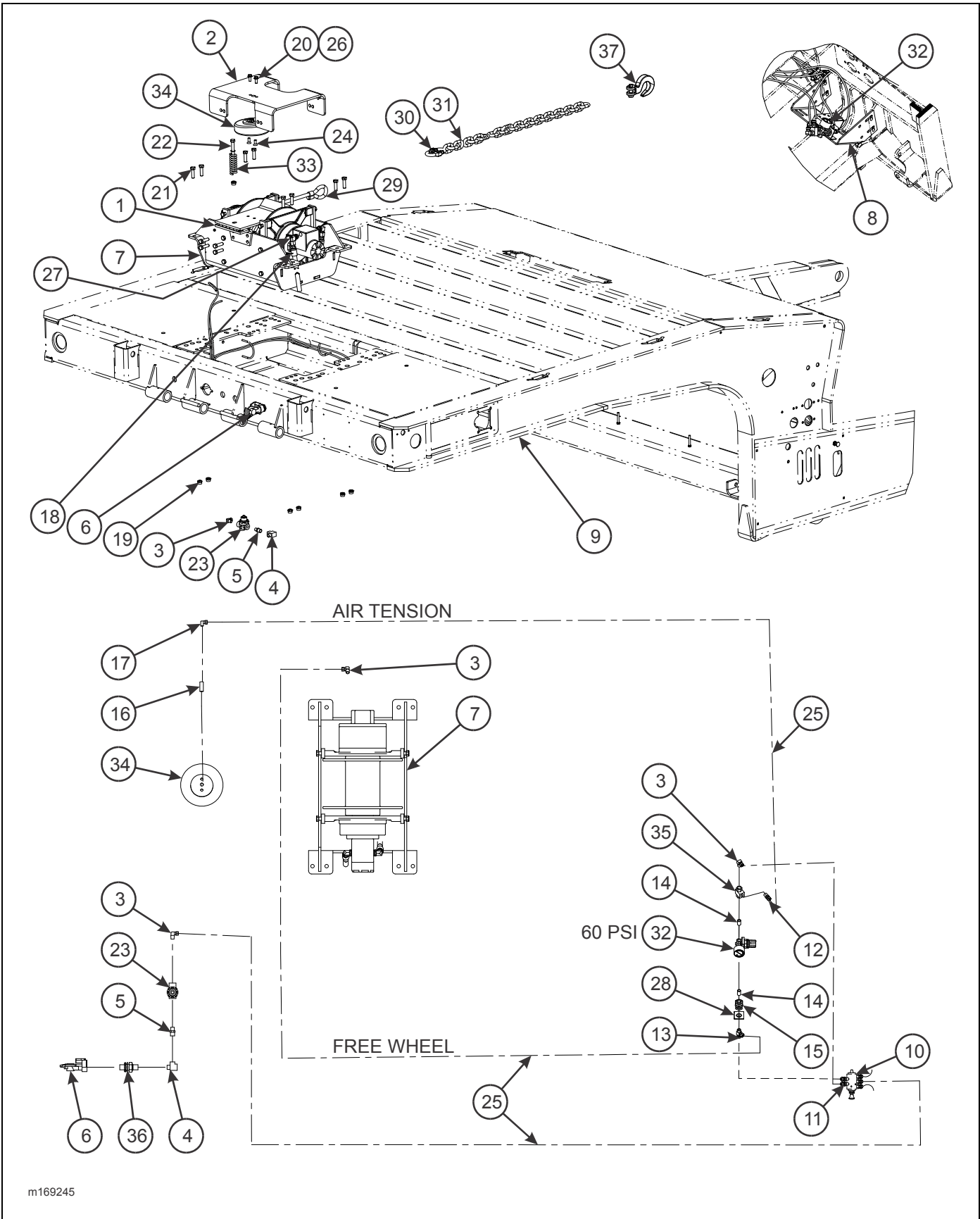
Figure 2-107: 20K Winch Installation, Air T/R (DP)
