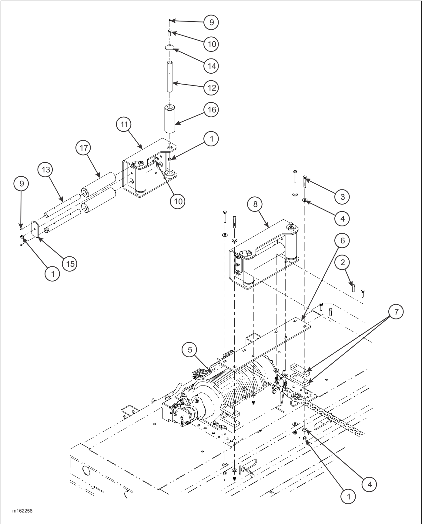
Figure 2-114: 4 Roller Guide Installation (Warn) (Option)
