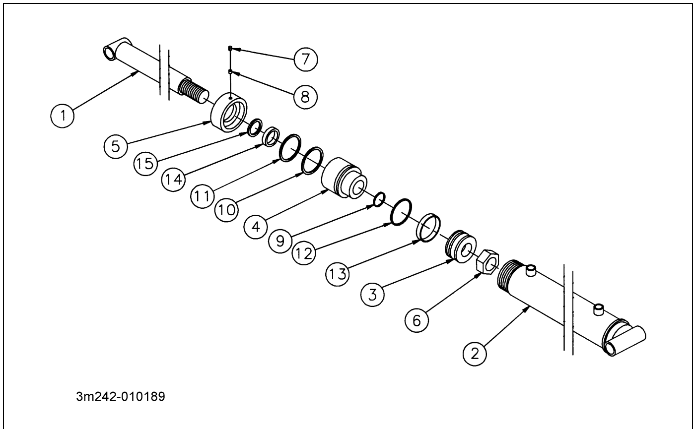
Figure 2-22: Cylinder, Hydraulic 6 X 41 (440 & 455)
