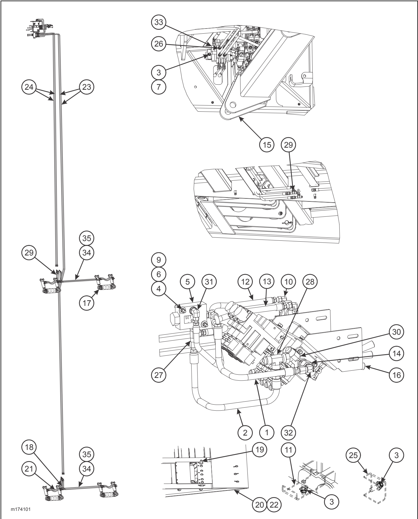
Figure 2-116: 4 Pop-Up Roller Installation (Option)
