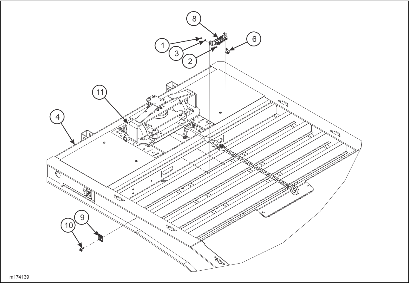
Figure 2-175: Electrical Disconnect Switch Installation (Option)
