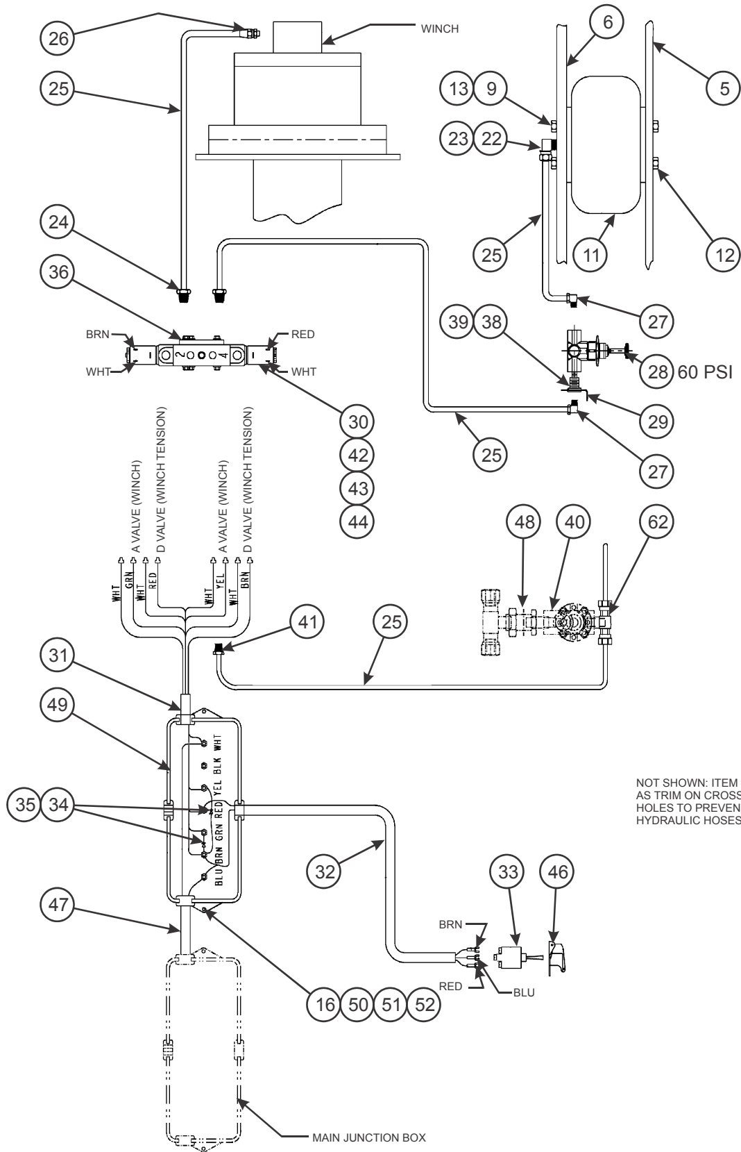
Figure 2-106: 12K, 15K, & 20K Upper Deck Winch (DP) (2 of 2)
