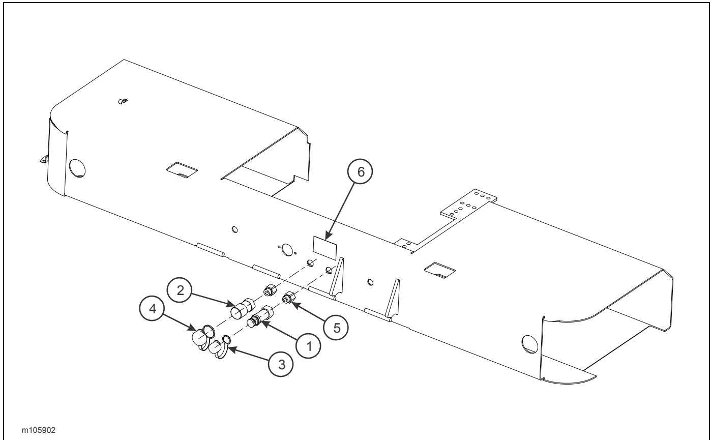
Figure 2-152: Hydraulic Conversion Kit, Ball to Flat (Option)
