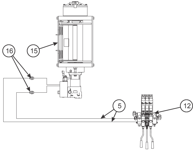
HYDRAULIC SCHEMATIC
