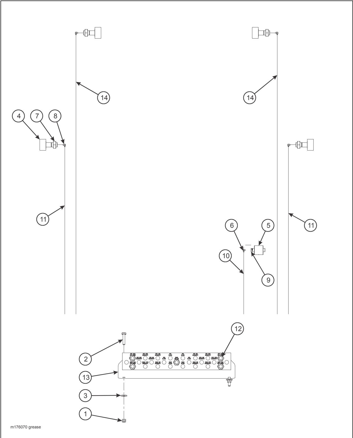
Figure 2-55: Disk Brake Suspension, Grease Assembly
