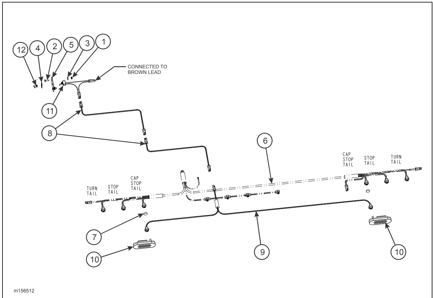
Figure 2-164: Strobe Installation, Bumper (Option)
