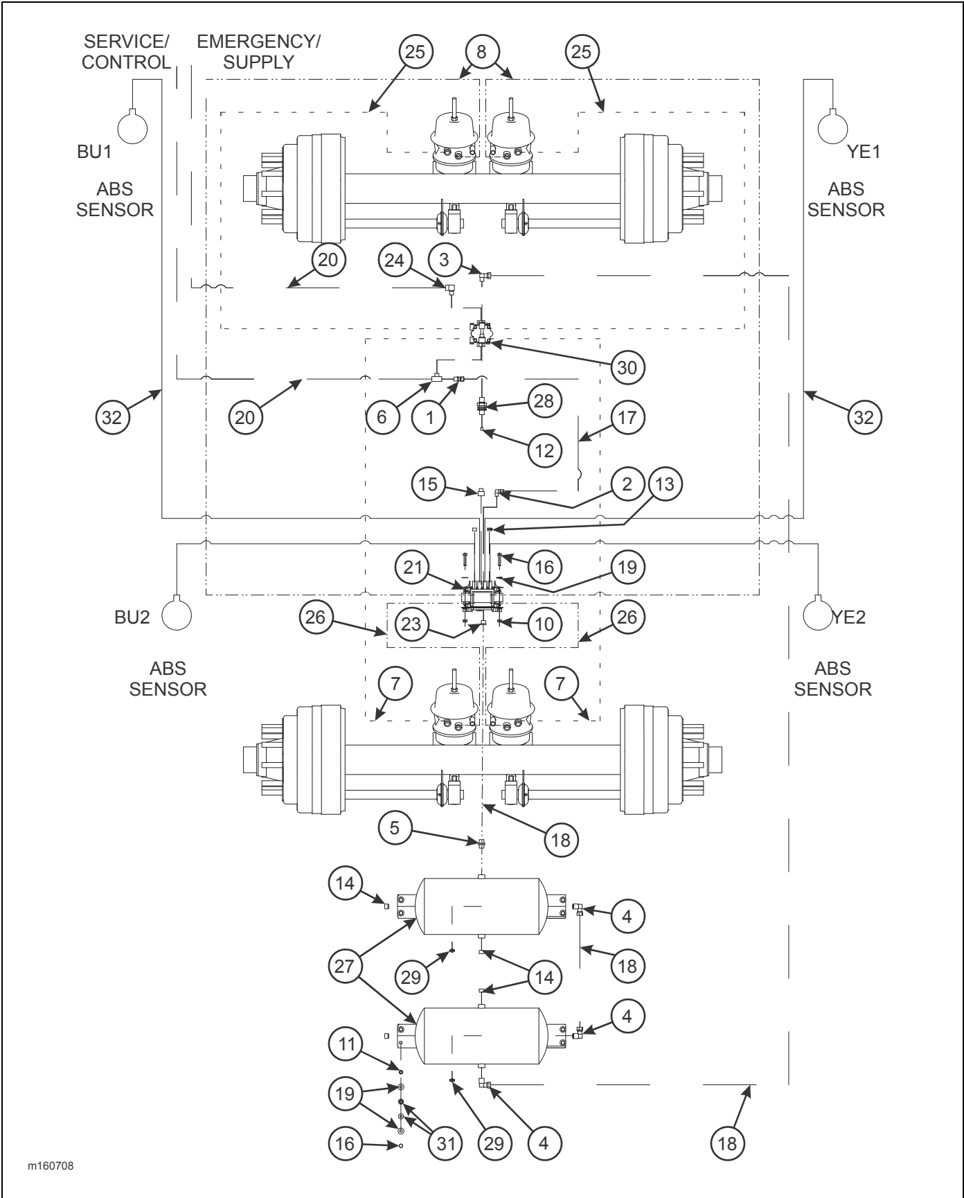
Figure 2-40: Spring Air Brake System w/ ABS (440 CA BB)
