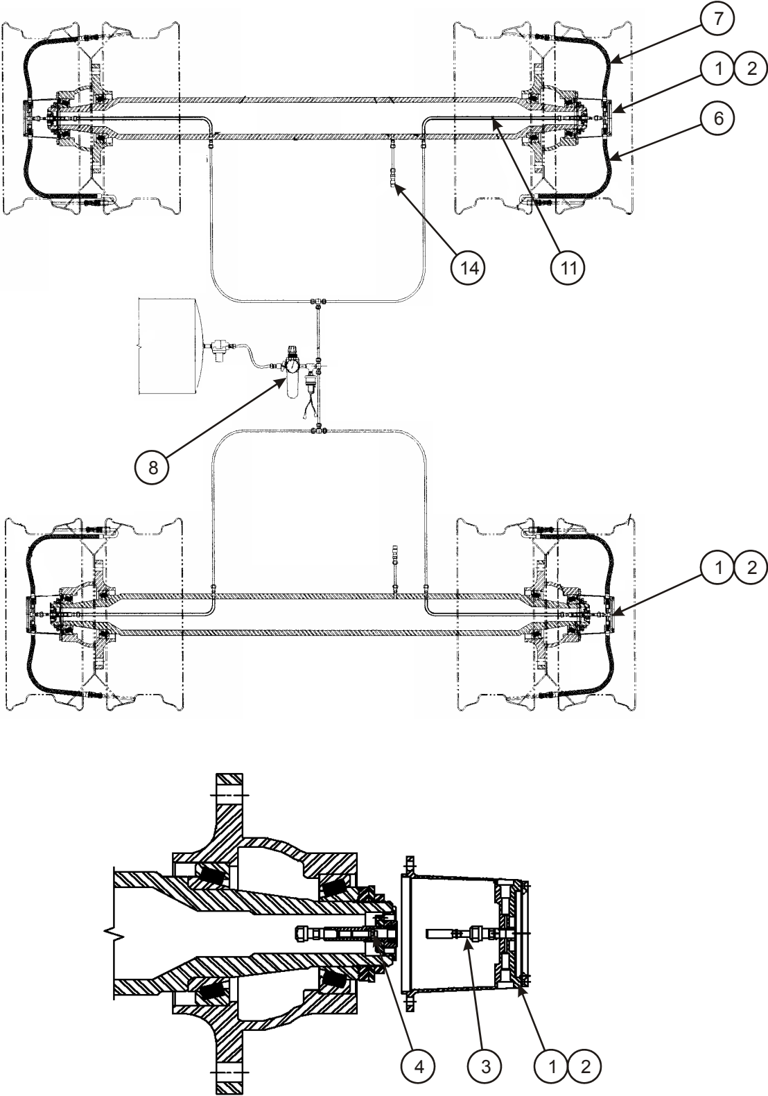
Figure 2-37: Tire Inflation System (Option)
