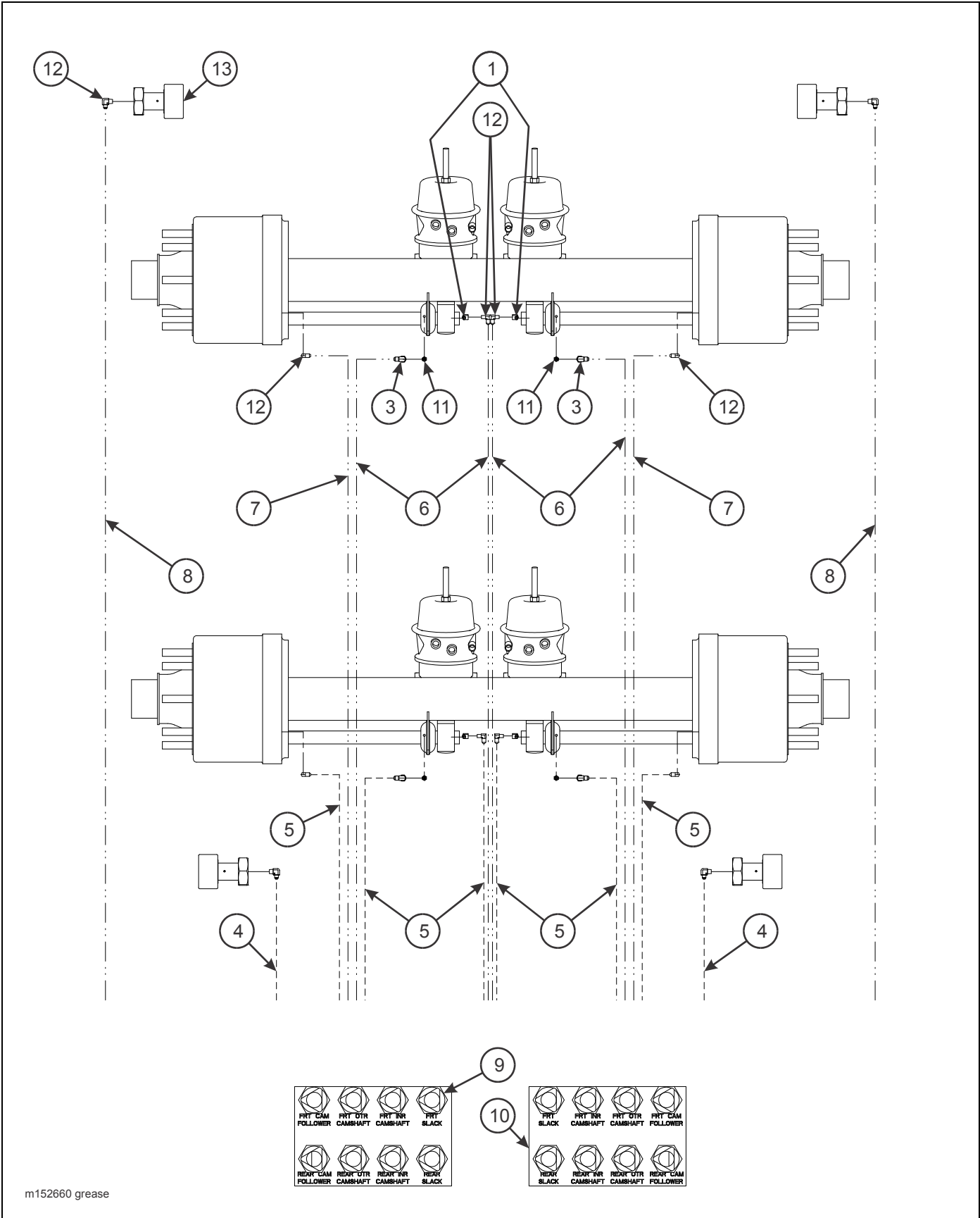
Figure 2-31: Suspension Assembly, Grease Items (425 & 440)
