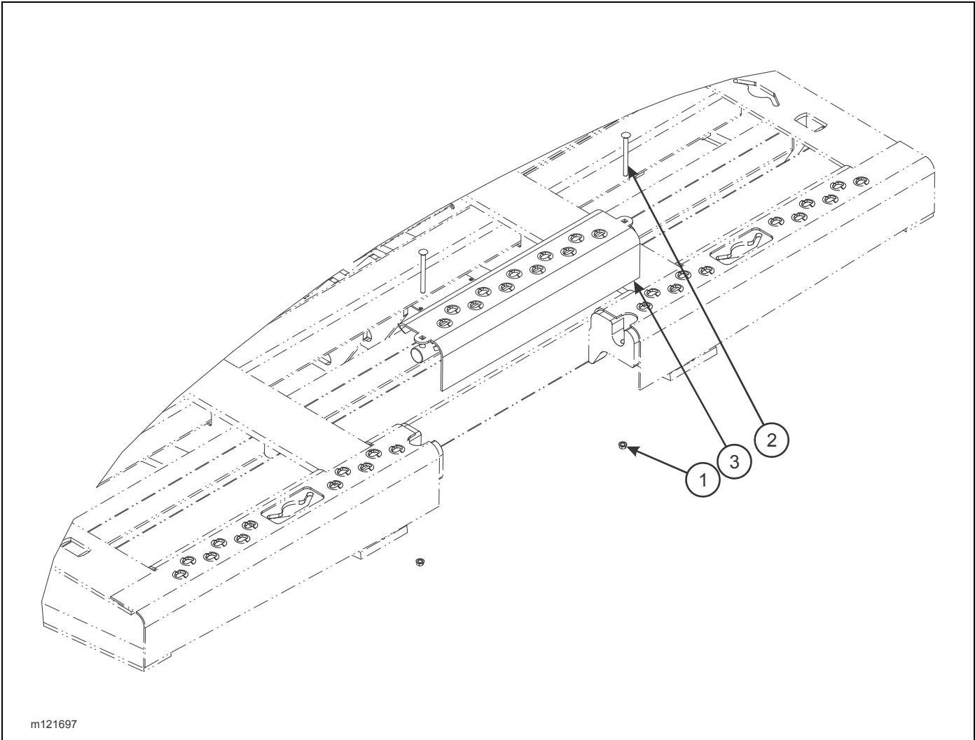
Figure 2-189: Center Rub Plate Cover Installation (Option)
