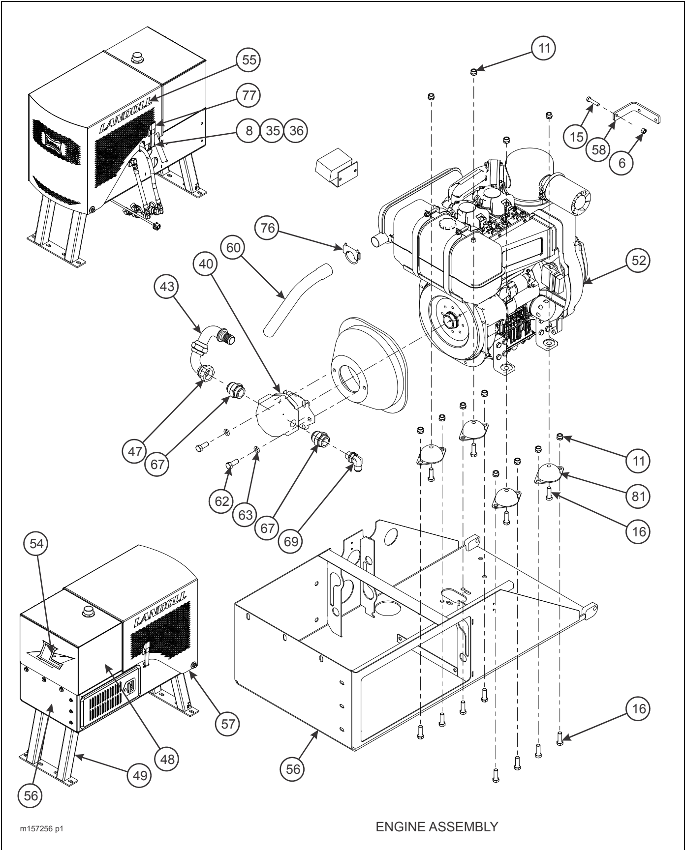
Figure 2-145: 25HP Diesel Engine Installation (1 of 4)
