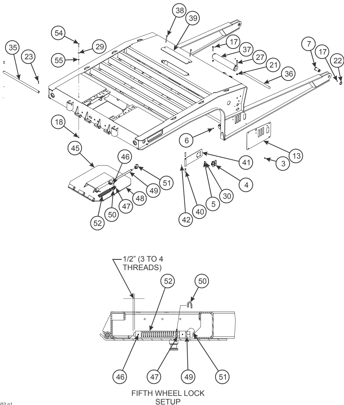
Figure 2-5: Upper Deck Assembly (1 of 2)
