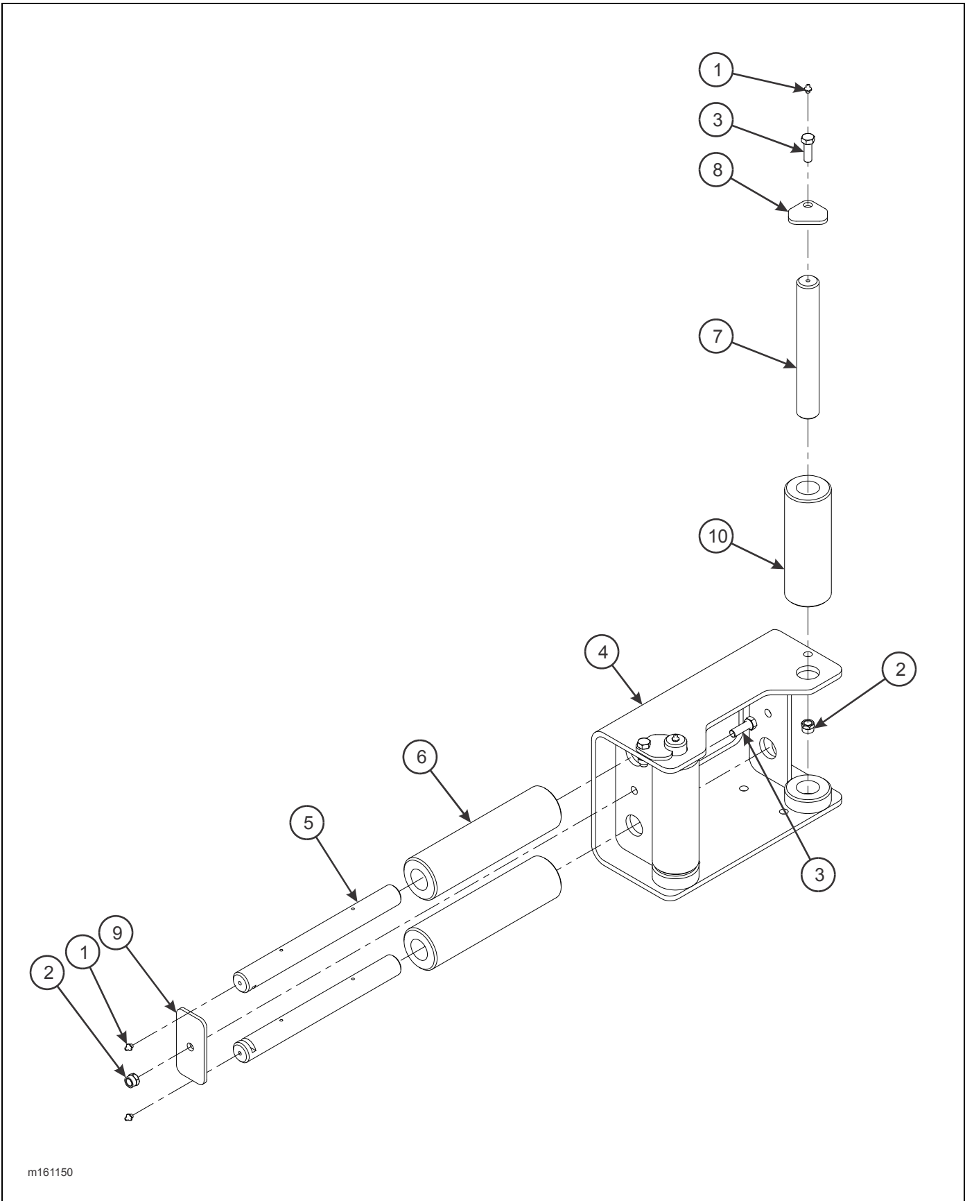
Figure 2-113: Guide Assembly, Winch 12K (Braden) (Option)
