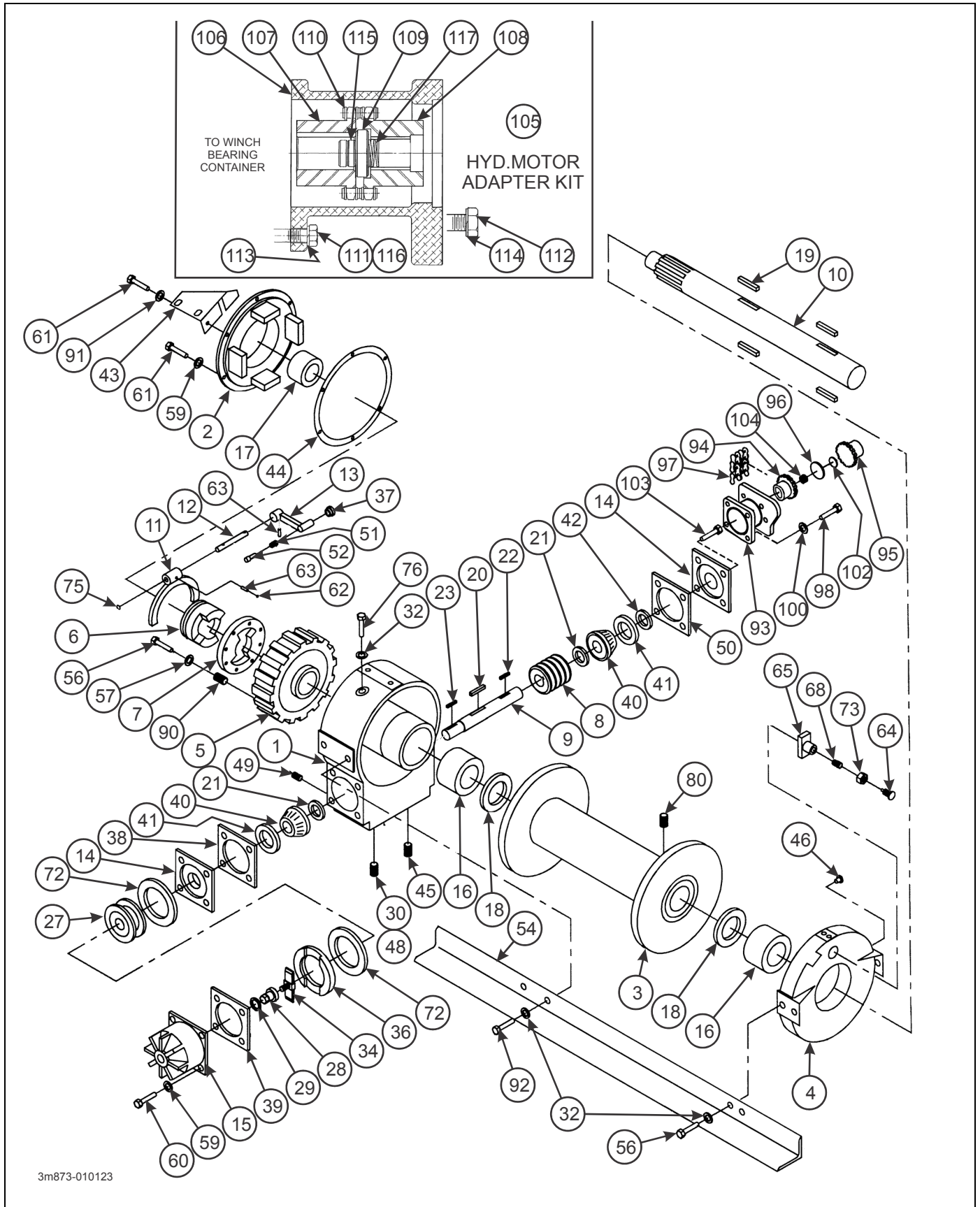
Figure 2-96: 20,000 Lb. Winch Items
