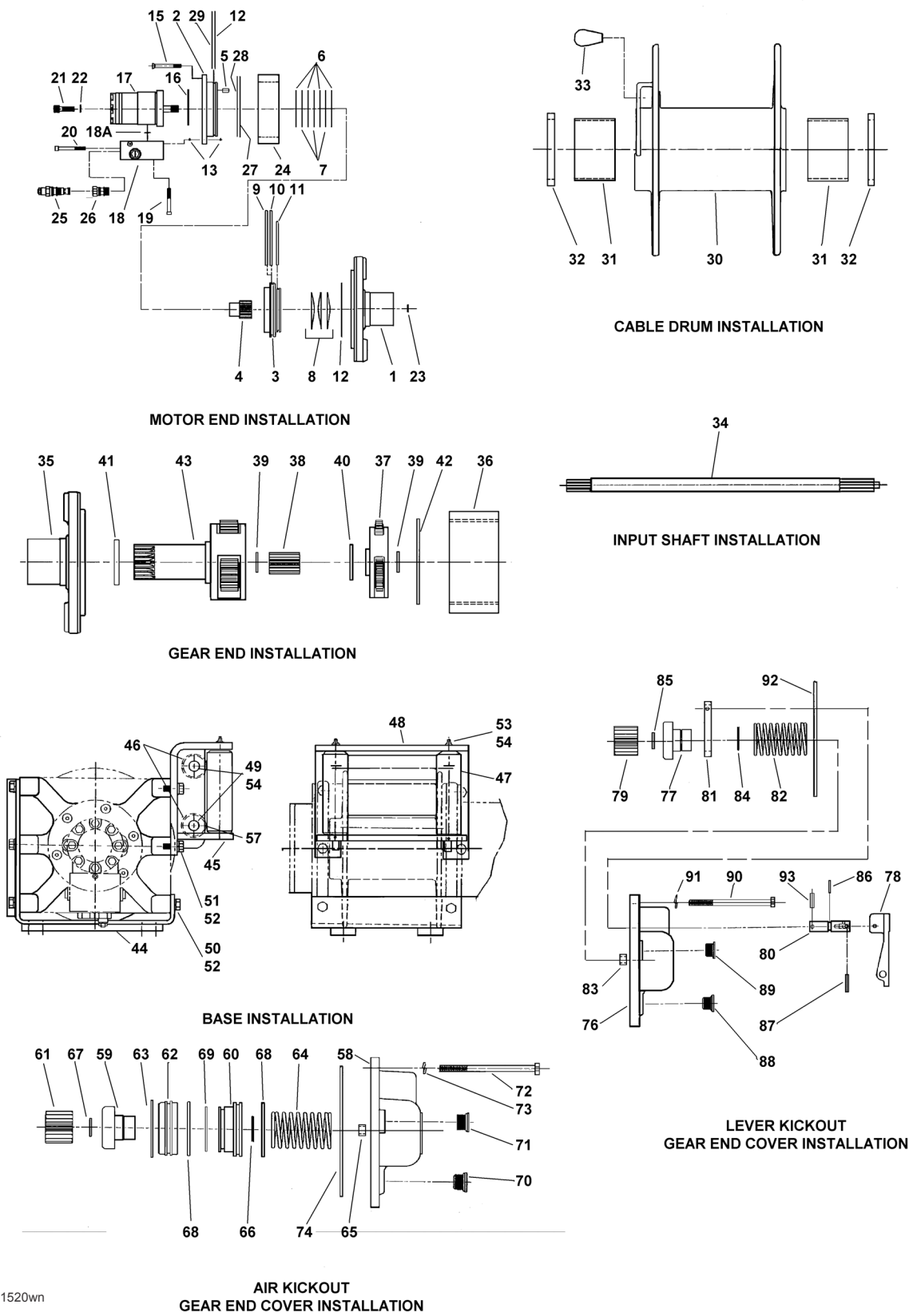
Figure 2-108: 12K, 15K, & 20K Winch Items (DP Planetary)
