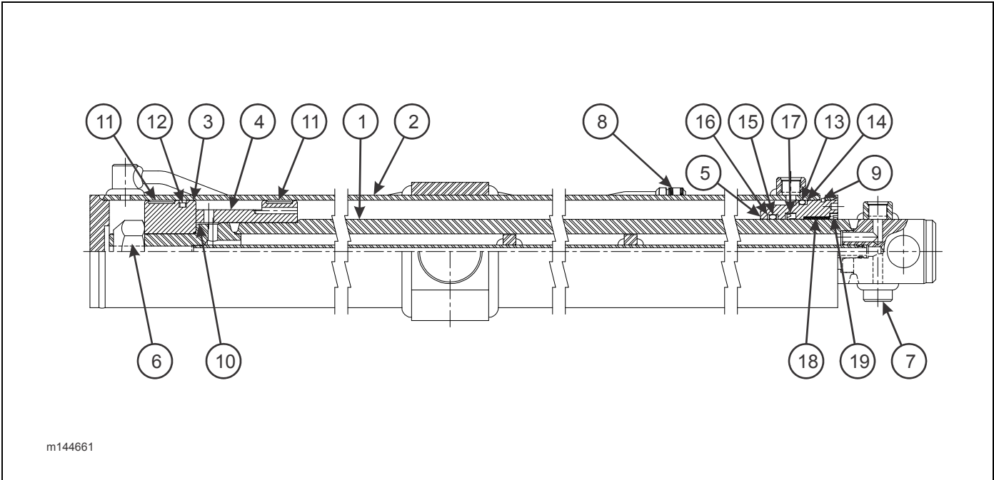
Figure 2-15: Cylinder, Hydraulic 4 x 100 Ported Rod (Streetside) (455-48/50CA, 425-41/45, 440-41)
