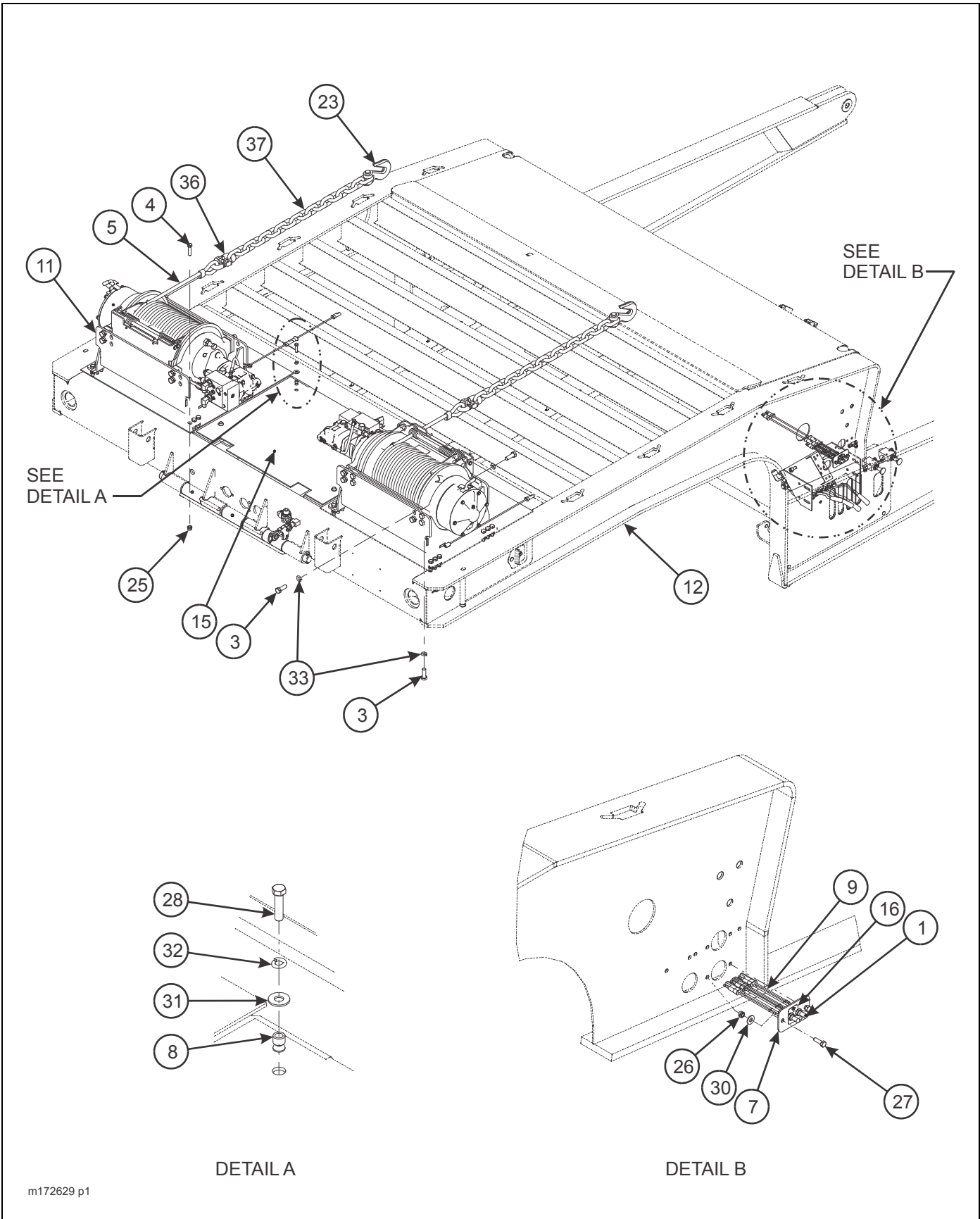
Figure 2-81: Dual Winch Installation, 30K (Warn) (1 of 3)
