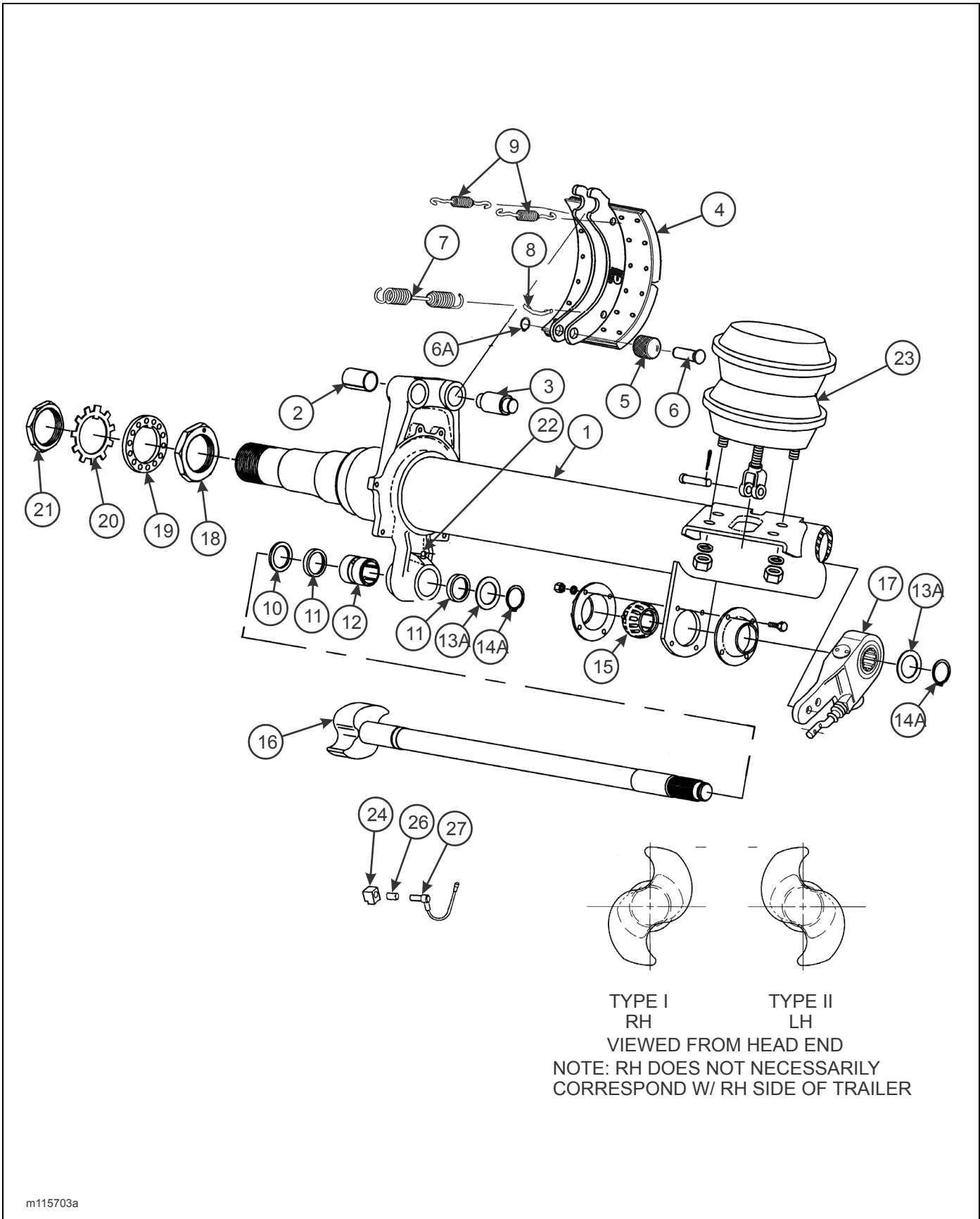
Figure 2-50: Axle and Brake Assembly (12-1/4 x 7-1/2'')
