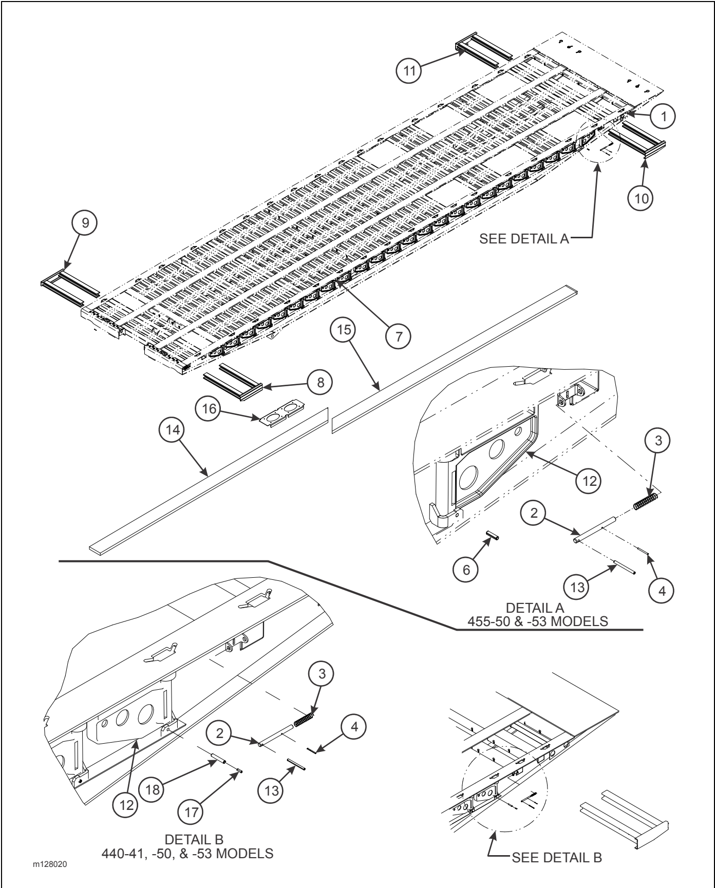
Figure 2-72: Outrigger Installation (Option)
