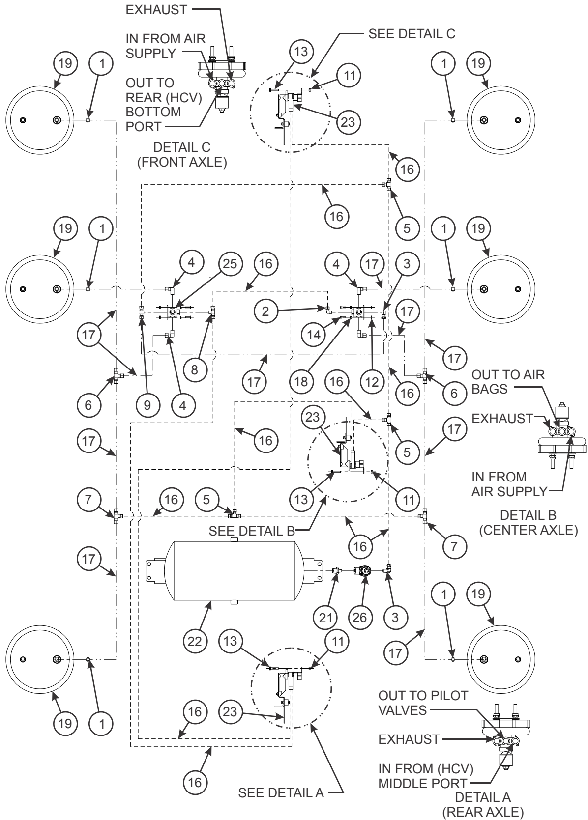
Figure 2-46: Air Ride Suspension, Air System (Triple)
