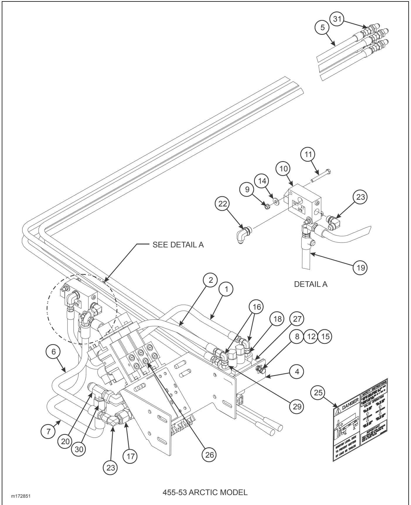
Figure 2-124: Dock Leveler Hydraulic Installation (2 of 2) (Option)
