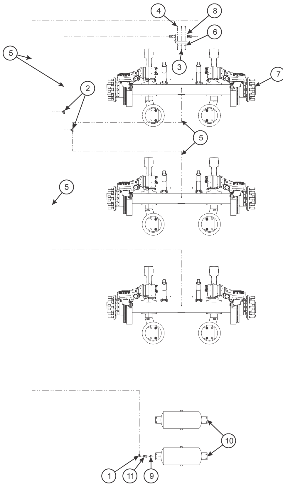
Figure 2-56: Disk Brake Suspension, Tire Inflation Assembly
