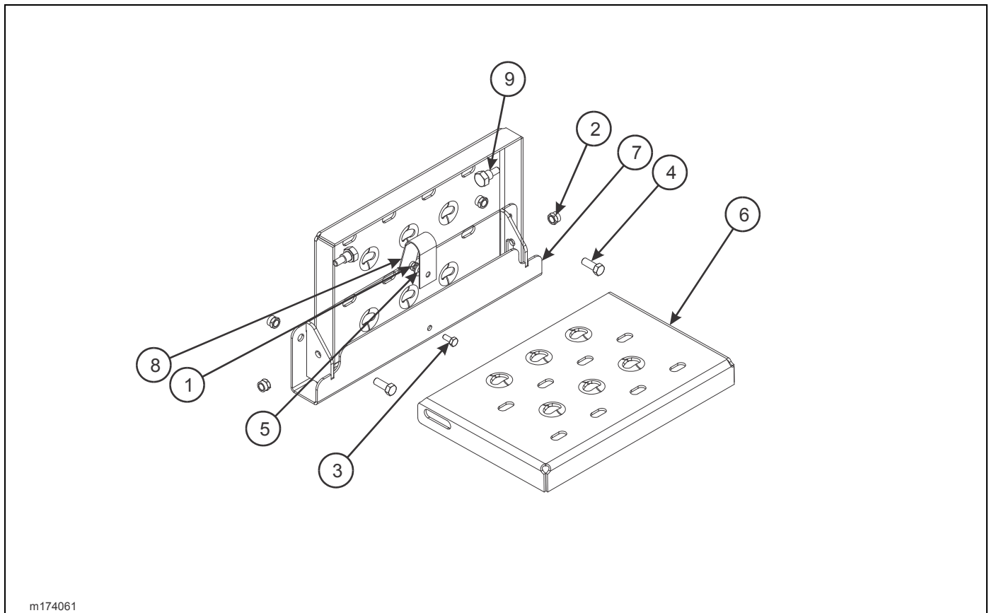
Figure 2-199: Folding Step Assembly (Option)
