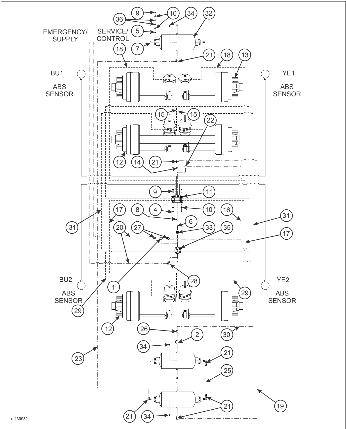
Figure 2-43: Spring Air Brake System w/ ABS Arctic (455)
