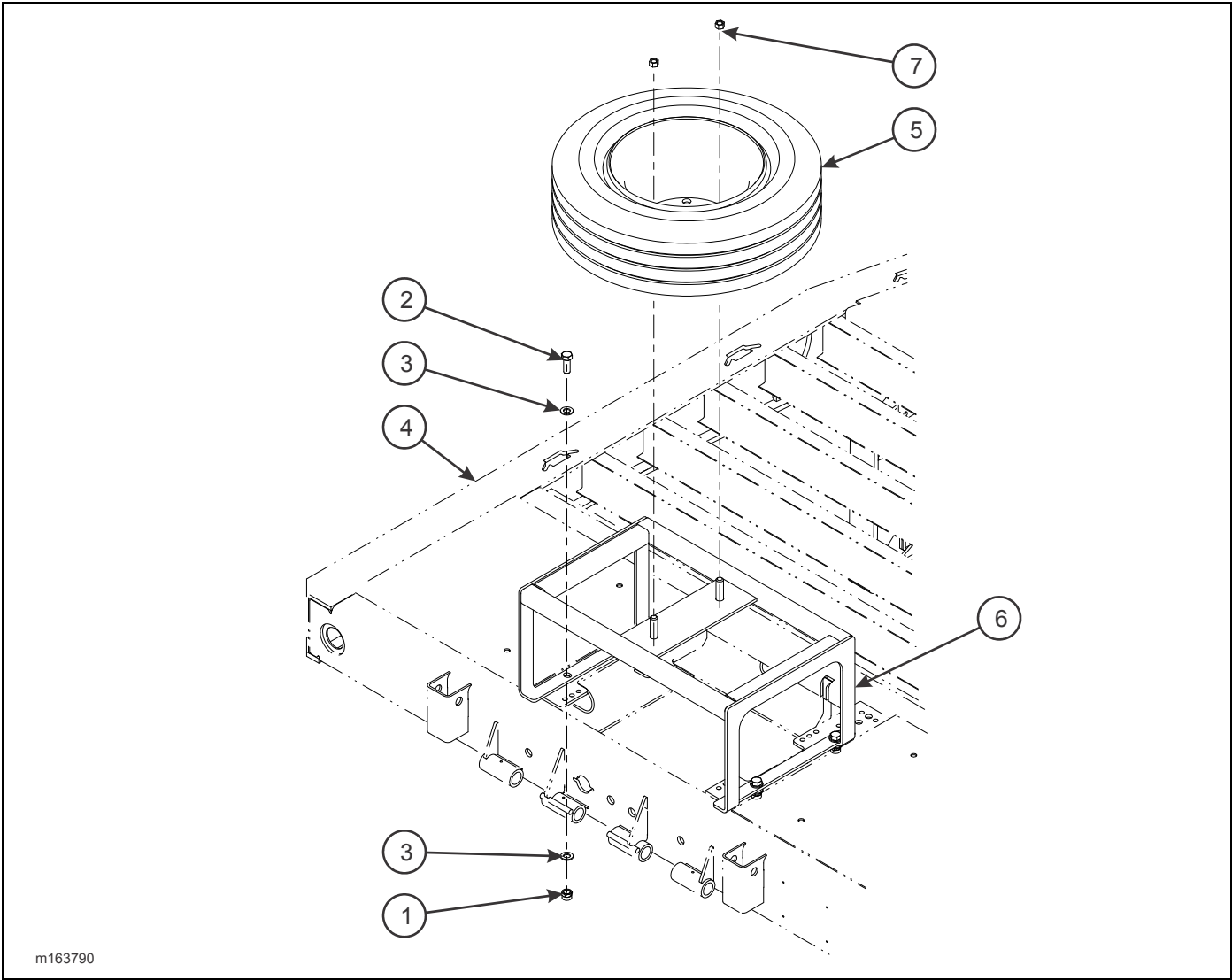
Figure 2-196: Horizontal Spare Tire Mount Assembly
