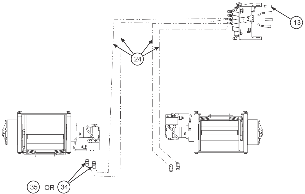
HYDRAULIC SCHEMATIC
