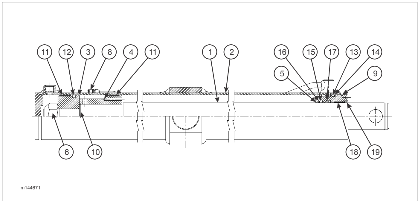
Figure 2-20: Cylinder, Hydraulic 4 x 138 (Curbside) (440-53)
