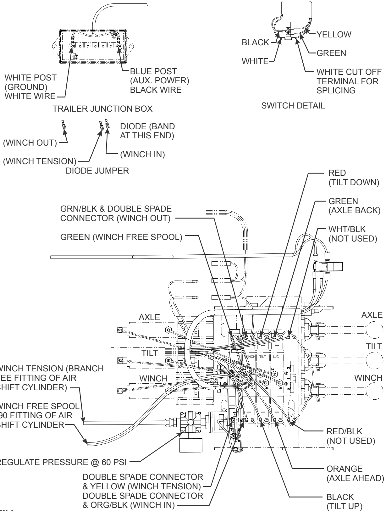
Figure 2-91: Winch Installation (2 of 2)
