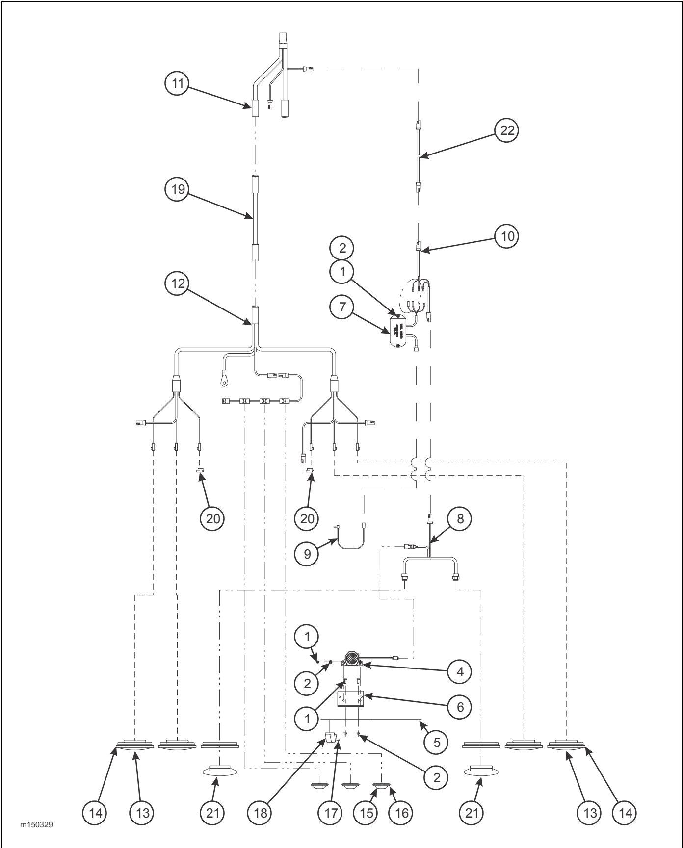
Figure 2-172: Backup Alarm/Light Installation (Option)
