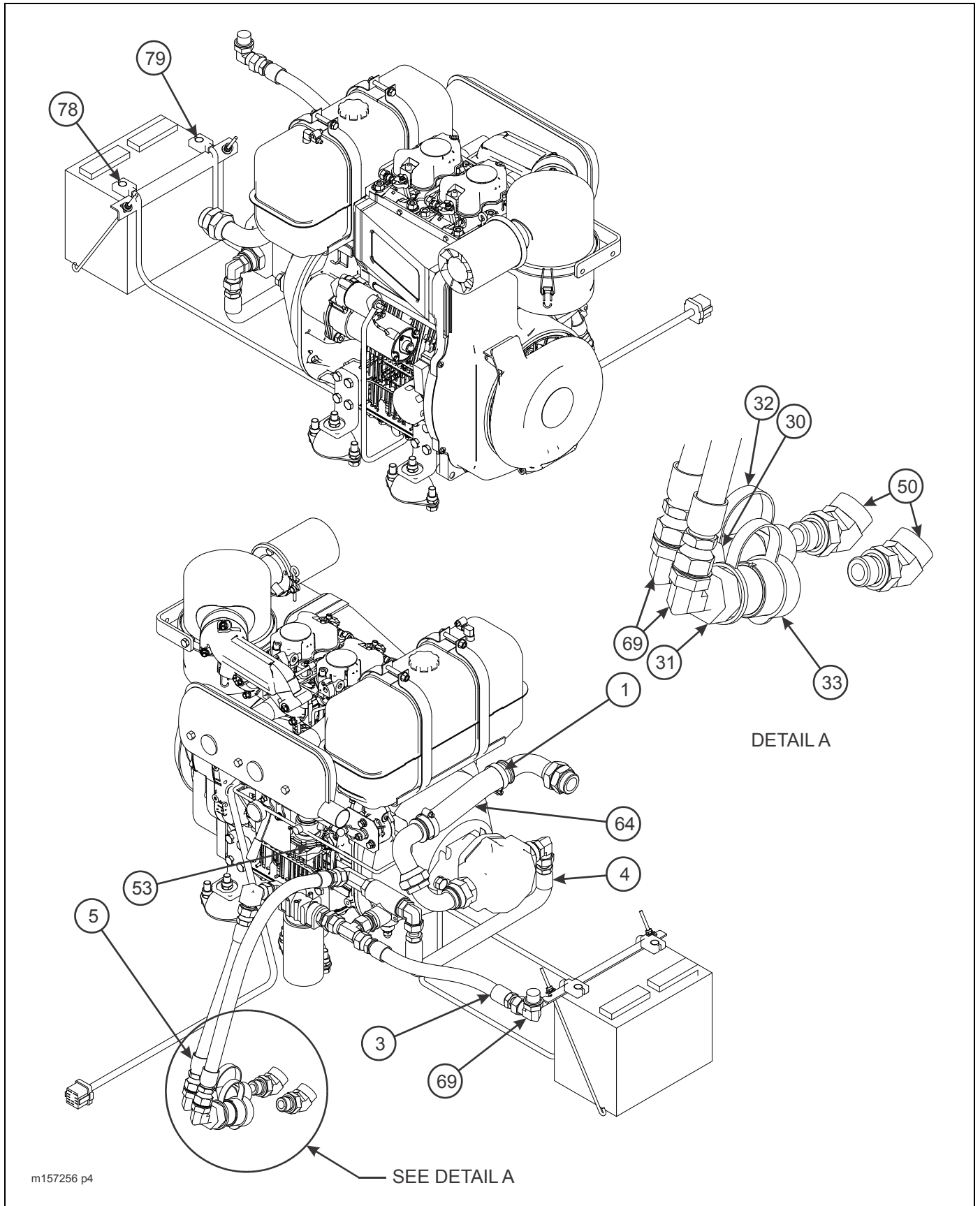
Figure 2-148: 25HP Diesel Engine Installation (4 of 4)
