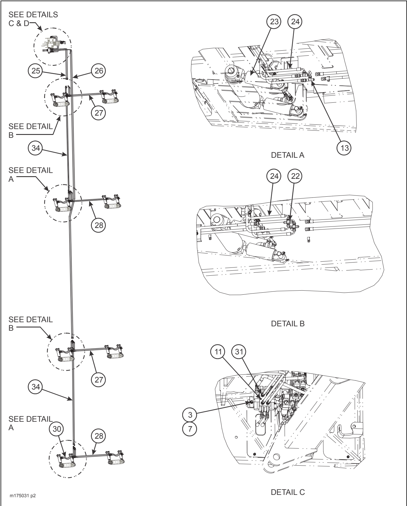
Figure 2-117: 8 Pop-Up Roller Installation (Option) (1 of 2)
