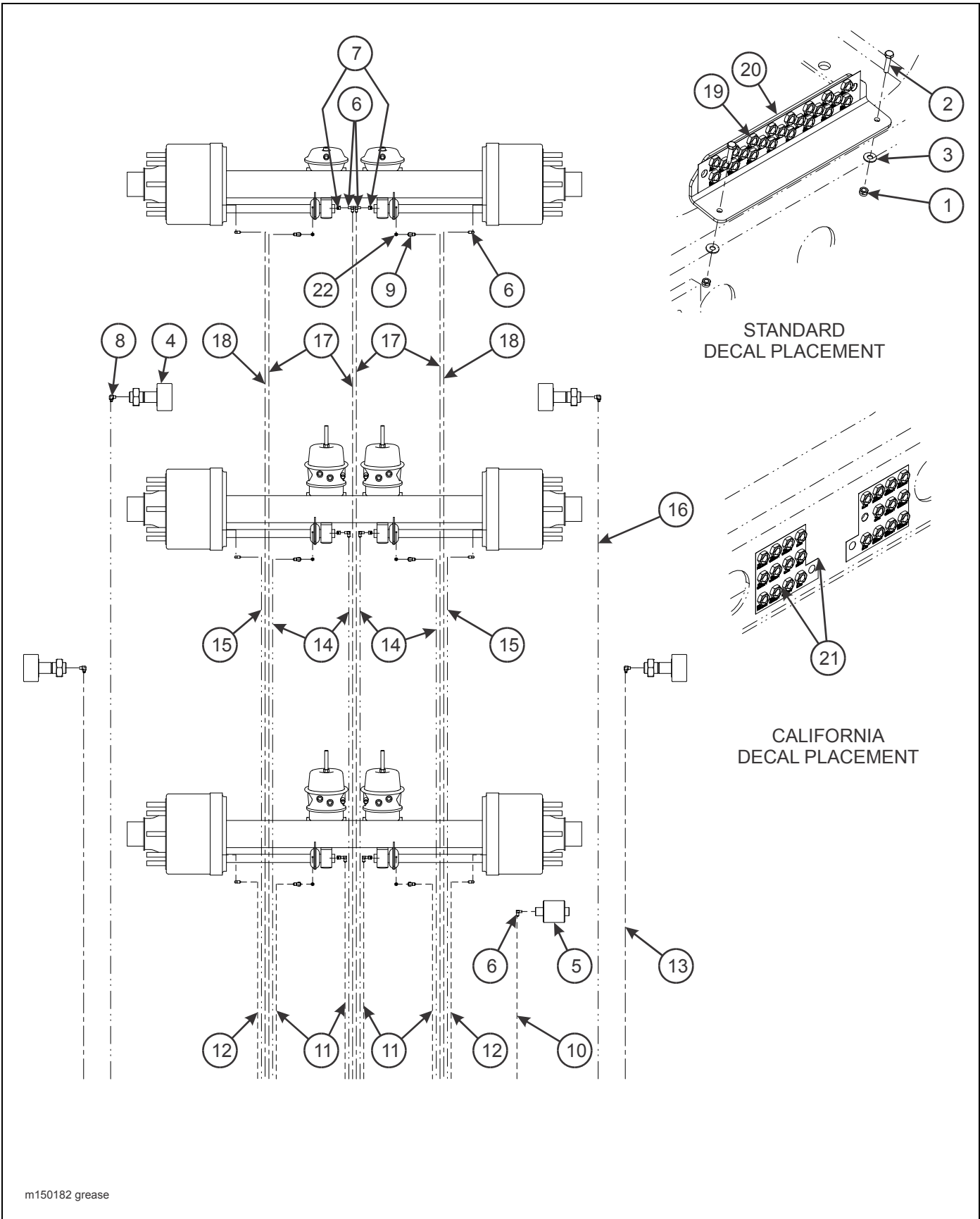
Figure 2-35: Suspension Assembly, Grease Items (455)
