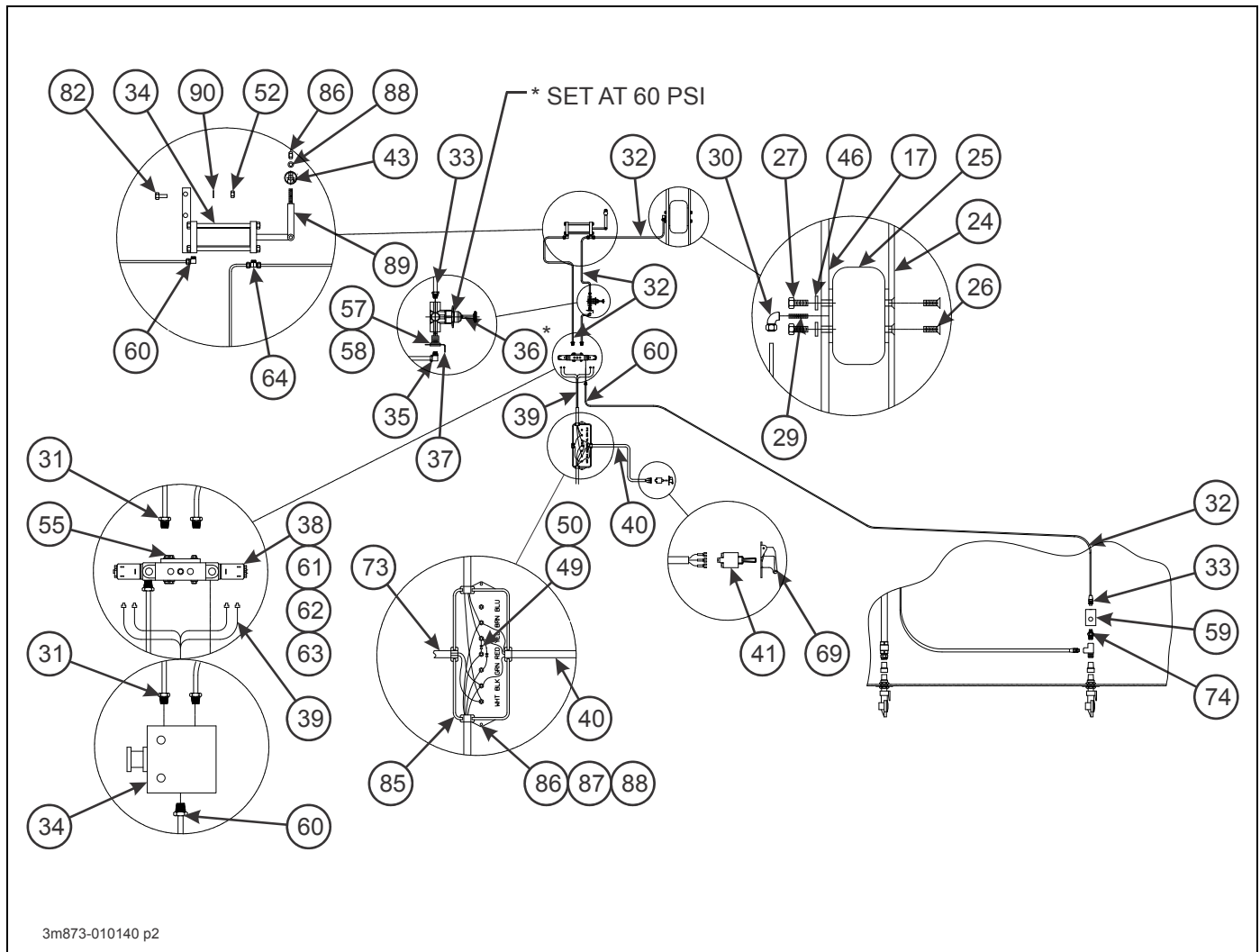
Figure 2-89: Winch Installation (2 of 2)
