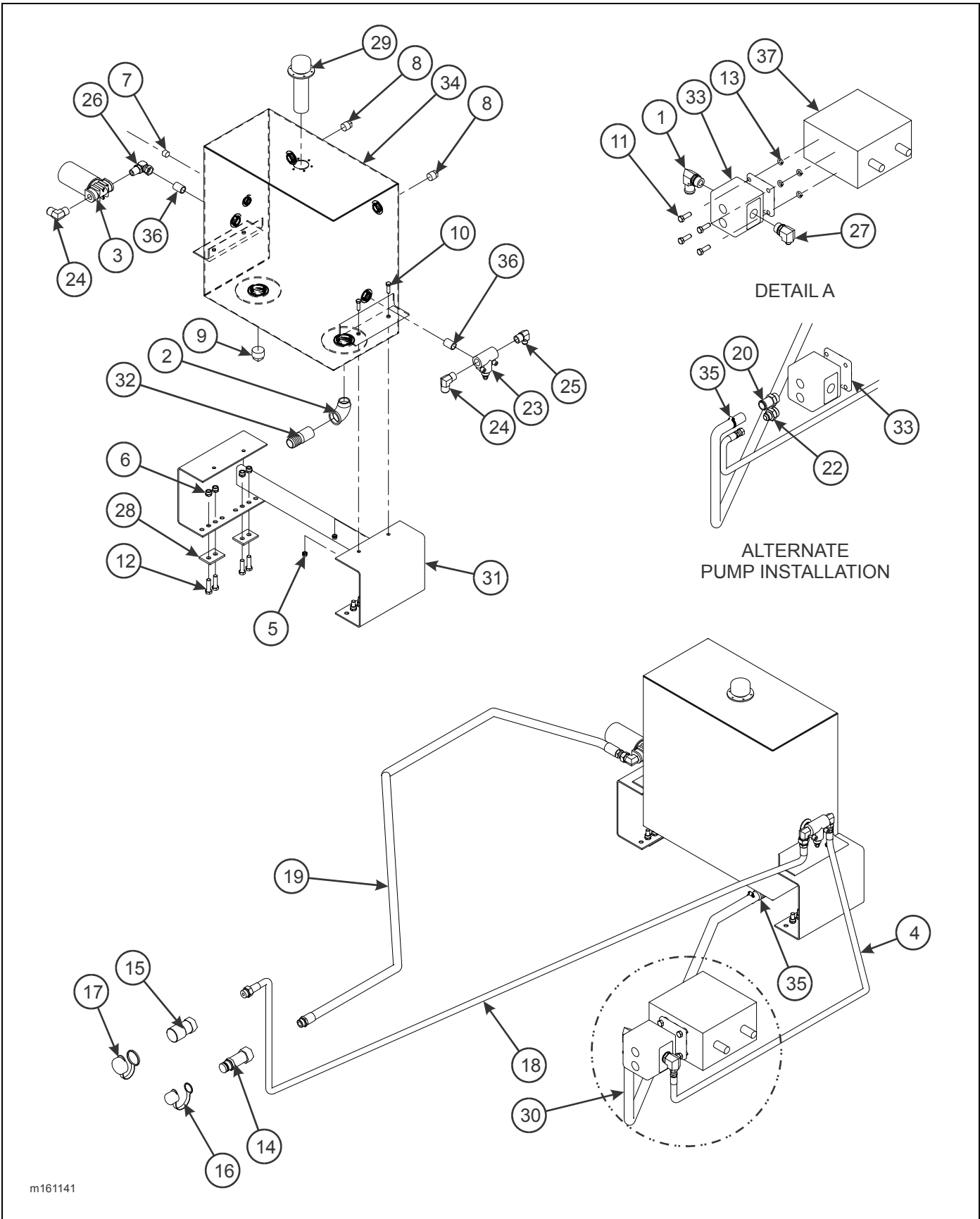
Figure 2-23: 30 Gallon Hydraulic Wet Kit Items
