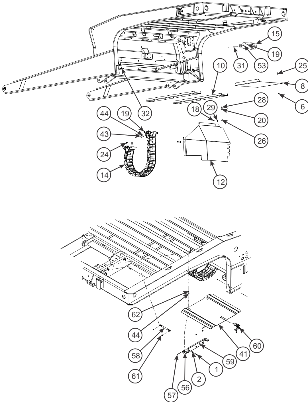
GALVANIZED FLIP-UP TOOLBOX OPTION
