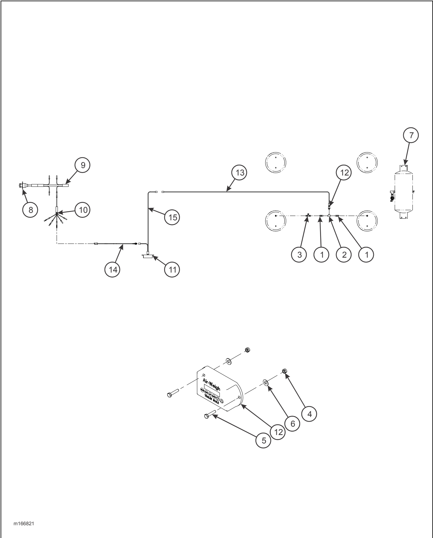
Figure 2-179: Air Digital Scale, Loadmaxx System (Option)
