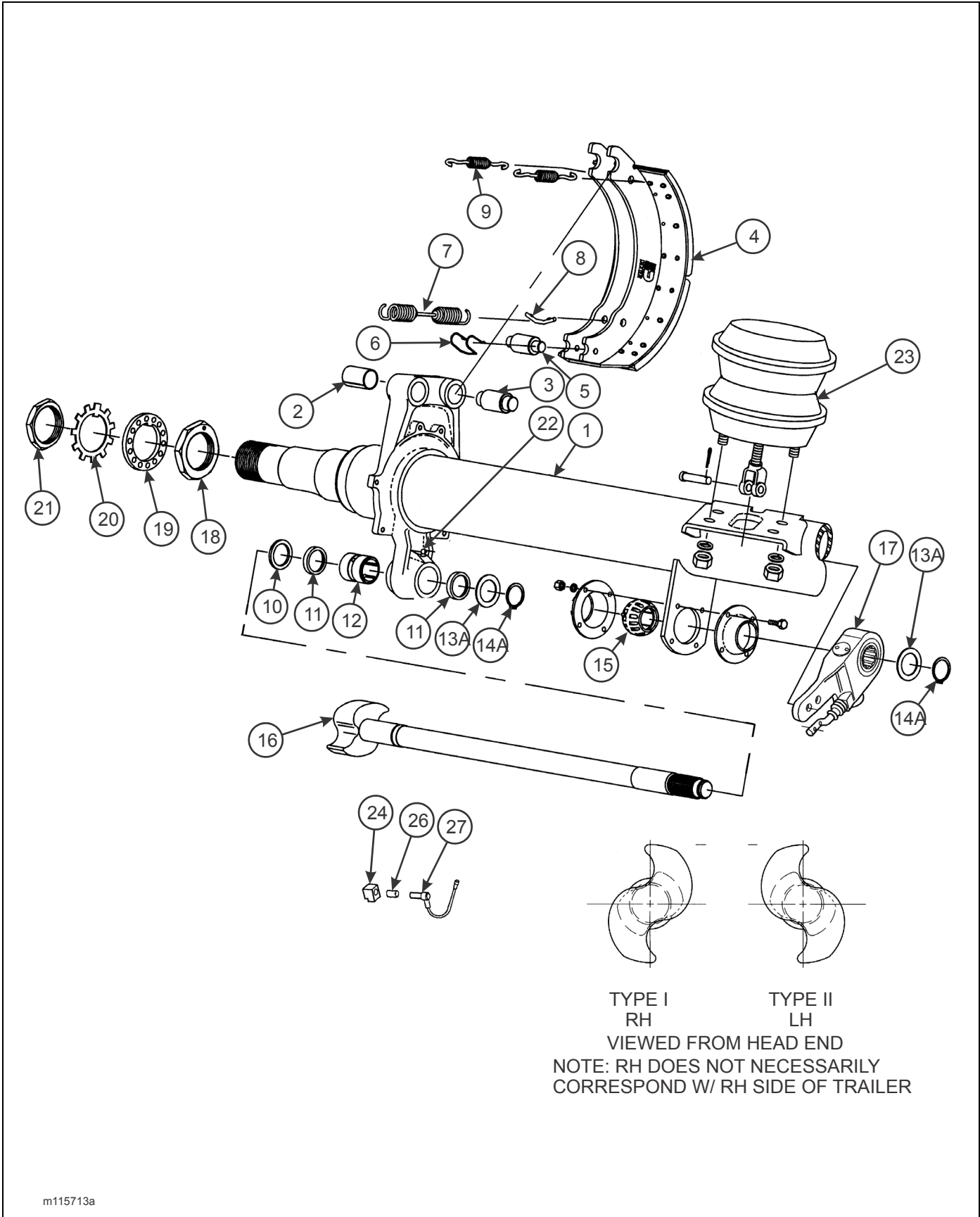
Figure 2-51: Axle and Brake Assembly (16-1/2" x 7")
