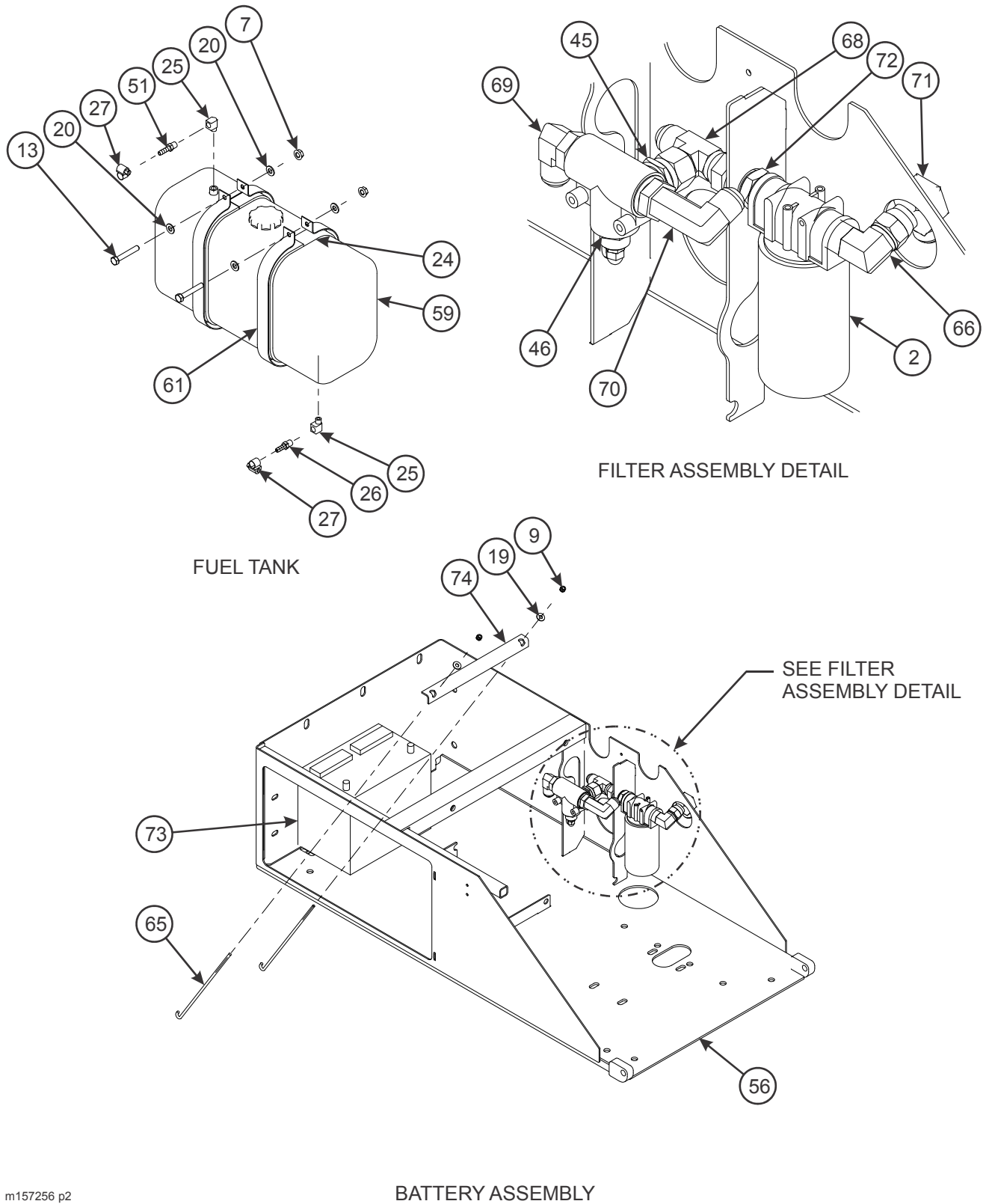
Figure 2-146: 25HP Diesel Engine Installation (2 of 4)
