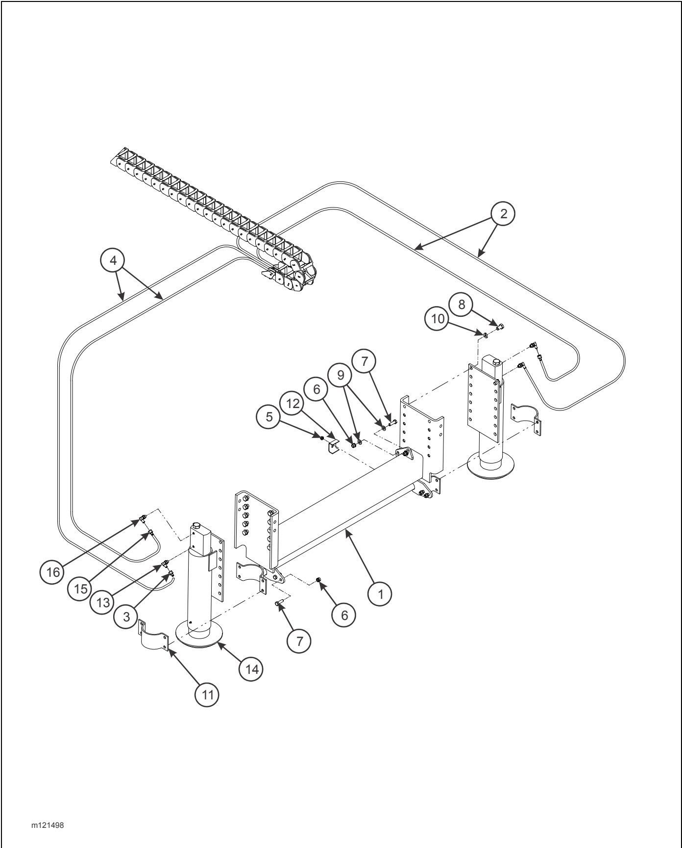
Figure 2-125: Dock Leveler Assembly, Single 60K
