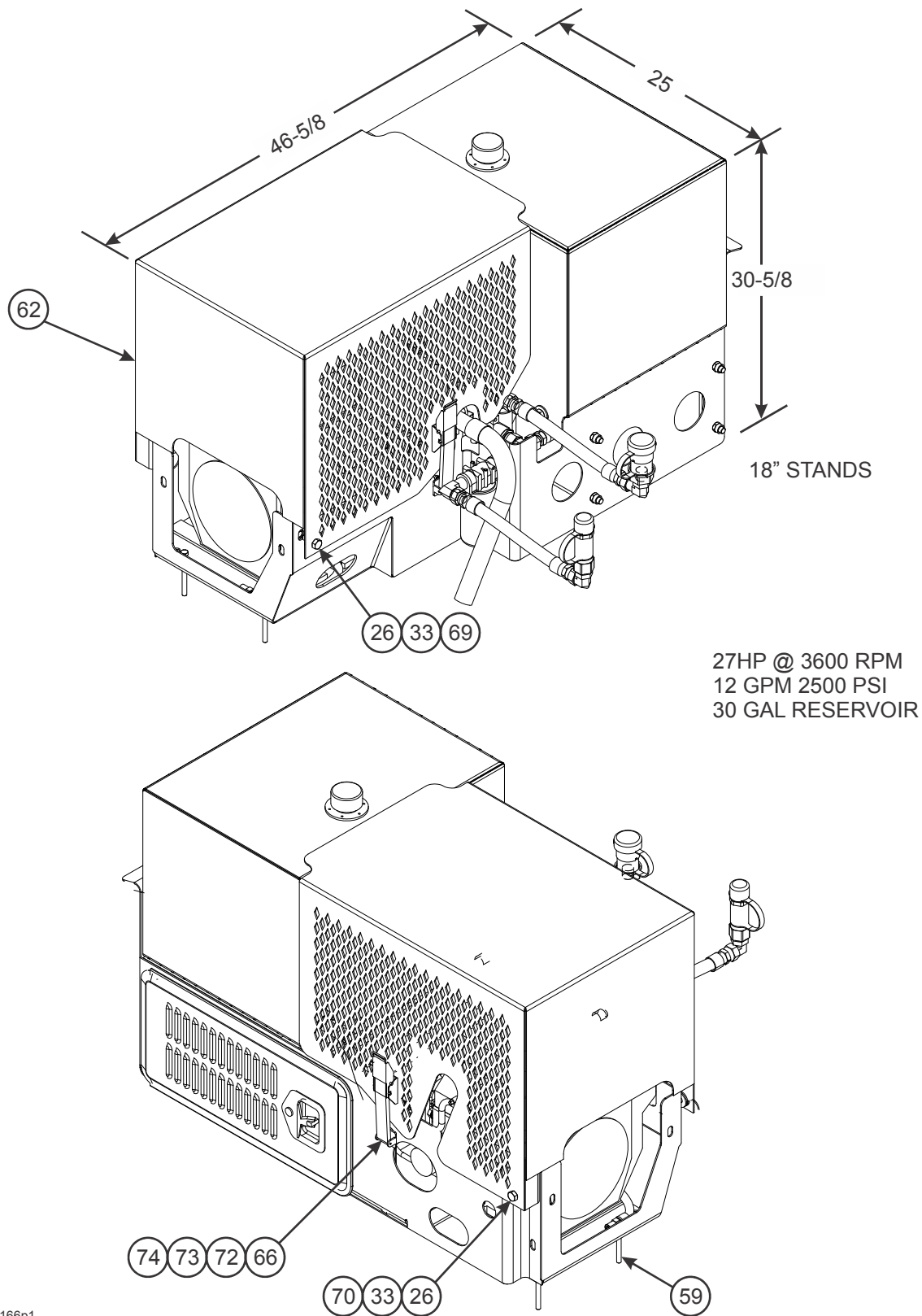
Figure 2-141: Upper Deck Engine Installation (1 of 4)
