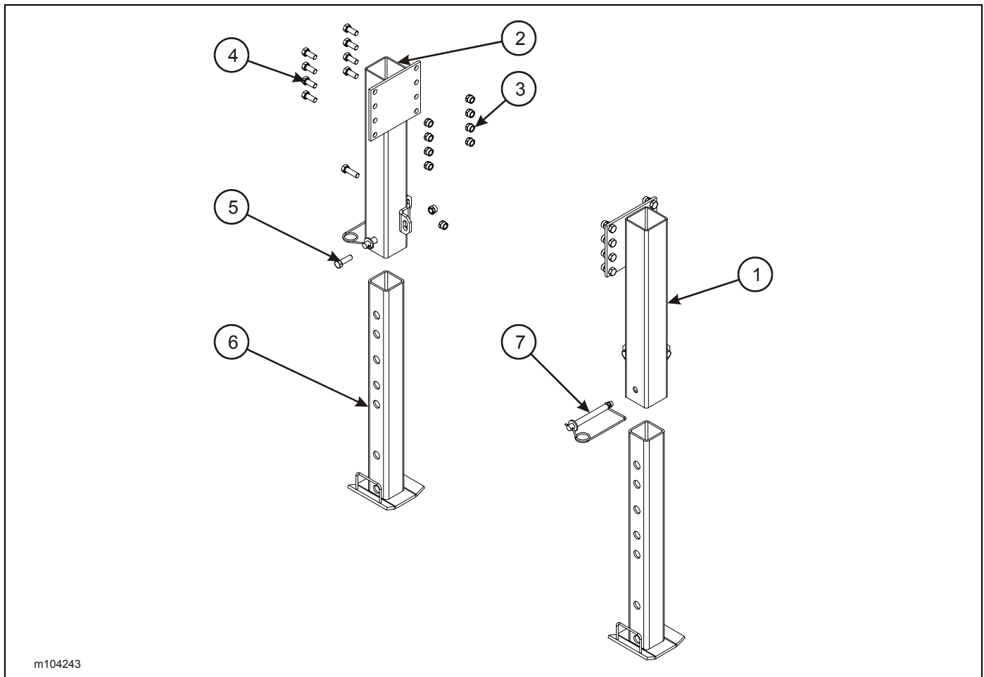
Figure 2-136: Landing Gear Installation
