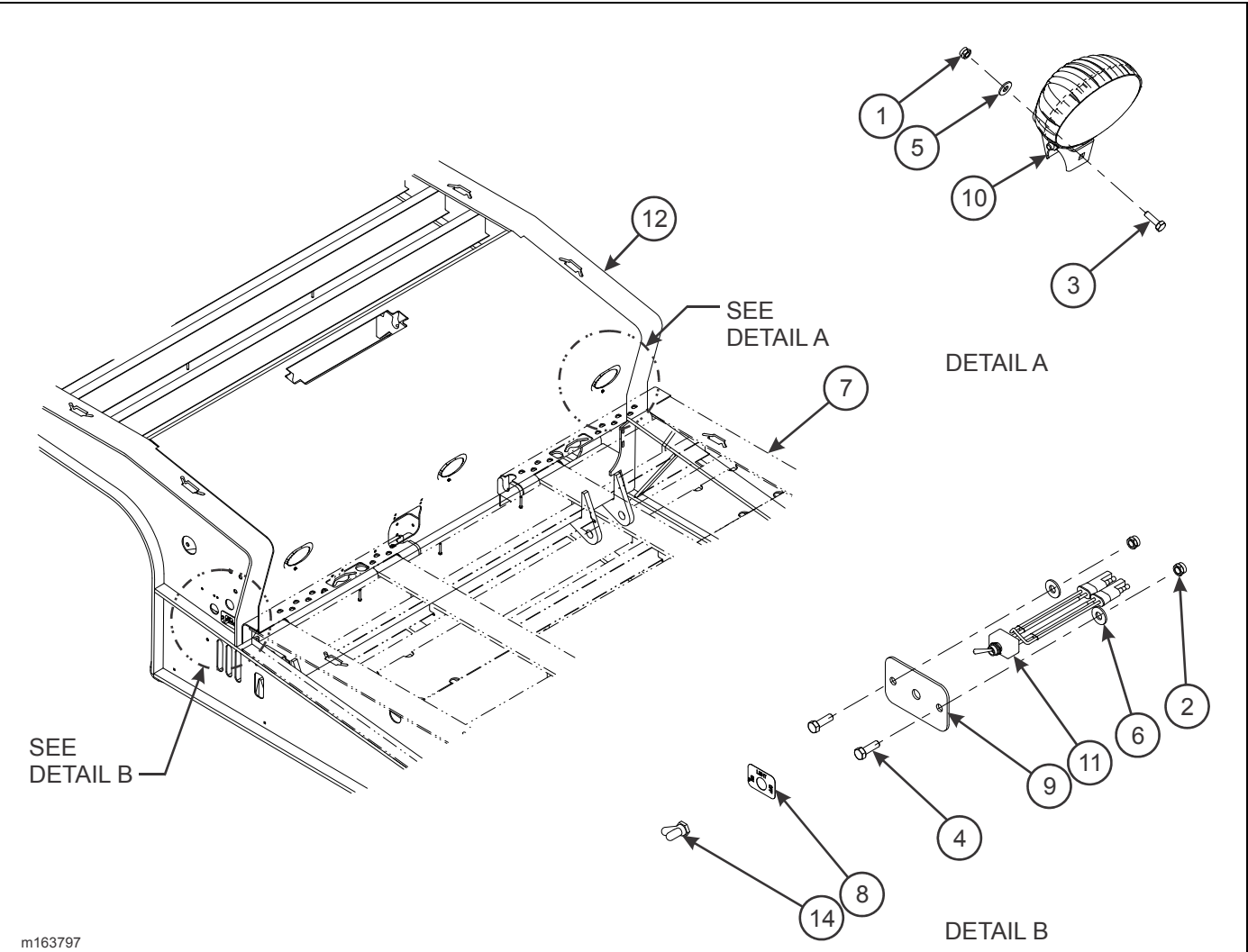
Figure 2-163: Slope Work Light Installation, LED (Option)
