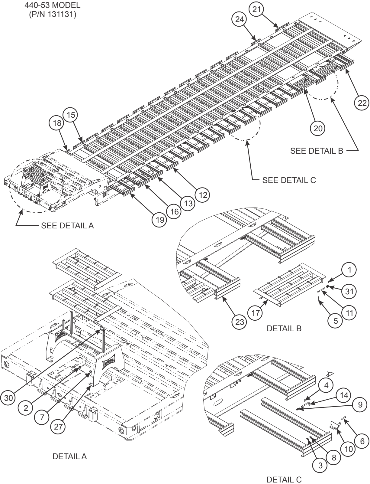
Figure 2-67: Pullout Installation (440) (3 of 3)
