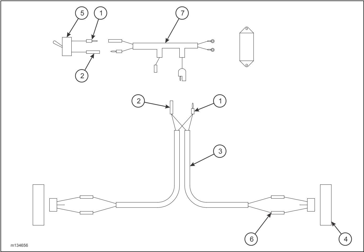
Figure 2-155: Strobe Light Installation Side (Option)
