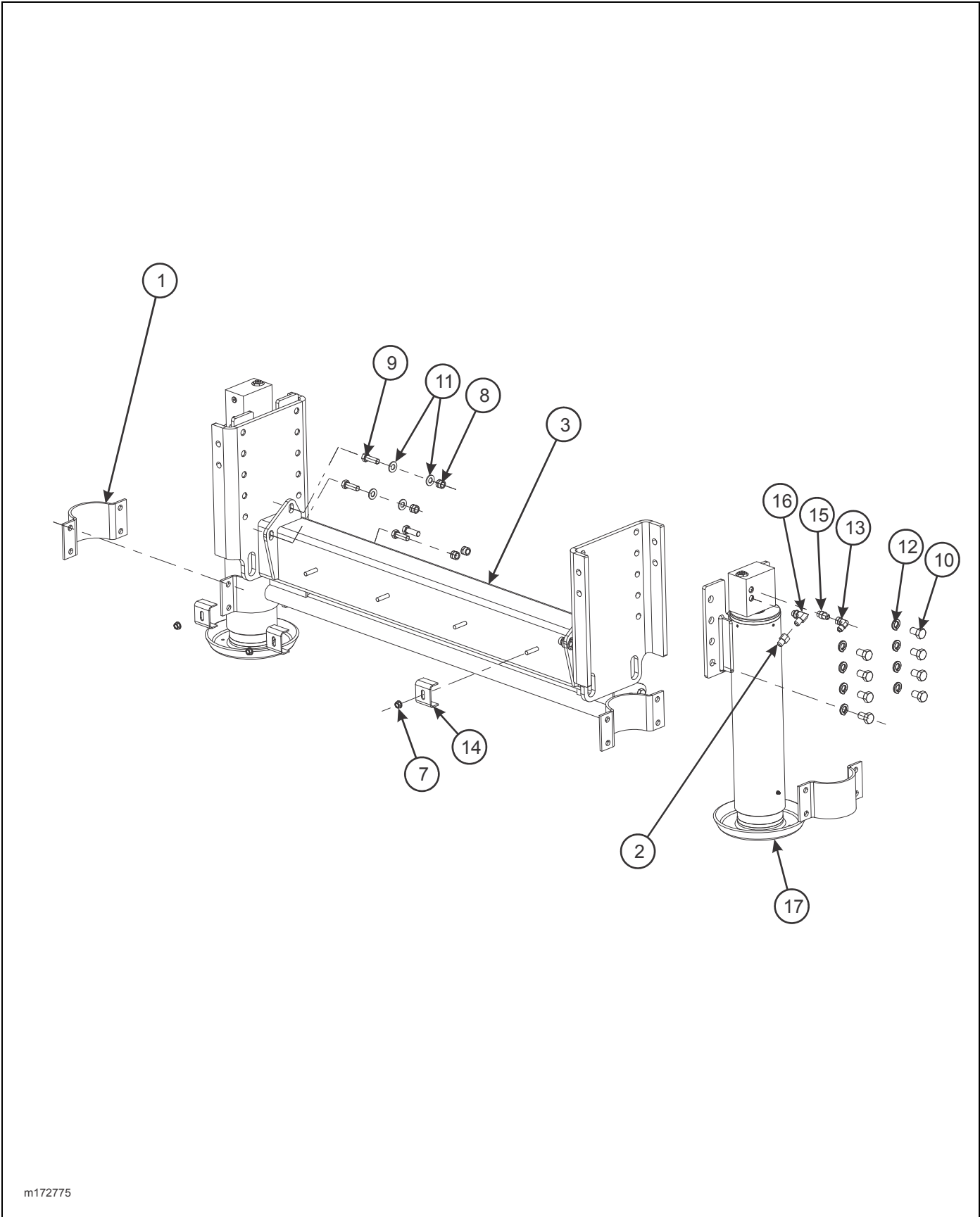
Figure 2-126: Dock Leveler Assembly, Single 60K Arctic
