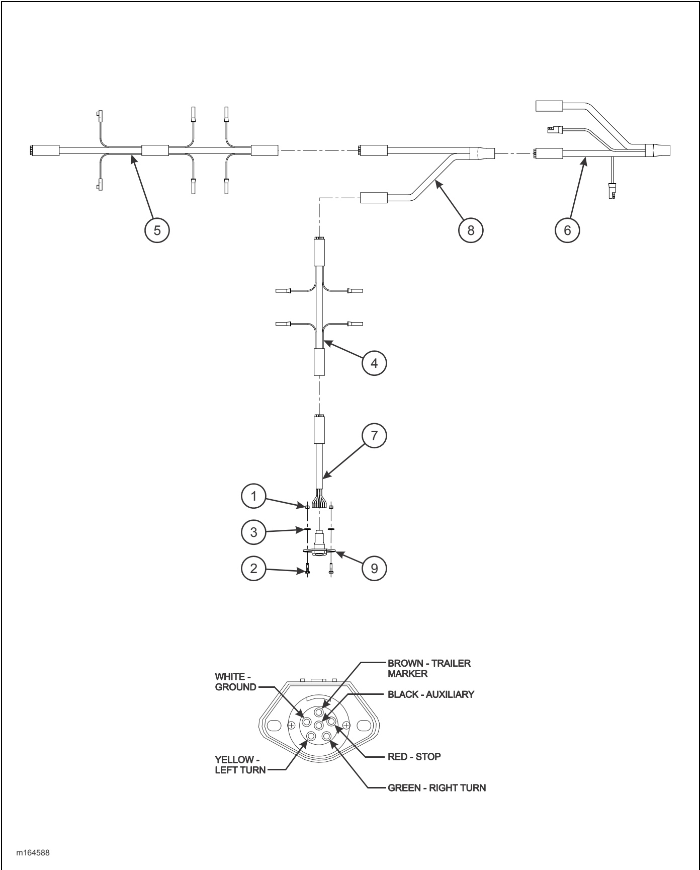
Figure 2-158: 6-Way Electrical Installation (Option)
