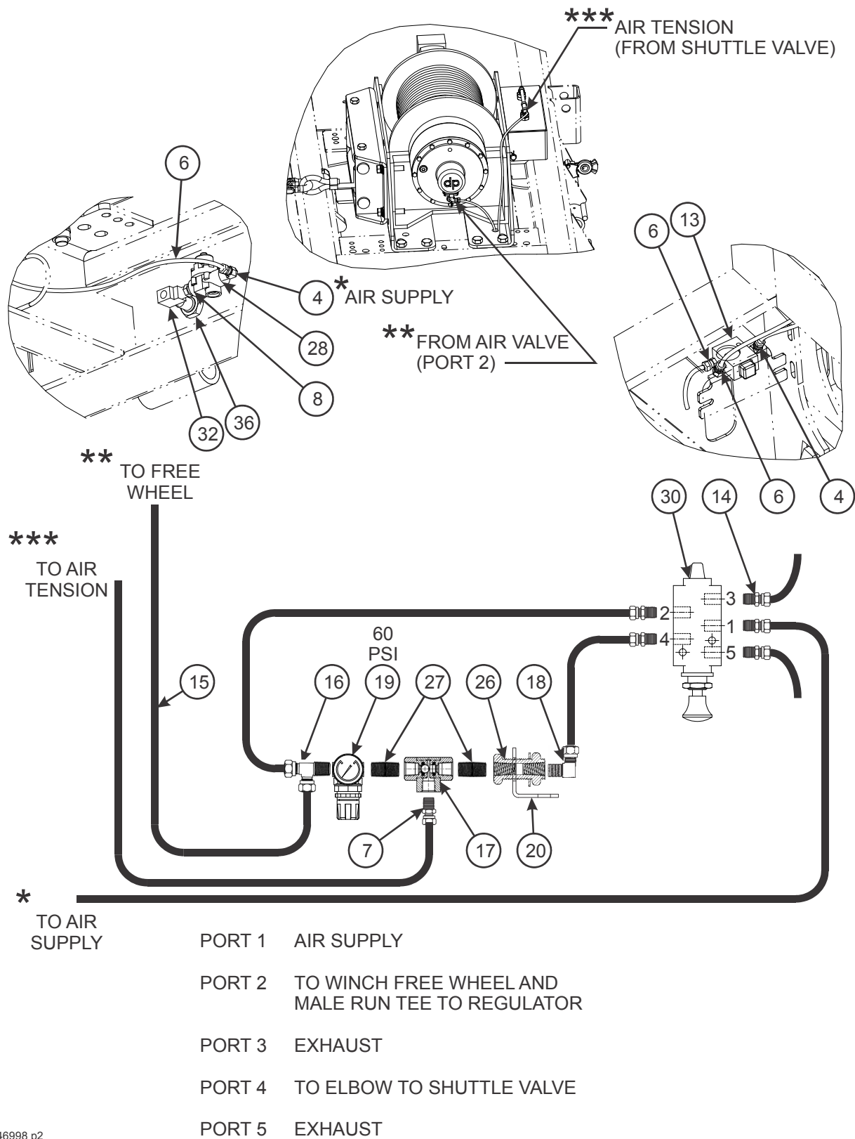
Figure 2-101: 30,000 Lb. Upper Deck Winch Installation (3 of 3)
