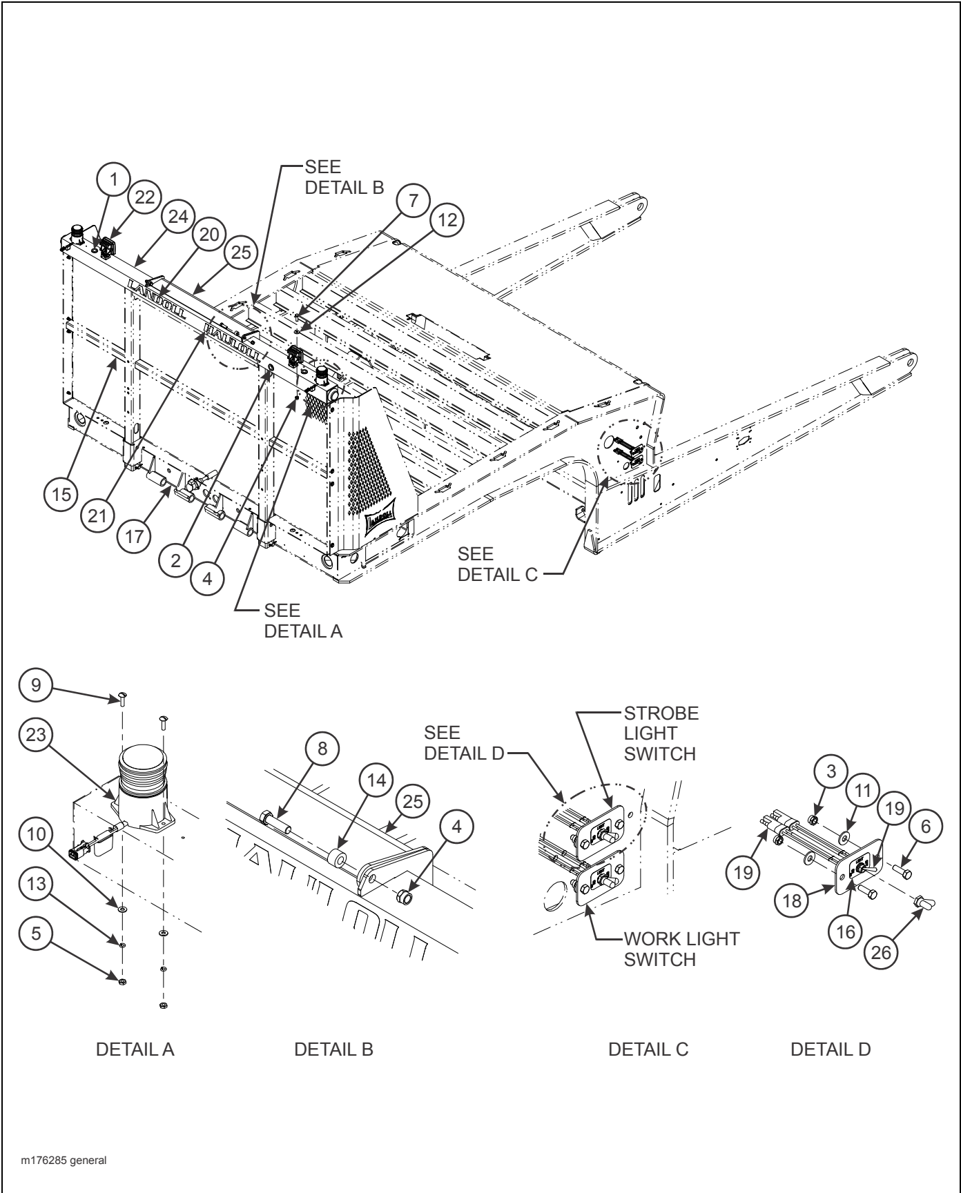
Figure 2-61: Bulkhead Chain Rack Light General Assembly
