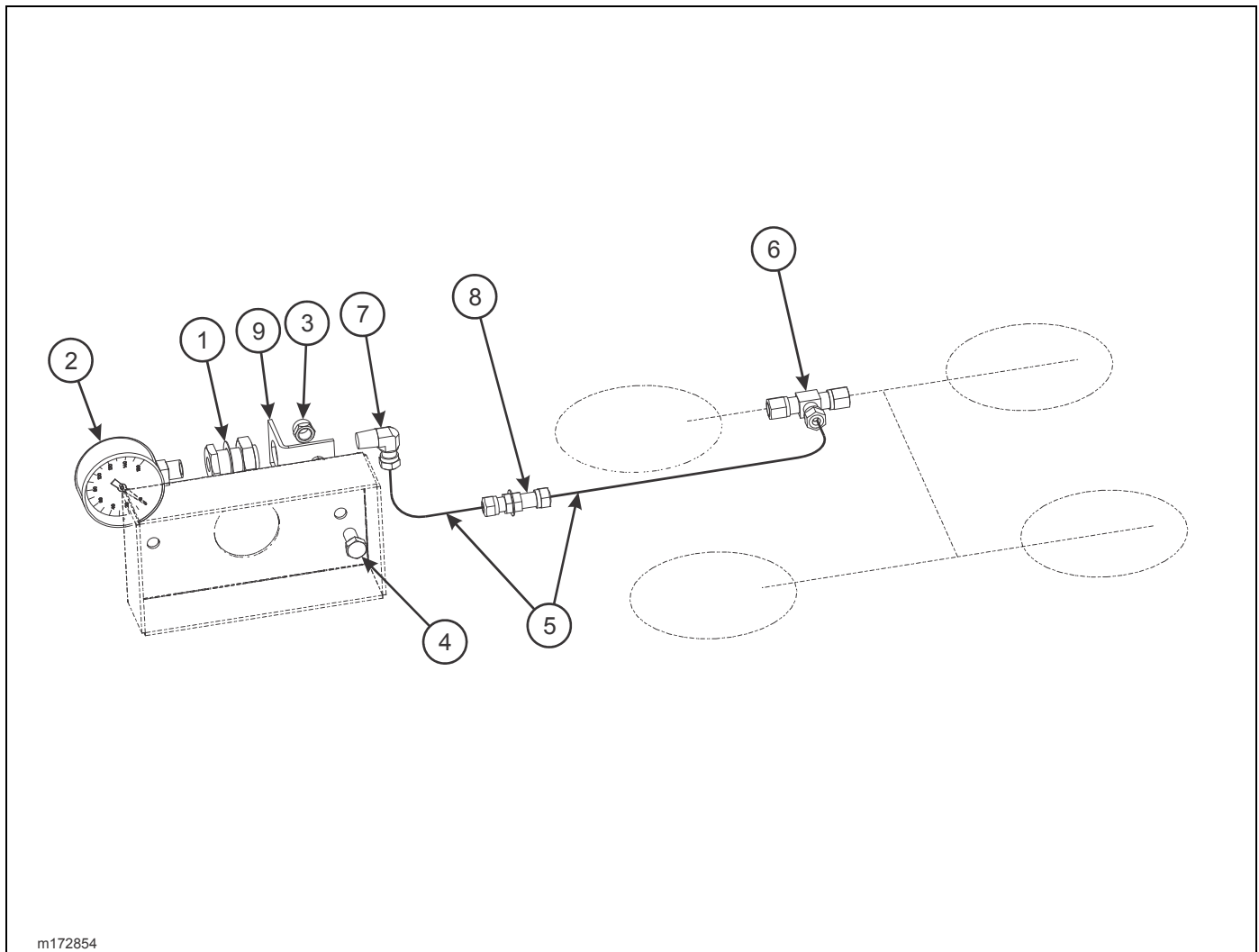
Figure 2-186: Pressure Gauge Installation, Arctic (Option)
