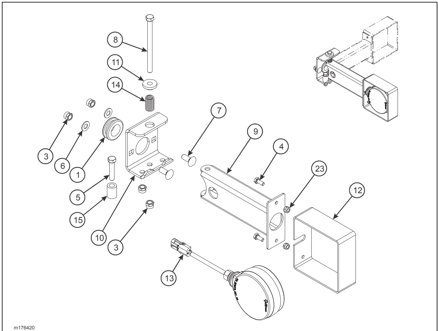
Figure 2-170: Swingout Light Installation (Option)
