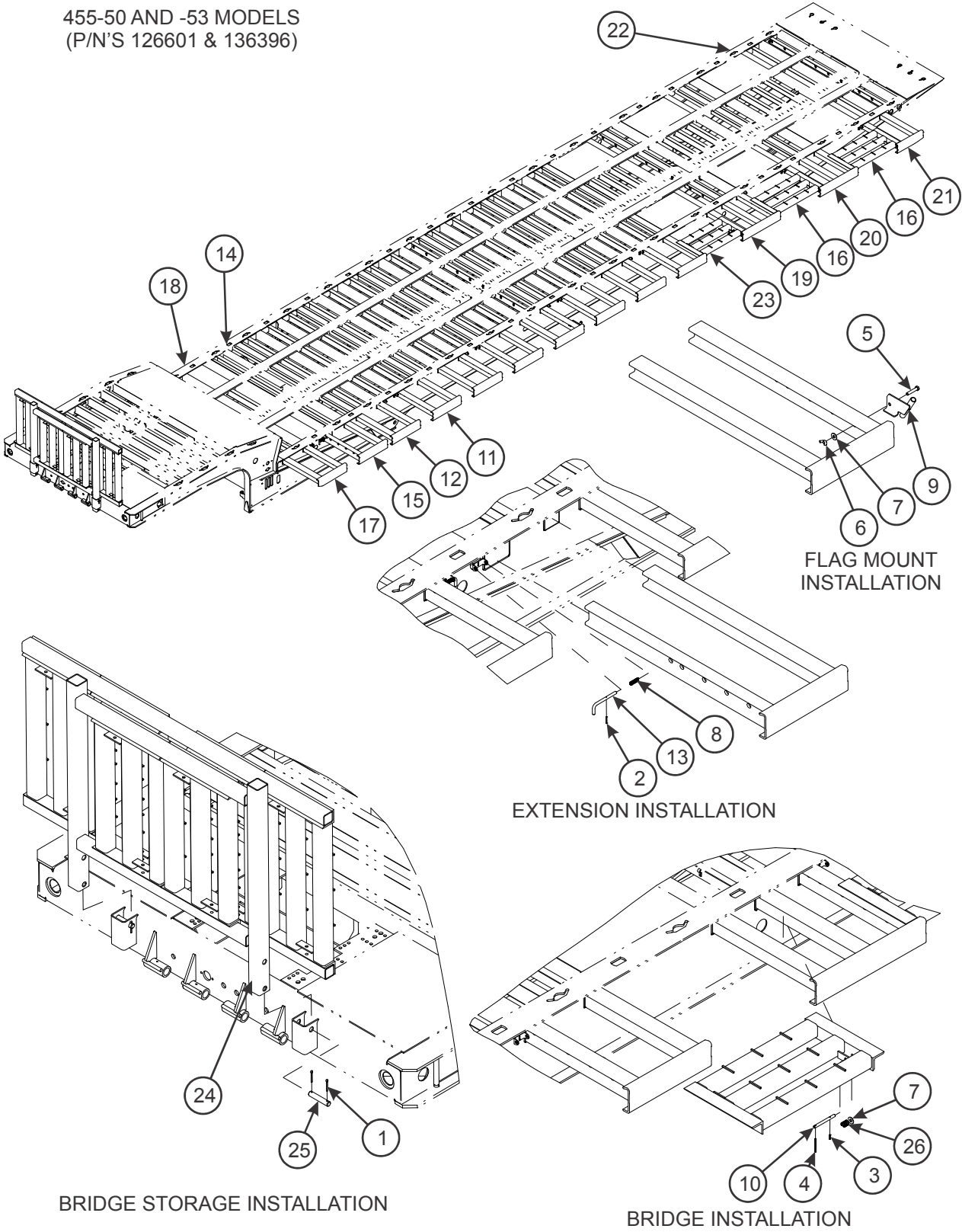
Figure 2-68: Pullout Installation (455) (1 of 3)
