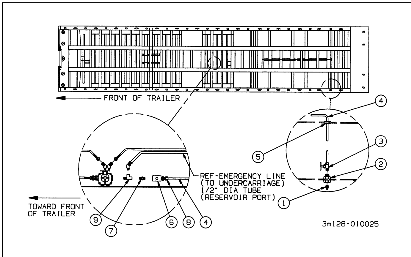
Figure 2-177: Air Outlet Accessory (Option)
