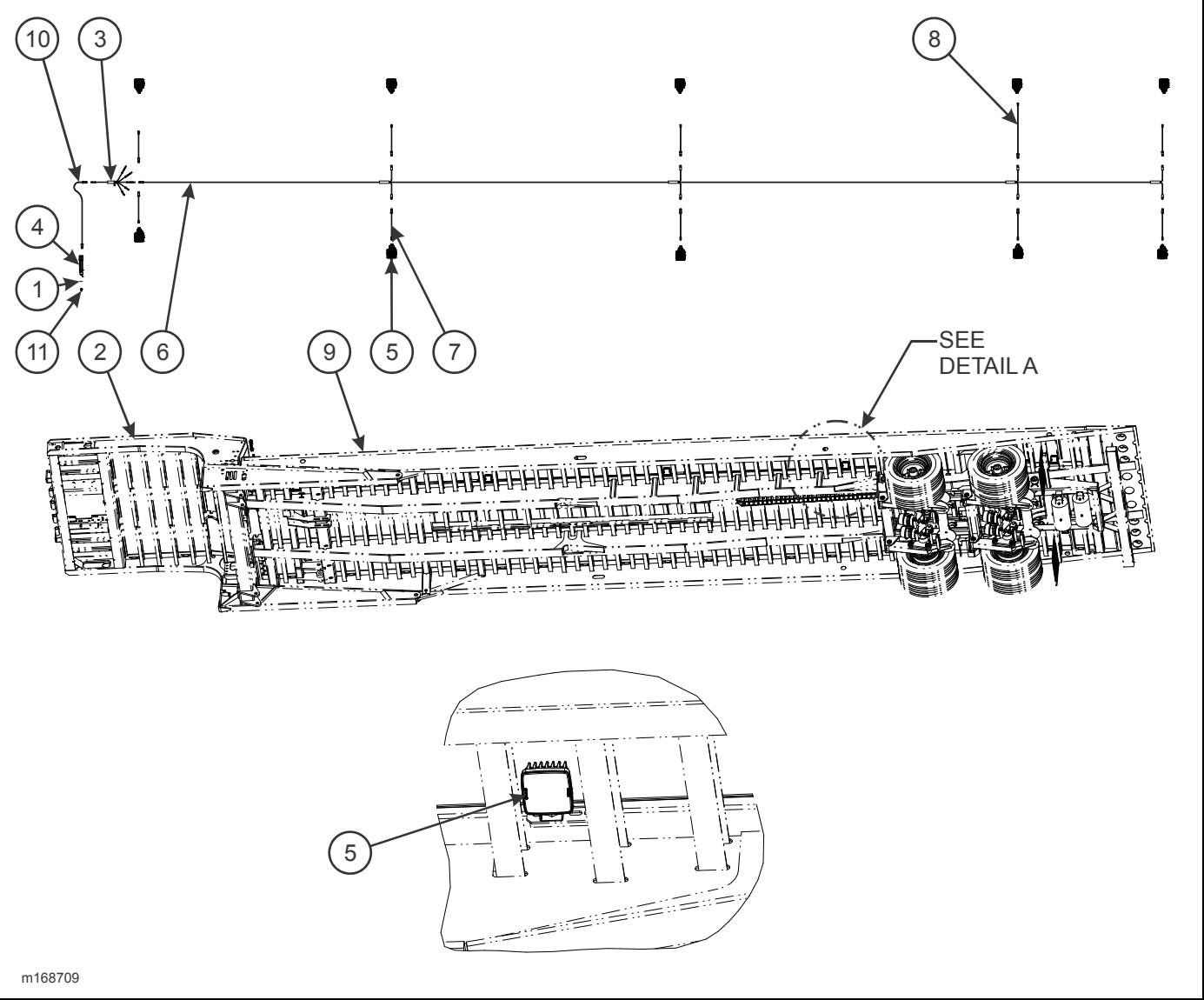
Figure 2-161: Underdeck Light Installation (440-53) (Option)
