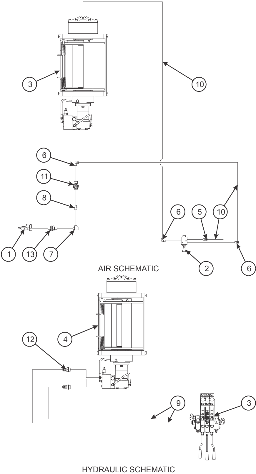
Figure 2-80: 30K Winch Installation, Hydraulic/Air Items (Warn)
