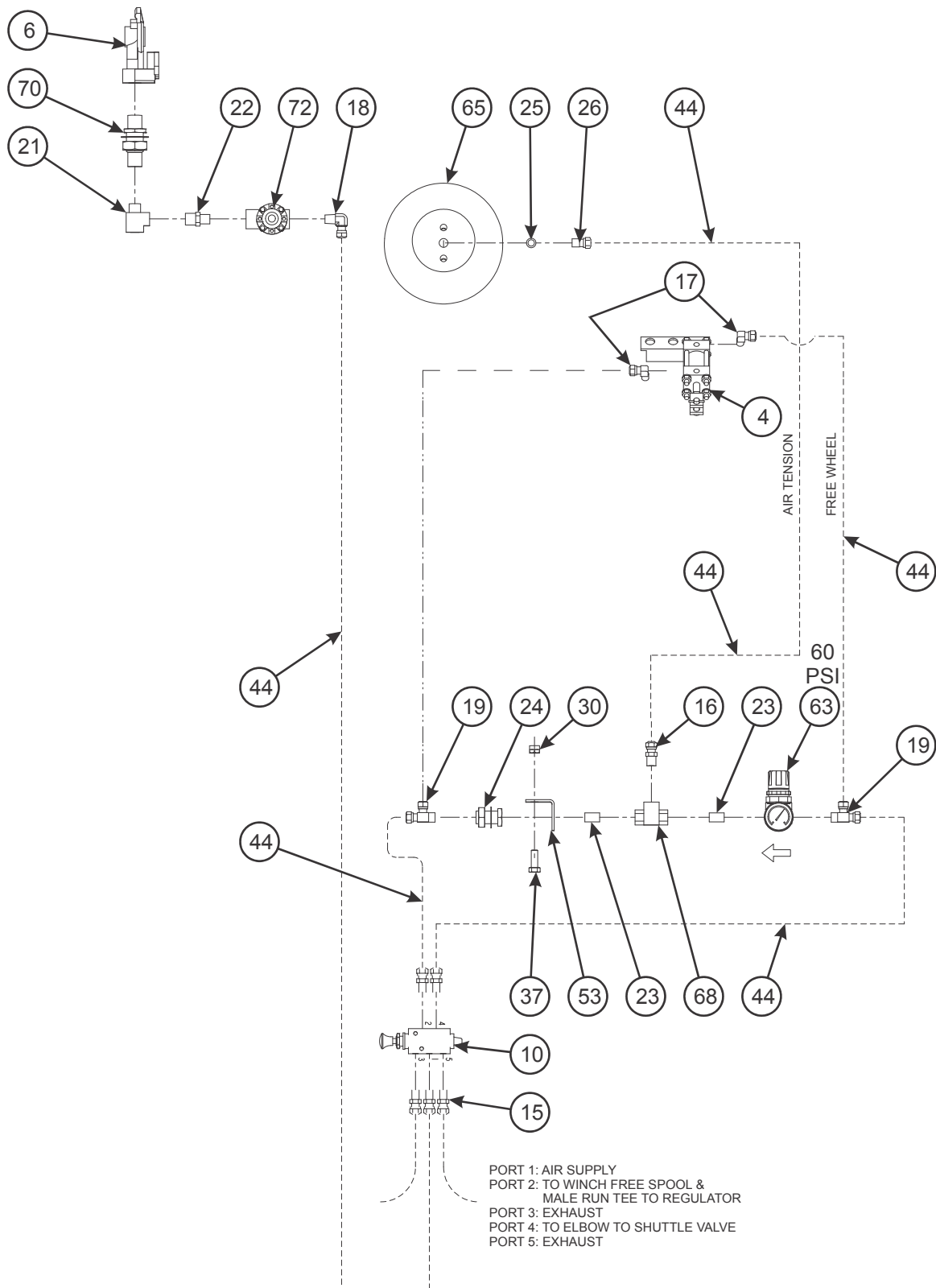
Figure 2-93: 20K Air Tension/Release Winch Installation (2 of 2)
