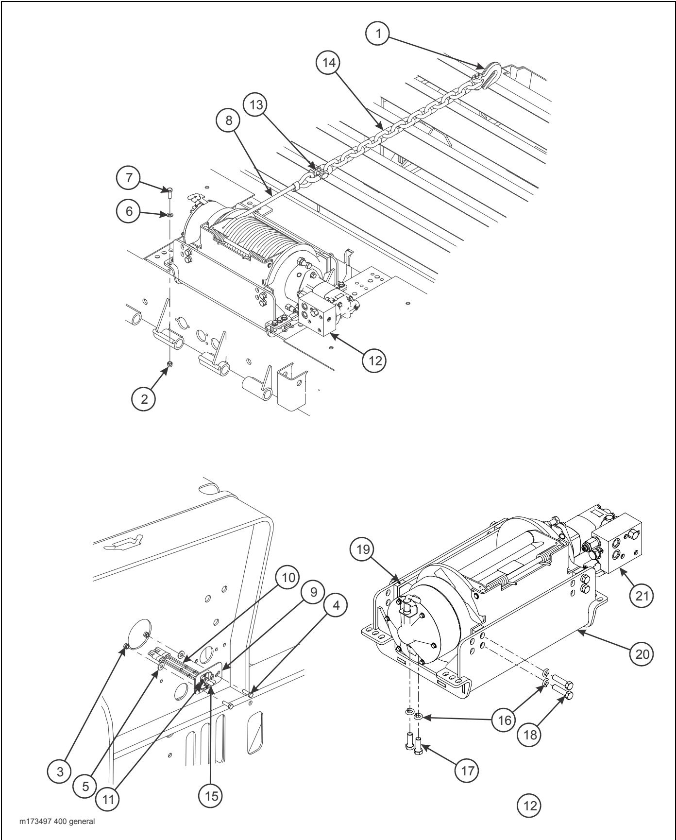
Figure 2-85: 30K 2 Speed Winch Installation, General Items (Warn)
