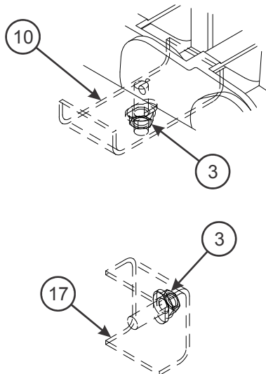
Figure 2-118: 8 Pop-Up Roller Installation (Option) (2 of 2)
