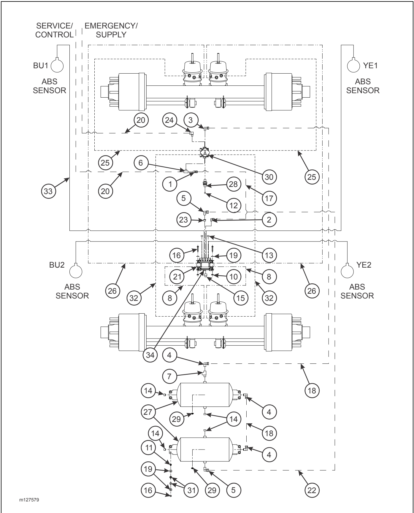
Figure 2-39: Spring Air Brake System w/ ABS (425 & 440 (Aqua Package))
