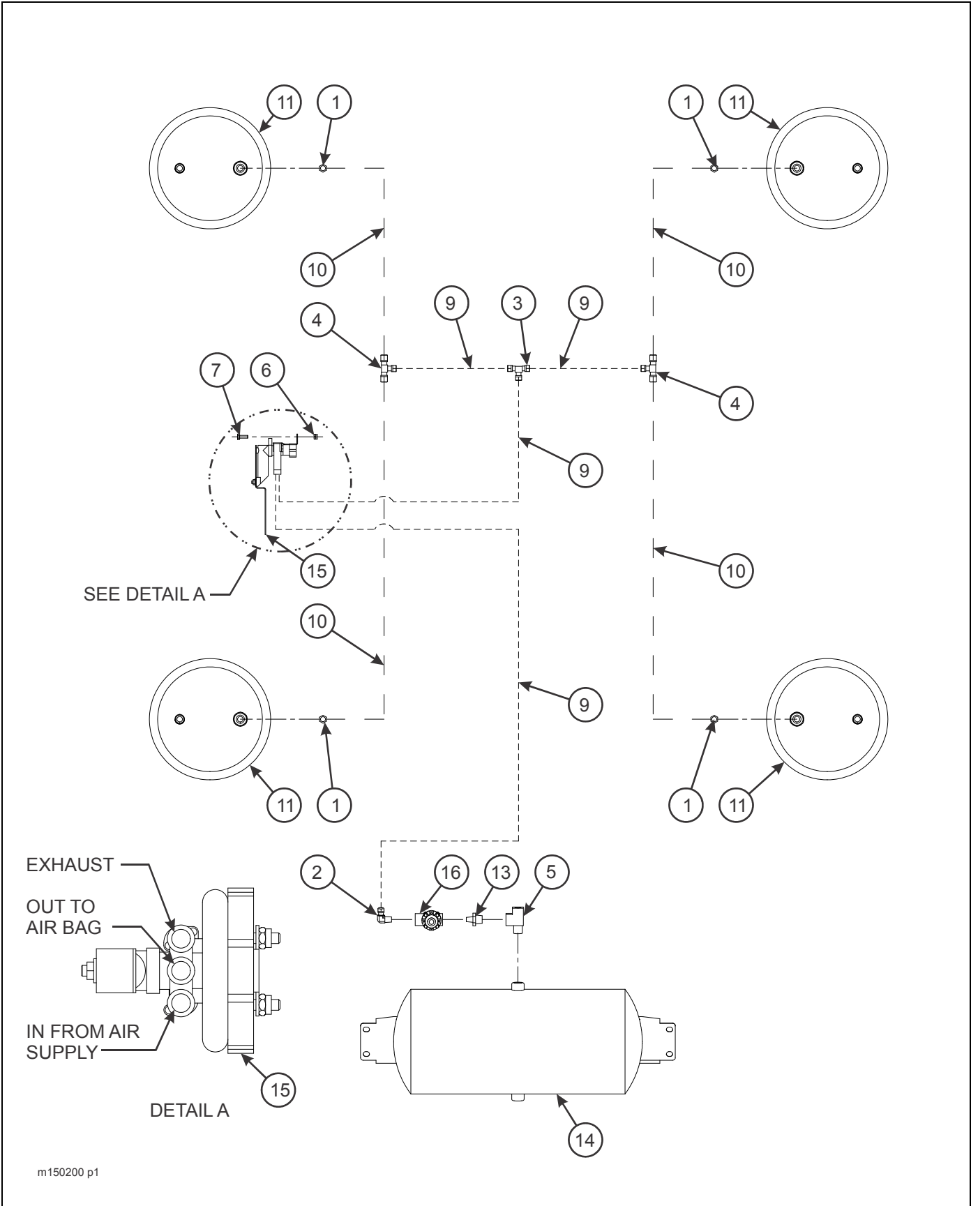
Figure 2-45: Air Ride Suspension, Air System (Tandem)
