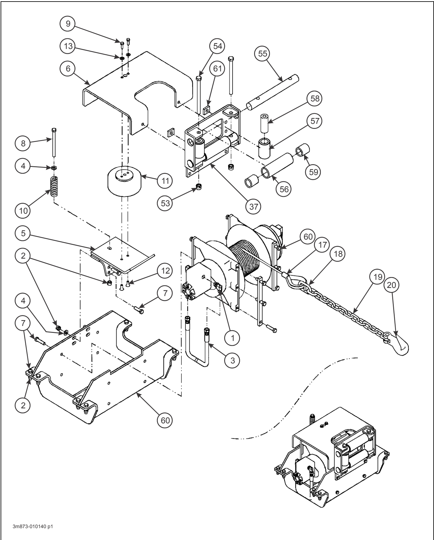
Figure 2-105: 12K, 15K, & 20K Upper Deck Winch (DP) (1 of 2)
