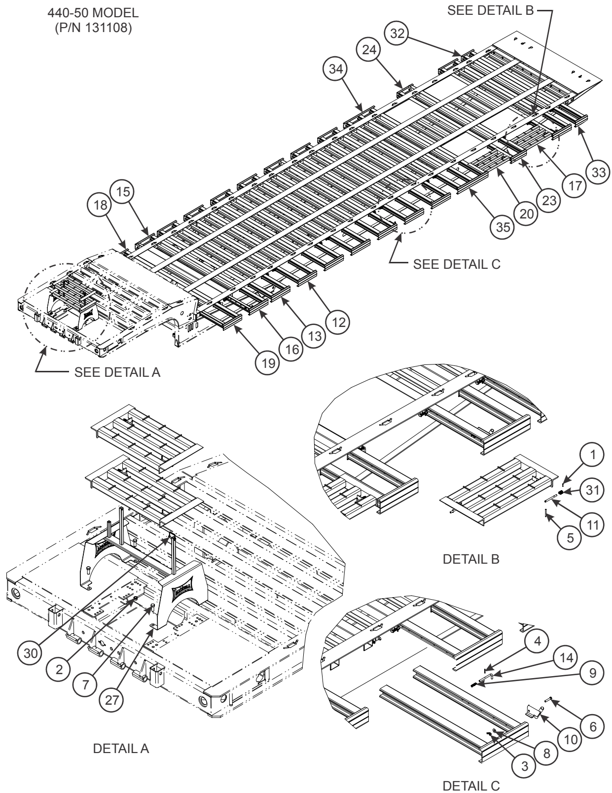
Figure 2-66: Pullout Installation (440) (2 of 3)
