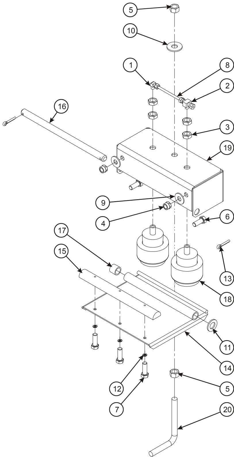
Figure 2-104: Winch, Cable Air Tension
