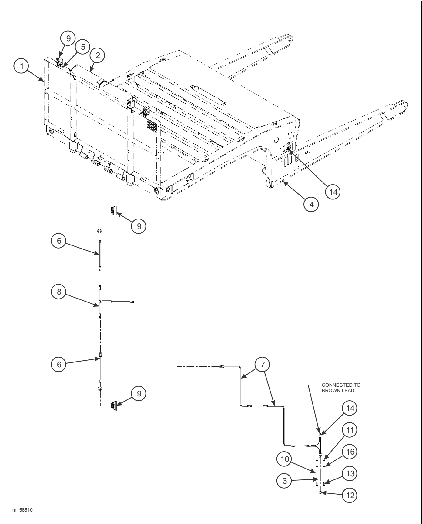
Figure 2-160: Work Light Assembly, Bulkhead (Option)
