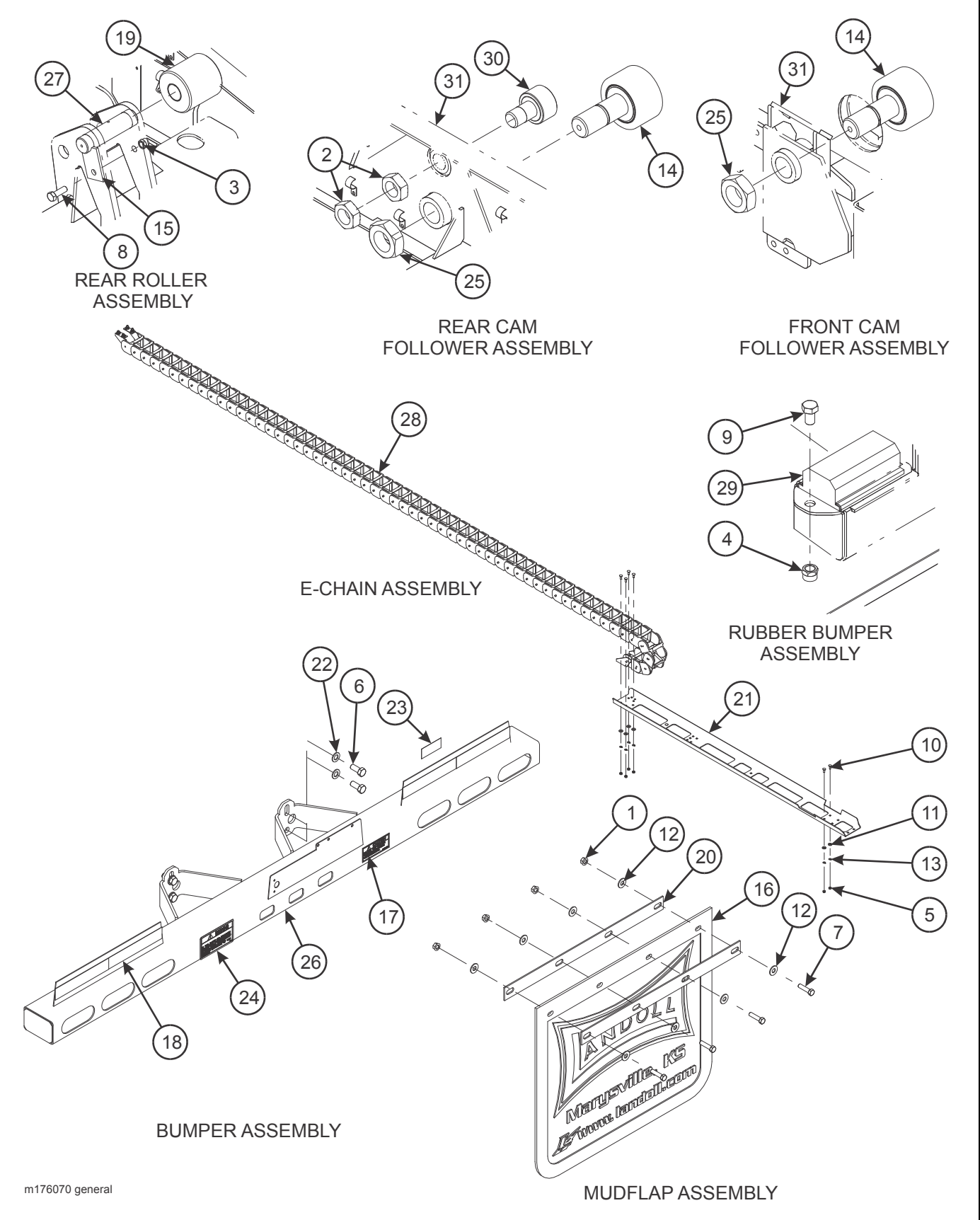
Figure 2-54: Disk Brake Suspension, General Assembly
