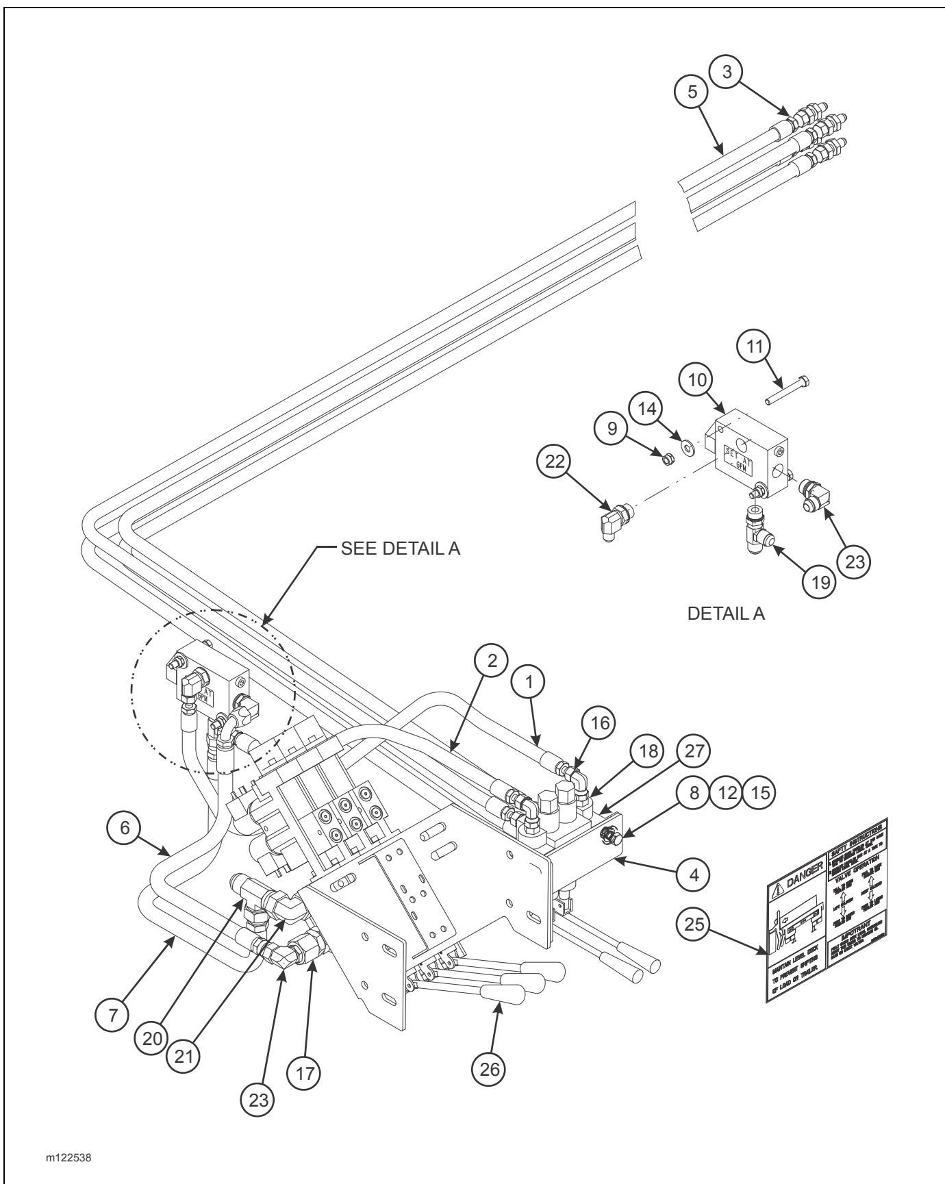
Figure 2-123: Dock Leveler Hydraulic Installation (1 of 2) (Option)
