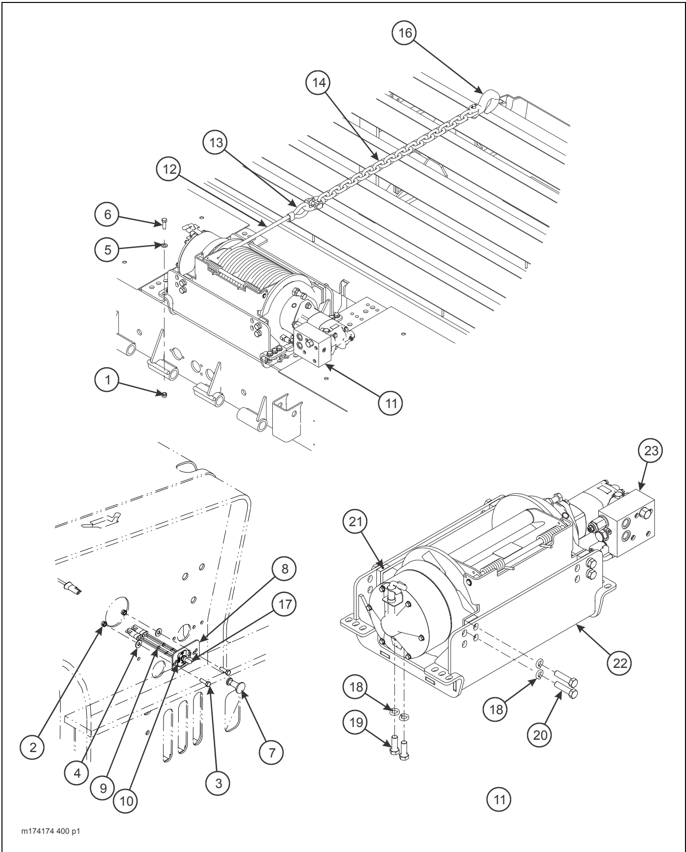
Figure 2-76: Winch Installation, 20K 2 Speed General Items (Warn)
