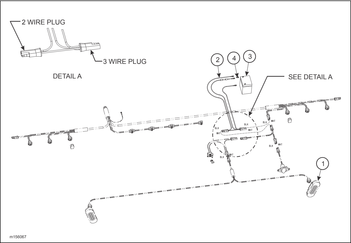
Figure 2-165: Battery Backup Bumper Strobe Light Installation (Option)
