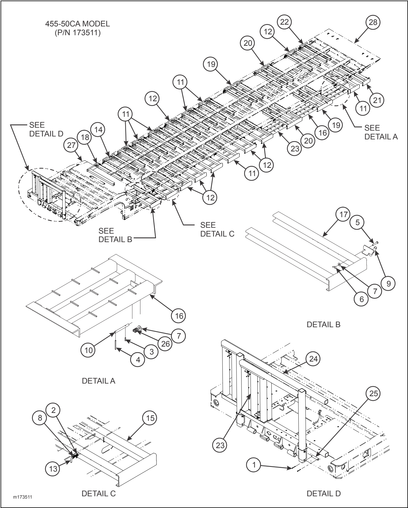
Figure 2-70: Pullout Installation (455) (3 of 3)
