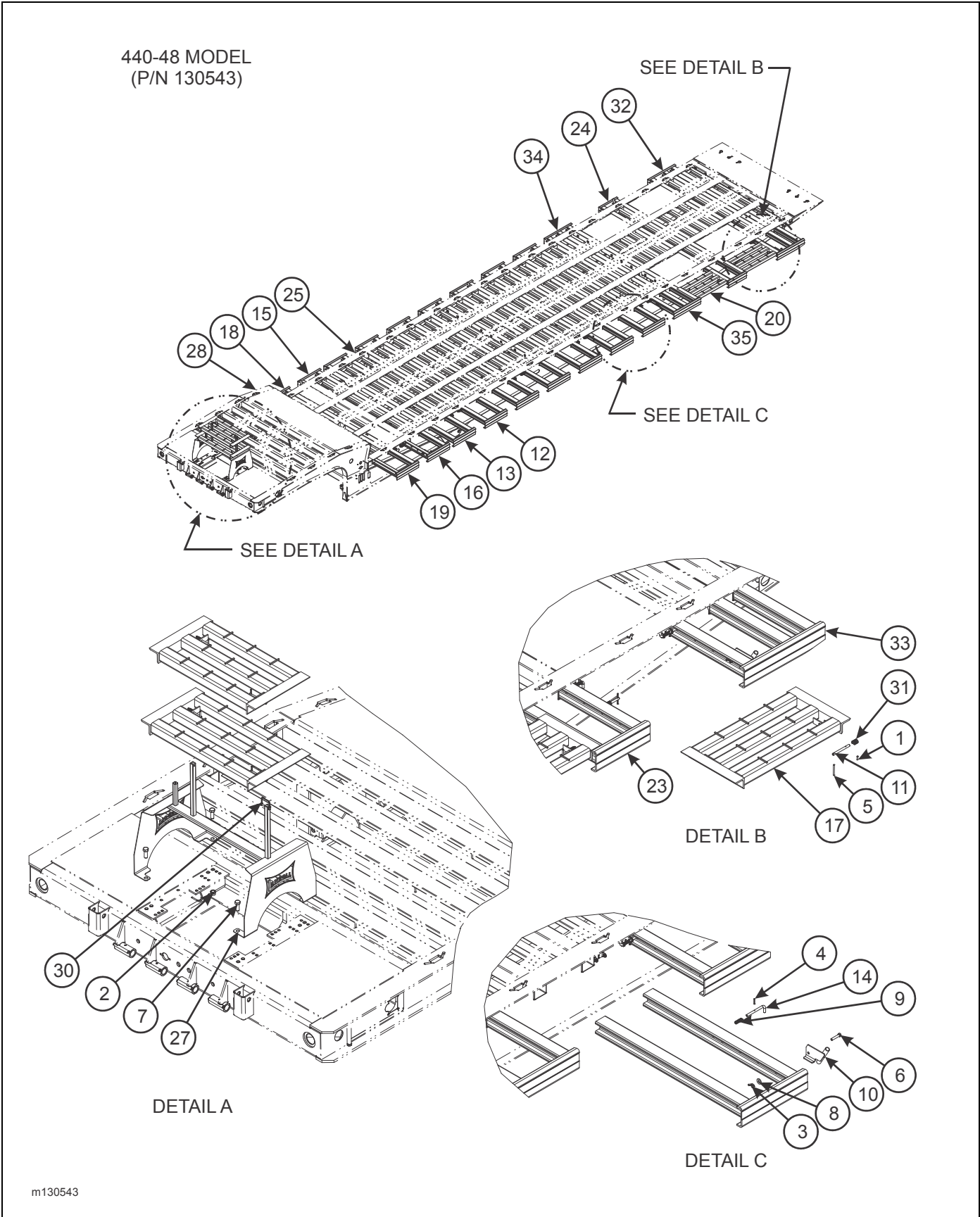
Figure 2-65: Pullout Installation (440) (1 of 3)
