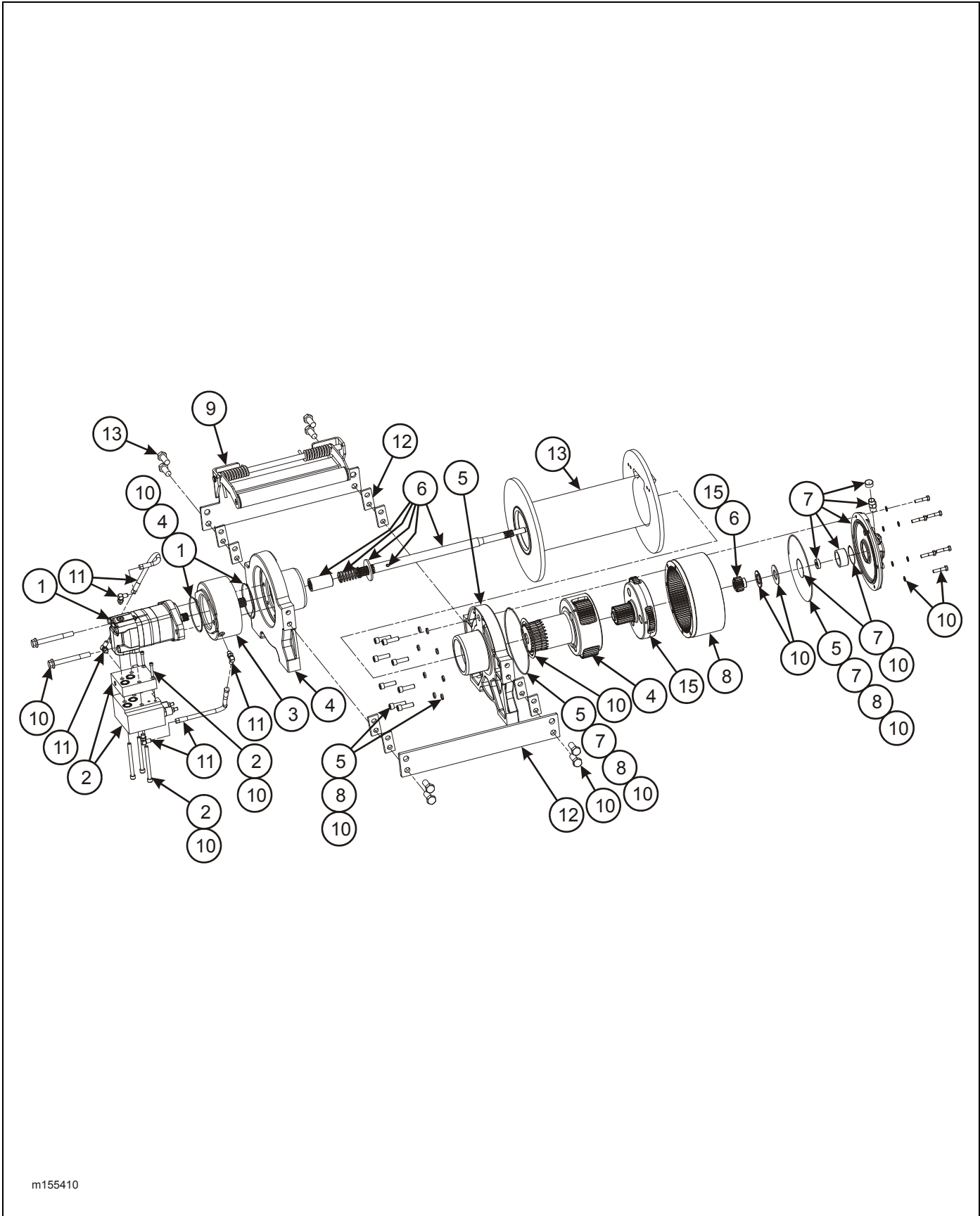
Figure 2-84: 30K Winch Items (Warn)
