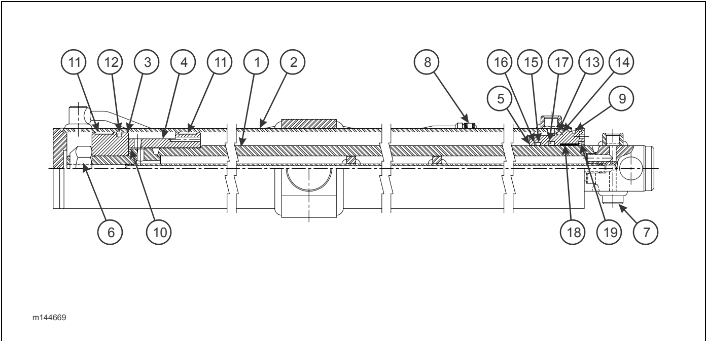
Figure 2-19: Cylinder, Hydraulic 4 x 138 Ported Rod (Streetside) (440-53)
