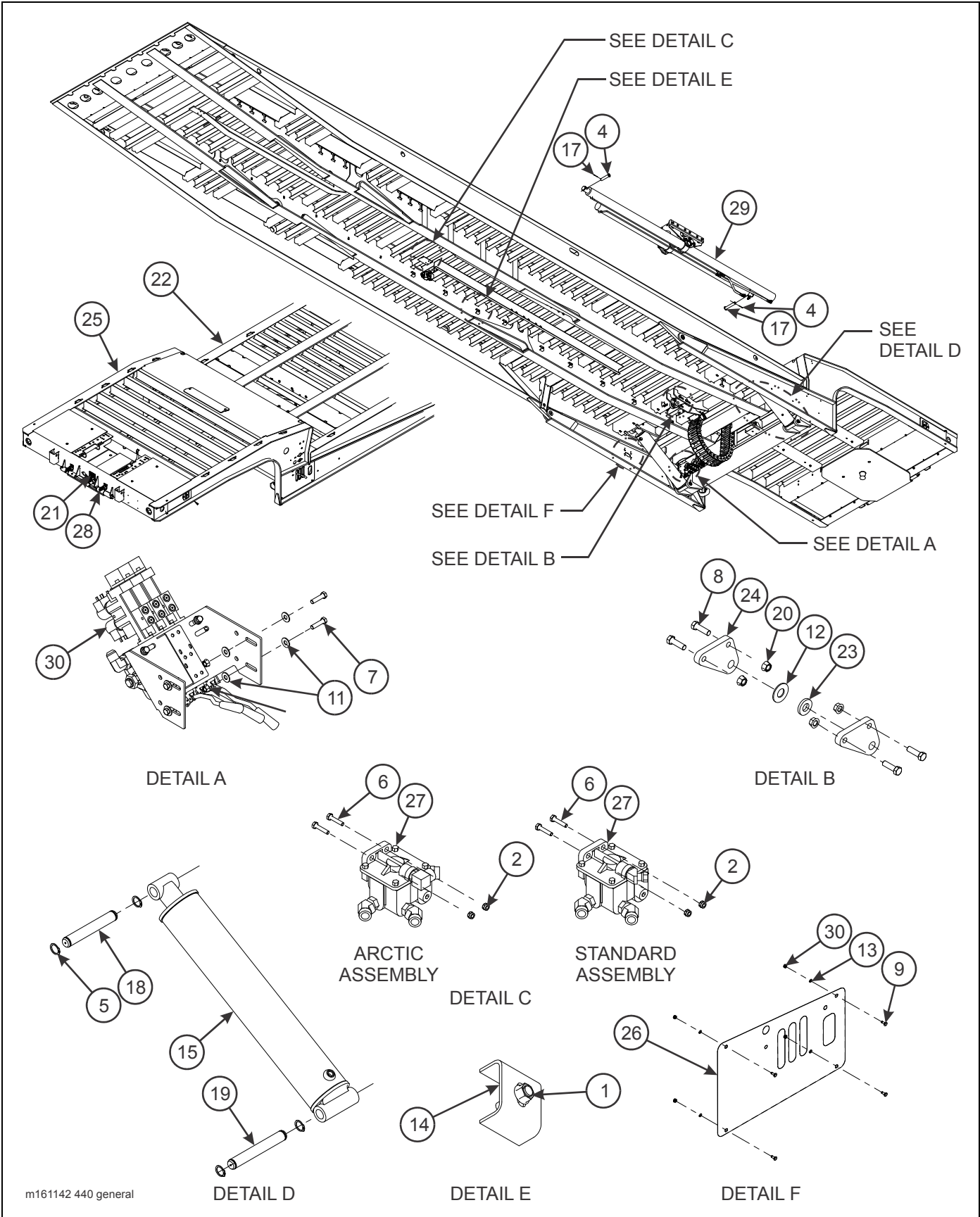
Figure 2-8: Hydraulic Electrical Air General Assembly (455)
