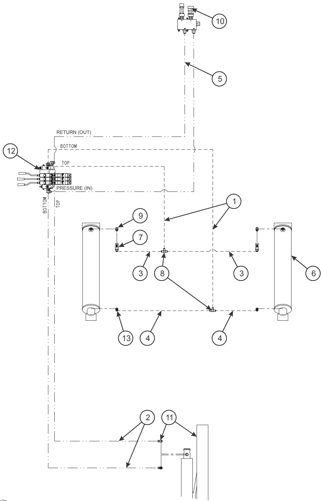
Figure 2-10: Hydraulic Assembly (455)
