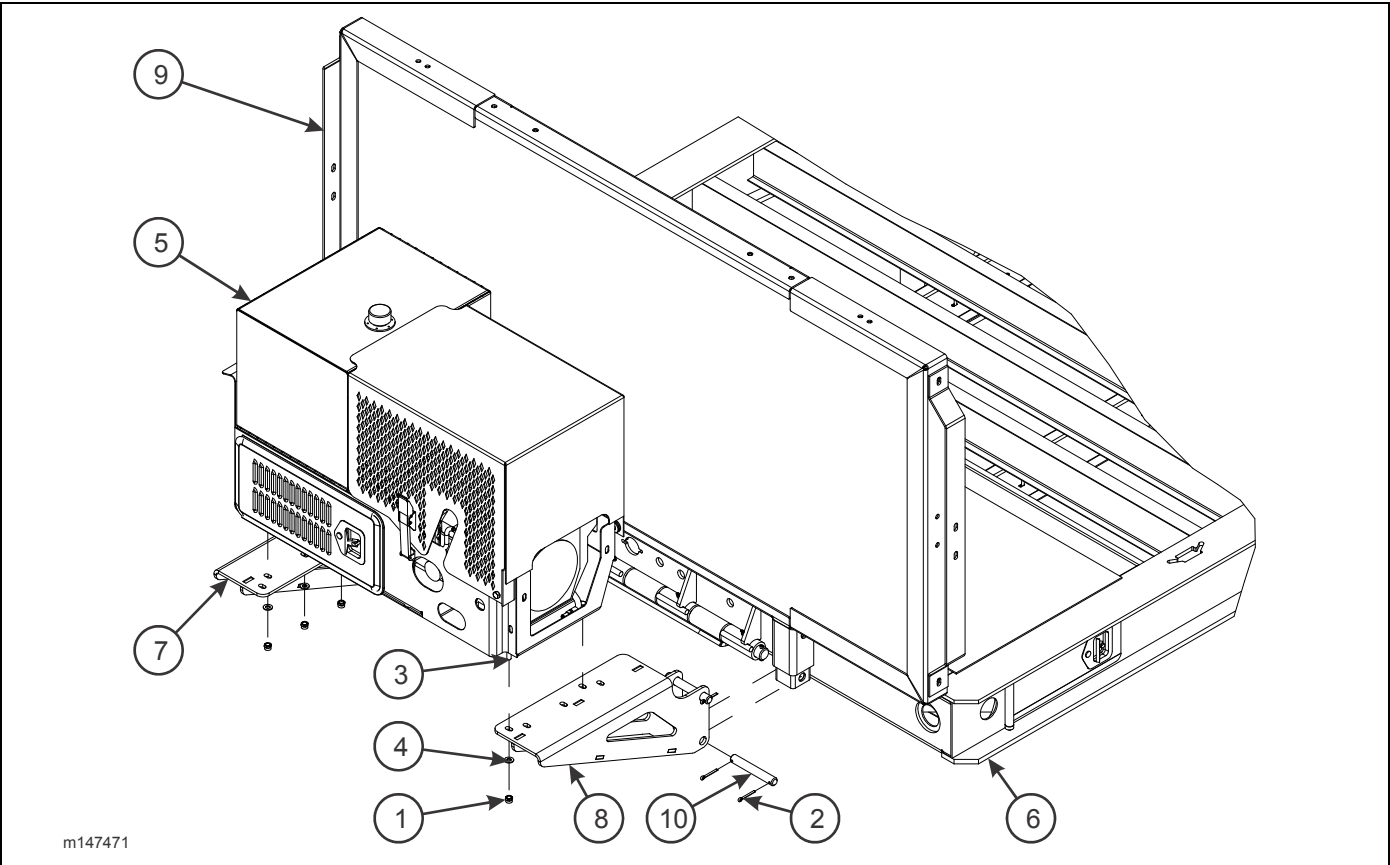
Figure 2-151: Front Extension Engine Package Mount Installation (Option)
