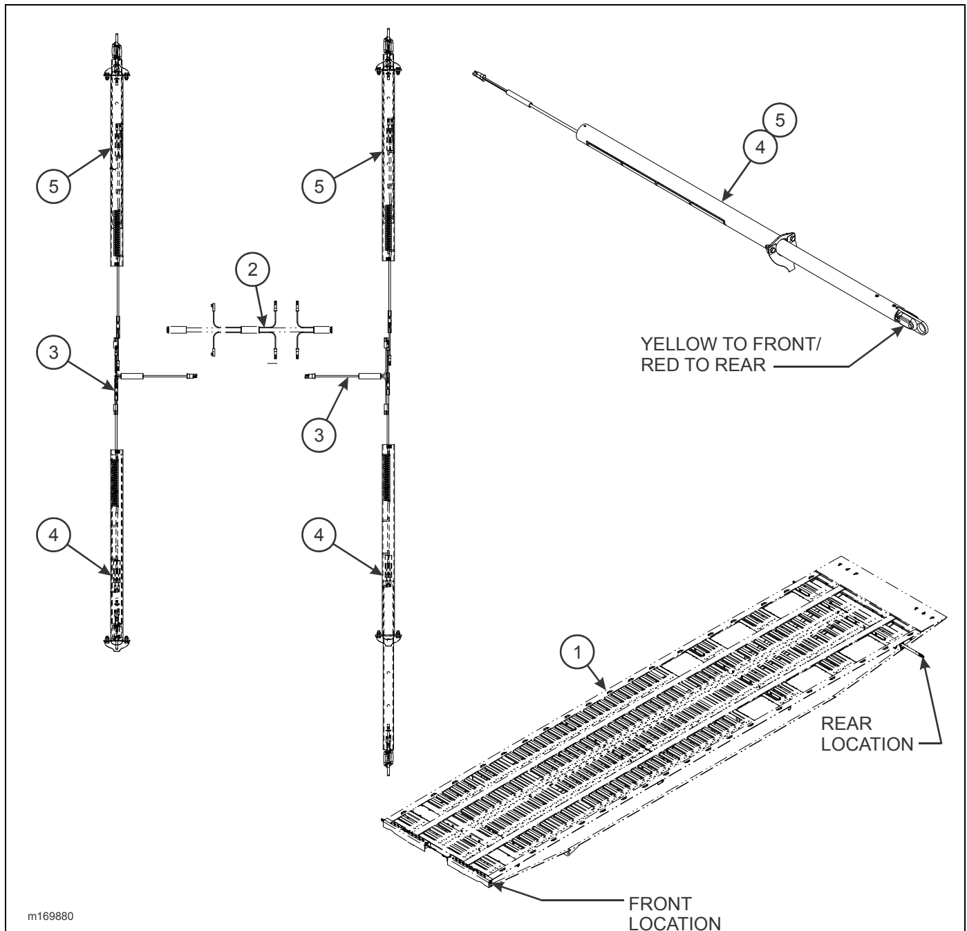
Figure 2-166: P/O Marker Light Installation (Option)
