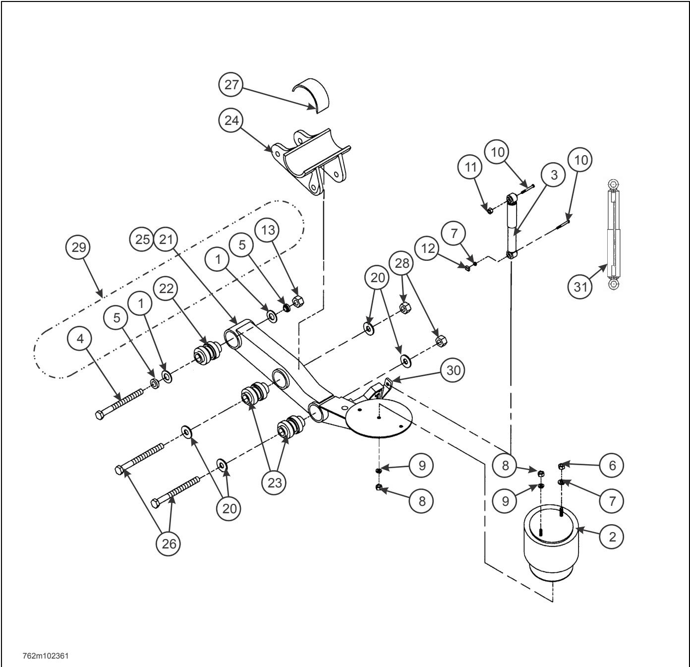
Figure 2-49: Suspension Hanger RLU-228
