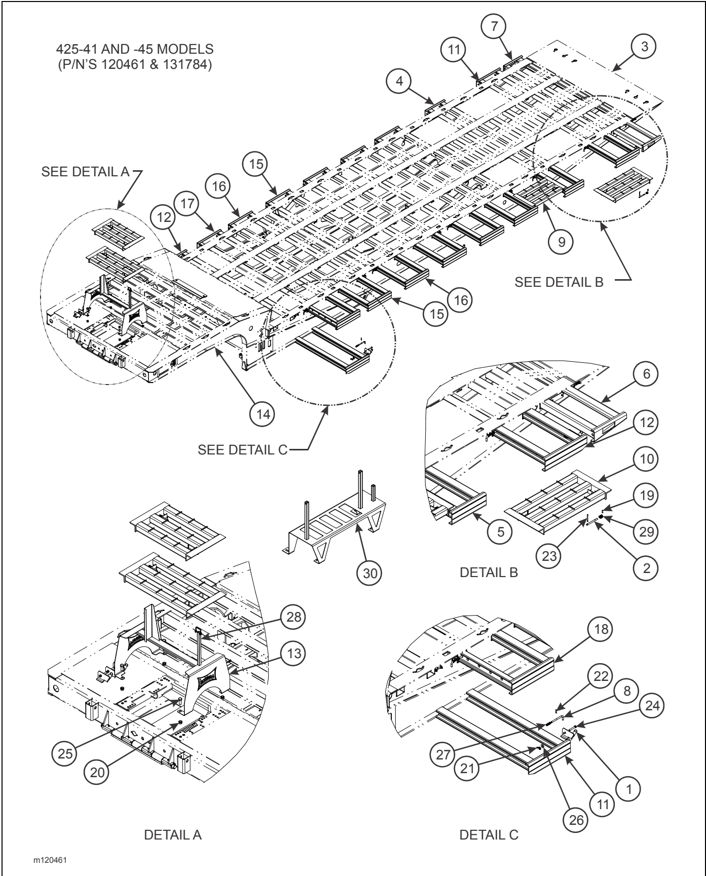
Figure 2-64: Pullout Installation (425)
