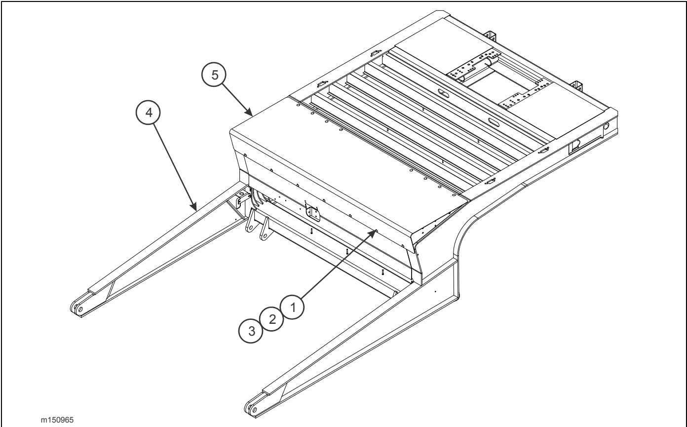
Figure 2-198: Slope Filler Deck Installation (Option)
