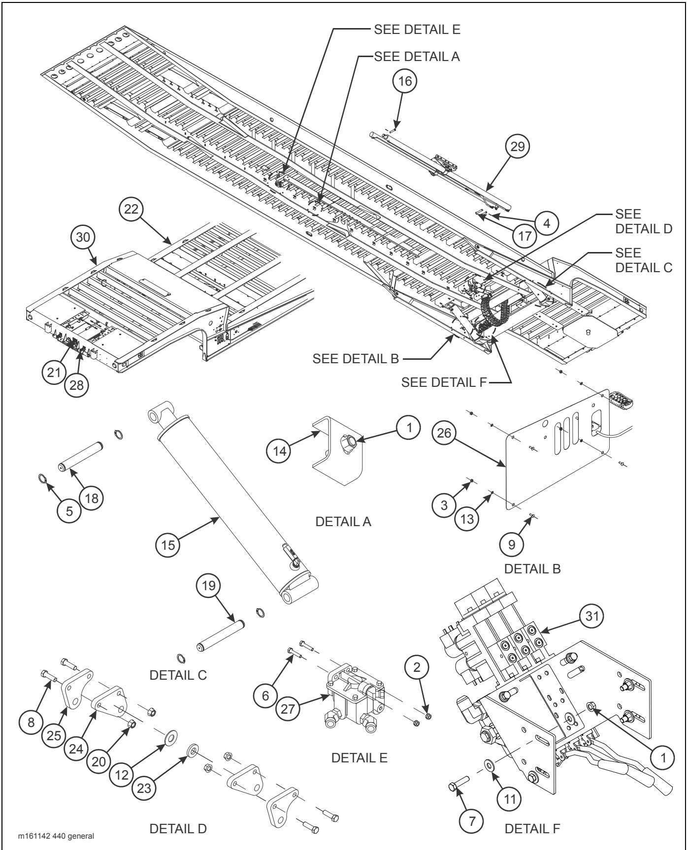
Figure 2-7: Hydraulic Electrical Air General Assembly (425 & 440)
