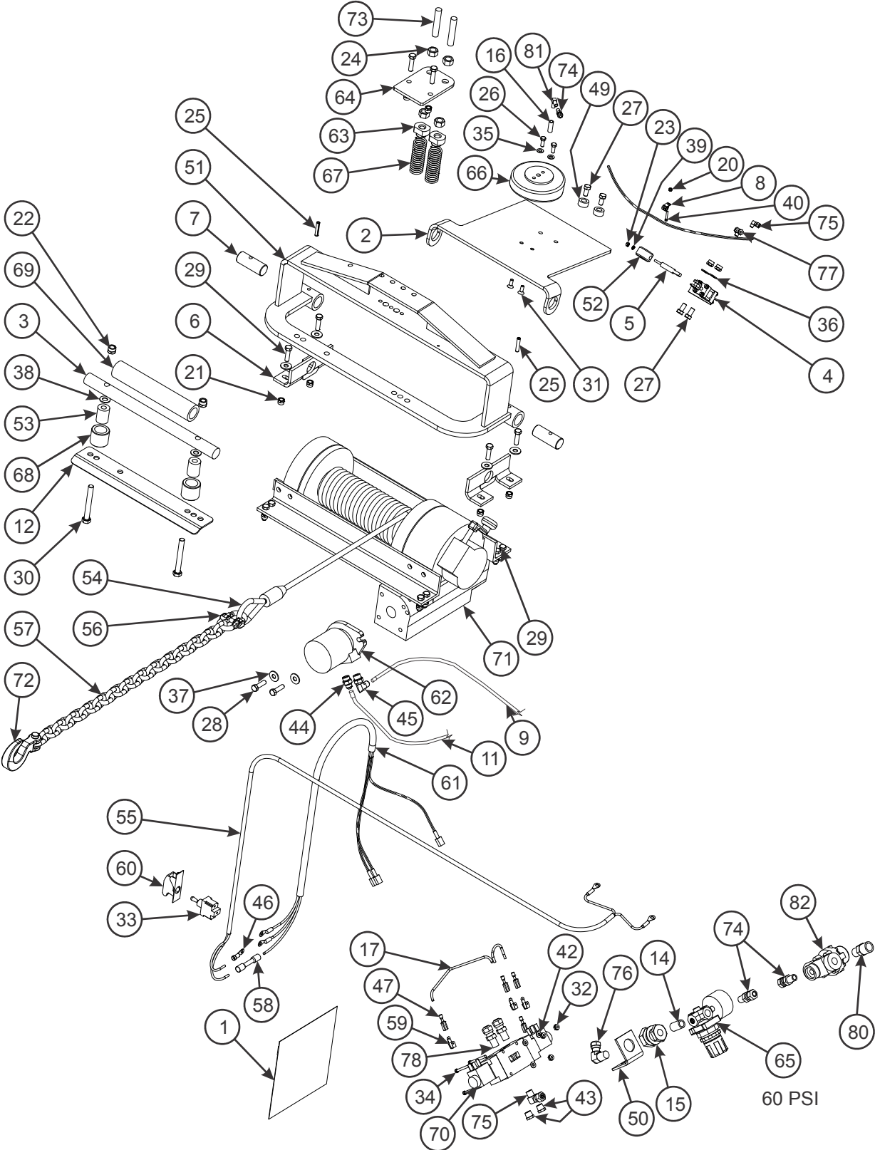
Figure 2-90: Winch Installation (1 of 2)
