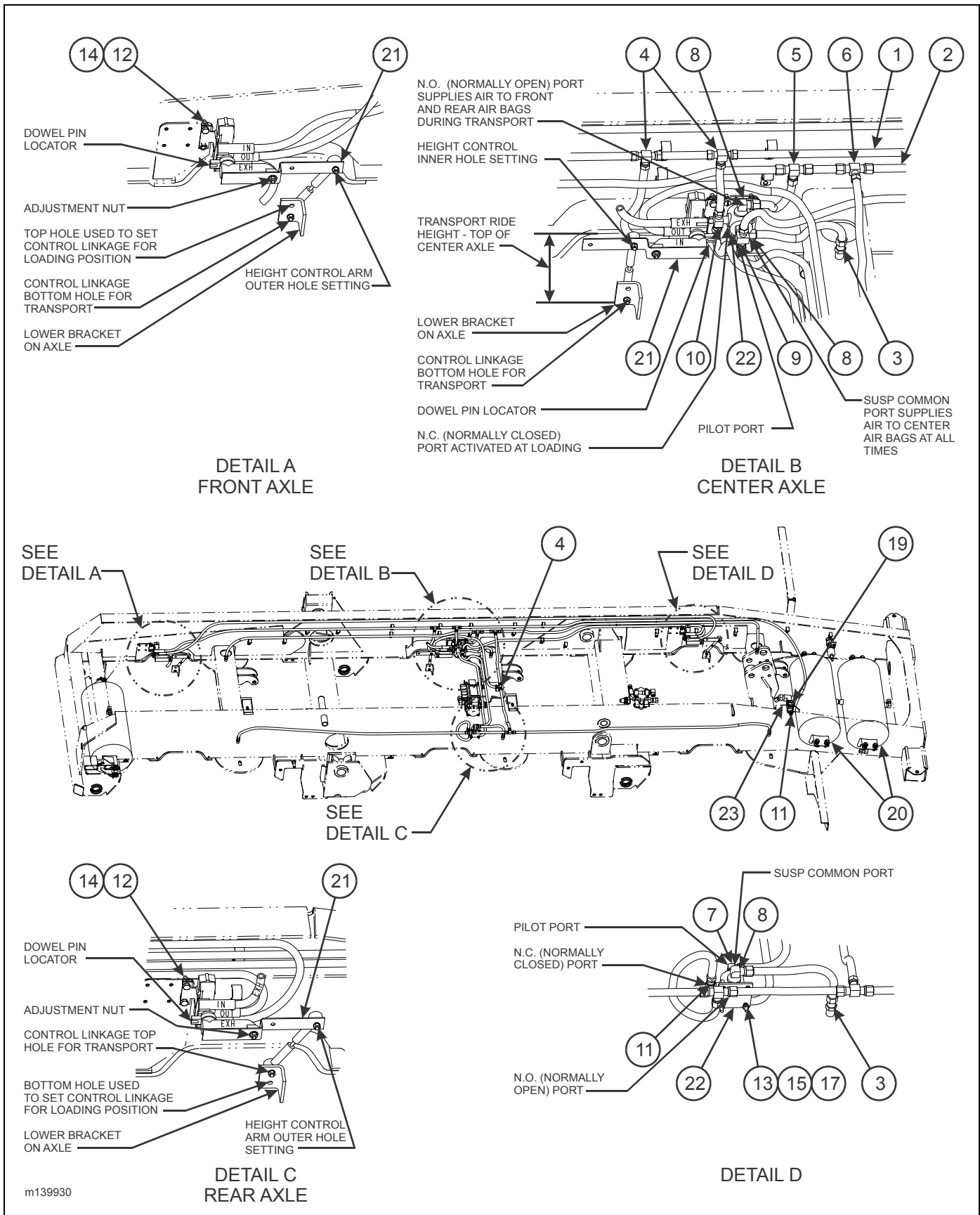
Figure 2-47: Air Ride Suspension, Air System Arctic (Triple)
