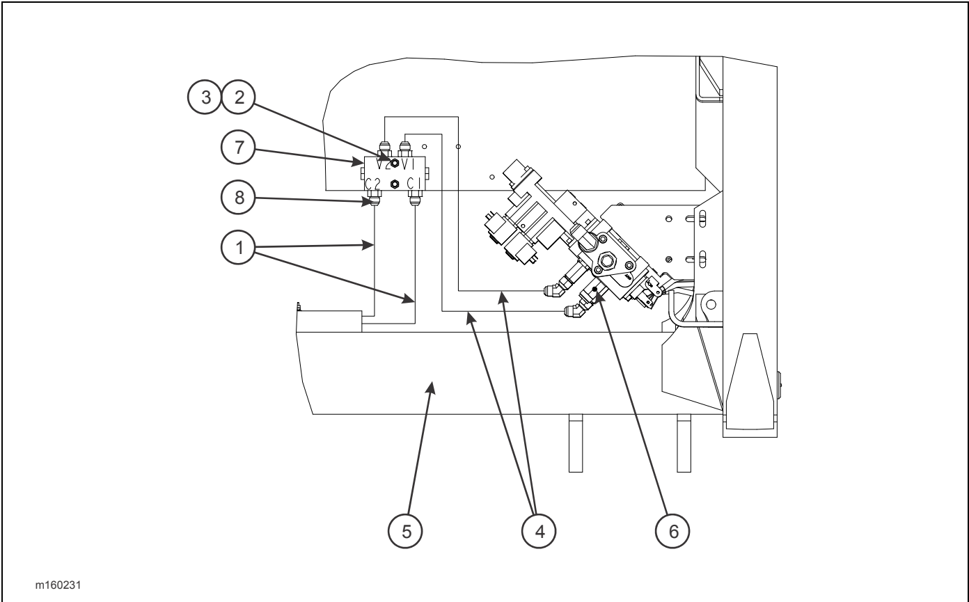
Figure 2-153: Tilt Check Valve Installation
