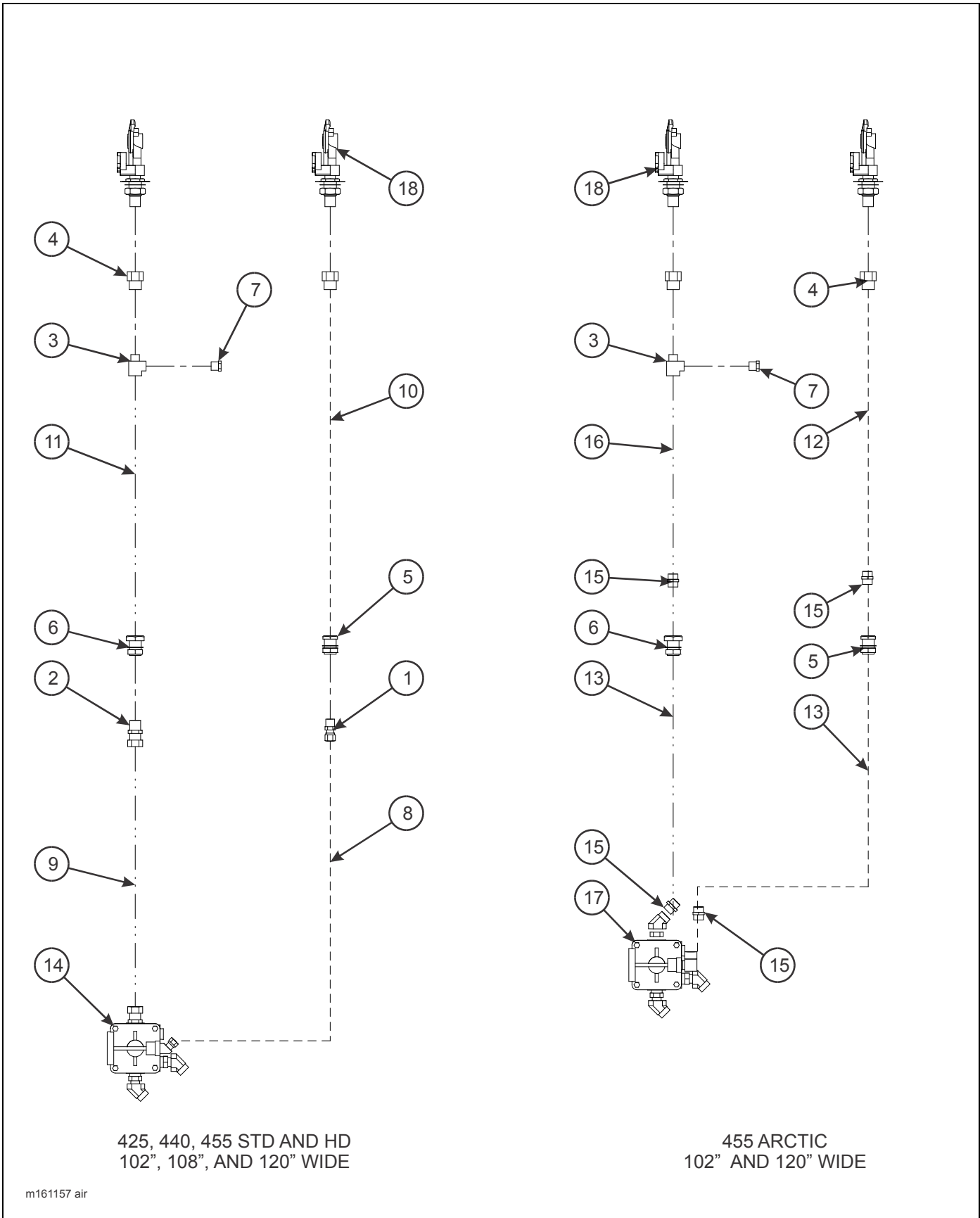
Figure 2-26: Air System, ABS
