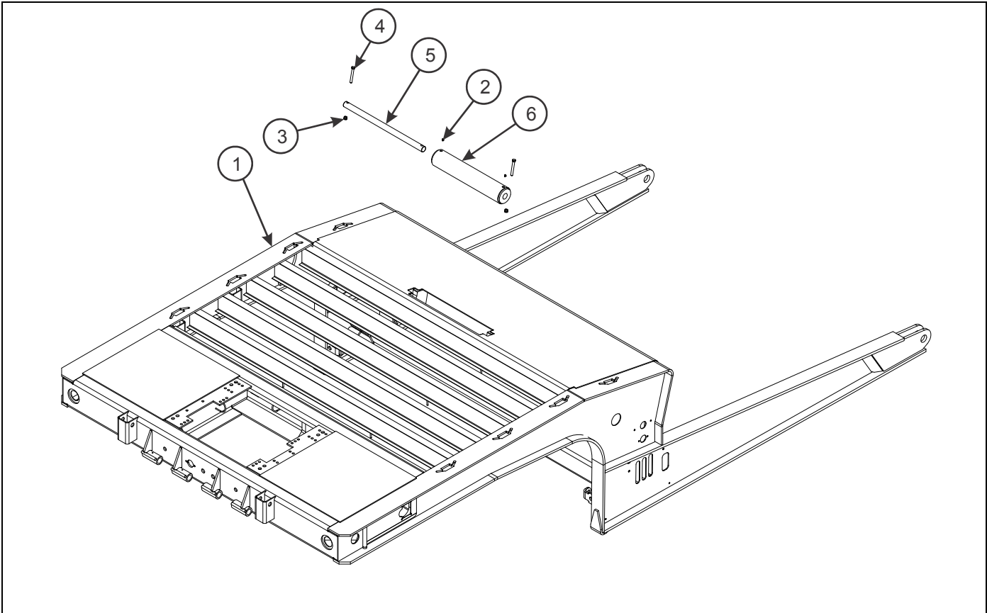
Figure 2-183: Upper Deck Extension Bridge Storage Rack (Option)
