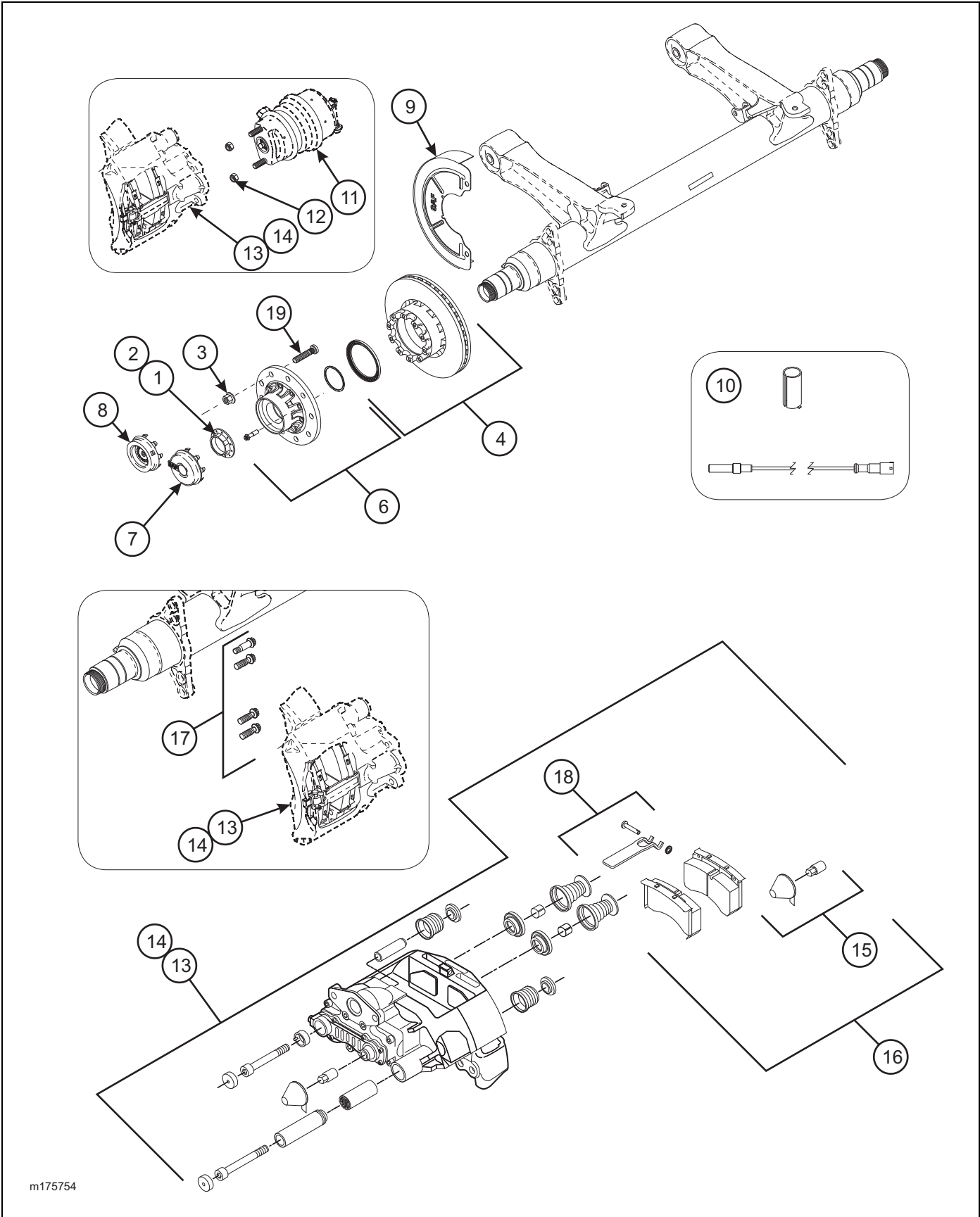
Figure 2-58: Disc Spring Brake Axle Items
