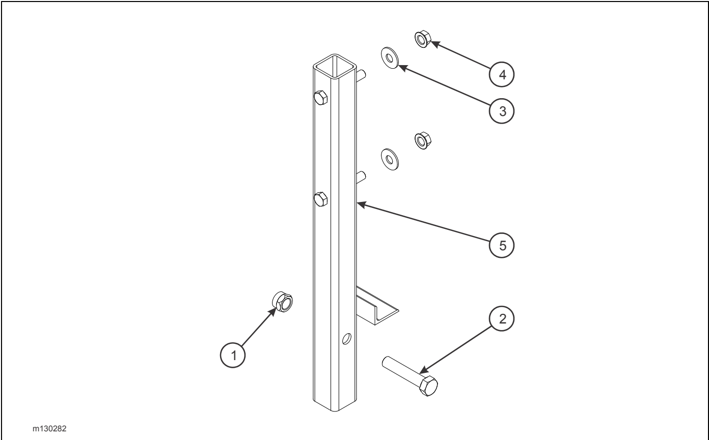
Figure 2-194: Spare Tire Mount Assembly
