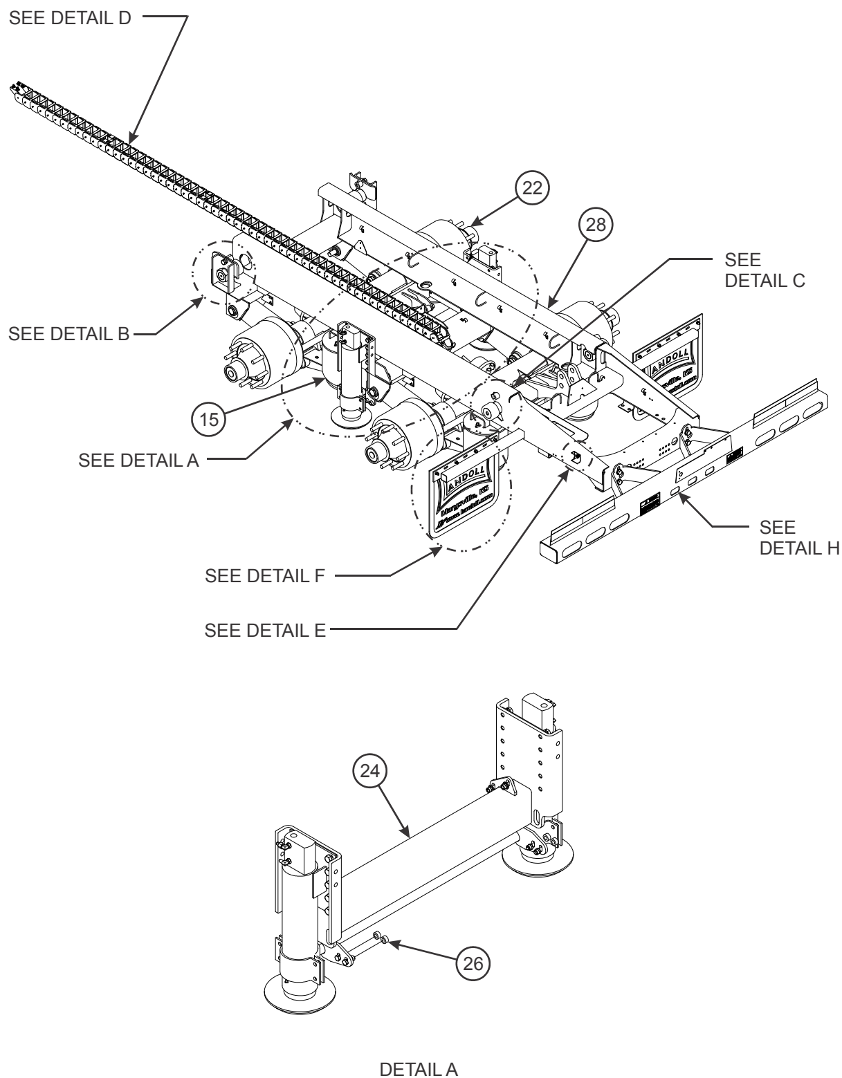
Figure 2-29: Suspension Assembly, General Items (425 & 440) (1 of 2)
