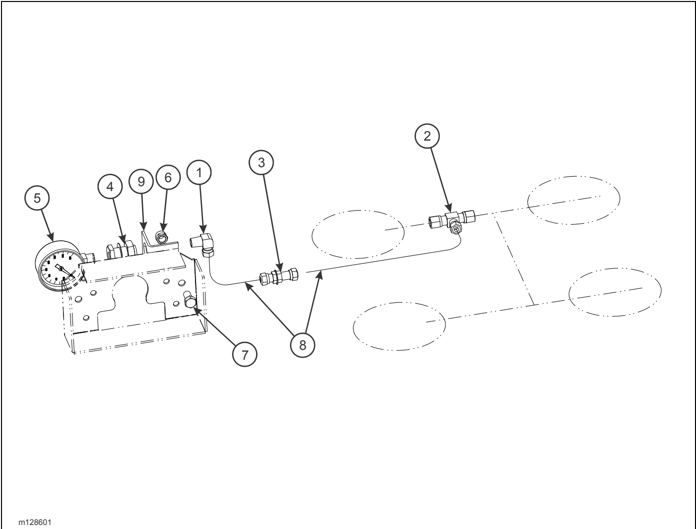
Figure 2-185: Pressure Gauge Installation (Option)
