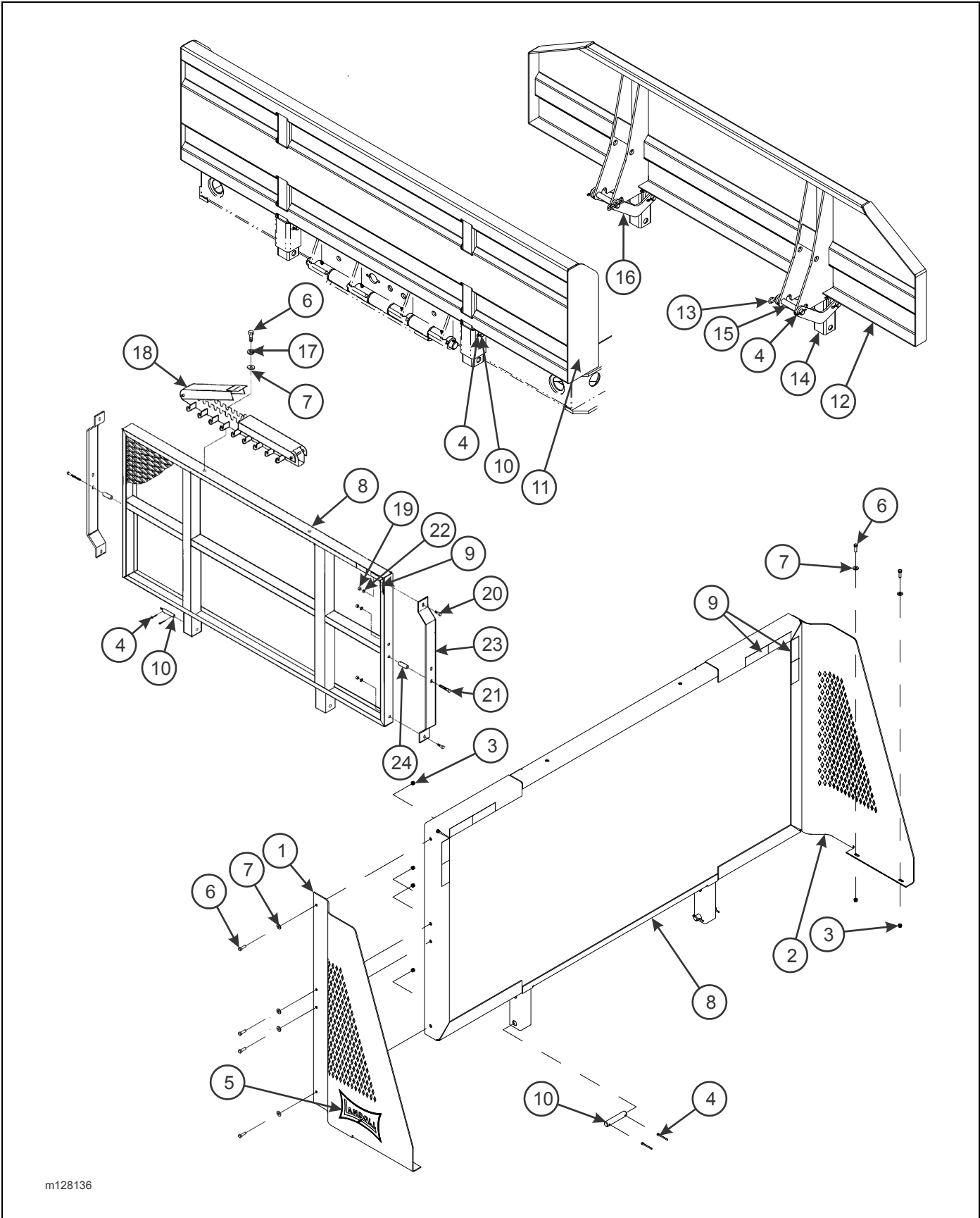
Figure 2-60: Bulkhead Assembly
