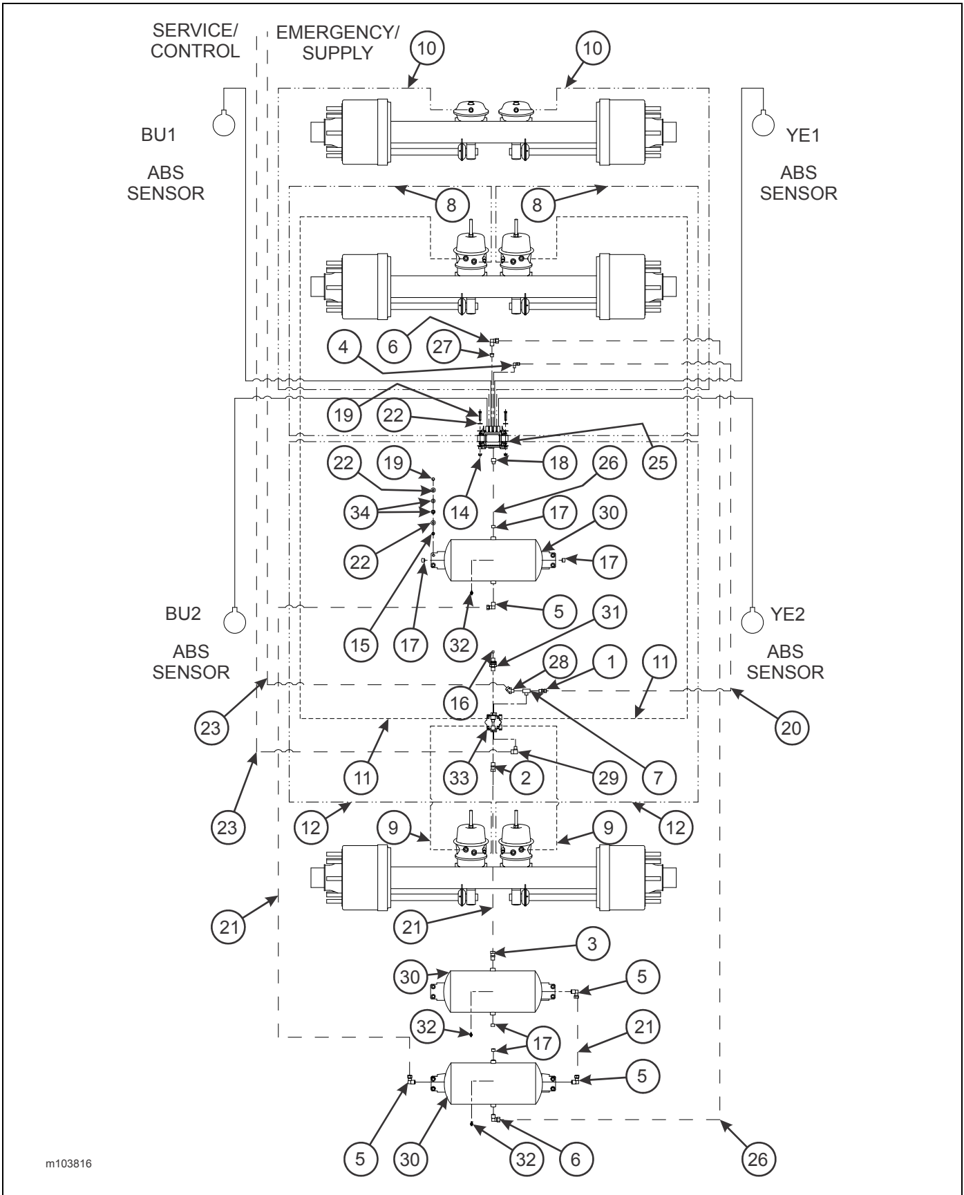
Figure 2-42: Spring Air Brake System w/ ABS (455)
