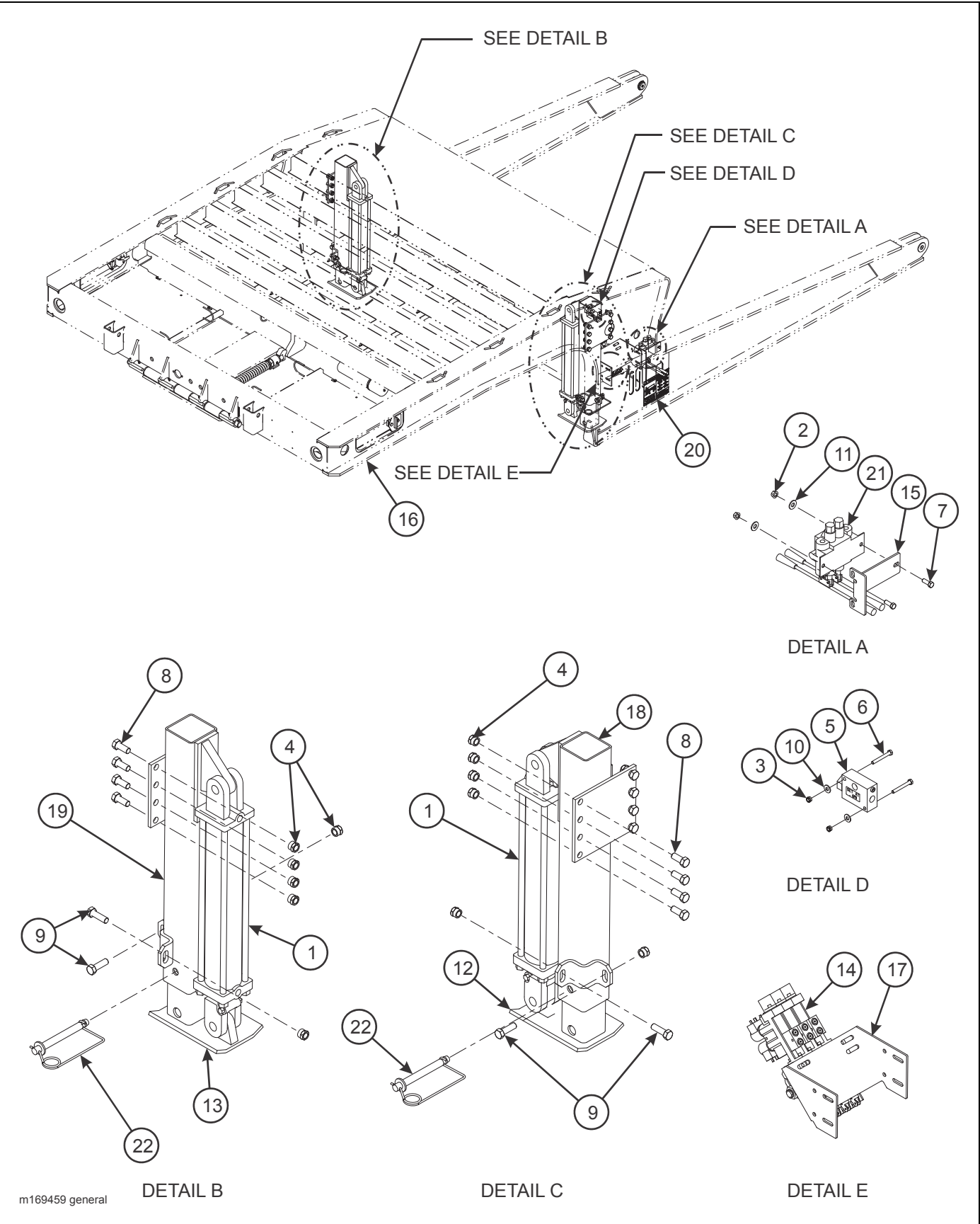
Figure 2-137: Hydraulic Park Stand Installation, General Items
