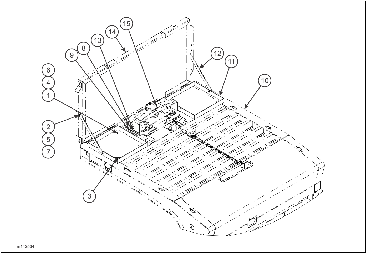
Figure 2-192: Chain Tray Assembly (Option)
