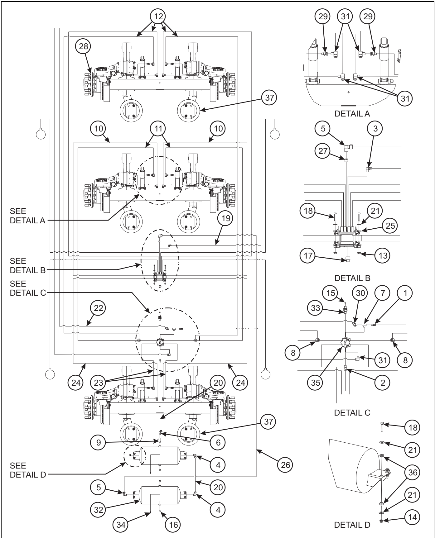
Figure 2-57: Air System, U/C ABS Disk Brake
