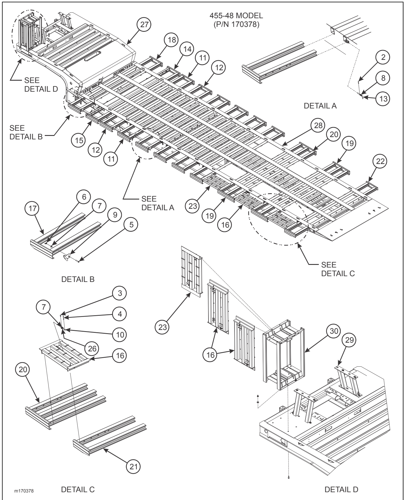
Figure 2-69: Pullout Installation (455) (2 of 3)
