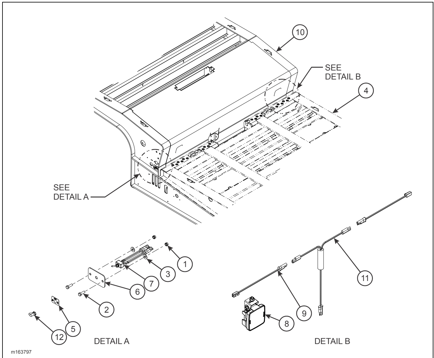
Figure 2-162: U/D Slope Light Installation (Option)
