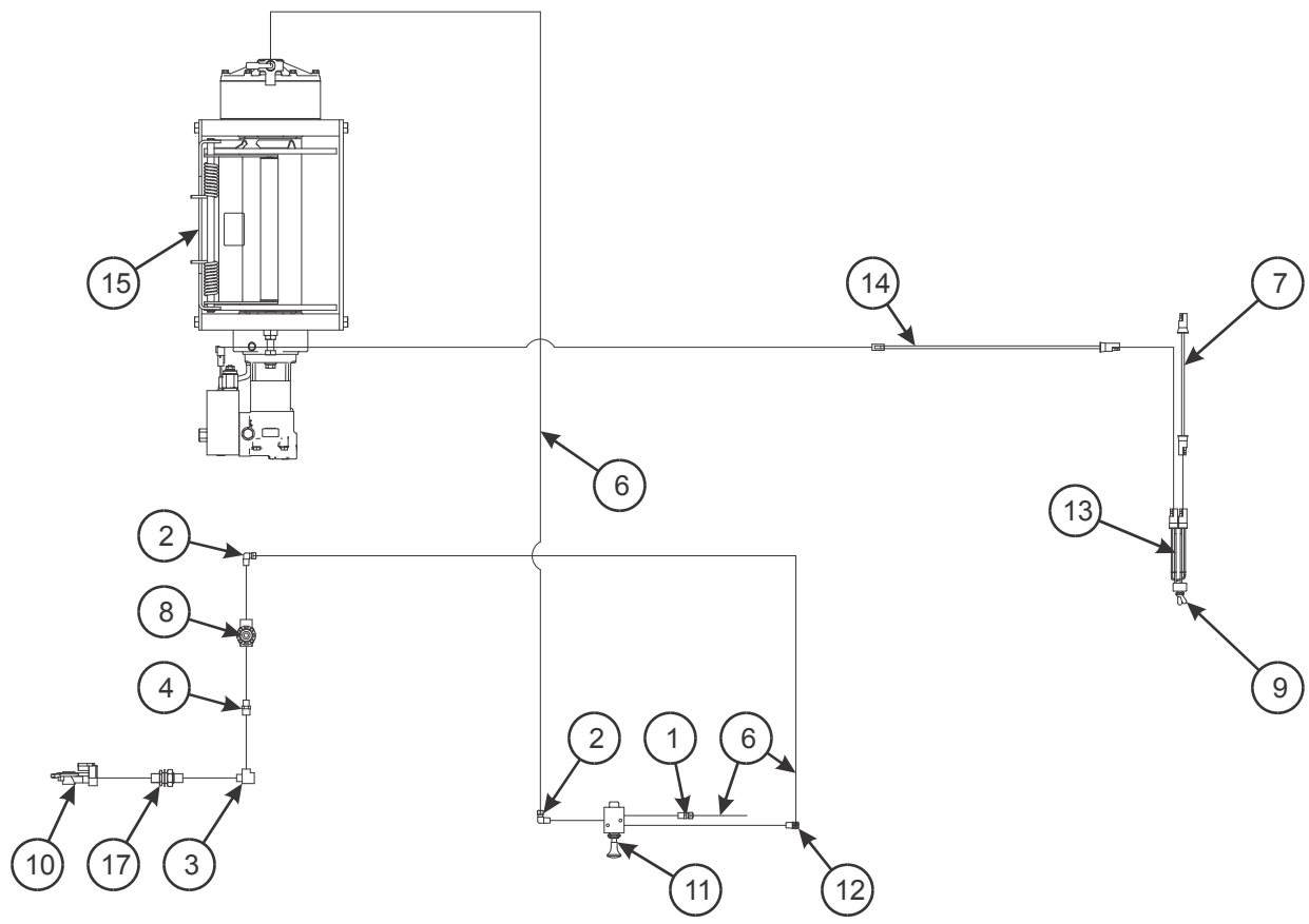
AIR SCHEMATIC
