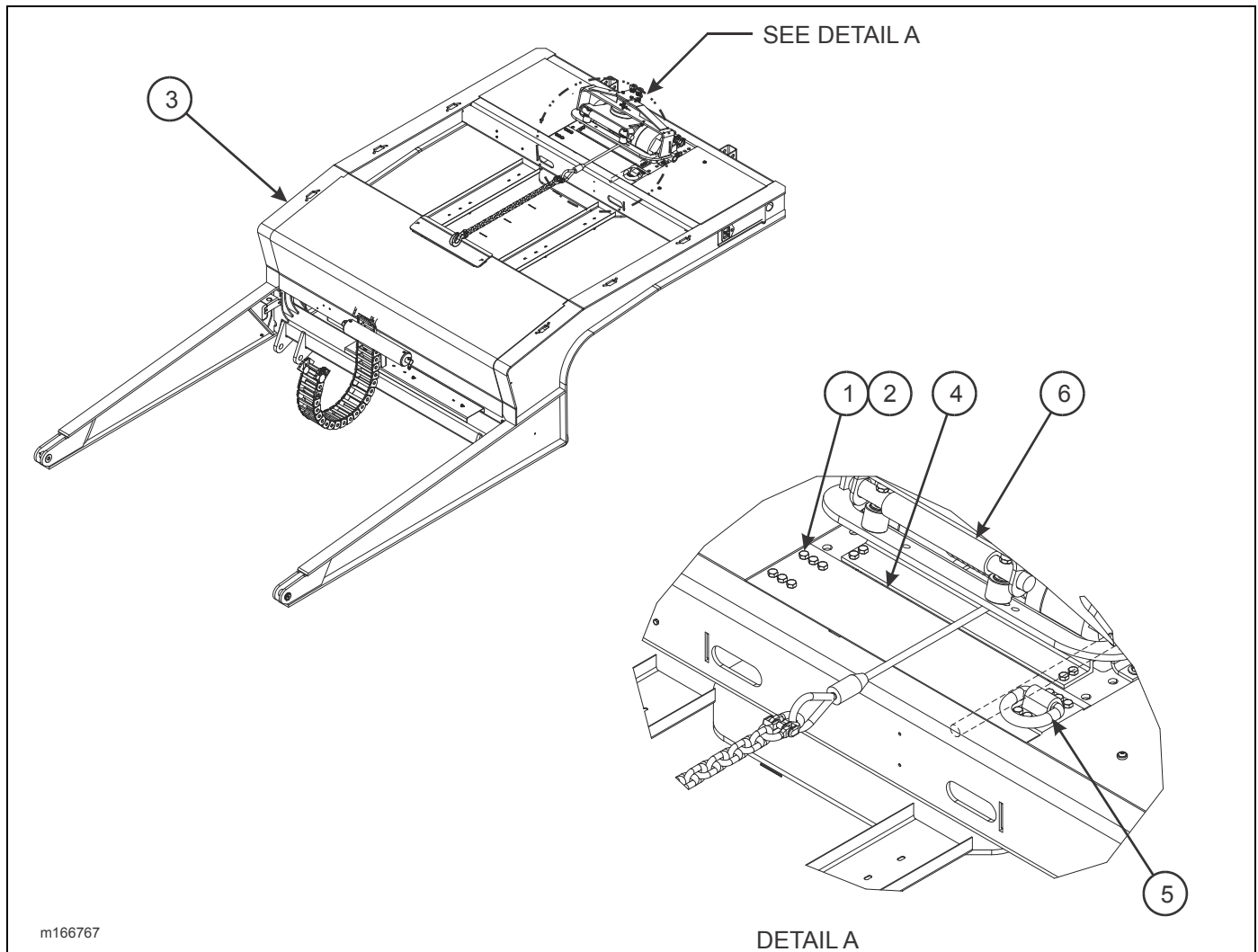
Figure 2-110: Winch Trim Plate Installation (Option)
