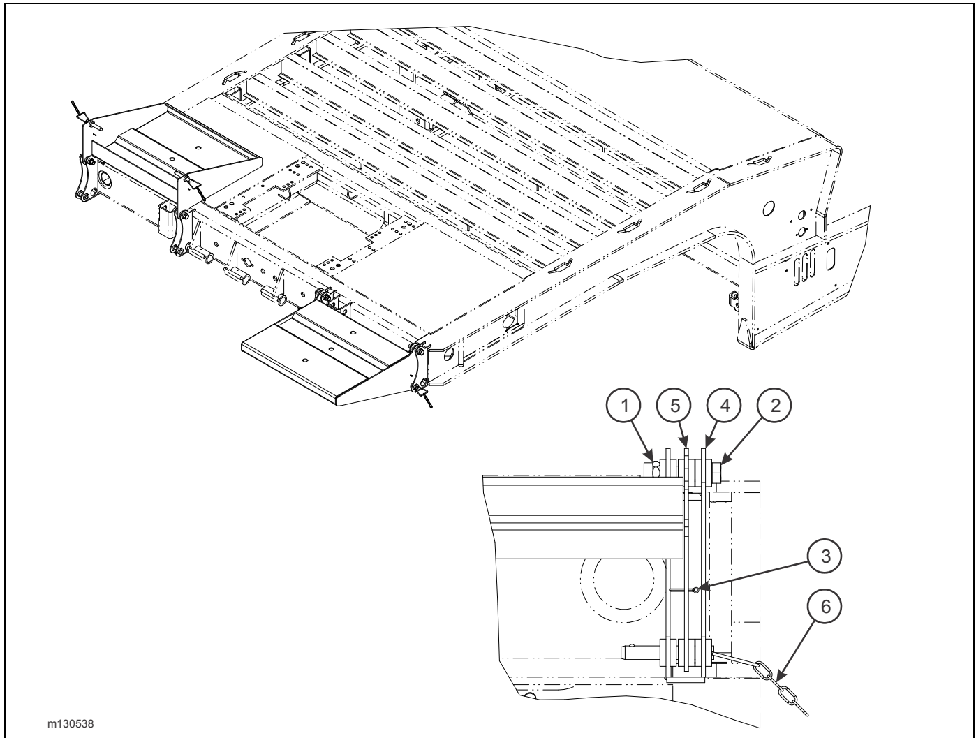
Figure 2-197: Front Flip Extension (Option)
