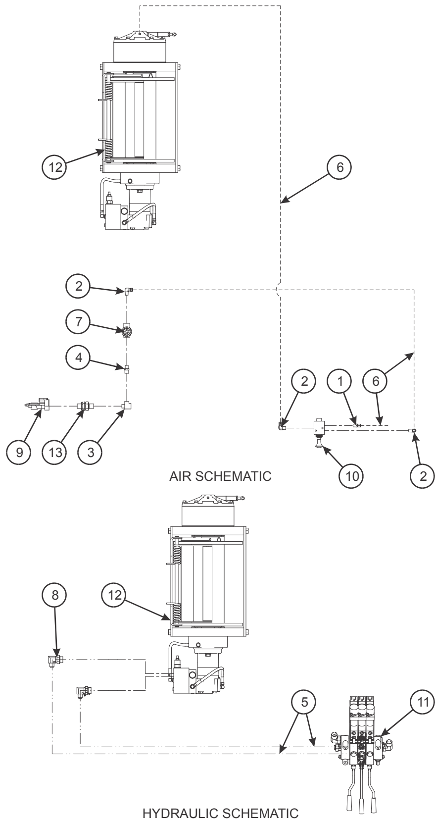
Figure 2-74: 20K Winch Installation, Hydraulic/Air Items (Warn)
