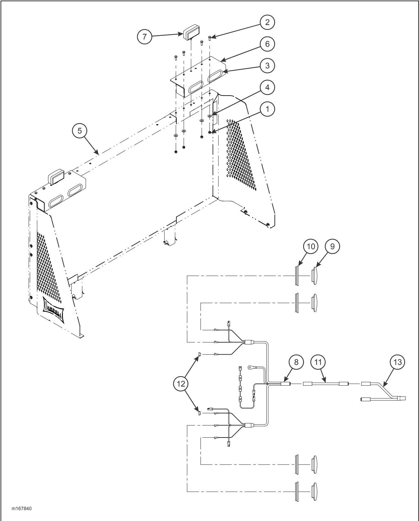
Figure 2-63: Bulkhead Stop/Tail/Turn Light Assembly
