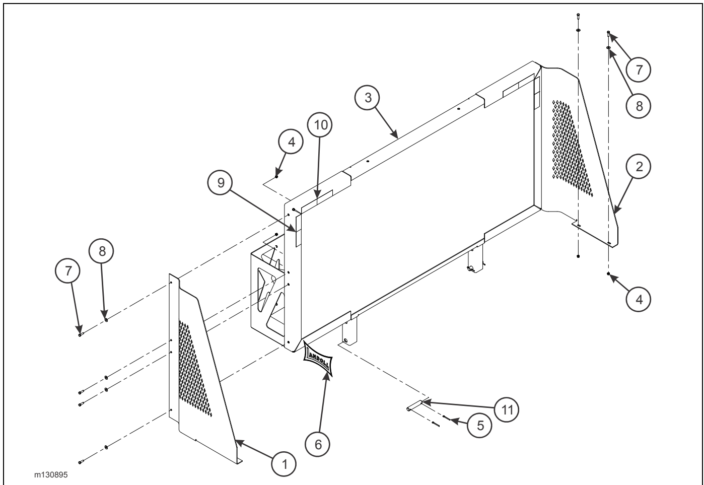
Figure 2-190: Special Bulkhead Installation (Option)
