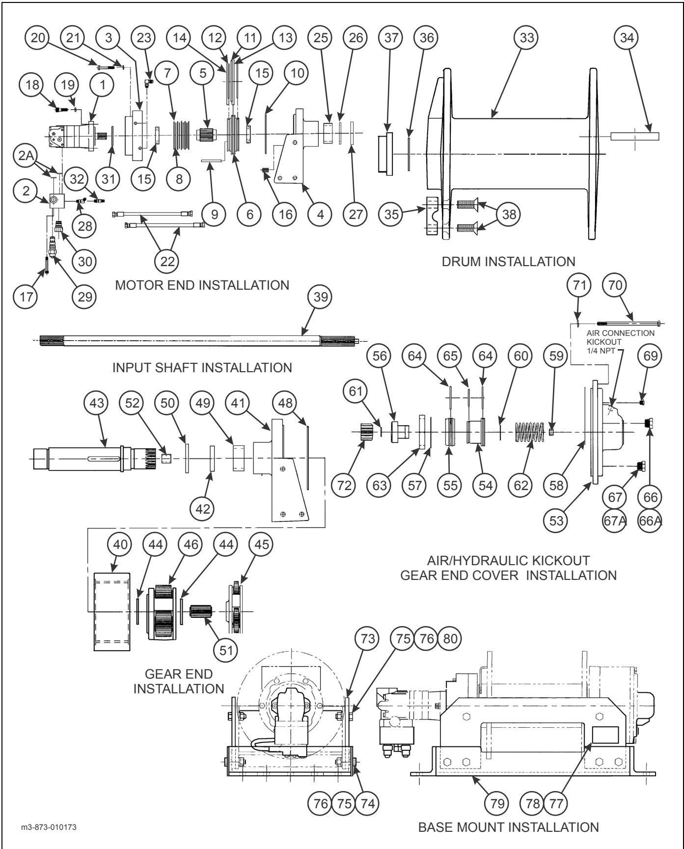
Figure 2-102: 30,000 Lb. Winch Items
