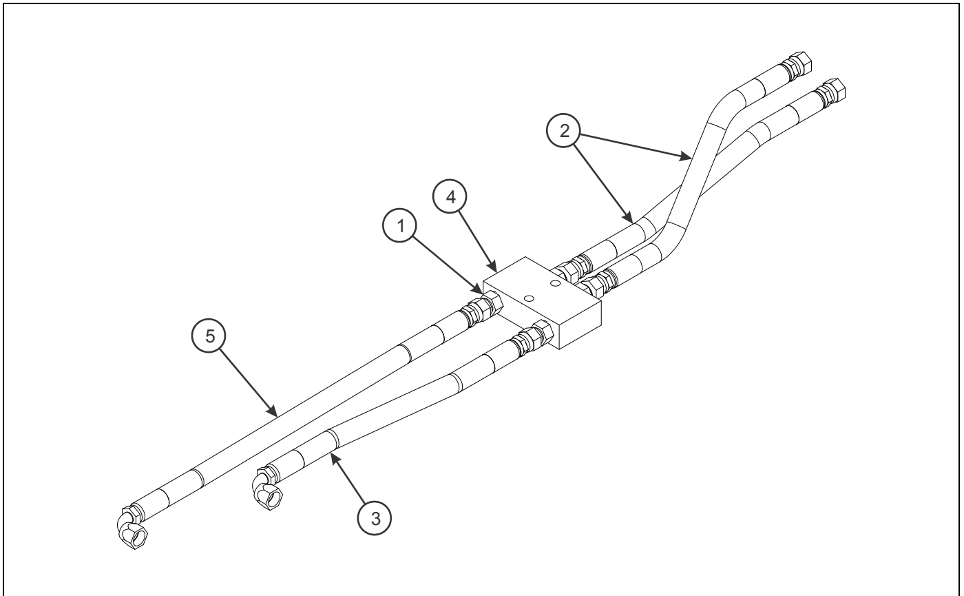
Figure 2-154: Tilt Cylinder Check Valve Installation (Option)
