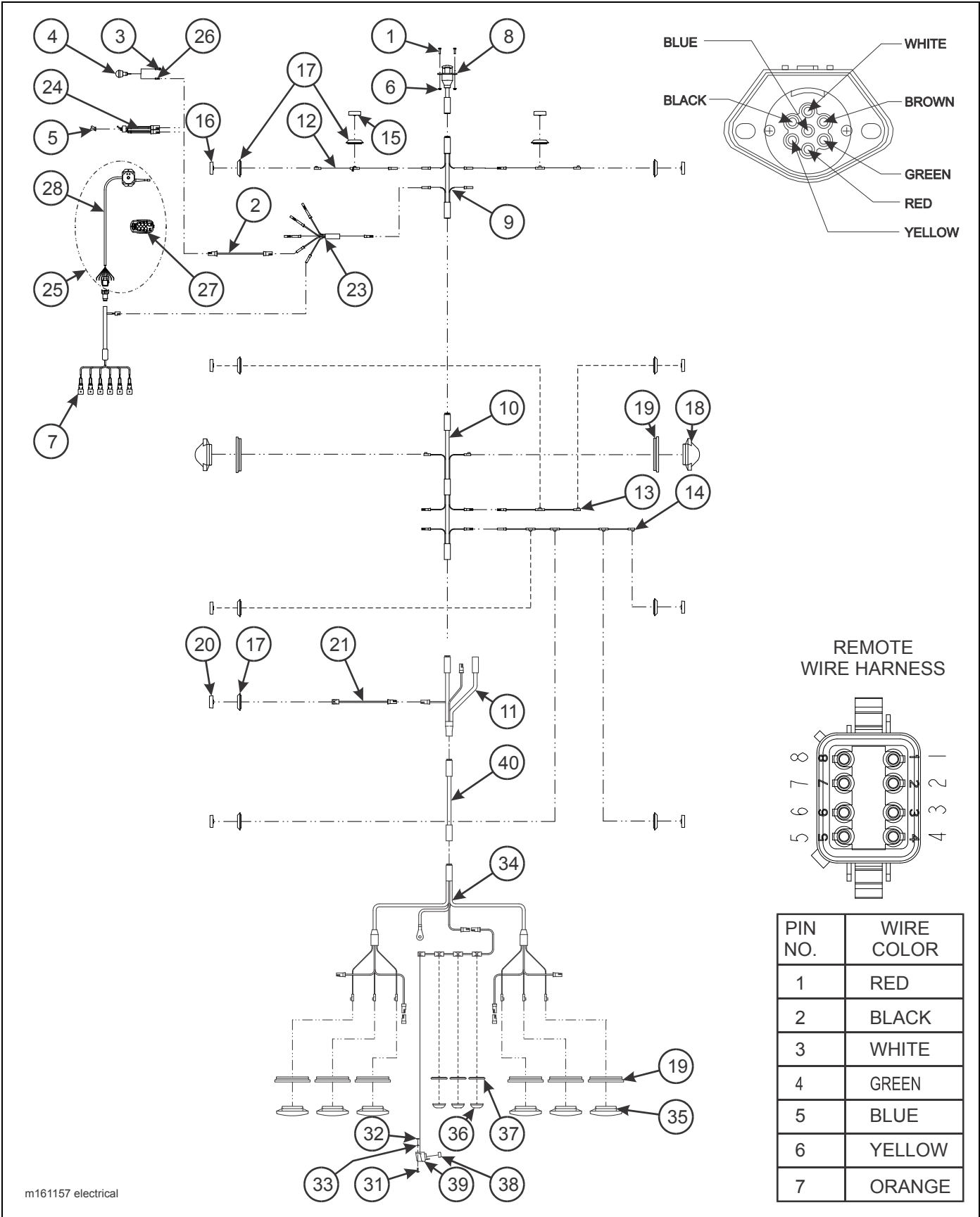
Figure 2-25: Electrical System
