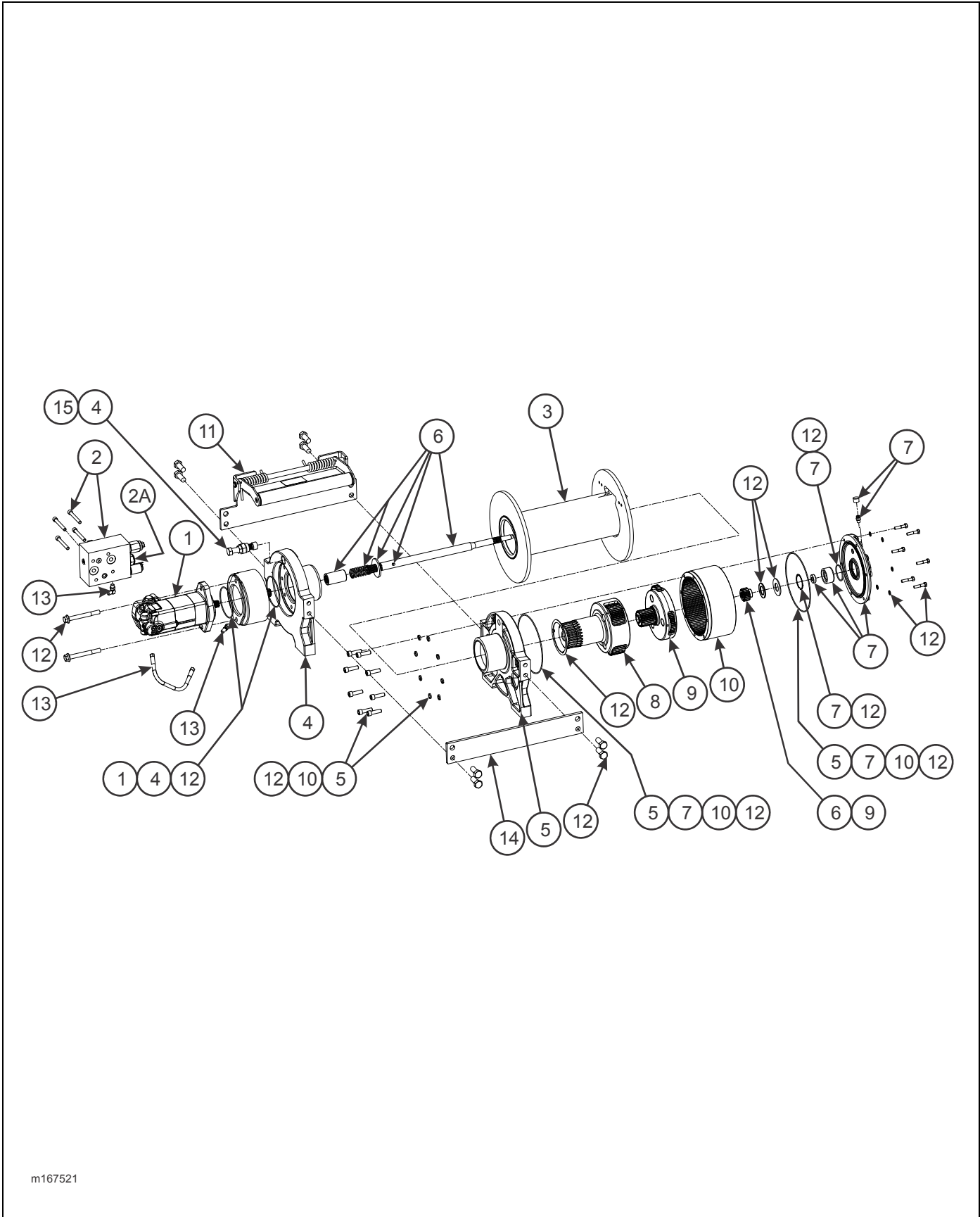
Figure 2-78: 20K Winch Items (Warn)
