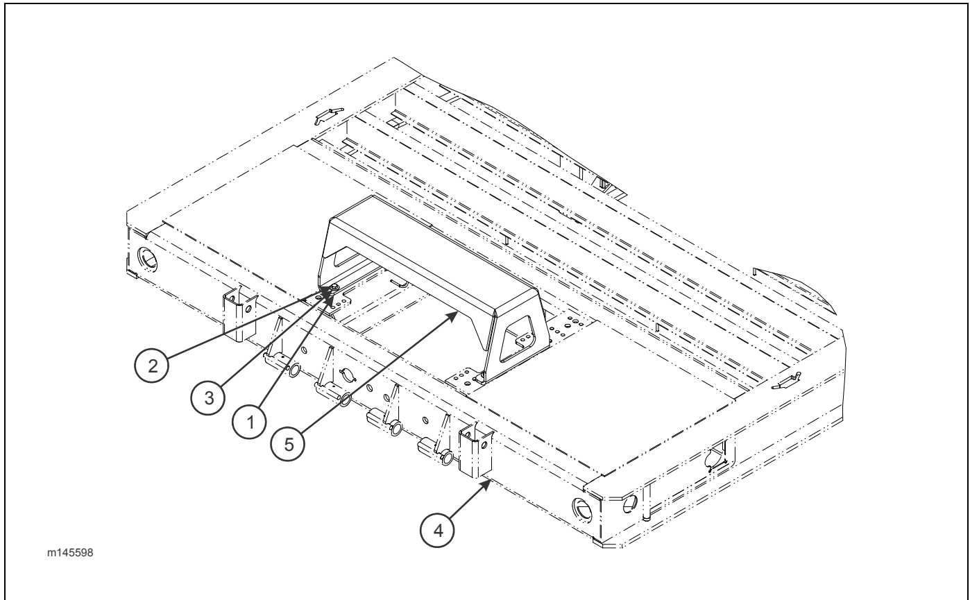
Figure 2-178: Special Bulkhead Installation (Option)
