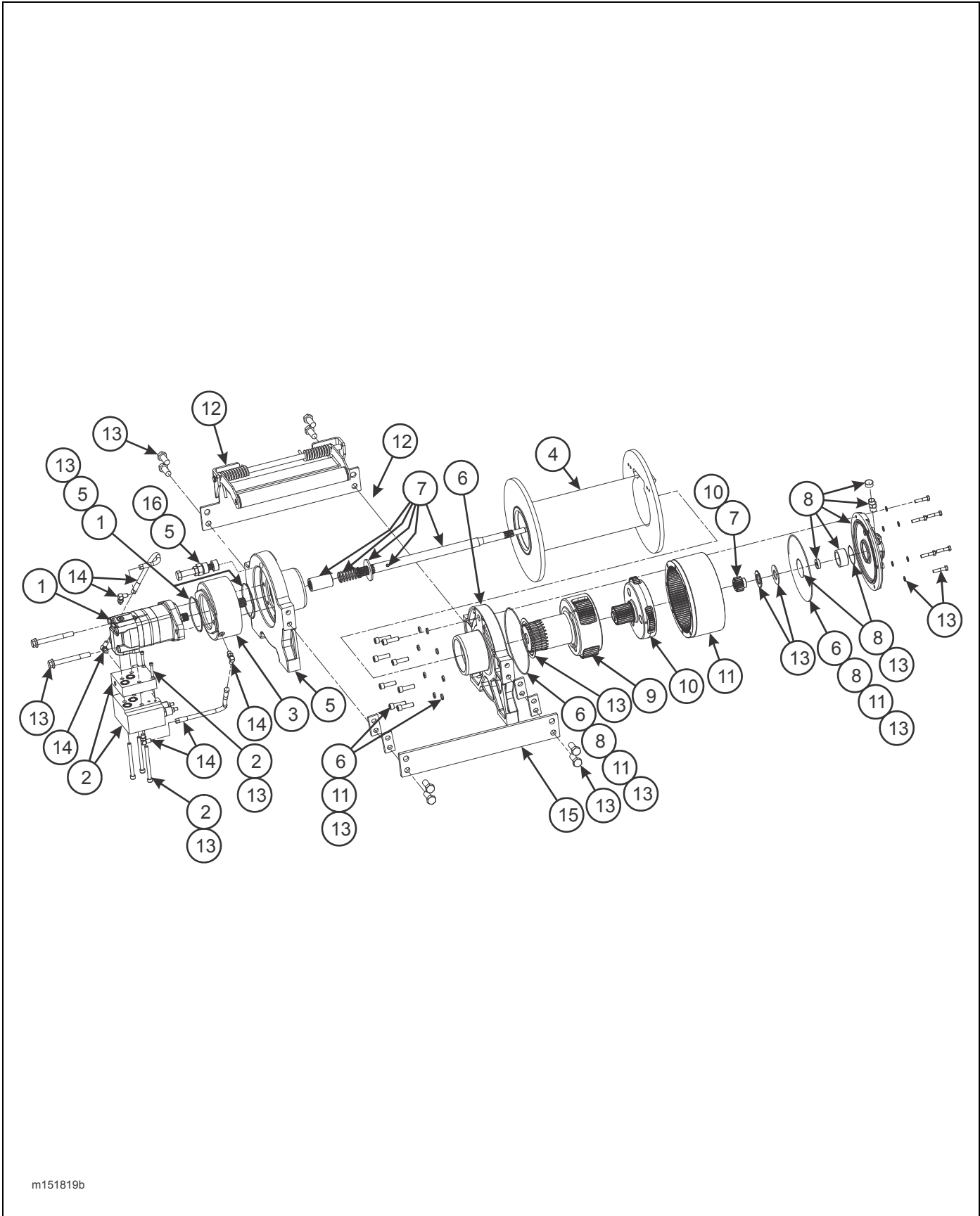
Figure 2-75: 20K Winch Items (Warn)
