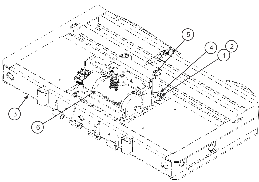
Figure 2-115: 4 Roller Guide Installation (Option)
