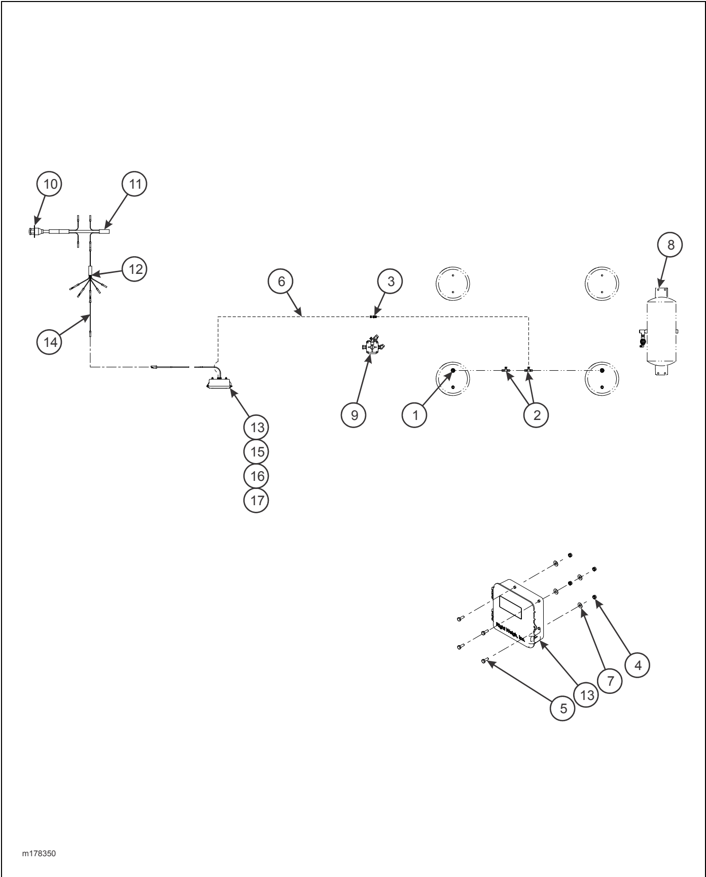
Figure 2-182: Air Digital Scale, Right Weigh System (Option)
