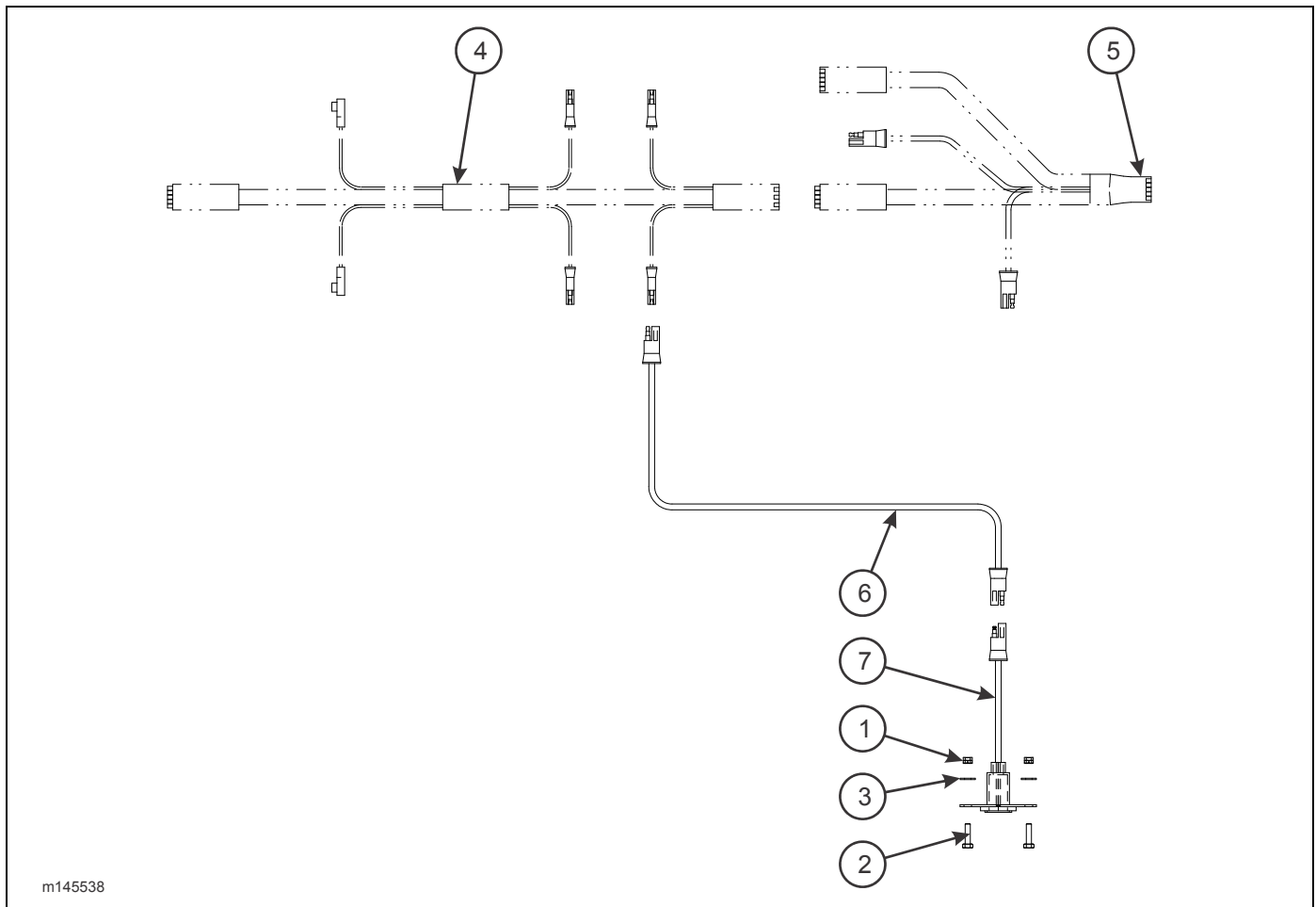
Figure 2-156: Rear Side Electrical Outlet Installation (Option)
