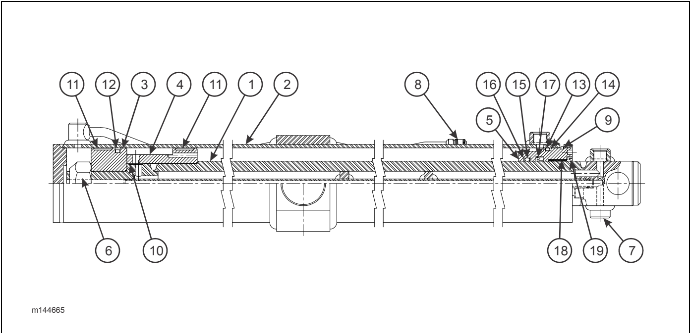
Figure 2-17: Cylinder, Hydraulic 4 x 126 Ported Rod (Streetside) (455-50/53/55HD, 440-48/50CA)
