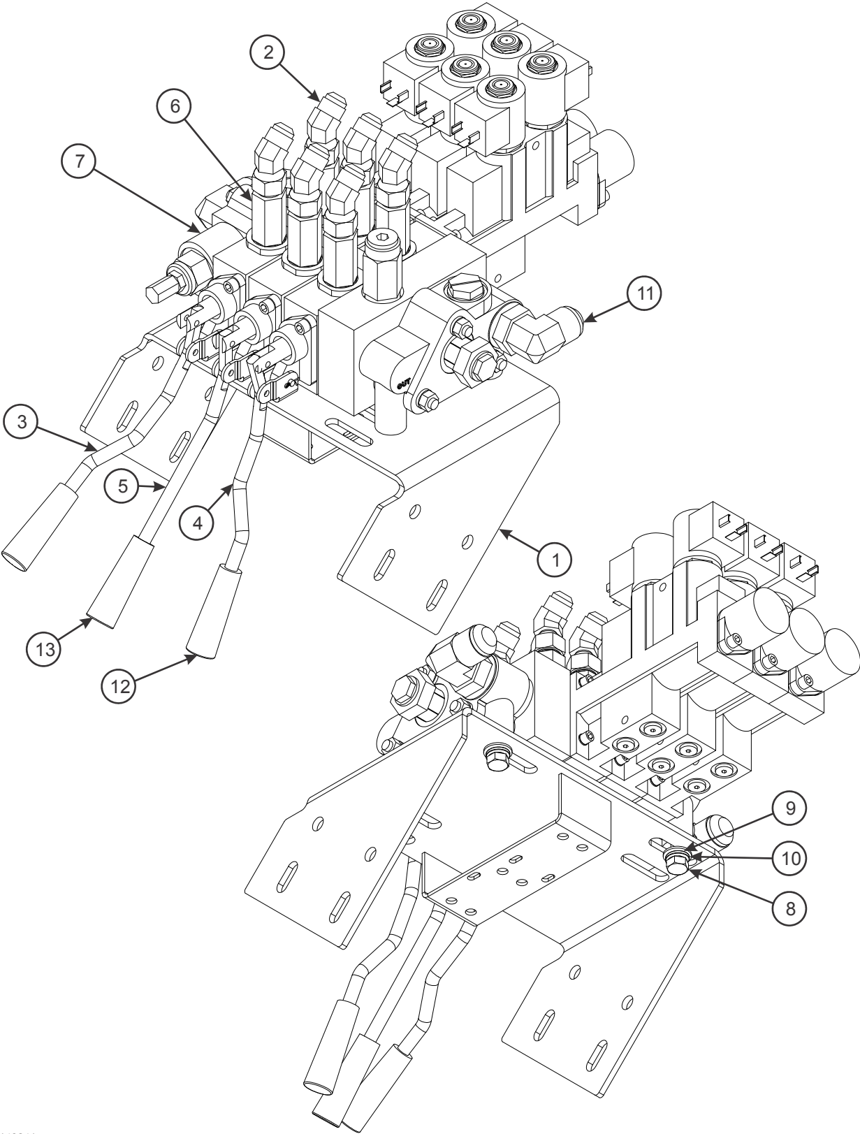
Figure 2-12: Three Spool Valve Assembly
