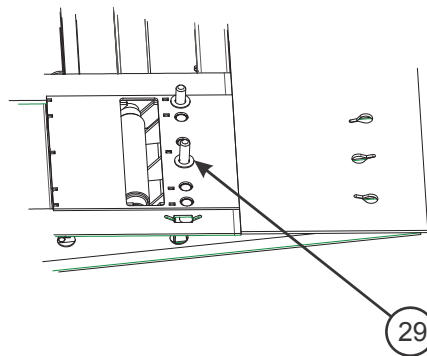
DETAIL D
