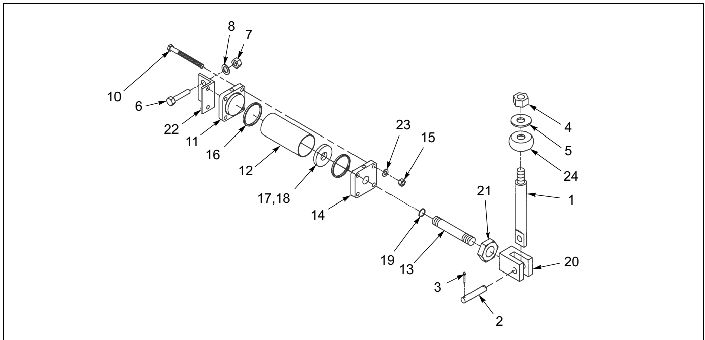
Figure 1-56: Winch - Air Shift Cylinder
