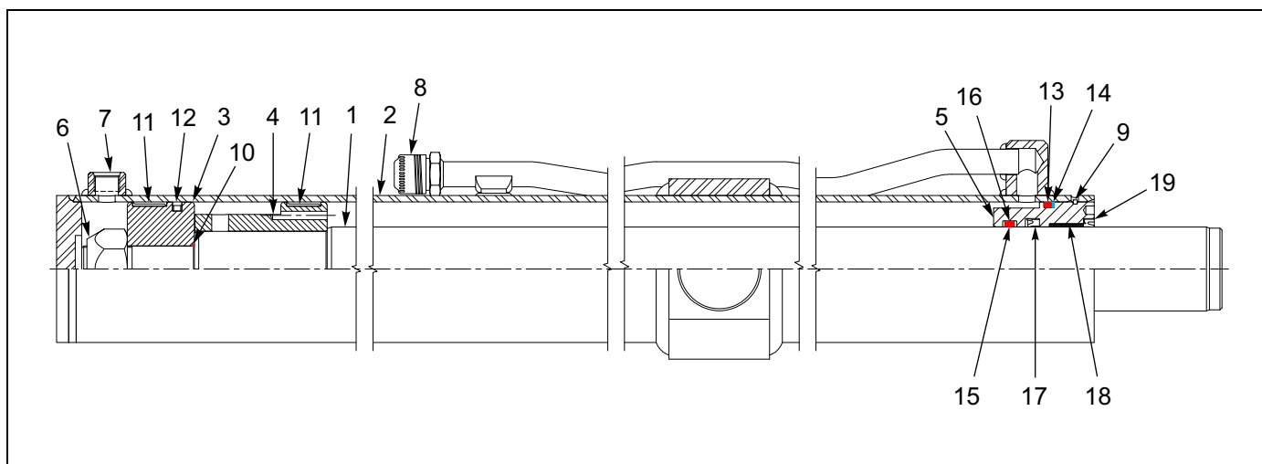
Figure 1-12: Cylinder Assembly - Hi Flow
