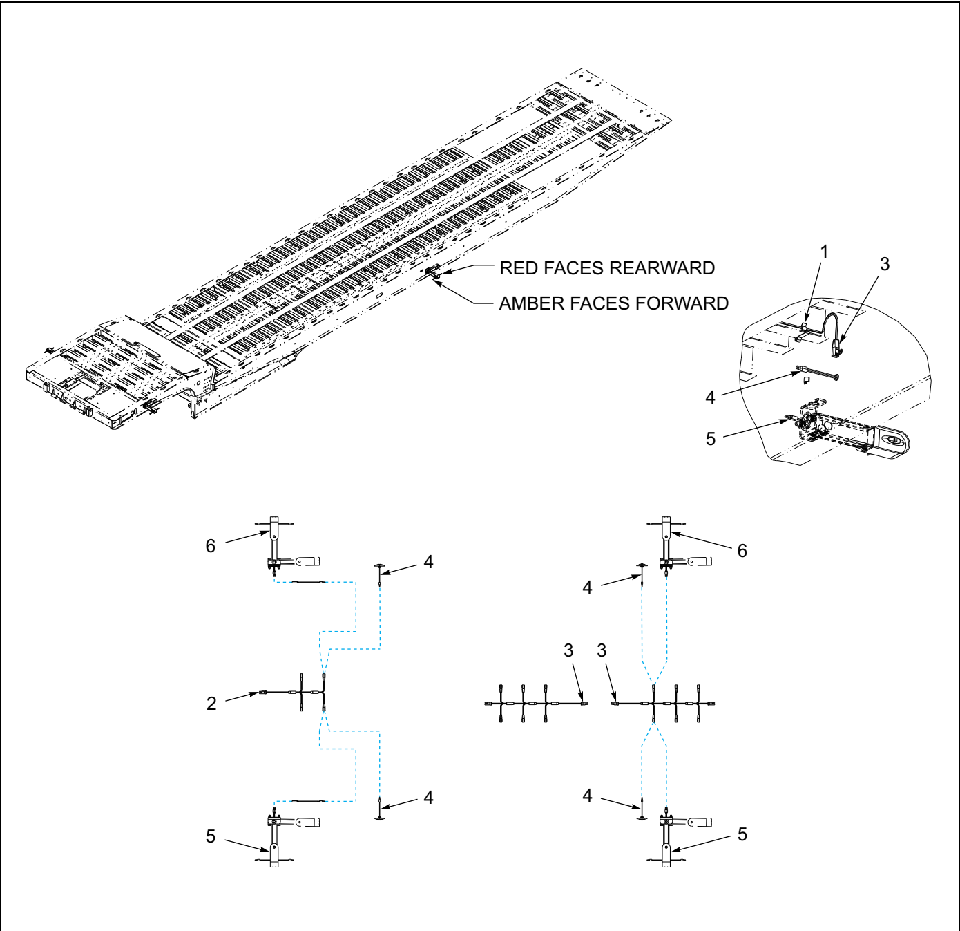
Figure 1-107: Swingout Marker Light Installation - Red/Amber
