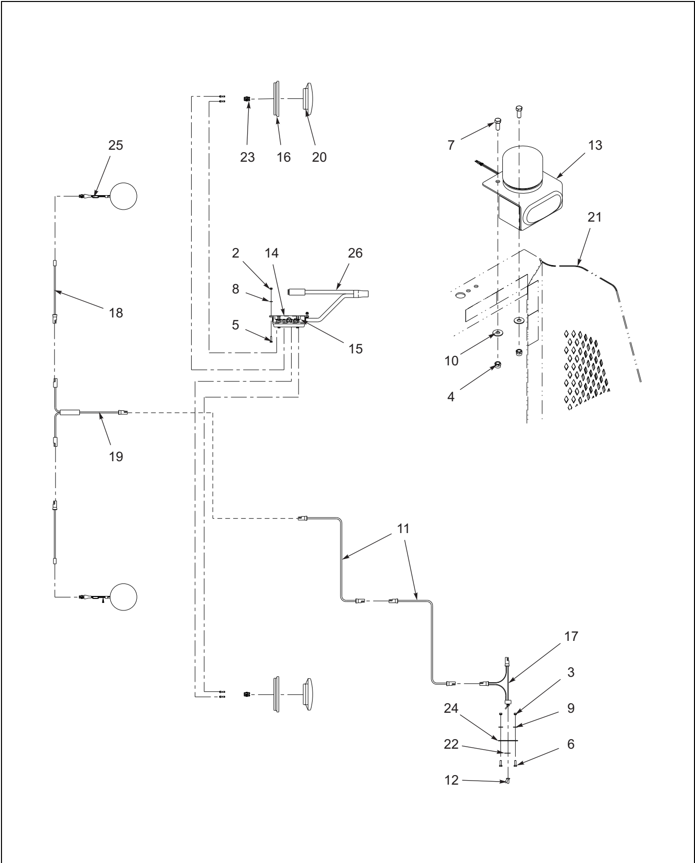
Figure 1-83: Bulkhead - Strobe & Turn Installation
