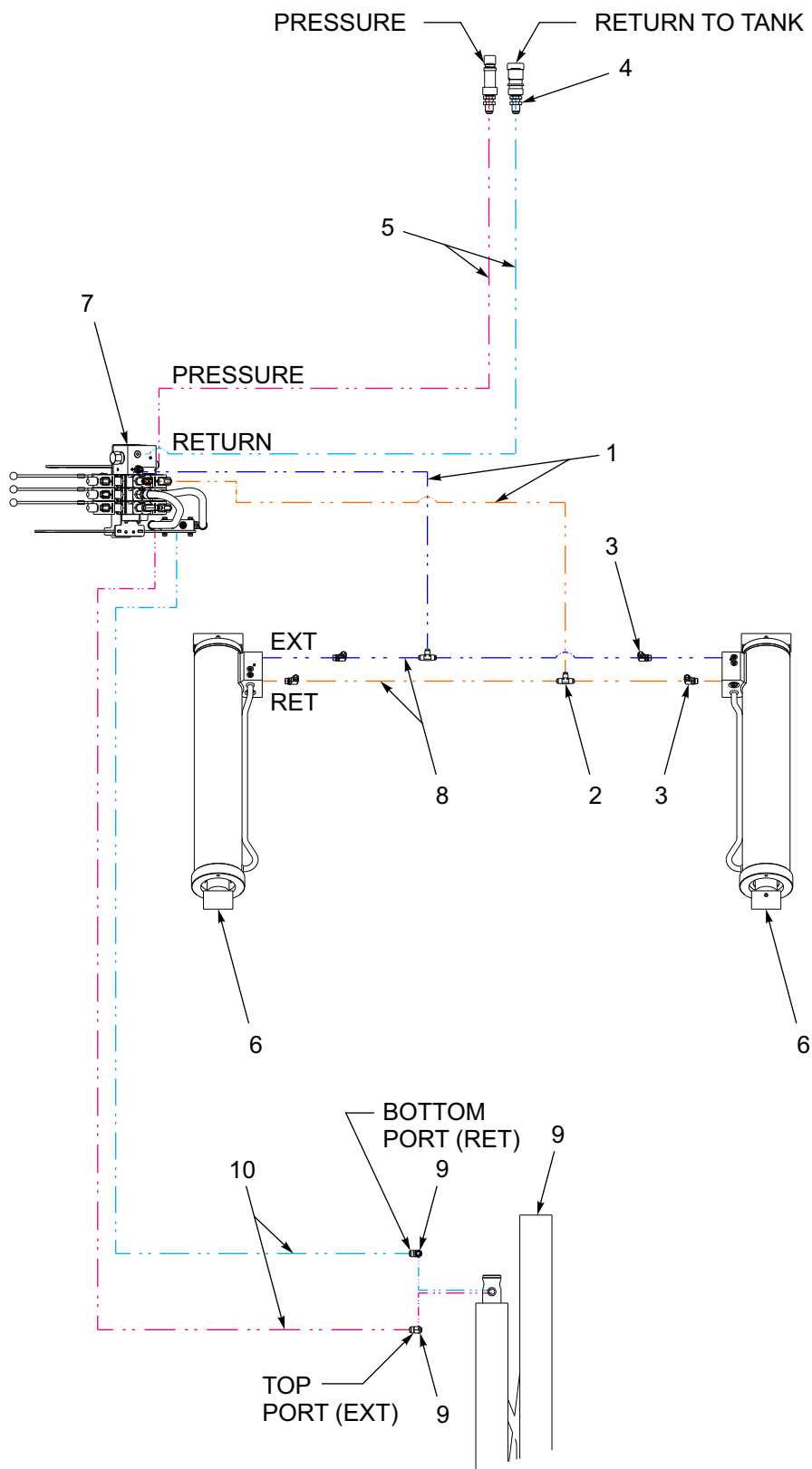
Figure 1-9: Hydraulic System
