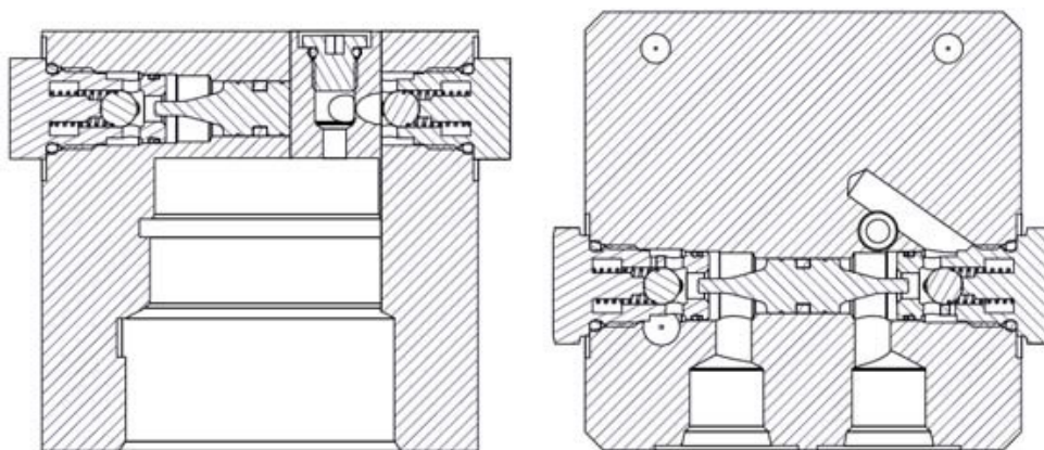
FRONT SECTION
