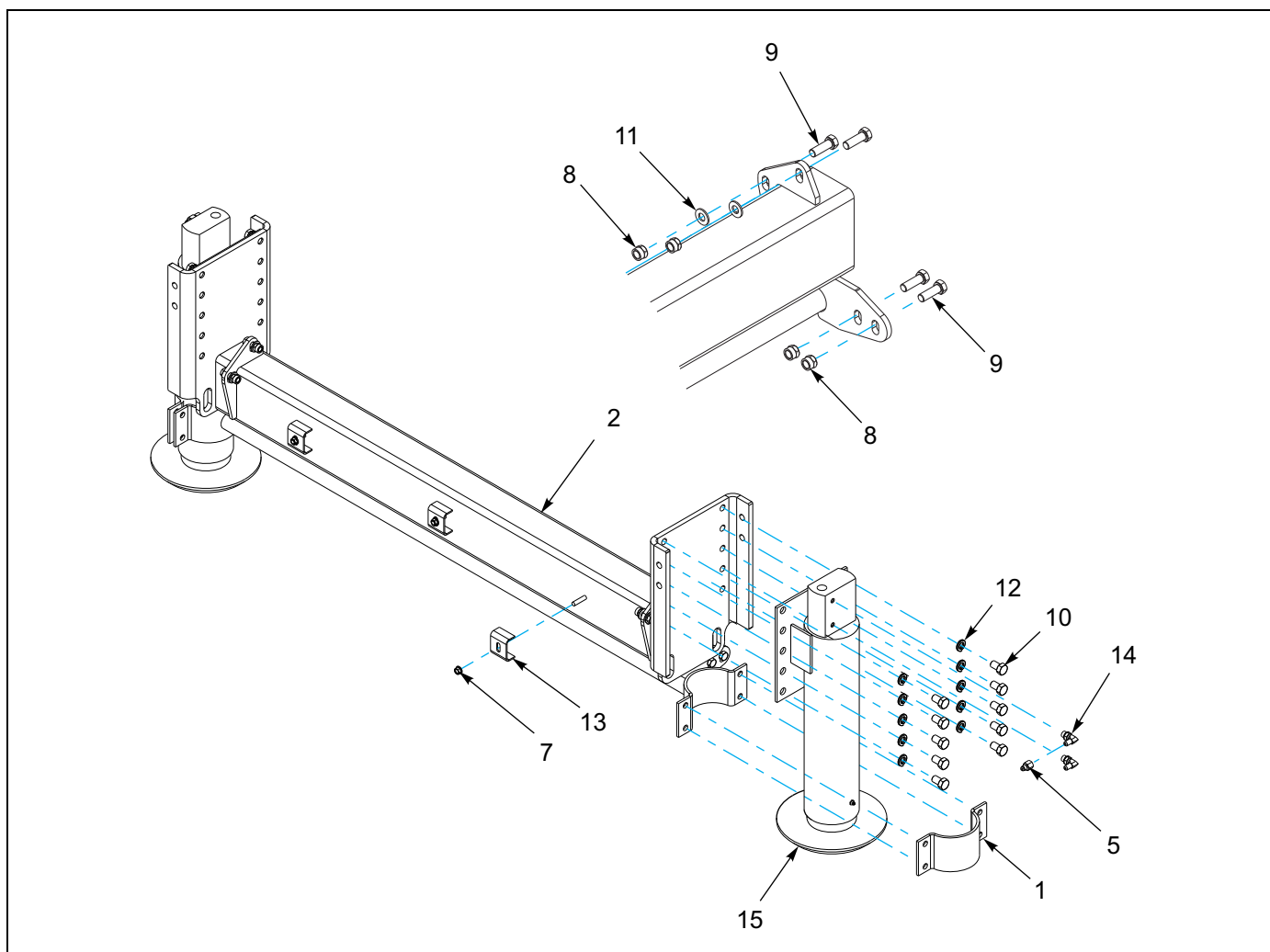
Figure 1-67: Dock Leveler Assembly - Single 60K (455A-120)
