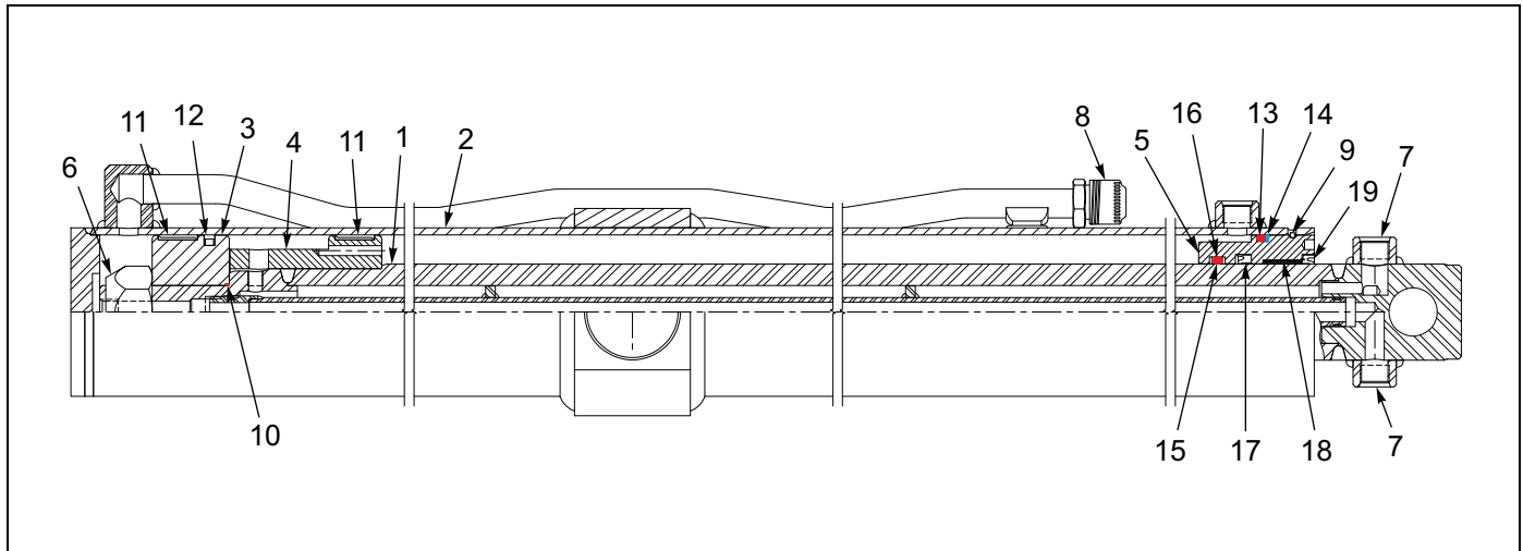
Figure 1-13: Cylinder Assembly - Ported Rod Hi Flow
