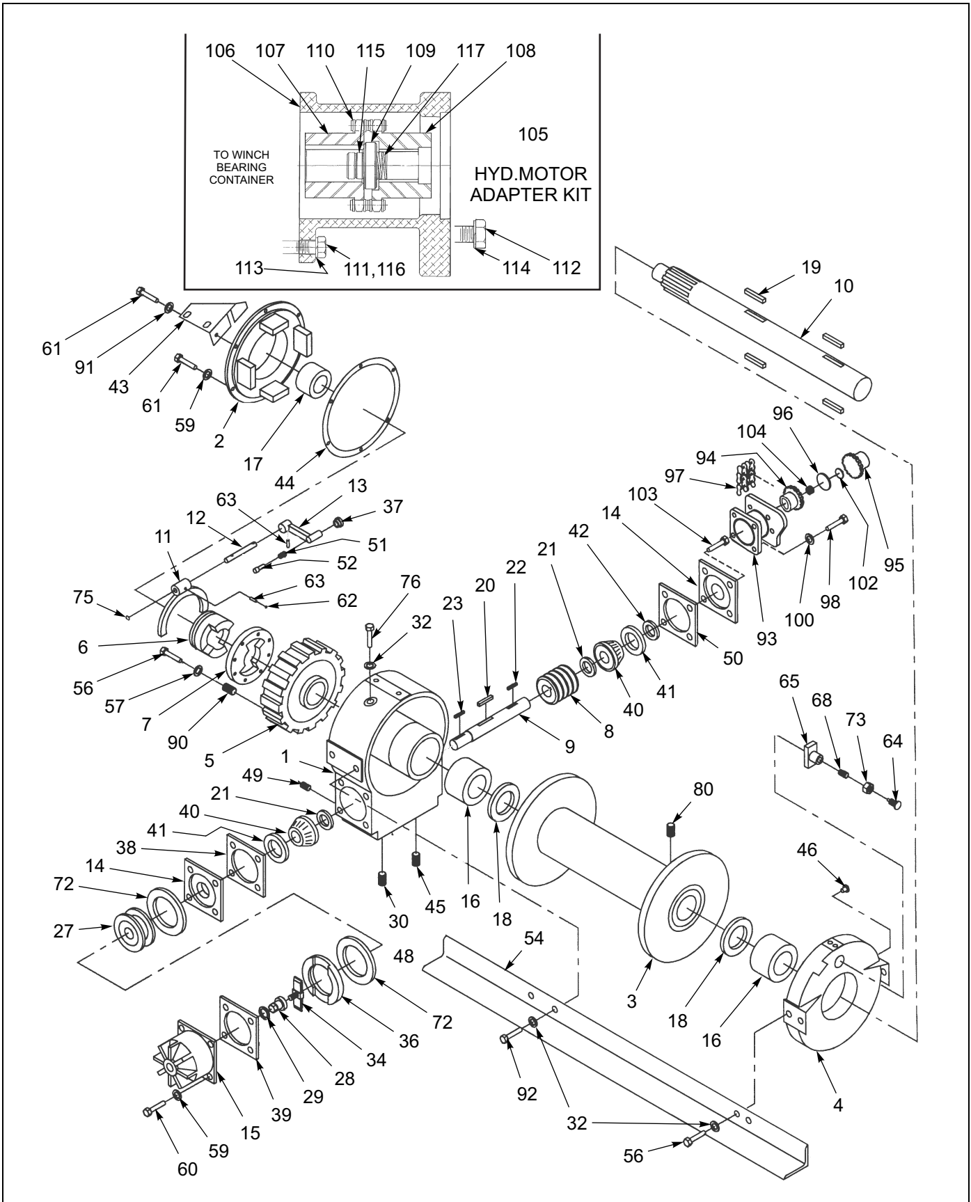
Figure 1-55: Winch Items - 20,000Lb. (BRADEN)
