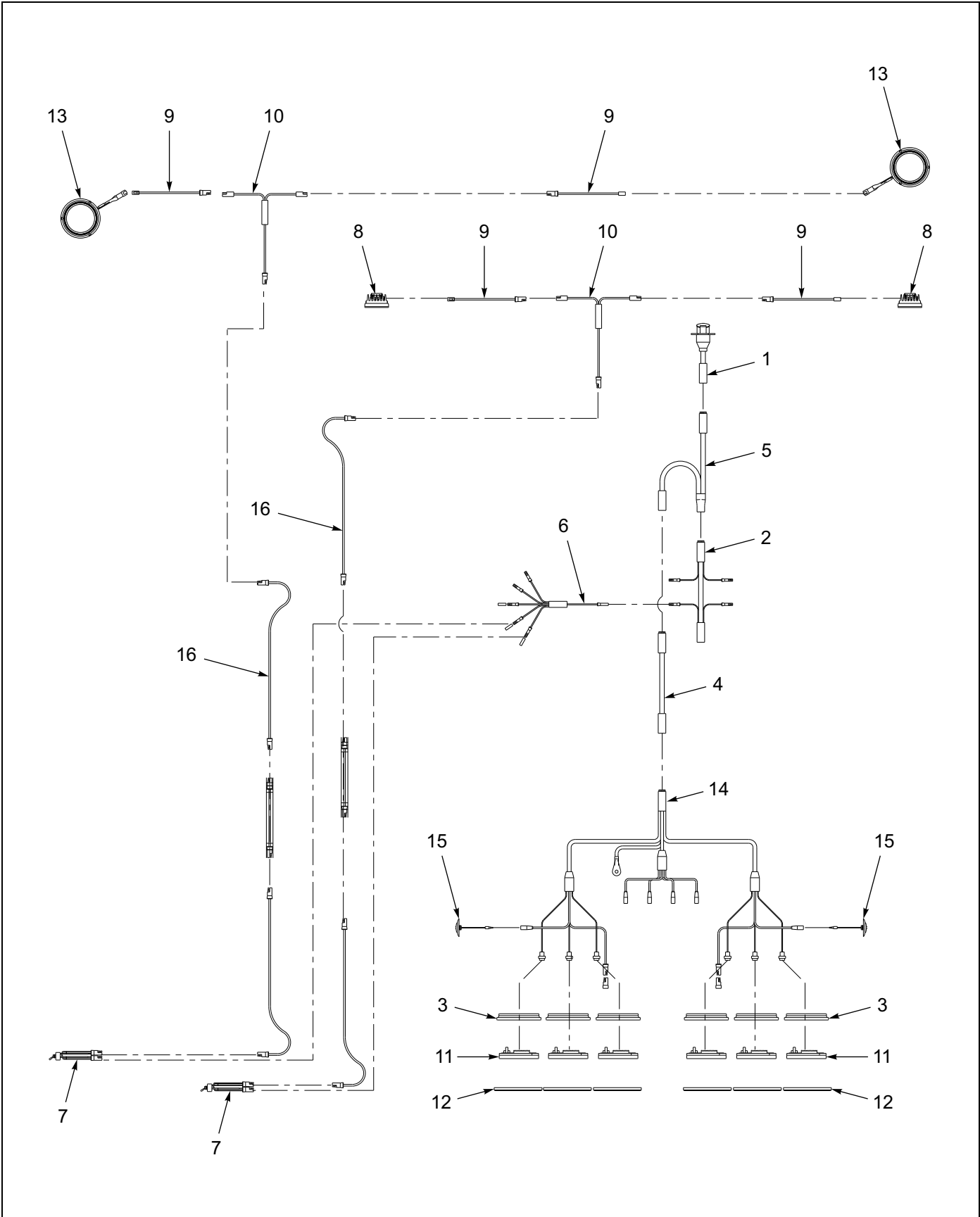
Figure 1-81: Bulkhead - Chain Rack Lights Electrical System
