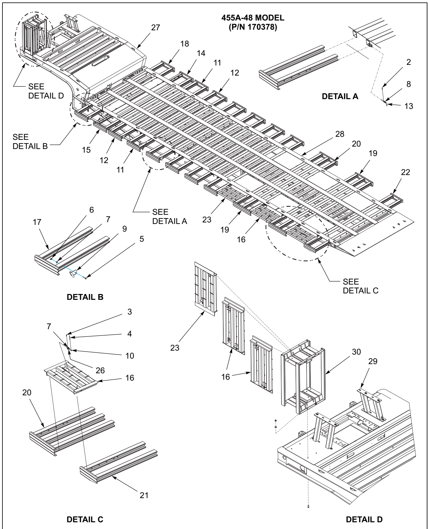
Figure 1-114: Pullout Extension Installation - 455A (2 of 3)
