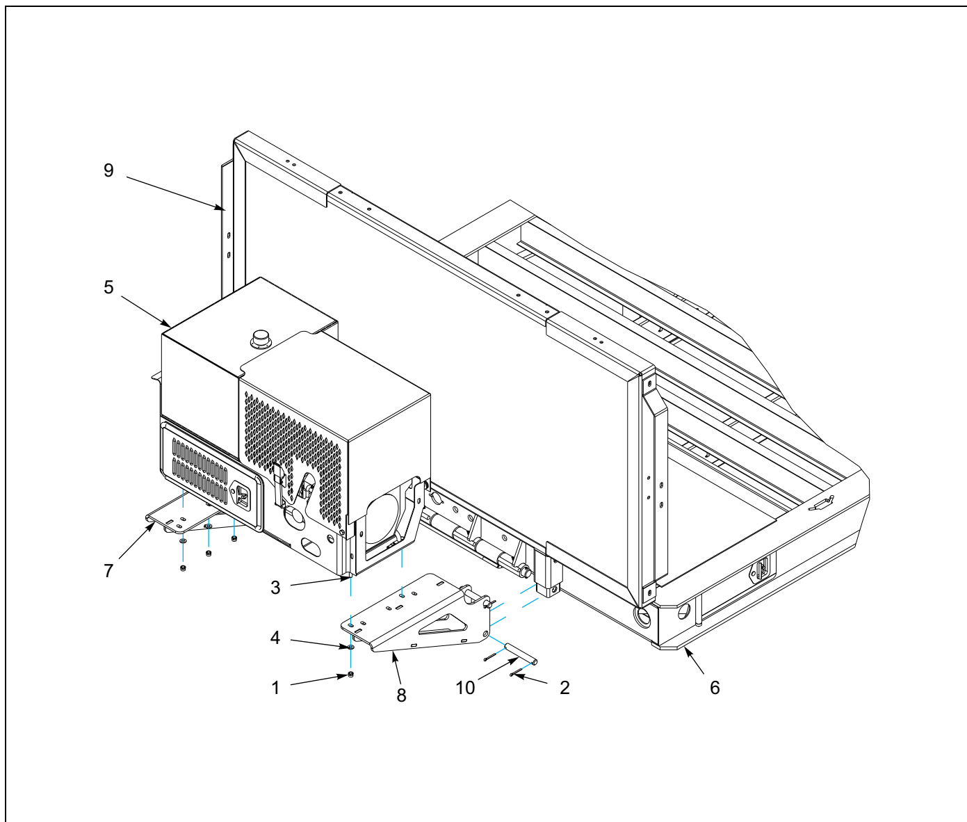
Figure 1-94: Engine - Front Mount Extension Package Installation
