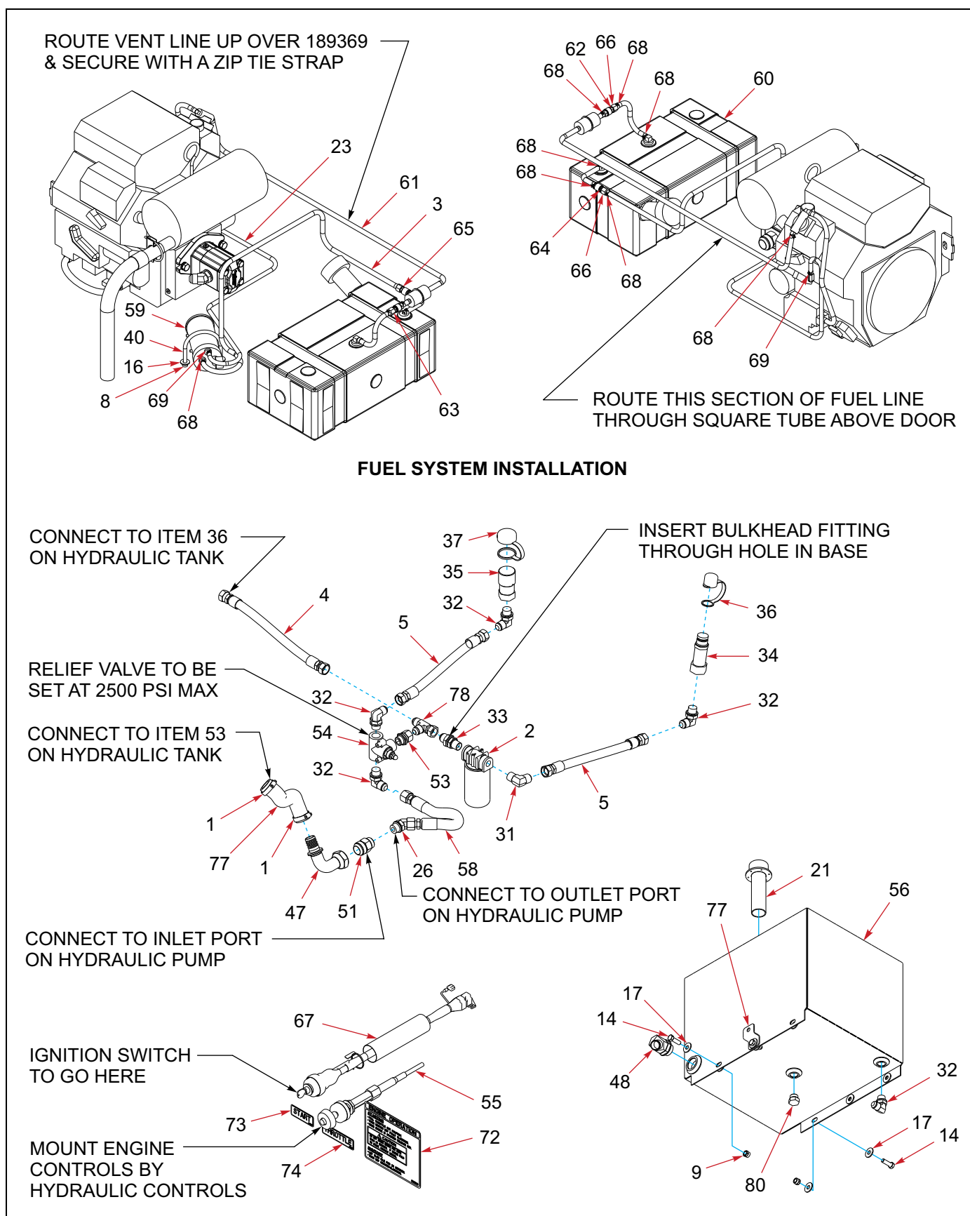
Figure 1-93: Engine - 25 HP Upper Deck Package (4 of 4)
