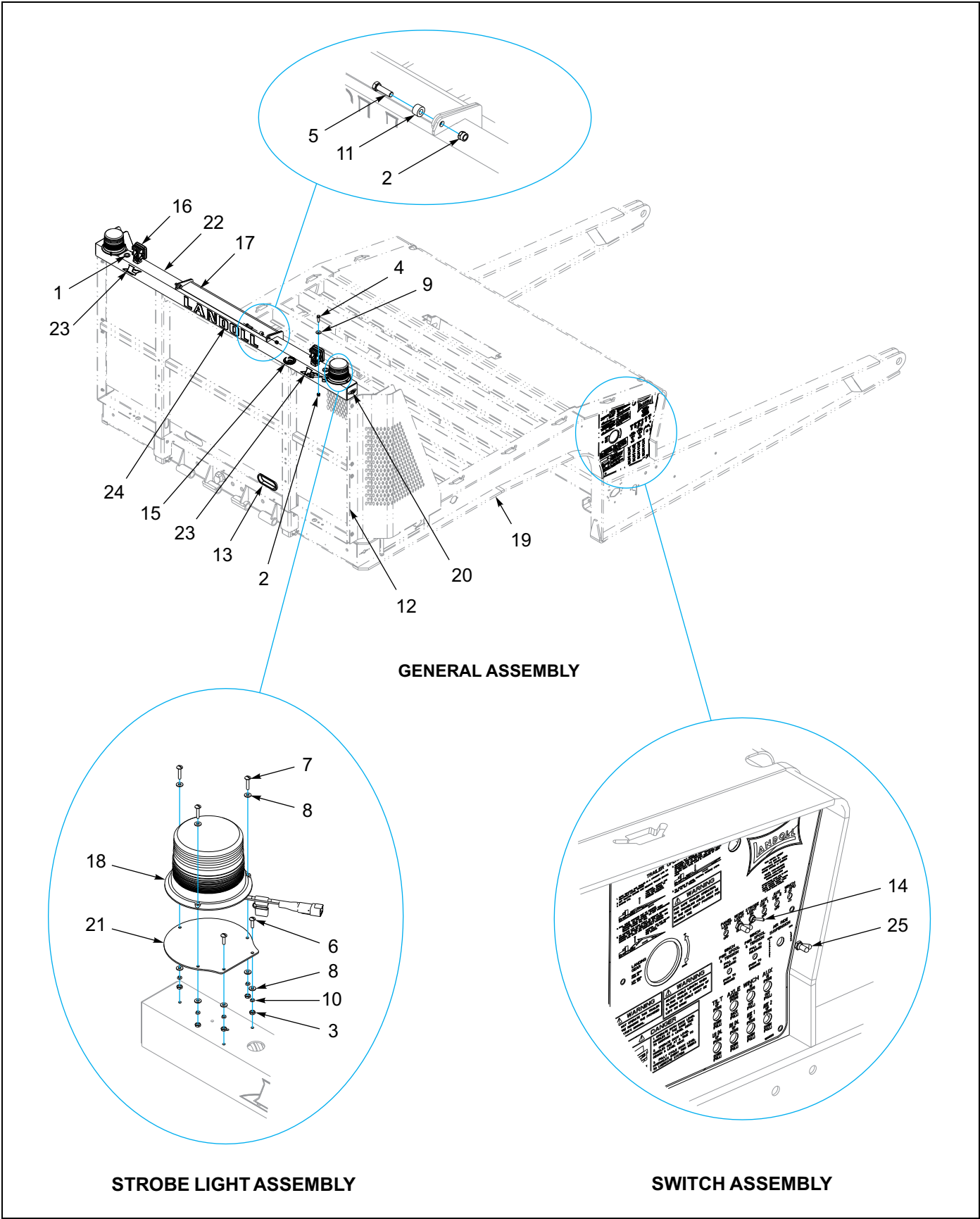
Figure 1-80: Bulkhead - Chain Rack Lights General Assembly
