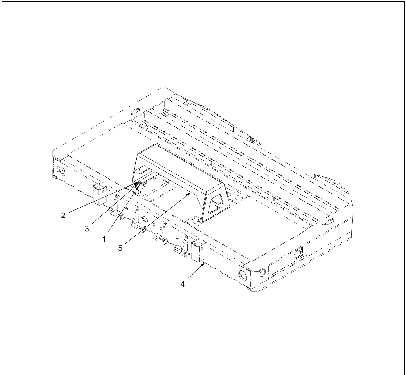
Figure 1-130: Winch - 12K/20K Guard Installation (BRADEN)
