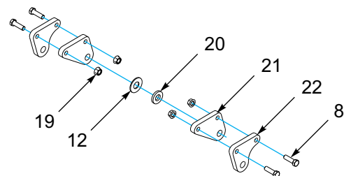
CYLINDER ANCHOR ASSEMBLY
