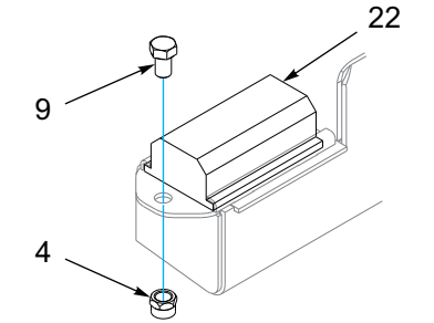
RUBBER BUMPER ASSEMBLY
