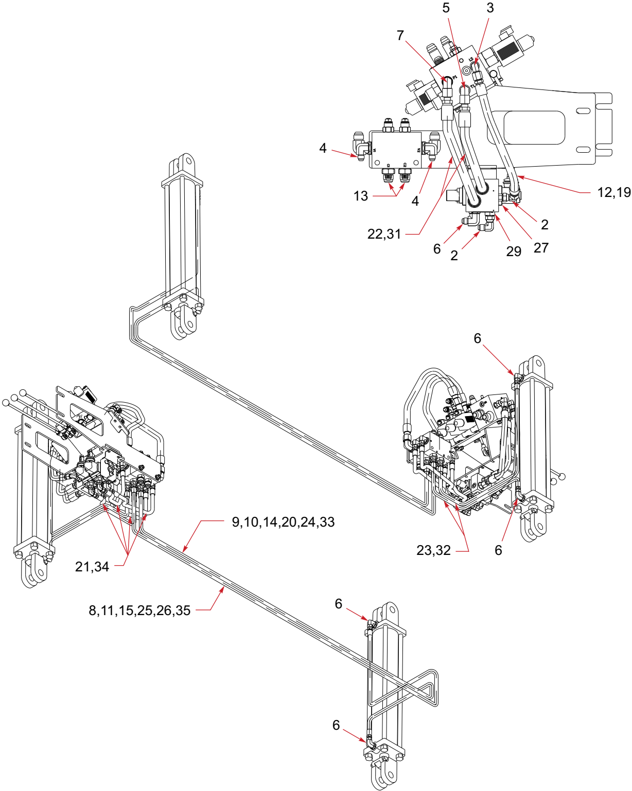
HYDRAULIC SCHEMATIC
