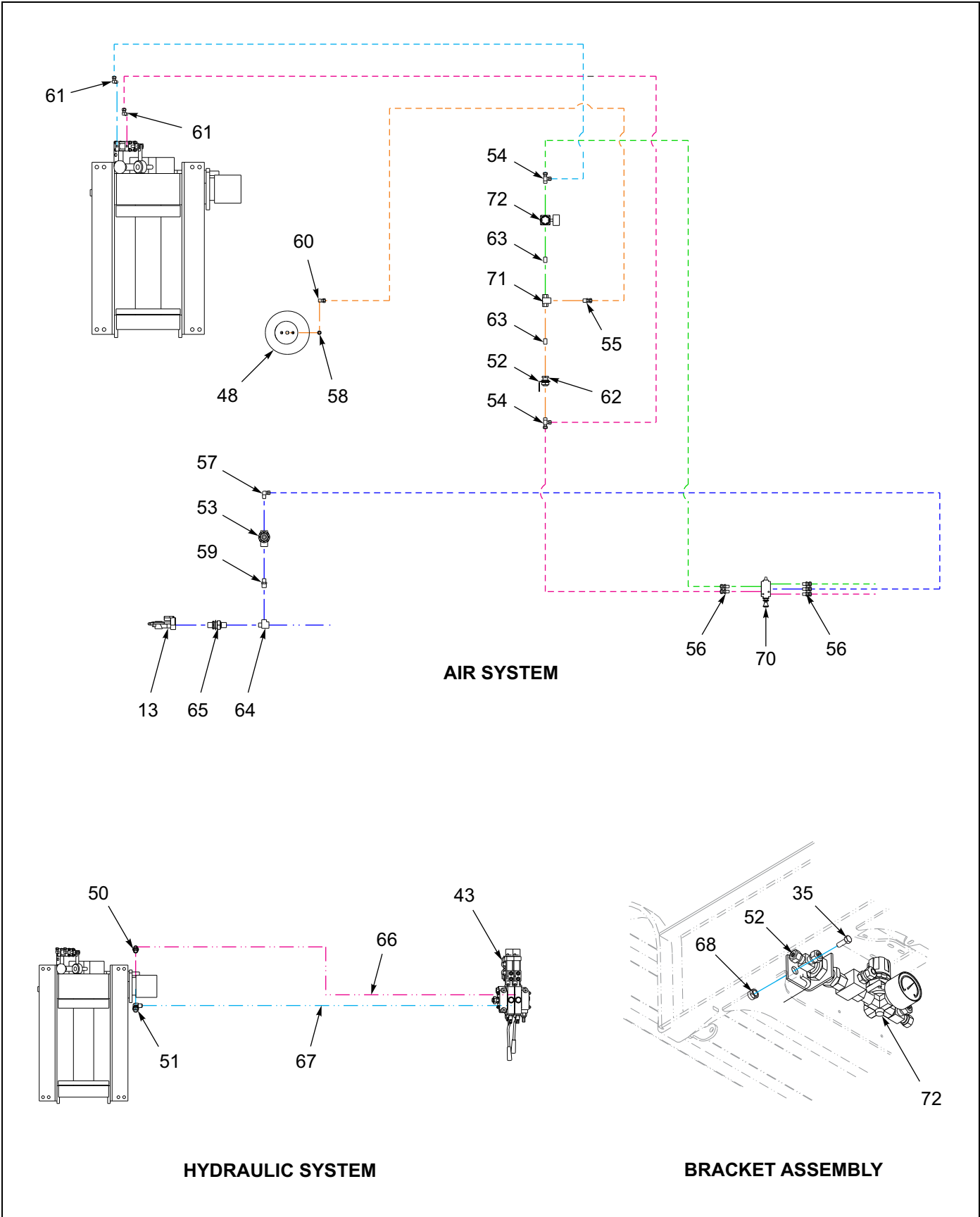
Figure 1-54: Winch Installation - 20K Air Tension/Release (BRADEN) (3 of 3)
