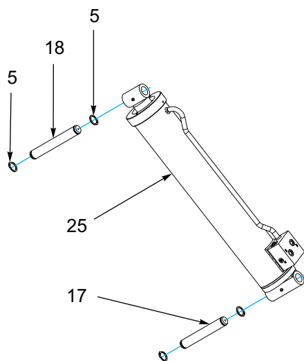
CYLINDER ASSEMBLY
