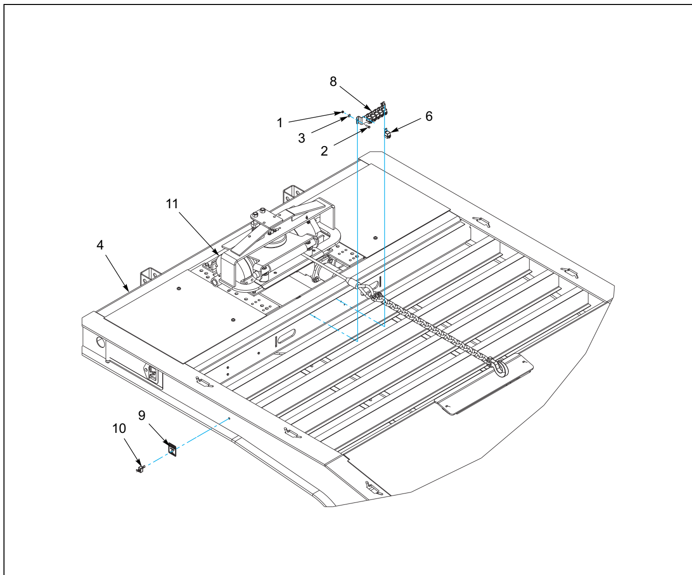
Figure 1-140: Electrical Disconnect Switch Installation
