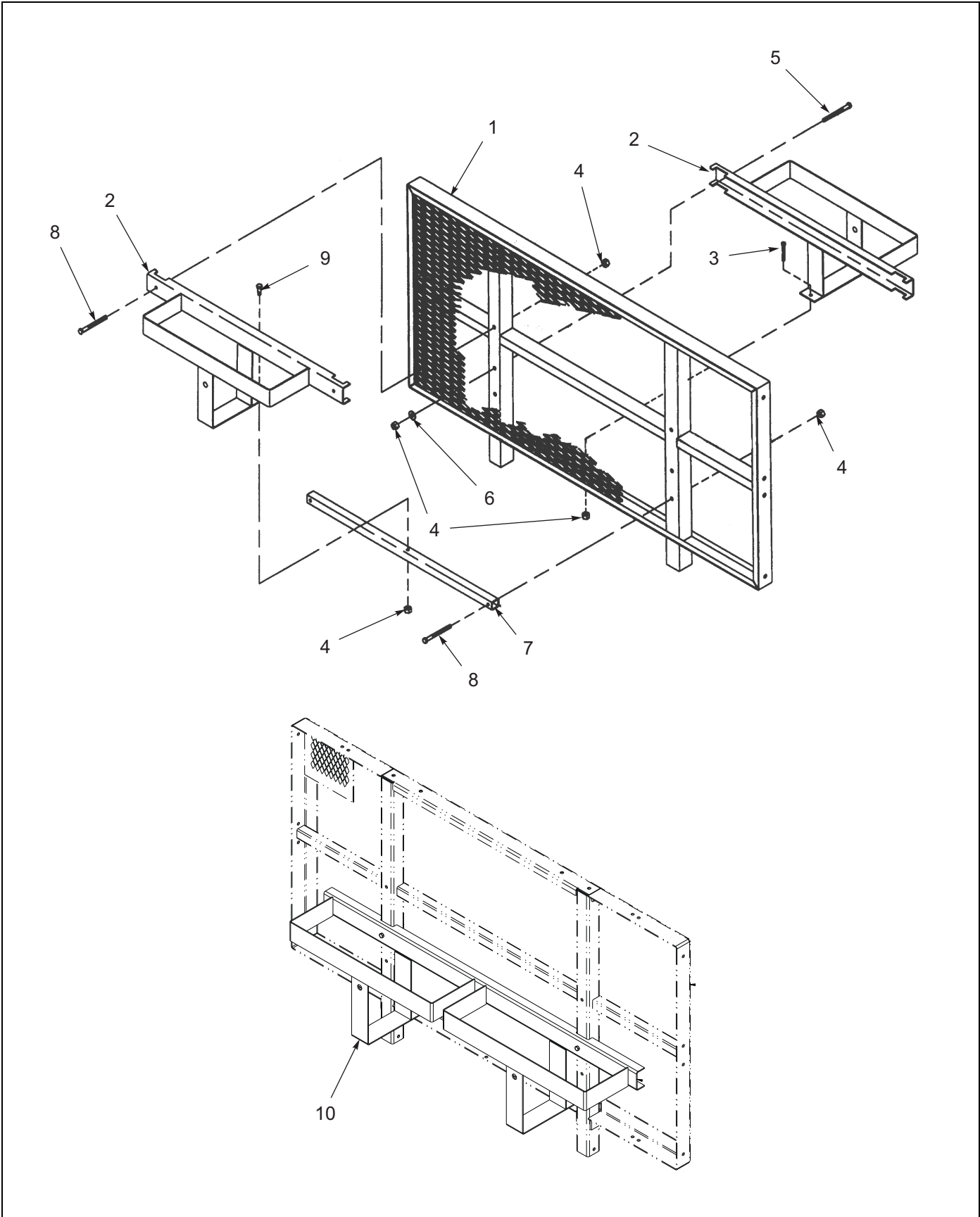
Figure 1-124: Spare Tire Carrier
