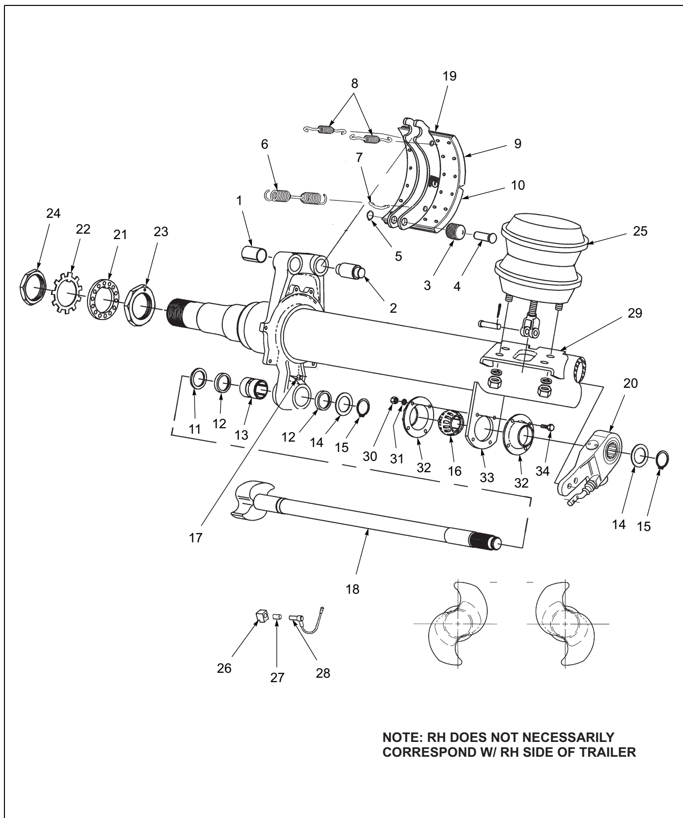
Figure 1-35: Axle and Brake Assembly - Dexter 12-1/4" X 7-1/2"
