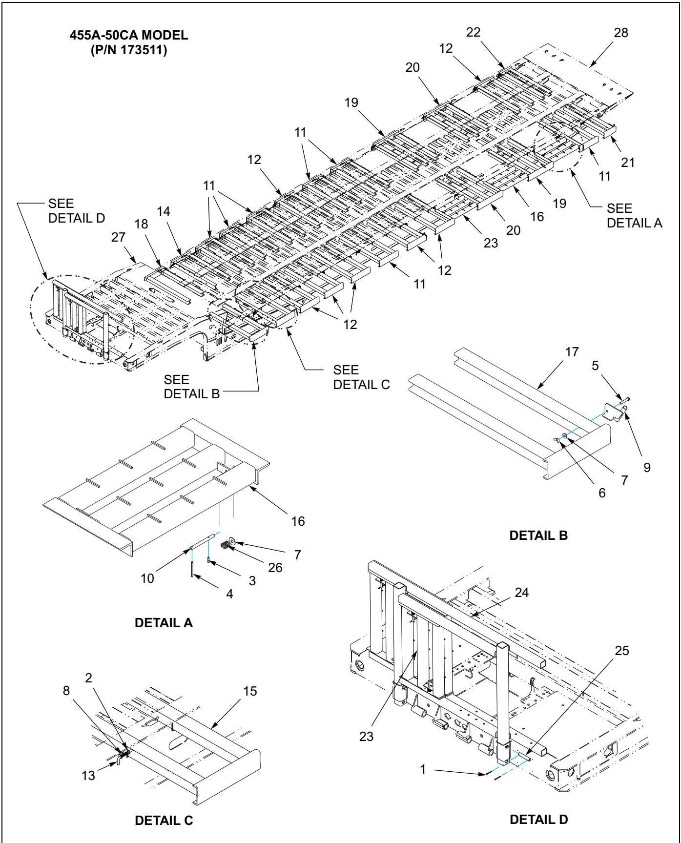
Figure 1-115: Pullout Extension Installation - 455A (3 of 3)
