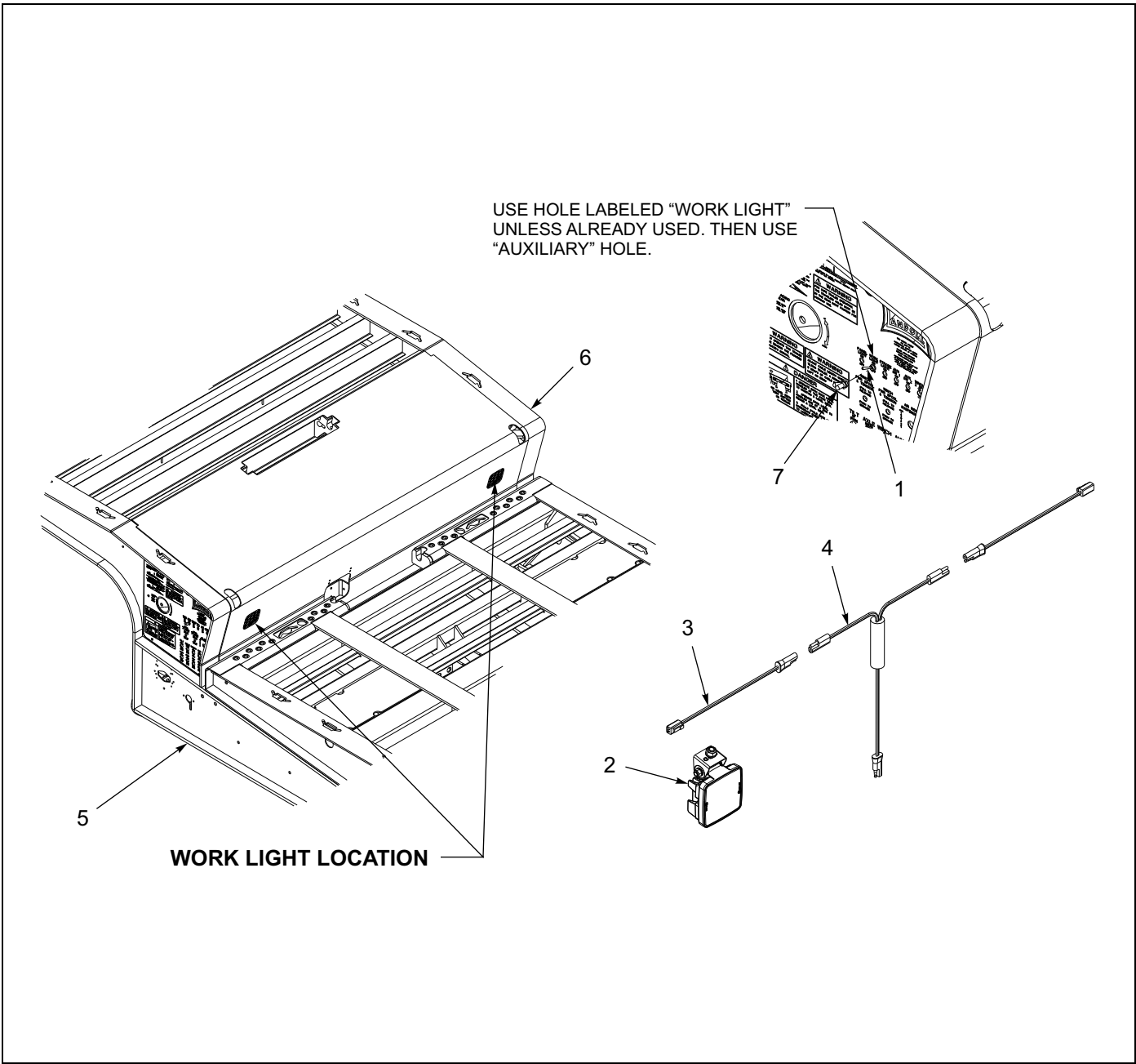
Figure 1-127: Upper Deck - Slope Light Installation
