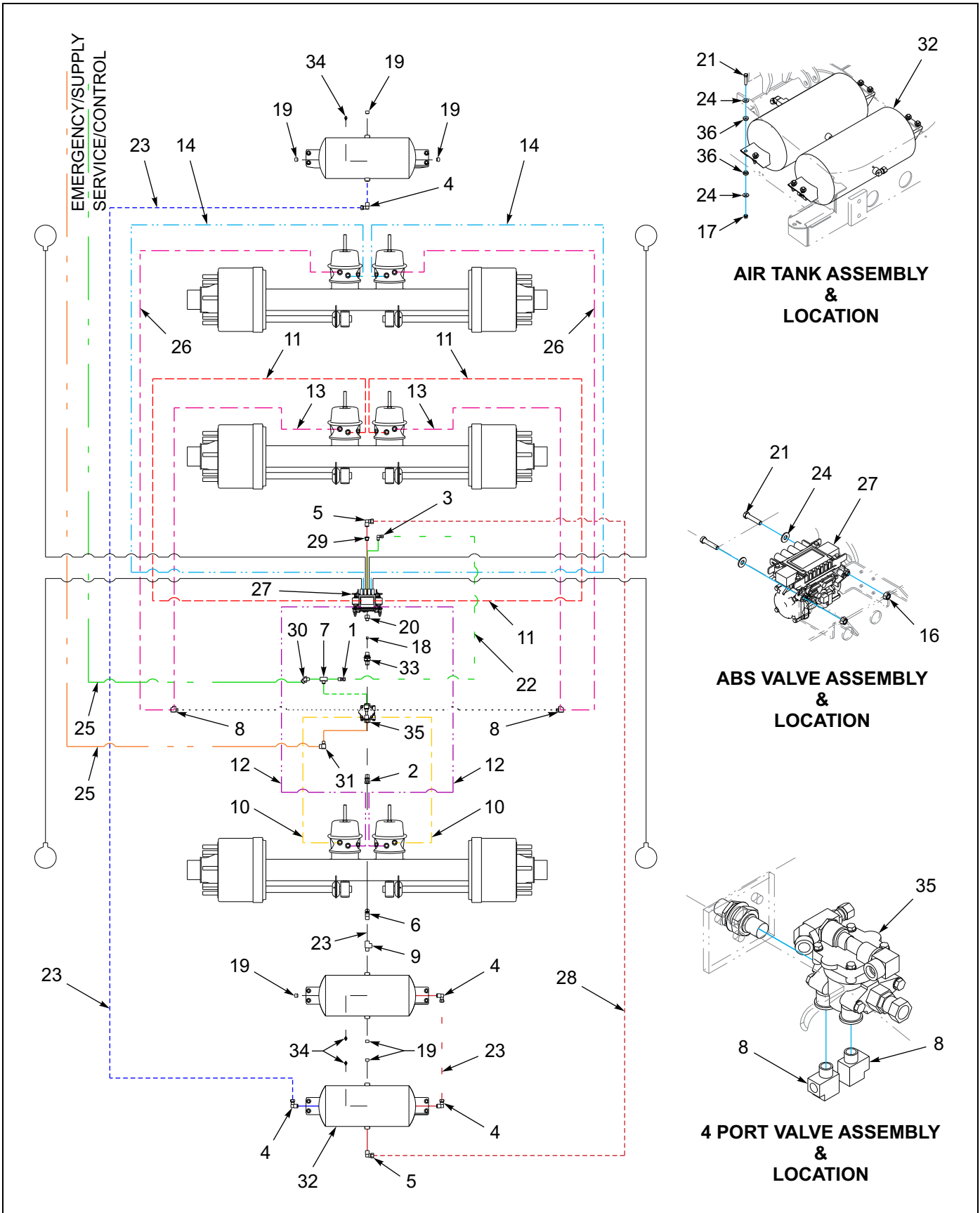
Figure 1-40: Air Brake System - 455A Spring Brake
