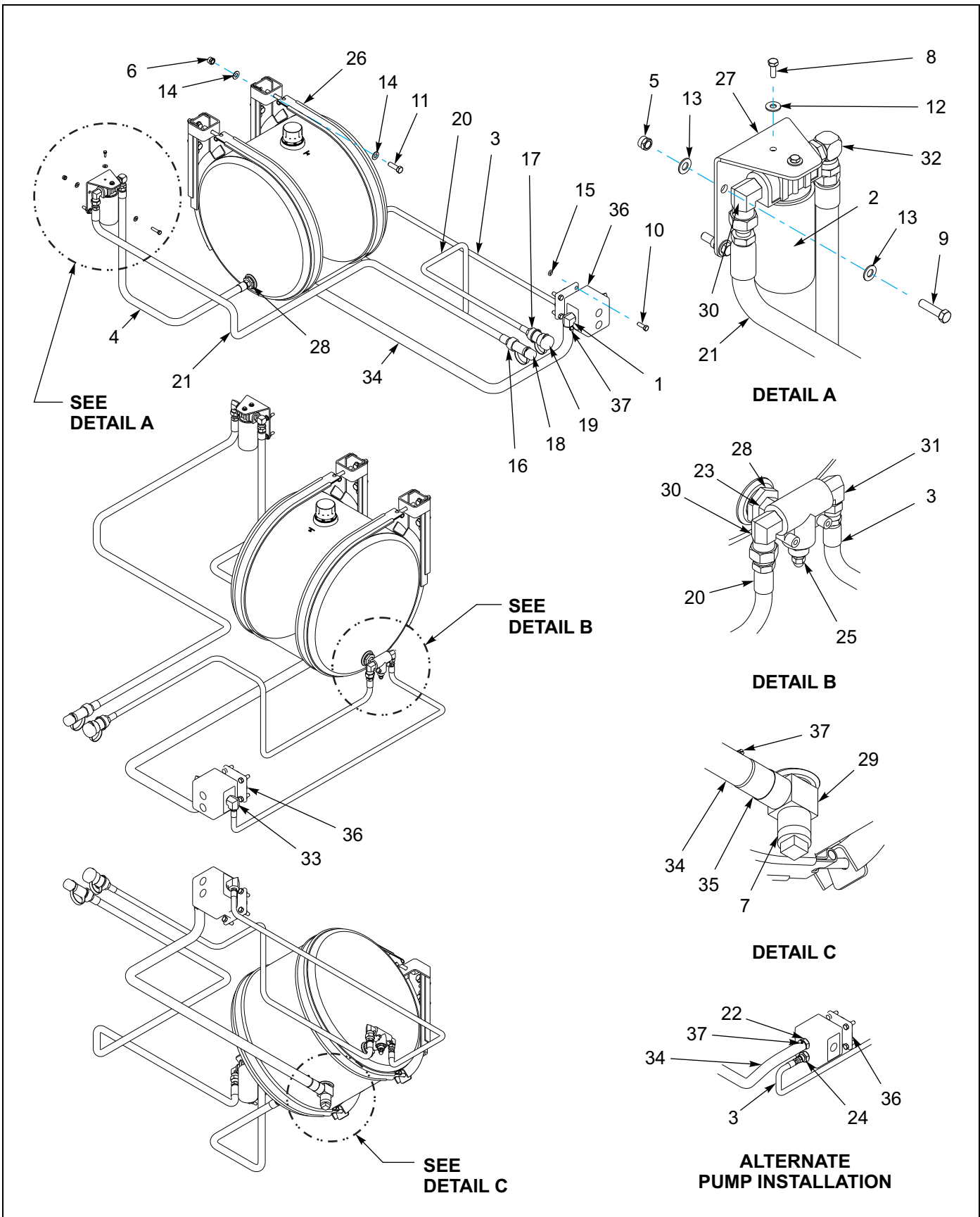
Figure 1-98: Hydraulic Wet Kit Items - 35 Gallon Aluminum
