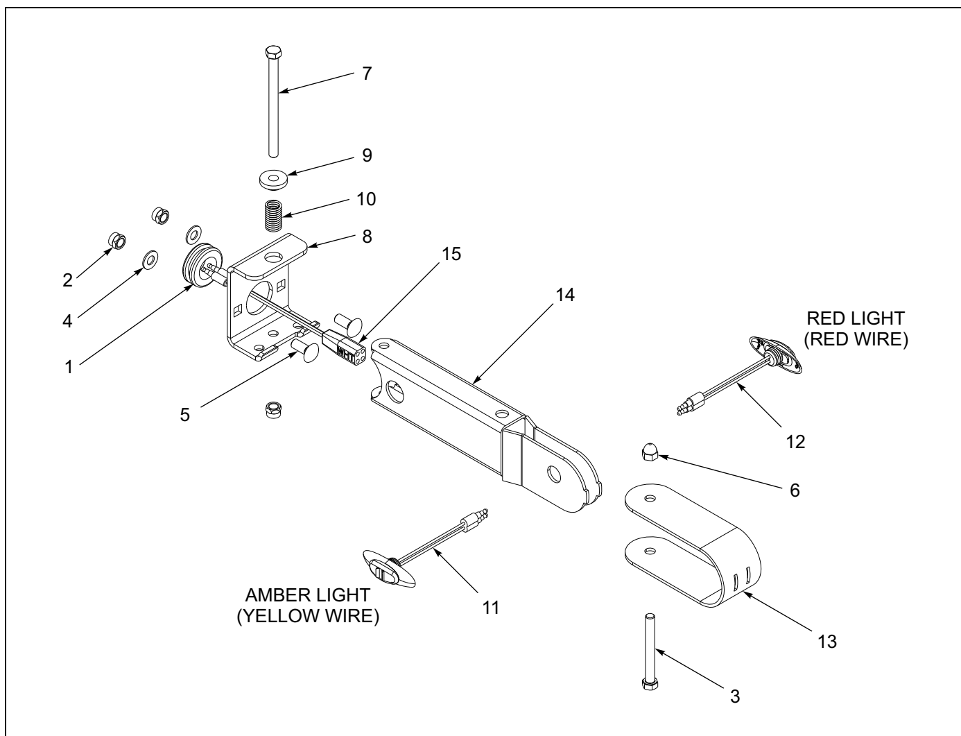
Figure 1-108: Swing-Arm Light Assembly - STREET
