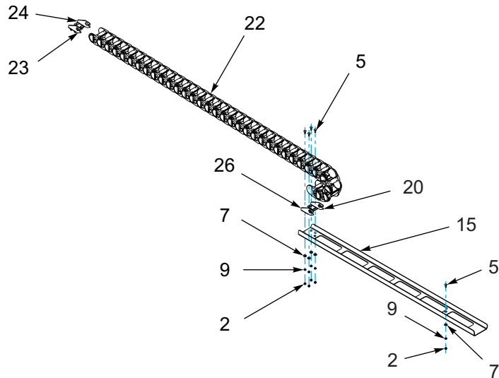
E-CHAIN ASSEMBLY
