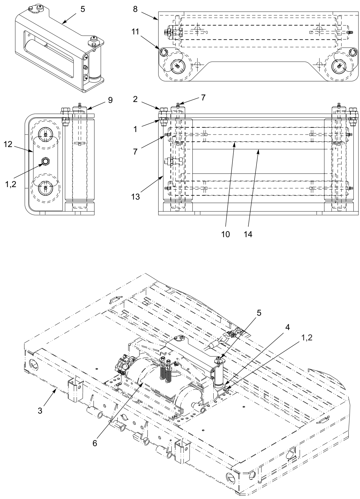
Figure 1-117: 4 Roller Guide Installation - 20K (BRADEN)
