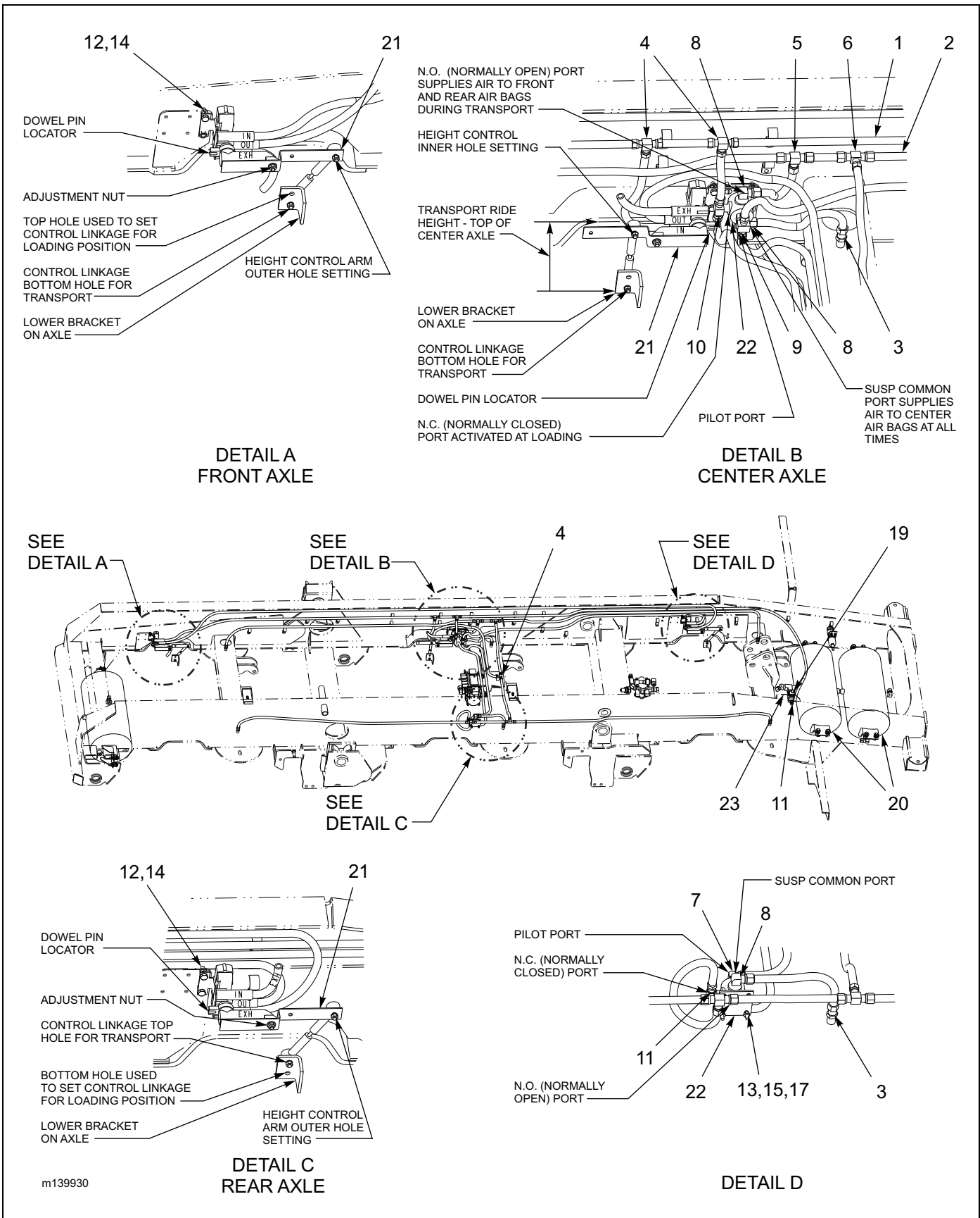
Figure 1-32: Air Ride Suspension - 455A (Arctic)
