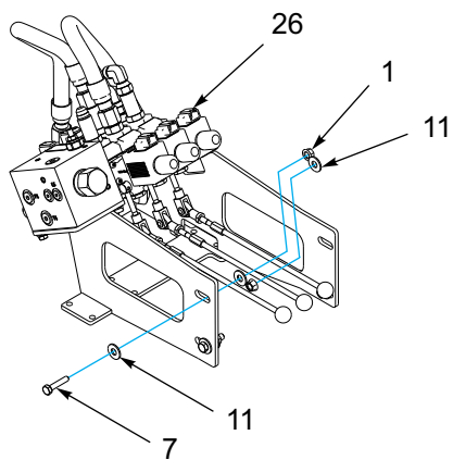
3-SPOOL VALVE ASSEMBLY
