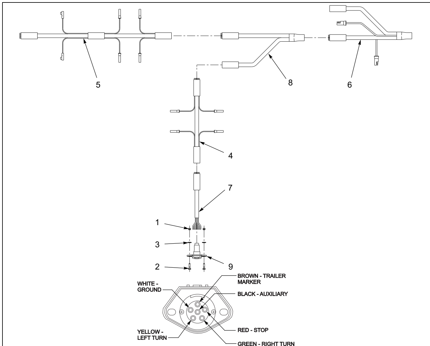
Figure 1-87: 6-Way Electrical Installation
