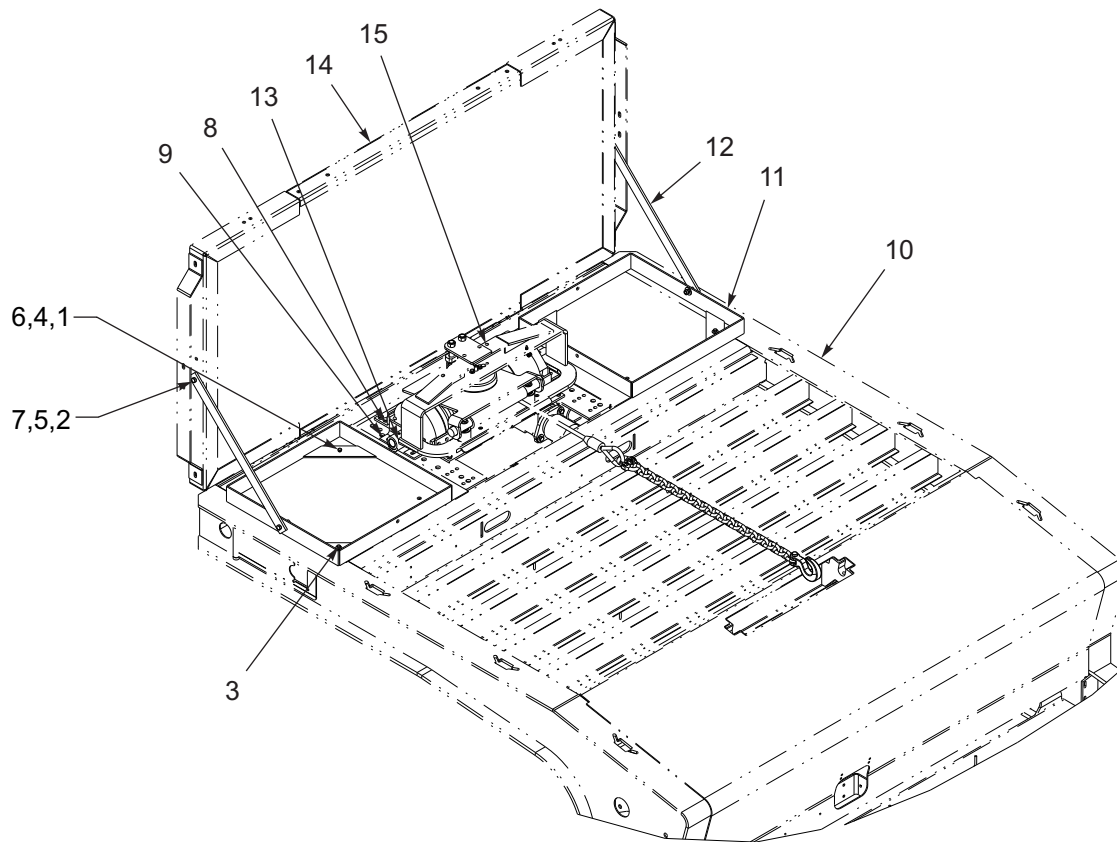
Figure 1-139: Chain Tray Assembly
