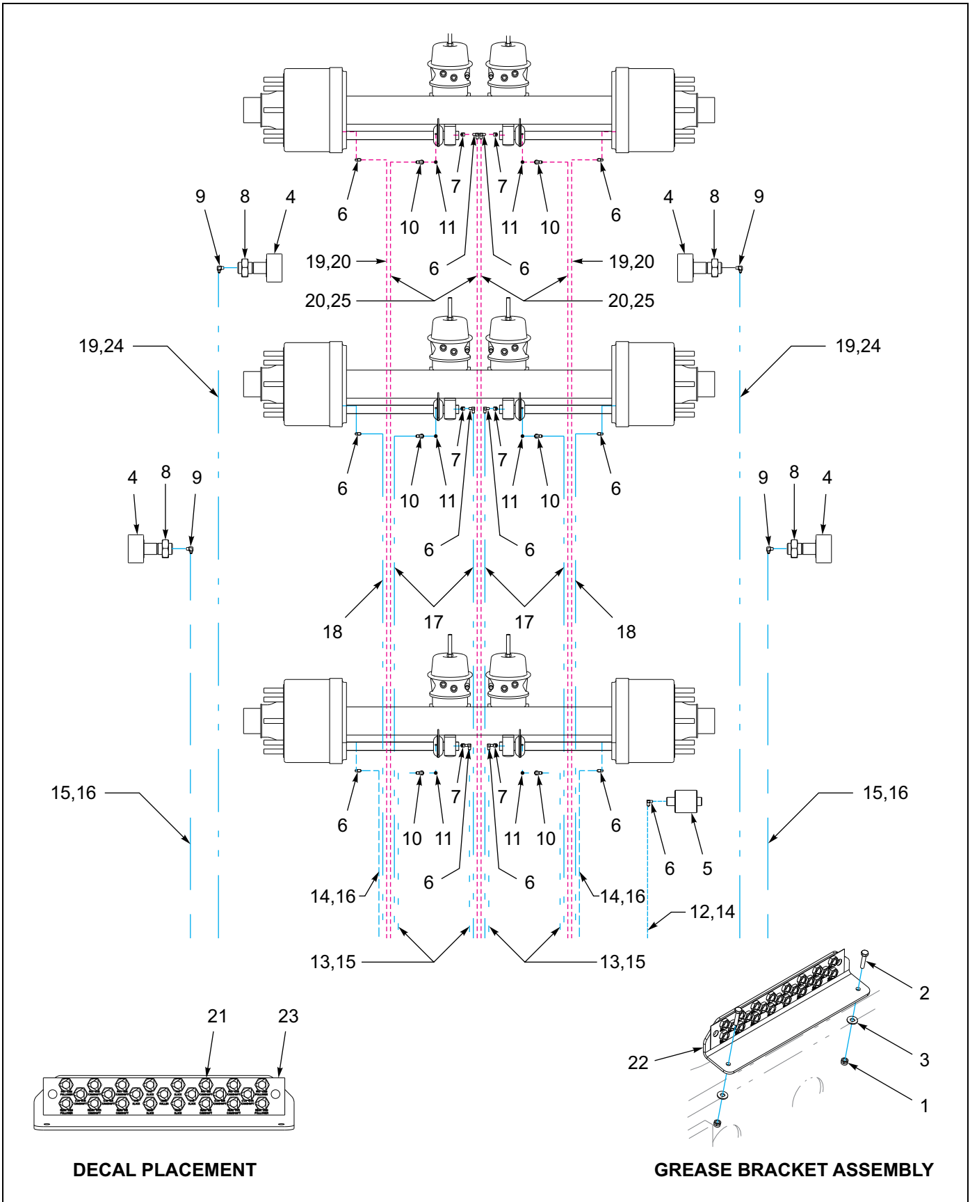
Figure 1-28: Grease System - 455A Spring Brake
