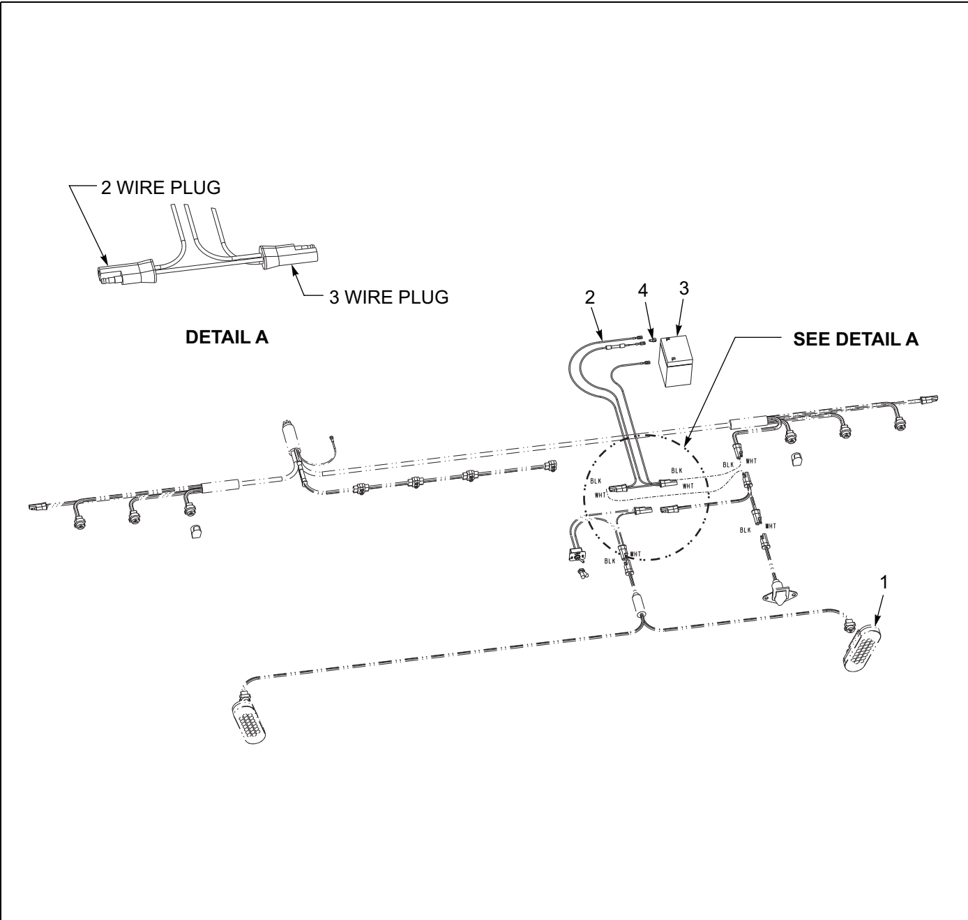
Figure 1-85: Bumper - Strobe Light Battery Backup
