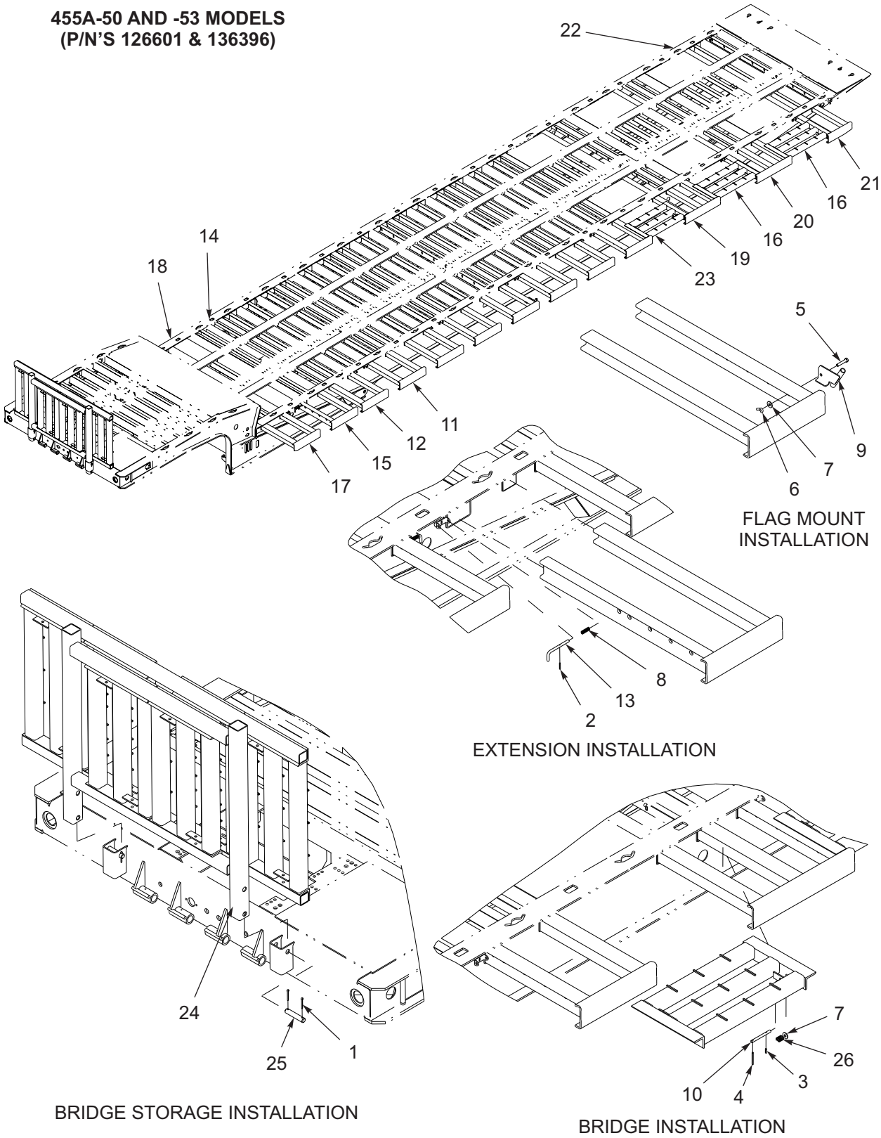
Figure 1-113: Pullout Extension Installation - 455A (1 of 3)
