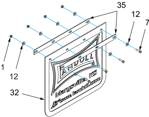
MUDFLAP ASSEMBLY
