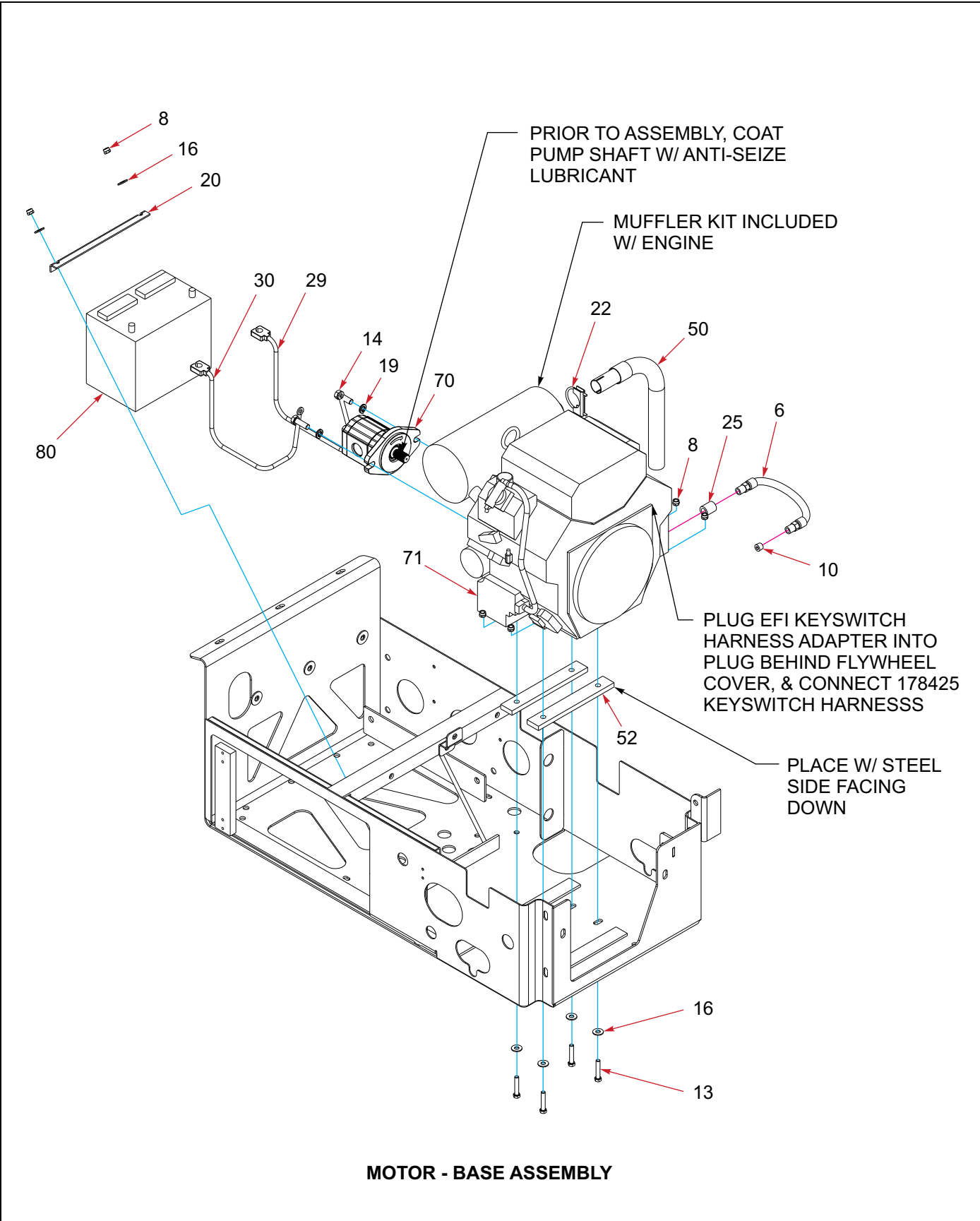
Figure 1-91: Engine - 25 HP Upper Deck Package (2 of 4)
