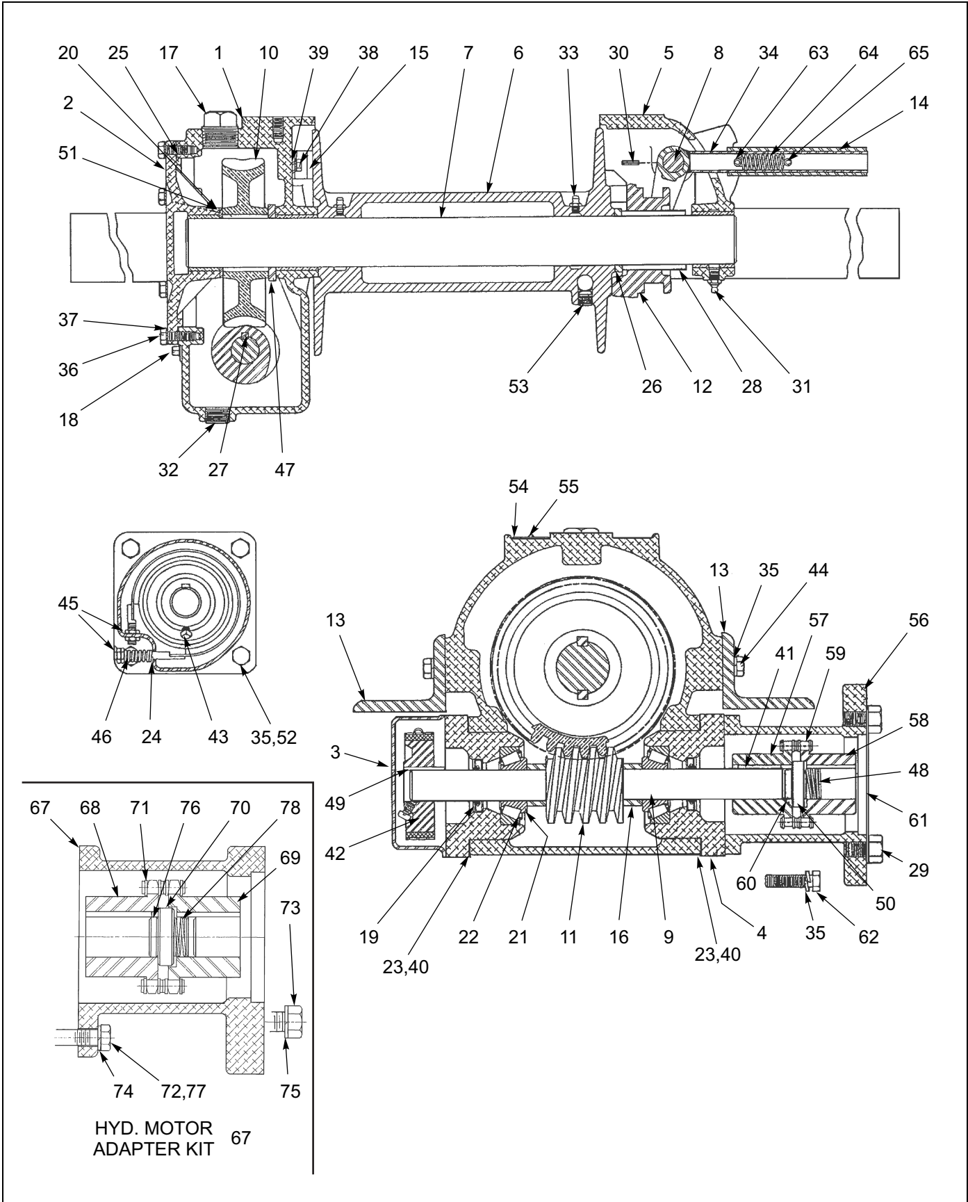
Figure 1-50: Winch Items - 12,000 Lb. (BRADEN)
