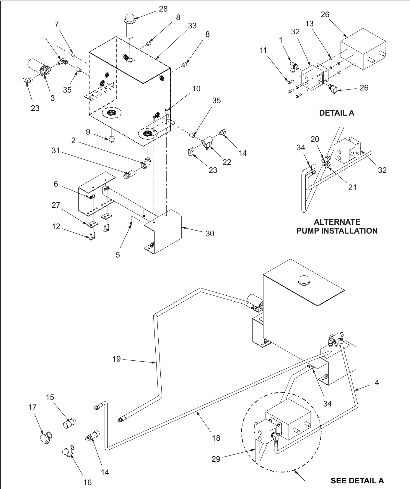
Figure 1-97: Hydraulic Wet Kit Items - 30 Gallon
