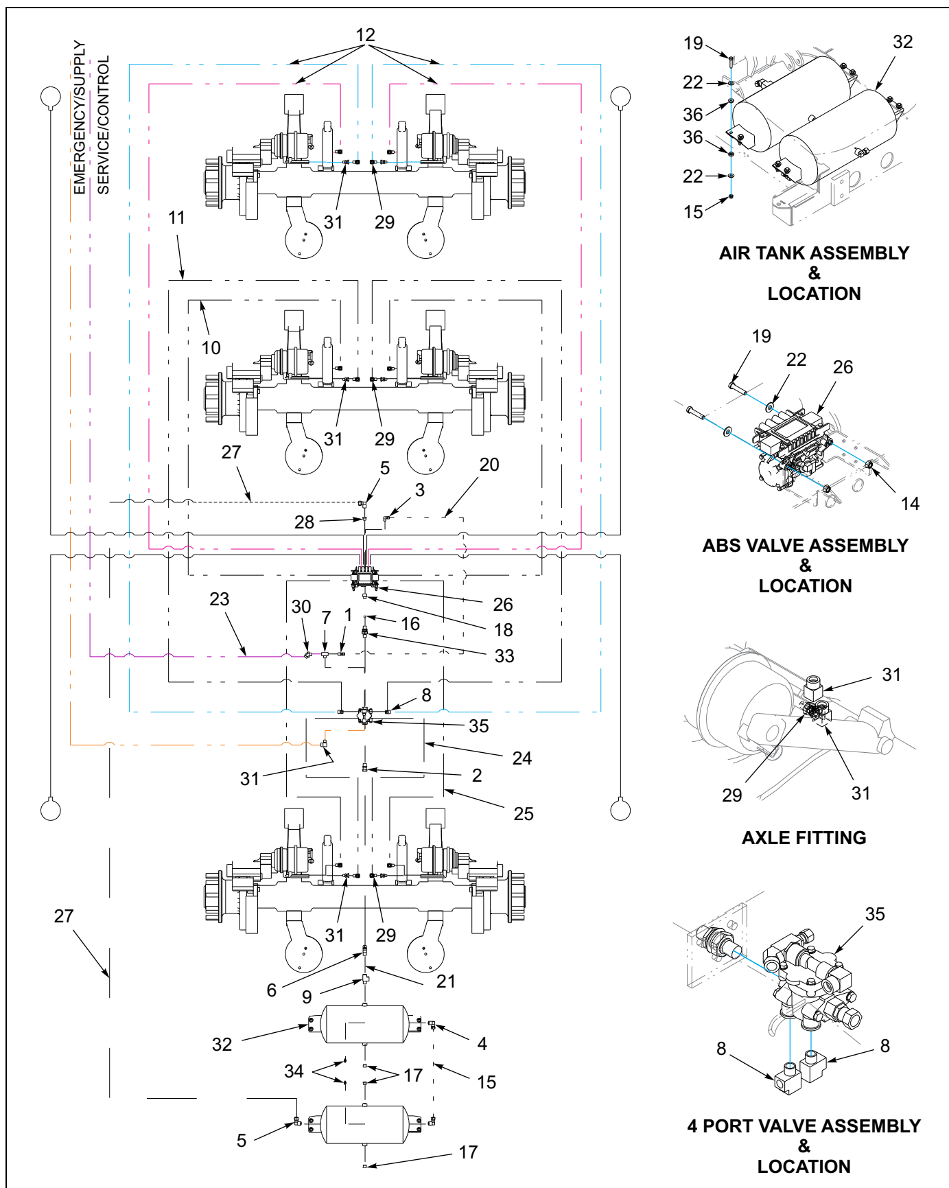
Figure 1-41: Air Brake System - 455A Disc Brake
