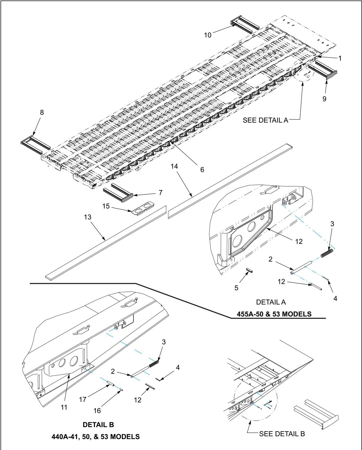
Figure 1-145: Outrigger Installation
