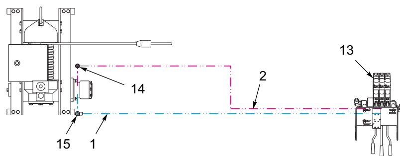
HYDRAULIC SYSTEM
