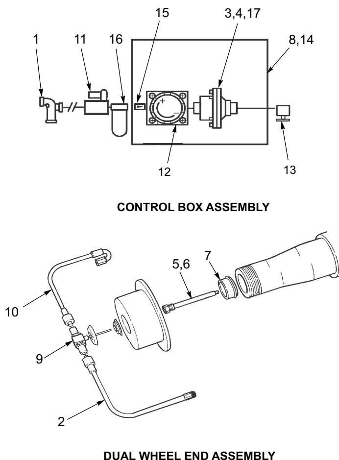
Figure 1-47: Tire Inflation System -Thermalert (3 SAF Axles)
