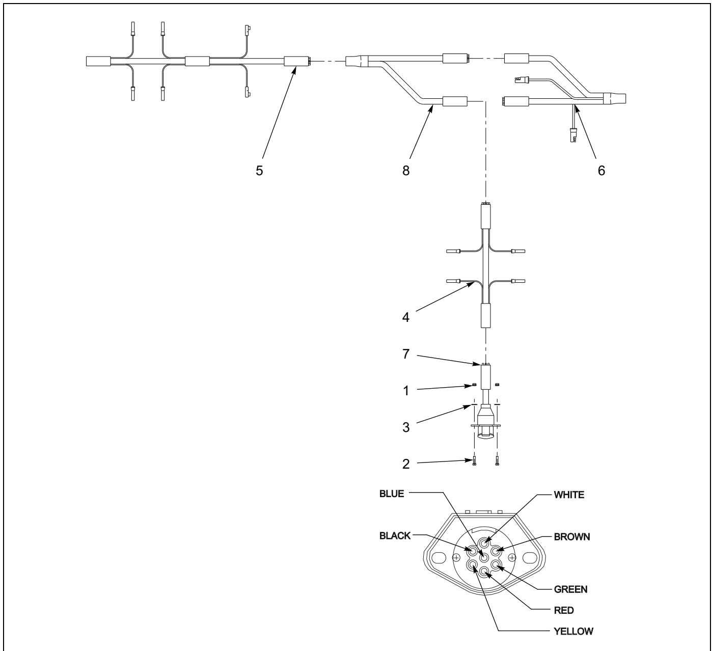
Figure 1-88: 7-Way Electrical Installation
