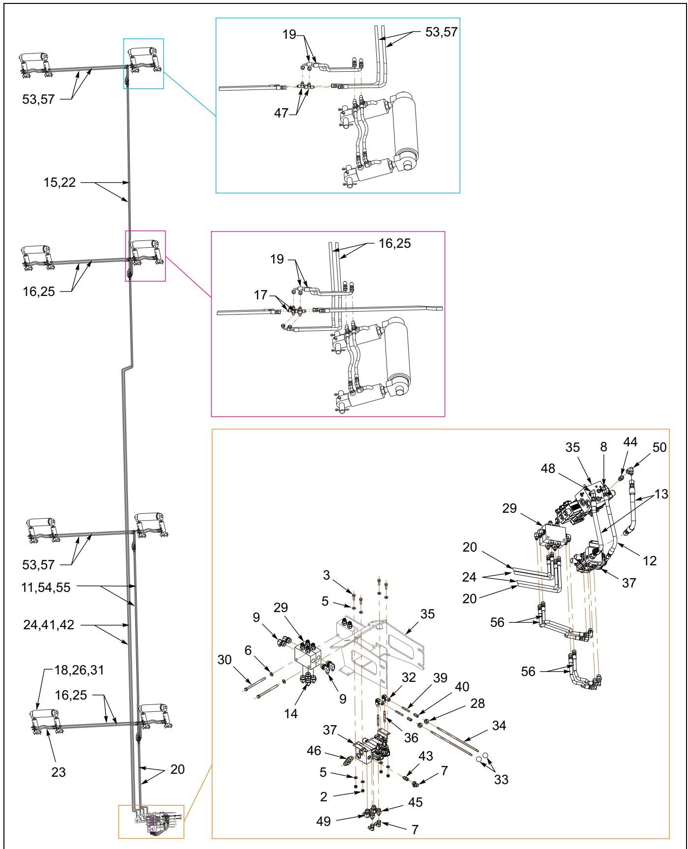
Figure 1-120: 8 Pop-Up Roller Installation (2 of 2)
