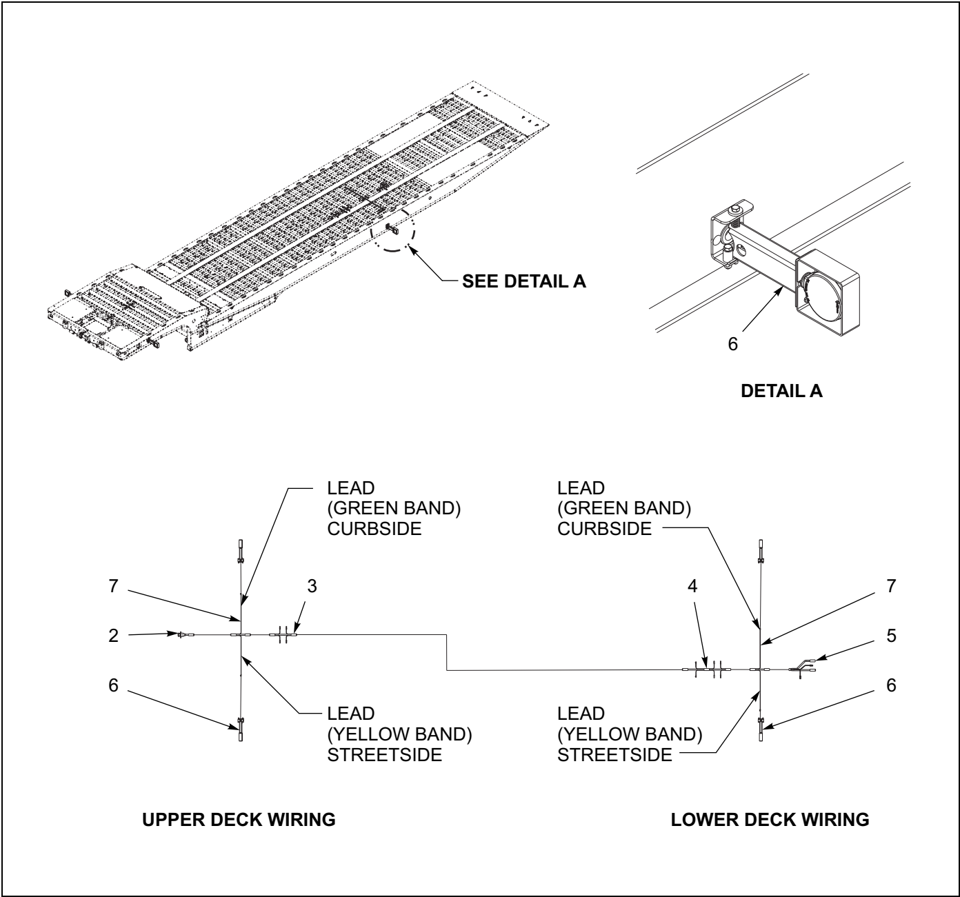
Figure 1-105: Swingout Light Installation
