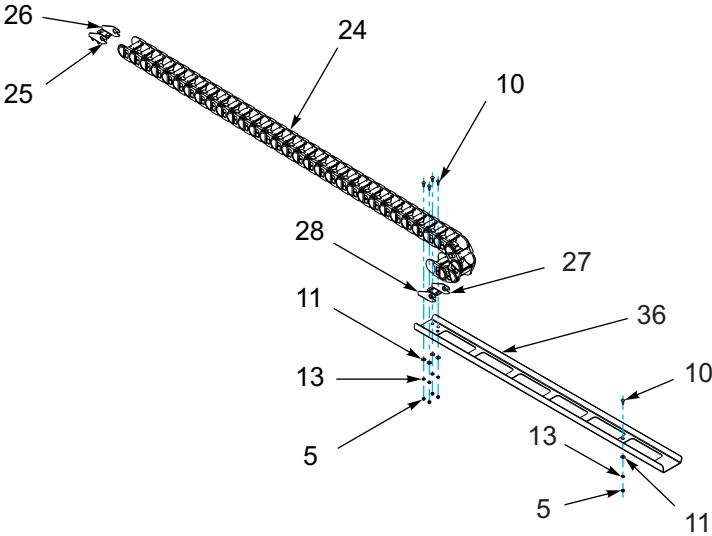
E-CHAIN ASSEMBLY
