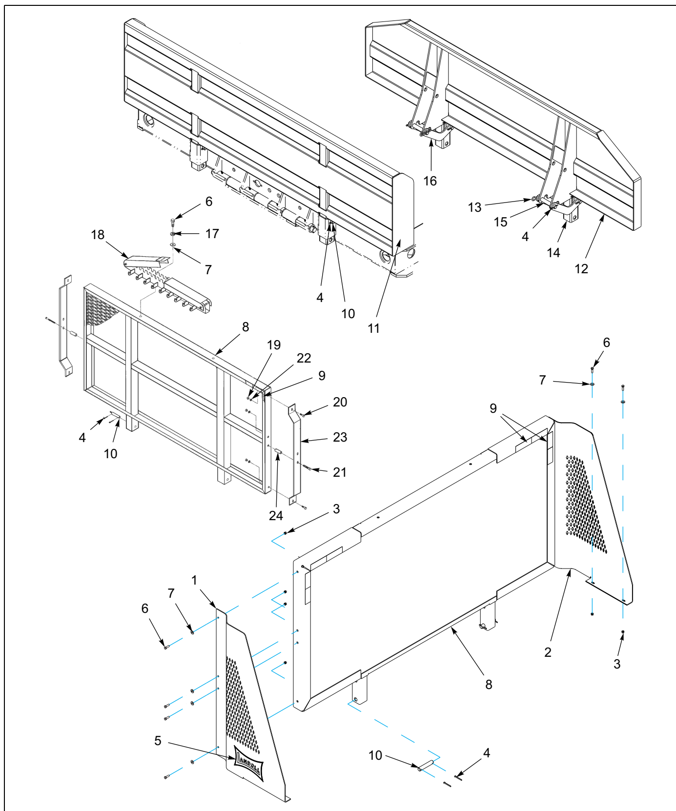
Figure 1-79: Bulkhead Assembly
