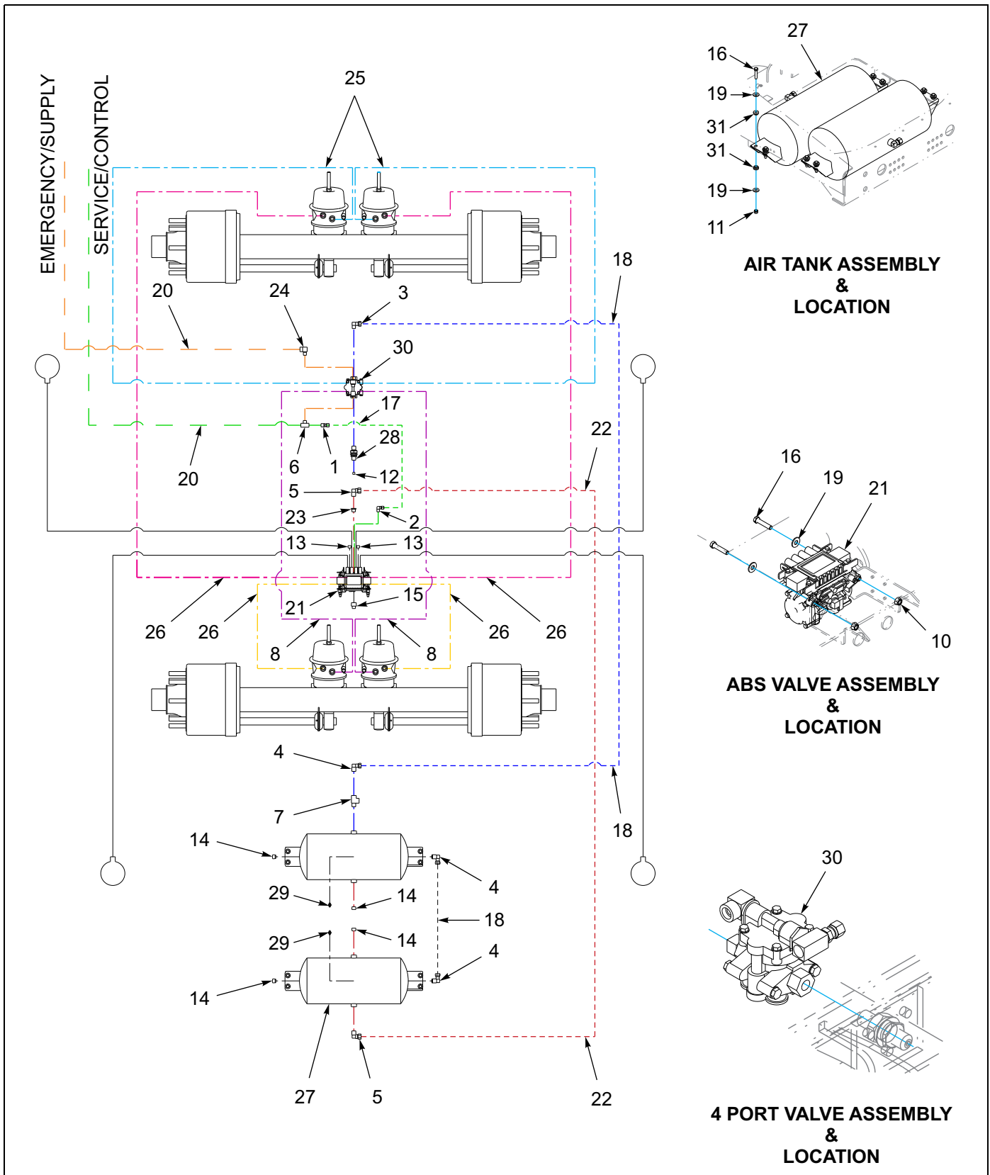
Figure 1-39: Air Brake System - 440A
