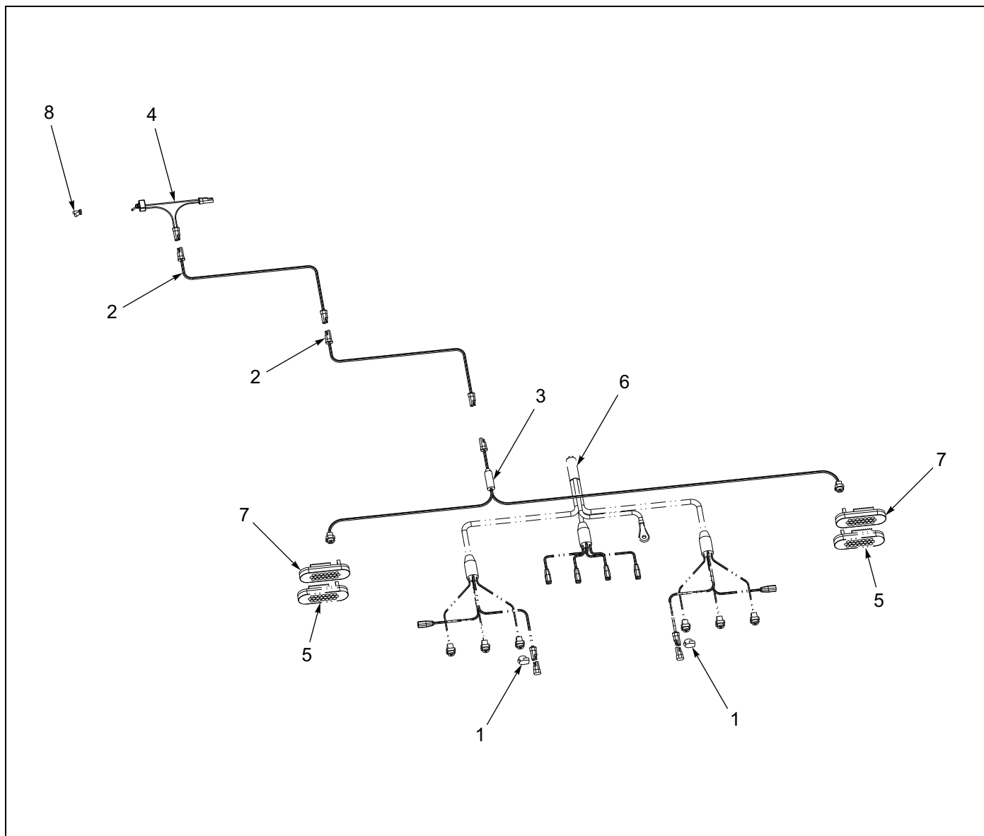
Figure 1-86: Bumper - Strobe Installation
