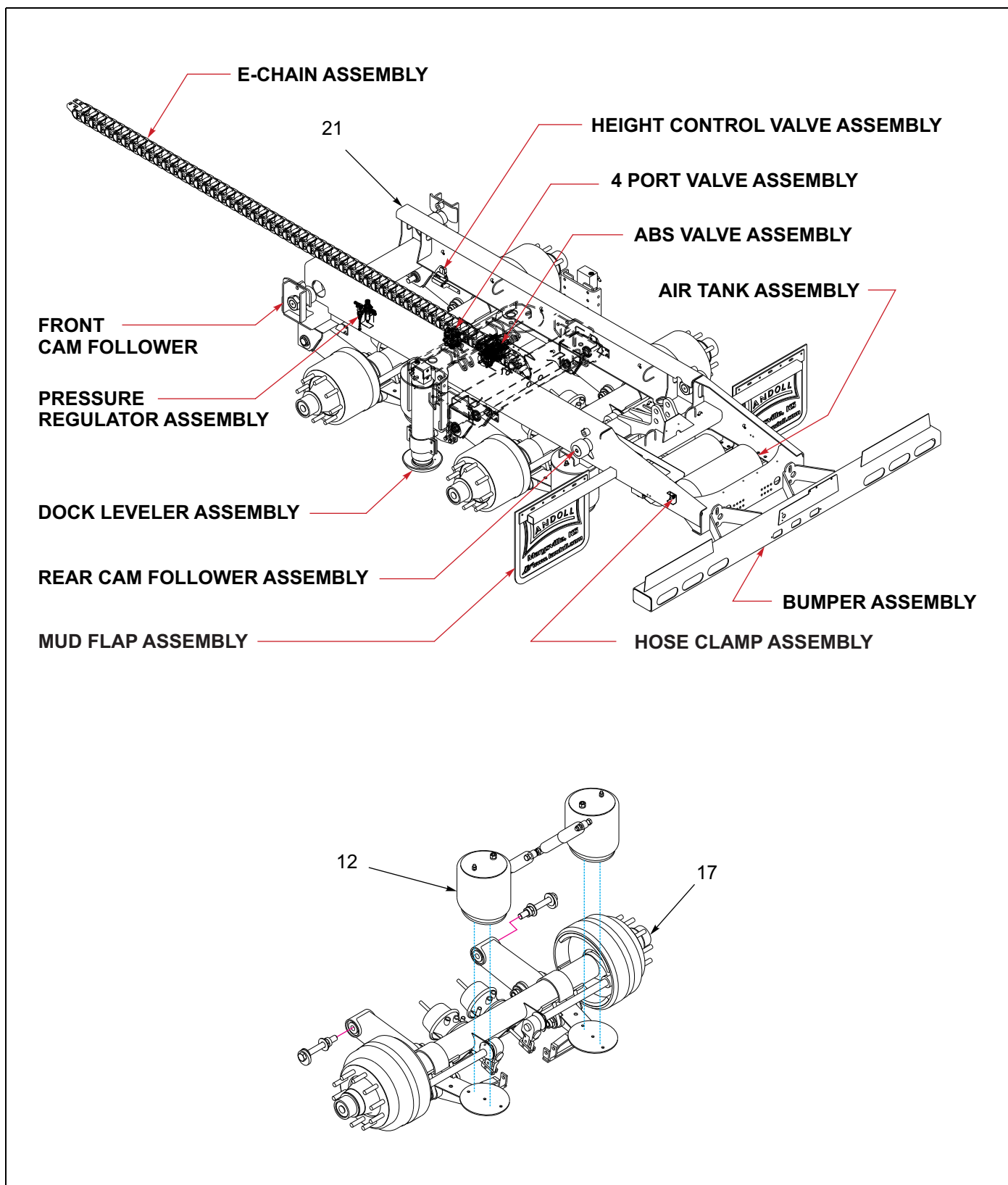
Figure 1-22: General Items - 440A (1 of 2)
