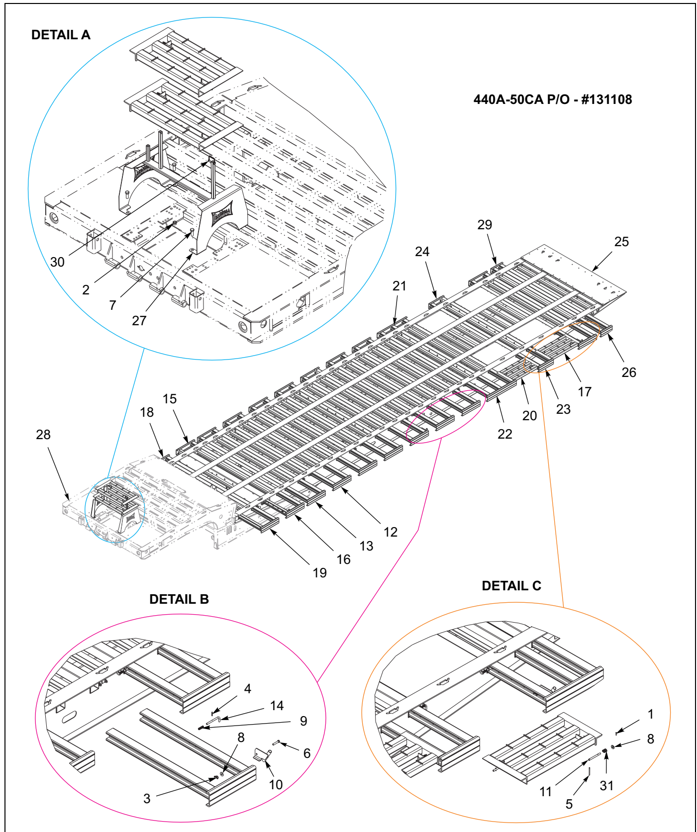
Figure 1-111: Pullout Extension Installation - 440A (1 of 2)
