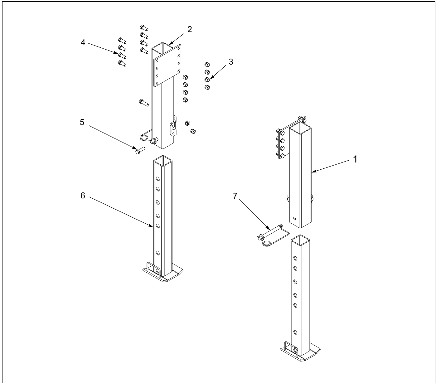
Figure 1-62: Landing Gear Installation - “Bolt On” Park Stand
