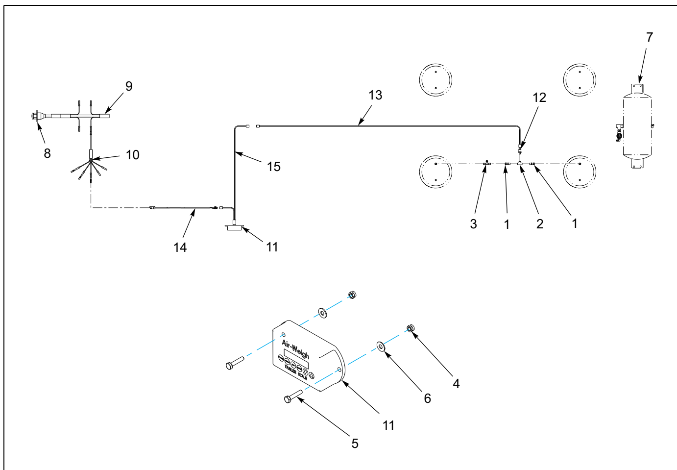
Figure 1-75: Air Digital Scale - Loadmaxx System
