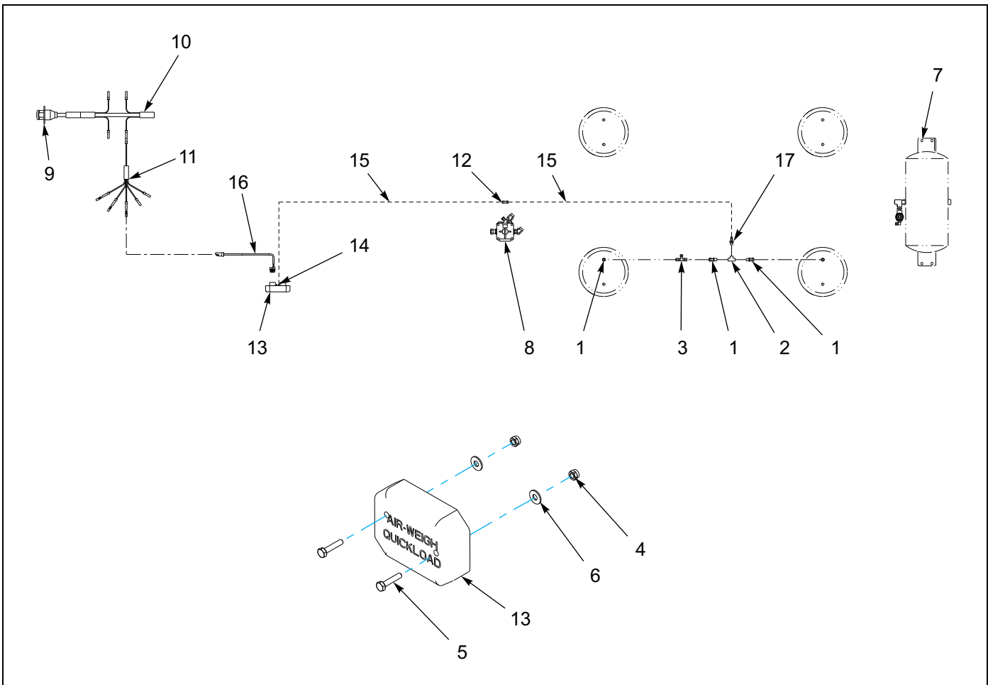
Figure 1-77: Air Digital Scale - Quickload System
