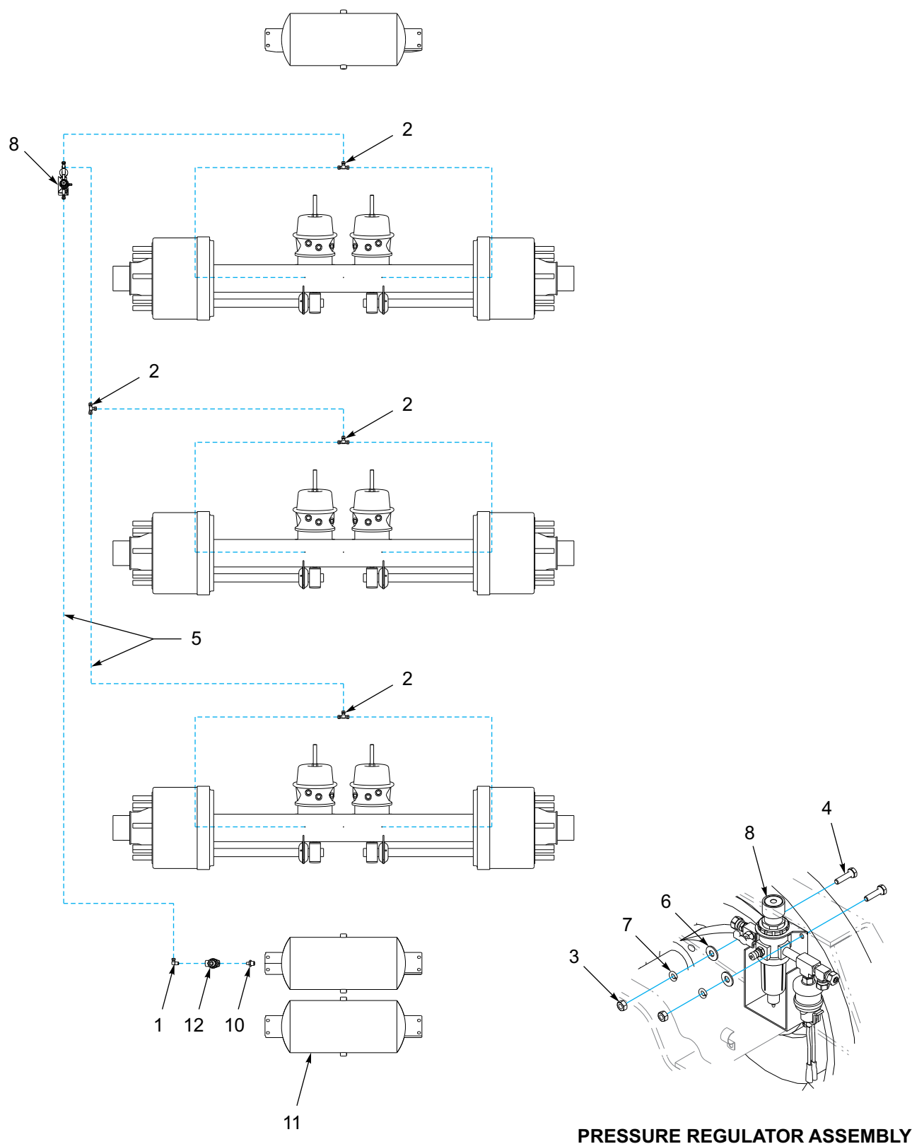
Figure 1-44: Tire Inflation System - 455A Spring Brake
