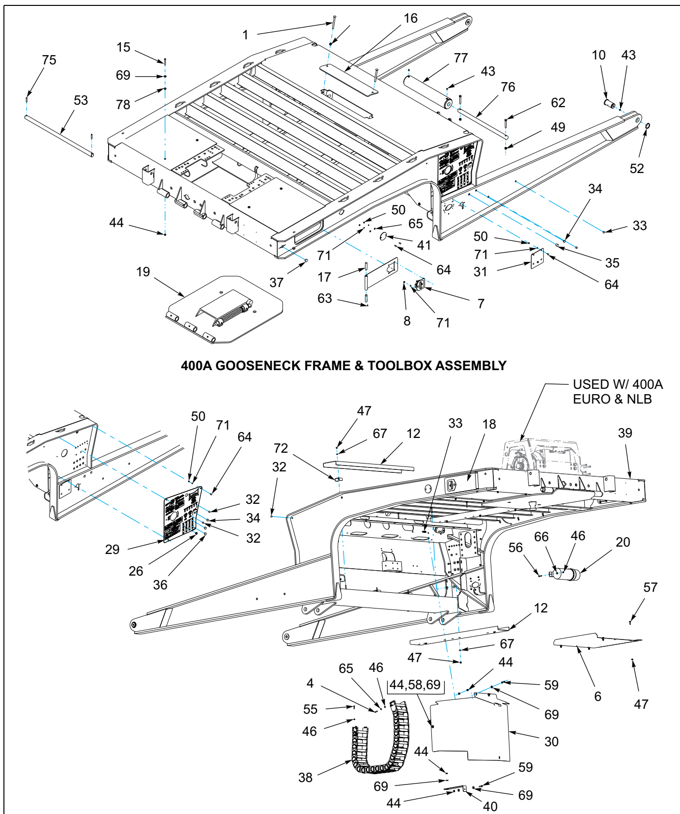
Figure 1-5: Upper Deck Assembly (1 of 2)
