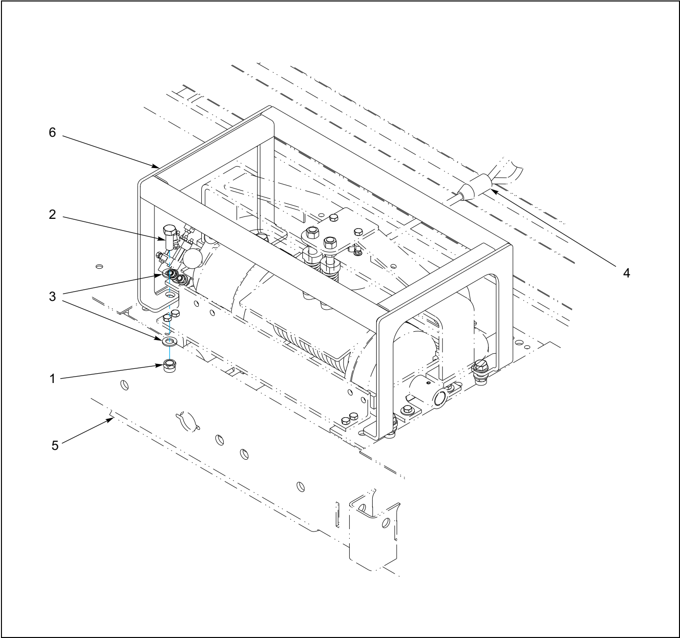
Figure 1-133: Guard Installation, Winch 20K Pivot
