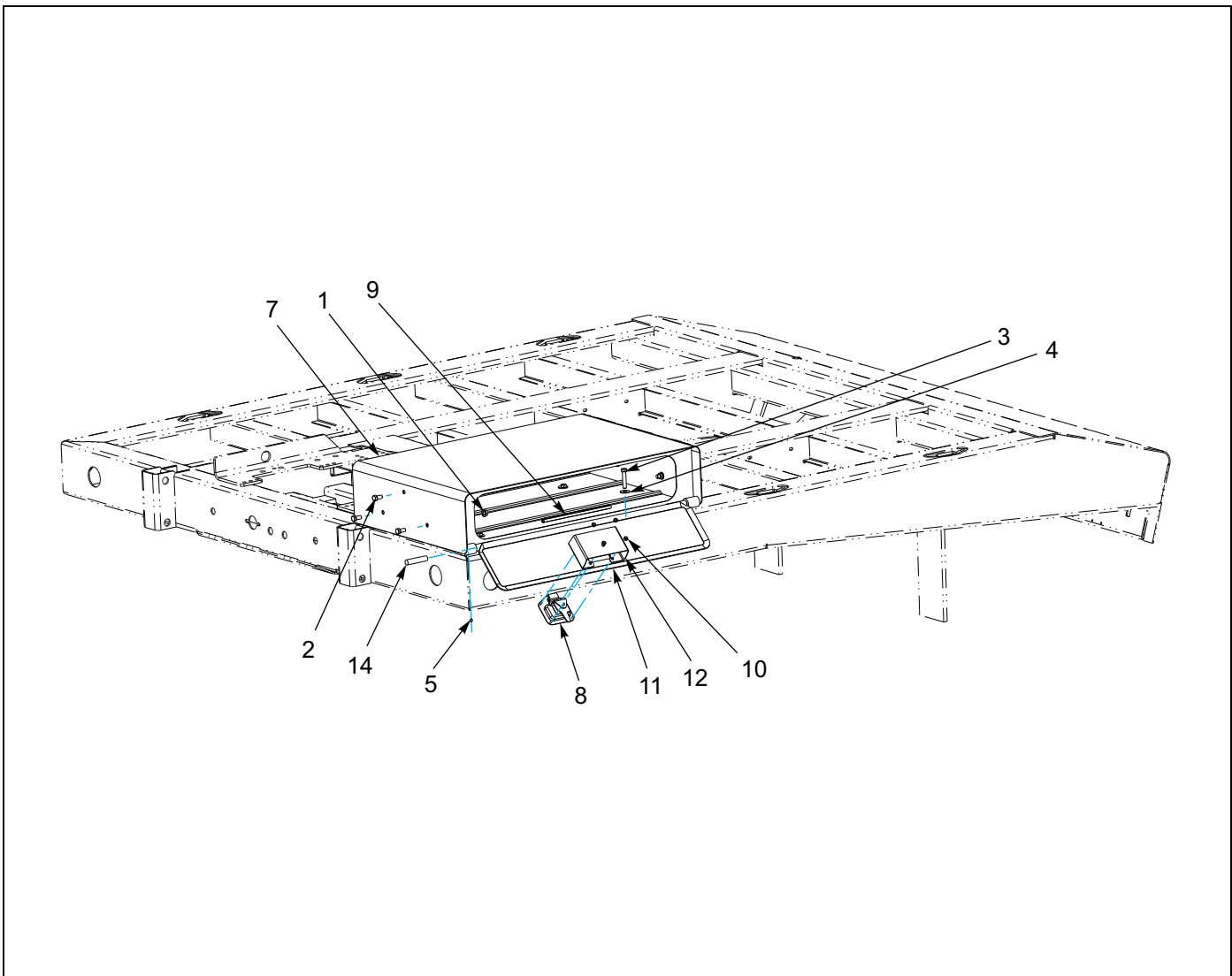
Figure 1-129: Upper Deck - Toolbox Installation
