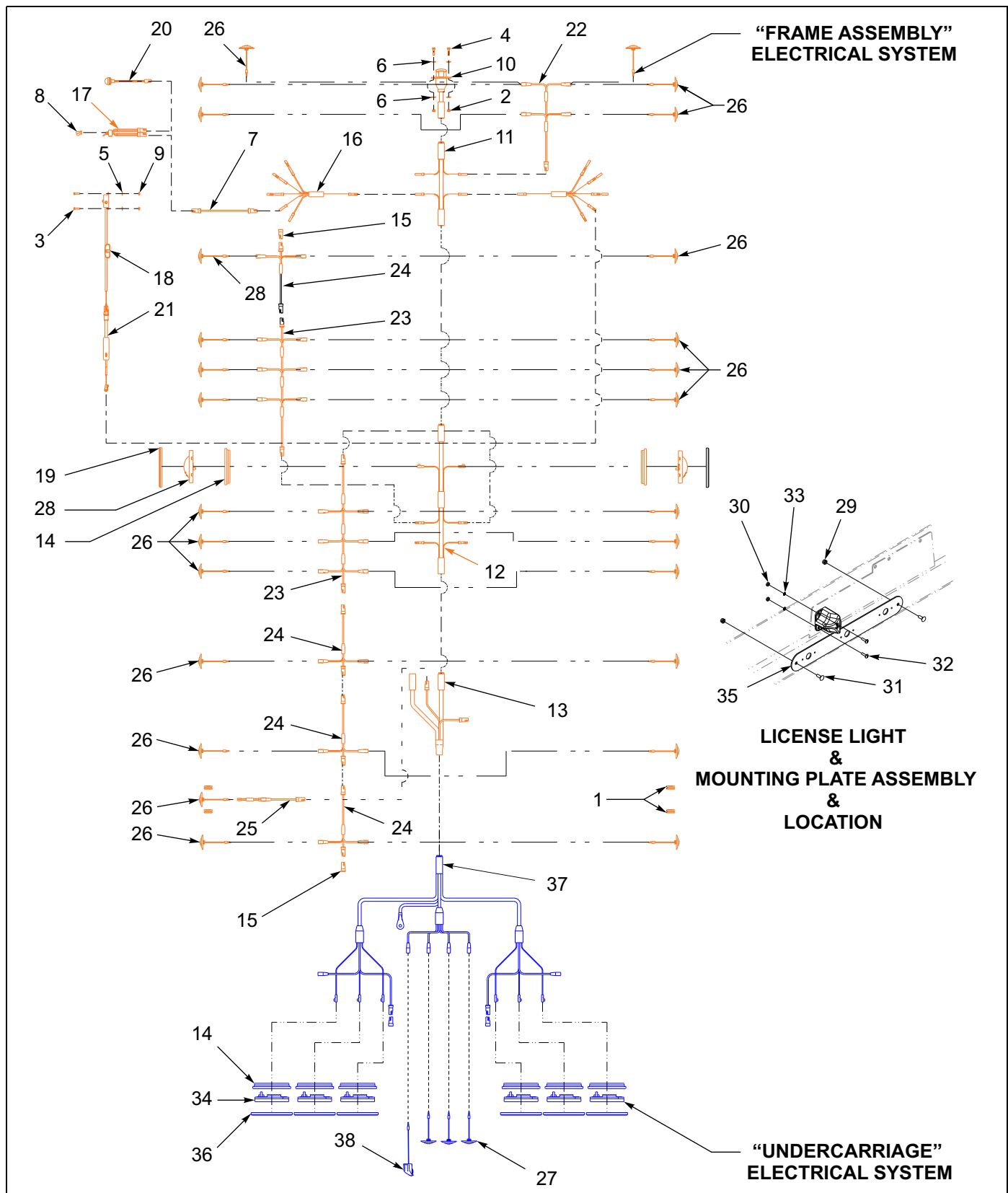
Figure 1-20: Electrical System
