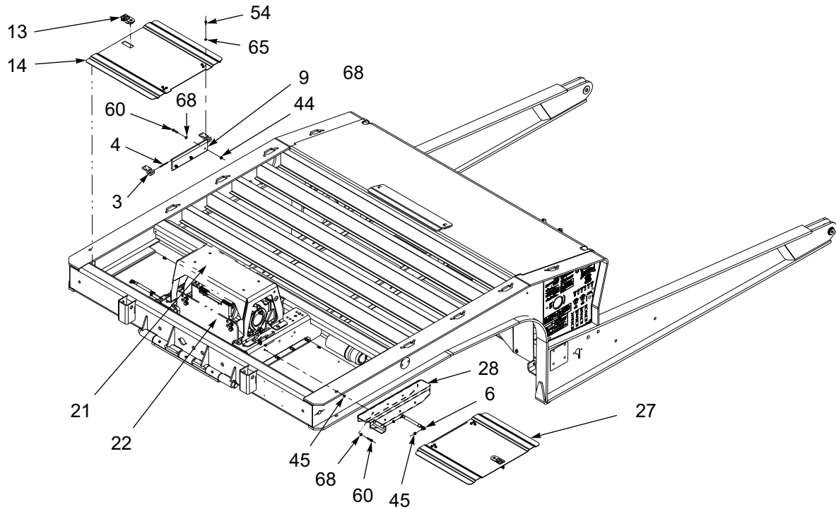
400A EURO GOOSENECK FRAME & TOOLBOX ASSEMBLY
