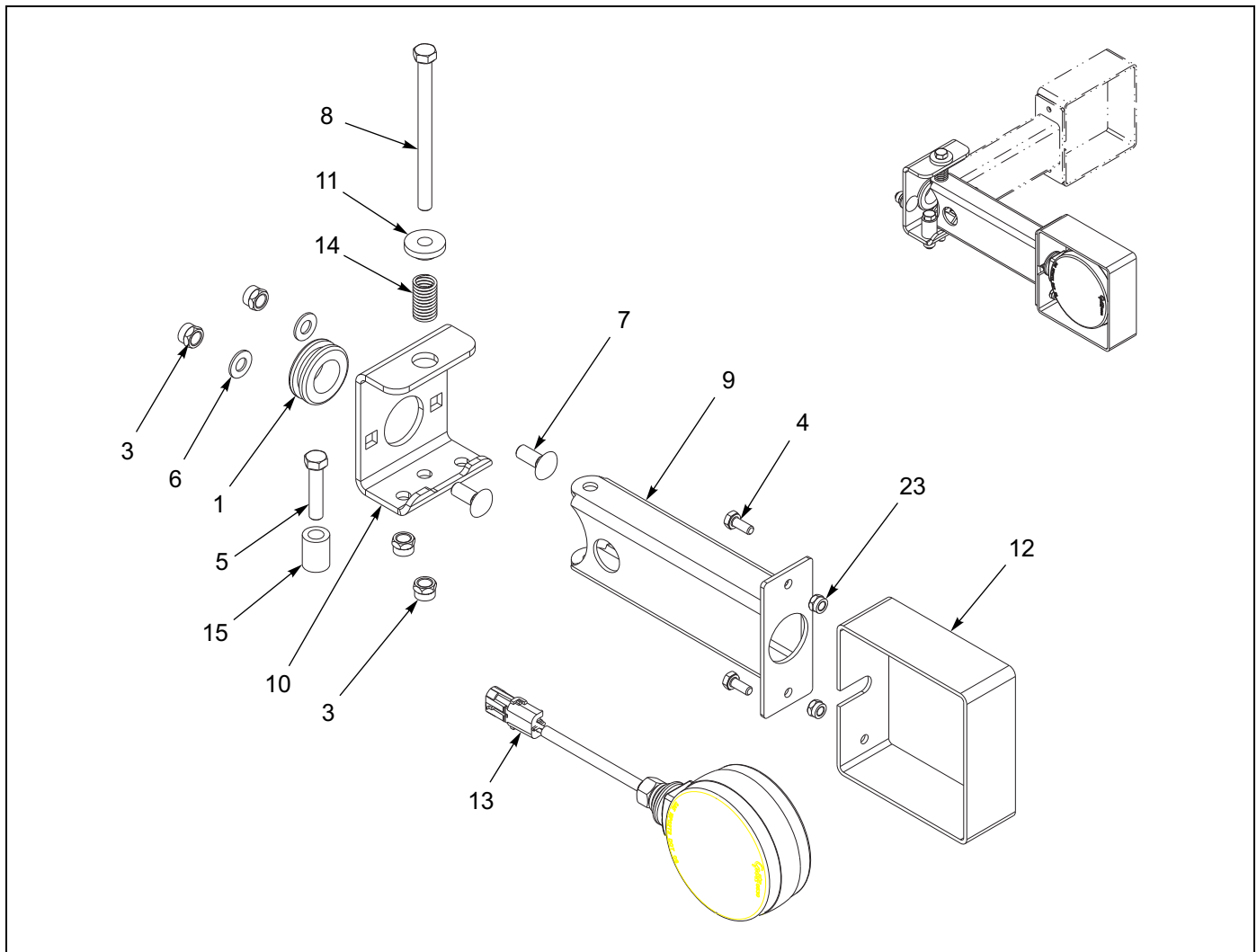
Figure 1-106: Swing-Arm Light Assembly - Turn Signal/Emergency Flasher
