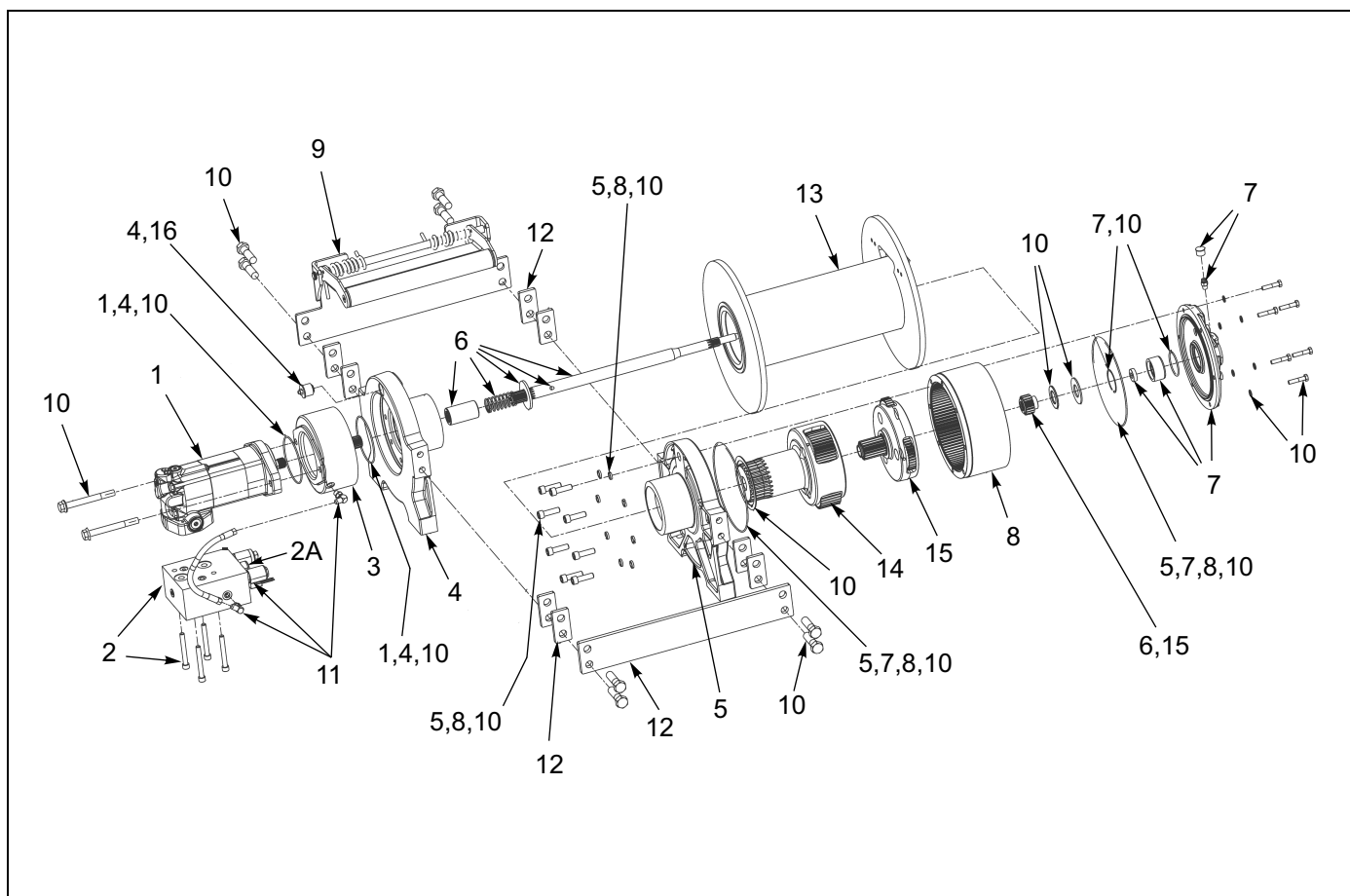
Figure 1-61: Winch Items - 30K 2 Speed (WARN)
