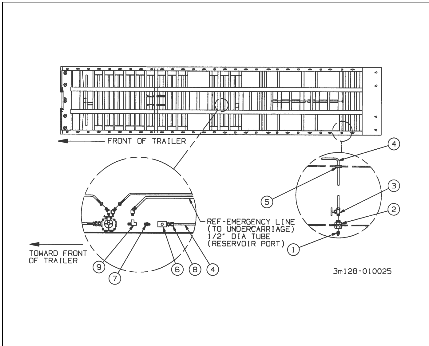
Figure 1-137: Air Outlet Accessory
