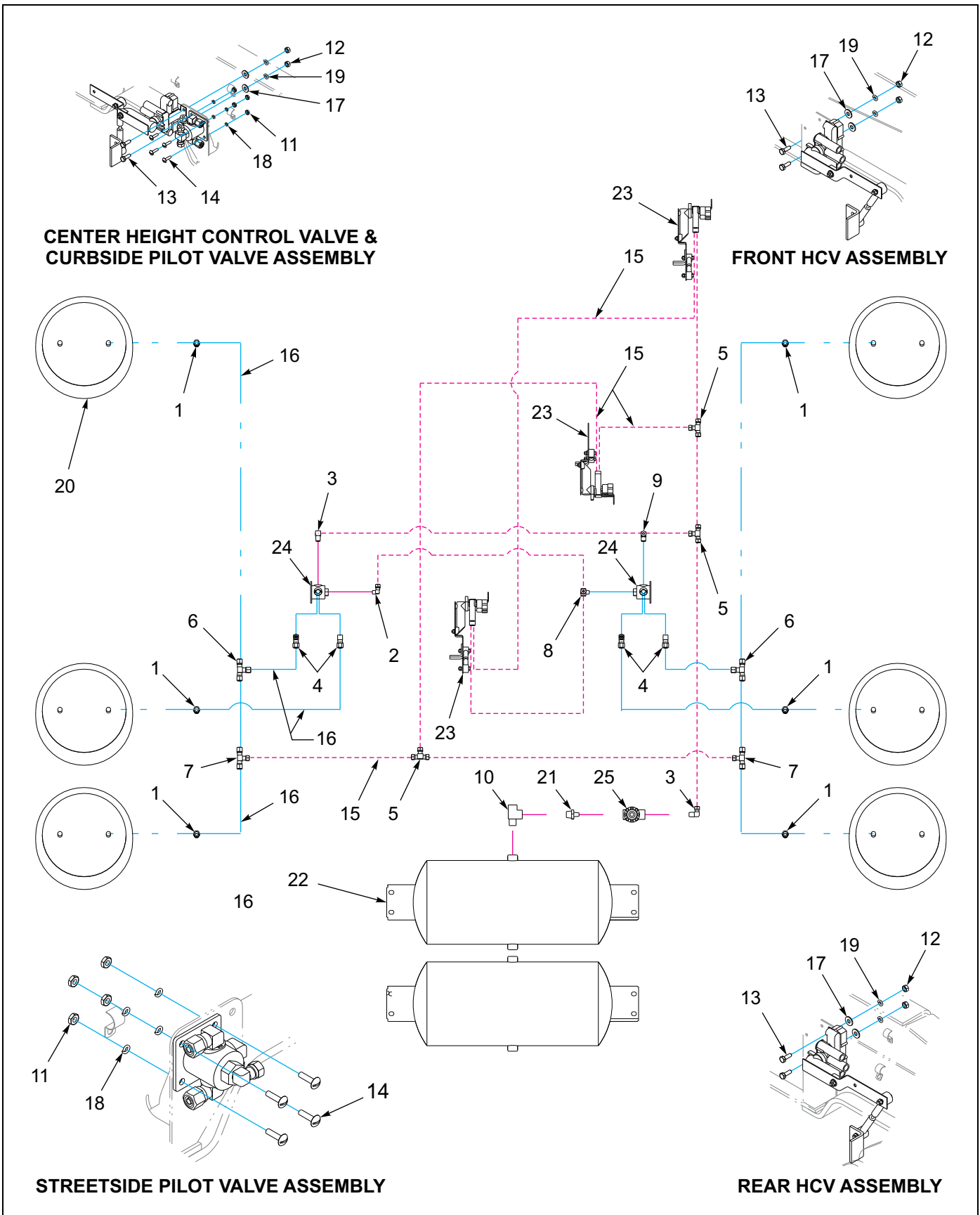
Figure 1-31: Air Ride Suspension - 455A
