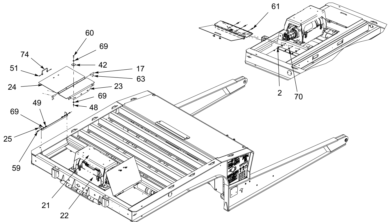
400A NLB GOOSENECK FRAME & TOOLBOX ASSEMBLY
