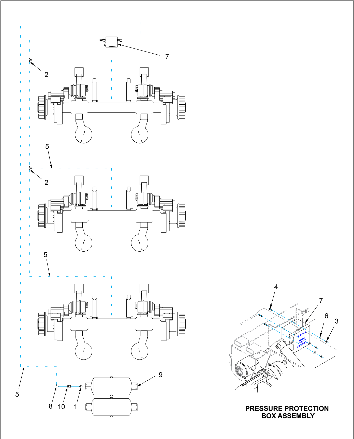
Figure 1-45: Tire Inflation System - 455A Disc Brake
