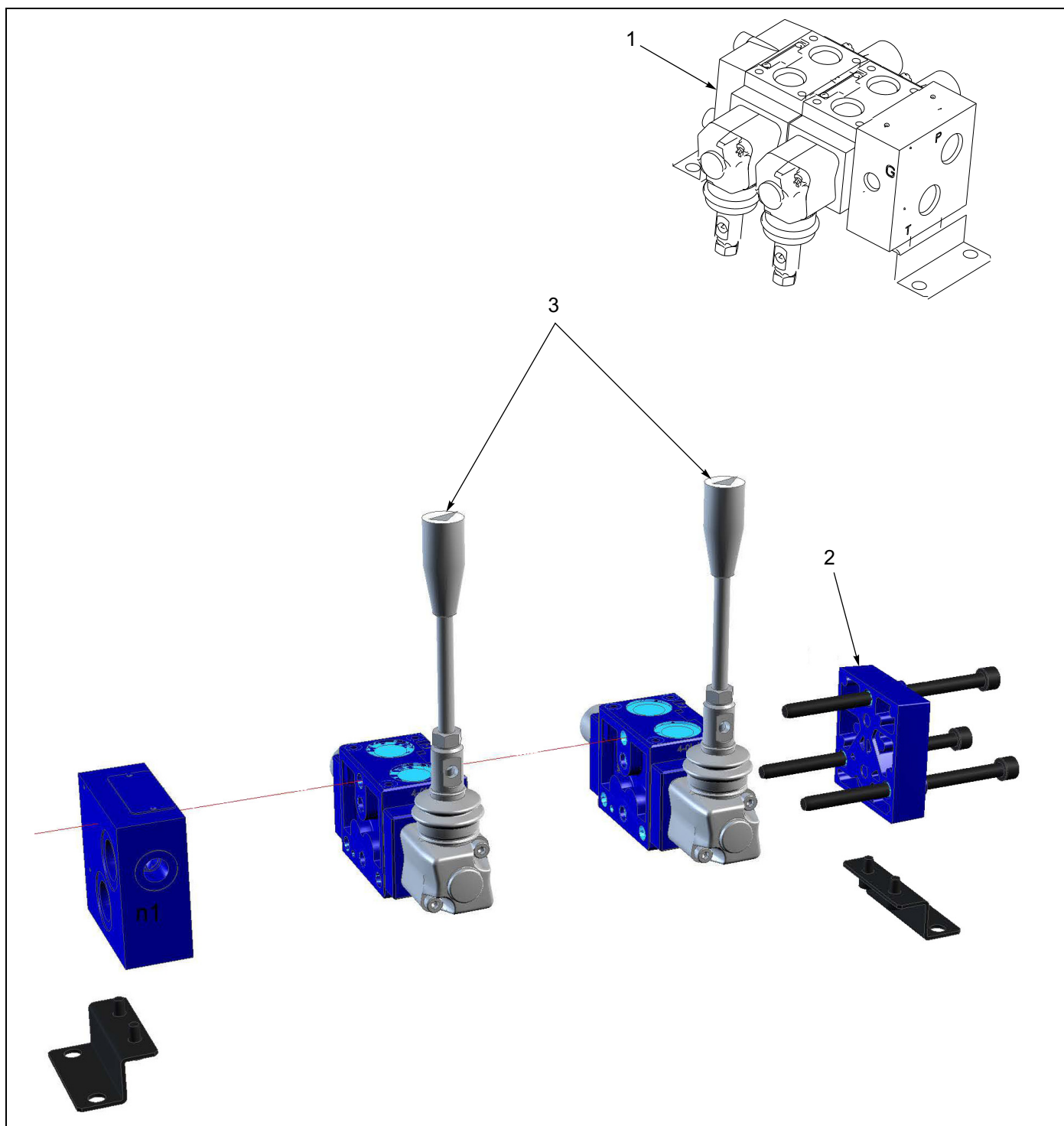
Figure 1-74: Dock Leveler Valve
