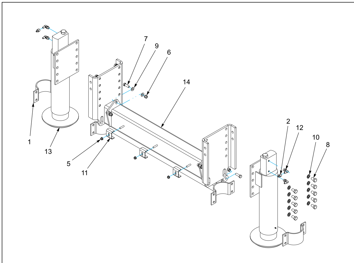
Figure 1-70: Dock Leveler Assembly - Single 60K (Euro)
