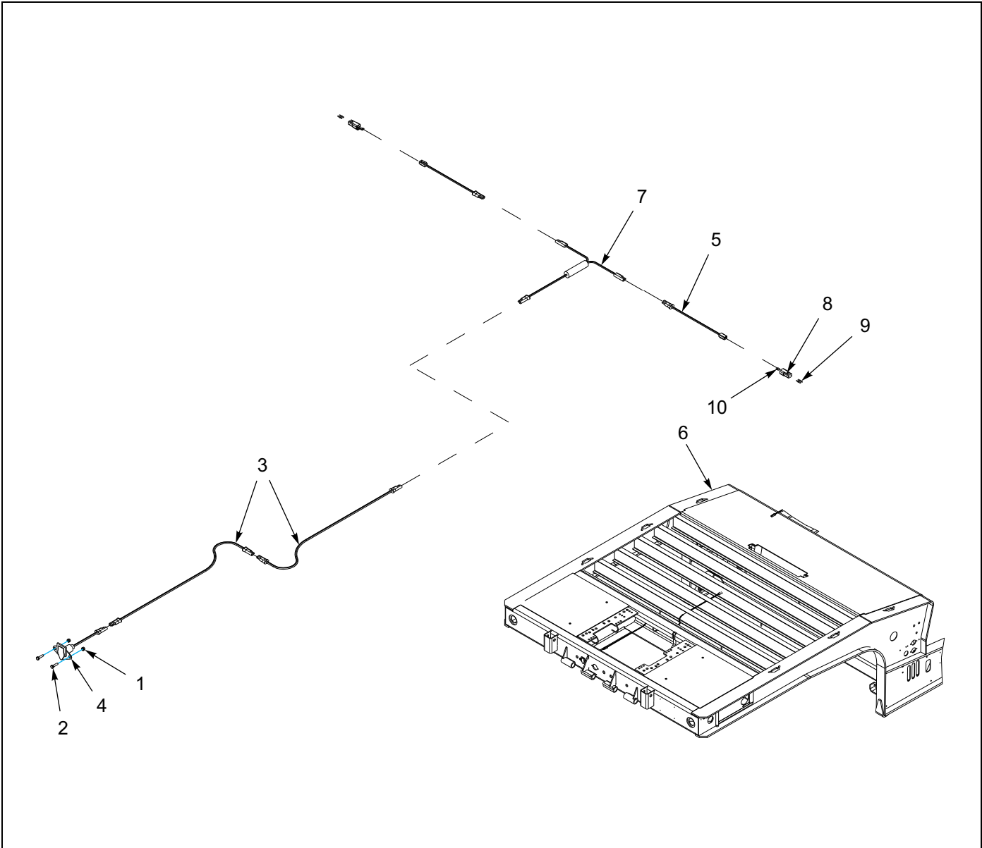
Figure 1-143: Front/Rear Harness Installation
