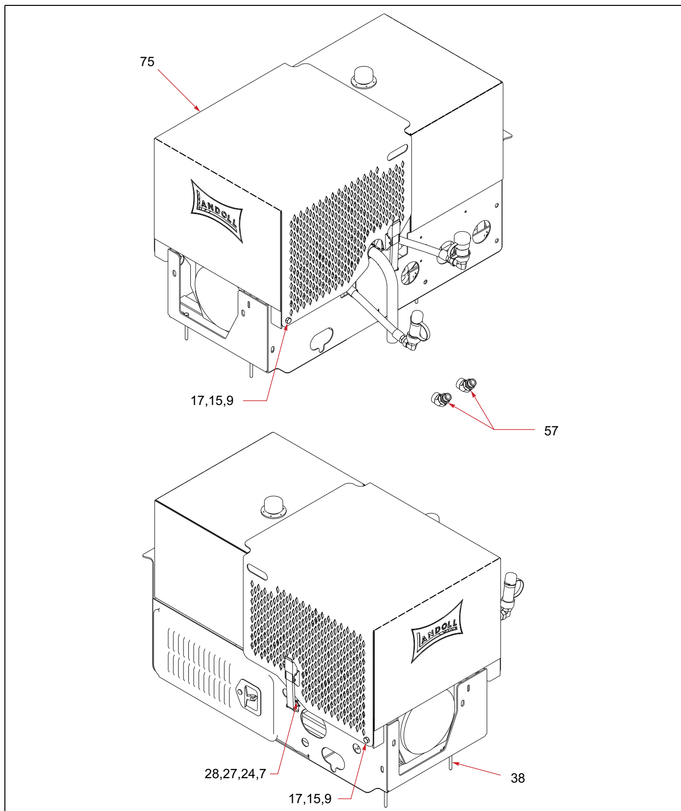
Figure 1-90: Engine - 25 HP Upper Deck Package (1 of 4)
