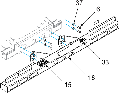
BUMPER ASSEMBLY
