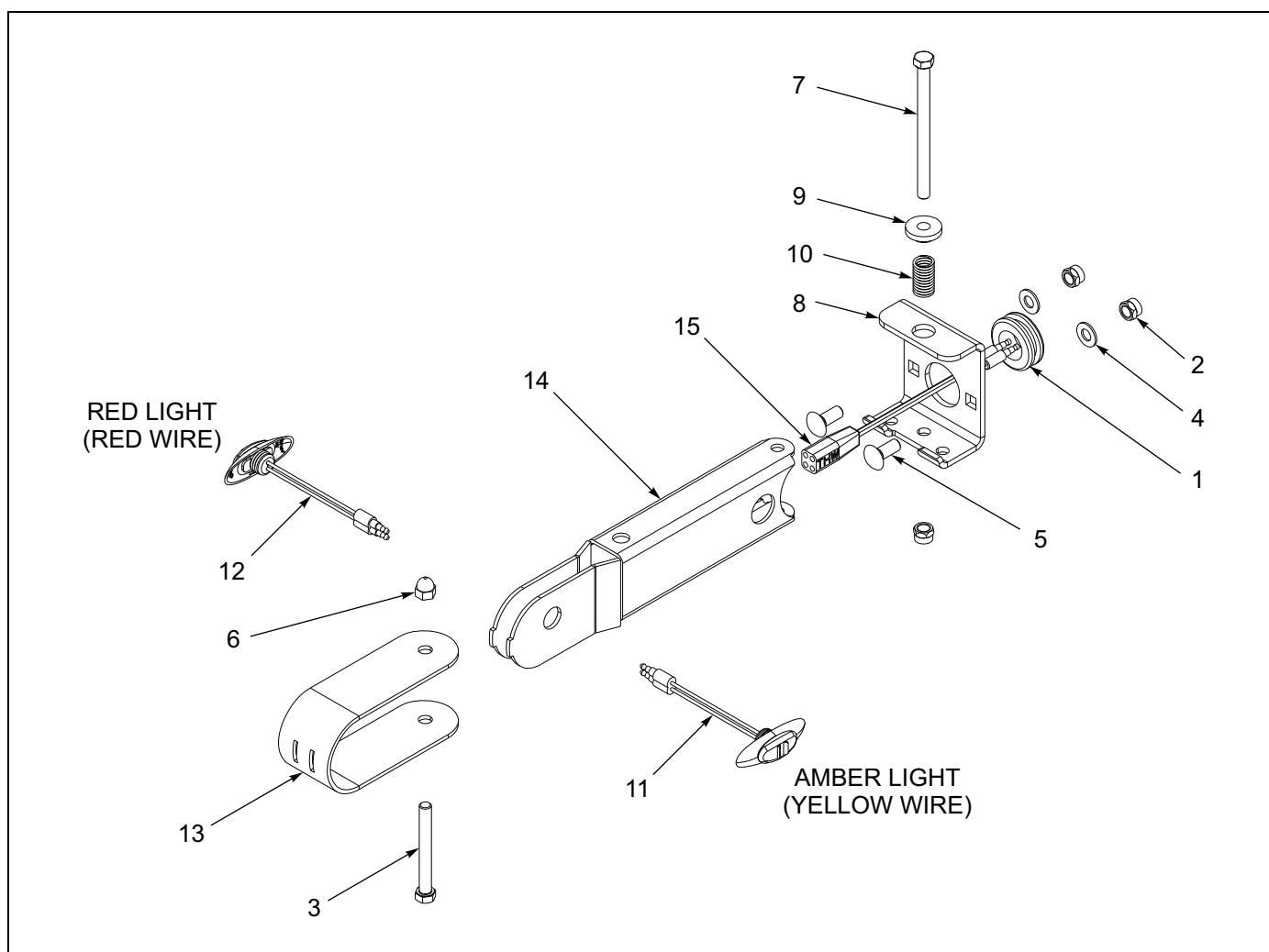
Figure 1-109: Swing-Arm Light Assembly - CURB
