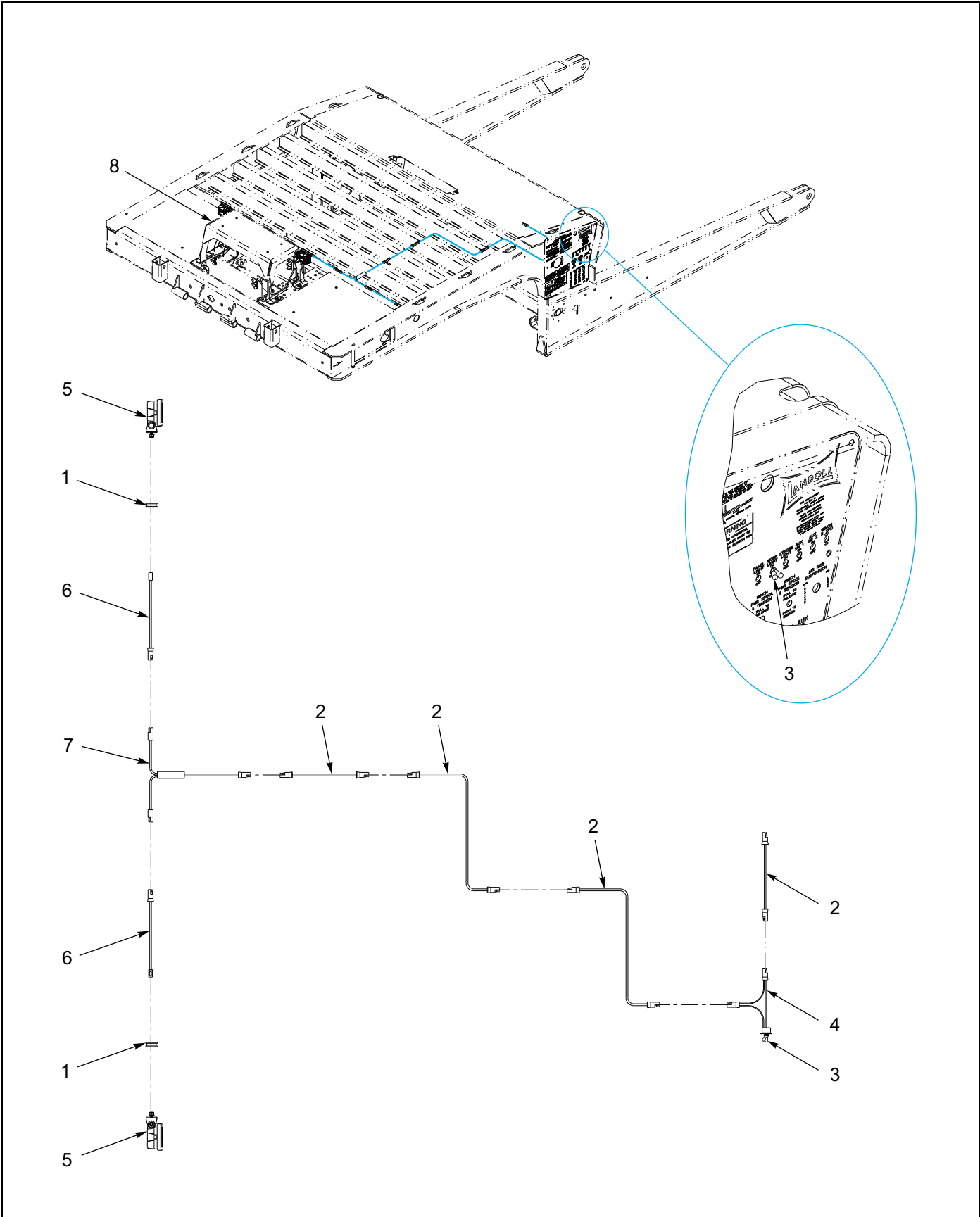
Figure 1-136: Winch - Work Light Installation
