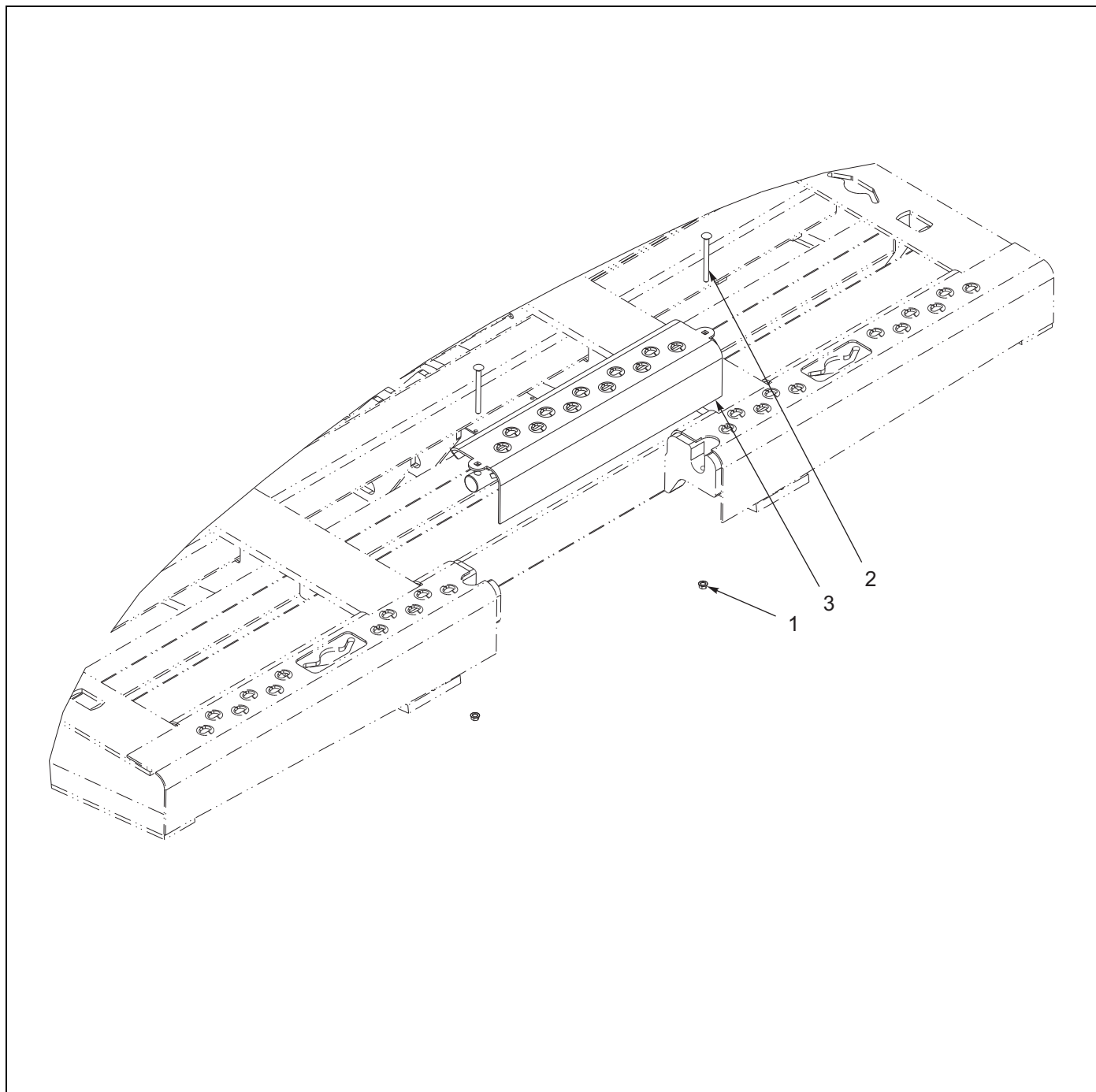
Figure 1-138: Center Rub Plate Cover Installation
