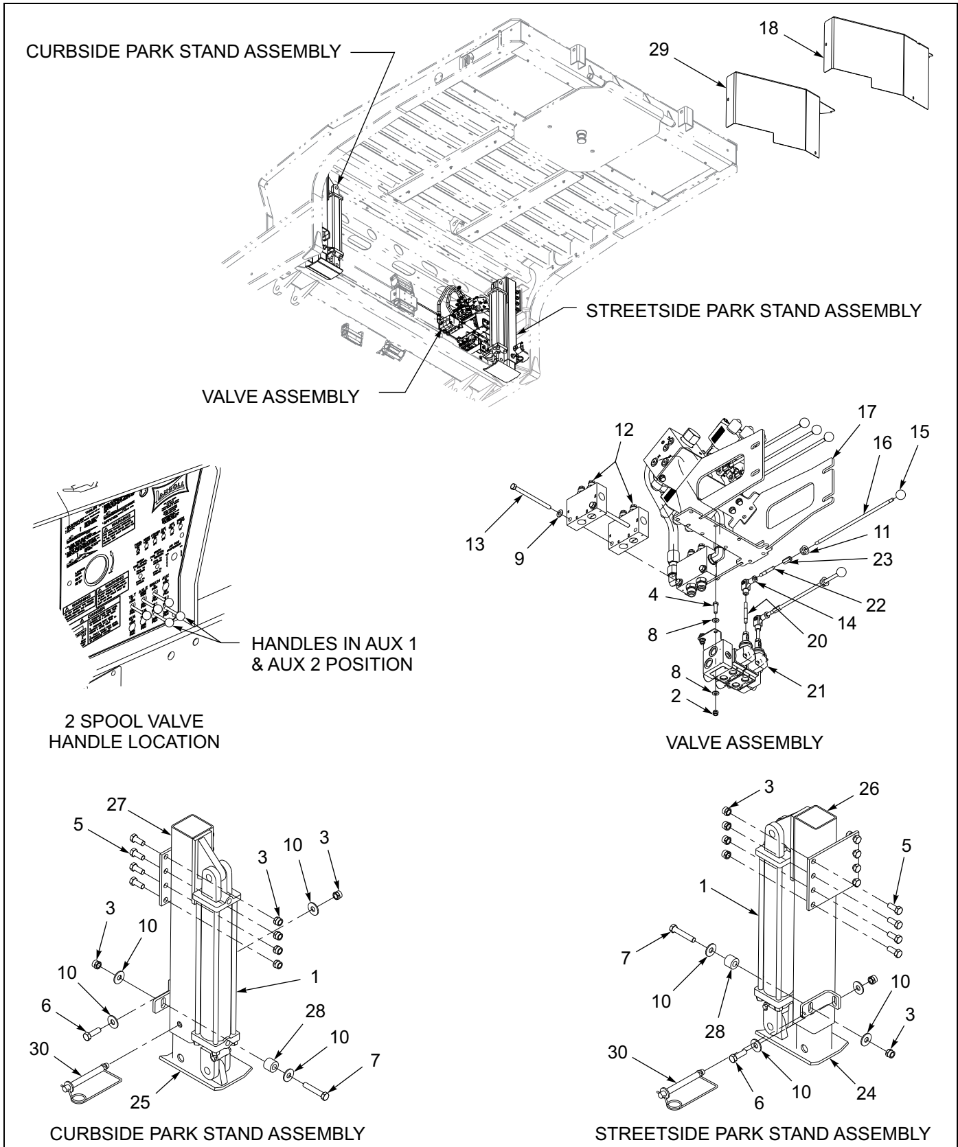
Figure 1-100: Hydraulic Park Stand - General Items
