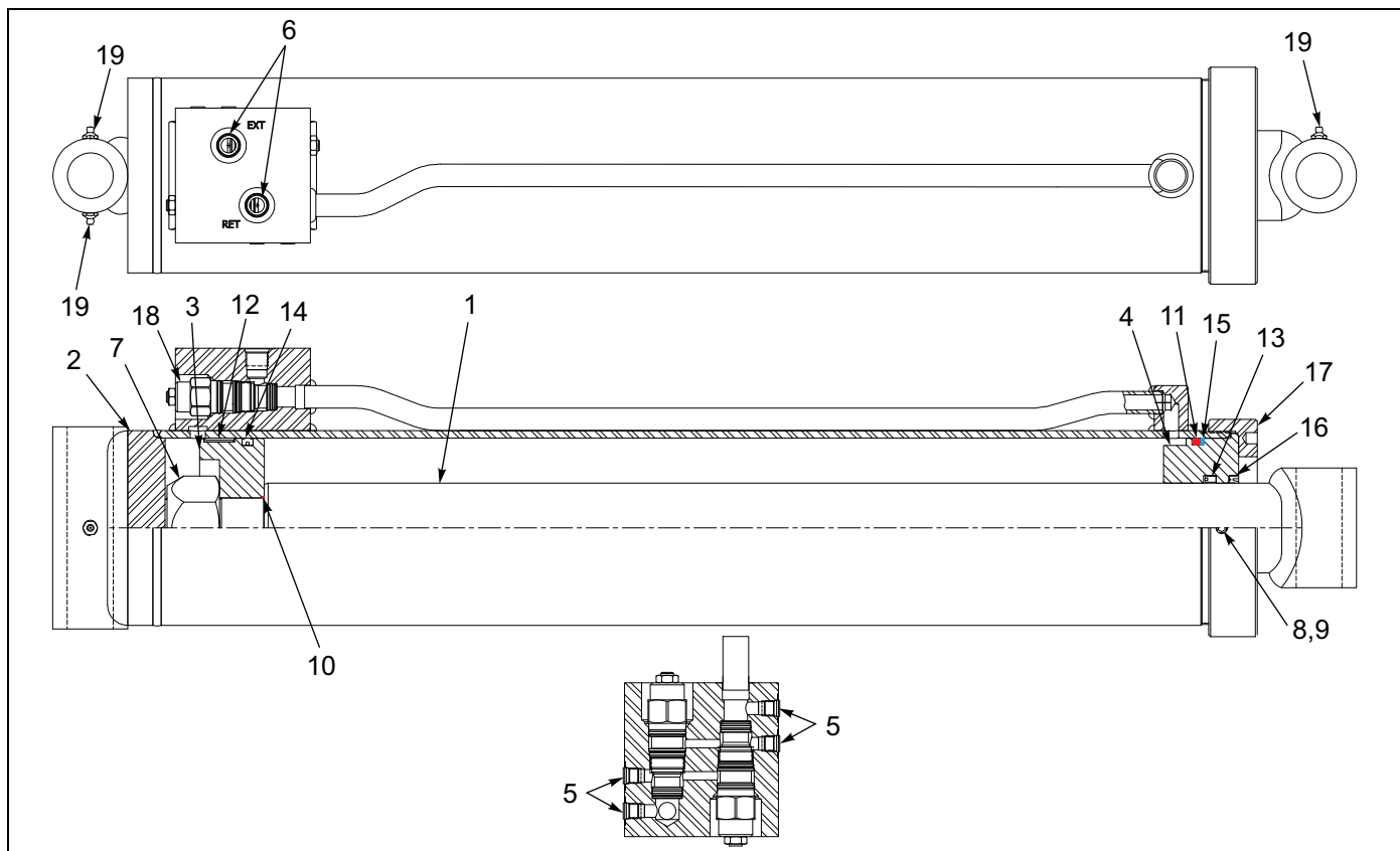
Figure 1-15: Cylinder - 6 X 30
