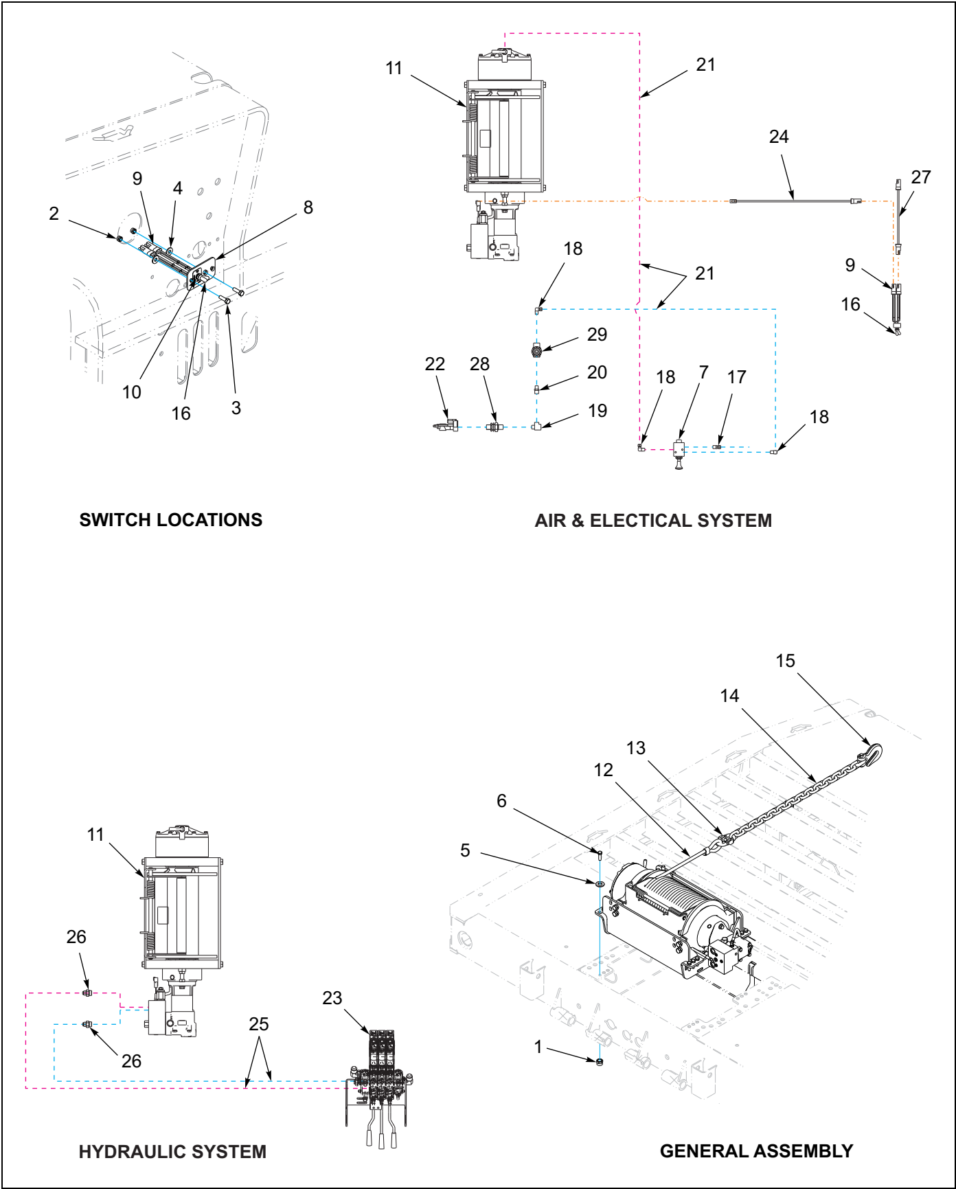
Figure 1-60: Winch Installation - 30K 2 Speed (WARN)
