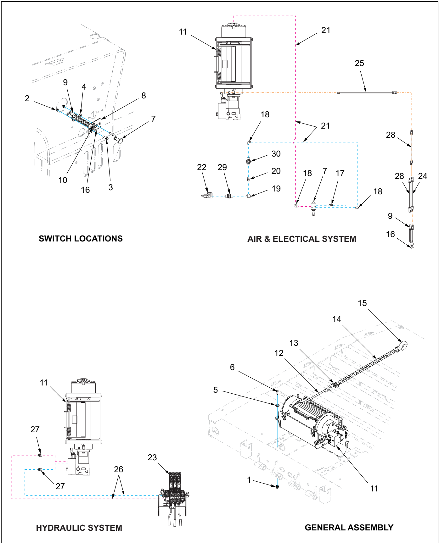
Figure 1-58: Winch Installation - 20K 2 Speed (WARN)
