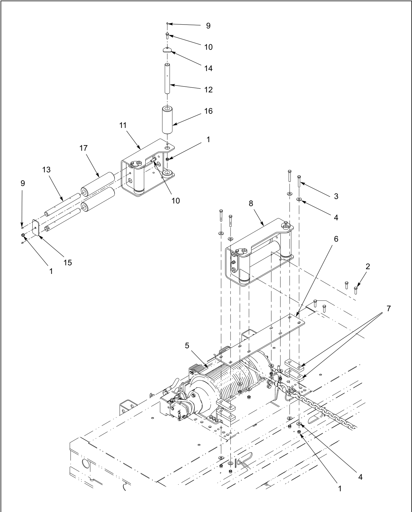
Figure 1-118: 4 Roller Guide Installation - 20K/30K (WARN)
