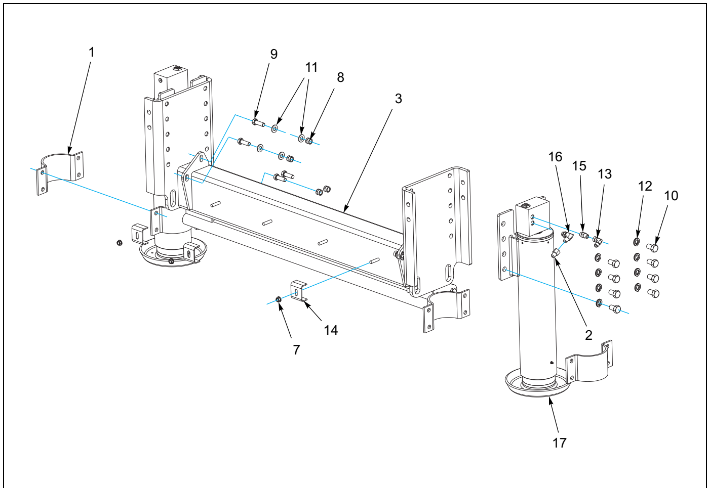
Figure 1-68: Dock Leveler Assembly - Single 60K (Arctic)
