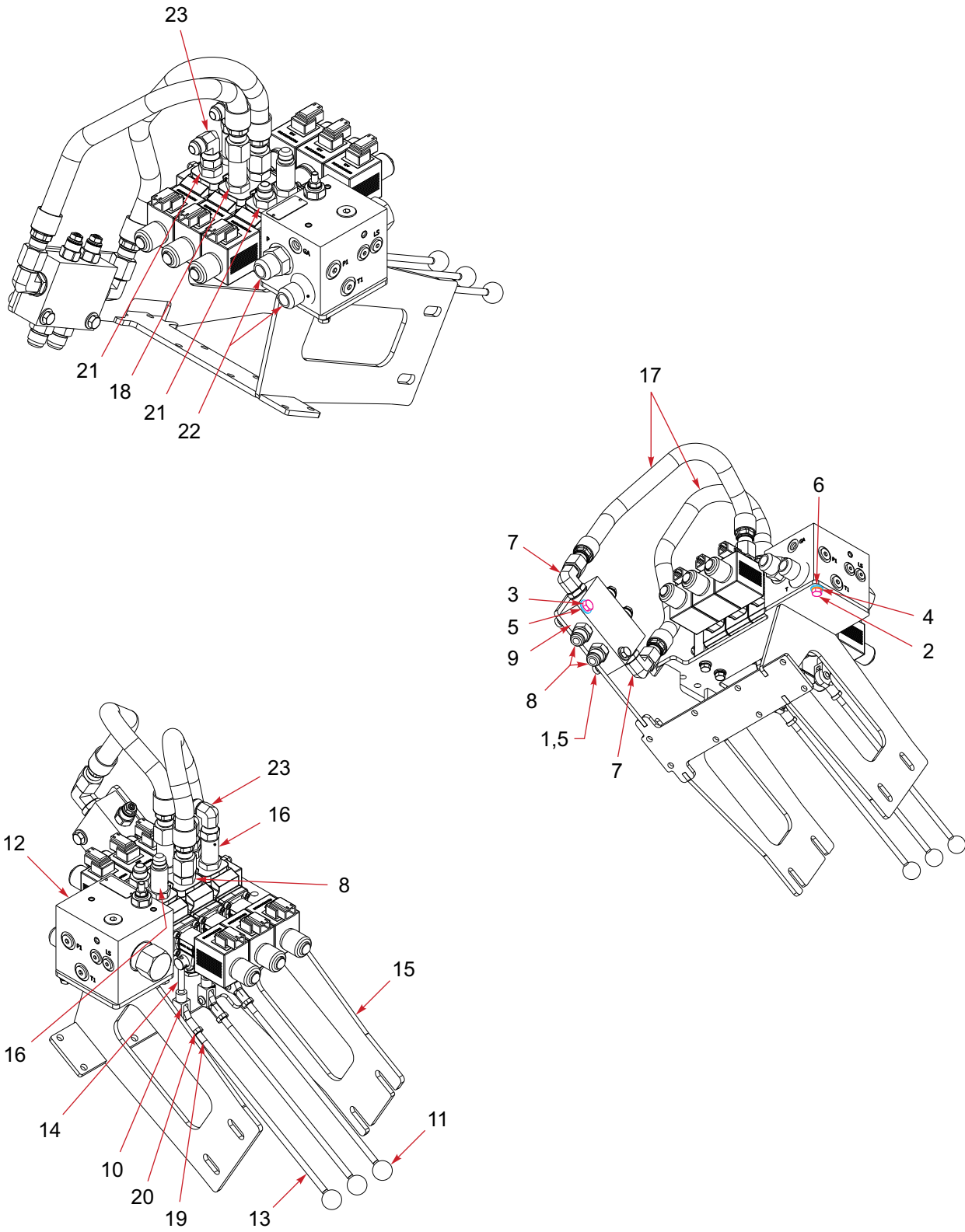
Figure 1-18: Valve Assembly - Three Spool
