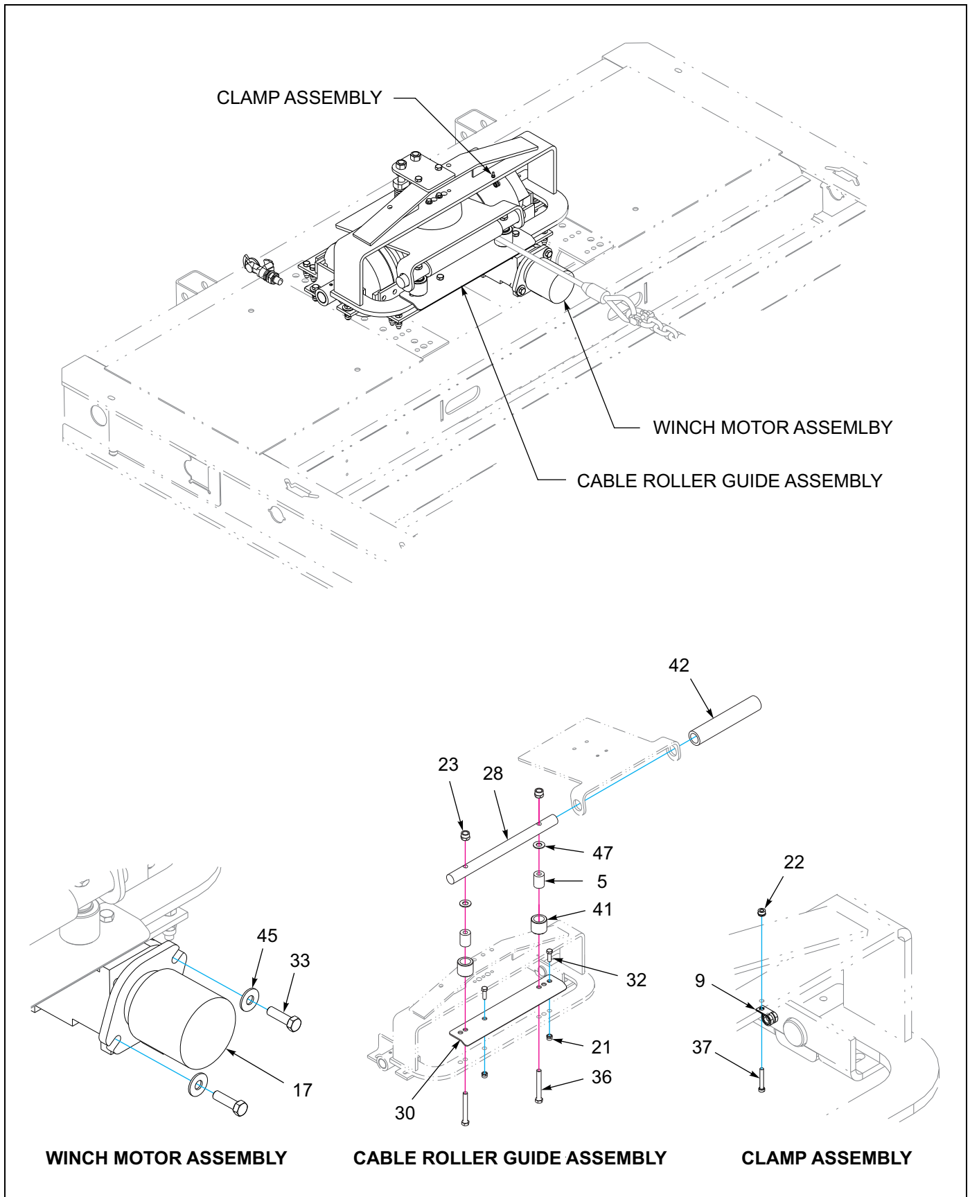
Figure 1-53: Winch Installation - 20K Air Tension/Release (BRADEN) (2 of 3)
