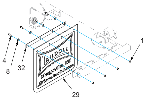
MUDFLAP ASSEMBLY
