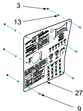
PLACARD ASSEMBLY
