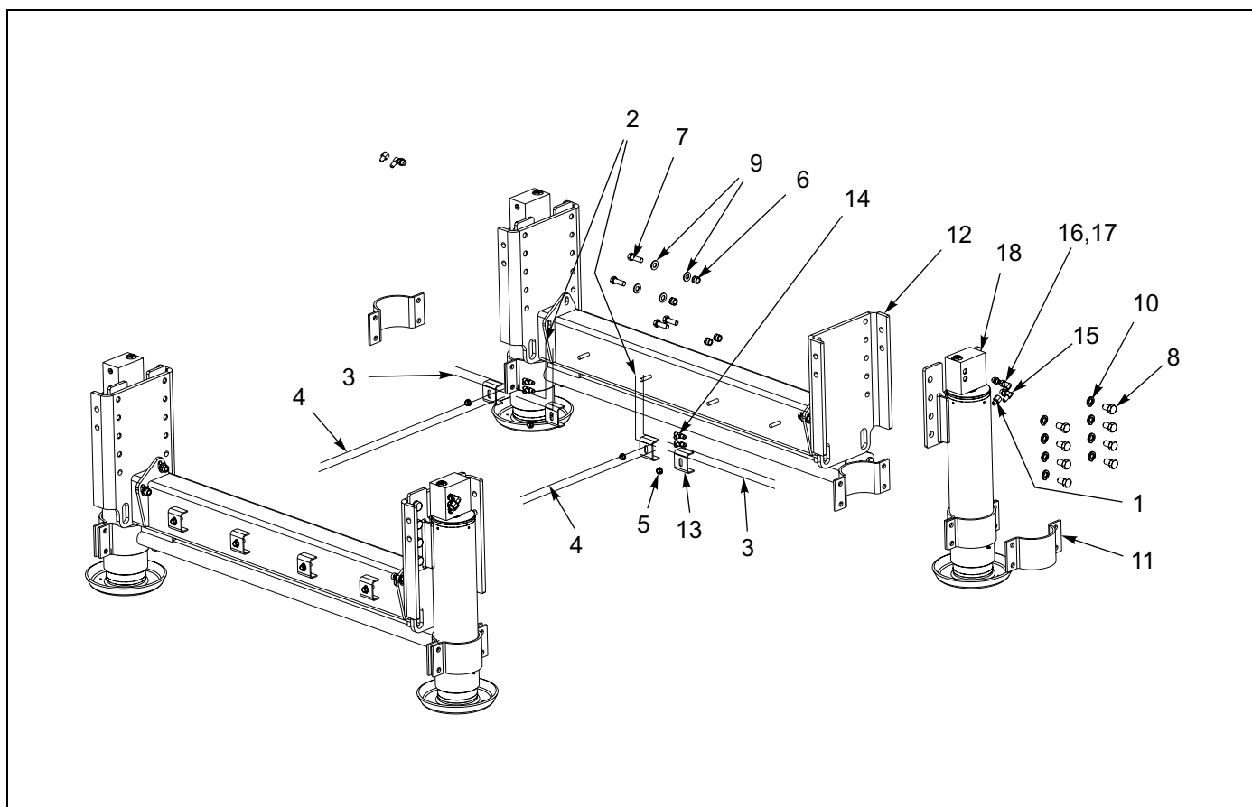
Figure 1-71: Dock Level Assembly - Single 120K
