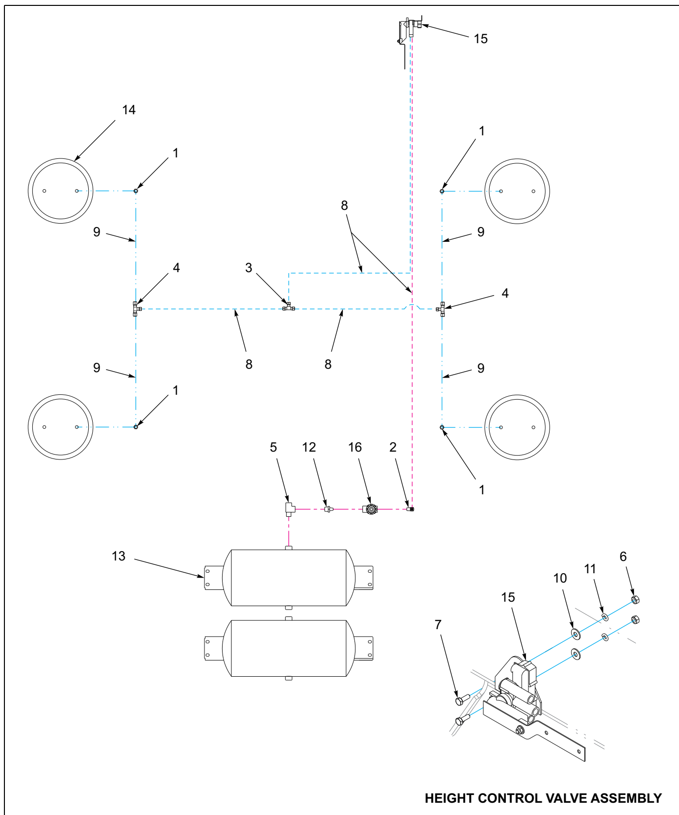
Figure 1-30: Air Ride Suspension - 440A
