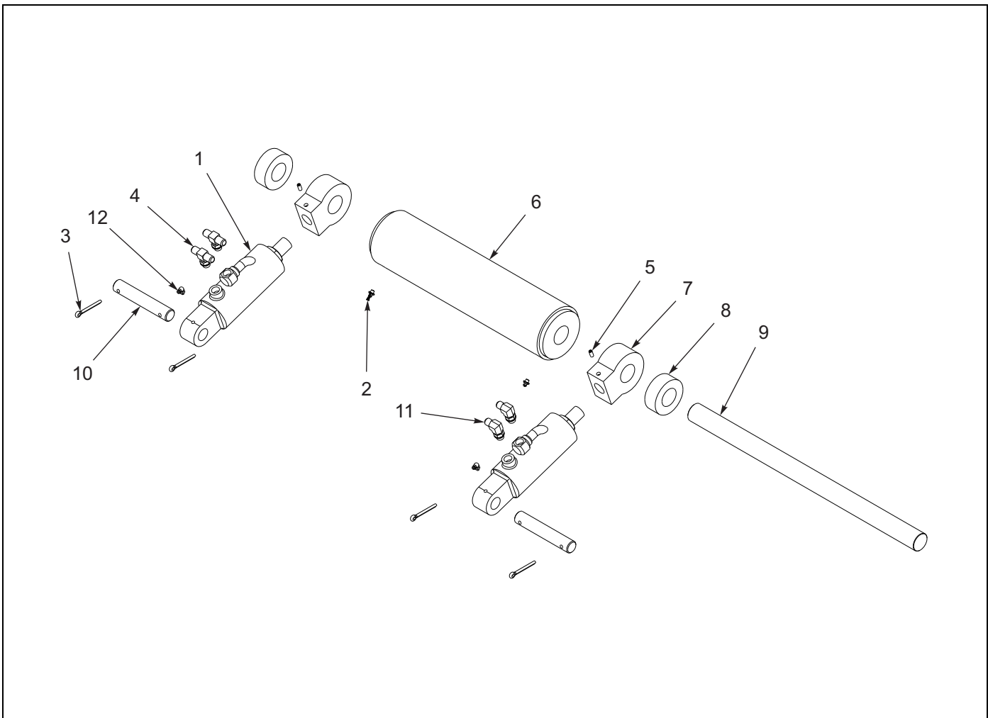
Figure 1-121: Pop-Up Roller Installation
