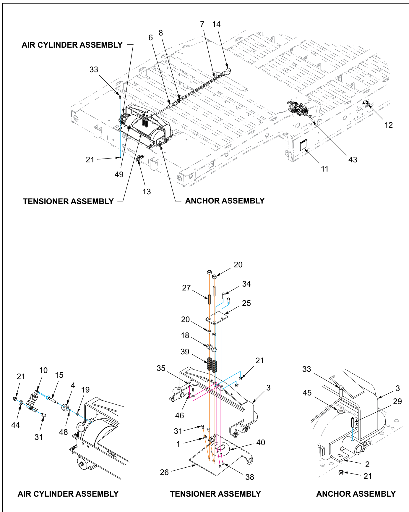
Figure 1-52: Winch Installation - 20K Air Tension/Release (BRADEN) (1 of 3)
