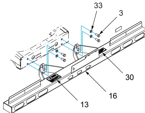
BUMPER ASSEMBLY
