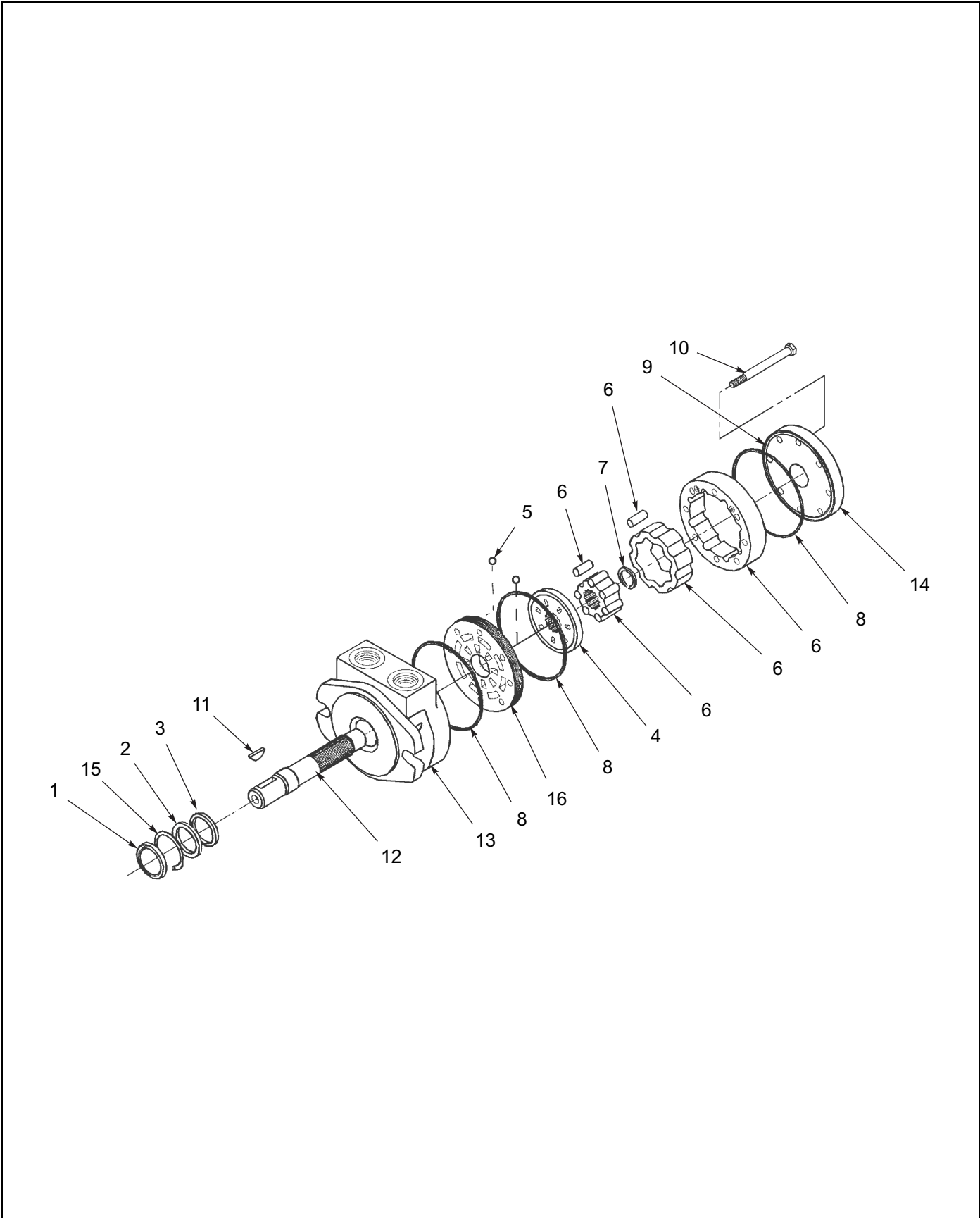
Figure 1-57: Winch - Motor Assembly
