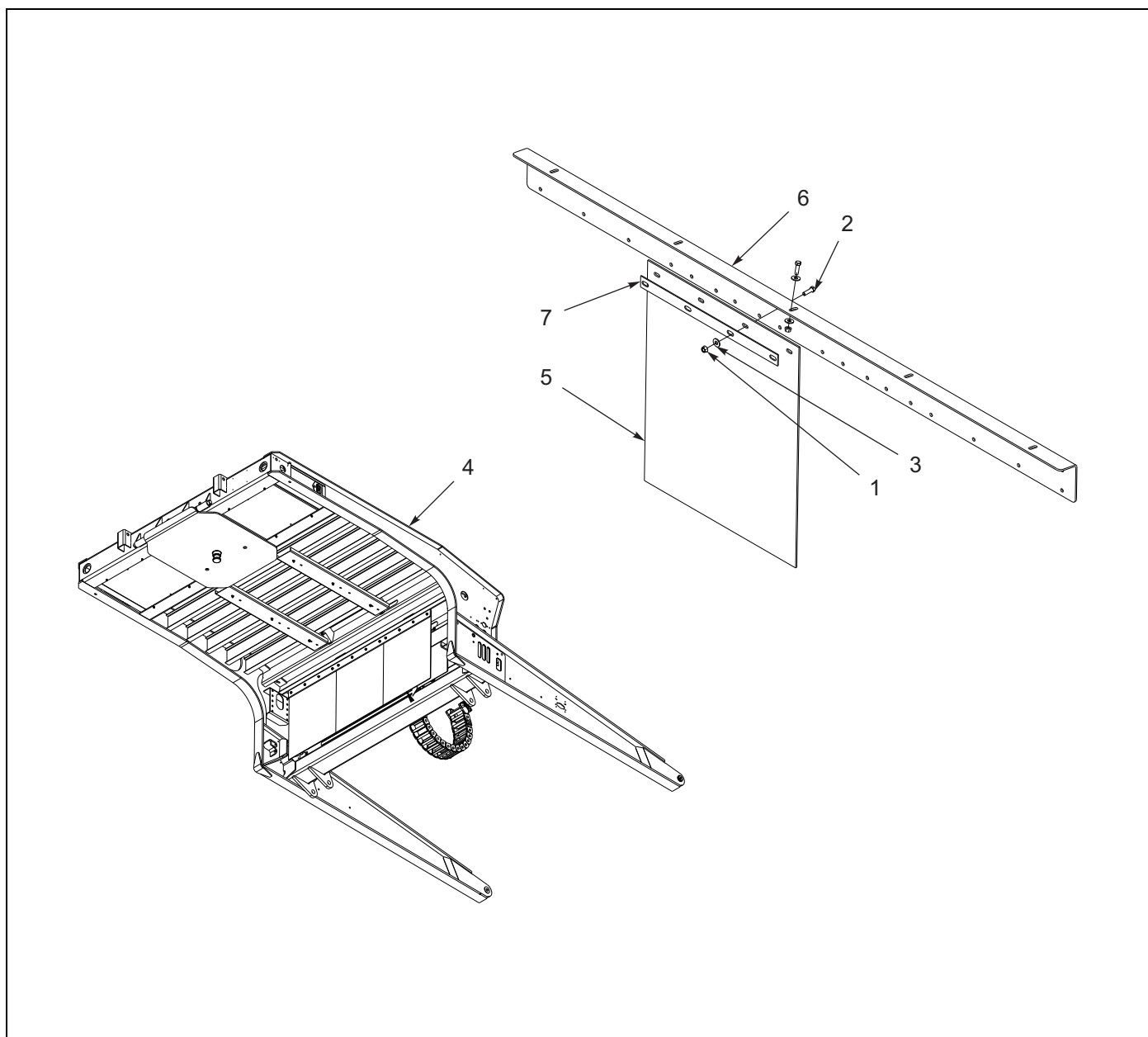
Figure 1-144: Mud Flap Installation - Located Under G/N
