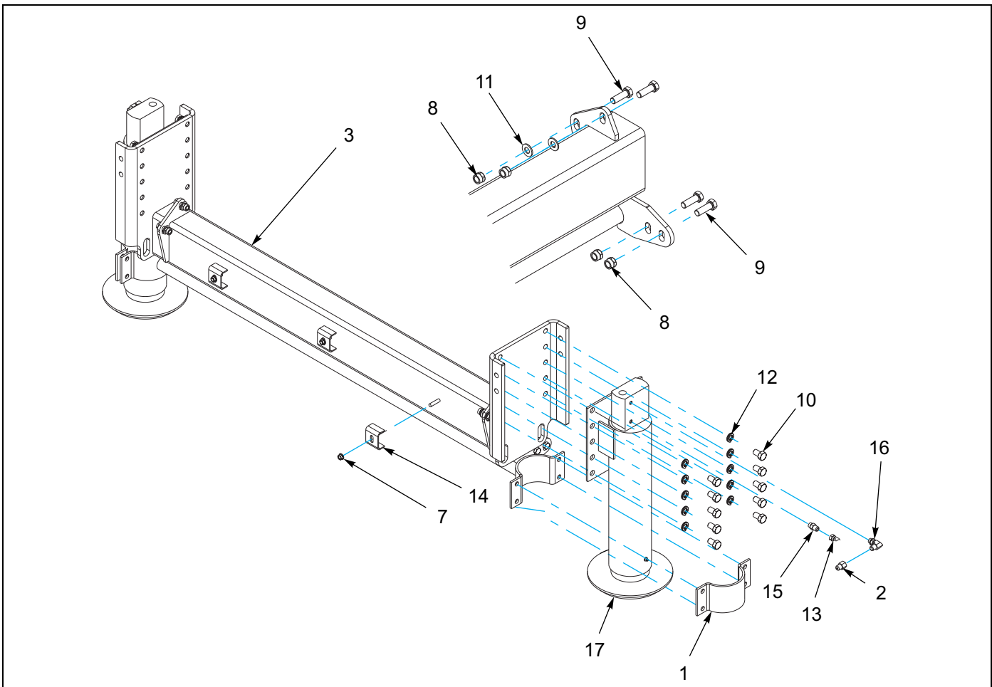
Figure 1-69: Dock Leveler Assembly - Single 60K (455A-120) (Arctic)
