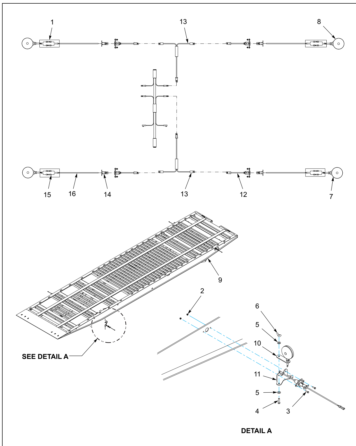
Figure 1-104: Four Corner Light Installation
