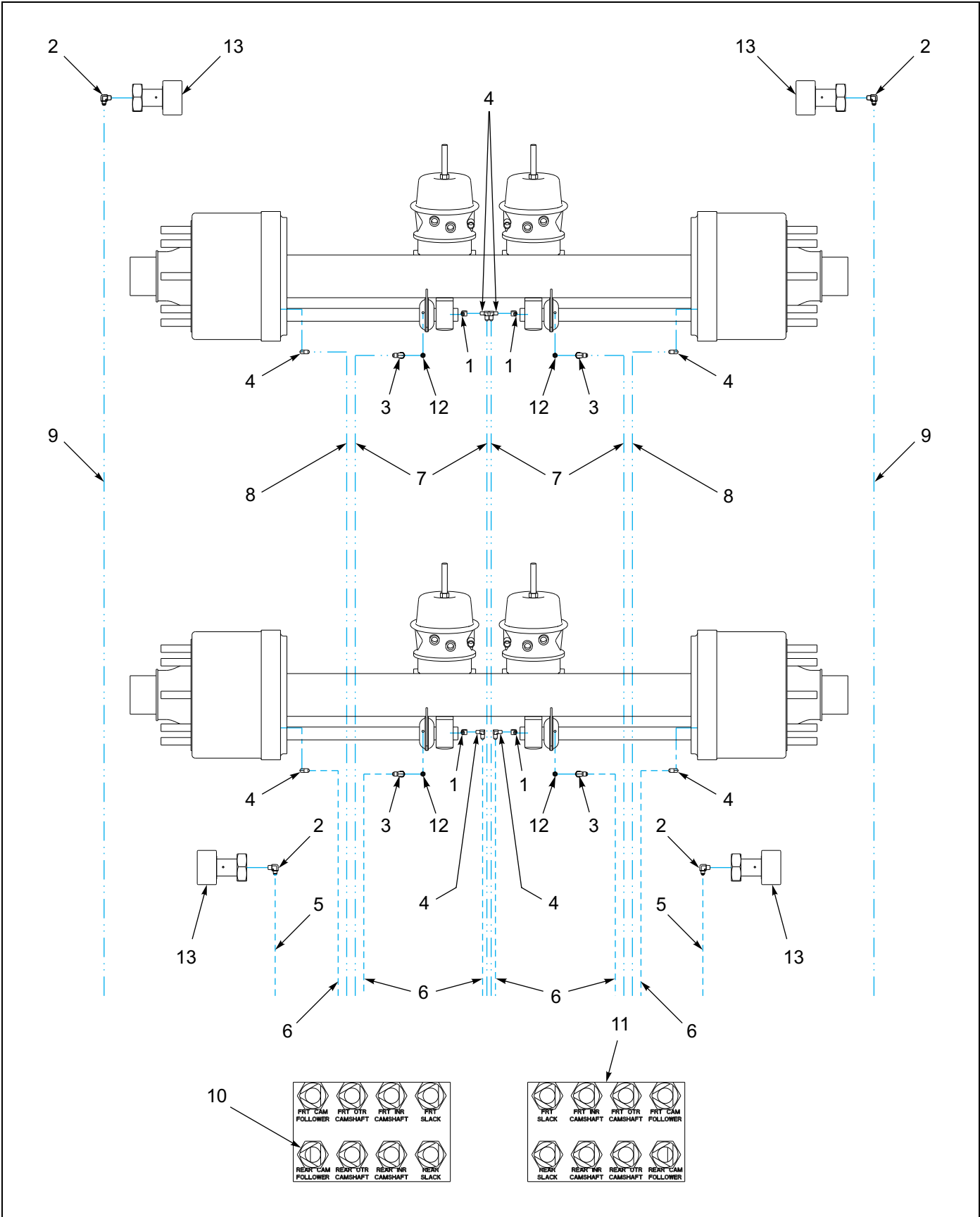
Figure 1-27: Grease System - 440A Spring Brake
