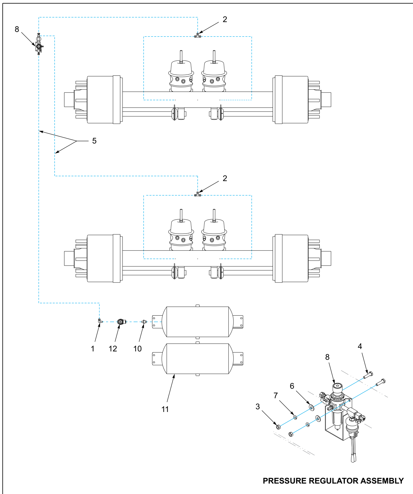
Figure 1-43: Tire Inflation System - 440A
