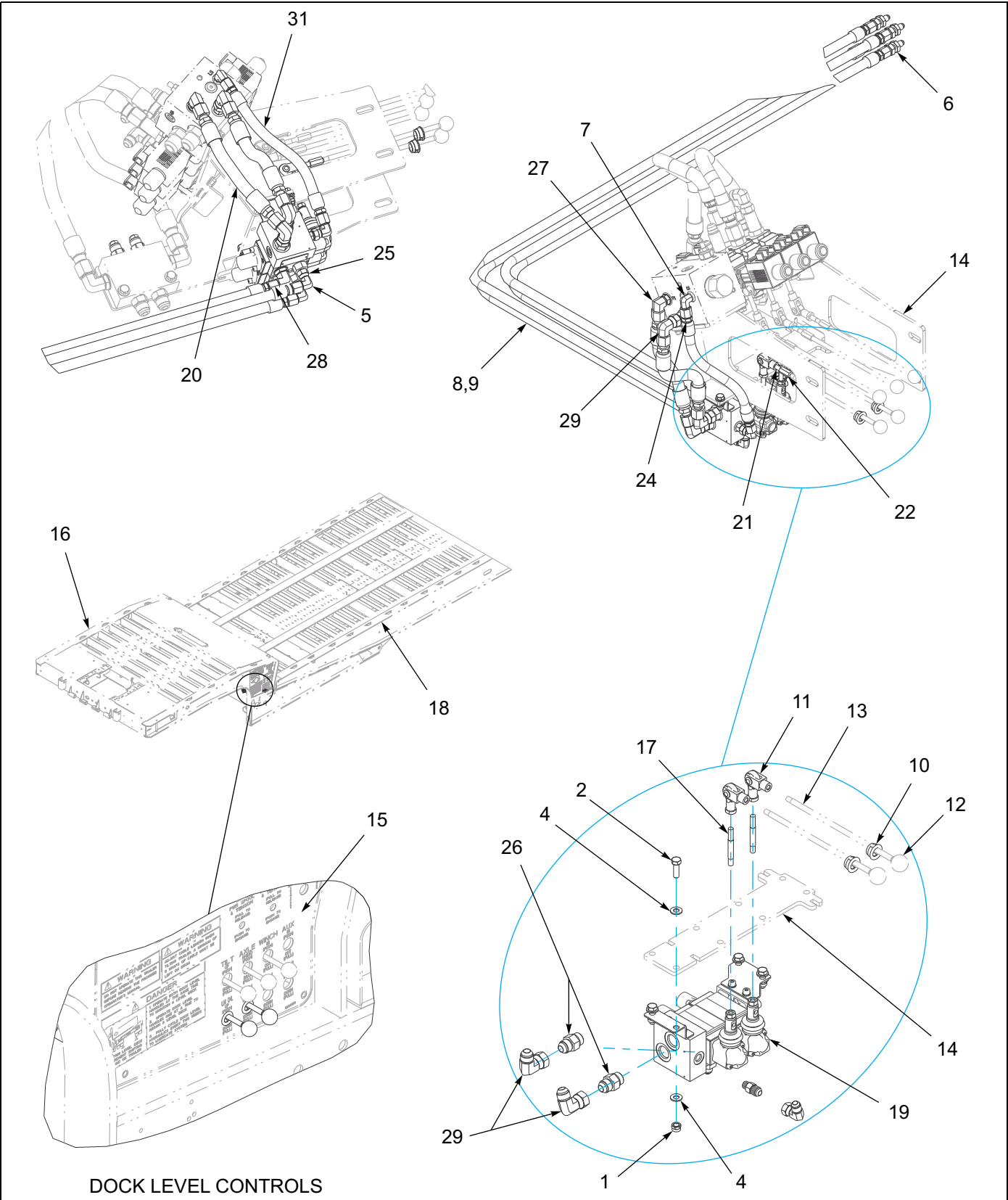
Figure 1-65: Dock Level Installation
