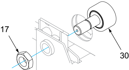
FRONT CAM FOLLOWER ASSEMBLY
