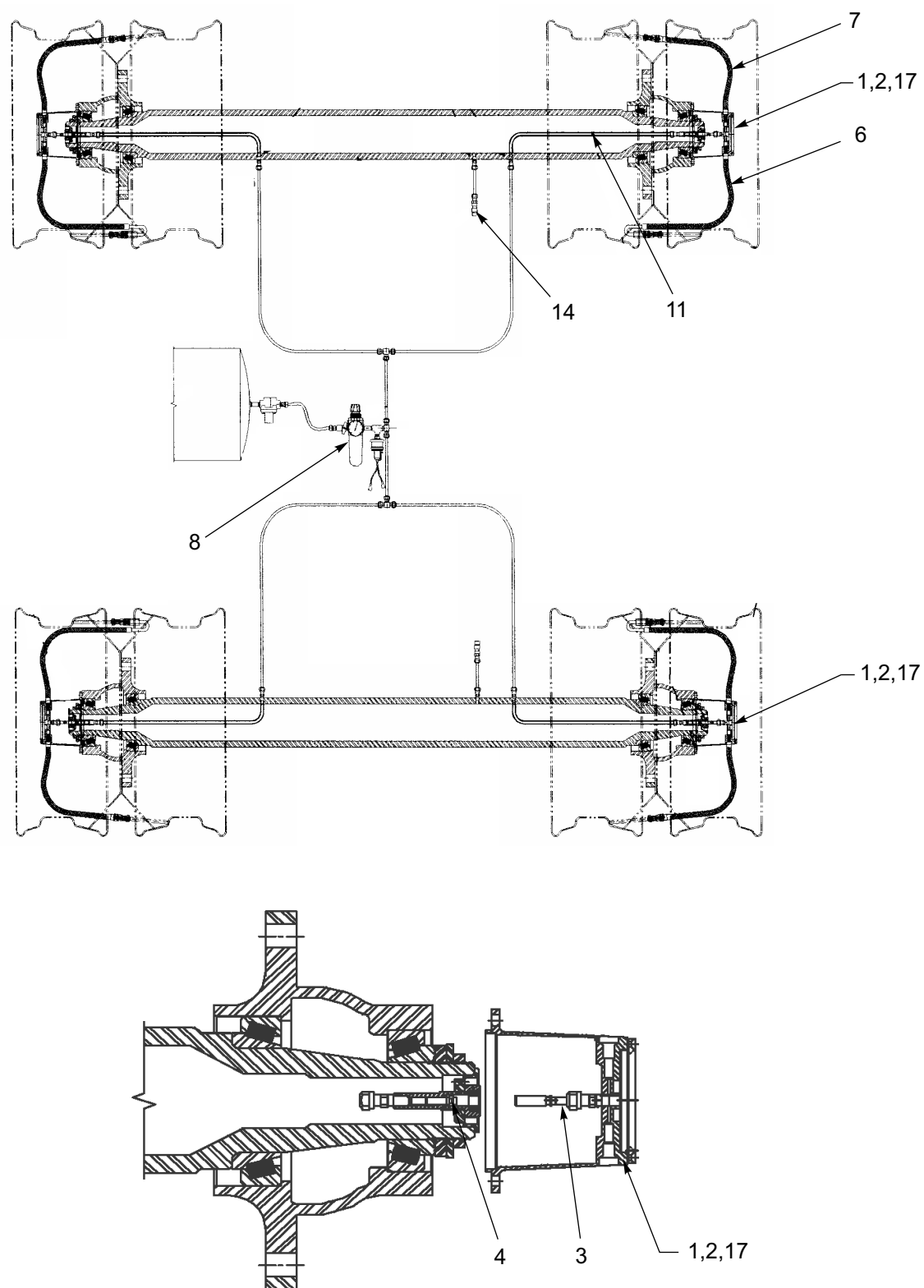
Figure 1-46: Tire Inflation System - 2AX/3AX (Option)
