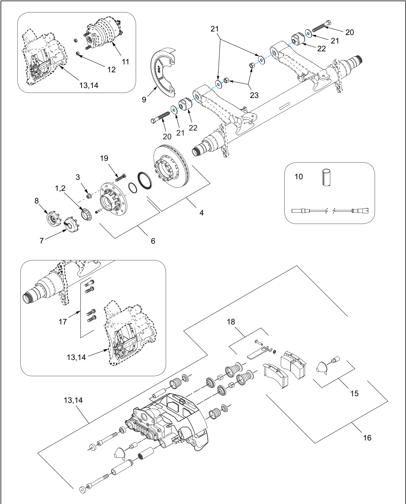
Figure 1-38: Axle & Disc Brake Items
