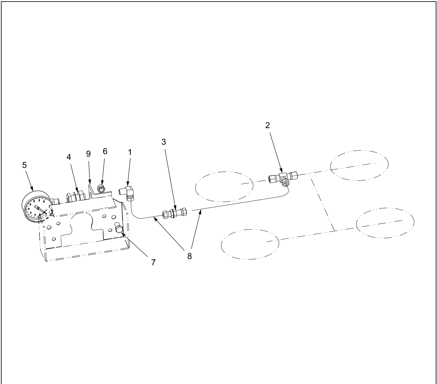
Figure 1-146: Pressure Gauge Installation
