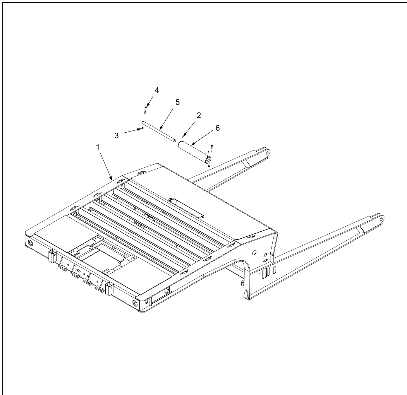
Figure 1-128: Upper Deck - Roller Installation
