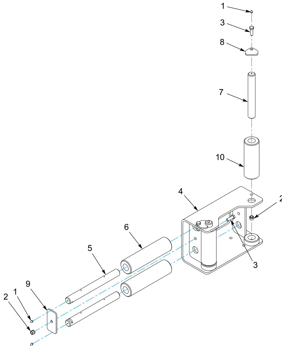
Figure 1-131: Winch - 12K Guide Assembly (BRADEN)
