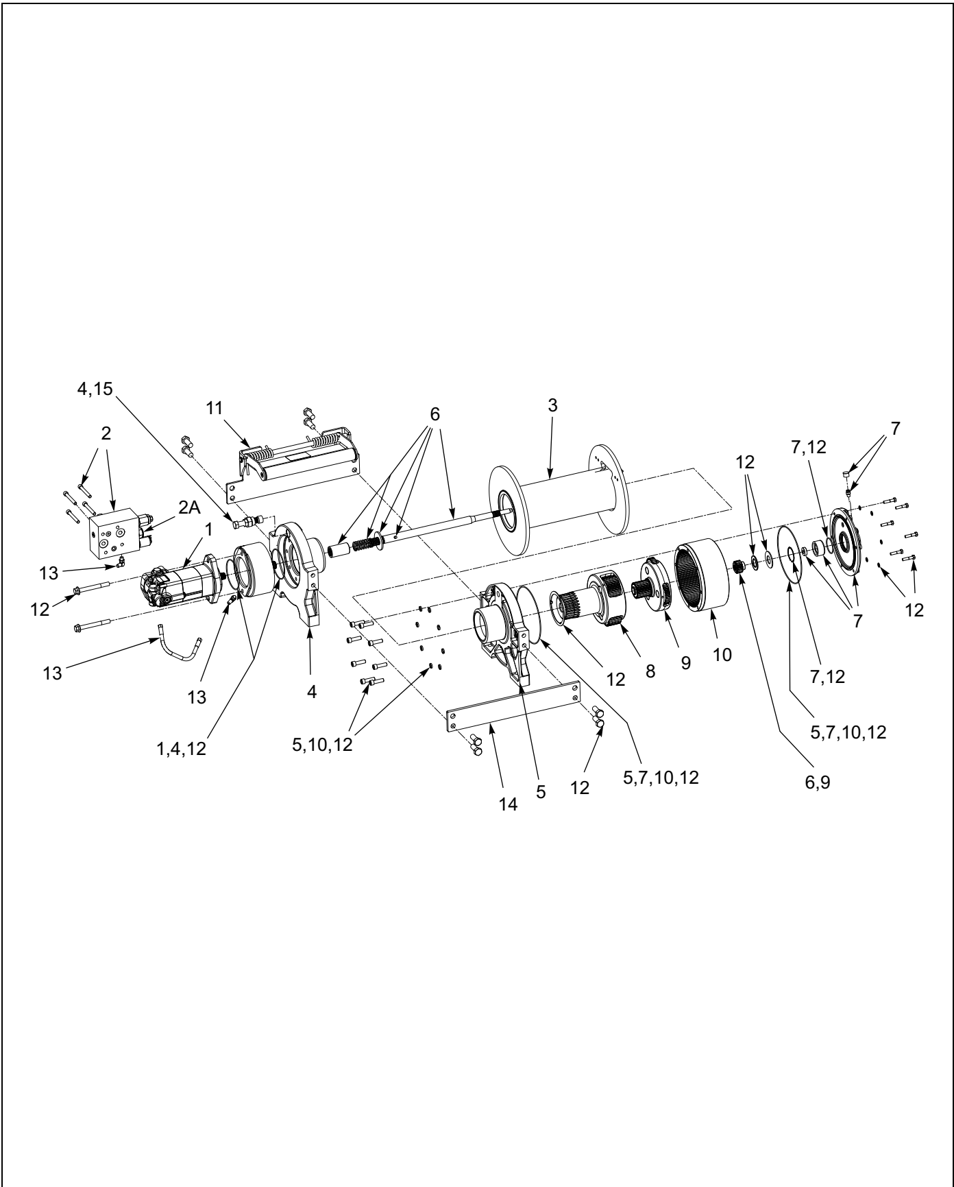
Figure 1-59: Winch Items - 20K 2 Speed (WARN)
