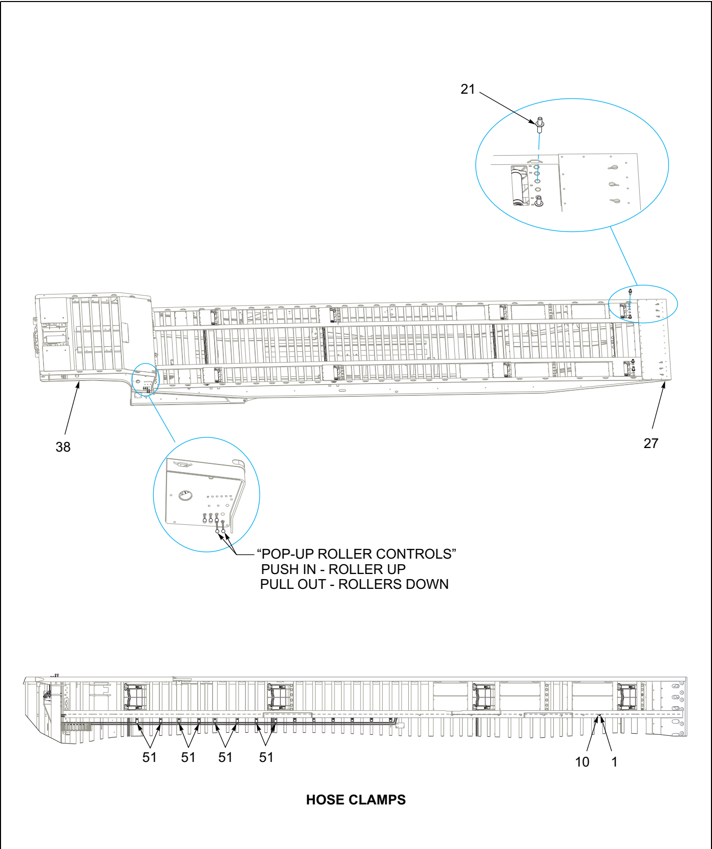
Figure 1-119: 8 Pop-Up Roller Installation (1 of 2)
