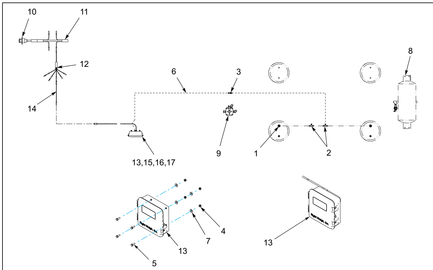
Figure 1-78: Air Digital Scale - Right Weigh System
