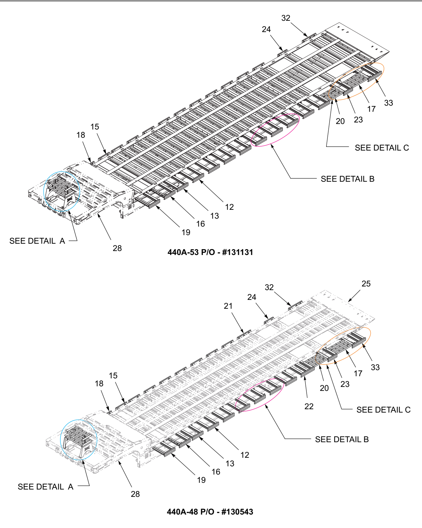
Figure 1-112: Pullout Extension Installation - 440A (2 of 2)
