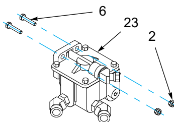
VALVE BOOSTER ASSEMBLY
