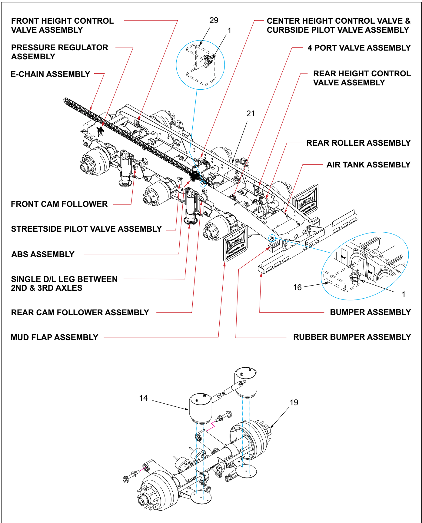
Figure 1-24: General Items - 455A Spring Brake (1 of 3)
