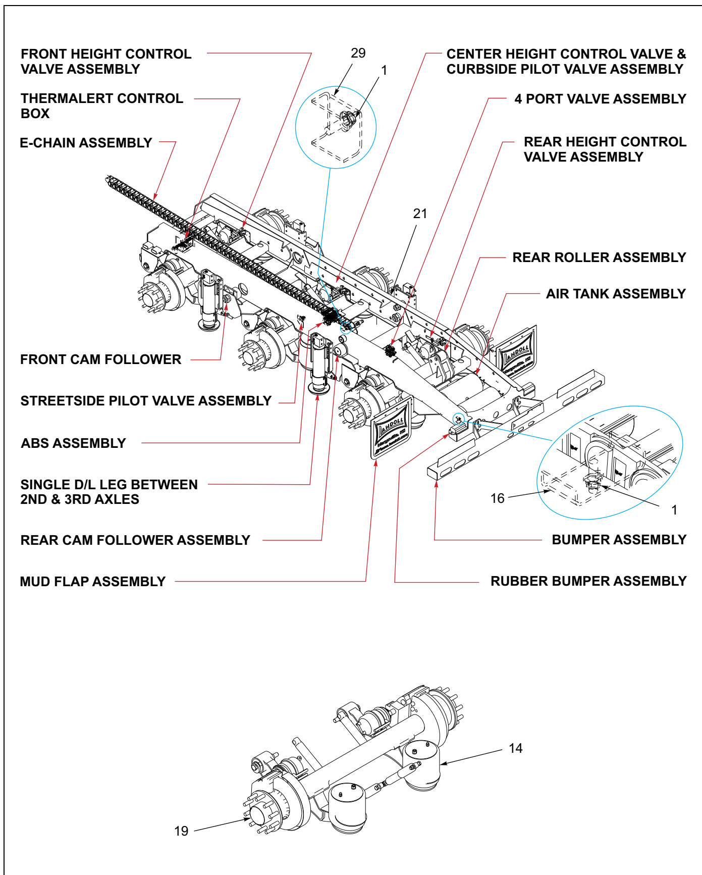
Figure 1-25: General Items - 455A Disc Brake (2 of 3)
