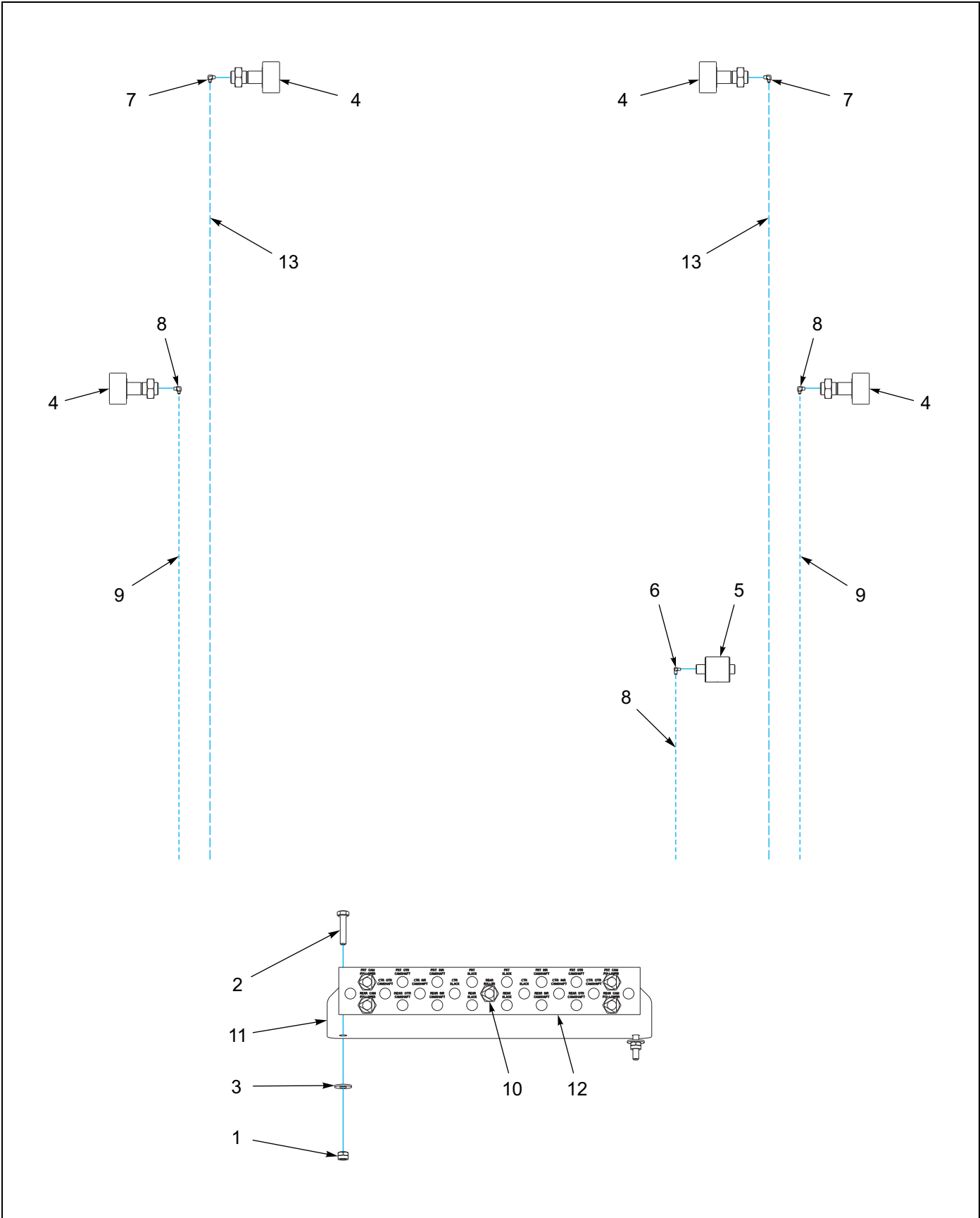
Figure 1-29: Grease System - 455A Disc Brake
