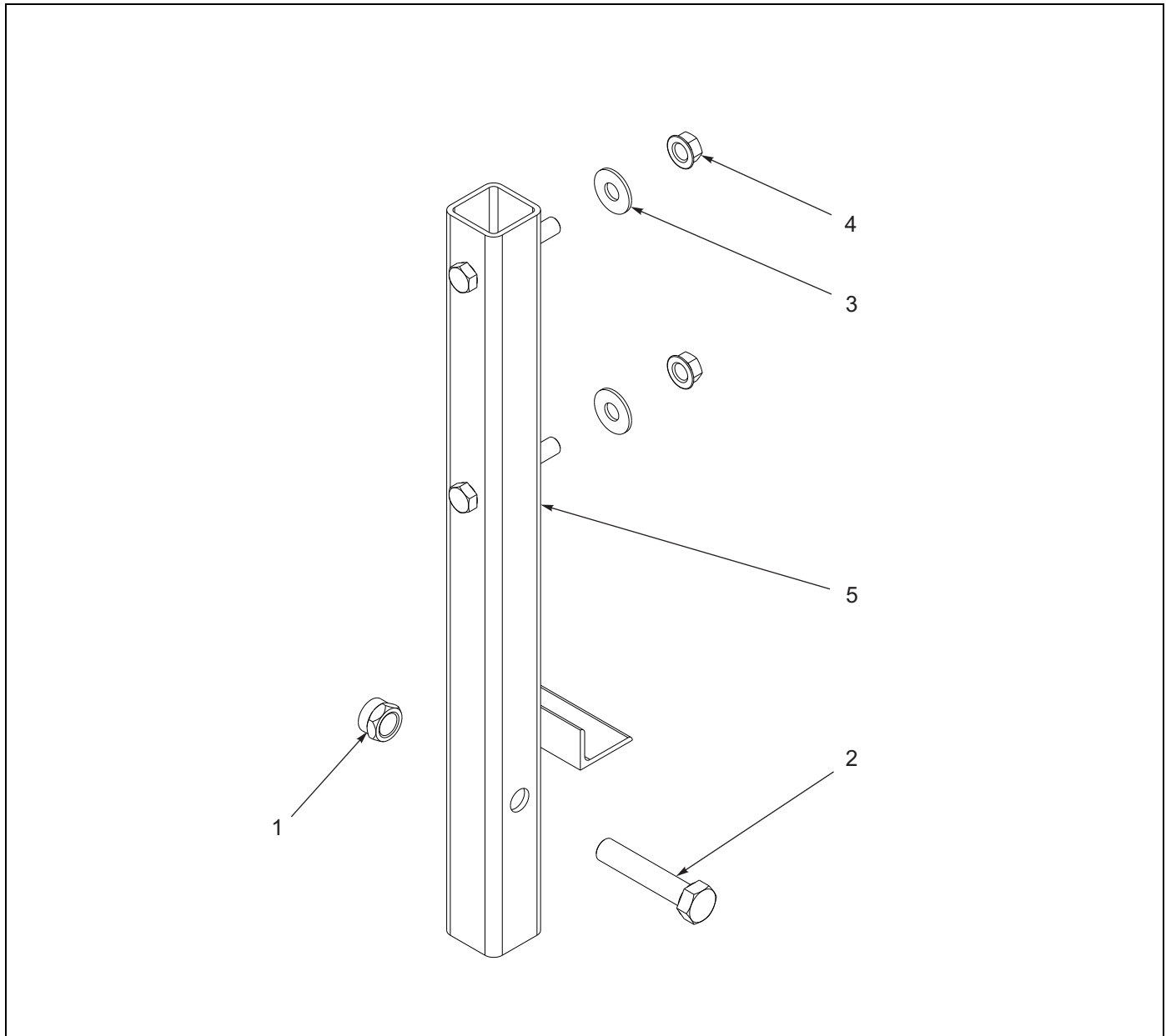
Figure 1-122: Spare Tire - Mount Assembly
