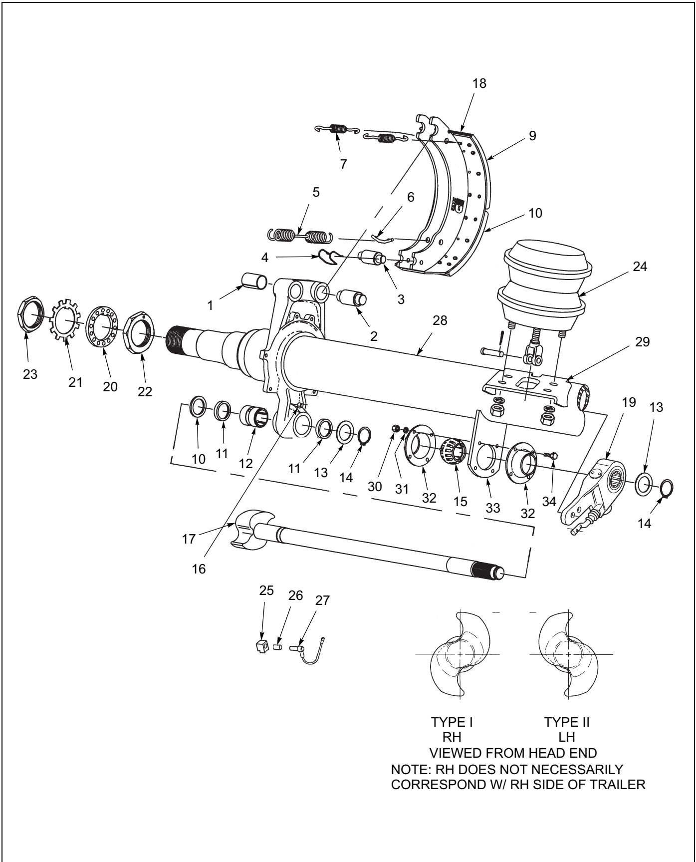
Figure 1-36: Axle and Brake Assembly - Dexter 16-1/2" X 7"
