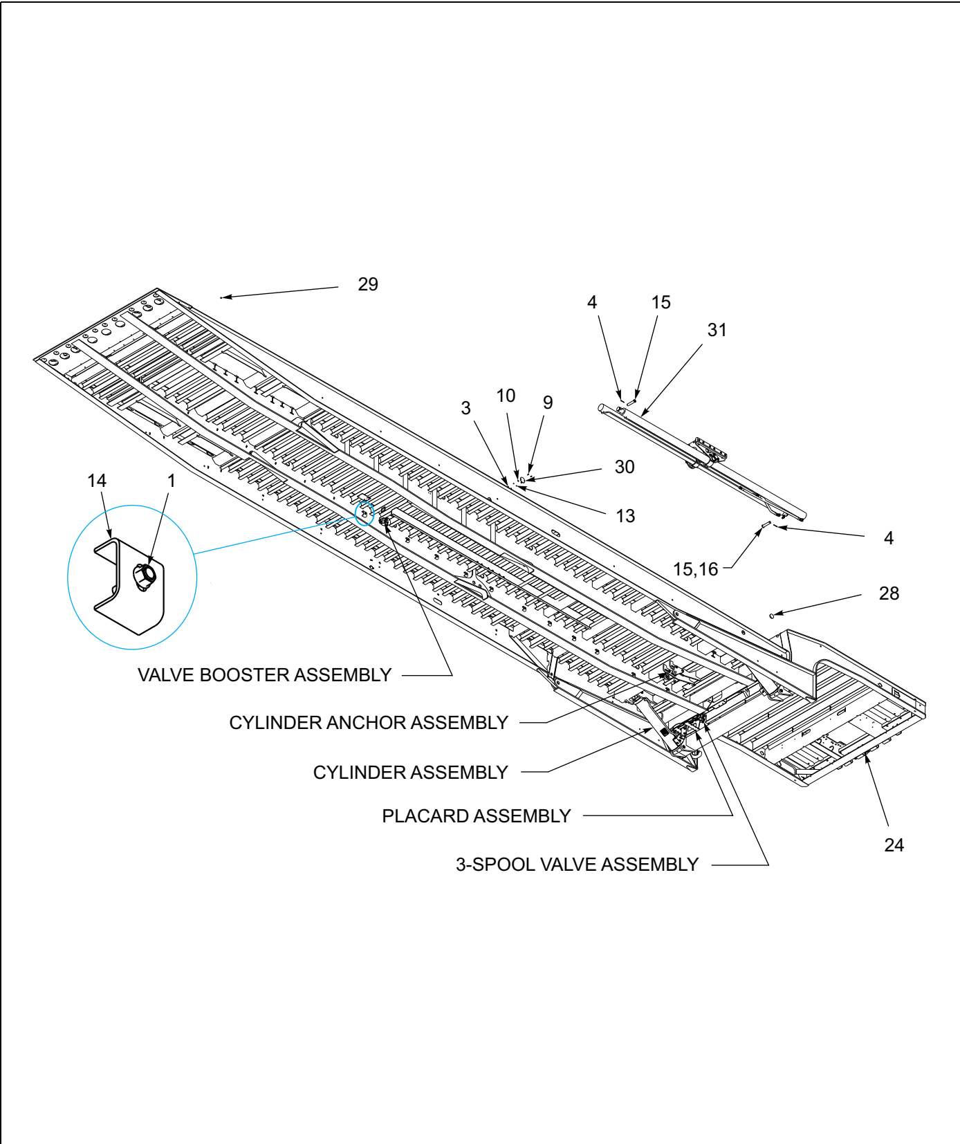
Figure 1-7: General Assembly (1 of 2)
