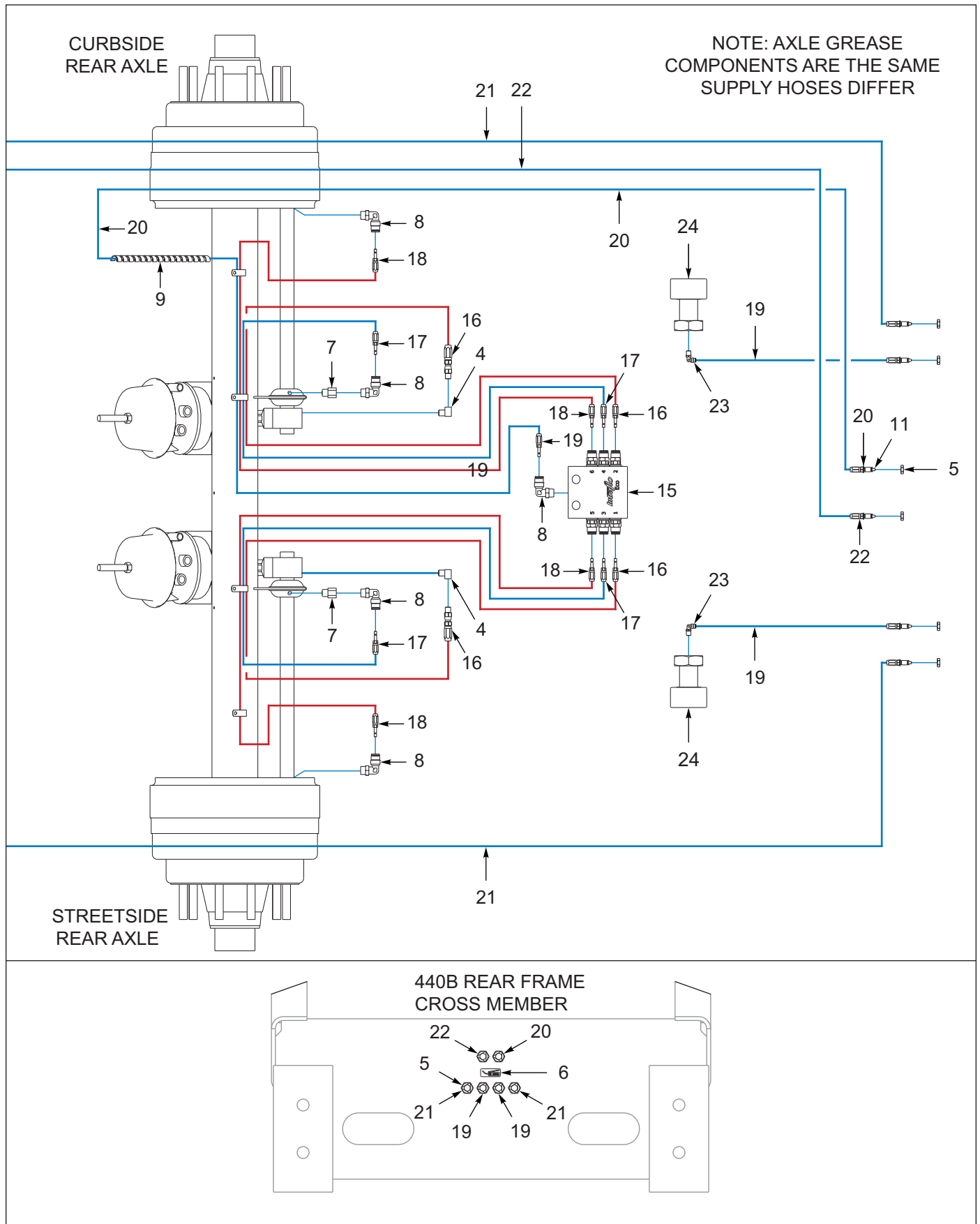
Figure 1-31: Grease System, 2 Axle (After 08/31/2020) (2 of 3)
