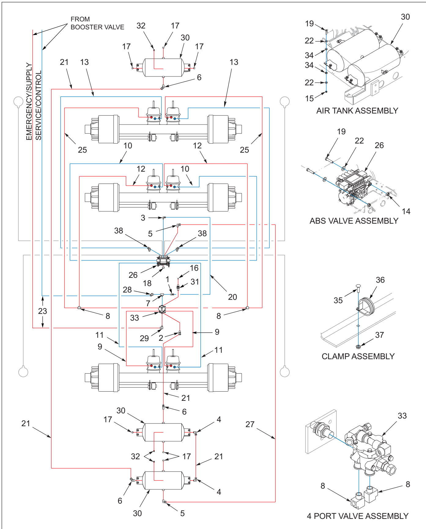
Figure 1-62: Air Brake System, 455B
