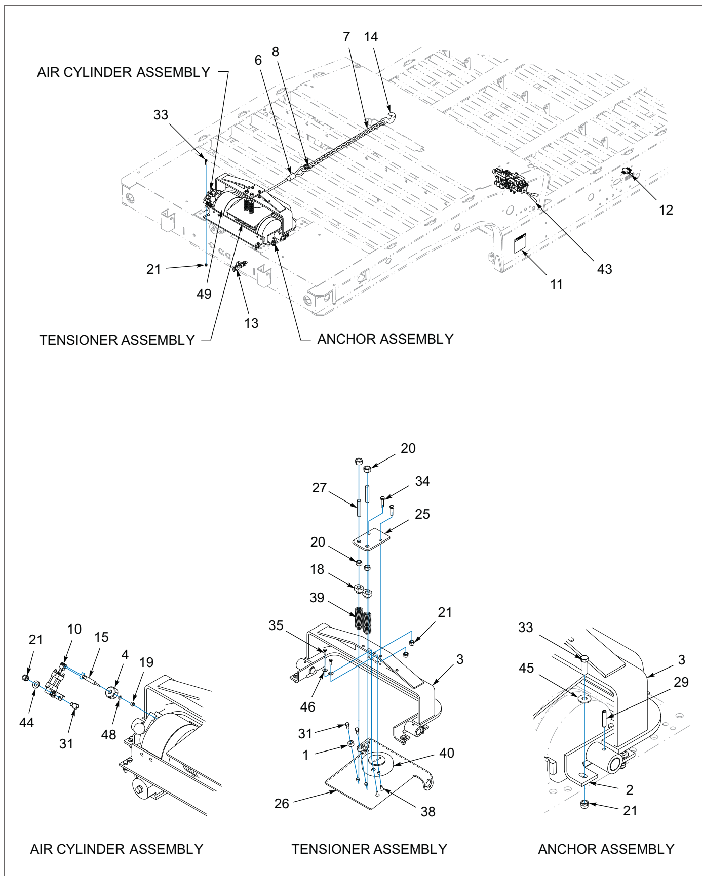
Figure 1-72: 20K Air Tension/Release (BRADEN) (1 of 3)
