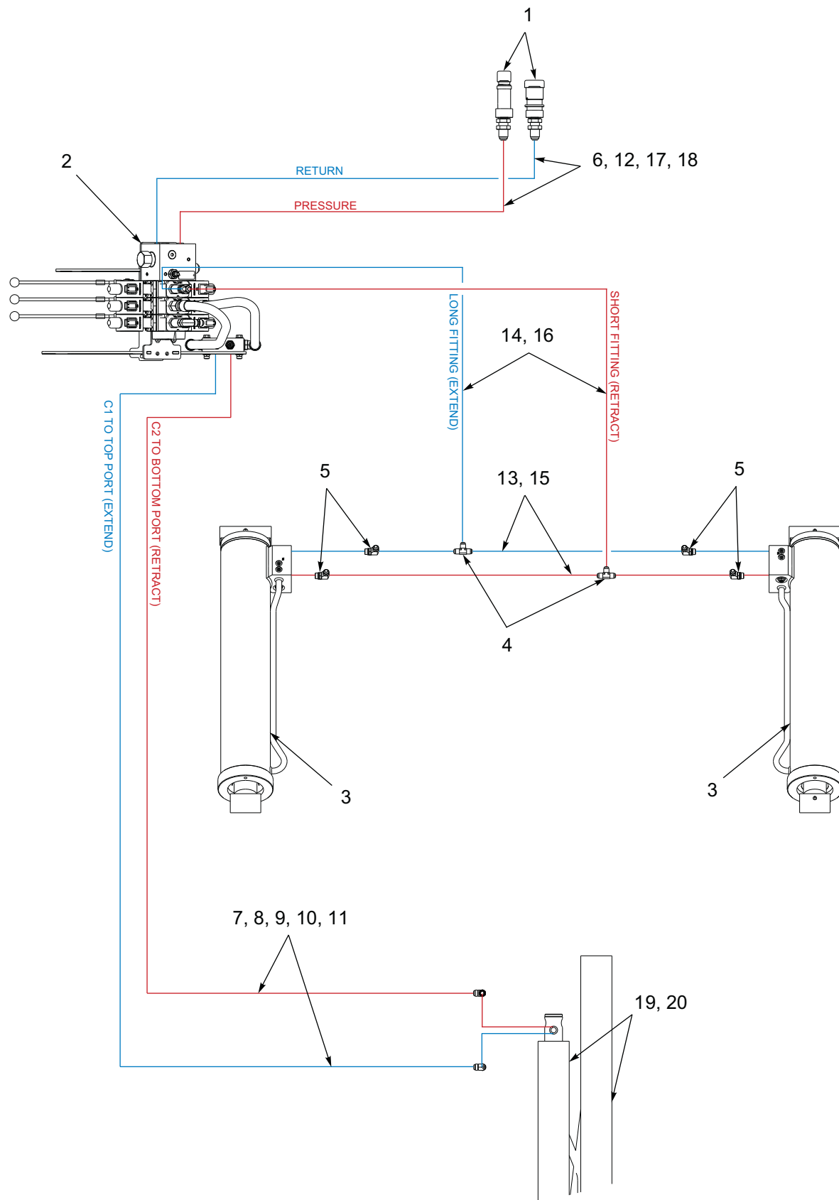
Figure 1-10: Hydraulic System
