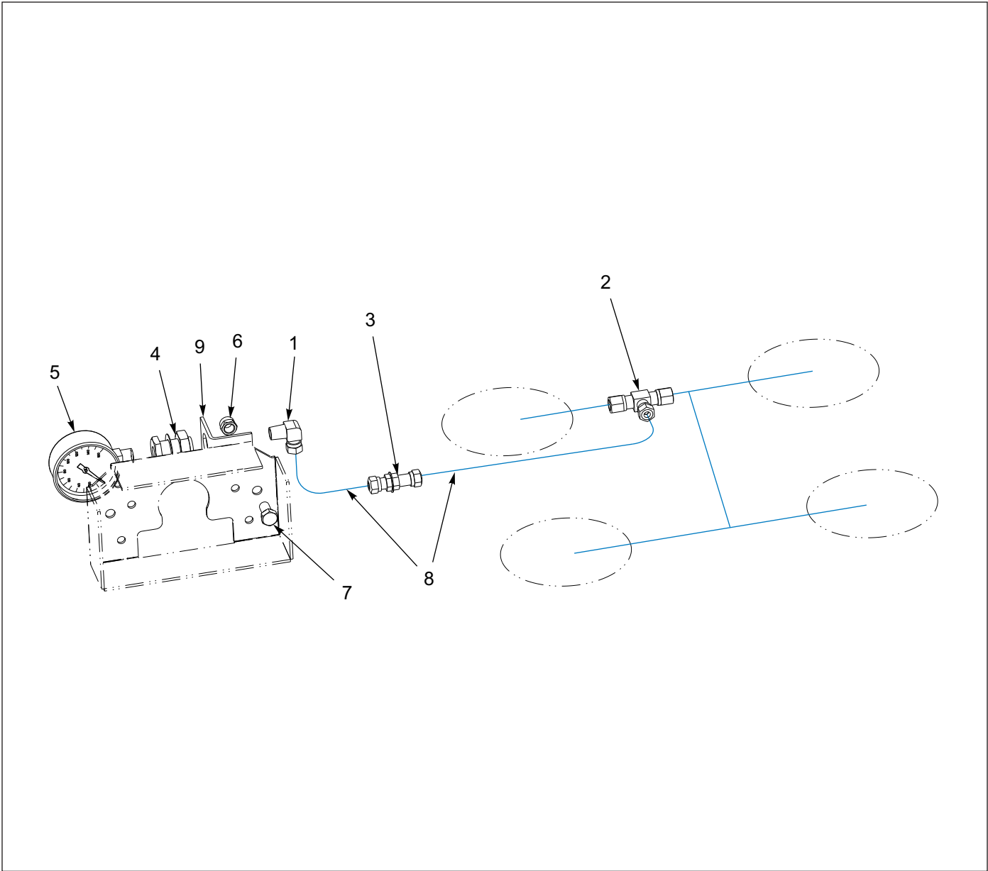
Figure 1-156: Suspension Pressure Gauge Installation
