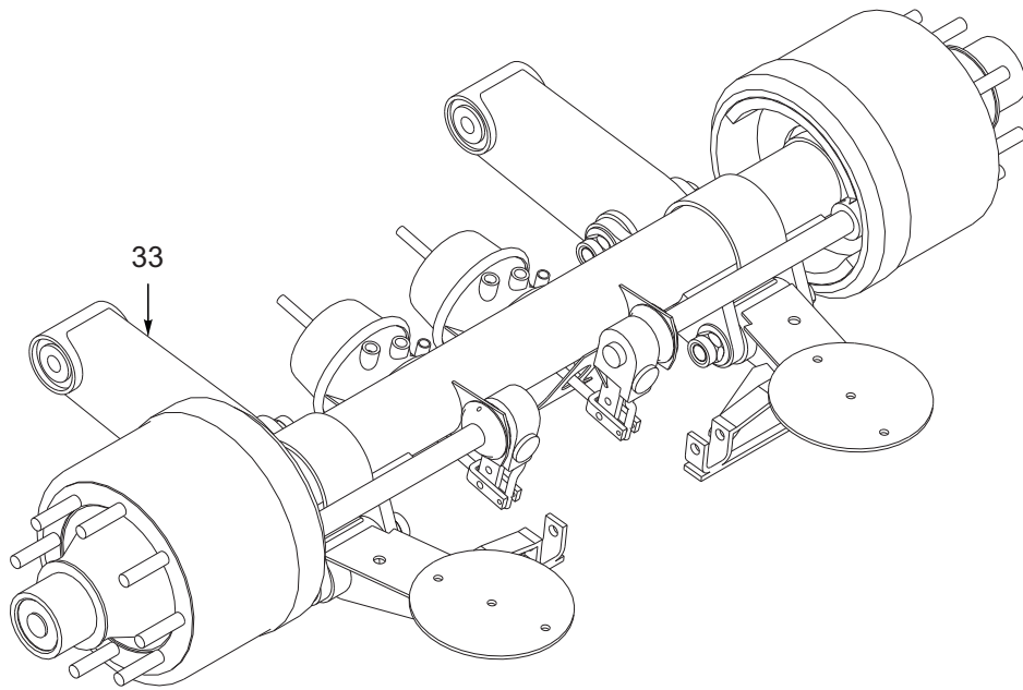
VIEW OF RLU-228-3.5, 12.25 X 7.5 DRUM BRAKES
