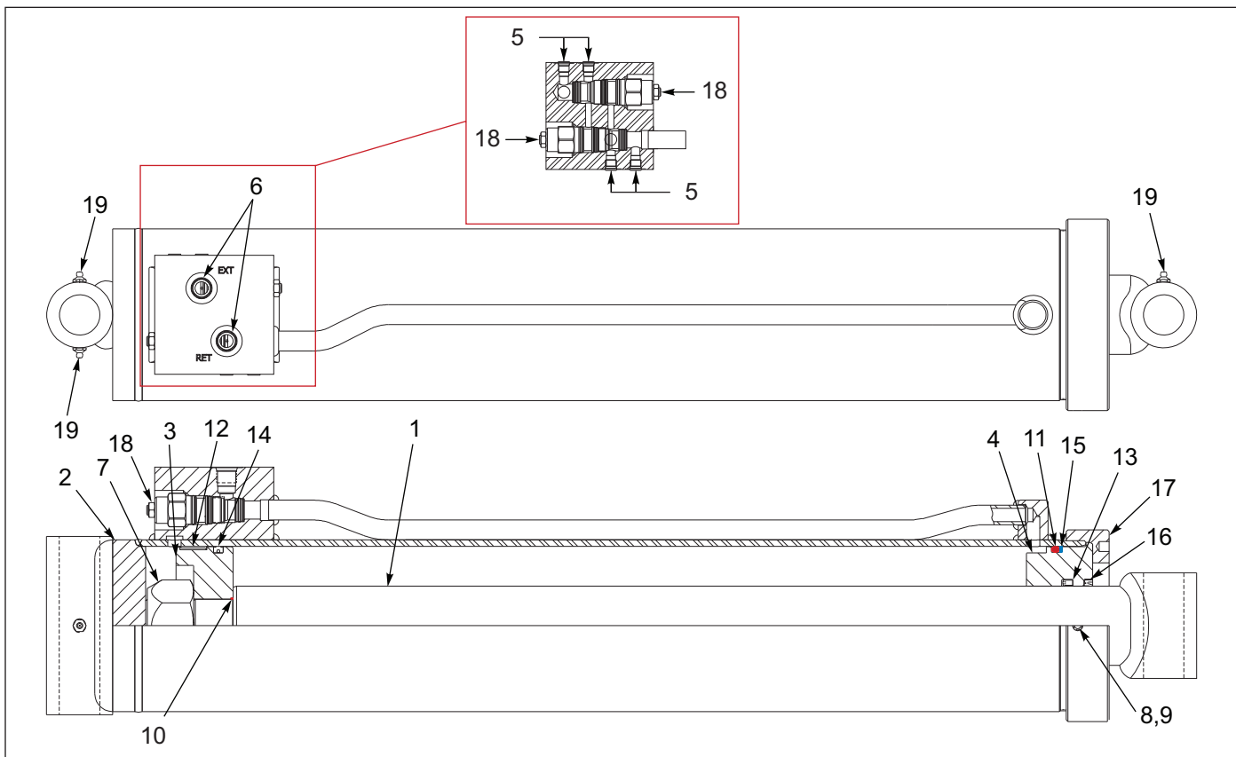
Figure 1-15: Cylinder - 6 X 30
