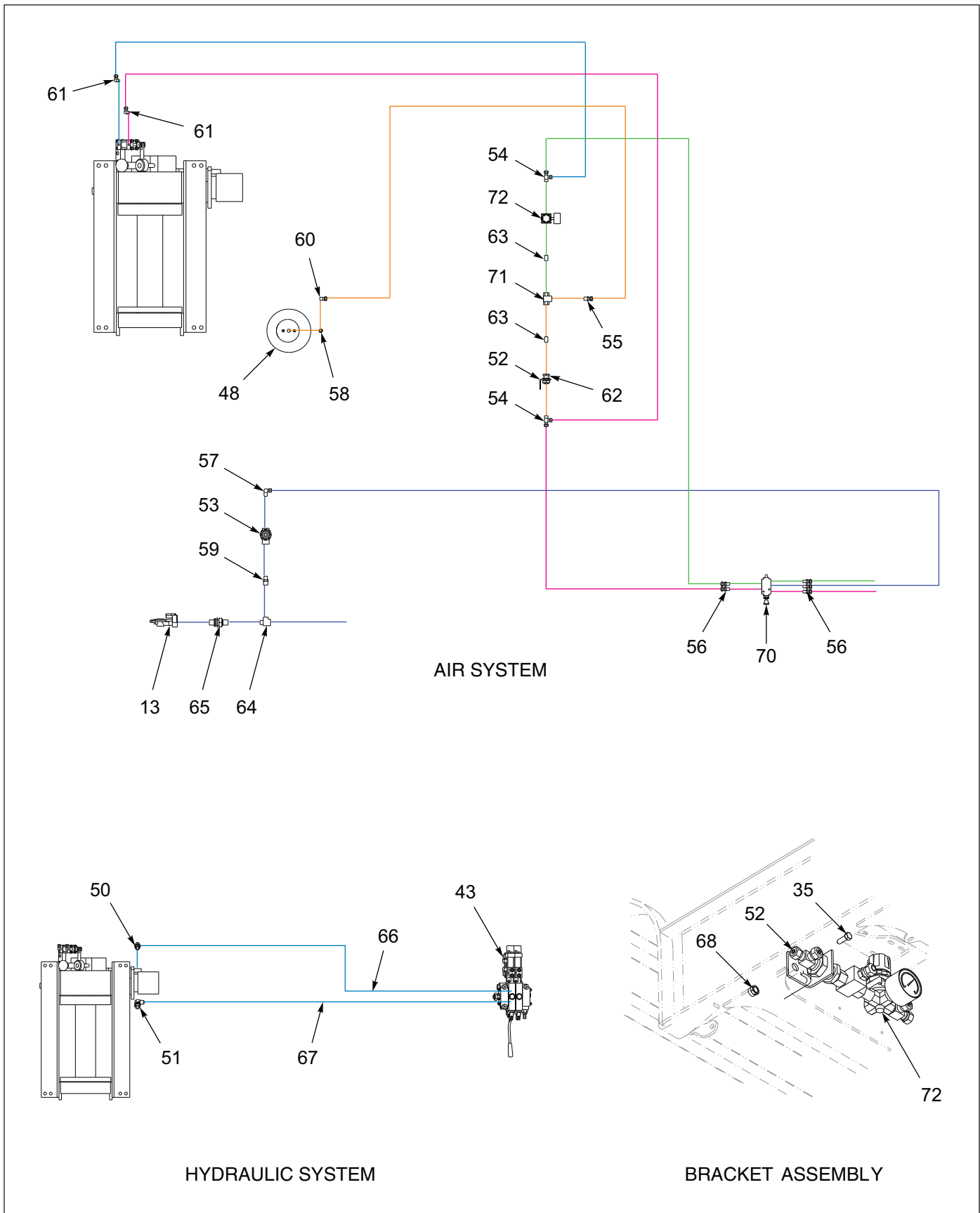
Figure 1-74: 20K Air Tension/Release (BRADEN) (3 of 3)
