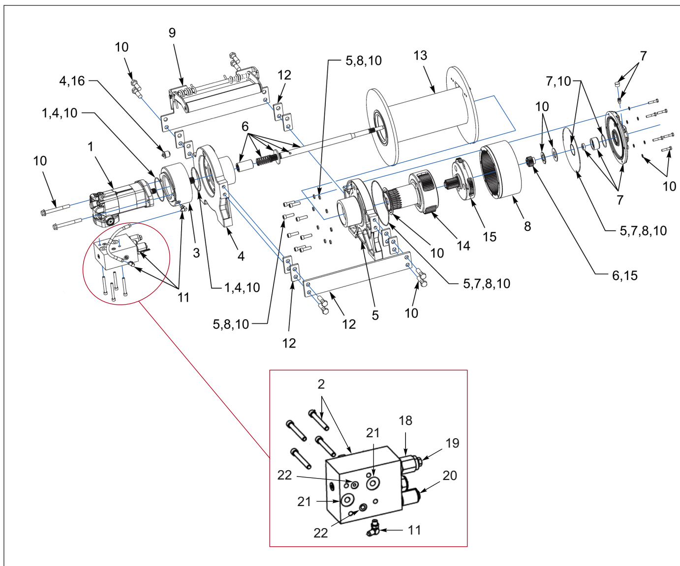
Figure 1-81: Winch Items - 30K 2 Speed (WARN)
