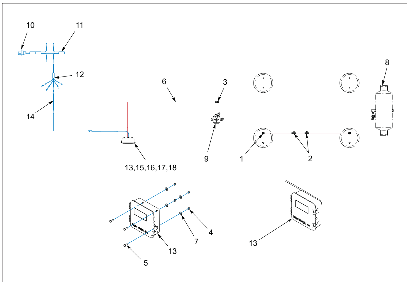
Figure 1-129: Right Weigh
