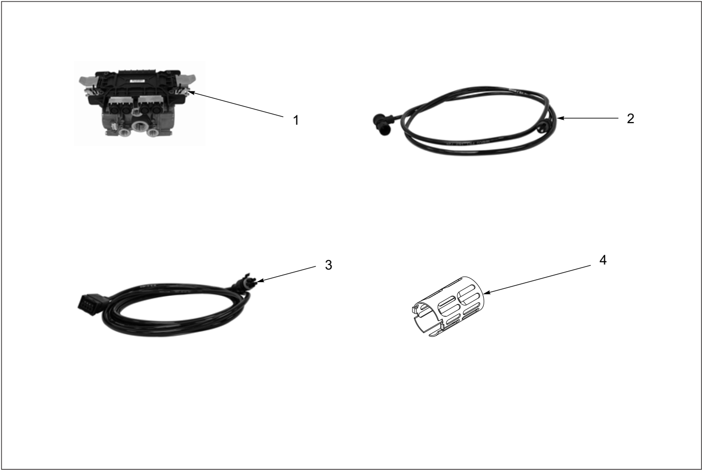
Figure 1-64: ABS Brake Kit - Rockwell
