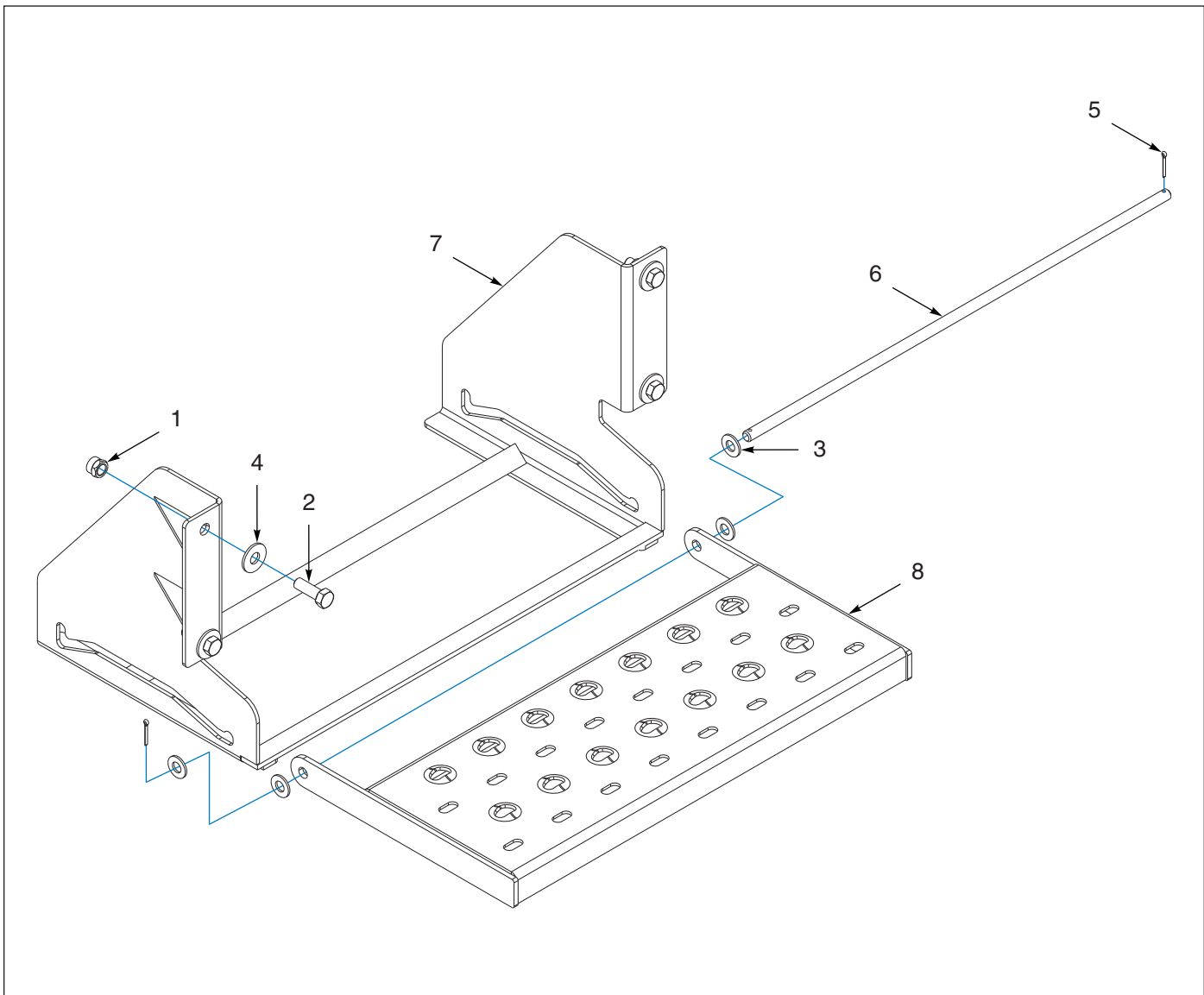
Figure 1-137: Step, Retractable Assembly-2162272
