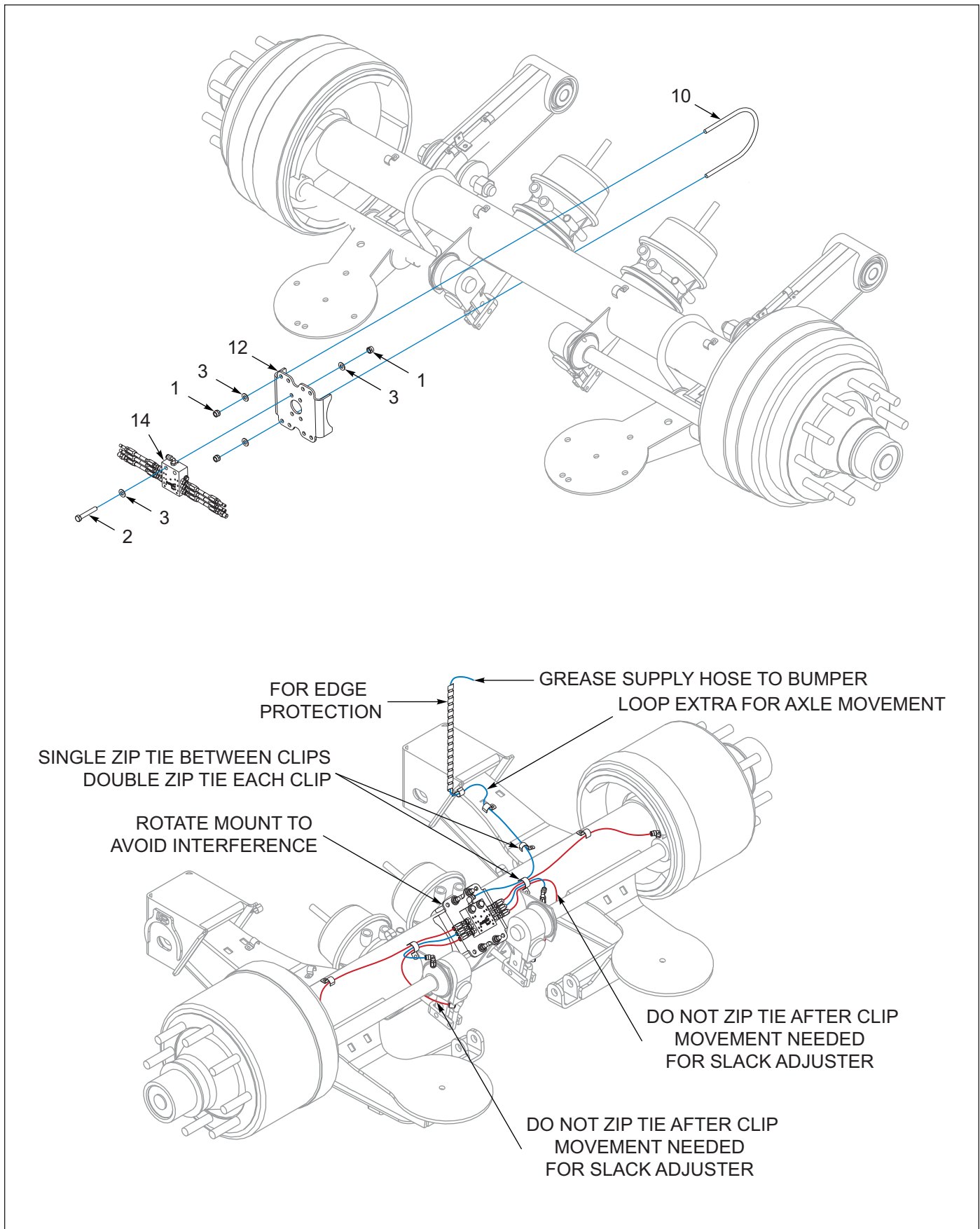
Figure 1-39: Grease System, 3 Axle (After 08/31/2020) (3 of 3)
