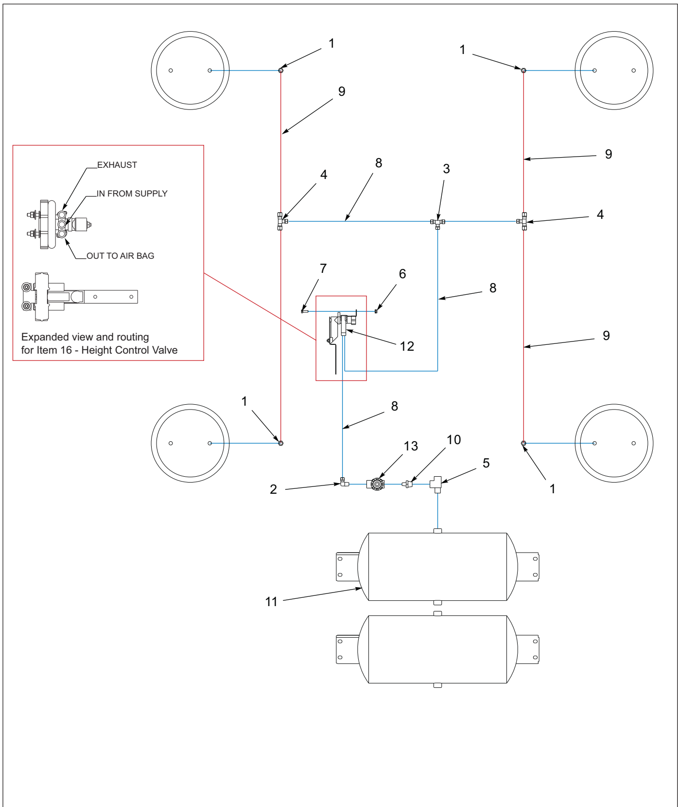
Figure 1-40: Air Ride Suspension - 440B
