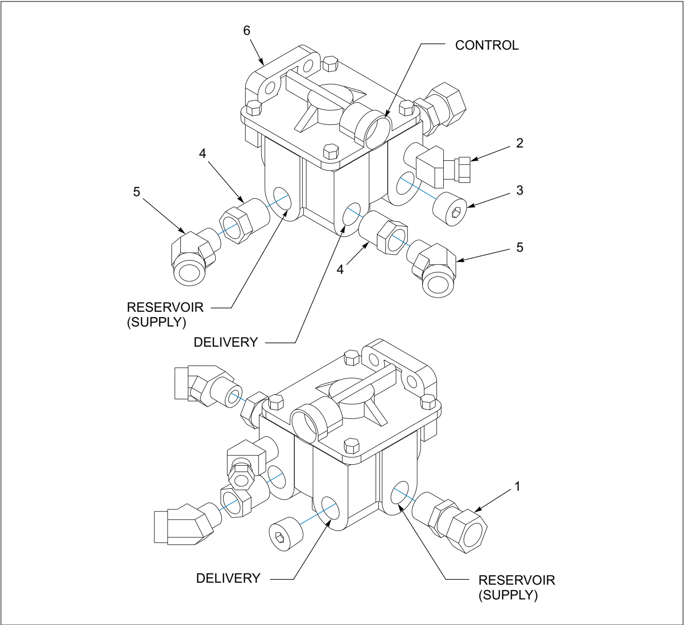
Figure 1-17: Valve Assembly - Air Booster
