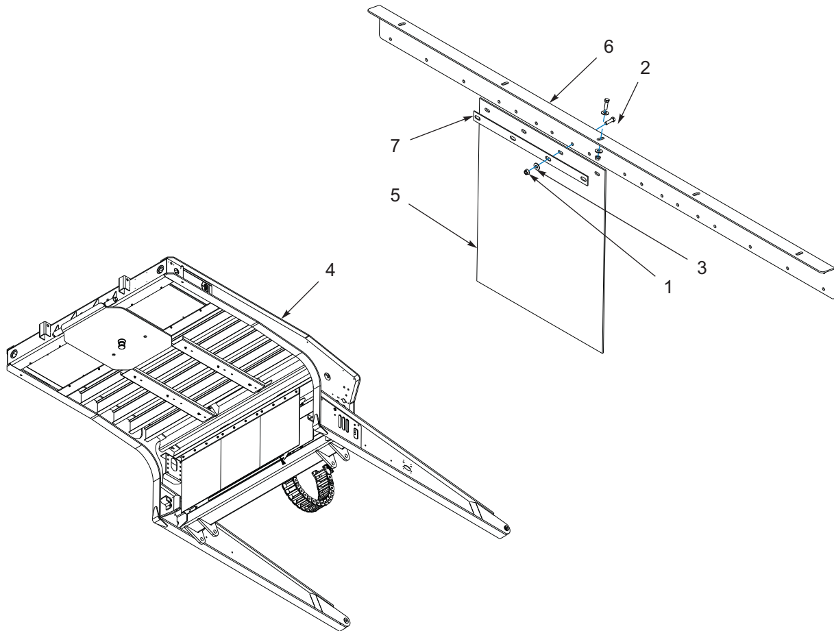
Figure 1-154: Gooseneck Mud Flap Installation
