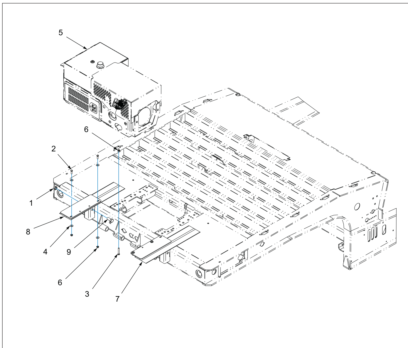
Figure 1-107: Engine - Front Mount Installation
