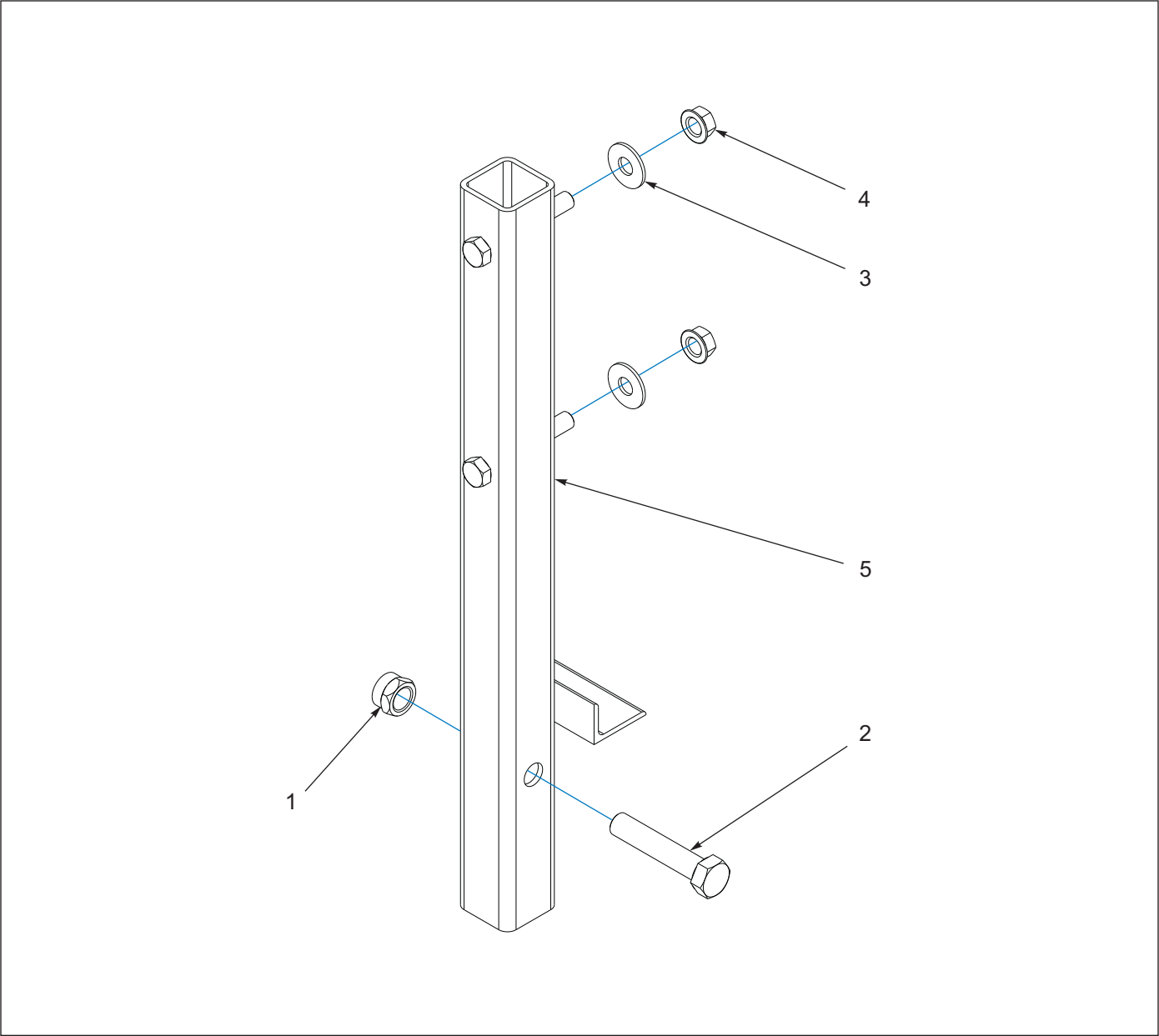
Figure 1-132: Spare Tire - Mount Assembly
