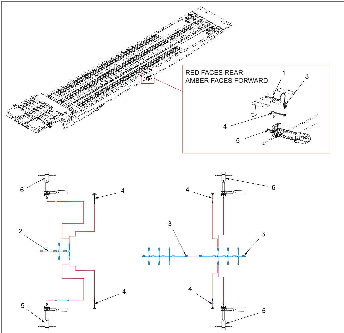
Figure 1-120: Swingout Marker Light Installation - Red/Amber
