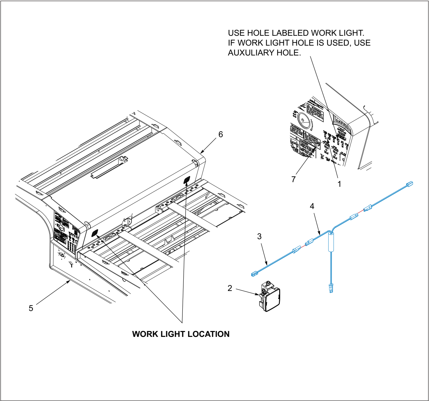
Figure 1-142: Upper Deck - Slope Light Installation
