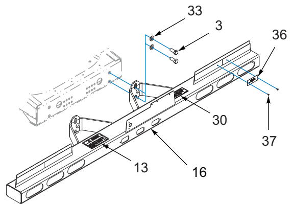
BUMPER ASSEMBLY
