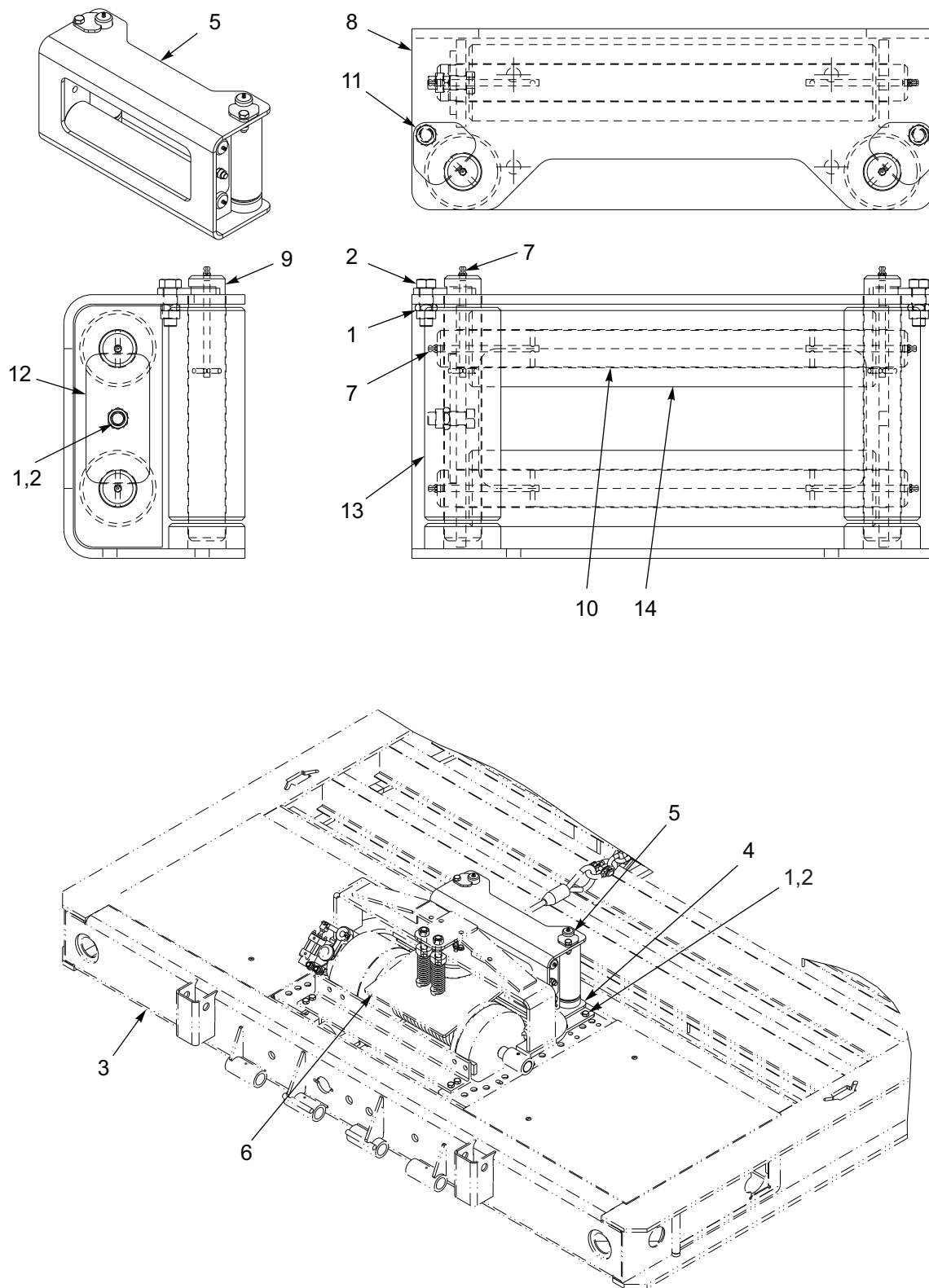
Figure 1-150: Guide Assembly, 4 Roller 20K (BRADEN)-145589
