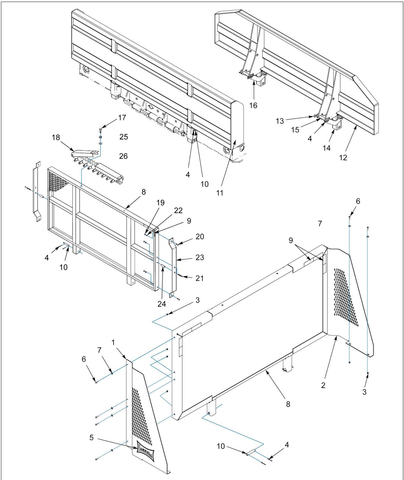
Figure 1-92: Bulkhead Assembly
