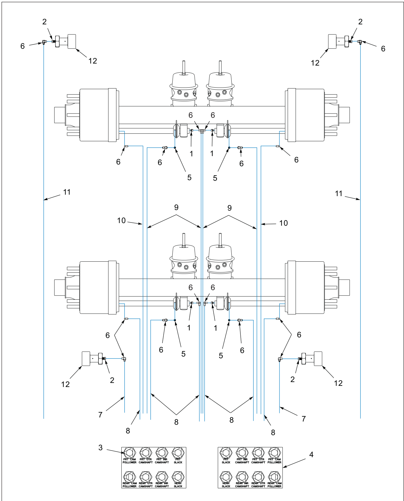
Figure 1-28: Grease System, 2 Axle (Before 11/07/2018)
