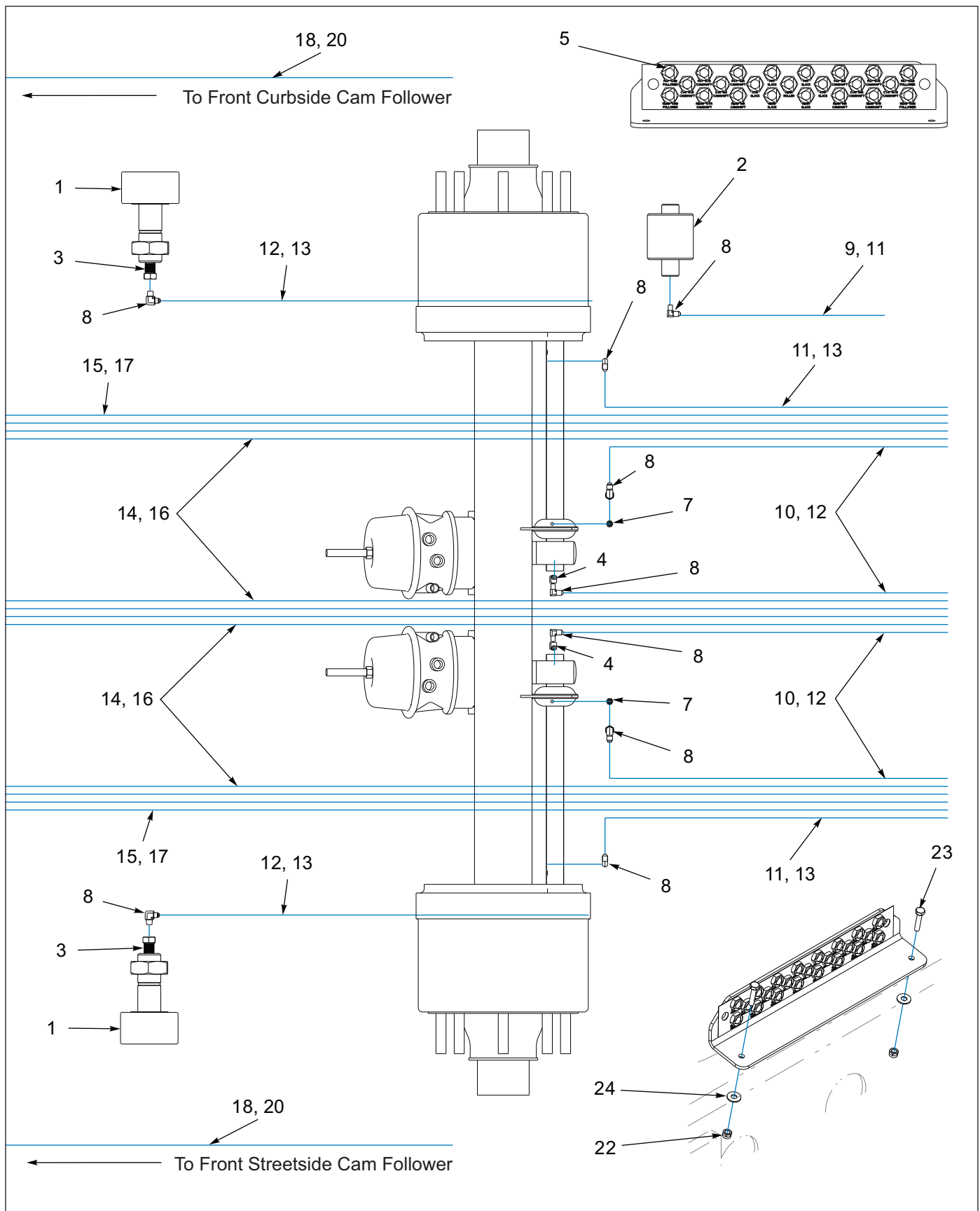
Figure 1-34: Grease System, 3 Axle (Before 11/07/2018) (2 of 2)
