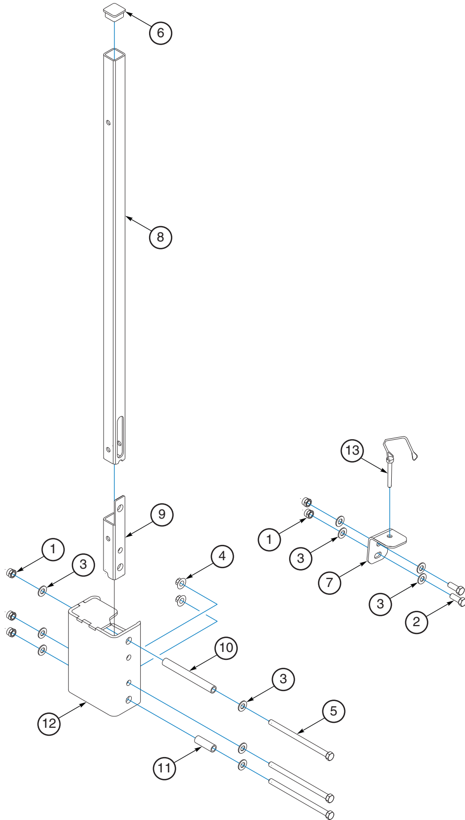
Figure 1-135: Step, Folding Handle Assembly-226645
