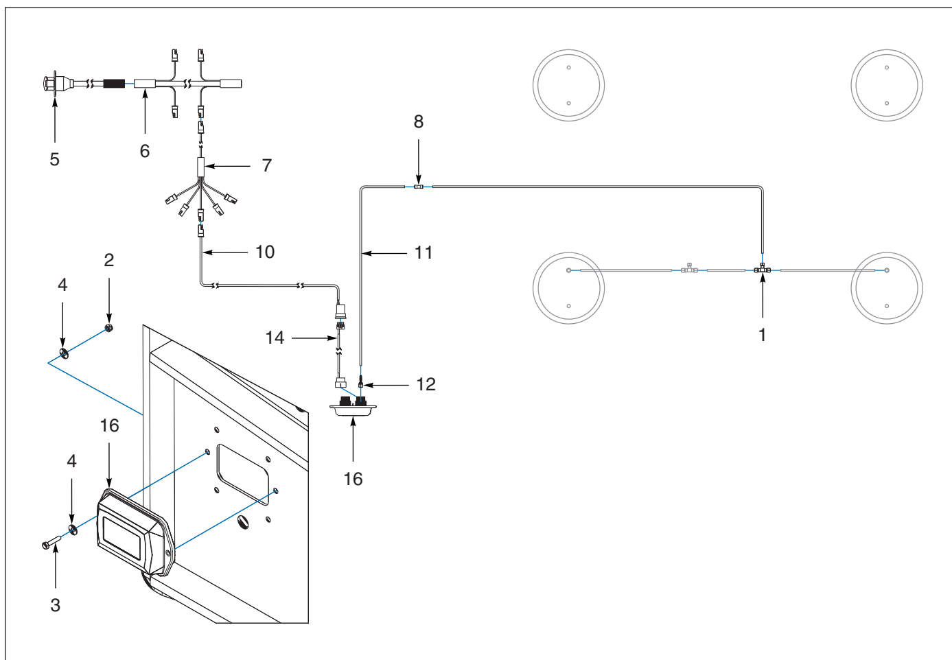
Figure 1-131: LOADMAXX PLUS-226661 (After 03/31/2020)
