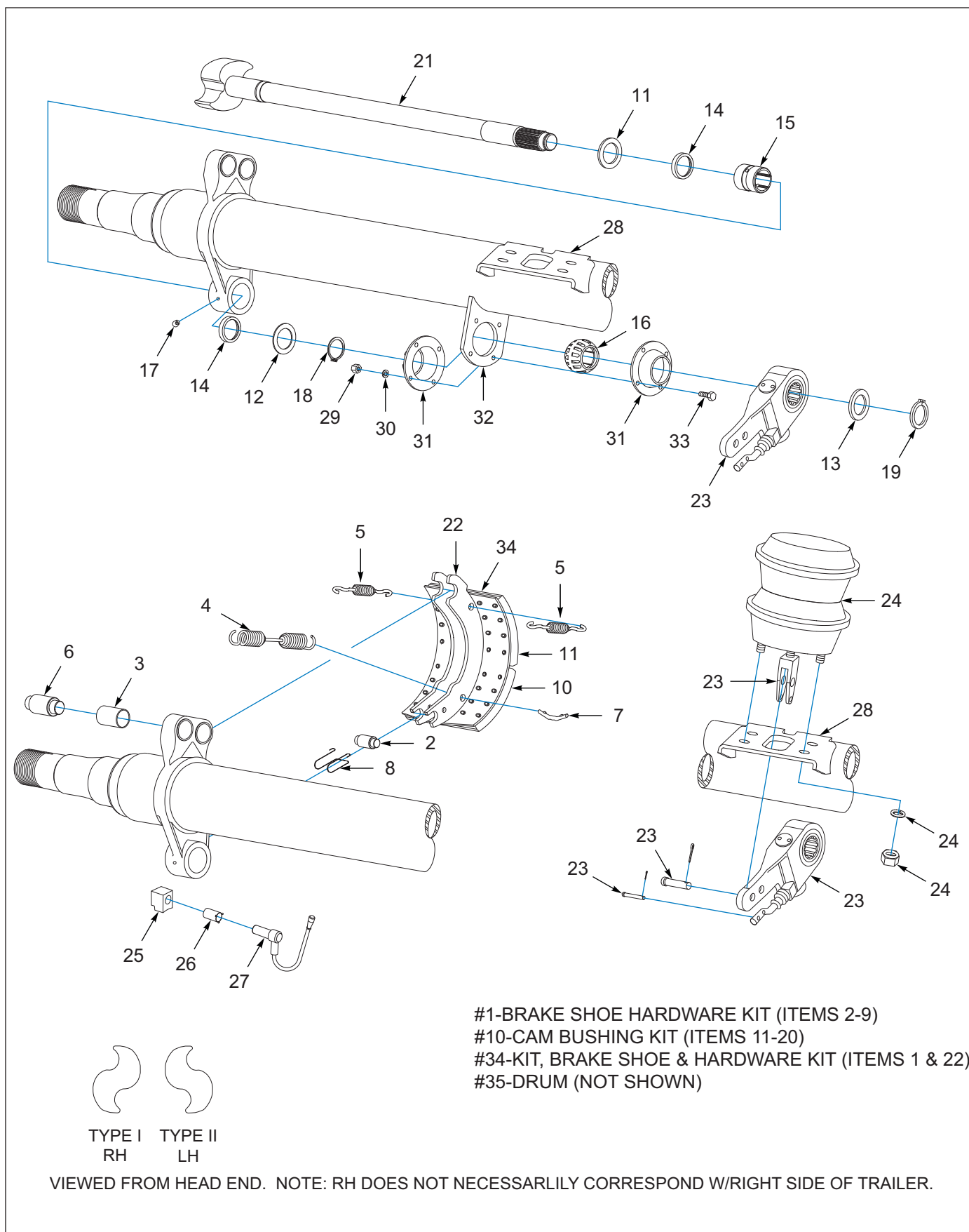
Figure 1-58: Axle 16.5 x 7 Drum Brakes, Dexter
