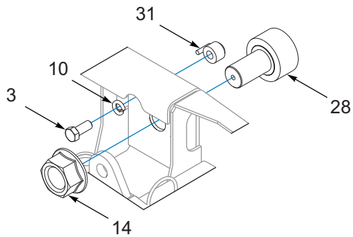
REAR CAM FOLLOWER ASSEMBLY
