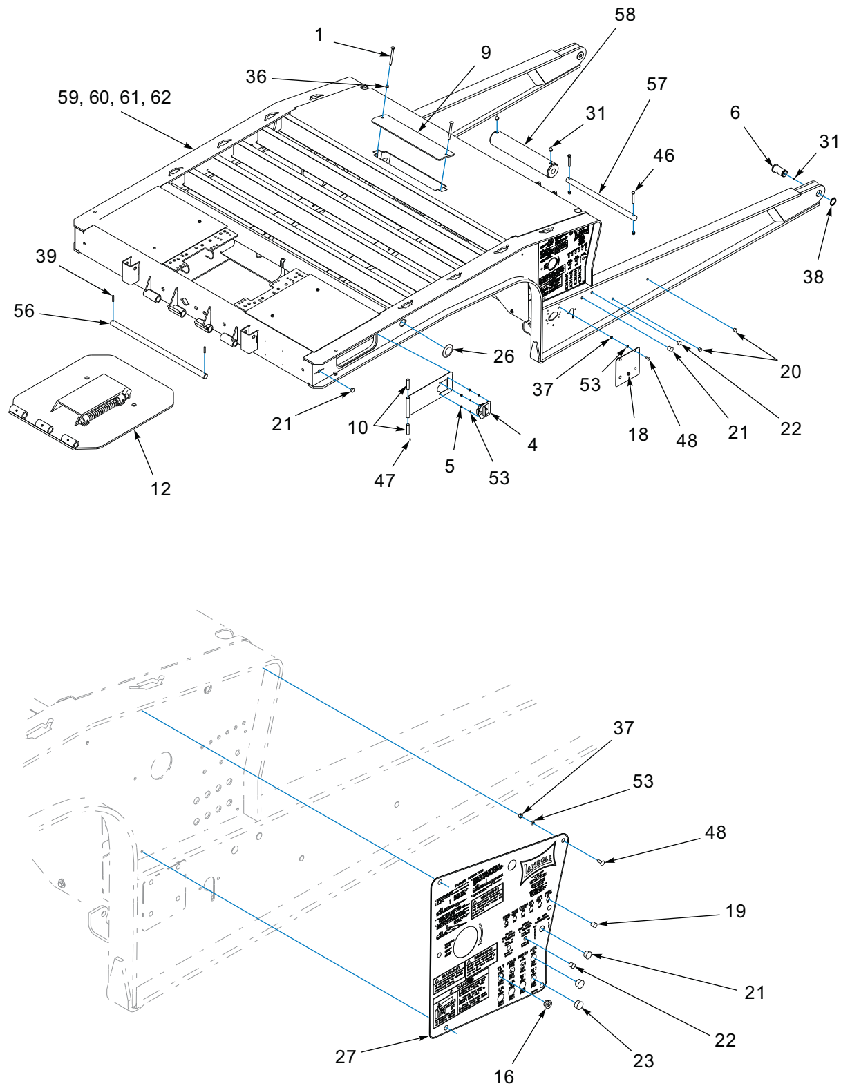
Figure 1-5: Upper Deck Assembly (1 of 3)
