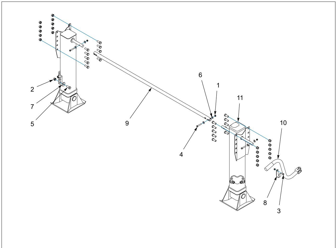
Figure 1-83: Landing Gear Installation - Jost 410
