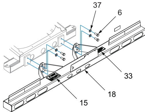
BUMPER ASSEMBLY
