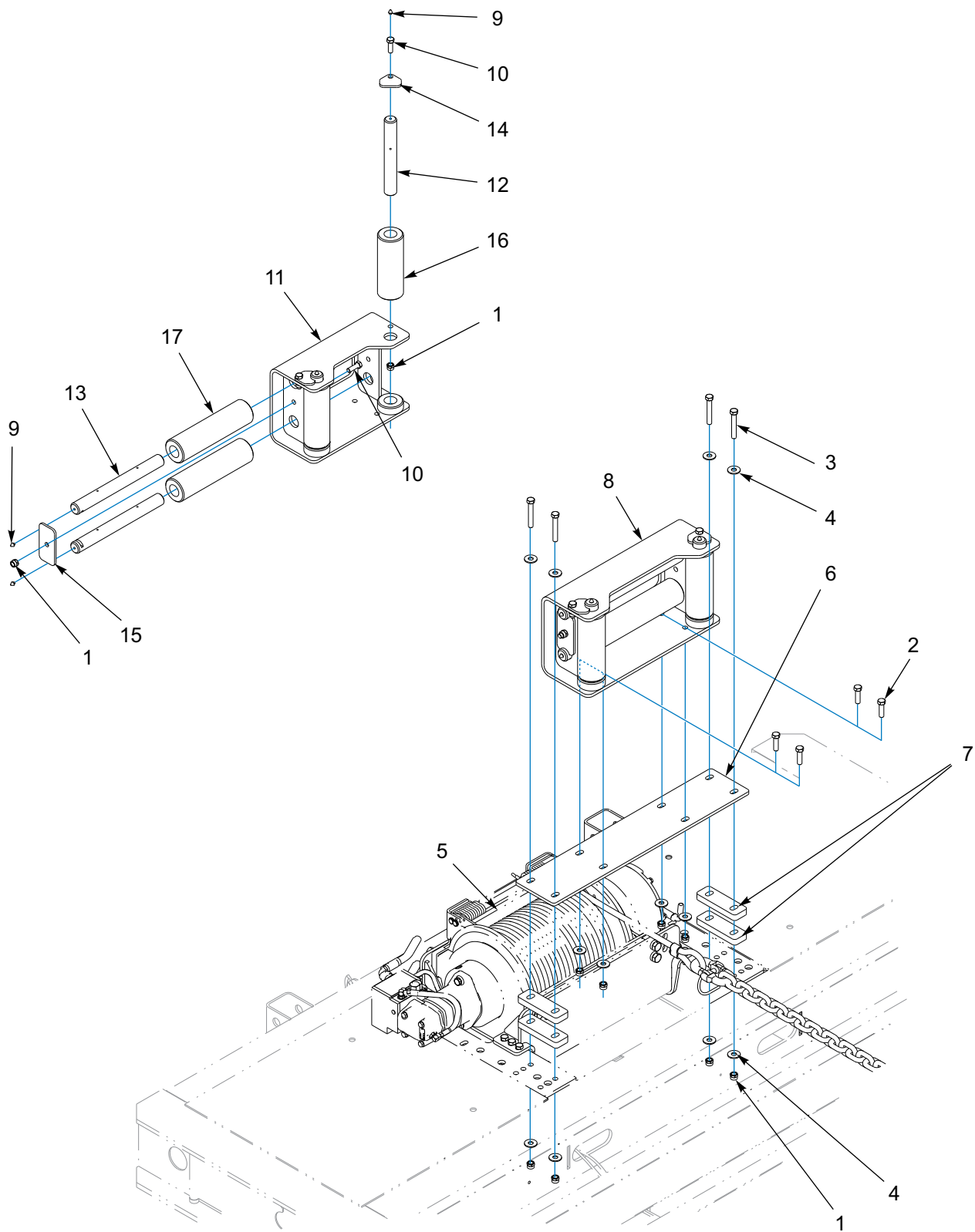
Figure 1-151: Guide Assembly, 4 Roller 20K/30K (WARN)-162258
