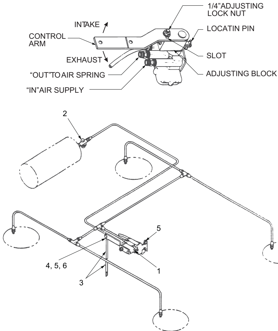
Figure 1-44: Air Control Kit - Neway
