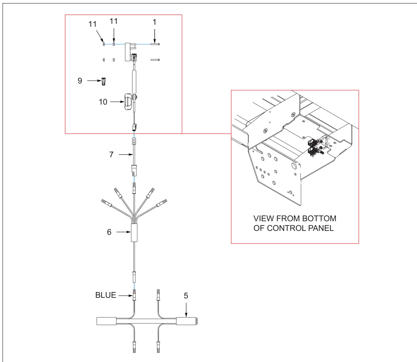
Figure 1-22: Wireless Remote Assembly, Brand (AFTER 08/01/2019)
