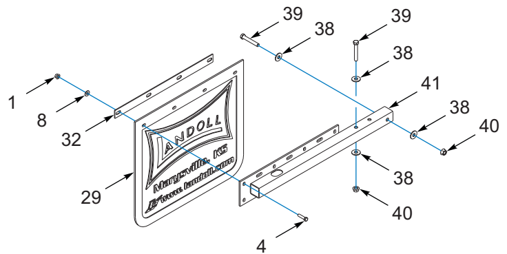
MUDFLAP ASSEMBLY
