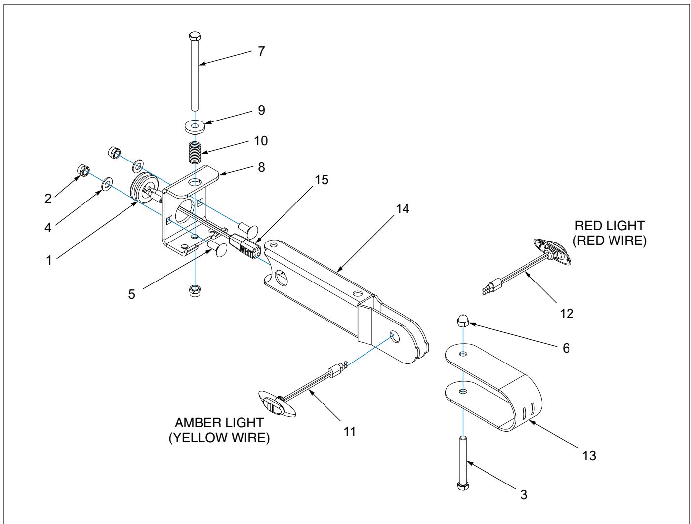
Figure 1-121: Swing-Arm Light Assembly - STREET
