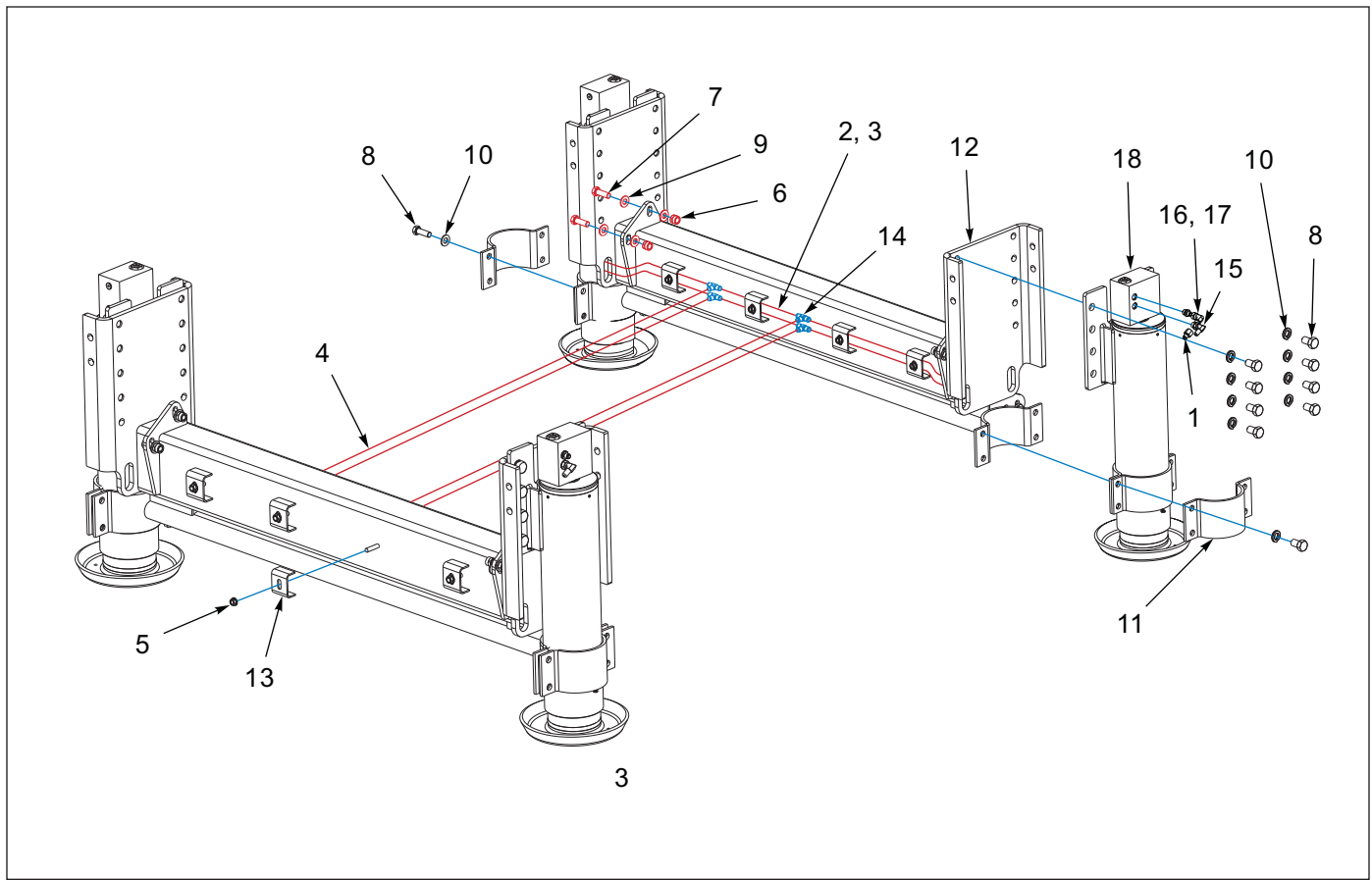
Figure 1-88: Dock Leveler Assembly - Single 120K
