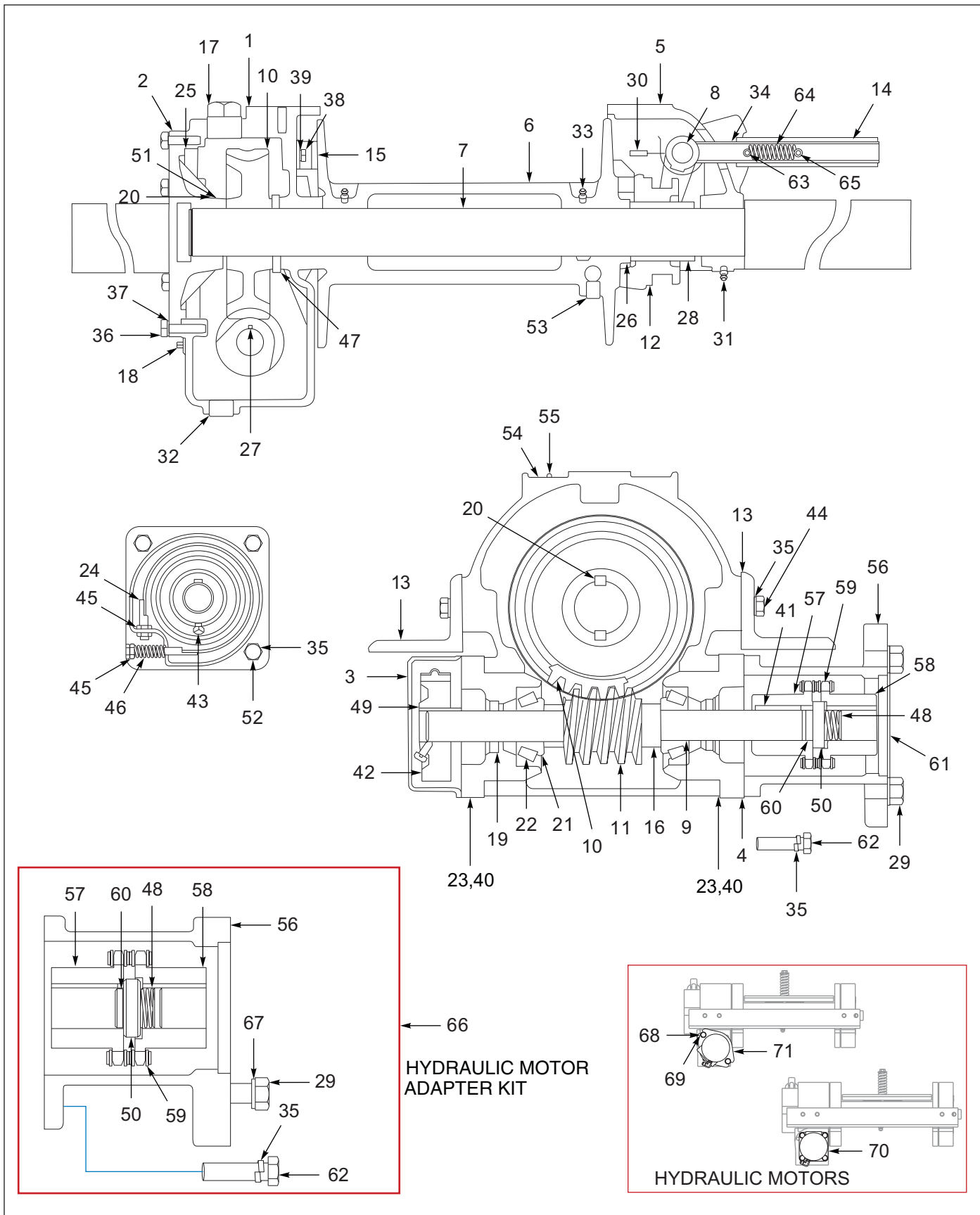
Figure 1-70: Winch Items - 12,000 Lb. (BRADEN)
