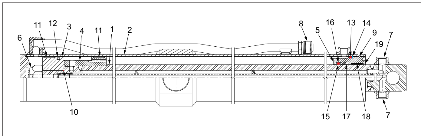
Figure 1-14: Cylinder Assembly - Ported Rod Hi Flow
