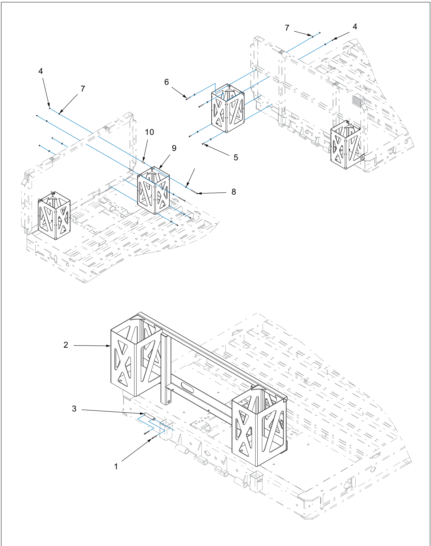
Figure 1-95: Bulkhead Installation - Special
