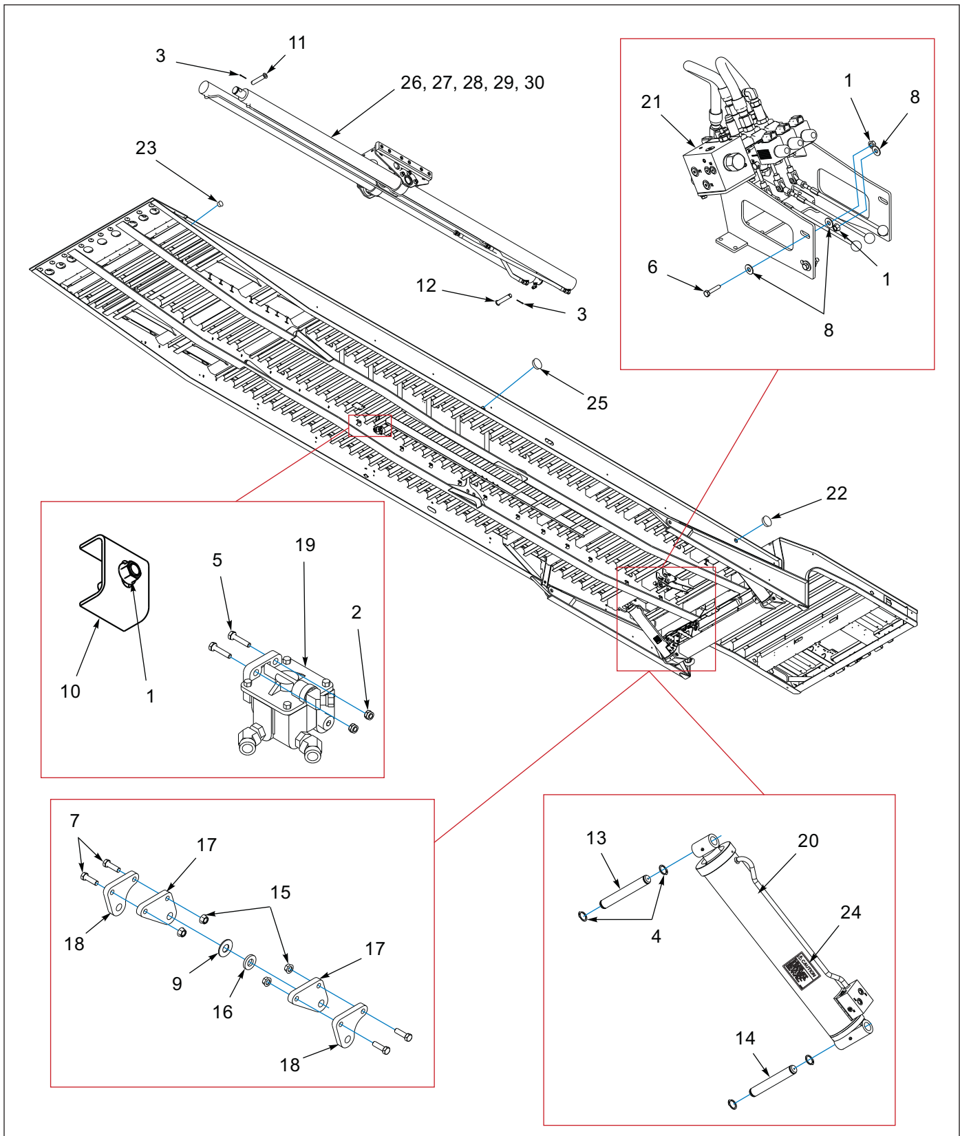
Figure 1-9: General Assembly
