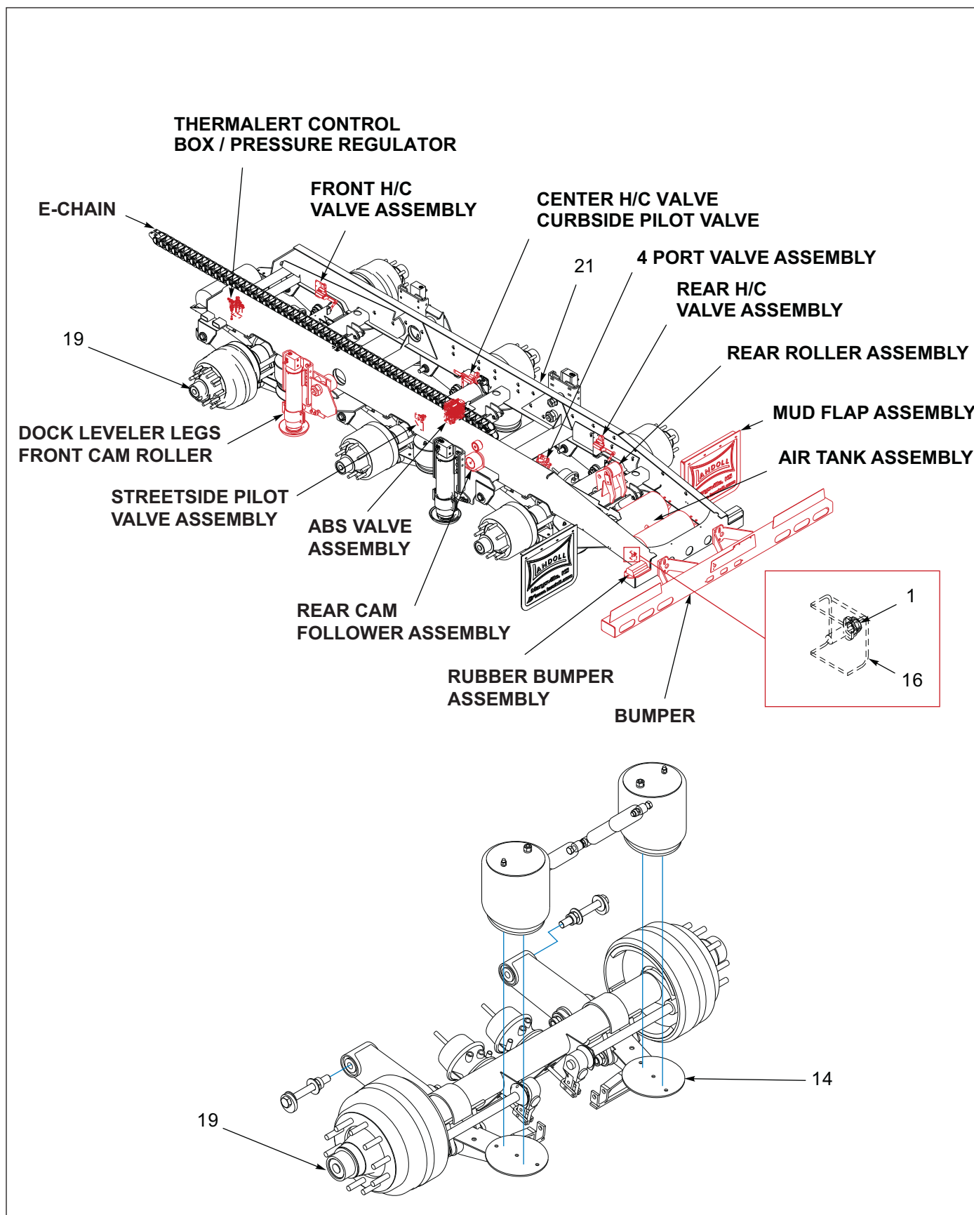
Figure 1-26: General Items - 455B (1 of 2)
