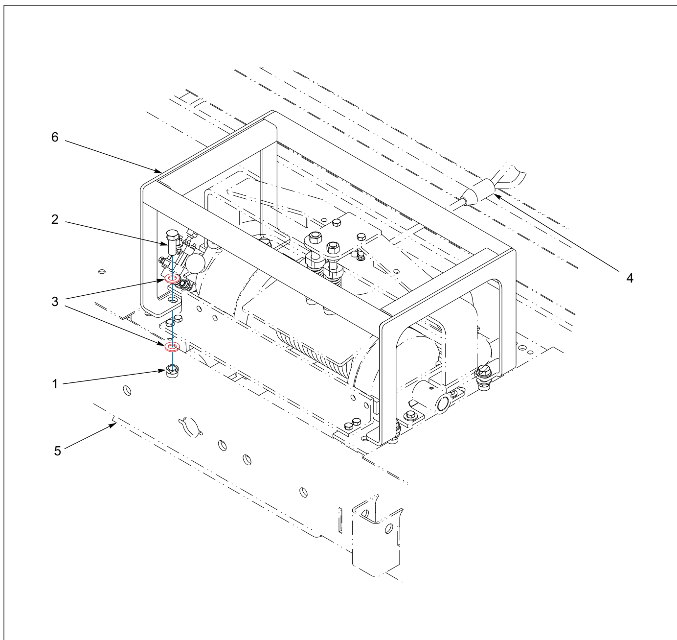
Figure 1-147: Guard Assembly, Pivot 20K-163769
