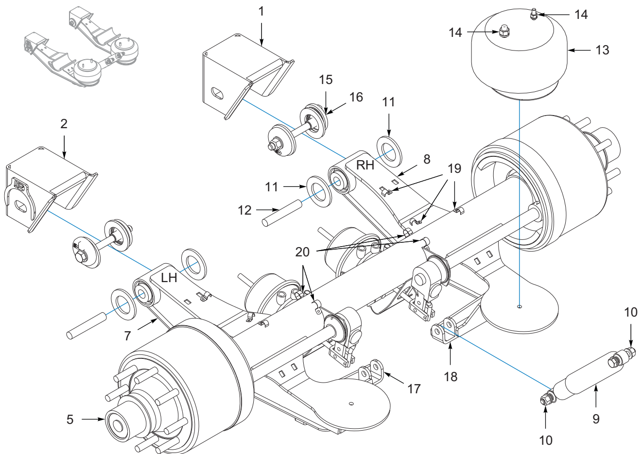
VIEW OF DRUM BRAKE ASSEMBLY
