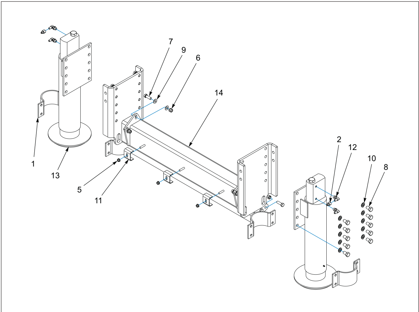
Figure 1-87: Dock Leveler Assembly - Single 60K (400-102 Big Brake)
