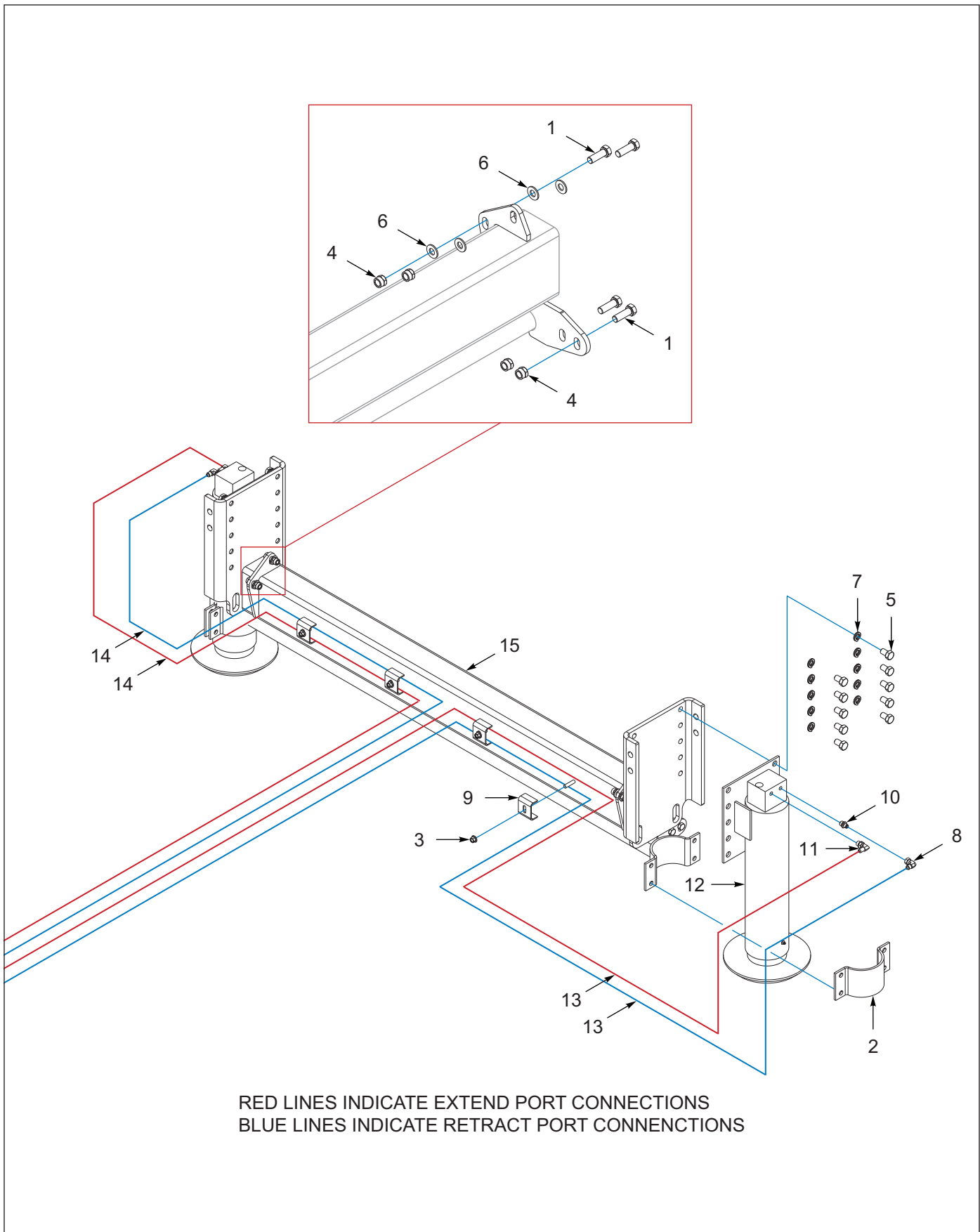
Figure 1-86: Dock Leveler Assembly - Single 60K
