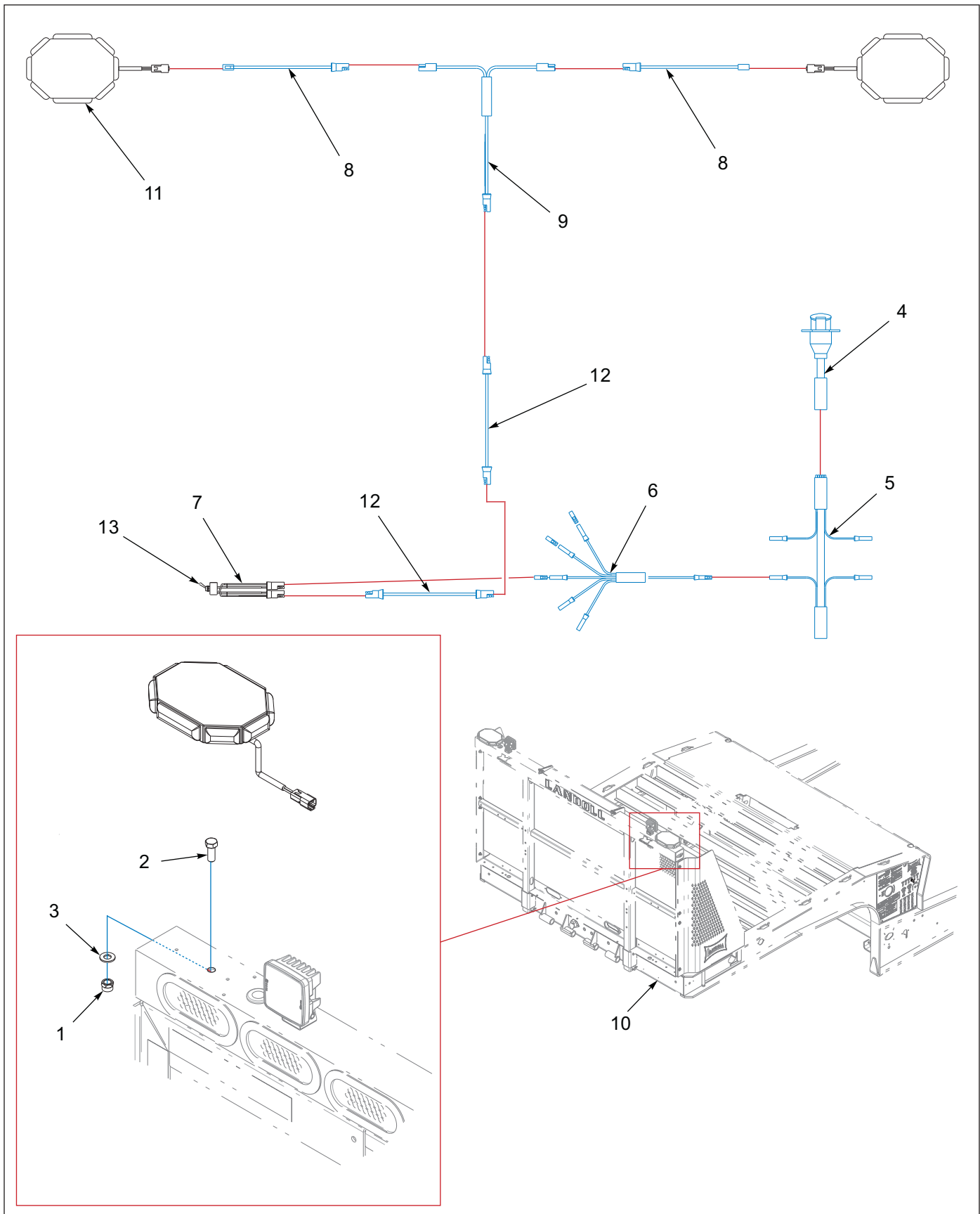
Figure 1-96: Towmate Strobe Installation
