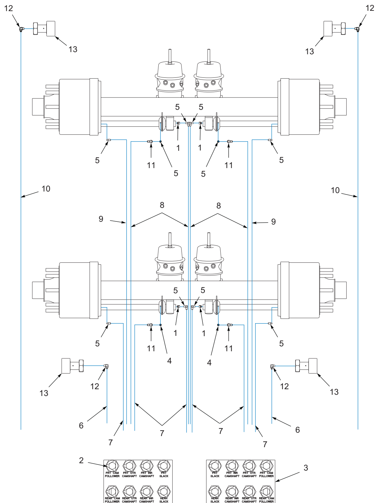
Figure 1-29: Grease System, 2 Axle (After 11/07/2018 - Before 08/31/2020)
