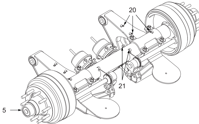
VIEW OF DRUM BRAKE CLAMP LOCATIONS (FOR BREAKDOWN SEE BELOW)
