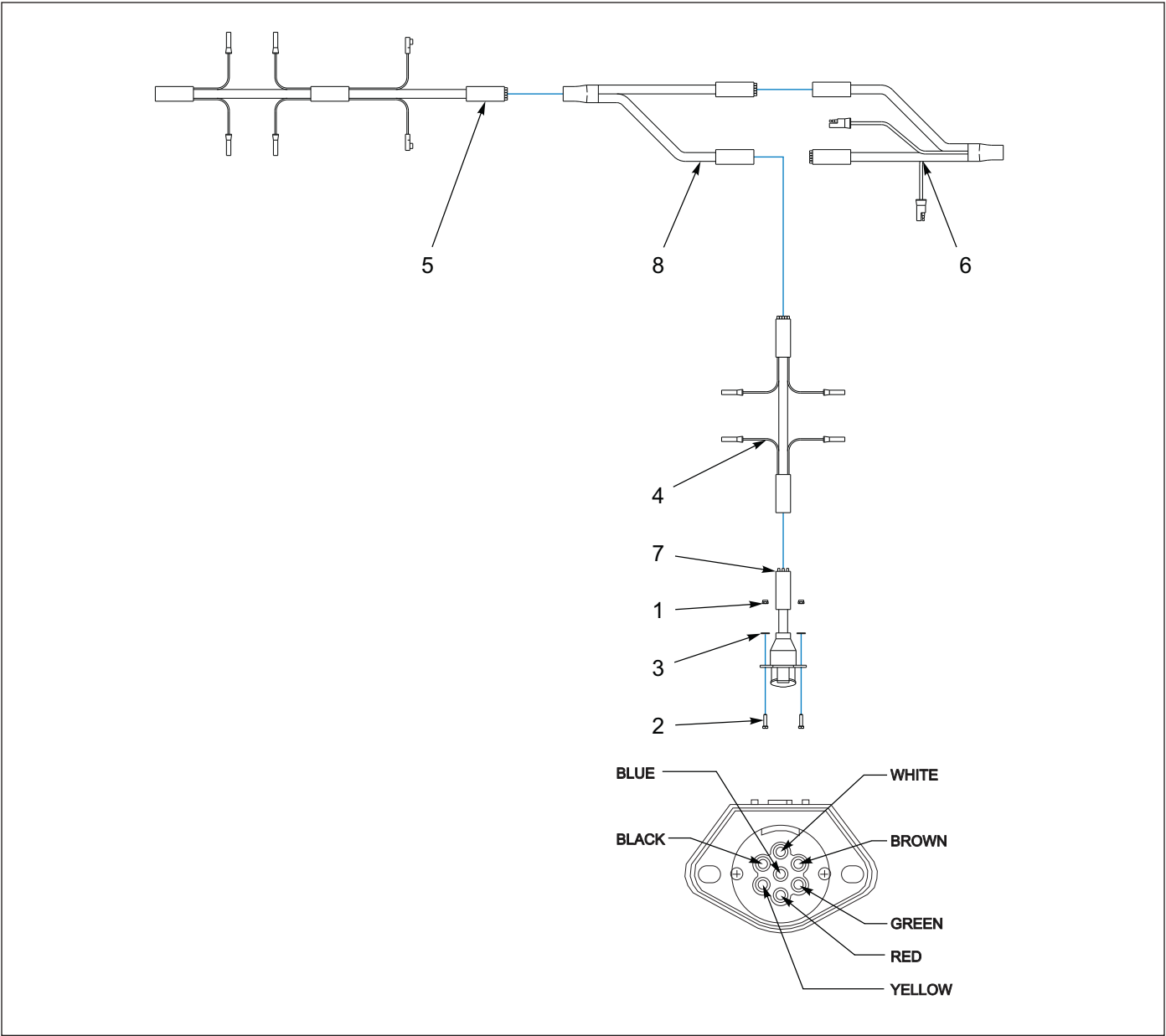
Figure 1-100: 7-Way Electrical Installation
