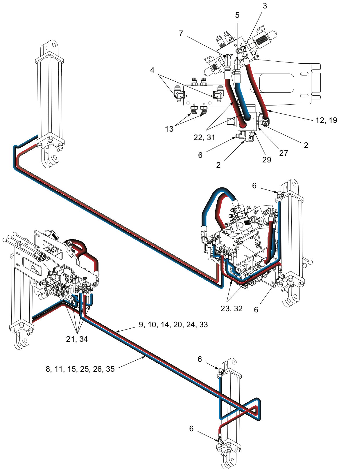
Figure 1-113: Hydraulic Park Stand - Hydraulic Items
