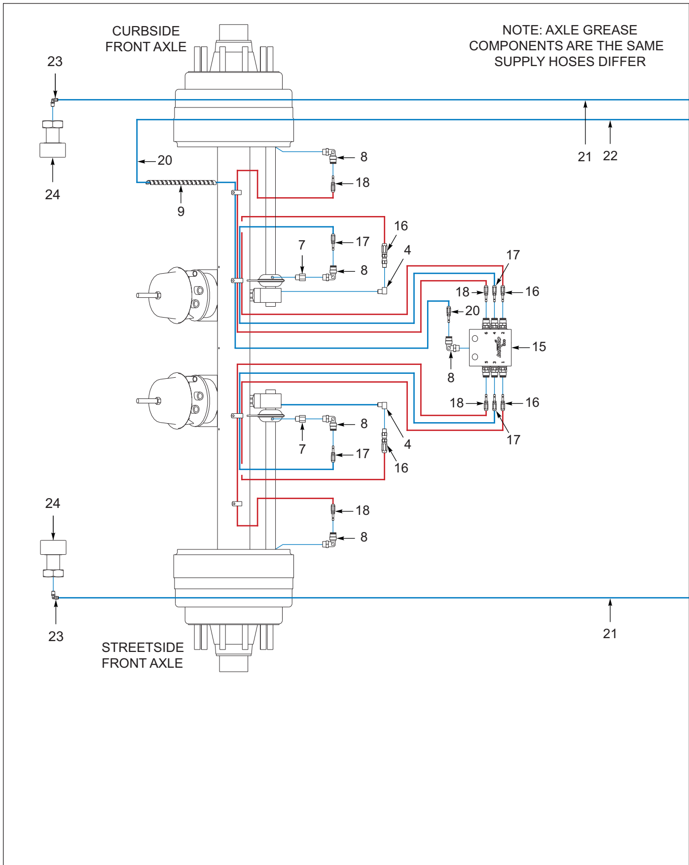
Figure 1-30: Grease System, 2 Axle (After 08/31/2020) (1 of 3)
