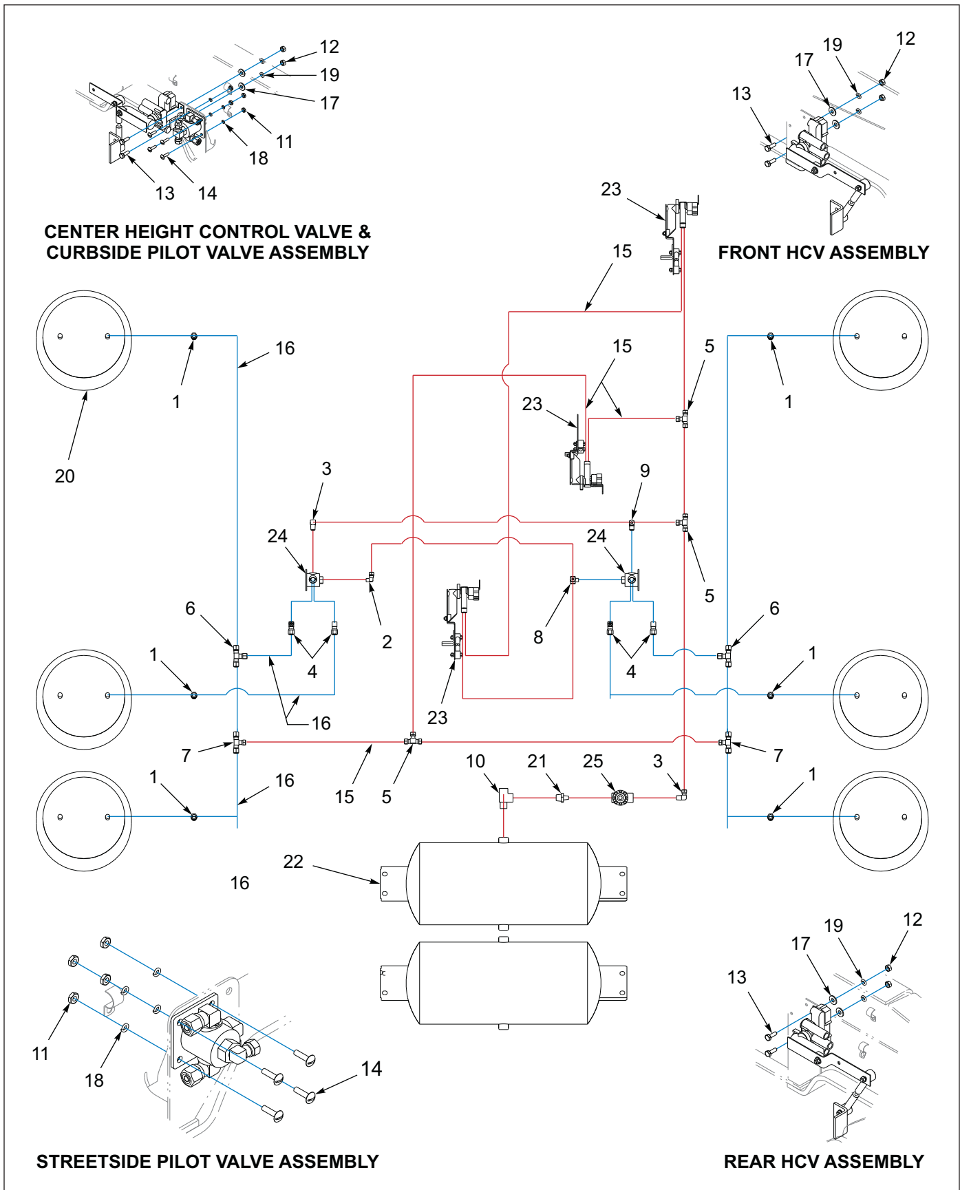
Figure 1-42: Air Ride Suspension - 455B
