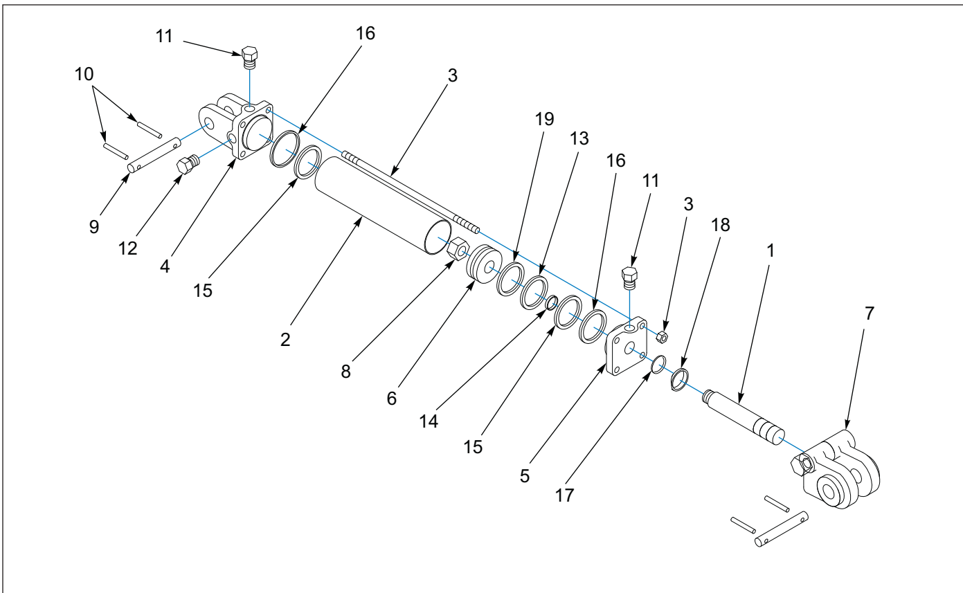
Figure 1-114: Hydraulic Cylinder - 3-1/2 X 20
