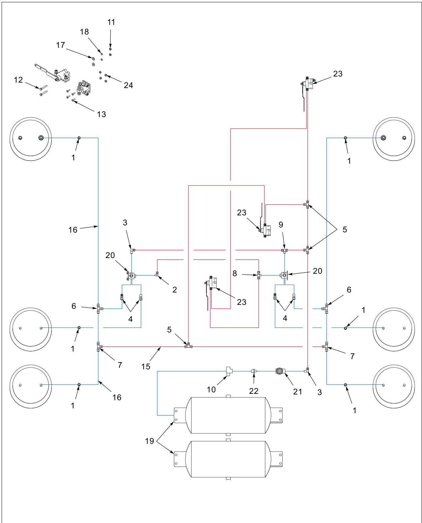
Figure 1-43: Air Ride Suspension - 440B Aqua
