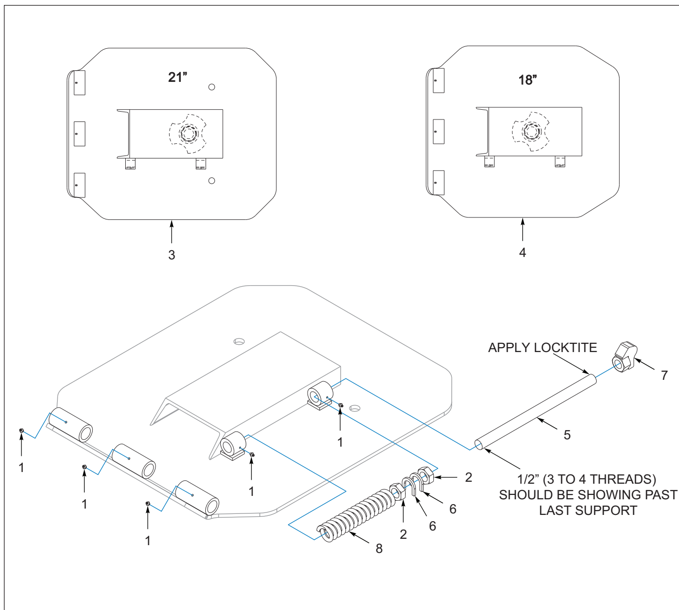
Figure 1-8: Hitch Plate Assembly
