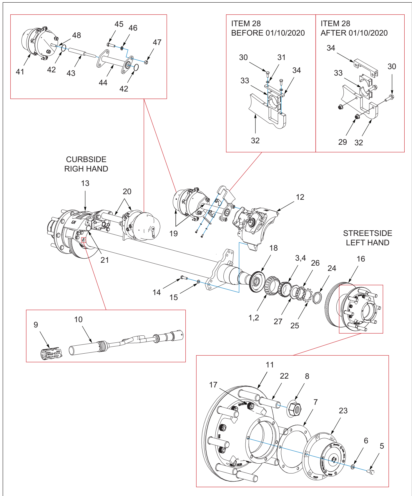
Figure 1-52: Axle 12.25 Disc Brakes & Hub Assembly, Dexter (OPTION) (1 of 2)
