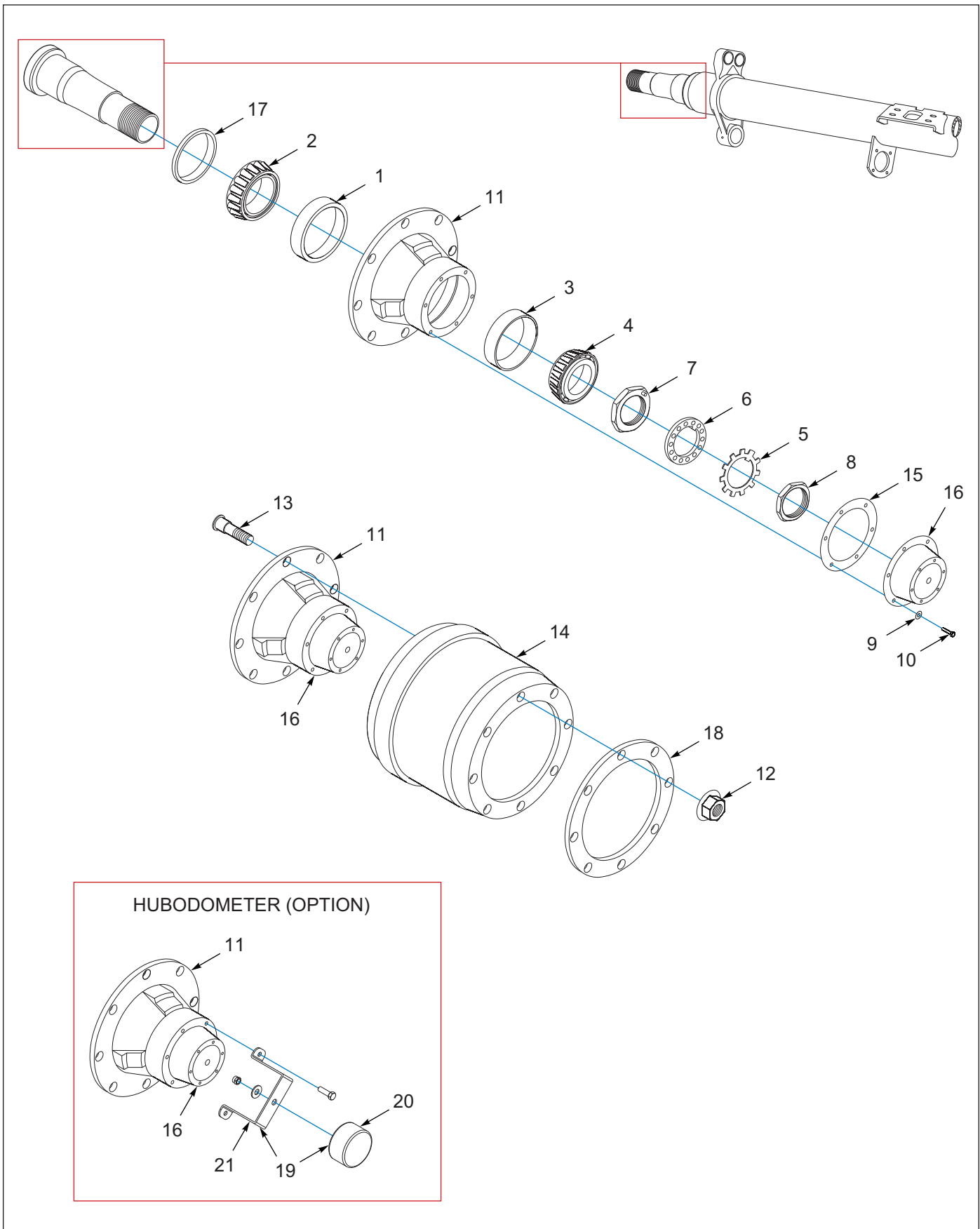
Figure 1-55: Axle 12.25 x 7.5 Drum and Hub Assembly
