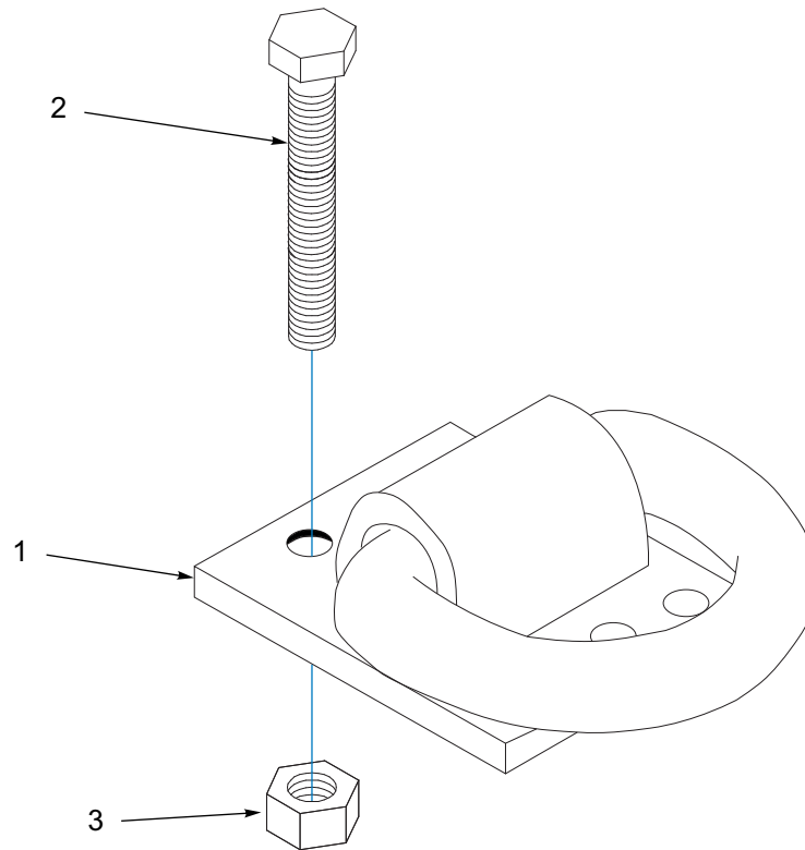
Figure 1-152: Tie Down Assembly, D-Ring-3-793-010041
