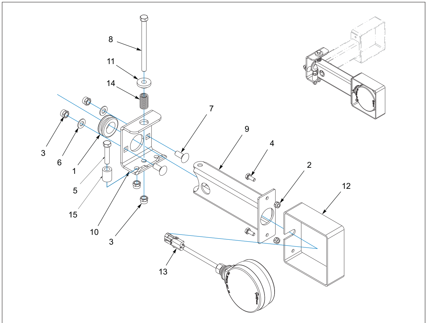
Figure 1-119: Swing-Arm Light Assembly - Turn Signal/Emergency Flasher
