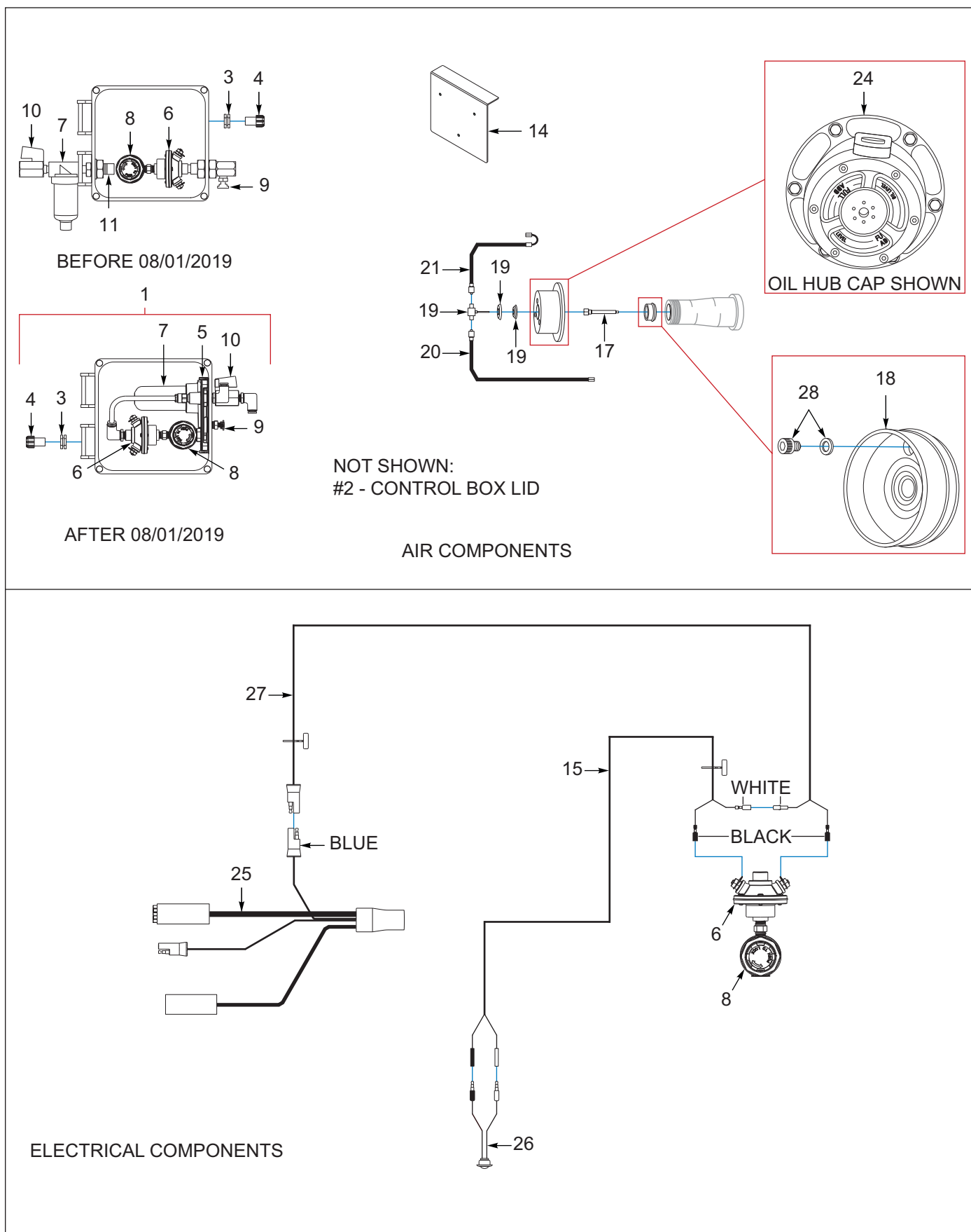
Figure 1-67: Thermalert Electrical System &amp; Components (OPTION)
