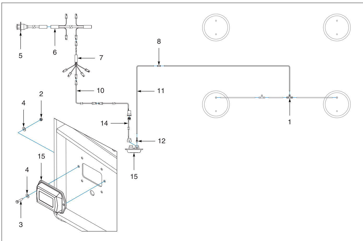
Figure 1-130: QUICKLOAD PLUS-226657 (After 03/31/2020)
