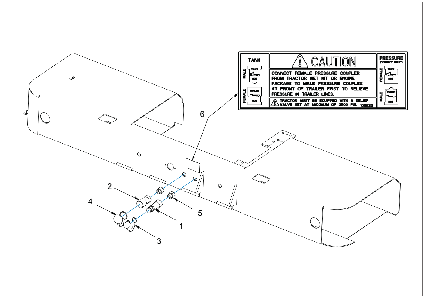
Figure 1-111: Hydraulic Conversion Kit - Ball to Flat
