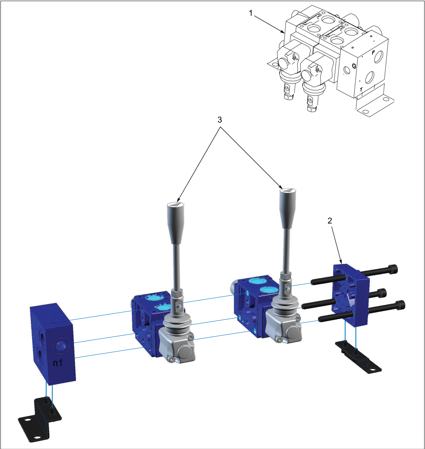
Figure 1-91: Dock Leveler Valve
