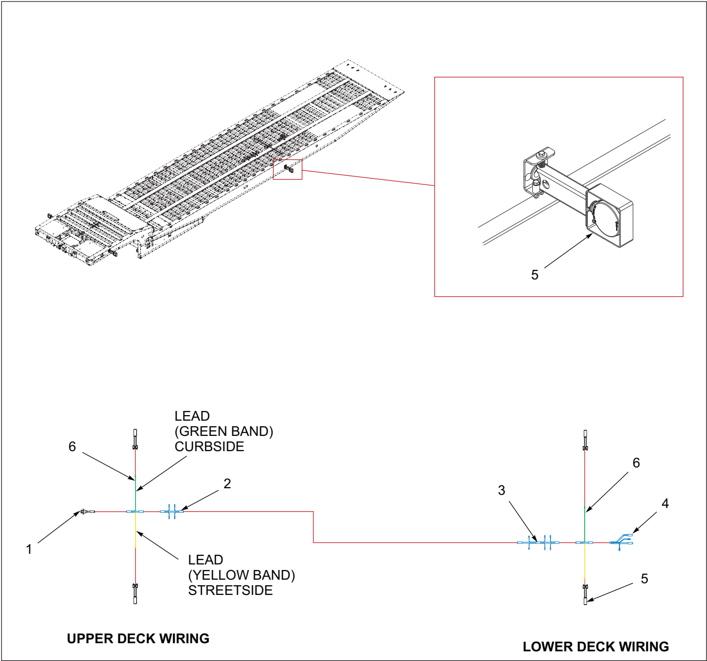
Figure 1-118: Swingout Light Installation
