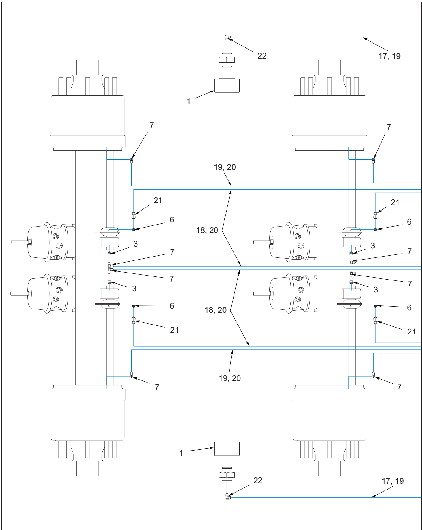
Figure 1-35: Grease System, 3 Axle (After 11/07/2018 - Before 08/31/2020) (1 of 2)
