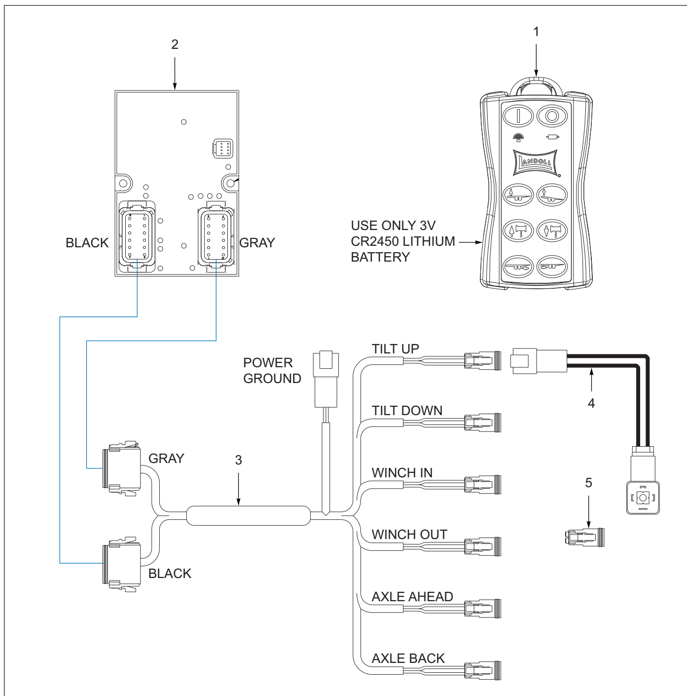
Figure 1-23: Wireless Remote Assy, Kit Components, Brand (AFTER 08/01/2019)
