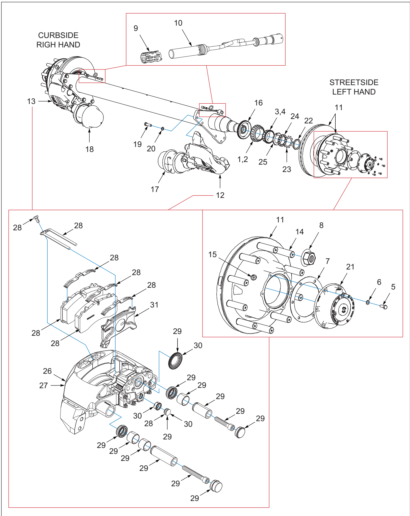
Figure 1-56: Axle 16.5 Disc Brakes & Hub Assembly, Dexter (OPTION) (1 of 2)
