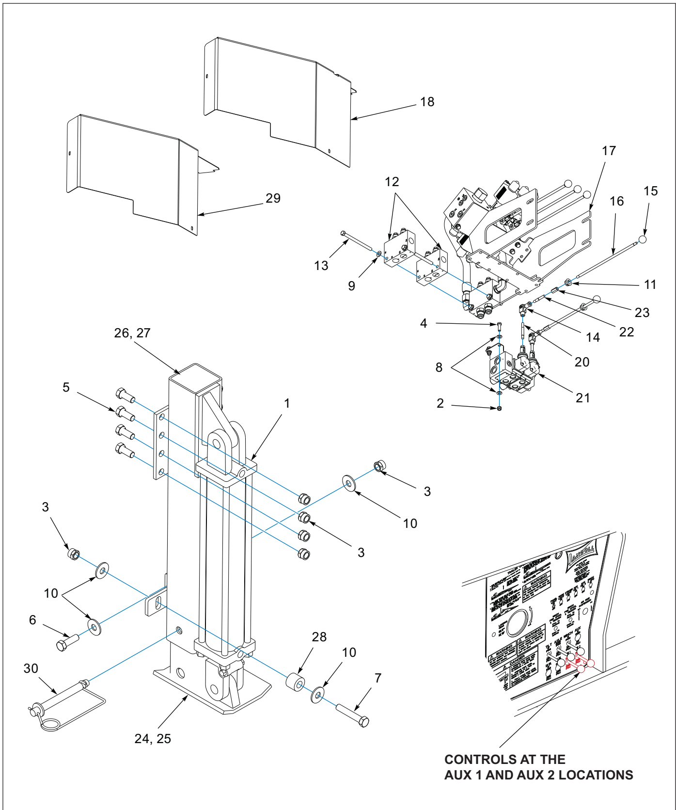
Figure 1-112: Hydraulic Park Stand - General Items
