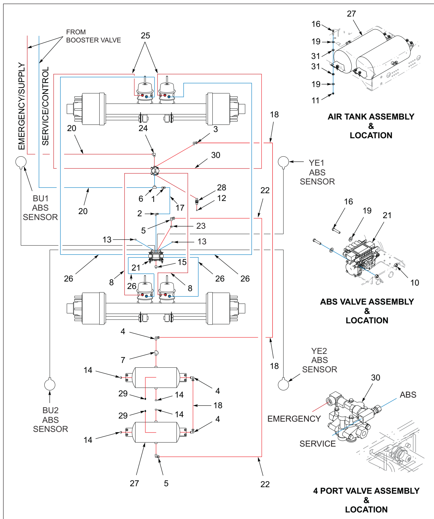
Figure 1-60: Air Brake System, 440B
