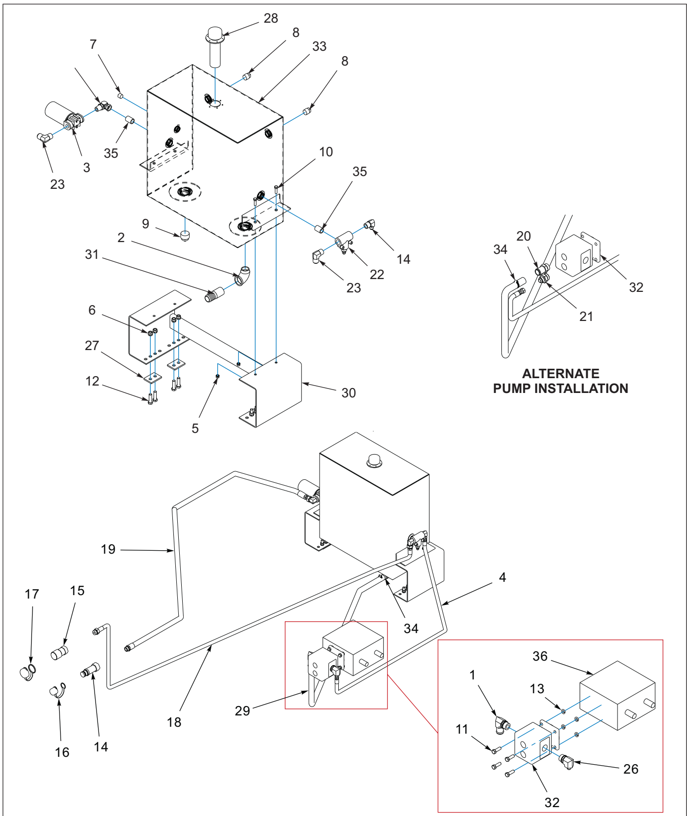
Figure 1-109: Hydraulic Wet Kit Items - 30 Gallon
