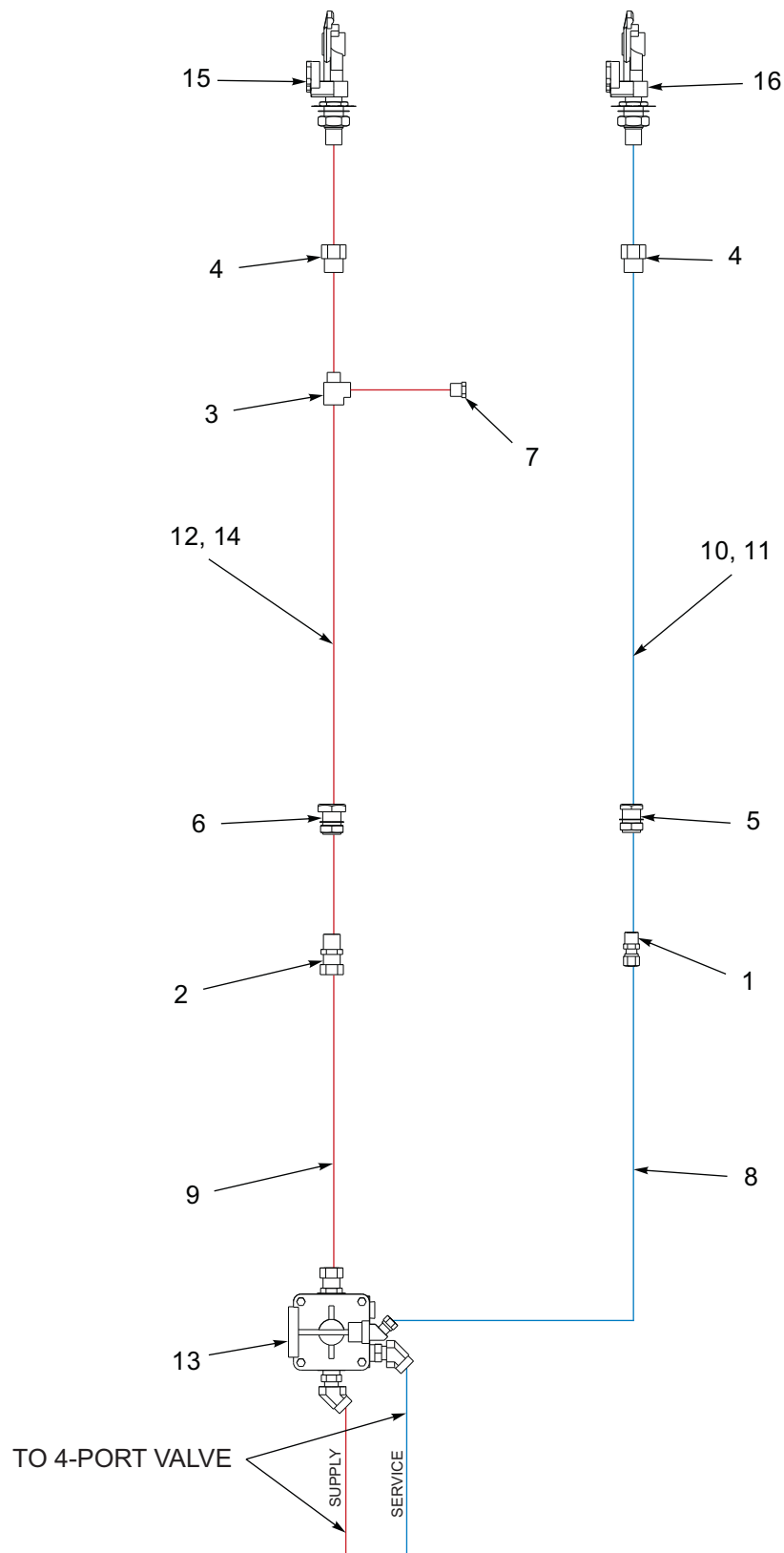
Figure 1-11: Air System
