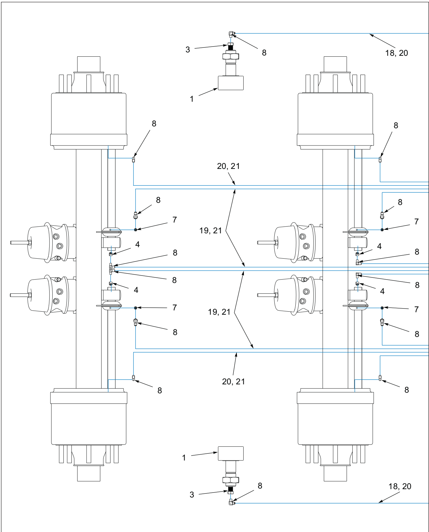
Figure 1-33: Grease System, 3 Axle (Before 11/07/2018) (1 of 2)
