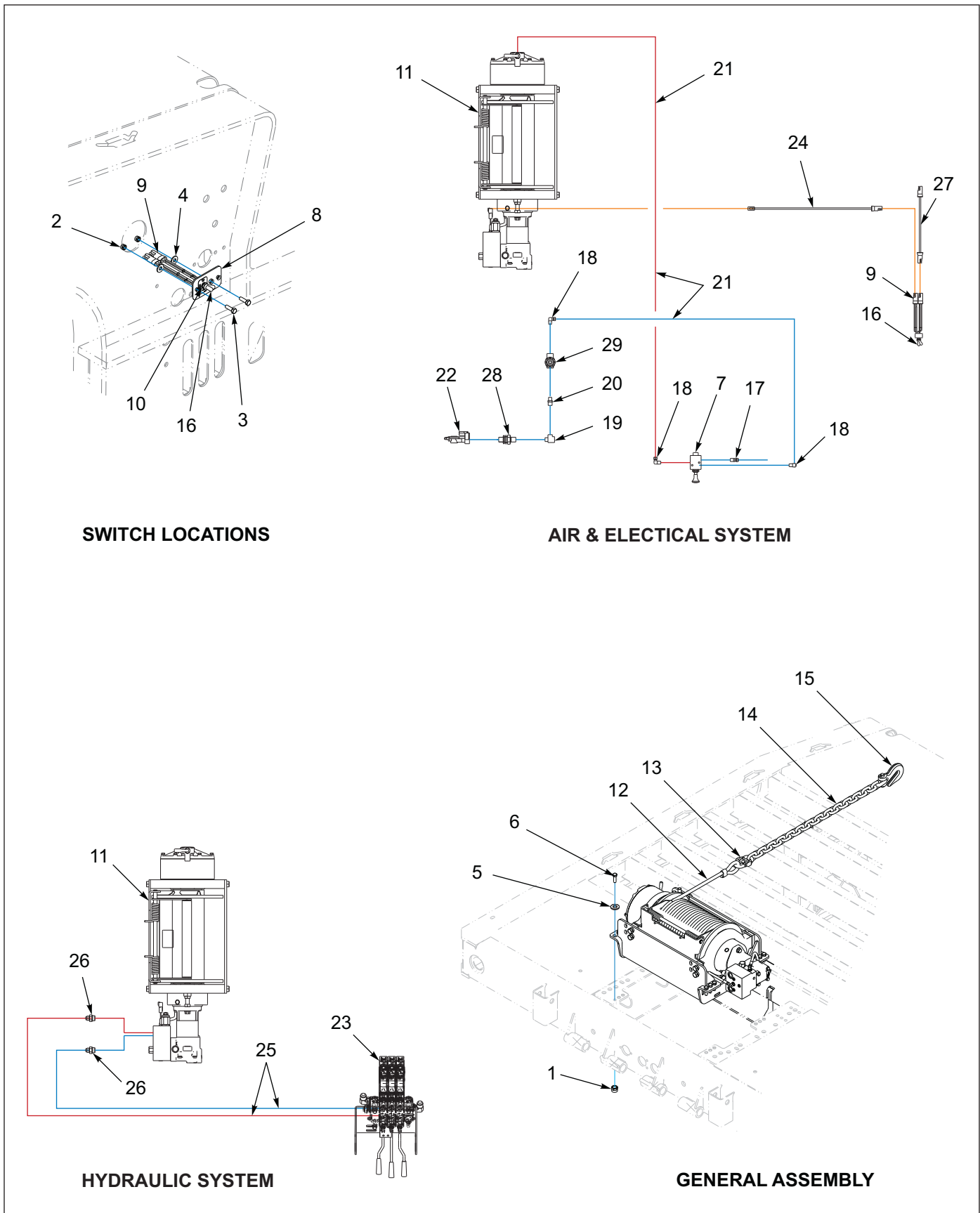
Figure 1-80: 30K 2 Speed (WARN)
