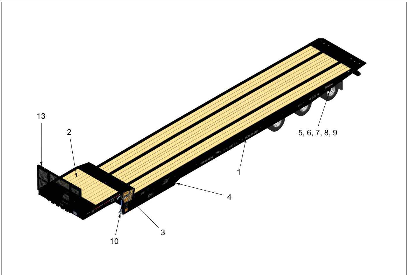
Figure 1-2: General Assembly
