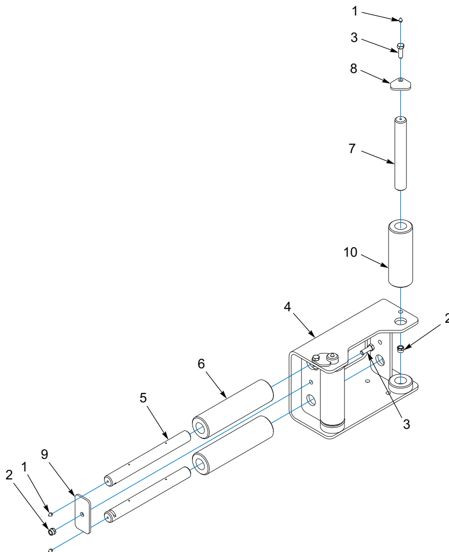
Figure 1-149: Guide Assembly Components, 4 Roller 12K (BRADEN)-161150
