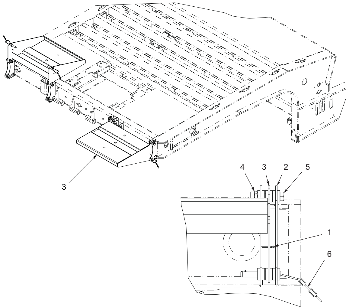
Figure 1-141: Front Flip Extension-103538, 174253, 197164
