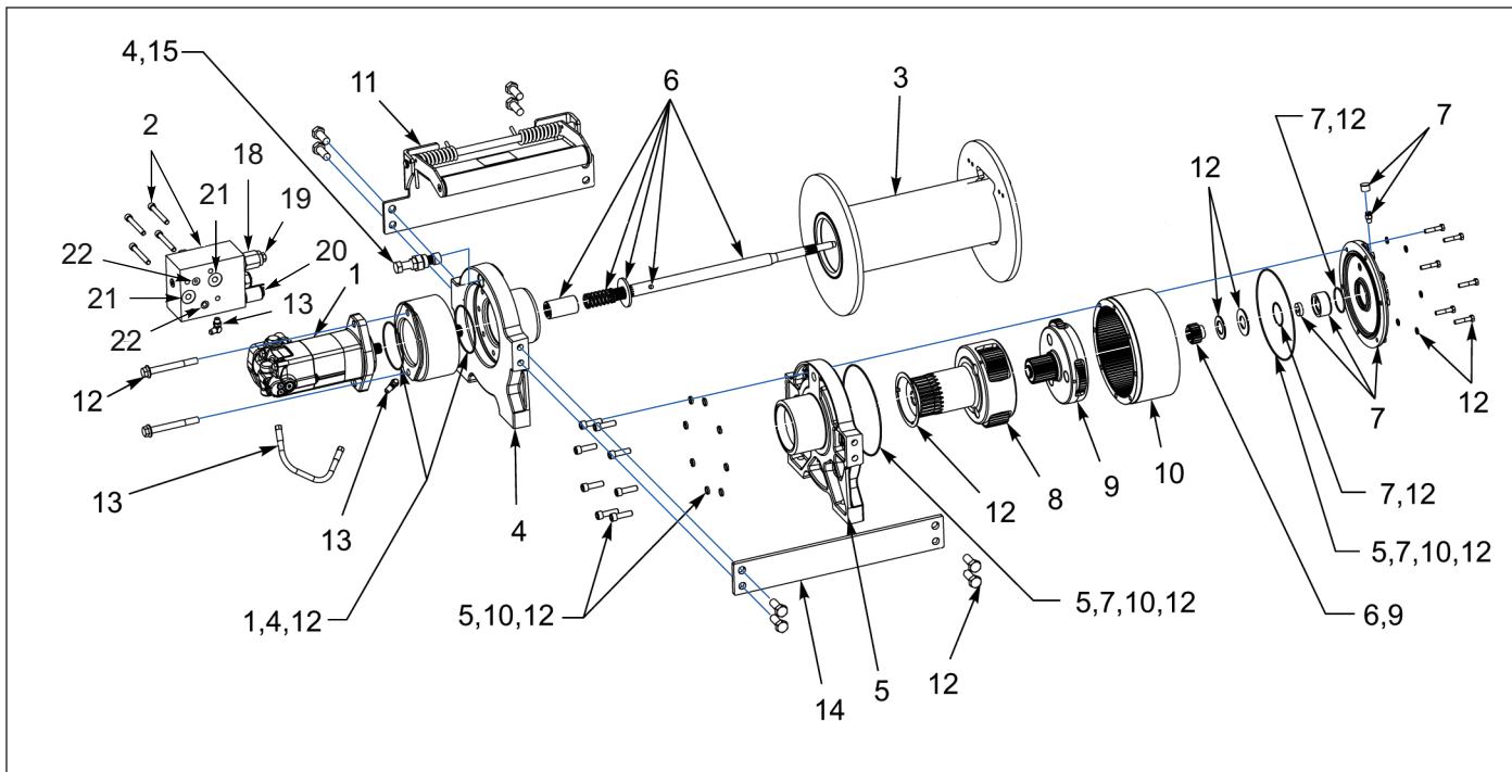
Figure 1-79: Winch Items - 20K 2 Speed (WARN)
