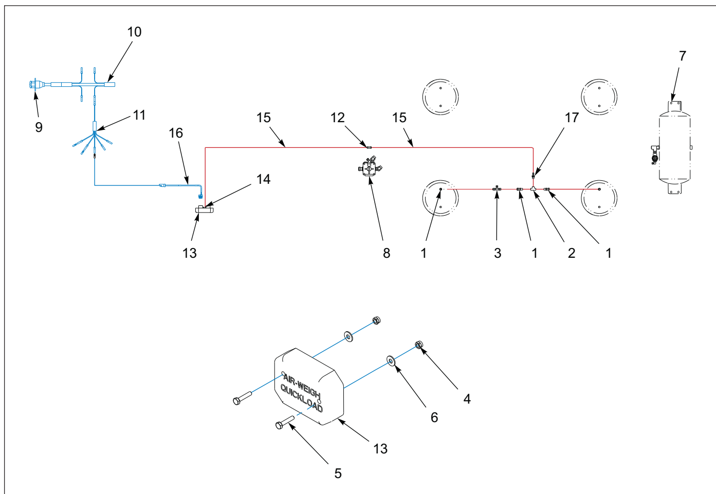
Figure 1-128: QUICKLOAD-175358 (Replaced by 226657, 226661)
