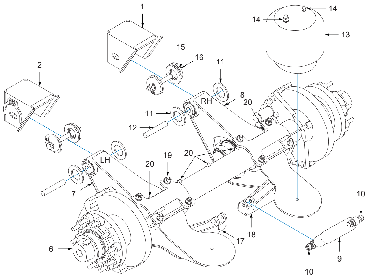
VIEW OF DISC BRAKE ASSEMBLY (OPTION)
