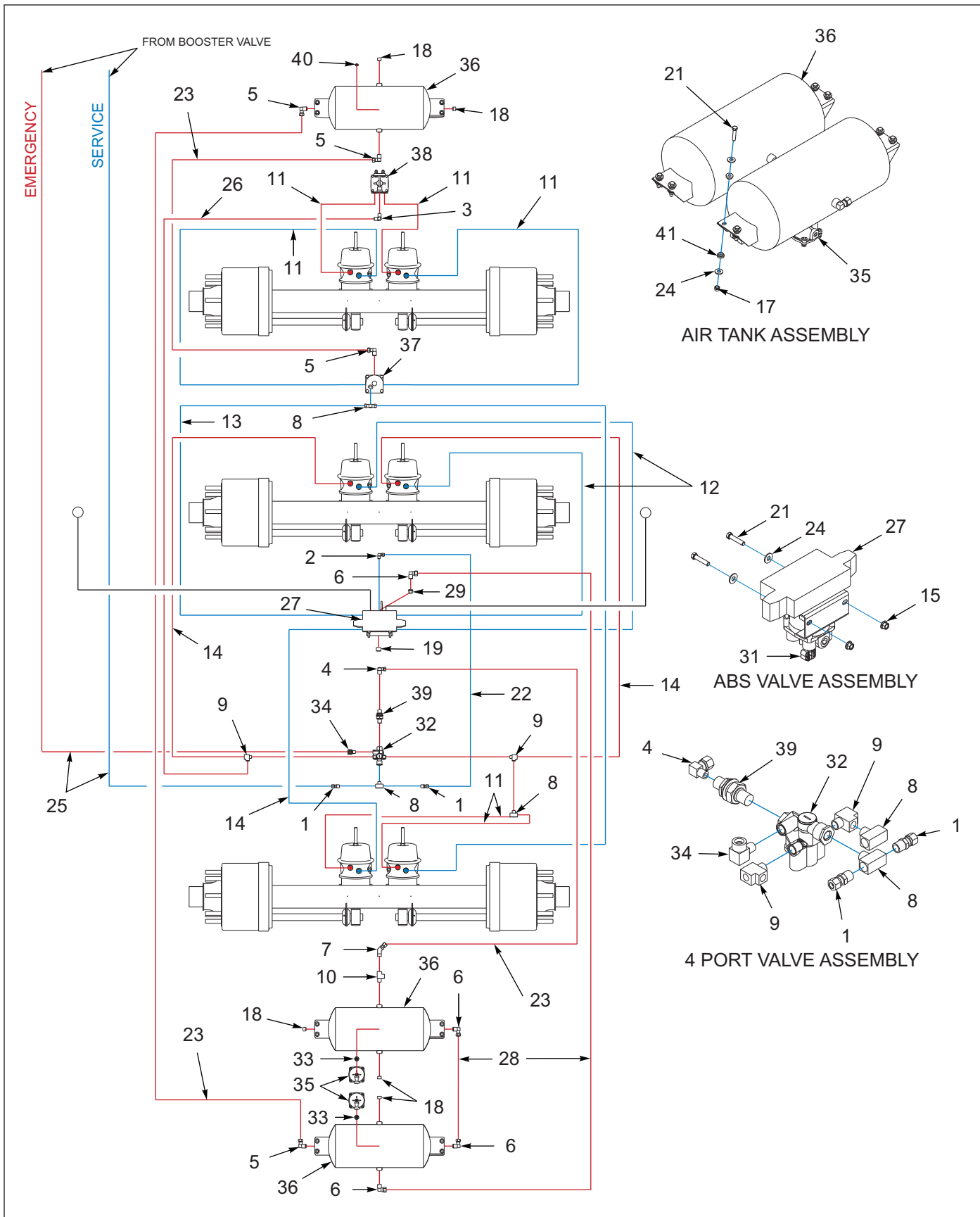
Figure 1-63: 455B Air Brakes - Aqua Package
