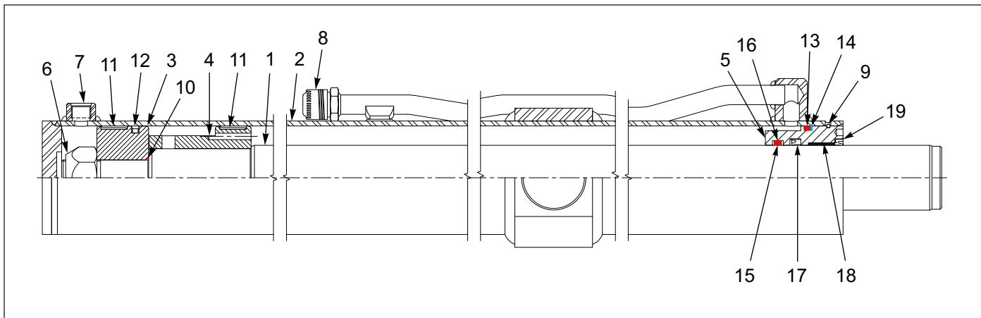
Figure 1-13: Cylinder Assembly - Hi Flow
