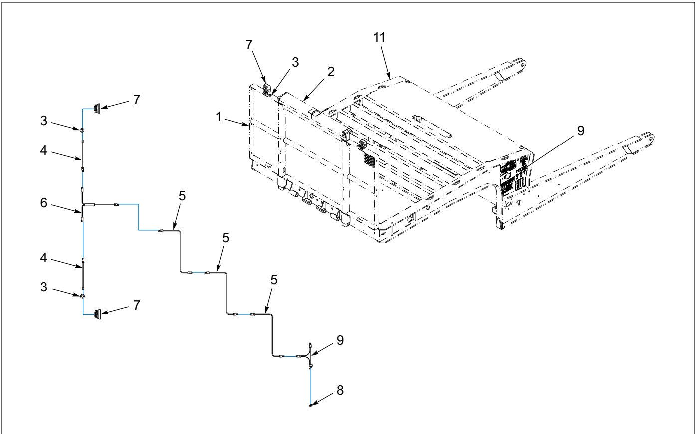
Figure 1-97: Bulkhead - Work Light Installation
