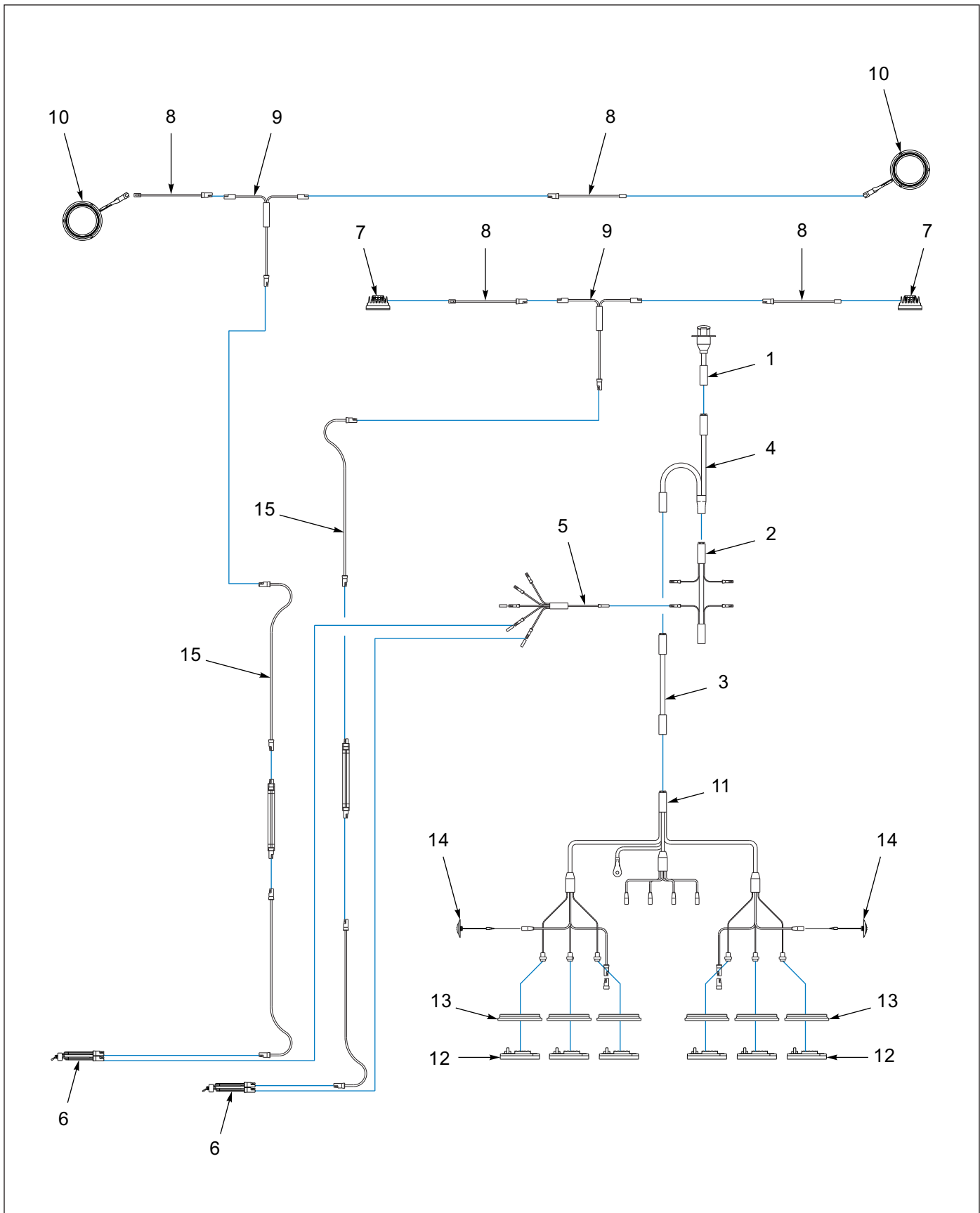
Figure 1-94: Bulkhead - Chain Rack Lights Electrical System
