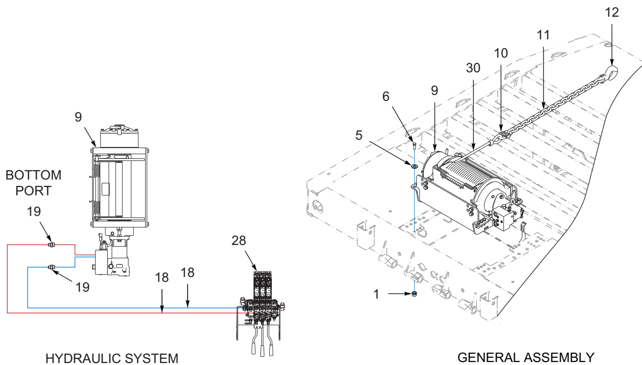
Figure 1-78: Winch Installation - 20K 2 Speed (Warn)
