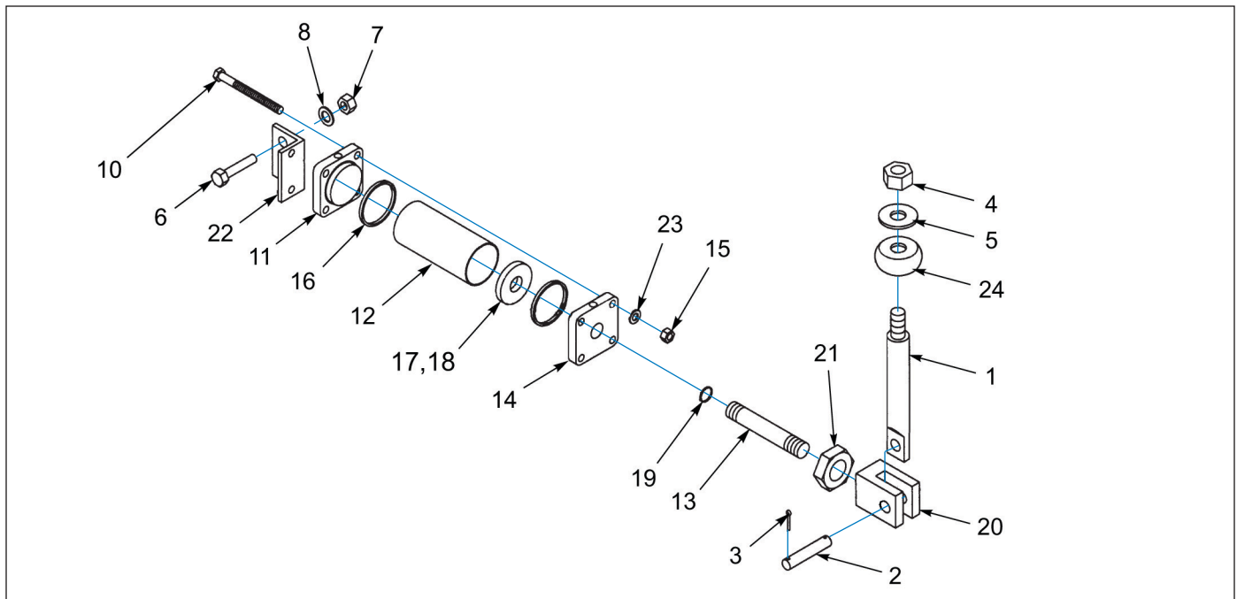
Figure 1-76: Winch - Air Shift Cylinder
