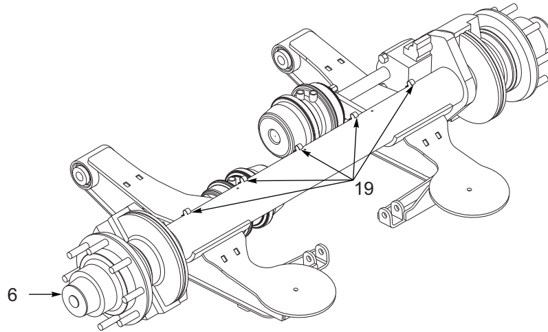
VIEW OF DISC BRAKE ASSEMBLY (OPTION) CLAMP LOCATIONS (FOR BREAKDOWN SEE BELOW)
