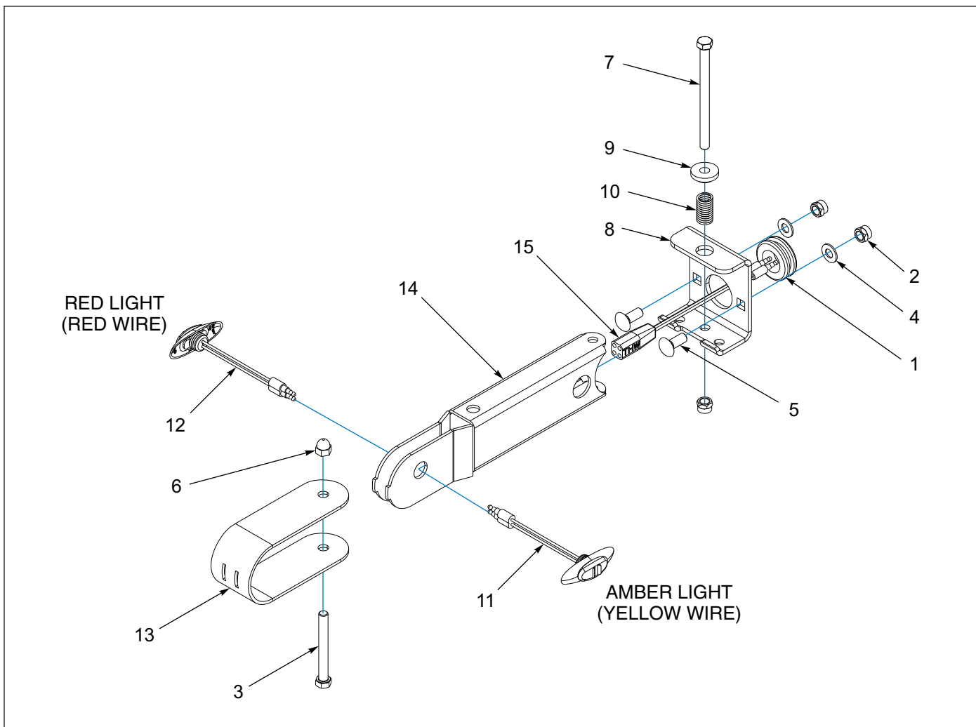
Figure 1-122: Swing-Arm Light Assembly - CURB
