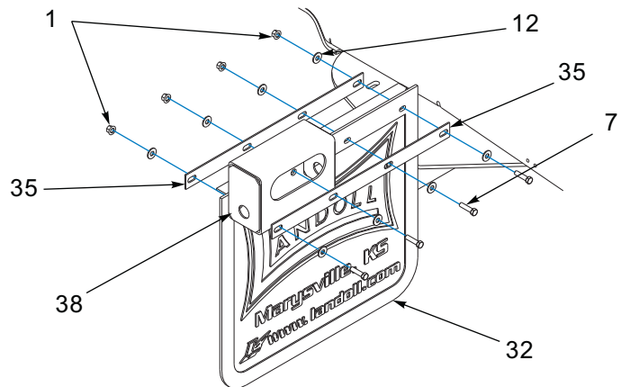
MUDFLAP ASSEMBLY
