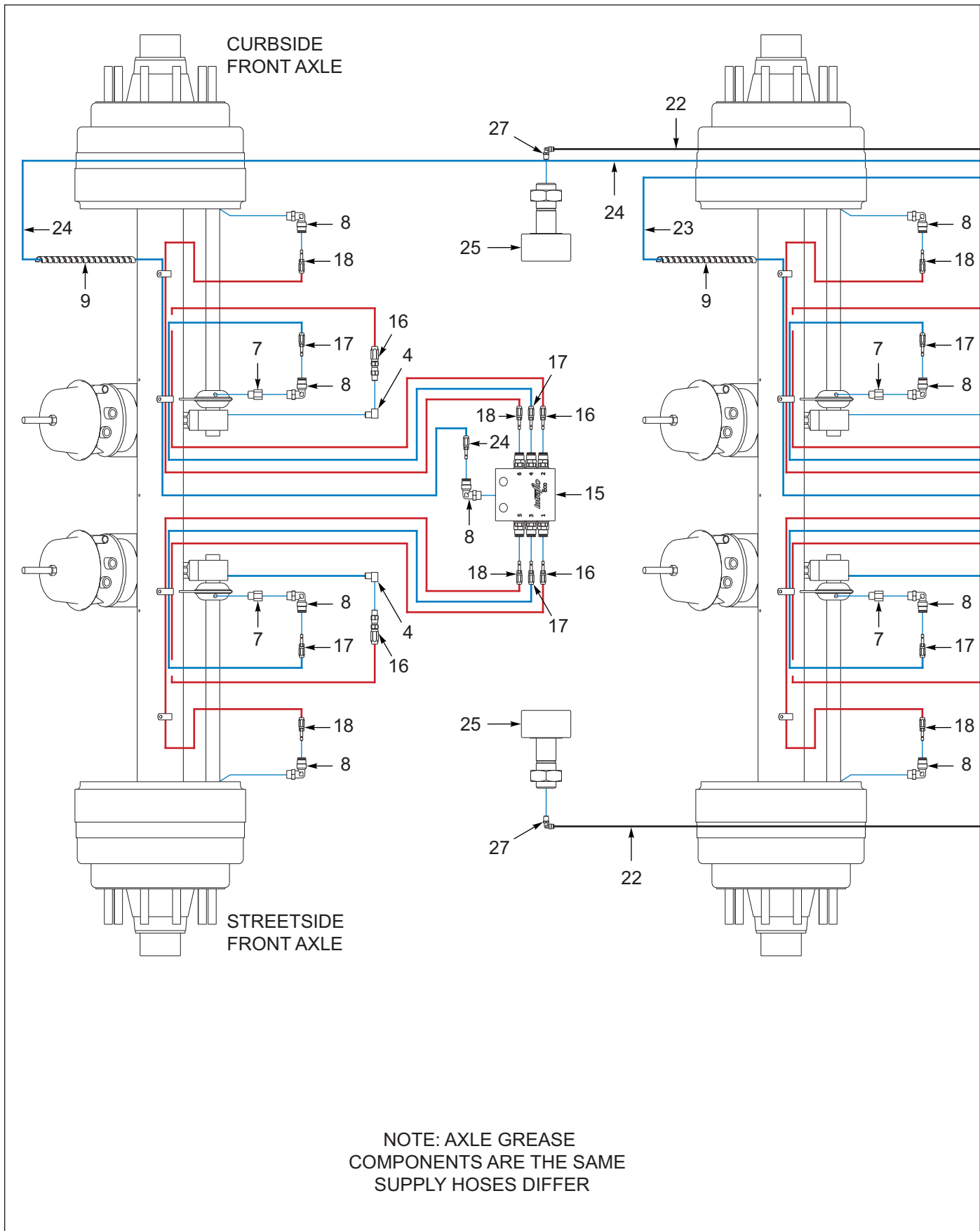
Figure 1-37: Grease System, 3 Axle (After 08/31/2020) (1 of 3)
