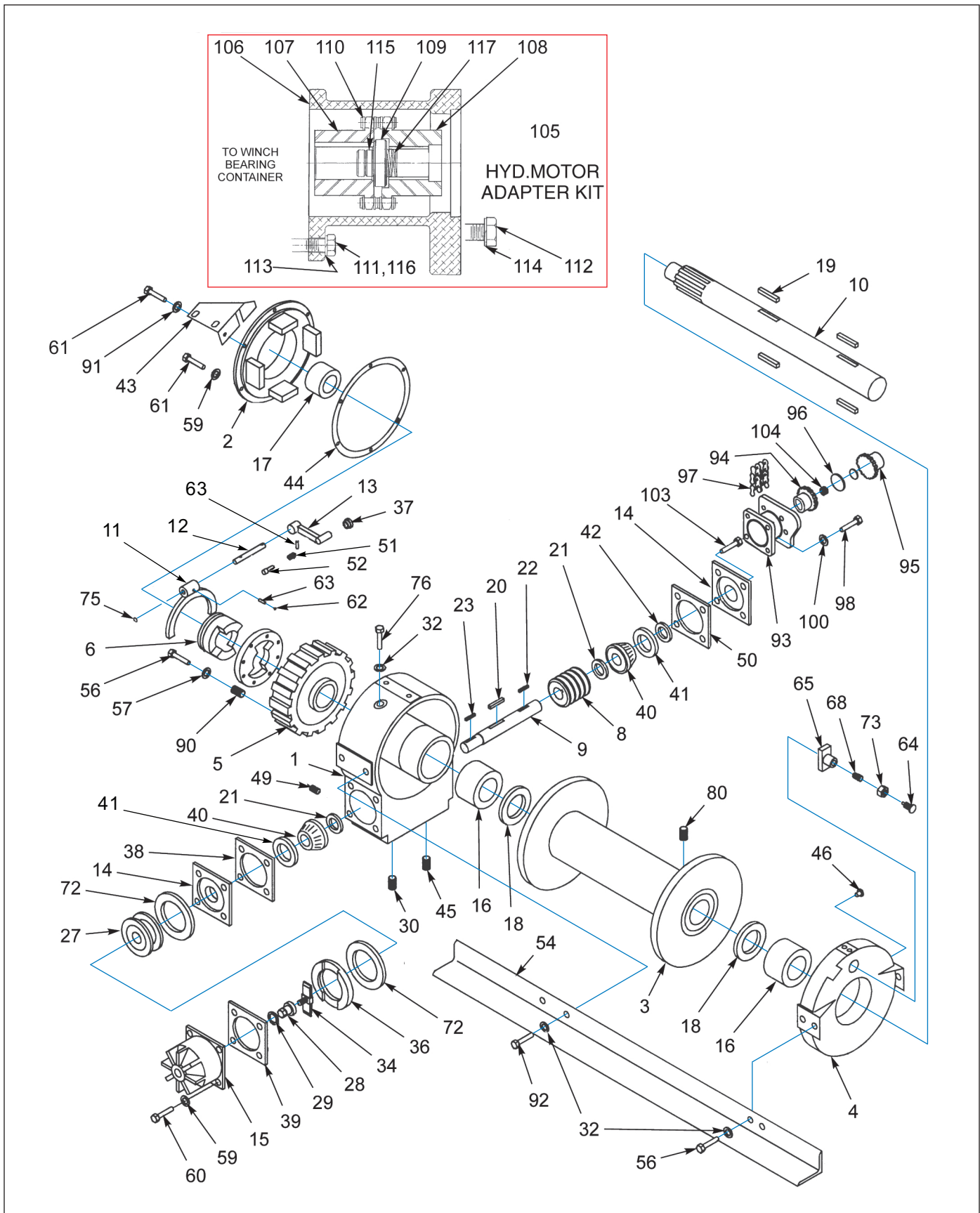
Figure 1-75: Winch Items - 20,000Lb. (BRADEN)
