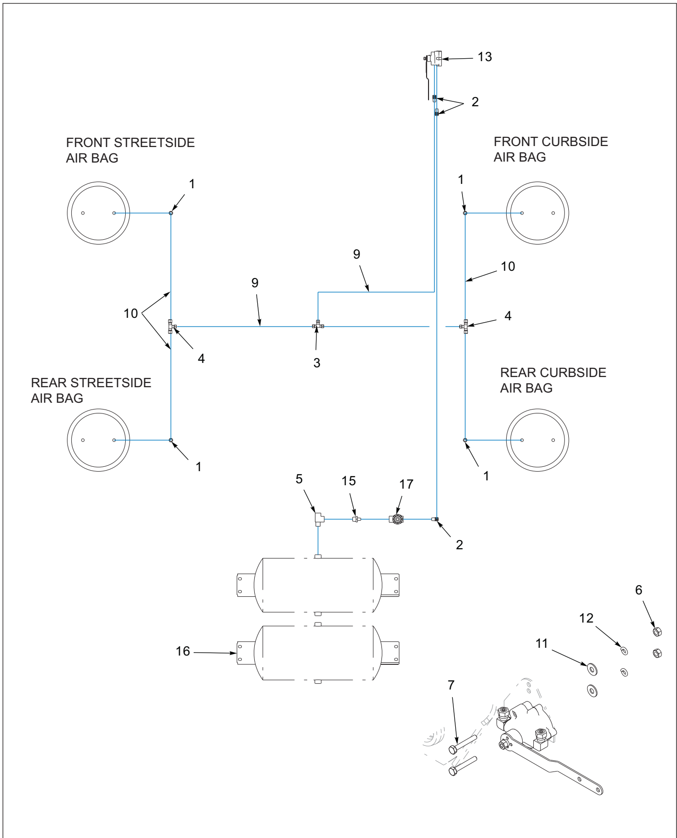
Figure 1-41: Air Ride Suspension - 440B Aqua
