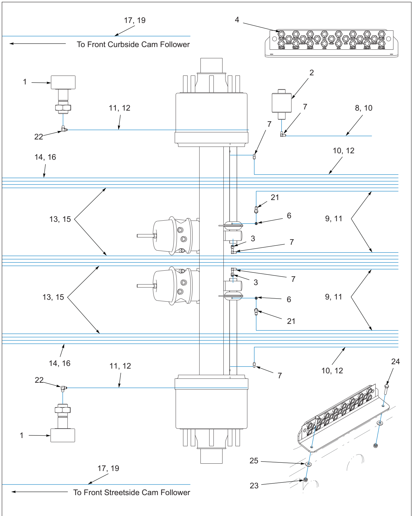
Figure 1-36: Grease System, 3 Axle (After 11/07/2018 - Before 08/31/2020) (1 of 2)
