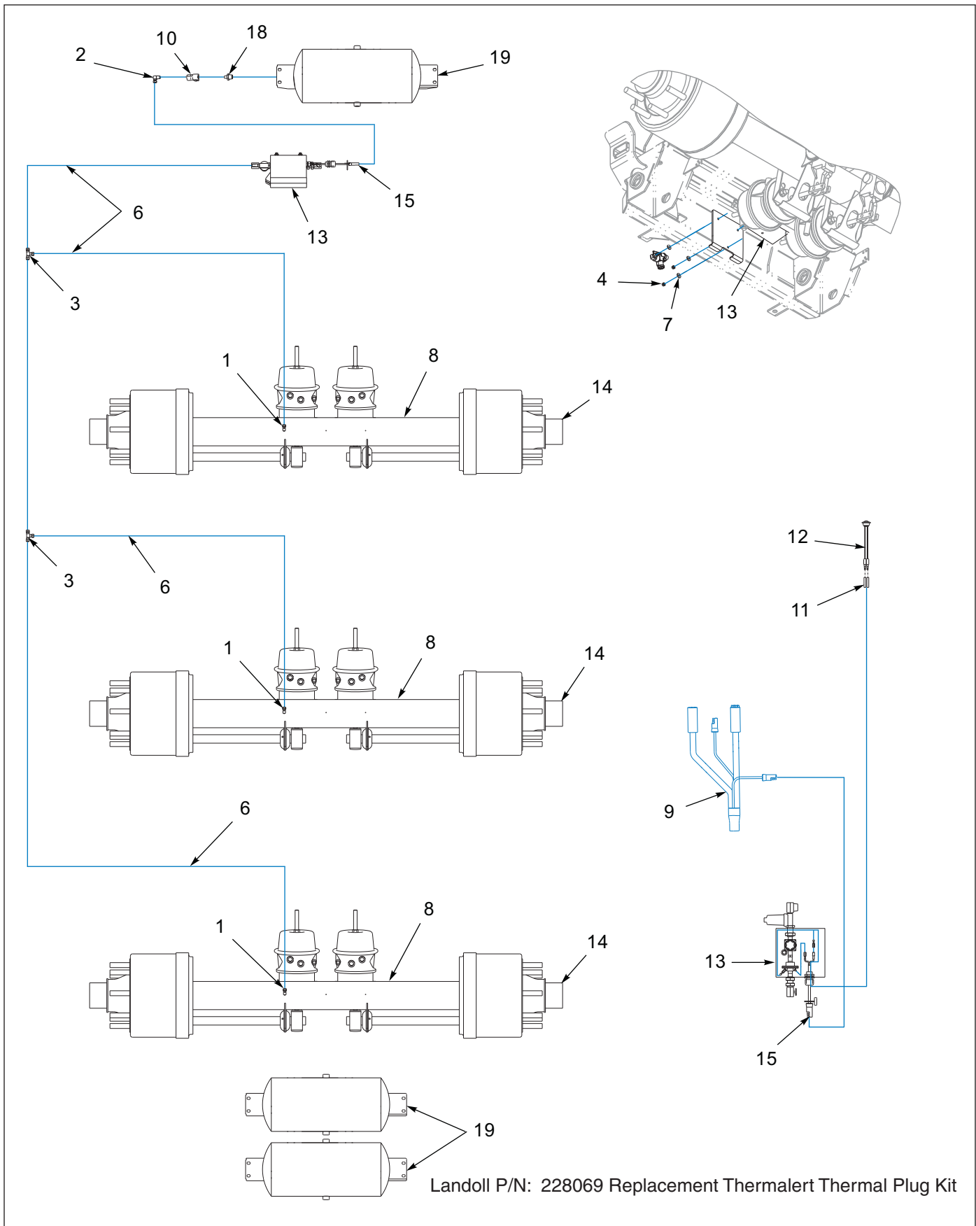
Figure 1-66: Thermalert, 3 Axle Air System (OPTION)
