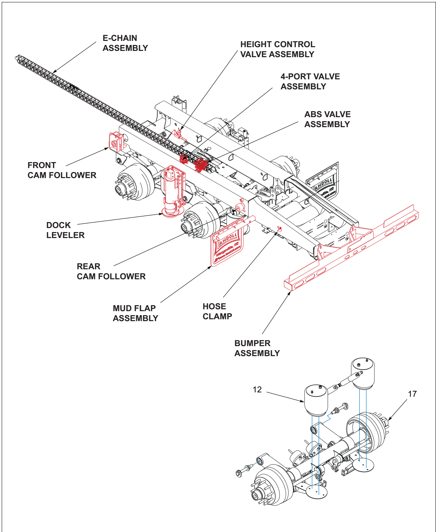
Figure 1-24: General Items - 440B (1 of 2)
