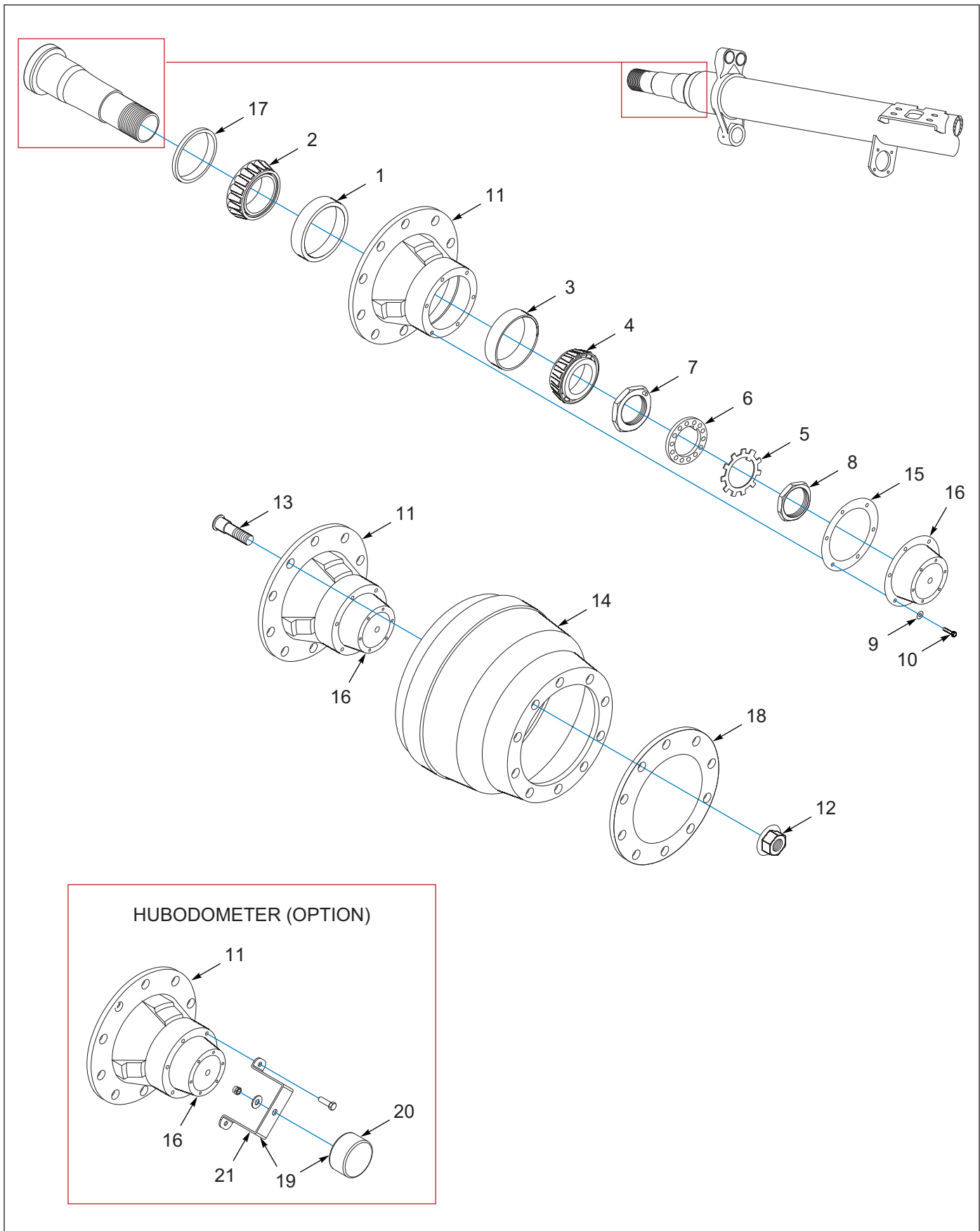
Figure 1-59: Axle 16.5 x 7 Drum and Hub Assembly, Dexter
