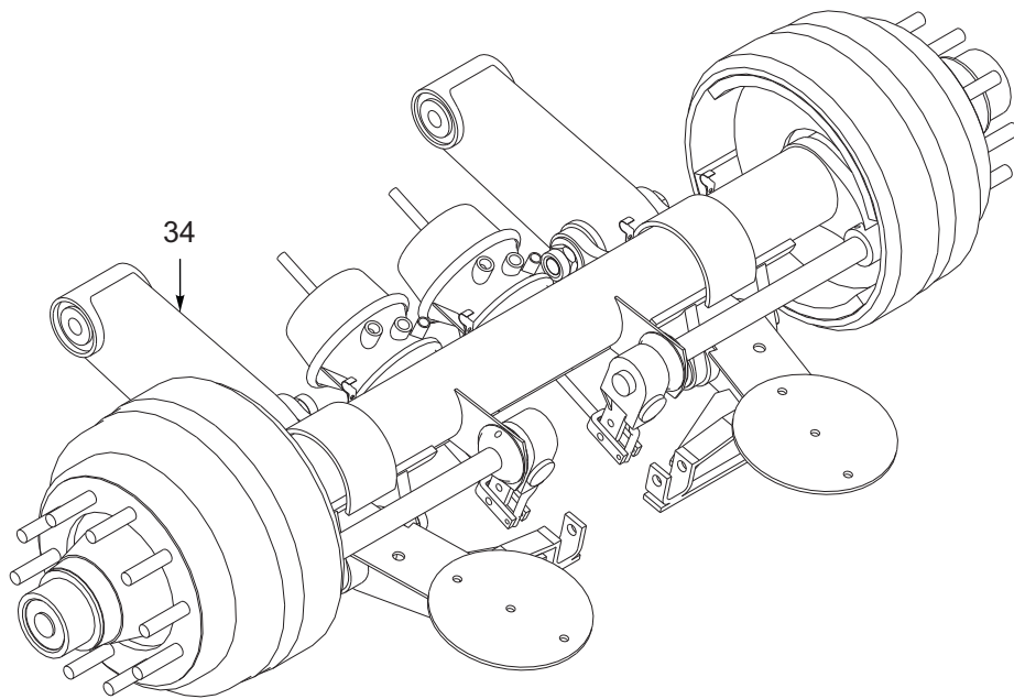
VIEW OF RLU-228-5.5, 16.5 X 7 DRUM BRAKES
