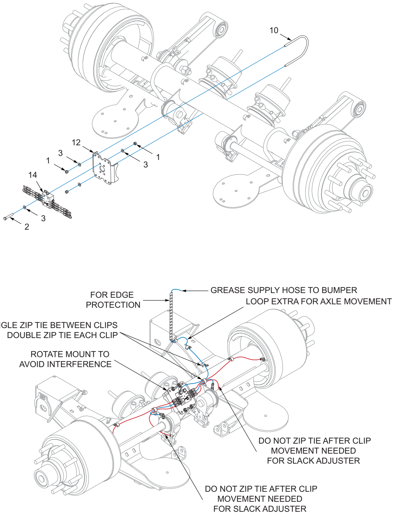
Figure 1-32: Grease System, 2 Axle (After 08/31/2020) (3 of 3)
