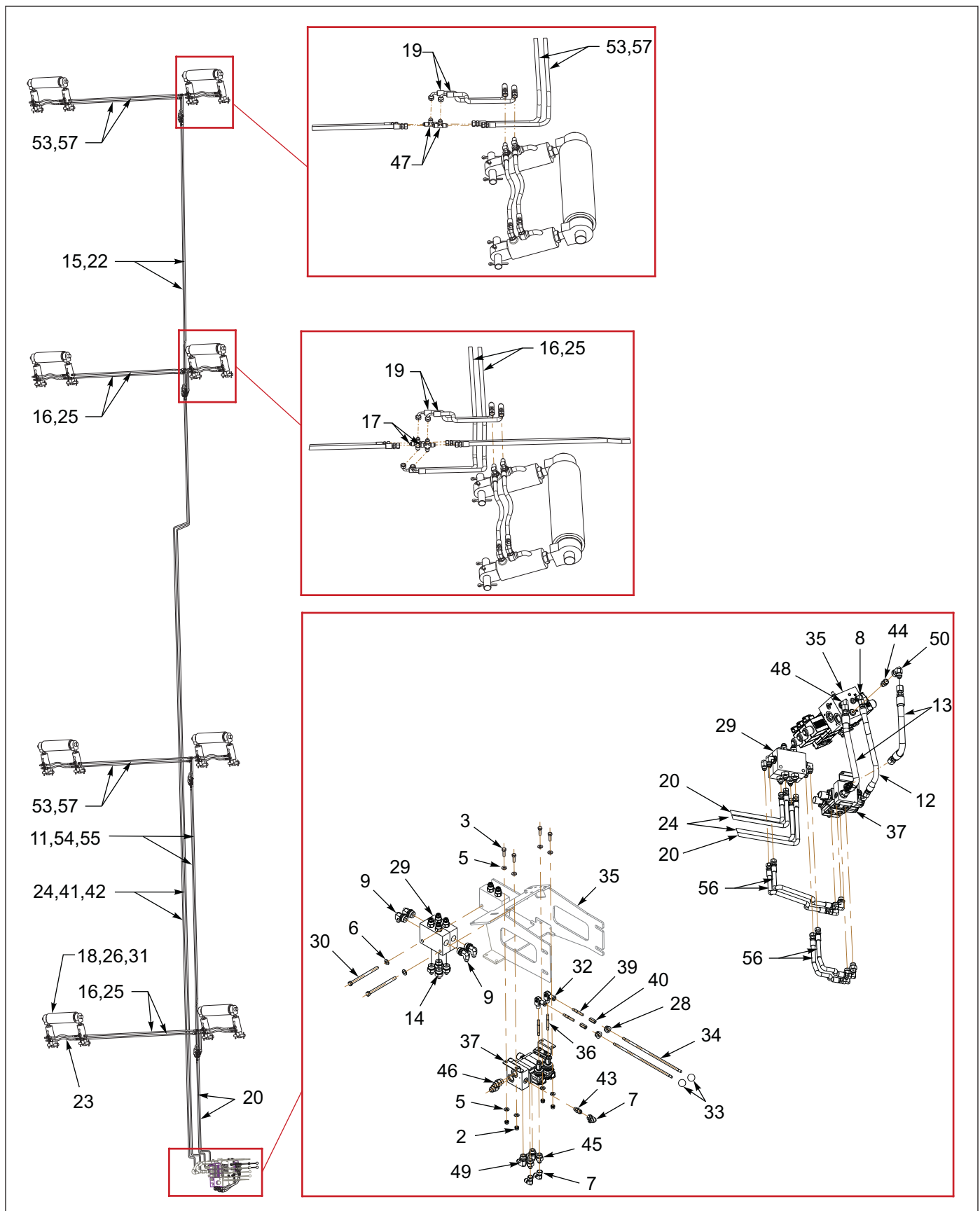
Figure 1-125: 8 Pop-Up Roller Installation (2 of 2)
