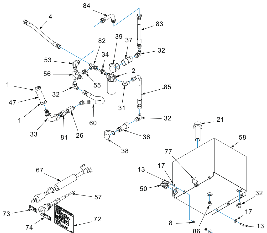
Figure 1-105: Engine - 25 HP Upper Deck Package (4 of 4)
