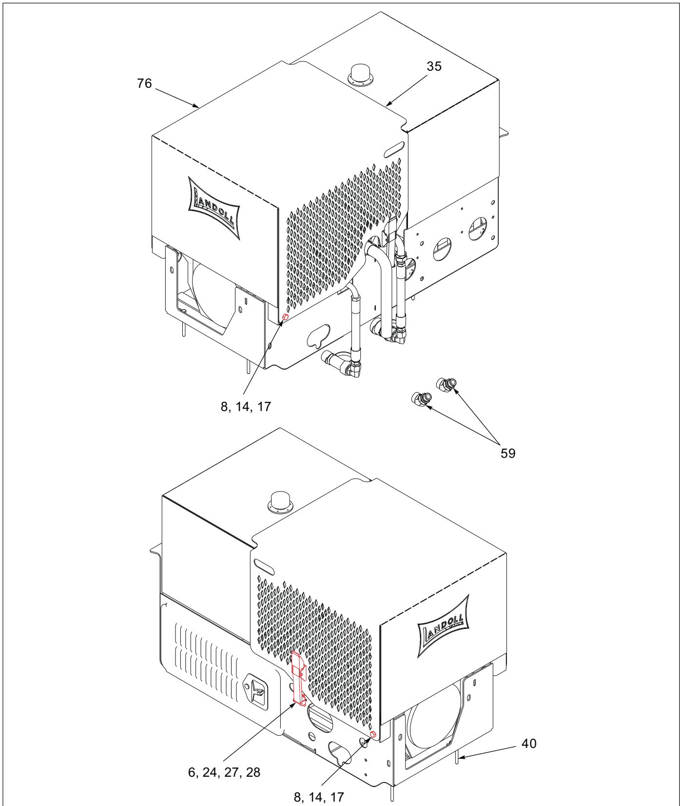
Figure 1-82: Engine - 25 HP Upper Deck Package (1 of 4)
