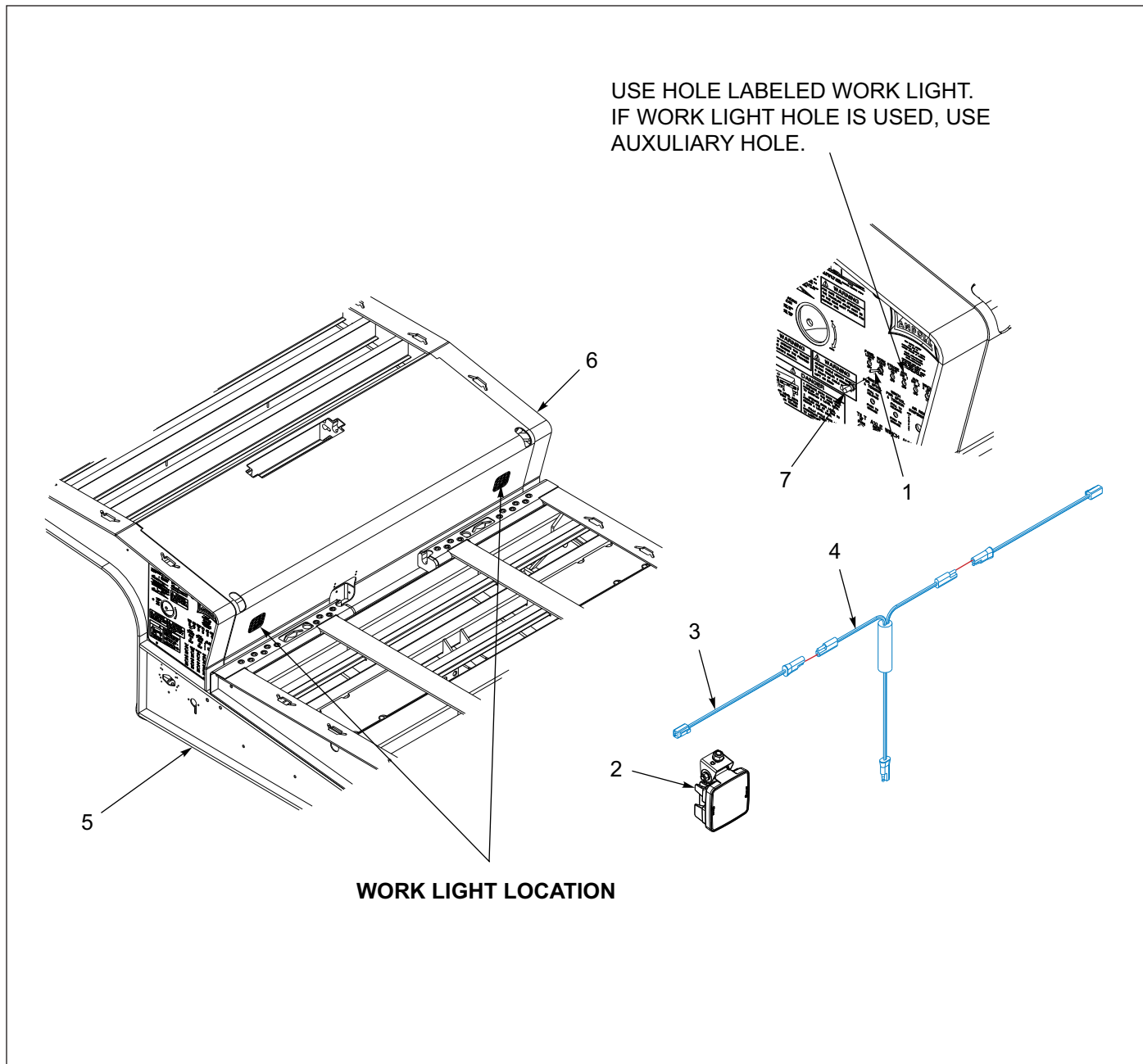
Figure 1-112: Upper Deck - Slope Light Installation
