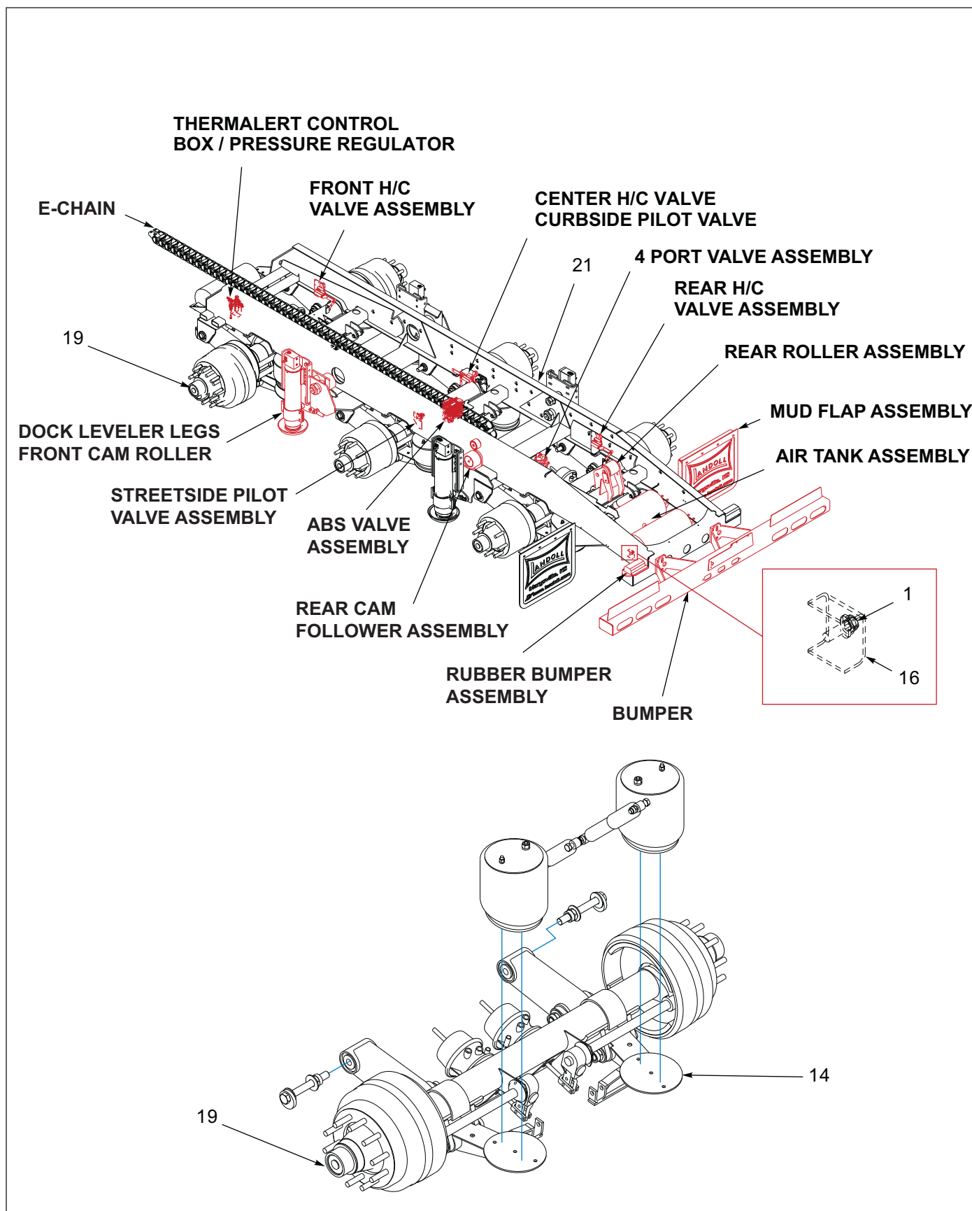
Figure 1-25: General Items - 455B Spring Brake (1 of 2)
