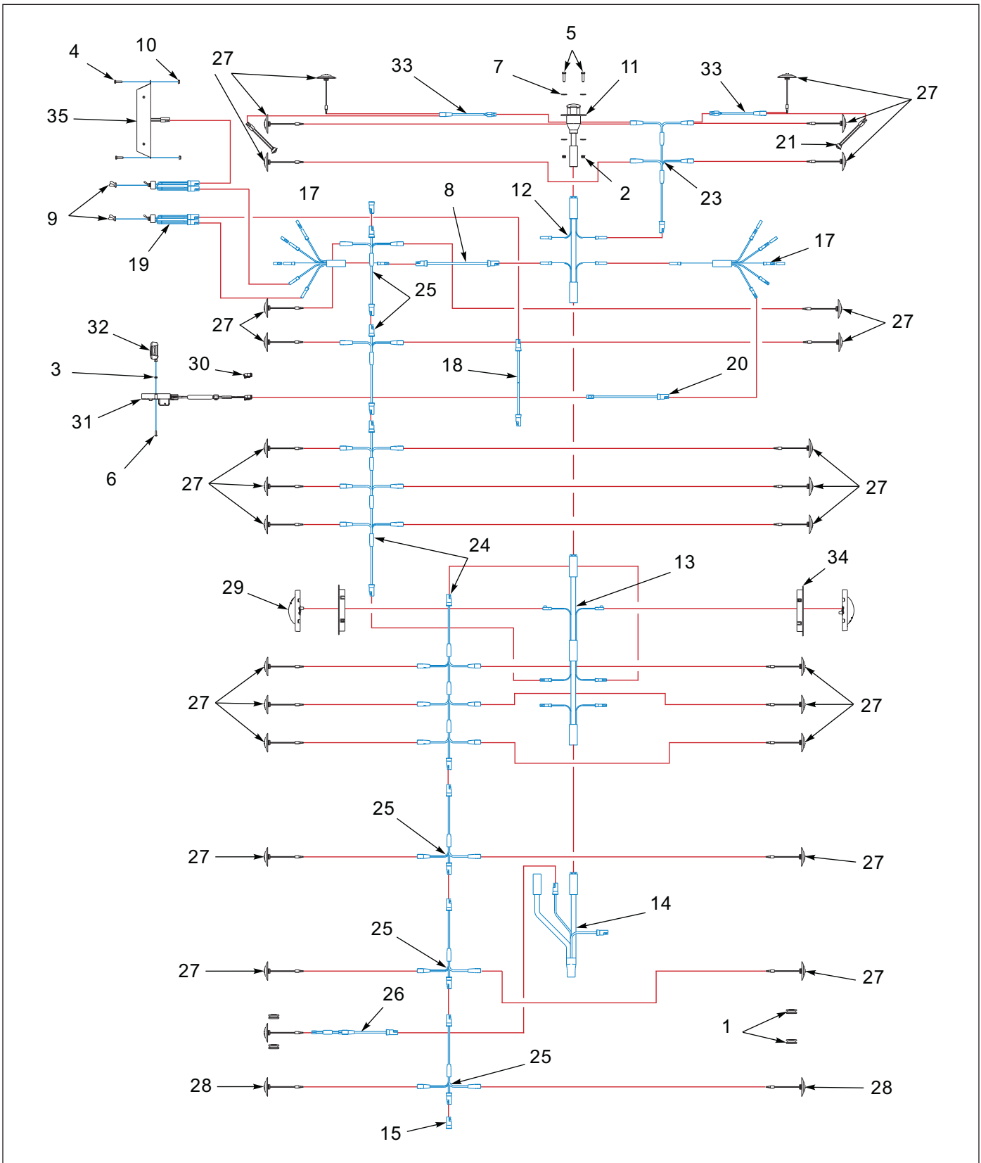
Figure 1-20: Electrical System, Frame (1 of 2)
