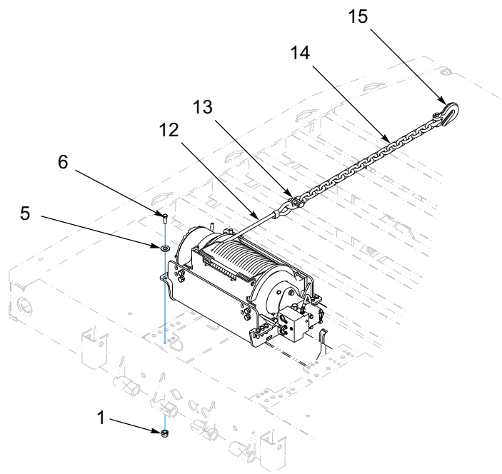
GENERAL ASSEMBLY
