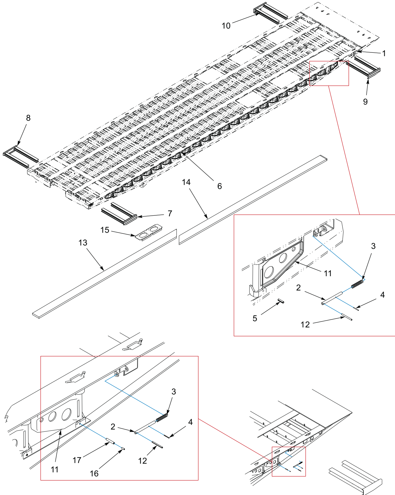
Figure 1-124: Outrigger Installation
