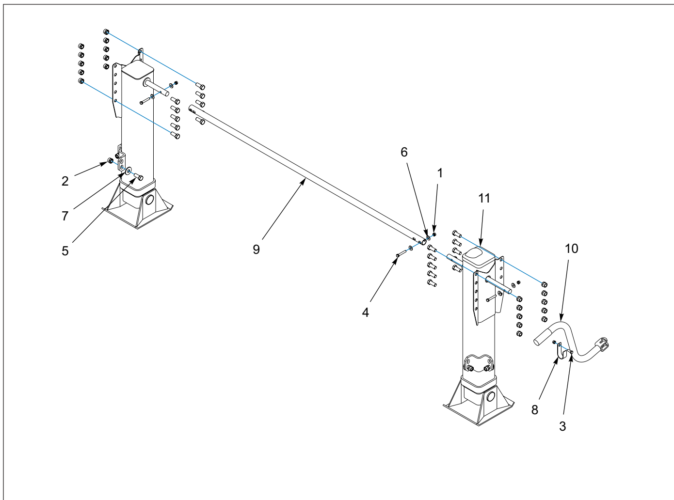
Figure 1-60: Landing Gear Installation - Jost 410
