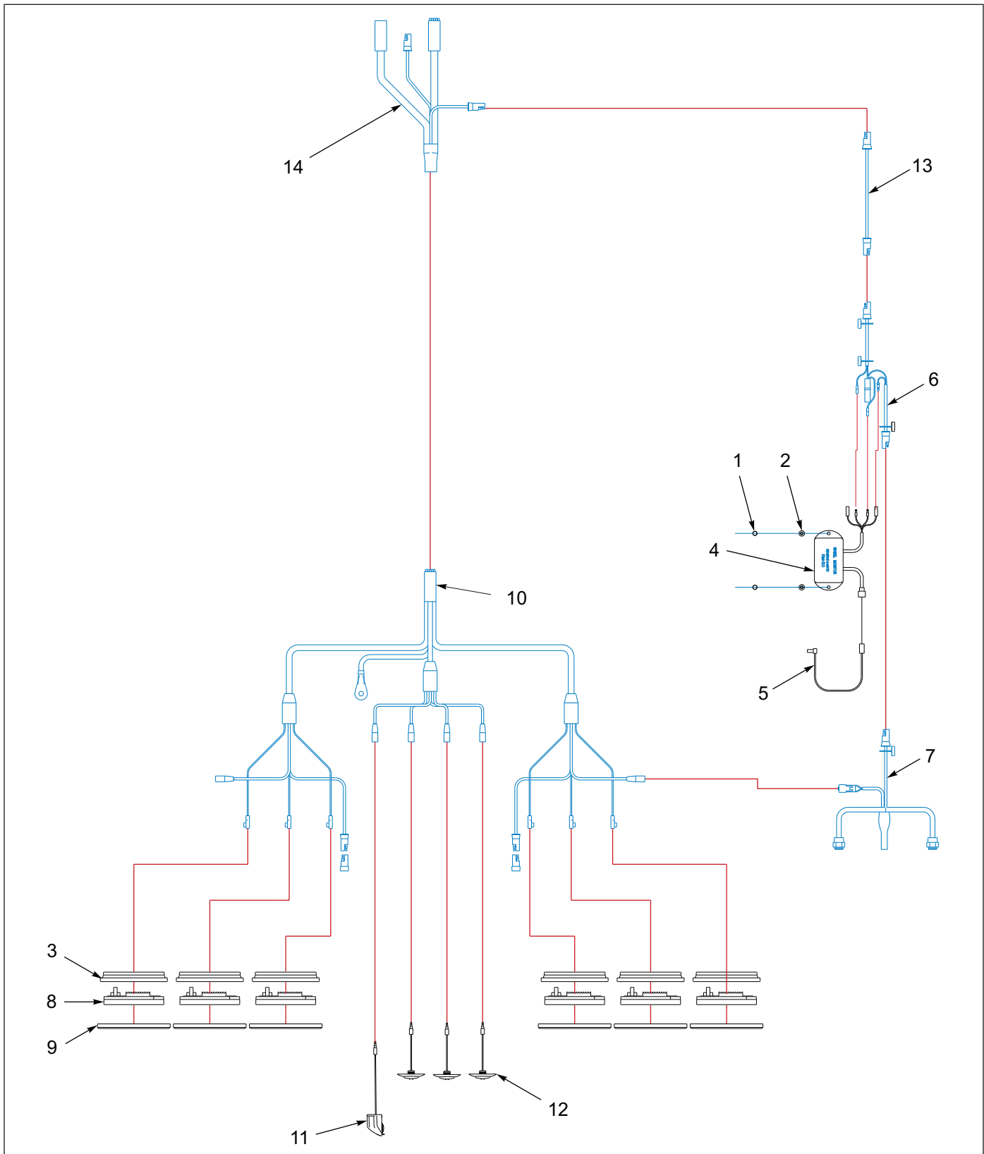
Figure 1-95: Backup Alarm/Light Installation
