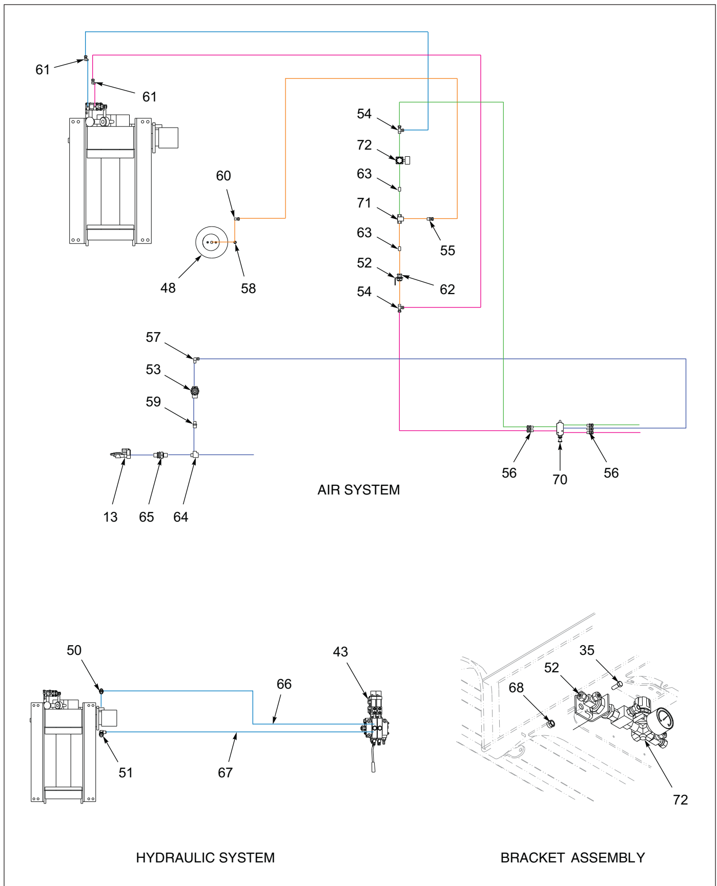
Figure 1-51: 20K Air Tension/Release (BRADEN) (3 of 3)
