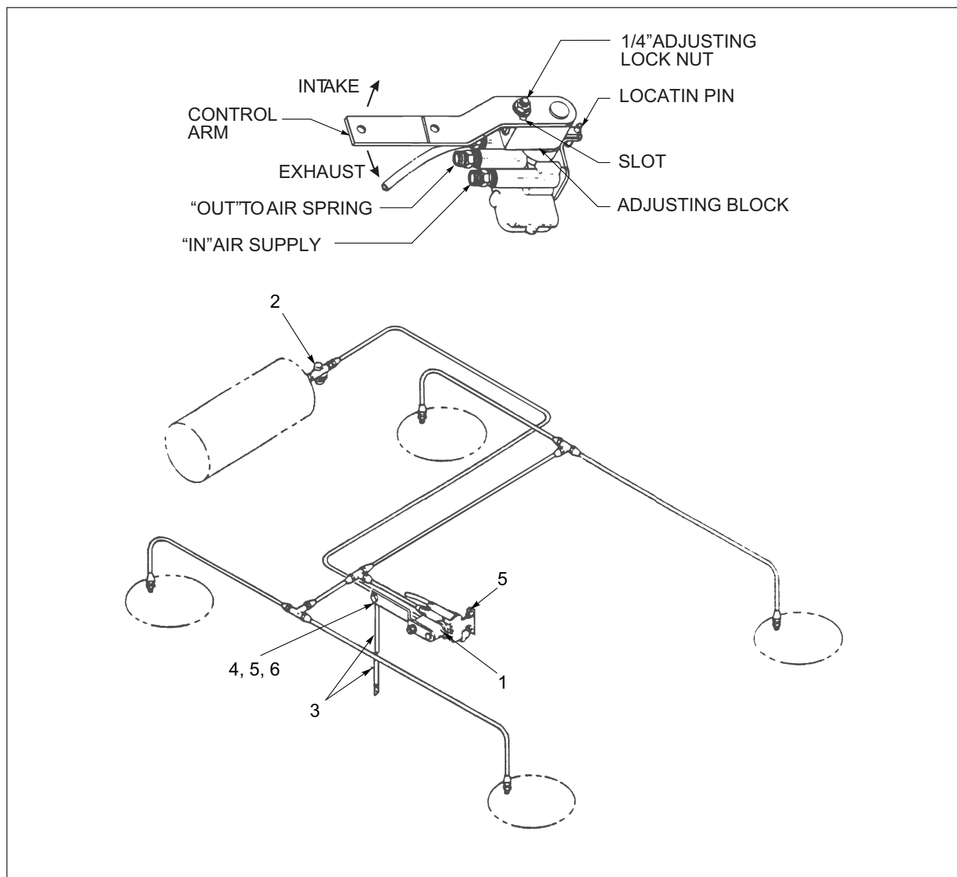
Figure 1-34: Air Control Kit - Neway
