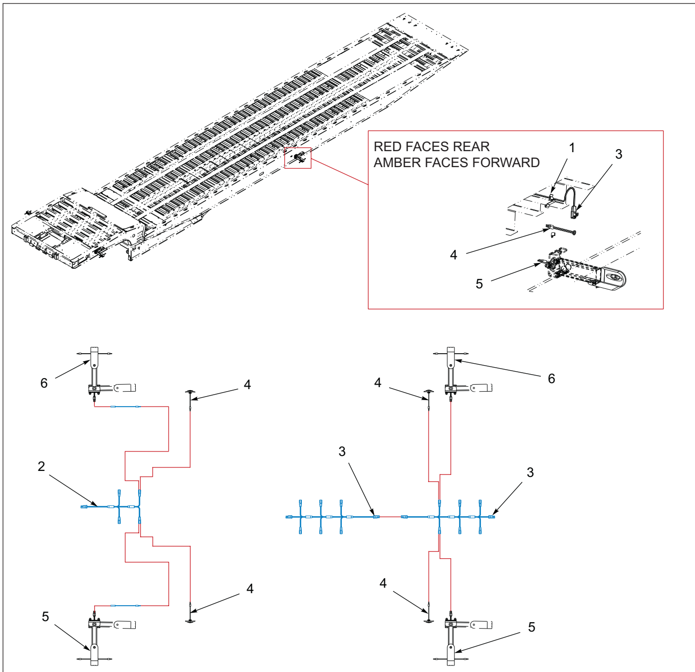
Figure 1-100: Swingout Marker Light Installation - Red/Amber
