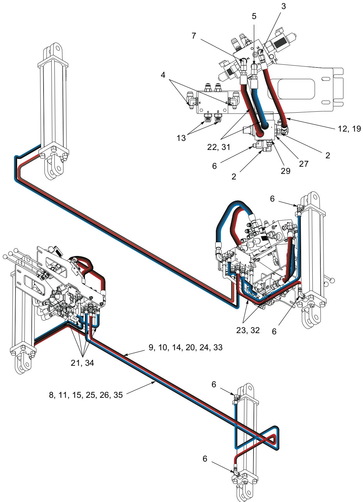
Figure 1-93: Hydraulic Park Stand - Hydraulic Items
