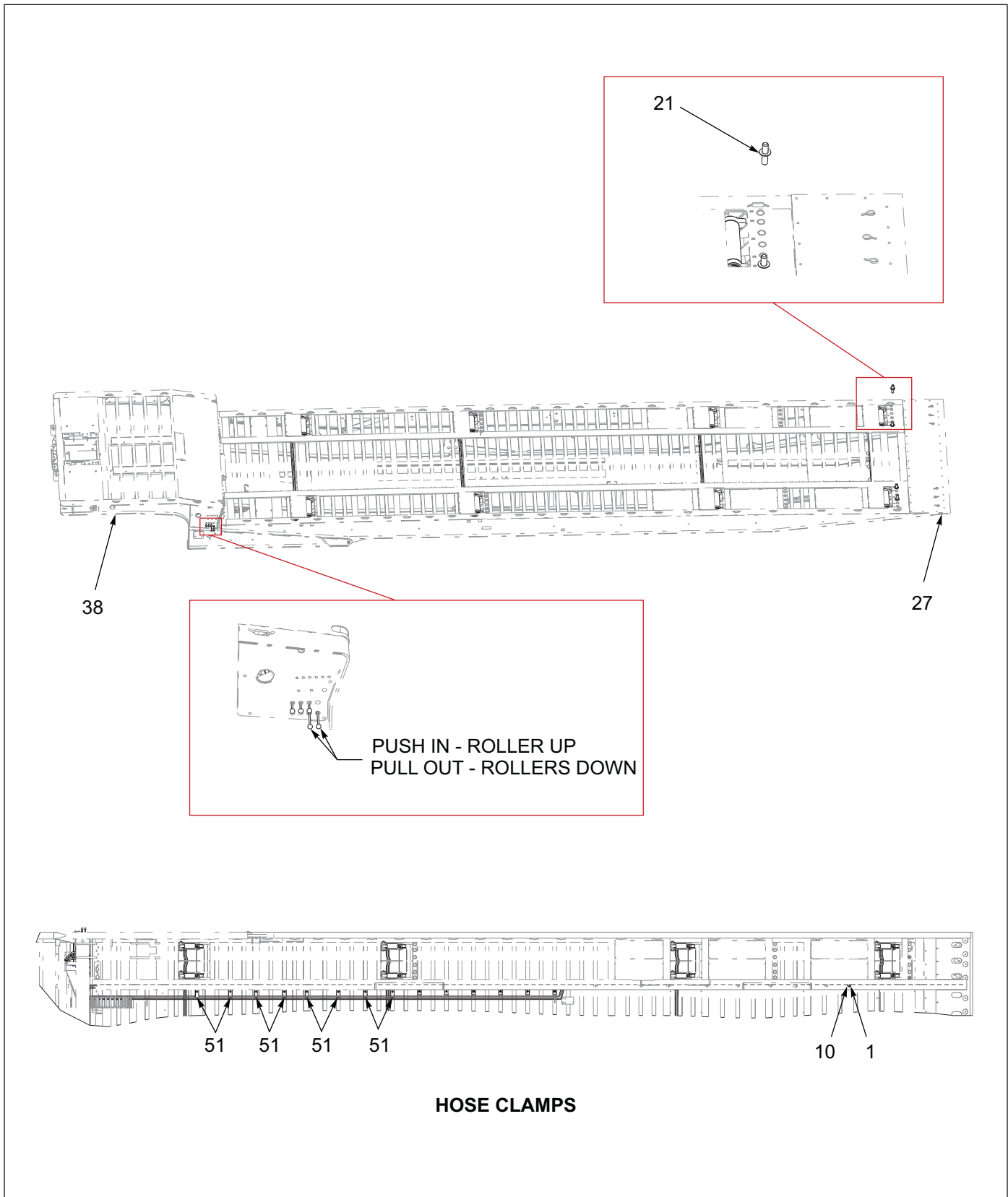
Figure 1-106: 8 Pop-Up Roller Installation (1 of 2)
