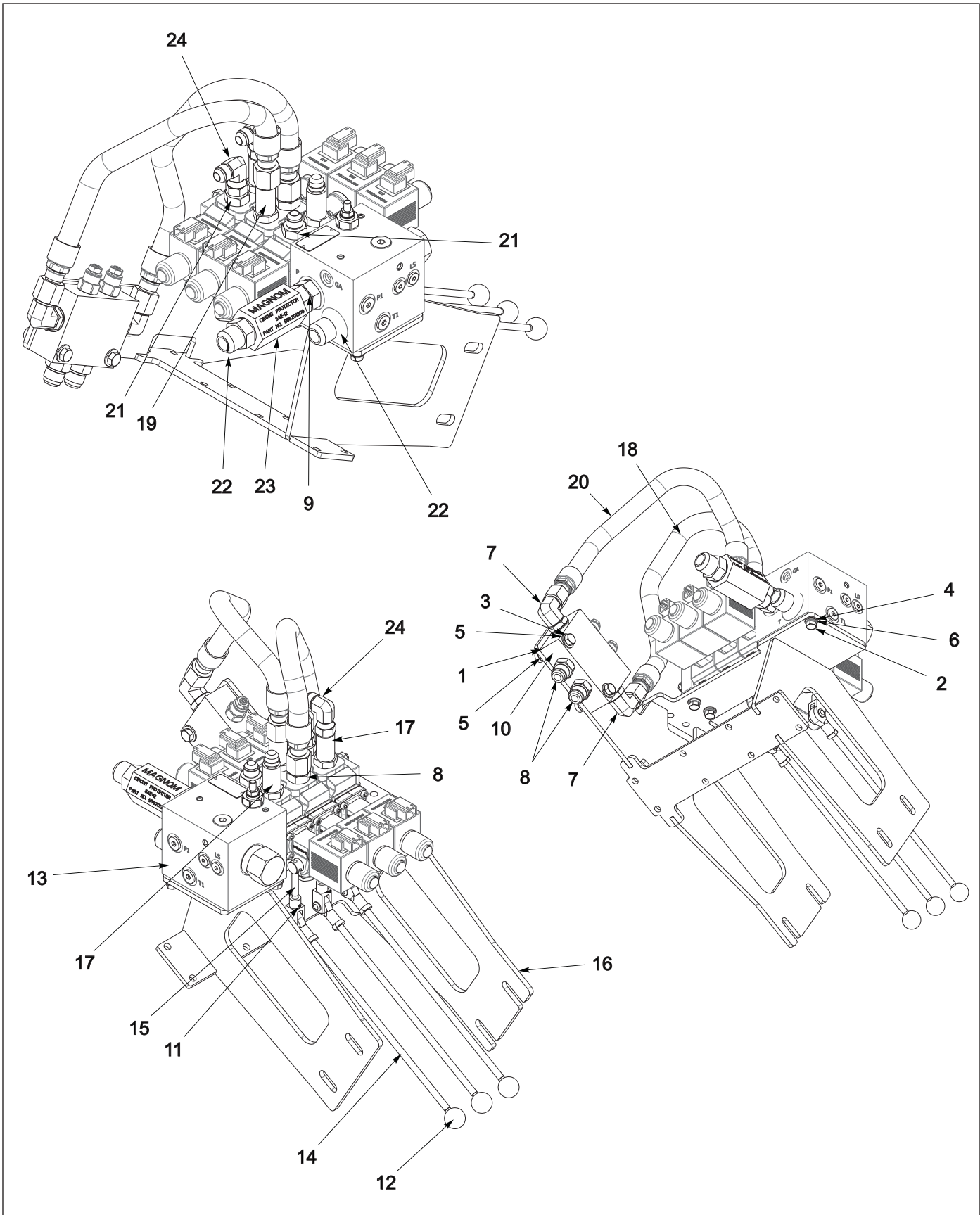
Figure 1-18: Valve Assembly - Three Spool
