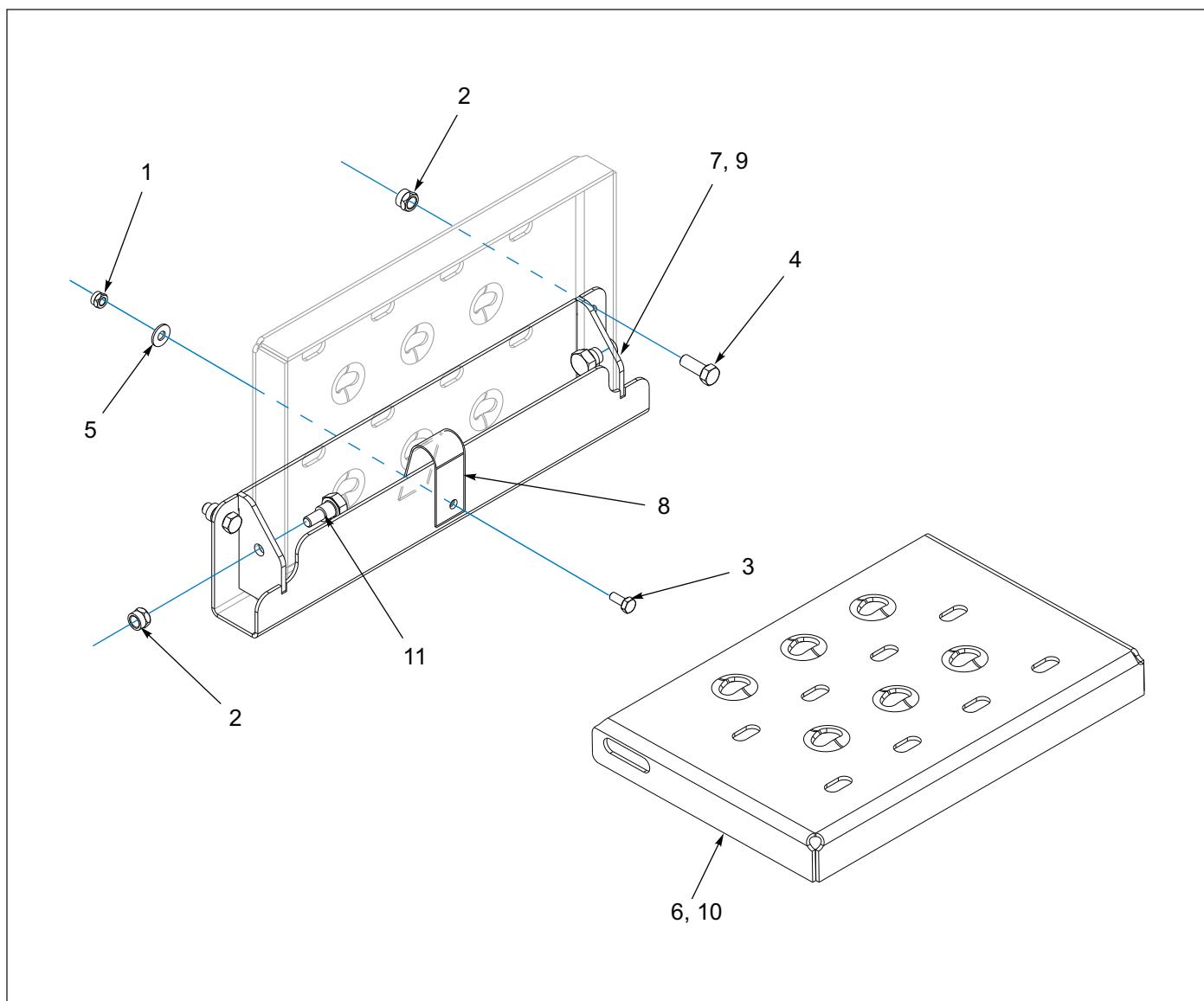
Figure 1-128: Folding Step - Option
