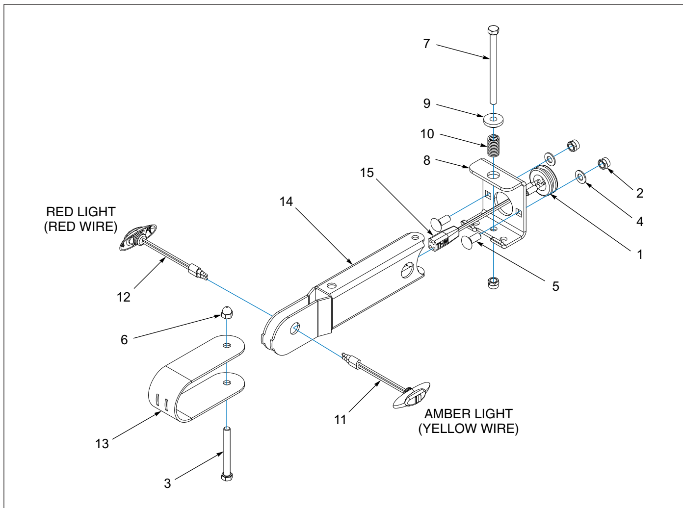
Figure 1-102: Swing-Arm Light Assembly - CURB
