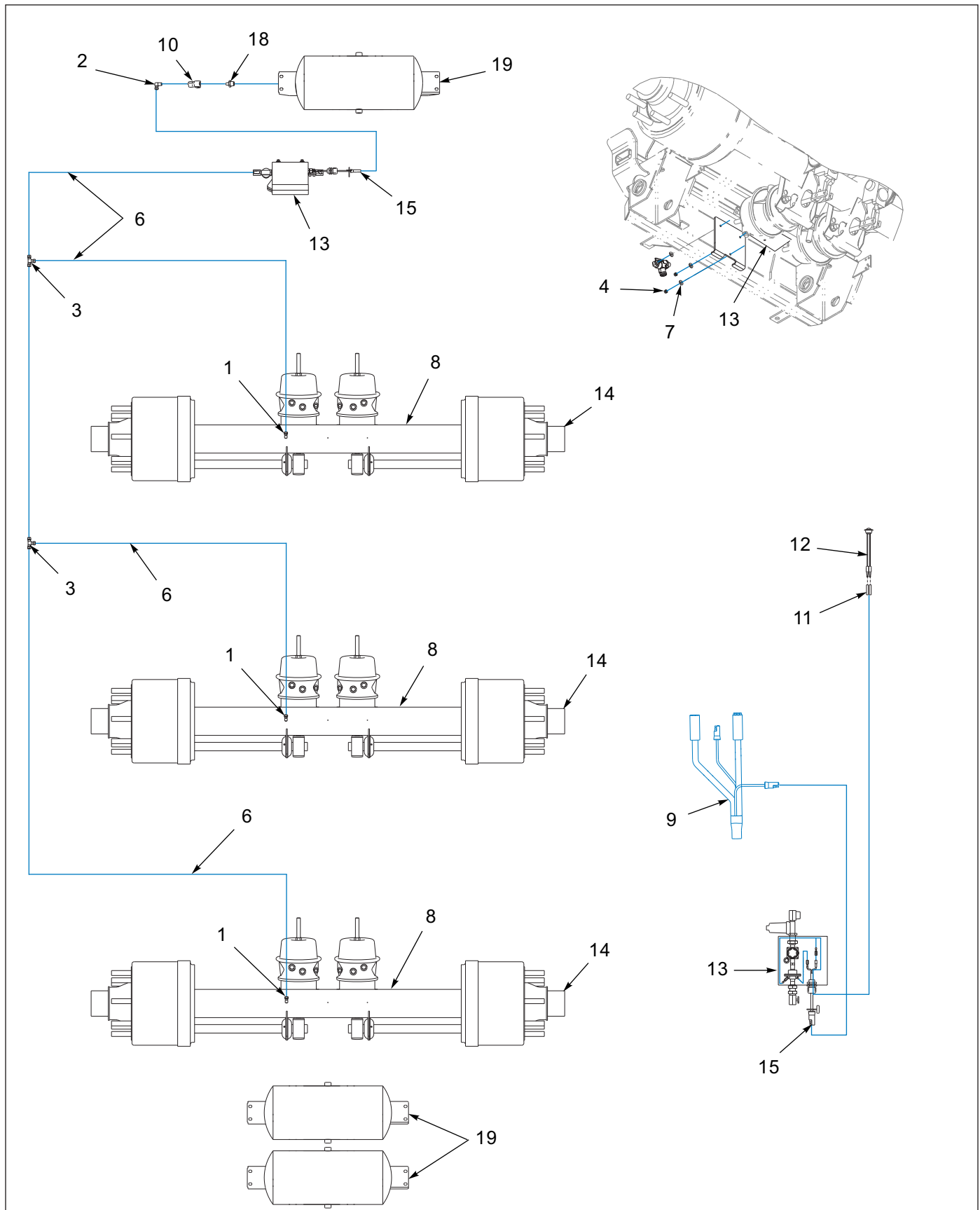
Figure 1-43: Thermalert Tire Inflation System - 455B
