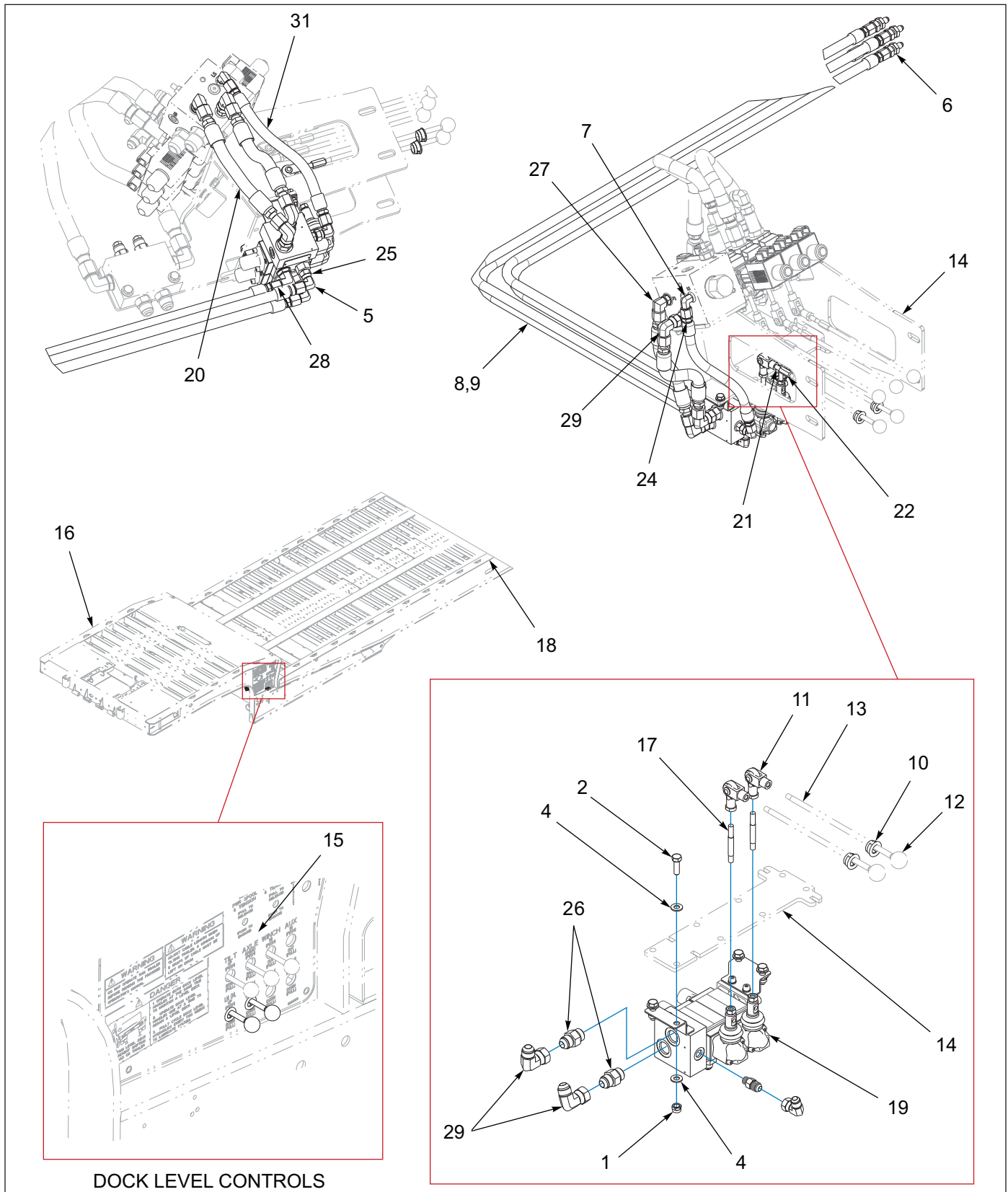
Figure 1-62: Dock Level Installation
