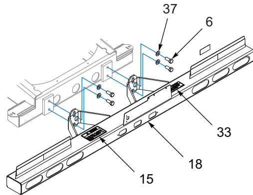
BUMPER ASSEMBLY
