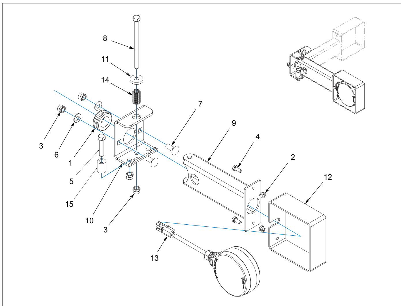
Figure 1-99: Swing-Arm Light Assembly - Turn Signal/Emergency Flasher
