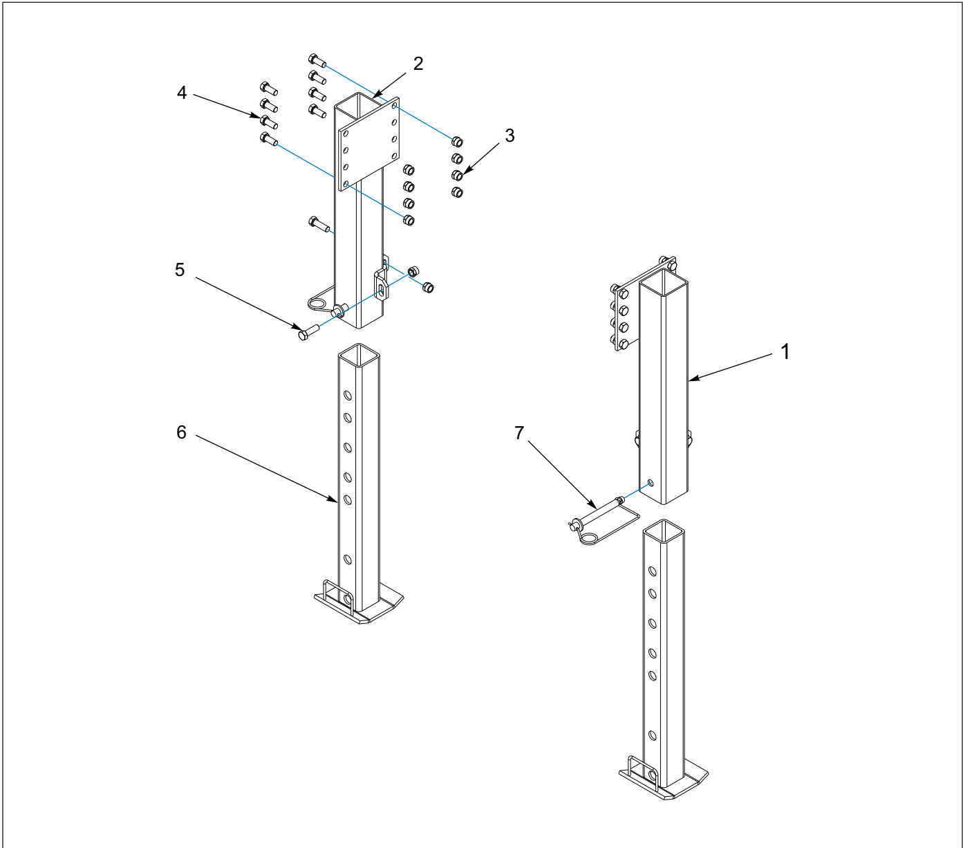
Figure 1-59: Landing Gear Installation - Bolt-On Park Stand
