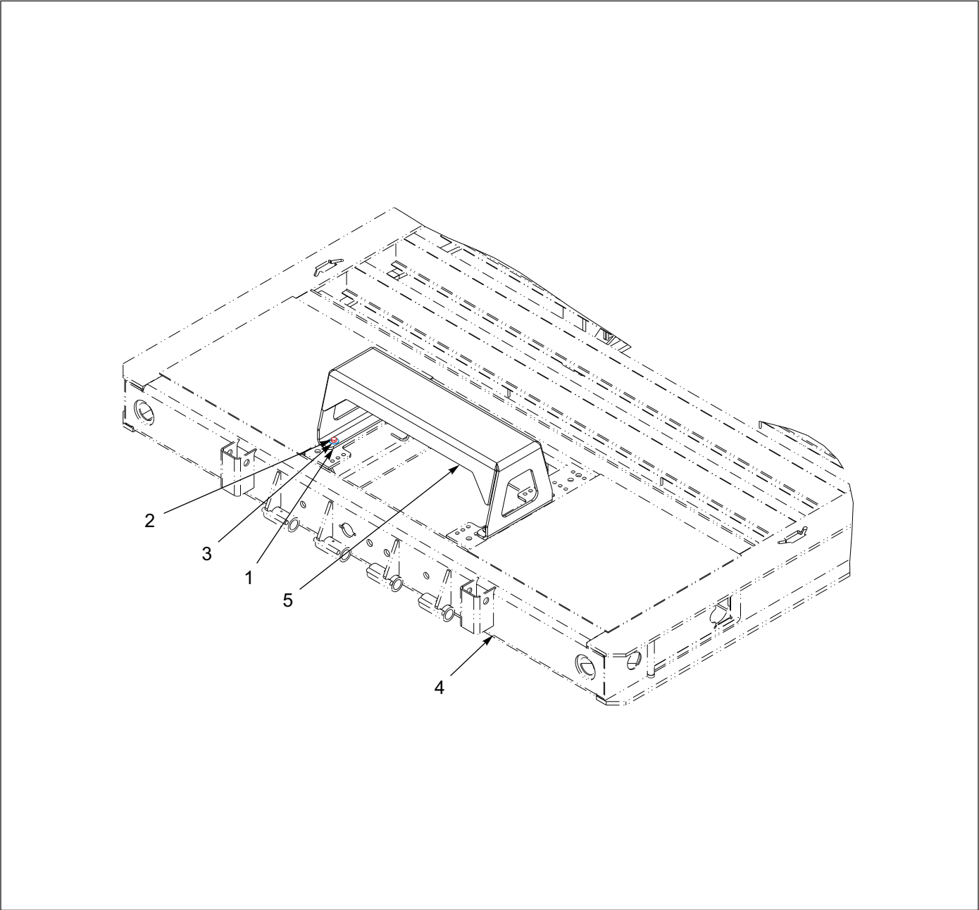
Figure 1-114: Winch - 12K/20K Guard Installation (BRADEN)
