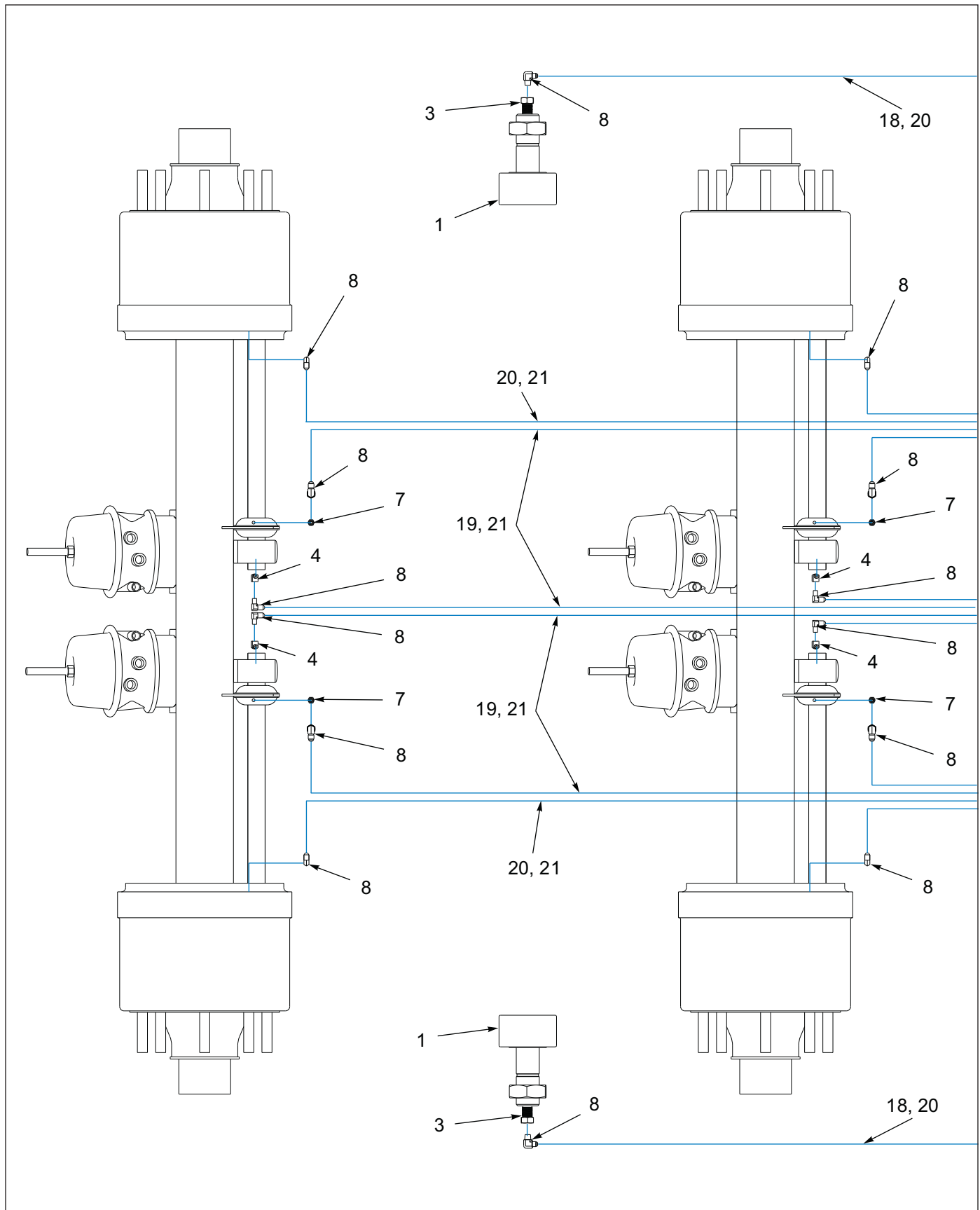
Figure 1-28: Grease System - 455B Spring Brake - Side A
