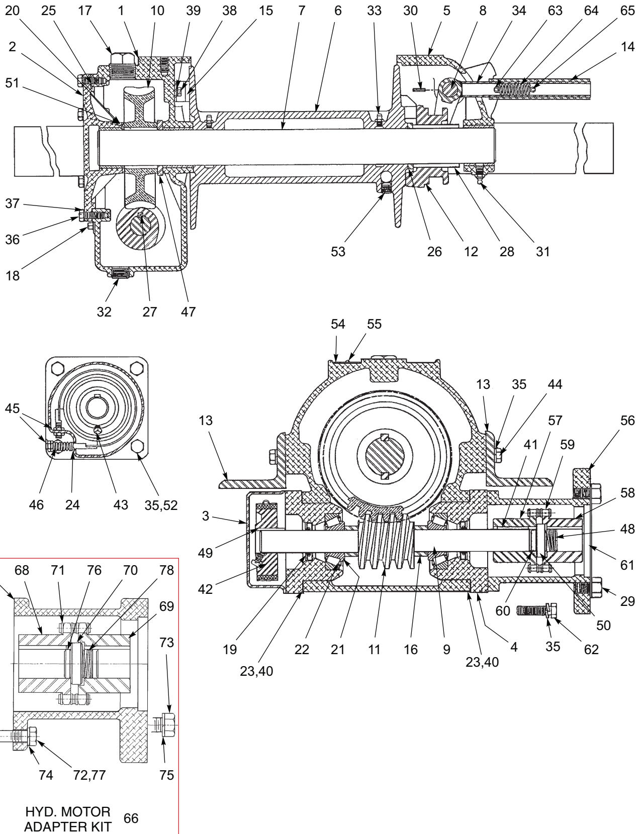
Figure 1-47: Winch Items - 12,000 Lb. (BRADEN)
