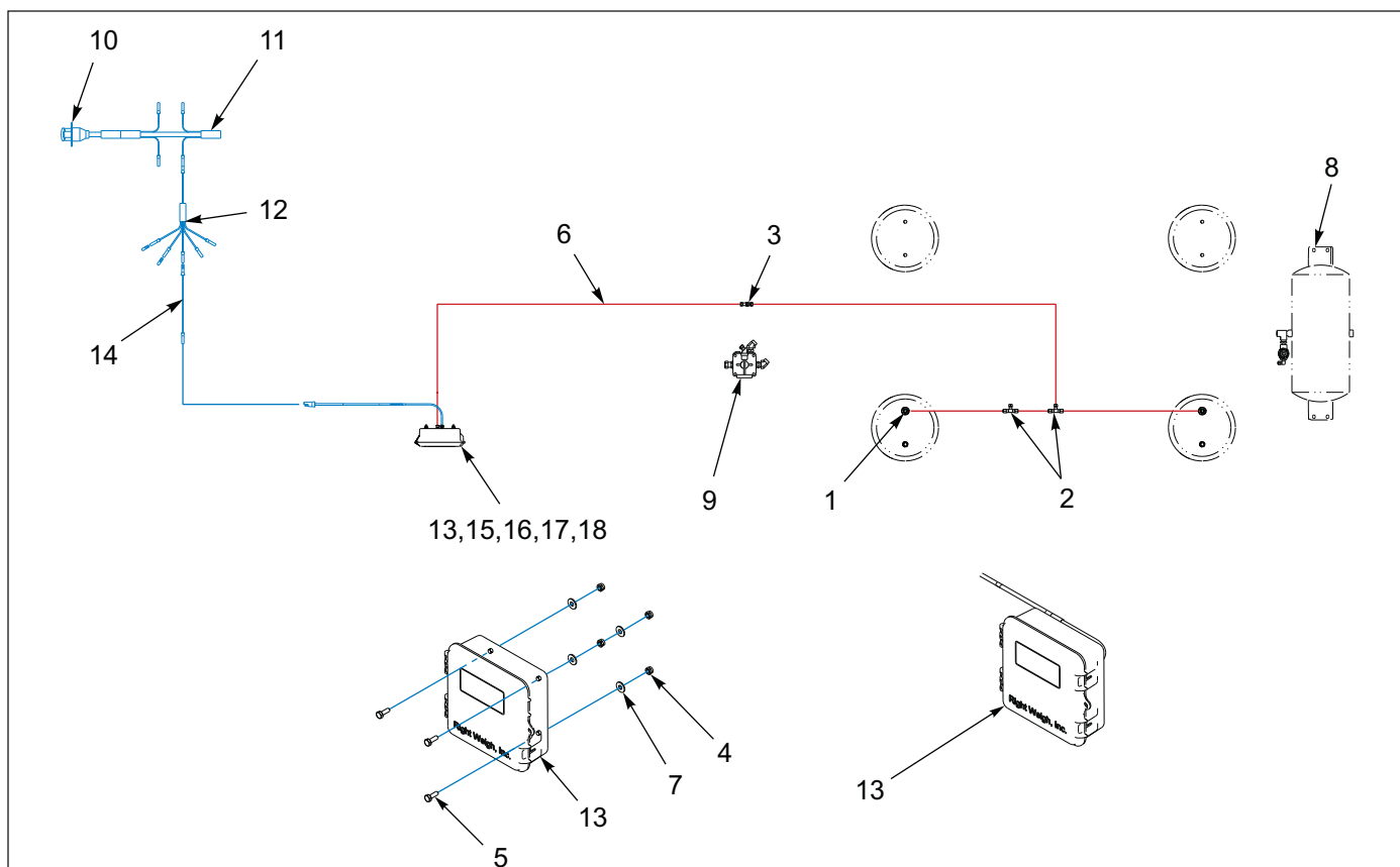
Figure 1-72: Air Digital Scale - Right Weigh System
