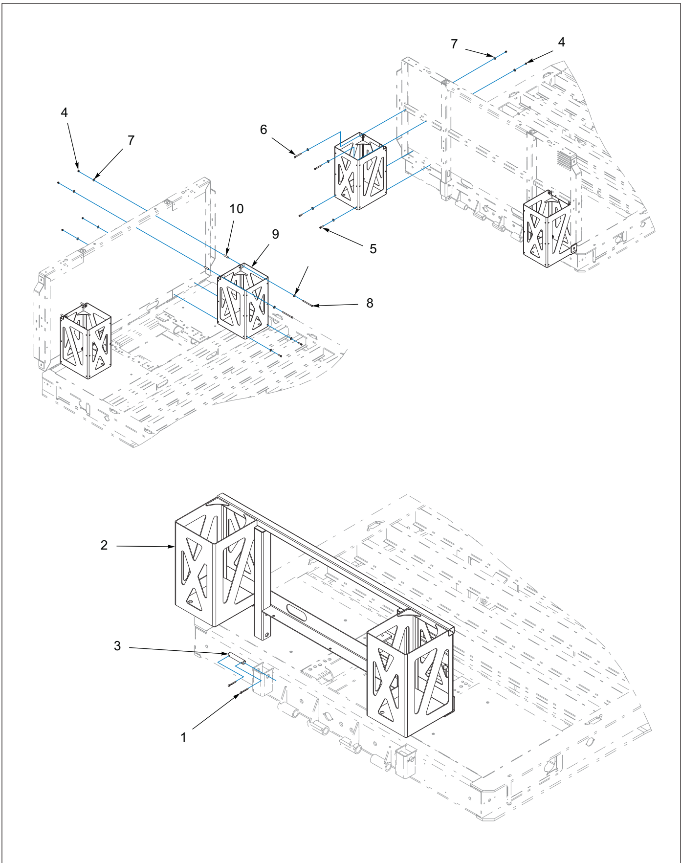
Figure 1-76: Bulkhead Installation - Special
