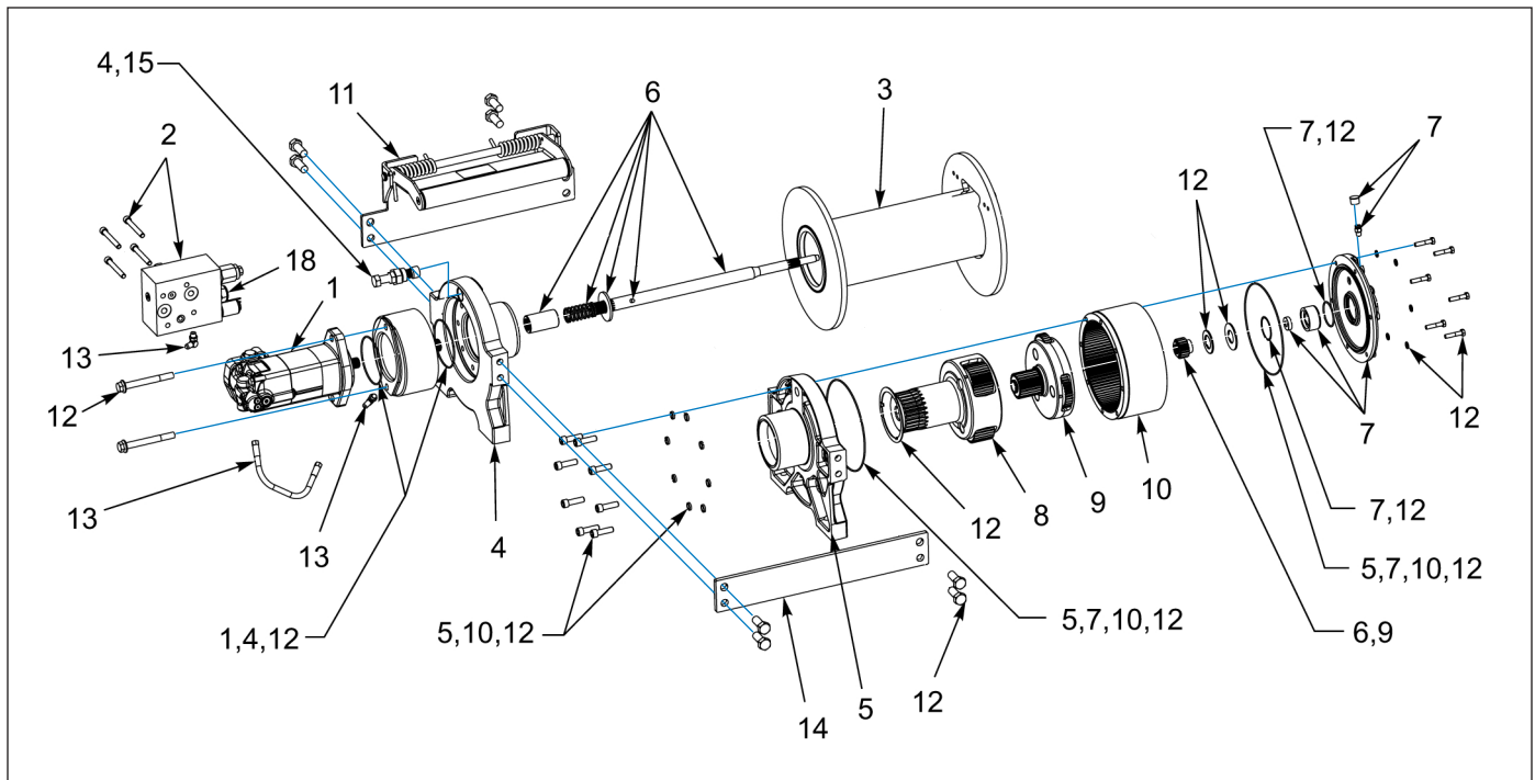
Figure 1-56: Winch Items - 20K 2 Speed (WARN)
