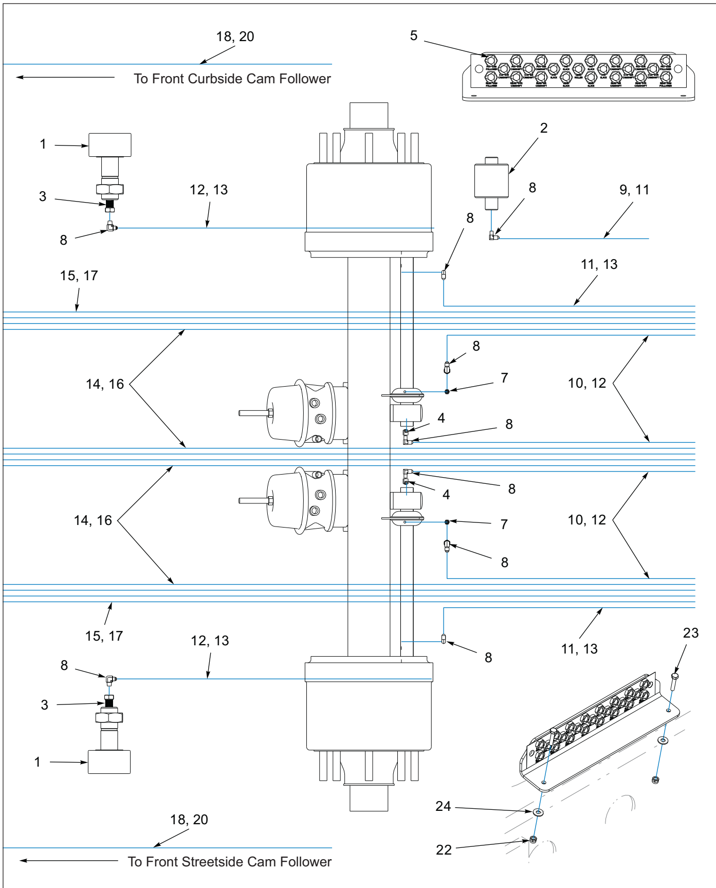
Figure 1-29: Grease System - 455B Spring Brake - Side B
