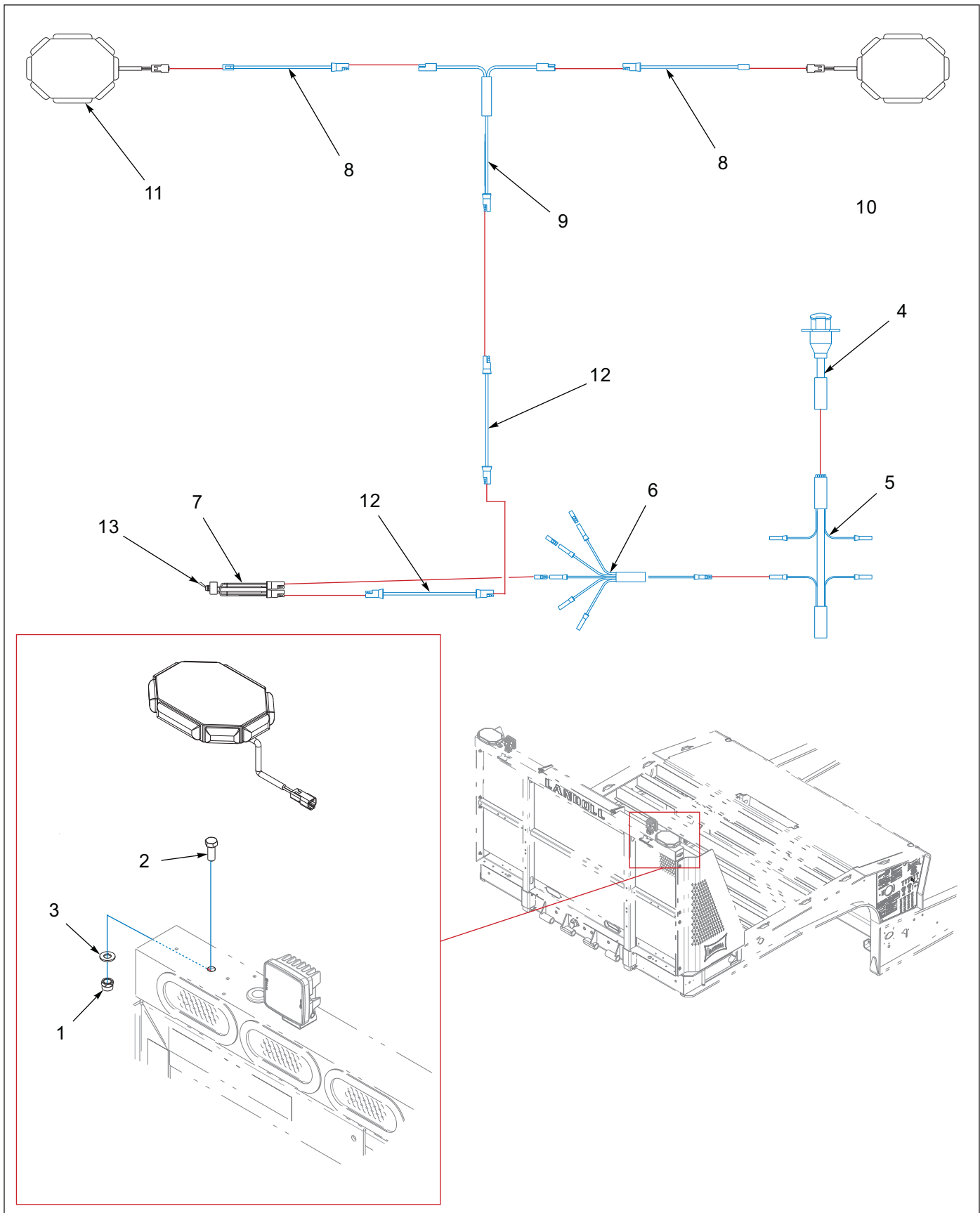
Figure 1-77: Towmate Strobe Installation
