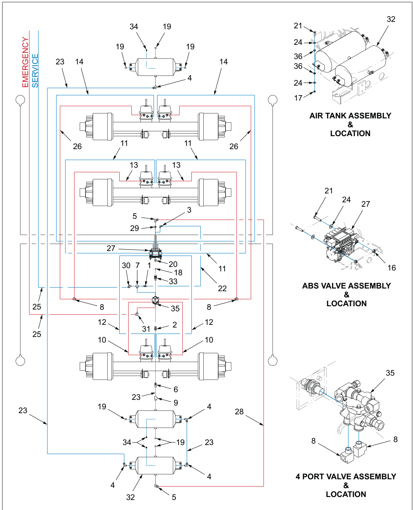
Figure 1-40: Air Brake System - 455B Spring Brake
