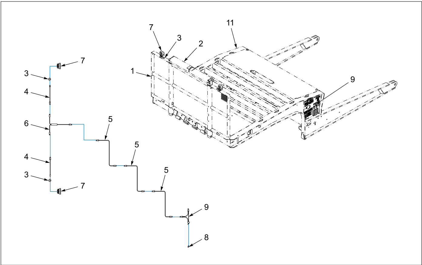
Figure 1-78: Bulkhead - Work Light Installation
