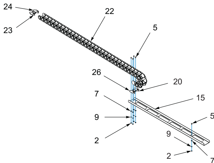
E-CHAIN ASSEMBLY
