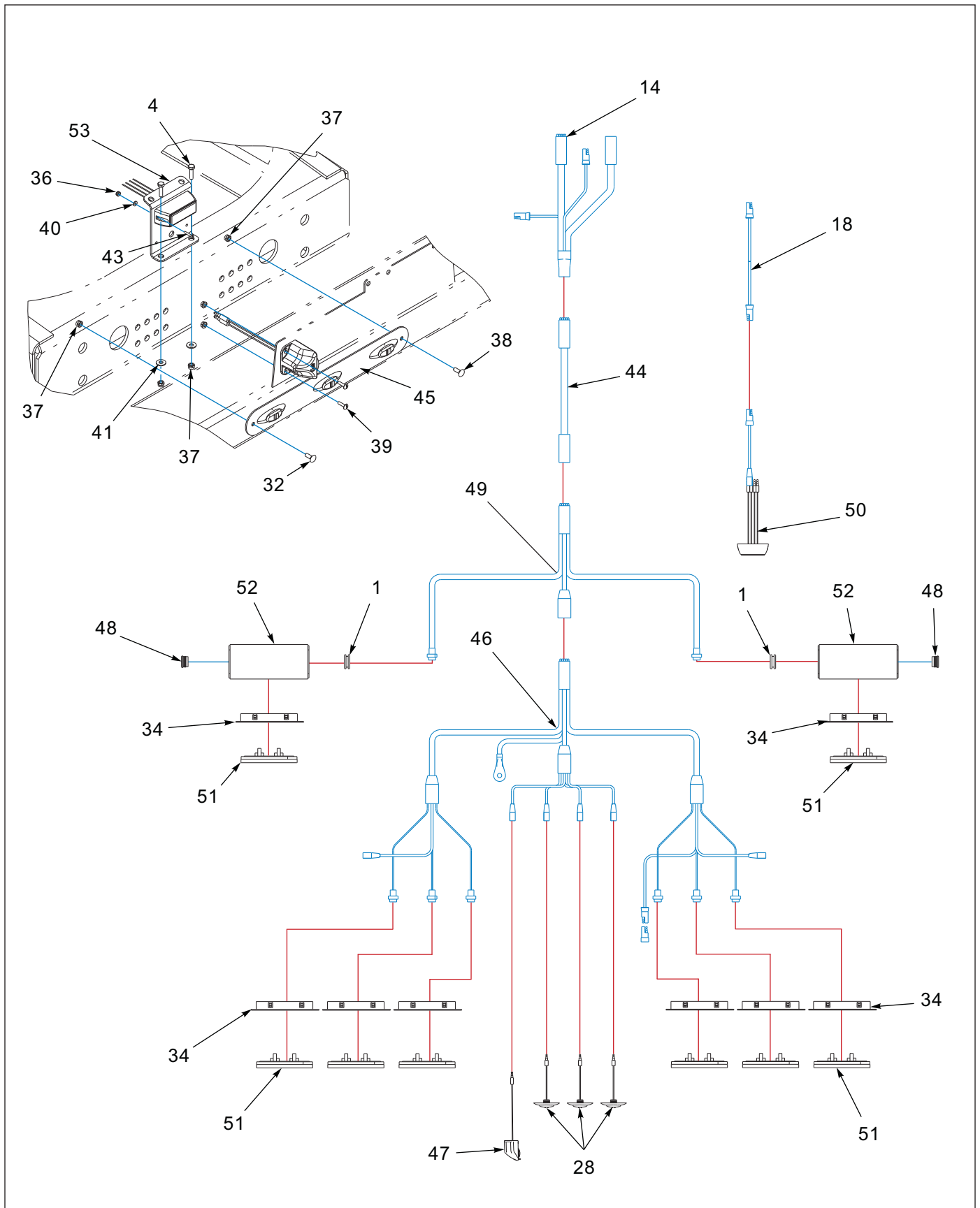
Figure 1-21: Electrical System, Bumper (2 of 2)
