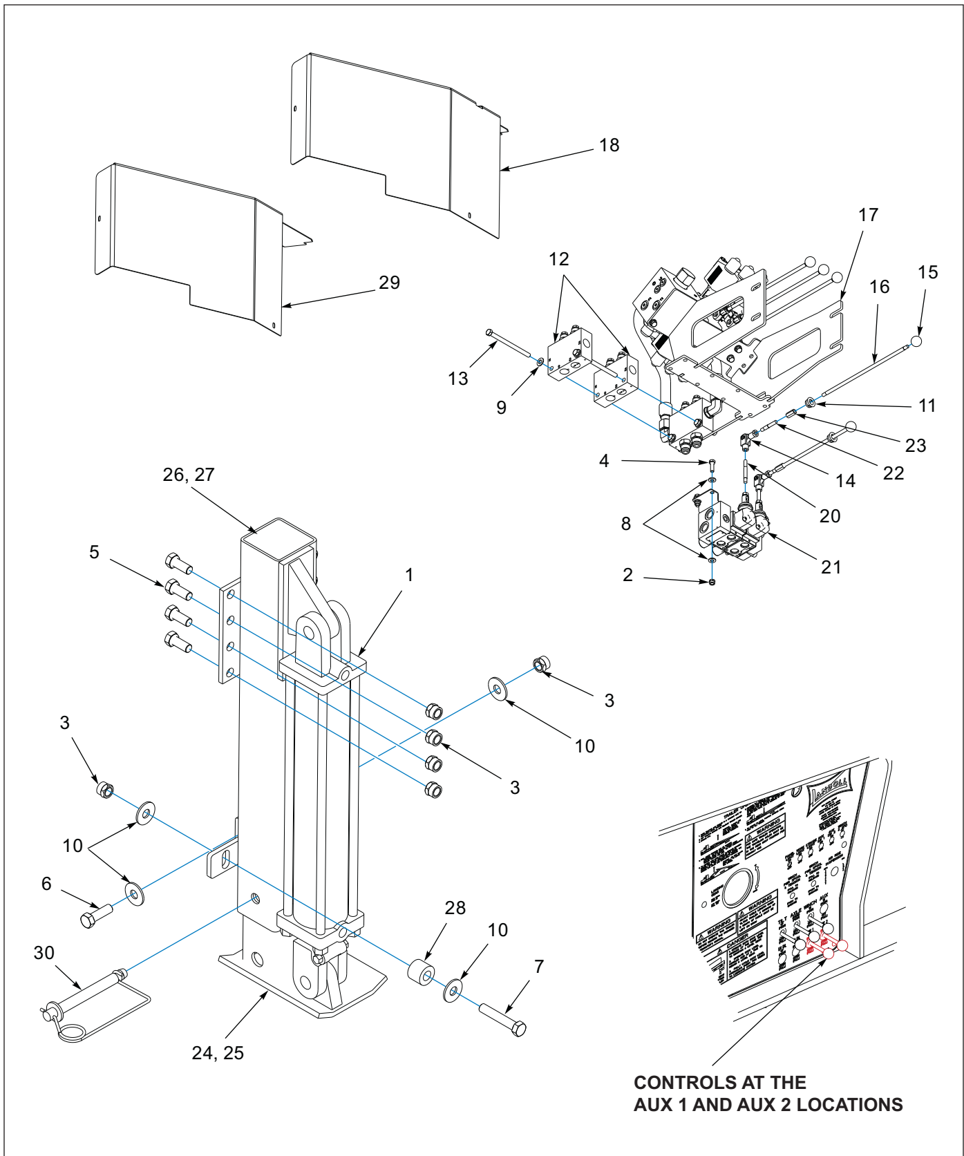
Figure 1-92: Hydraulic Park Stand - General Items
