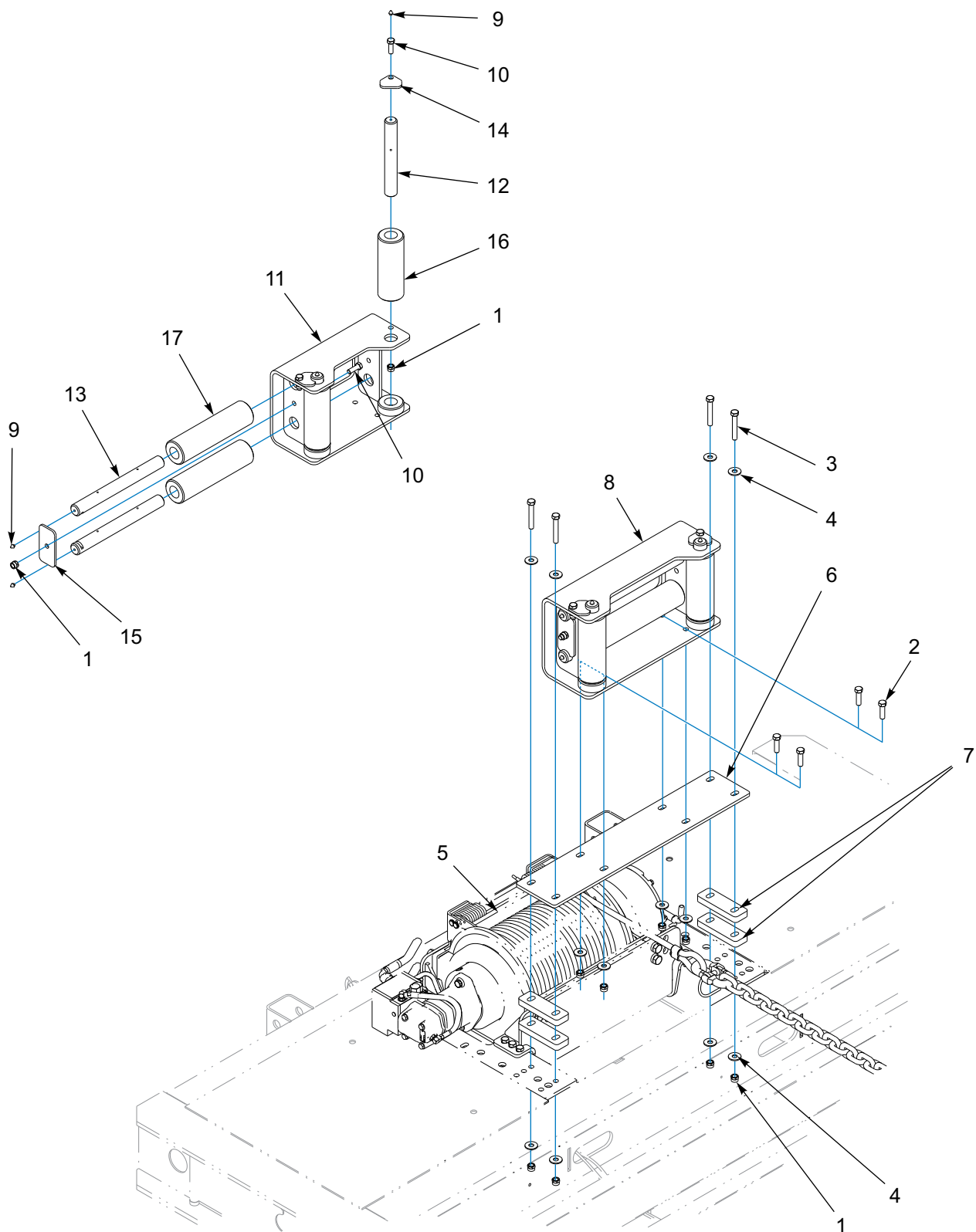
Figure 1-105: 4 Roller Guide Installation - 20K/30K (WARN)
