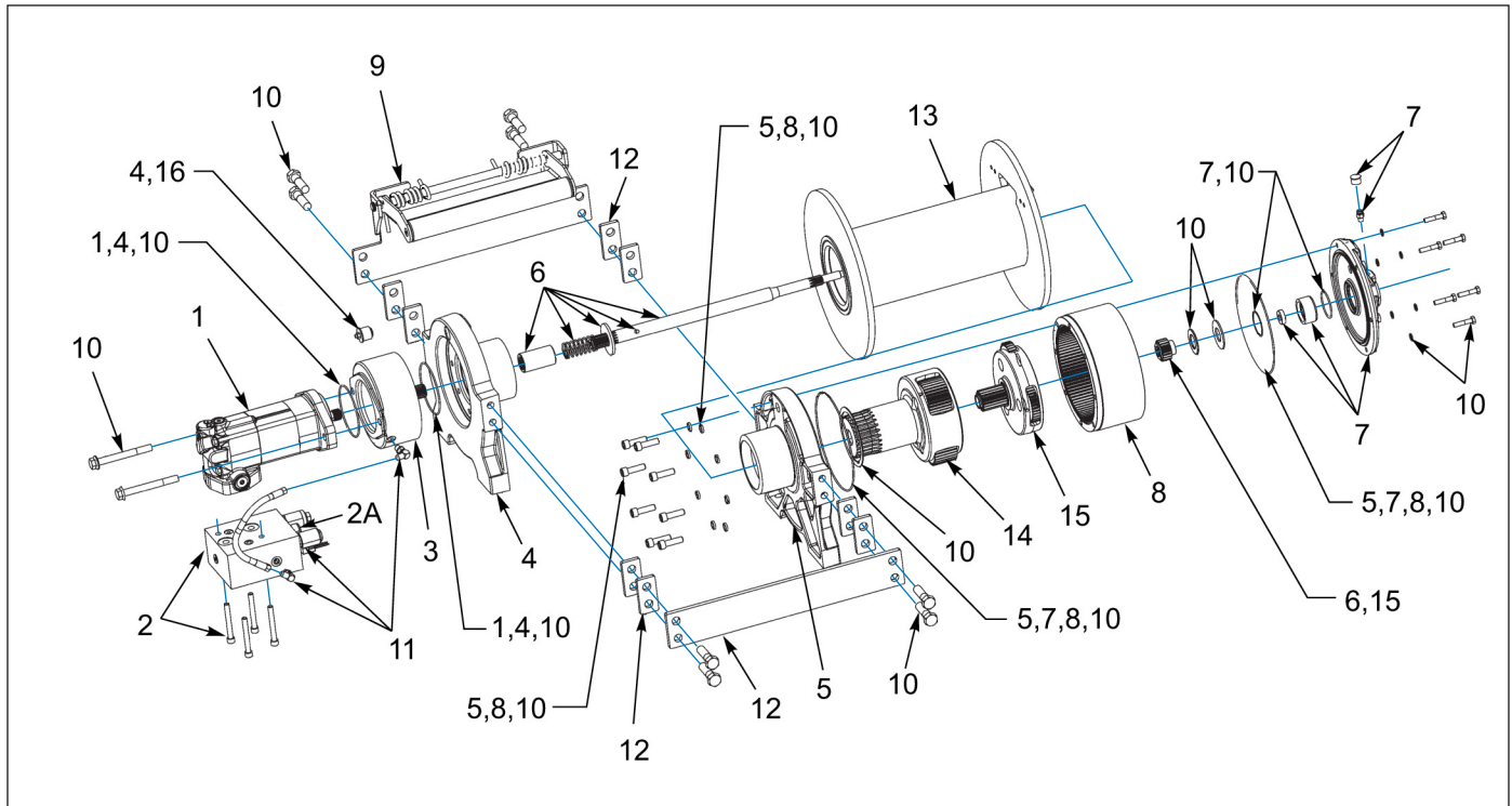
Figure 1-58: Winch Items - 30K 2 Speed (WARN)
