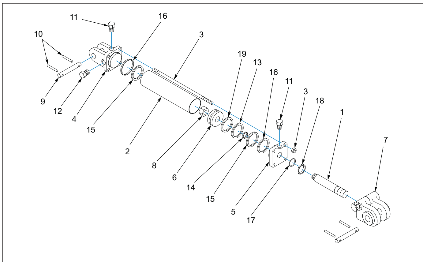
Figure 1-94: Hydraulic Cylinder - 3-1/2 X 20
