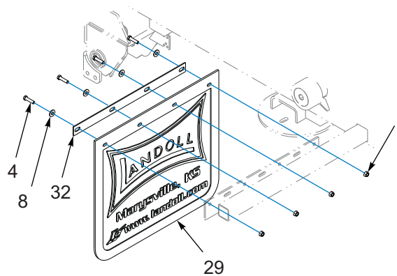
MUDFLAP ASSEMBLY
