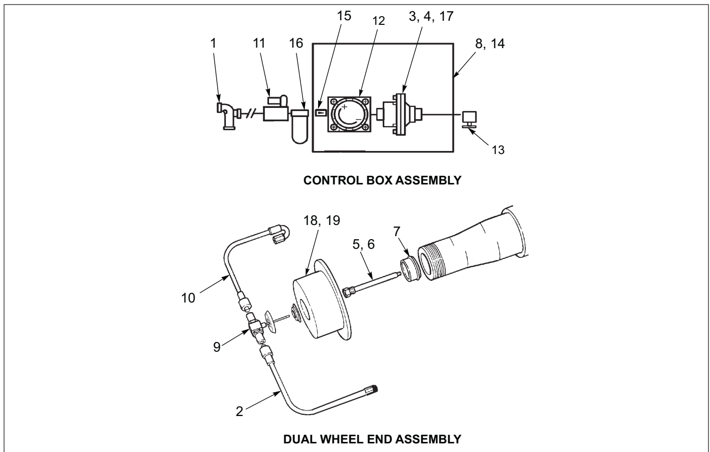
Figure 1-44: Tire Inflation System -Thermalert (3 SAF Axles)
