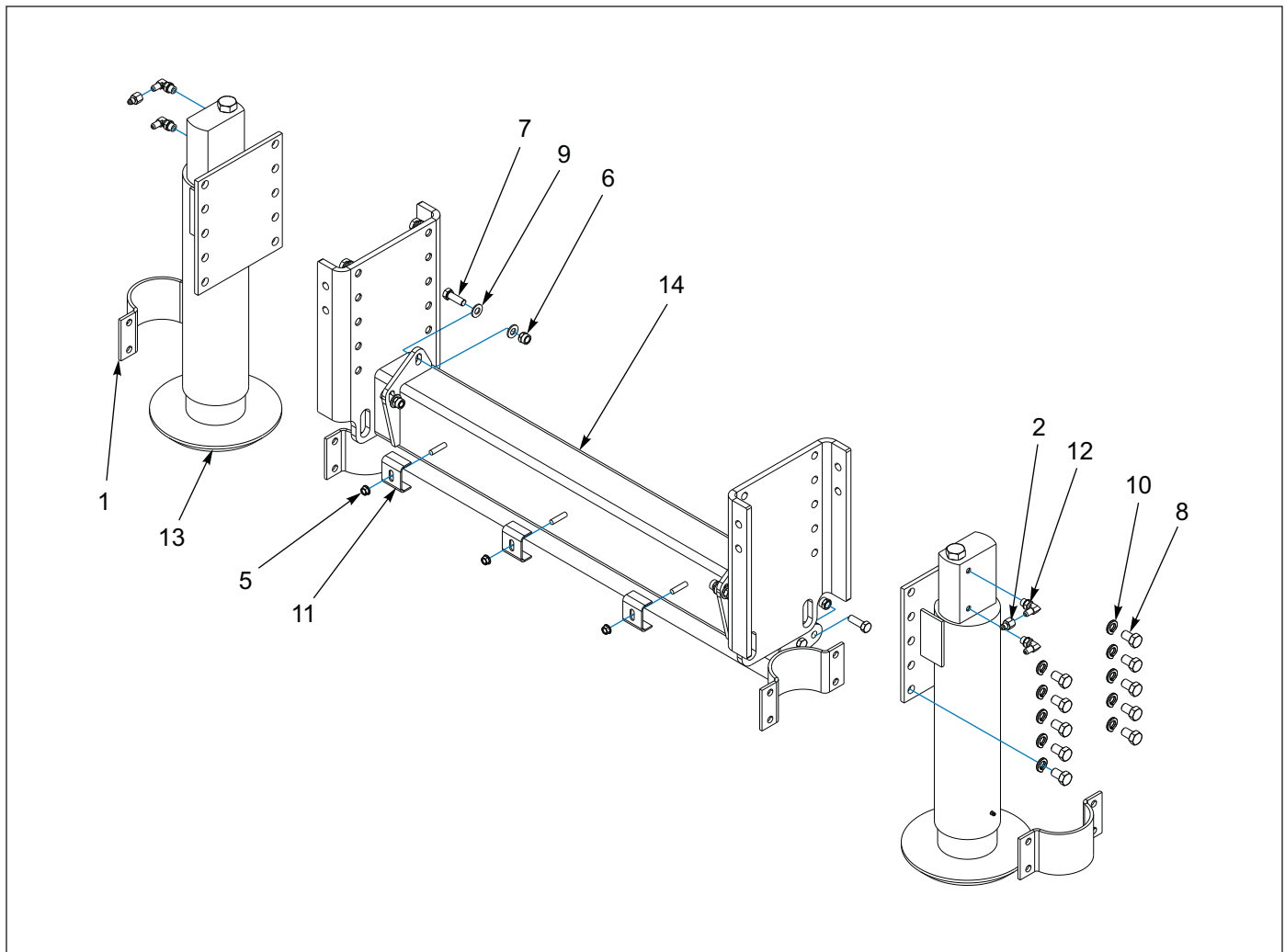
Figure 1-65: Dock Leveler Assembly - Single 60K (400-102 Big Brake)
