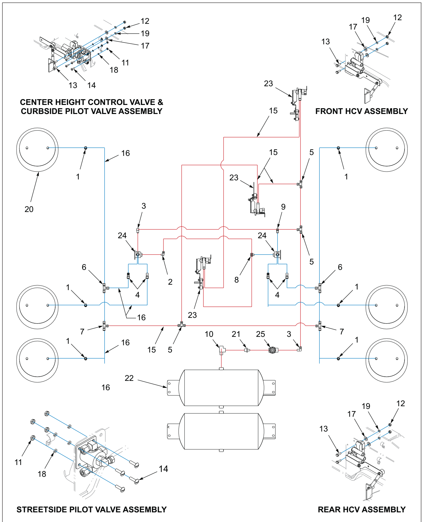
Figure 1-31: Air Ride Suspension - 455B
