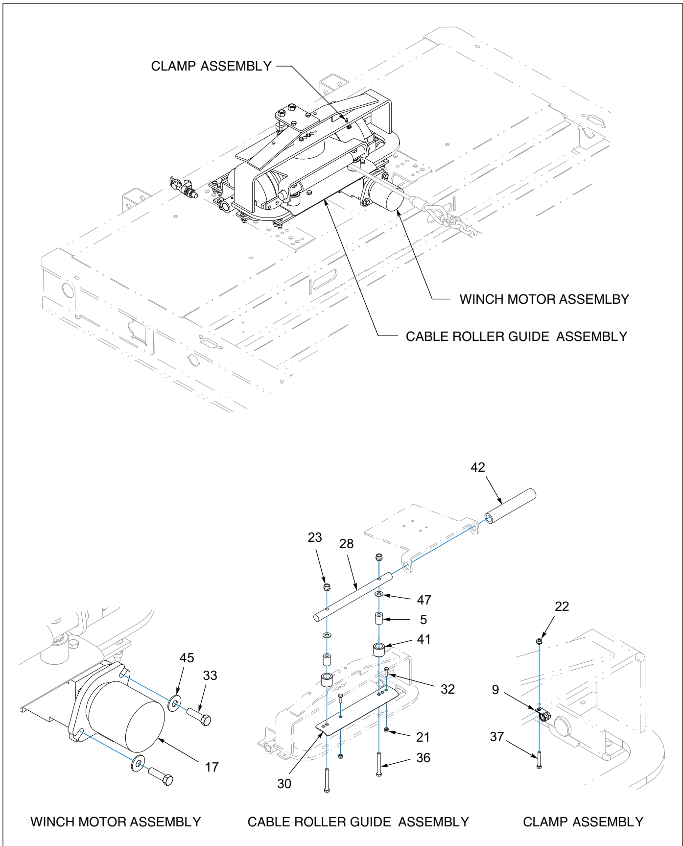
Figure 1-50: 20K Air Tension/Release (BRADEN) (2 of 3)
