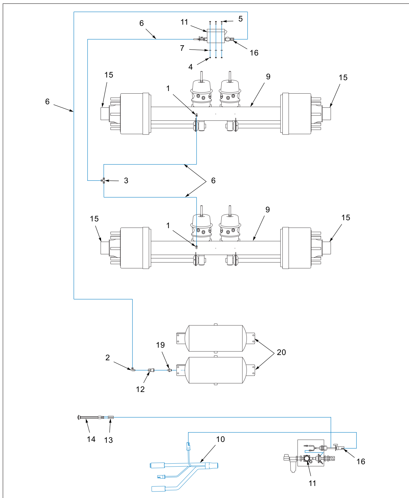
Figure 1-42: Thermalert Tire Inflation System - 440B
