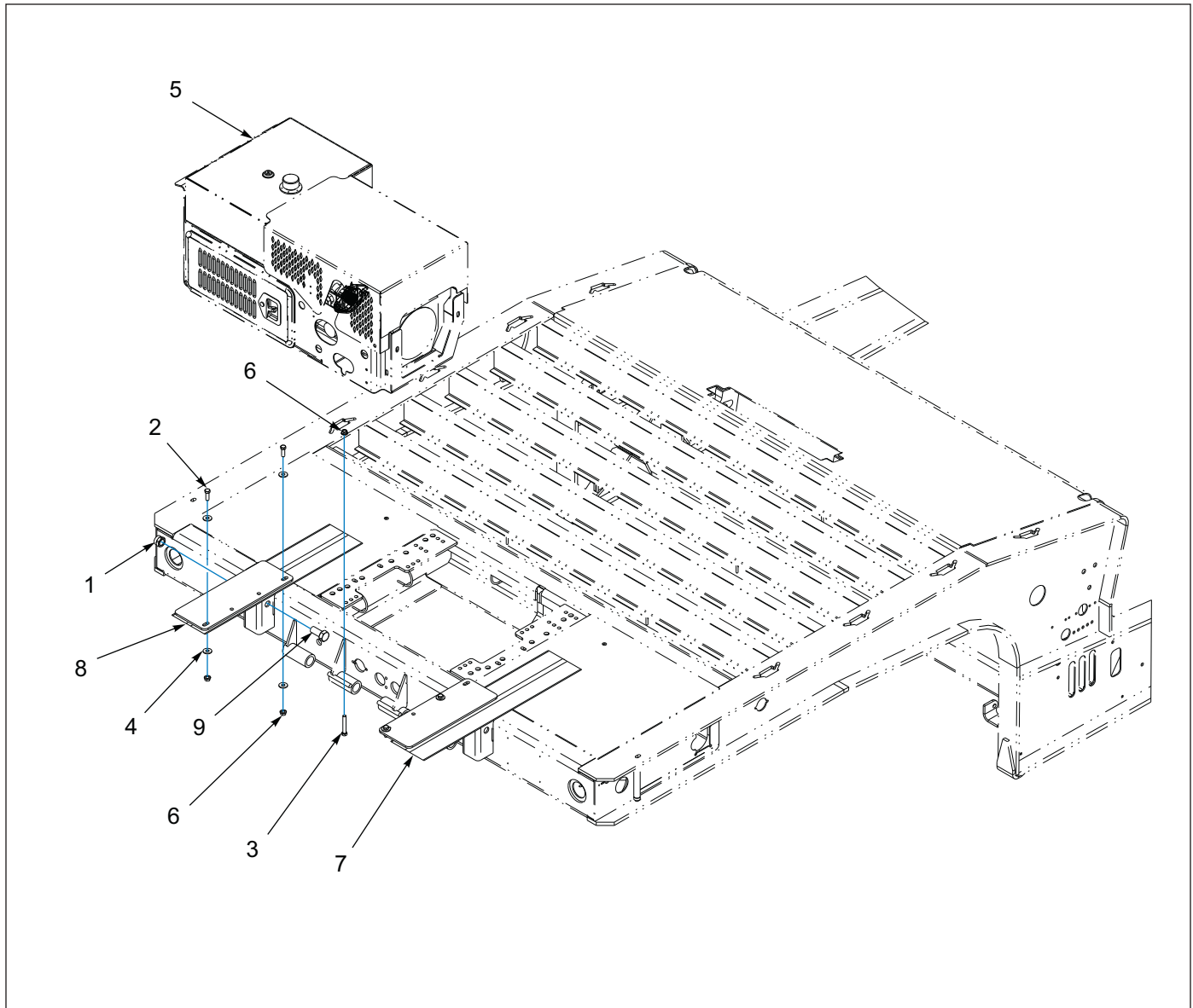
Figure 1-87: Engine - Front Mount Installation
