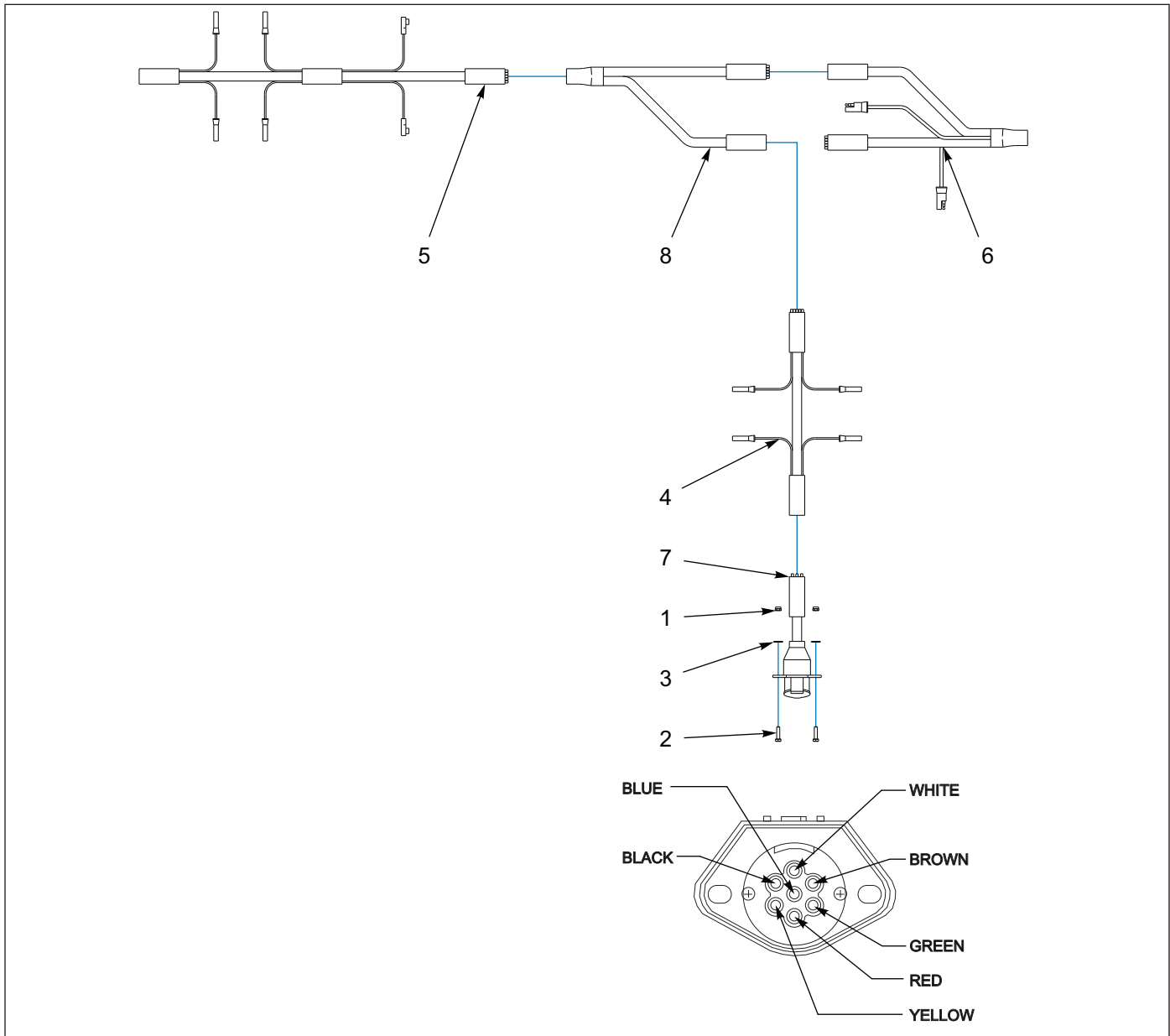
Figure 1-80: 7-Way Electrical Installation
