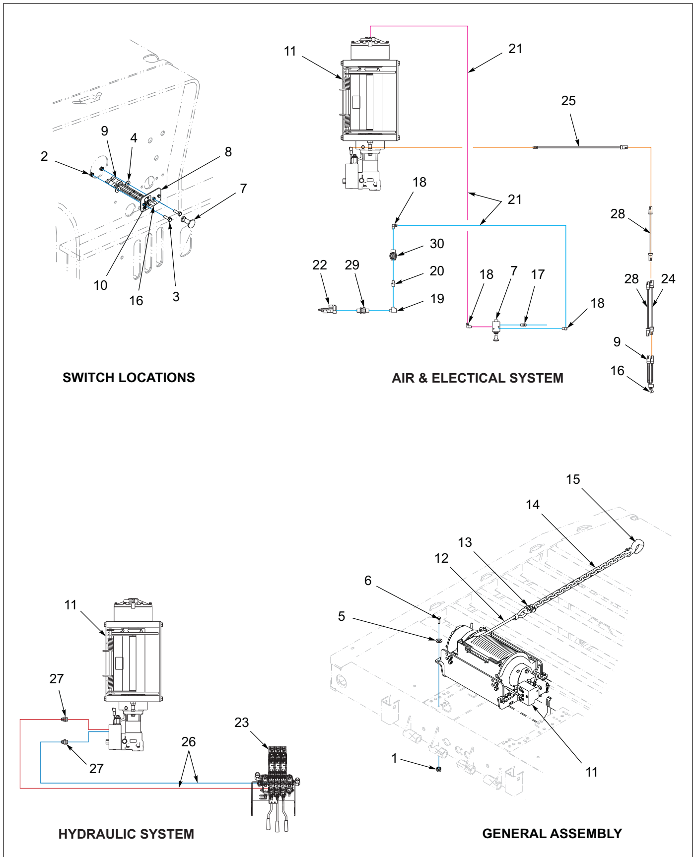
Figure 1-55: 20K 2 Speed (WARN)
