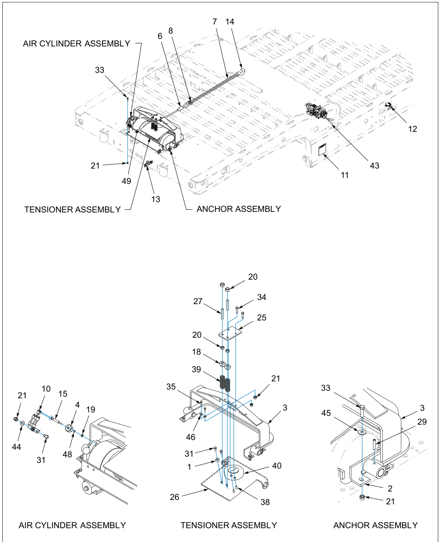
Figure 1-49: 20K Air Tension/Release (BRADEN) (1 of 3)
