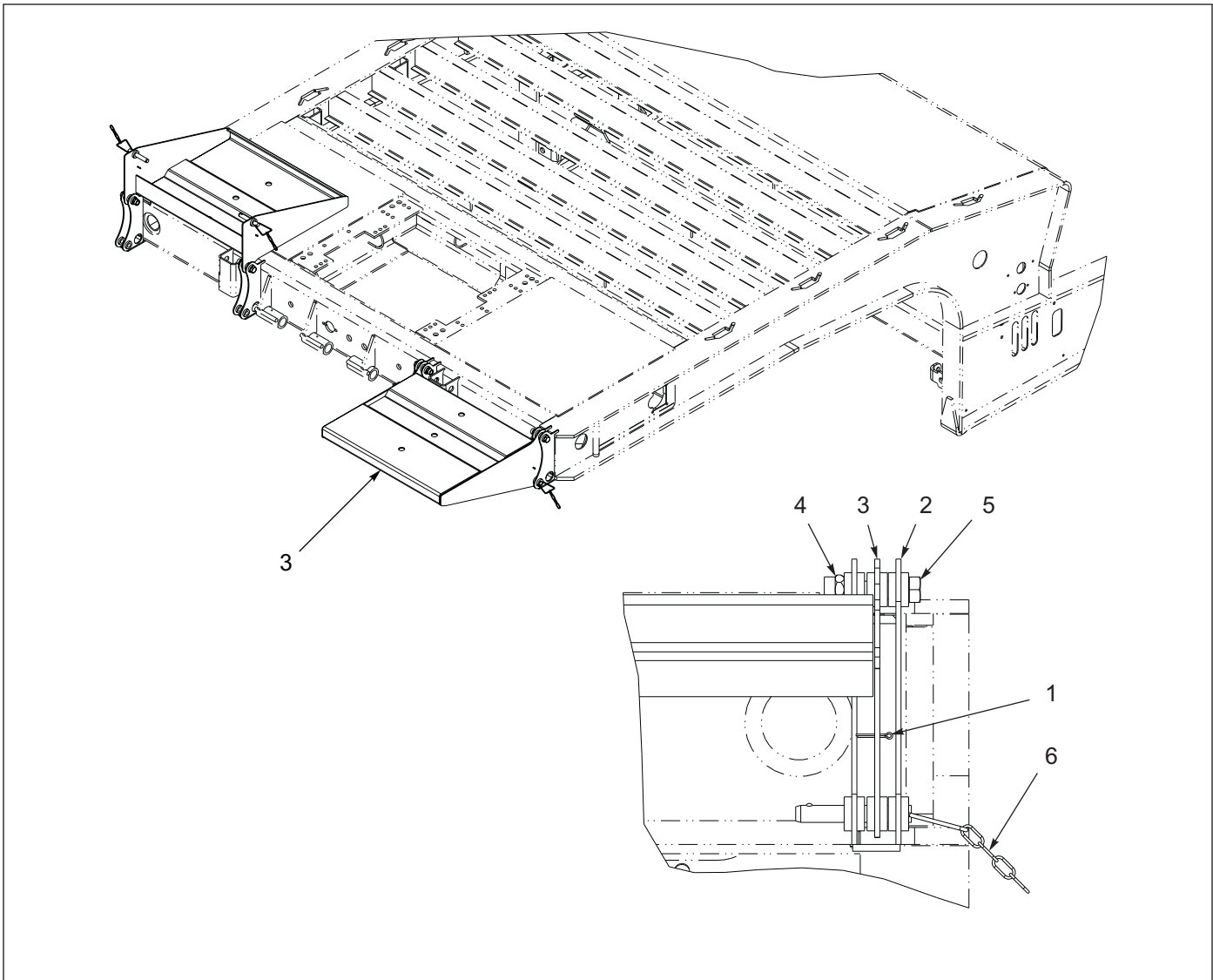
Figure 1-122: Front Flip Extension
