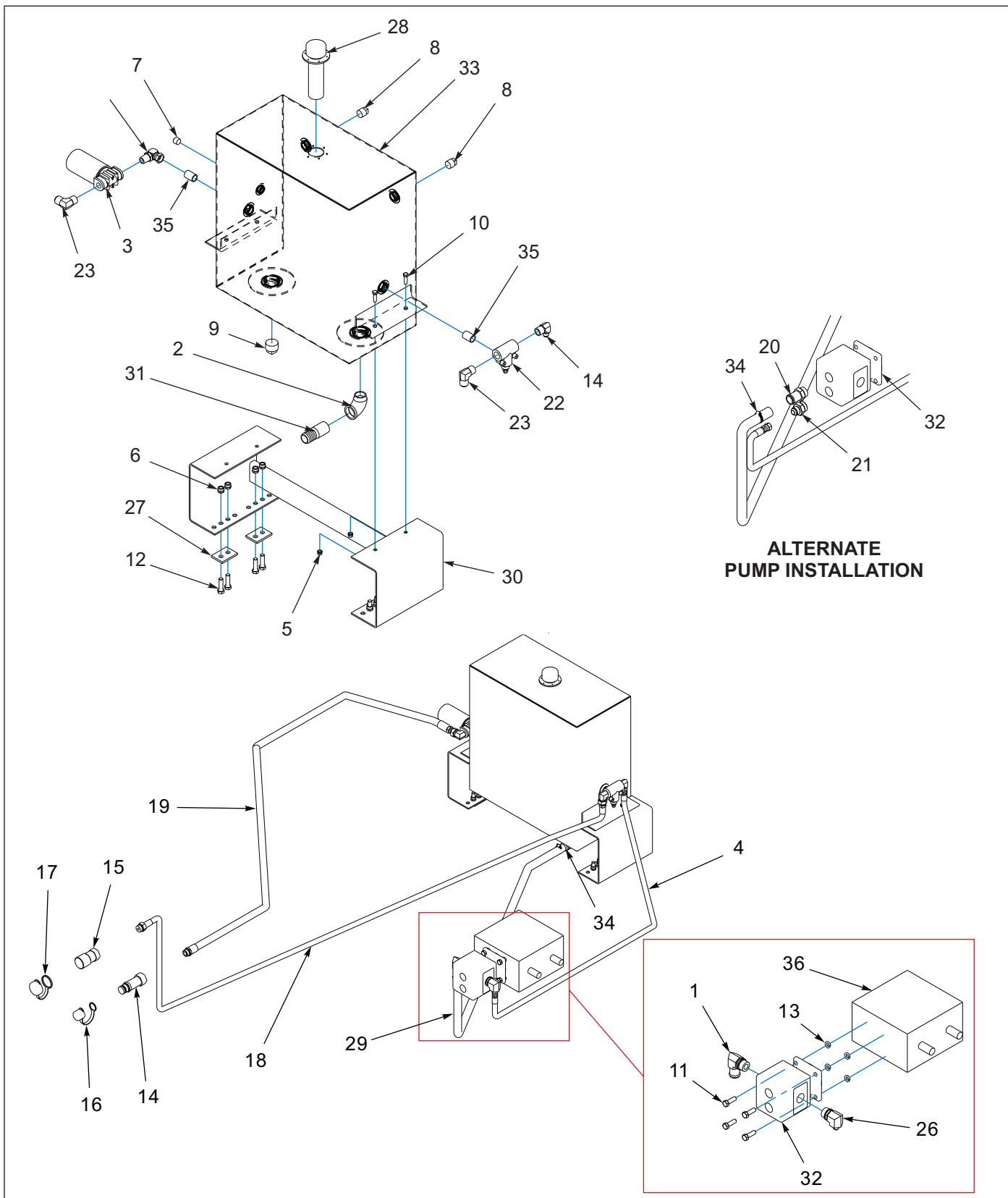
Figure 1-89: Hydraulic Wet Kit Items - 30 Gallon
