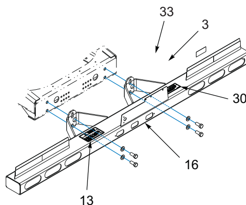
BUMPER ASSEMBLY
