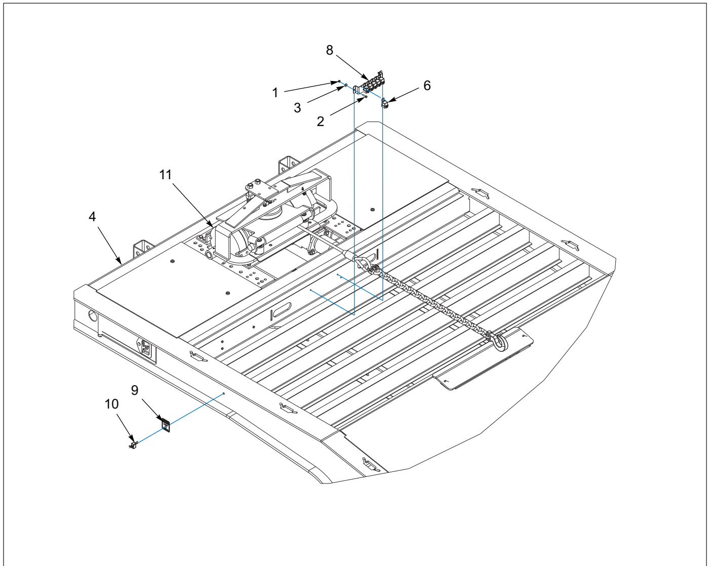
Figure 1-121: Electrical Disconnect Switch Installation
