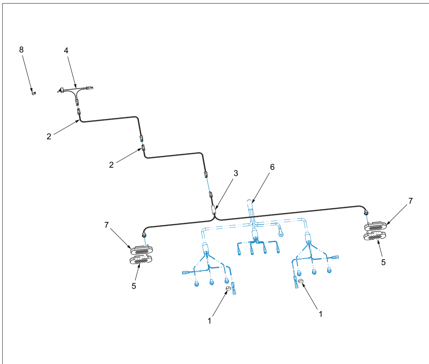
Figure 1-79: Bumper - Strobe Installation - Option
