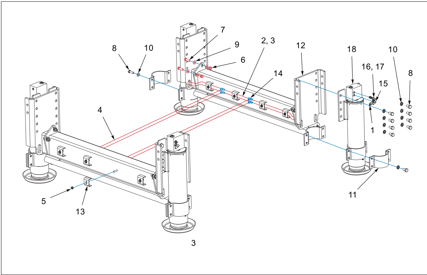
Figure 1-66: Dock Level Assembly - Single 120K
