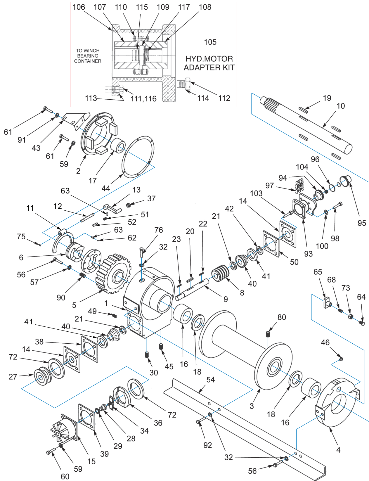
Figure 1-52: Winch Items - 20,000Lb. (BRADEN)
