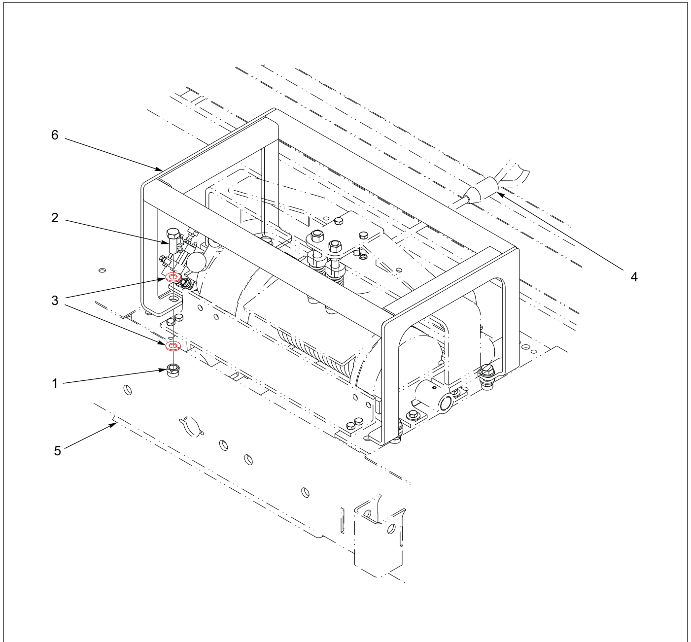
Figure 1-117: Guard Installation, Winch 20K Pivot
