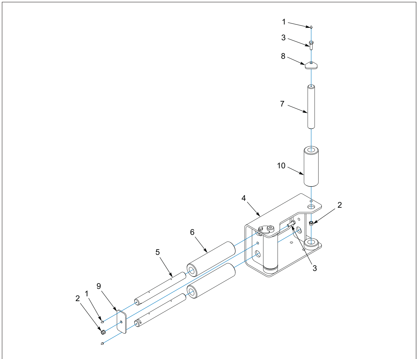
Figure 1-115: Winch - 12K Guide Assembly (BRADEN)
