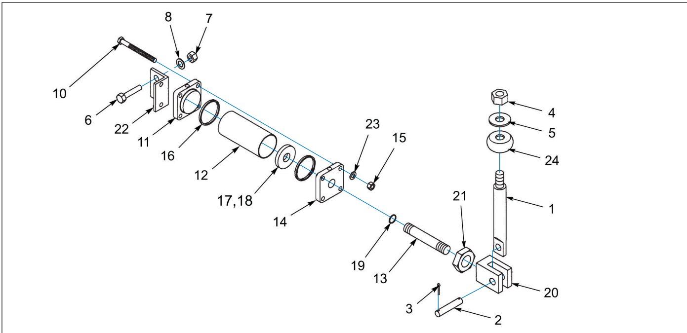
Figure 1-53: Winch - Air Shift Cylinder
