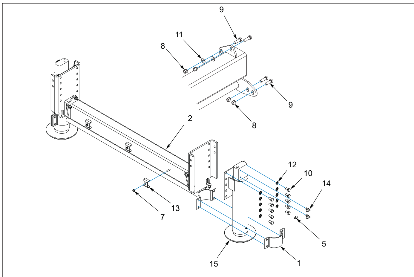
Figure 1-64: Dock Leveler Assembly - Single 60K
