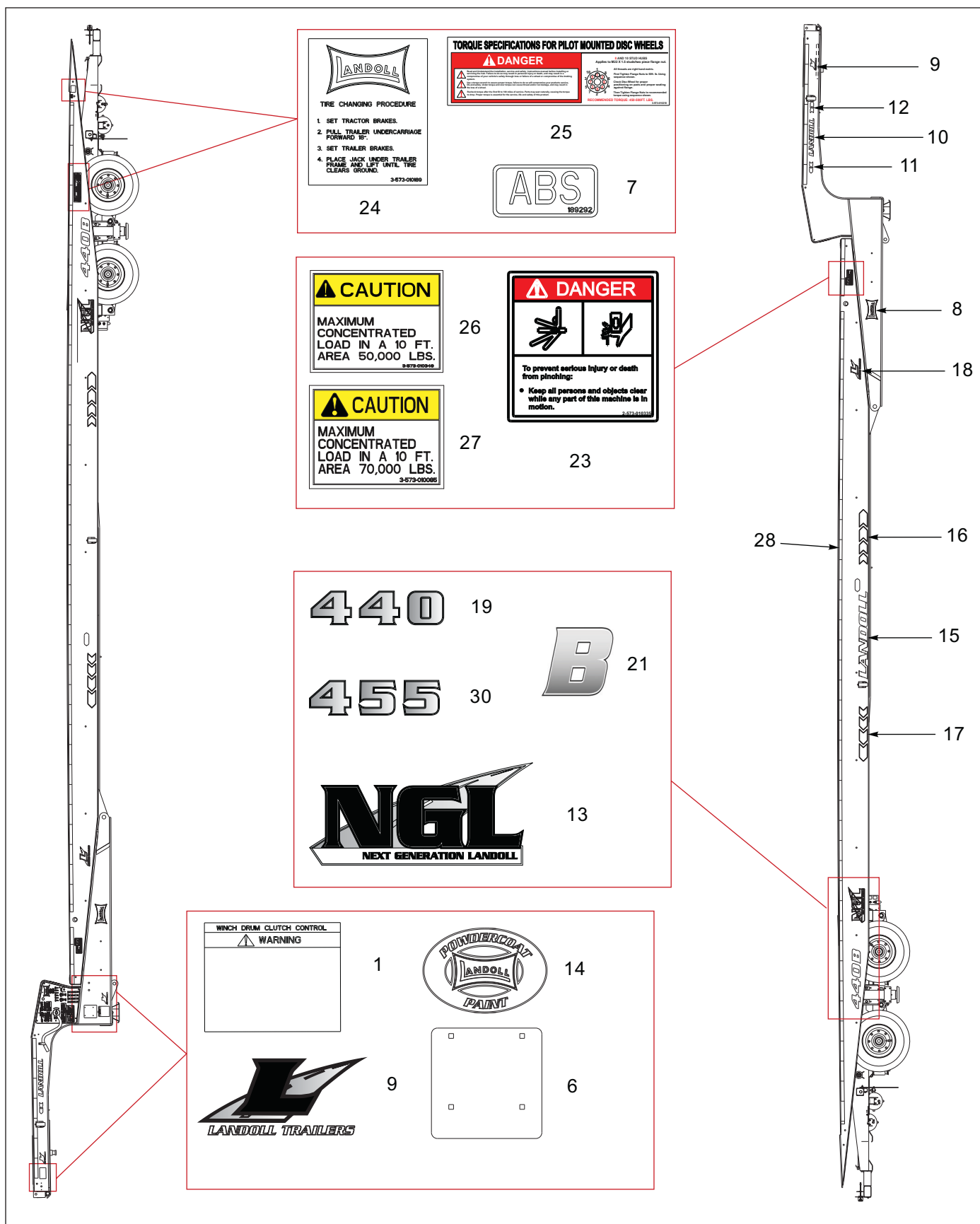
Figure 1-4: Decal Installation (2 of 2)
