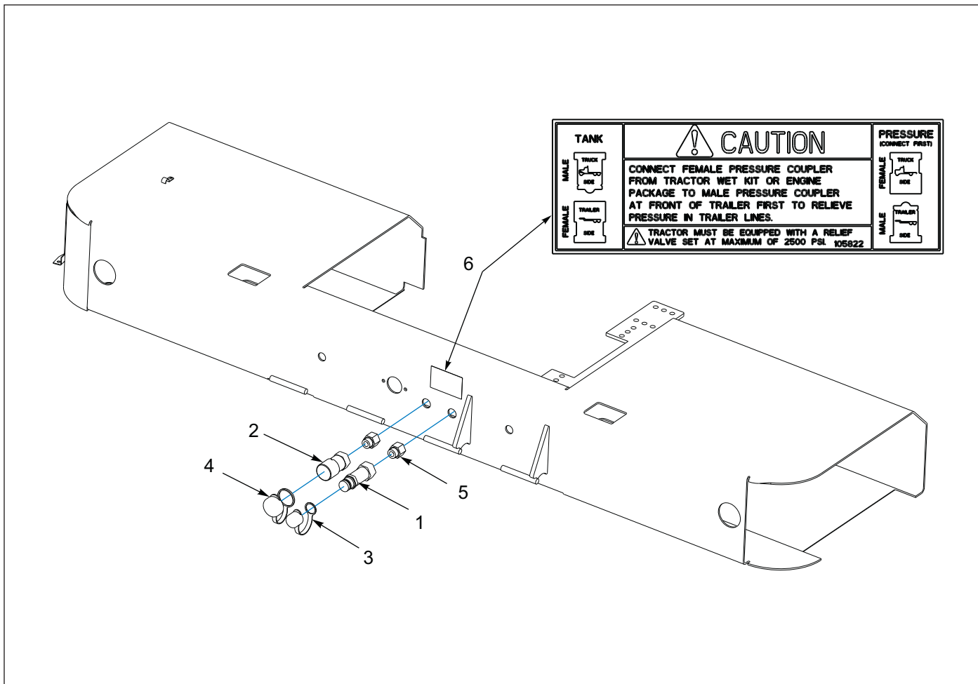
Figure 1-91: Hydraulic Conversion Kit - Ball to Flat
