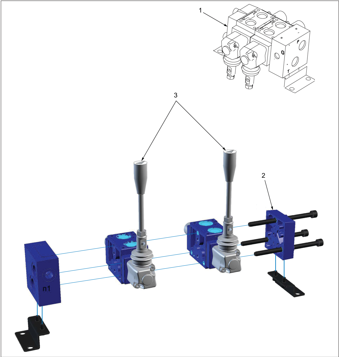
Figure 1-69: Dock Leveler Valve
