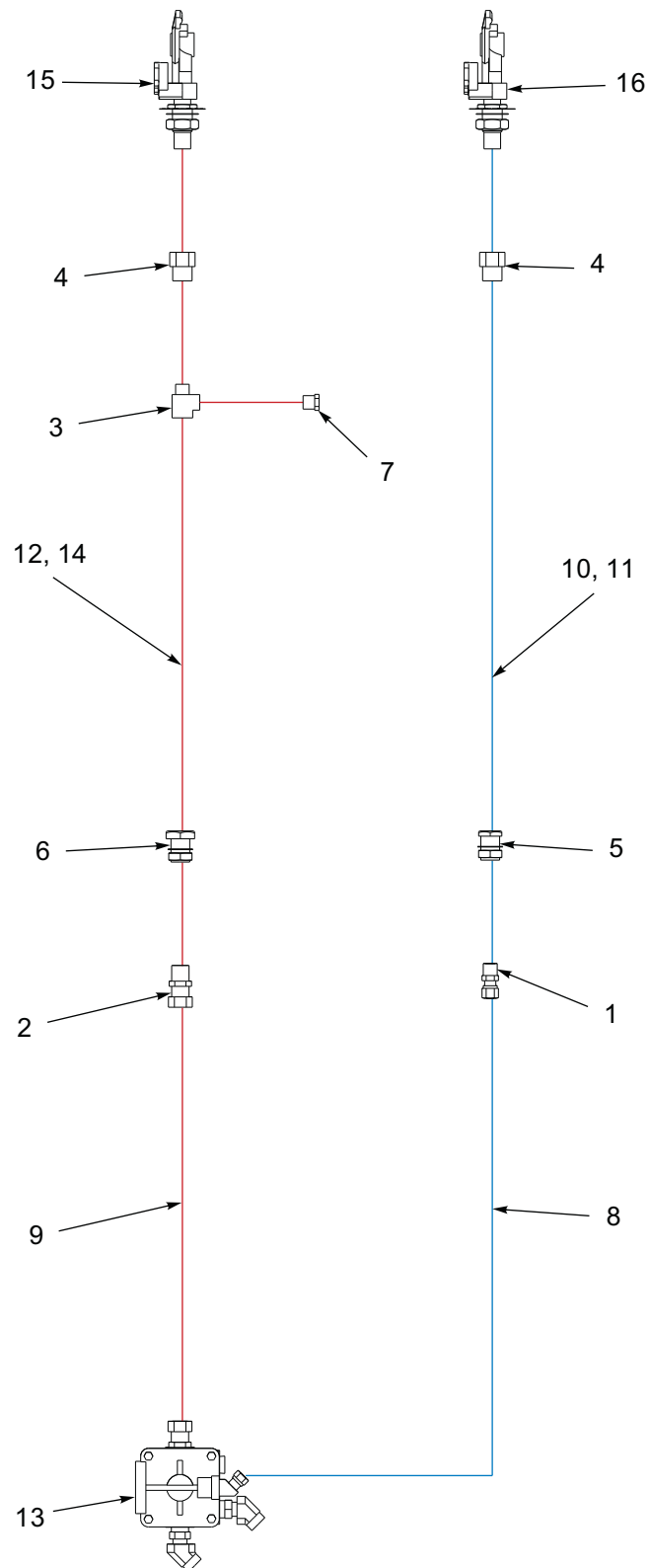
Figure 1-10: Air System
