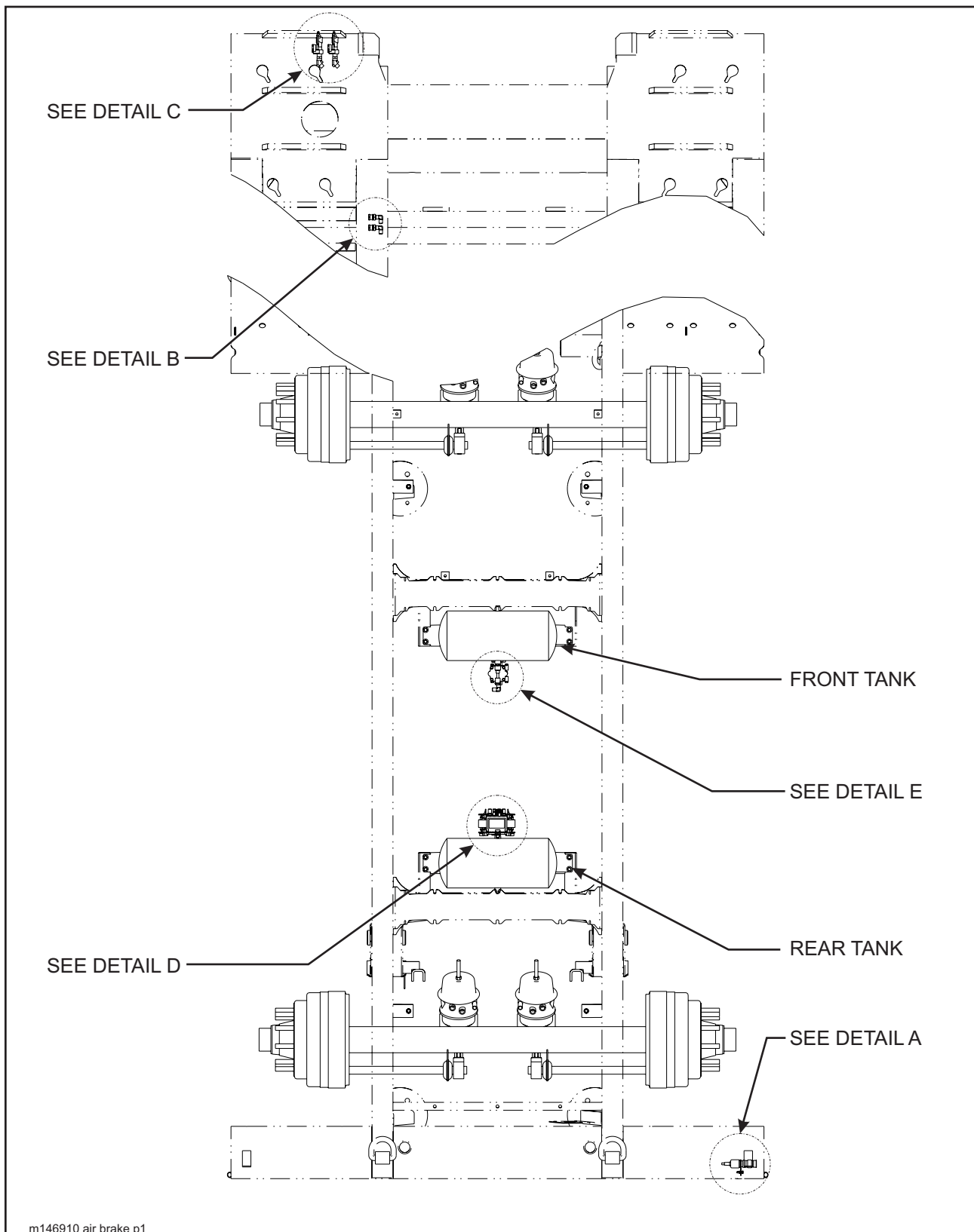
Figure 1-37 Air Brake System (835B Spread Axle)
