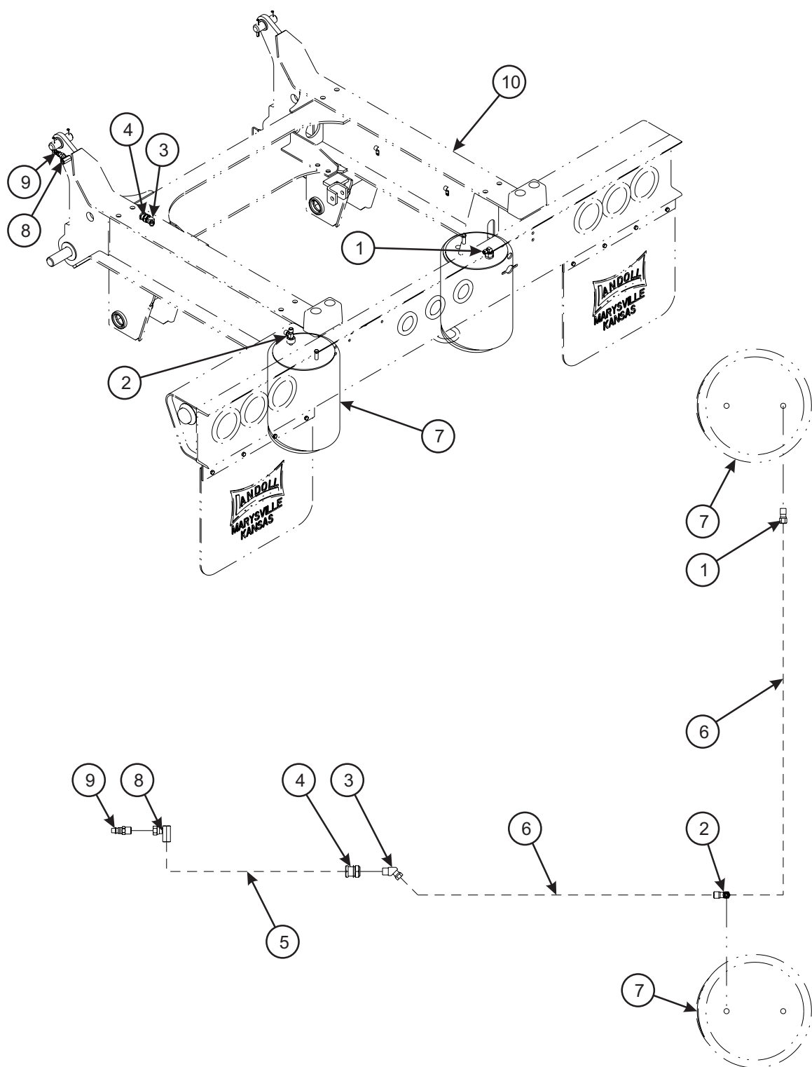
Figure 1-19 Flip Assembly - Air Ride Suspension
