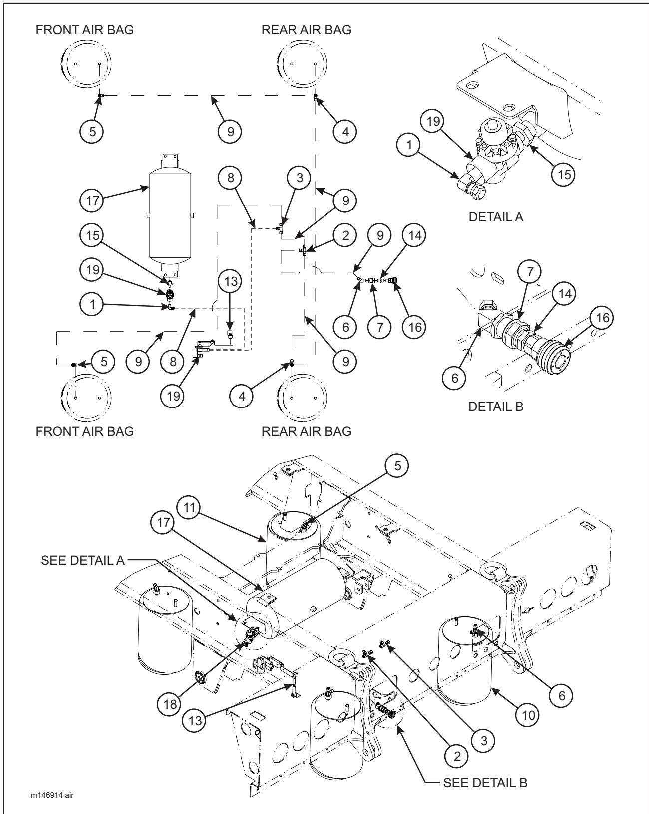
Figure 1-18 Frame Assembly - Air Ride Suspension (835B)
