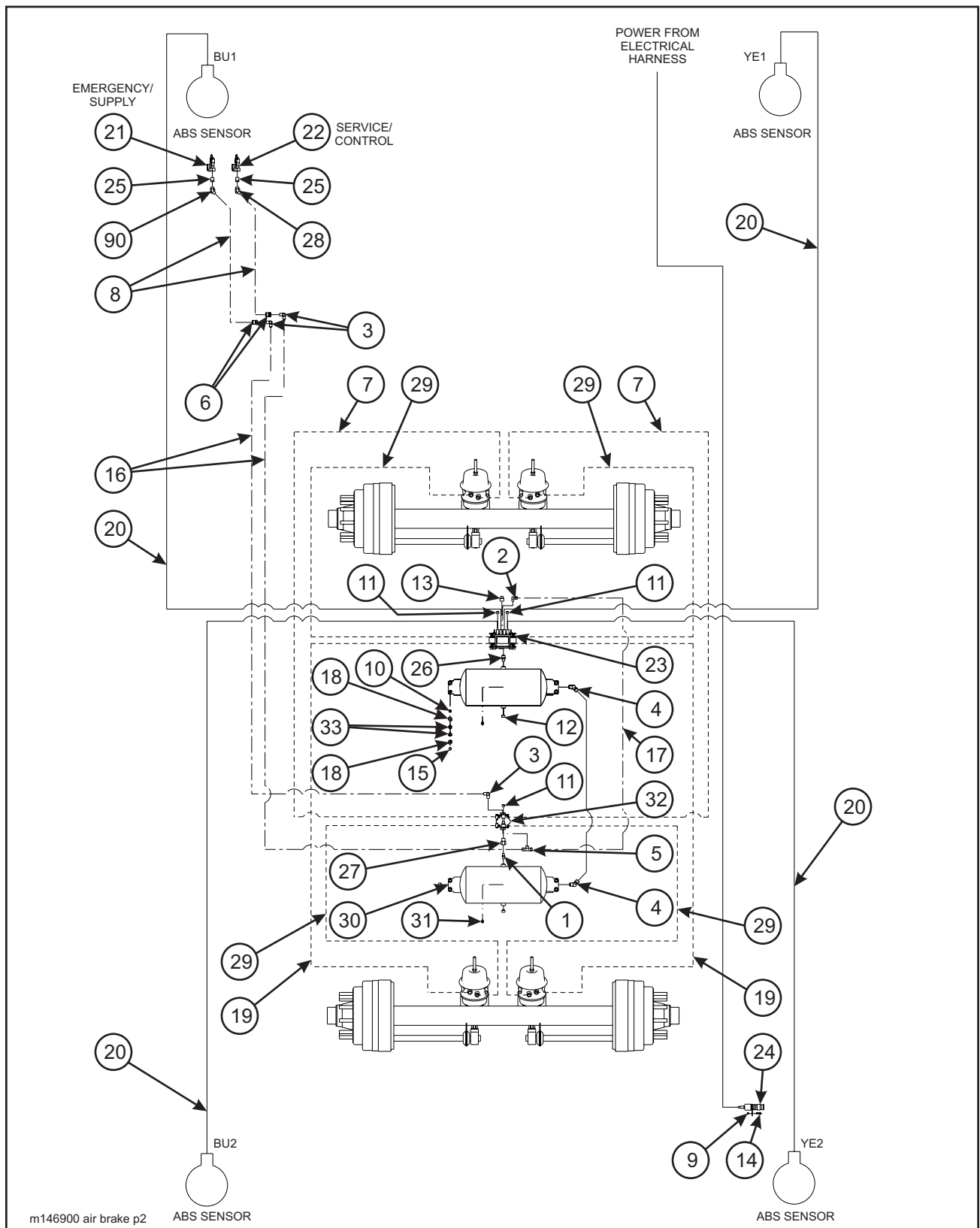
Figure 1-34 Air Brake System (825B)
