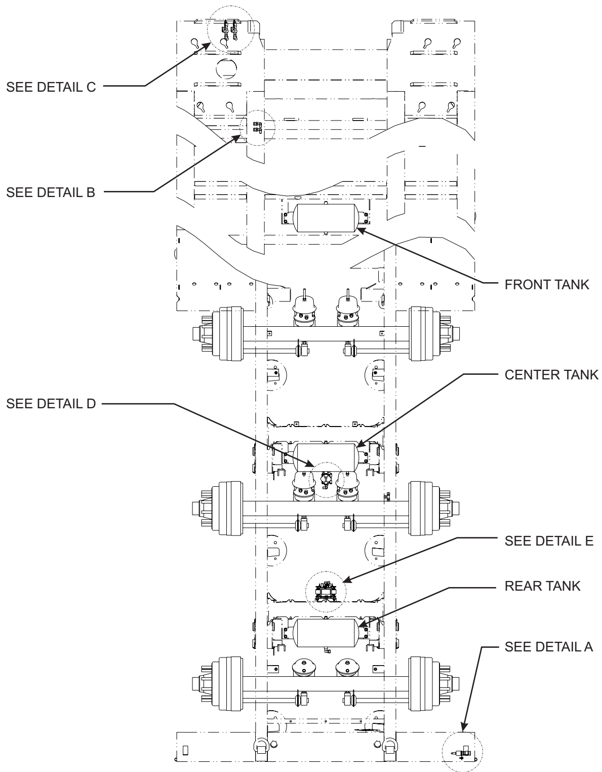
Figure 1-40 Air Brake System (835B Triple Axle) (1 of 3)
