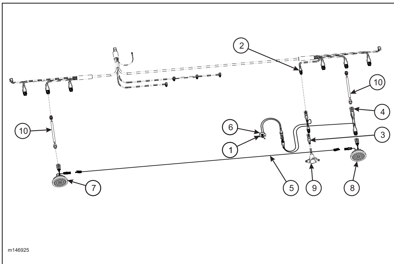
Figure 1-74 Rear Turn/Strobe Light Assembly (Option)
