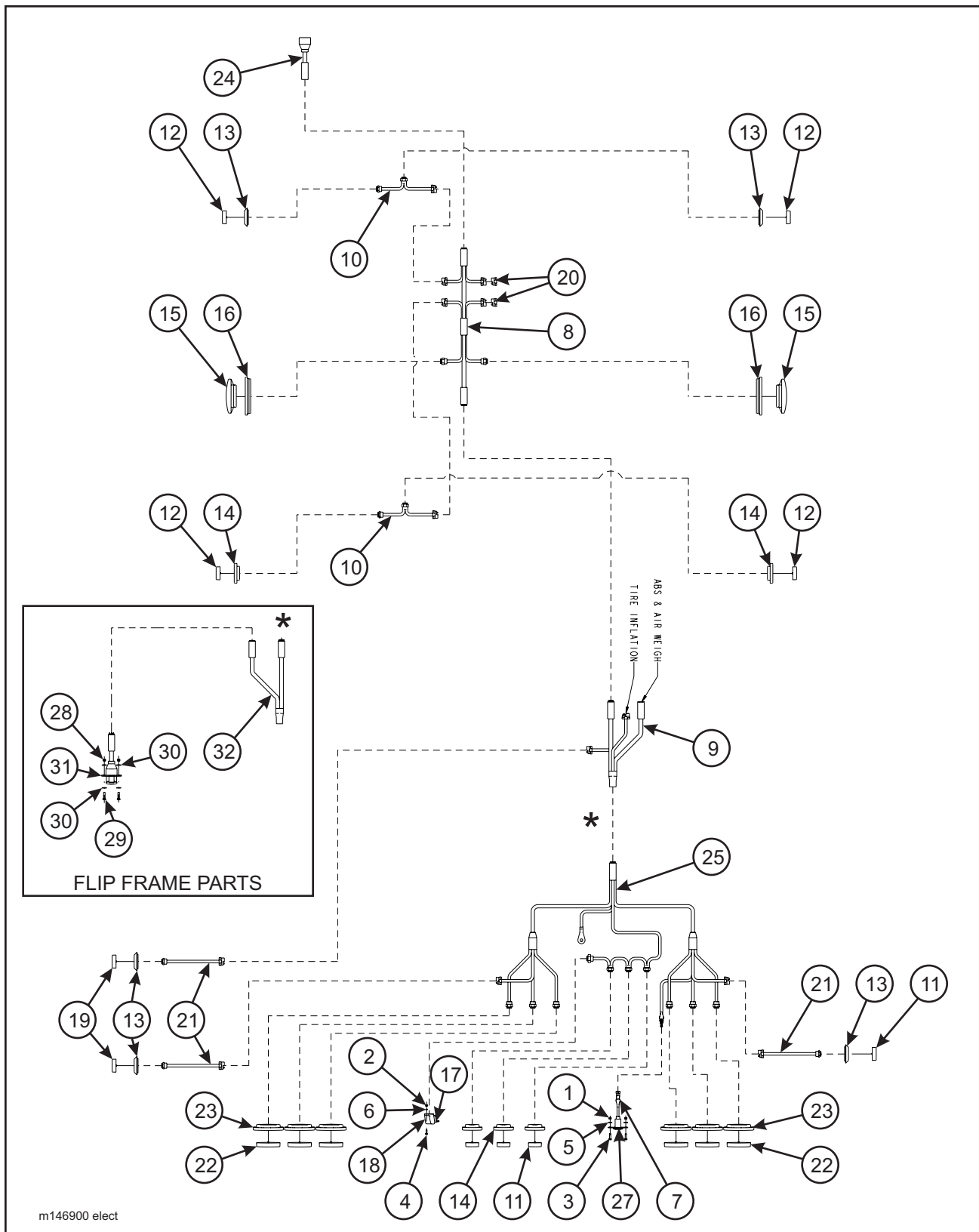
Figure 1-31 Frame Electrical System
