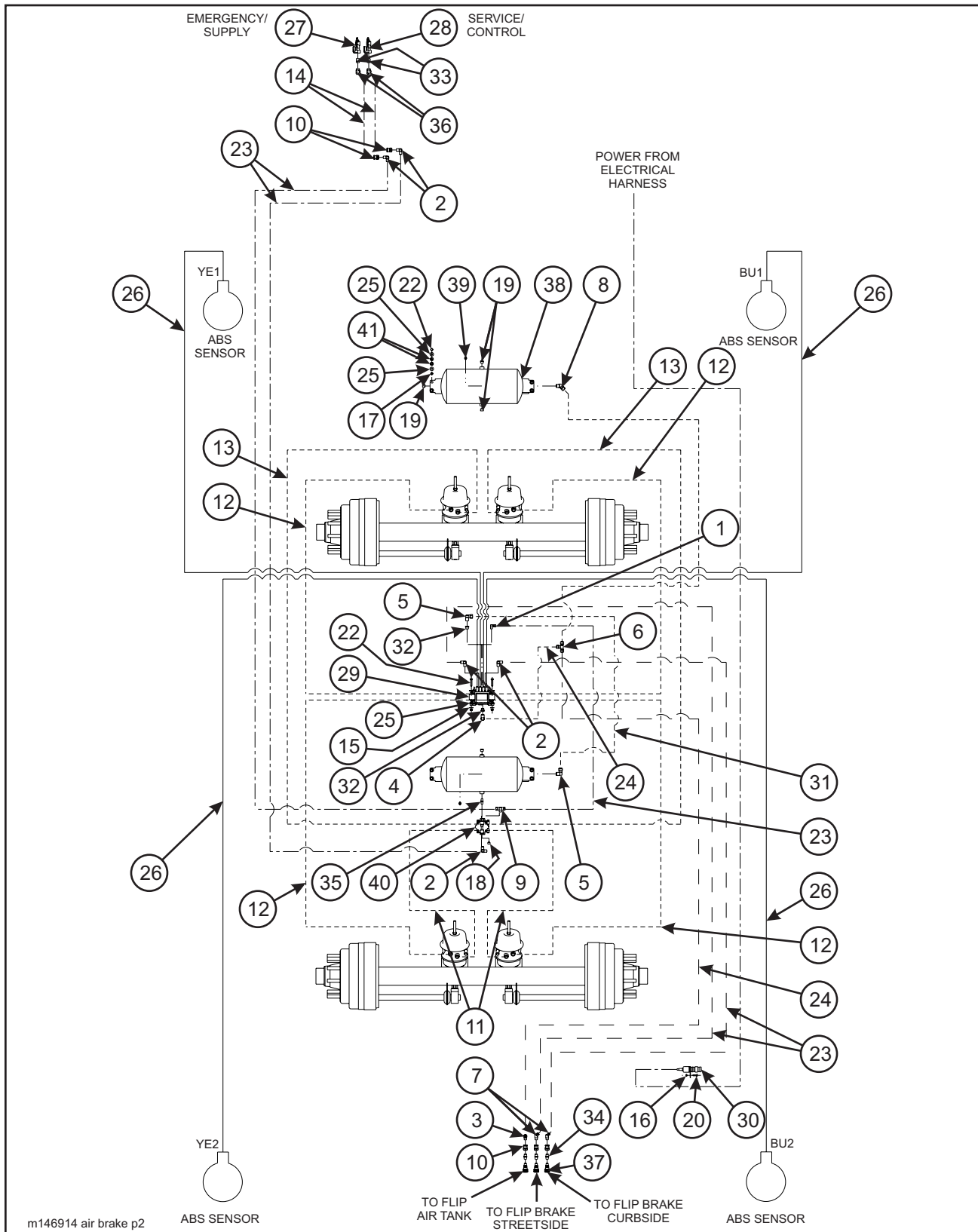
Figure 1-36 Air Brake System (835B w/ Flip Provision)
