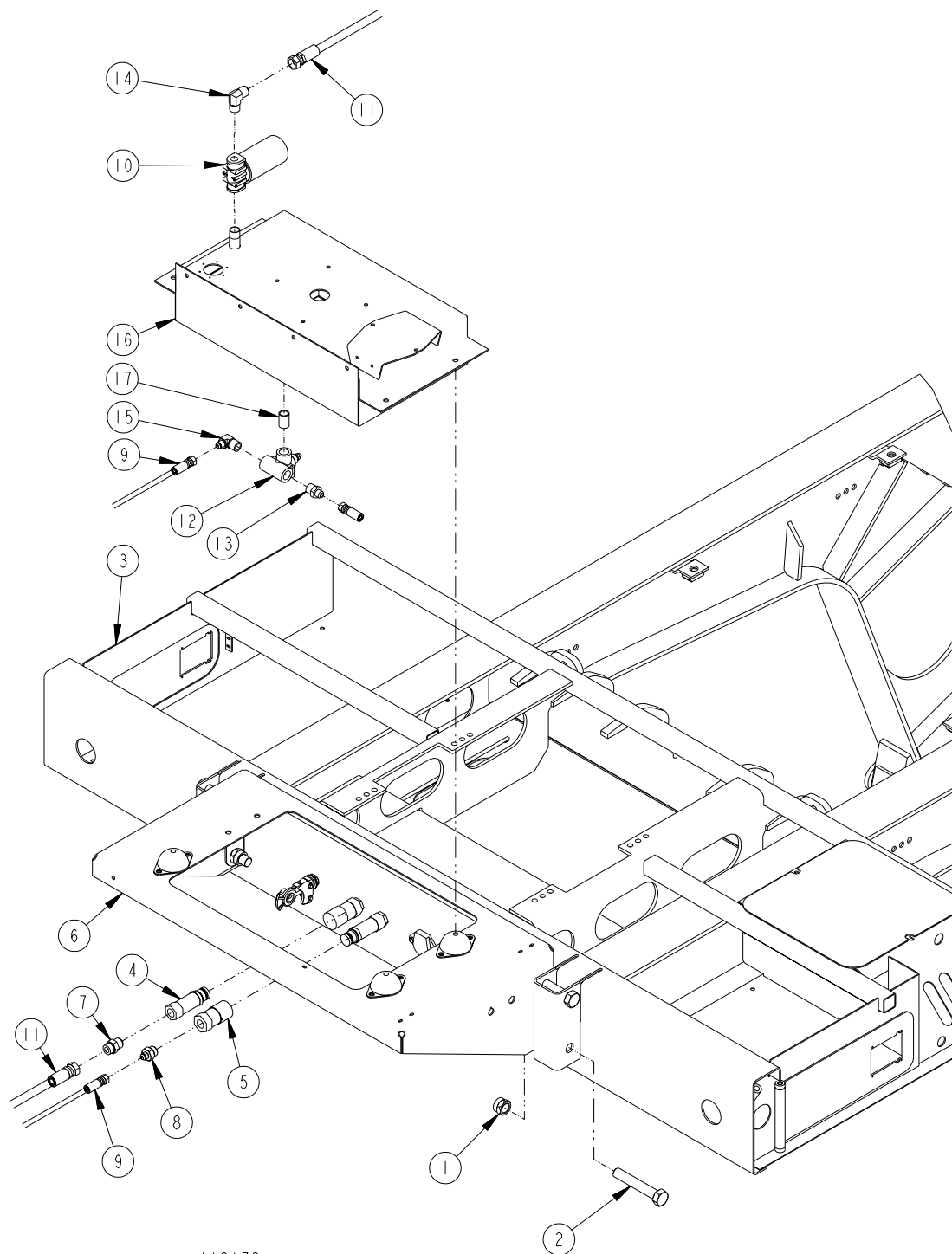
Figure 1-57 Engine Installation Front Mount (Option)
