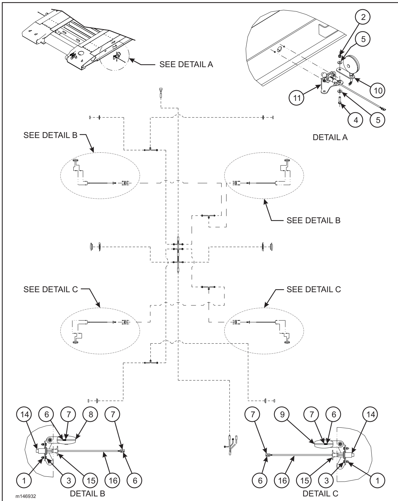
Figure 1-77 Web Mounted Four Corner Light Package (Option)
