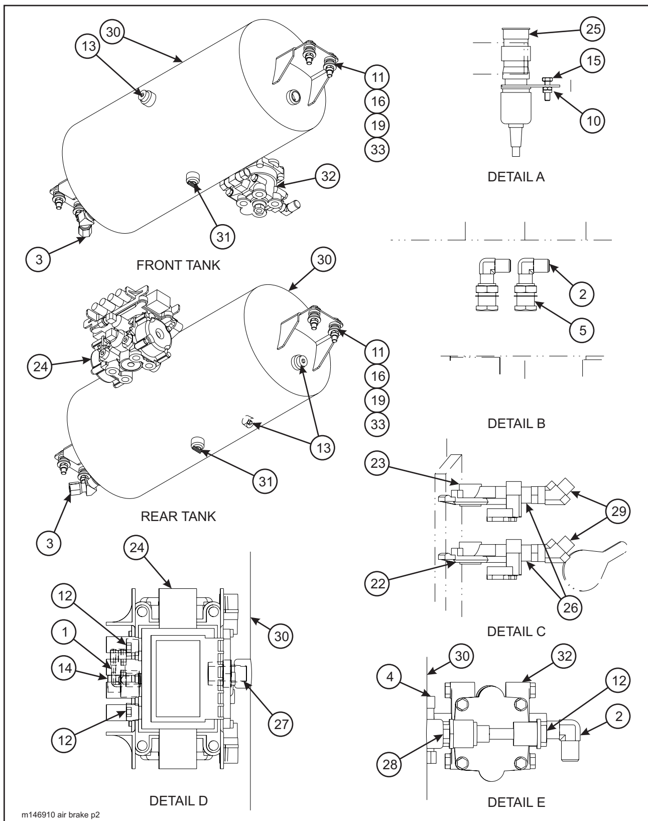
Figure 1-38 Air Brake System (835B Spread Axle)
