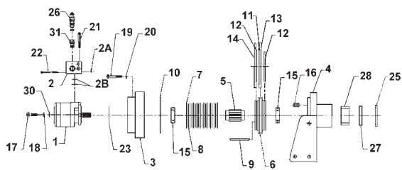
MOTOR END INSTALLATION
