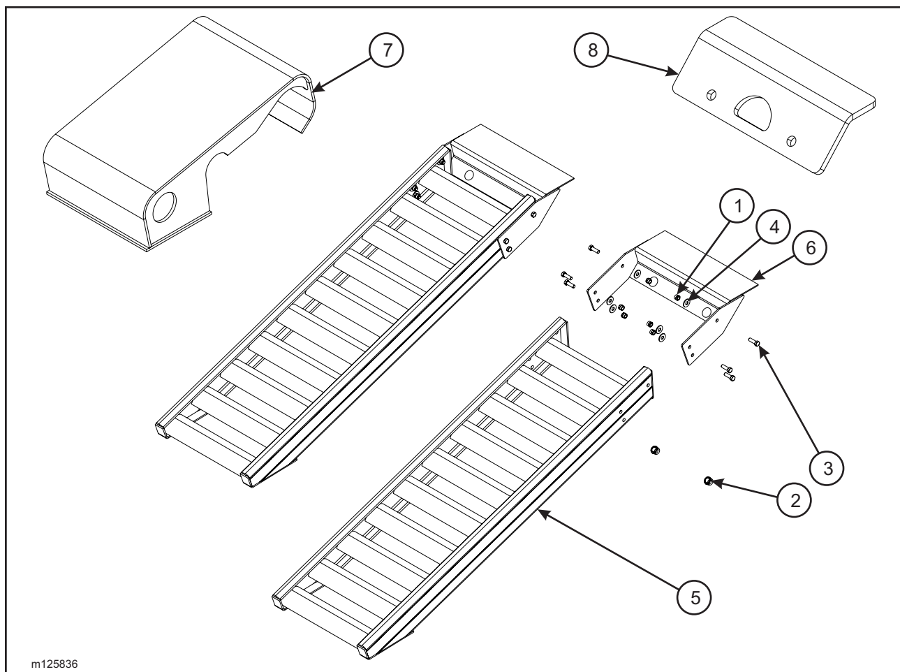
Figure 1-66 Aluminum Trunnion Ramp Assembly (Option)
