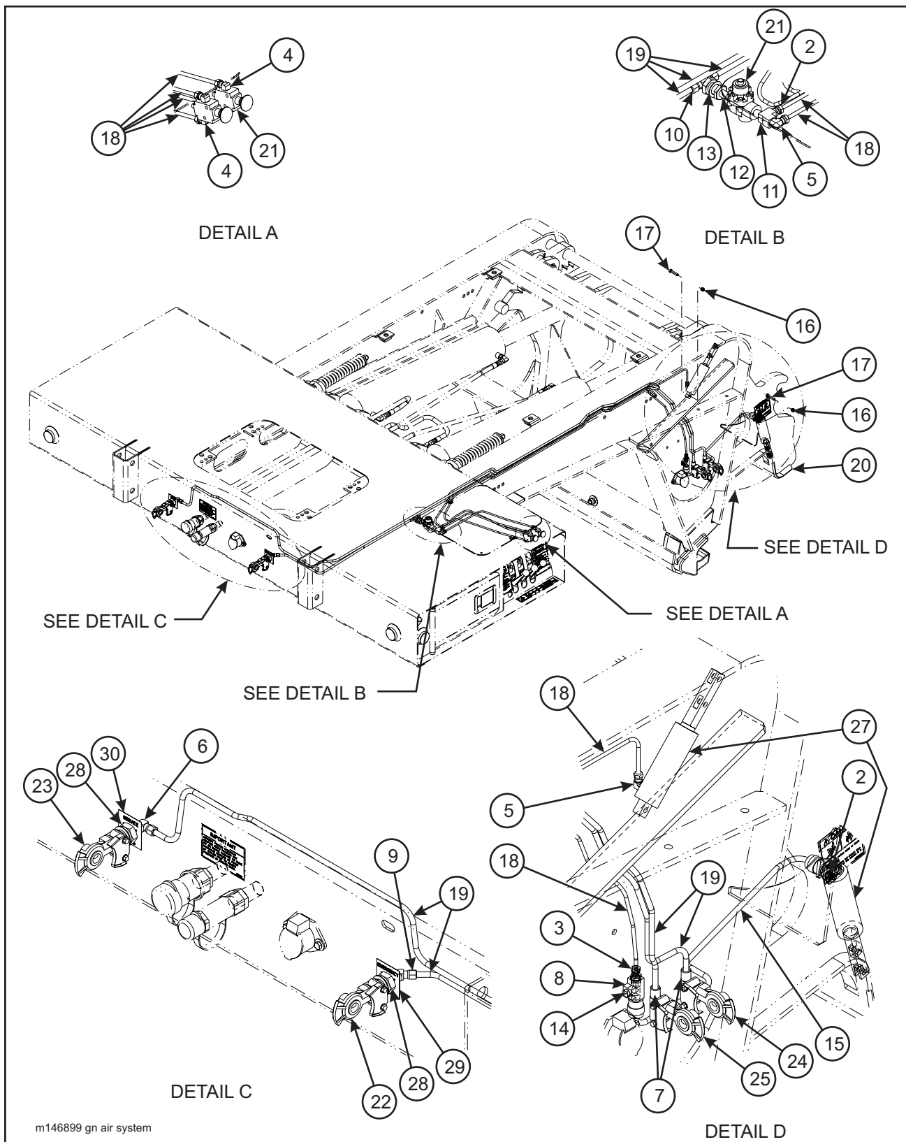
Figure 1-16 Gooseneck Air System
