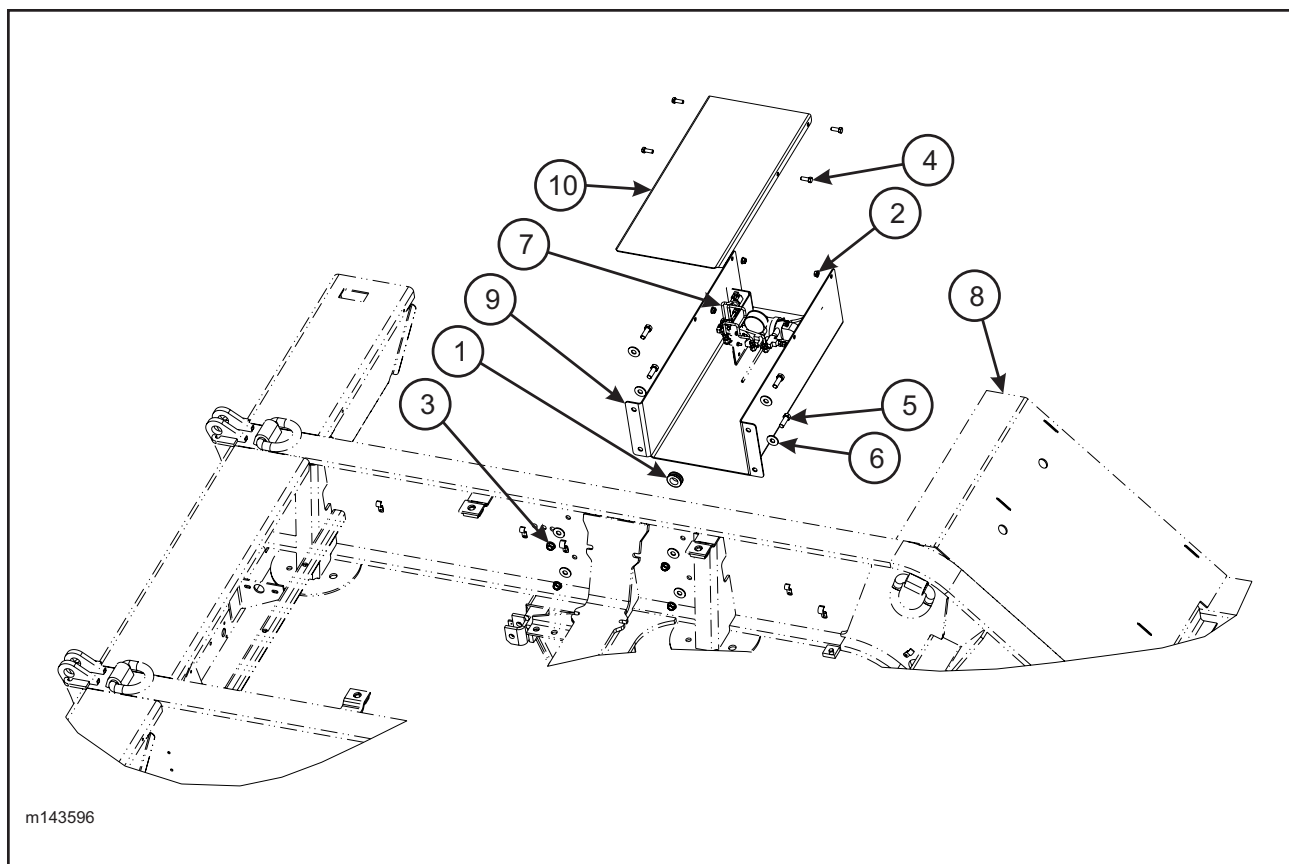
Figure 1-68 Air R/L Mount Kit (Option)
