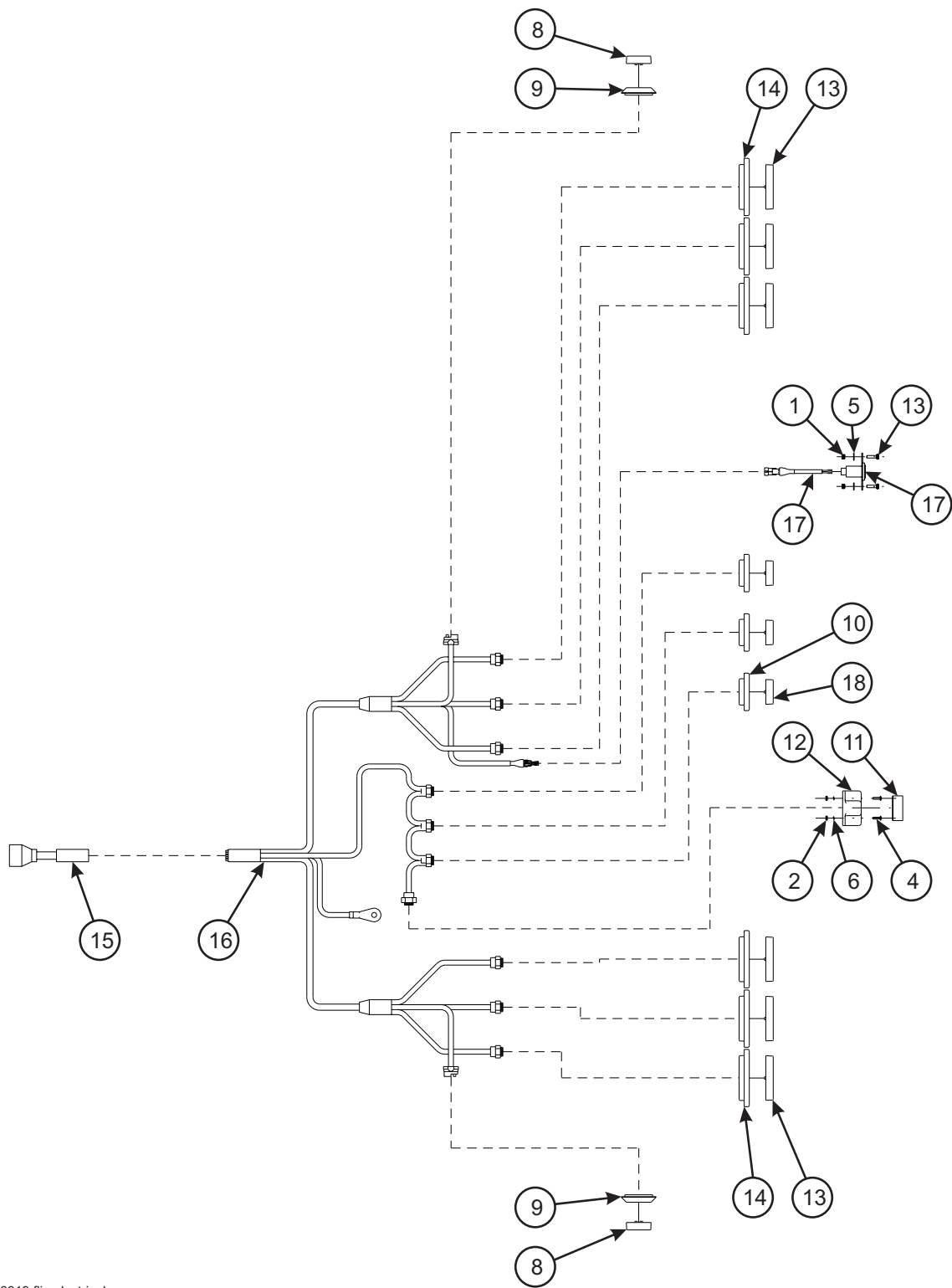
Figure 1-32 Flip Axle Electrical System (835B)
