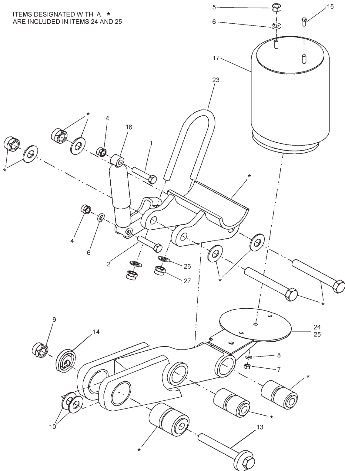
Figure 1-22 Suspension Fastener, AR-80-9 FMT
