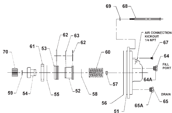
DRUM INSTALLATION
