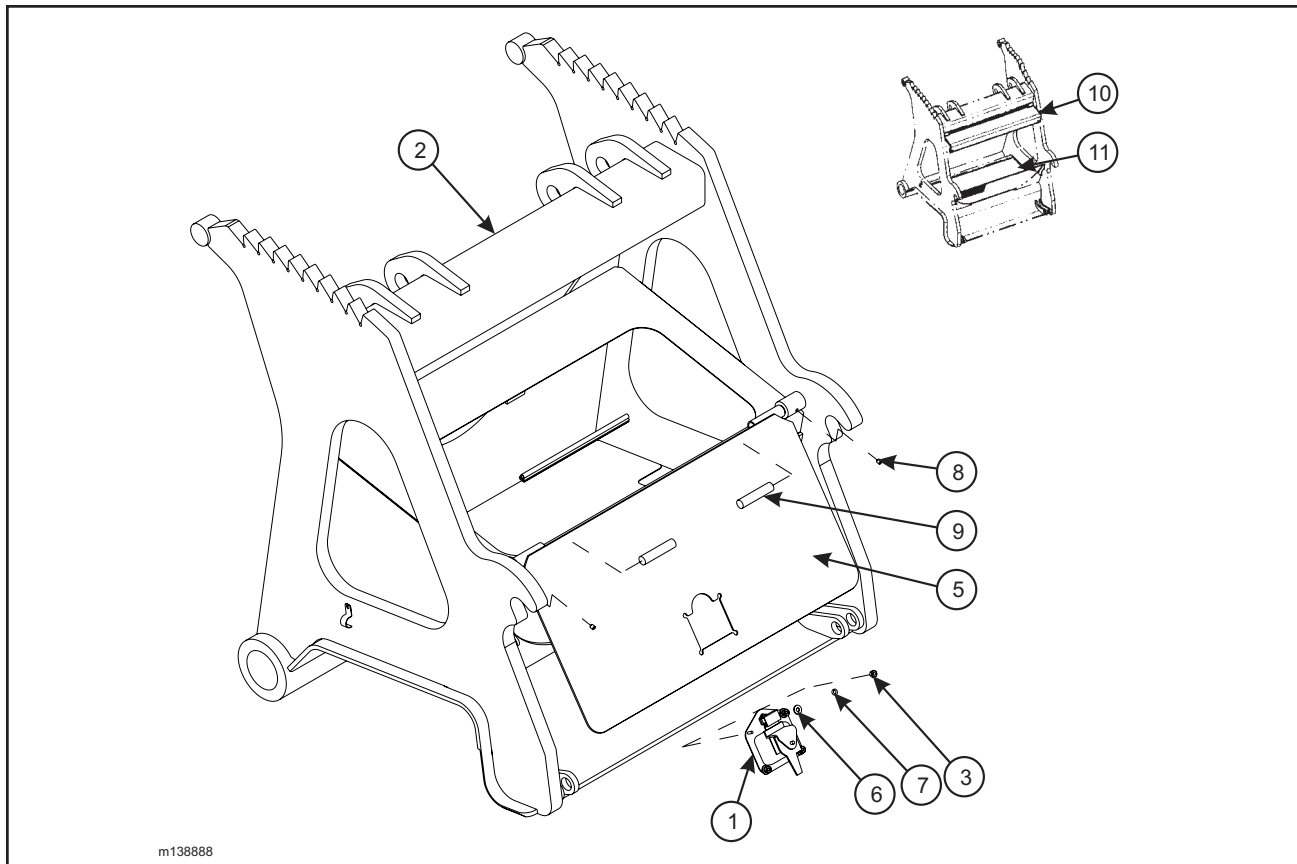
Figure 1-72 Toolbox Assembly (Option)
