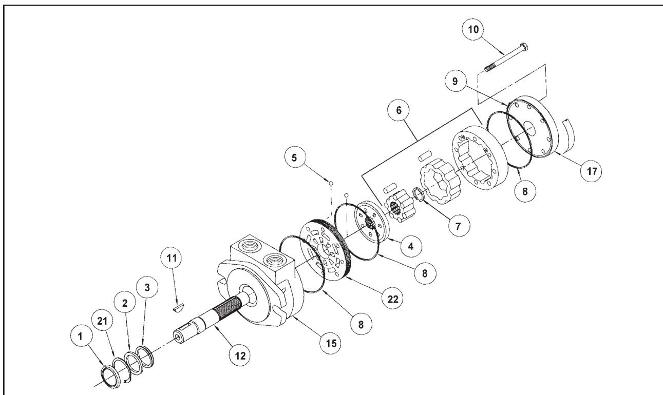
Figure 1-49 Winch Motor Assembly
