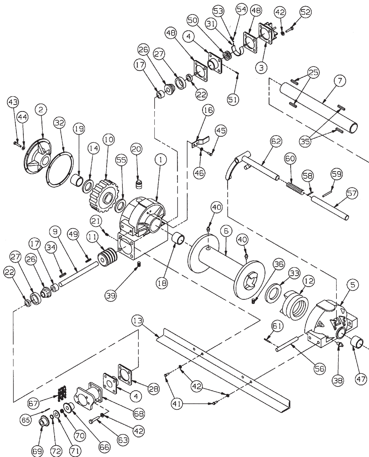
Figure 1-47 12,000# Winch Assembly
