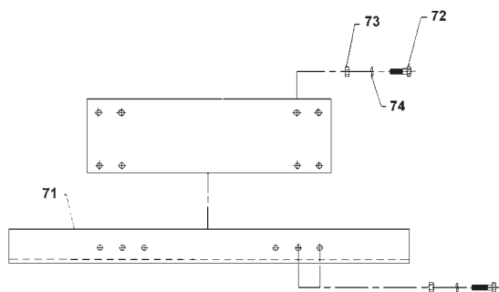
AIR/HYDRAULIC KICKOUT GEAR END COVER INSTALLATION
