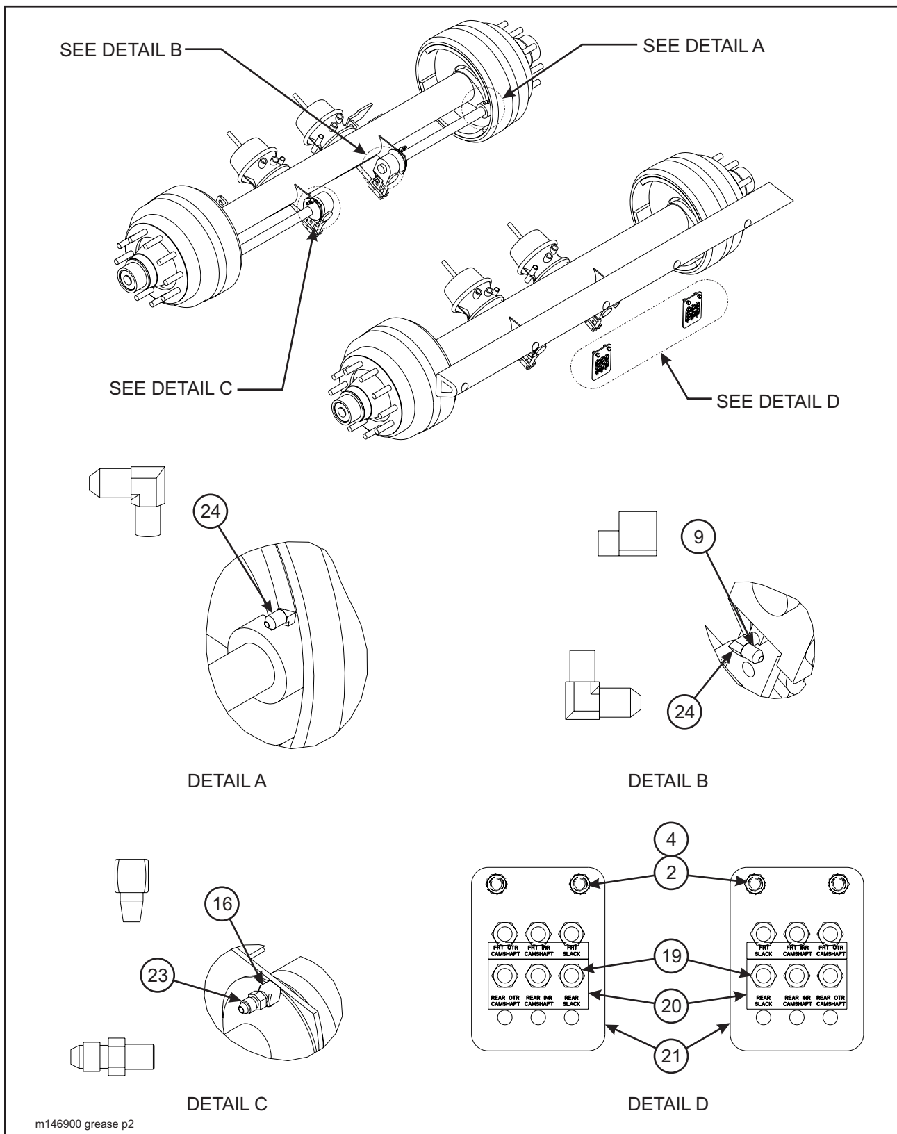
Figure 1-10 Frame Assembly and Grease System (825B) (3 of 3)
