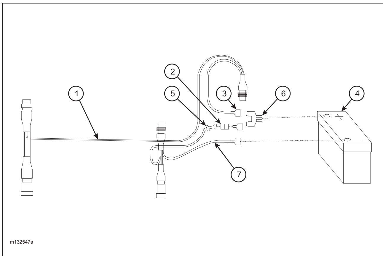
Figure 1-75 Battery Backup, Bumper Strobe Light (Option)
