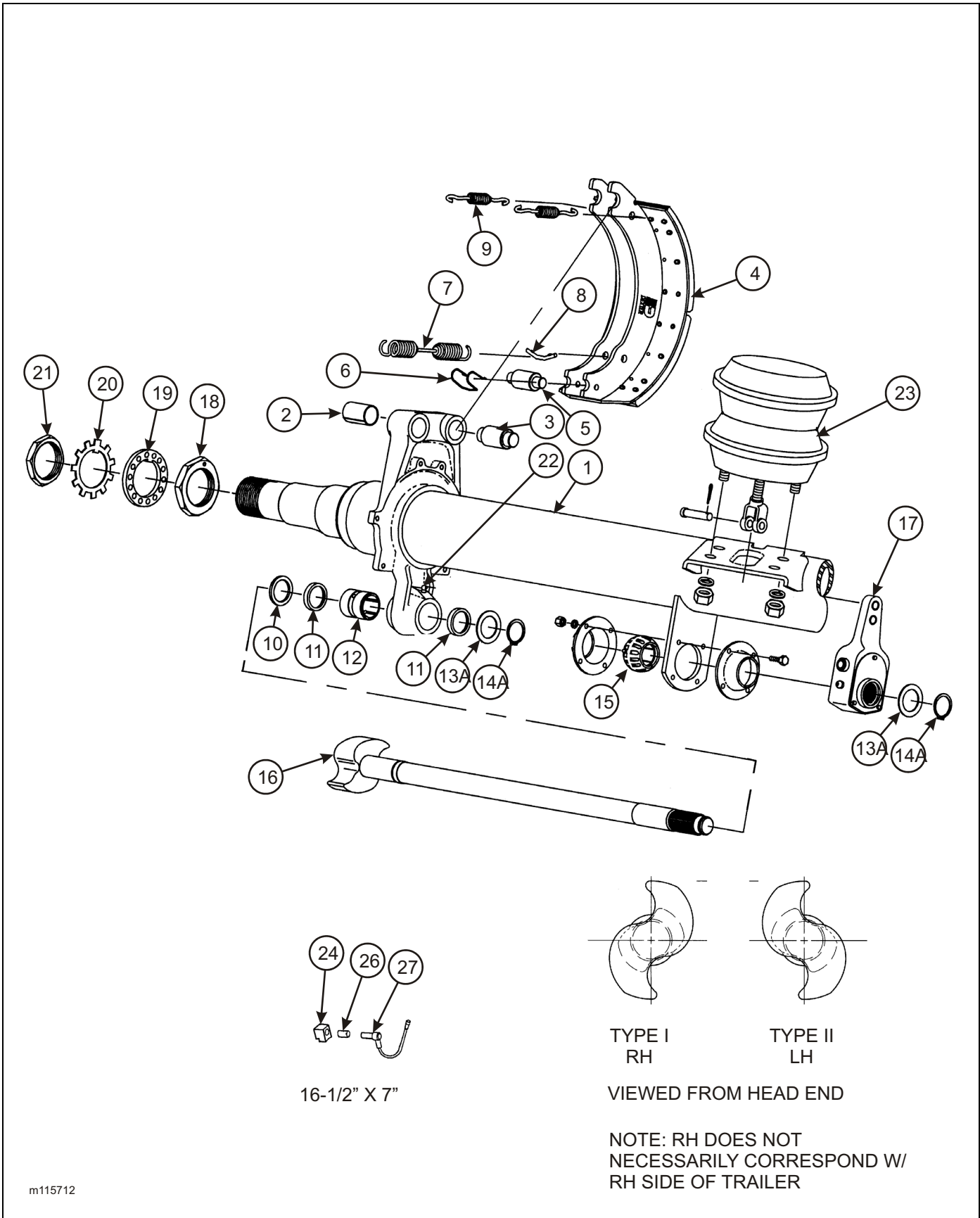
Figure 1-25 Axle and Brake Assembly
