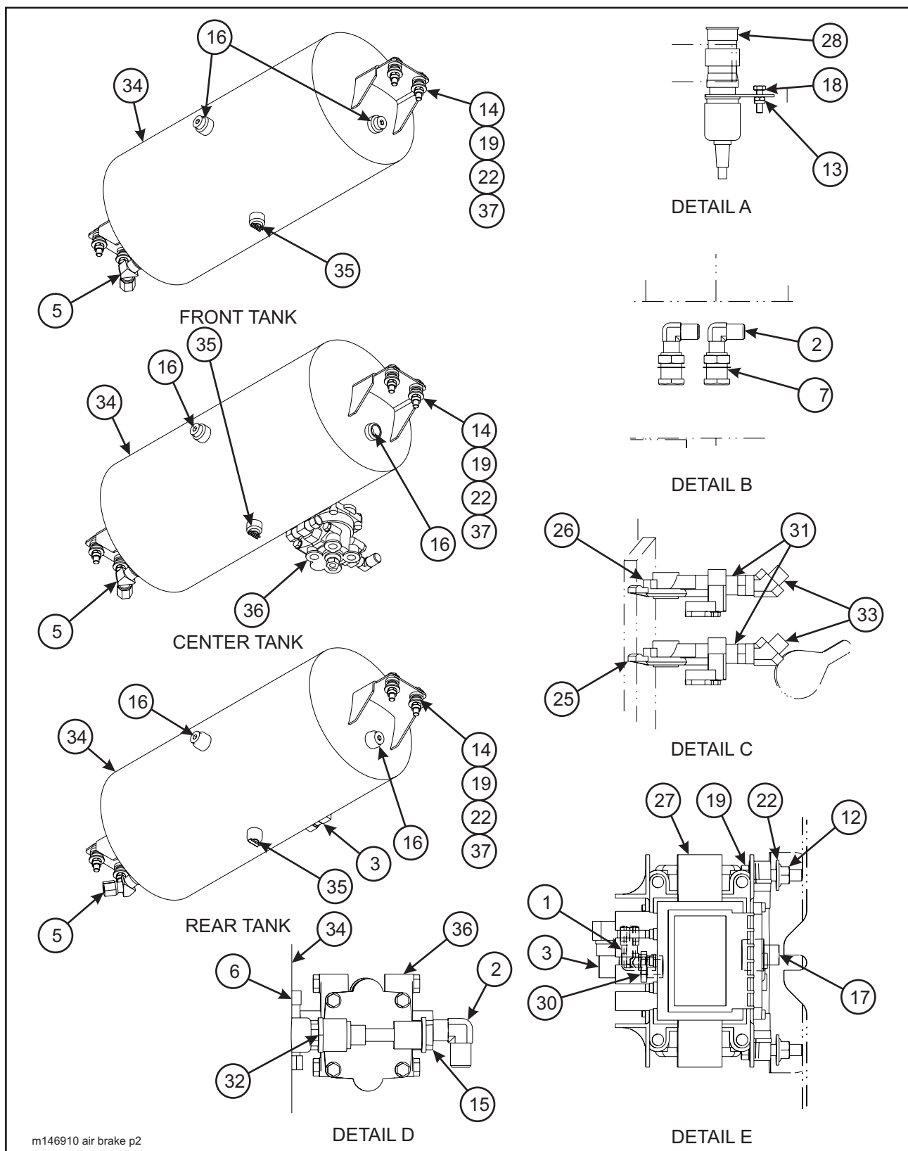
Figure 1-41 Air Brake System (835B Triple Axle)
