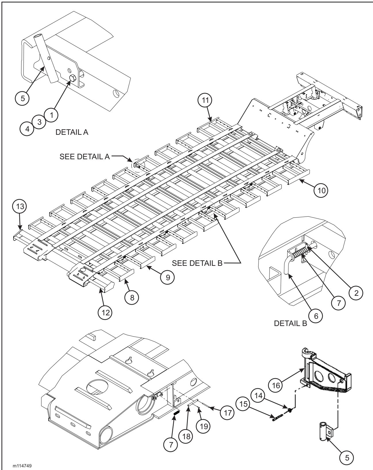
Figure 1-7 Pull and Swing Out Installations
