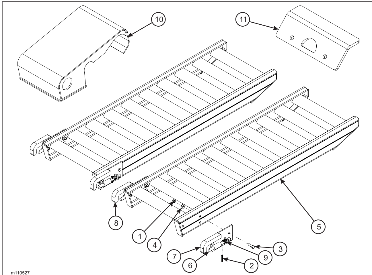
Figure 1-65 Aluminum Beavertail Ramp Assembly (Option)
