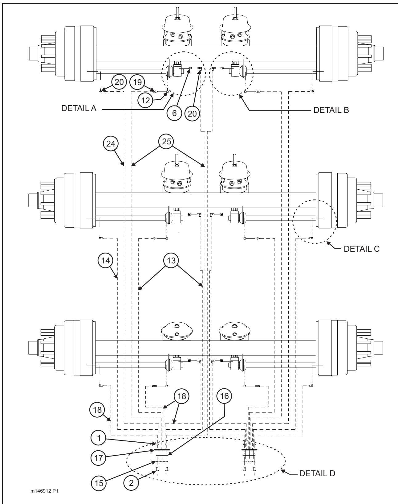
Figure 1-14 Frame Assembly and Grease System (835B - Triple) (4 of 5)
