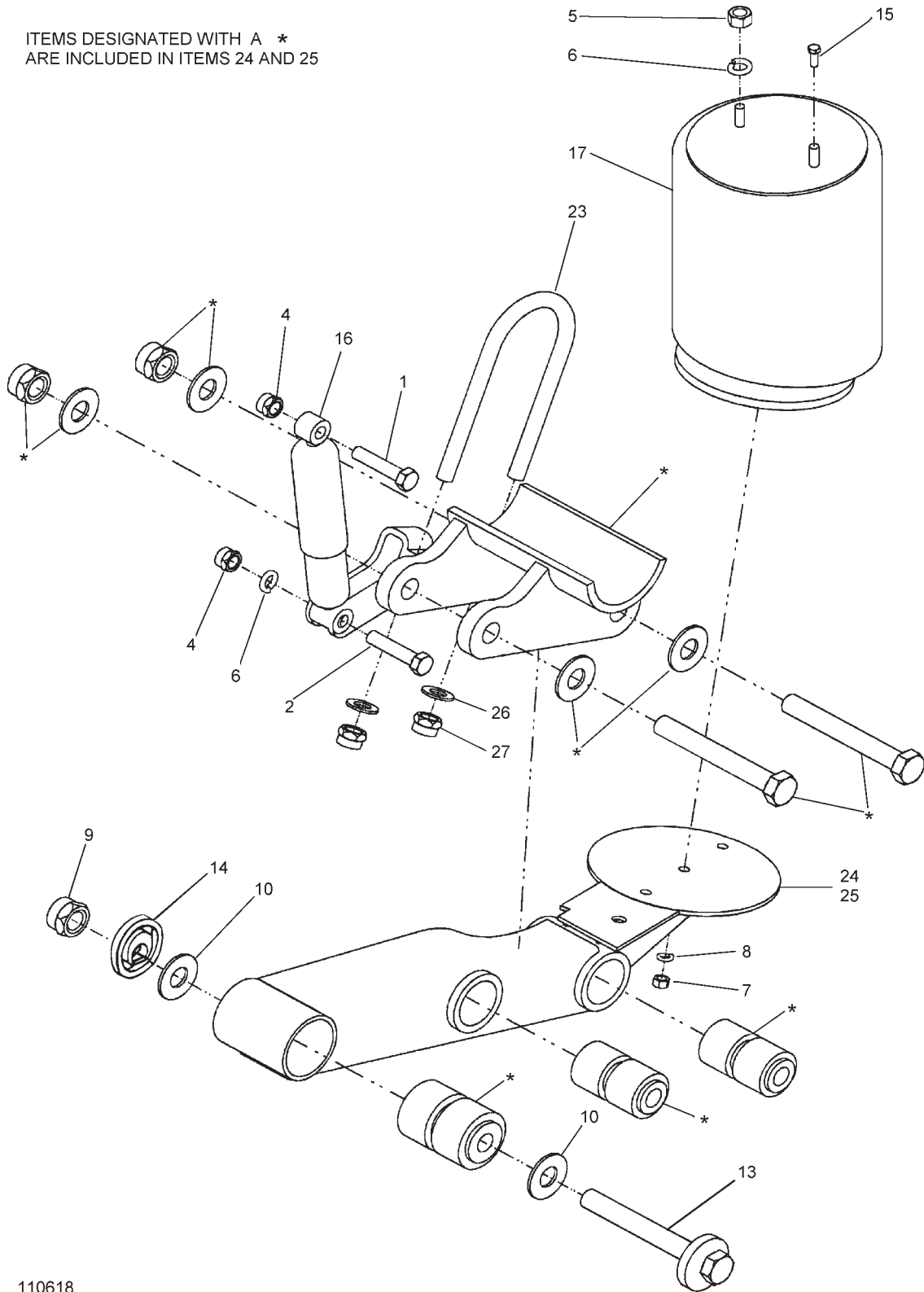
Figure 1-21 Suspension, Fastener RLU-250-9-4
