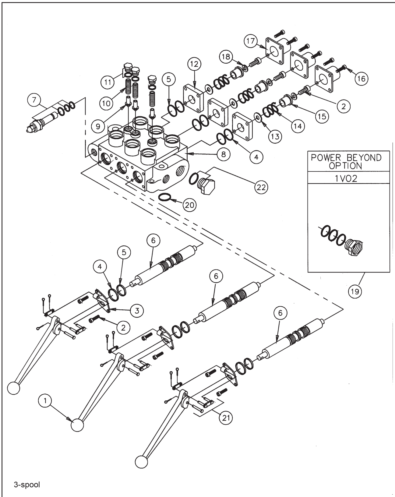
Figure 1-29 Three Spool Valve
