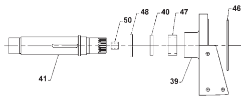
INPUT SHAFT INSTALLATION
