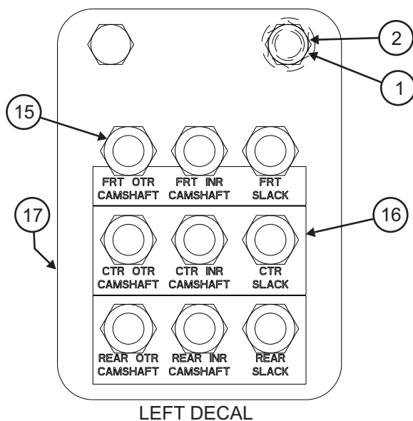
DETAIL D
