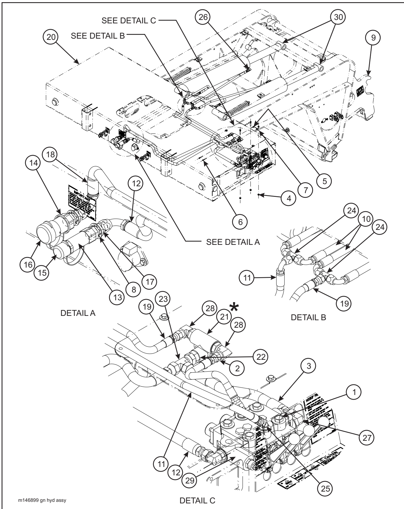
Figure 1-26 Gooseneck Hydraulic System (825B)
