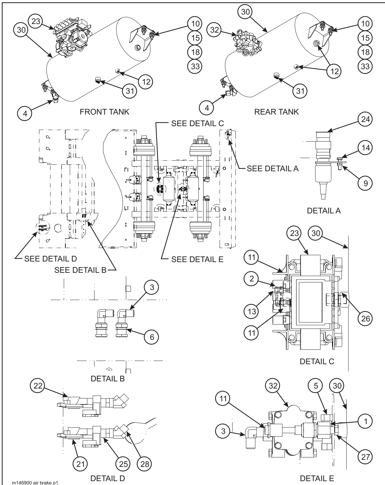
Figure 1-33 Air Brake System (825B)
