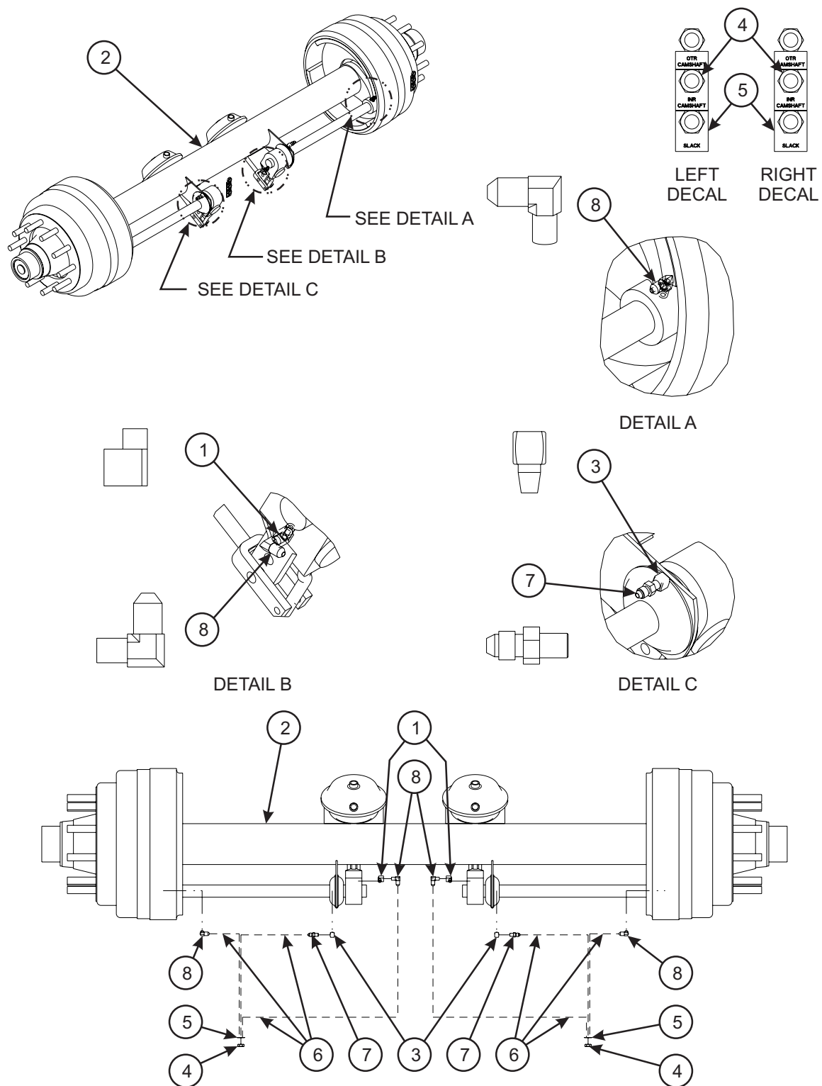
Figure 1-20 Flip Assembly - Air Ride Suspension
