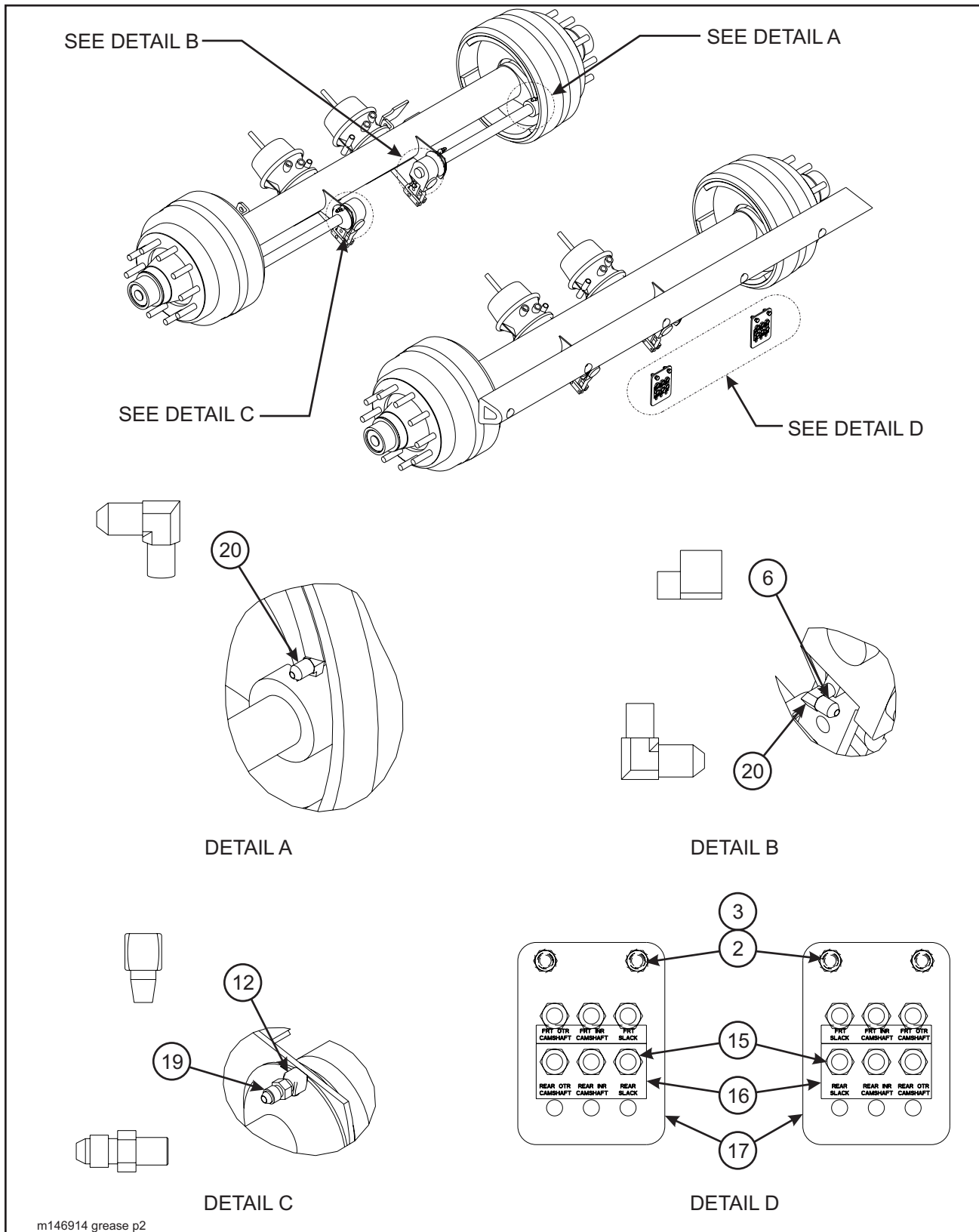
Figure 1-13 Frame Assembly and Grease System (835B - Tandem) (3 of 5)
