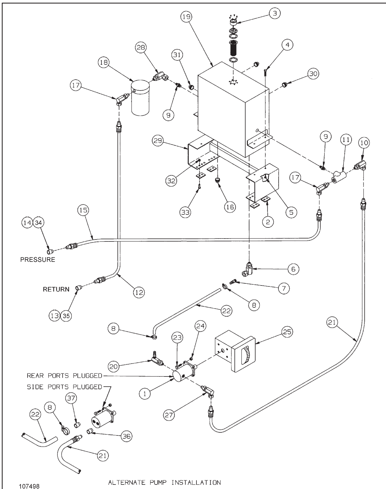
Figure 1-61 Hydraulic Wet Kit Assembly (Option)
