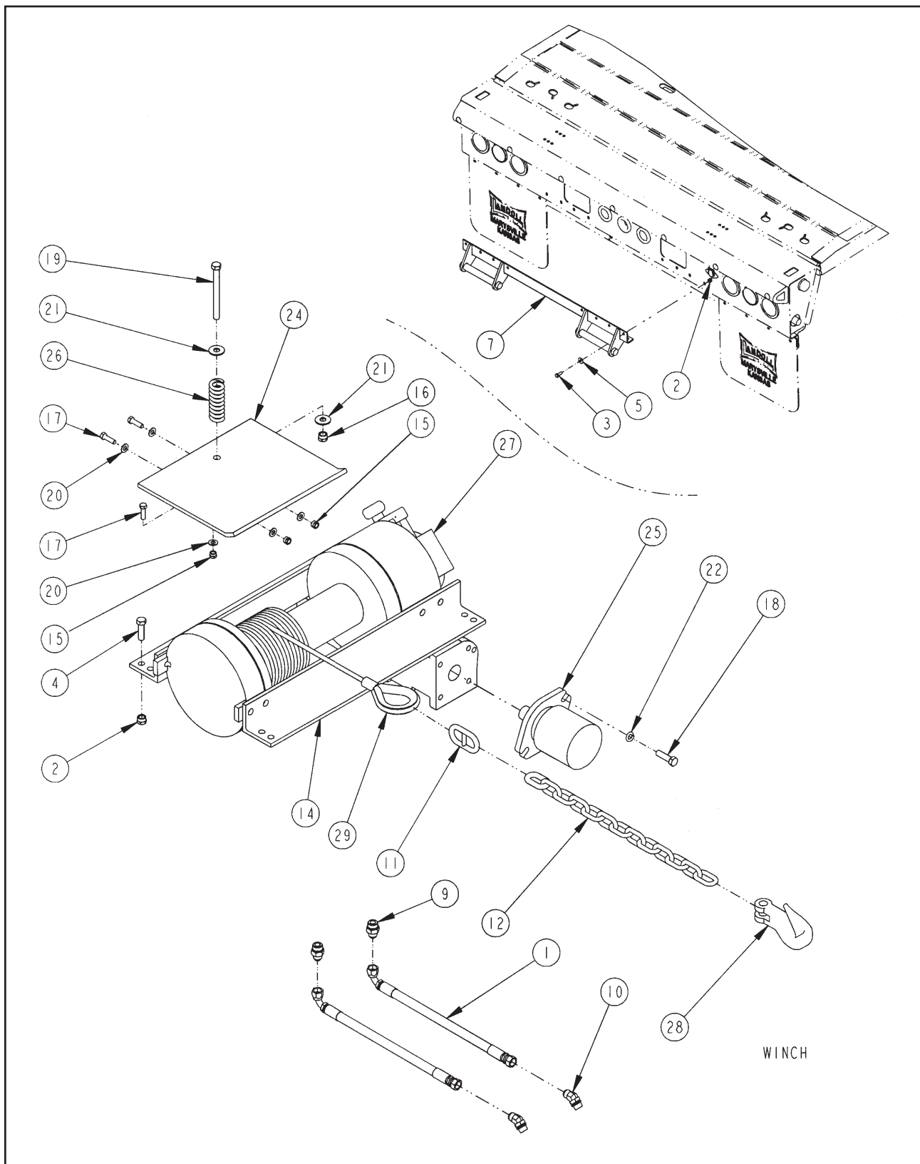
Figure 1-46 Winch Installation
