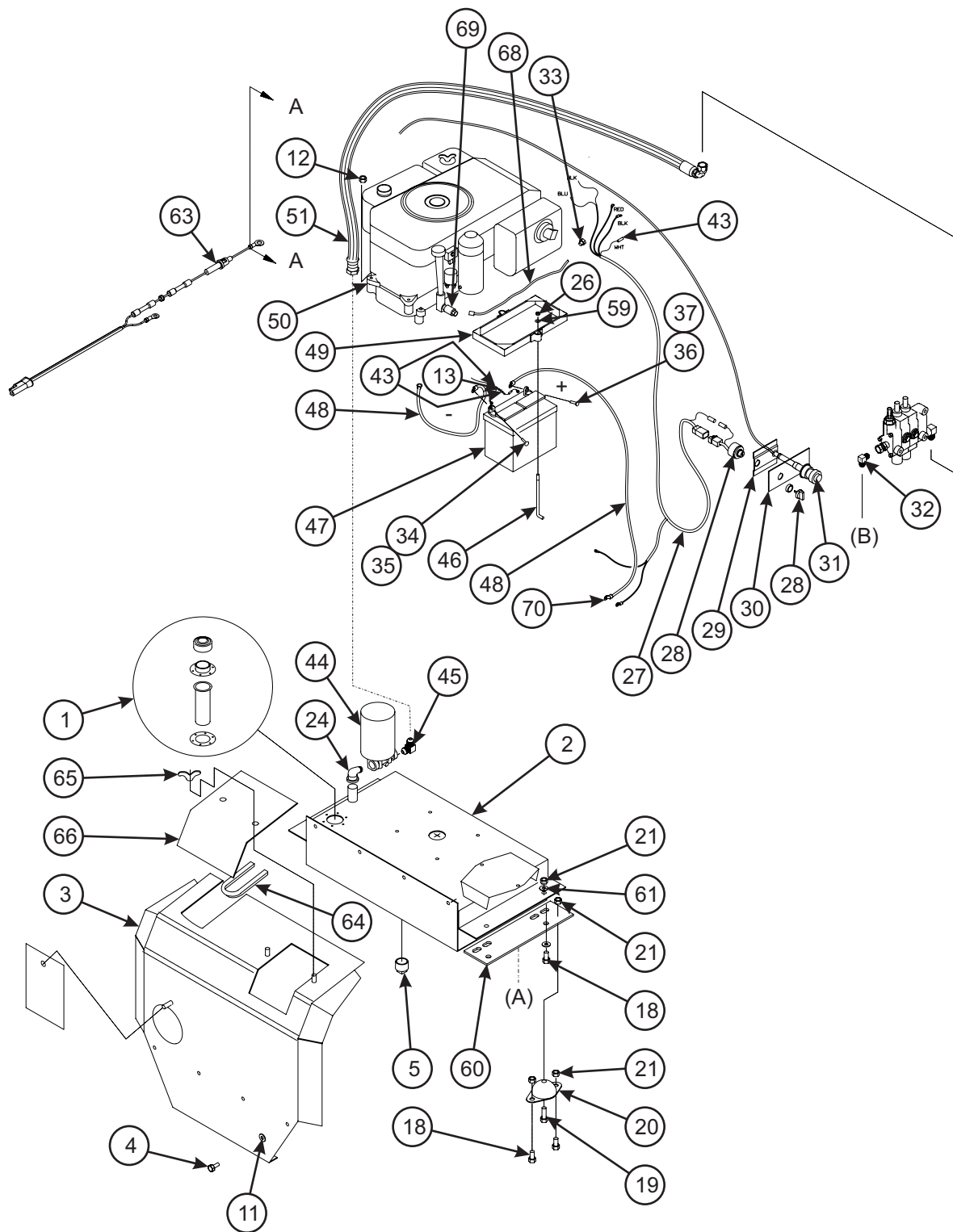
Figure 1-58 42-11 HP Honda Engine Drive Installation (Option) (1 of 2)
