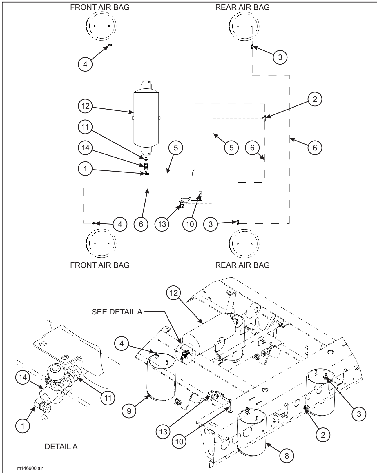
Figure 1-17 Frame Assembly - Air Ride Suspension (825B)
