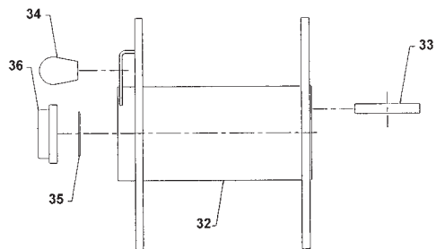
DRUM INSTALLATION
