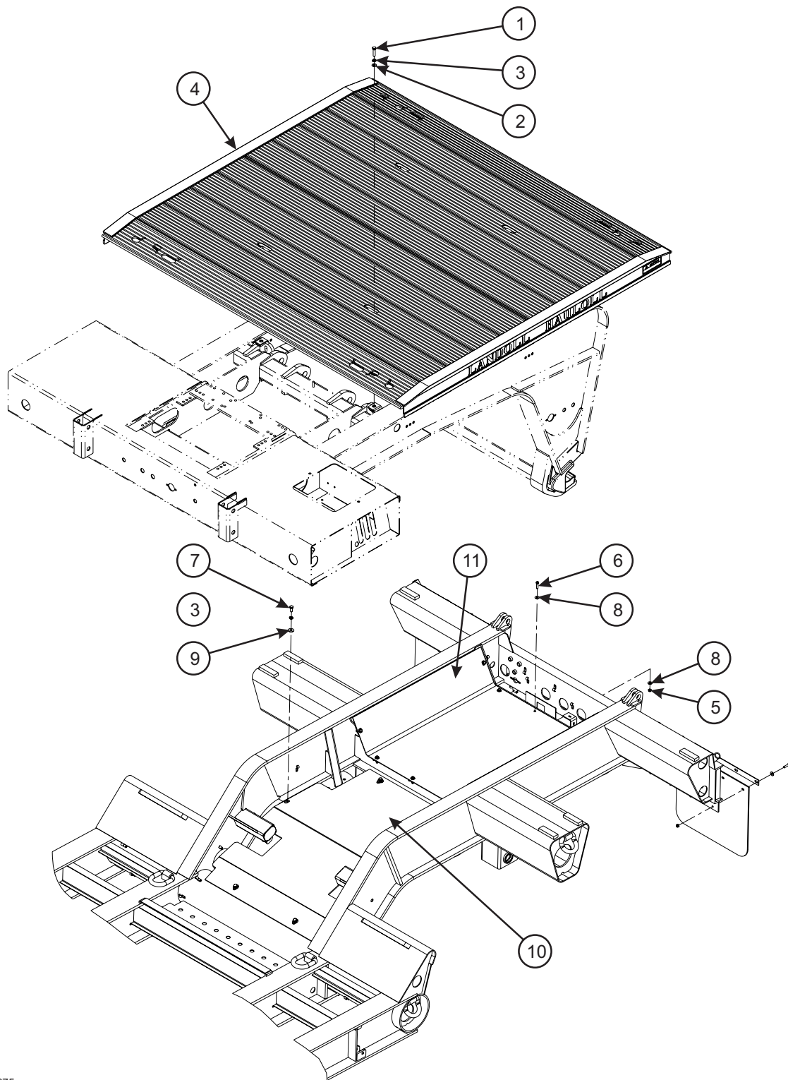
Figure 1-5 Bed Installation (Trunnion and Gooseneck)
