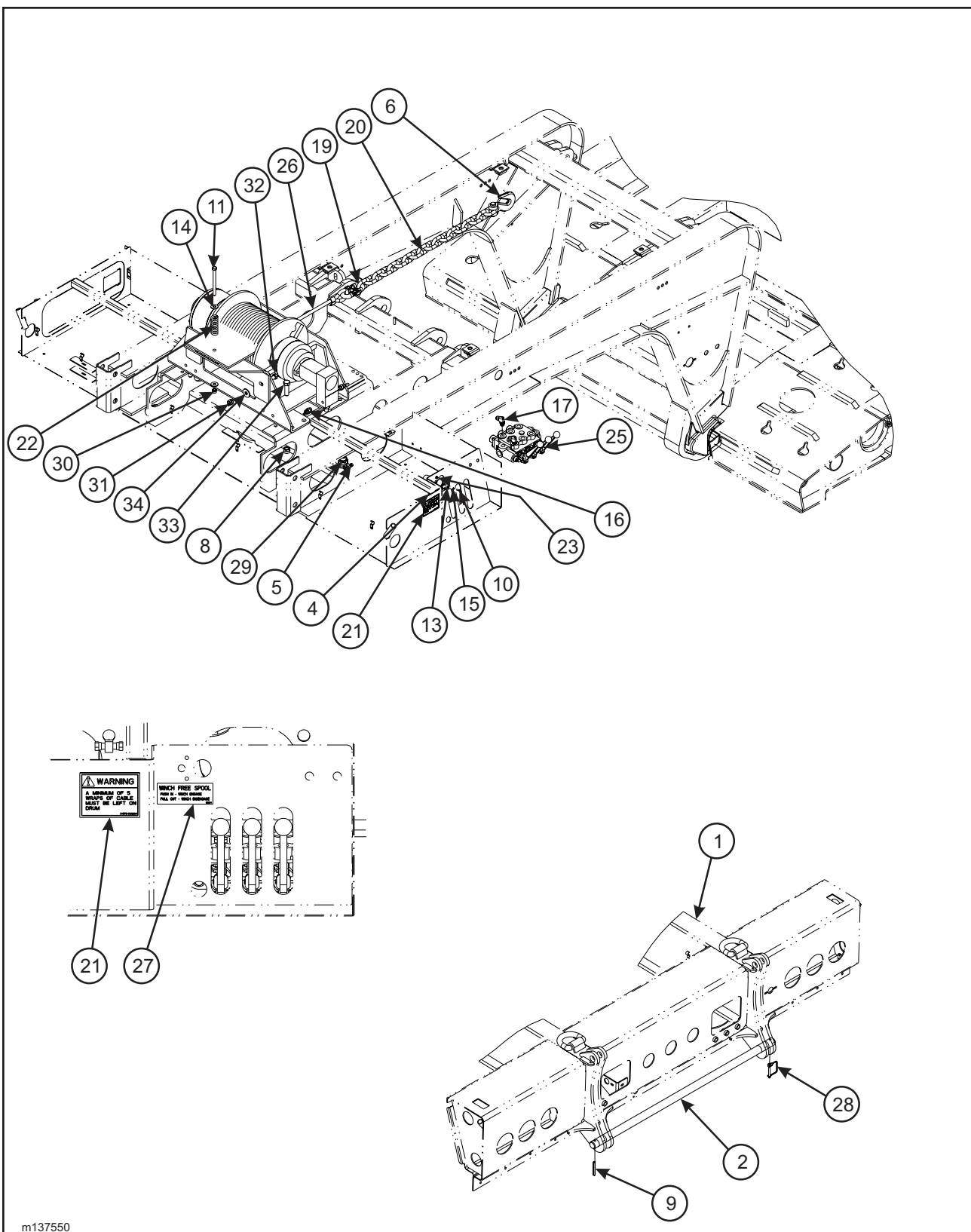
Figure 1-52 30K DP Winch Installation
