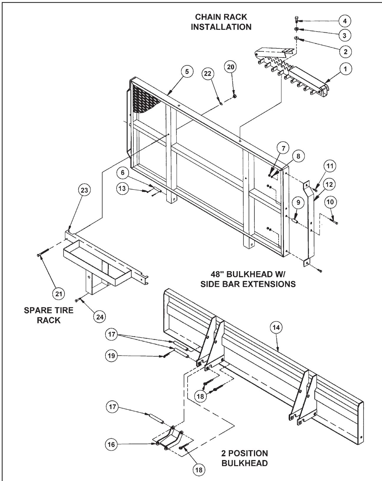
Figure 1-64 Bulkhead and Chain Rack Installation (Option)
