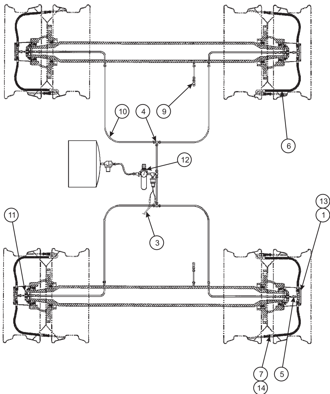
Figure 1-78 Tire Inflation System (Option)
