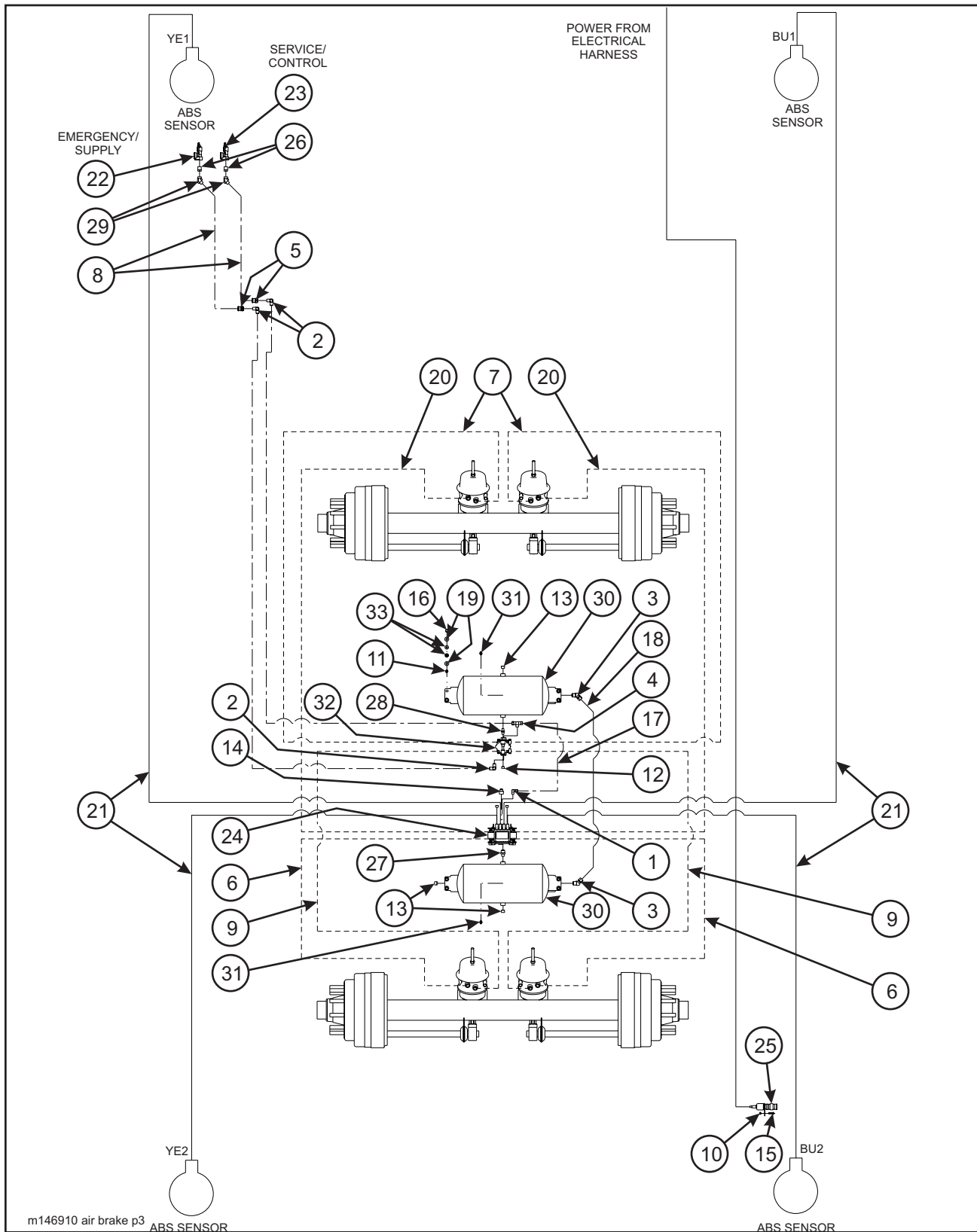
Figure 1-39 Air Brake System (835B Spread Axle)
