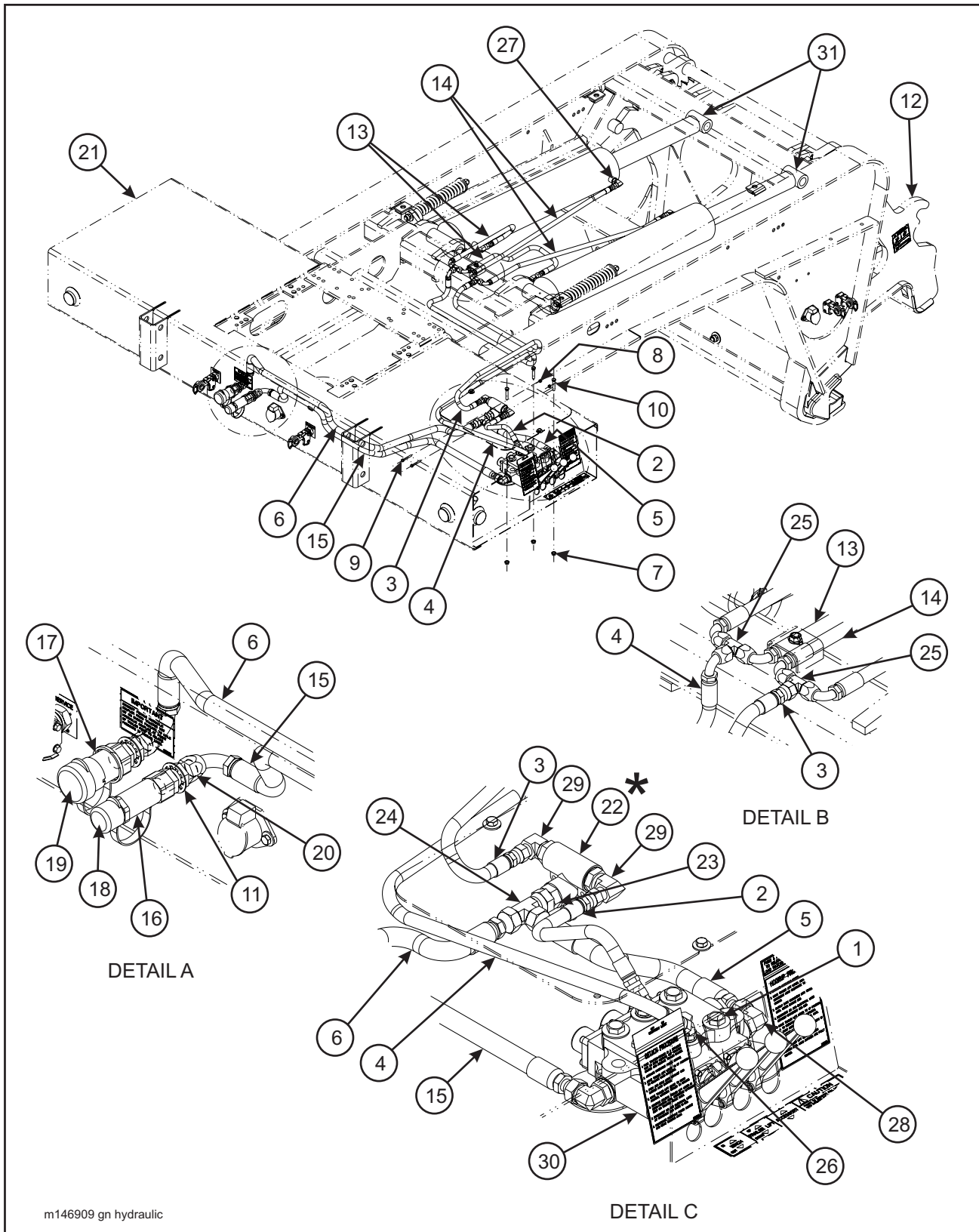
Figure 1-27 Gooseneck Hydraulic System (835B)
