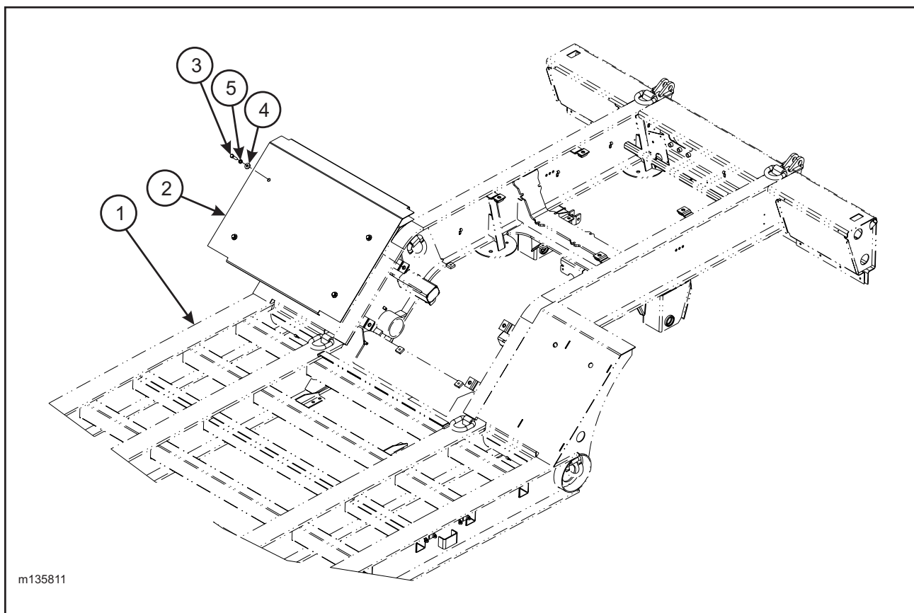
Figure 1-69 Slope Cover Assembly (Option)
