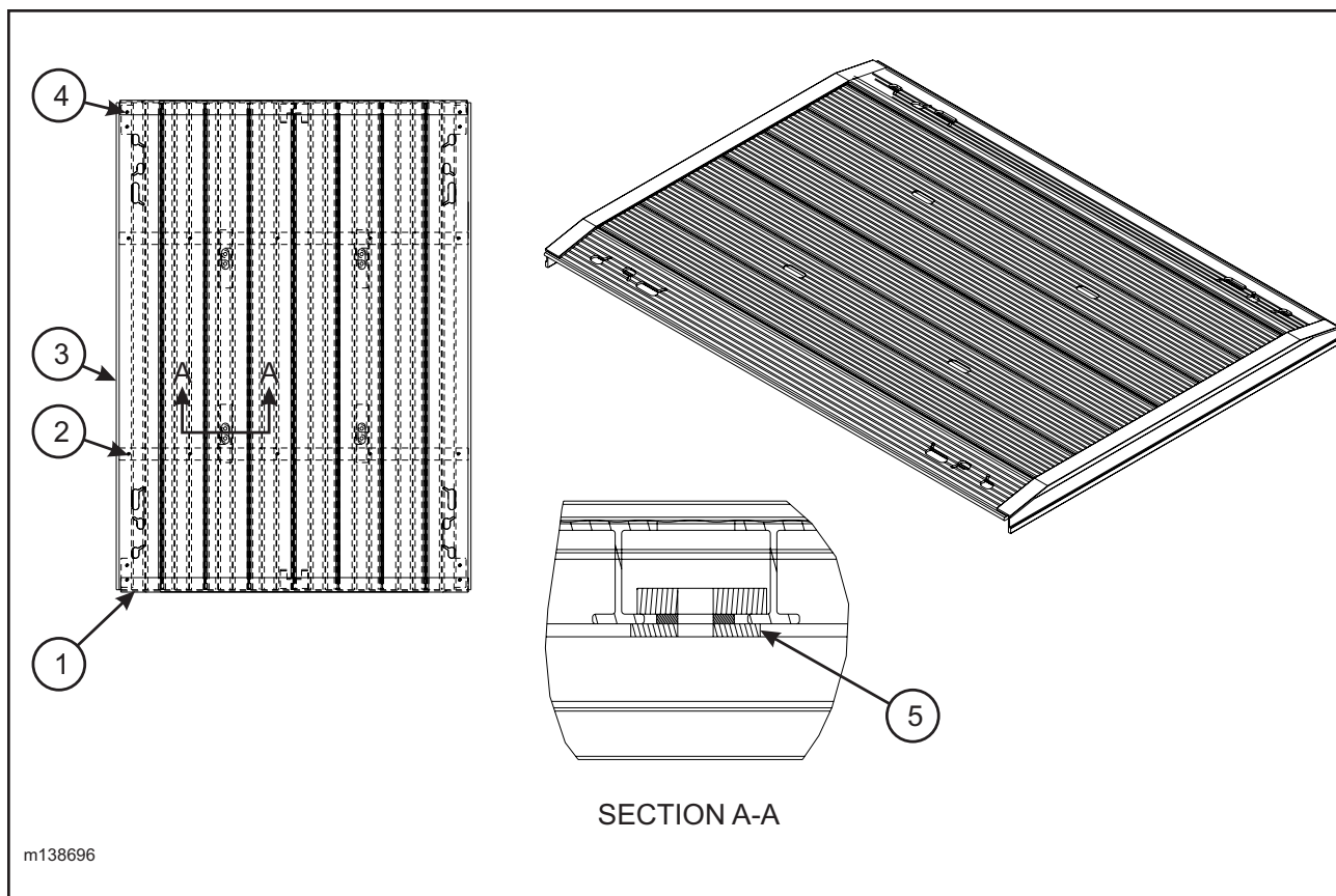
Figure 1-73 UHMW Under Aluminum Deck (Option)
