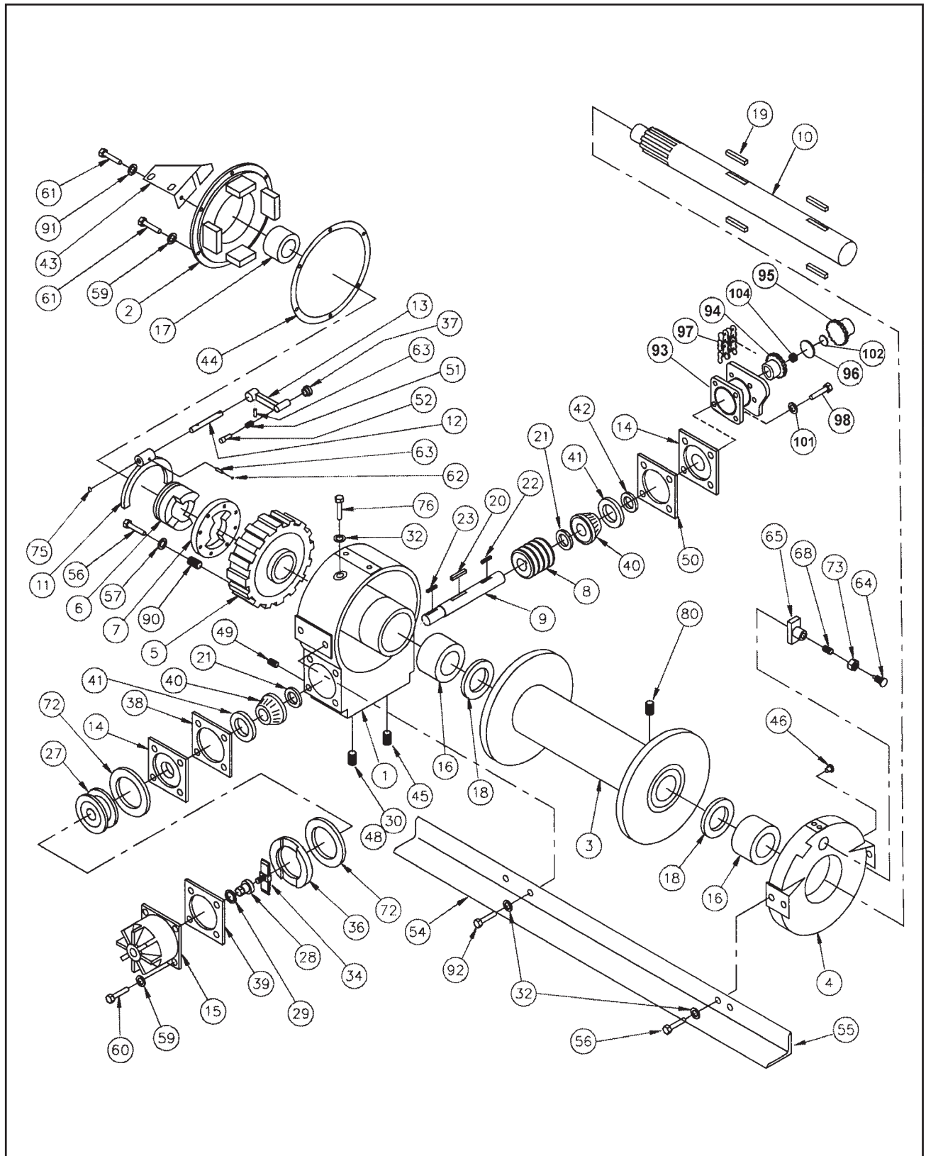
Figure 1-48 20,000# Winch Assembly
