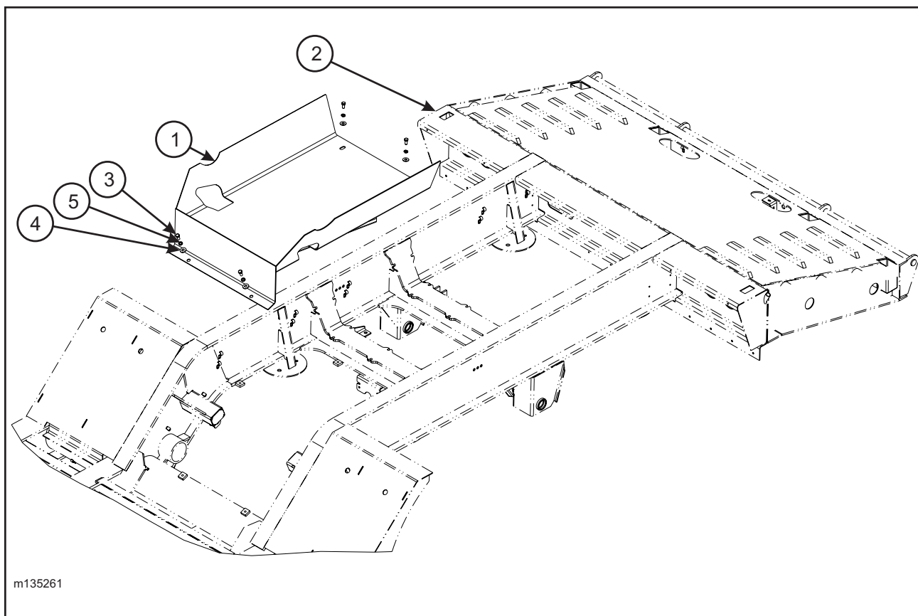
Figure 1-70 Tray Assembly (Option)
