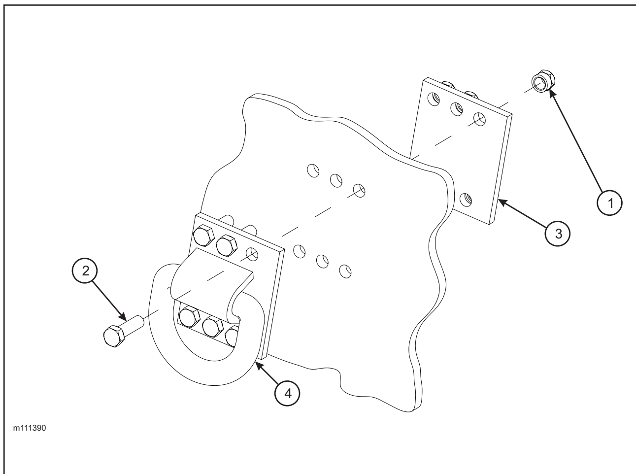
Figure 1-50 Bolt-On D-Ring Assembly (Option)
