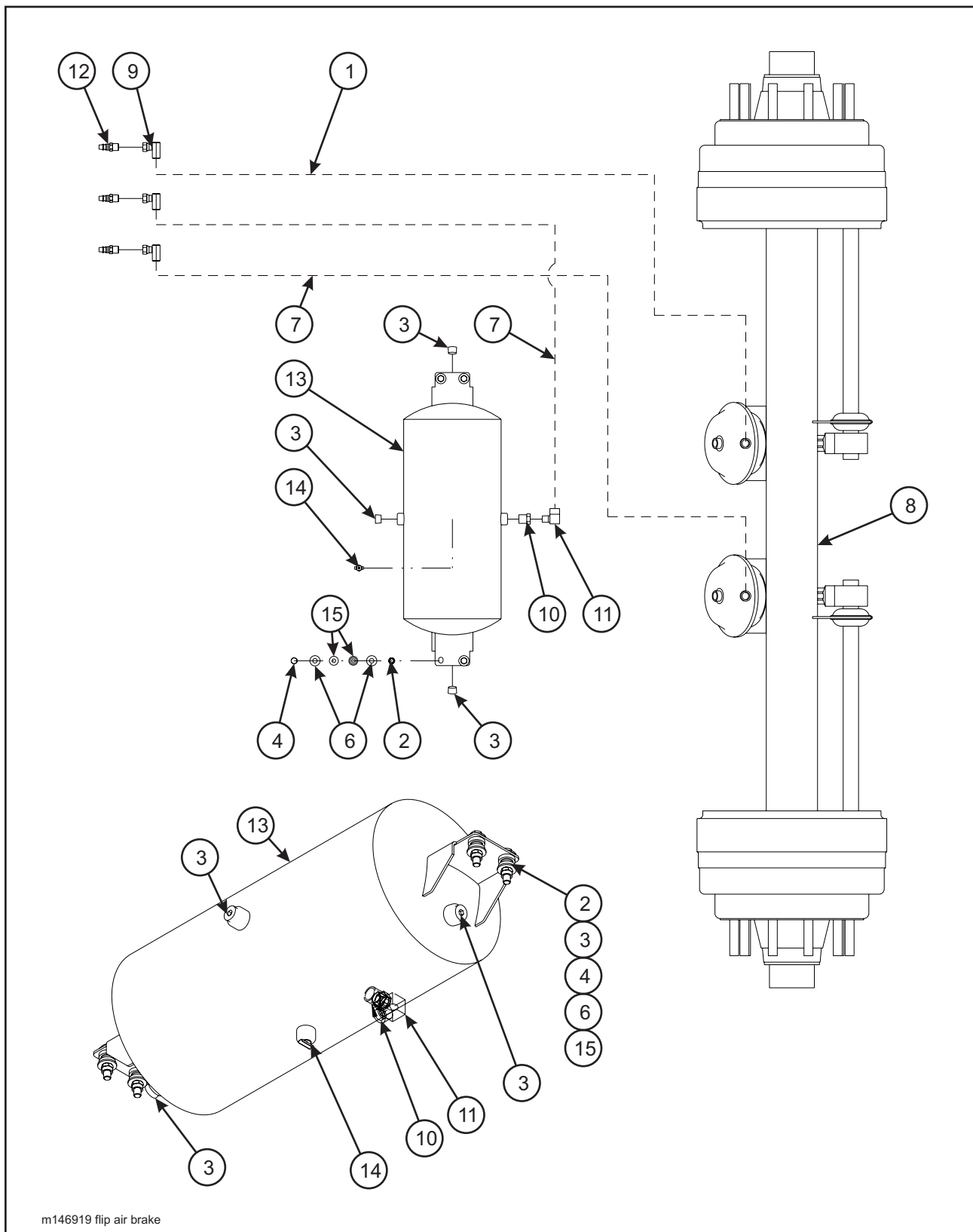
Figure 1-43 Air Brake System - Flip Axle (835B)
