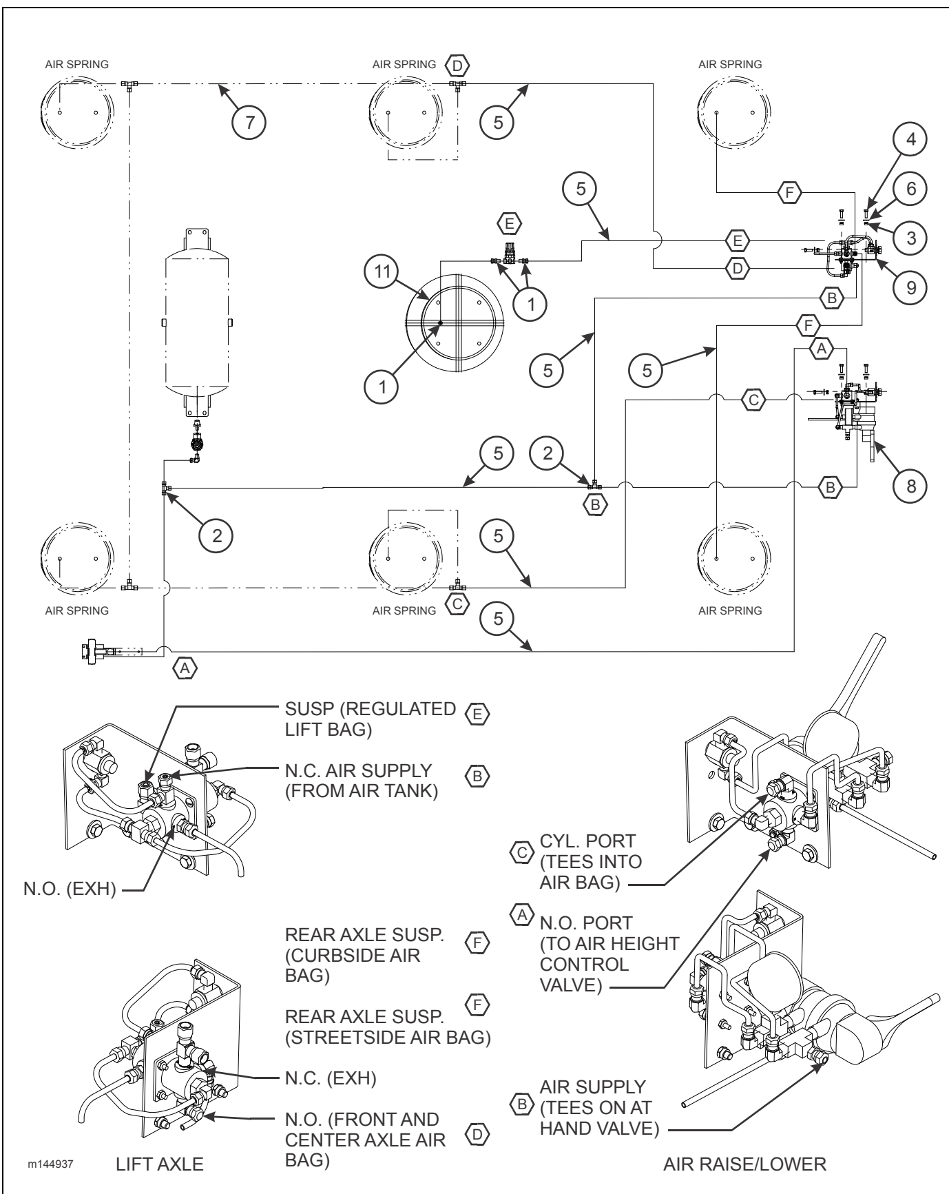
Figure 2-105: Lift Control Installation, 3rd R/L (Option)
