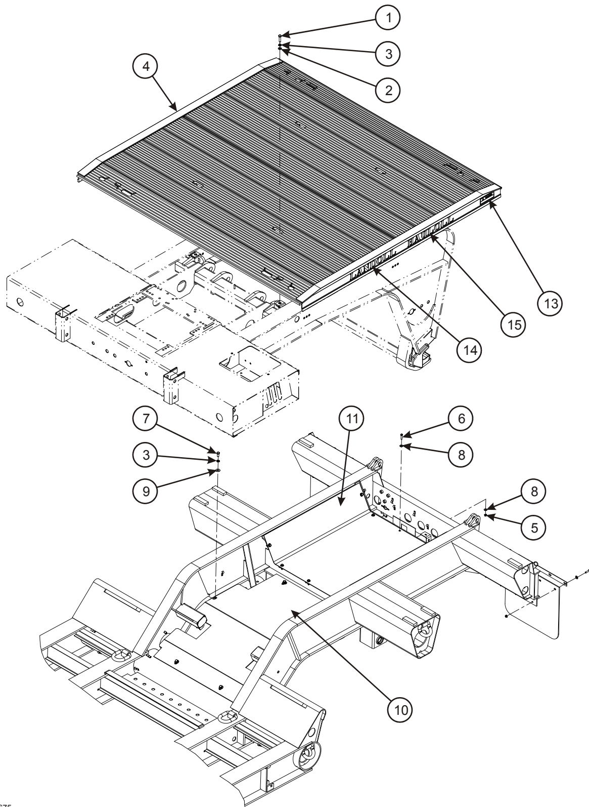
Figure 2-67: Bed Installation (Trunnion and Gooseneck)
