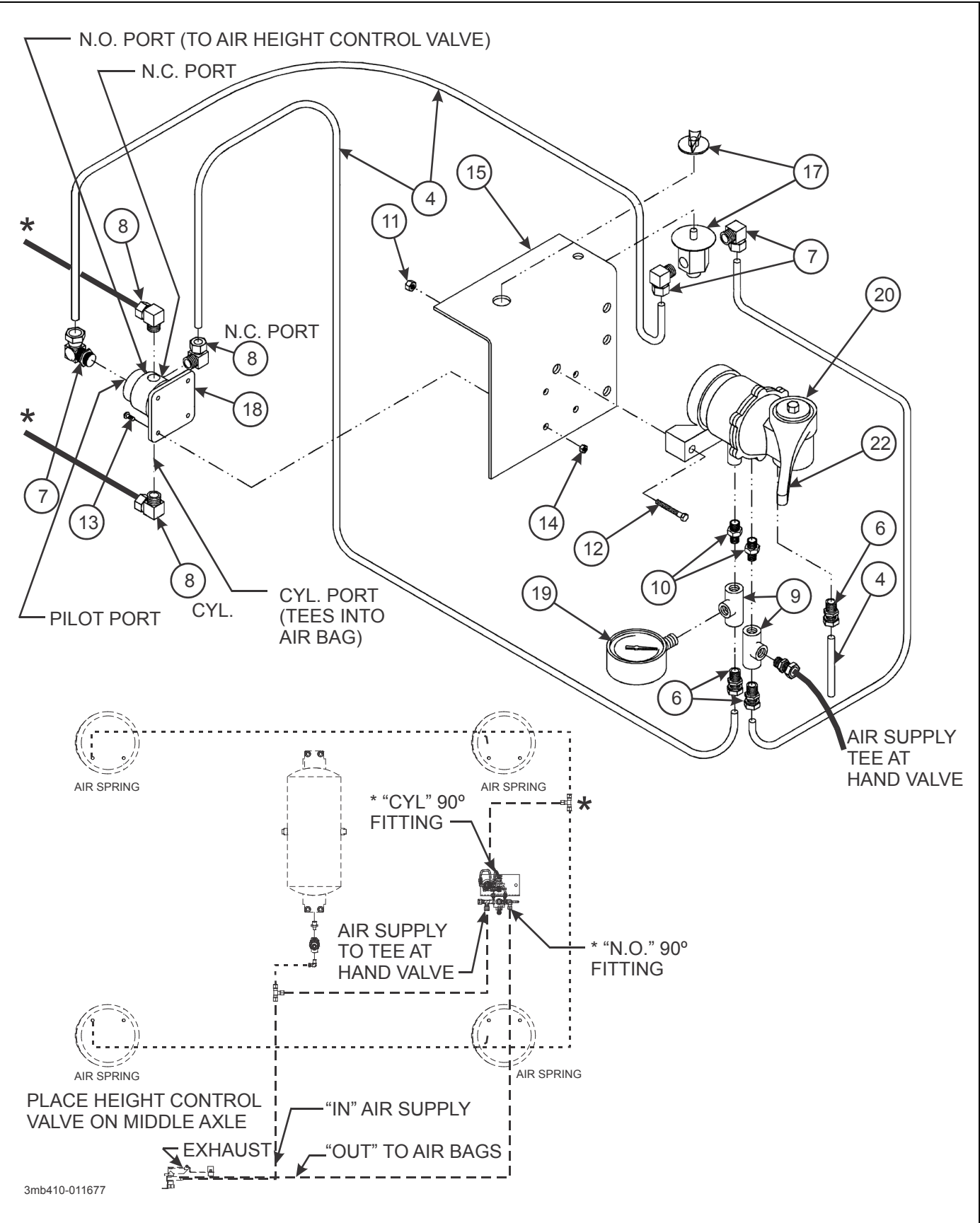
Figure 2-51: Manual Air Height Control Assembly (Option)
