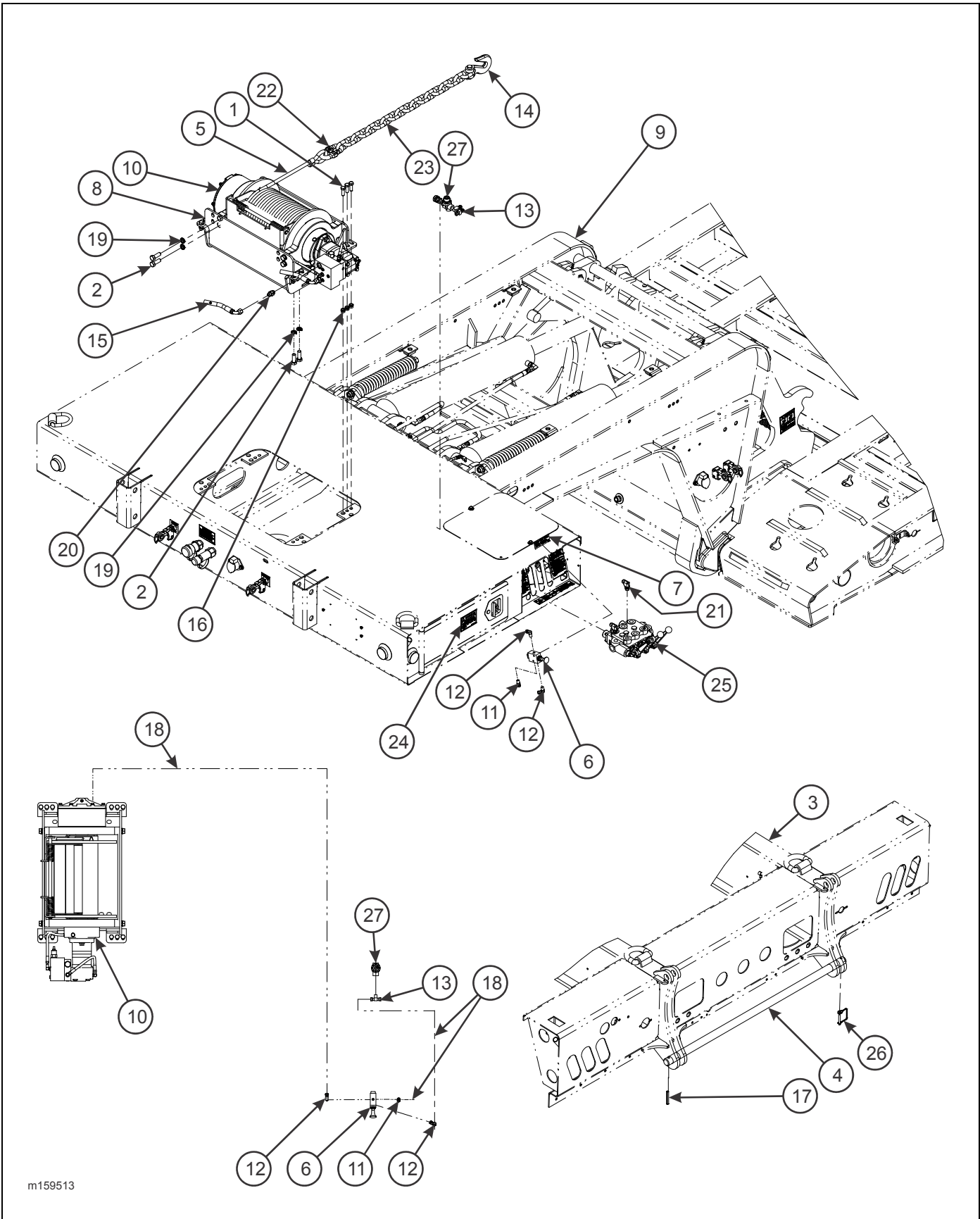
Figure 2-88: 30,000 Lb. Winch Installation (Warn)
