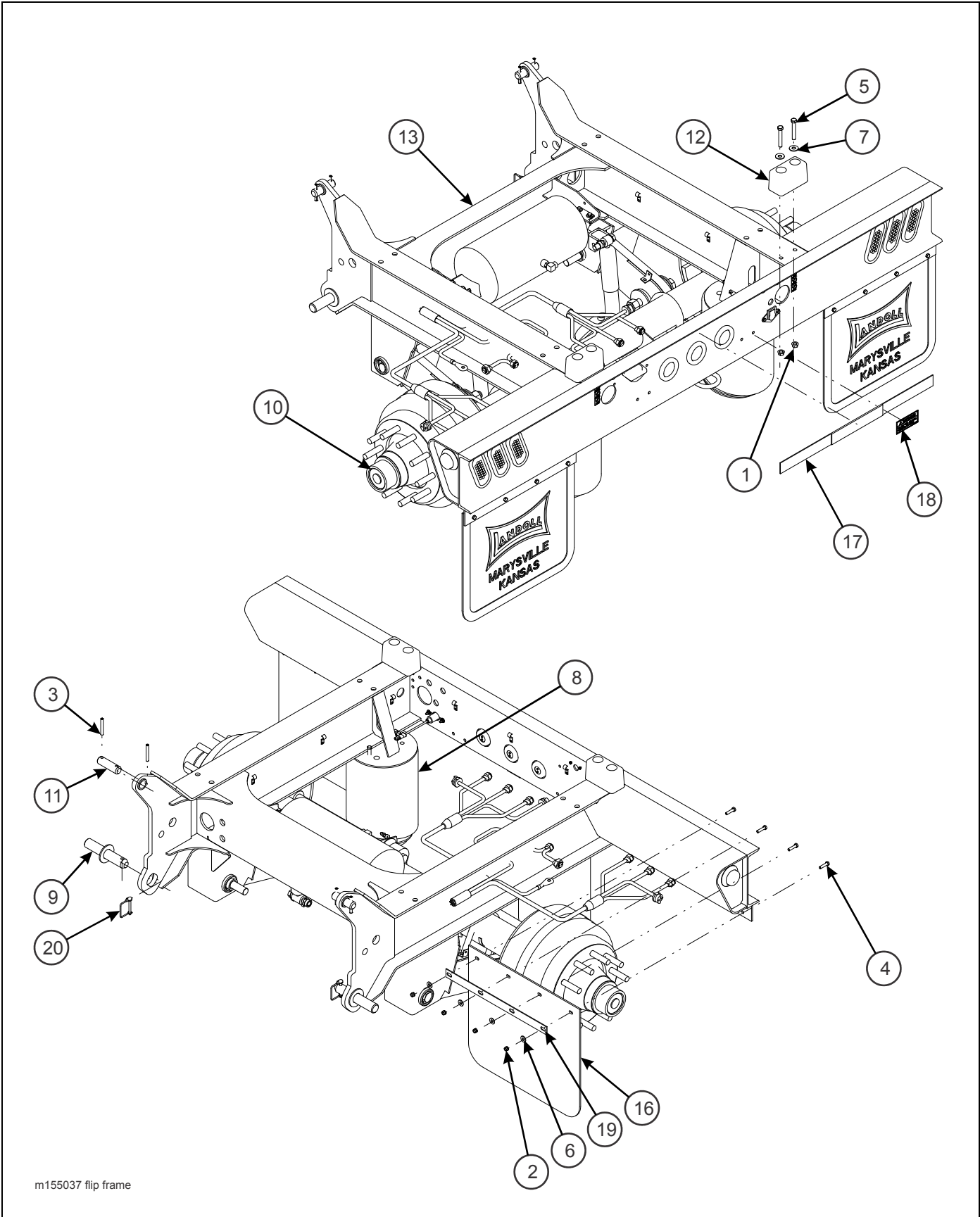
Figure 2-57: Flip Assembly - Frame
