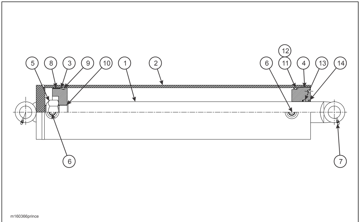
Figure 2-19: Cylinder, Hydraulic 7 x 34 (Prince)
