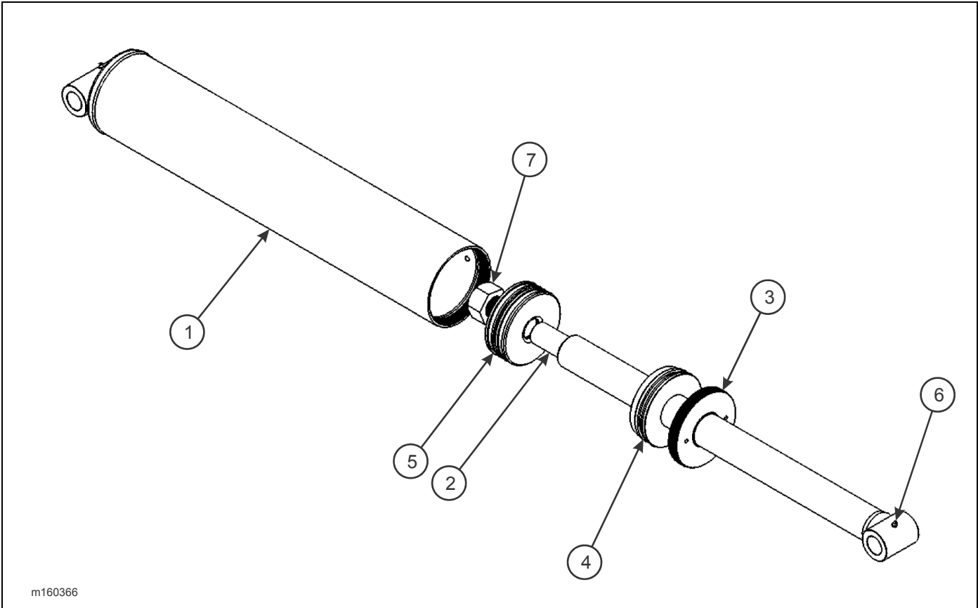
Figure 2-18: Cylinder, Hydraulic 7 x 34 (Carlson)
