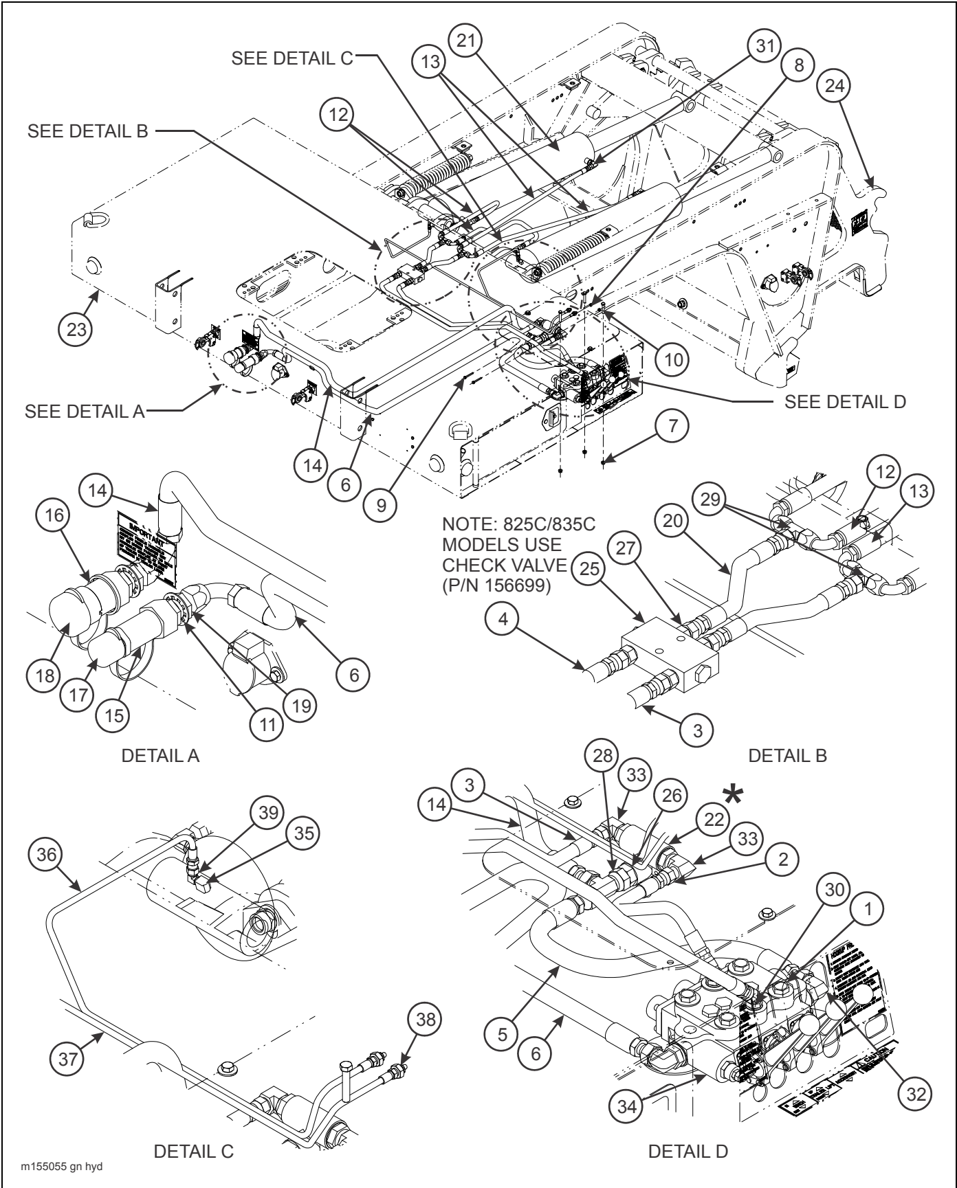
Figure 2-11: Gooseneck Hydraulic and Grease System (835C)
