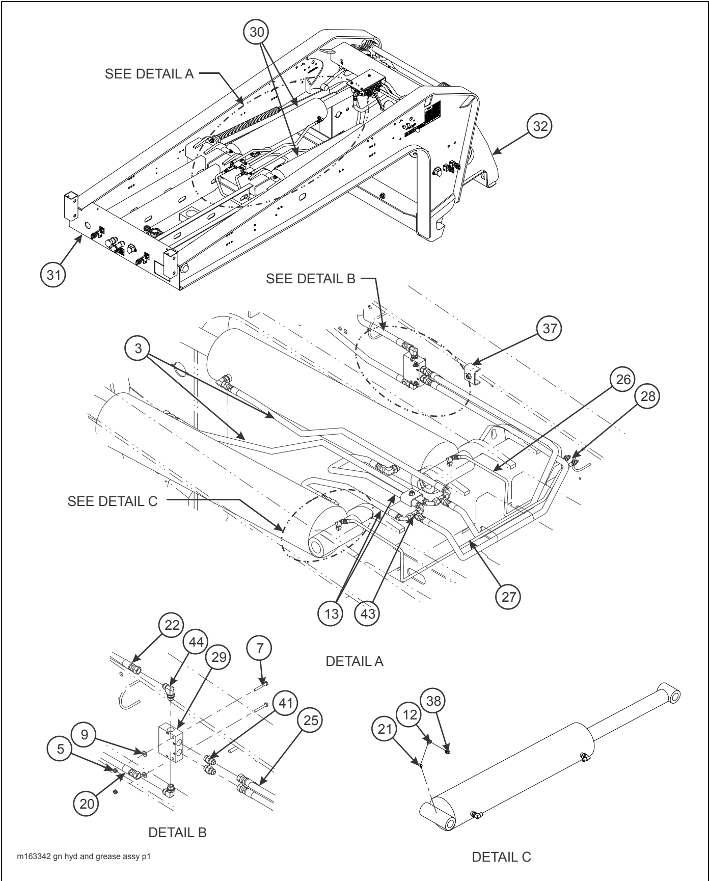
Figure 2-14: Gooseneck Hydraulic and Grease System (855C) (1 of 2)
