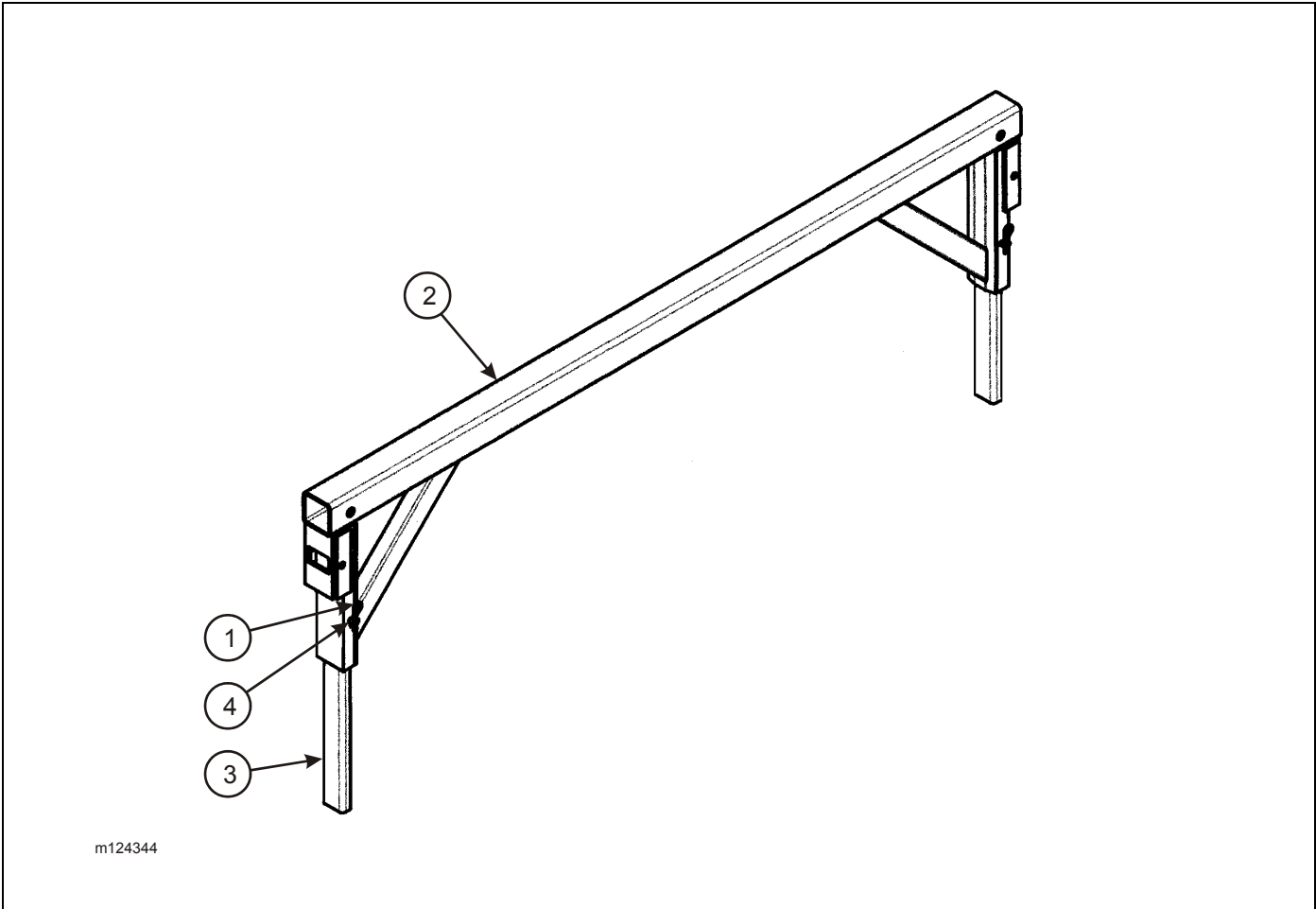
Figure 2-100: Header Rack Assembly, Adjustable Legs (Option)
