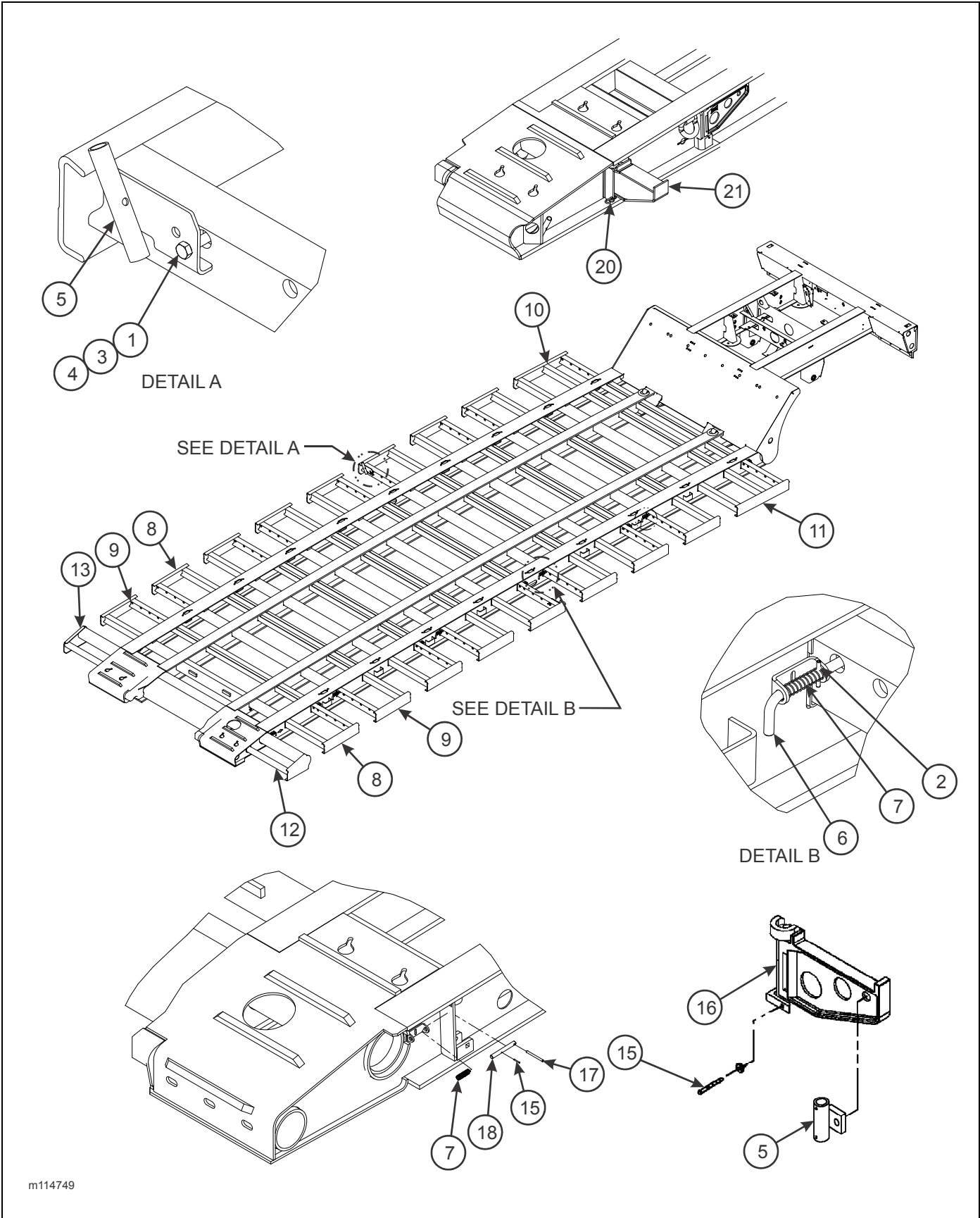
Figure 2-69: Pull and Swing Out Installation
