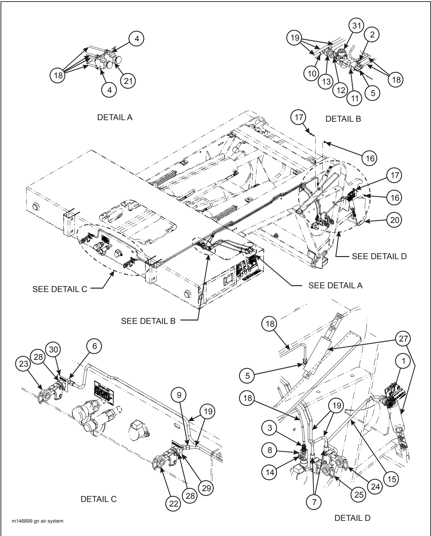
Figure 2-9: Gooseneck Air System (825C/835C)
