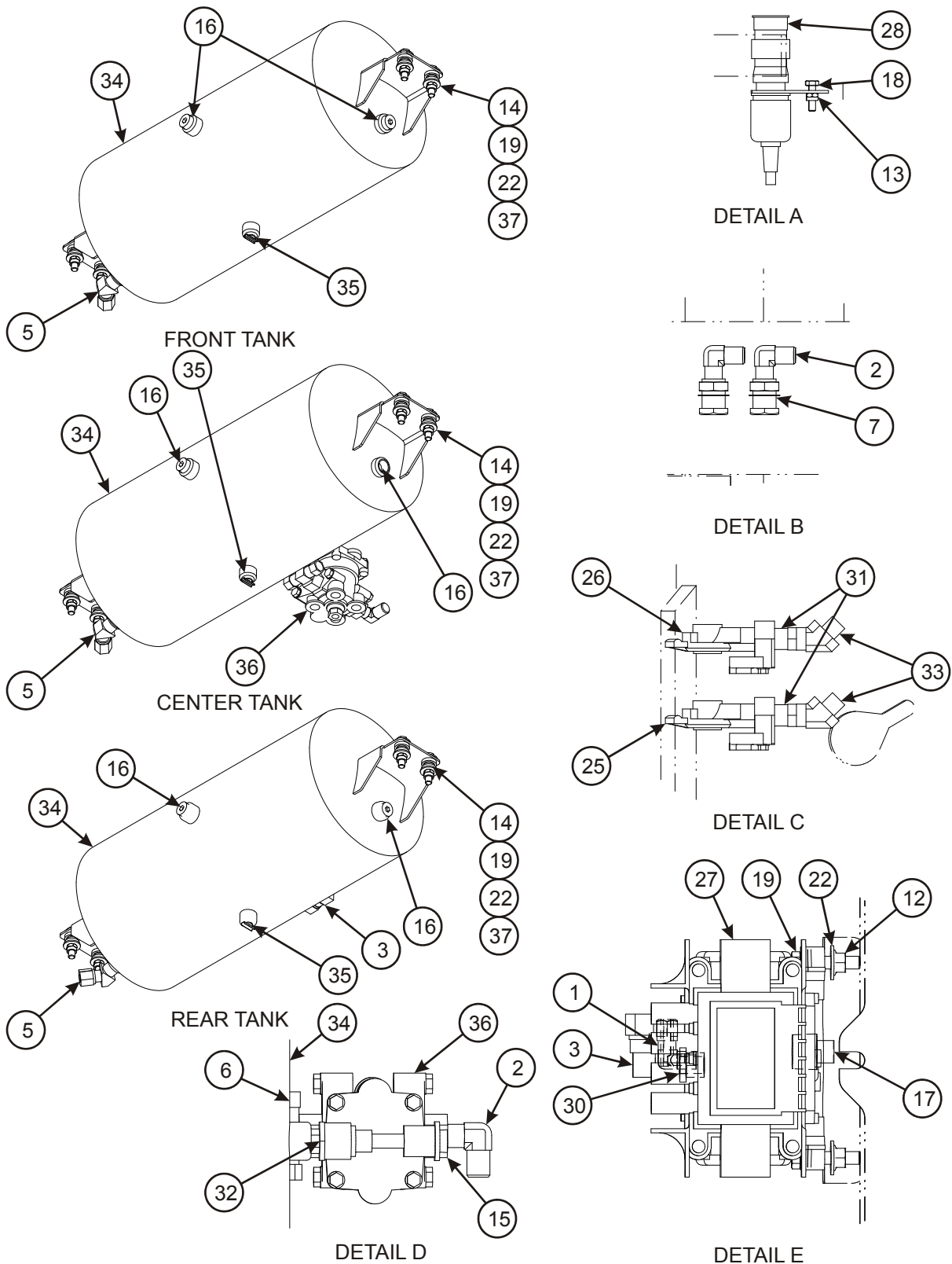
Figure 2-30: Air Brake System (835C Triple Axle) (2 of 3)
