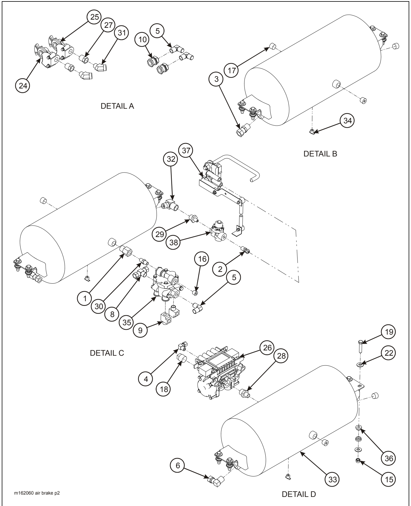
Figure 2-33: Air Brake System (855C) (2 of 3)
