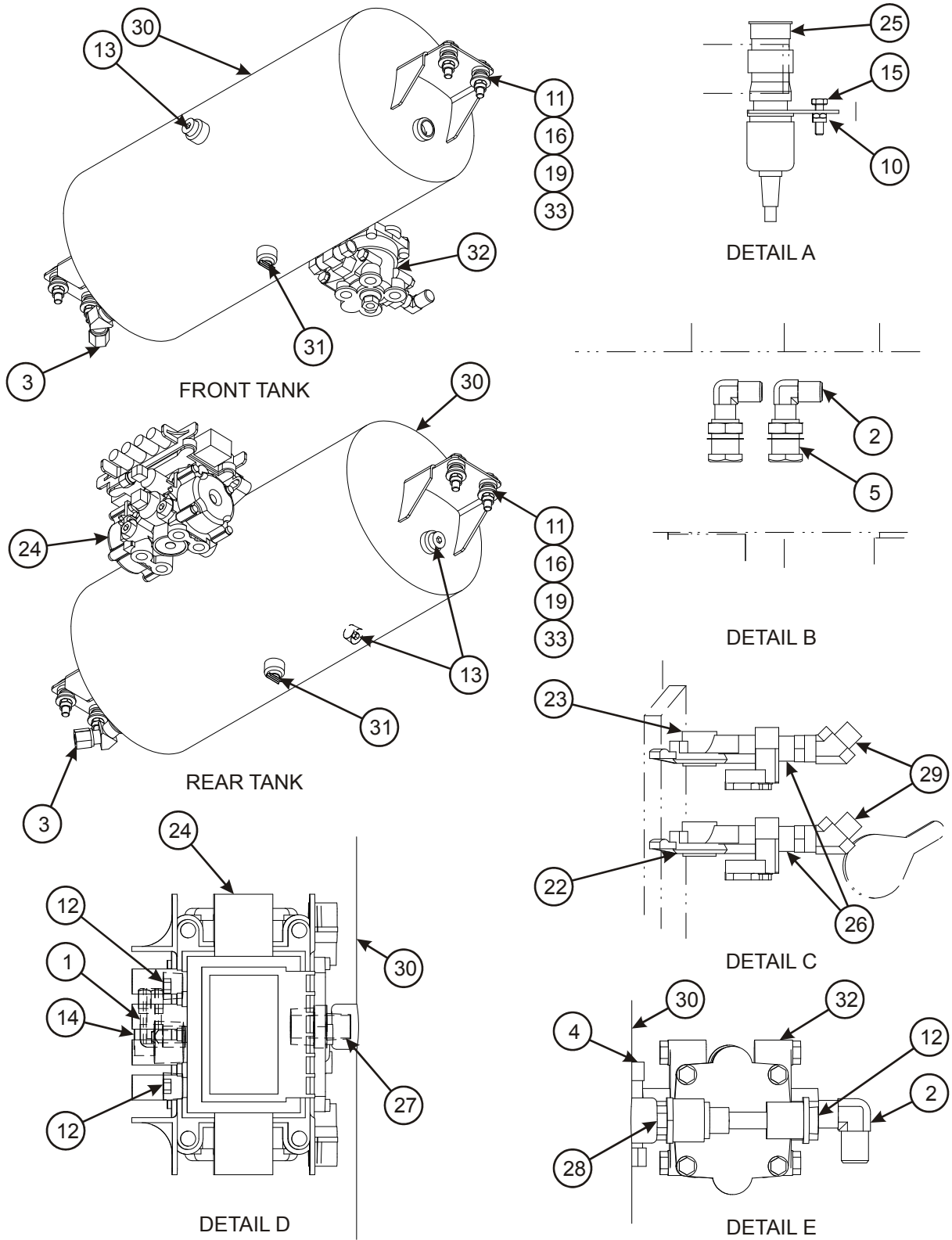
Figure 2-27: Air Brake System (835C Spread Axle) (2 of 3)
