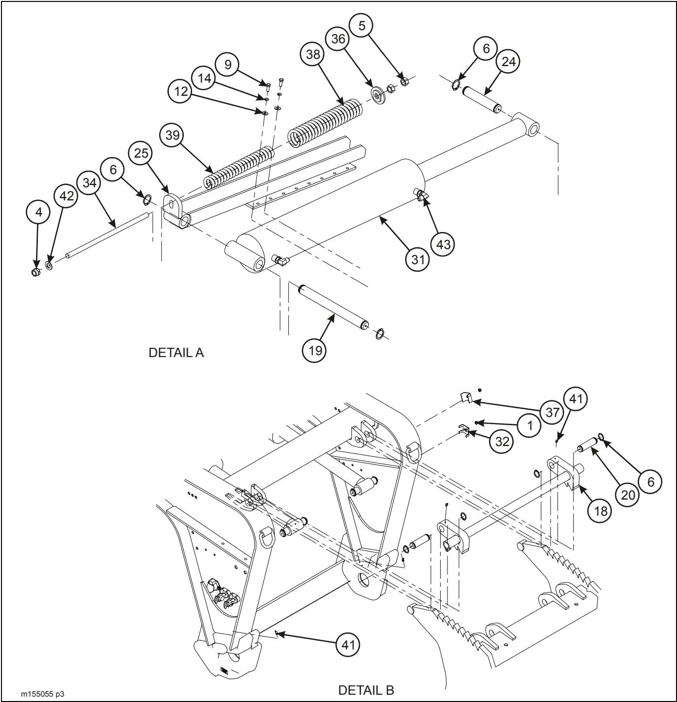
Figure 2-7: Gooseneck Assembly (825C/835C) (3 of 3)
