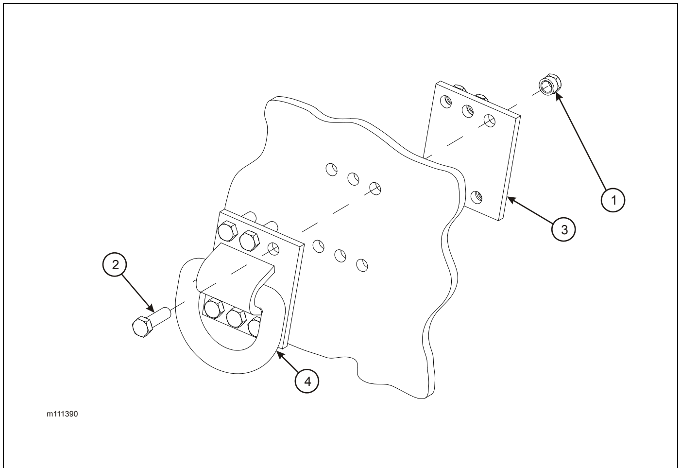
Figure 2-108: Bolt-On D-Ring Assembly (Option)
