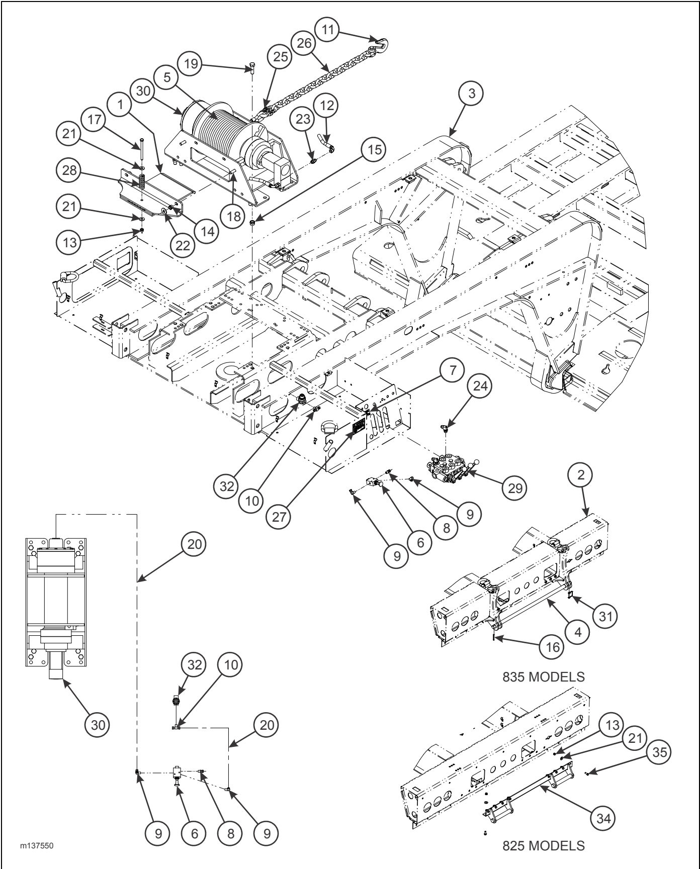
Figure 2-86: 30,000 Lb. Winch Installation (DP)
