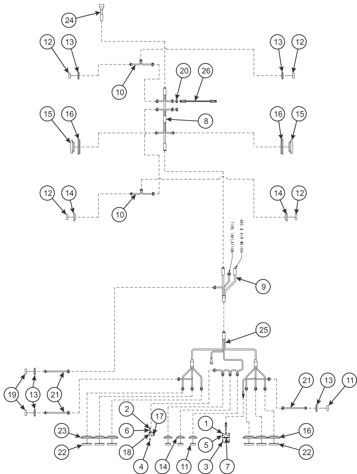
Figure 2-21: Frame Electrical System (855C)
