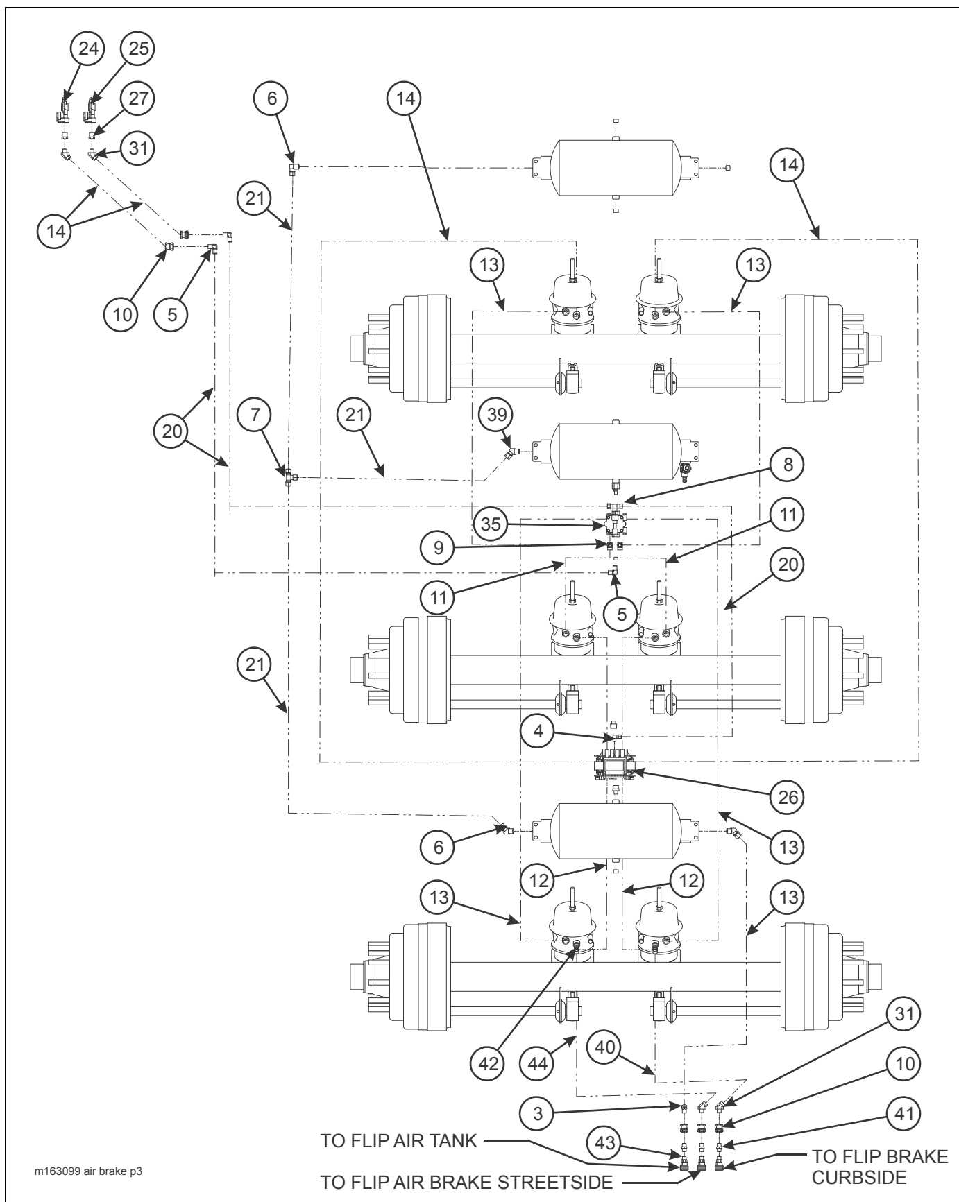
Figure 2-34: Air Brake System (855C) (3 of 3)
