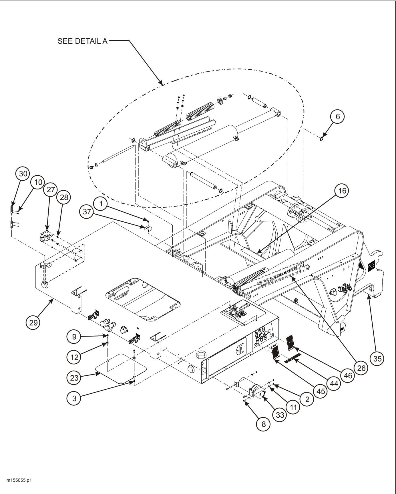
Figure 2-5: Gooseneck Assembly (825C/835C)(1 of 3)
