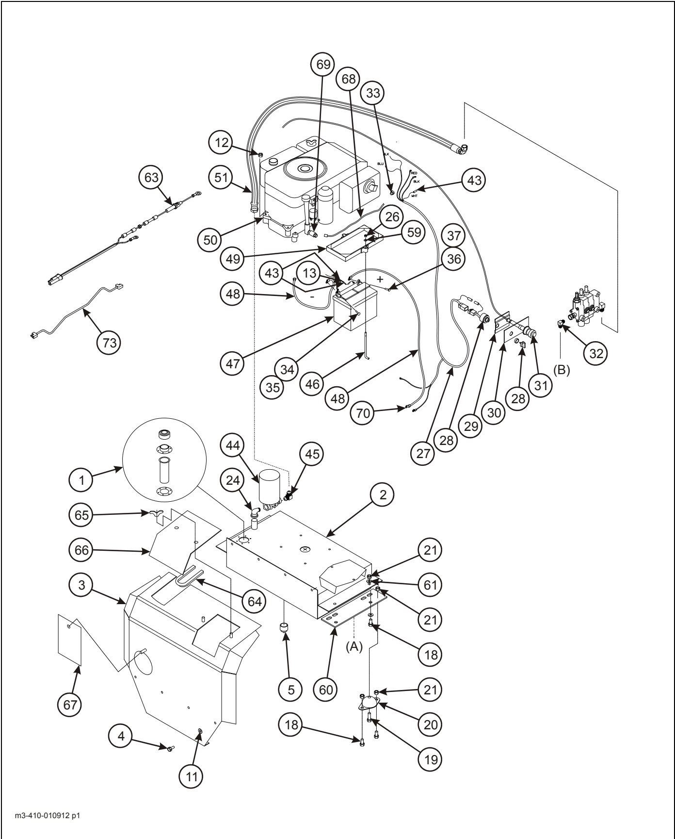
Figure 2-79: 42-11 HP Honda Engine Drive Installation (Option) (1 of 2)
