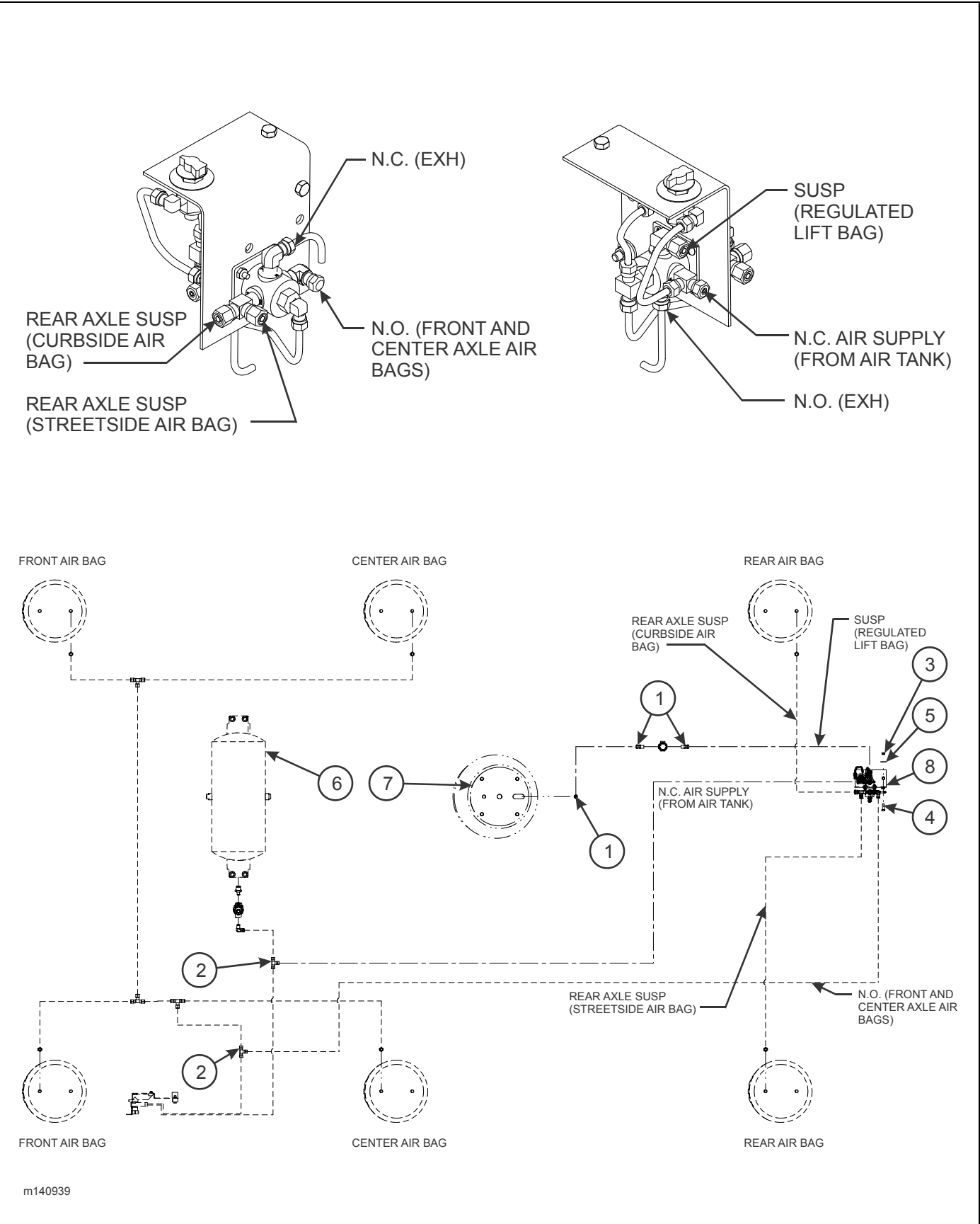
Figure 2-104: Axle Lift Control (Option)
