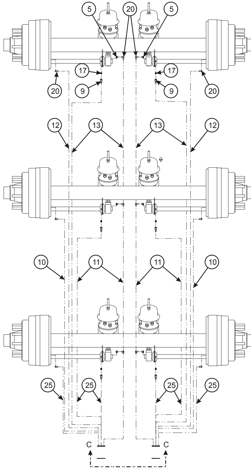
Figure 2-45: Frame Assembly and Grease System (855C) (2 of 3)
