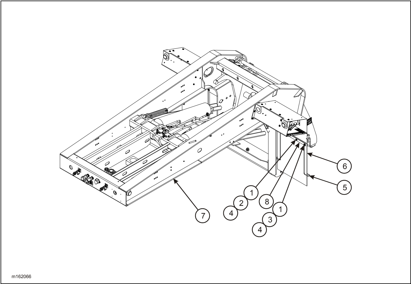
Figure 2-72: Gooseneck Mud Flaps (Option)
