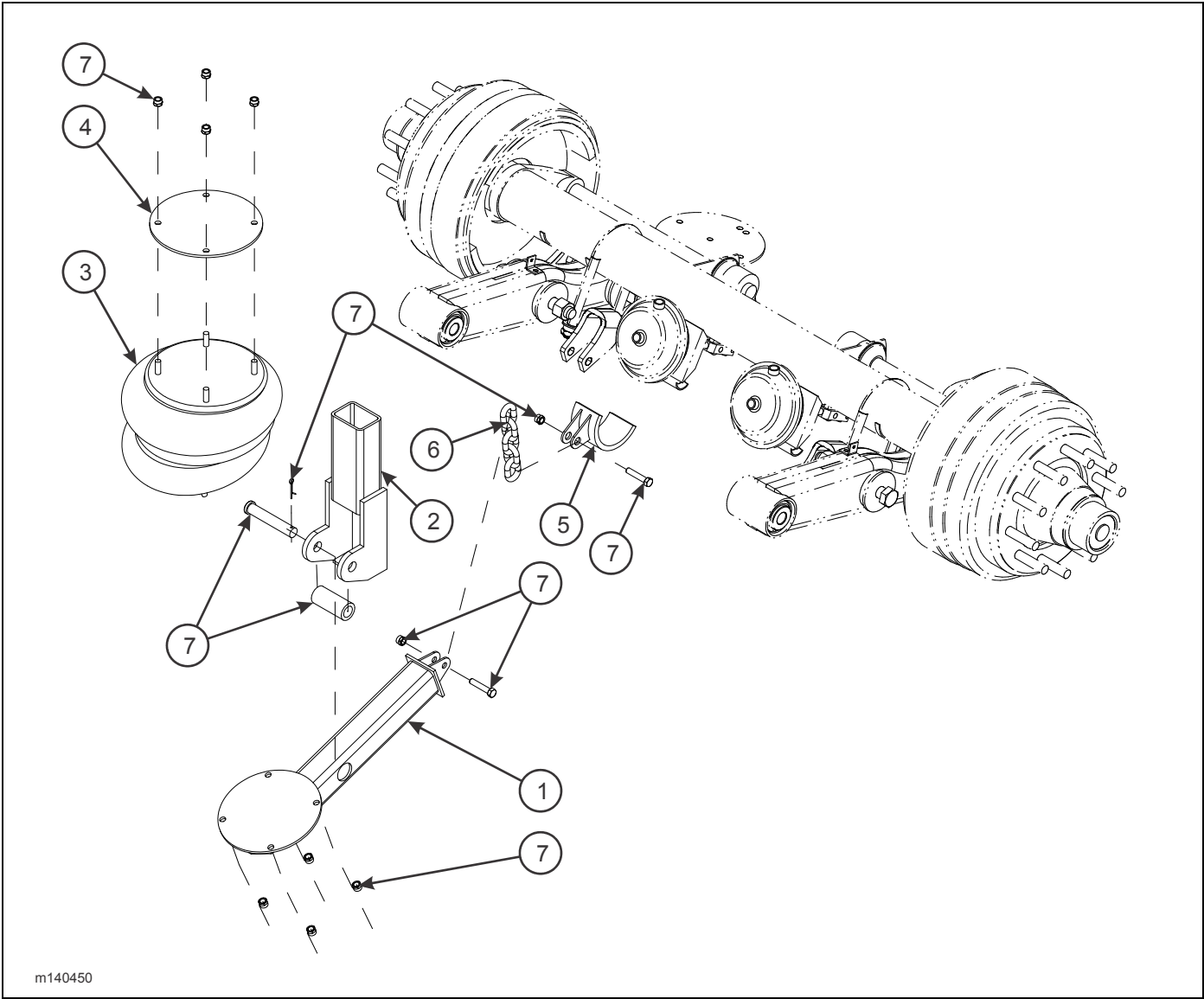
Figure 2-107: Rear Suspension Air Lift Assembly (Option)
