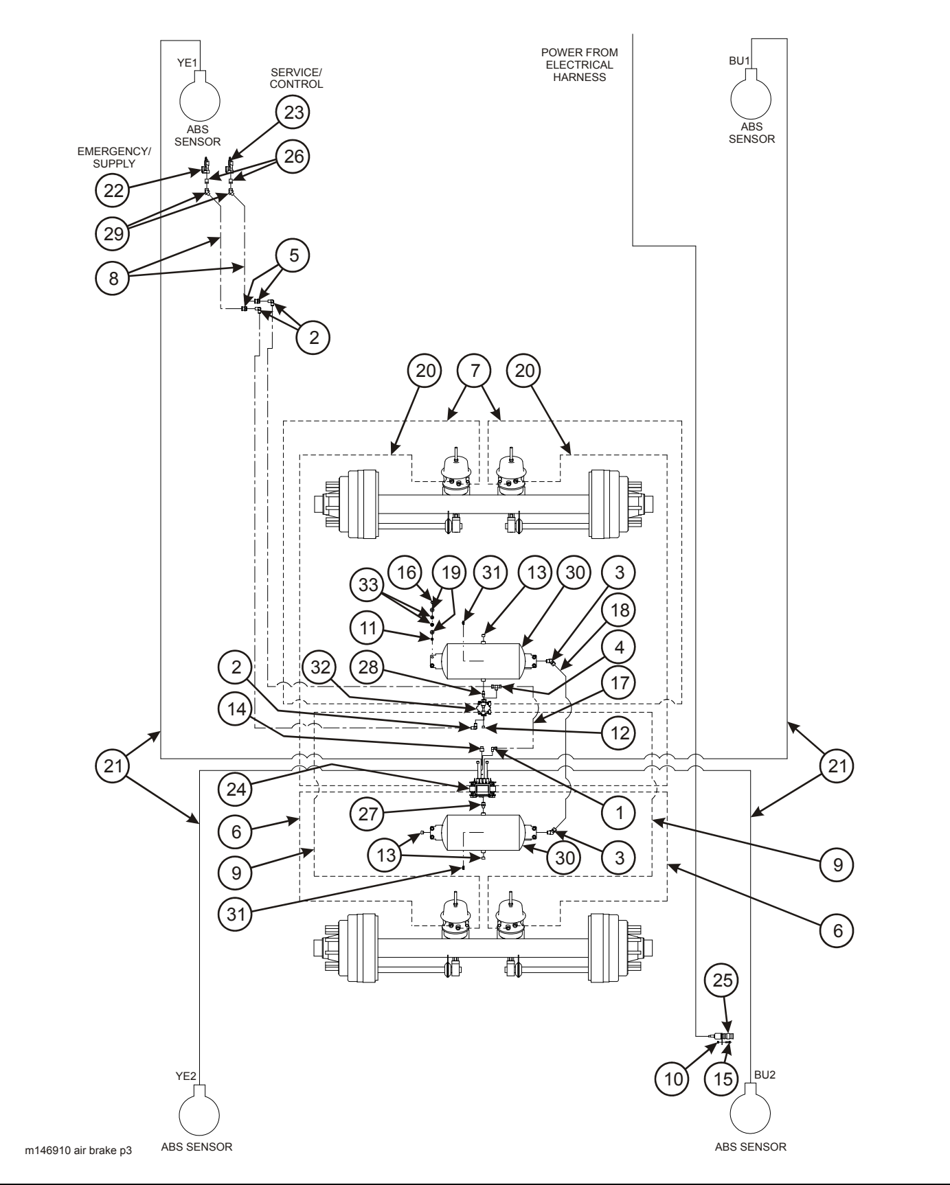
Figure 2-28: Air Brake System (835C Spread Axle) (3 of 3)
