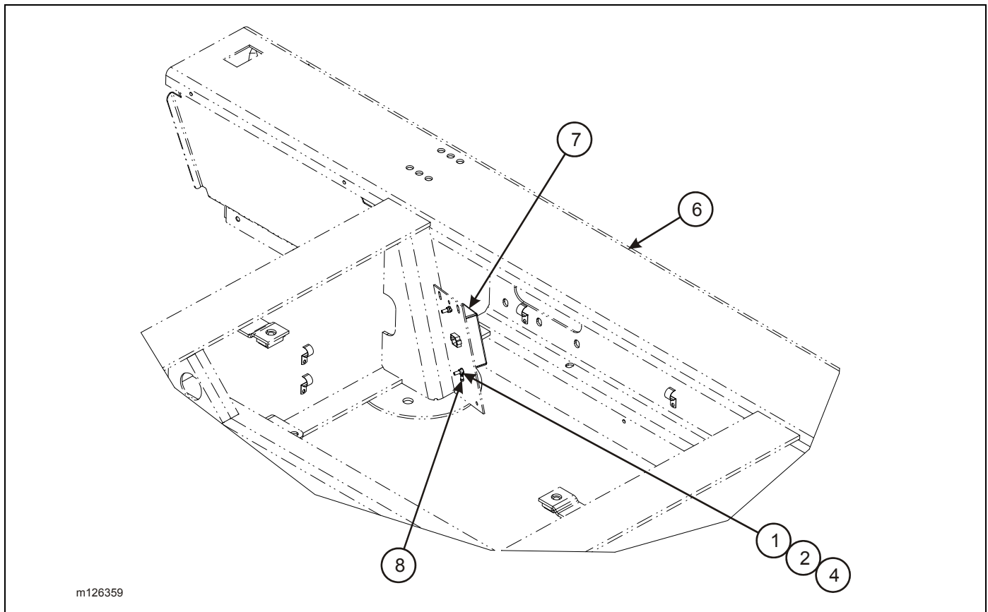
Figure 2-99: Air Weigh Scale Installation (Option)
