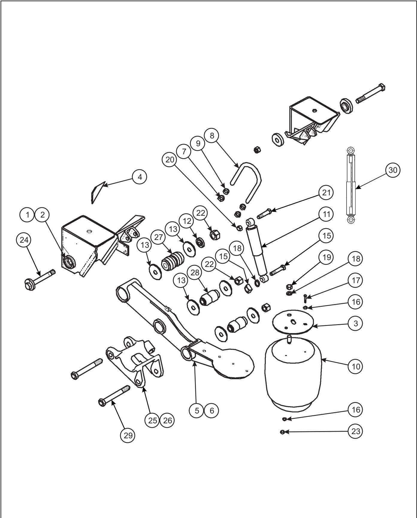
Figure 2-54: Suspension, Fastener RLU-250-9-4
