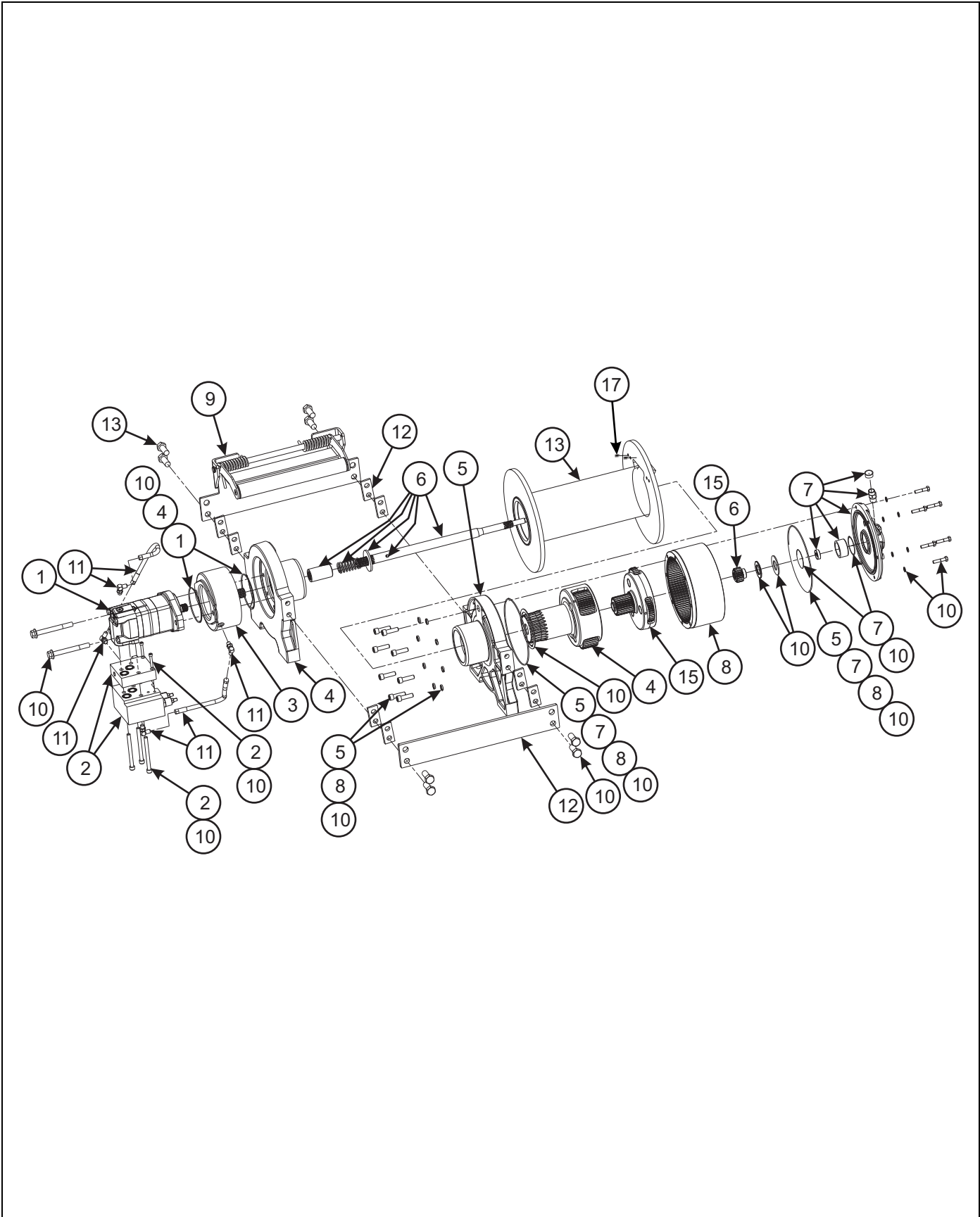
Figure 2-89: 30,000 Lb. Winch Items (Warn)
