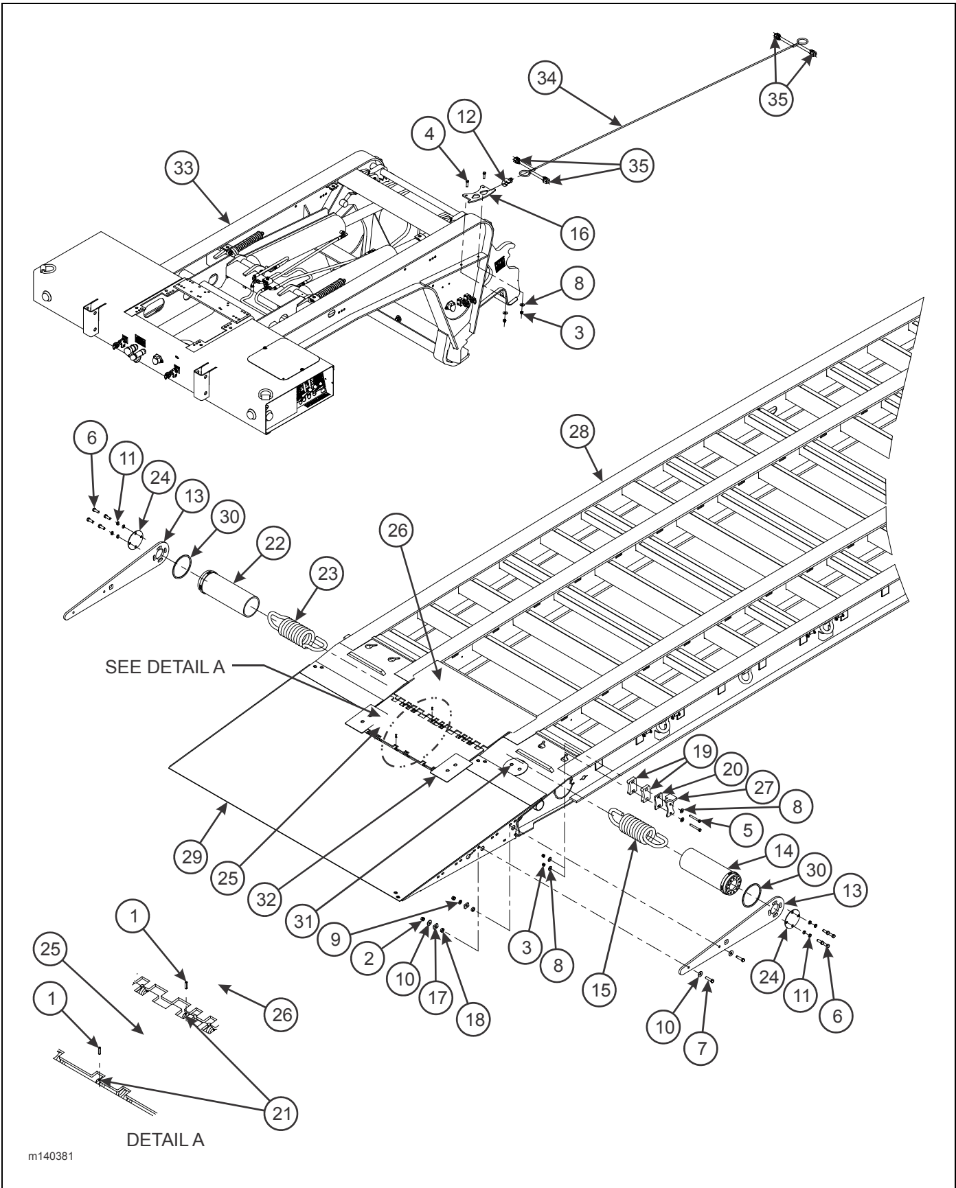
Figure 2-92: Front Fold Ramp Installation (Option)
