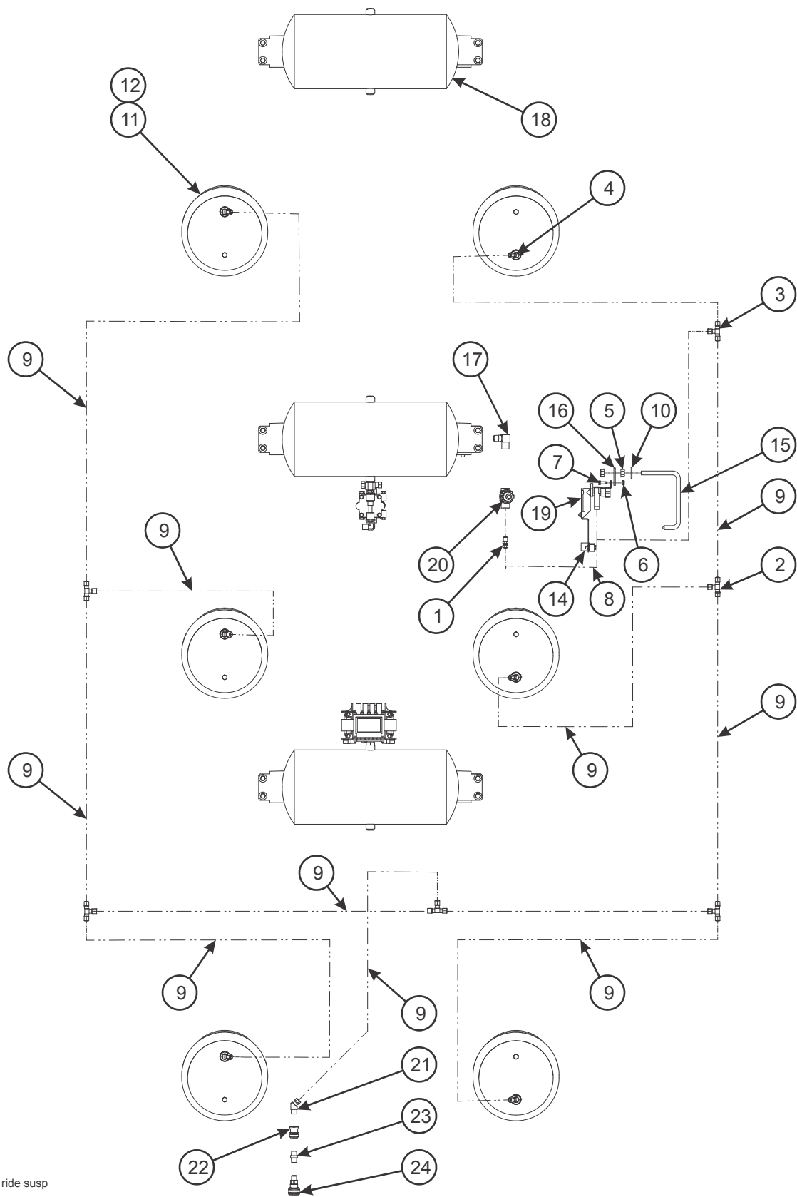
Figure 2-50: Frame Assembly - Air Ride Suspension (855C)
