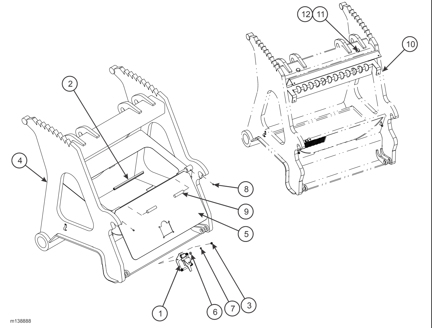
Figure 2-74: Chain Rack and Toolbox Assembly (Option)
