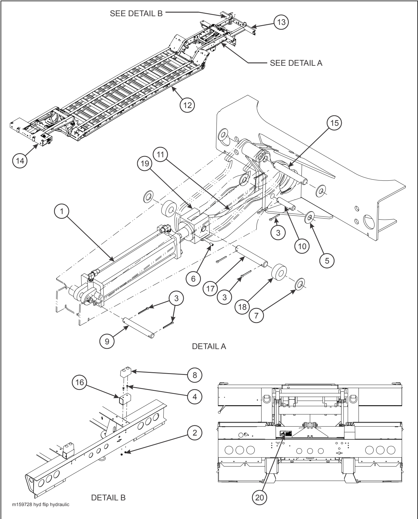
Figure 2-62: Hydraulic Flip Assembly - Frame and Cylinder Placement
