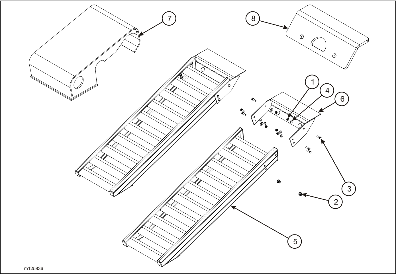
Figure 2-90: Aluminum Trunnion Ramp Assembly (Option)
