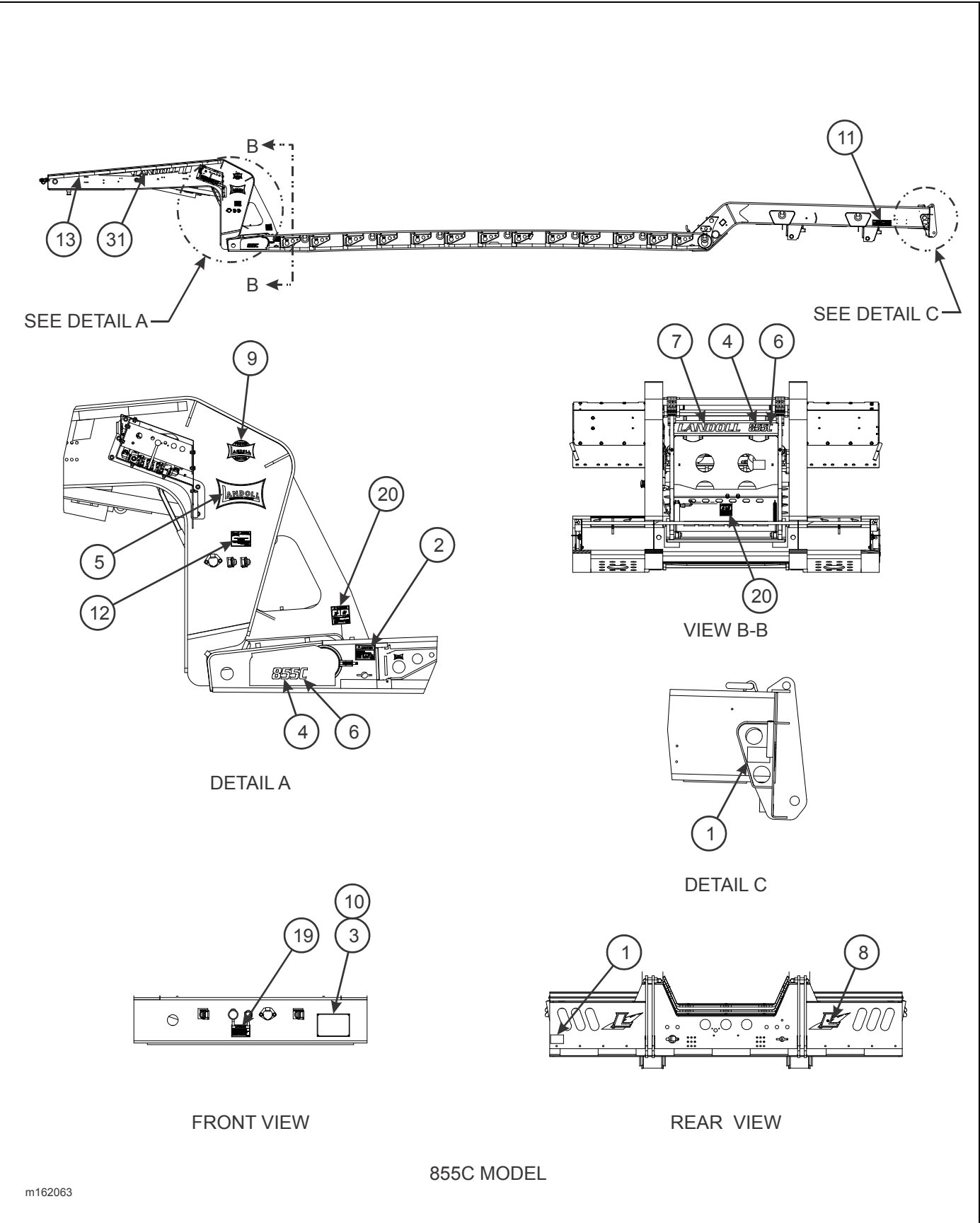
Figure 2-4: Decal Placement
