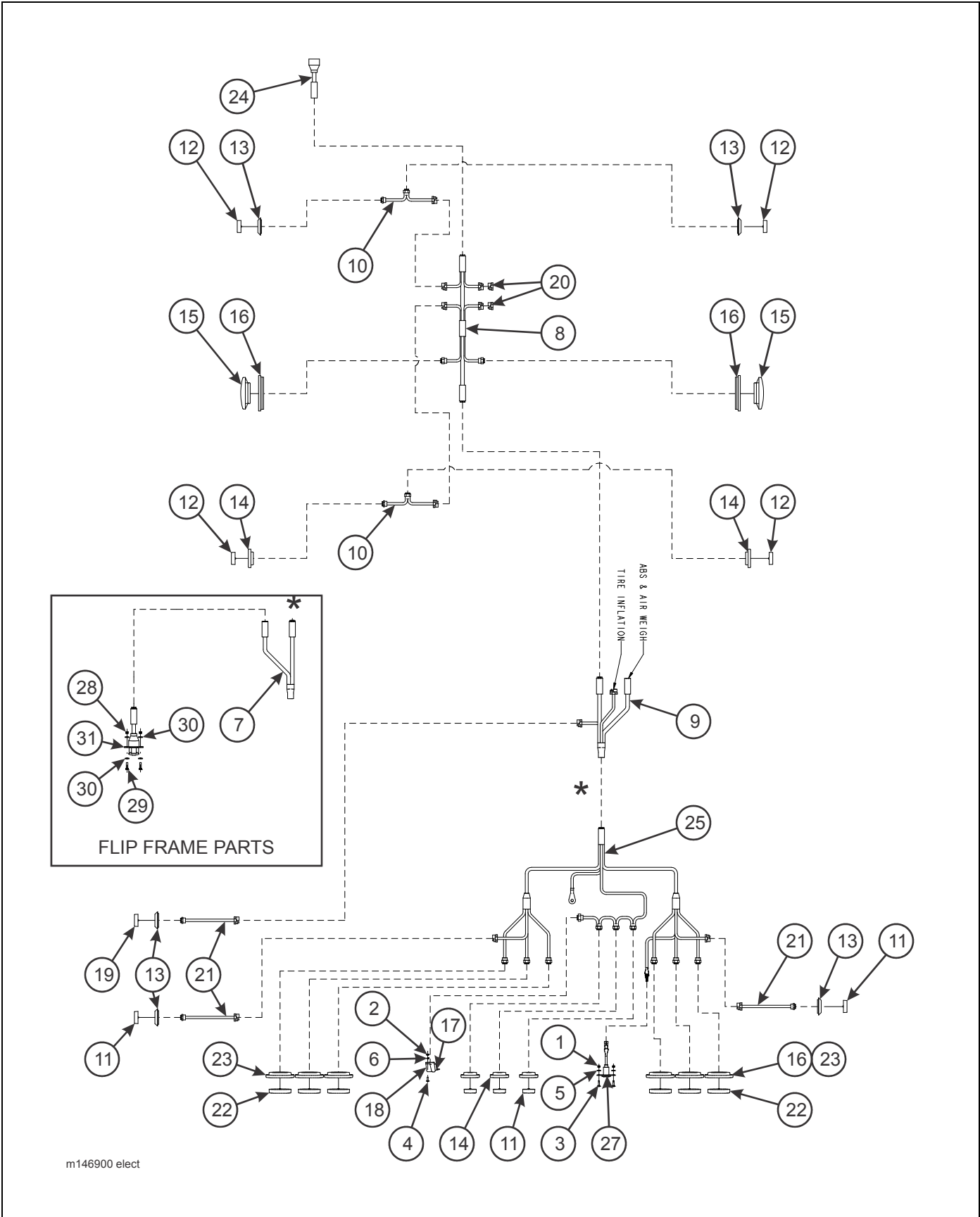
Figure 2-20: Frame Electrical System (825C/835C)
