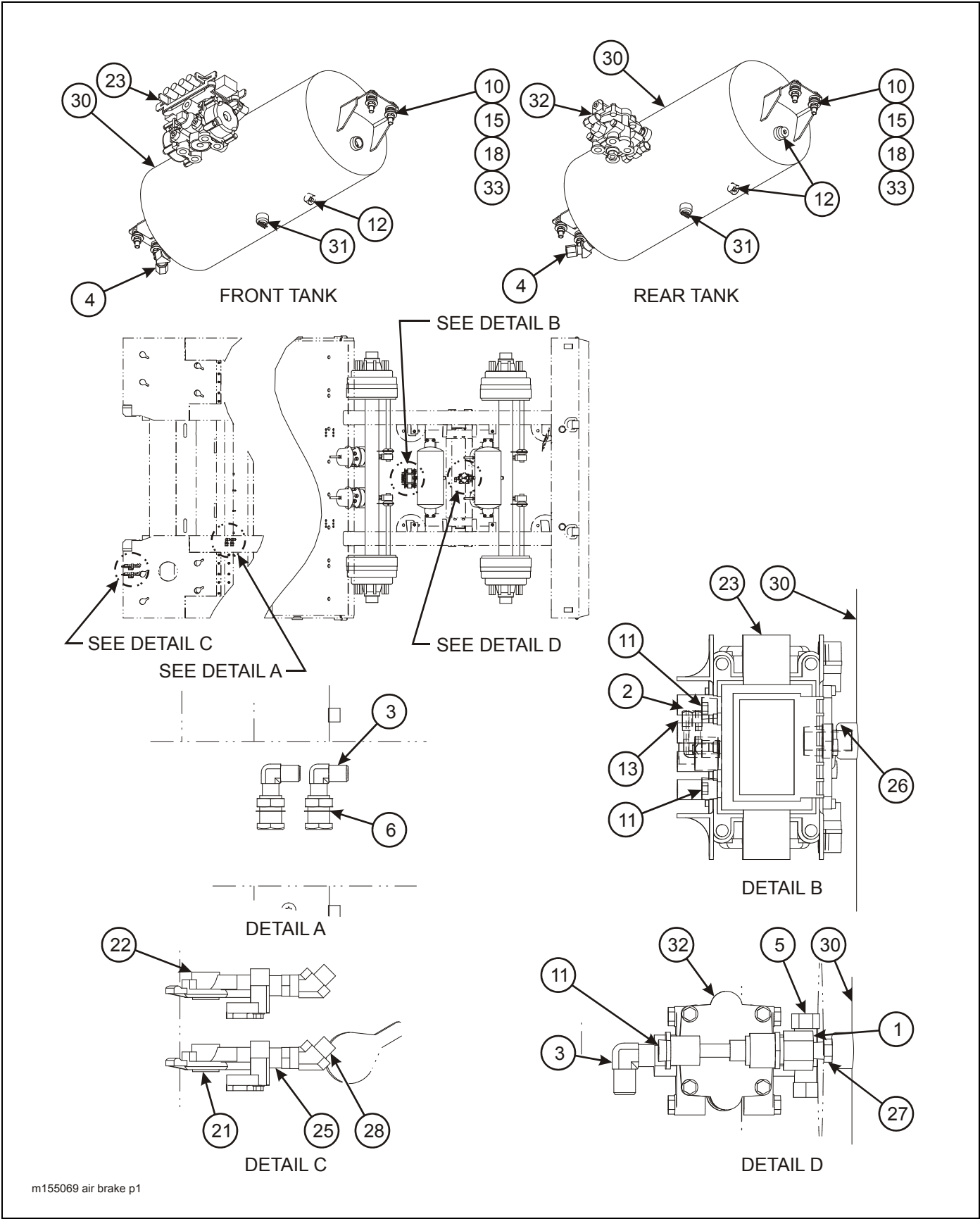
Figure 2-22: Air Brake System (825C) (1 of 2)
