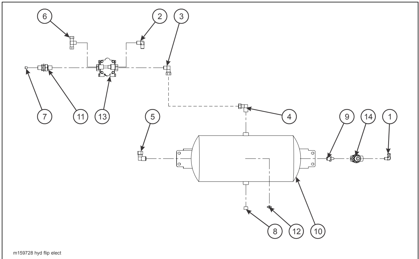
Figure 2-66: Hydraulic Flip Assembly - Air
