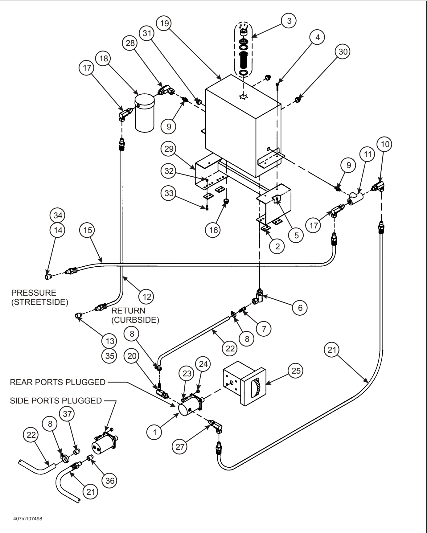
Figure 2-81: Hydraulic Wet Kit (Option)
