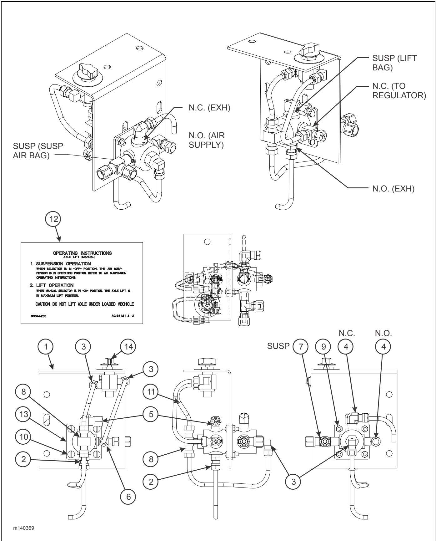
Figure 2-106: Lift Axle (Flip) Control Assembly (835) (Option)
