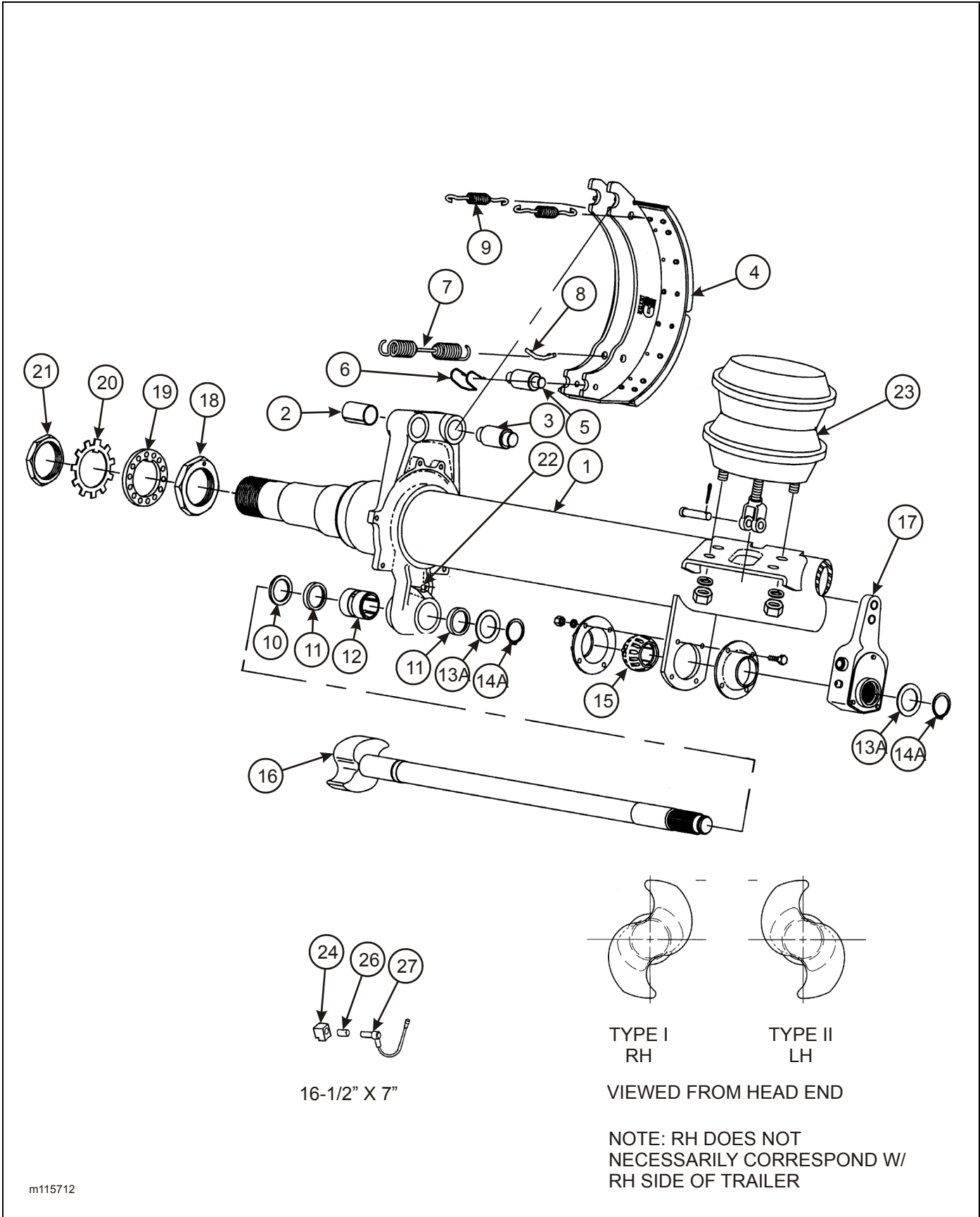
Figure 2-55: Axle and Brake Assembly
