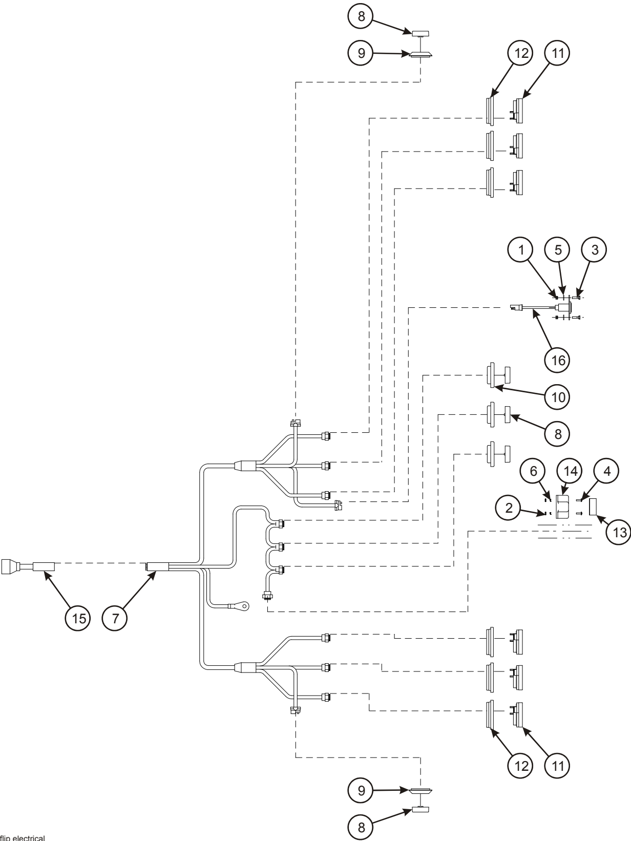
Figure 2-61: Flip Assembly - Electrical System
