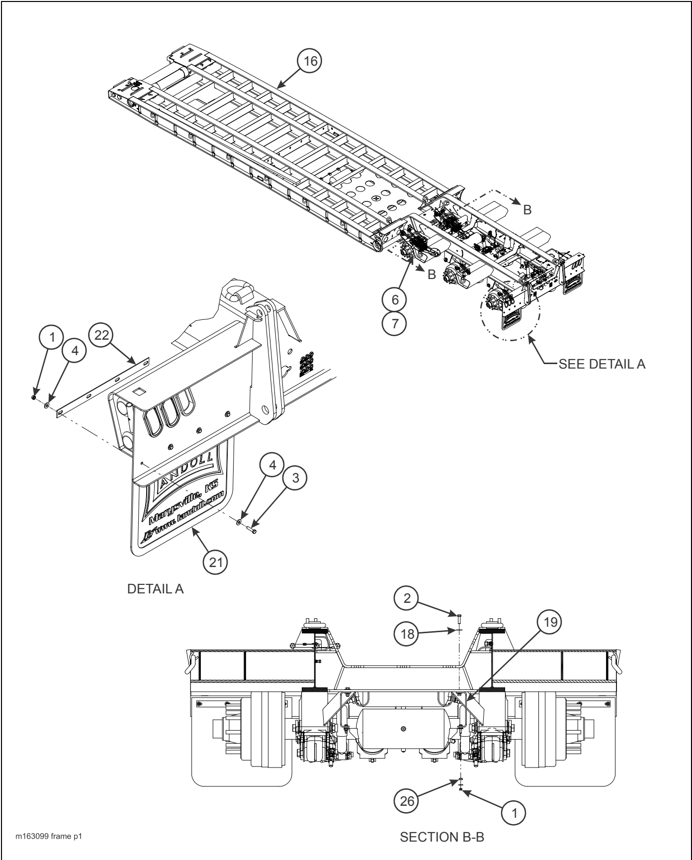
Figure 2-44: Frame Assembly and Grease System (855C) (1 of 3)
