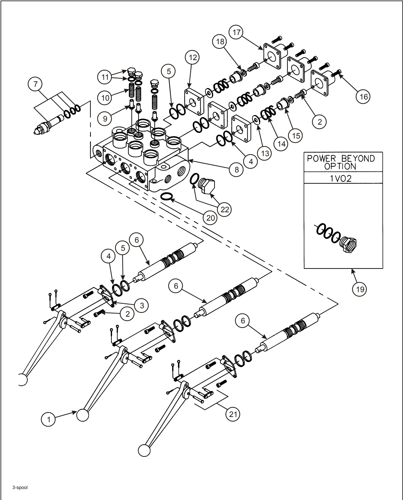
Figure 2-16: Three Spool Valve
