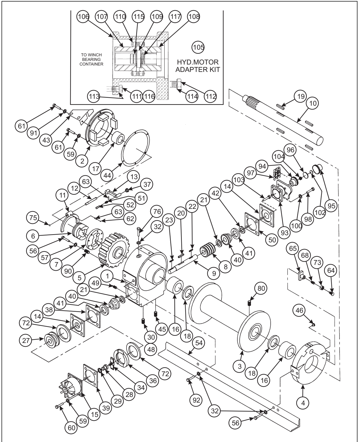
Figure 2-84: 20,000 Lb. Winch Assembly
