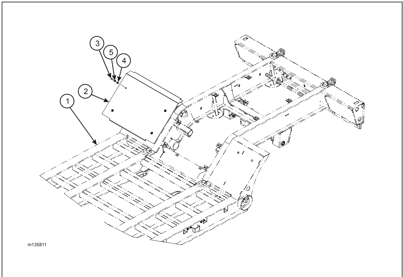
Figure 2-101: Slope Cover Assembly (Option)
