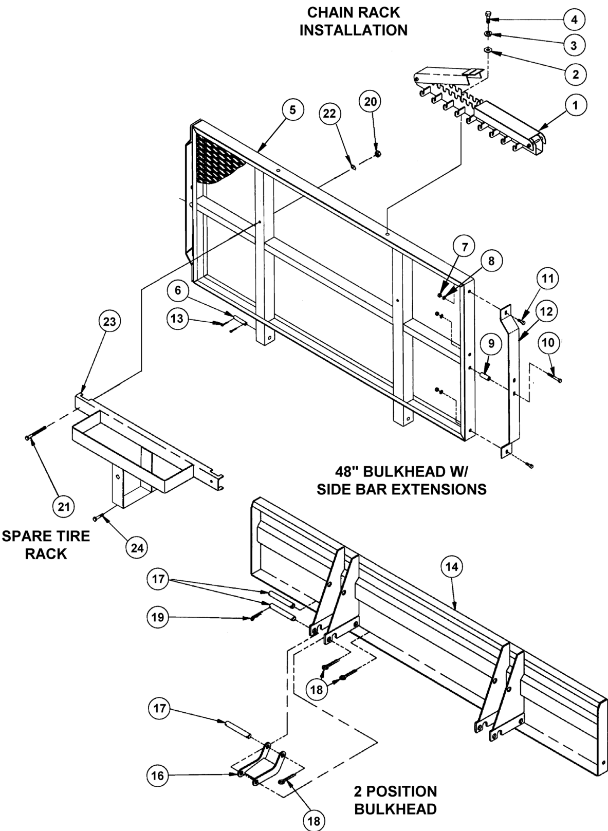
Figure 2-70: Bulkhead and Chain Rack Installation (Option)
