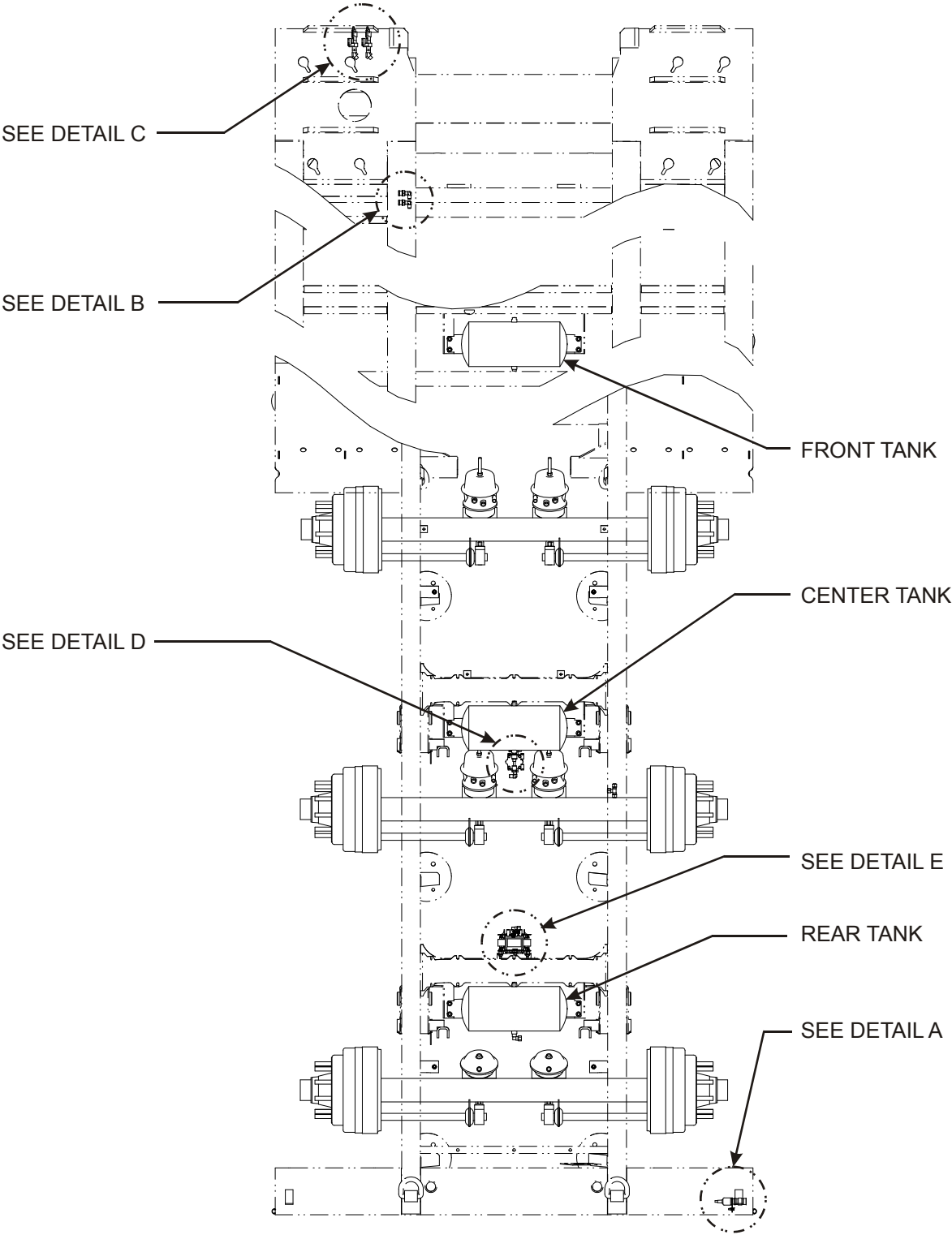
Figure 2-29: Air Brake System (835C Triple Axle) (1 of 3)
