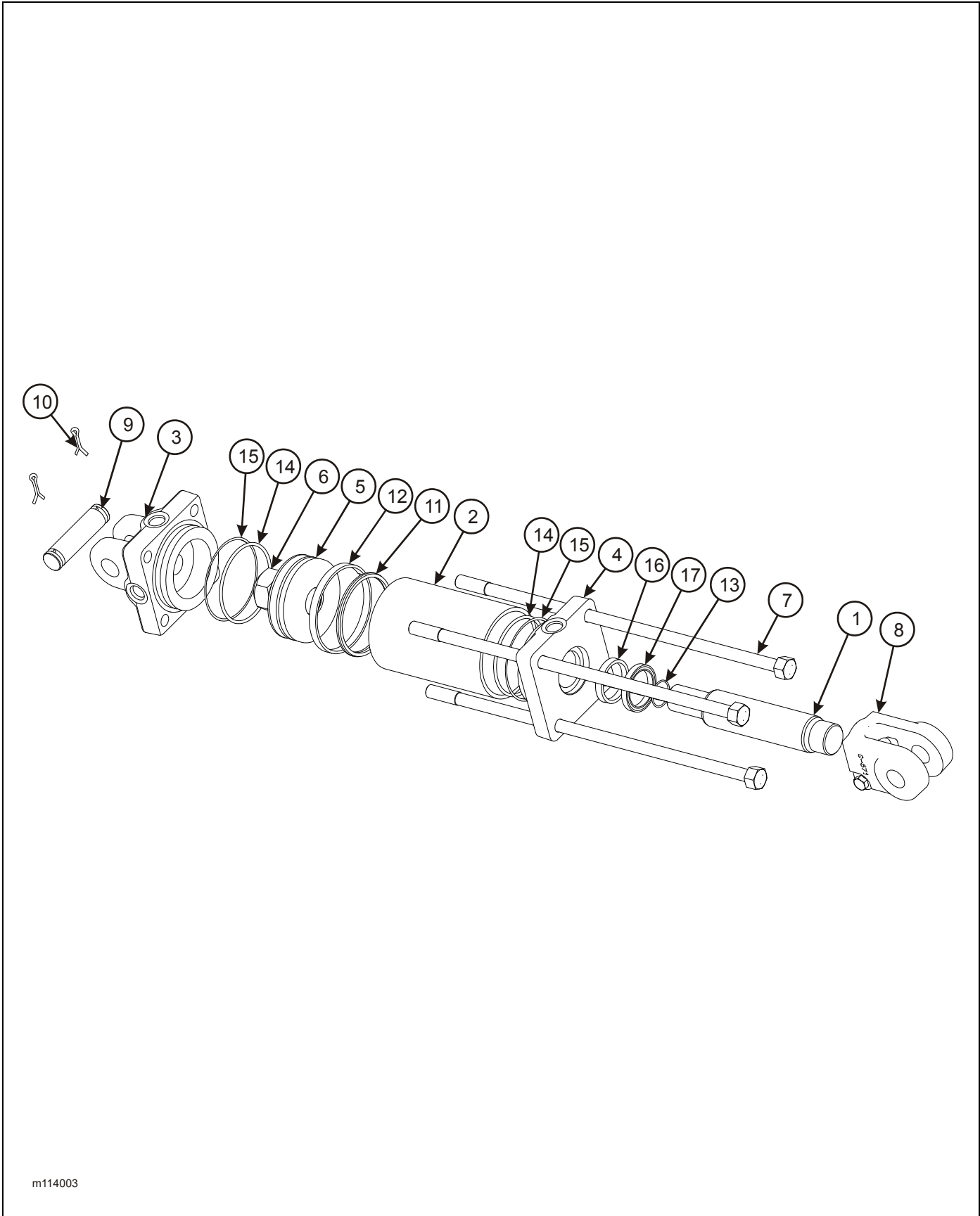
Figure 2-64: Cylinder, Hydraulic 4 X 20
