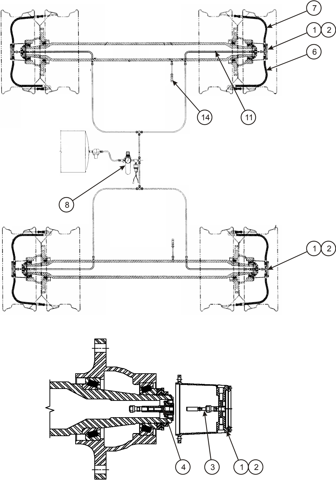
Figure 2-103: Tire Inflation System (Option)
