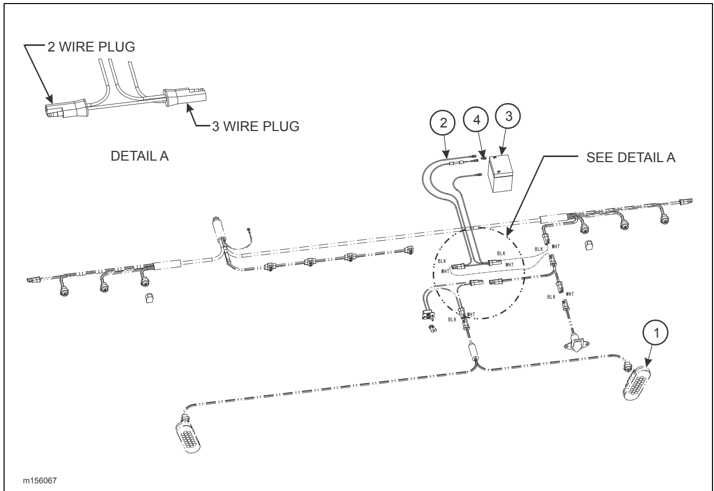
Figure 2-97: Battery Backup Bumper Strobe Light (Option)
