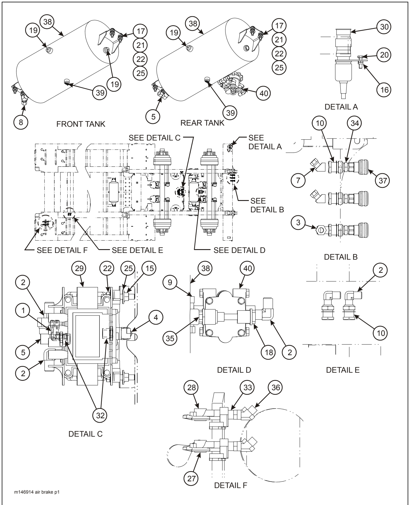
Figure 2-24: Air Brake System (835C) (1 of 2)
