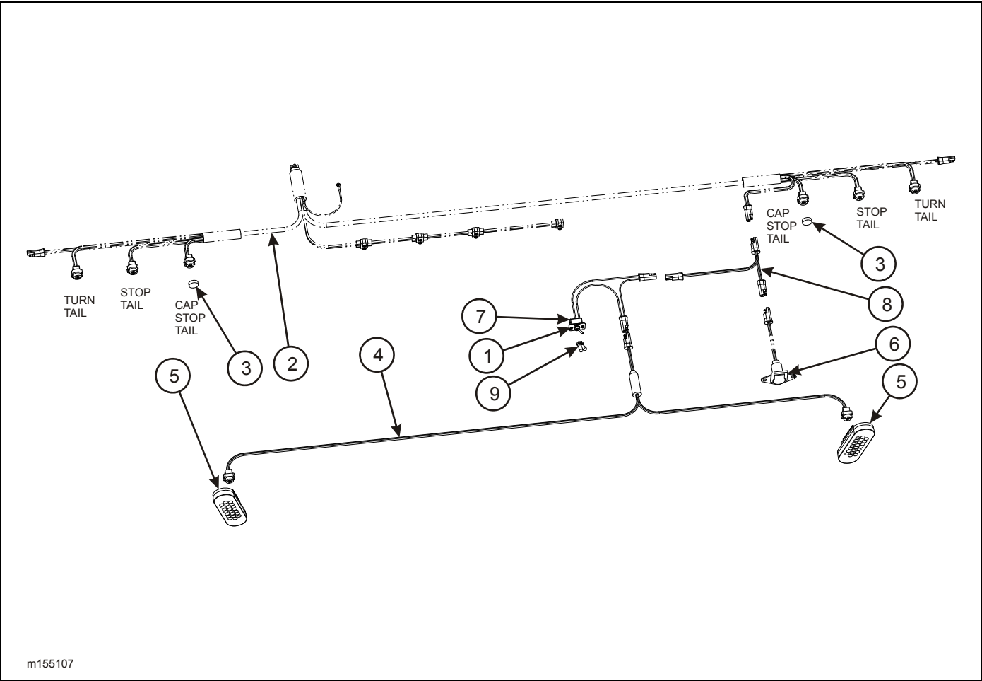
Figure 2-96: Bumper Strobe Light (Option)
