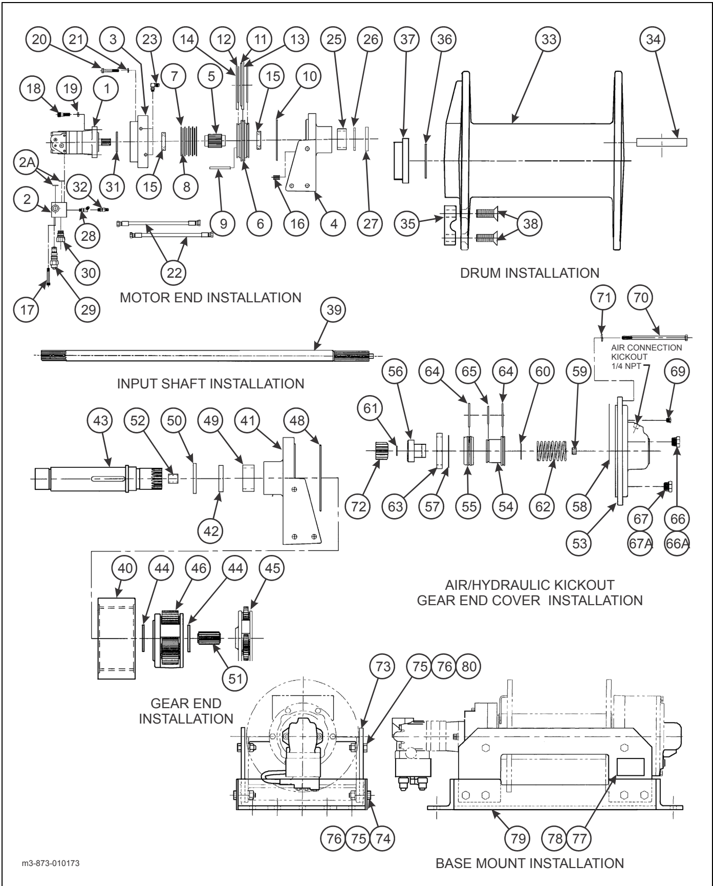
Figure 2-87: 30,000 Lb. Winch Items (DP)
