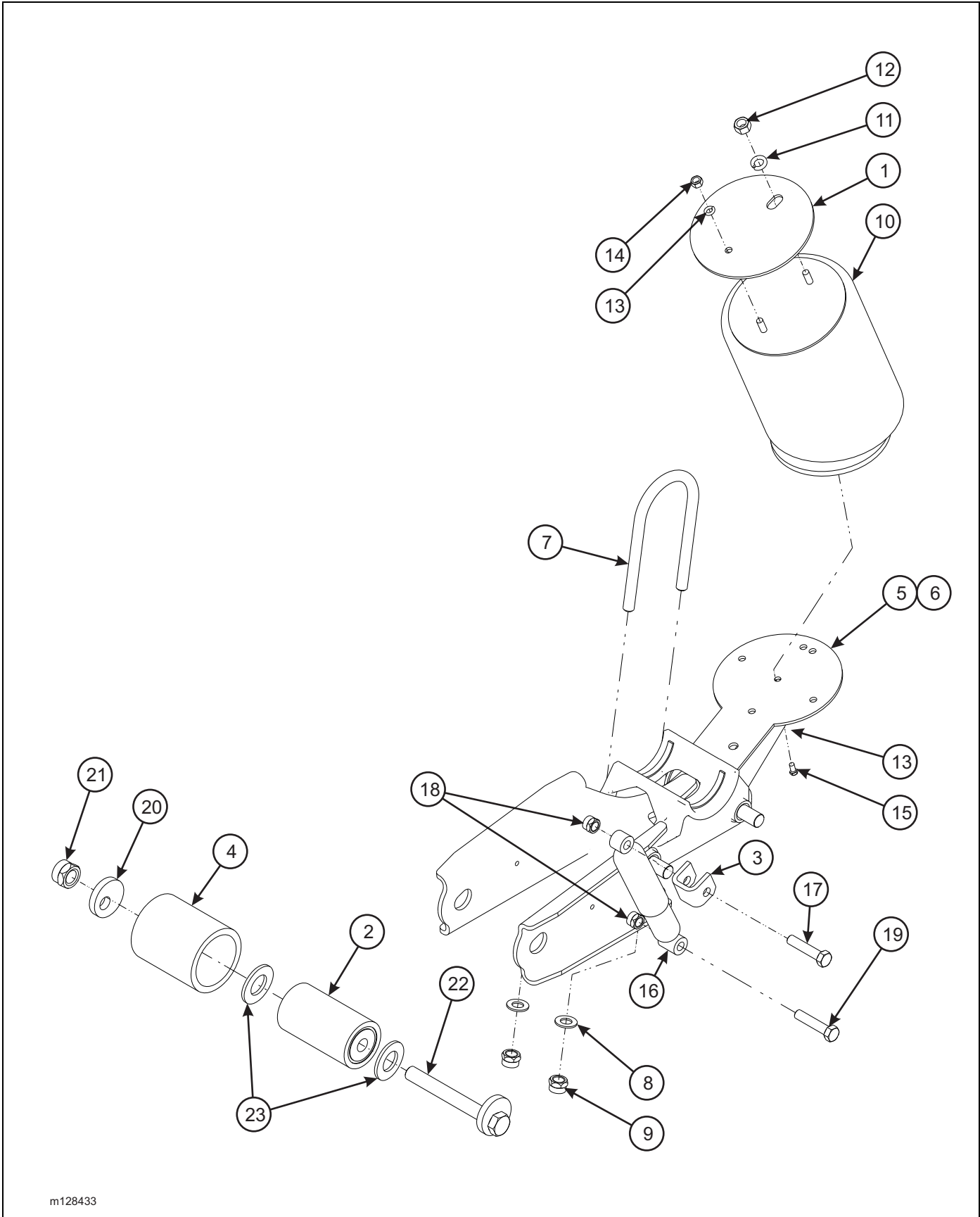
Figure 2-53: Suspension, Fastener RLU 250 FMT
