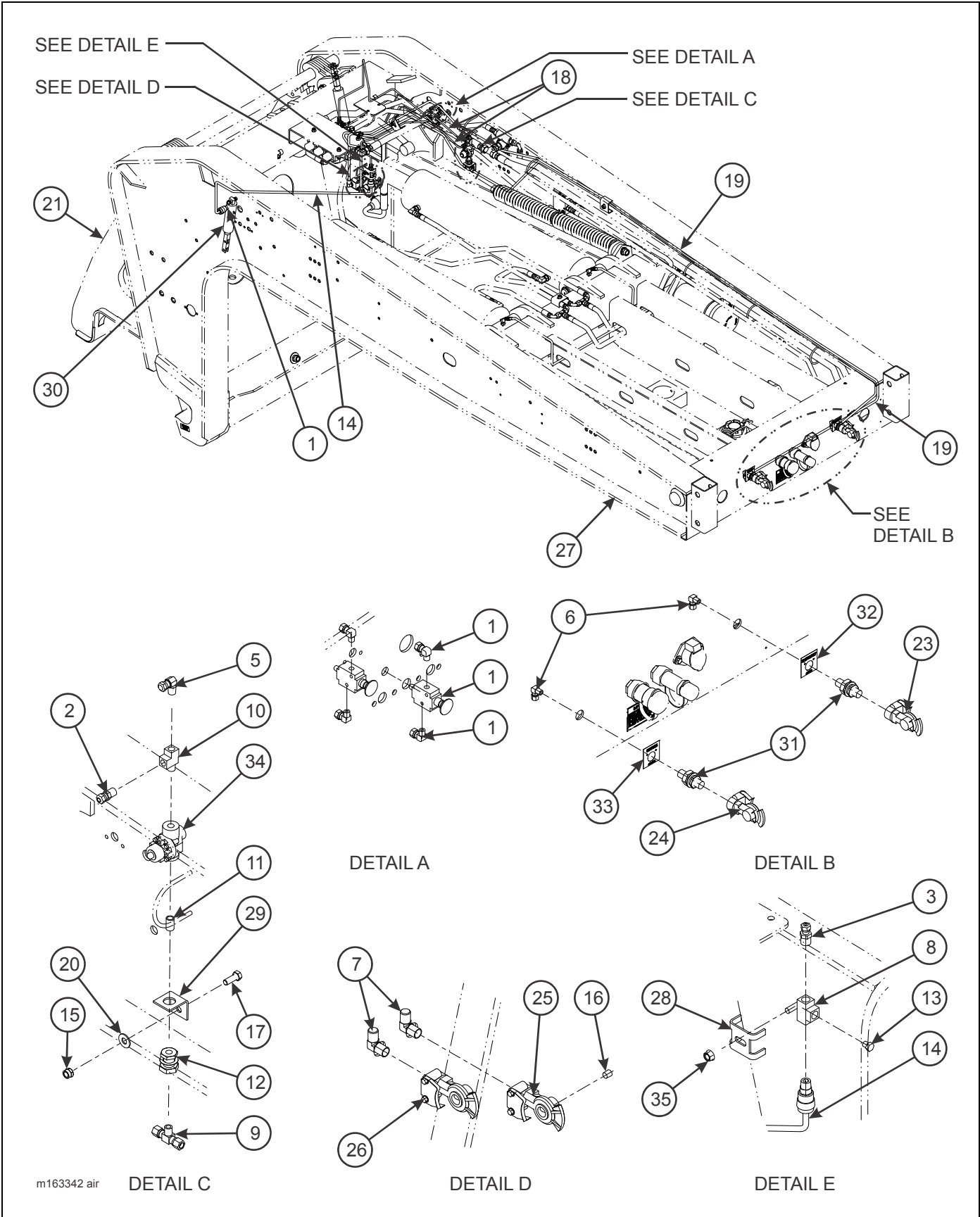
Figure 2-13: Gooseneck Air System (855C)
