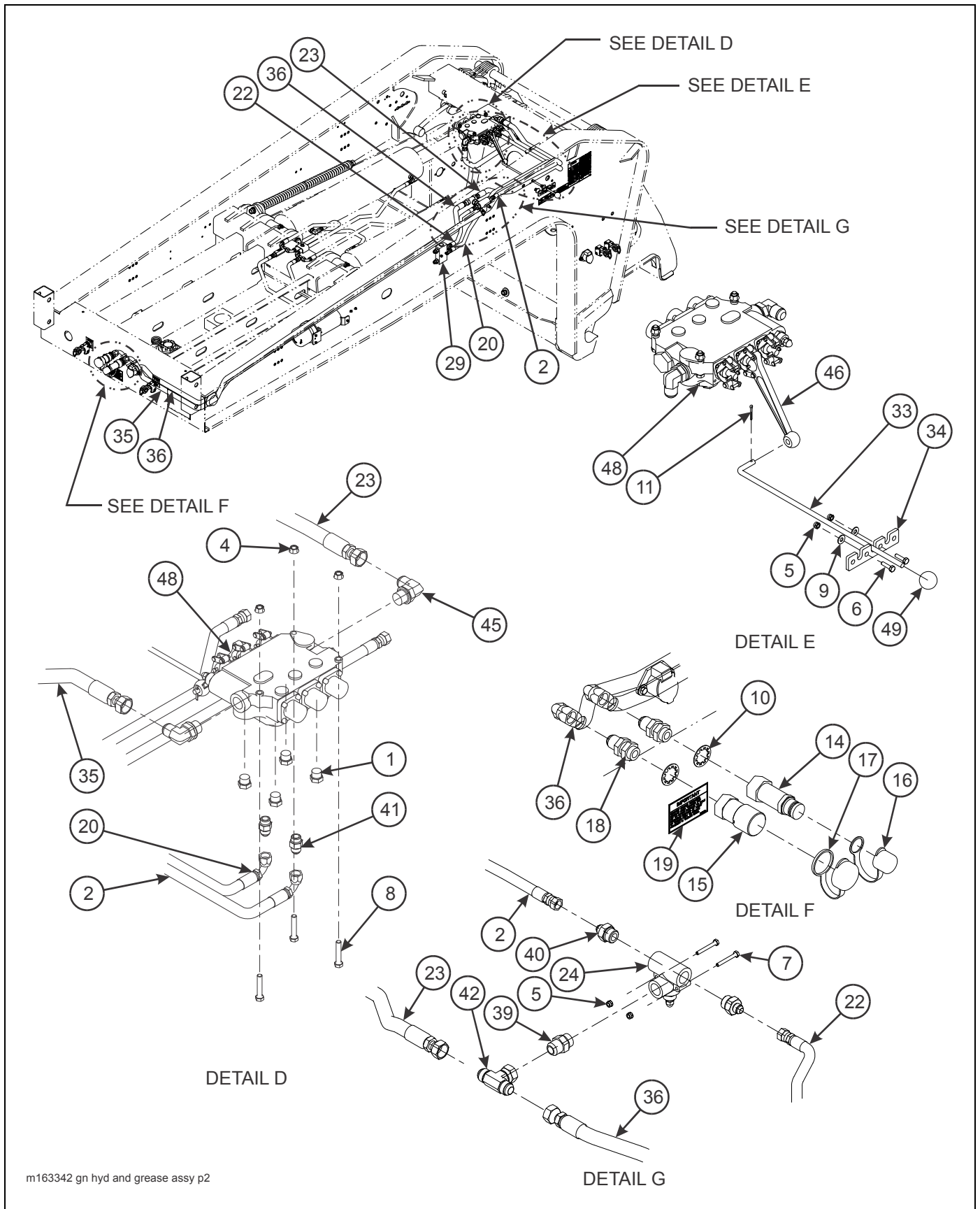
Figure 2-15: Gooseneck Hydraulic and Grease System (855C) (2 of 2)
