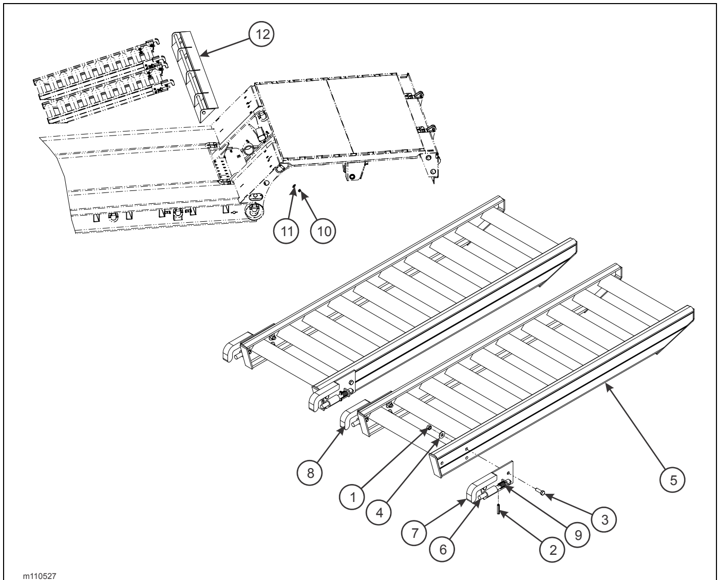
Figure 2-91: Aluminum Beavertail Ramp Assembly (Option)
