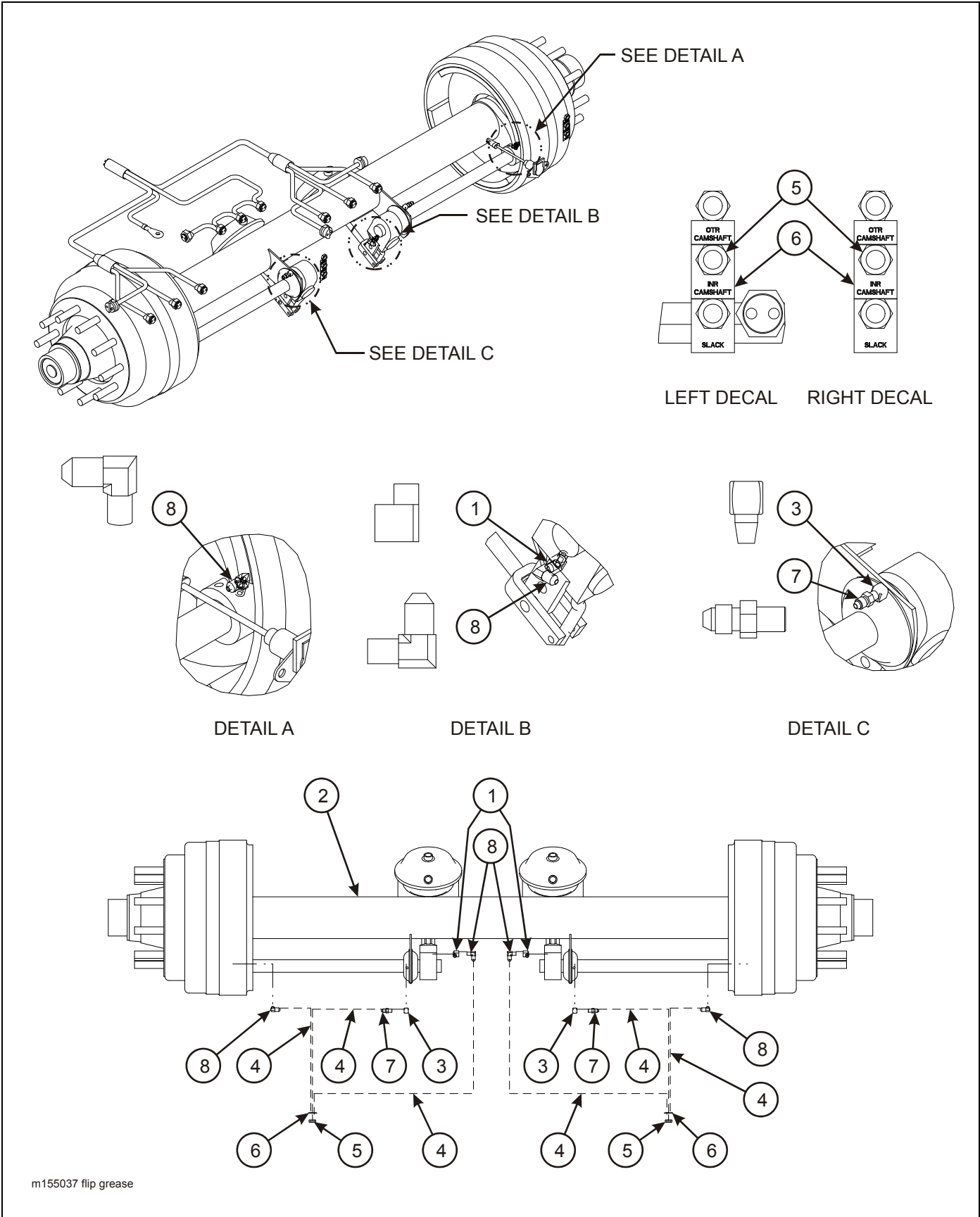
Figure 2-60: Flip Assembly - Grease System
