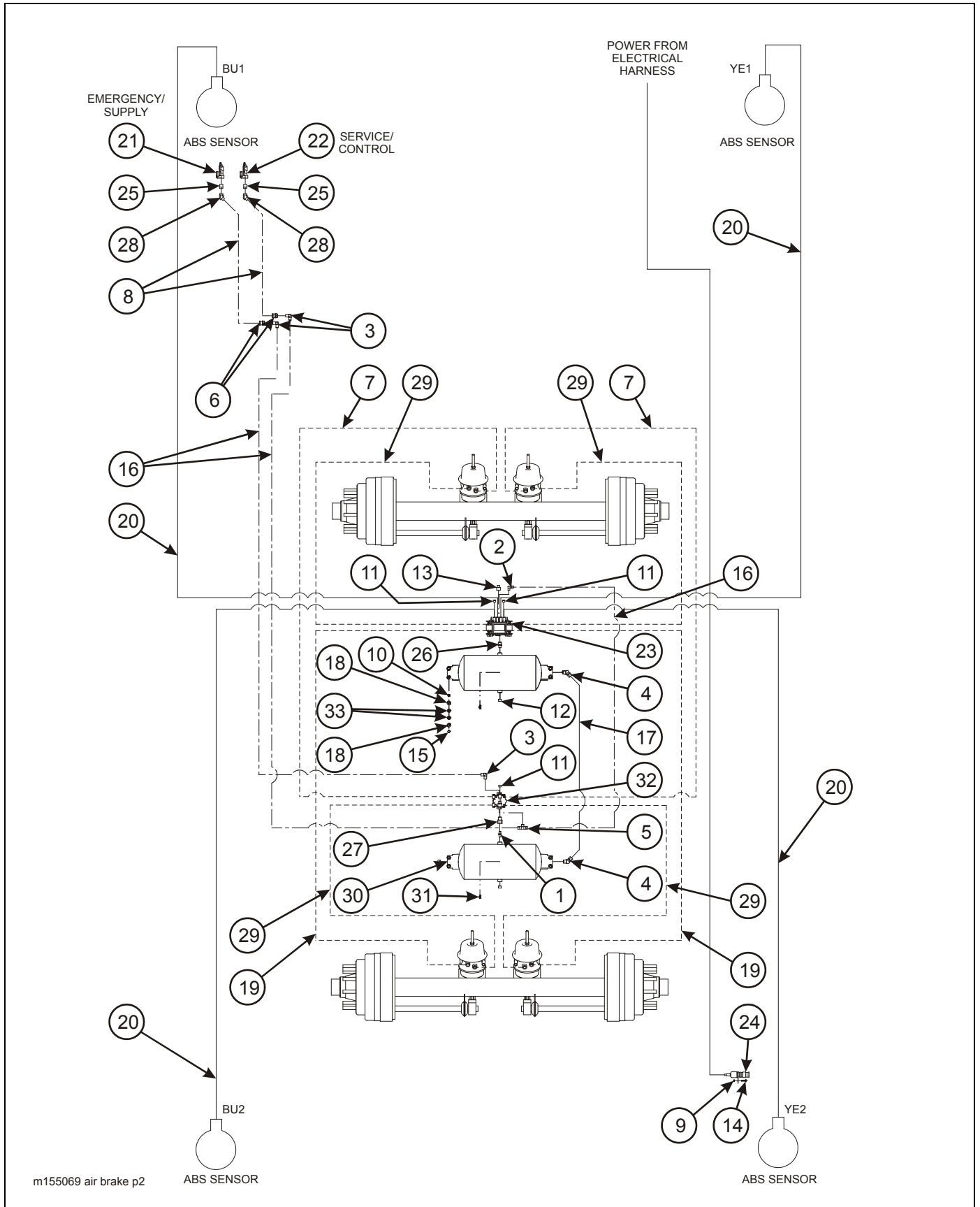
Figure 2-23: Air Brake System (825C) (2 of 2)
