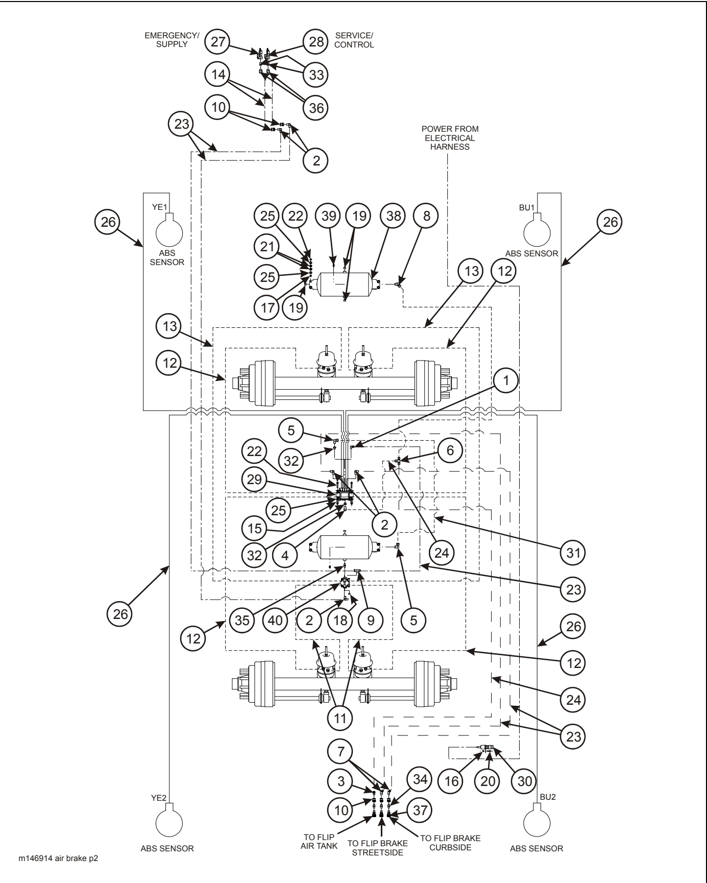
Figure 2-25: Air Brake System (835C w/ Flip Provision) (2 of 2)
