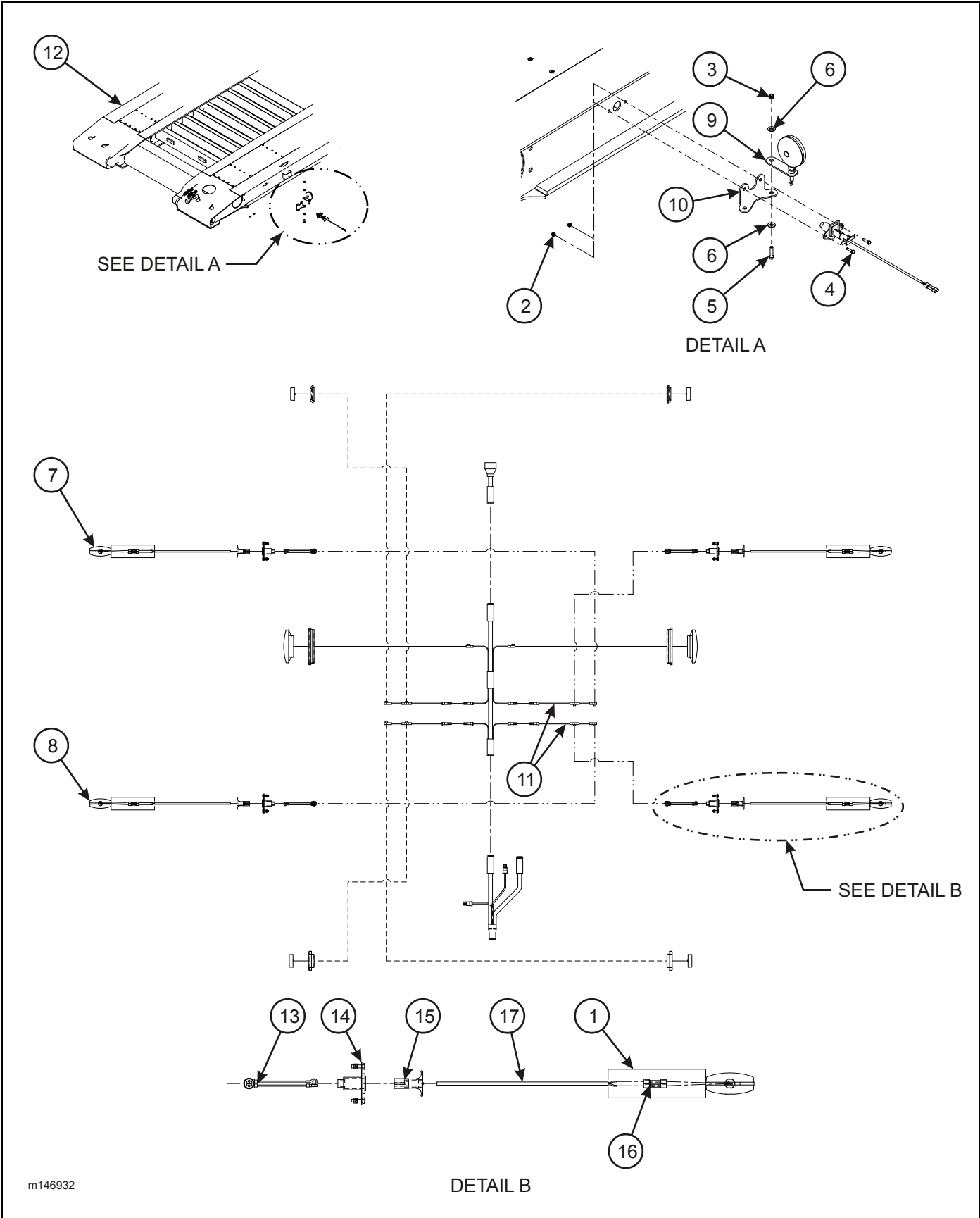
Figure 2-95: Web Mounted Four Corner Light Package (Option)
