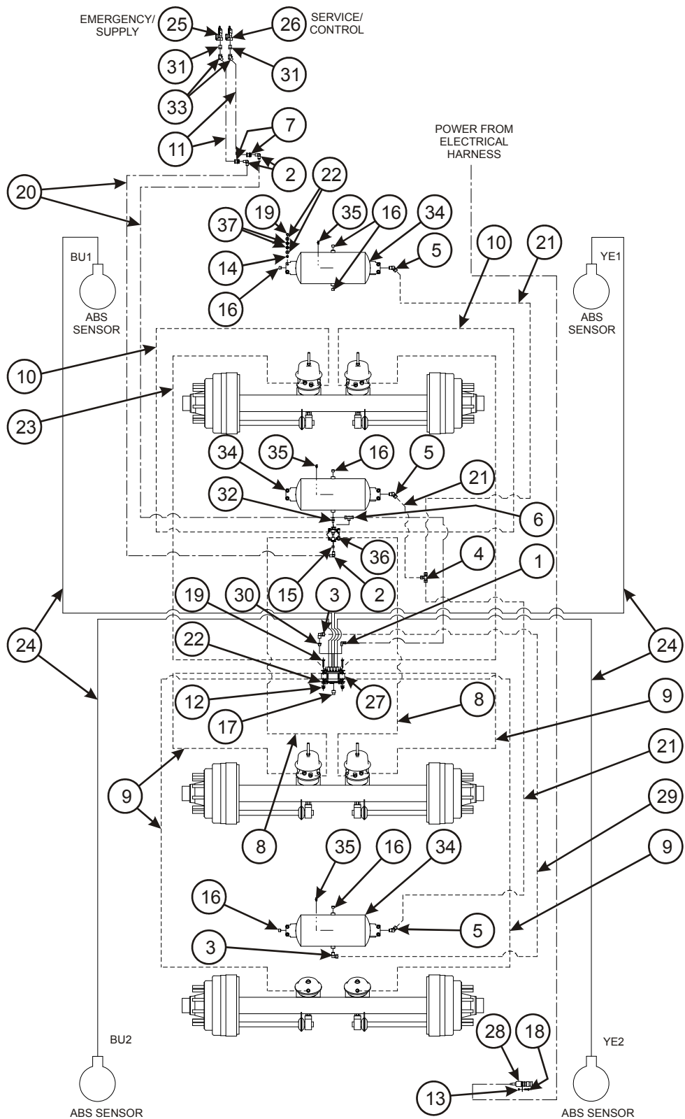
Figure 2-31: Air Brake System (835C Triple Axle) (3 of 3)
