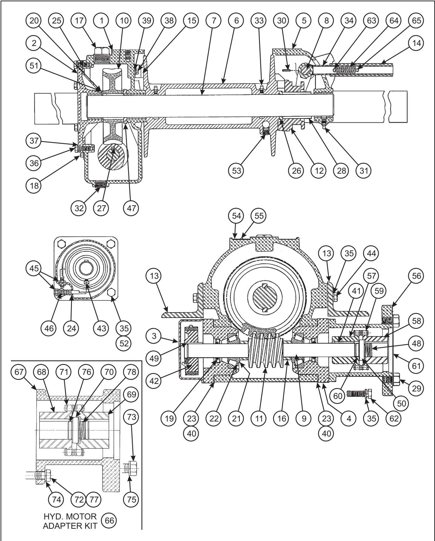
Figure 2-83: 12,000 Lb. Winch Assembly
