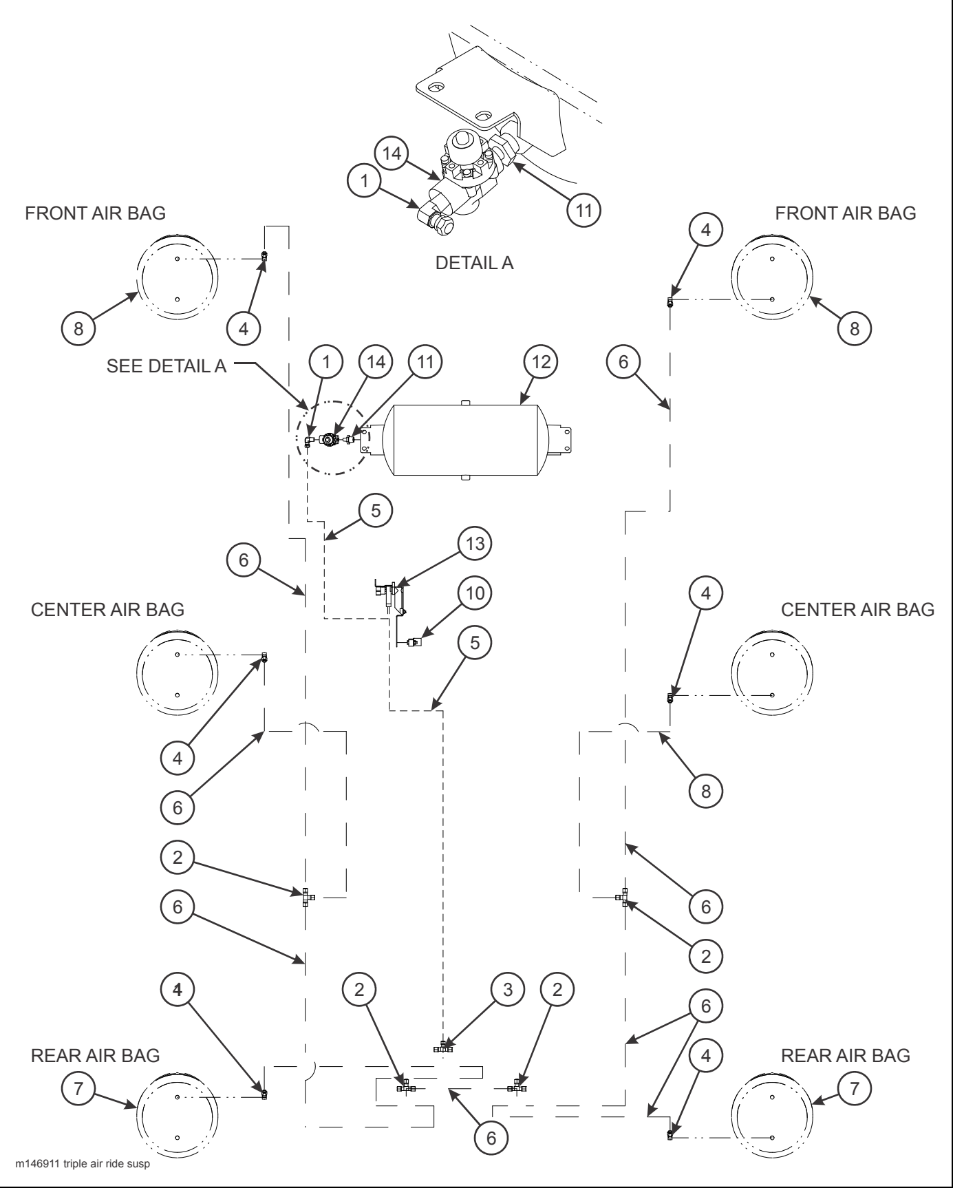
Figure 2-49: Frame Assembly - Air Ride Suspension (Triple) (835C)
