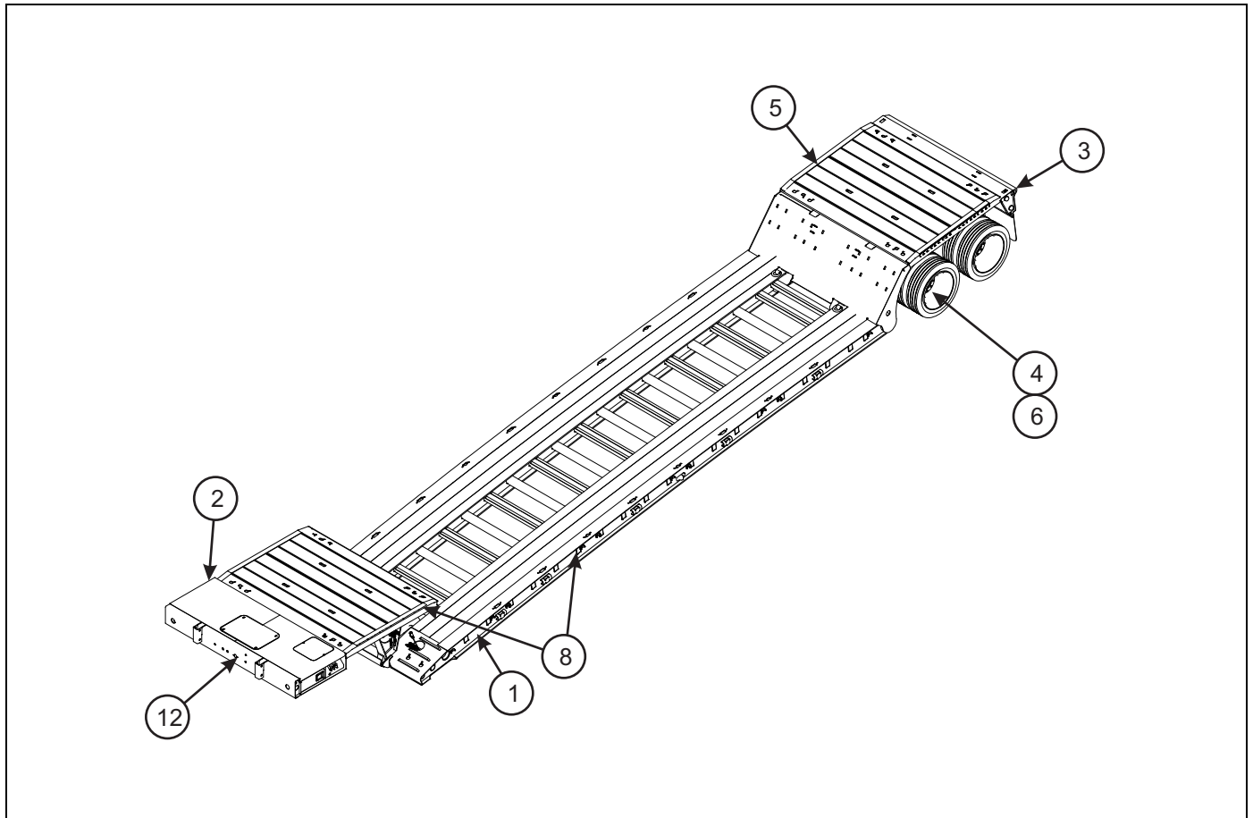
Figure 2-1: General Assembly
