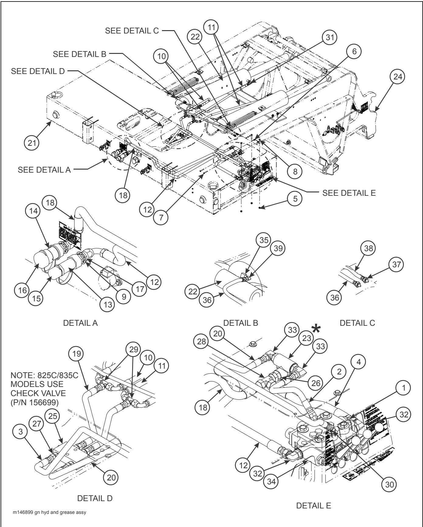
Figure 2-10: Gooseneck Hydraulic and Grease System (825C)
