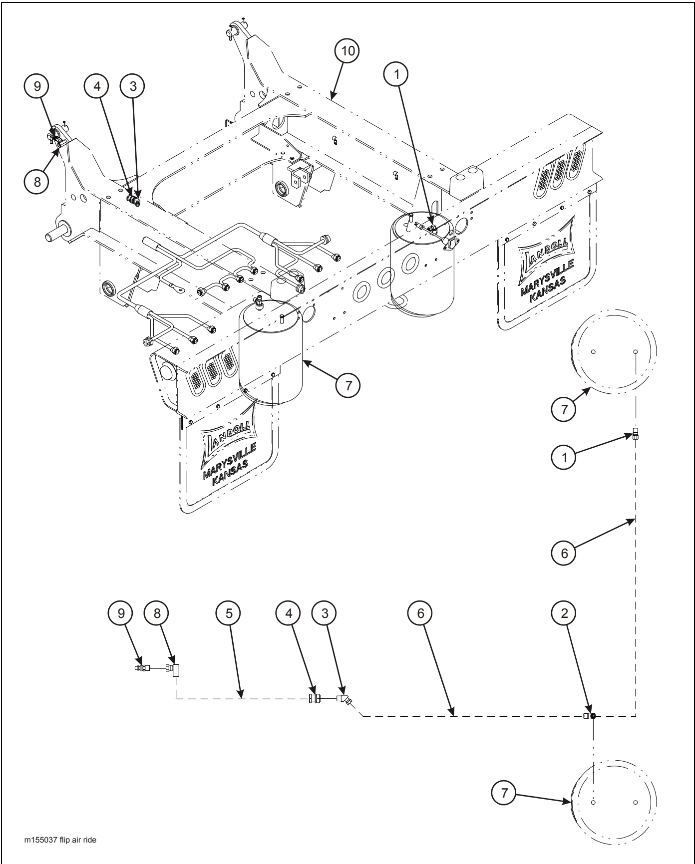
Figure 2-58: Flip Assembly - Air Ride Suspension
