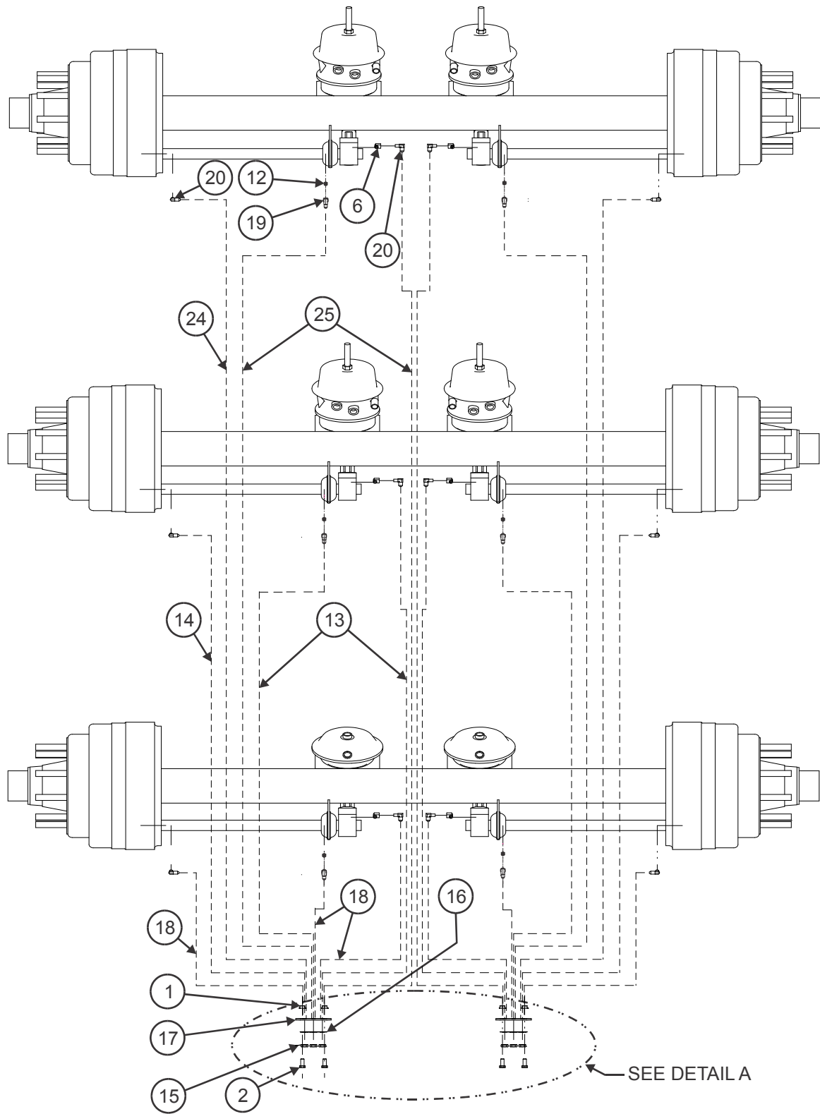
Figure 2-42: Frame Assembly and Grease System (835C - Triple) (4 of 5)
