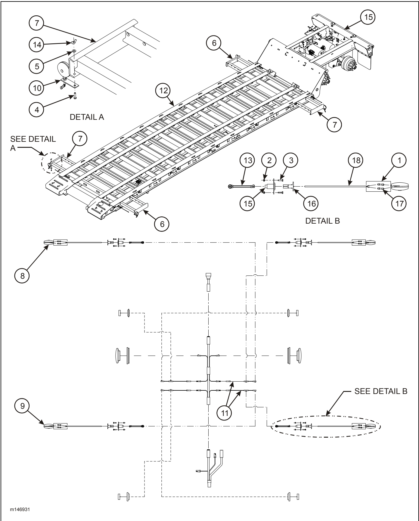
Figure 2-94: Pullout Extension Mounted Light Package (Option)
