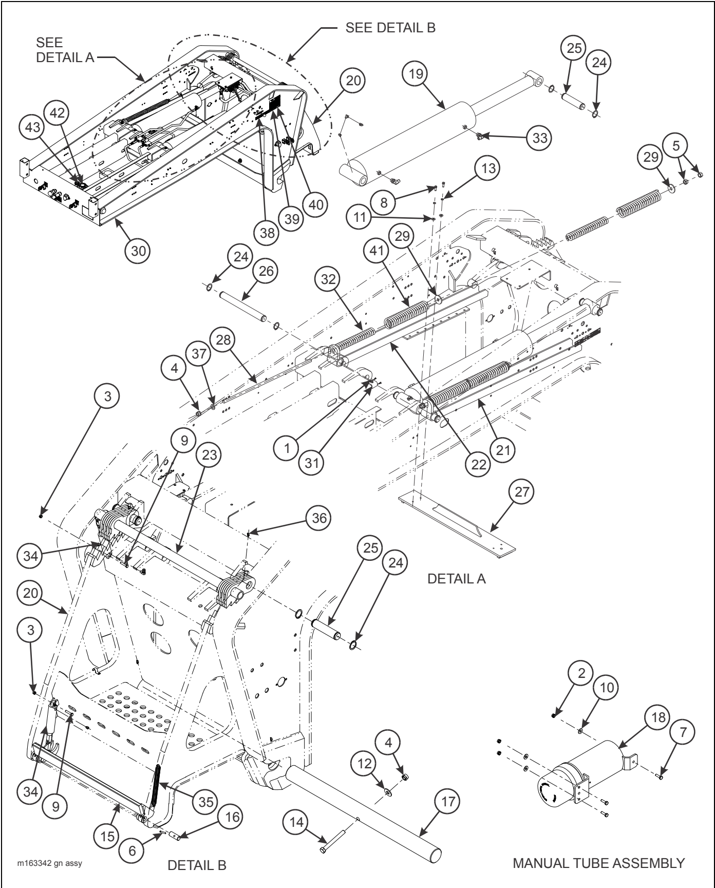
Figure 2-12: Gooseneck Assembly (855C)
