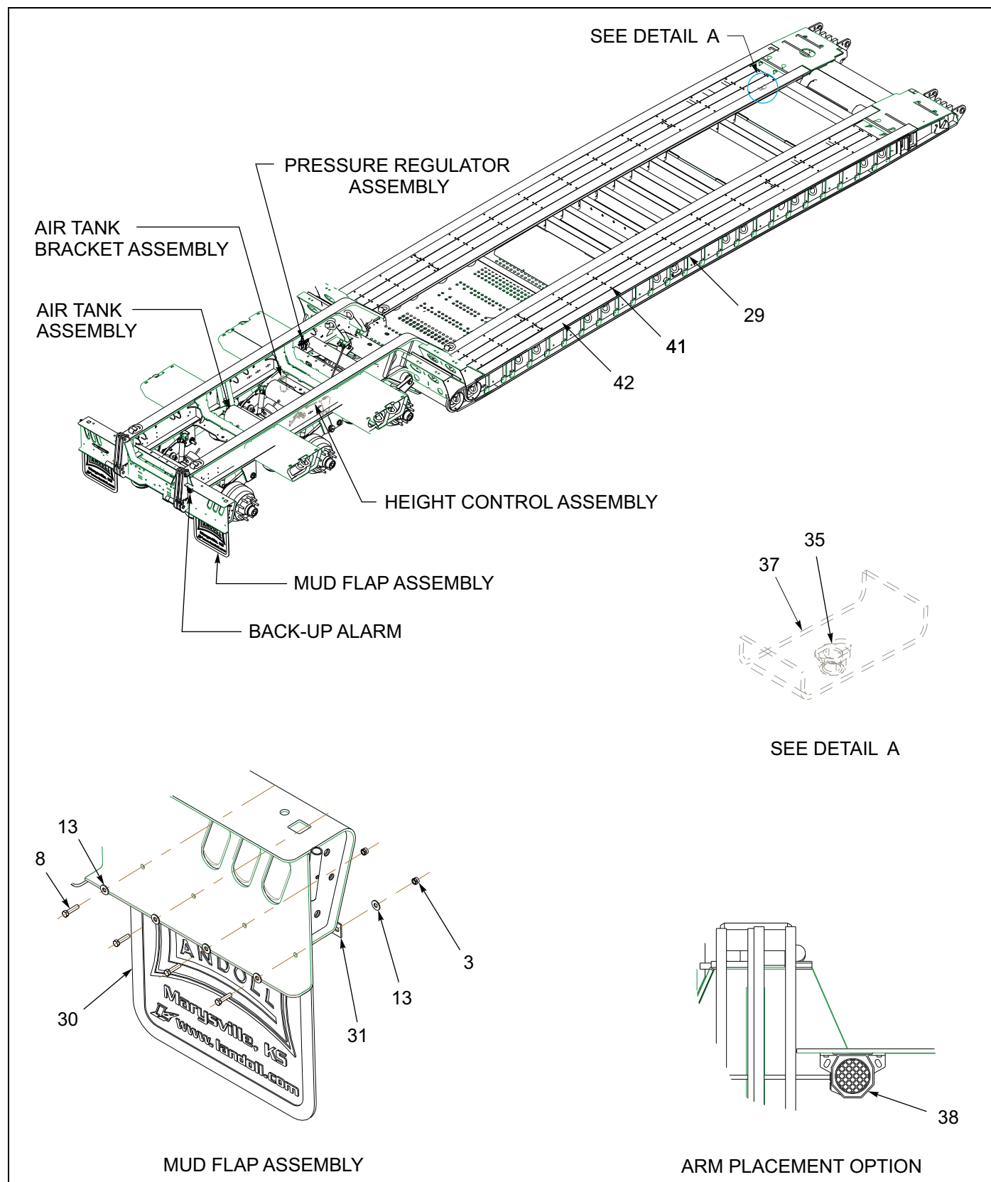
Figure 1-26: General Assembly - 855E (1 of 2)
