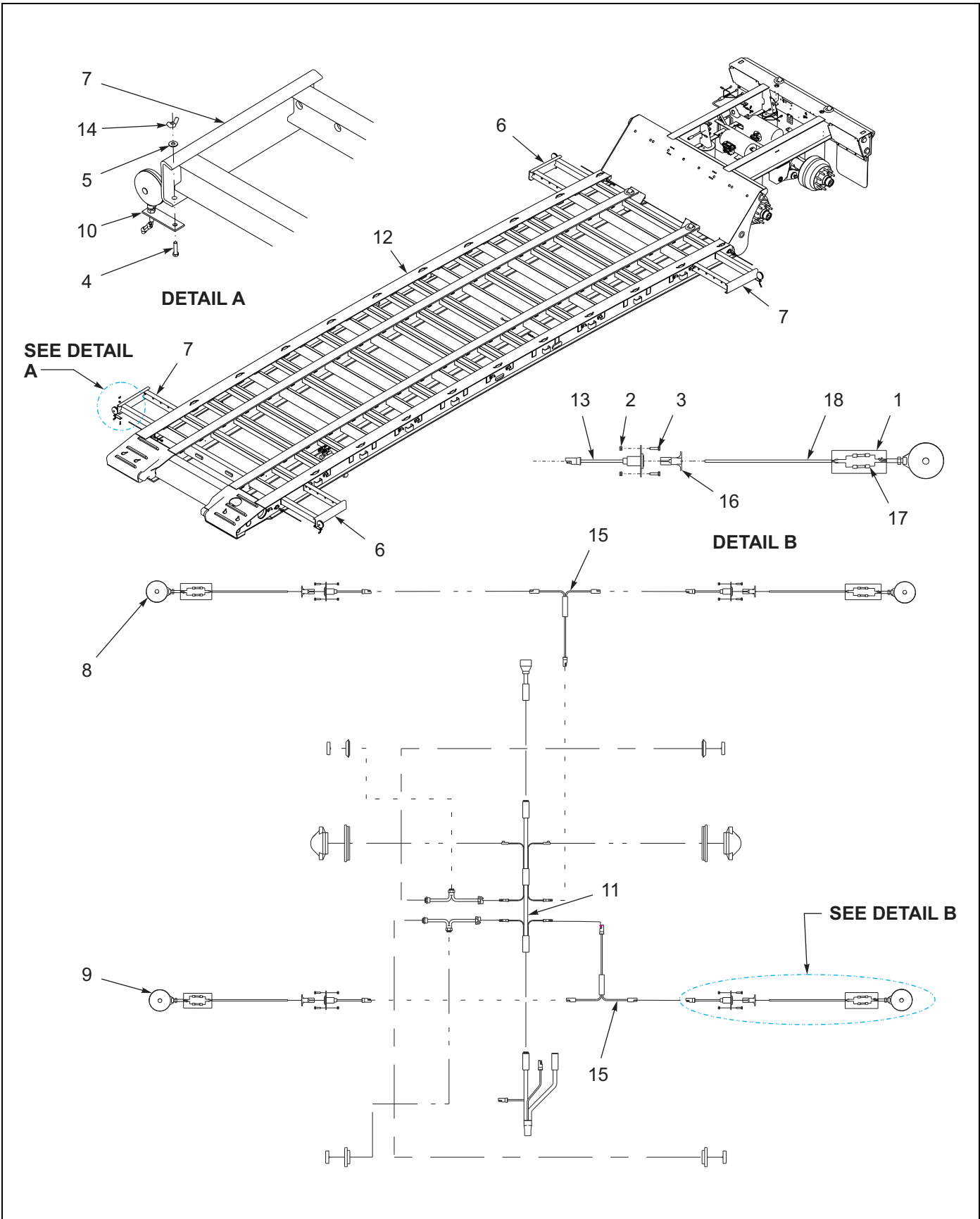
Figure 1-96: Pullout Extension Mounted Light Package
