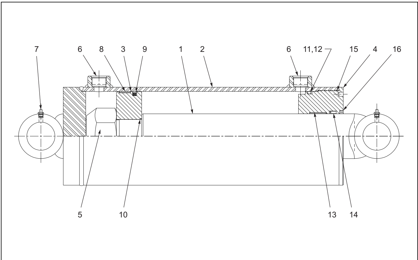
Figure 1-21: Hydraulic Cylinder 8 X 36
