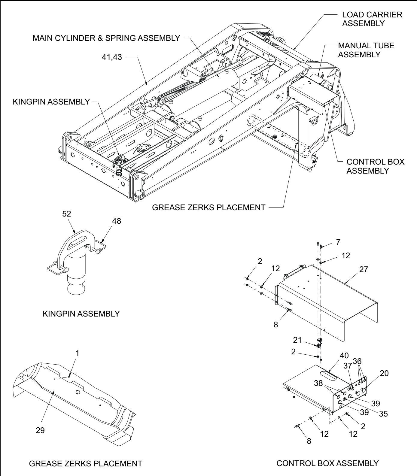
Figure 1-13: General Assembly - 855E HD (1 of 2)
