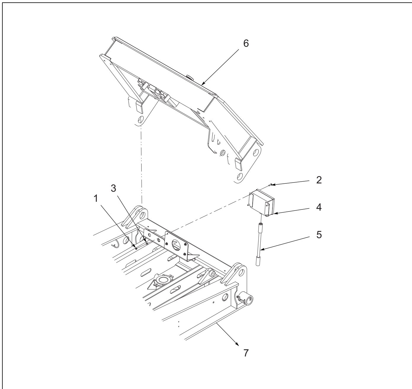
Figure 1-104: 24/12V Electrical Conversion Box Installation
