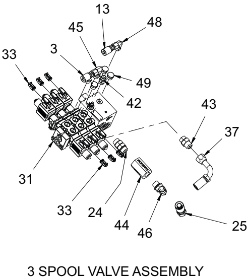
Figure 1-19: Hydraulic & Grease System - 855E HD (2 of 2)
