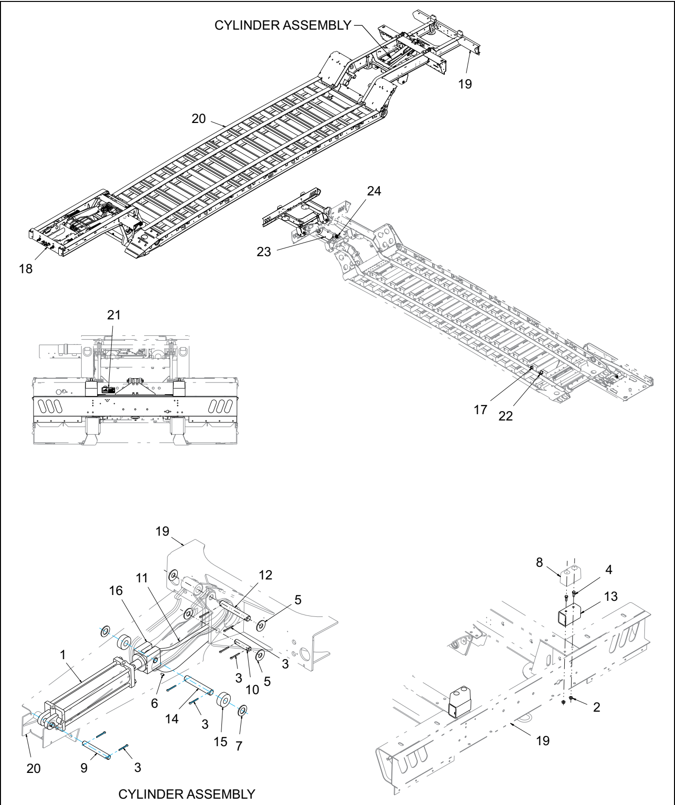
Figure 1-63: Frame & Cylinder Assembly
