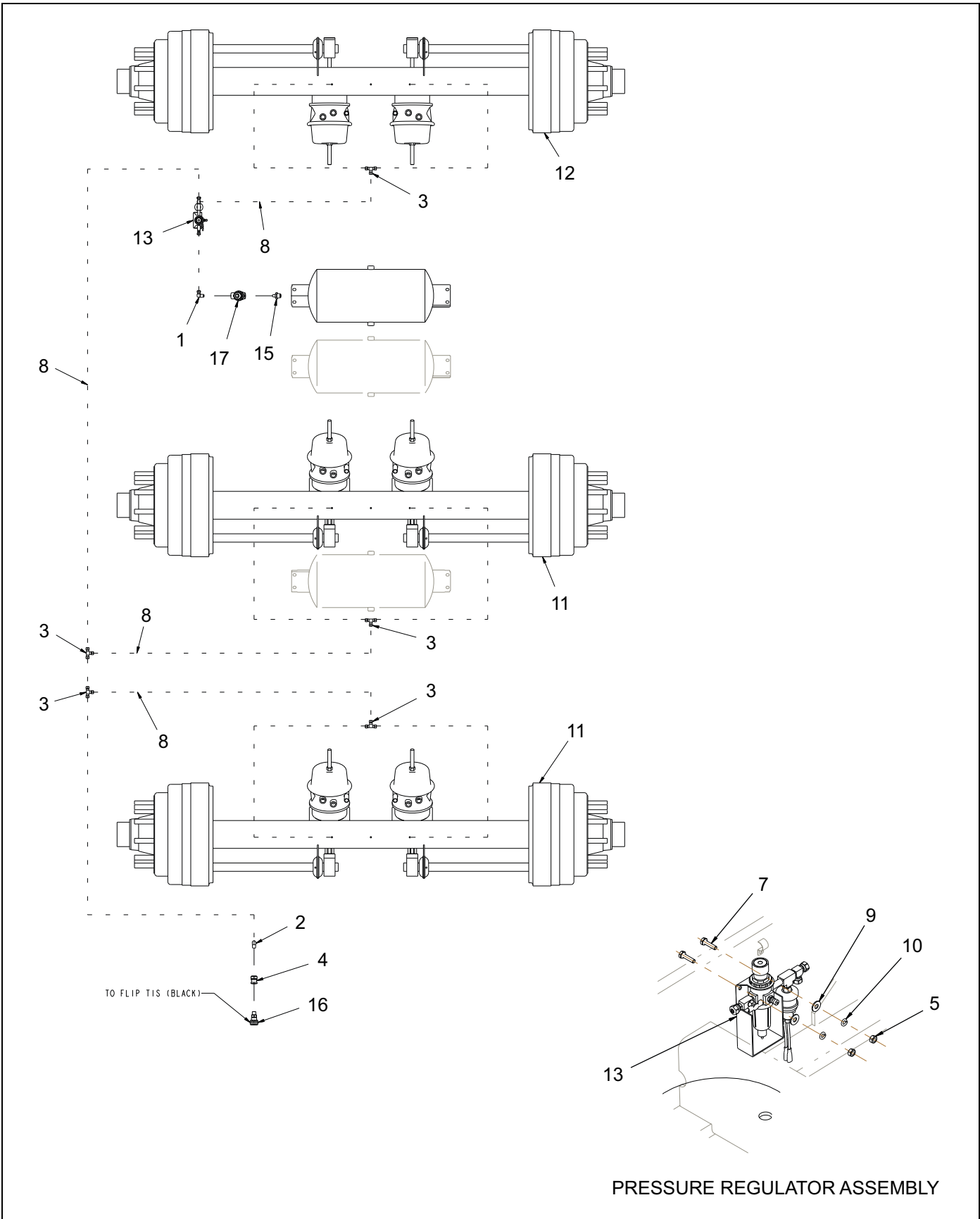
Figure 1-32: Tire Inflation System - 855E
