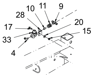
BRAKE PROTECTION VALVE FITTING ASSEMBLY
