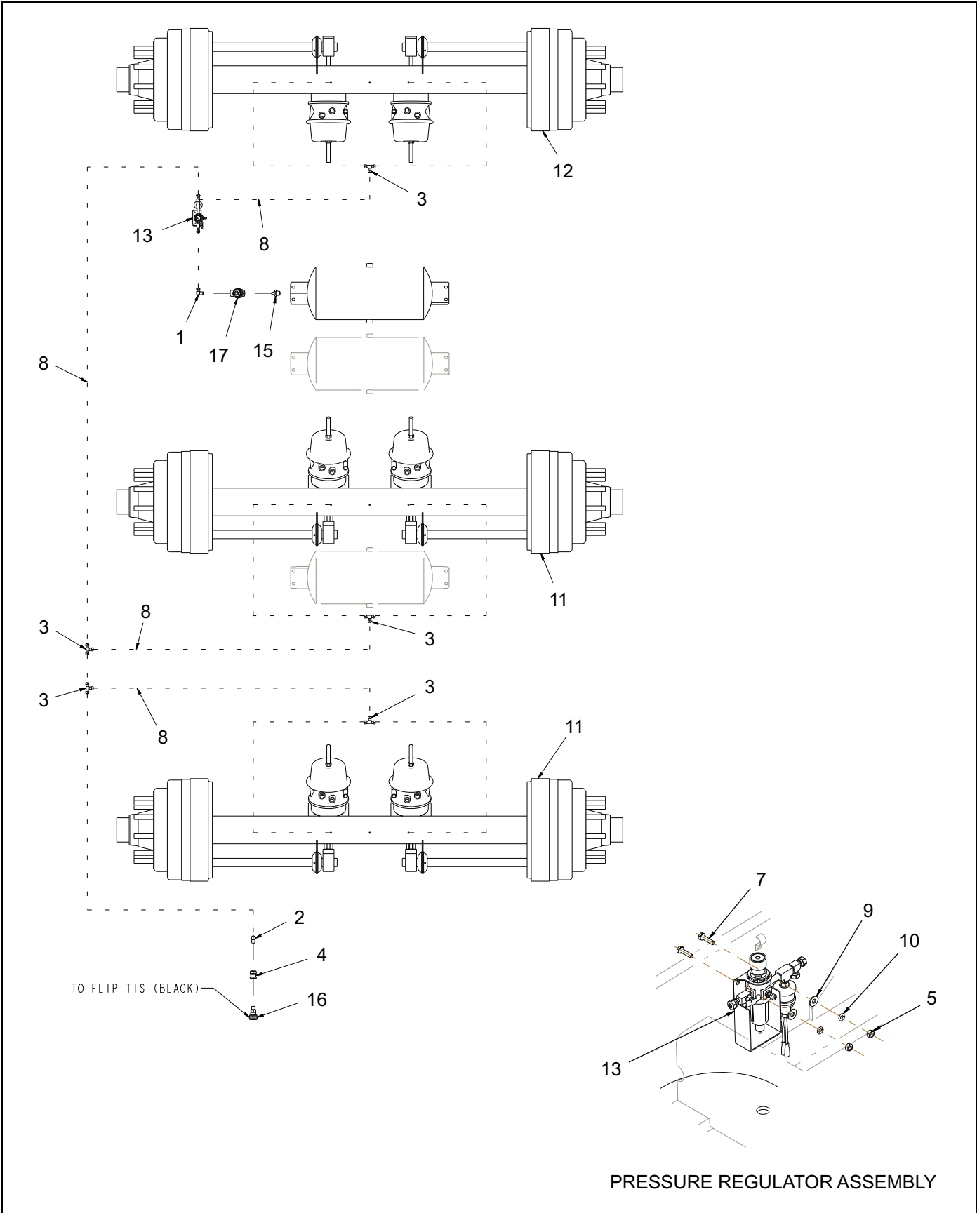
Figure 1-40: Tire Inflation System - 855E HD {P/N 198492, 198493, 198494, 198515, & 198516} (1 of 2)
