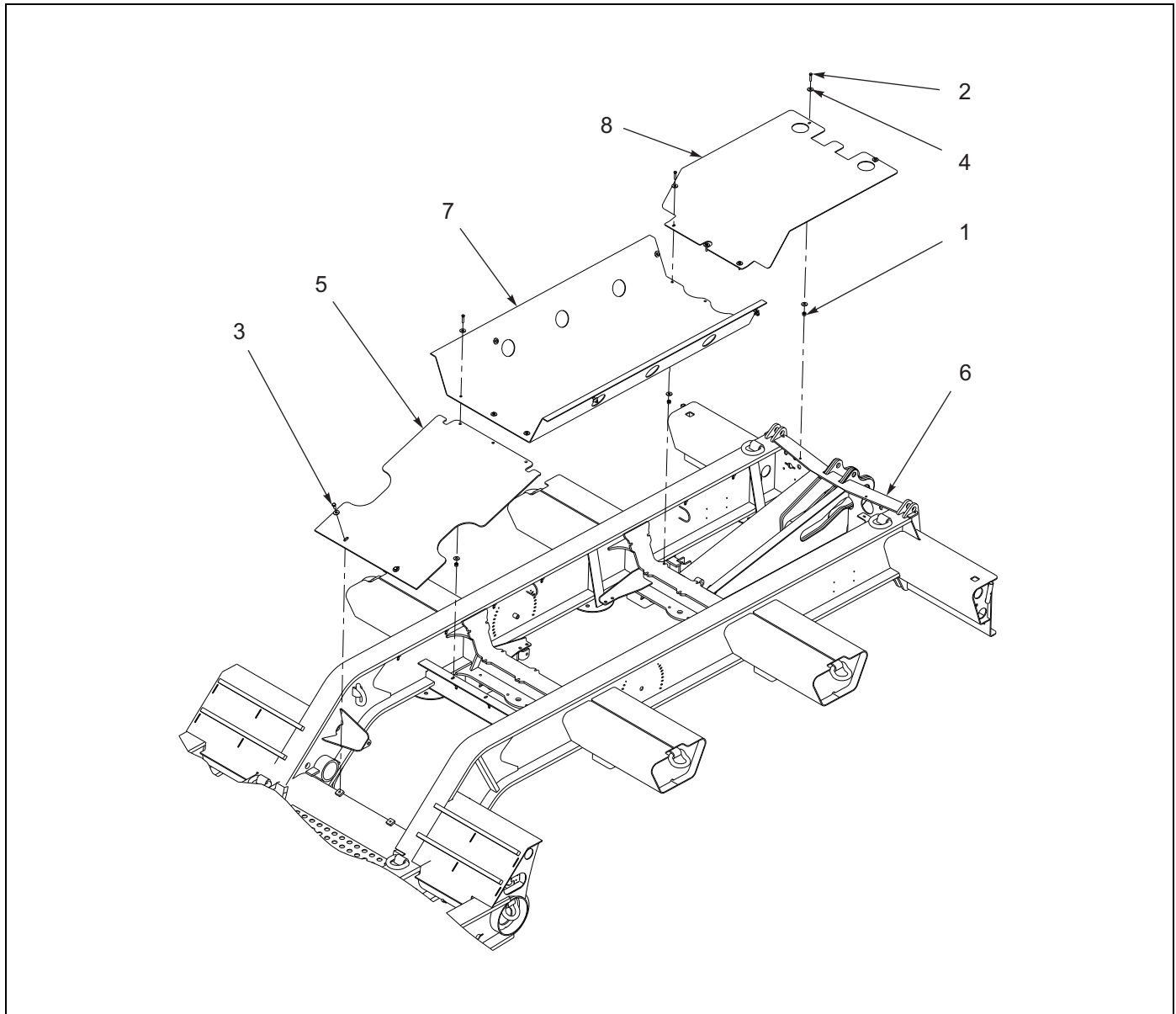
Figure 1-71: Cover Boom Trough Assembly - Flip
