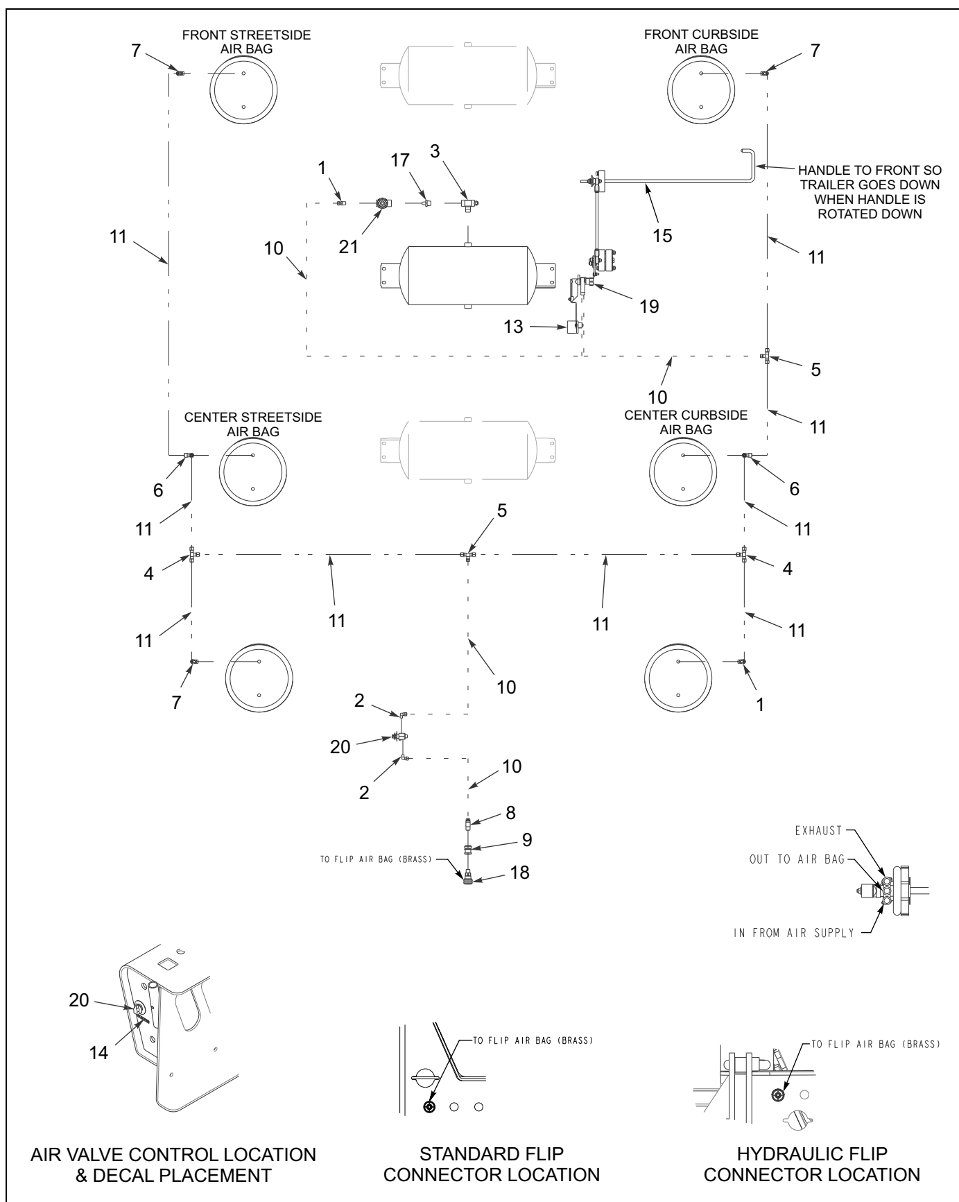
Figure 1-38: Air Ride Suspension - 855E HD
