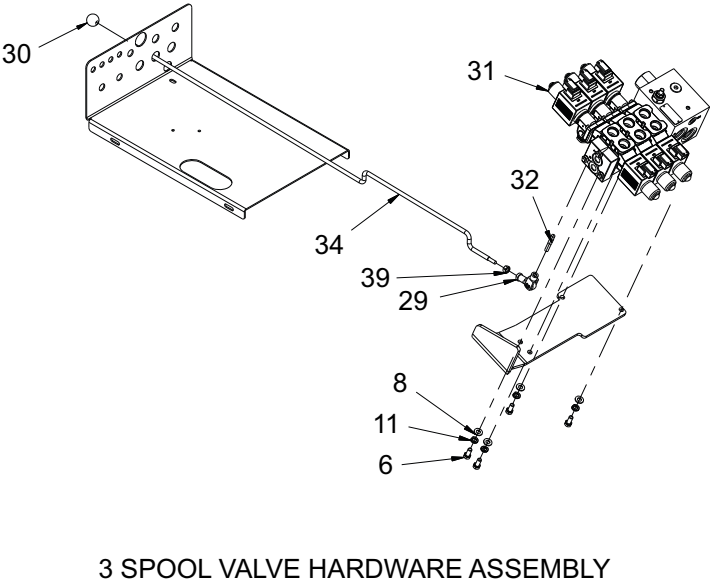
Figure 1-19: Hydraulic & Grease System - 855E HD (2 of 2)
