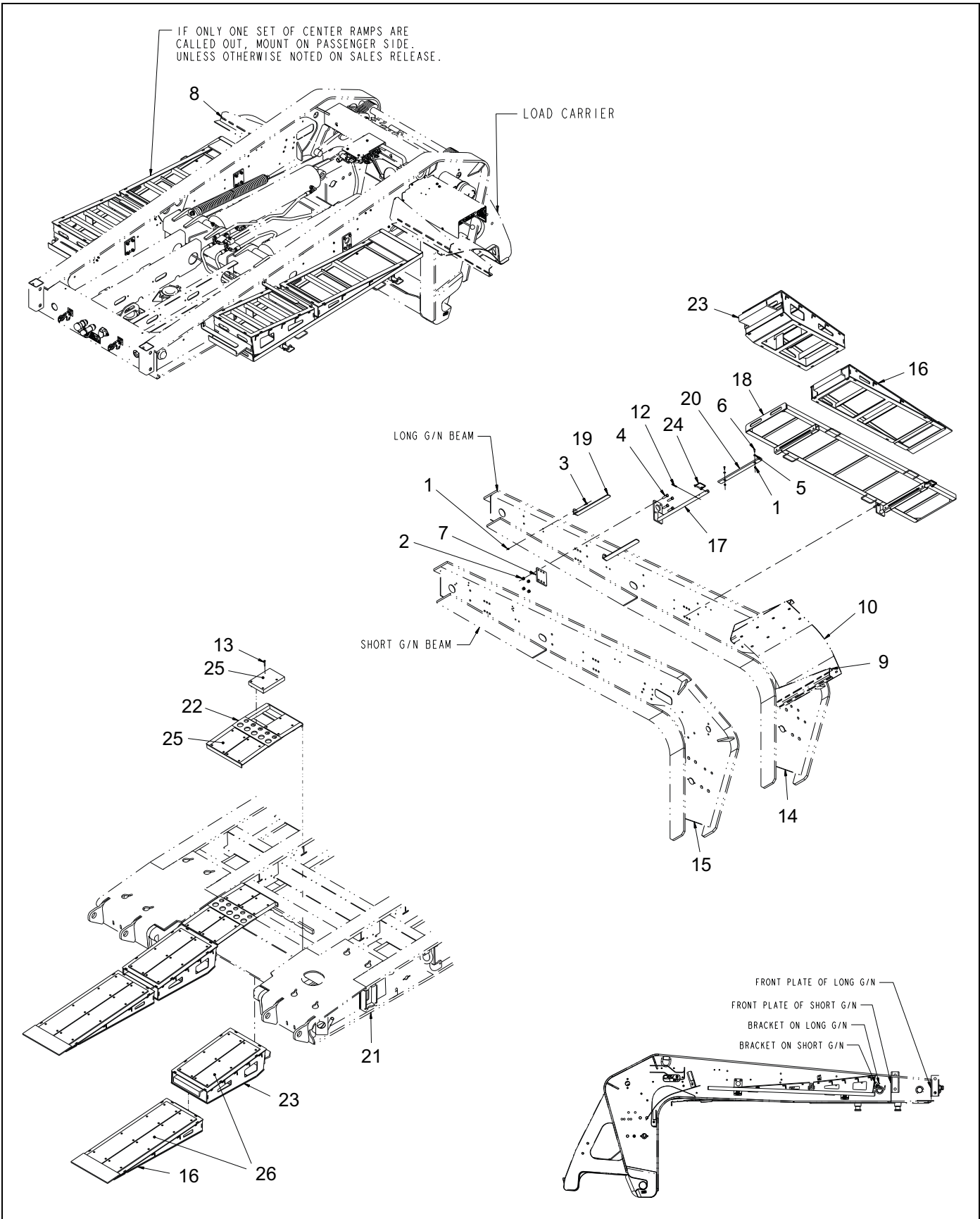
Figure 1-56: Ramp Assembly - Front Center (855E Paver)
