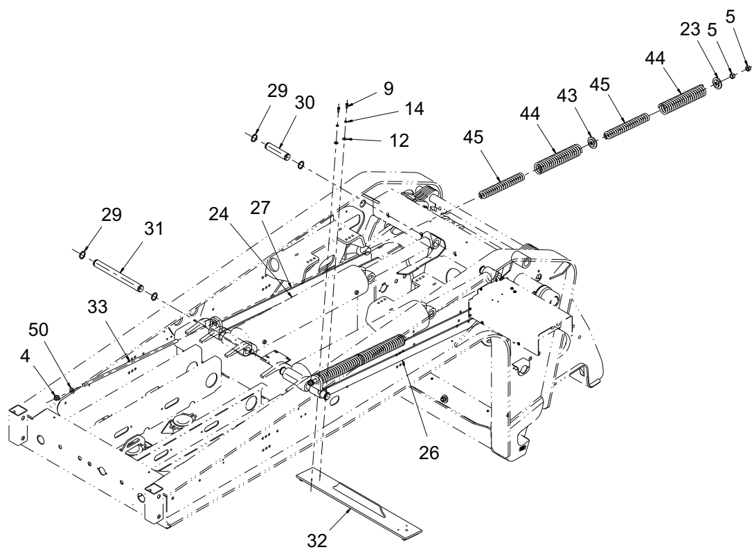
MAIN CYLINDER & SPRING ASSEMBLY
