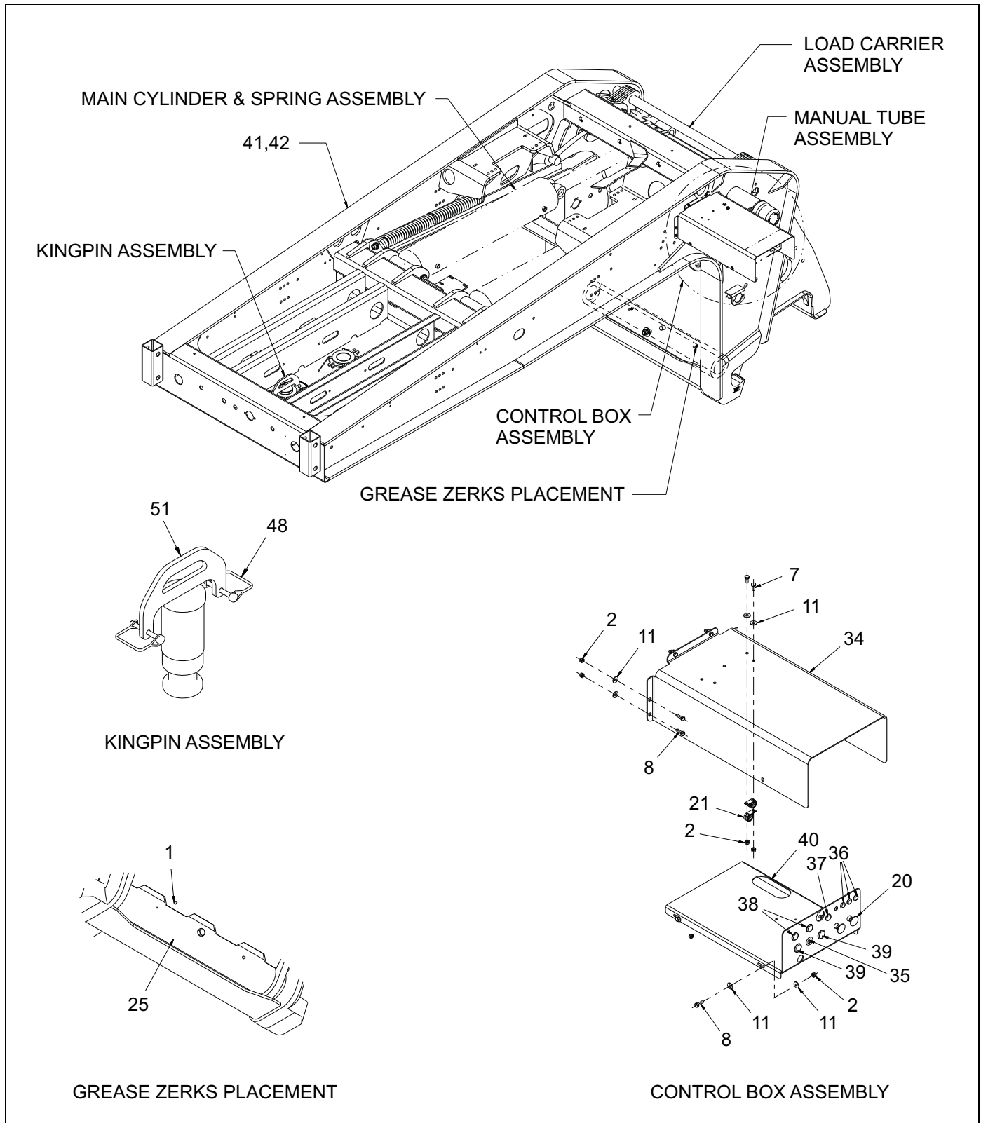
Figure 1-6: General Assembly - 855E (1 of 2)
