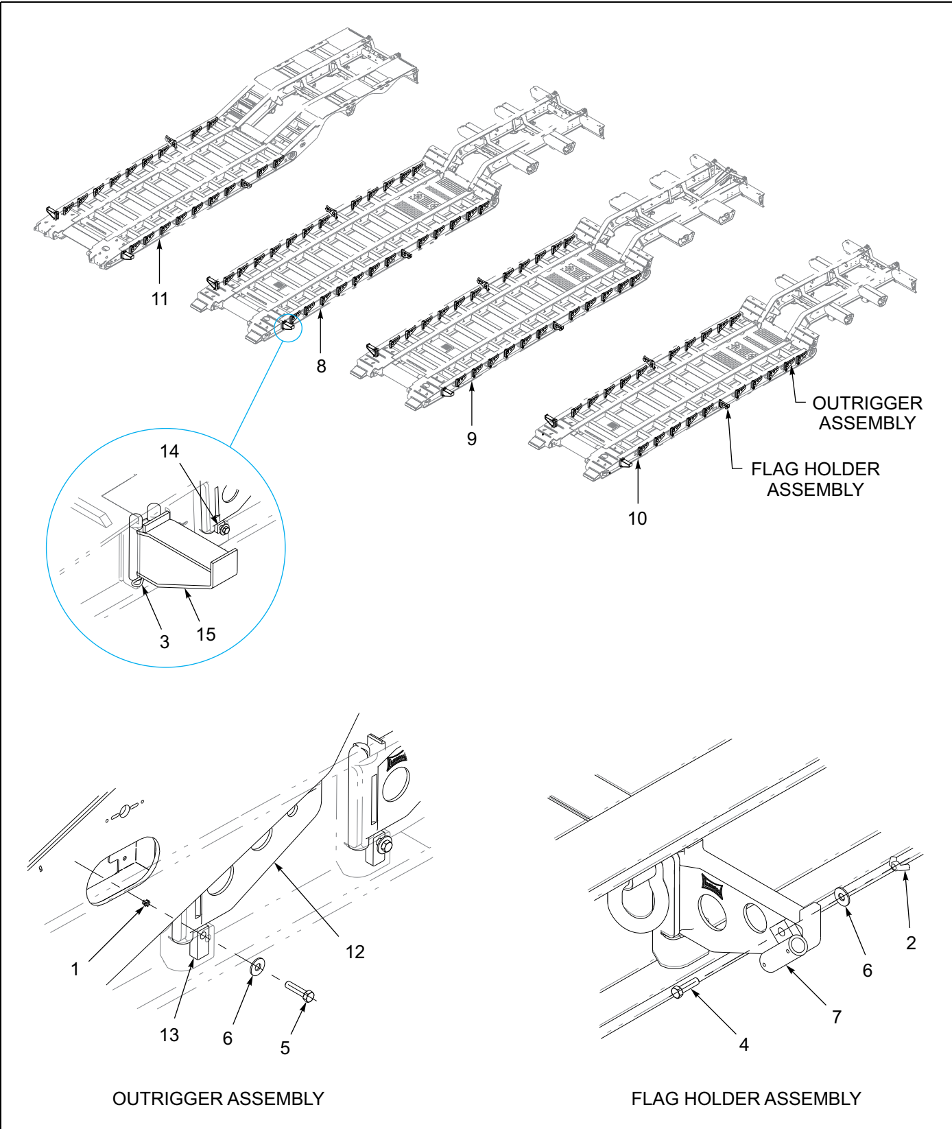
Figure 1-66: Swing Out Installation
