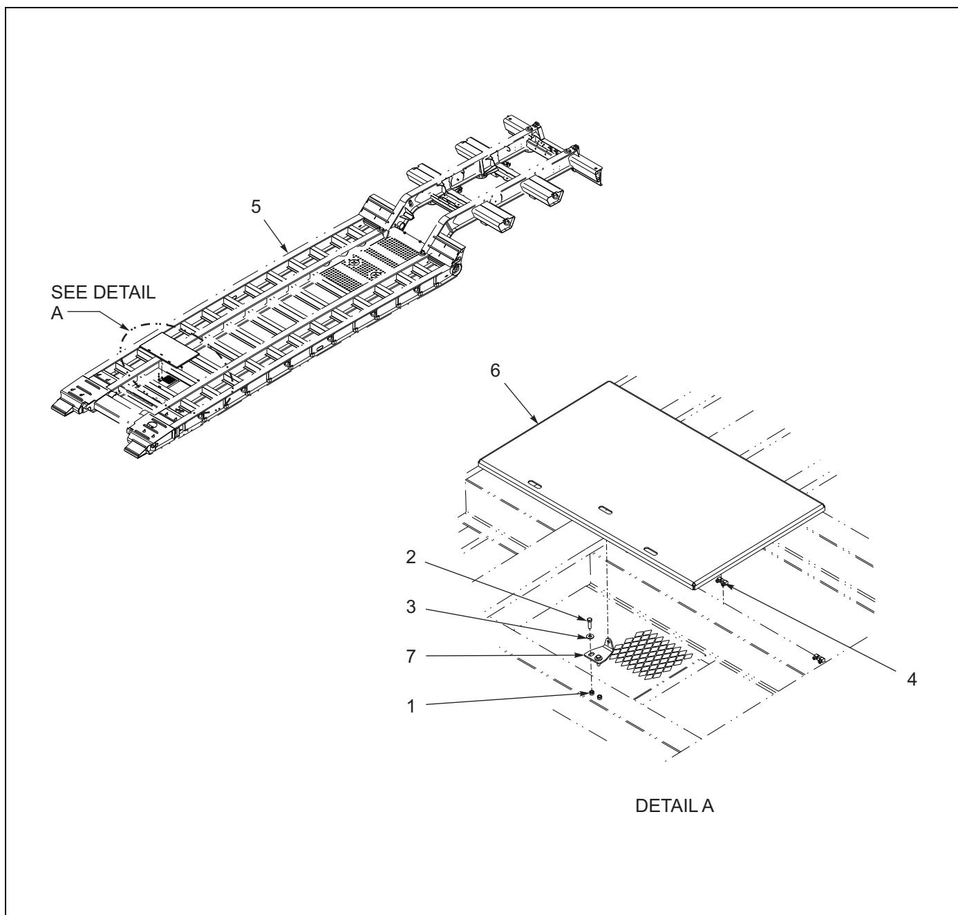
Figure 1-114: Lid Assembly - Storage Area Center
