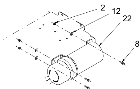
MANUAL TUBE ASSEMBLY
