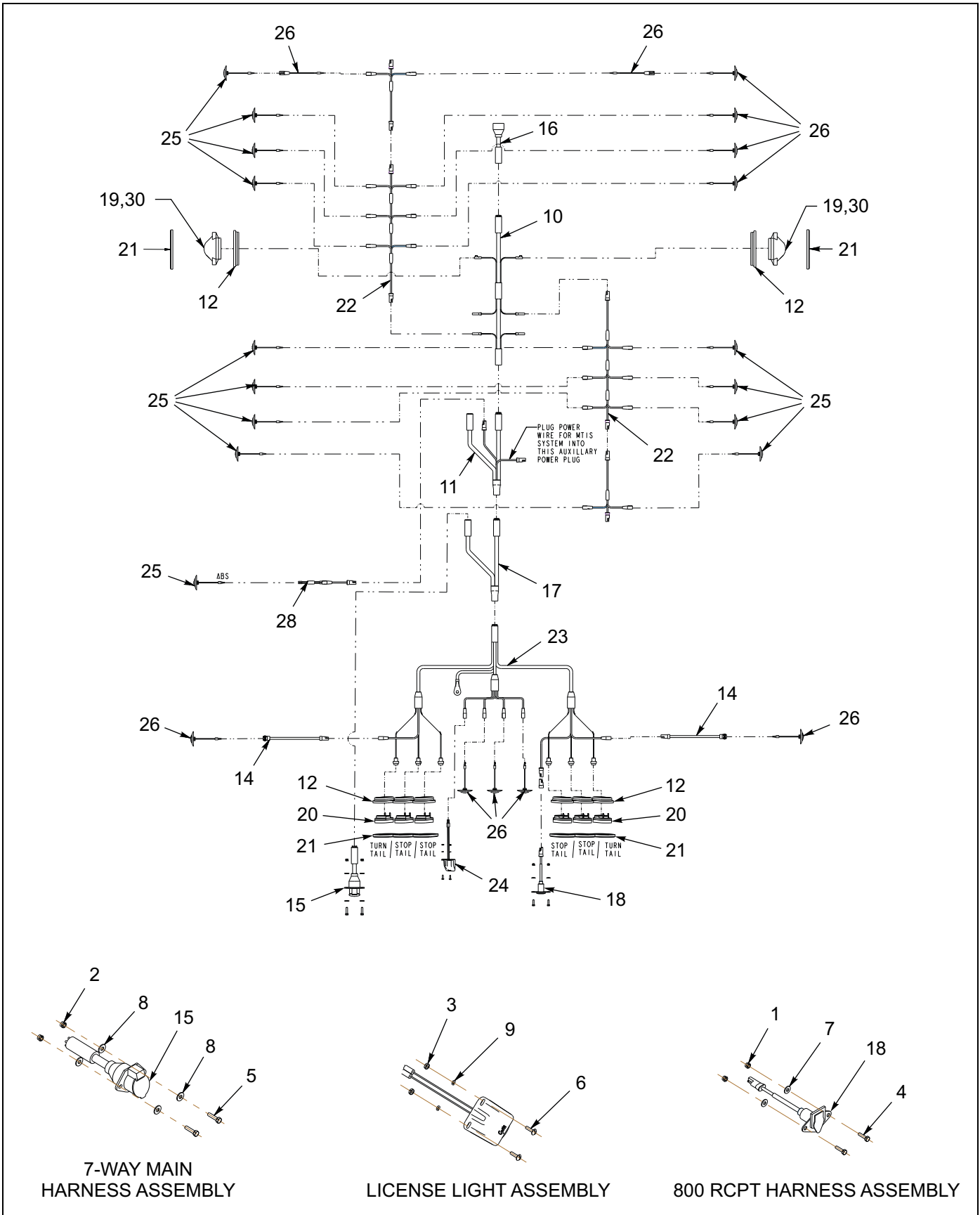
Figure 1-44: Electrical System - 855E Paver
