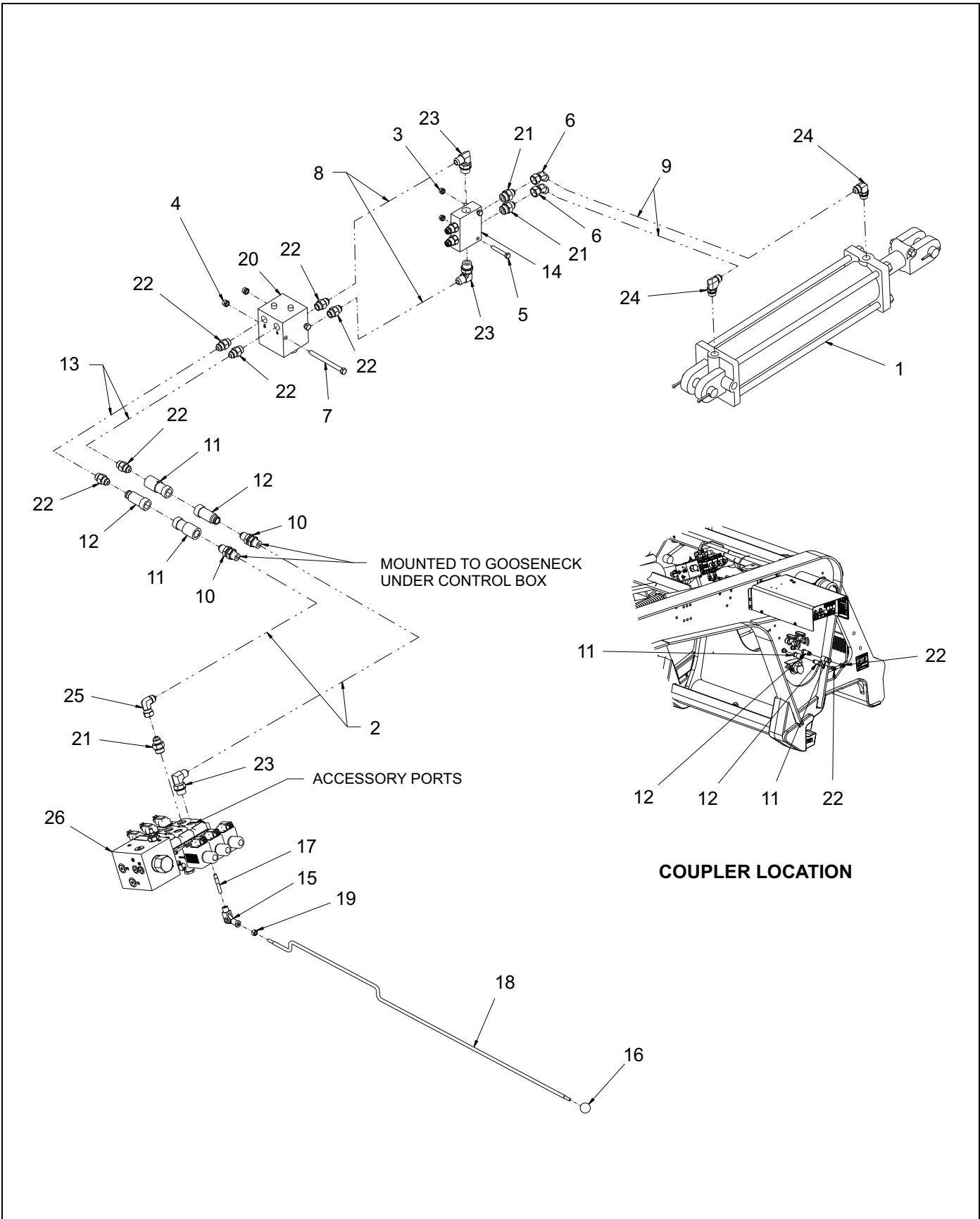
Figure 1-64: Hydraulic System
