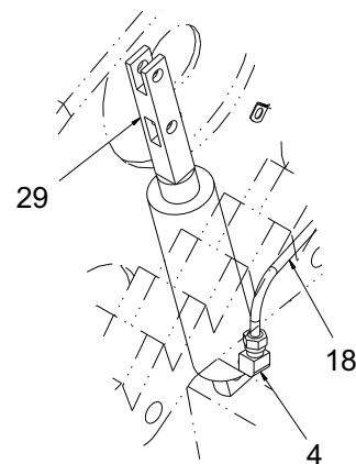
LOAD RATCHET CYLINDER ASSEMBLY
