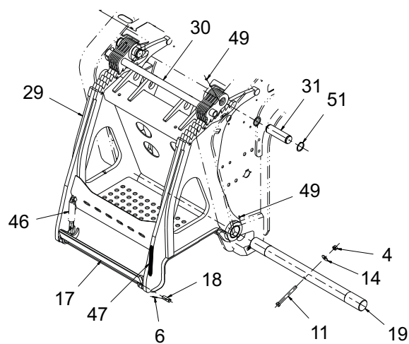
LOAD CARRIER ASSEMBLY
