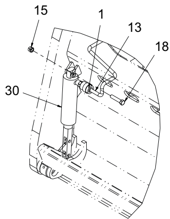
CARRIER LOCK CYLINDER ASSEMBLY
