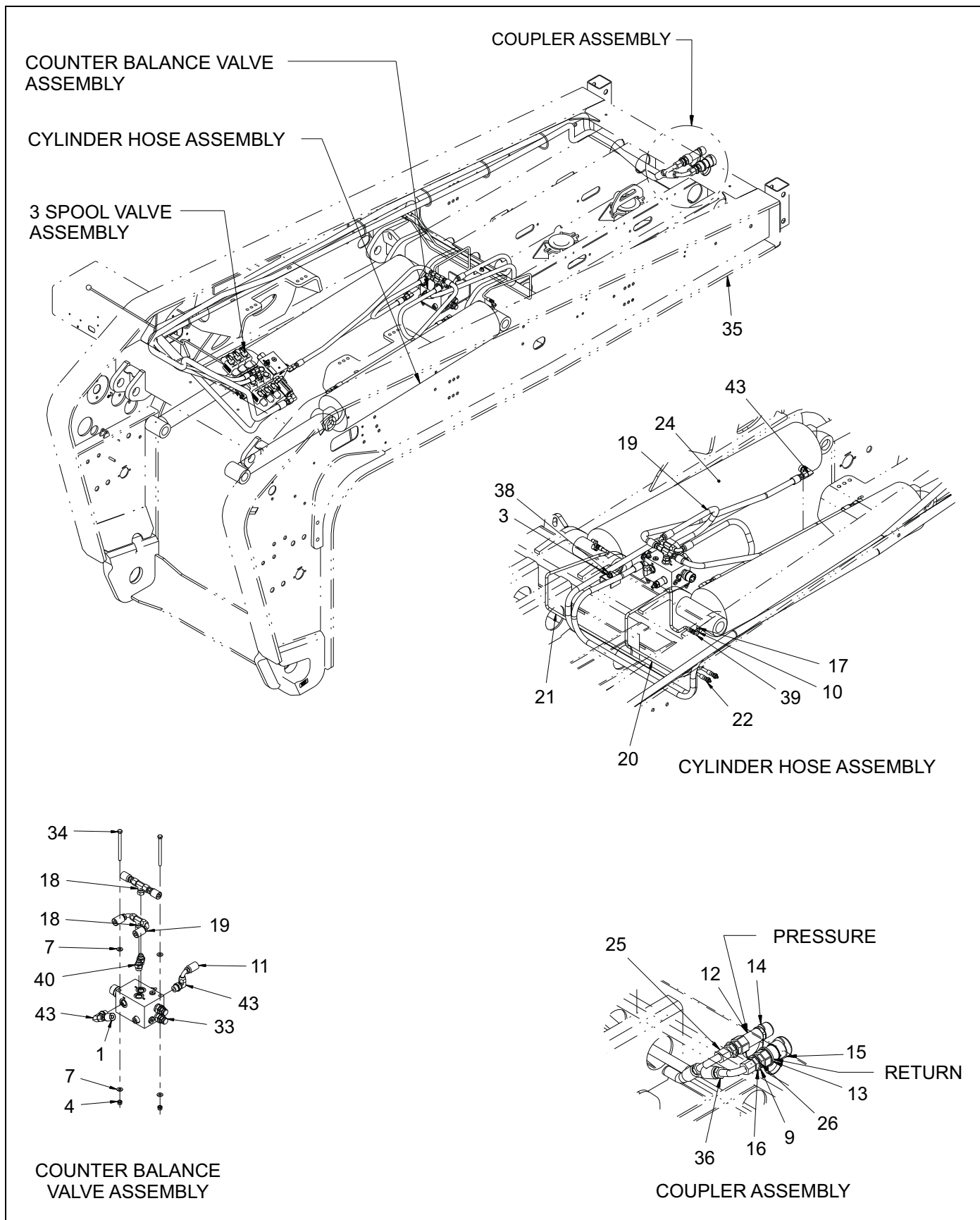
Figure 1-11: Hydraulic & Grease System - 855E (1 of 2)
