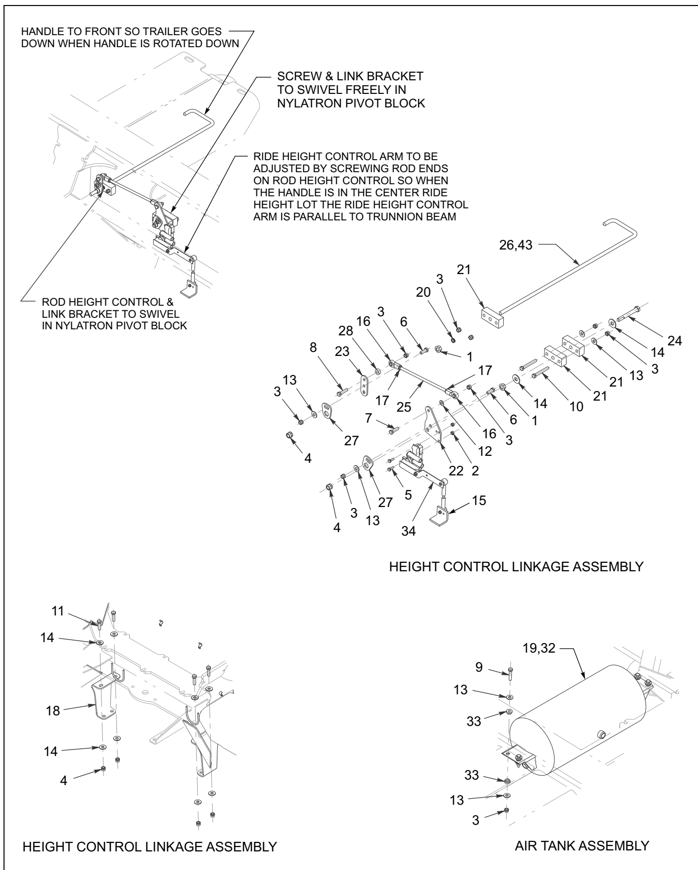
Figure 1-34: General Assembly - 855E HD (2 of 2)
