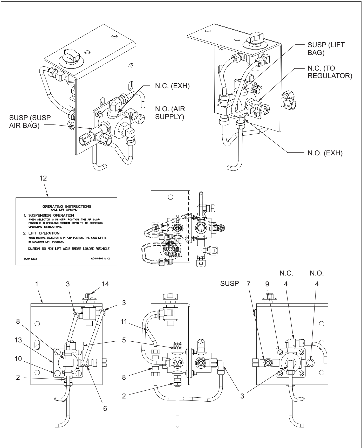
Figure 1-93: Lift Axle (Flip) Control Assembly
