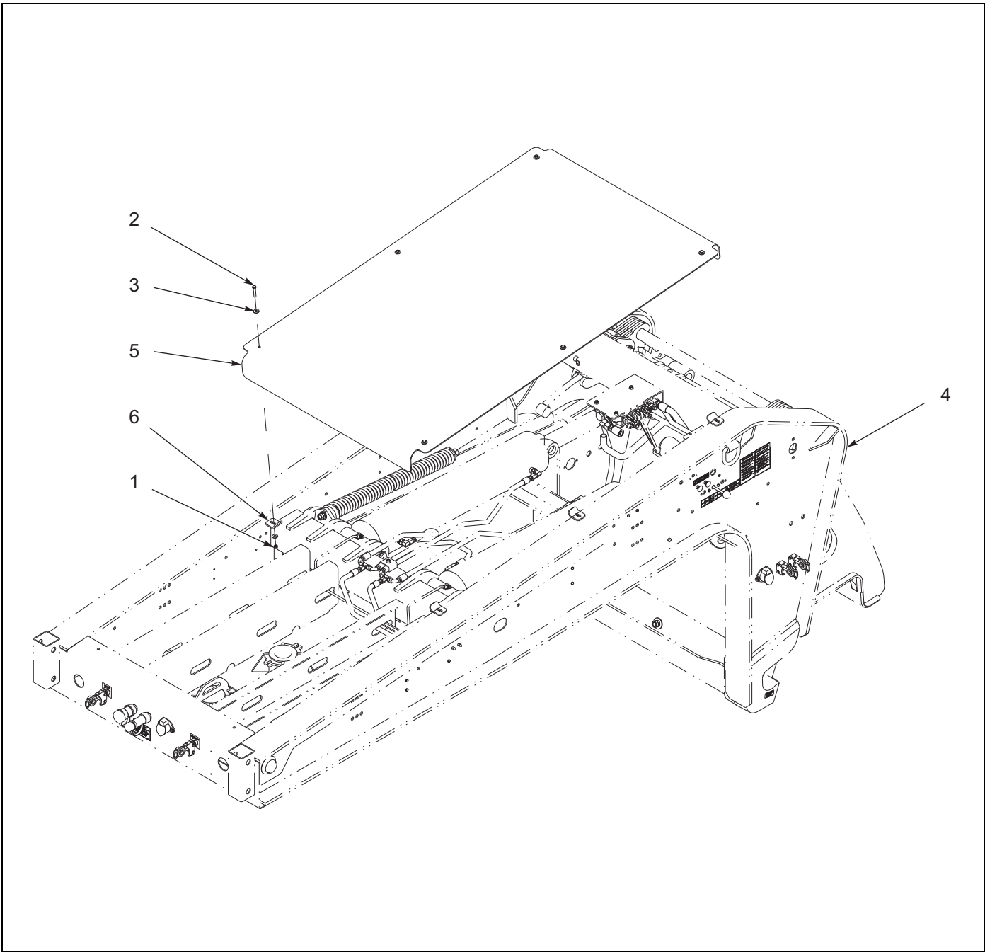
Figure 1-72: Gooseneck Cover Assembly - 855E
