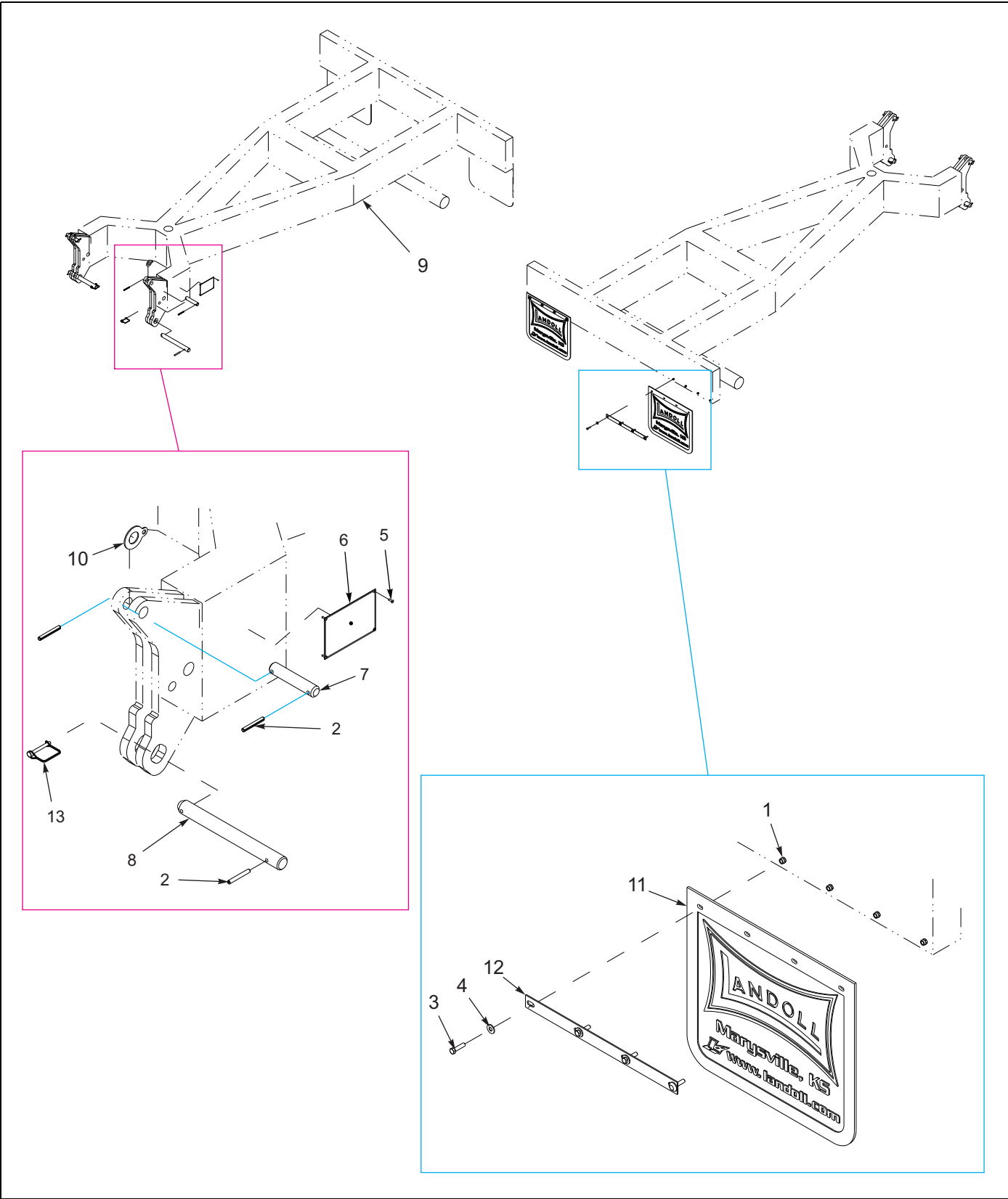
Figure 1-68: Stinger Assembly - 855E HD
