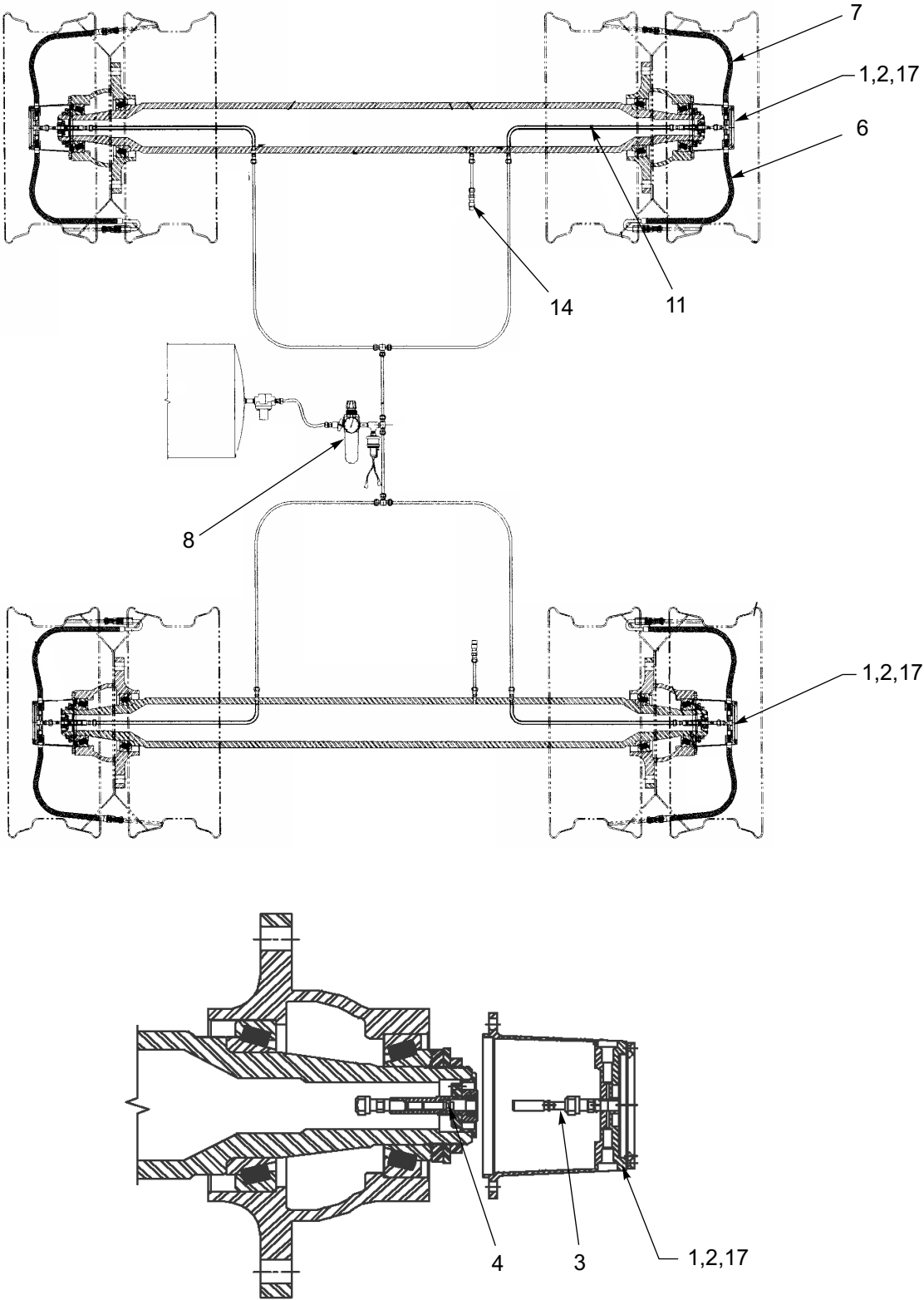
Figure 1-117: Tire Inflation System
