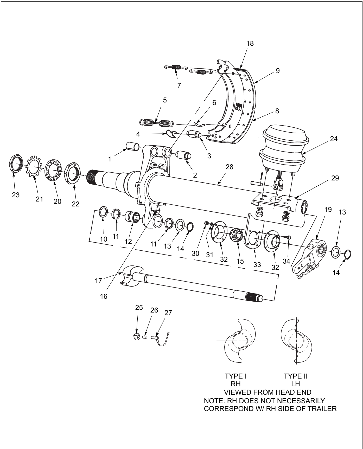
Figure 1-53: Axle and Brake Assembly - Dexter 16-1/2" X 7"
