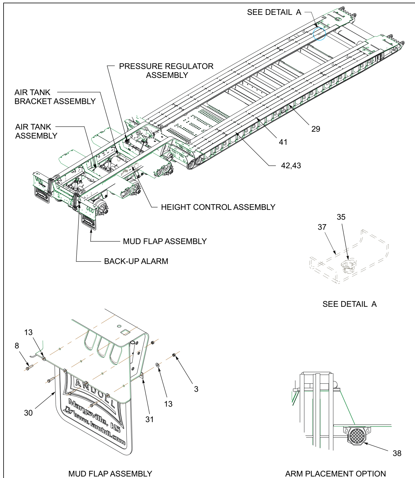
Figure 1-42: General Assembly - 855E Paver (1 of 2)
