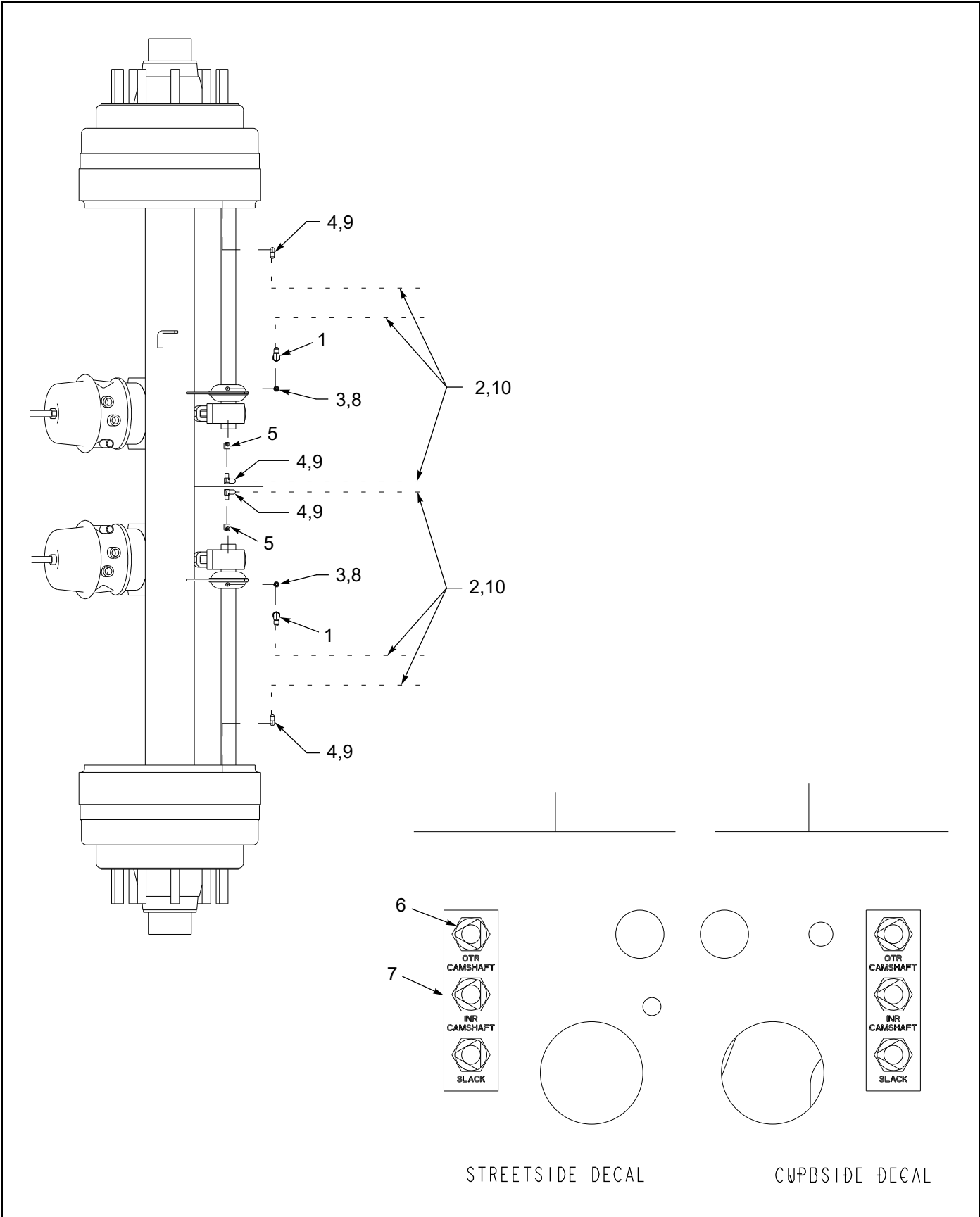
Figure 1-61: Grease Assembly
