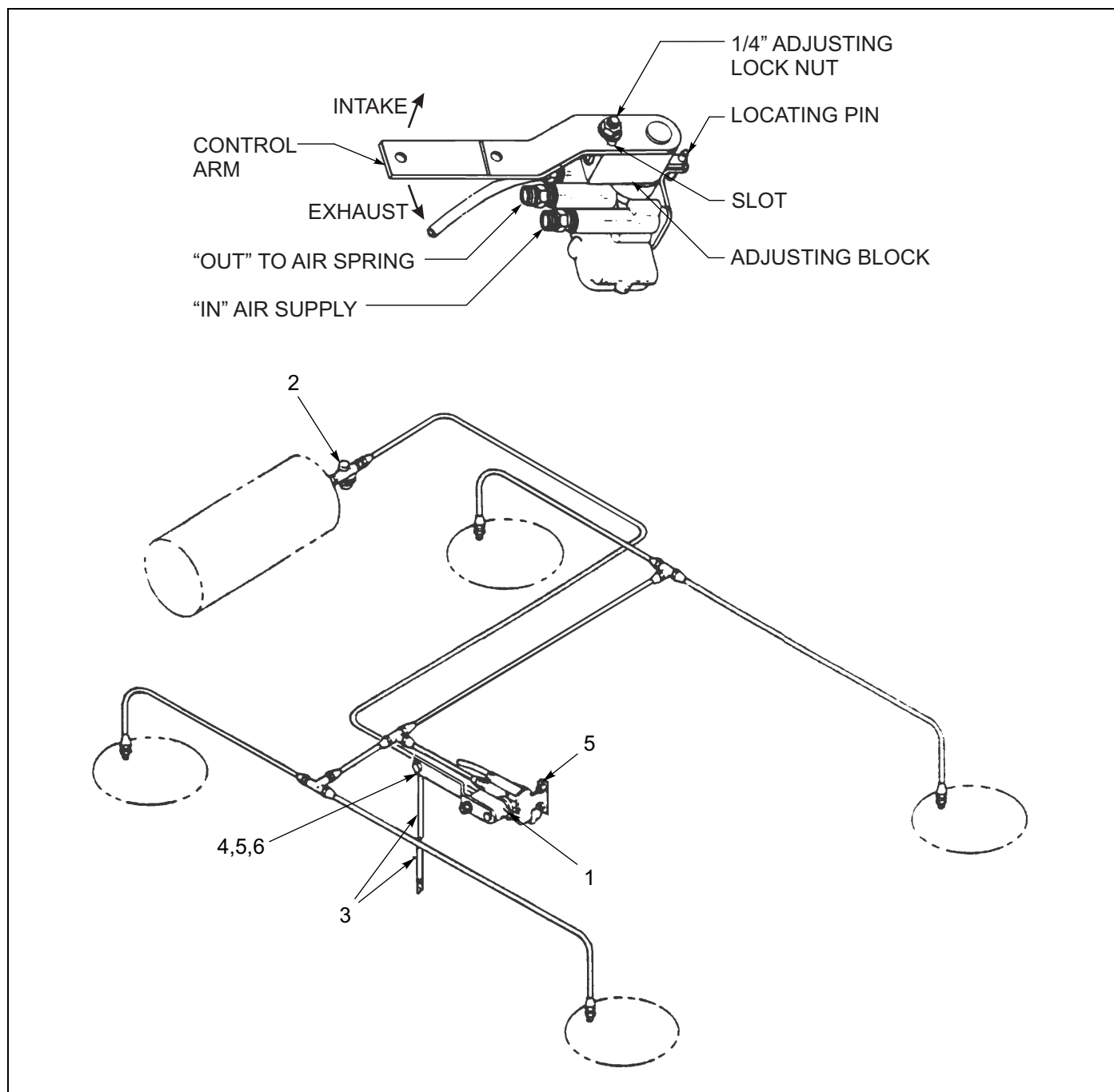
Figure 1-50: Air Control Kit
