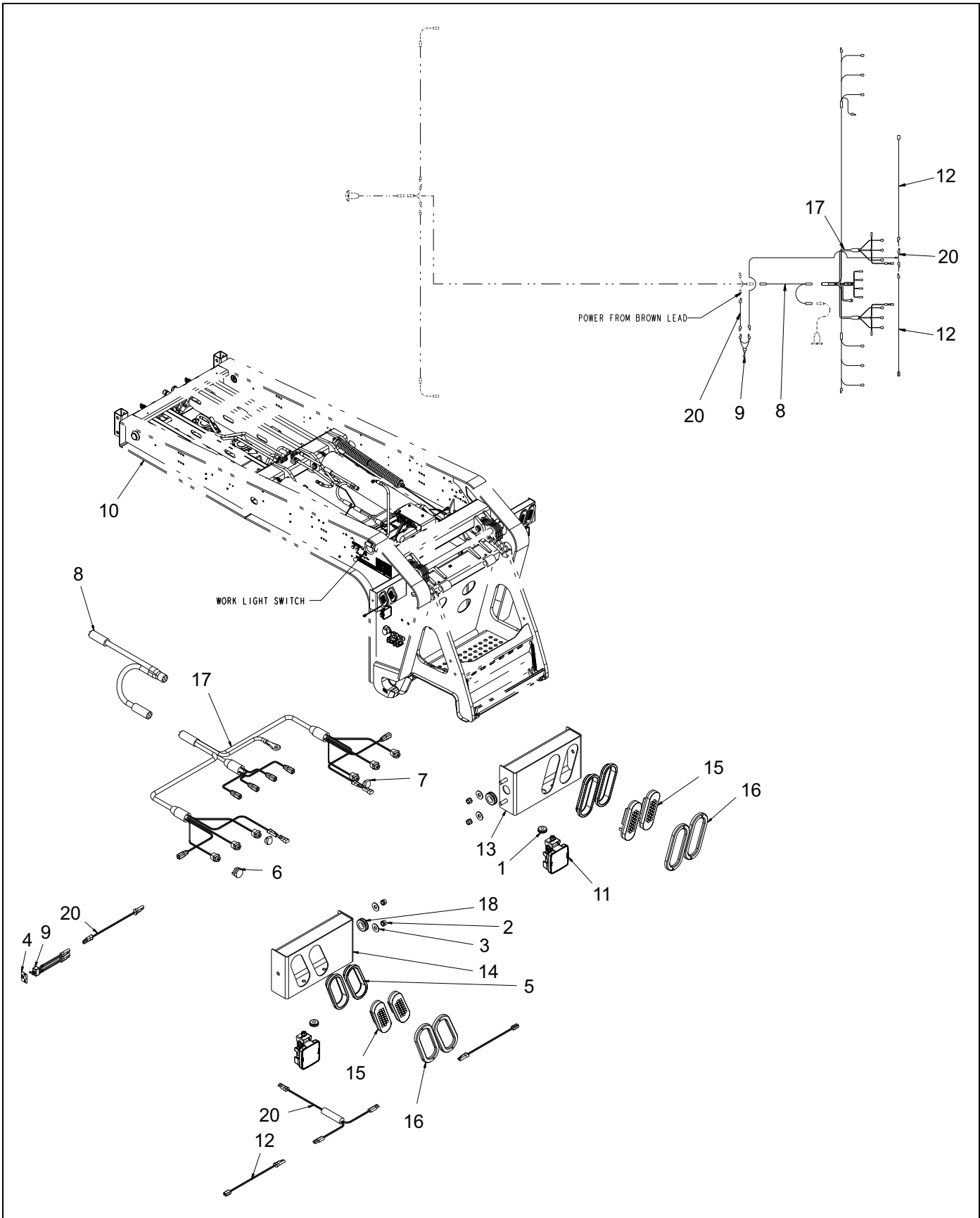
Figure 1-100: S/T/T Light Installation - 800E
