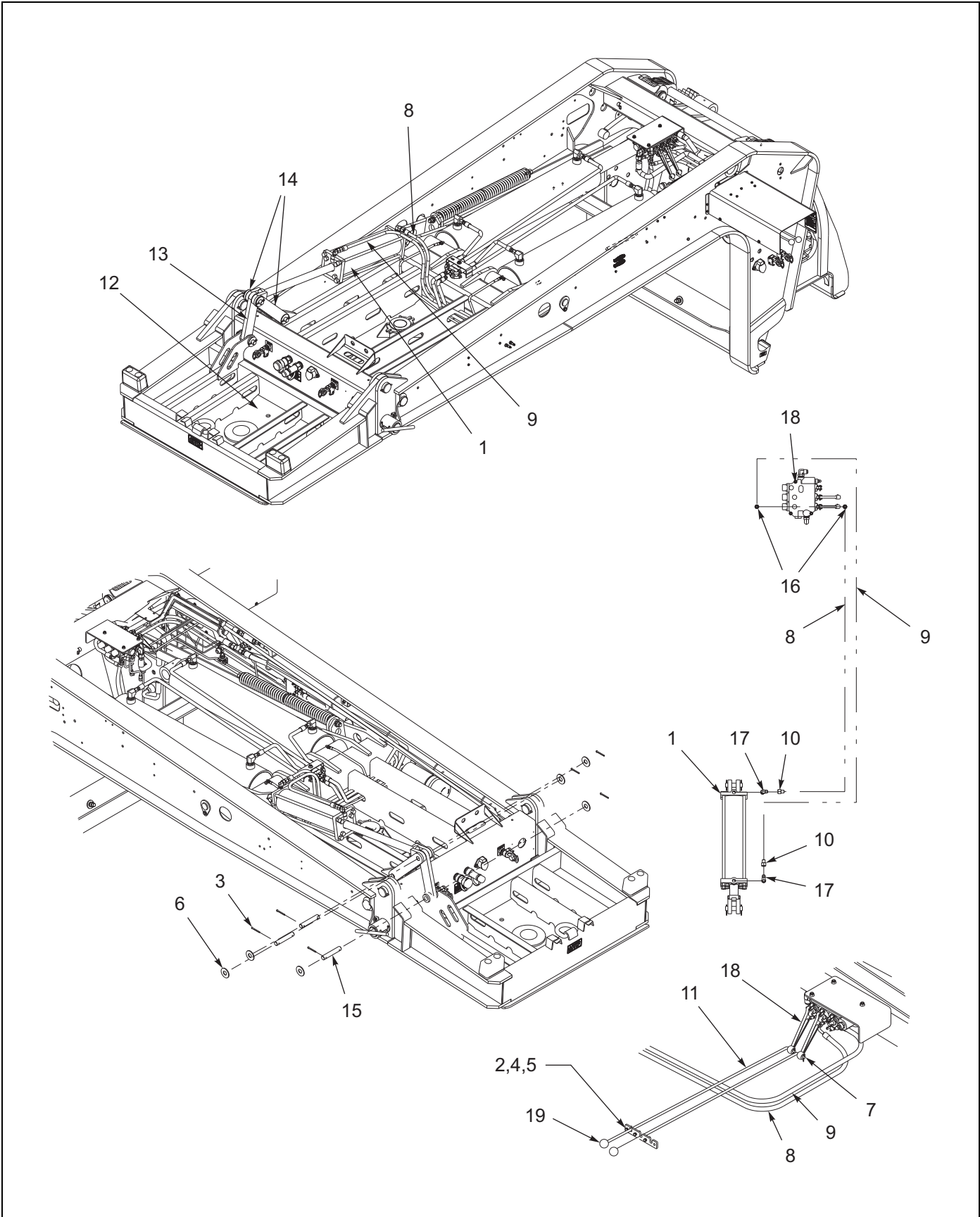
Figure 1-24: Front G/N Hydraulic Flip Extension Installation - 855E HD
