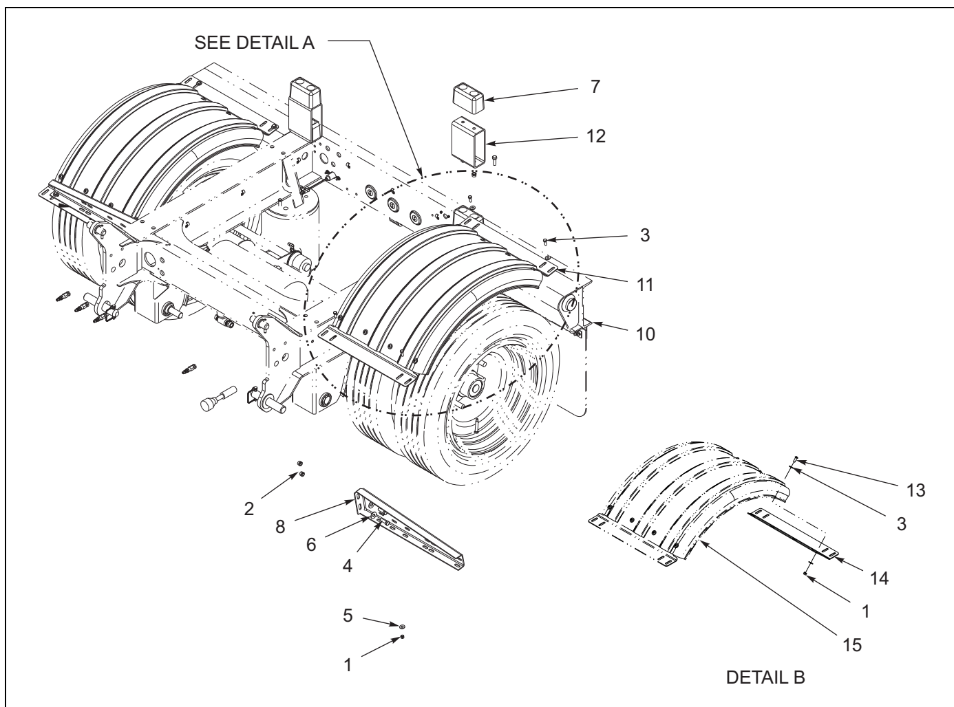
Figure 1-90: Chrome Poly Fender Installation - Flip Axle
