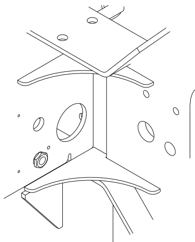
BULKHEAD ADAPTER LOCATION FOR TIRE INFLATION SYSTEM
