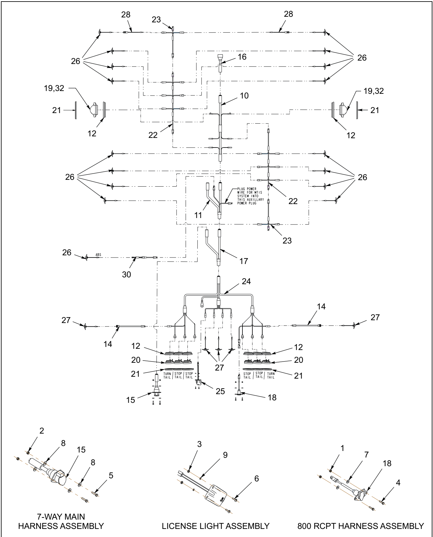
Figure 1-28: Electrical System - 855E
