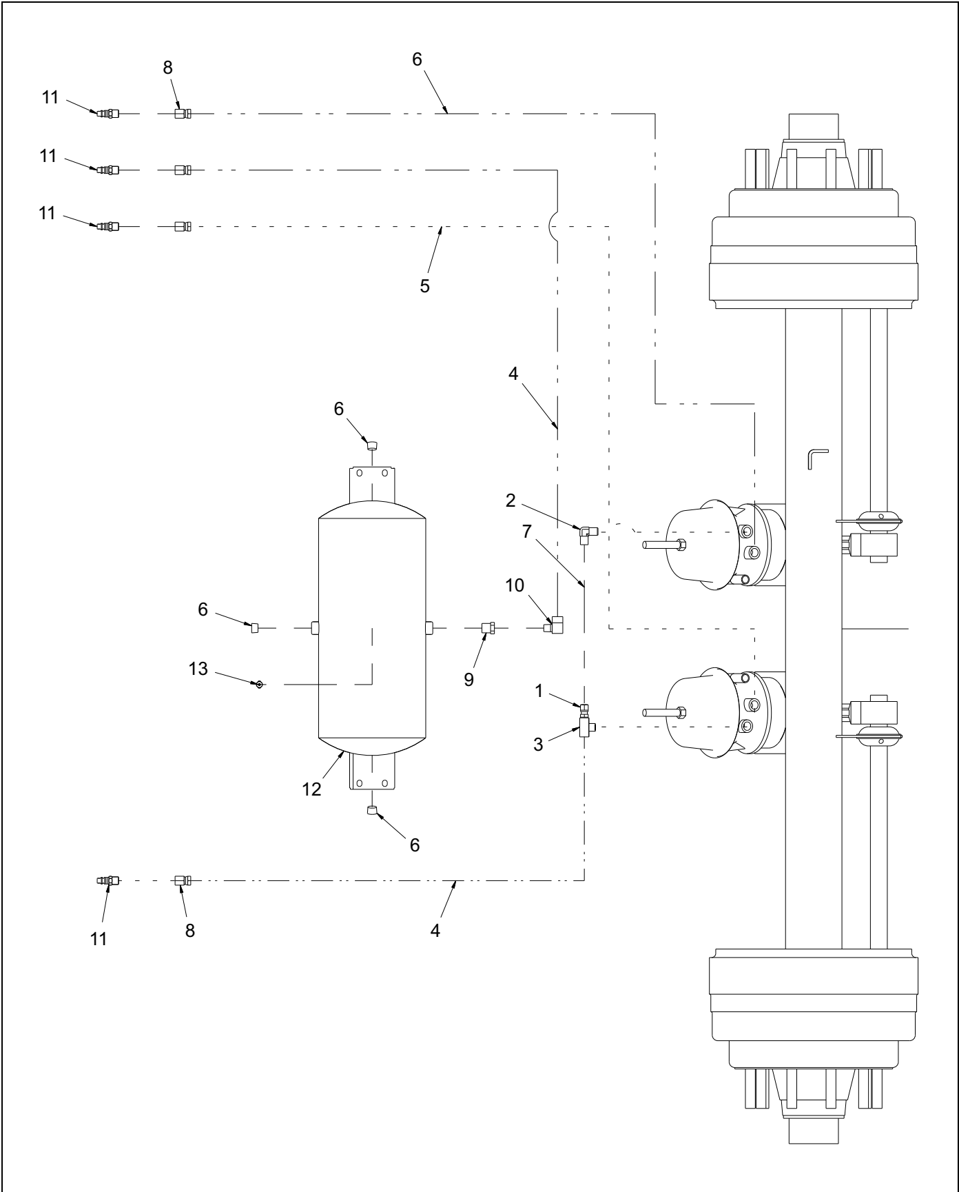
Figure 1-59: Air Brake System
