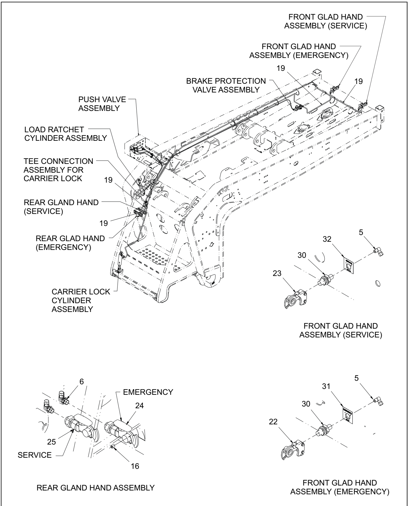
Figure 1-9: Air System - 855E (1 of 2)
