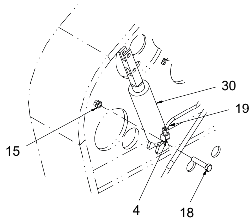
LOAD RATCHET CYLINDER ASSEMBLY
