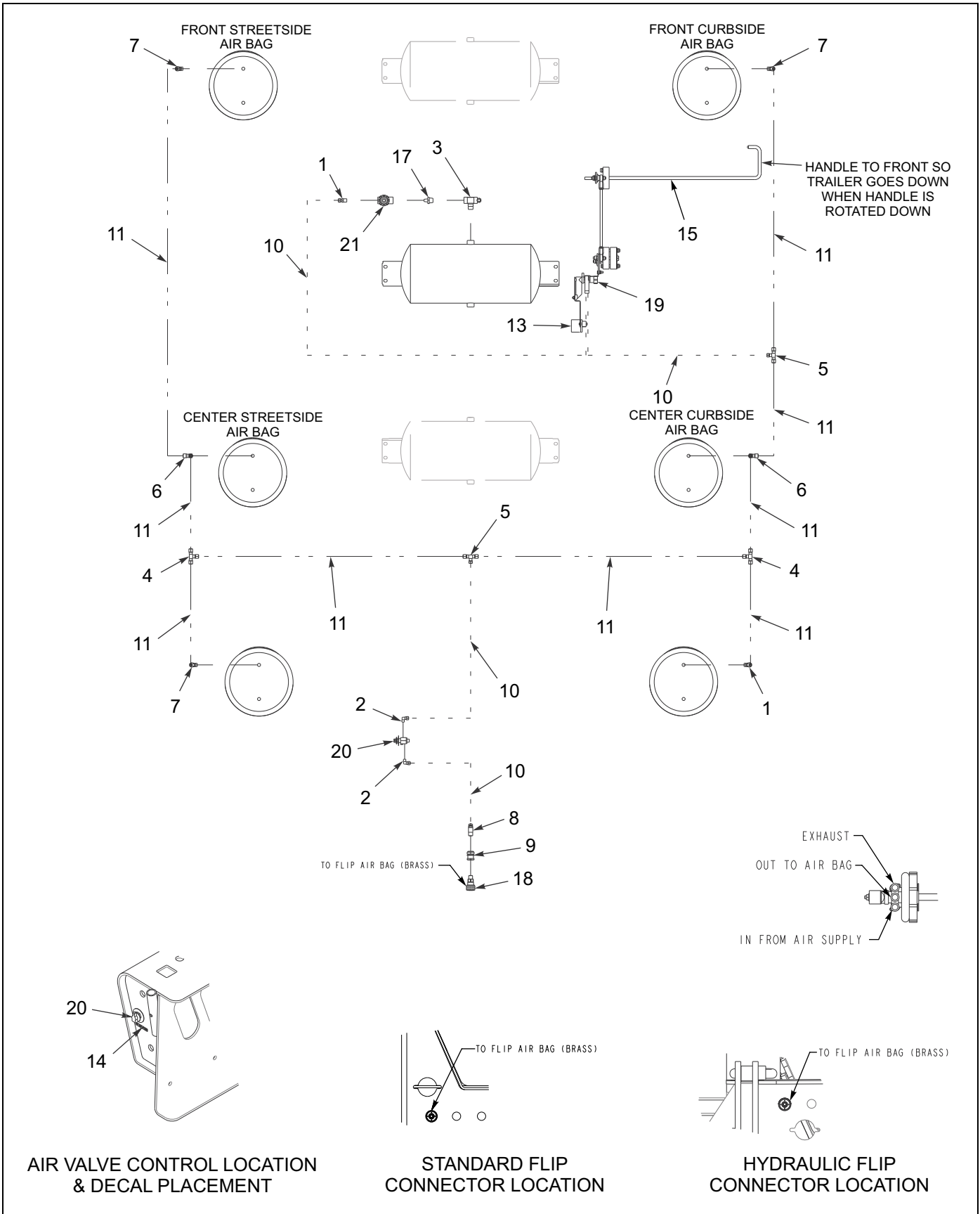
Figure 1-30: Air Ride Suspension - 855E
