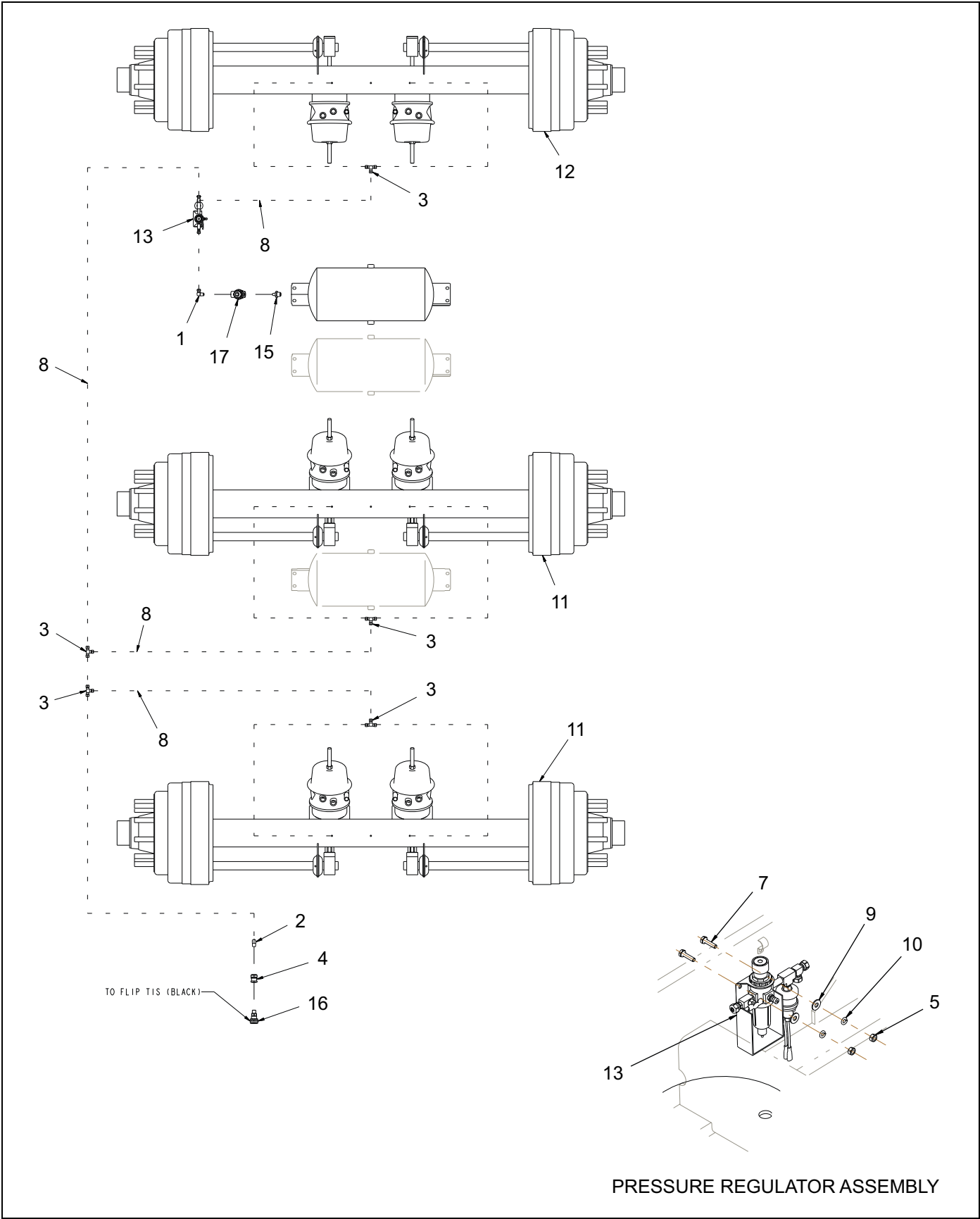
Figure 1-48: Tire Inflation System - 855E Paver
