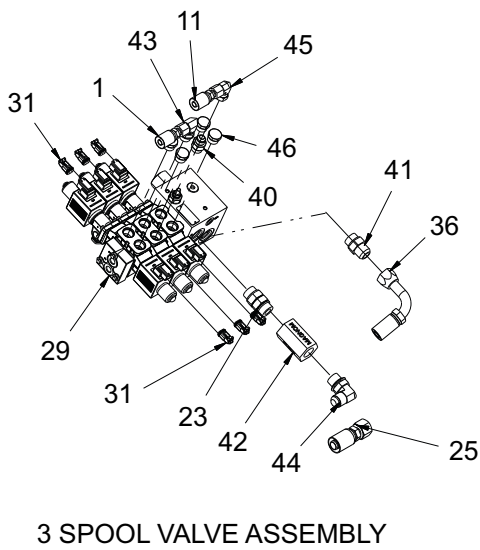
Figure 1-12: Hydraulic & Grease System - 855E (2 of 2)
