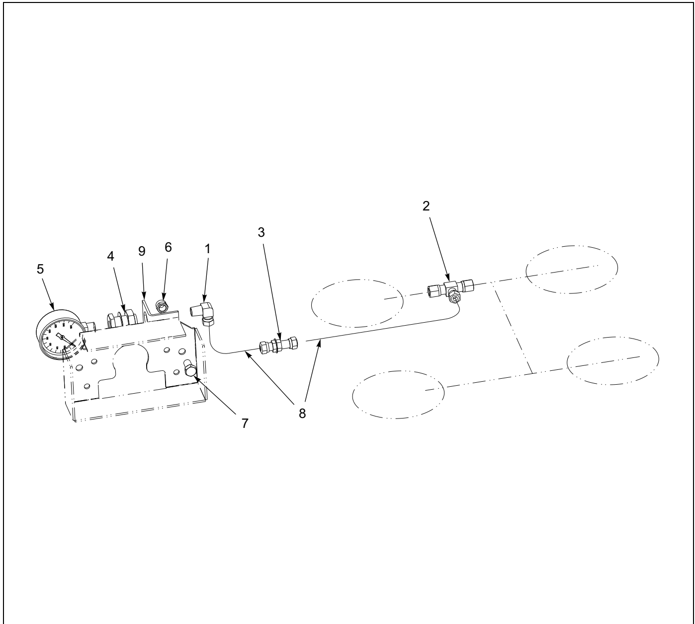
Figure 1-115: Pressure Gauge Installation
