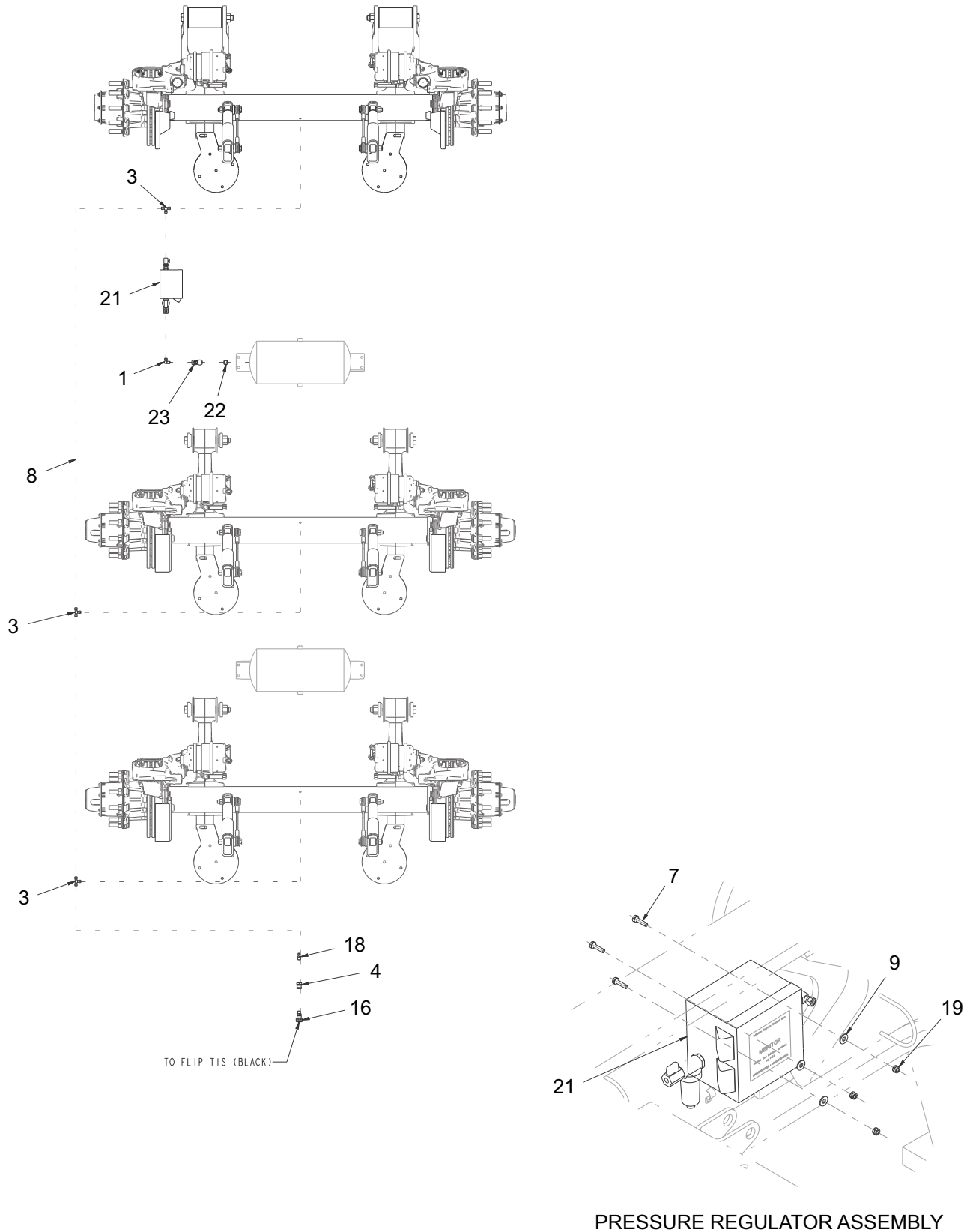
Figure 1-41: Tire Inflation System - 855E HD {P/N 198519, & 198520} (2 of 2)
