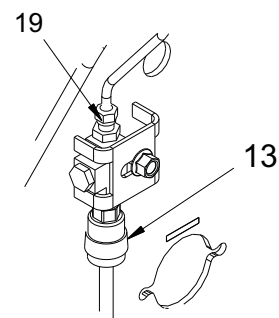
TEE CONNECTION ASSEMBLY FOR CARRIER LOCK
