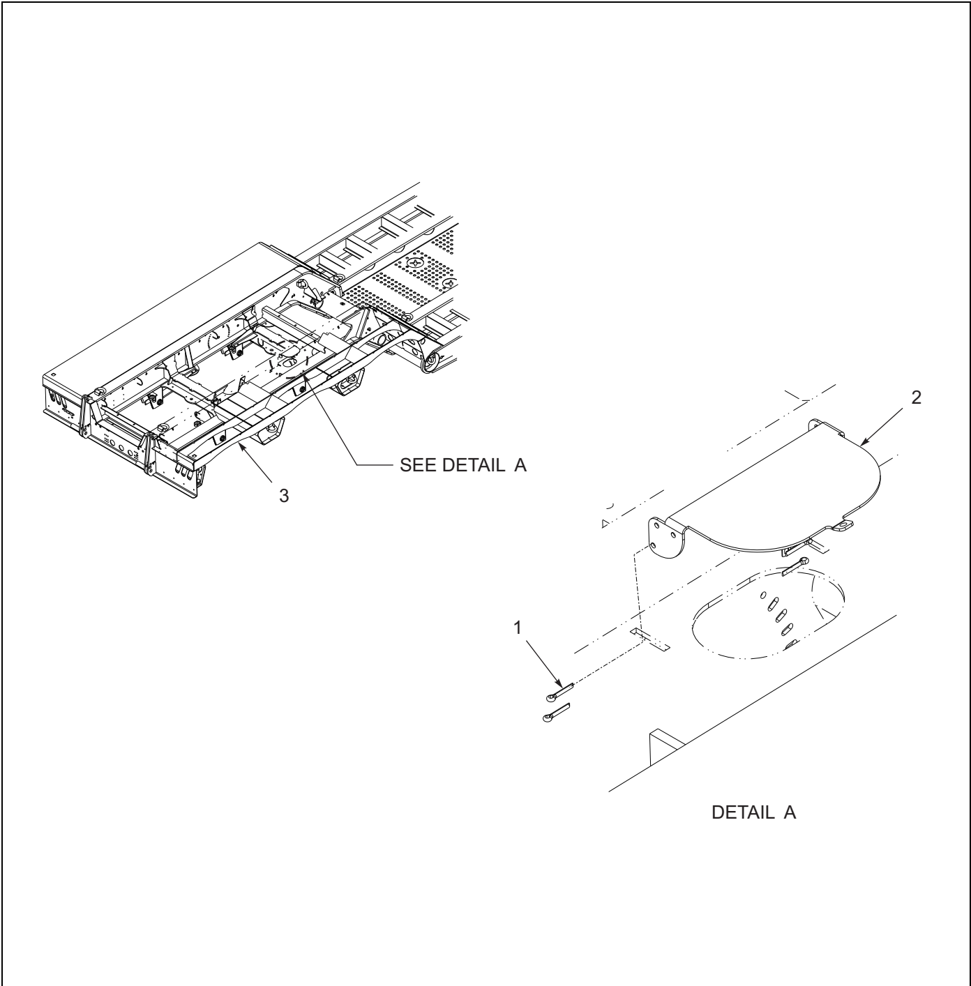
Figure 1-74: Trunnion Cover Installation
