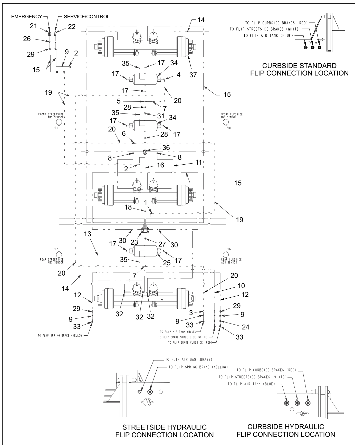
Figure 1-45: Air Brake System - 855E Paver
