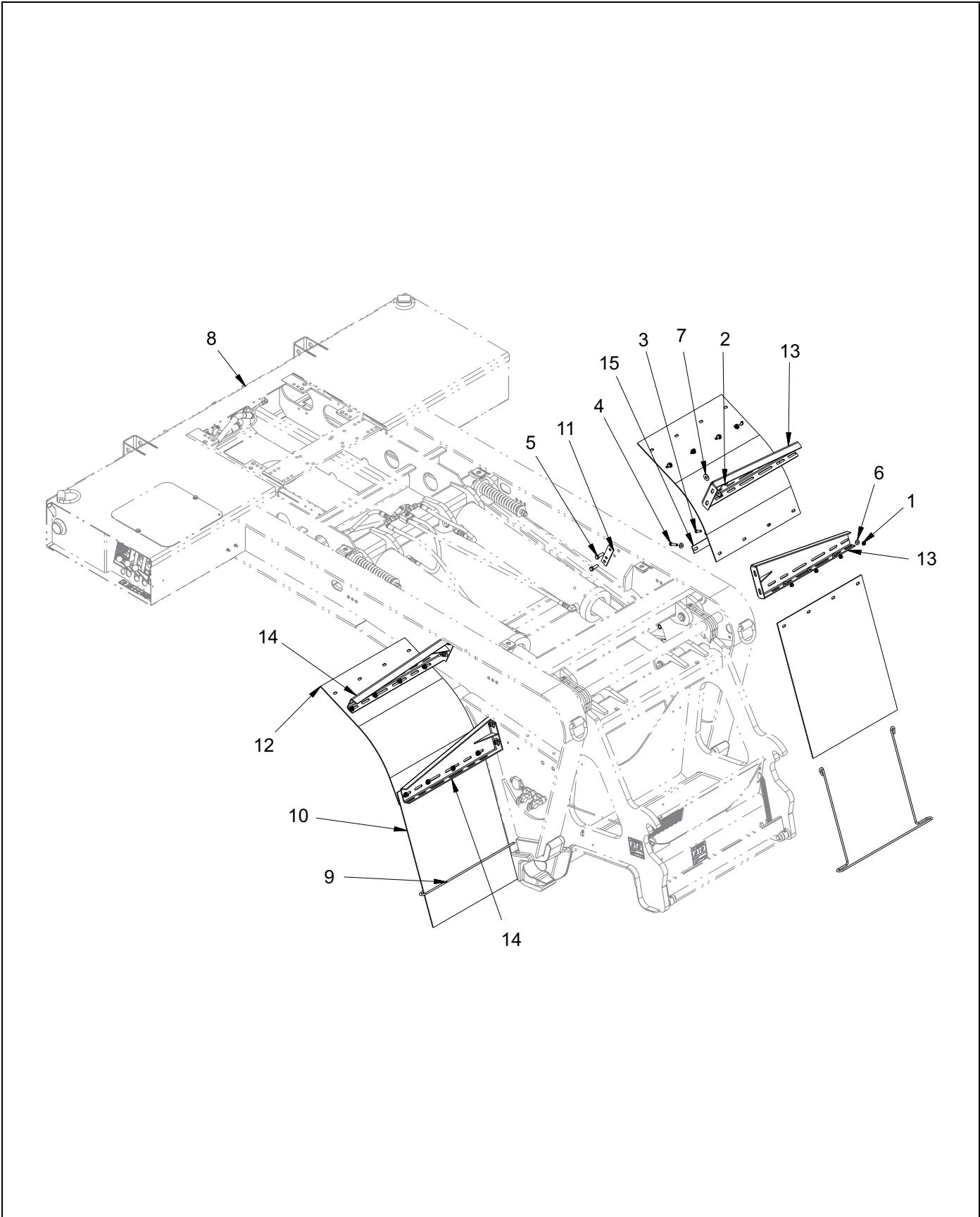
Figure 1-112: Gooseneck Mud Flap Installation
