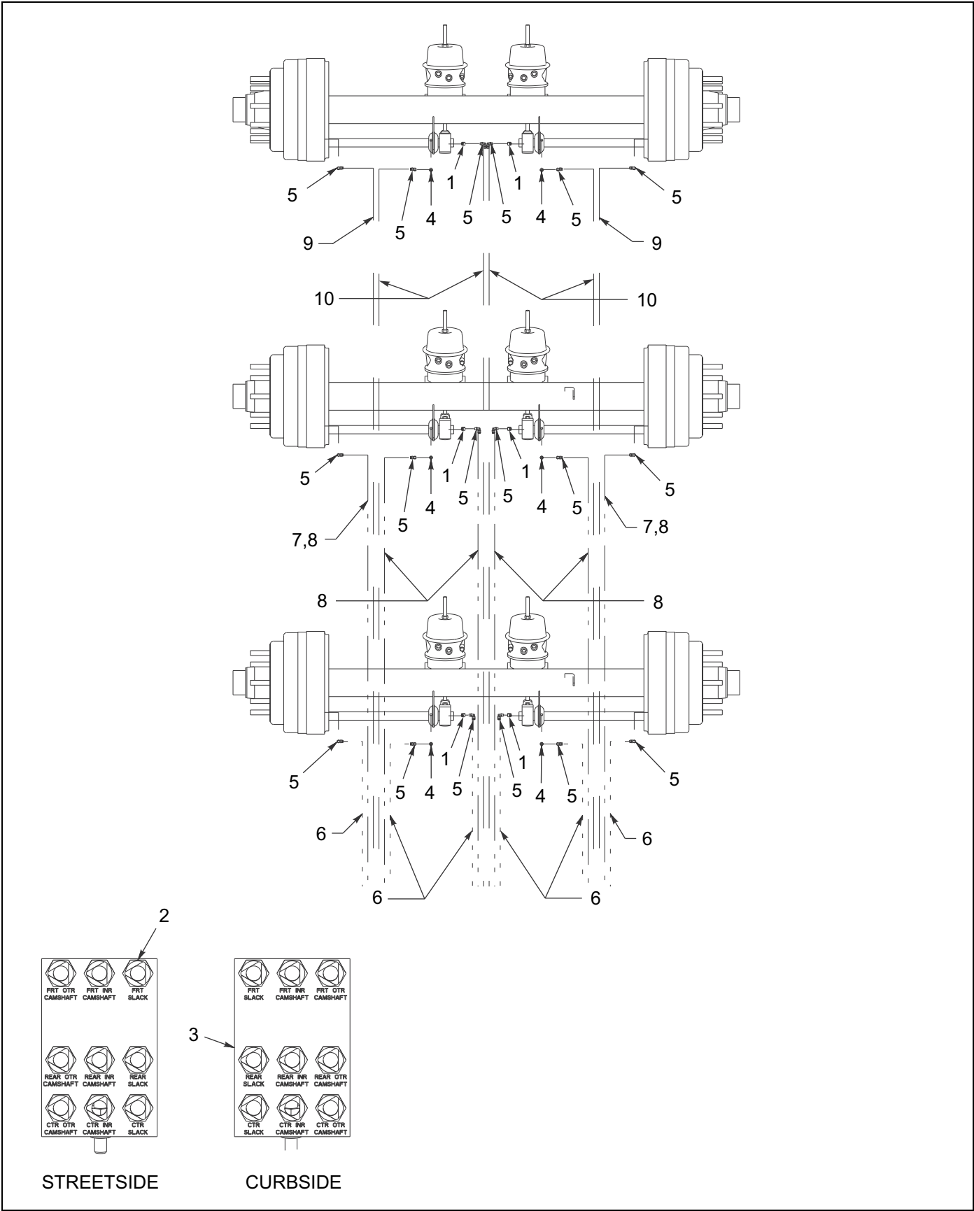
Figure 1-47: Grease System - 855E Paver
