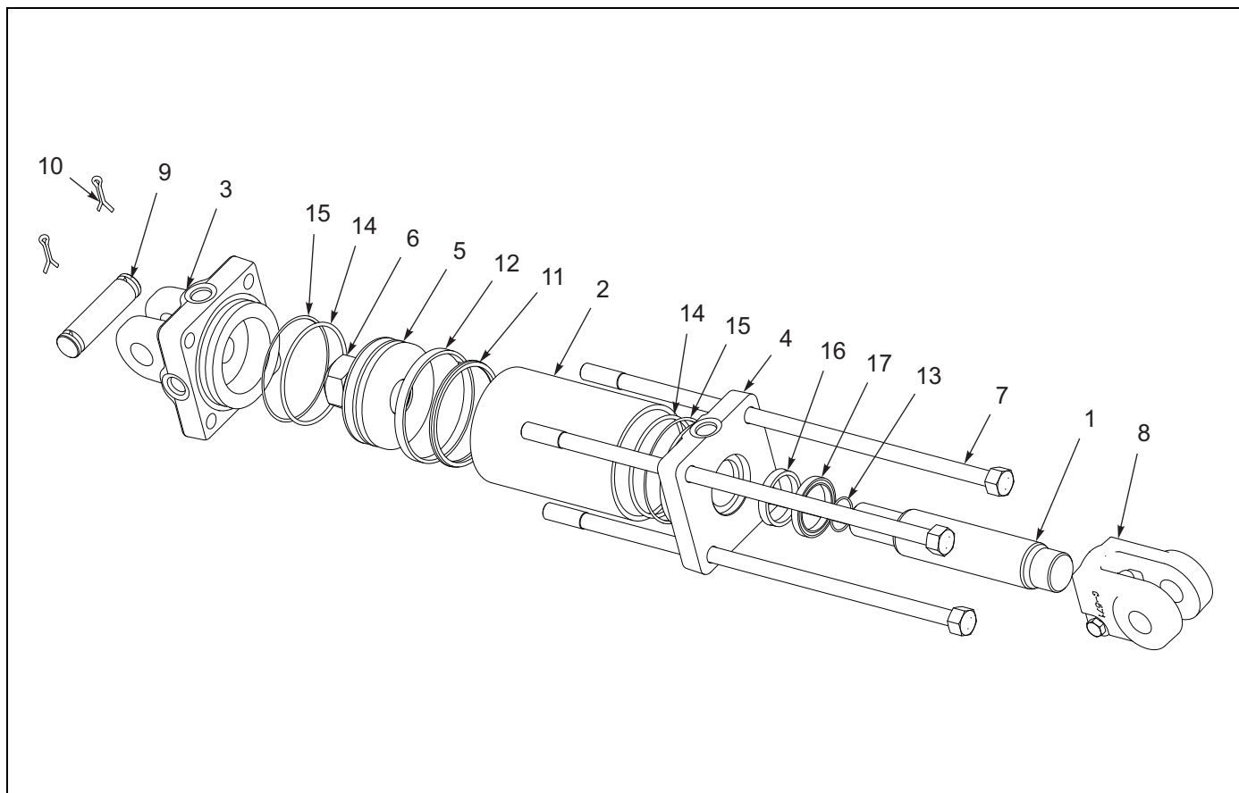
Figure 1-25: Hydraulic Cylinder - 4 X 20
