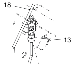
TEE CONNECTION ASSEMBLY FOR CARRIER LOCK
