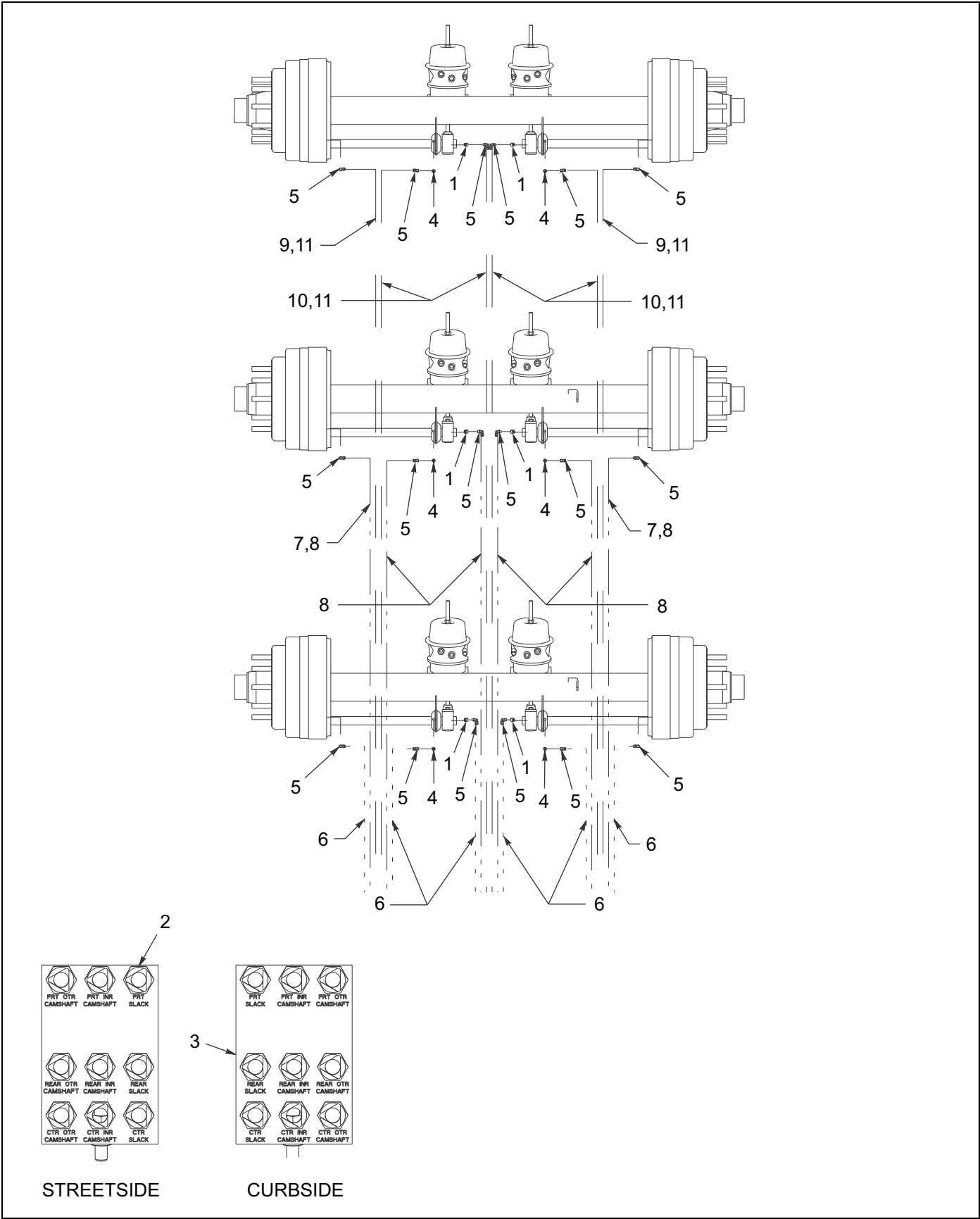
Figure 1-31: Grease System - 855E
