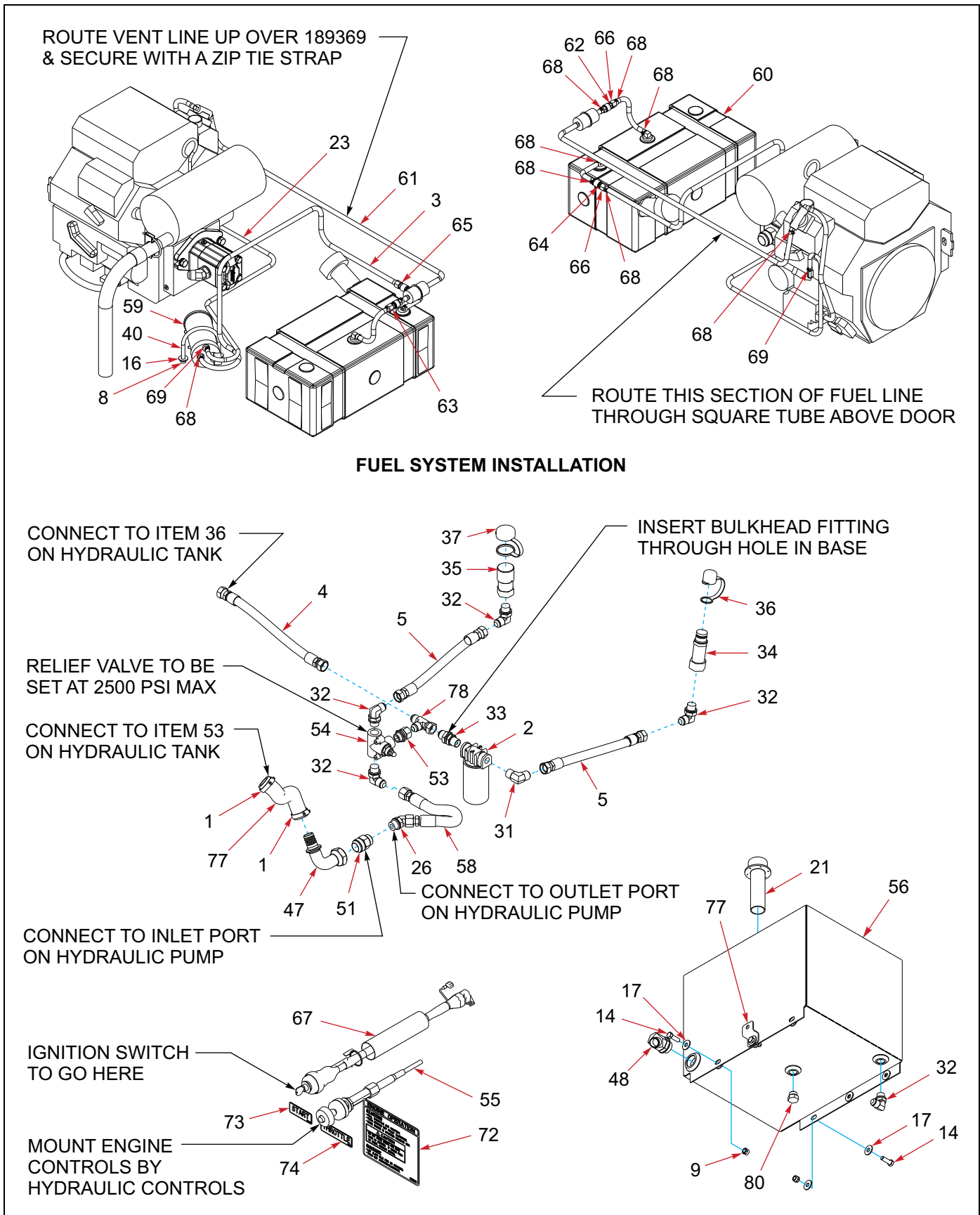
Figure 1-80: 25 HP Upper Deck Engine Package (4 of 4)
