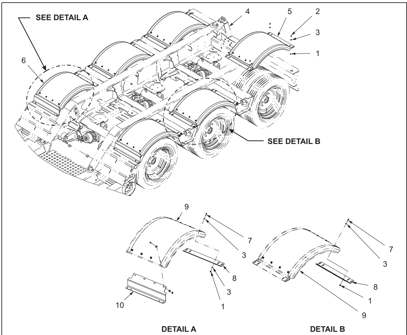
Figure 1-87: Black Poly Fender Installation - 3 Axle
