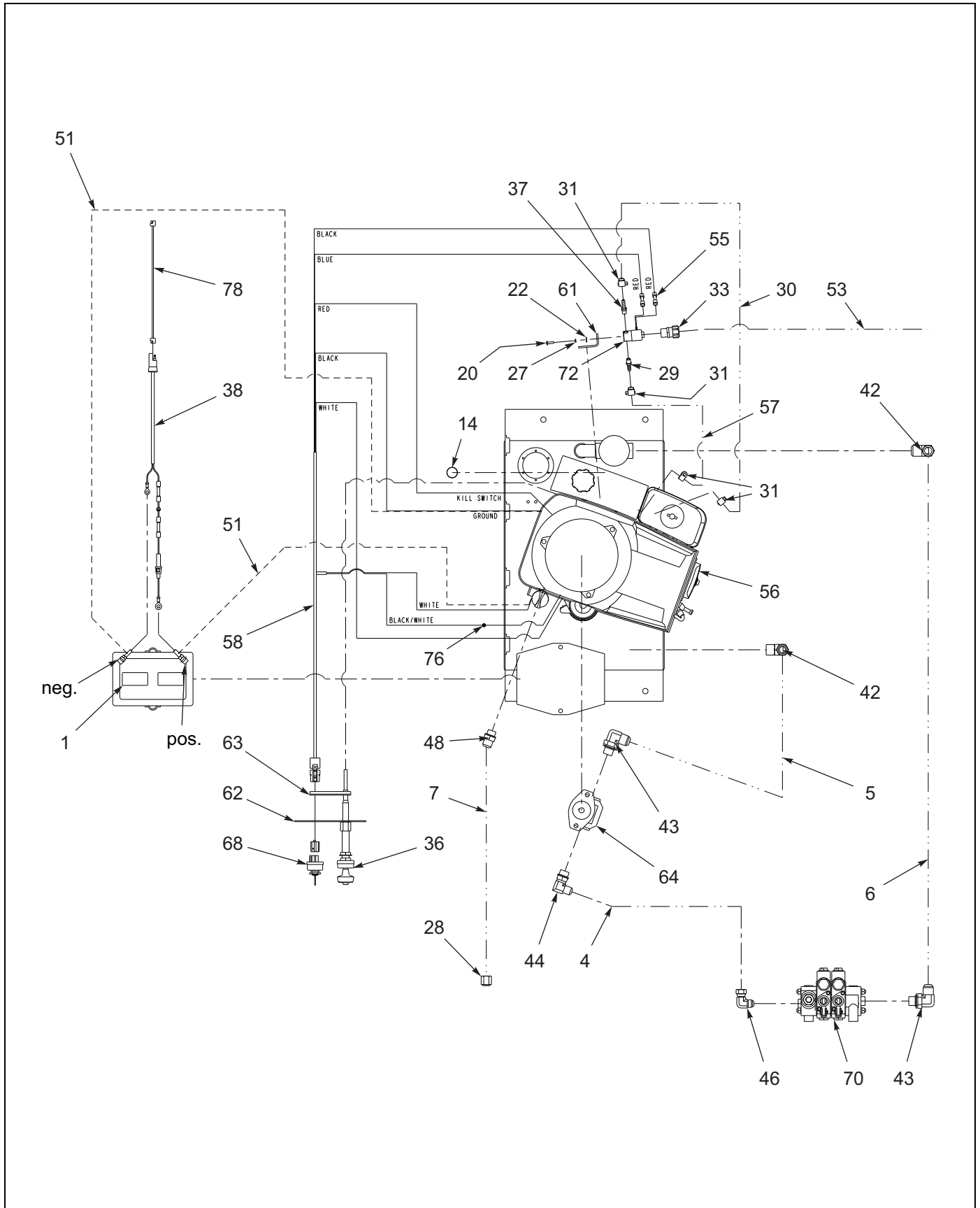
Figure 1-85: 42-11 HP Honda Engine Drive Installation (2 of 2)
