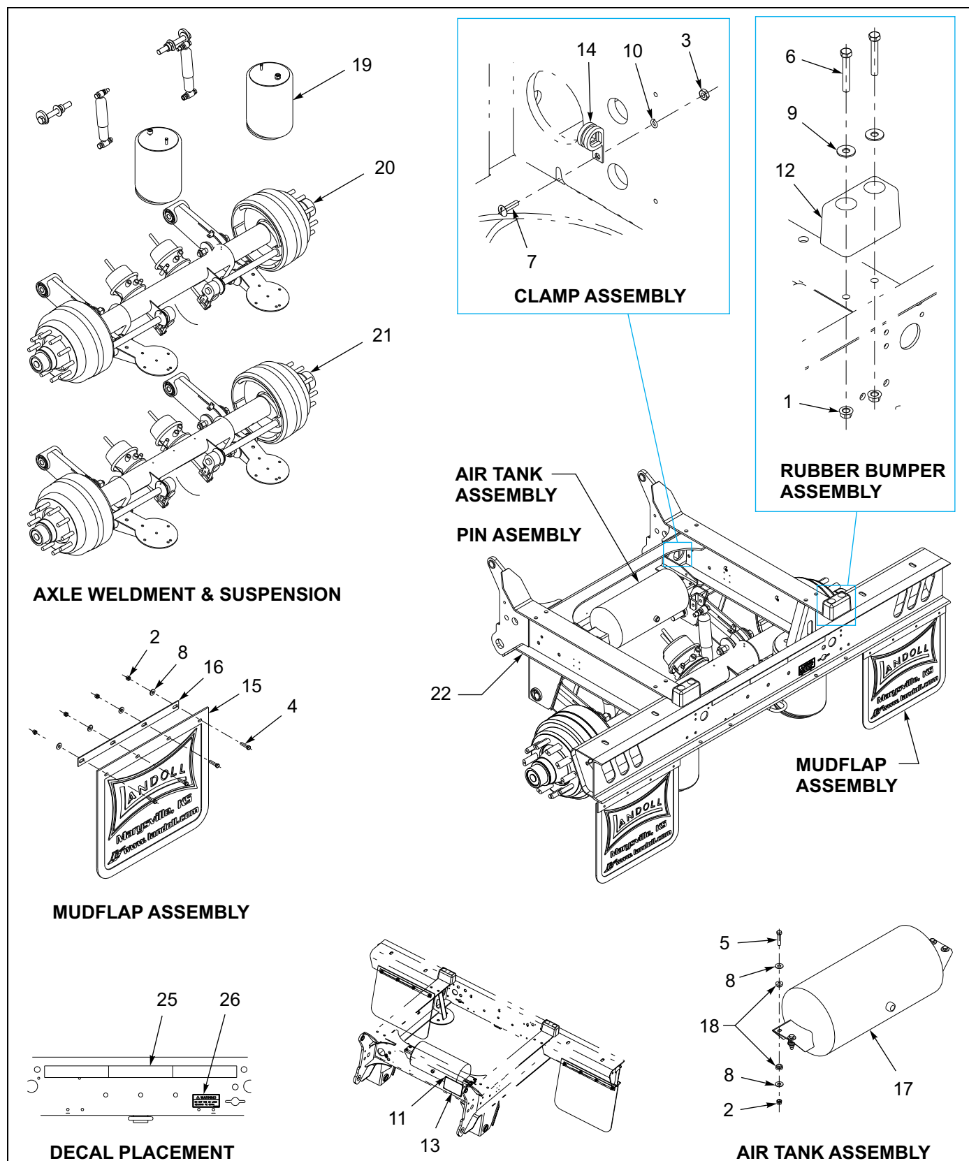
Figure 1-57: General Assembly
