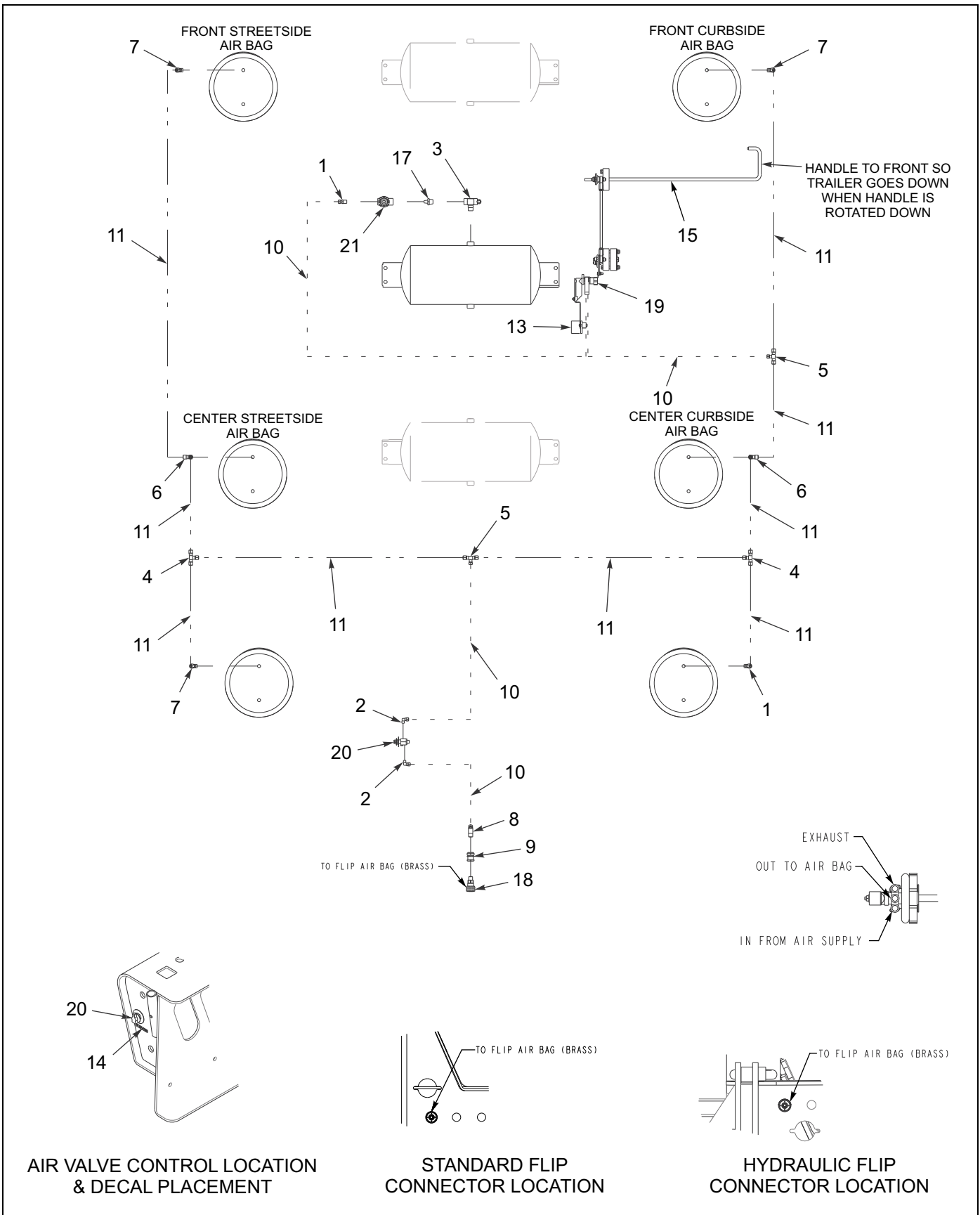
Figure 1-46: Air Ride Suspension - 855E Paver
