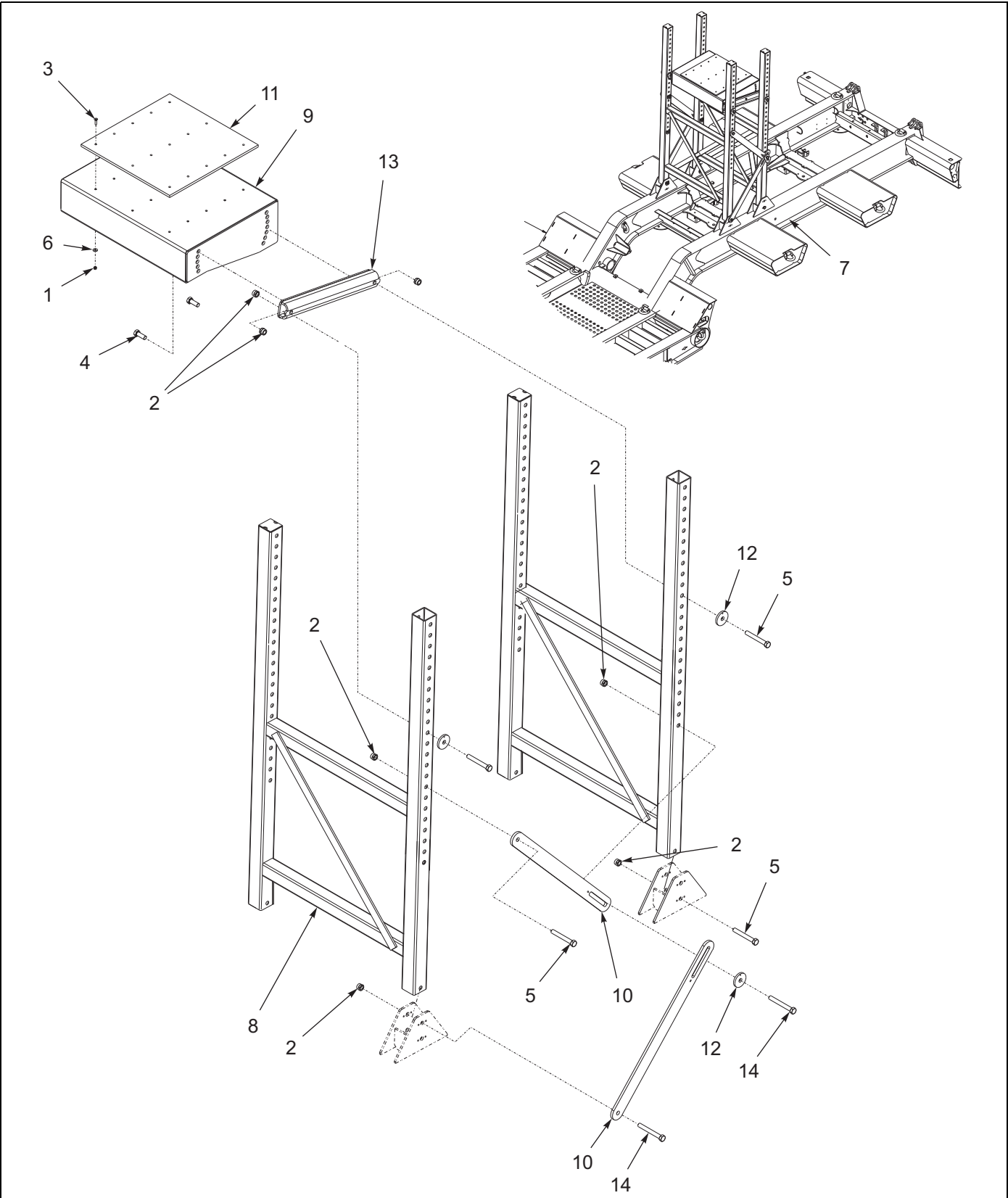
Figure 1-69: Support Boom Assembly - 855E HD
