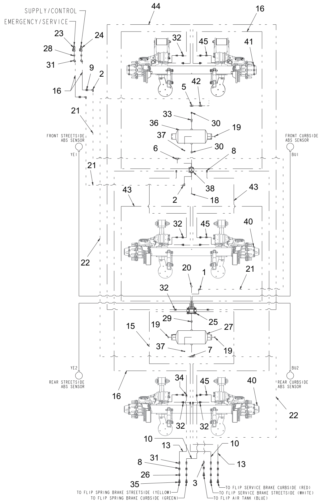
Figure 1-37: Air Brake System - 855E HD {P/N 198518 &amp; 198519} (2 of 2)
