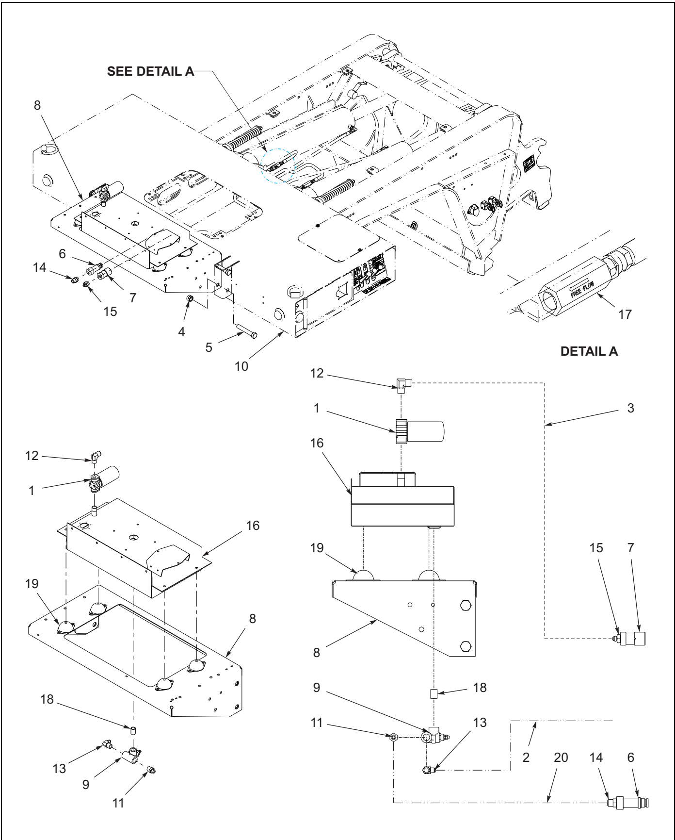
Figure 1-82: Front Engine Mount Installation
