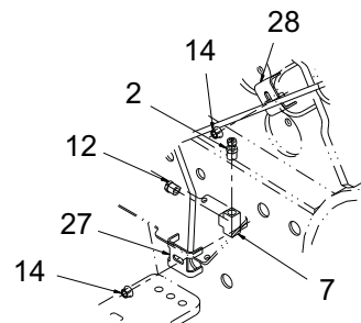
HOSE CLAMPS & TEE CONNECTION FOR CARRIER LOCK
