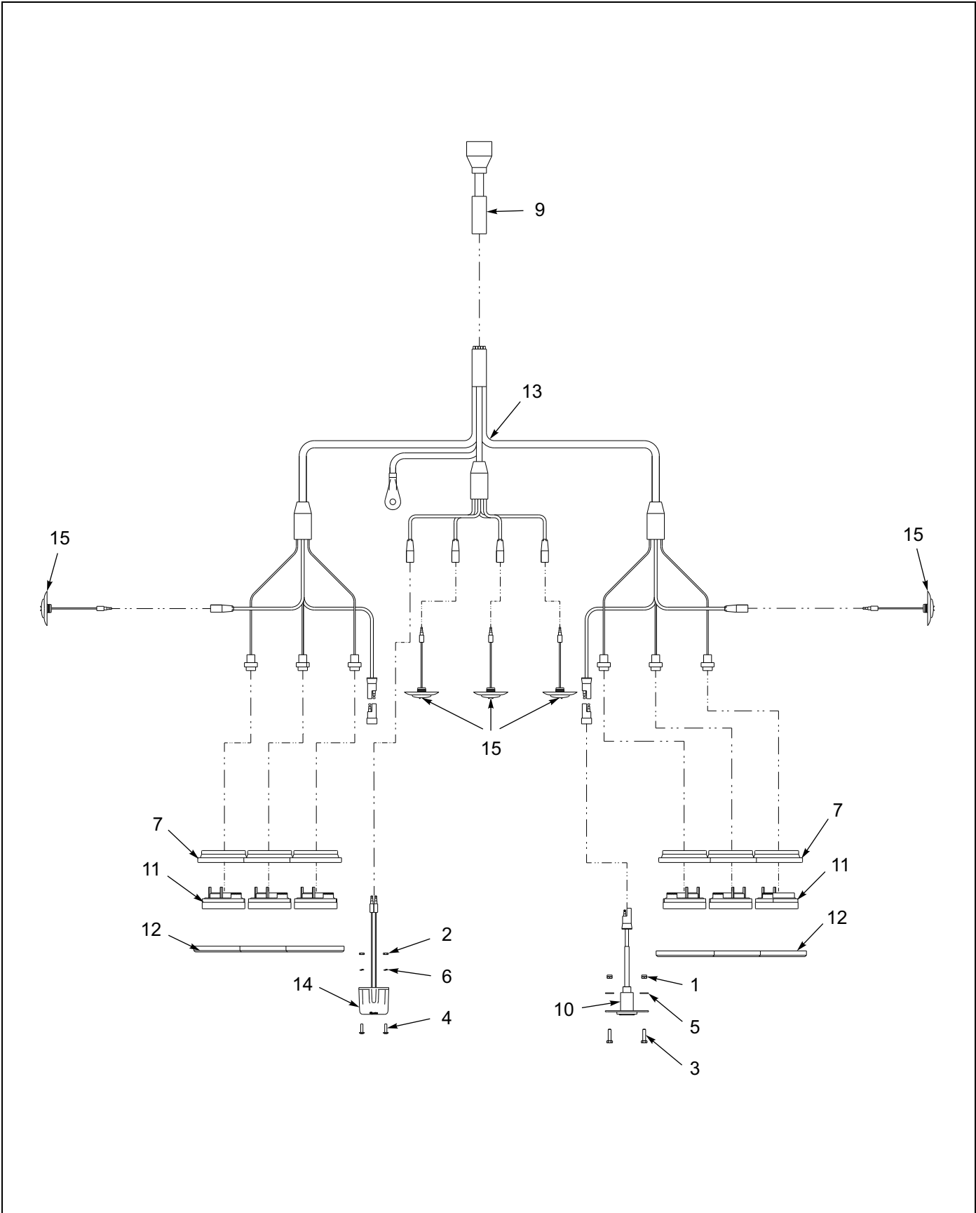
Figure 1-58: Electrical System
