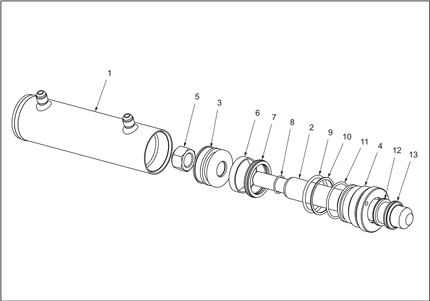
Figure 1-103: 1-1/2 x 8 Hydraulic Cylinder - 855E HD
