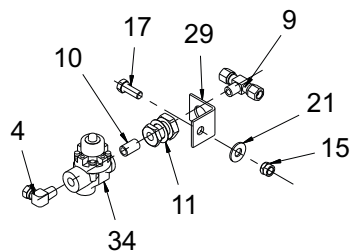
BRAKE PROTECTION VALVE FITTING ASSEMBLY
