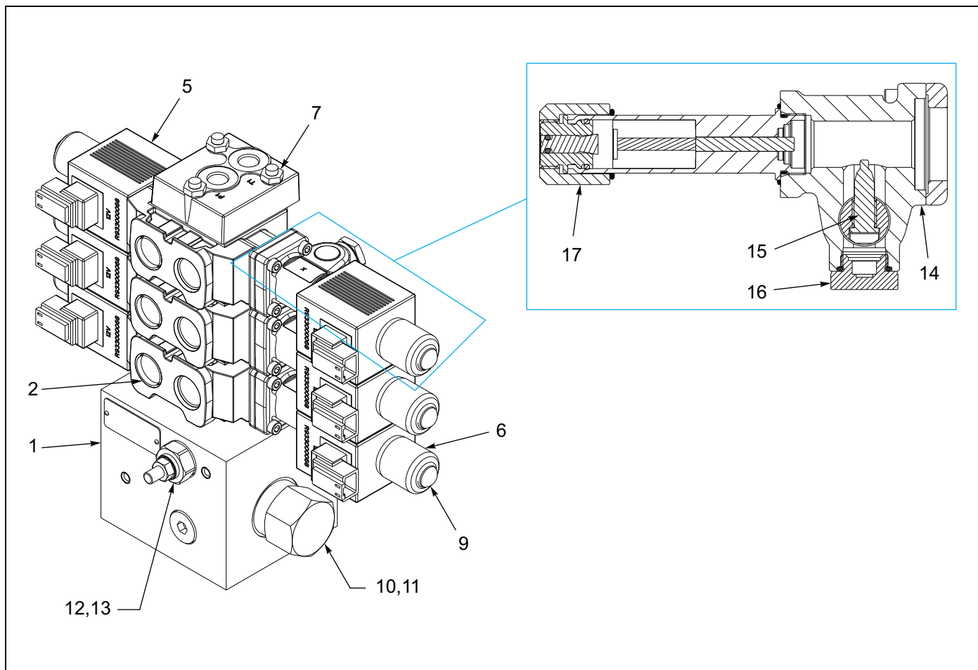
Figure 1-22: Three Spool Valve
