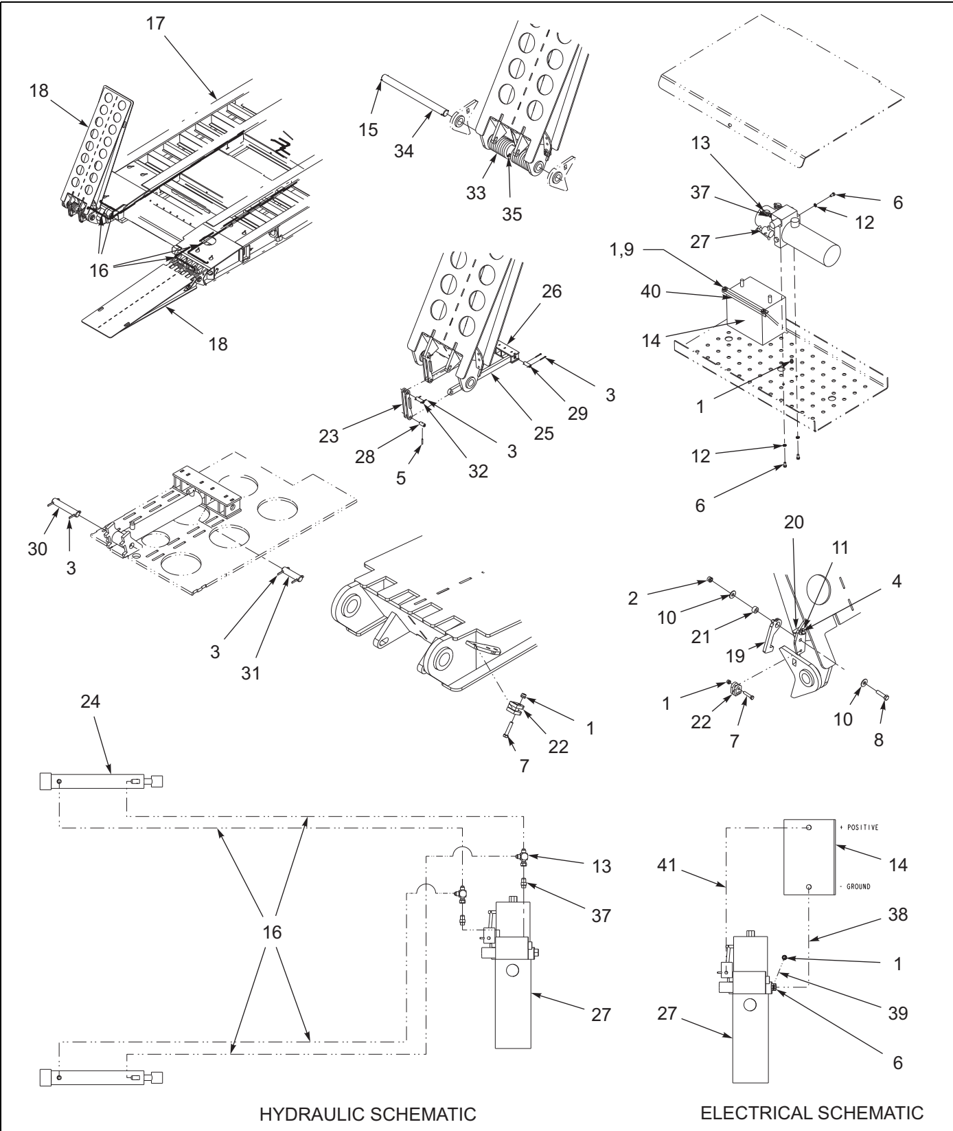
Figure 1-102: 6-1/2' Front Ramp Assembly - 855E HD
