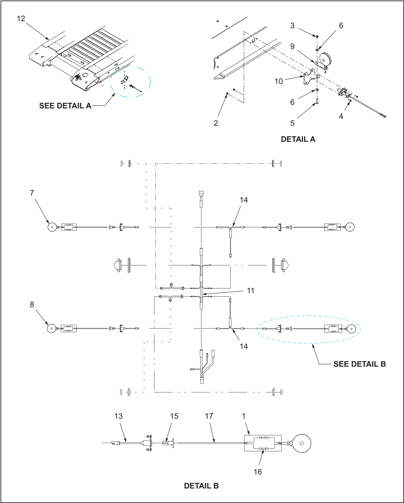
Figure 1-101: Web Mounted Four Corner Light Package
