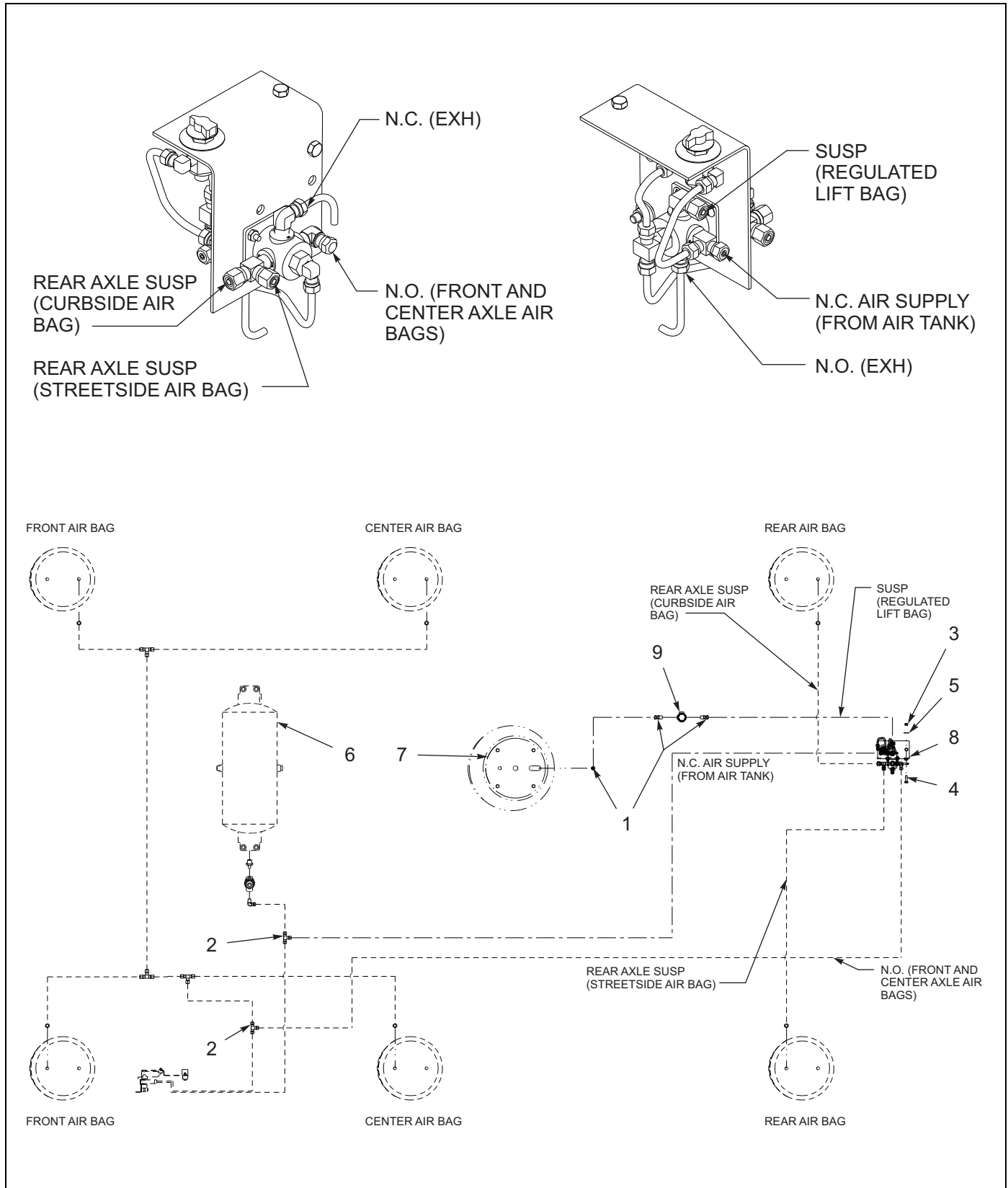
Figure 1-92: Lift Axle Control - 855E
