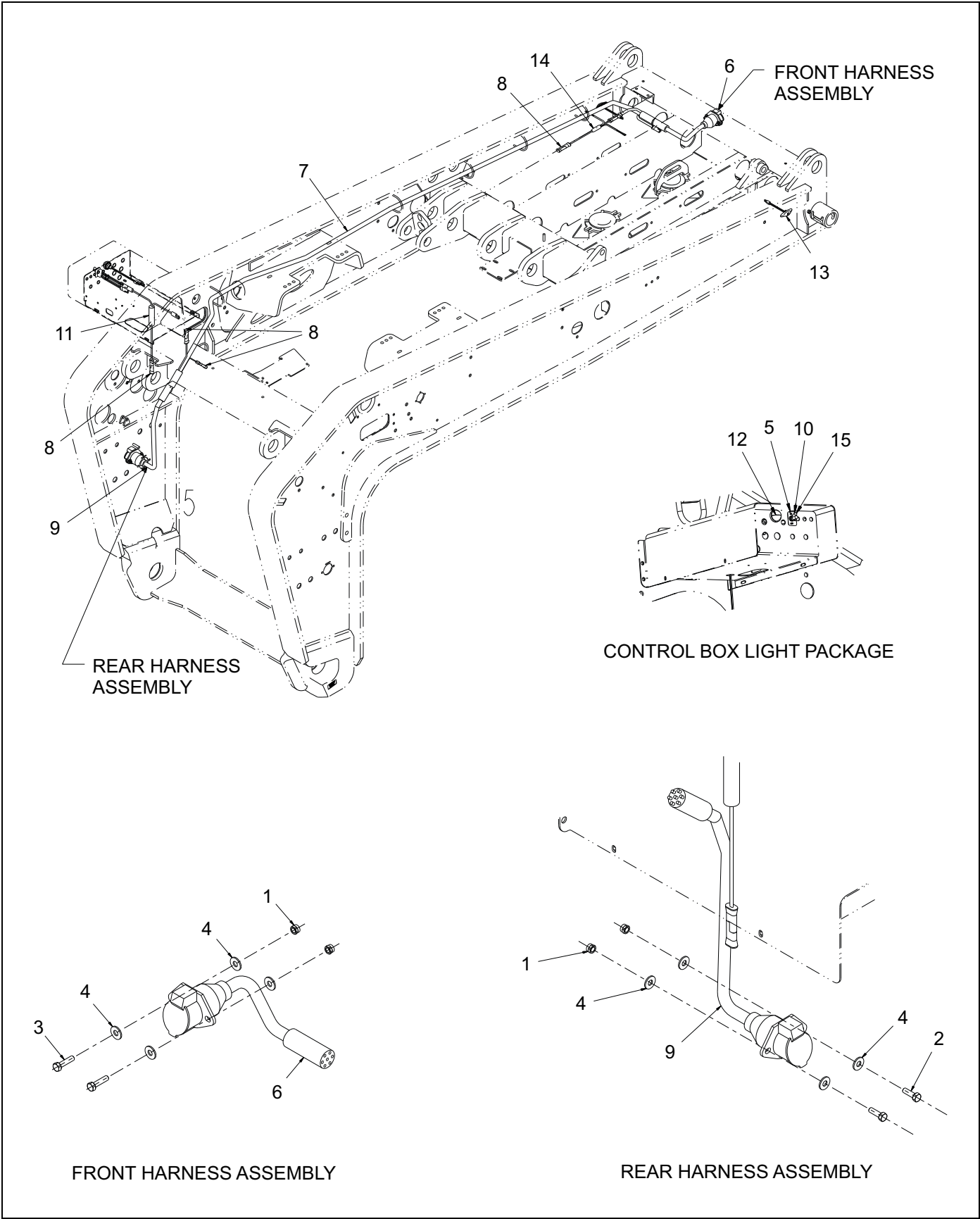
Figure 1-15: Electrical System - 855E HD
