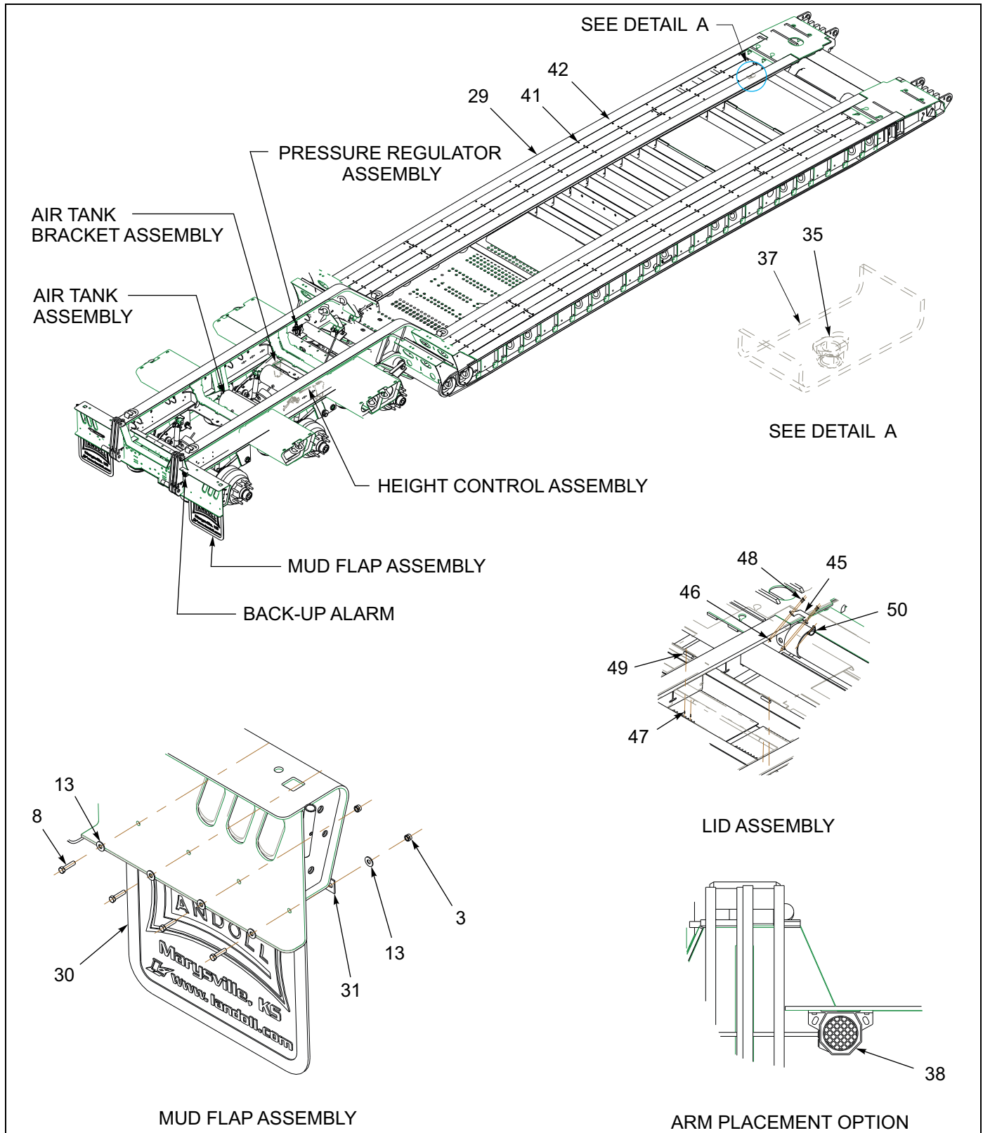
Figure 1-33: General Assembly - 855E HD (1 of 2)
