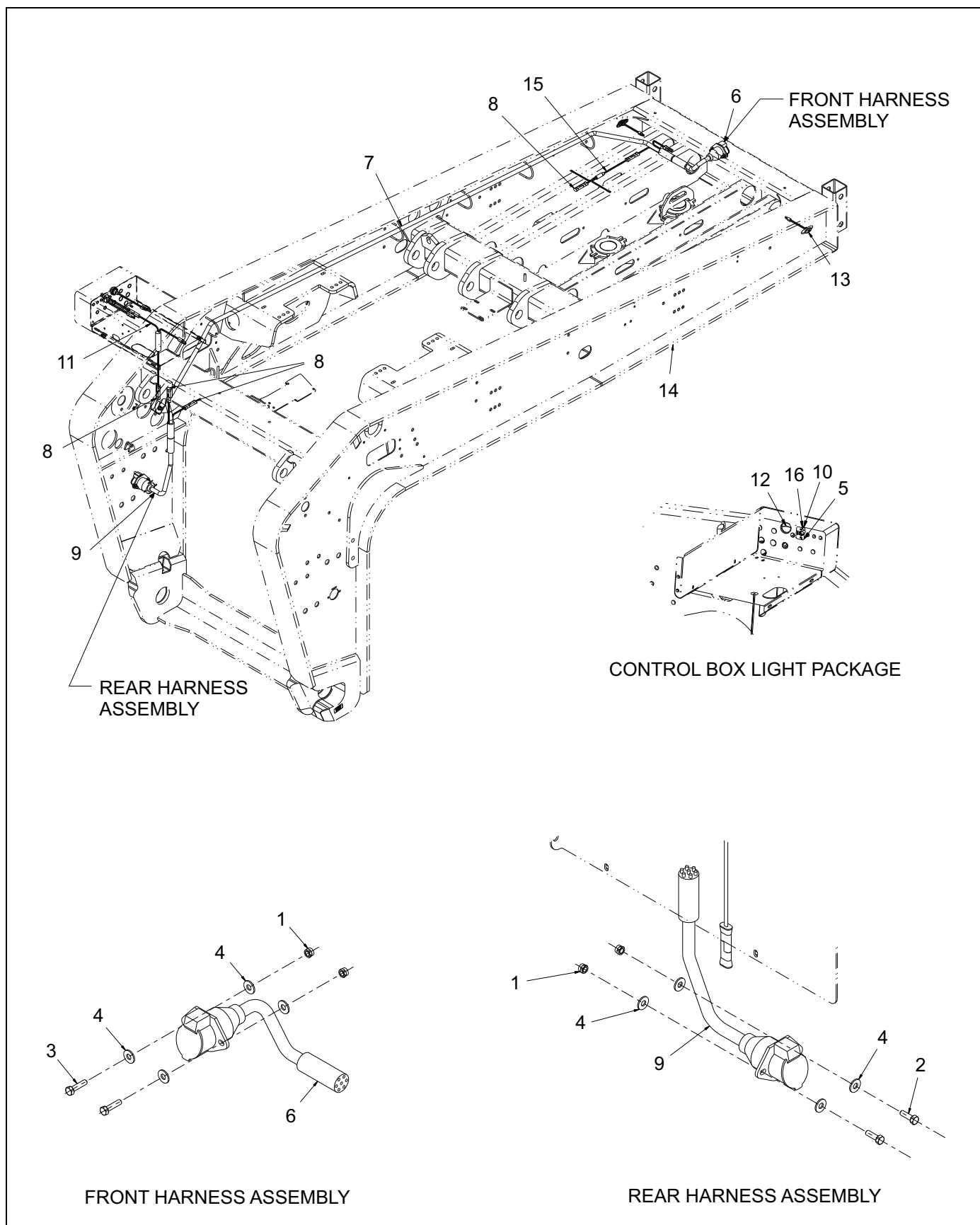
Figure 1-8: Electrical System - 855E
