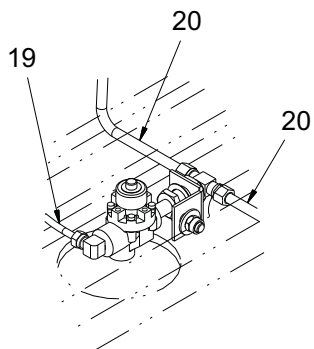
BRAKE PROTECTION VALVE HOSE ASSEMBLY
