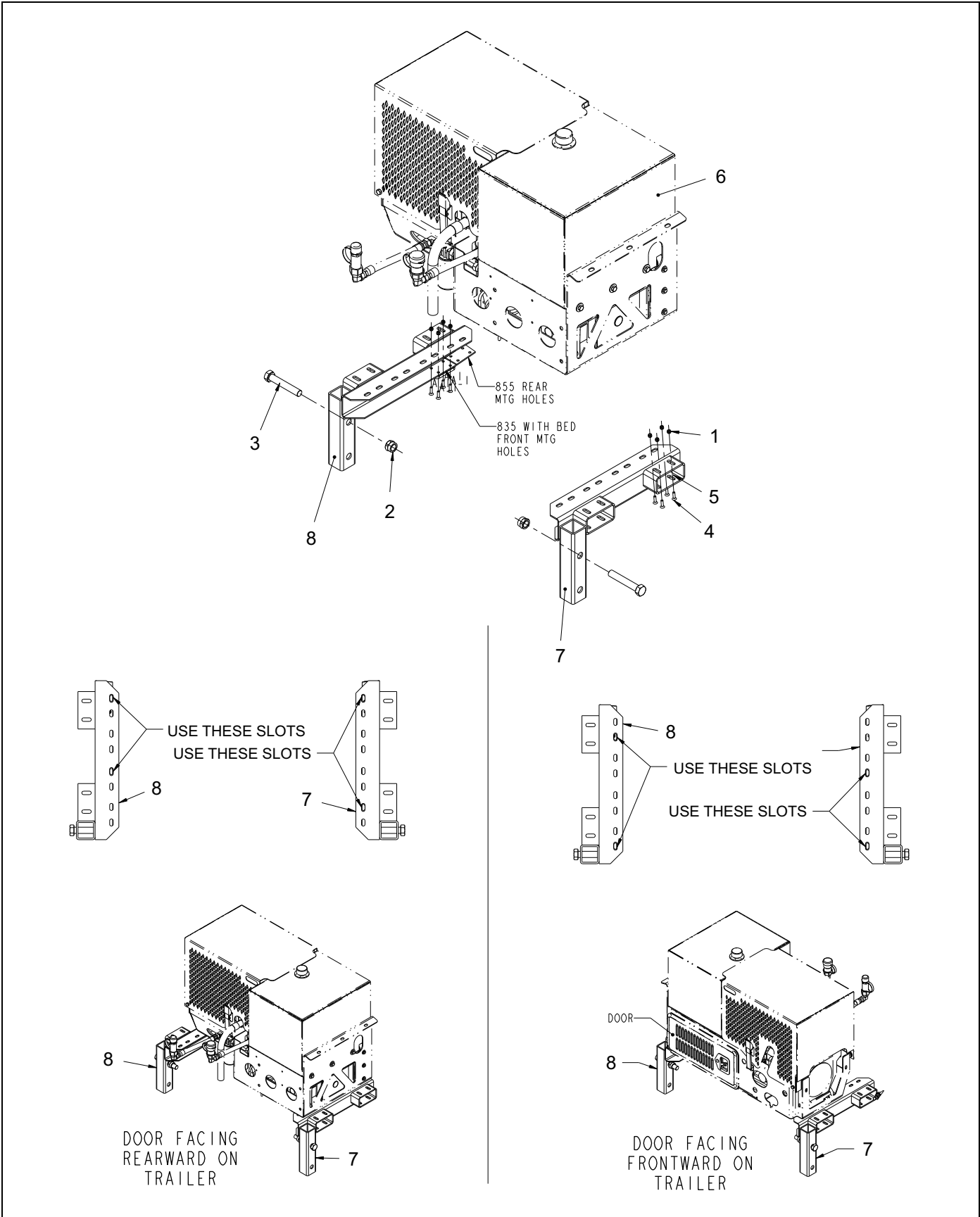
Figure 1-81: 800 Engine Mount Installation
