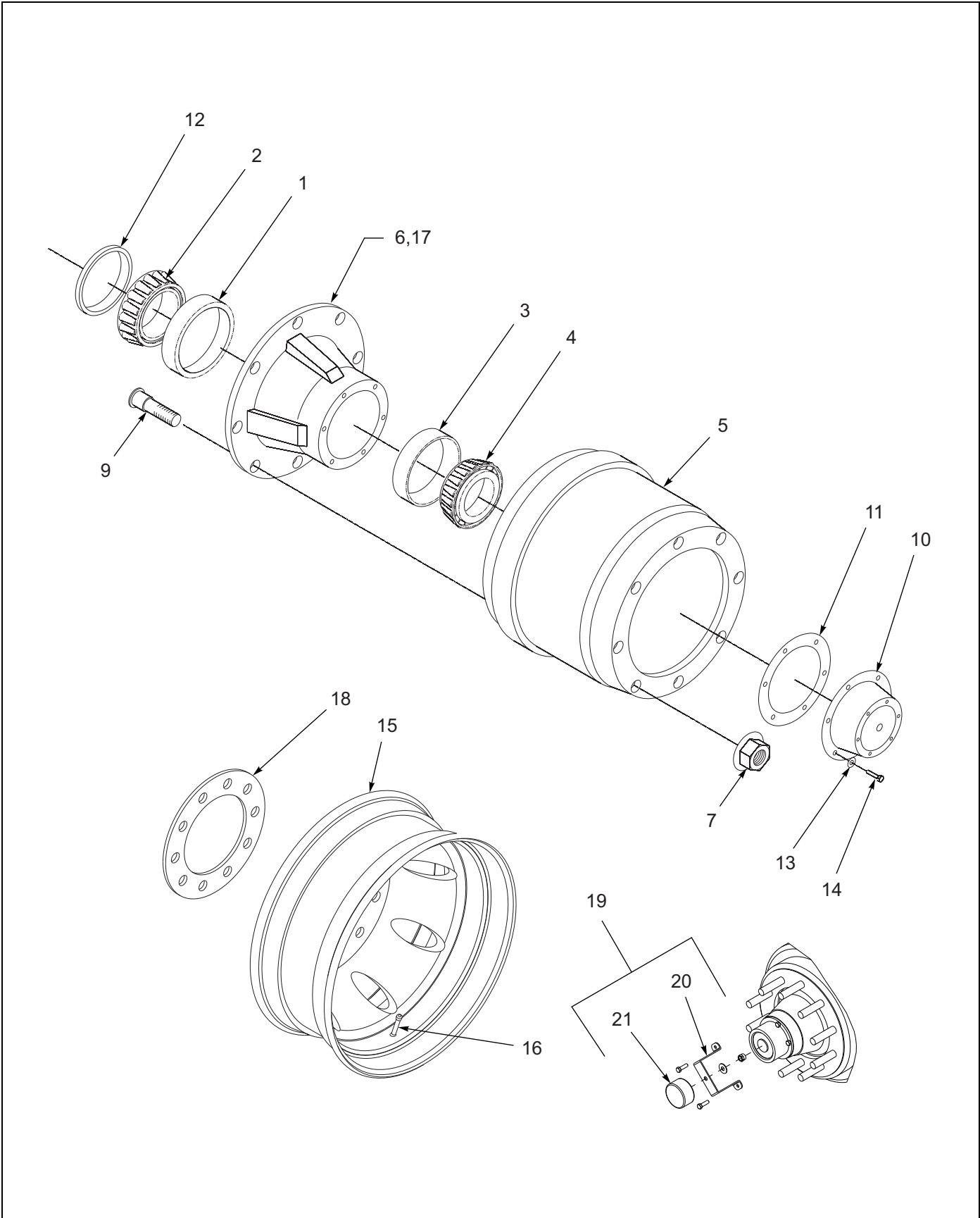
Figure 1-54: Outboard Pilot Mount Hub and Drum
