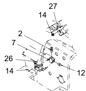
HOSE CLAMPS & TEE CONNECTION FOR CARRIER LOCK
