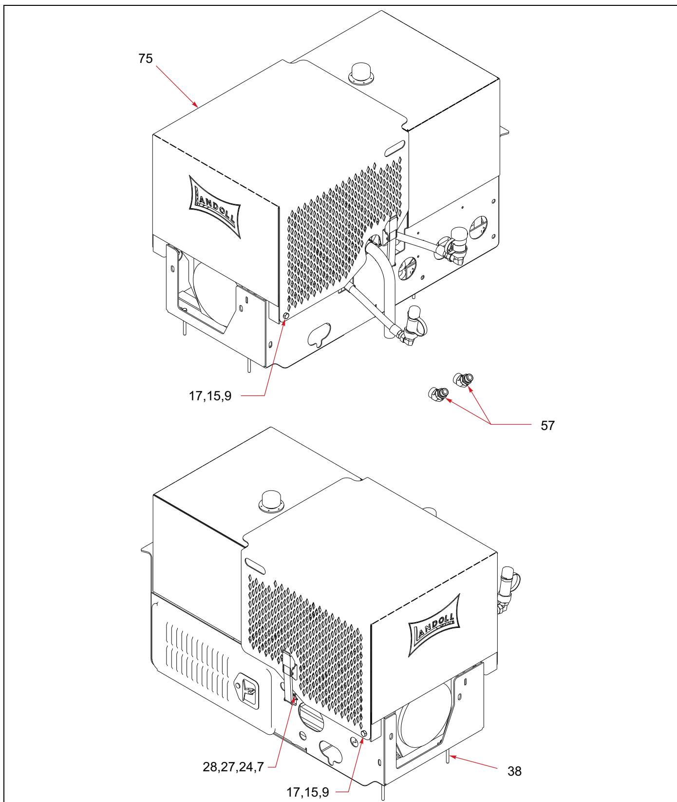
Figure 1-77: 25 HP Upper Deck Engine Package (1 of 4)
