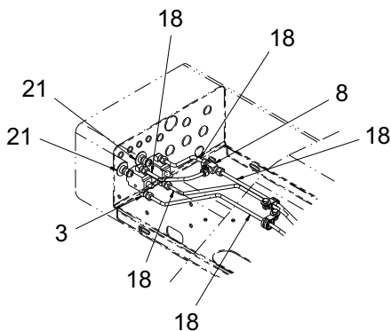
PUSH VALVE ASSEMBLY
