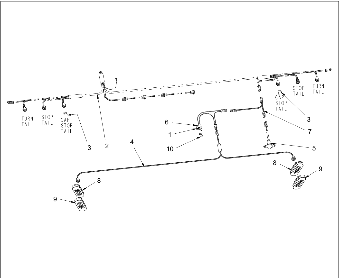
Figure 1-97: Strobe Light - 800E Bumper
