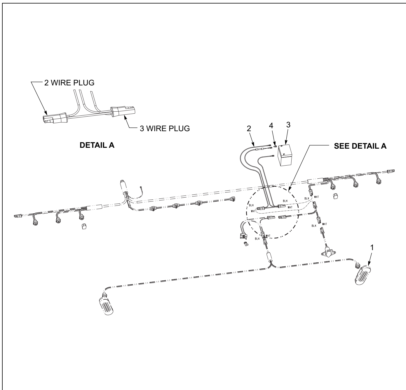
Figure 1-98: Strobe Light - Battery Backup Bumper (Installed on Frame Only)
