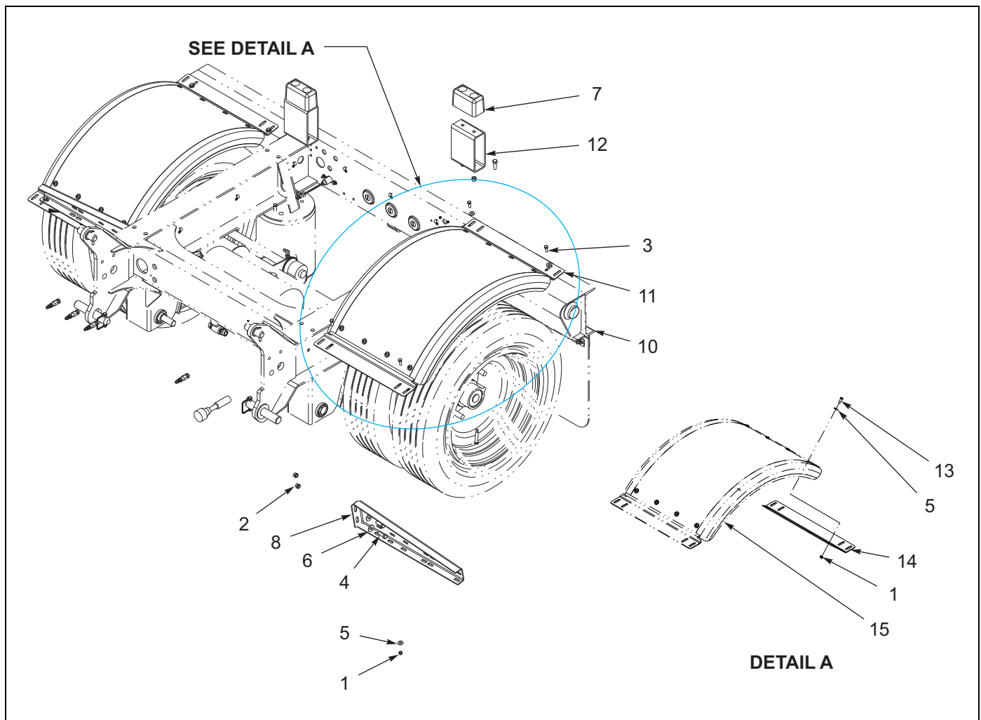
Figure 1-88: Black Poly Fender Installation - Flip Axle
