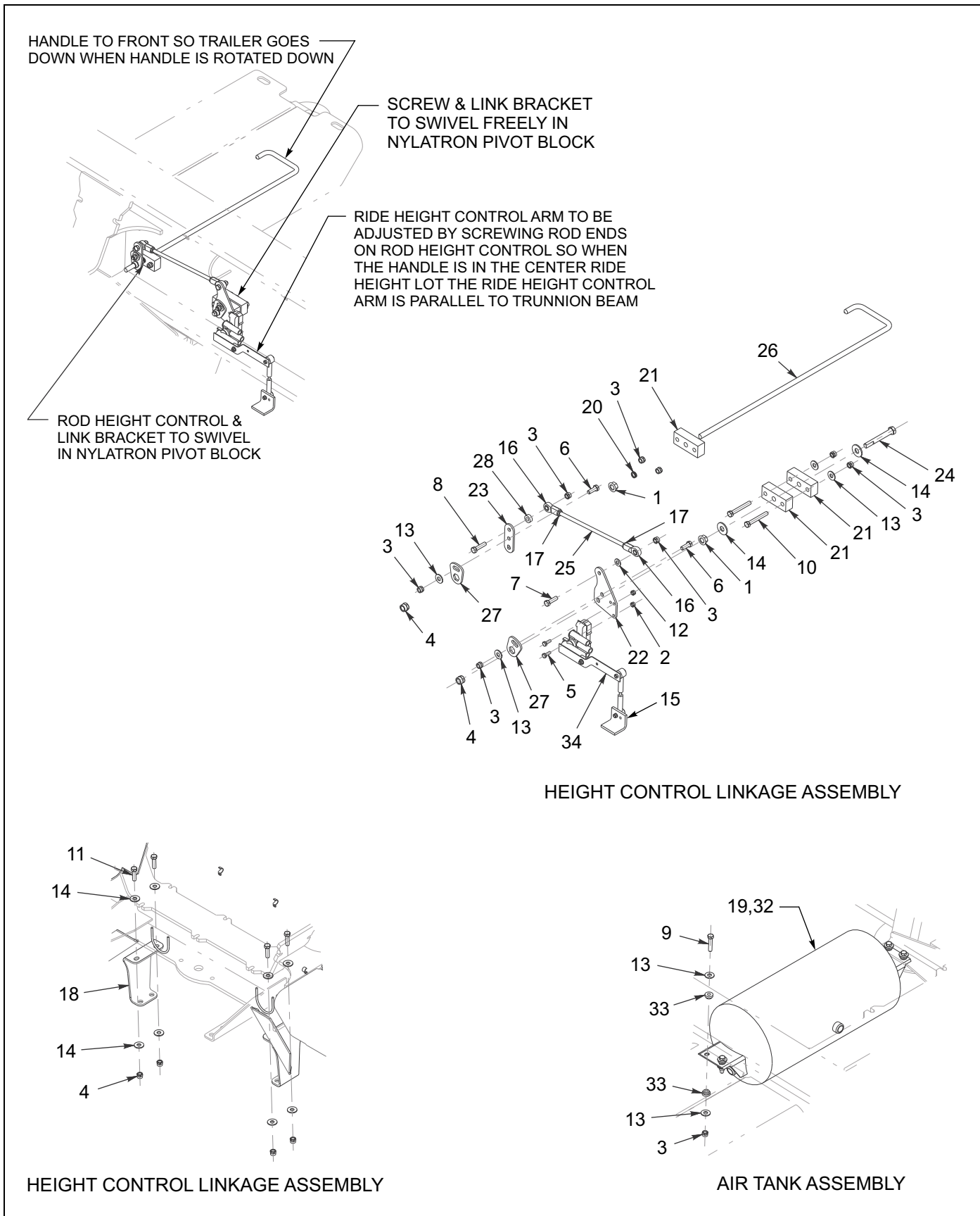
Figure 1-43: General Assembly - 855E Paver (2 of 2)
