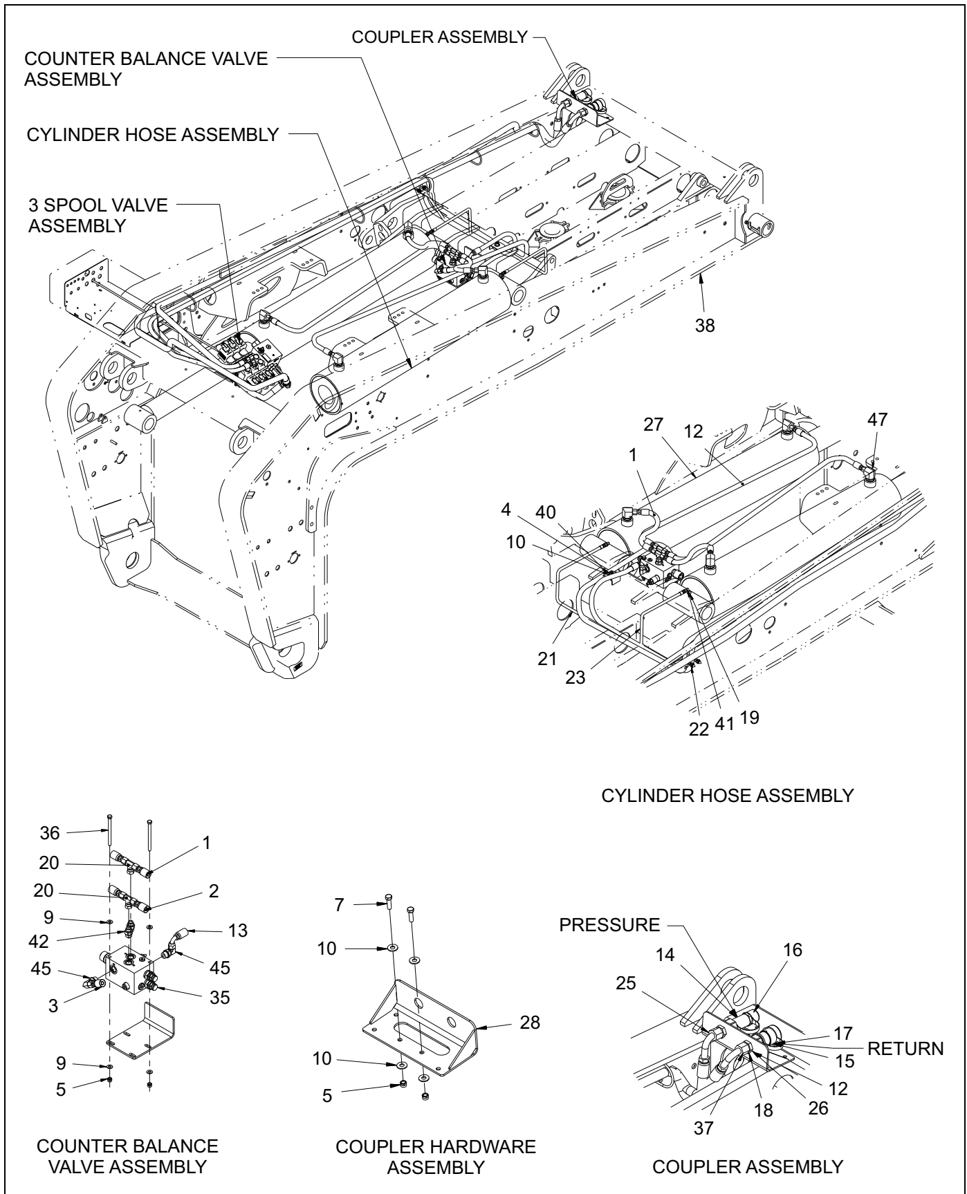
Figure 1-18: Hydraulic & Grease System - 855E HD (1 of 2)
