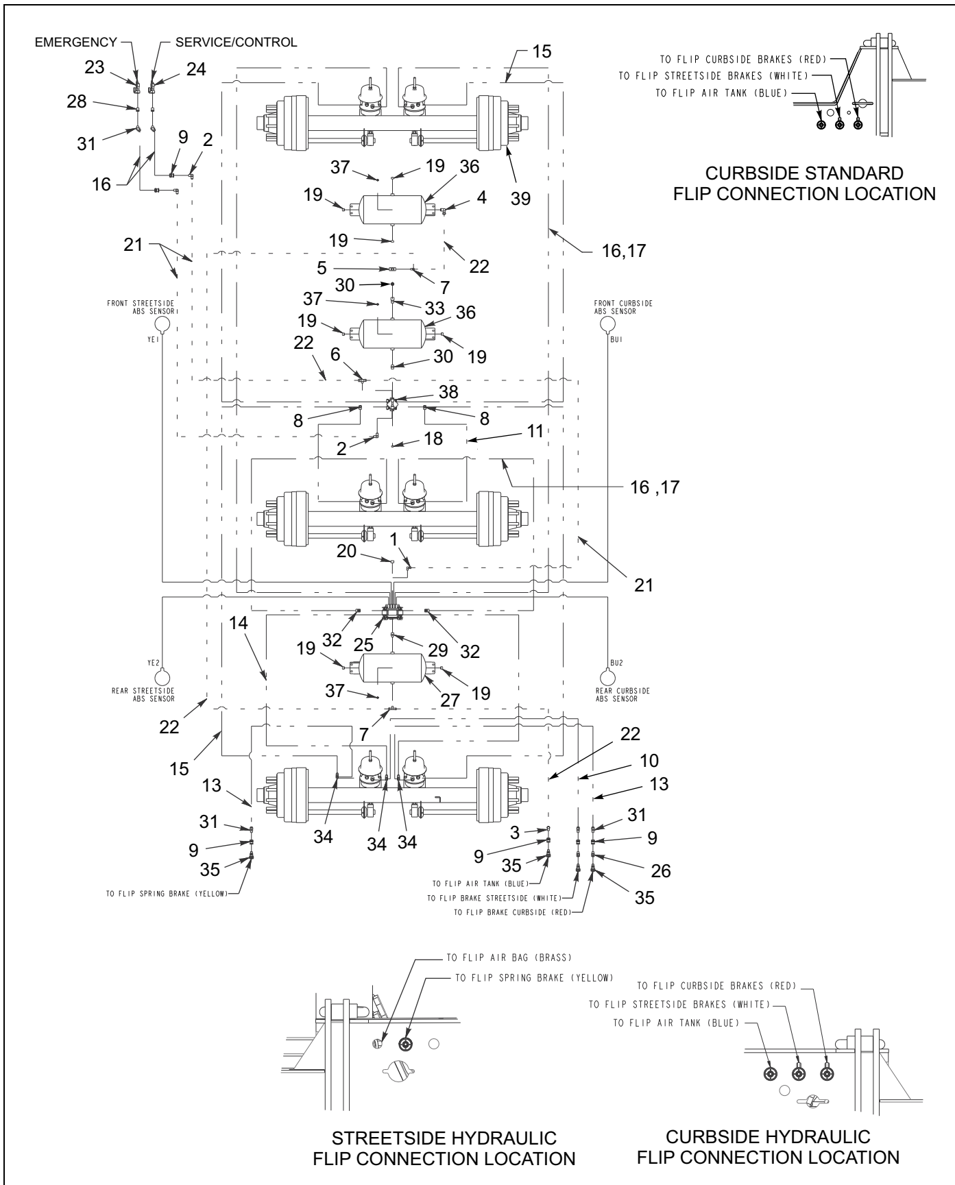
Figure 1-36: Air Brake System - 855E HD {P/N 198492, 198493, 198494, 198515, & 198516} (1 of 2)
