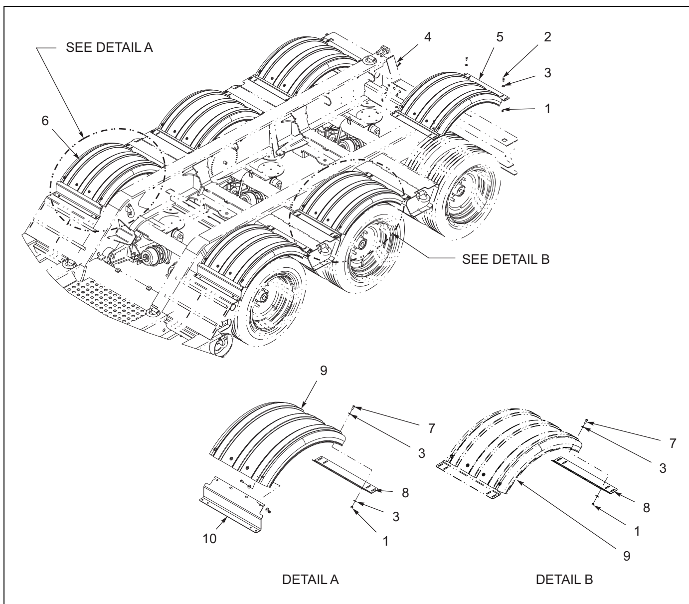
Figure 1-89: Chrome Poly Fender Installation - 3 Axle
