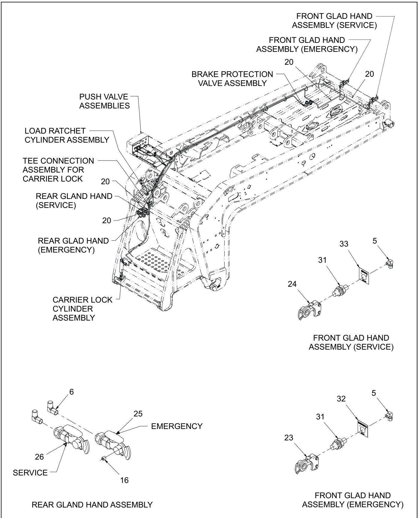
Figure 1-16: Air System - 855E HD (1 of 2)
