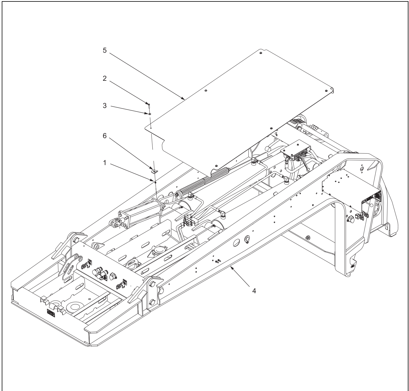
Figure 1-73: Gooseneck Cover Assembly - 855E HD
