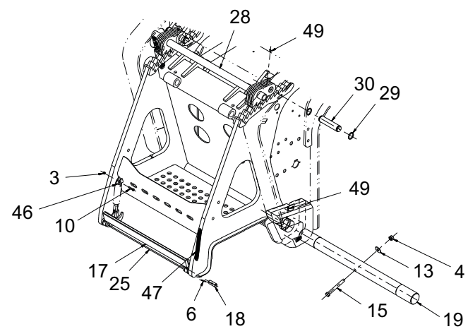
LOAD CARRIER ASSEMBLY
