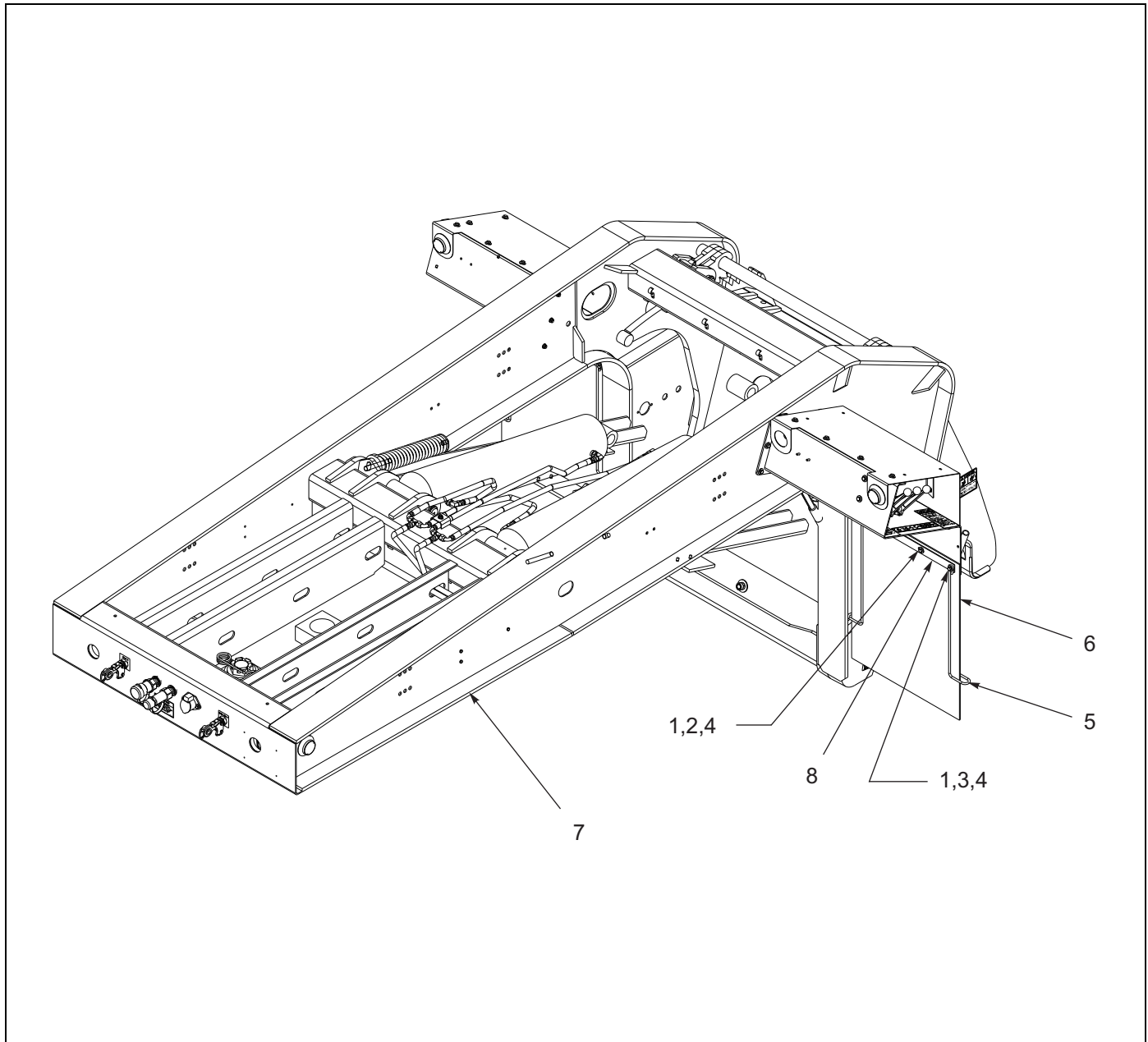
Figure 1-111: Gooseneck Mud Flaps - 855E
