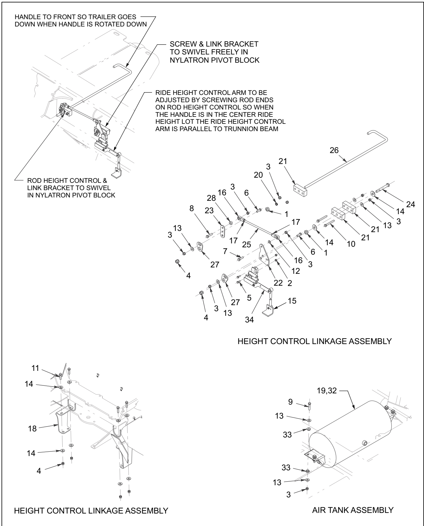
Figure 1-27: General Assembly - 855E (2 of 2)
