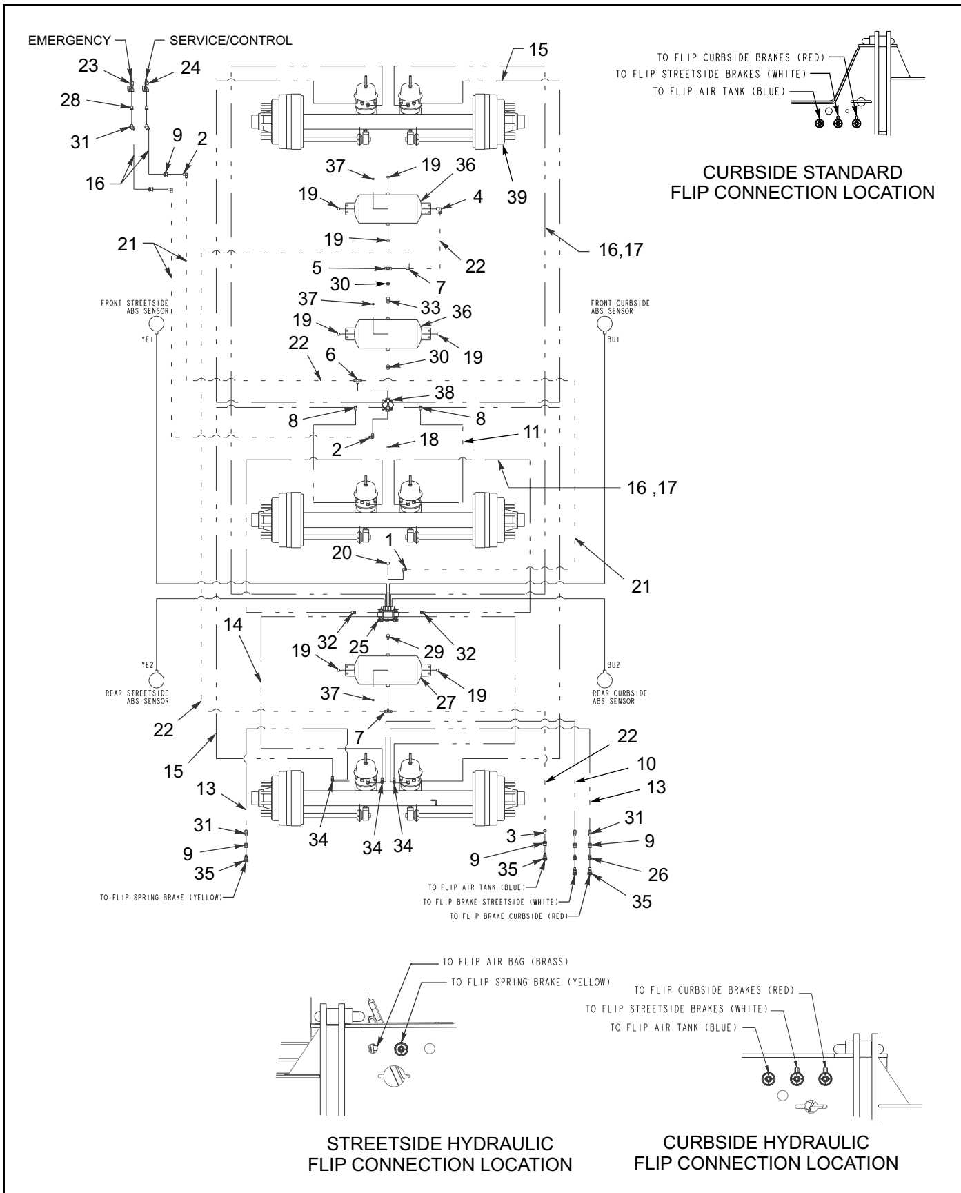
Figure 1-29: Air Brake System - 855E
