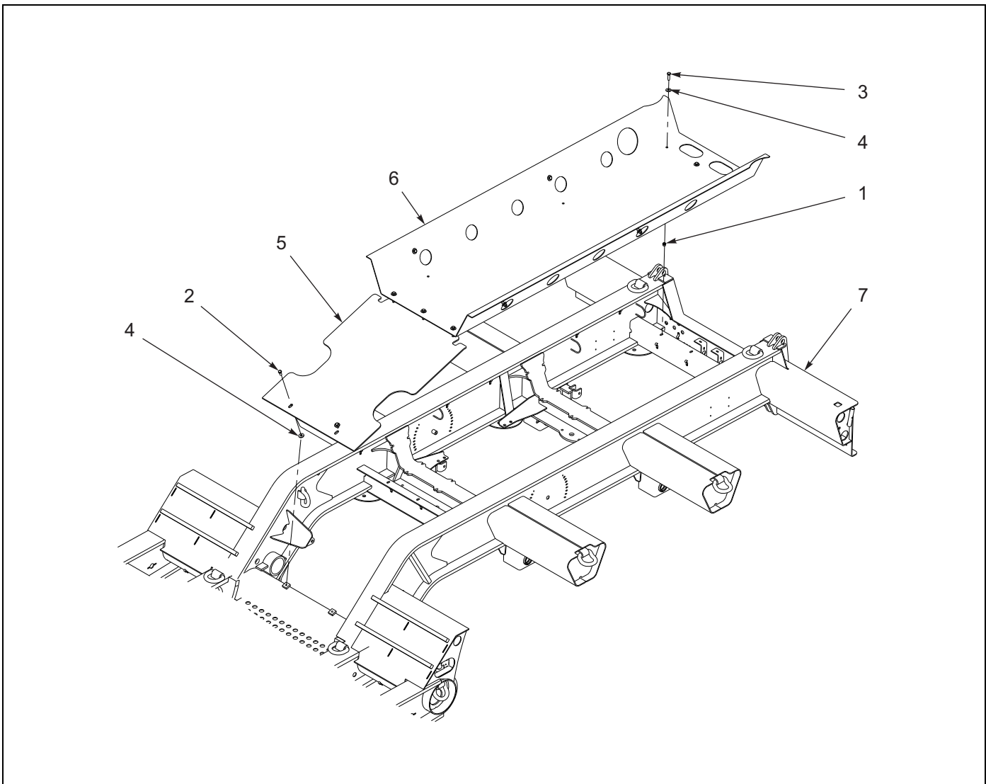
Figure 1-70: Cover Boom Trough Assembly
