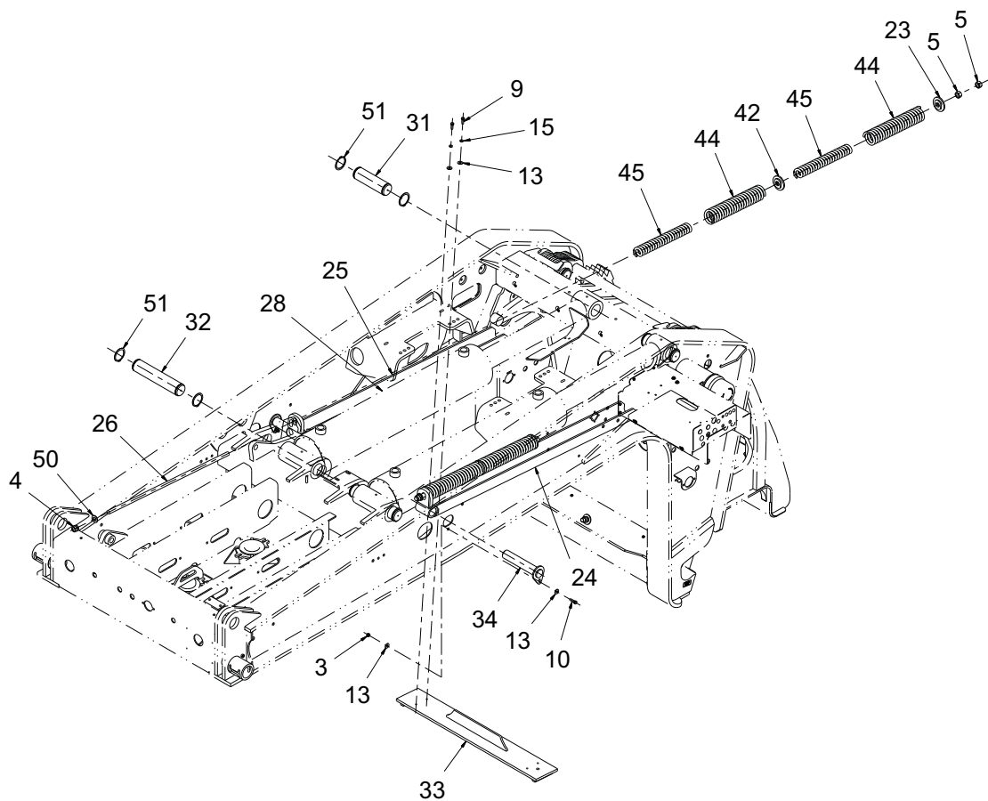
MAIN CYLINDER & SPRING ASSEMBLY
