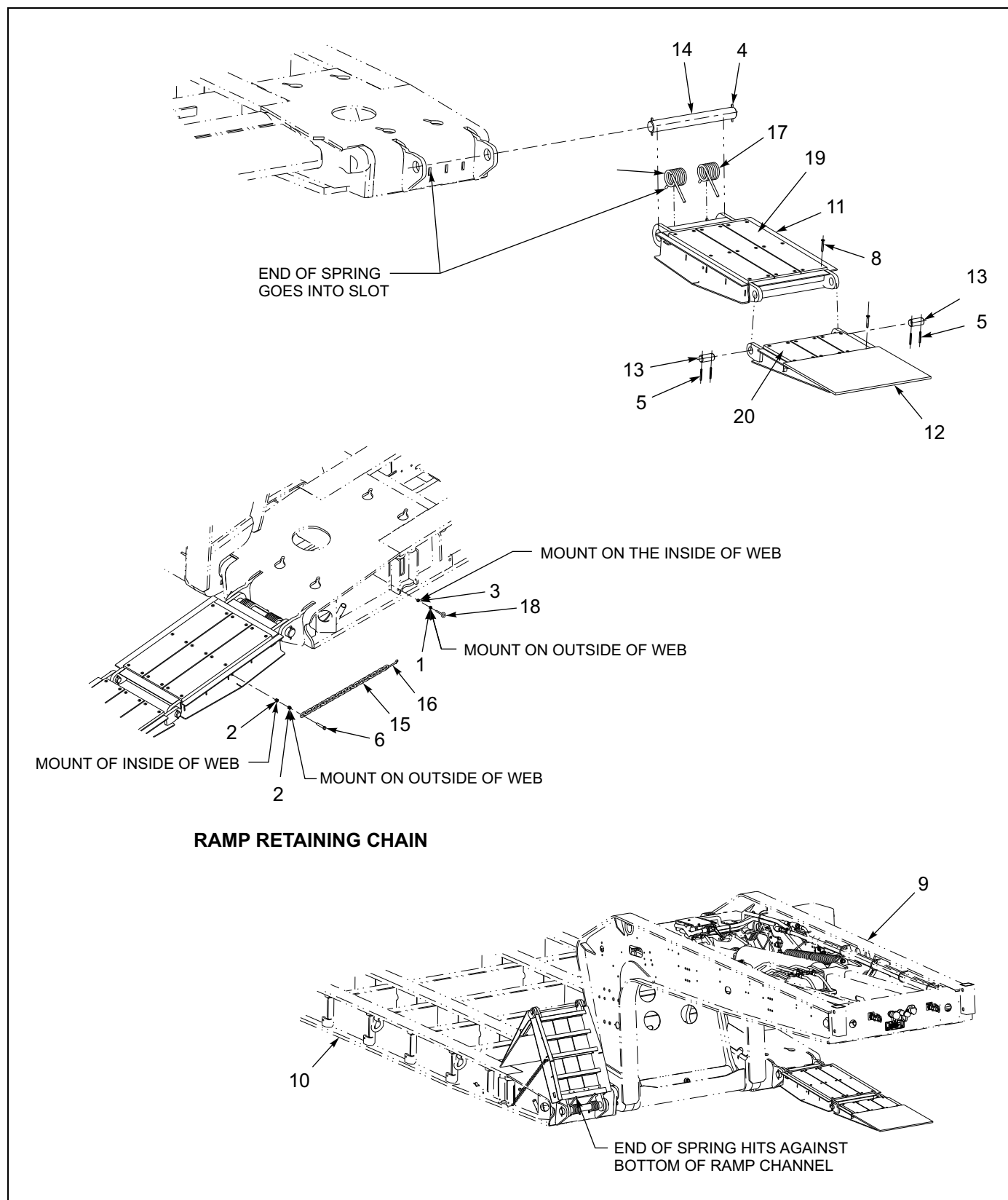
Figure 1-55: Ramp Assembly - Front Bi-Fold (855E Paver)
