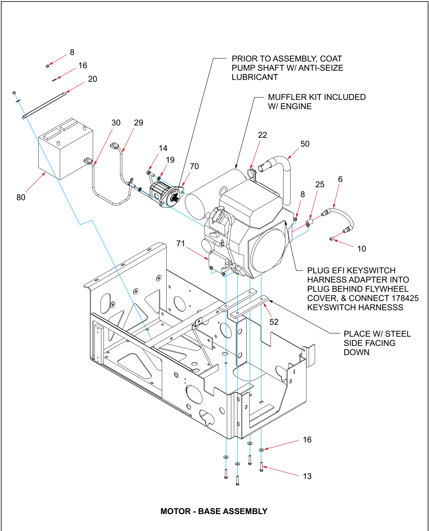
Figure 1-78: 25 HP Upper Deck Engine Package (2 of 4)
