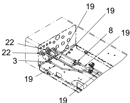
PUSH VALVE ASSEMBLY
