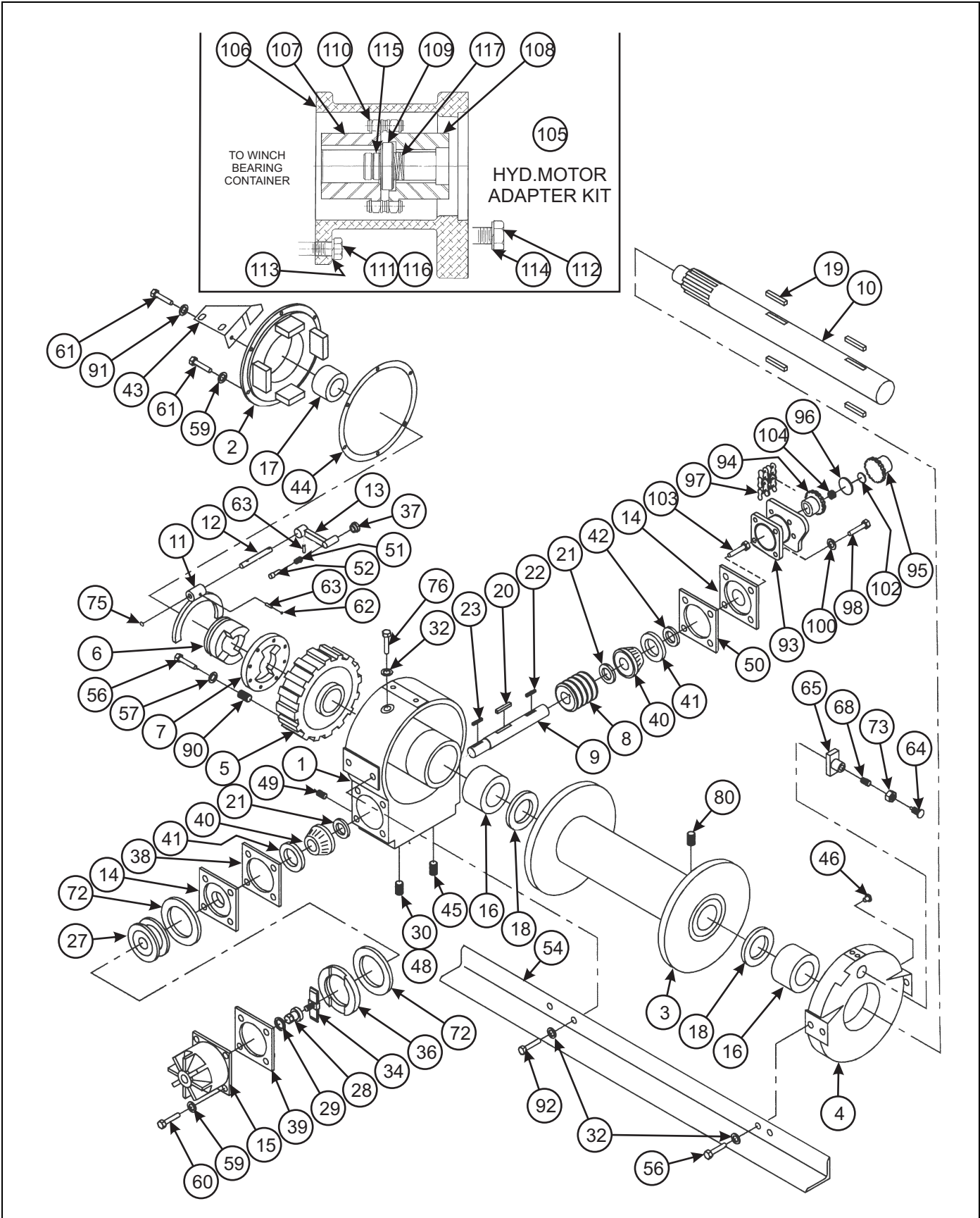
Figure 1-54: Winch Items - 20,000Lb. (BRADEN)
