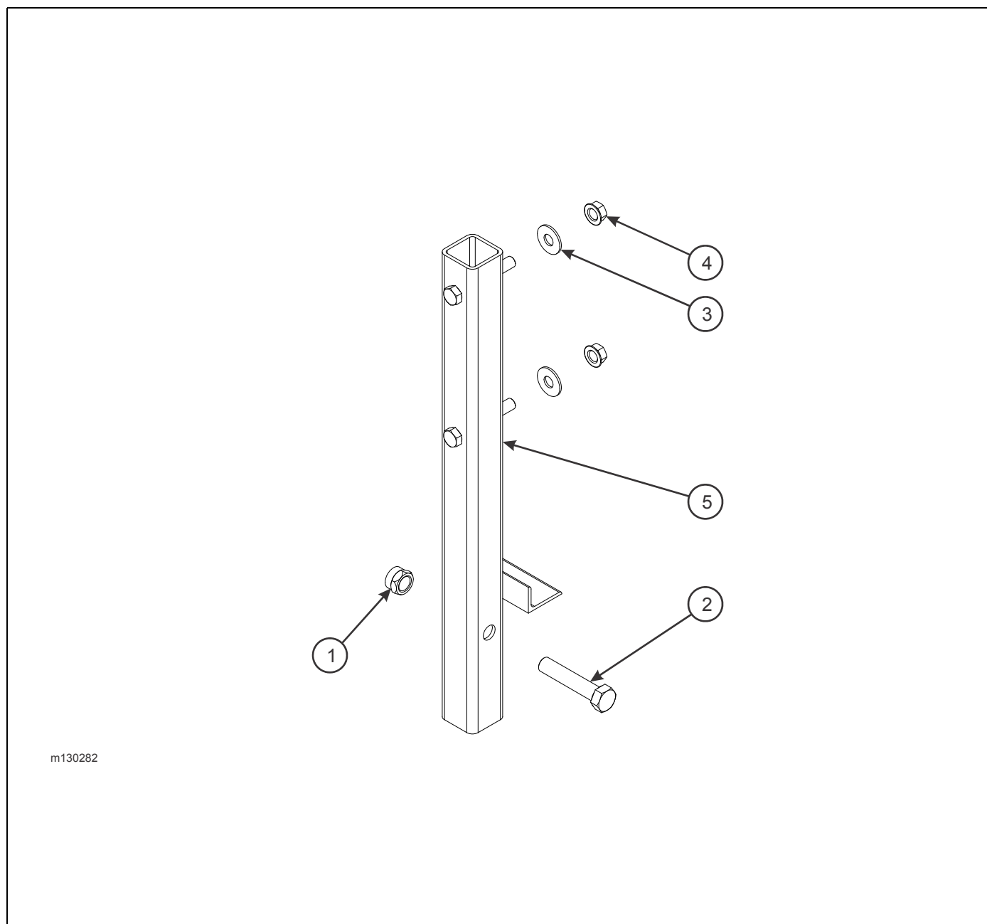
Figure 1-118: Spare Tire - Mount Assembly
