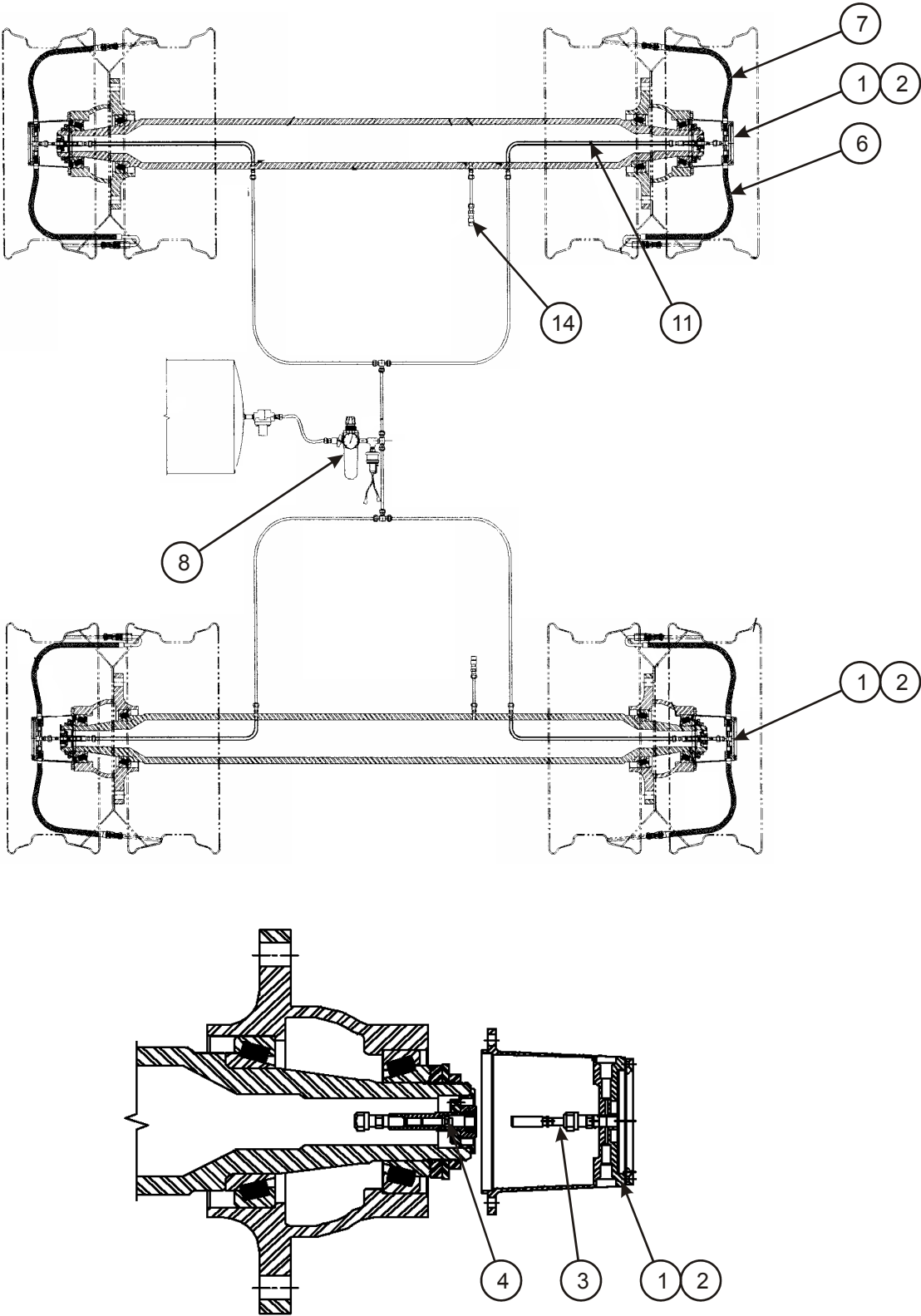
Figure 1-42: Tire Inflation System - 2AX/3AX (Option)
