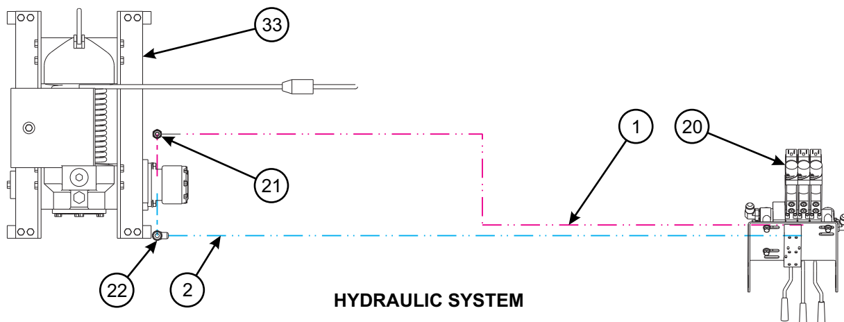
Figure 1-45: Winch Installation - 12K Upper Deck (BRADEN) (2 of 2)
