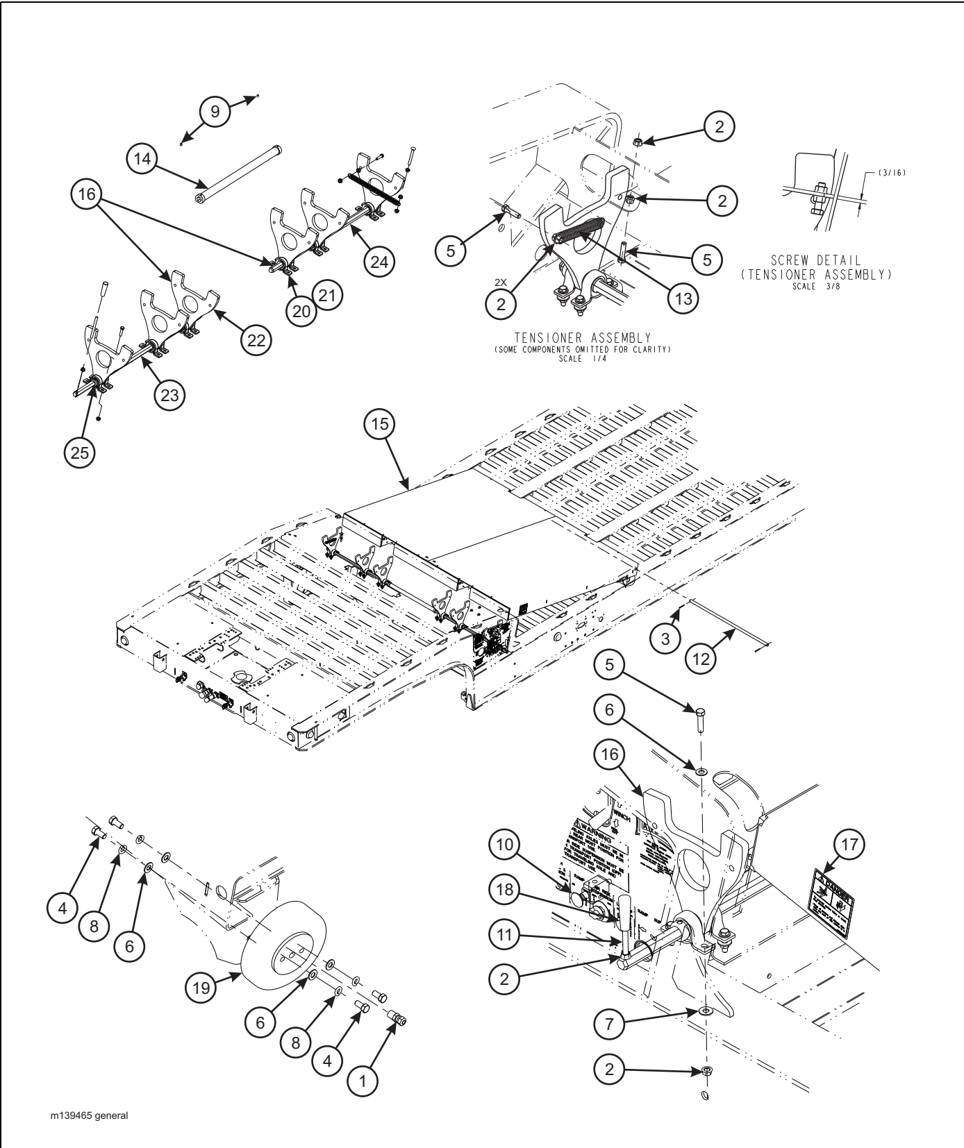
Figure 1-5: 6' Air Ramp - General Assembly
