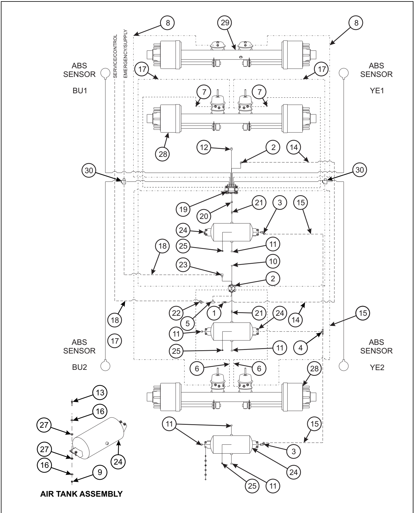
Figure 1-34: Air Brake System - 950C
