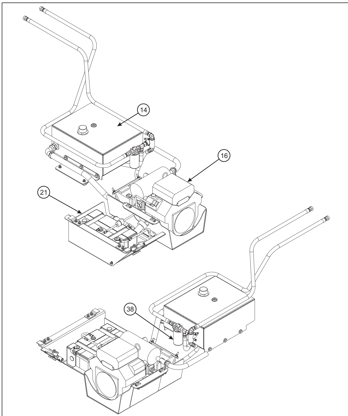
Figure 1-95: Engine - 27 HP Slope Package (1 of 4)
