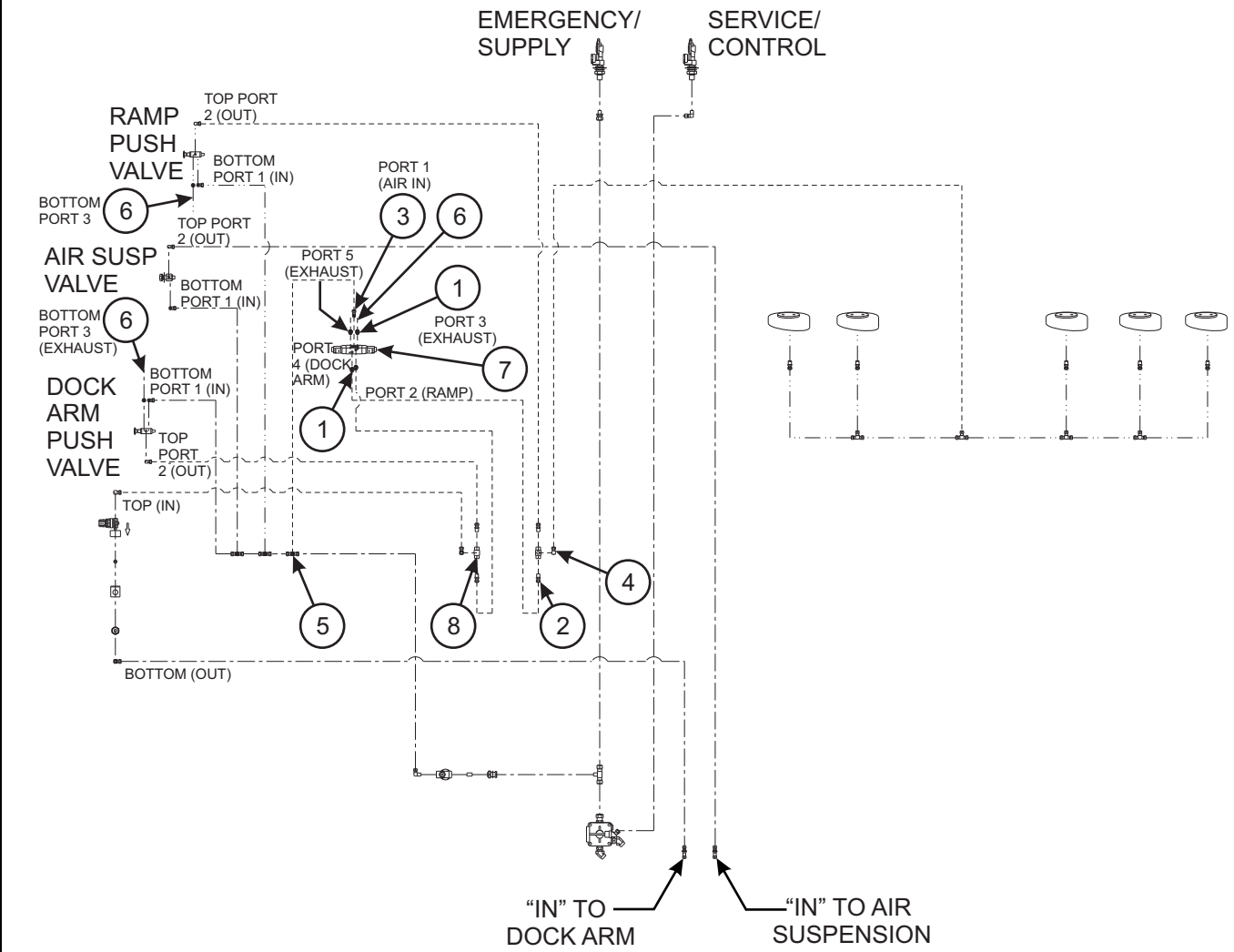
Figure 1-115: Remote Control - Ramp and Dock Lift Air Items
