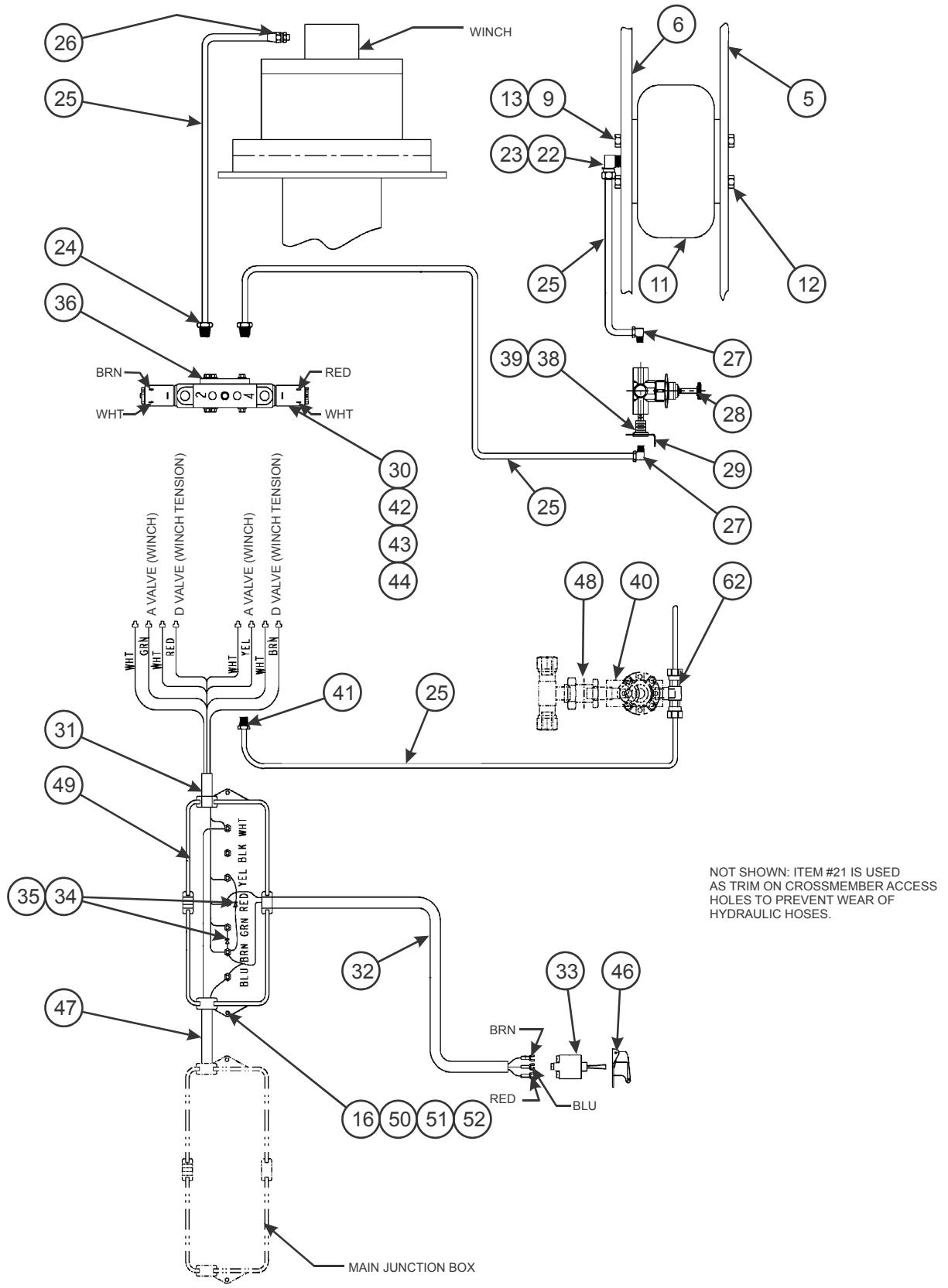
Figure 1-64: Winch Installation - 12K, 15K, & 20K Upper Deck (DP) (2 of 2)
