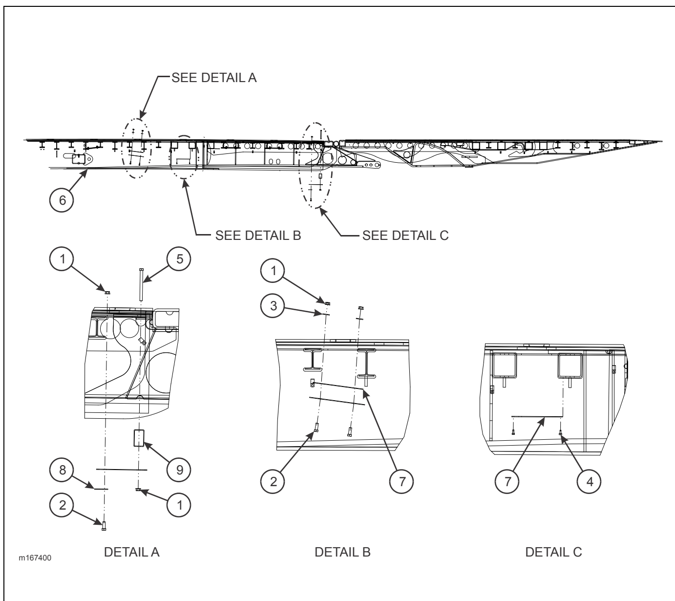
Figure 1-117: Shield Installation - Center Gotcha
