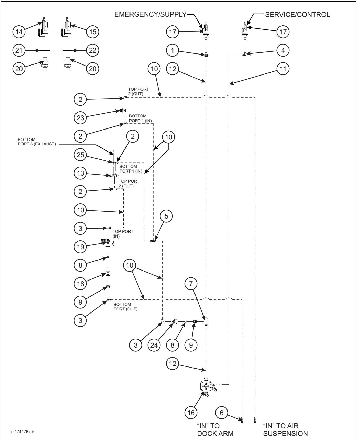
Figure 1-9: Air System
