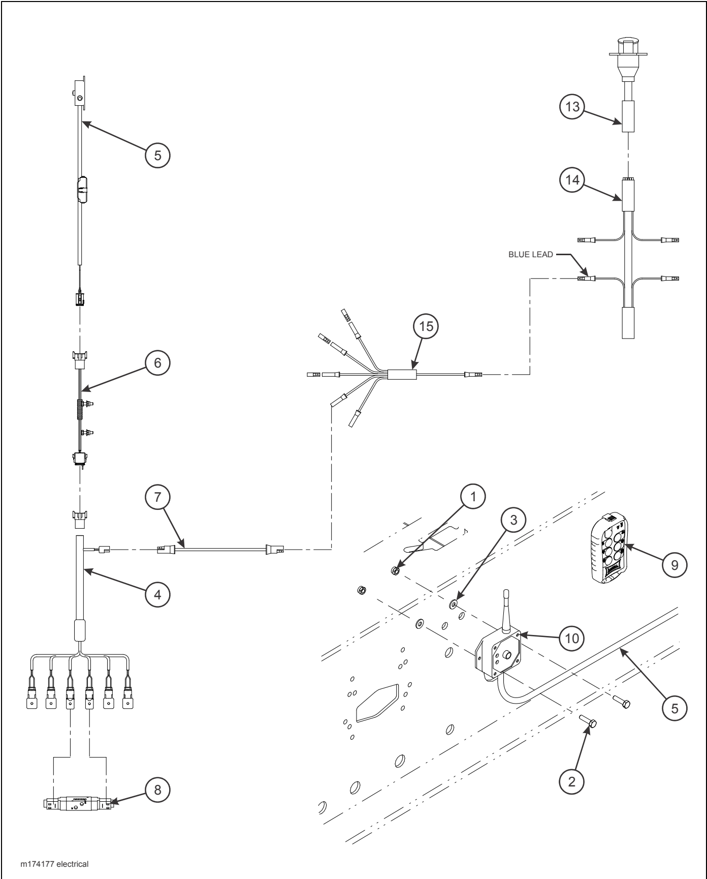
Figure 1-19: Remote Control - Electrical System
