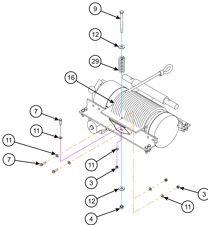
SPRING TENSIONER ASSEMBLY
