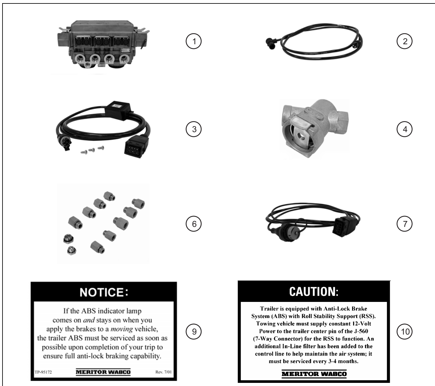
Figure 1-36: ABS Brake Kit - w/ RSS Rockwell
