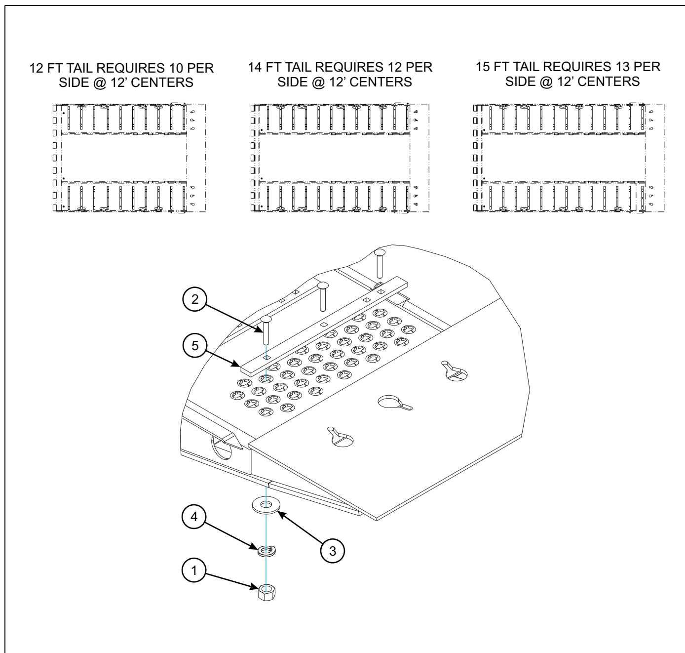
Figure 1-126: Traction Bar Assembly
