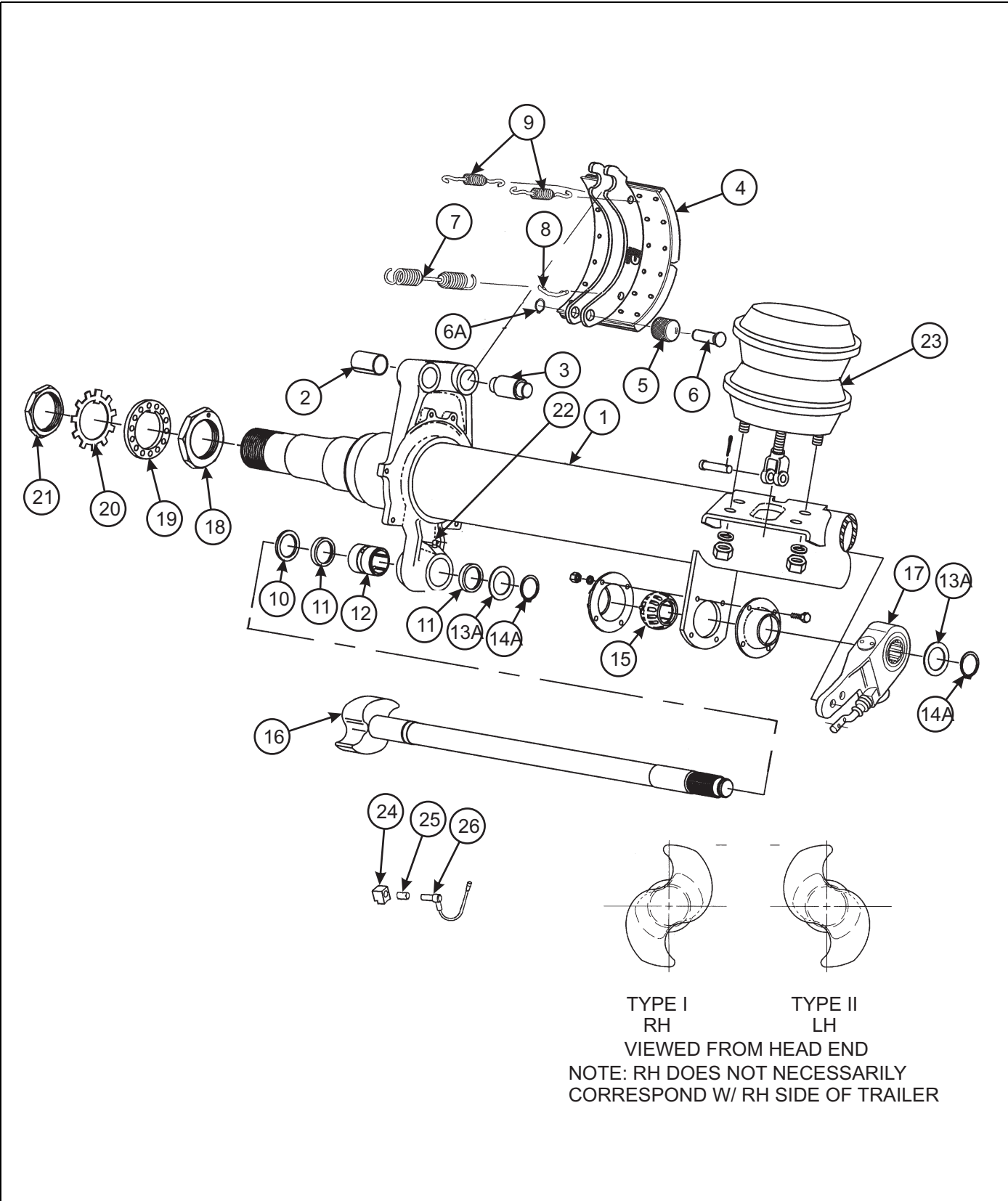
Figure 1-37: Axle and Brake Assembly - Dexter 12-1/4" X 7-1/2"
