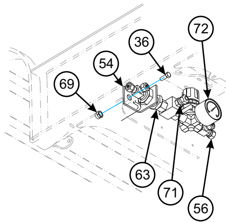
BRACKET ASSEMBLY
