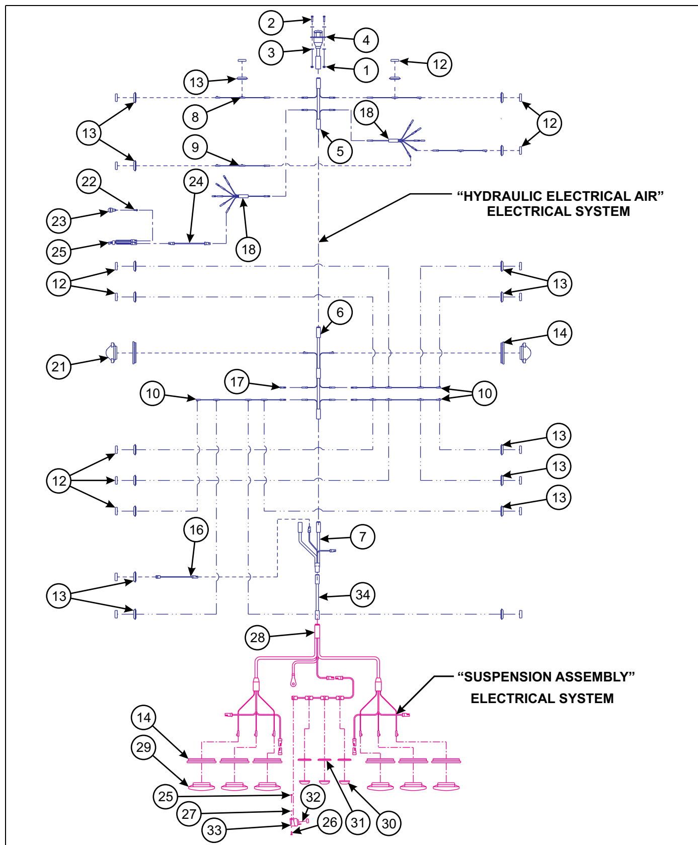
Figure 1-17: Electrical System
