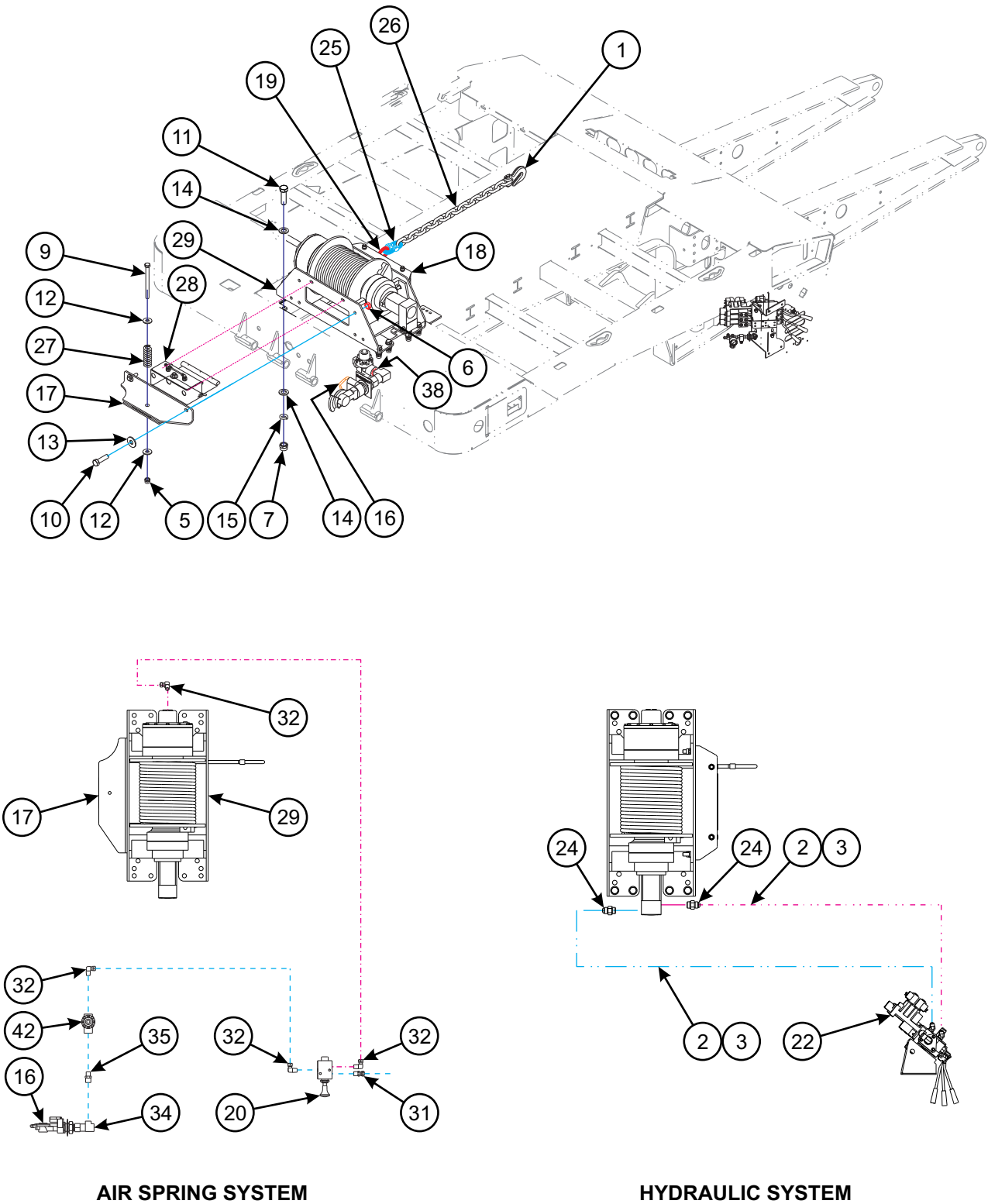
Figure 1-66: Winch Installation - 30K Upper Deck (DP) (1 of 2)
