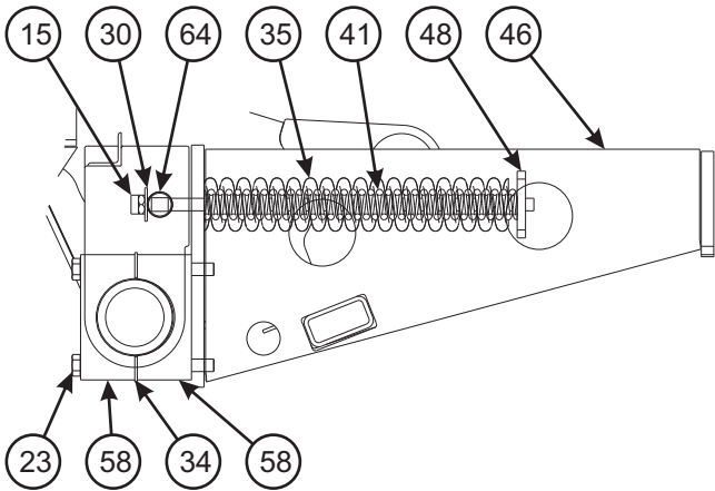
TAIL ASSEMBLY
