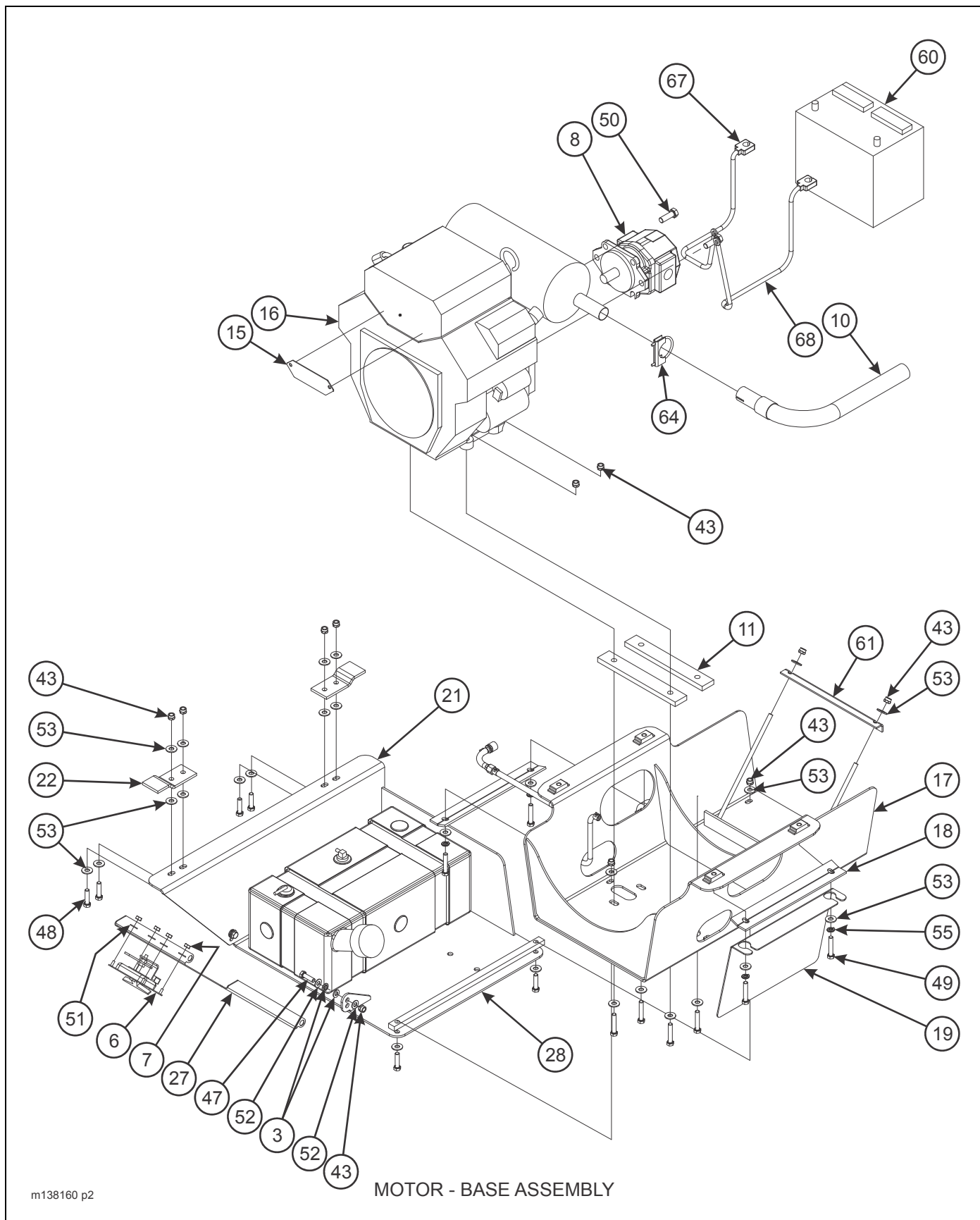
Figure 1-96: 27 HP Slope Engine Package (2 of 4)
