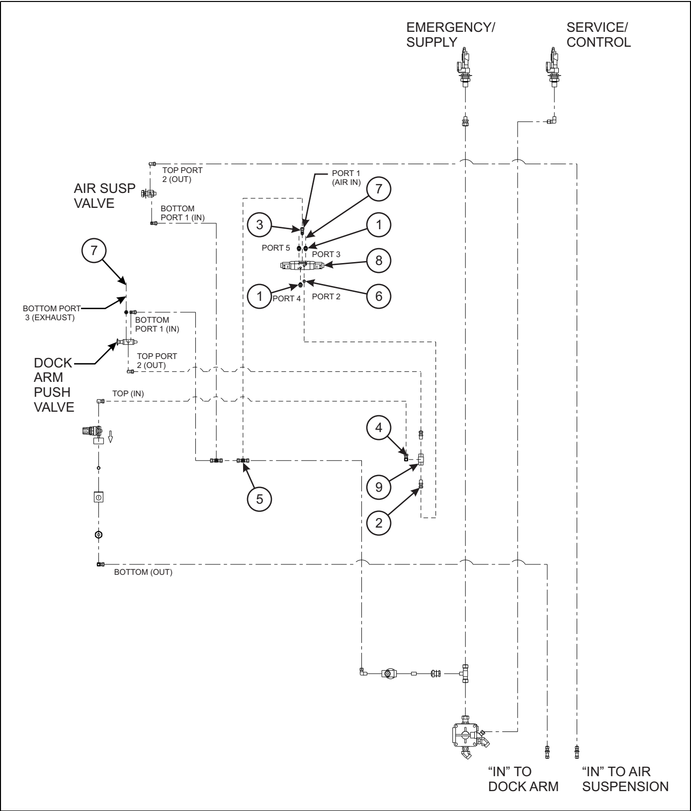
Figure 1-114: Remote Control - Dock Lift Air Items
