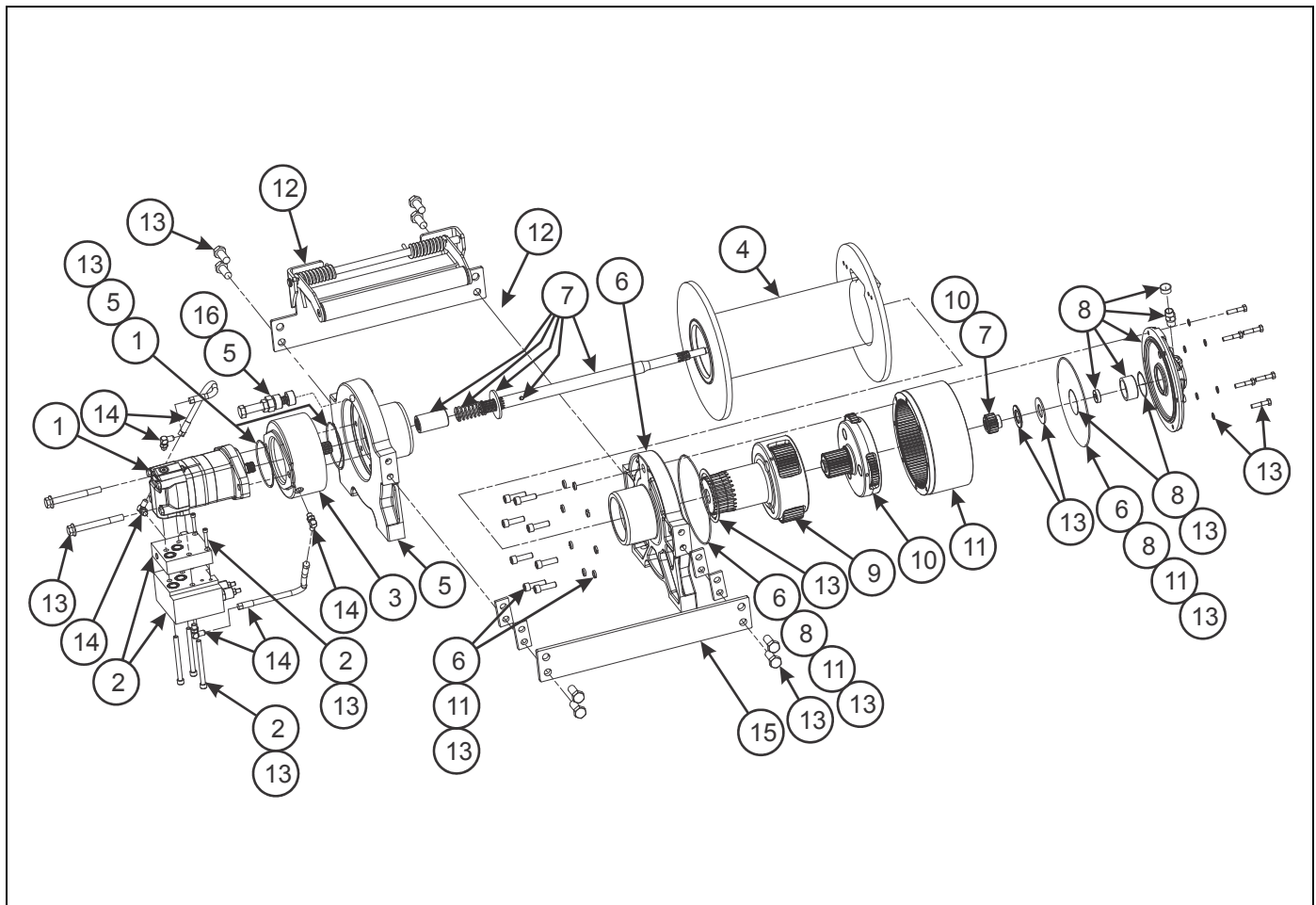
Figure 1-59: Winch Items - 20K (WARN)
