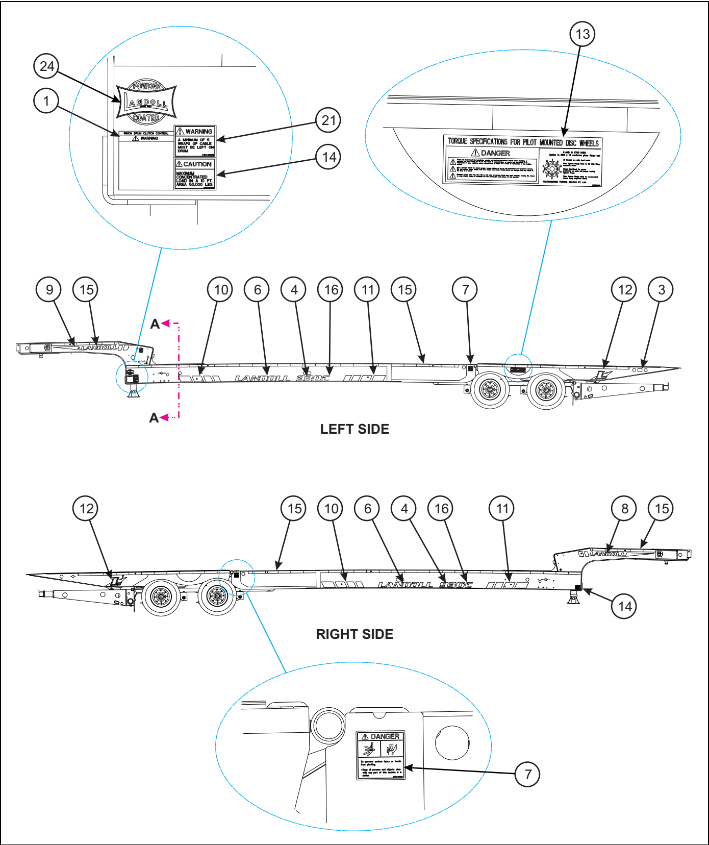
Figure 1-75: Decal Installation (1 of 2)
