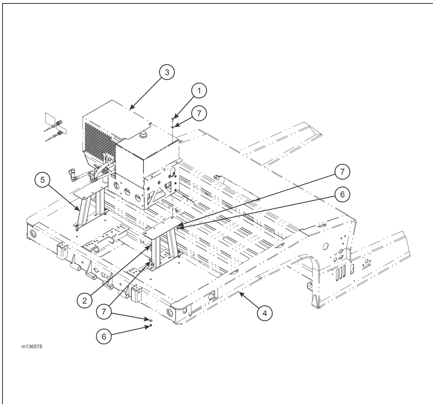
Figure 1-106: Engine - Upper Deck Stand Installation
