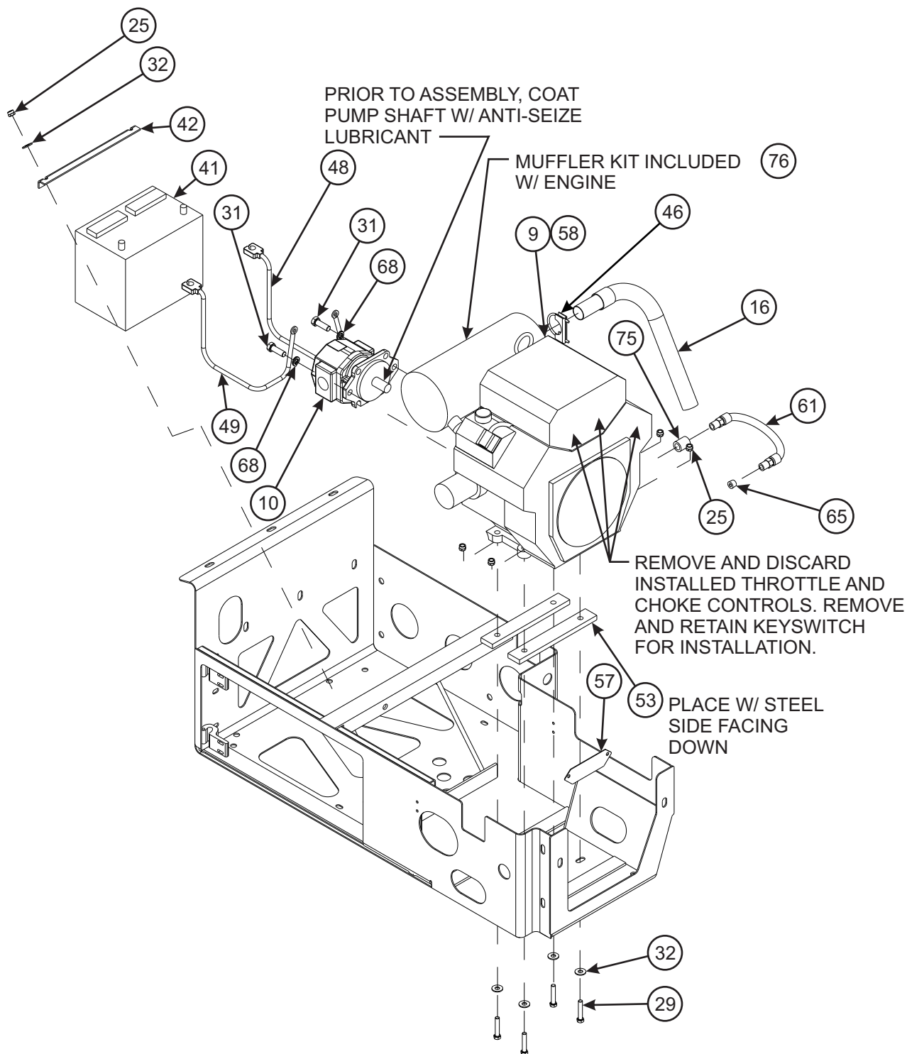
MOTOR - BASE ASSEMBLY
