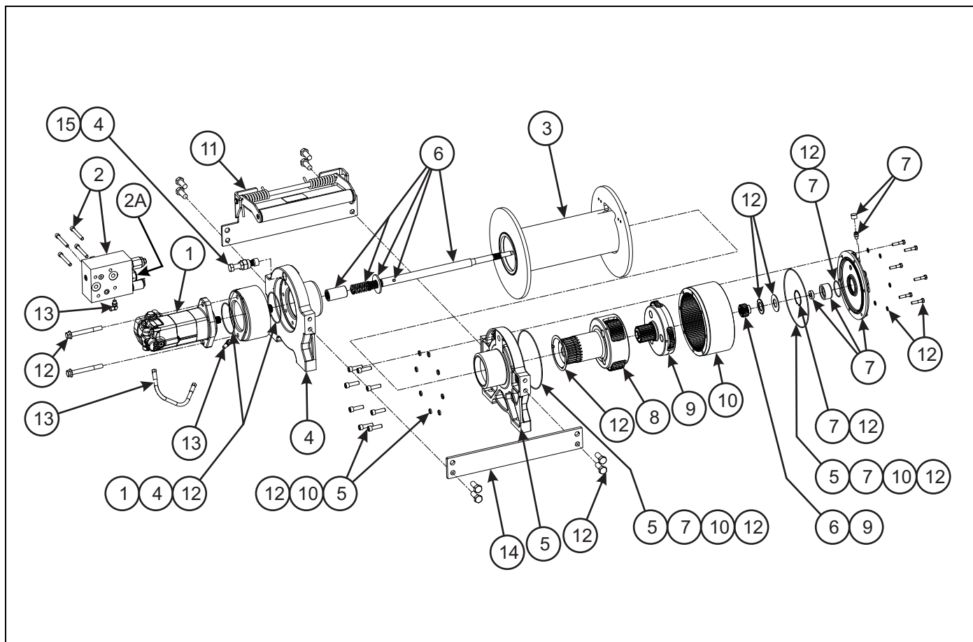
Figure 1-62: Winch Items - 20K 2 Speed (WARN)
