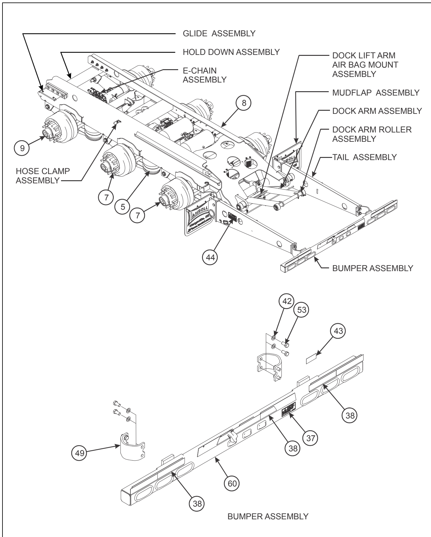
Figure 1-23: General Items - 950C (1 of 3)
