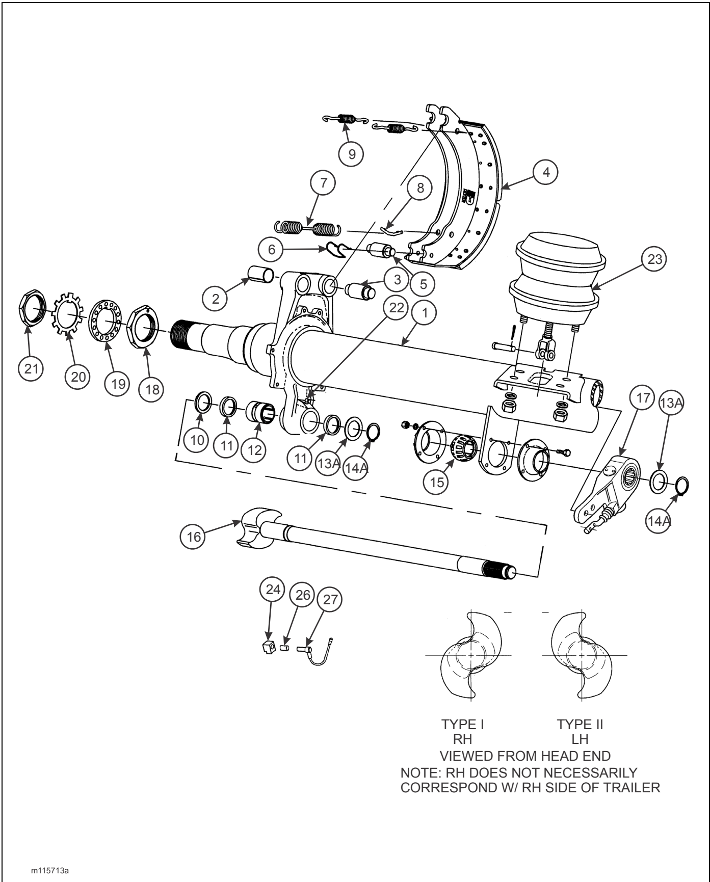
Figure 1-38: Axle and Brake Assembly - Dexter 16-1/2" X 7"
