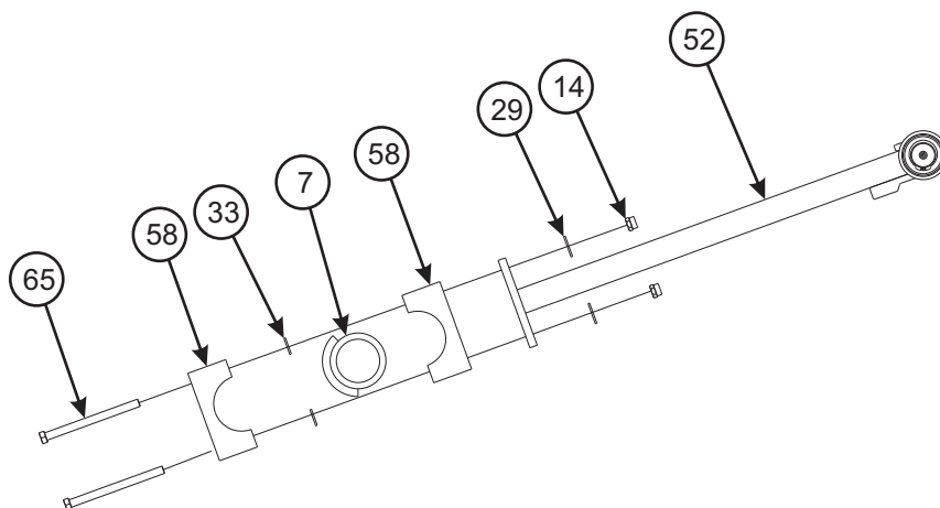
DOCK ARM ASSEMBLY
