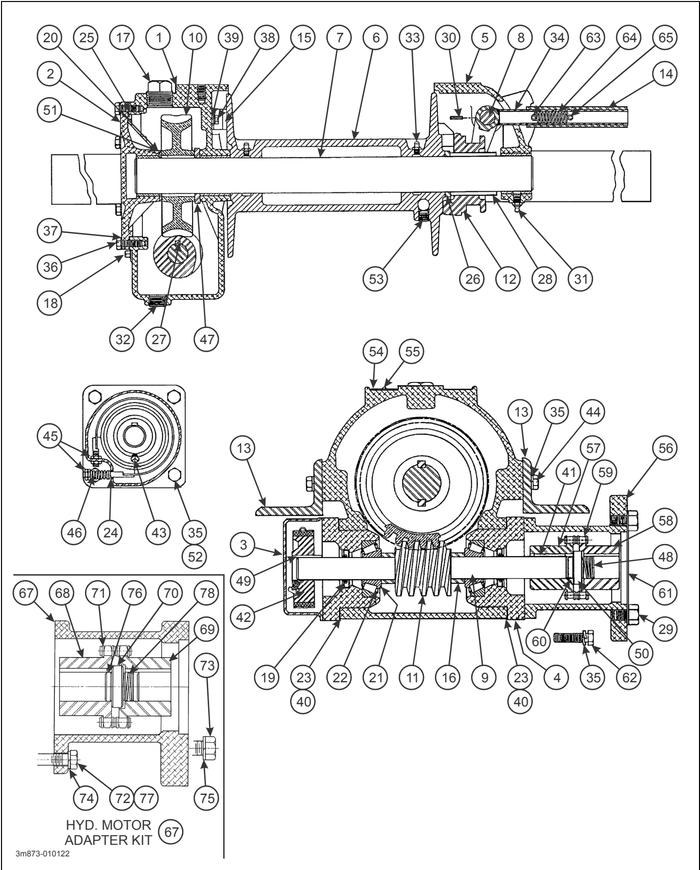
Figure 1-48: Winch Items - 12,000 Lb. (BRADEN)
