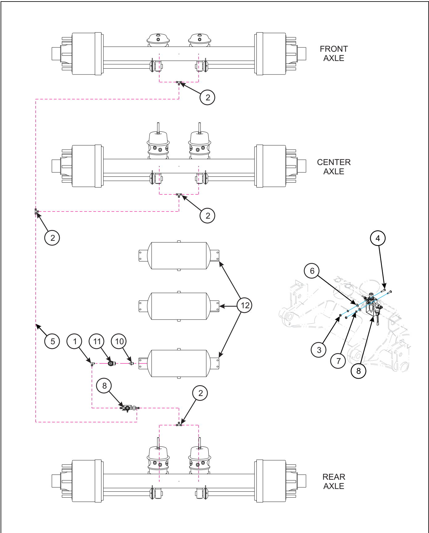
Figure 1-41: Tire Inflation System - 950C
