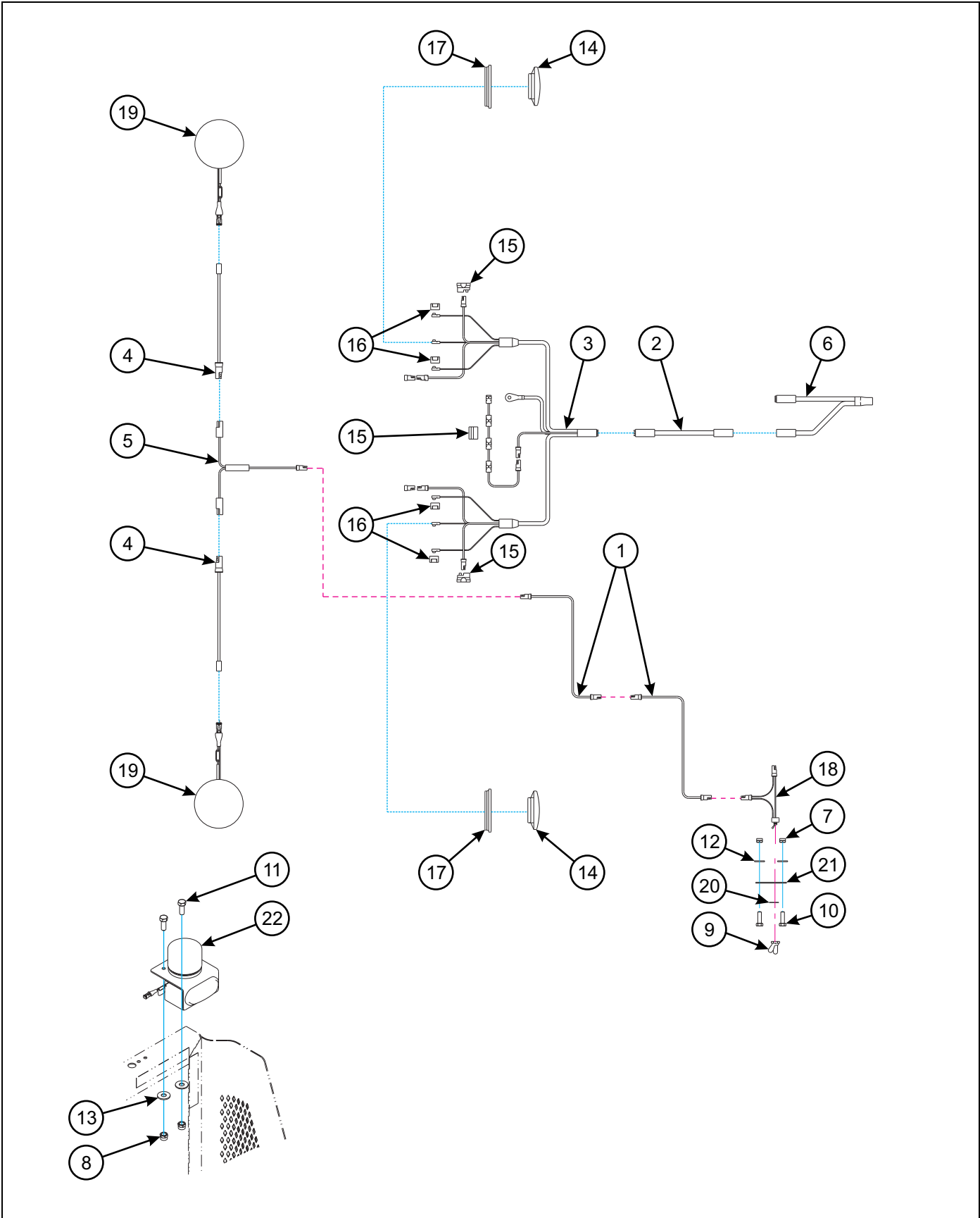
Figure 1-89: Bulkhead - Strobe and Turn
