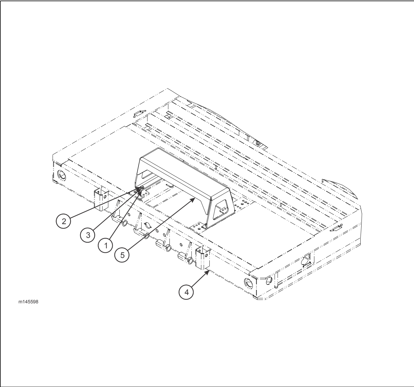
Figure 1-130: Winch - 12K/20K Guard Installation (BRADEN)
