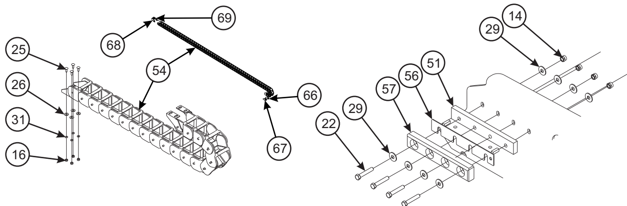
E-CHAIN ASSEMBLY
