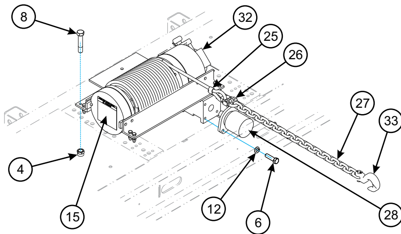
WINCH ASSEMBLY
