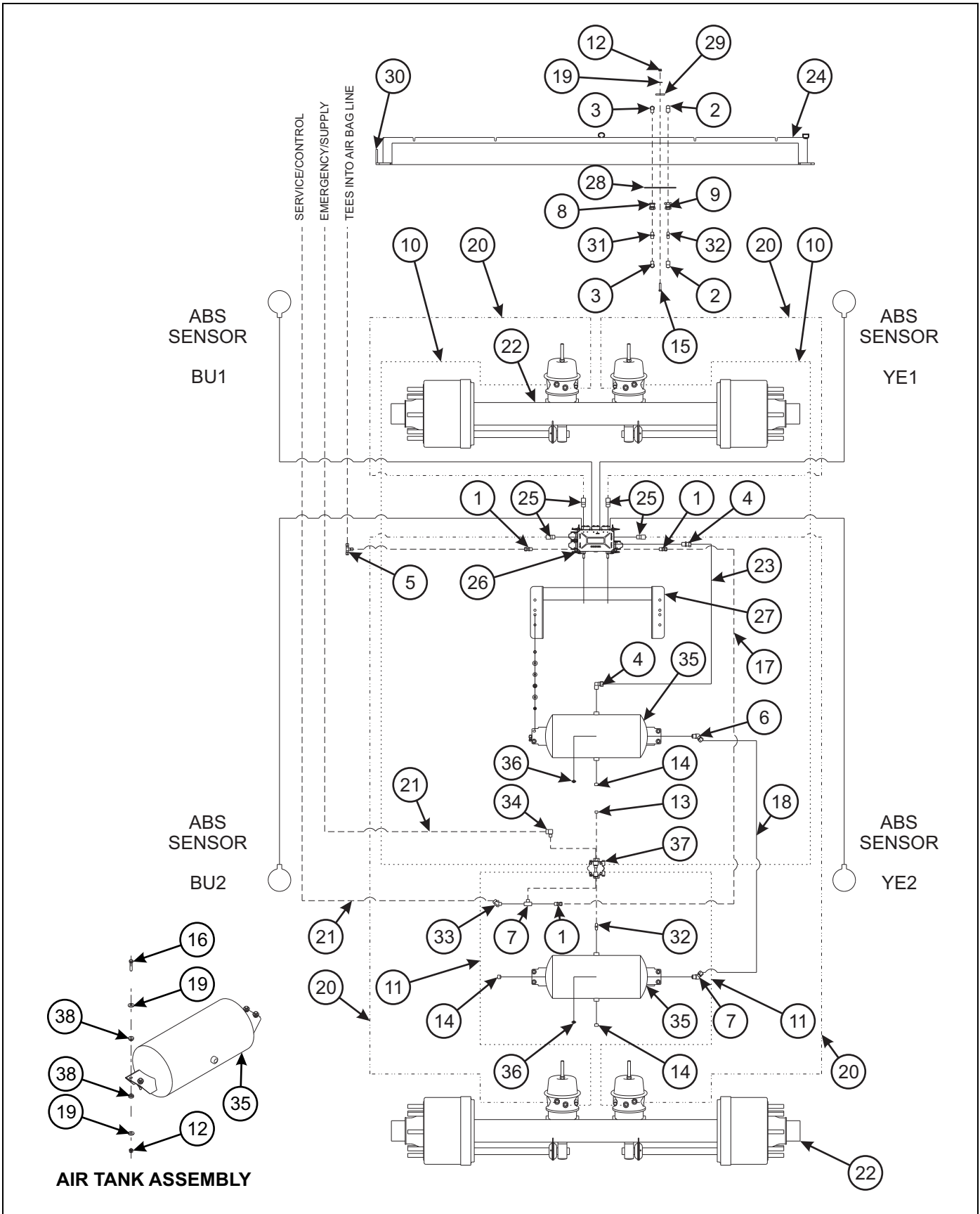
Figure 1-33: Air Brake System - 930C w/ Role Stability Support
