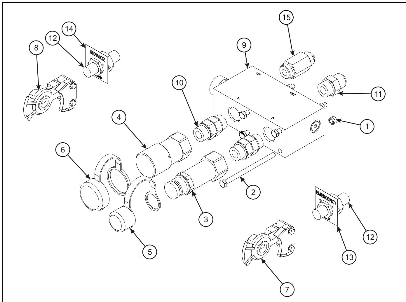
Figure 1-11: Hydraulic Air Connectors - Flow Control
