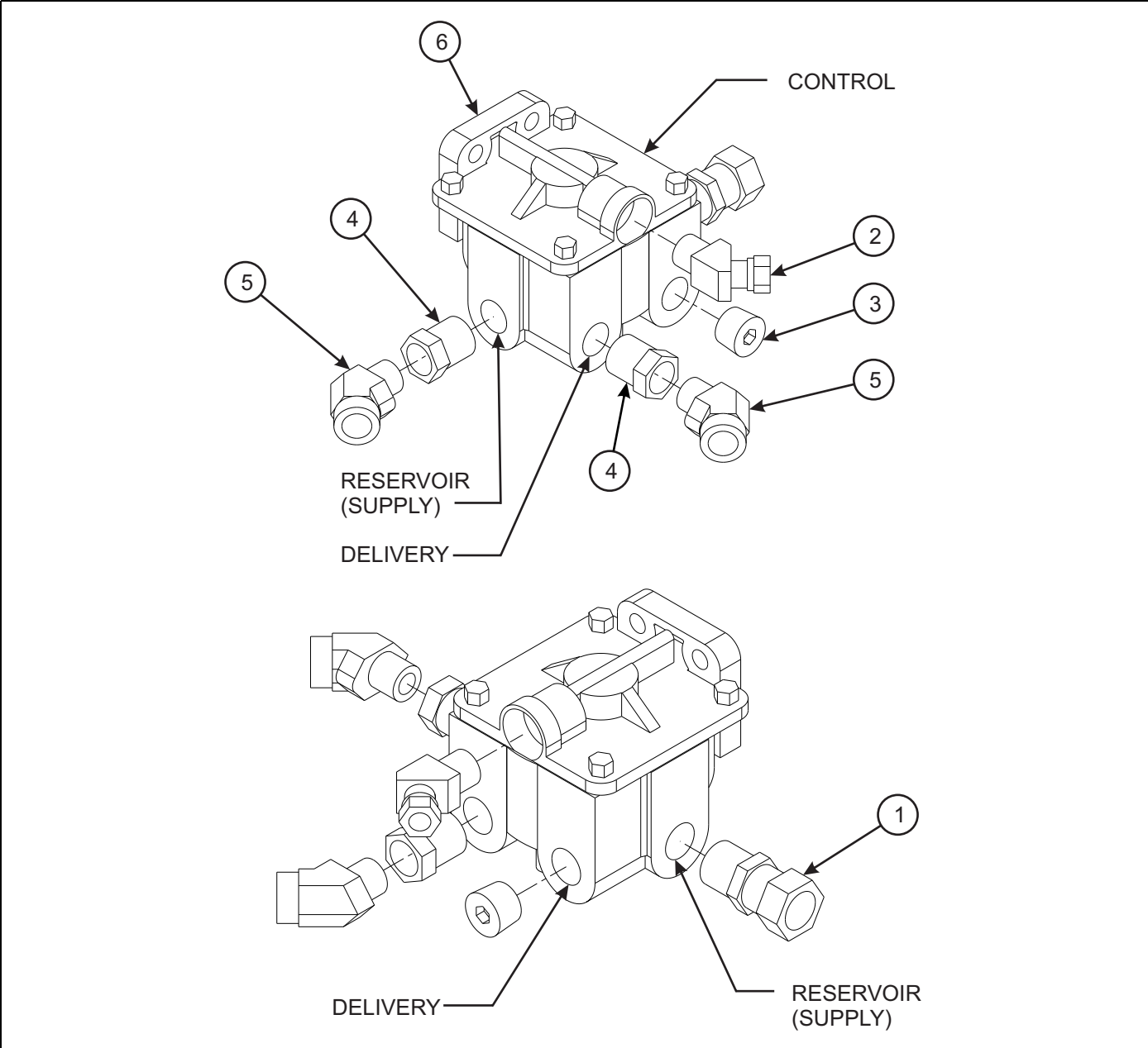
Figure 1-12: Valve Assembly - Air Booster
