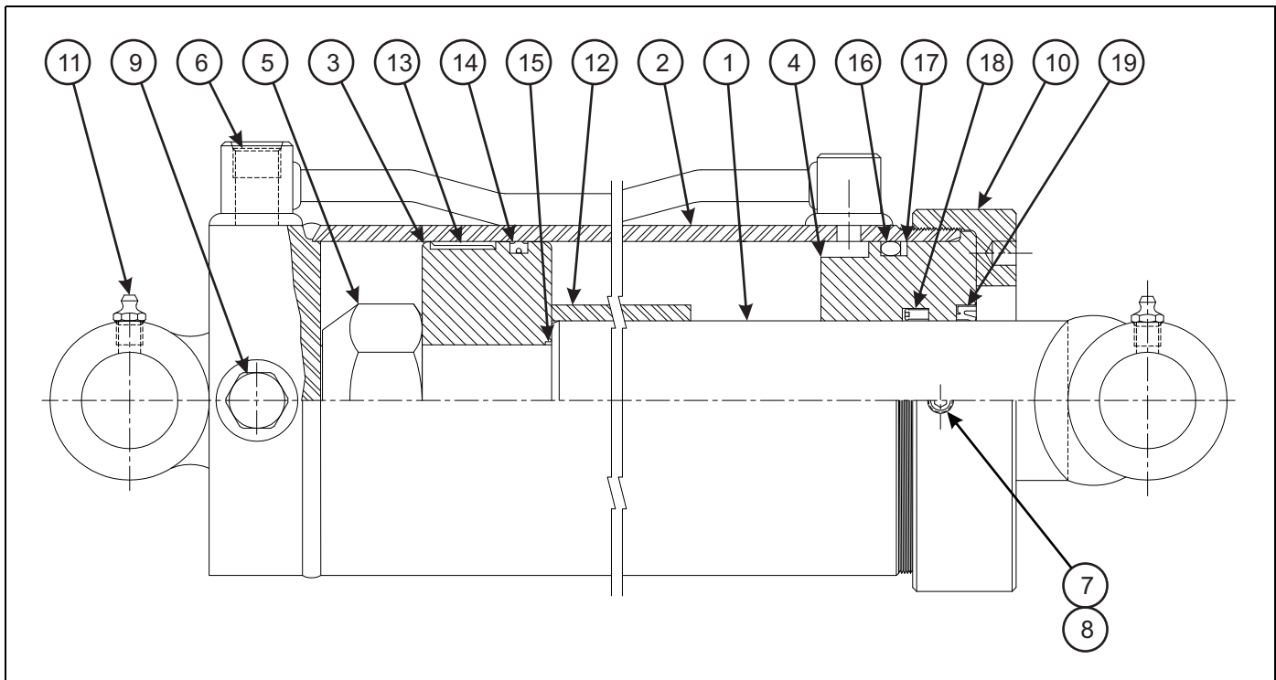
Figure 1-10: Hydraulic Cylinder - 5 x 60
