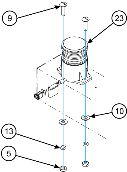
STROBE LIGHT ASSEMBLY
