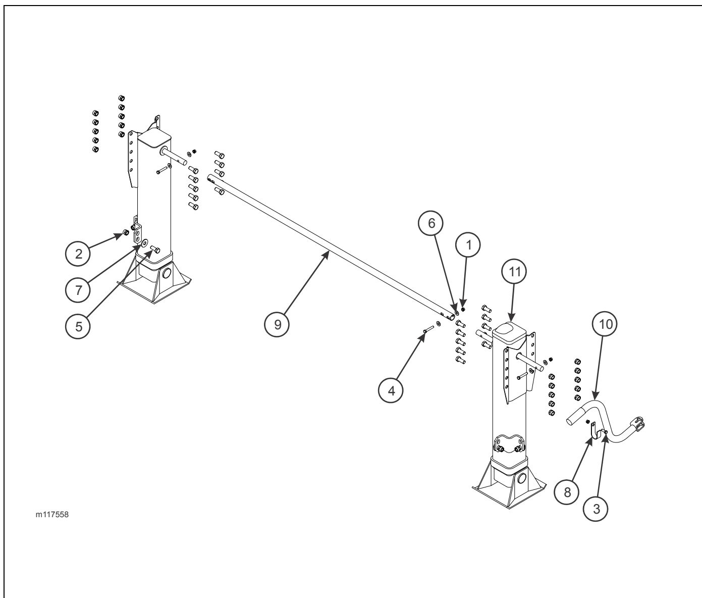
Figure 1-73: Landing Gear Installation - Jost 410
