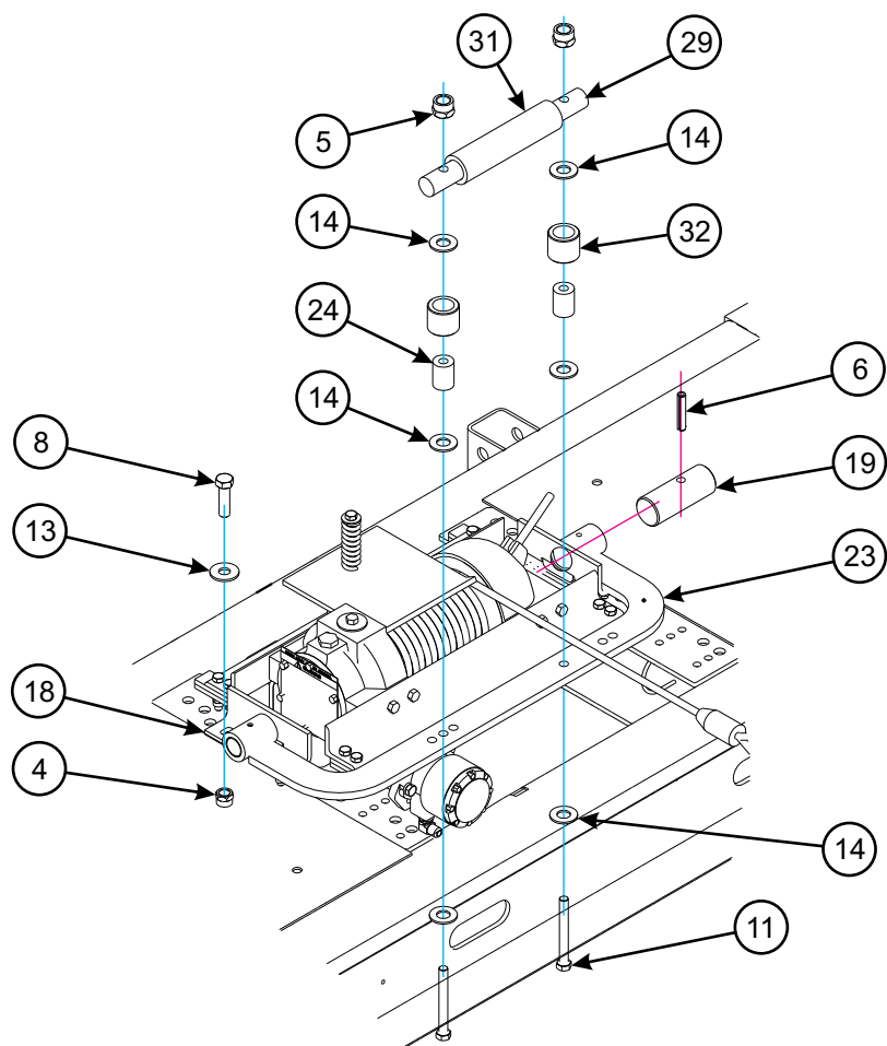
CABLE ROLLER GUIDE ASSEMBLY
