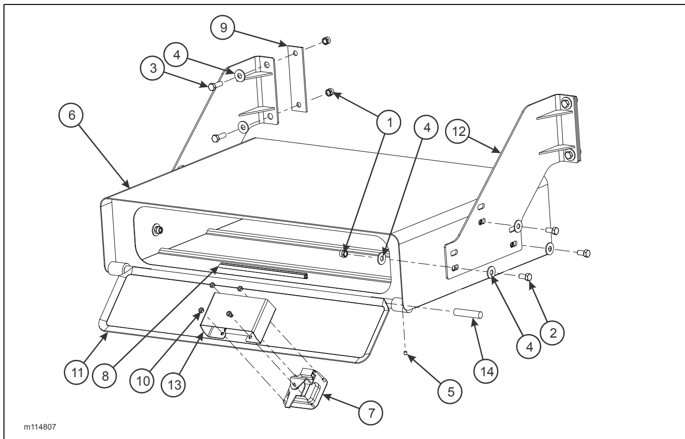
Figure 1-124: Toolbox Installation - Steel/Aluminum Door
