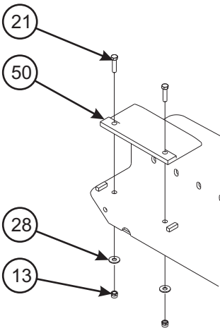
GLIDE ASSEMBLY
