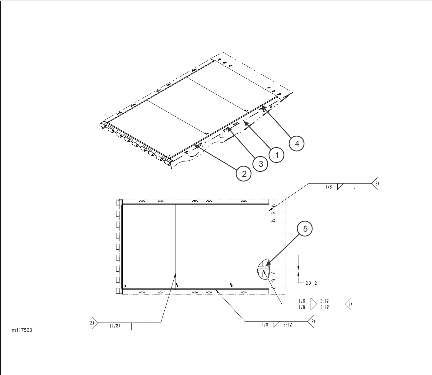
Figure 1-93: Deck Tread Grip/ Over Wood - 15' Tail
