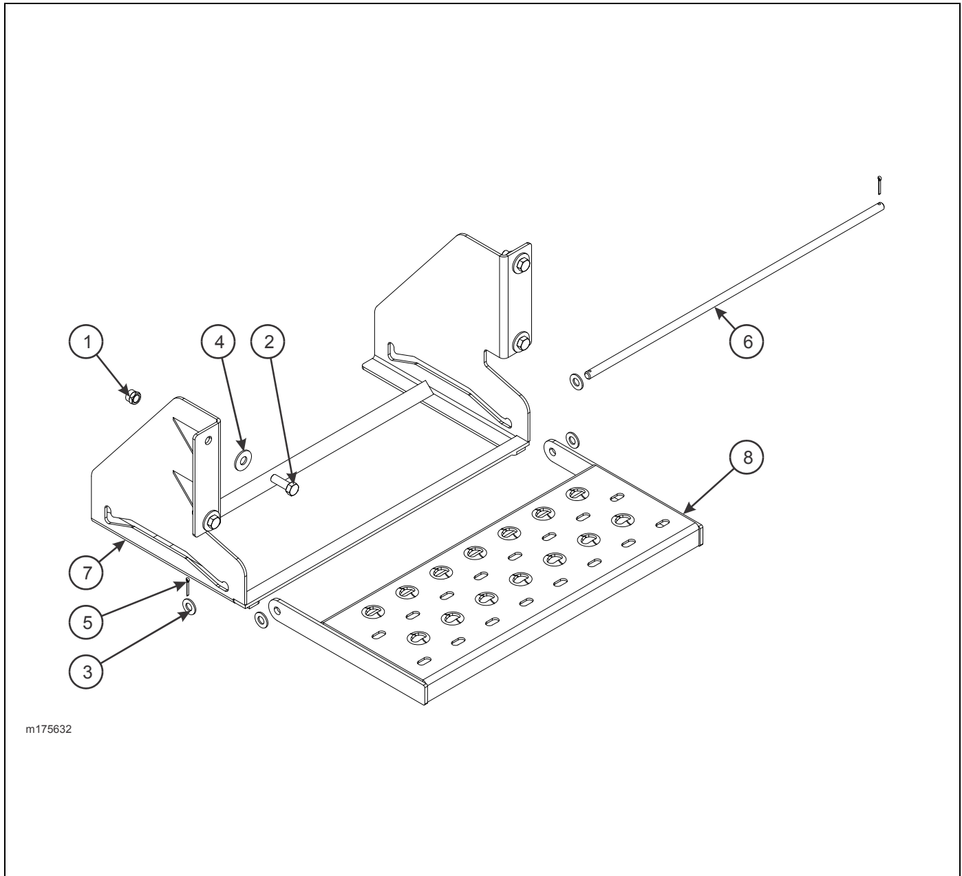
Figure 1-122: Step Assembly - Retractable
