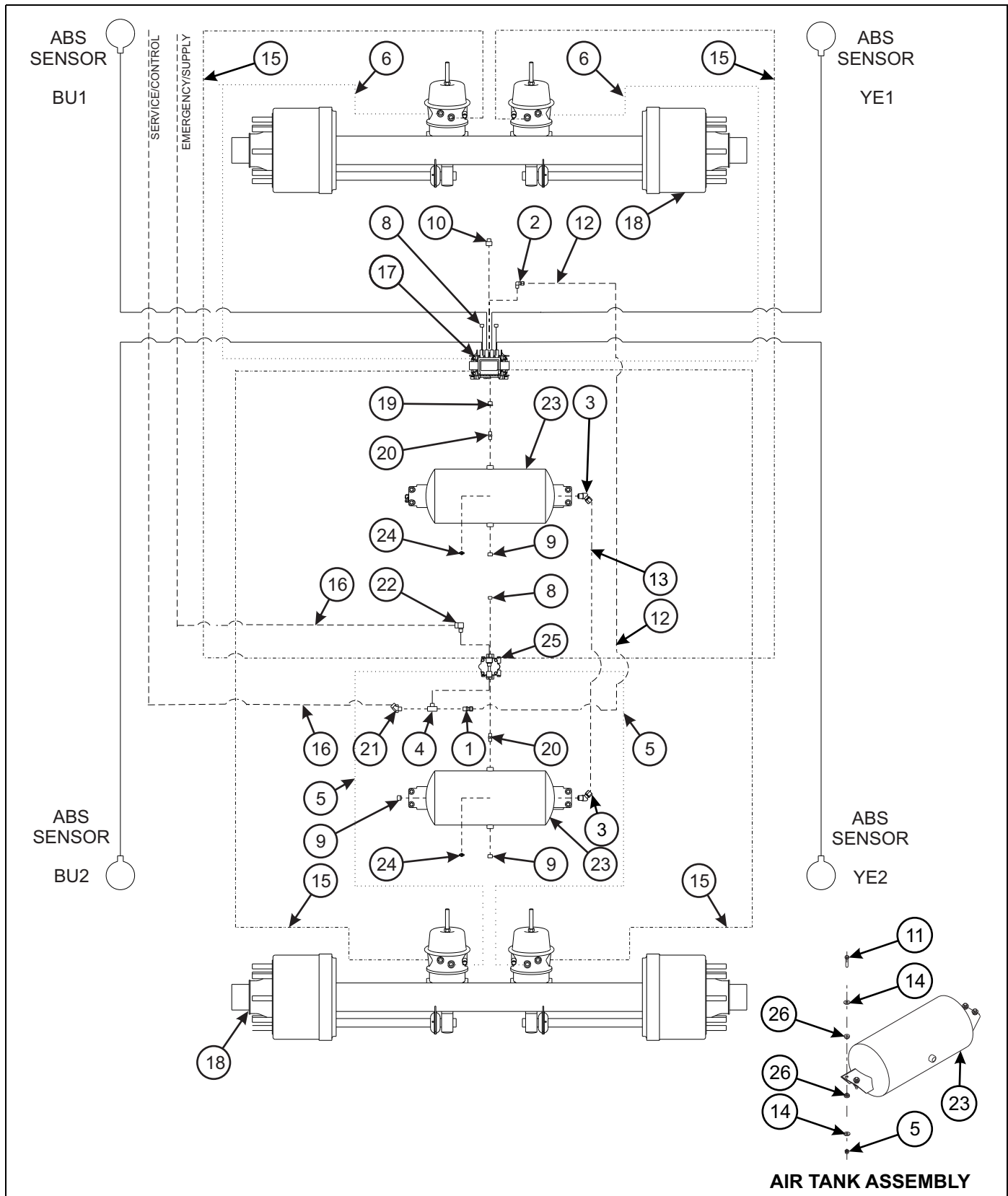
Figure 1-32: Air Brake System - 930C
