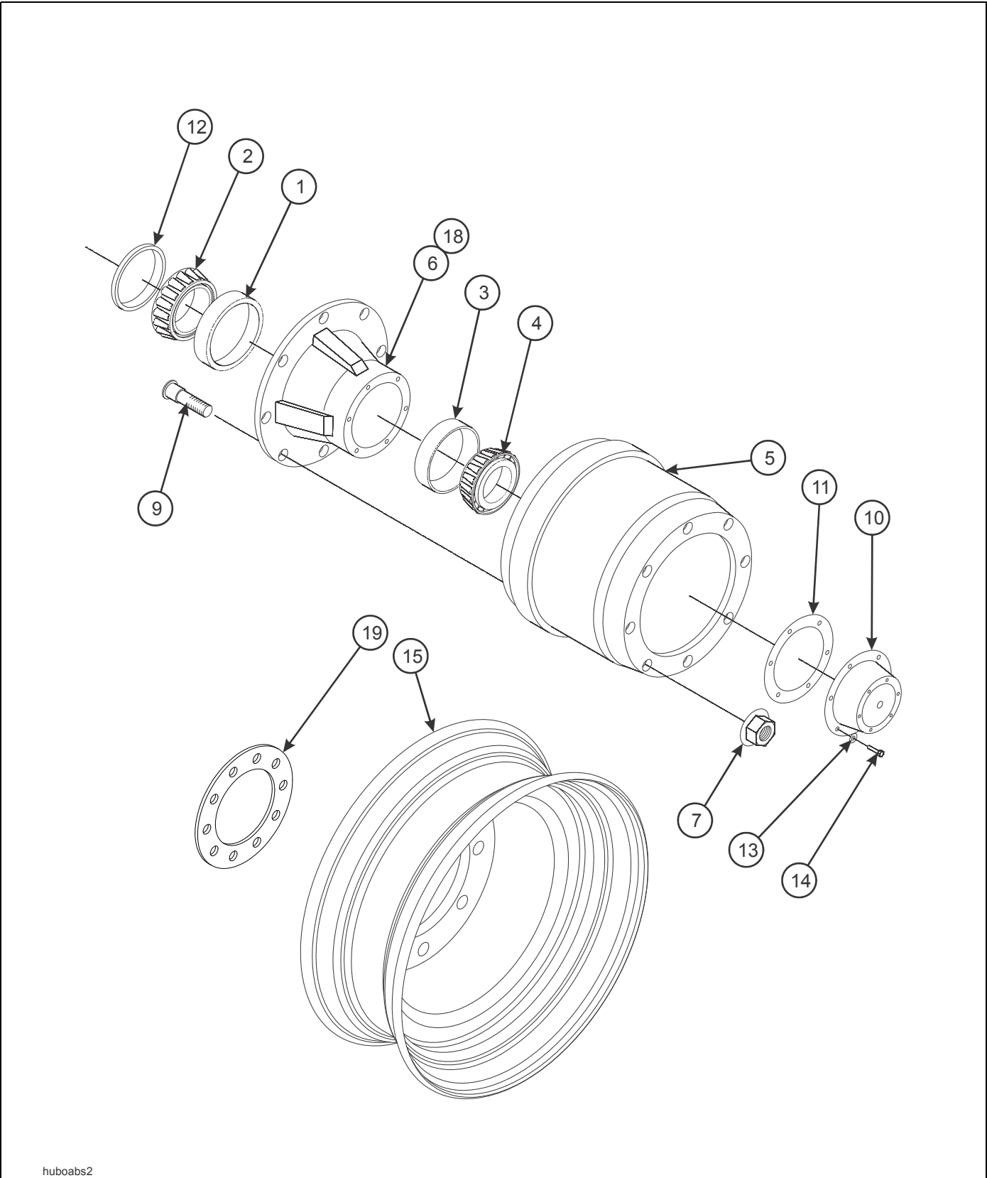
Figure 1-39: Outboard Pilot Mount Hub and Drum Assembly
