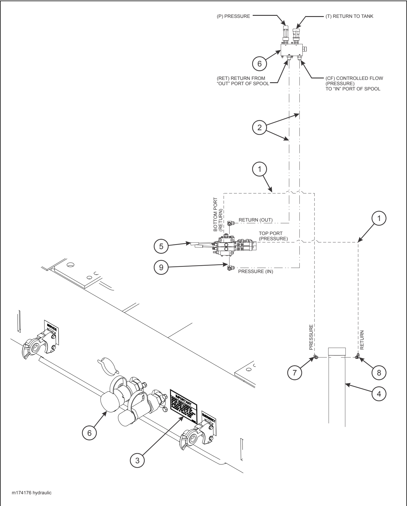
Figure 1-8: Hydraulic System
