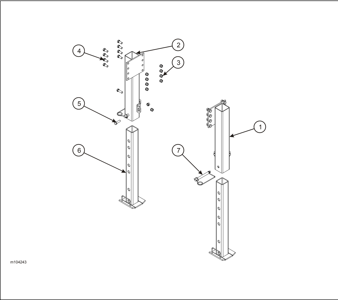
Figure 1-72: Landing Gear Installation - “Bolt On” Park Stand
