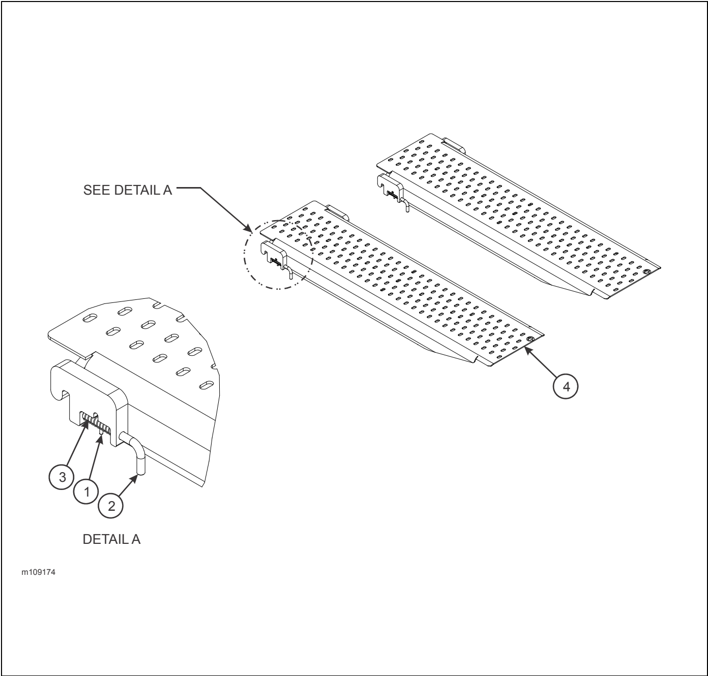
Figure 1-111: Ramp Assembly - Aluminum
