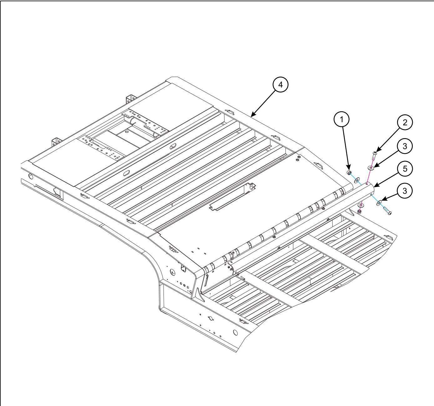
Figure 1-91: Bumper - Fork Lift Plate Installation
