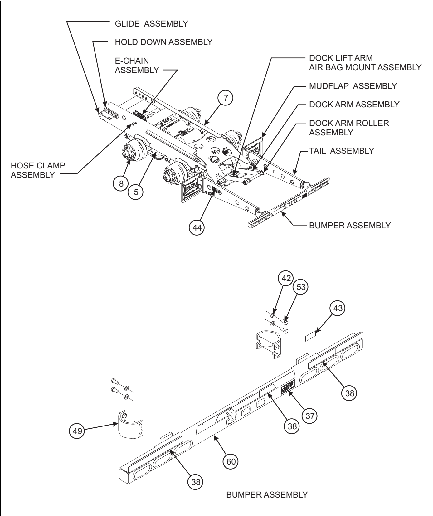
Figure 1-20: General Items - 930C (1 of 3)
