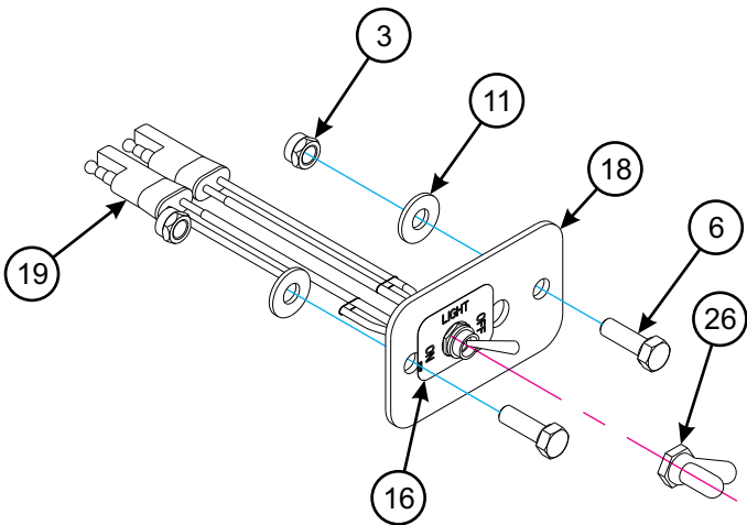
SWITCH ASSEMBLY
