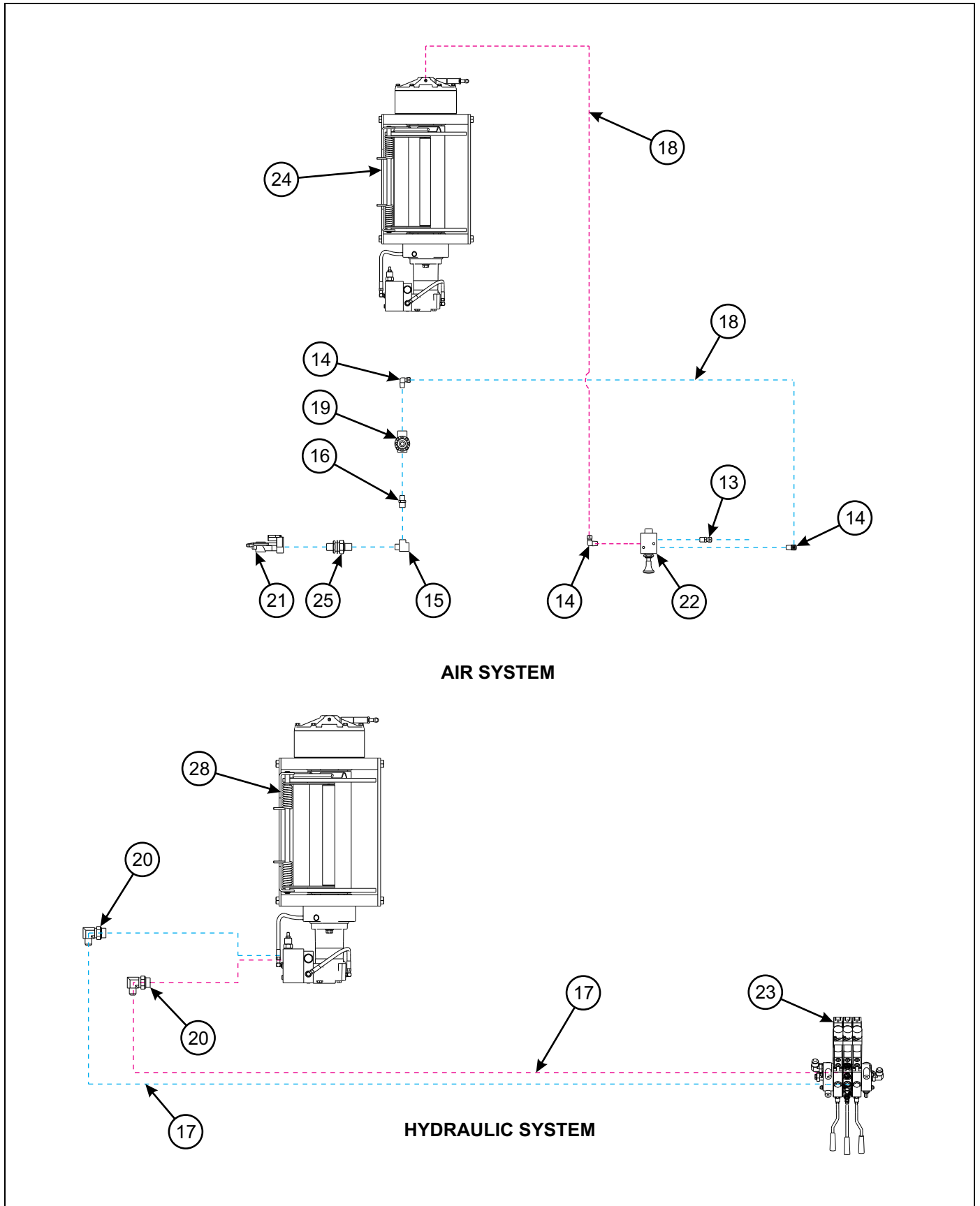
Figure 1-58: Winch Installation - 20K (WARN) (2 of 2)
