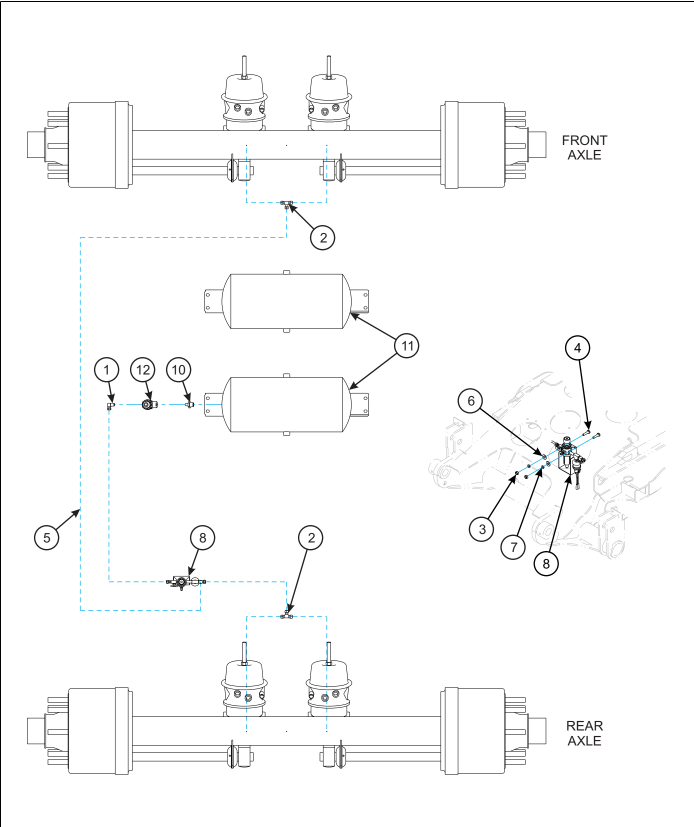
Figure 1-40: Tire Inflation System - 930C
