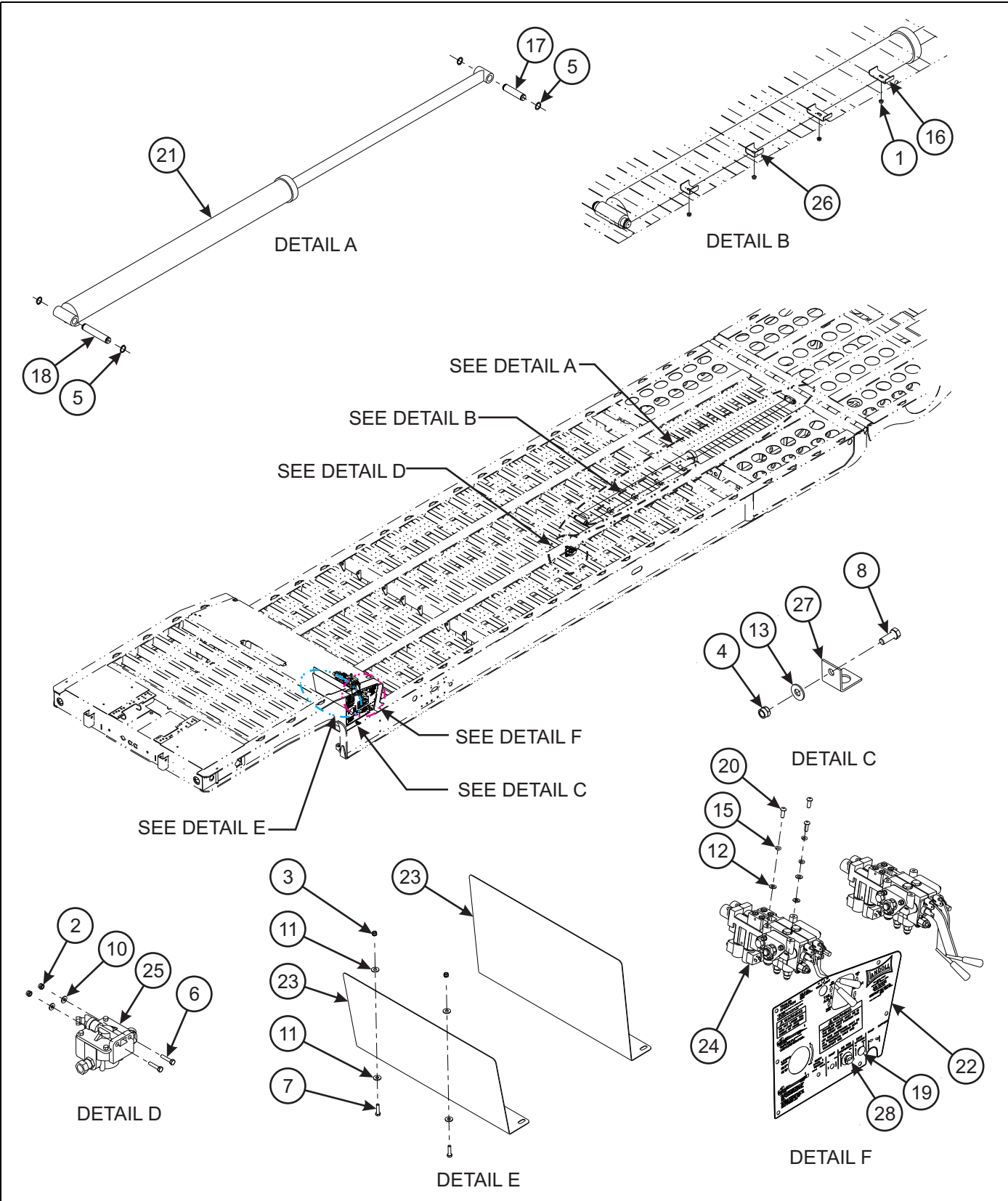
Figure 1-7: General Assembly
