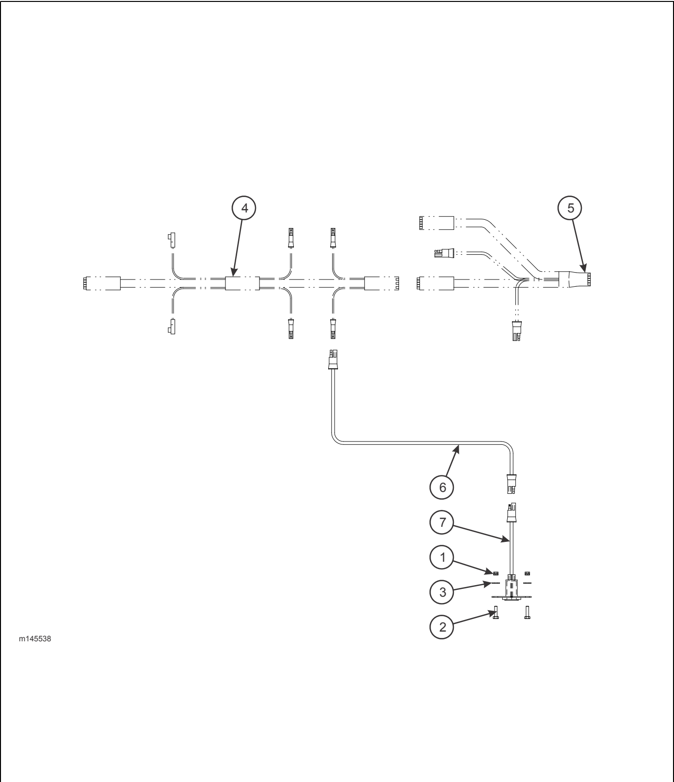
Figure 1-113: Rear Side Electrical Outlet Installation
