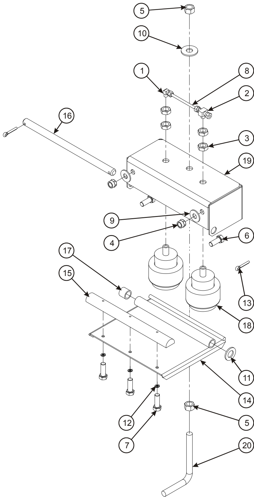
Figure 1-71: Winch - 30K Cable Air Tension (DP)
