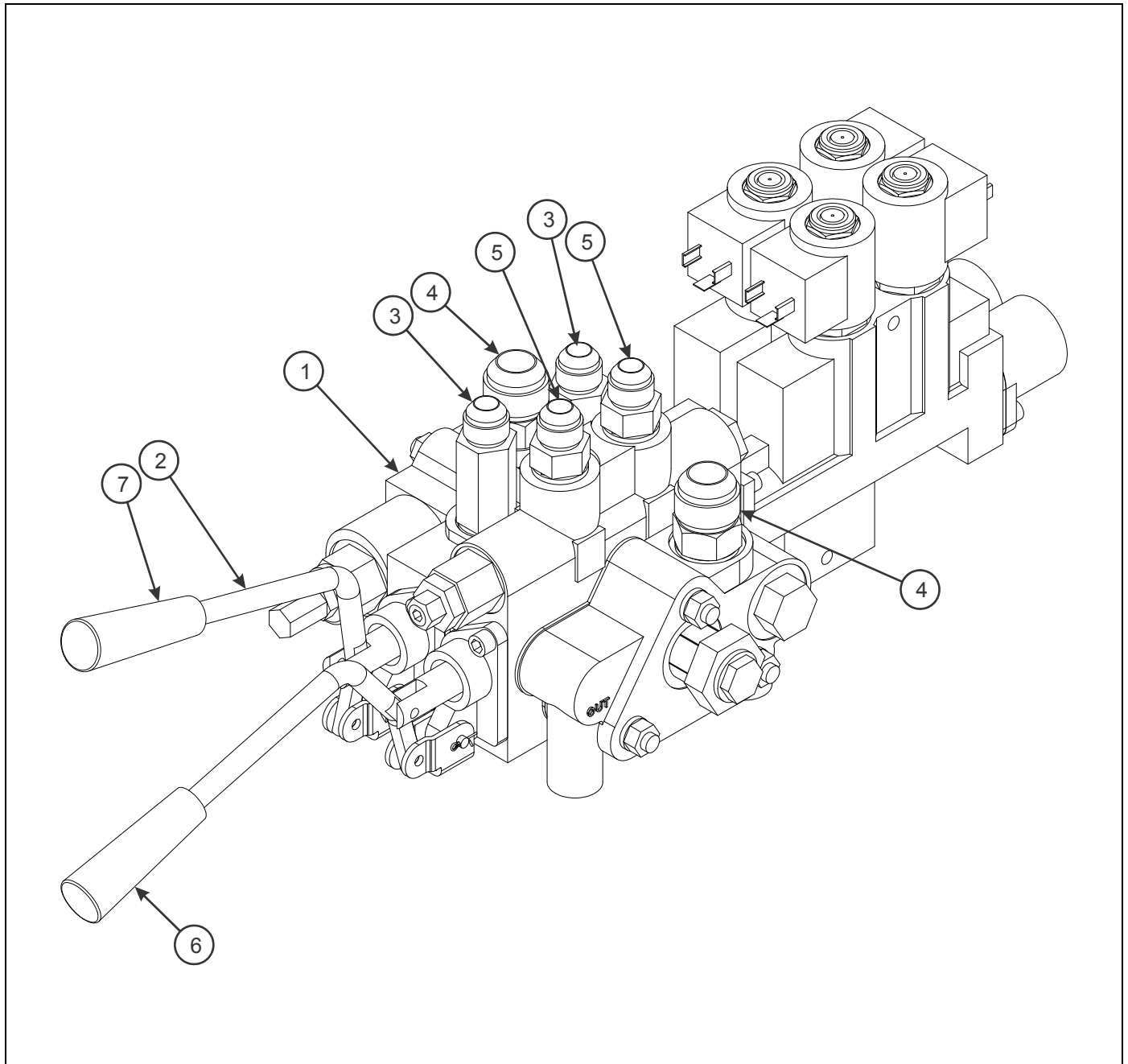
Figure 1-13: Valve Assembly - Two Spool
