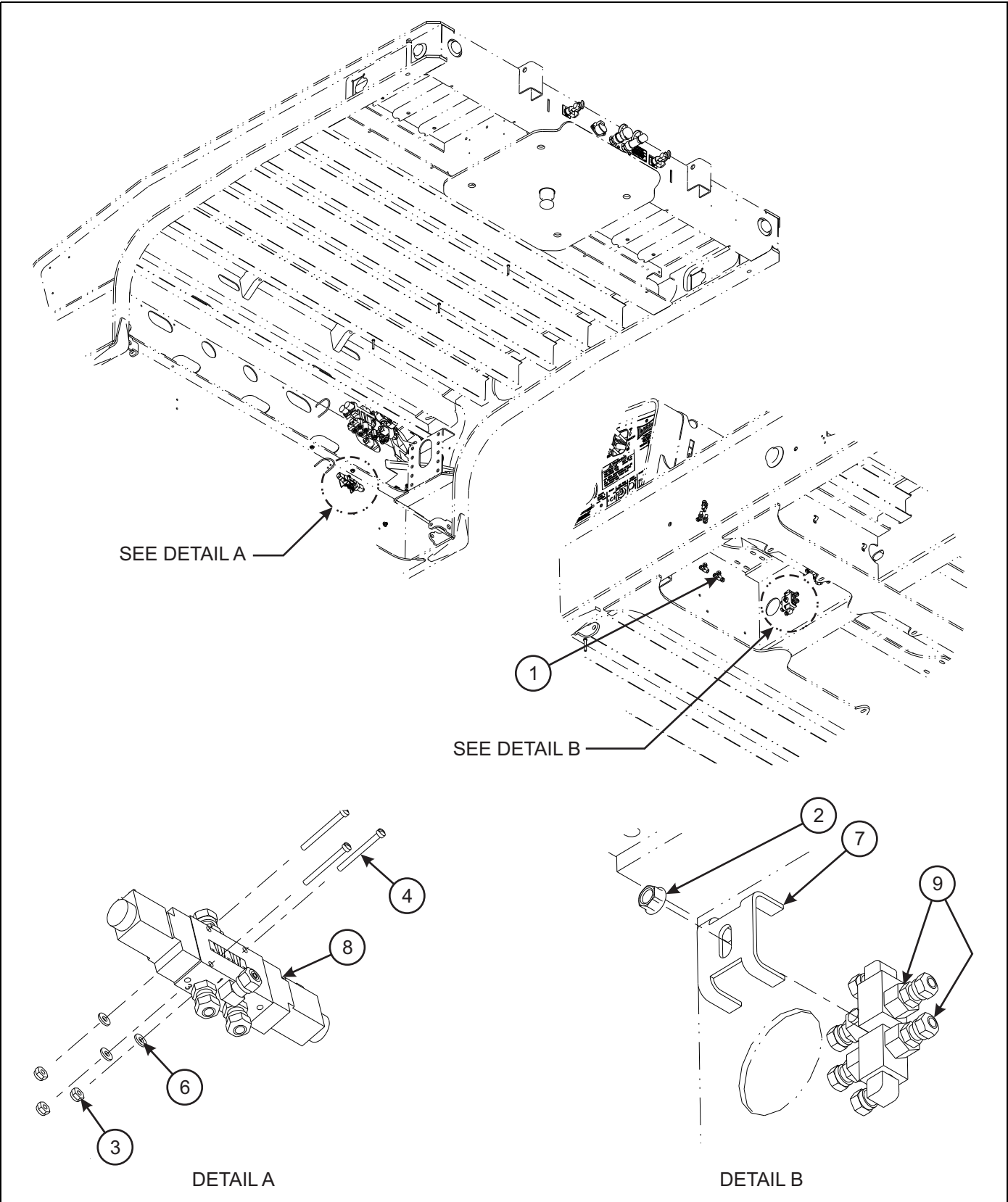
Figure 1-18: Remote Control - General Items
