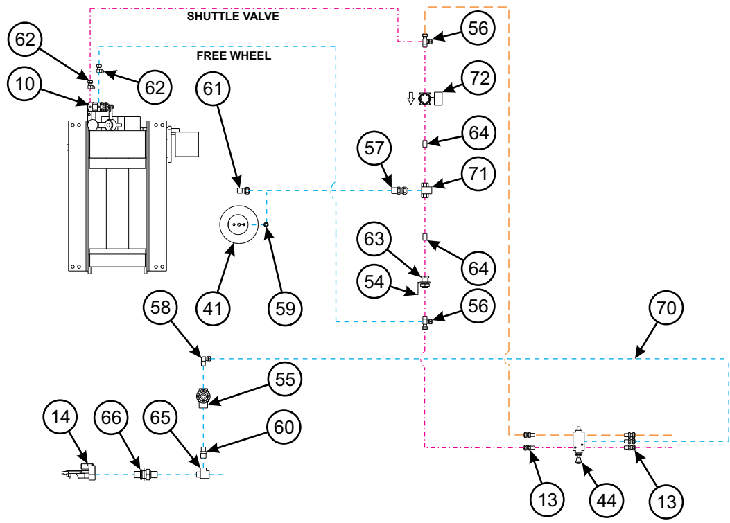
AIR SYSTEM
