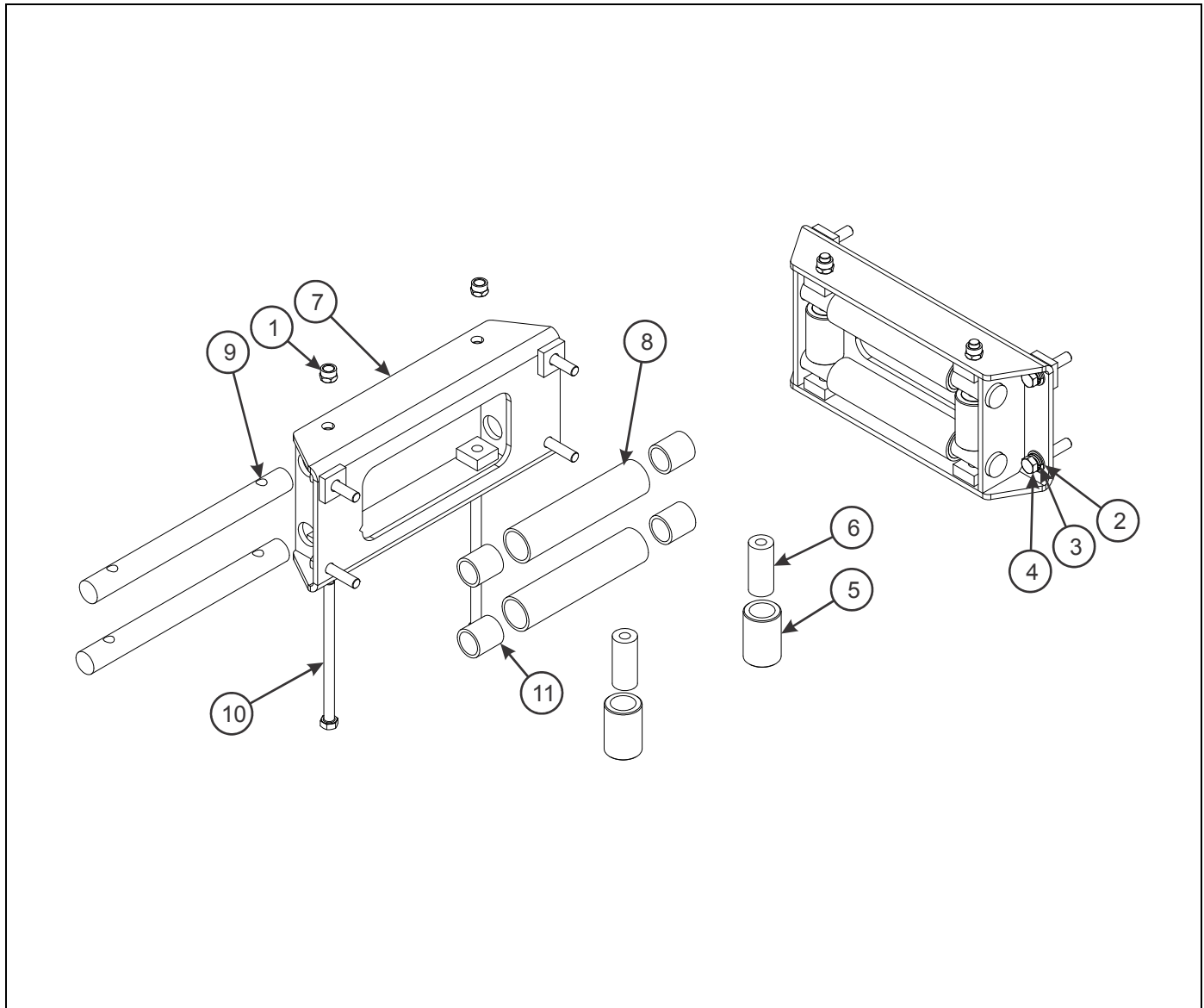
Figure 1-70: Winch - 30K Roller Guide (DP)
