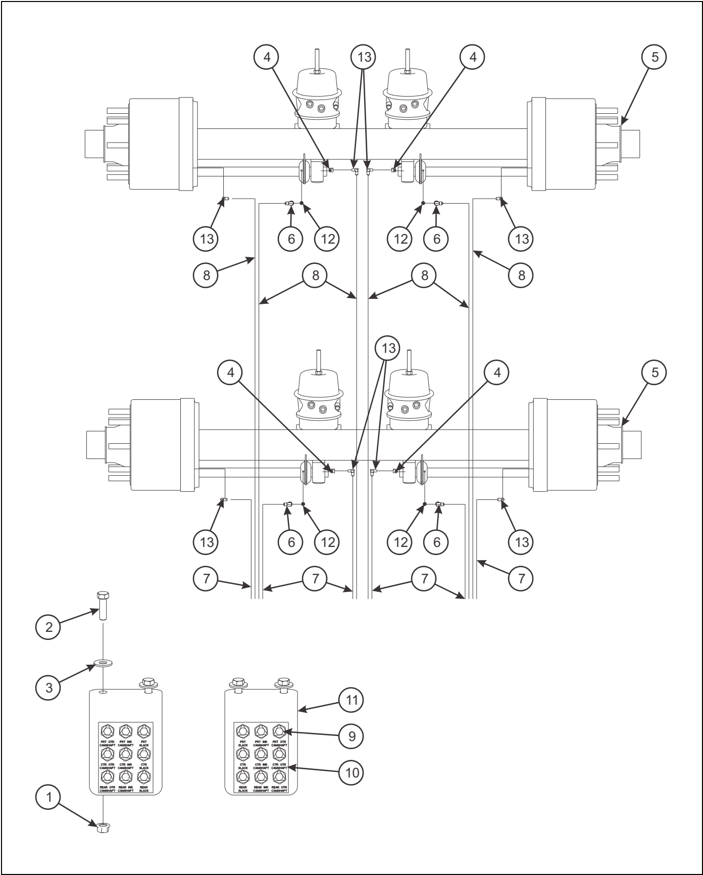
Figure 1-26: Grease System - 930C
