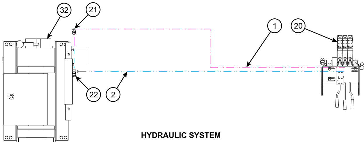
Figure 1-50: Winch Installation - 20K Upper Deck (BRADEN) (2 of 2)
