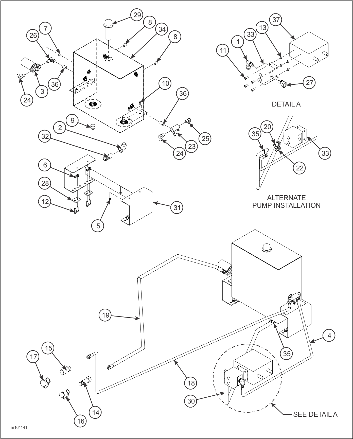
Figure 1-109: Hydraulic Wet Kit Items - 30 Gallon
