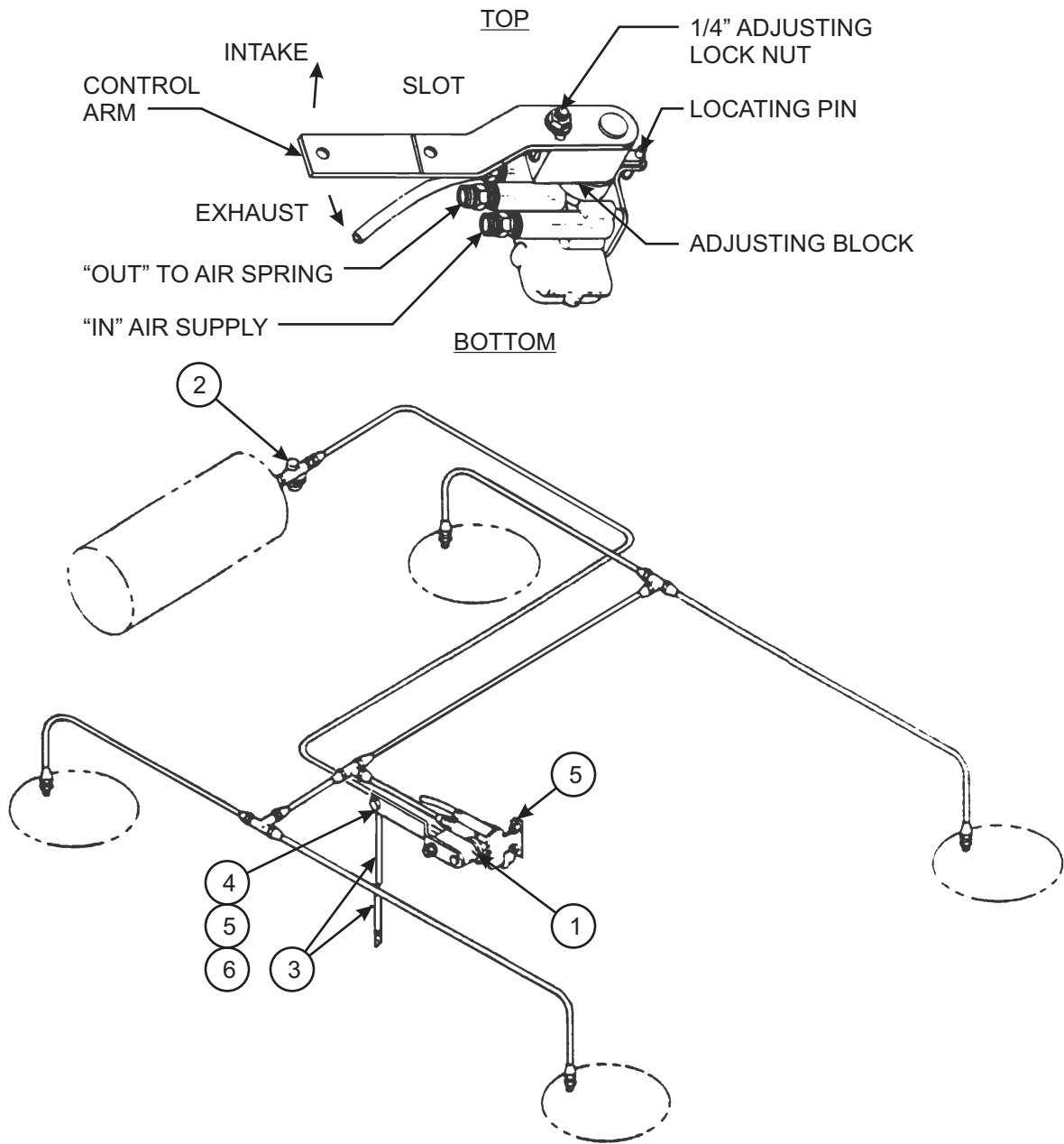
Figure 1-29: Air Control Kit - Neway
