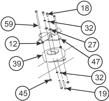
DOCK ARM ASSEMBLY
