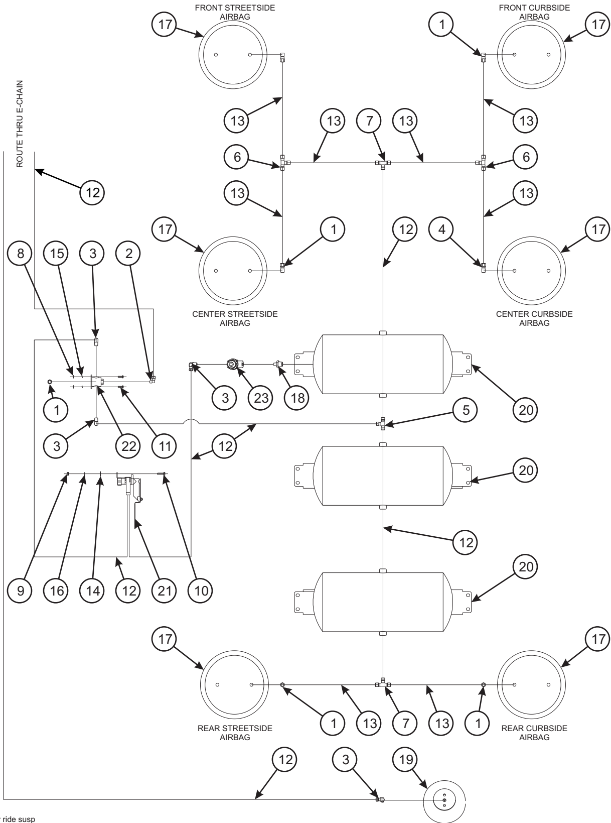
Figure 1-28: Air Ride Suspension - 950C
