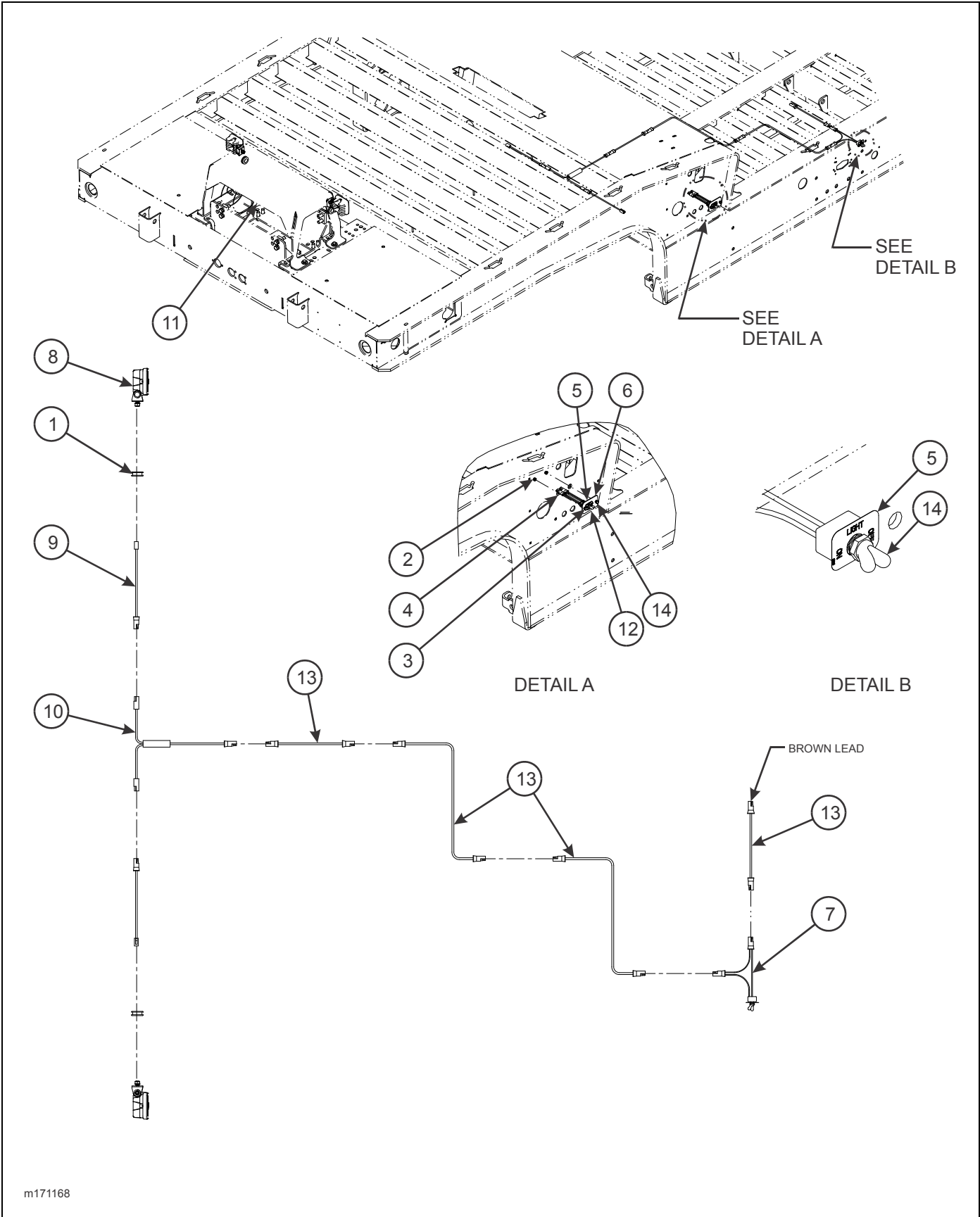
Figure 1-135: Winch - Work Light Installation
