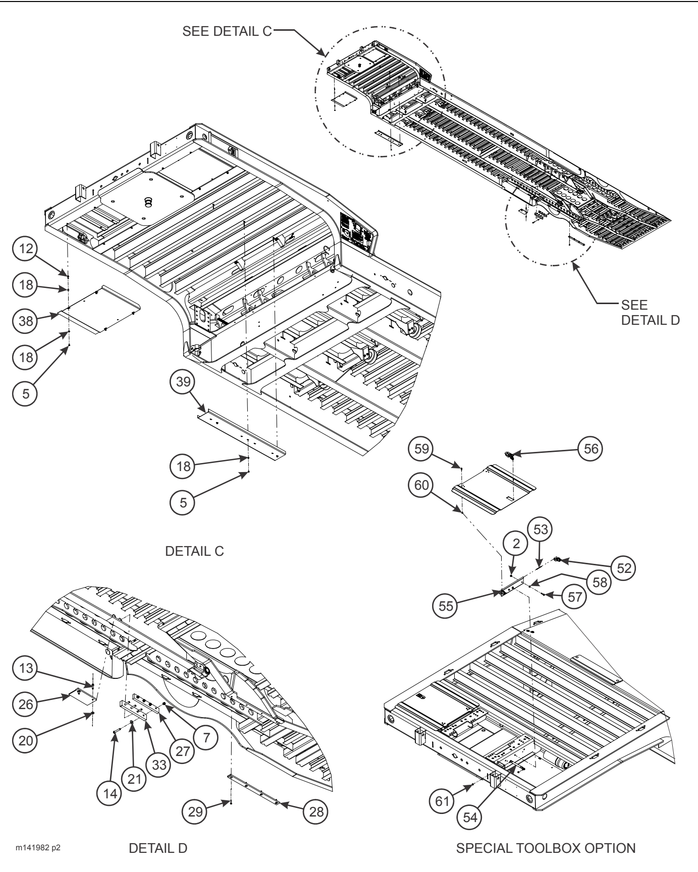
Figure 1-4: Frame Assembly (2 of 2)
