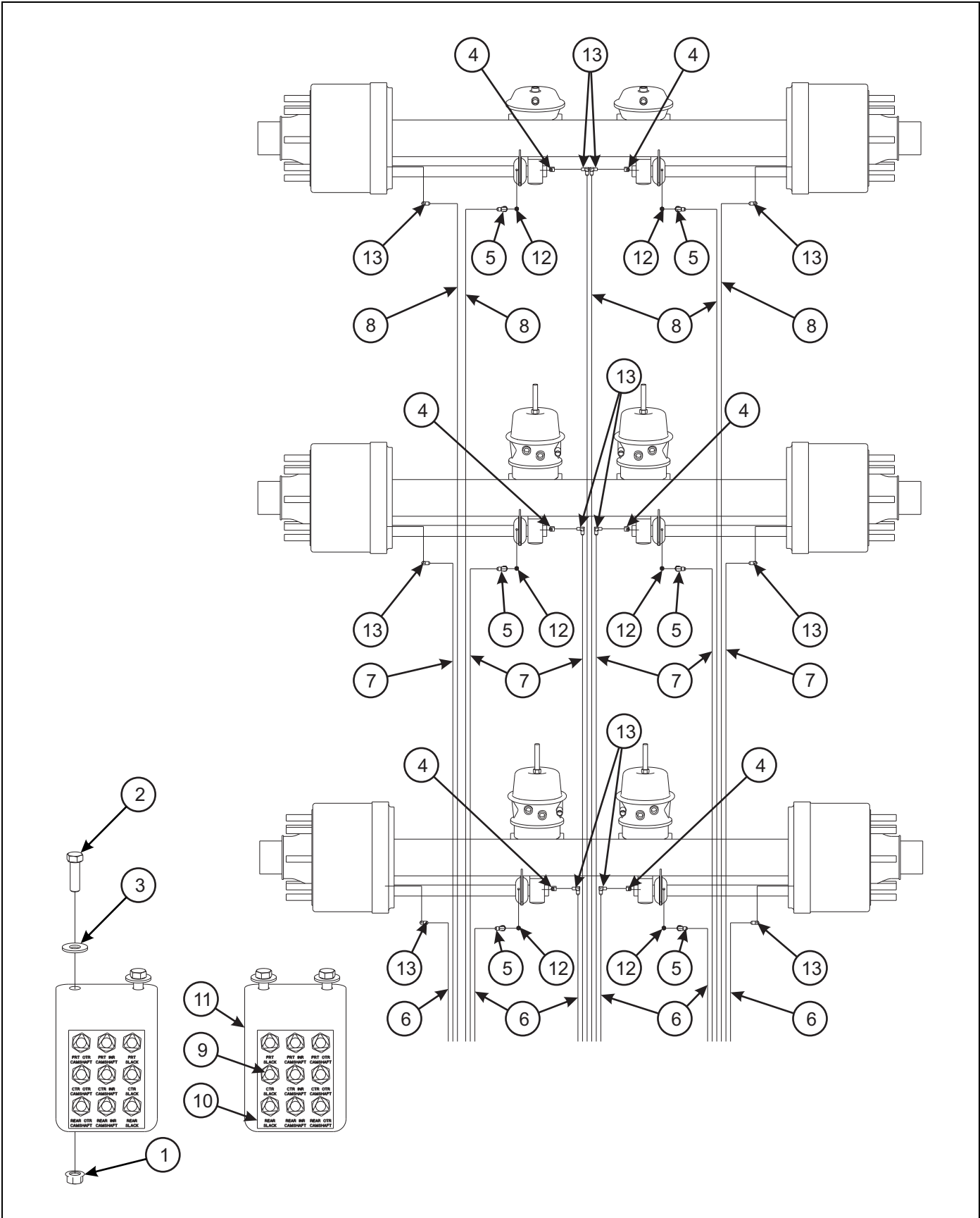
Figure 1-1: Grease System - 950C
