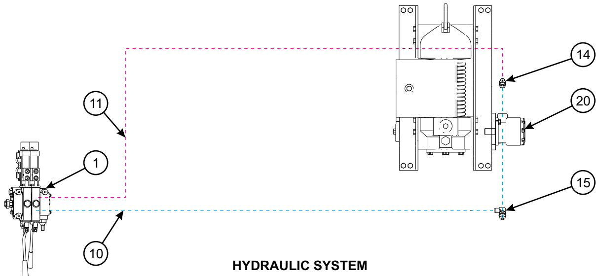
Figure 1-46: Winch Installation - 12K Lower Deck (BRADEN) (1 of 2)
