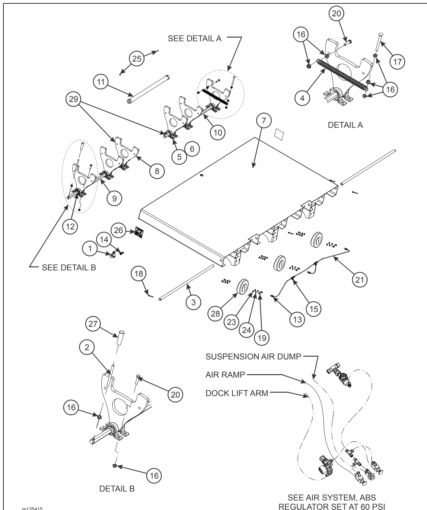
Figure 1-110: Ramp Assembly - 4'
