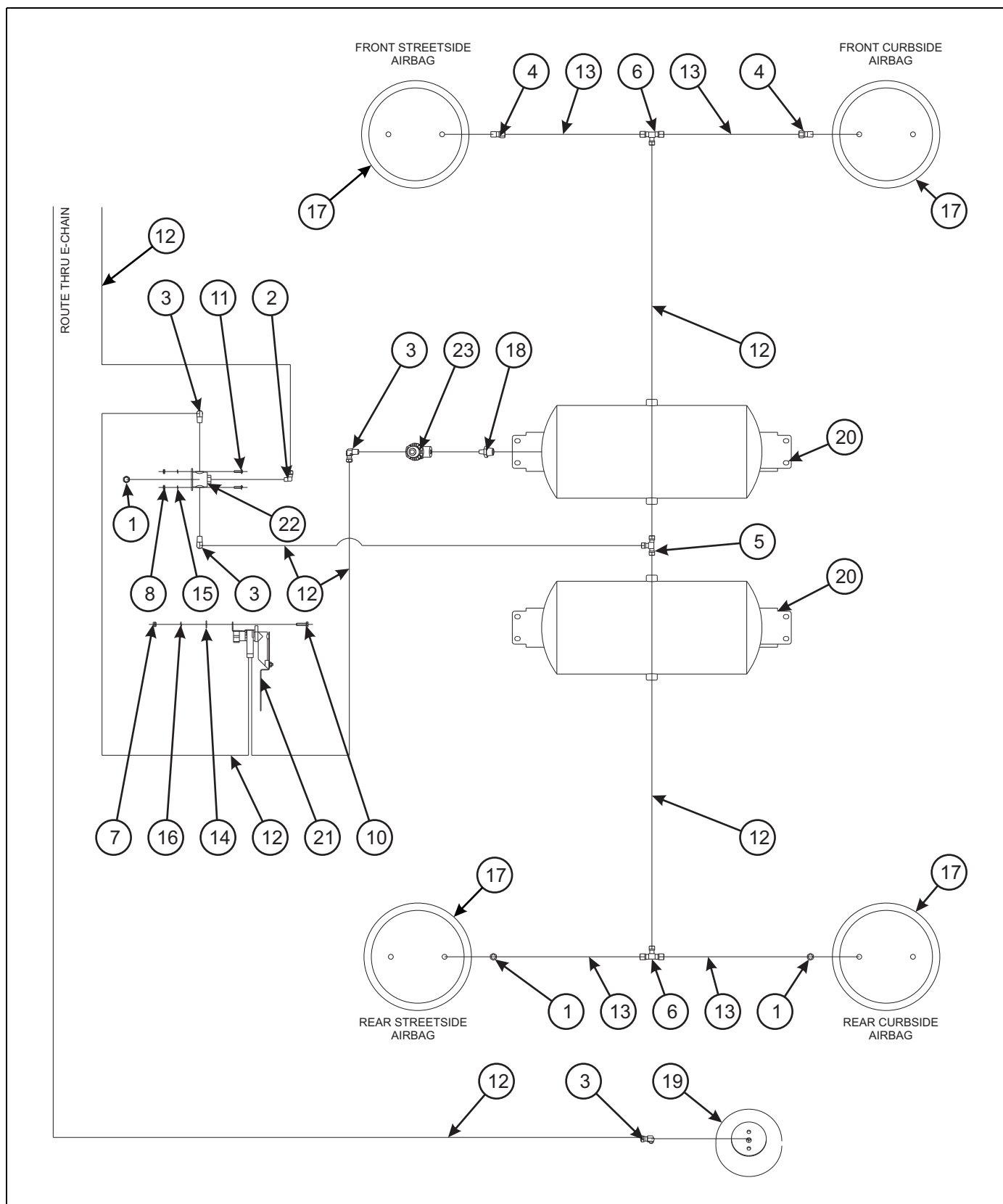
Figure 1-27: Air Ride Suspension - 930C
