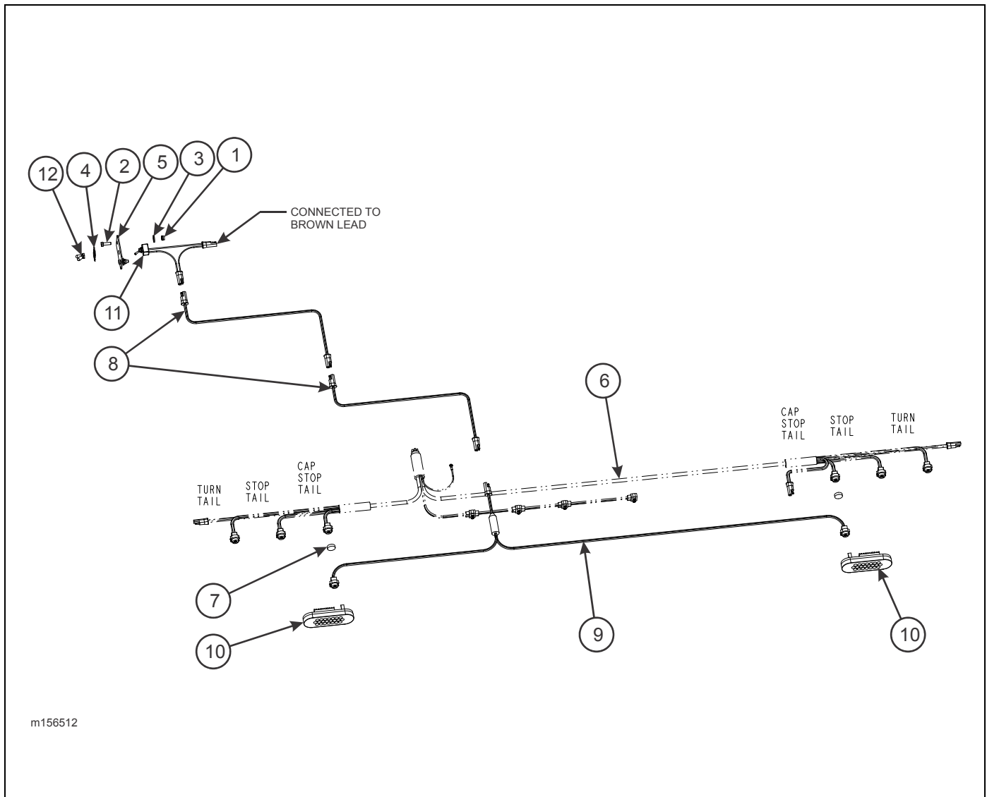
Figure 1-92: Bumper - Strobe Installation
