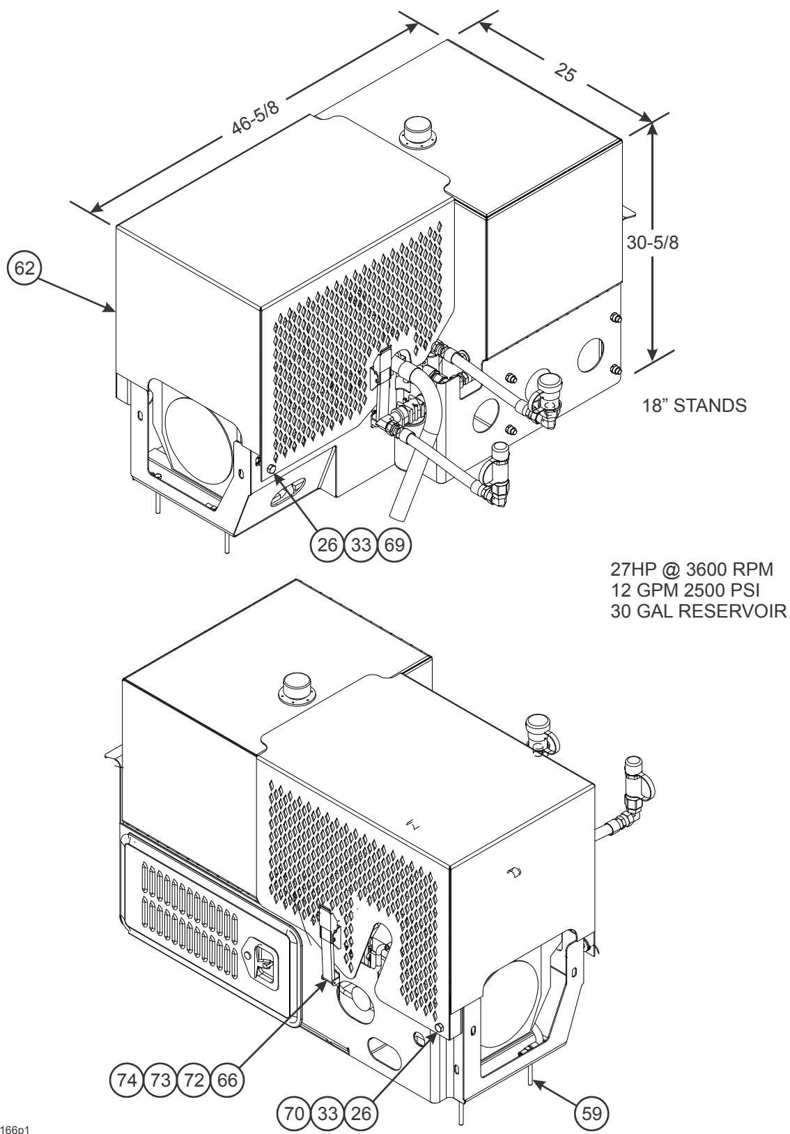
Figure 1-99: Engine - 27 HP Upper Deck Package (1 of 4)
