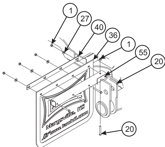
MUD FLAP ASSEMBLY
