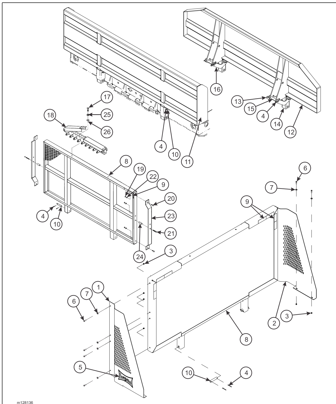
Figure 1-85: Bulkhead Assembly
