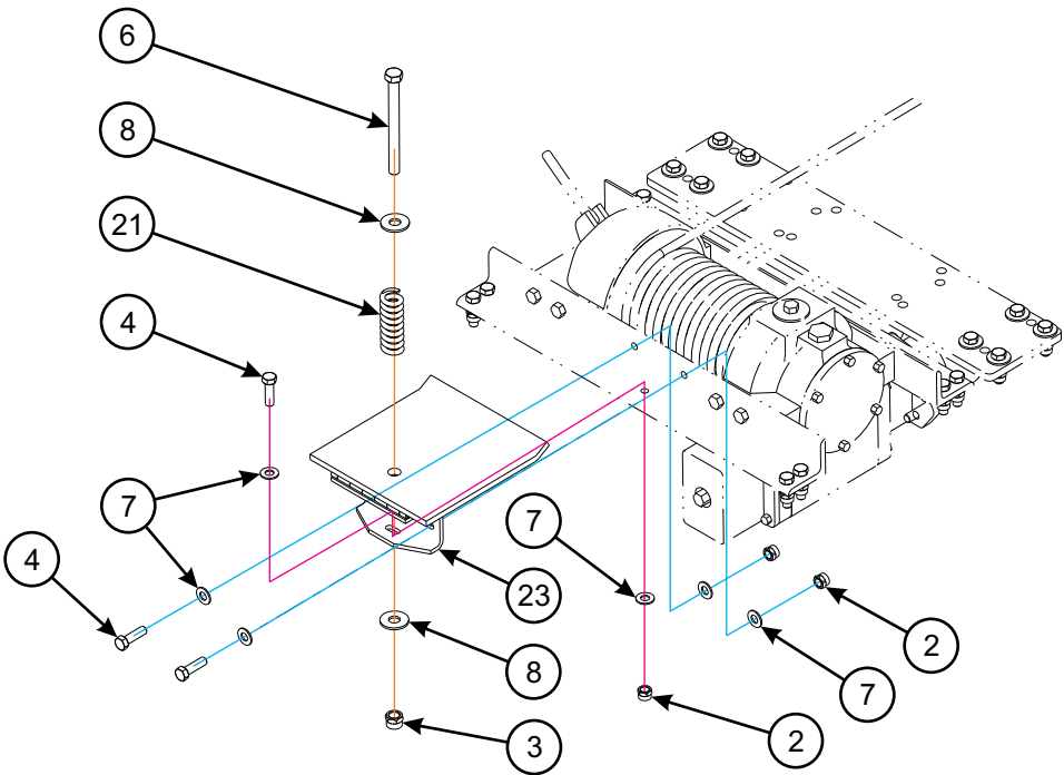
SPRING TENSIONER SYSTEM
