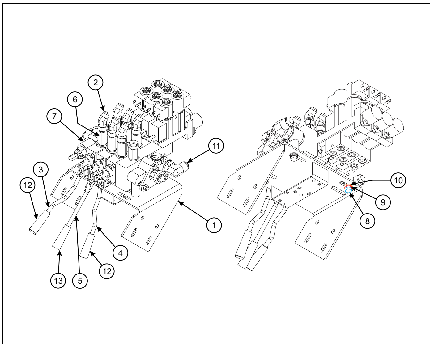
Figure 1-15: Valve Assembly - Three Spool
