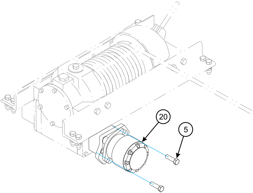
MOTOR ASSEMBLY
