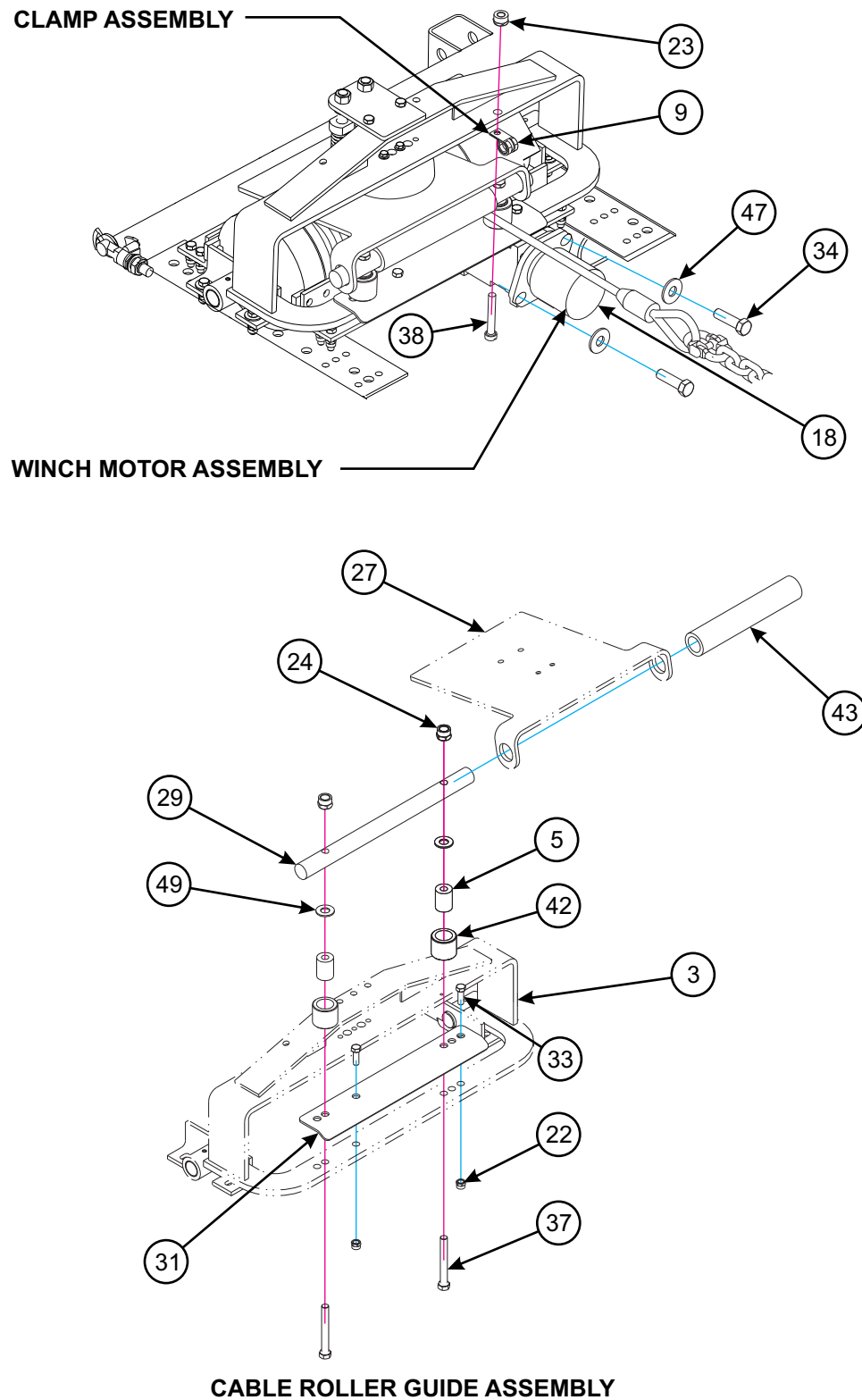
Figure 1-52: Winch Installation - 20K Air Tension/Release (BRADEN) (2 of 3)
