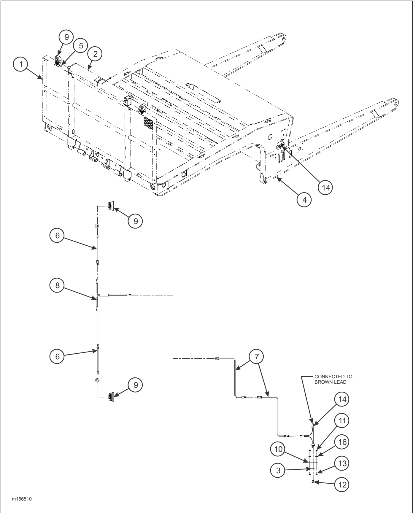
Figure 1-90: Bulkhead - Work Light Assembly
