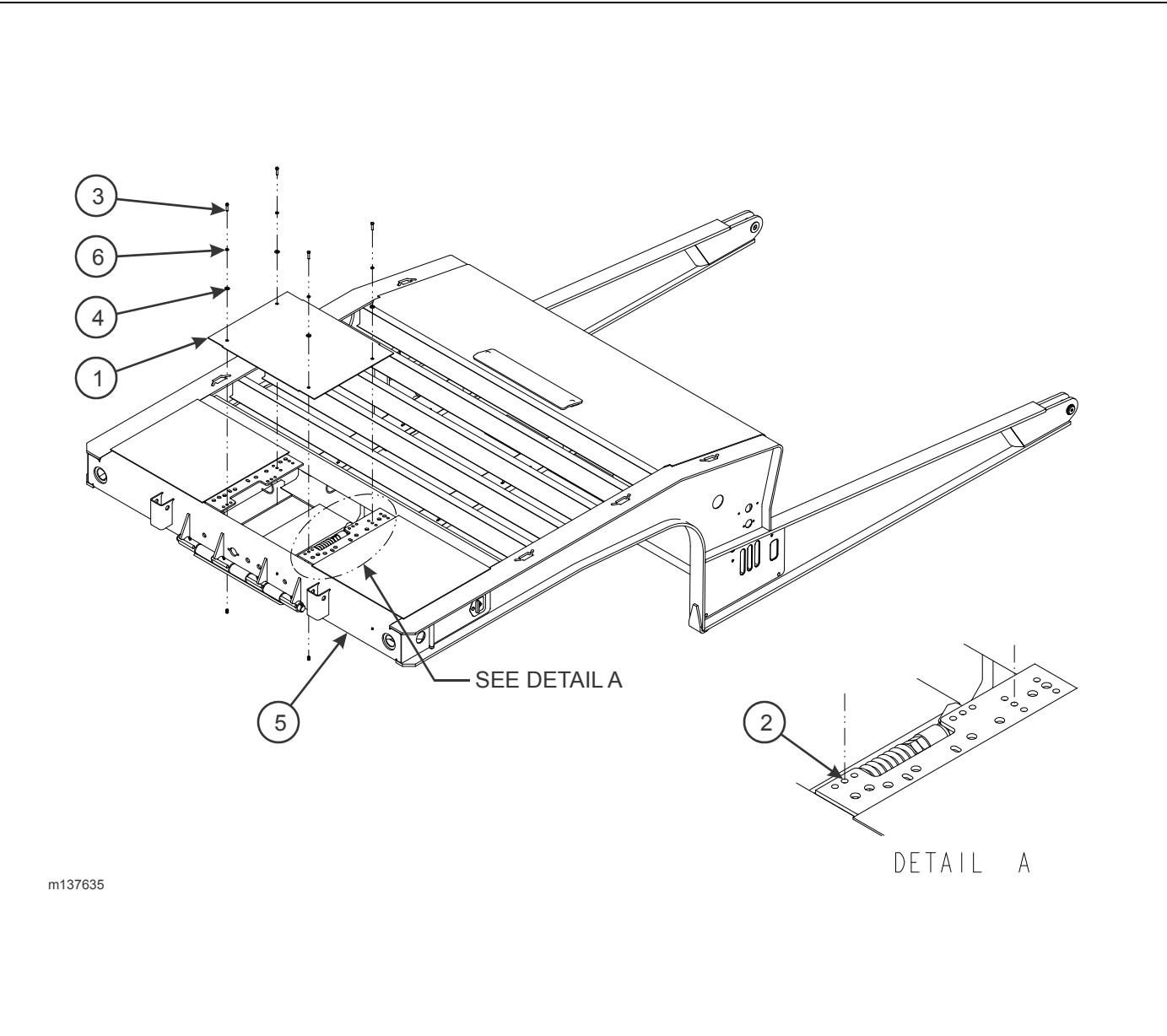
Figure 1-127: Upper Deck Cover Assembly
