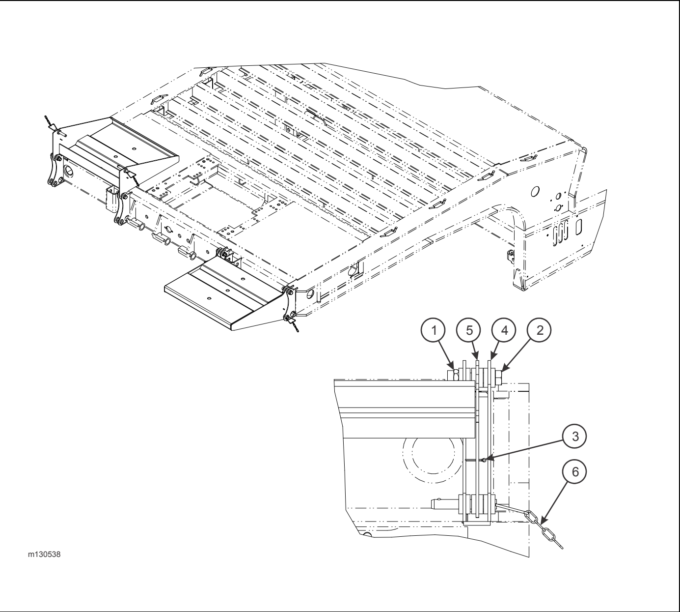
Figure 1-107: Front Flip Extension
