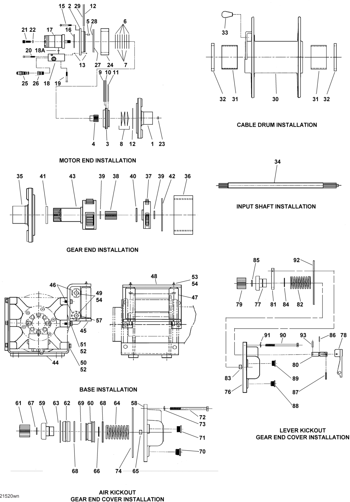
Figure 1-65: Winch Items -12K, 15K, &amp; 20K (DP)
