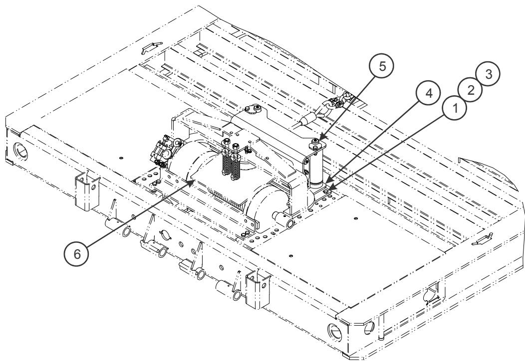
Figure 1-79: 4 Roller Guide Installation - 20K (BRADEN)
