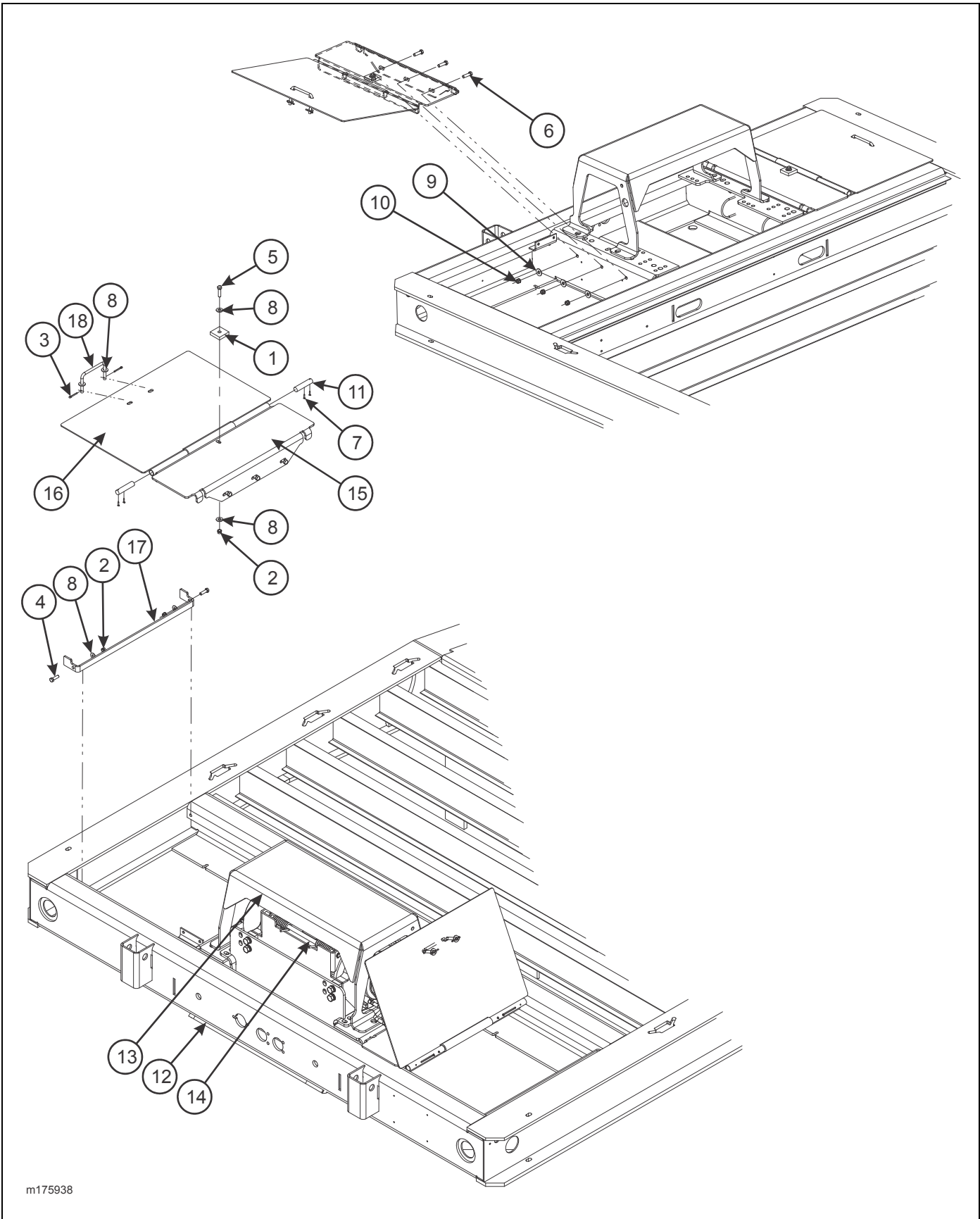
Figure 1-129: Upper Deck - Toolbox Lid Installation “Non-Weight Bearing”
