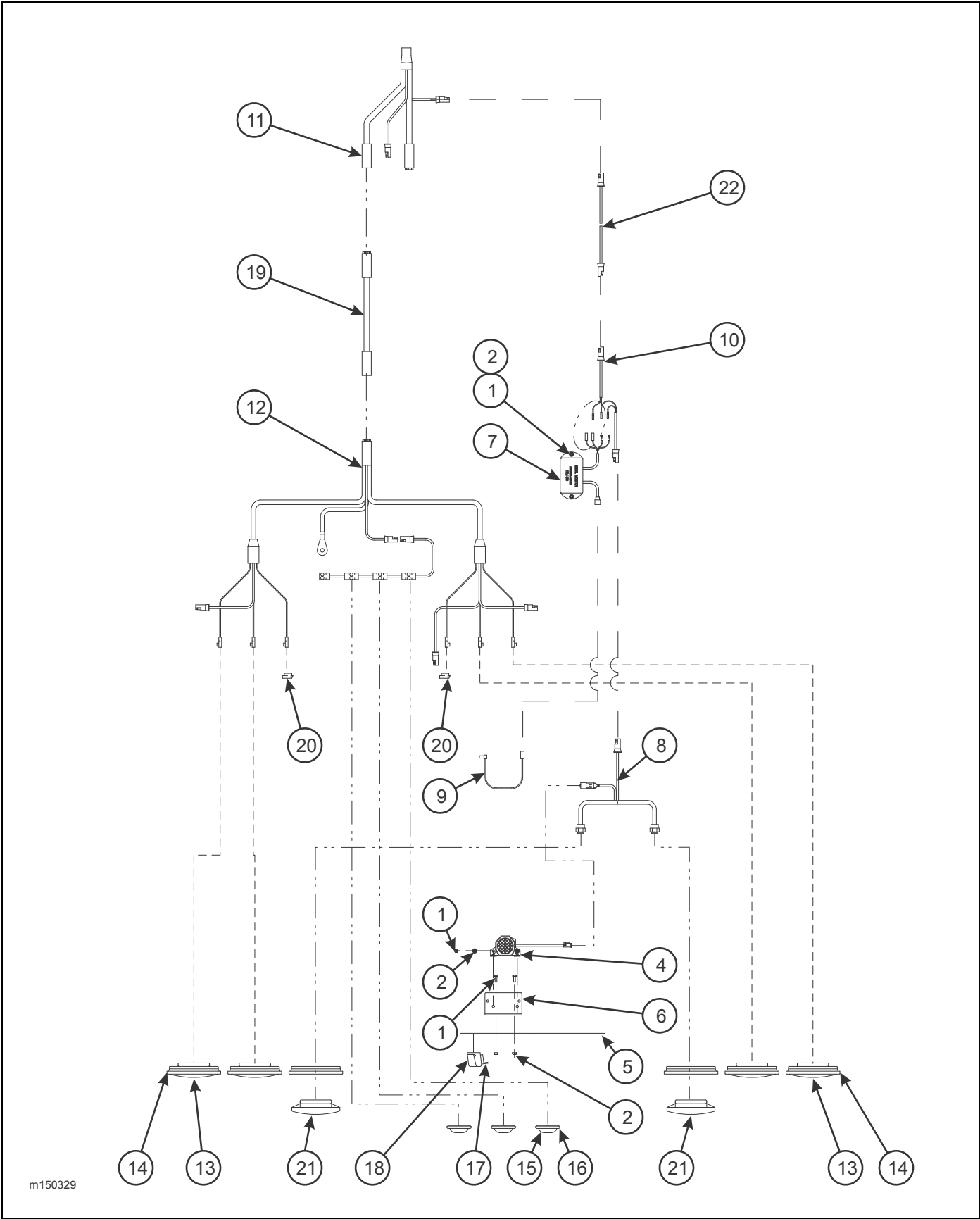
Figure 1-84: Backup Alarm/Light Installation
