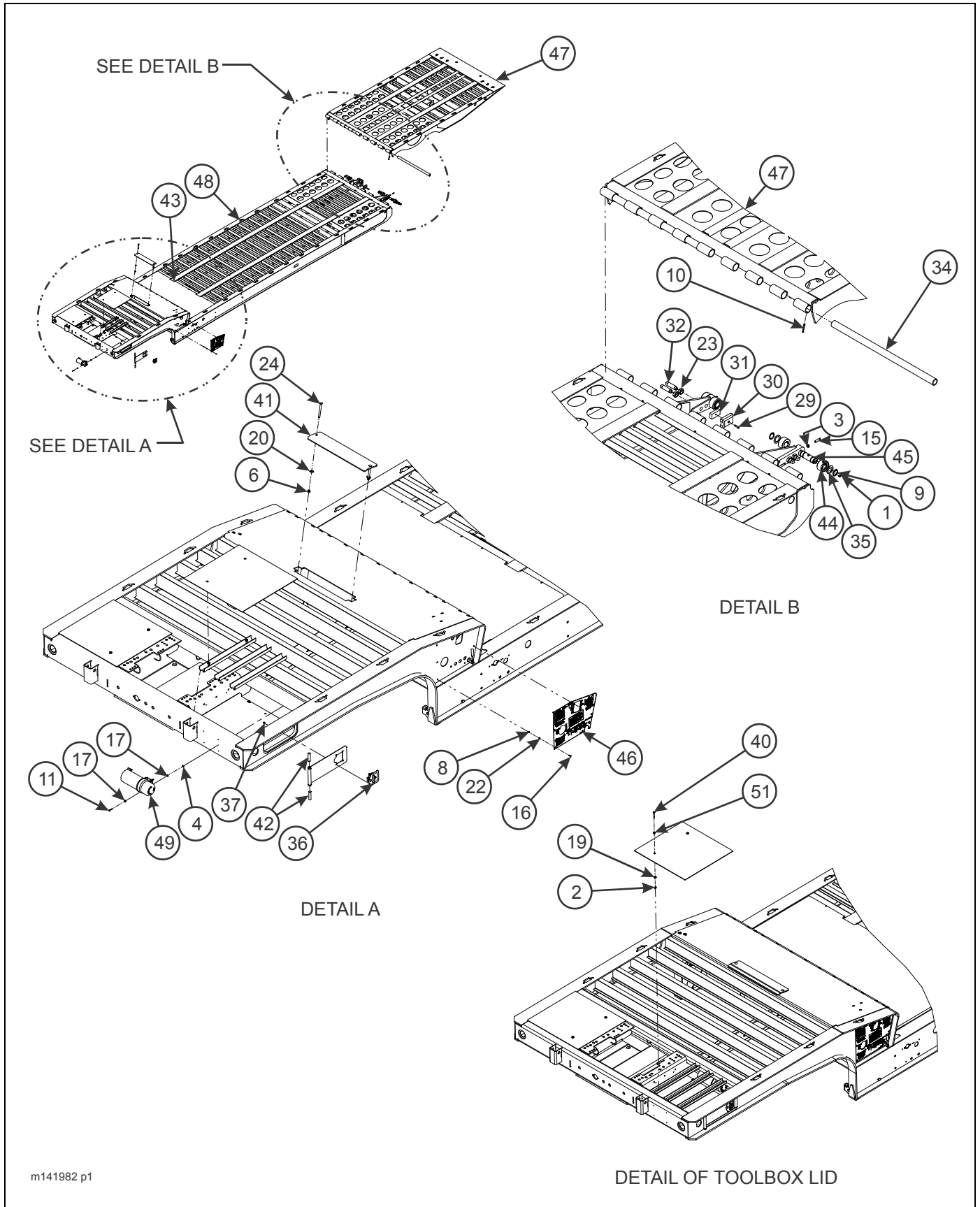
Figure 1-3: Frame Assembly (1 of 2)
