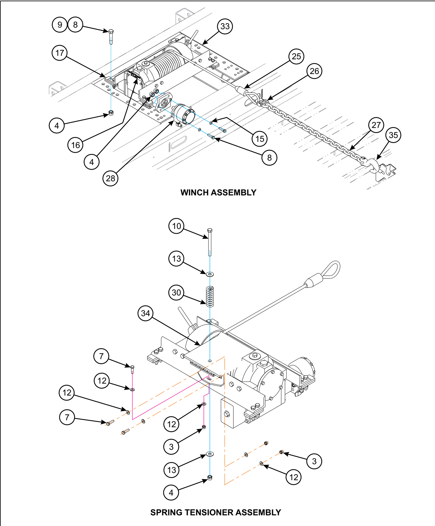
Figure 1-44: Winch Installation - 12K Upper Deck (BRADEN) (1 of 2)
