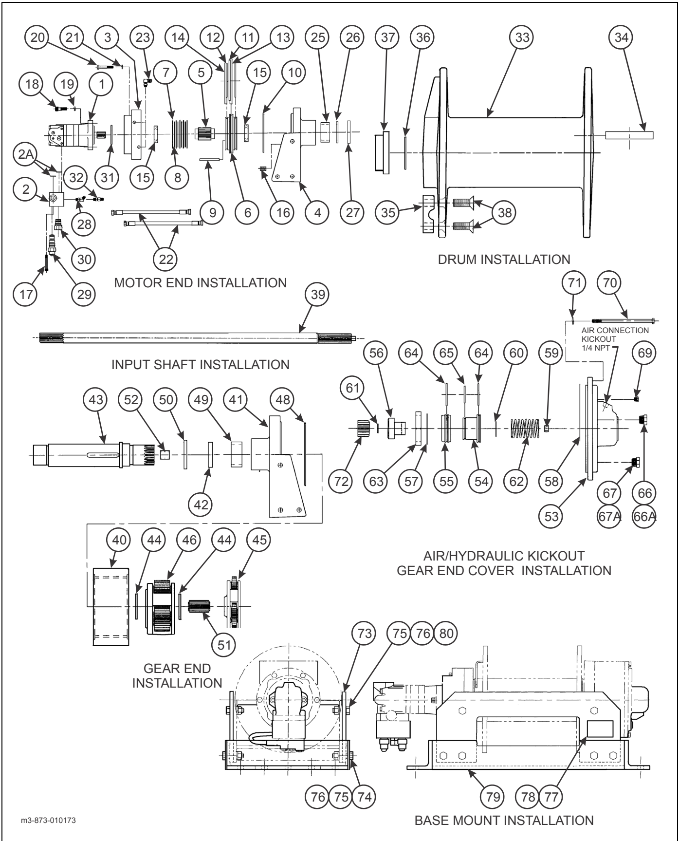
Figure 1-69: 30,000 Lb. Winch Items
