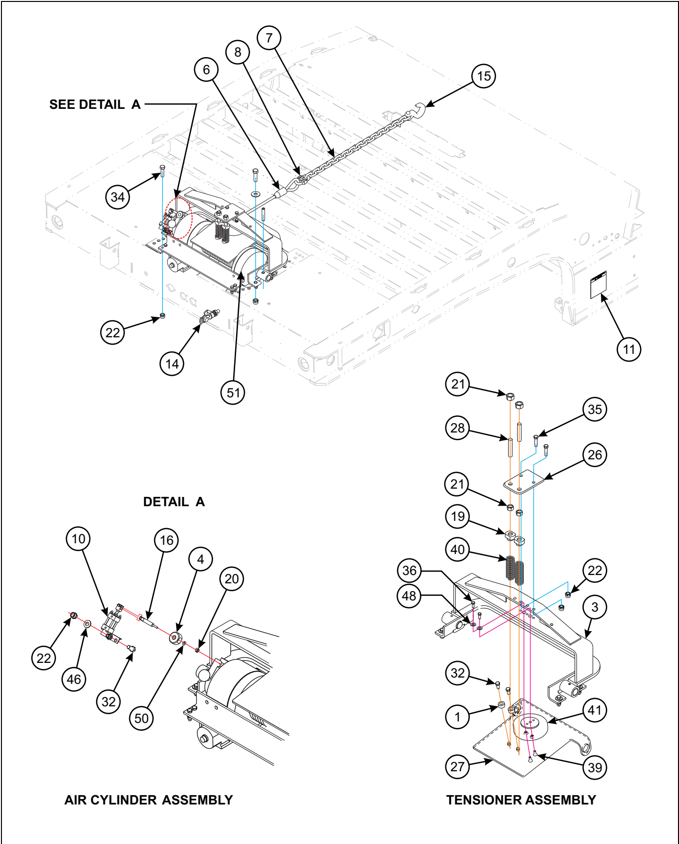
Figure 1-51: Winch Installation - 20K Air Tension/Release (BRADEN) (1 of 3)
