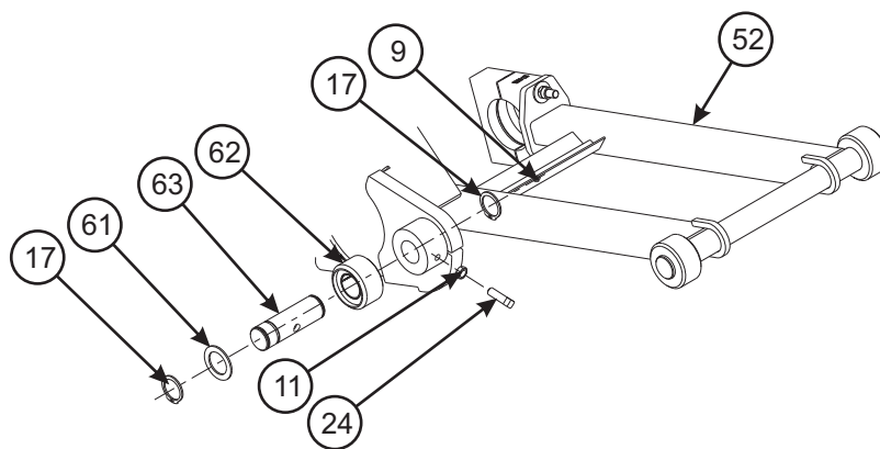
DOCK ARM ROLLER ASSEMBLY
