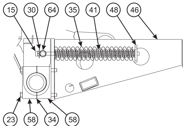
TAIL ASSEMBLY
