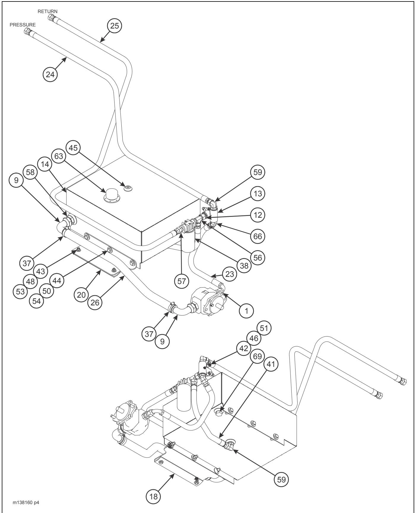
Figure 1-98: 27 HP Slope Engine Package (4 of 4)
