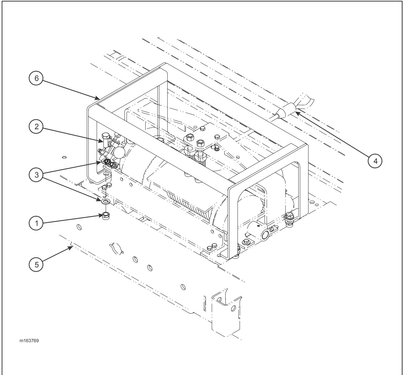
Figure 1-133: Guard Installation, Winch 20K Pivot
