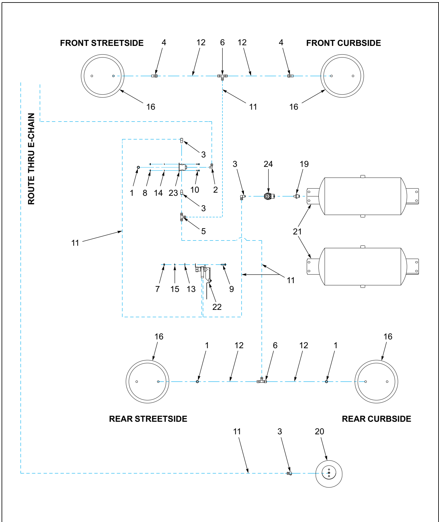
Figure 1-35: Air Ride Suspension - 930D
