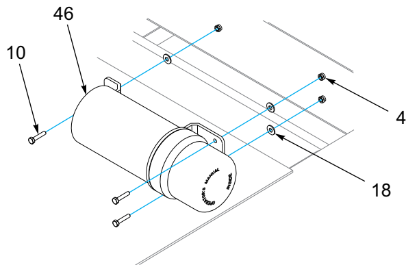
MANUAL TUBE ASSEMBLY
