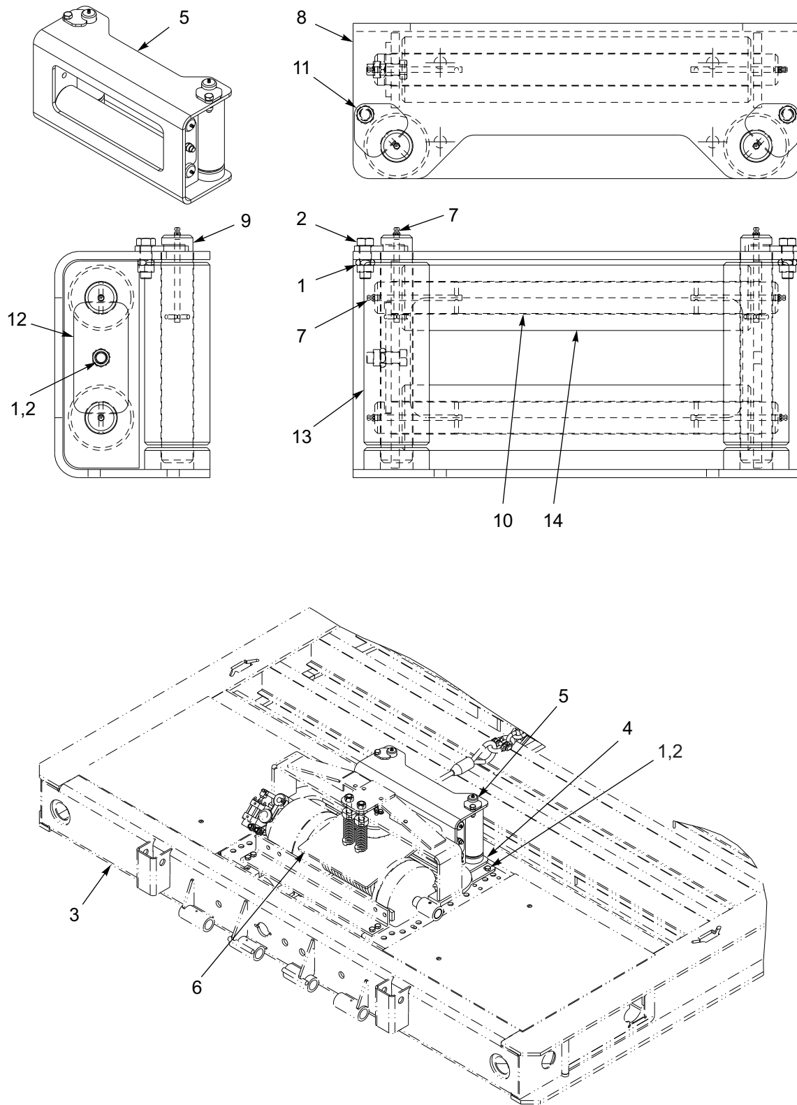
Figure 1-109: 4 Roller Guide Installation - 20K (BRADEN)
