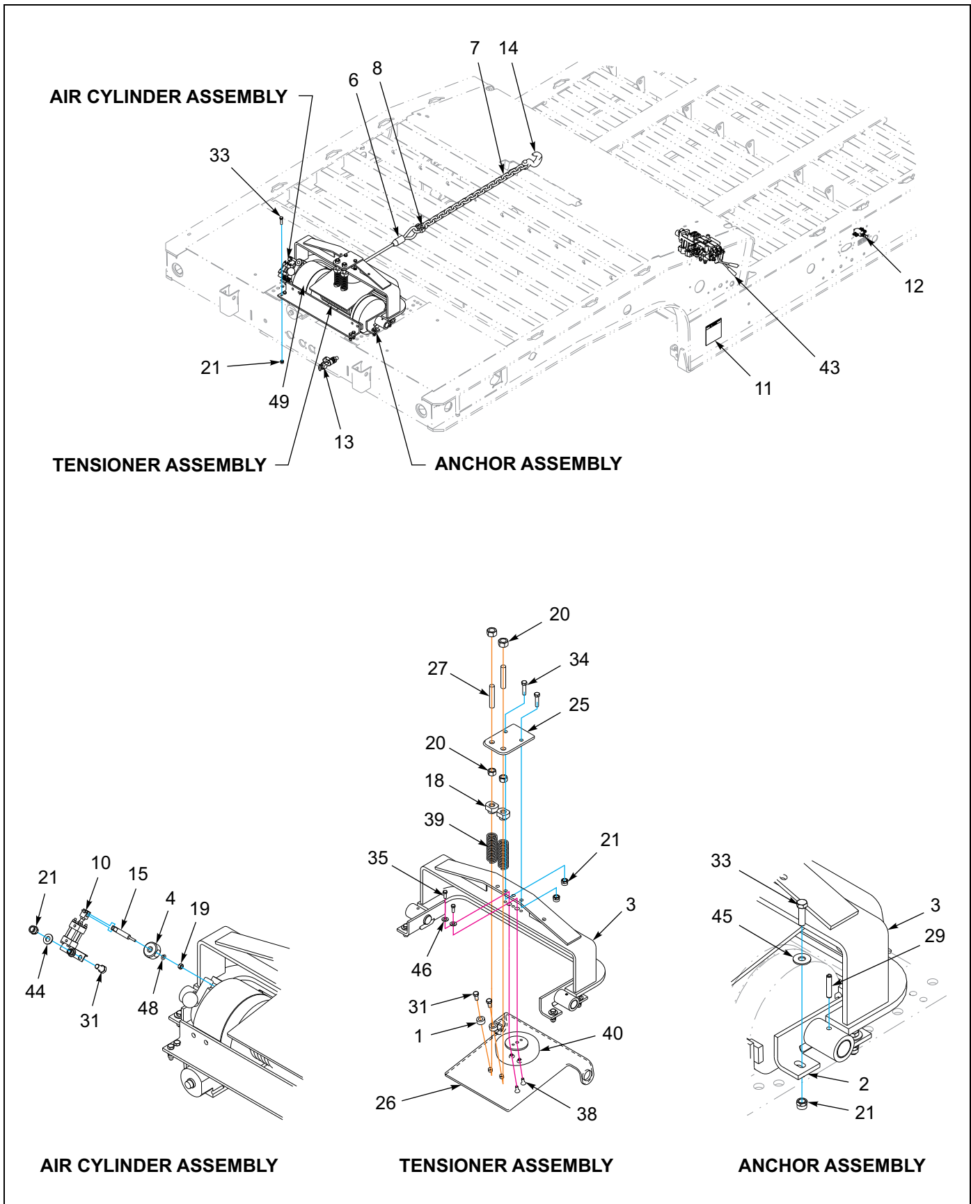
Figure 1-55: Winch Installation - 20K Air Tension/Release (BRADEN) (1 of 3)
