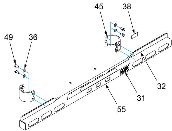
BUMPER ASSEMBLY
