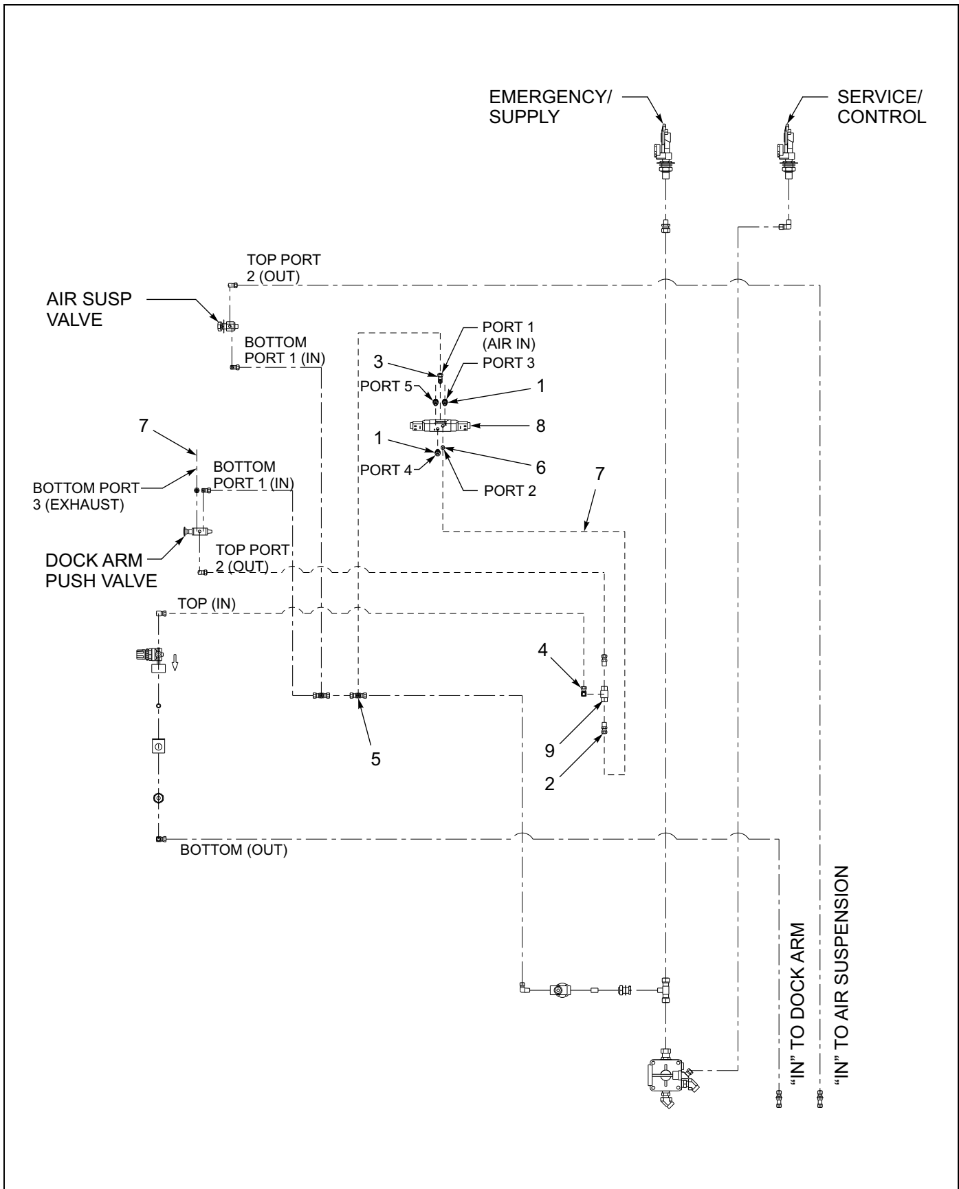
Figure 1-18: Remote Control - Dock Lift Air Items
