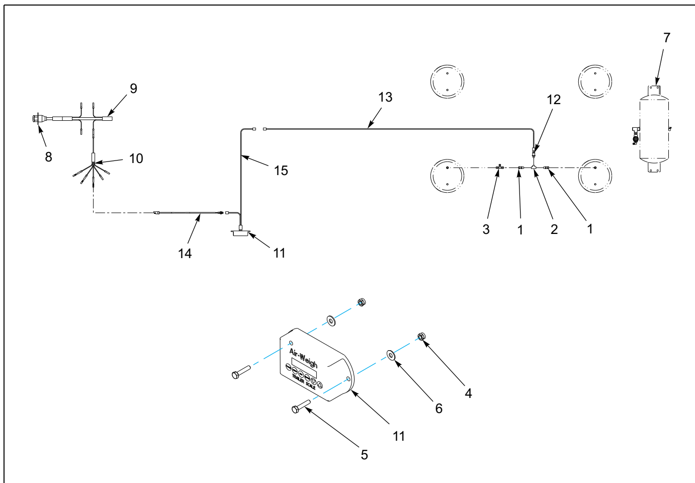
Figure 1-70: Air Digital Scale - Loadmaxx System
