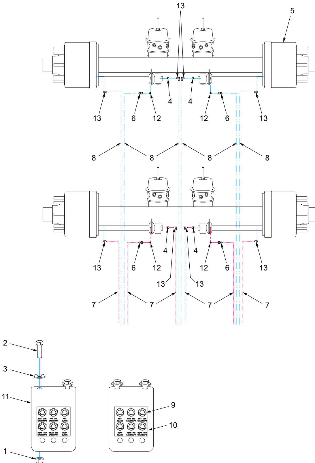
Figure 1-33: Grease System - 930D
