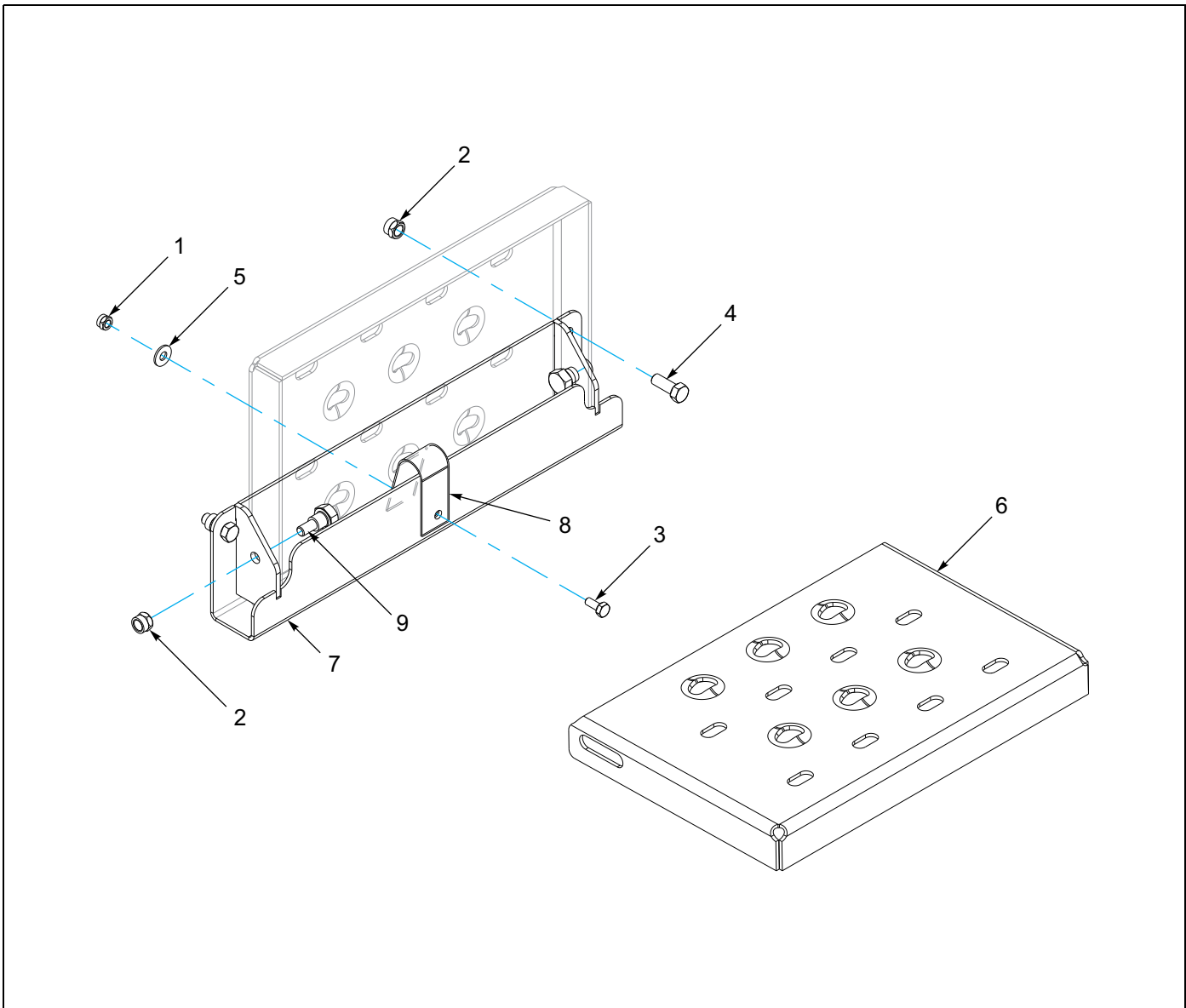
Figure 1-113: Folding Step Assembly - Double Drop Frame
