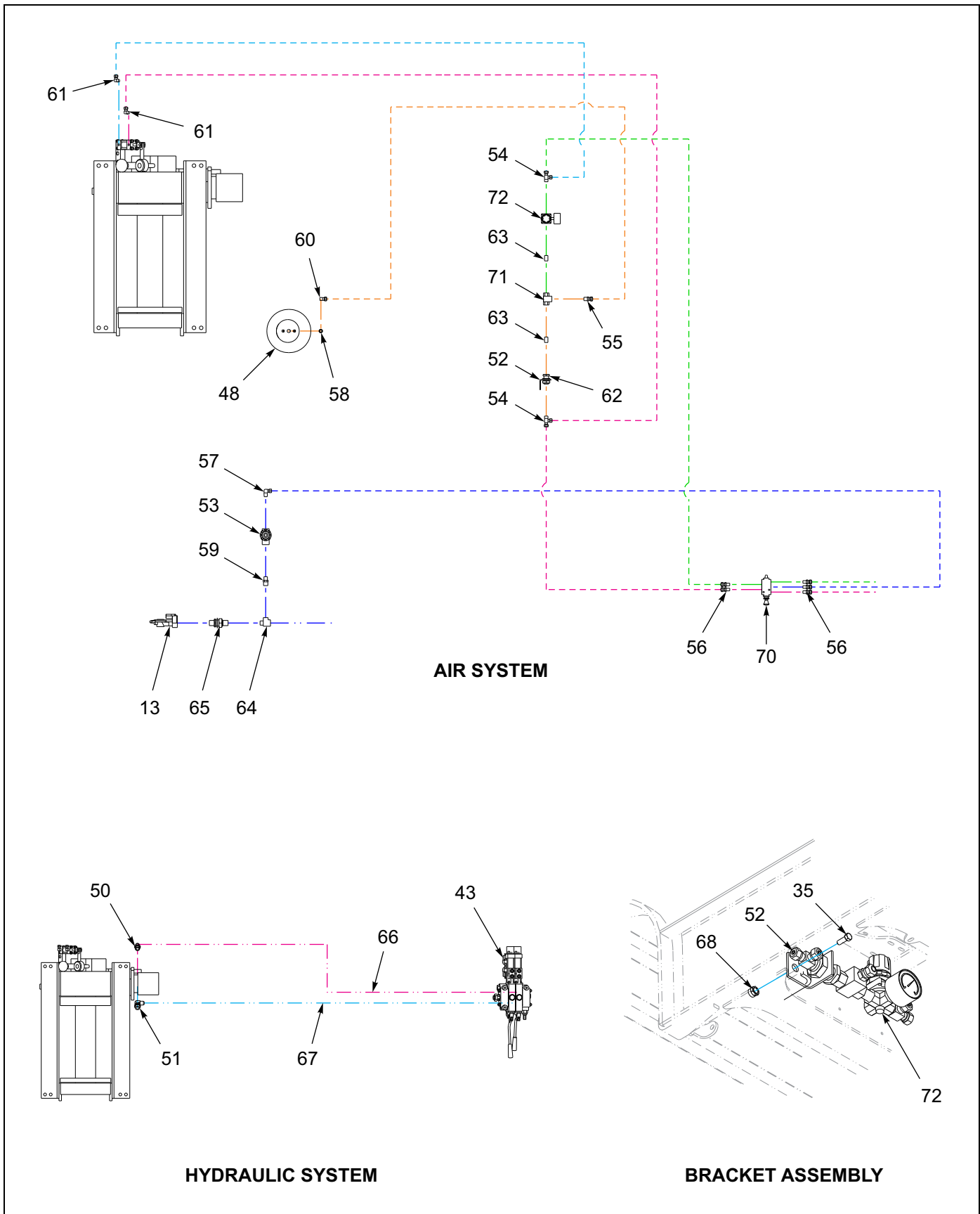
Figure 1-57: Winch Installation - 20K Air Tension/Release (BRADEN) (3 of 3)
