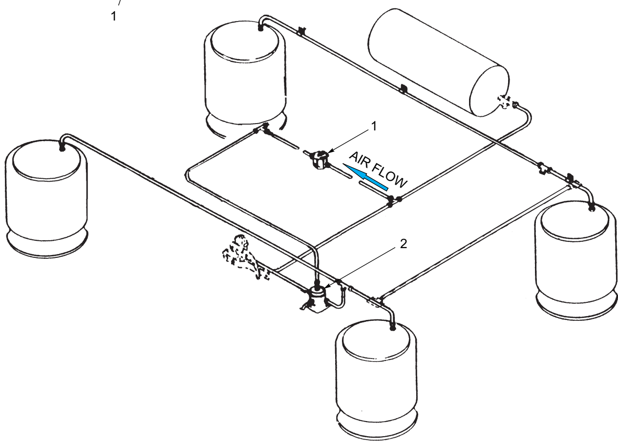
Figure 1-38: Air Control Kit - Lower Suspension
