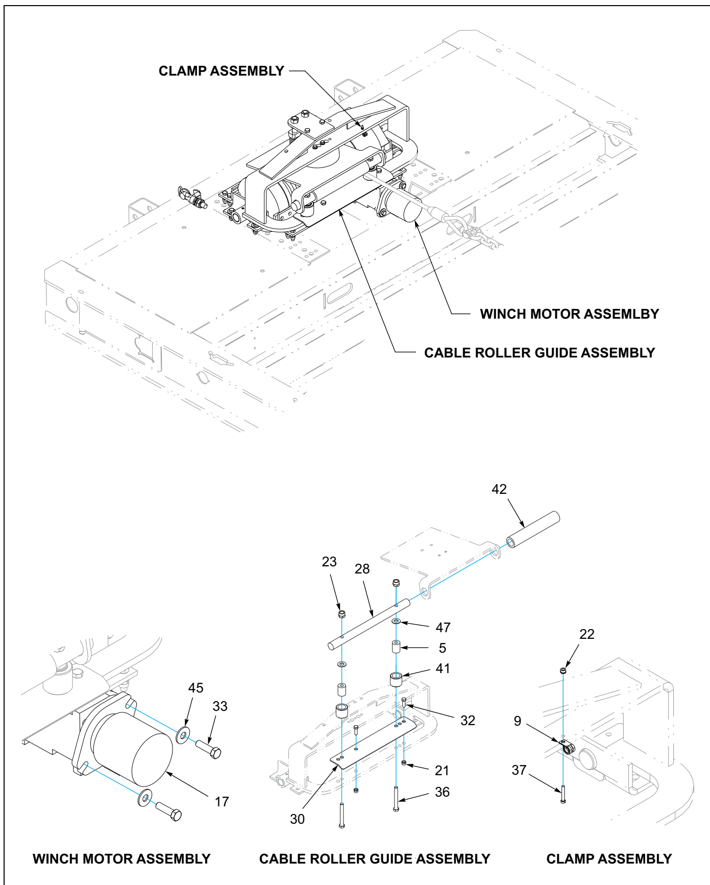
Figure 1-56: Winch Installation - 20K Air Tension/Release (BRADEN) (2 of 3)
