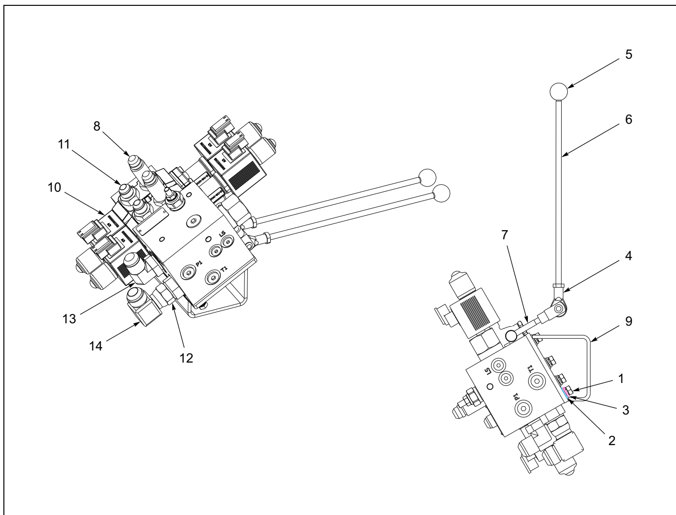
Figure 1-23: Valve Assembly - 2 Spool Control
