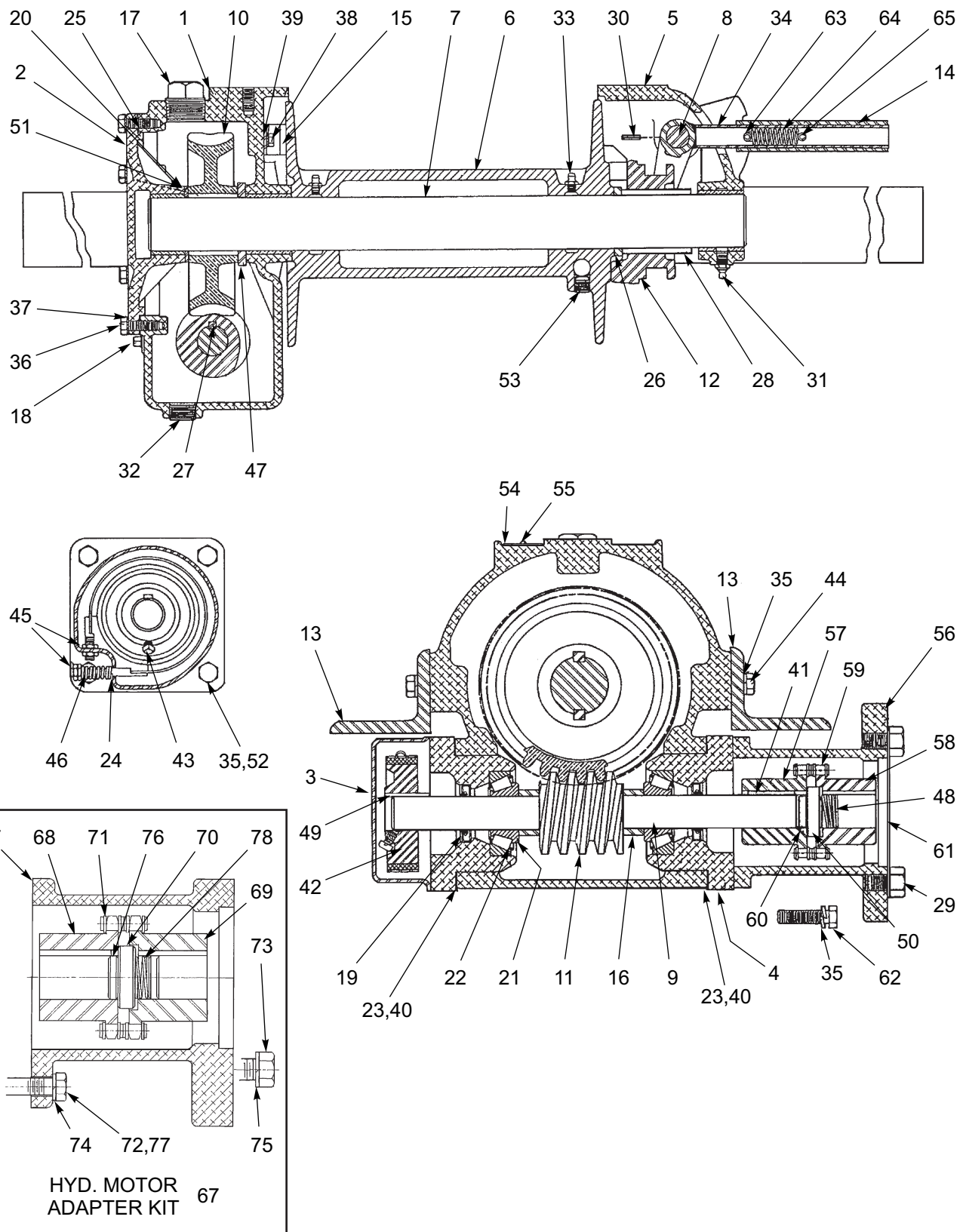
Figure 1-53: Winch Items - 12,000 Lb. (BRADEN)
