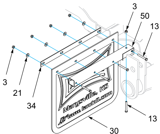
MUD FLAP ASSEMBLY
