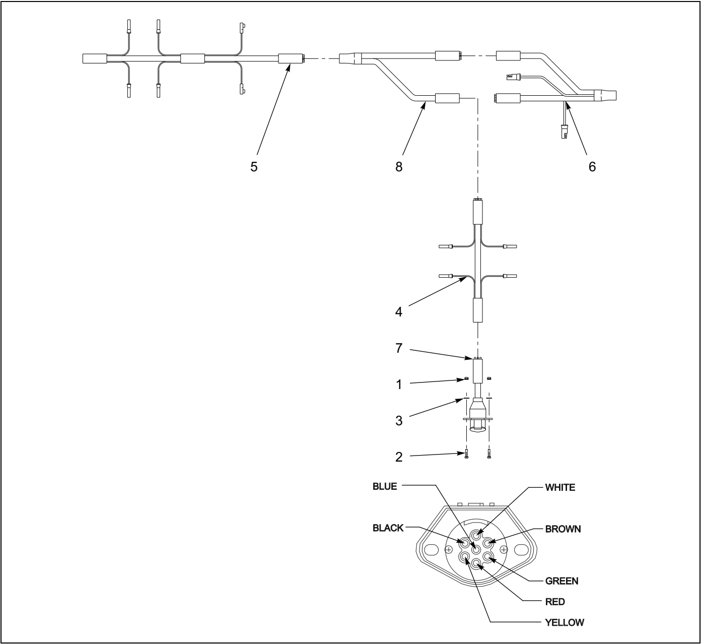
Figure 1-83: 7-Way Electrical Installation
