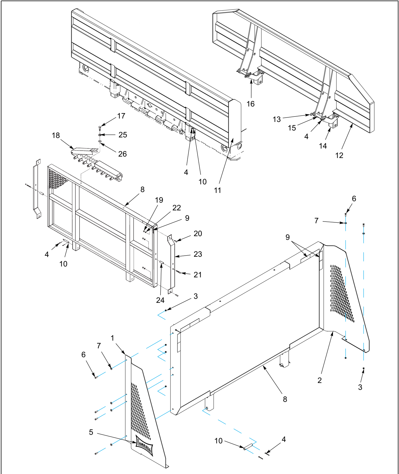
Figure 1-73: Bulkhead Assembly
