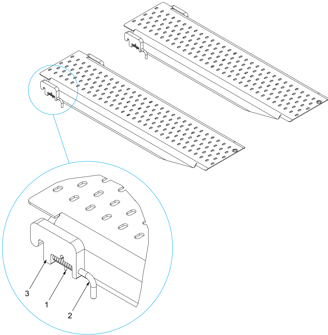
Figure 1-106: Ramp Assembly - Aluminum
