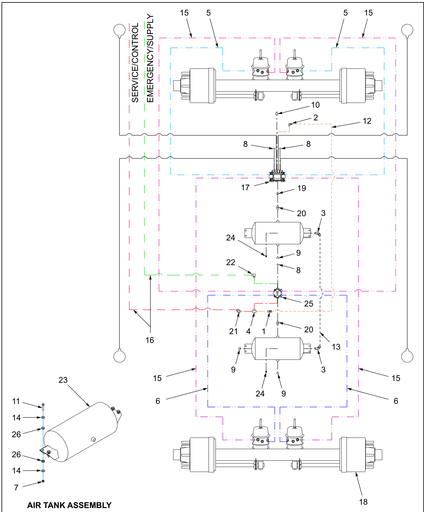
Figure 1-43: Air Brake System - 930D
