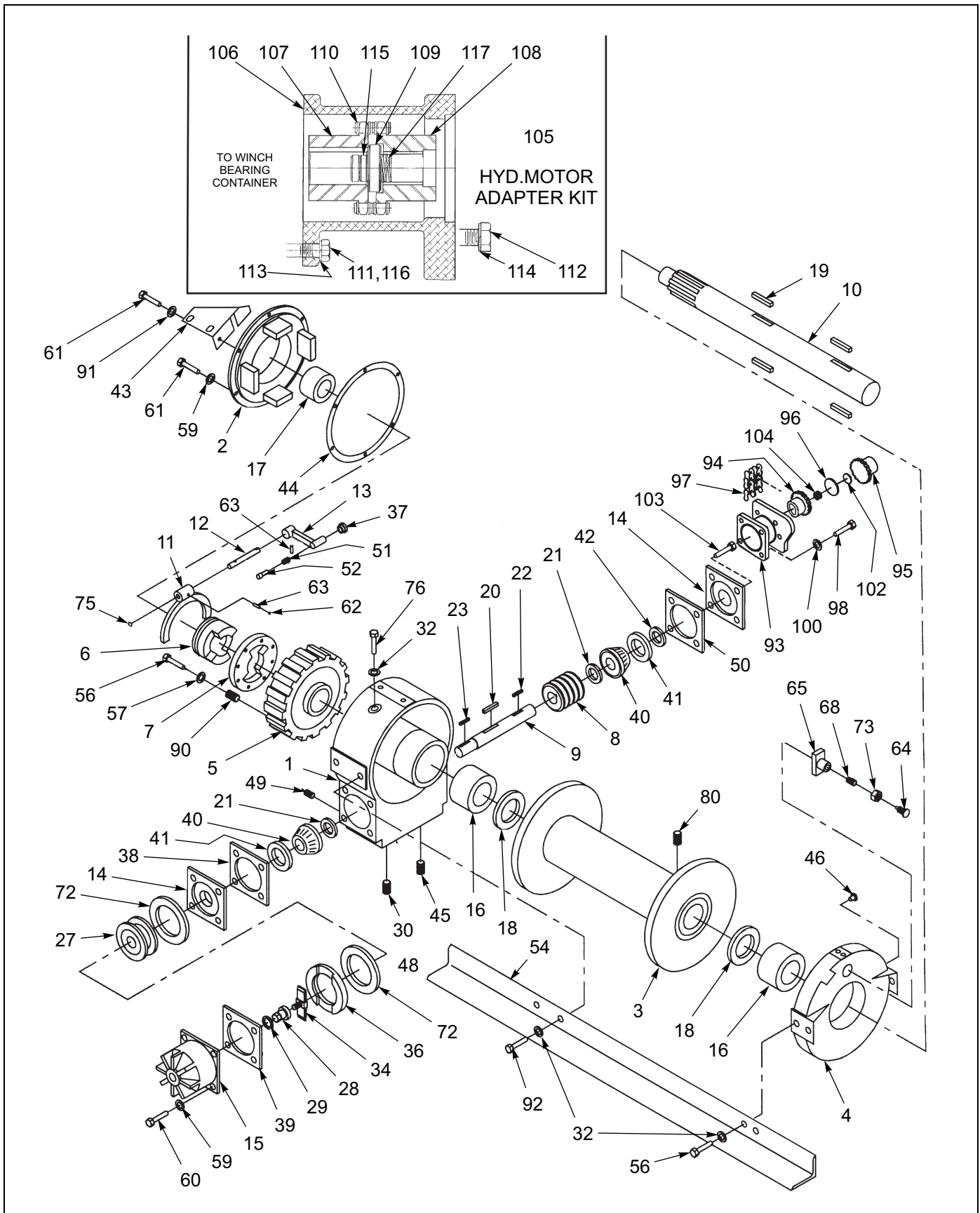
Figure 1-58: Winch Items - 20,000Lb. (BRADEN)
