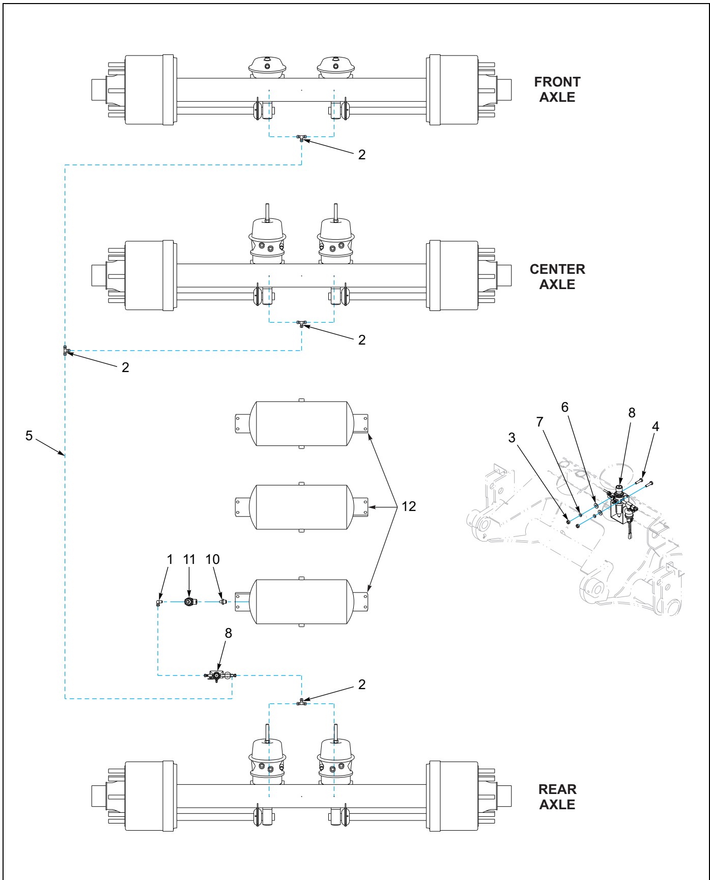
Figure 1-49: Tire Inflation System - 950D
