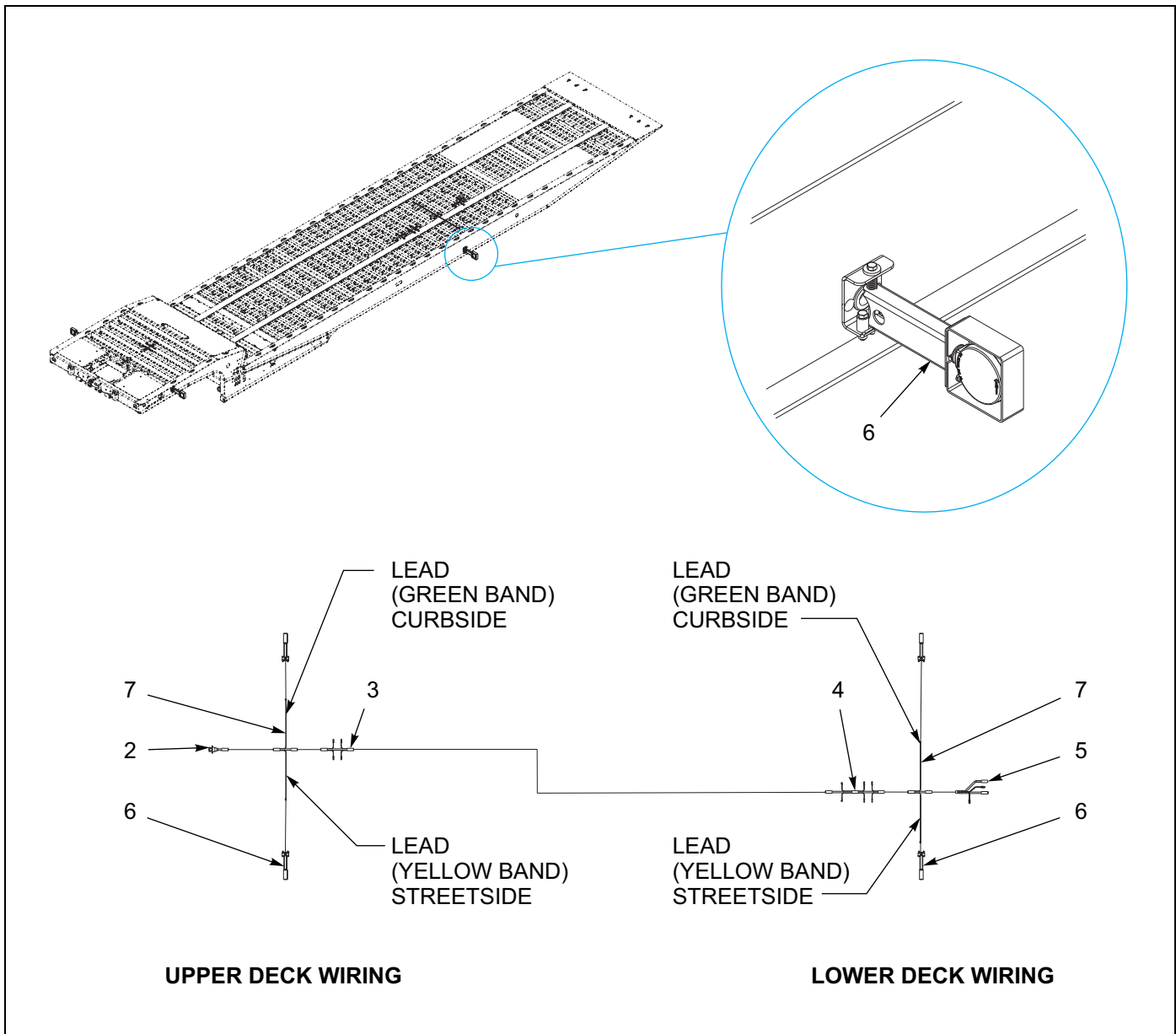
Figure 1-100: Swingout Light Installation
