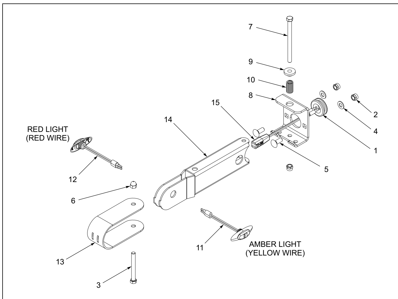
Figure 1-104: Swing-Arm Light Assembly - CURB
