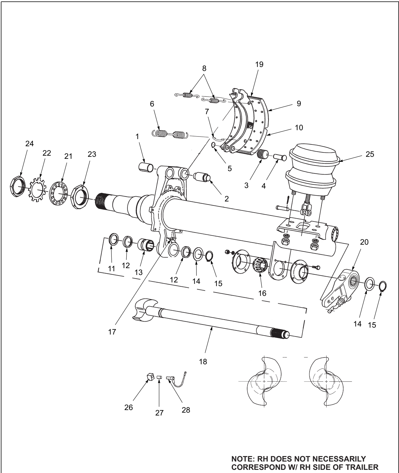
Figure 1-40: Axle and Brake Assembly - Dexter 12-1/4" X 7-1/2"
