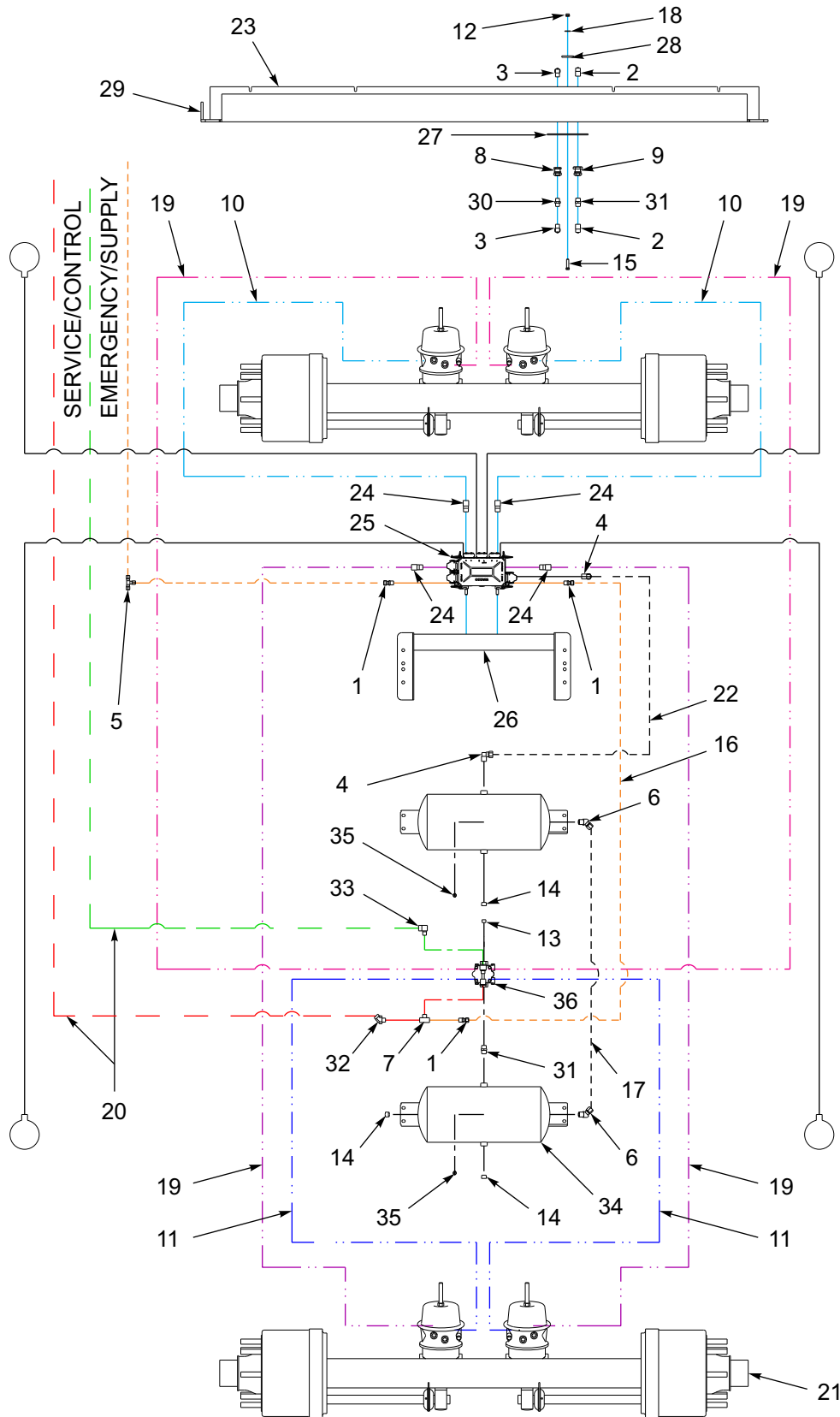
Figure 1-44: Air Brake System - 930D W/ RSS
