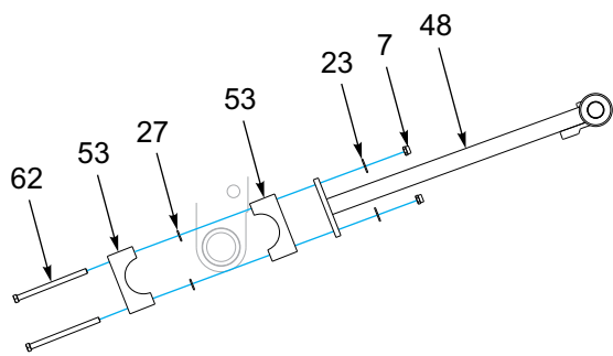
DOCK ARM ASSEMBLY
