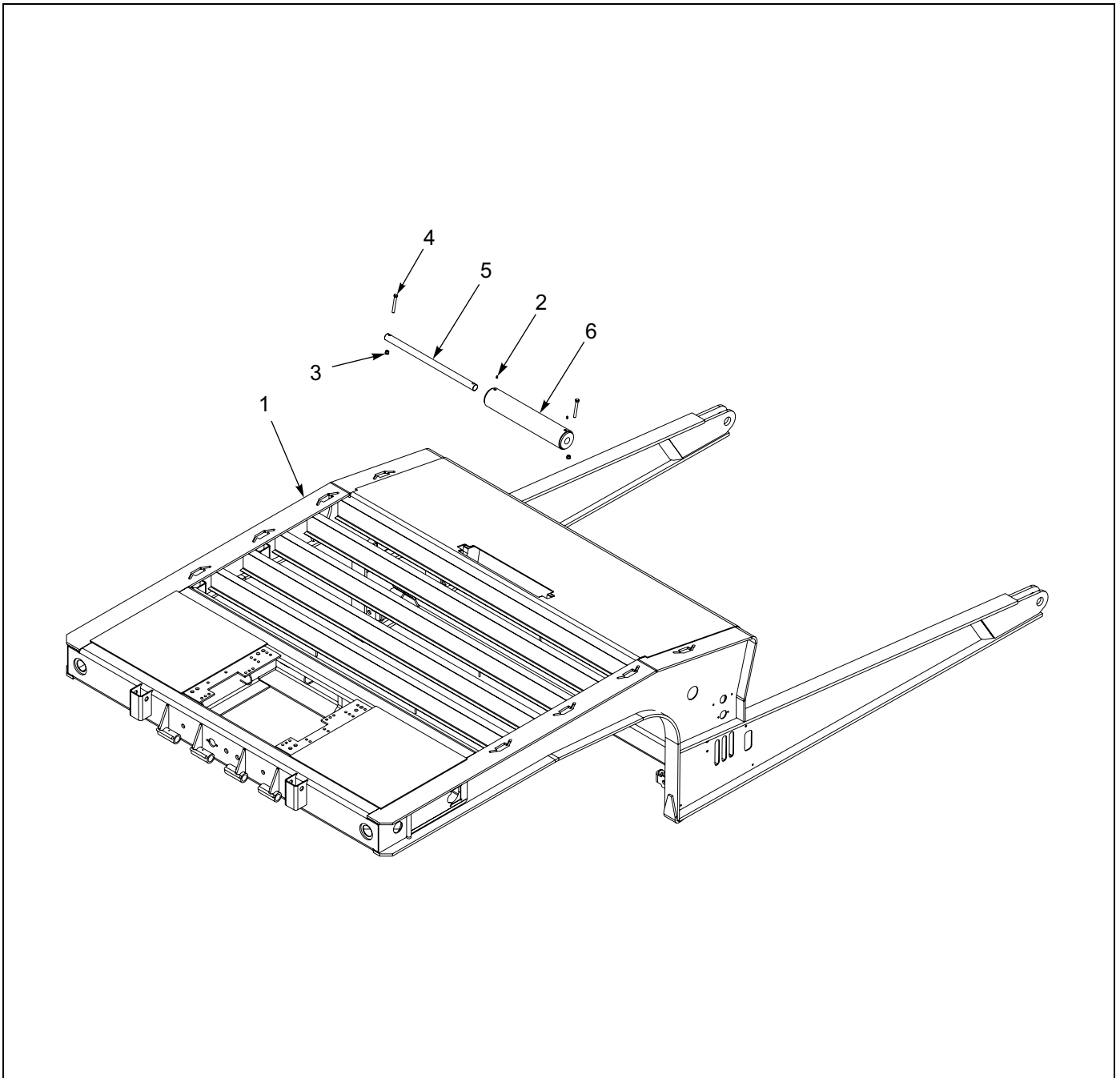
Figure 1-118: Upper Deck - Roller Installation
