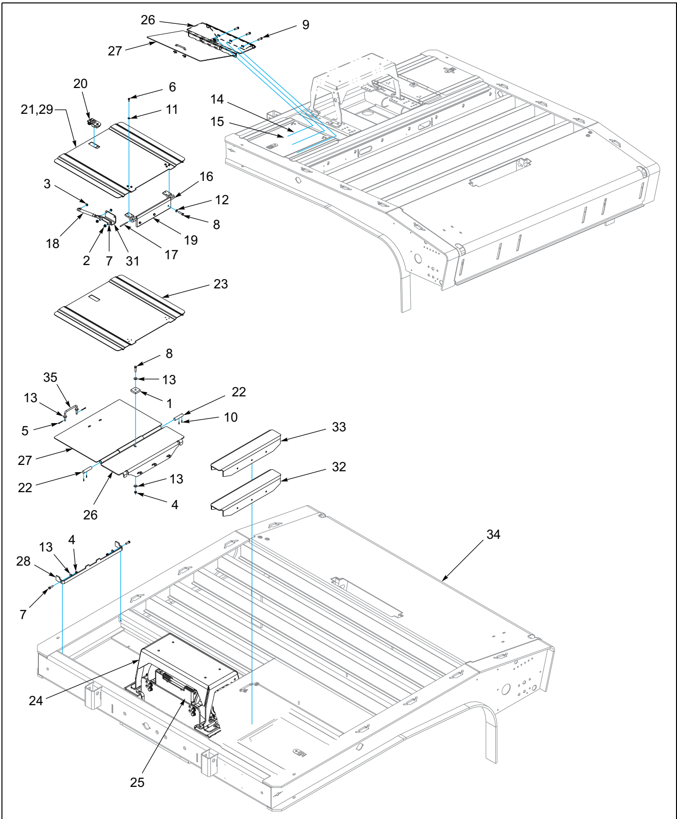
Figure 1-11: Top Lid Installation
