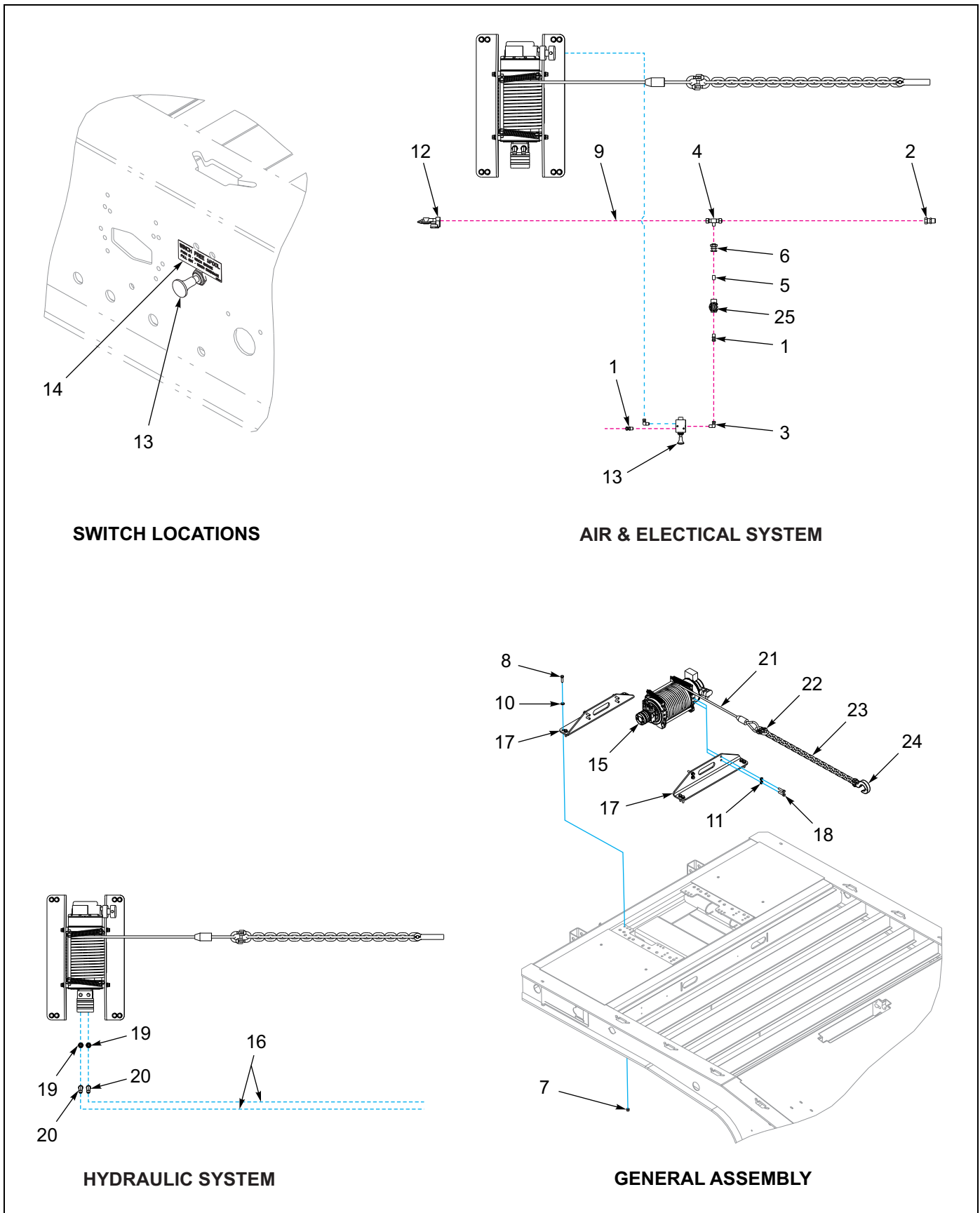
Figure 1-61: Winch Installation - 12K (WARN)
