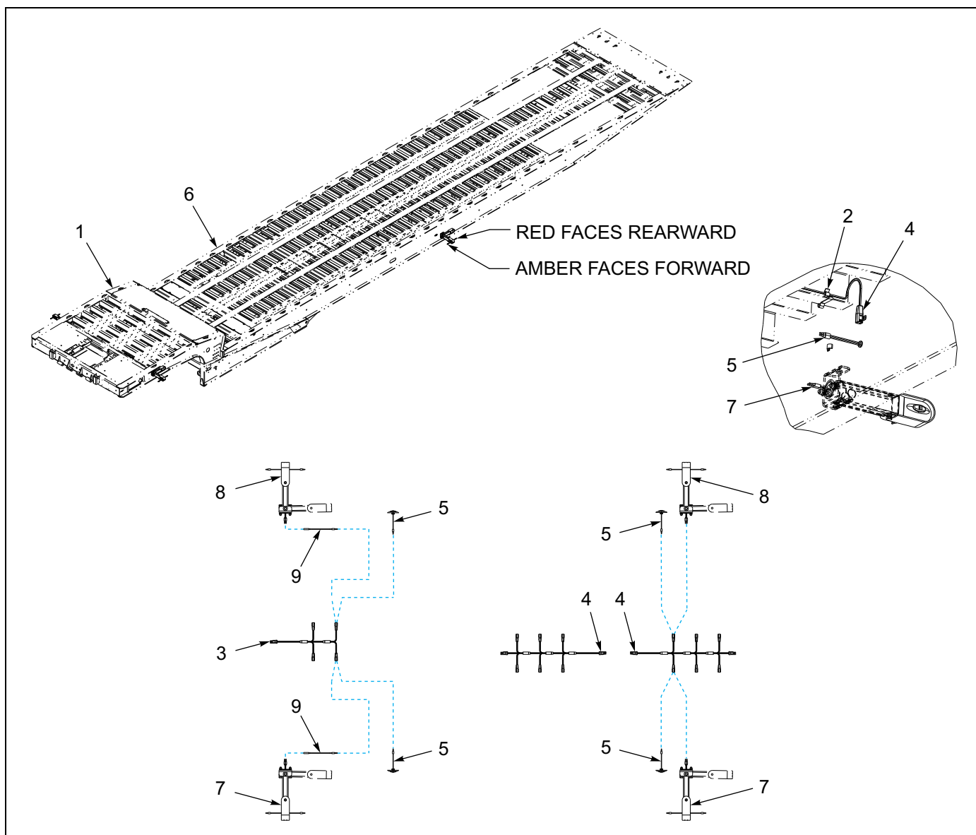
Figure 1-102: Swingout Marker Light Installation - Red/Amber
