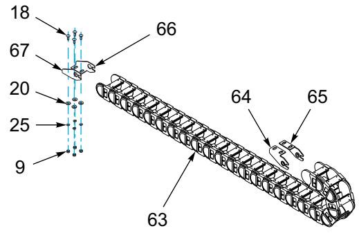
E-CHAIN ASSEMBLY
