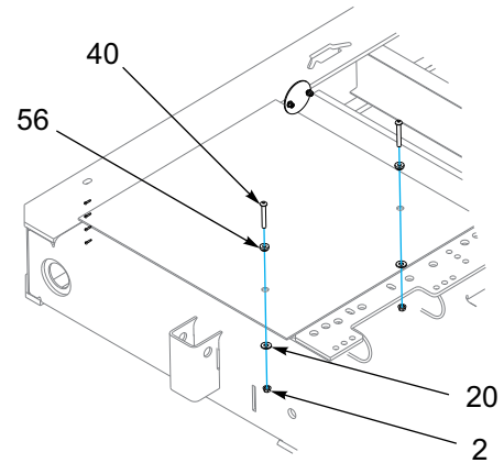
TOP TOOLBOX COVER (ONLY P/N 56 IS USED TO PLUG HOLES WHEN OPTIONAL ENGINE STANDARD IS NOT AVAILABLE)
