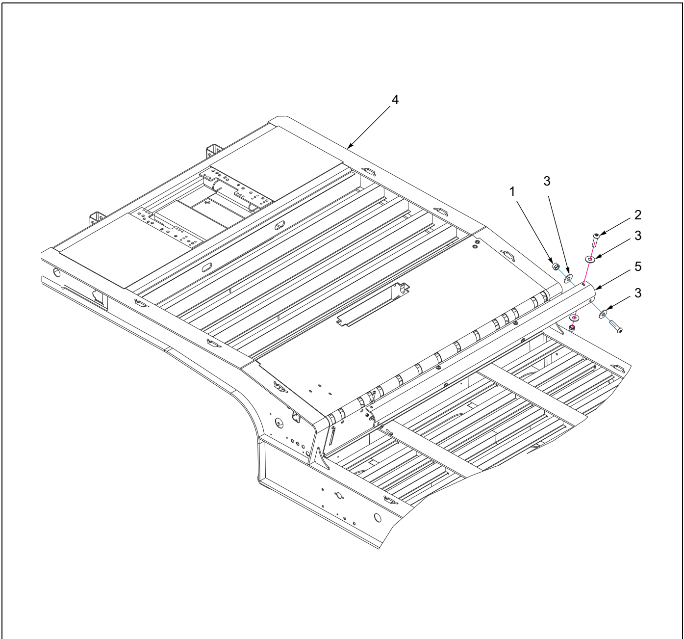
Figure 1-78: Bumper - Fork Lift Plate Installation
