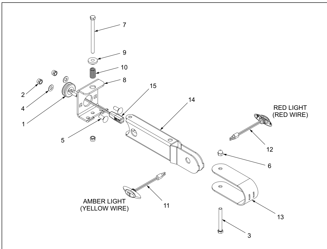
Figure 1-103: Swing-Arm Light Assembly - STREET
