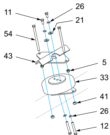
DOCK LIFT ARM AIR BAG MOUNT ASSEMBLY
