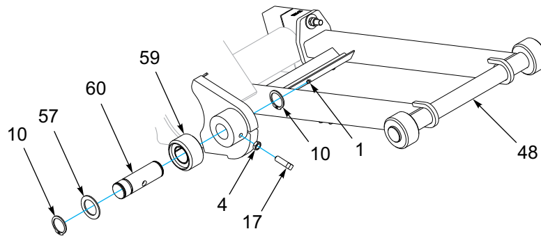
DOCK ARM ROLLER ASSEMBLY
