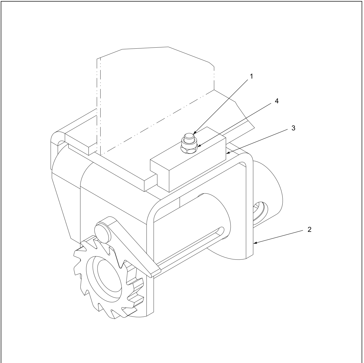
Figure 1-124: Winch - 4" Webbing Sliding Assembly
