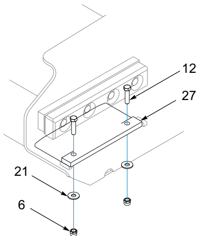
UNDERCARRIAGE GLIDE ASSEMBLY
