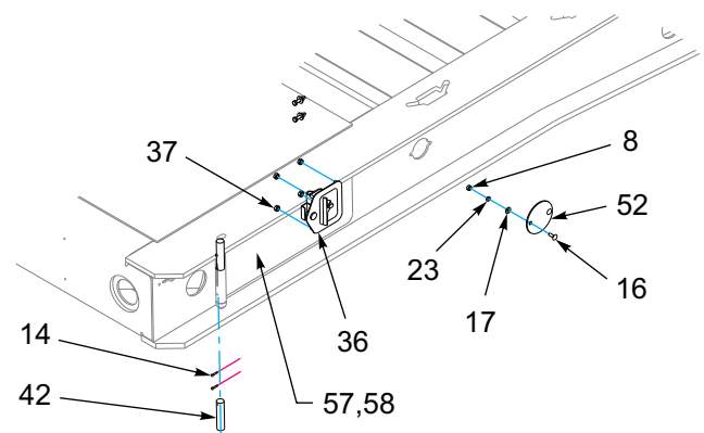
TOOLBOX & LATCH ASSEMBLY
