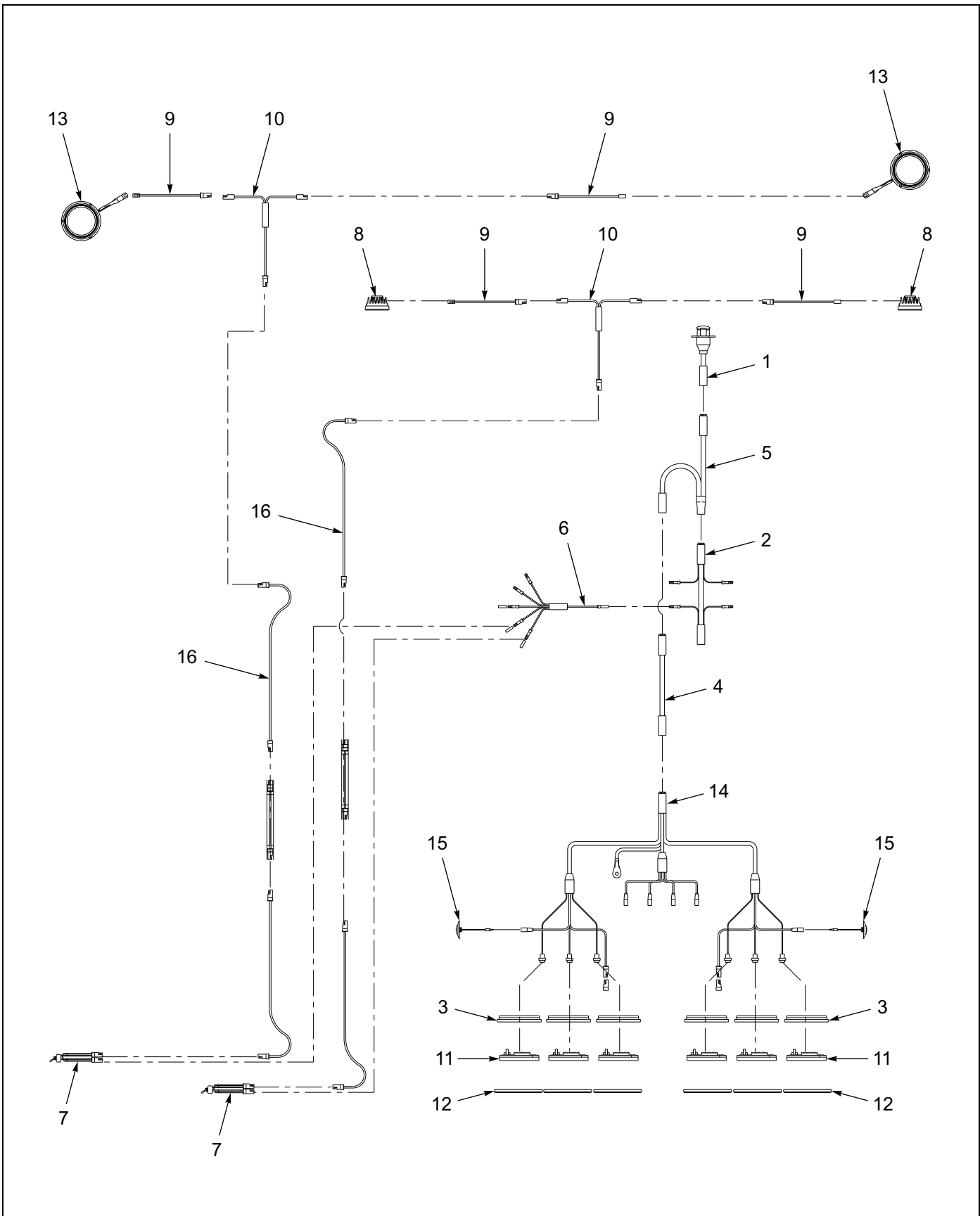
Figure 1-75: Bulkhead - Chain Rack Lights Electrical System
