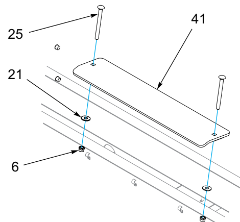
WEAR PLATE ASSEMBLY
