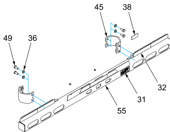
BUMPER ASSEMBLY
