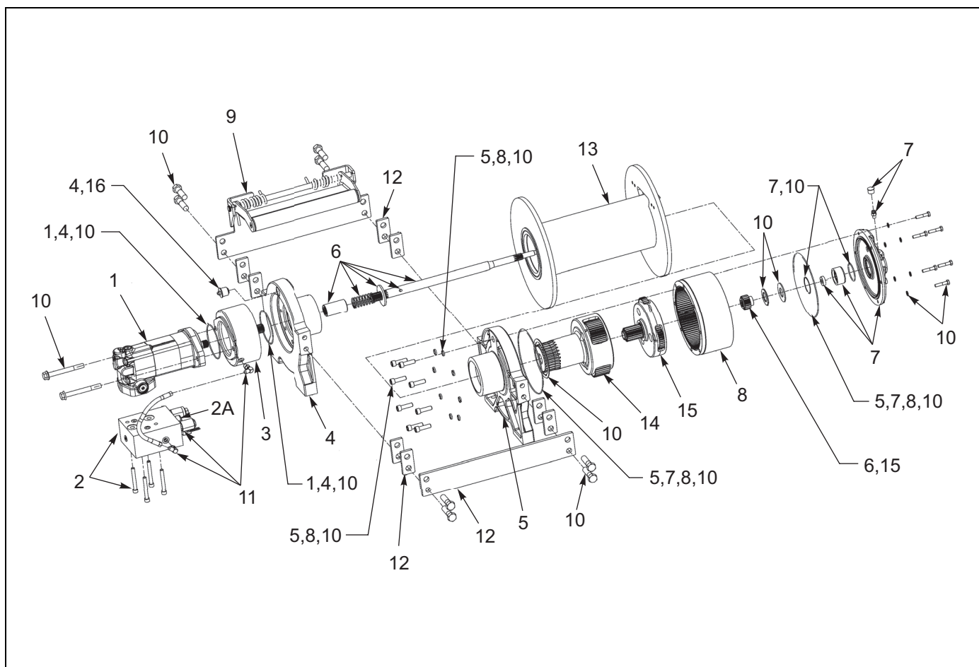
Figure 1-66: Winch Items - 30K 2 Speed (WARN)
