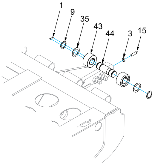
ROLLER ASSEMBLY
