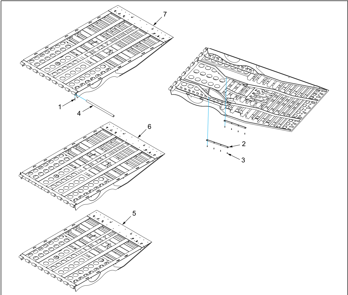
Figure 1-12: Tail Assembly - General Assembly (12', 14', 15')
