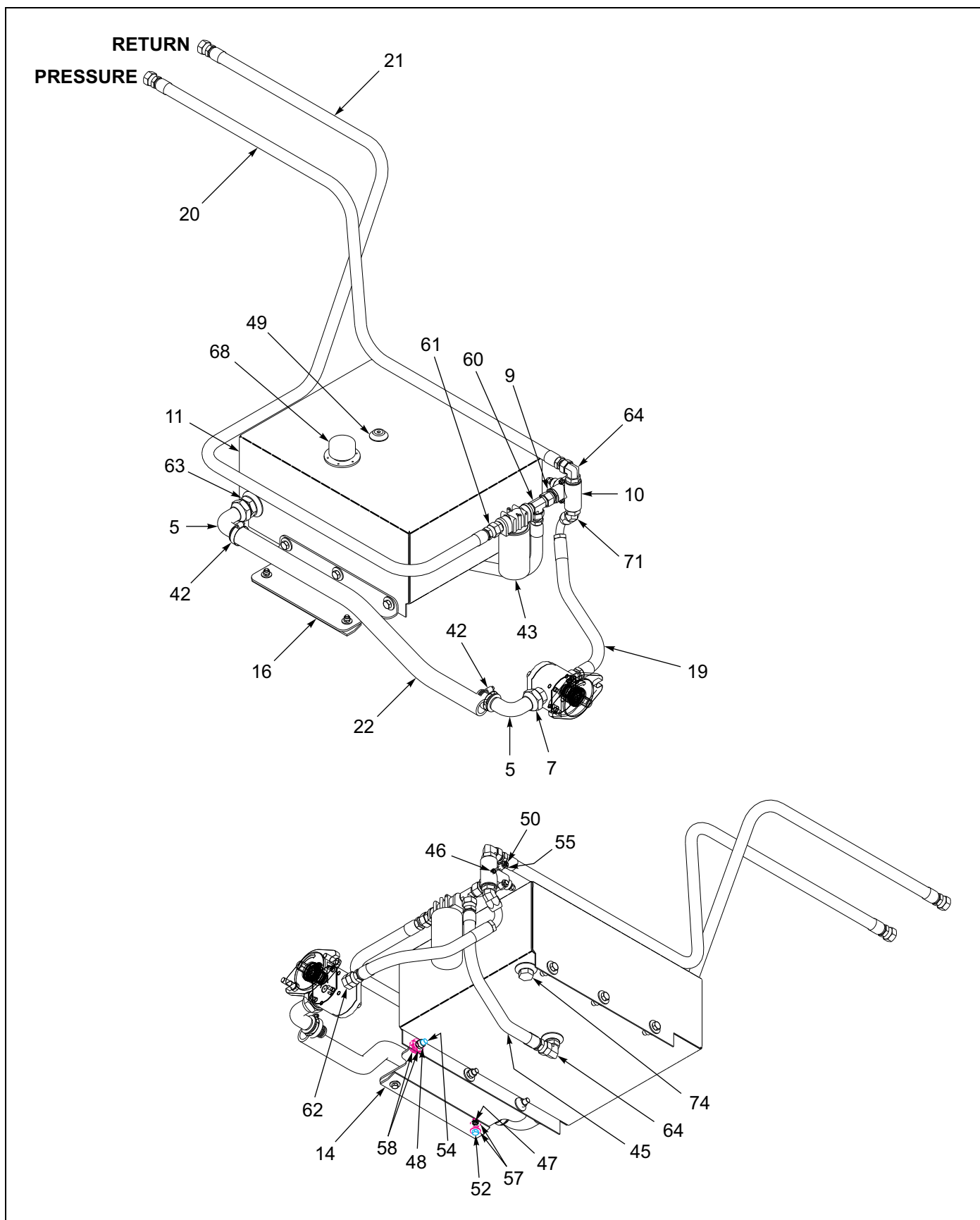
Figure 1-91: Engine - 25 HP Slope Package (4 of 4)
