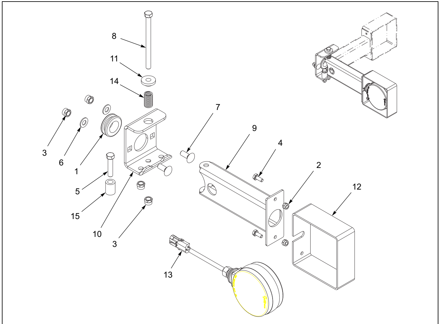
Figure 1-101: Swing-Arm Light Assembly - Turn Signal/Emergency Flasher
