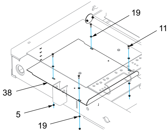
BOTTOM TOOLBOX COVER
