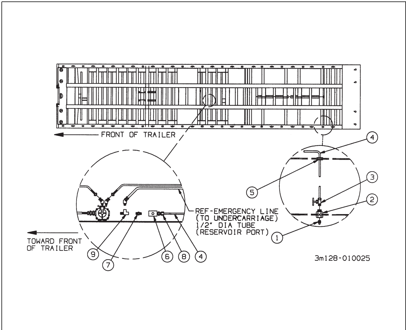
Figure 1-126: Air Outlet Accessory
