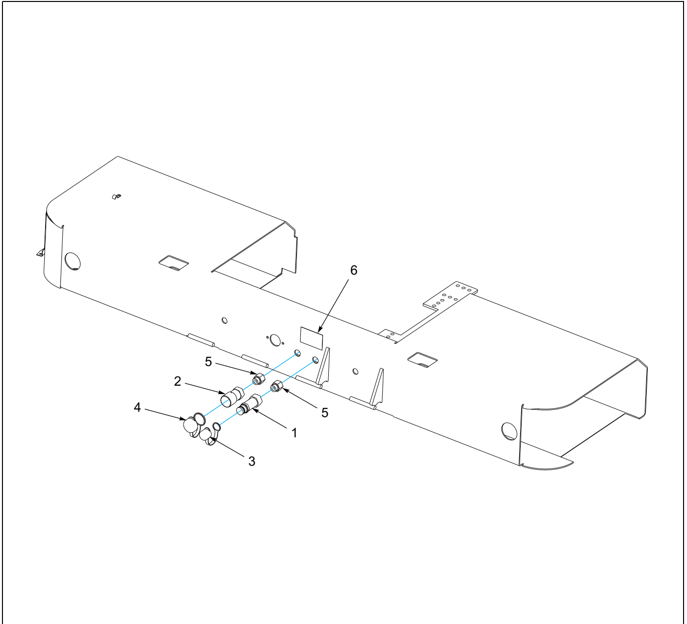
Figure 1-97: Hydraulic Conversion Kit - Ball to Flat
