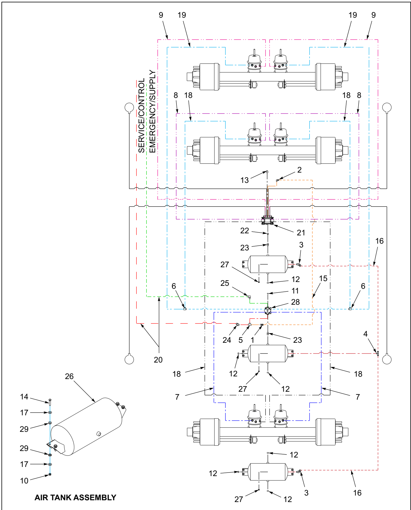
Figure 1-45: Air Brake System - 950D
