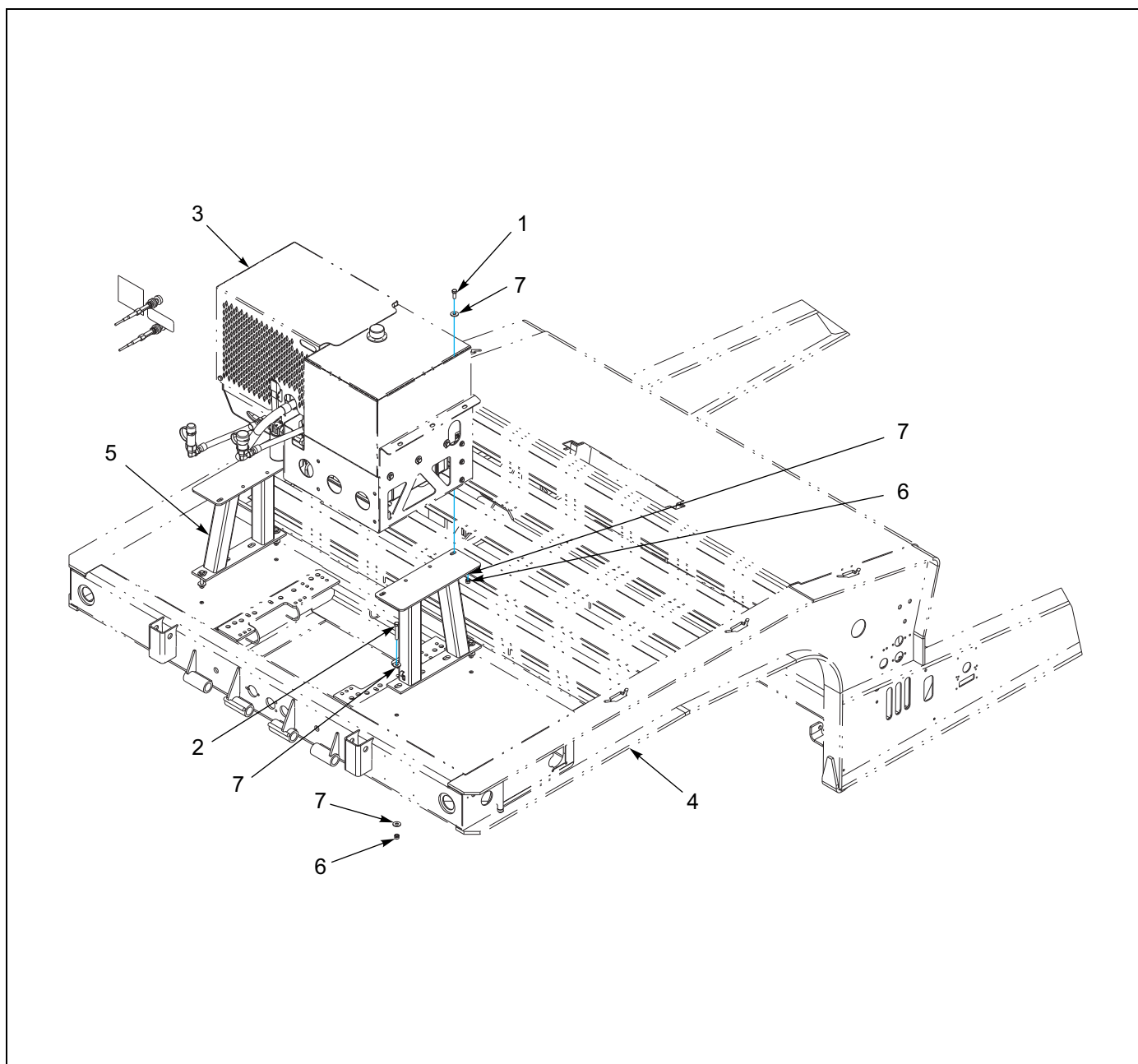
Figure 1-96: Engine - Upper Deck Stand Installation
