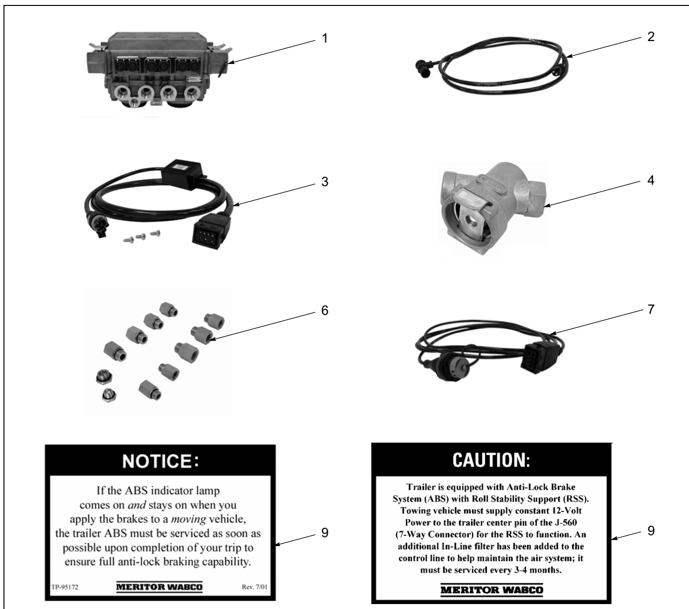
Figure 1-47: ABS Brake Kit - W/ RSS Rockwell
