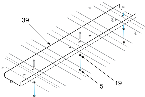
HOSE CHANNEL ASSEMBLY
