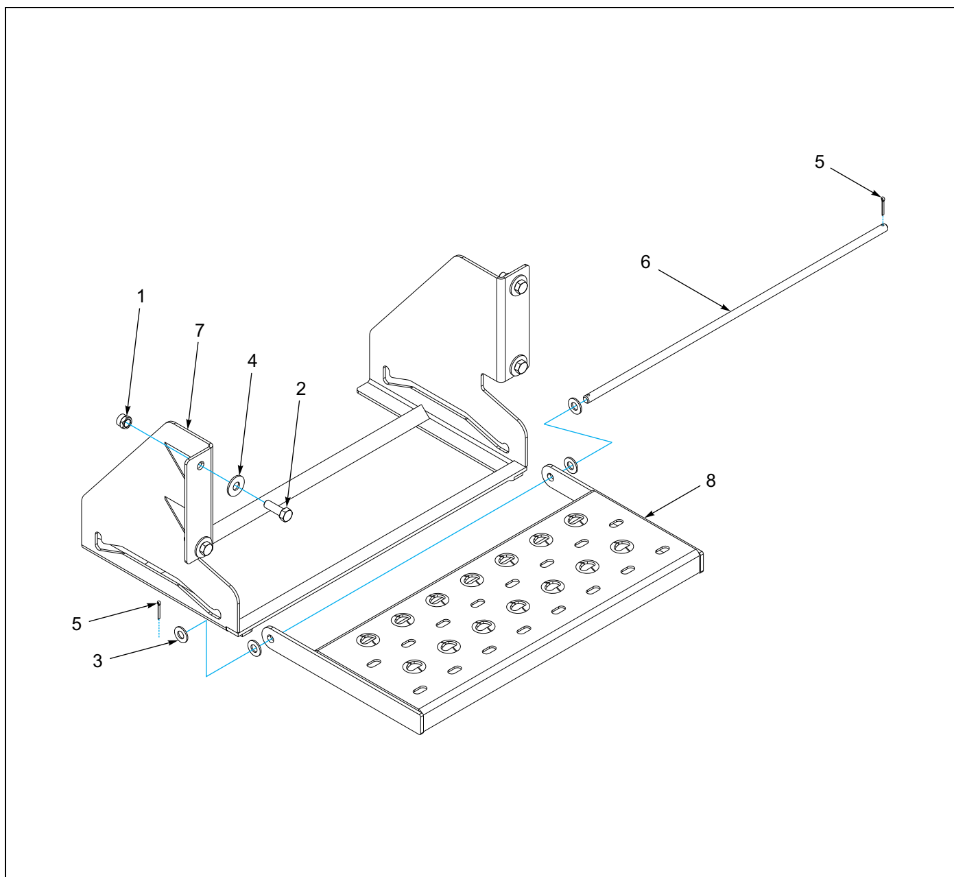
Figure 1-114: Retractable Step Assembly
