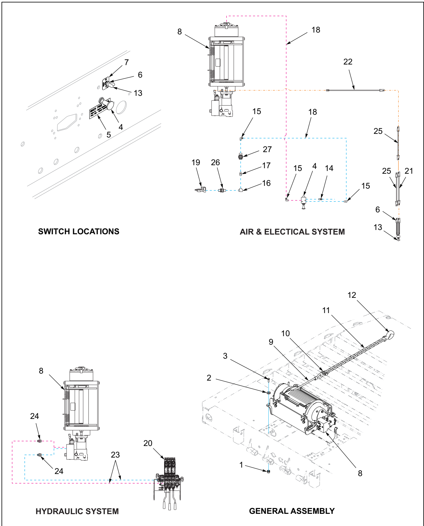
Figure 1-63: Winch Installation - 20K 2 Speed (WARN)
