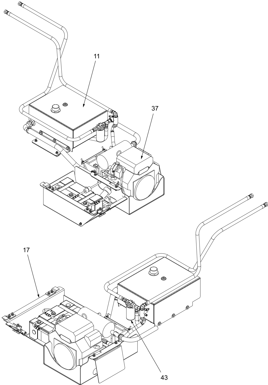
Figure 1-88: Engine - 25 HP Slope Package (1 of 4)
