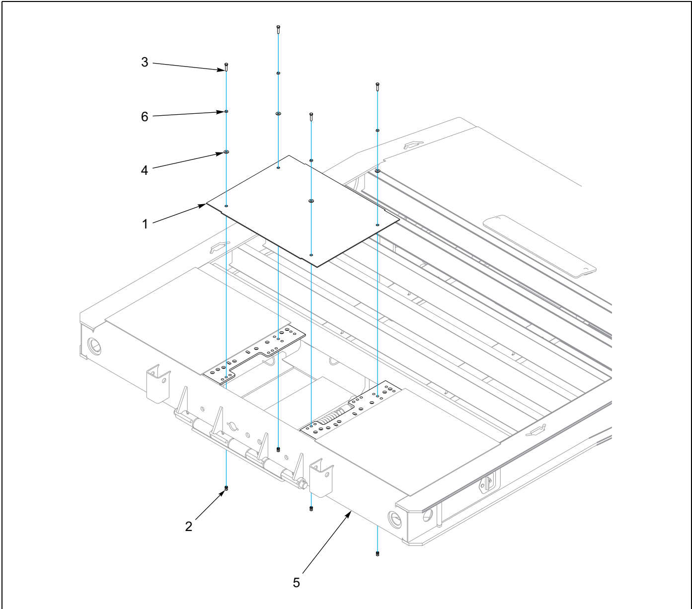
Figure 1-117: Upper Deck Cover Assembly
