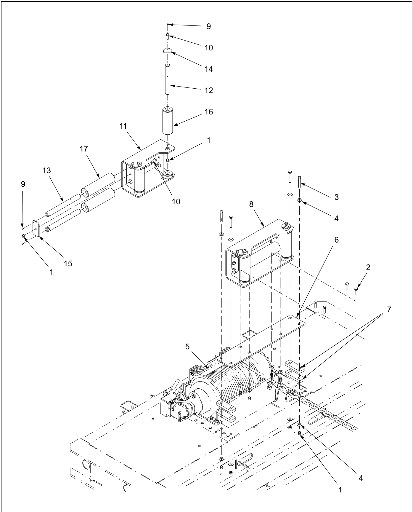
Figure 1-110: 4 Roller Guide Installation - 20K/30K (WARN)
