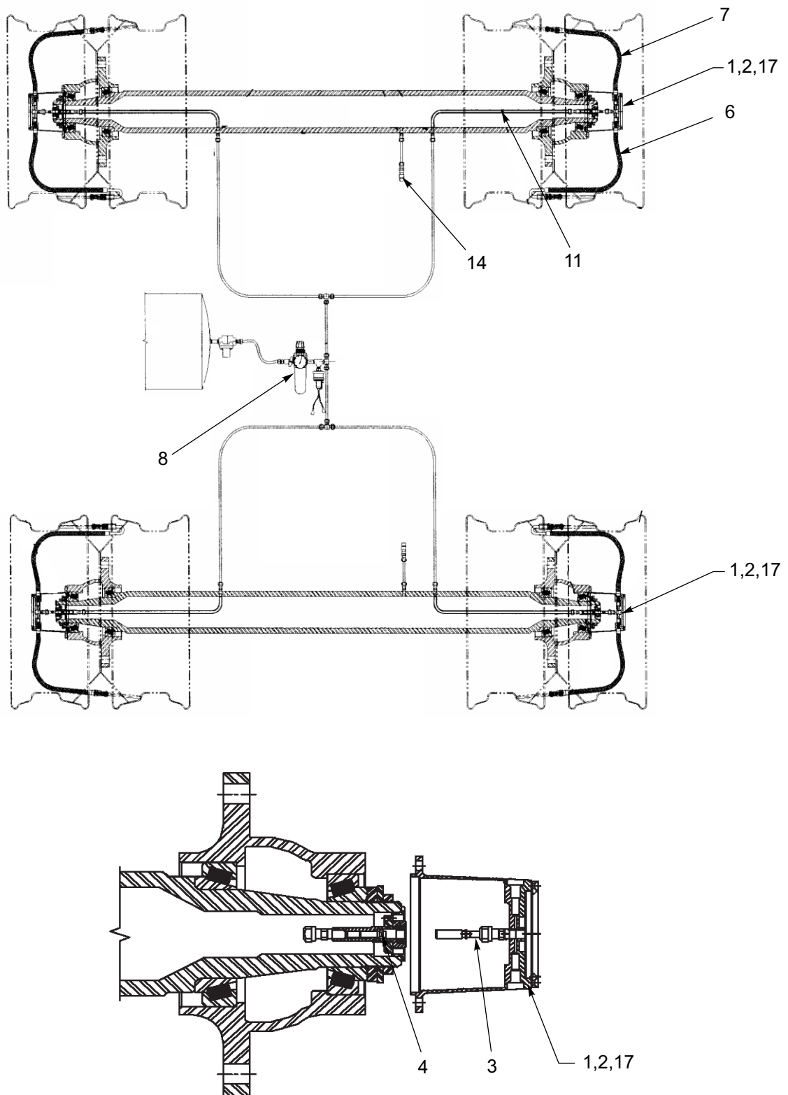
Figure 1-50: Tire Inflation System - 2AX/3AX
