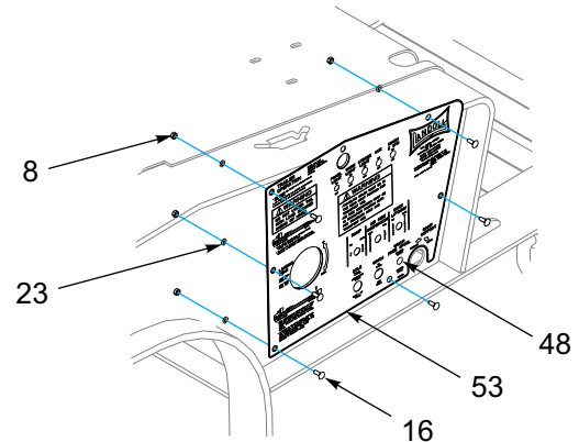
PLACARD ASSEMBLY
