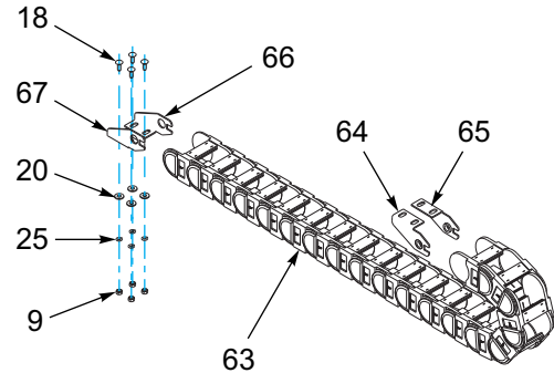
E-CHAIN ASSEMBLY
