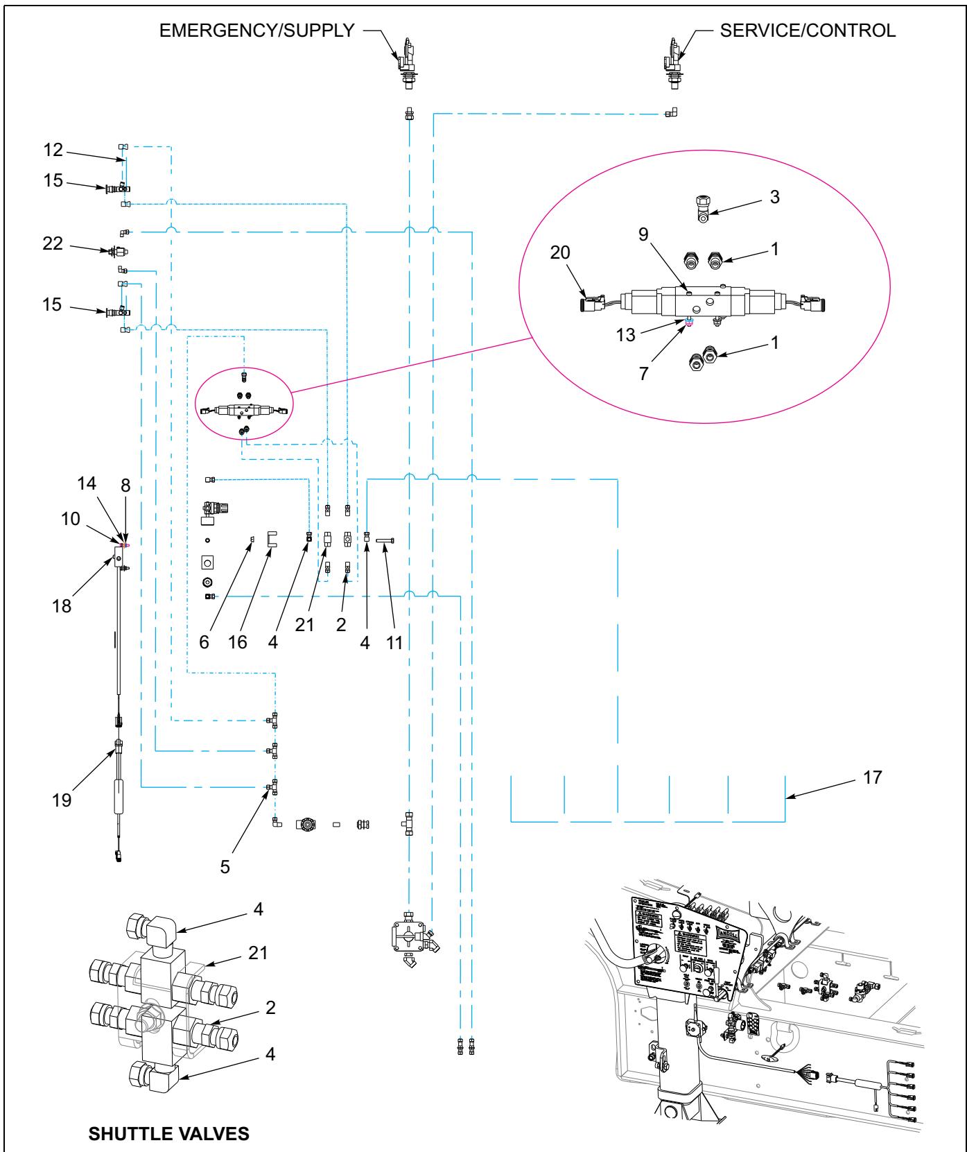
Figure 1-17: Remote Components
