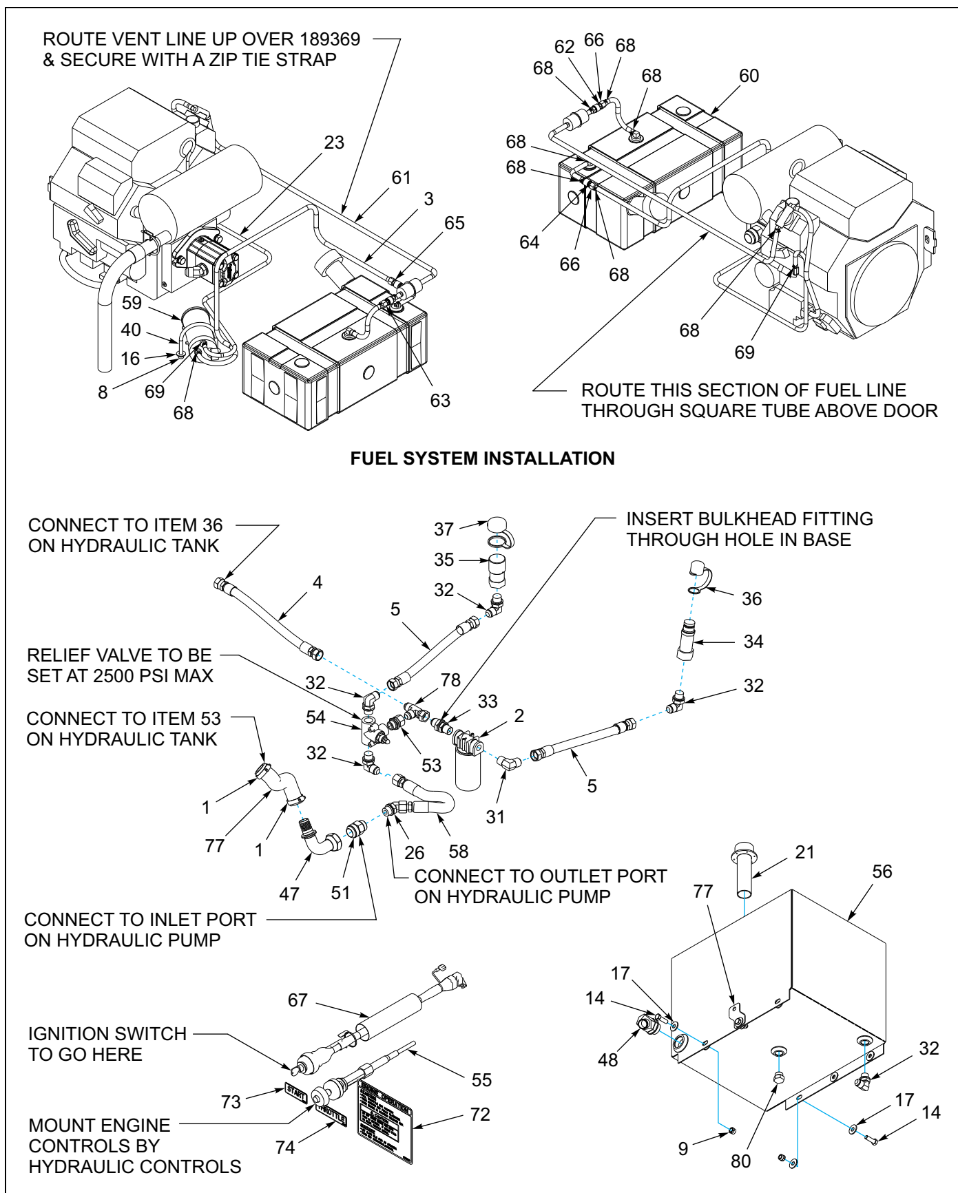
Figure 1-87: Engine - 25 HP Upper Deck Package (4 of 4)
