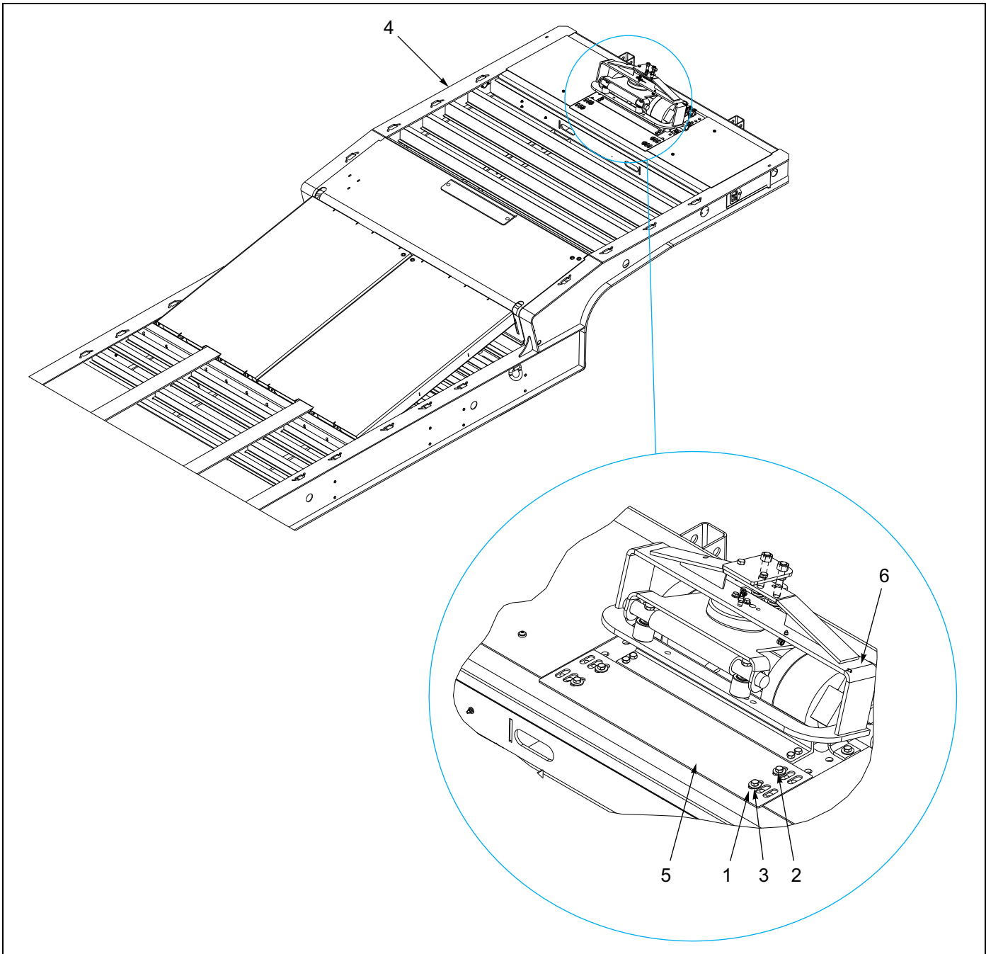
Figure 1-123: Winch - Trim Plate Installation
