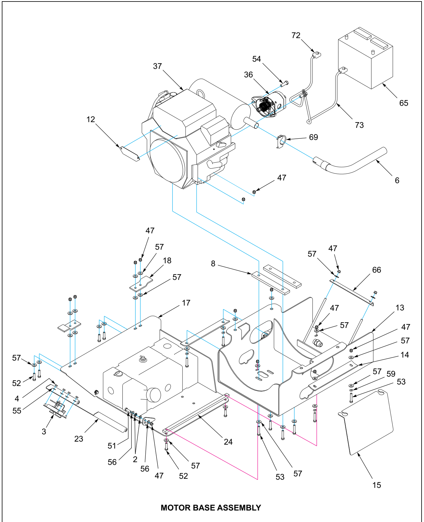
Figure 1-89: Engine - 25 HP Slope Package (2 of 4)
