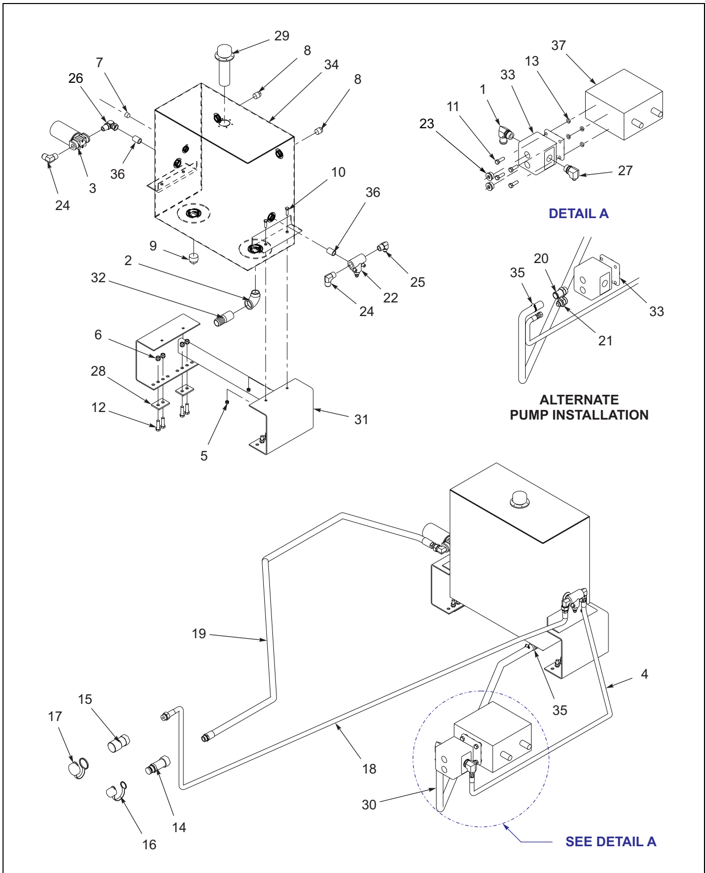
Figure 1-98: Hydraulic Wet Kit Items - 30 Gallon
