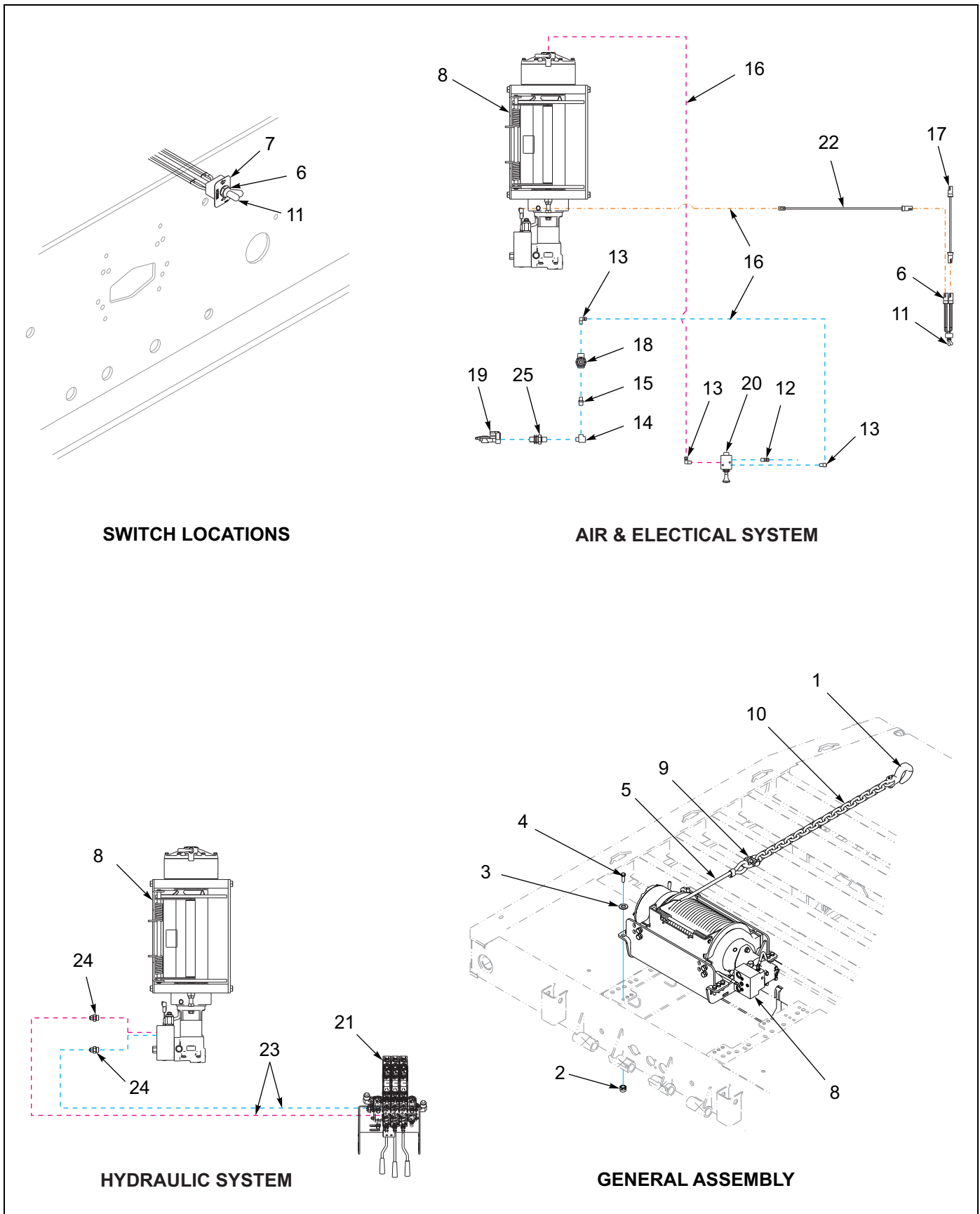
Figure 1-65: Winch Installation - 30K 2 Speed (WARN)
