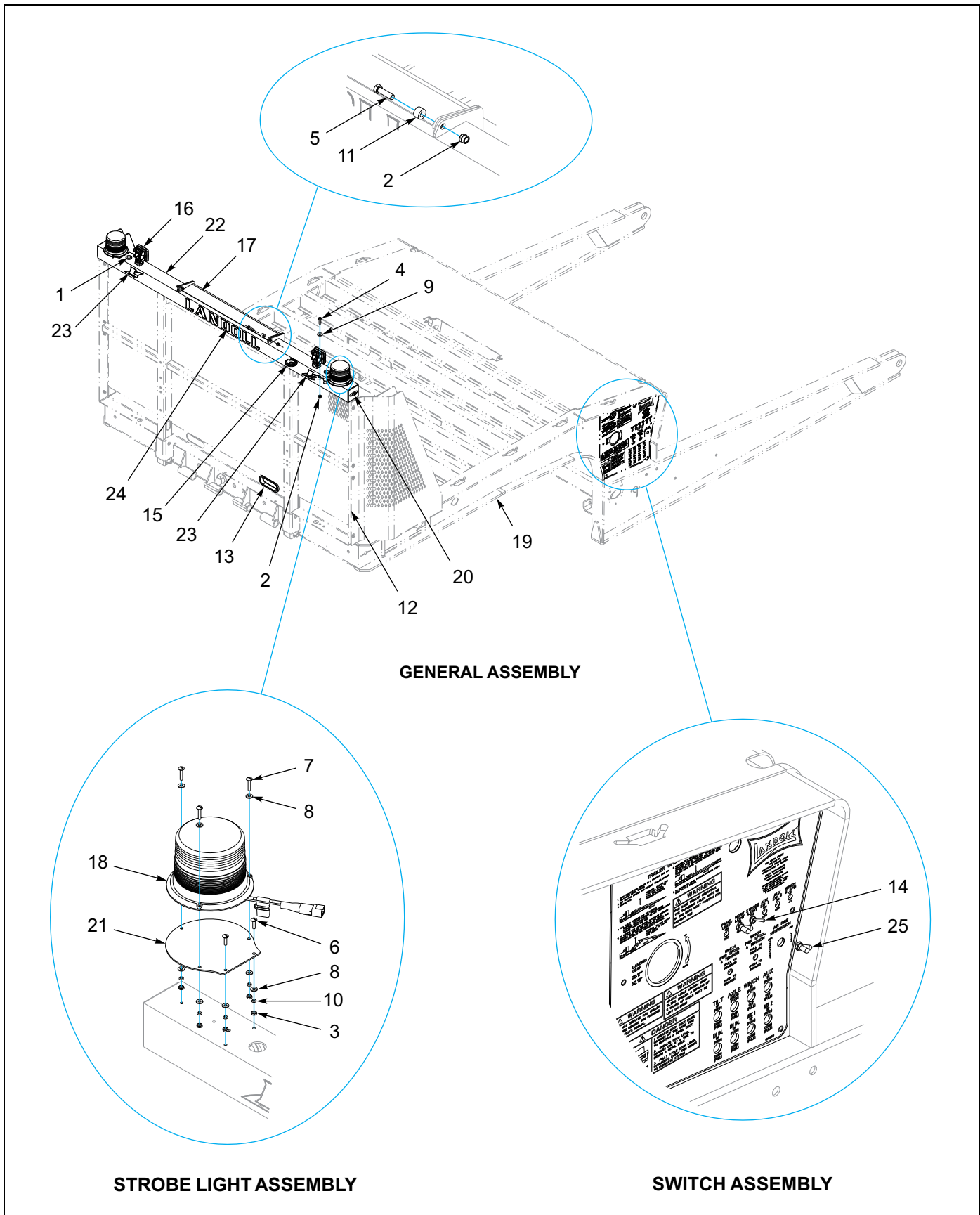
Figure 1-74: Bulkhead - Chain Rack Lights General Assembly
