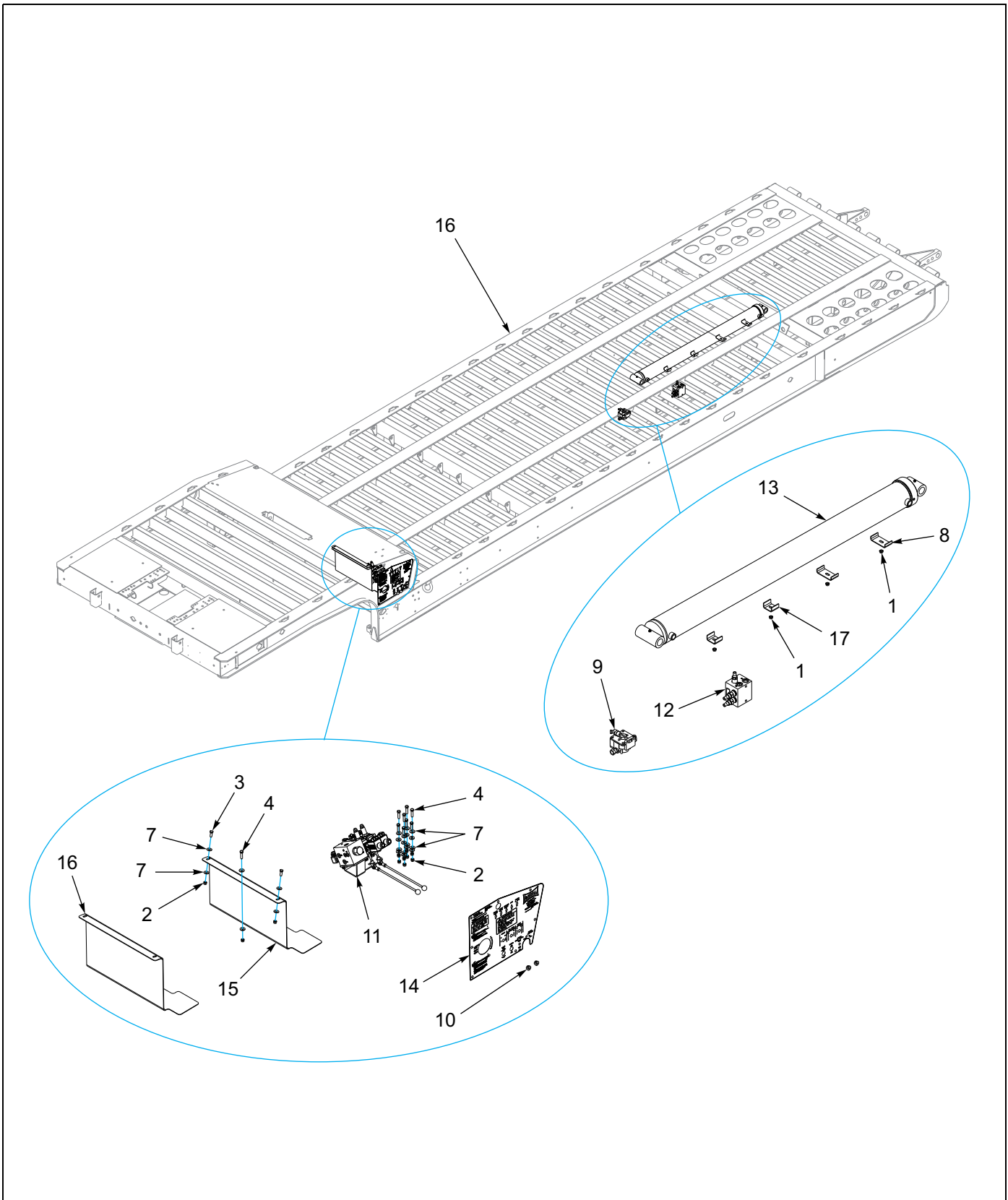
Figure 1-14: General Assembly
