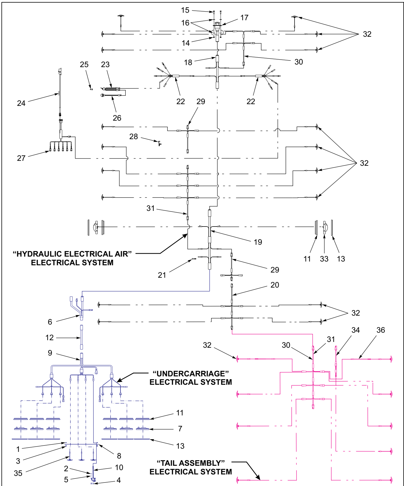
Figure 1-25: Electrical System
