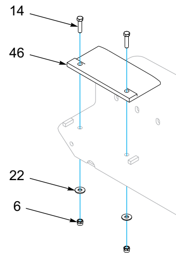
GLIDE ASSEMBLY
