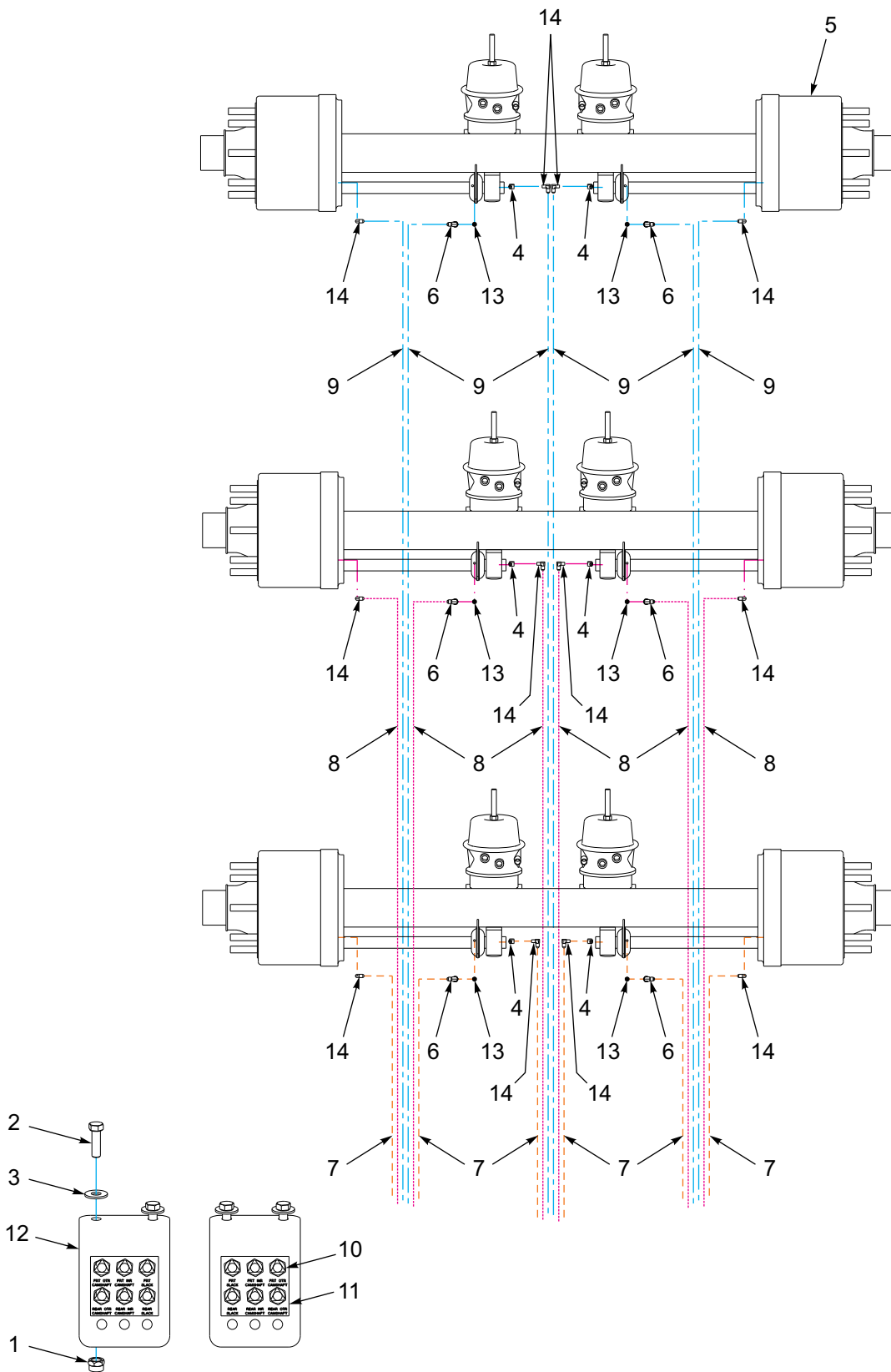
Figure 1-34: Grease System - 950D
