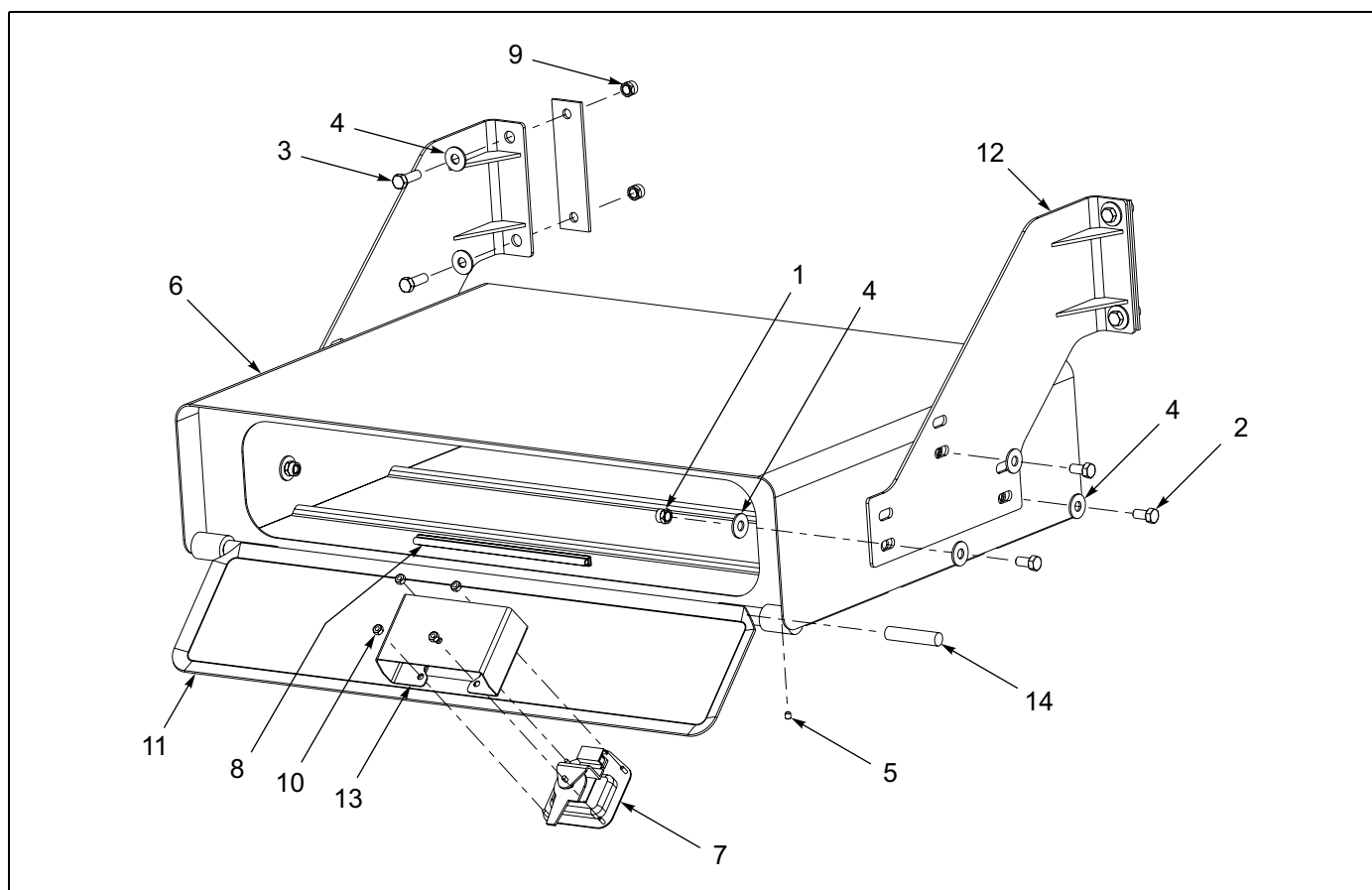
Figure 1-115: Toolbox Installation - Steel/Aluminum Door
