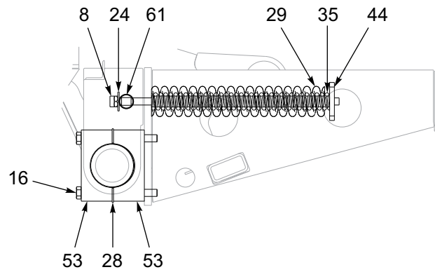
TAIL ASSEMBLY
