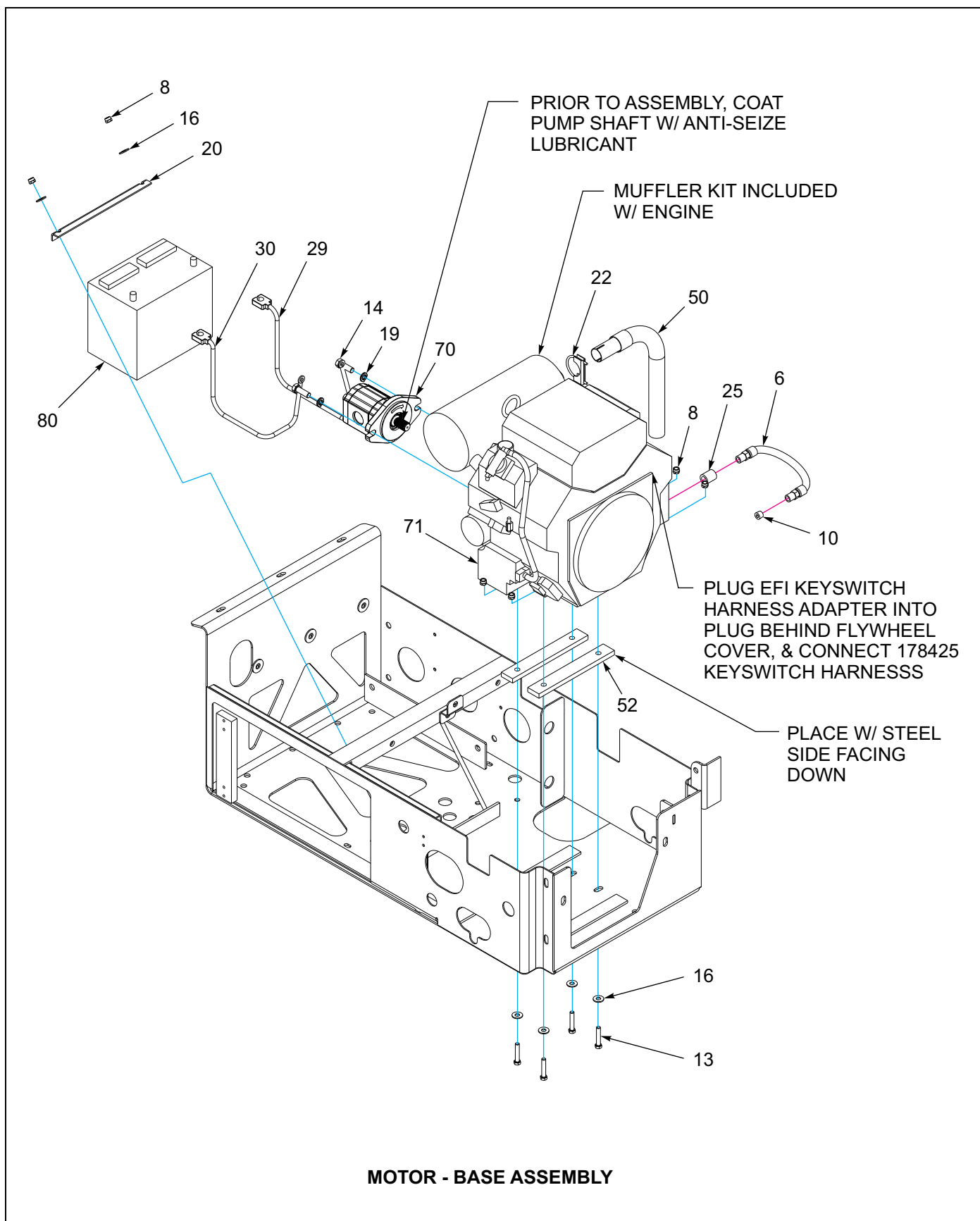
Figure 1-85: Engine - 25 HP Upper Deck Package (2 of 4)
