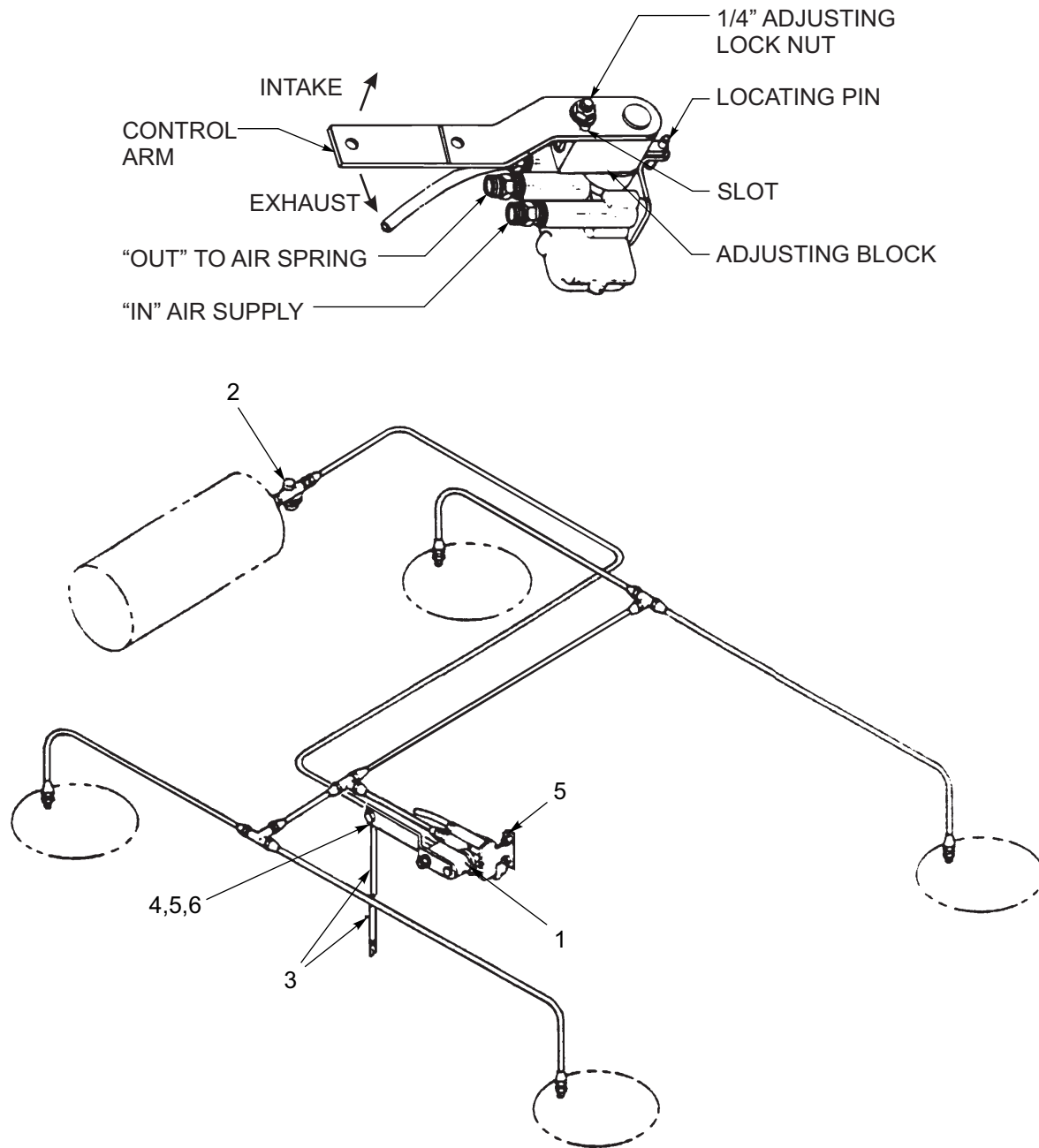
Figure 1-37: Air Control Kit - Neway
