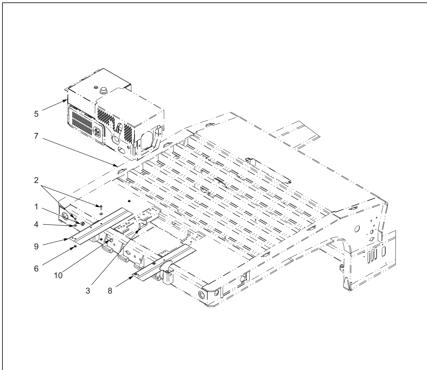
Figure 1-93: Engine - Front Mount Installation
