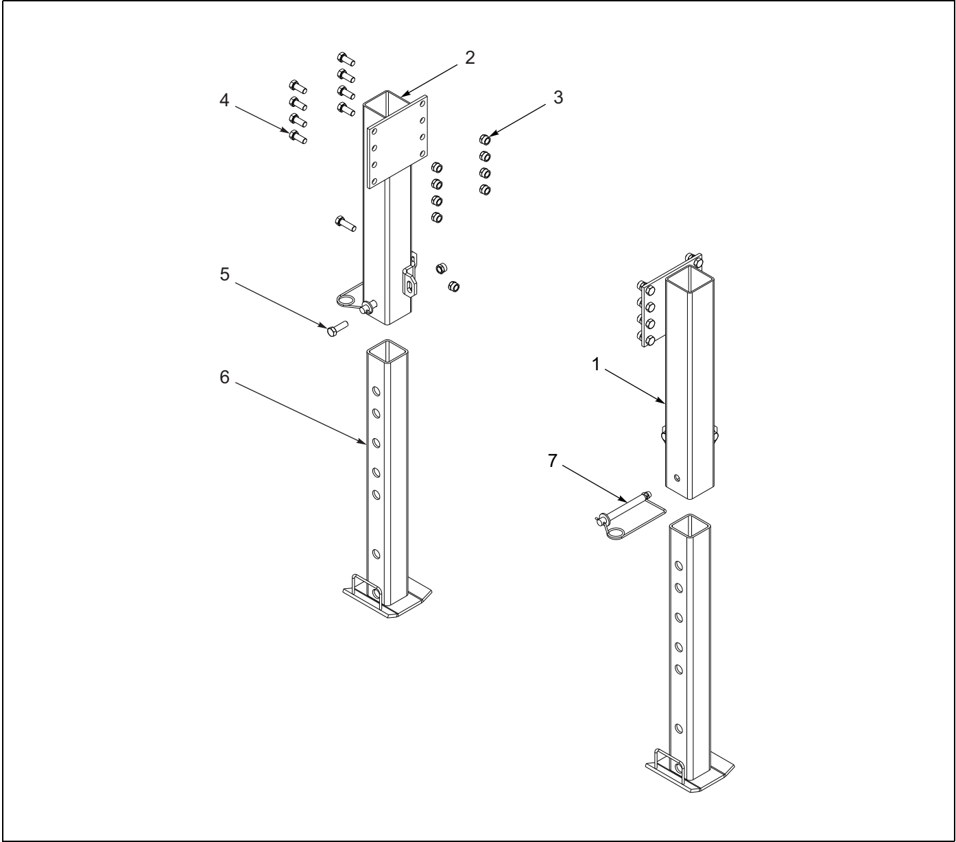
Figure 1-67: Landing Gear Installation - “Bolt On” Park Stand
