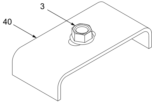
CLAMP ASSEMBLY
