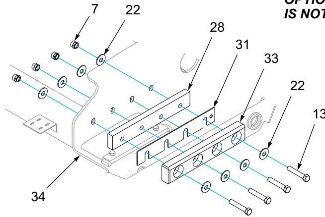
HOLD-DOWN ASSEMBLY
