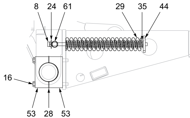
TAIL ASSEMBLY
