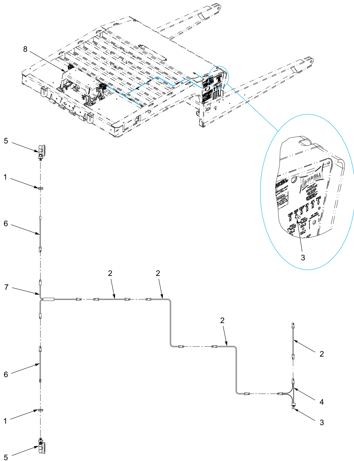
Figure 1-125: Winch - Work Light Installation
