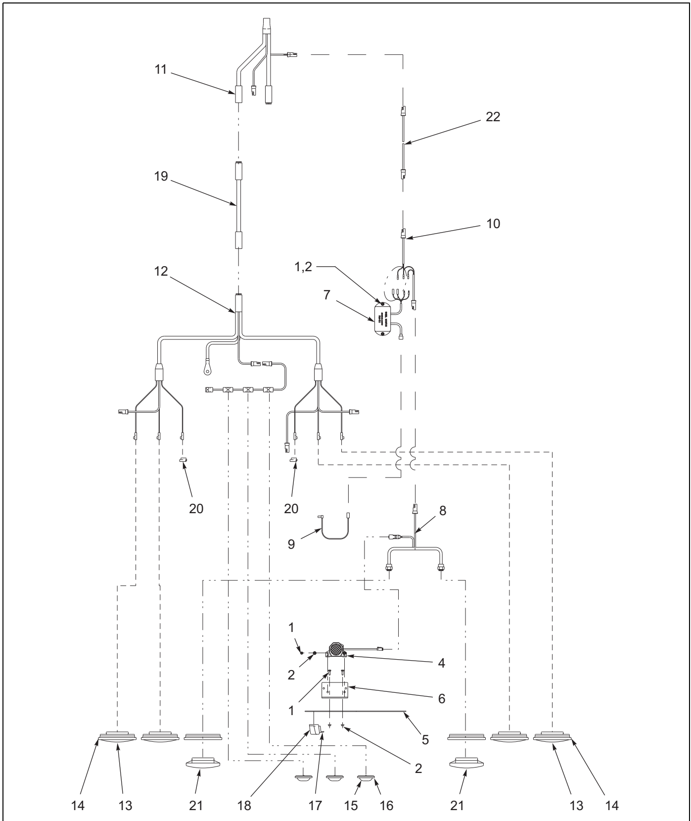
Figure 1-99: Backup Alarm/Light Installation
