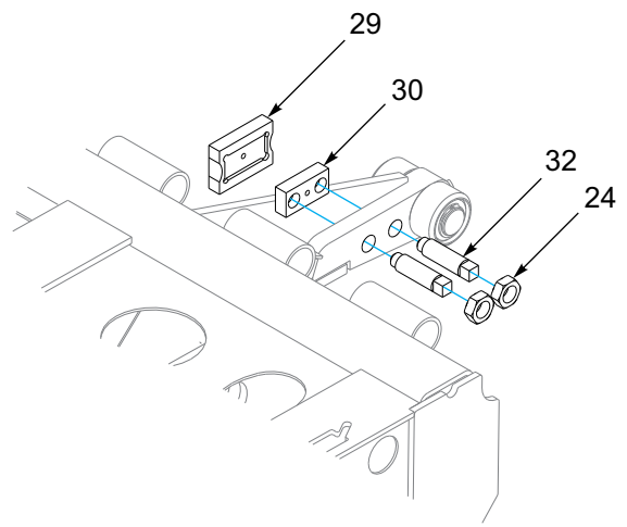
CENTERING BLOCK ASSEMBLY
