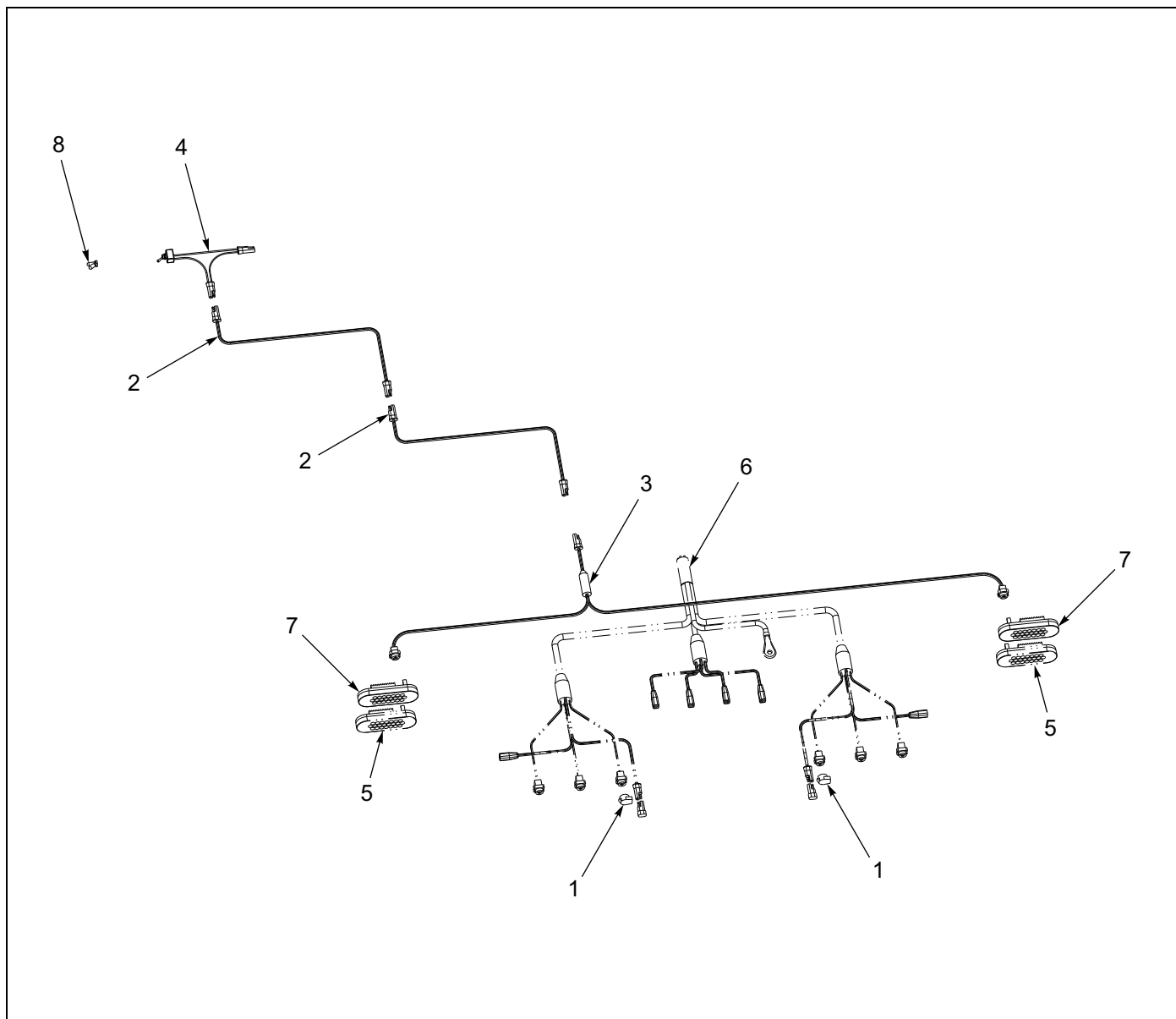
Figure 1-79: Bumper - Strobe Installation
