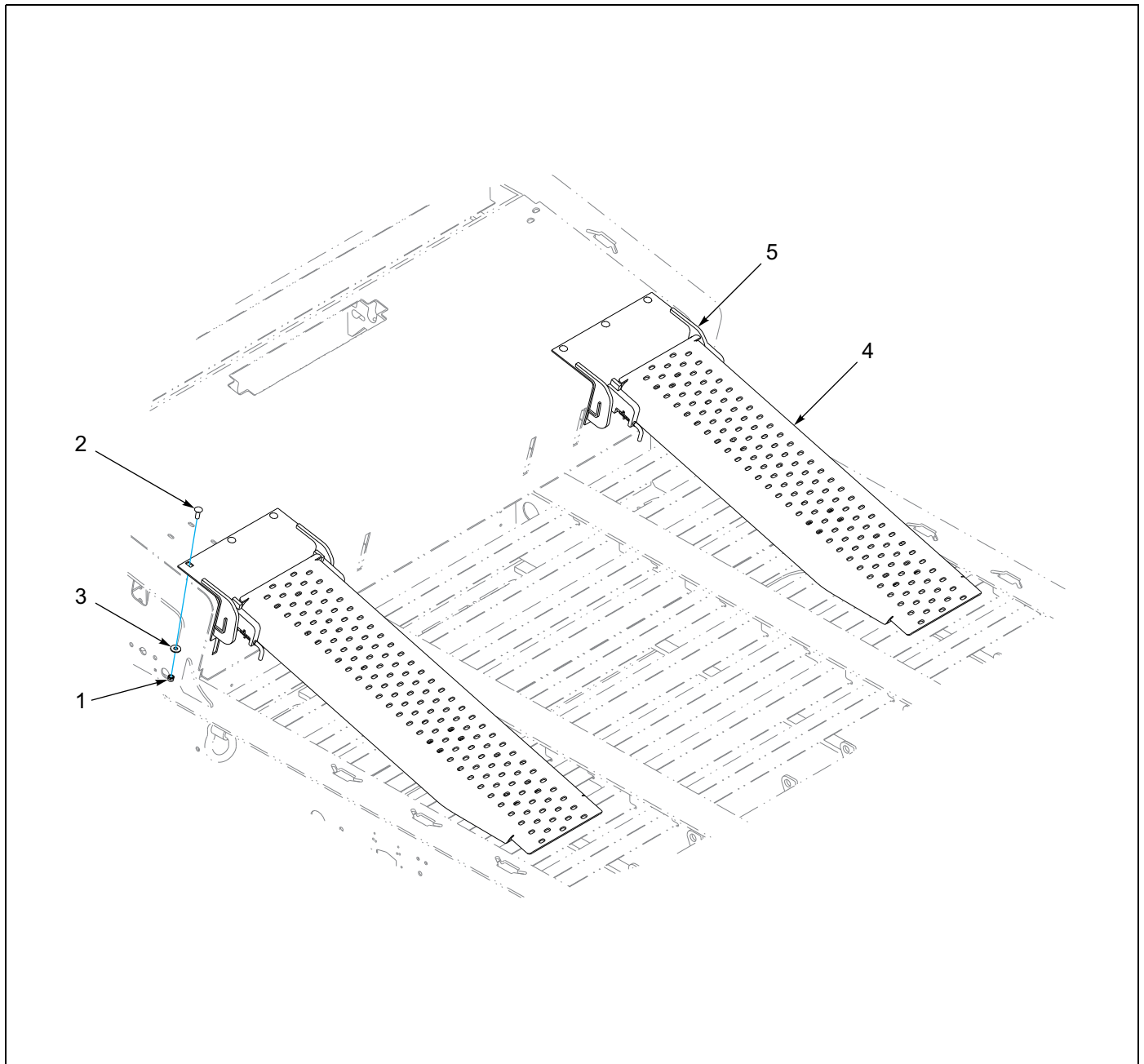
Figure 1-105: Ramp Assembly - Front Slope
