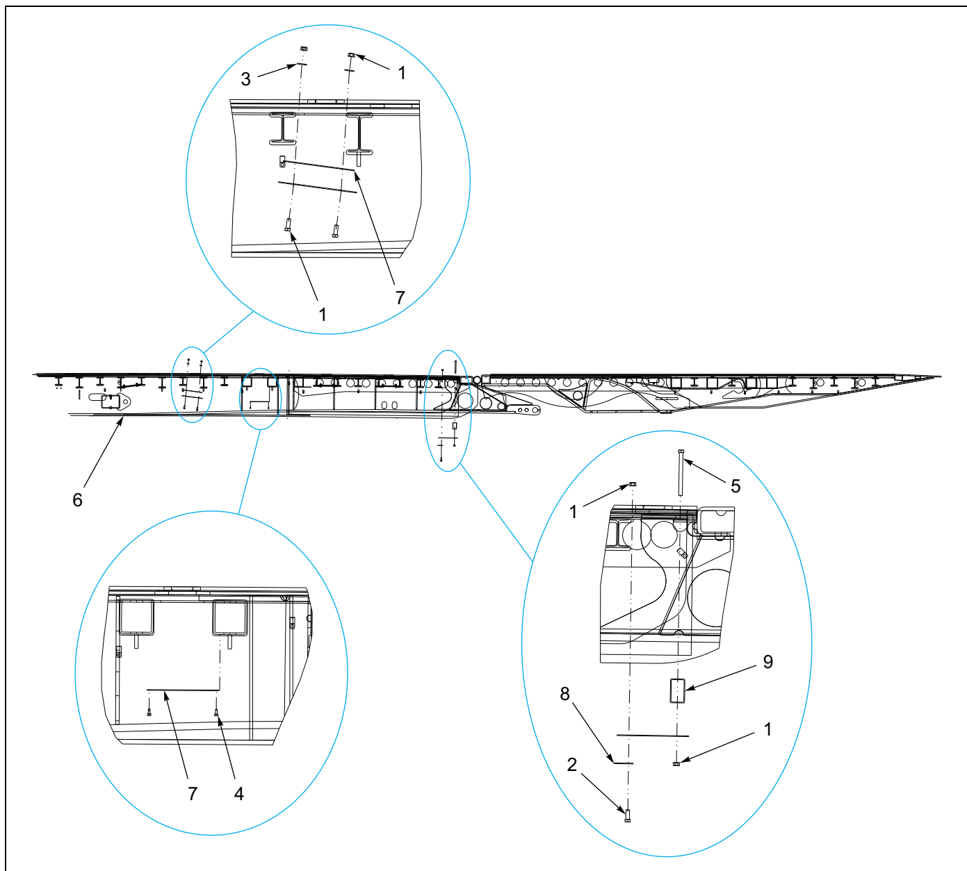
Figure 1-131: Shield Installation - Center Gotcha
