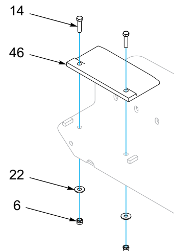
GLIDE ASSEMBLY
