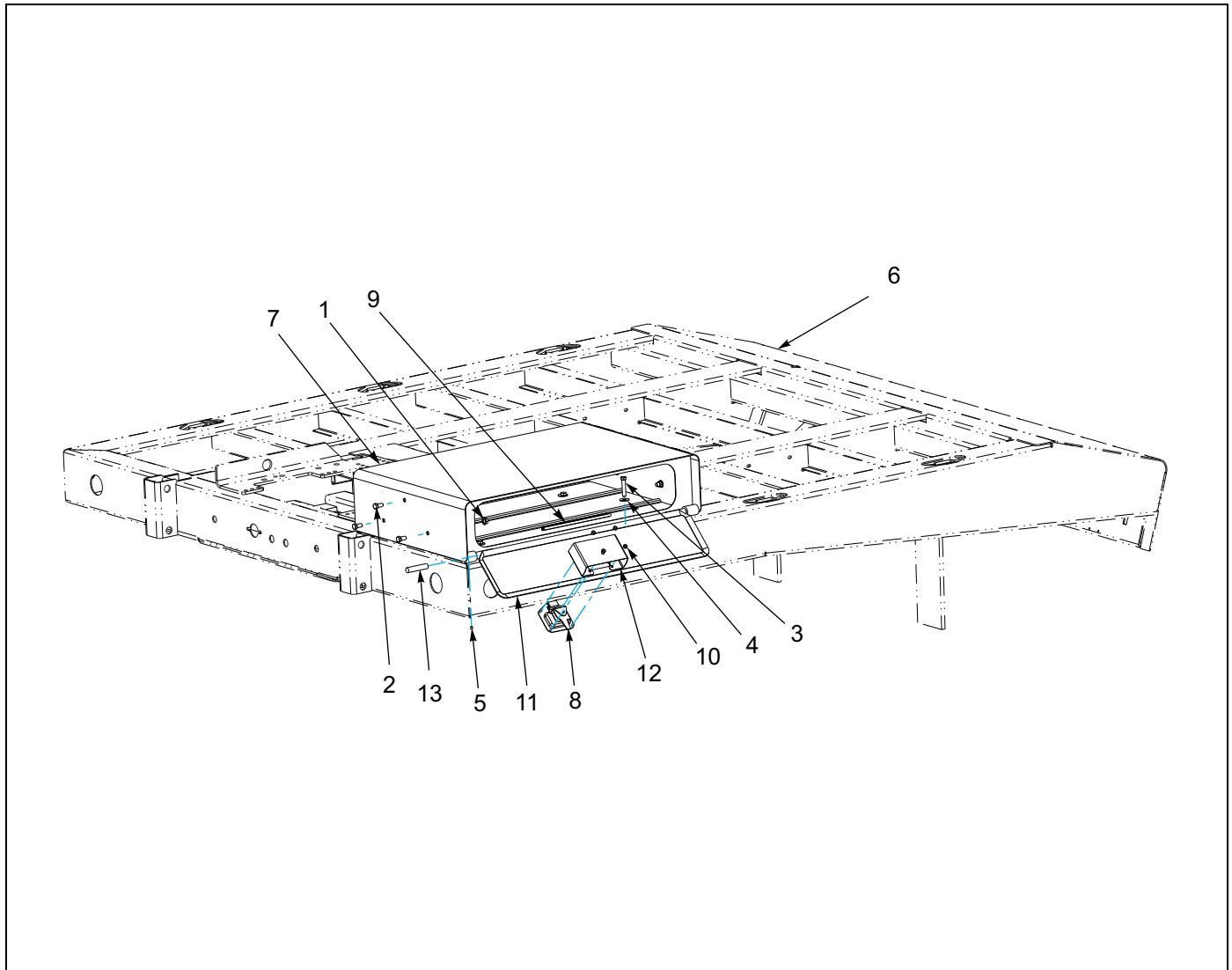
Figure 1-116: Toolbox Installation - Upper Deck
