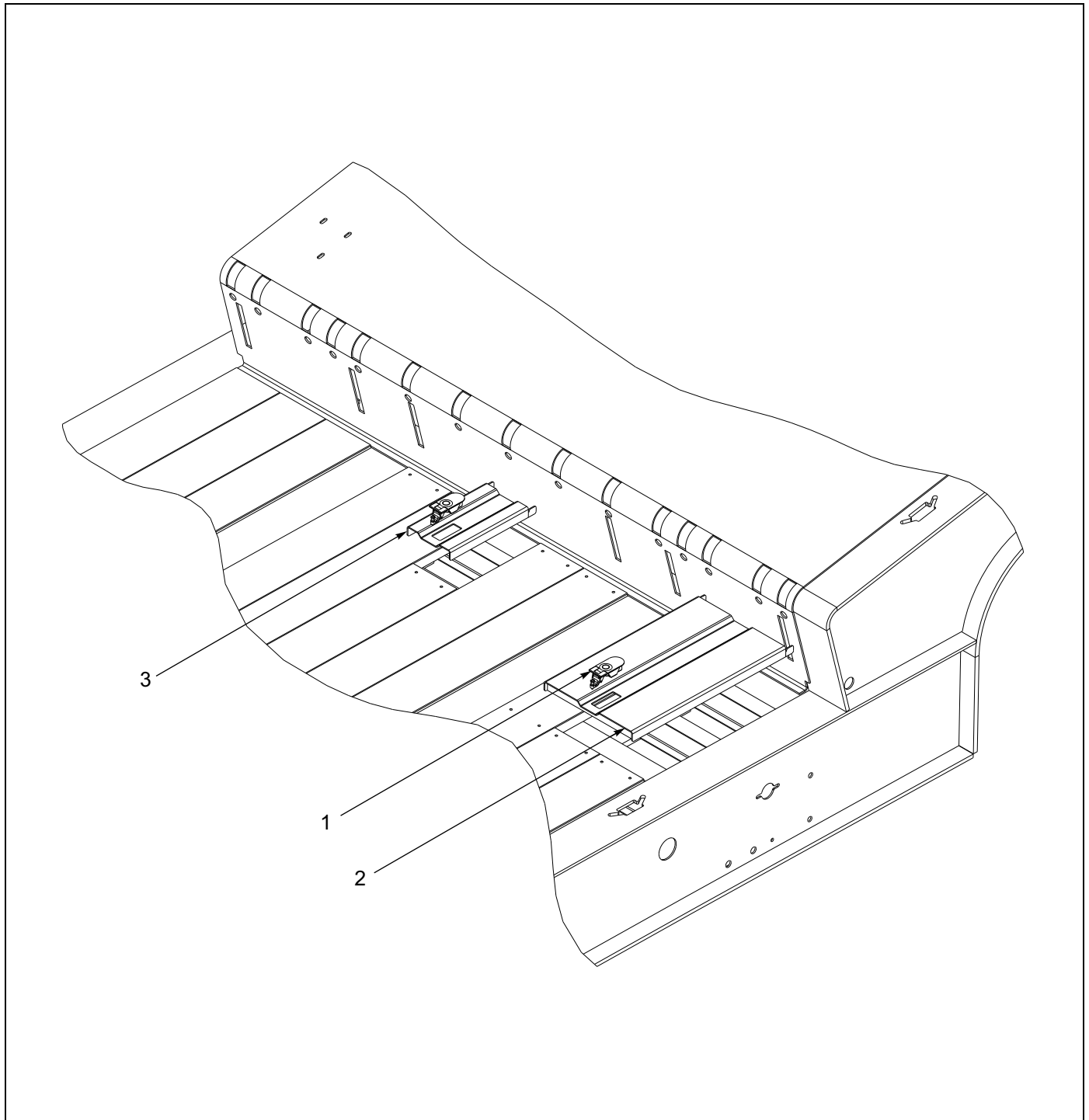
Figure 1-95: Engine - Slope Cover Installation (Used On Trailers W/O Ramp)
