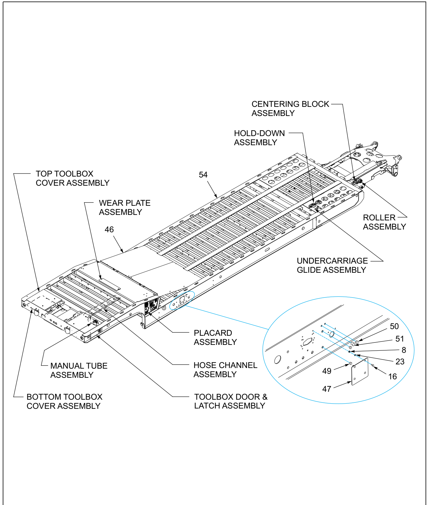
Figure 1-6: Frame Assembly (1 of 3)
