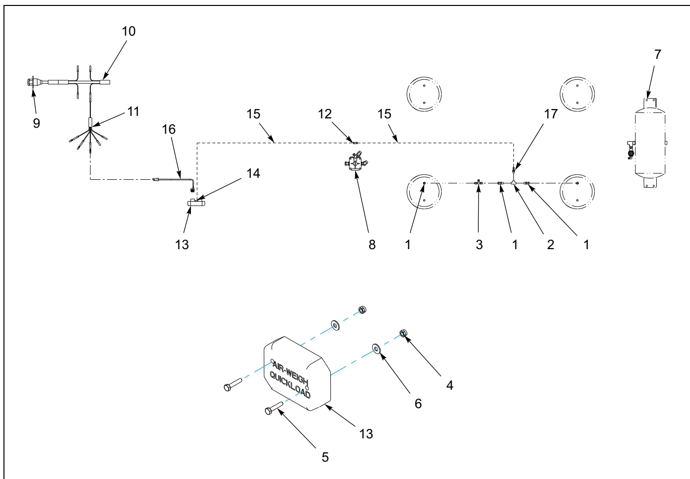
Figure 1-71: Air Digital Scale - Quickload System
