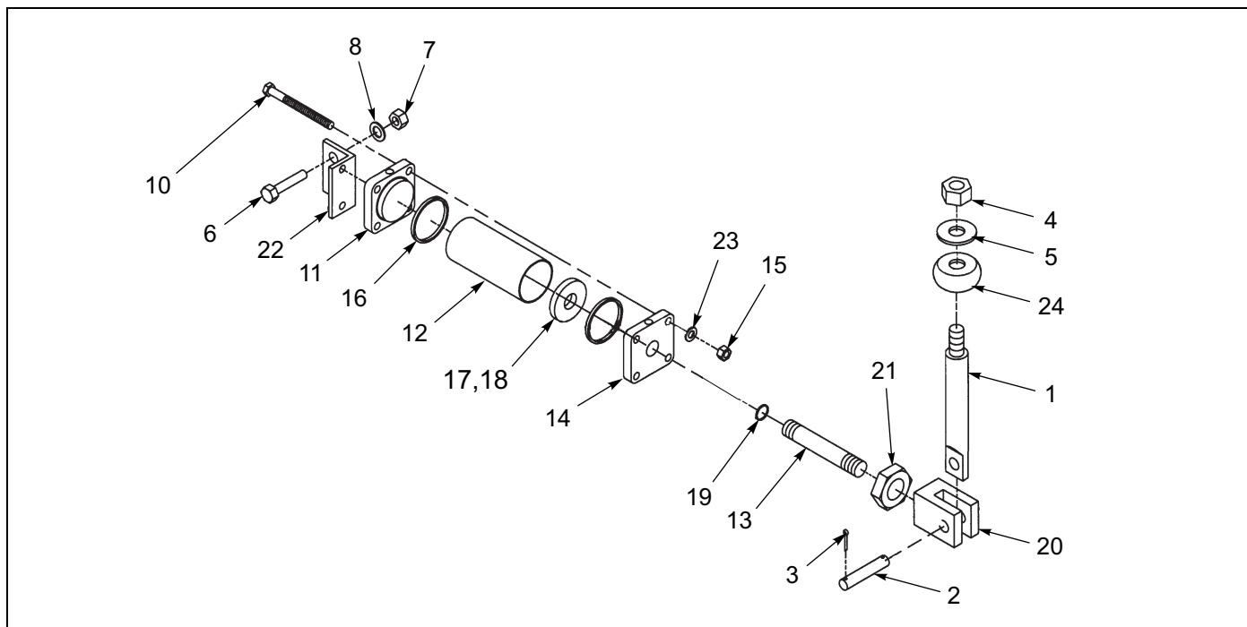
Figure 1-59: Winch - Air Shift Cylinder
