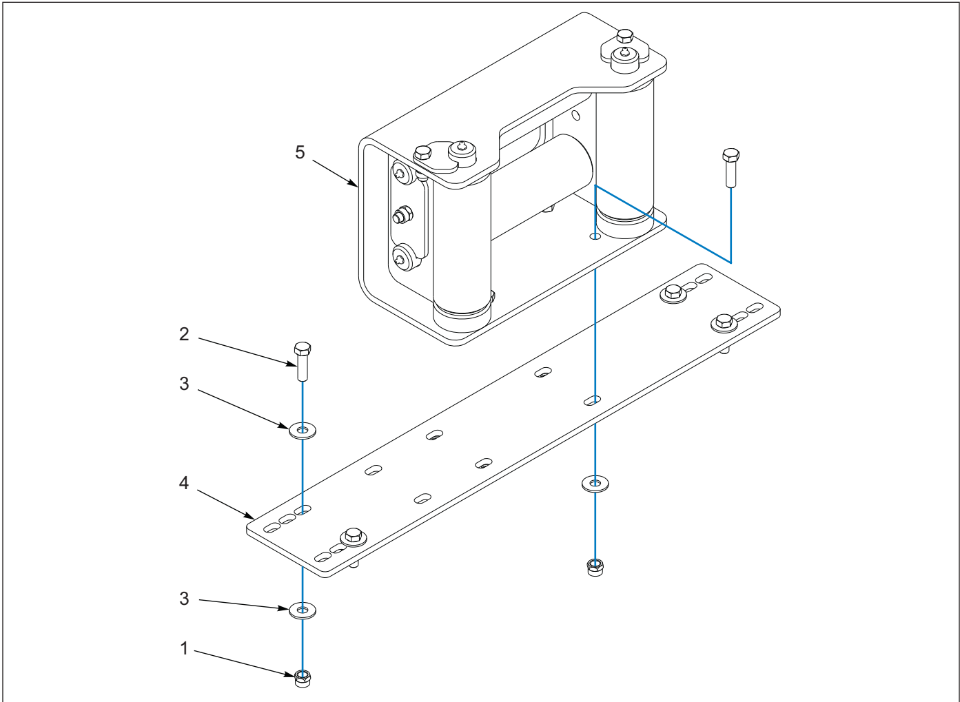
Figure 1-103: 4 Roller Guide Installation - 12K (BRADEN)
