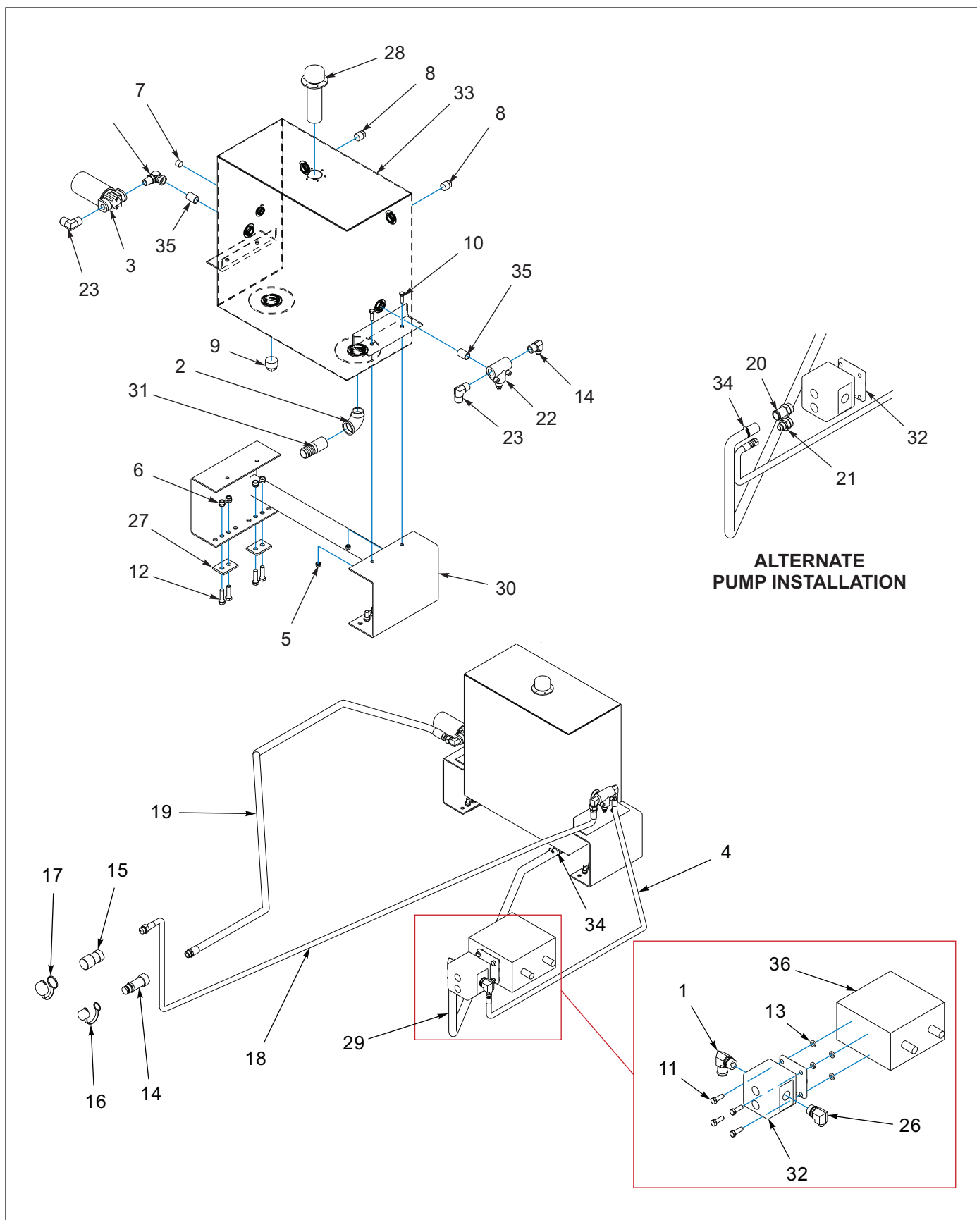
Figure 1-95: Hydraulic Wet Kit Items - 30 Gallon
