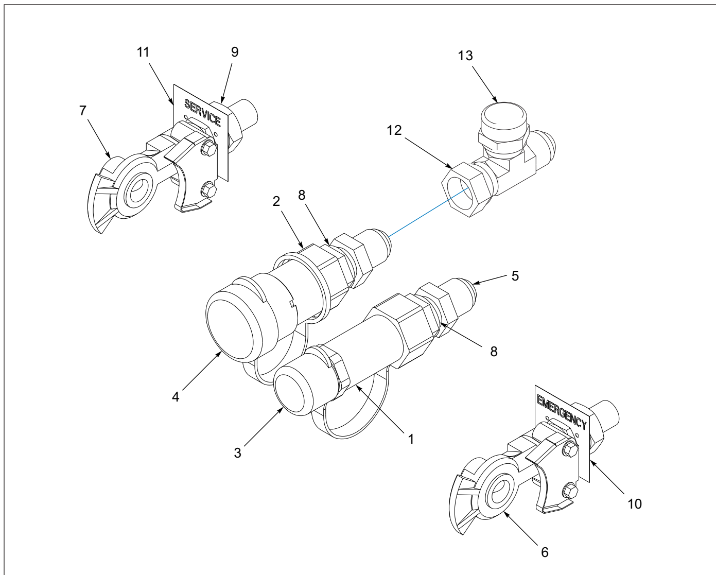
Figure 1-21: Connectors - Front Sub Assembly
