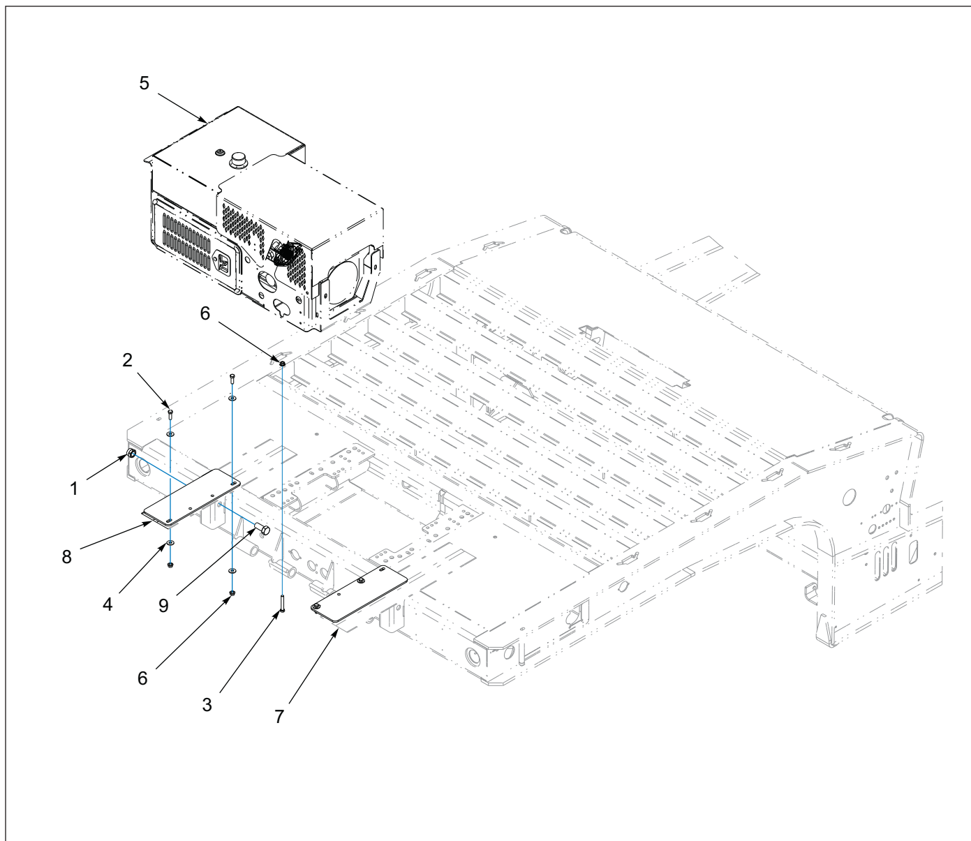
Figure 1-90: Front Mount Installation
