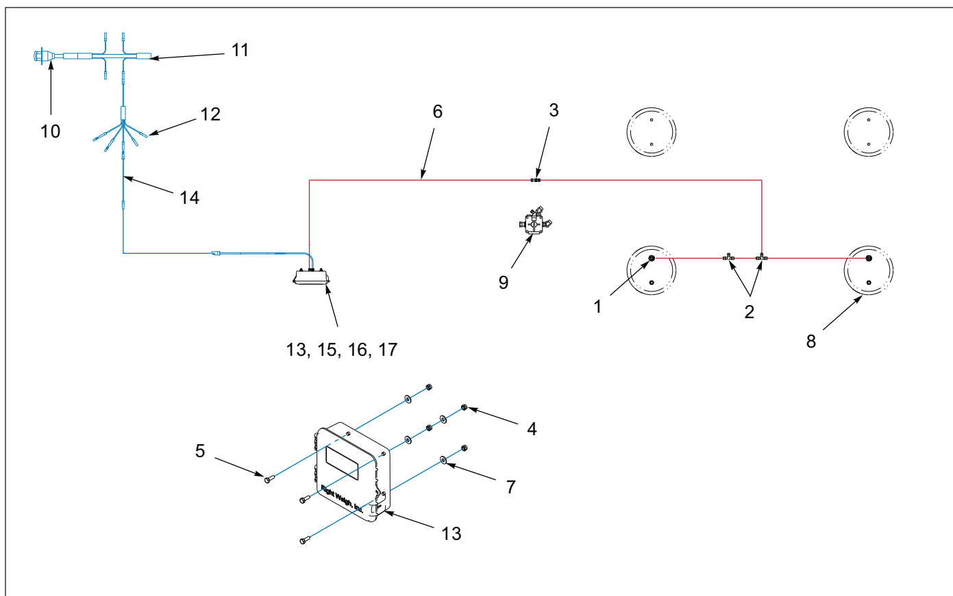
Figure 1-69: Right Weigh System
