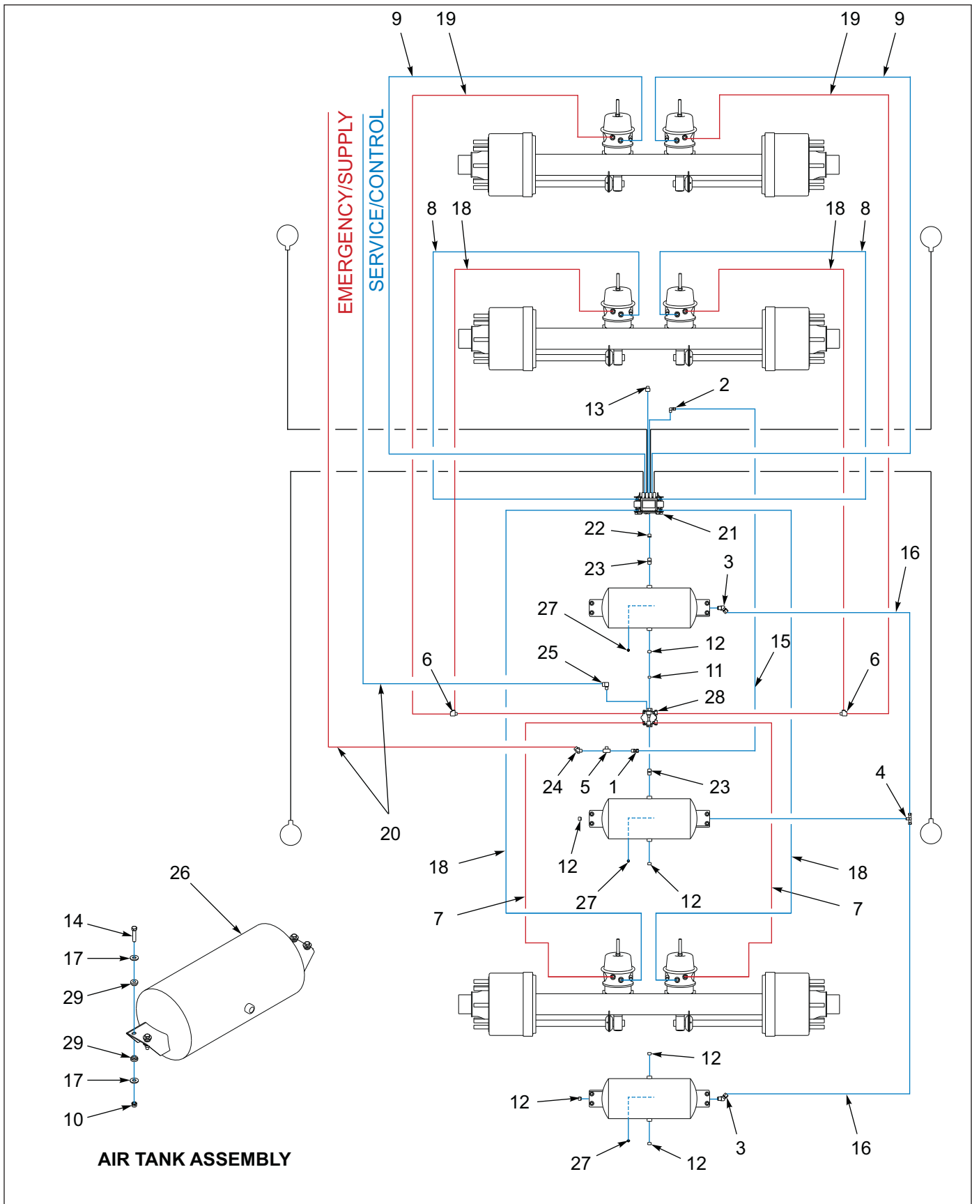
Figure 1-45: Air Brake System - 950E
