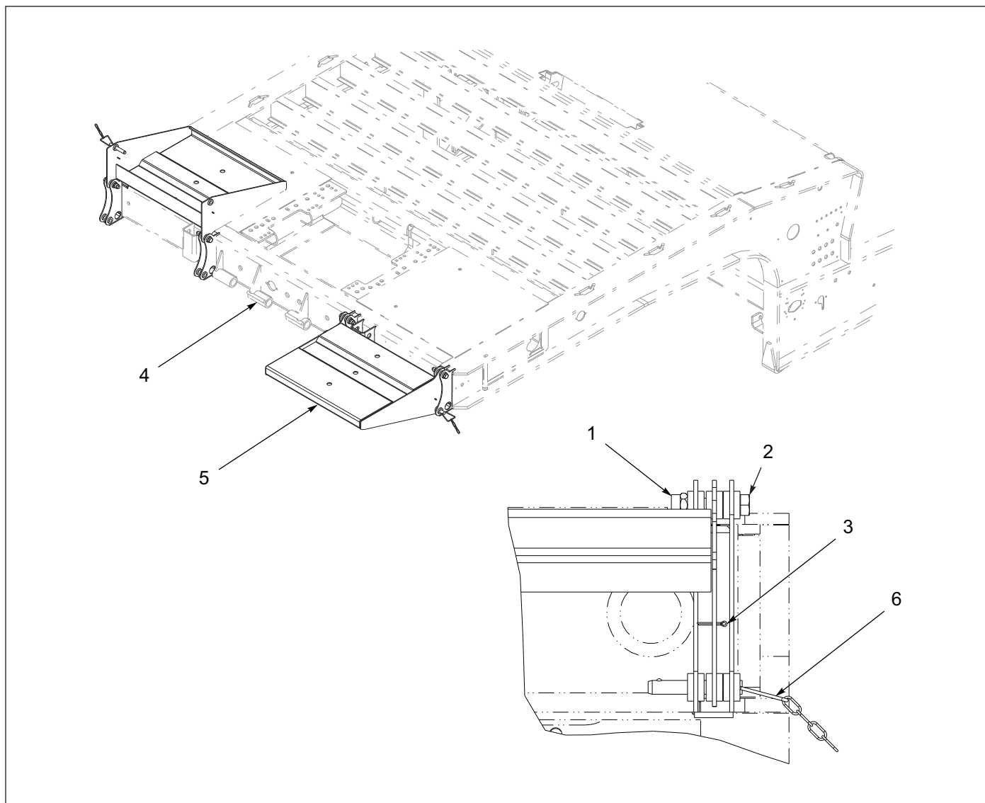
Figure 1-121: Front Flip Option
