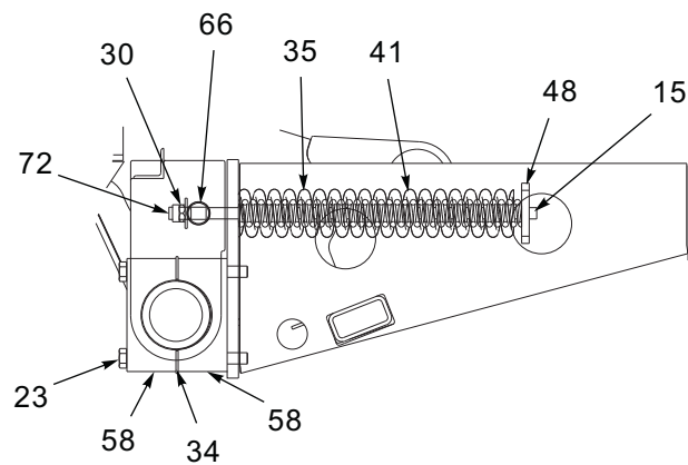
TAIL ASSEMBLY
