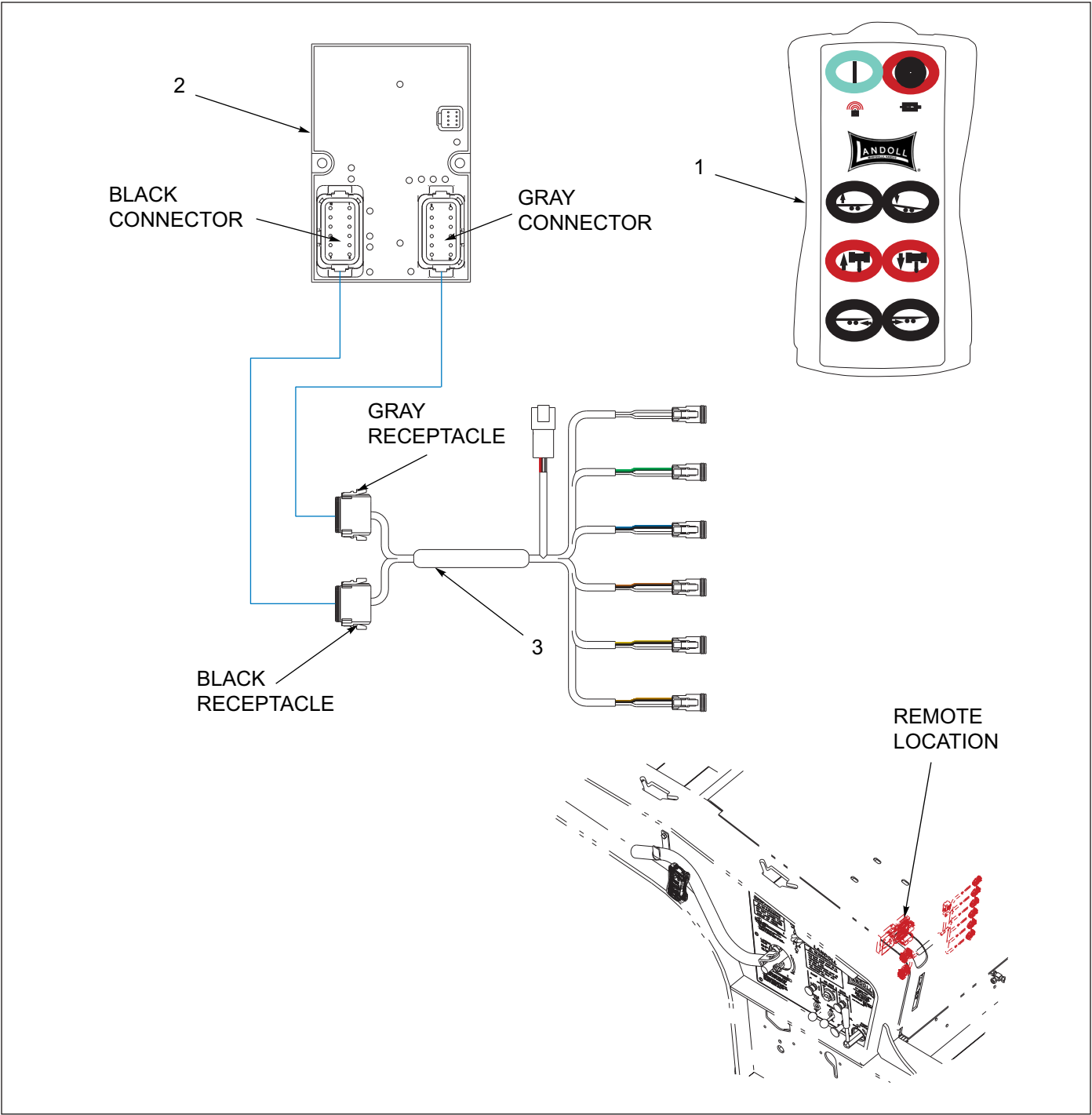
Figure 1-27: Remote - Brand 6-Function
