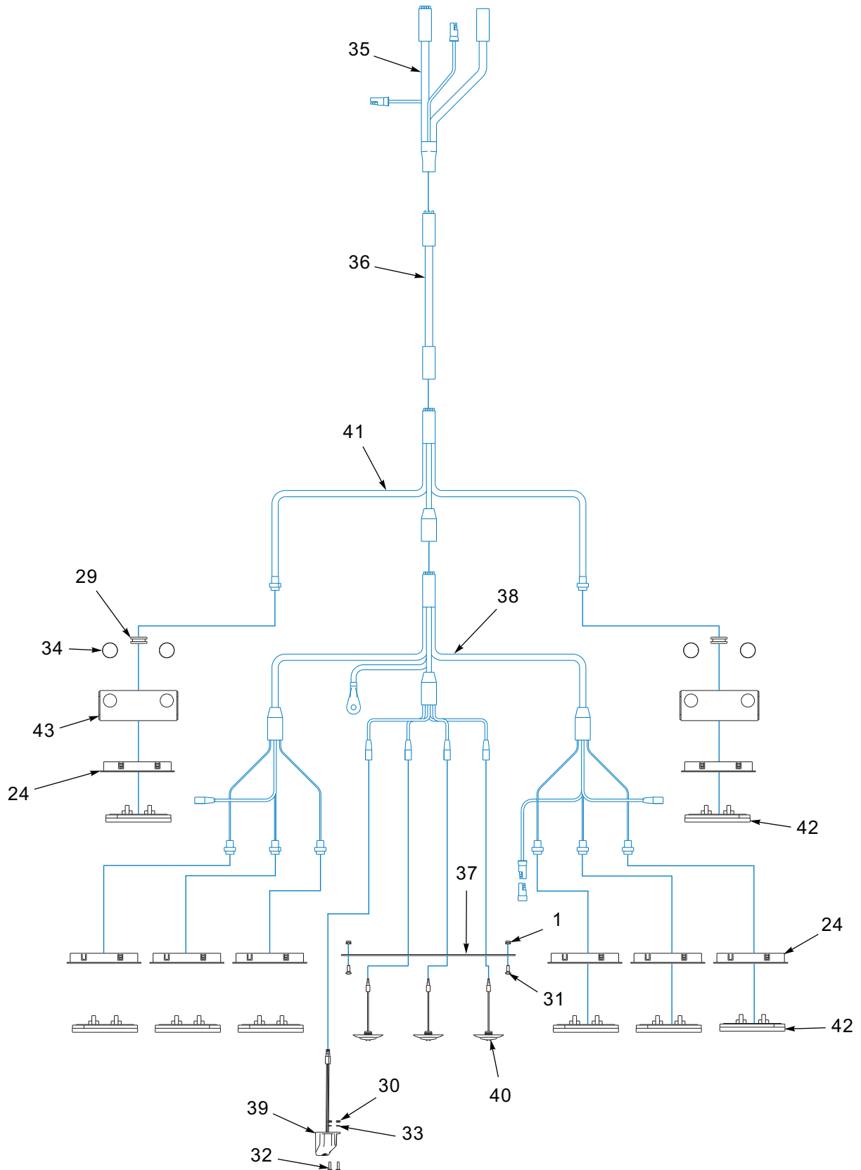
Figure 1-26: Electrical System (2 of 2)
