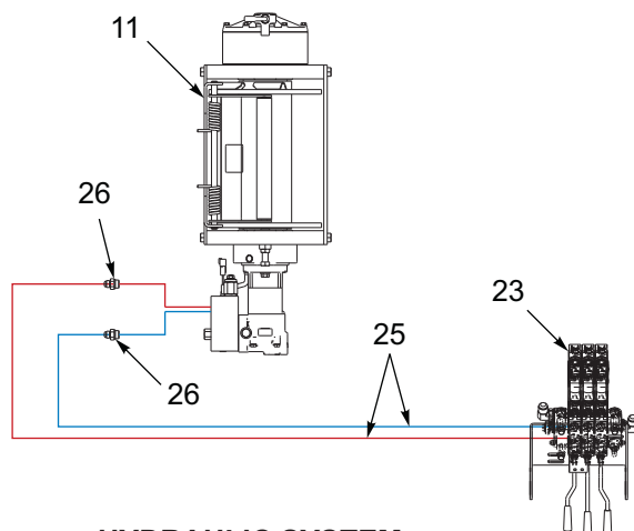
HYDRAULIC SYSTEM
