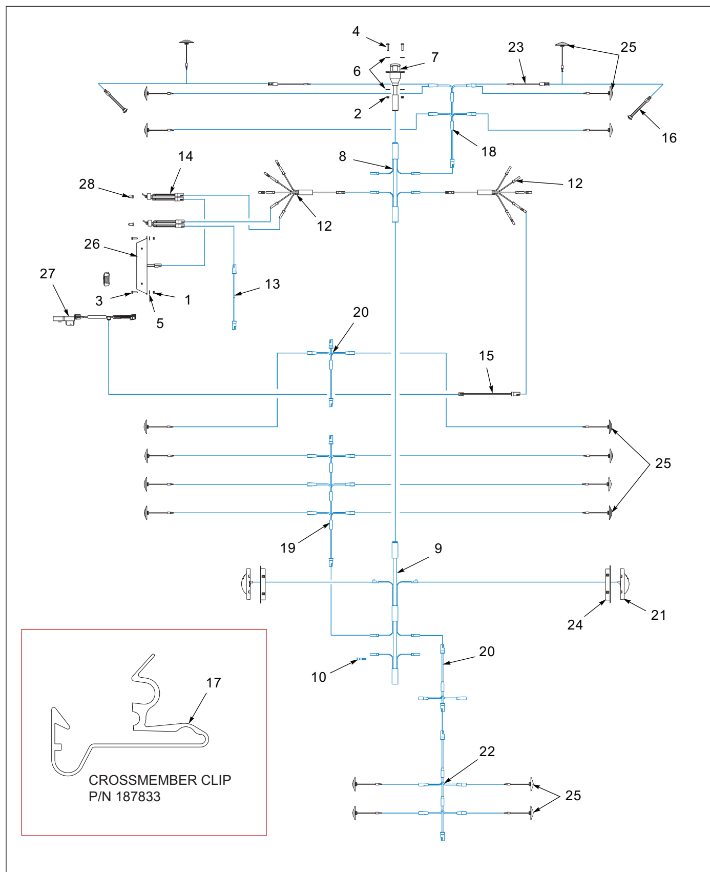
Figure 1-25: Electrical System (1 of 2)
