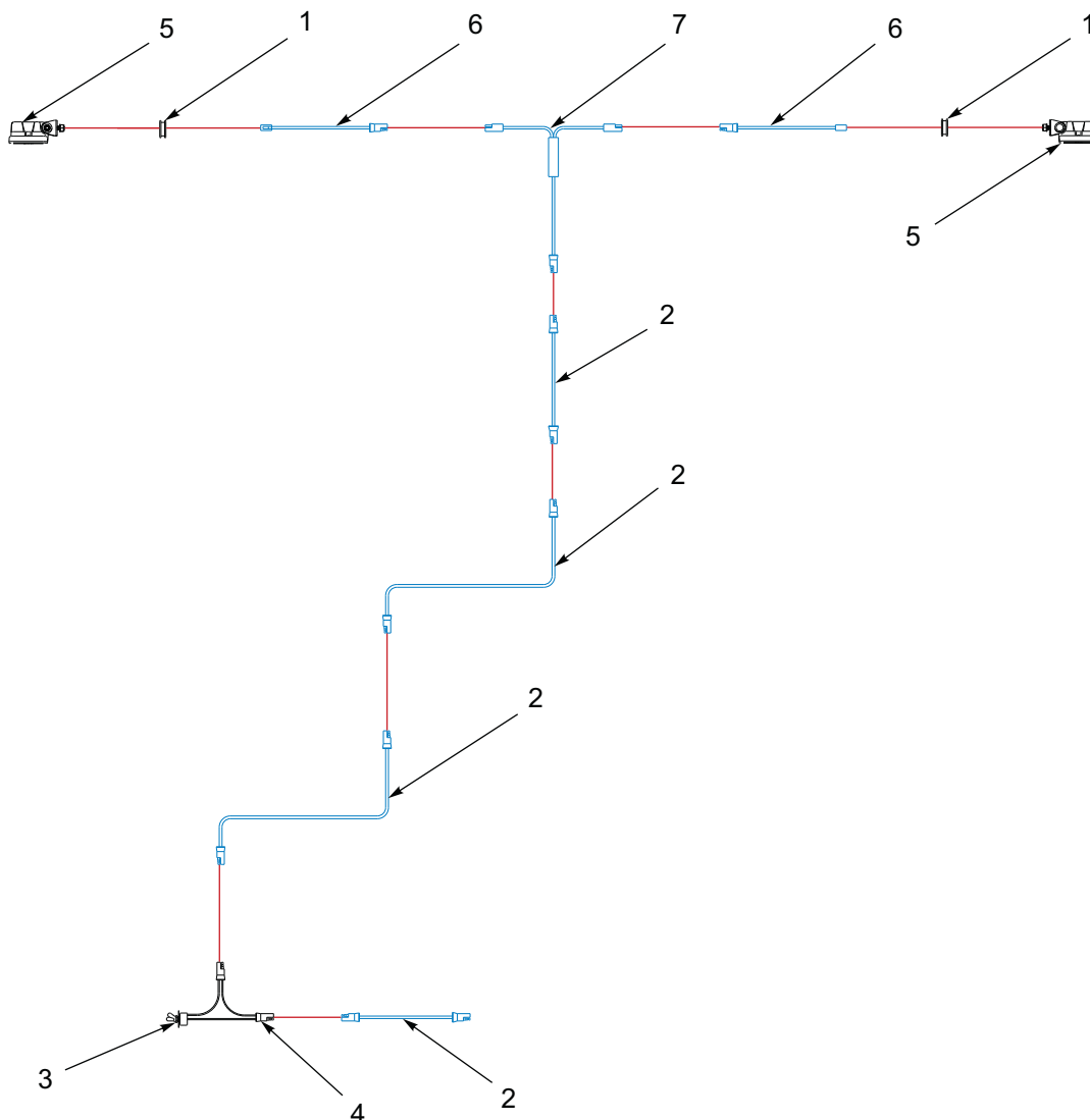
Figure 1-120: Work Light Installation
