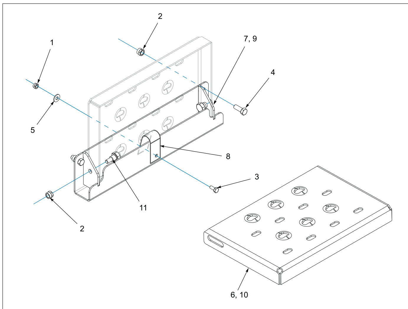
Figure 1-108: Folding Step Assembly - Double Drop Frame
