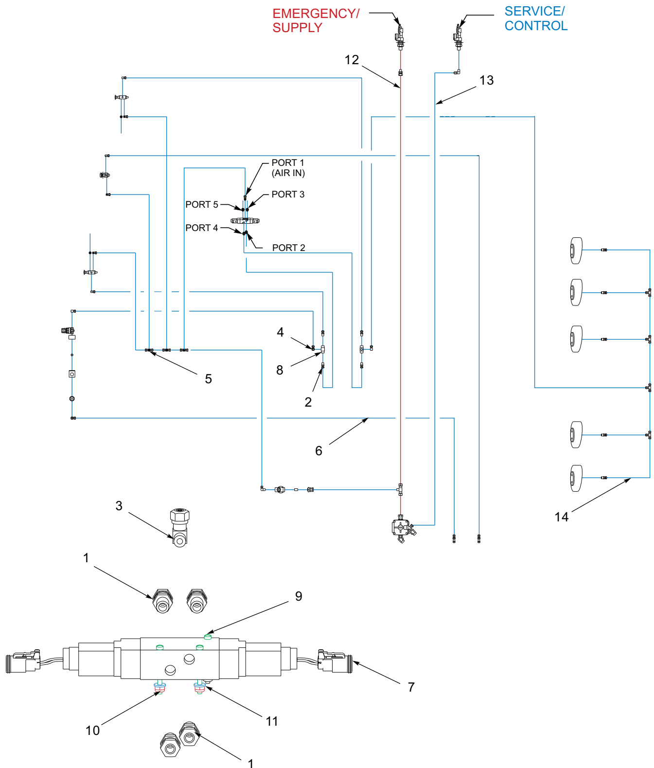
Figure 1-19: Ramp and Dock Lift Air Items
