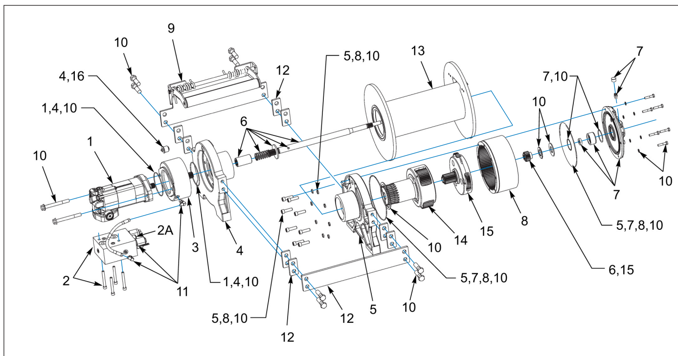
Figure 1-64: Winch Items - 30K 2 Speed (WARN)
