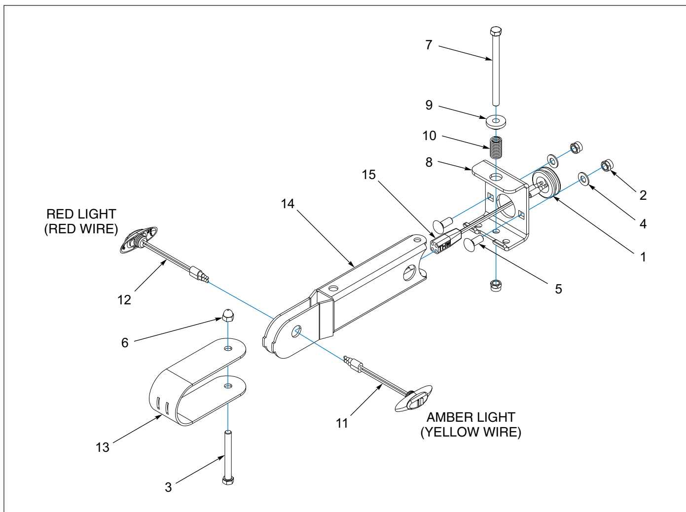
Figure 1-100: Swing-Arm Light Assembly - CURB
