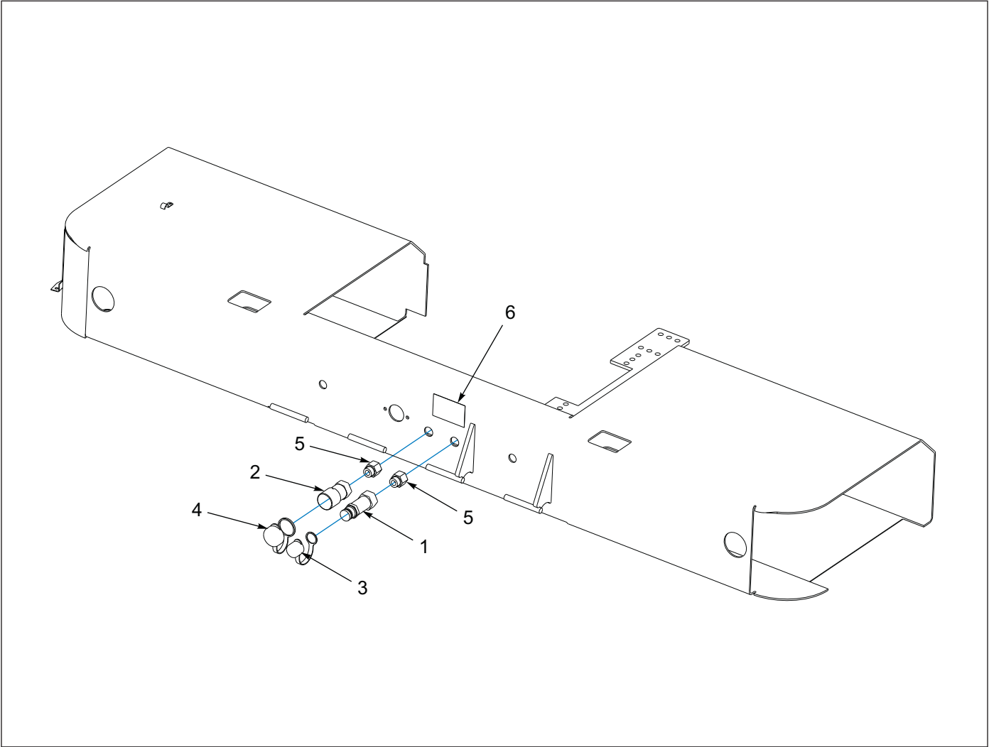
Figure 1-94: Hydraulic Conversion Kit - Ball to Flat
