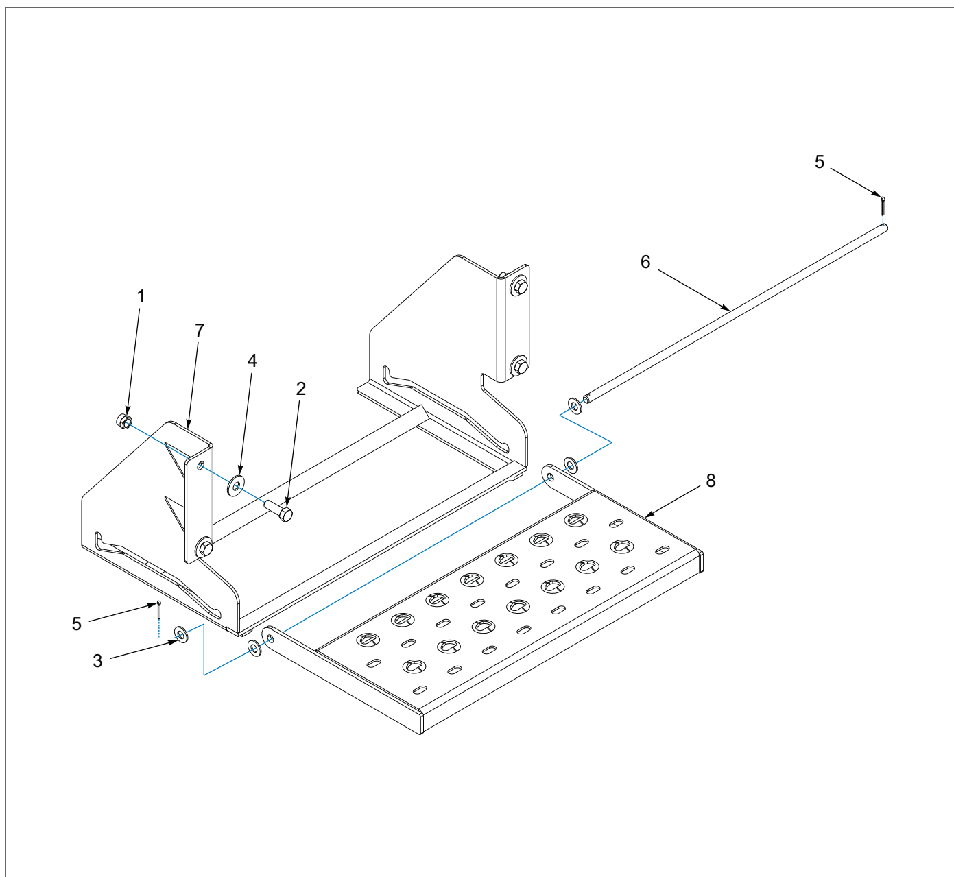
Figure 1-109: Retractable Step Assembly
