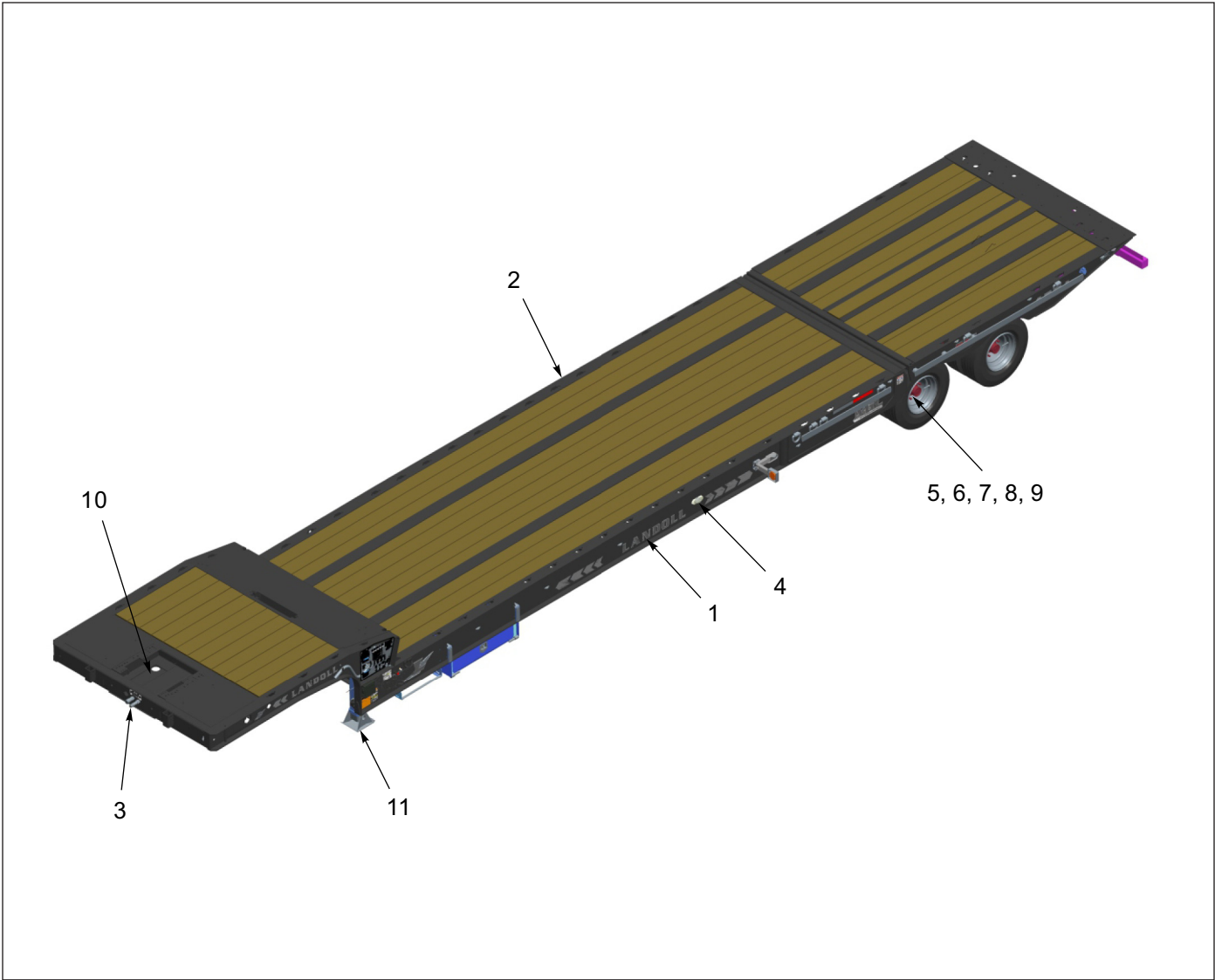
Figure 1-2: General Assembly
