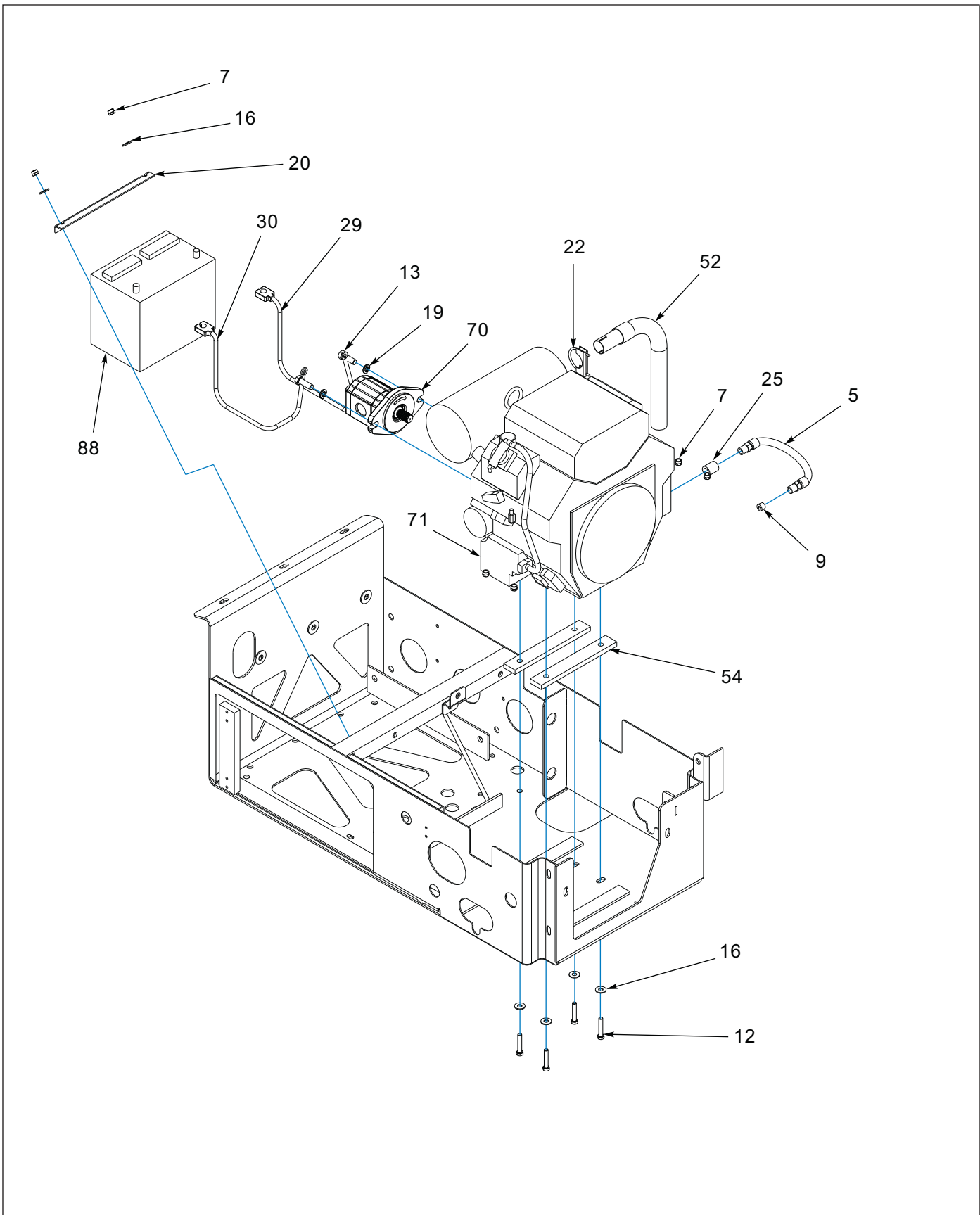
Figure 1-82: 25 HP Upper Deck Package (2 of 4)
