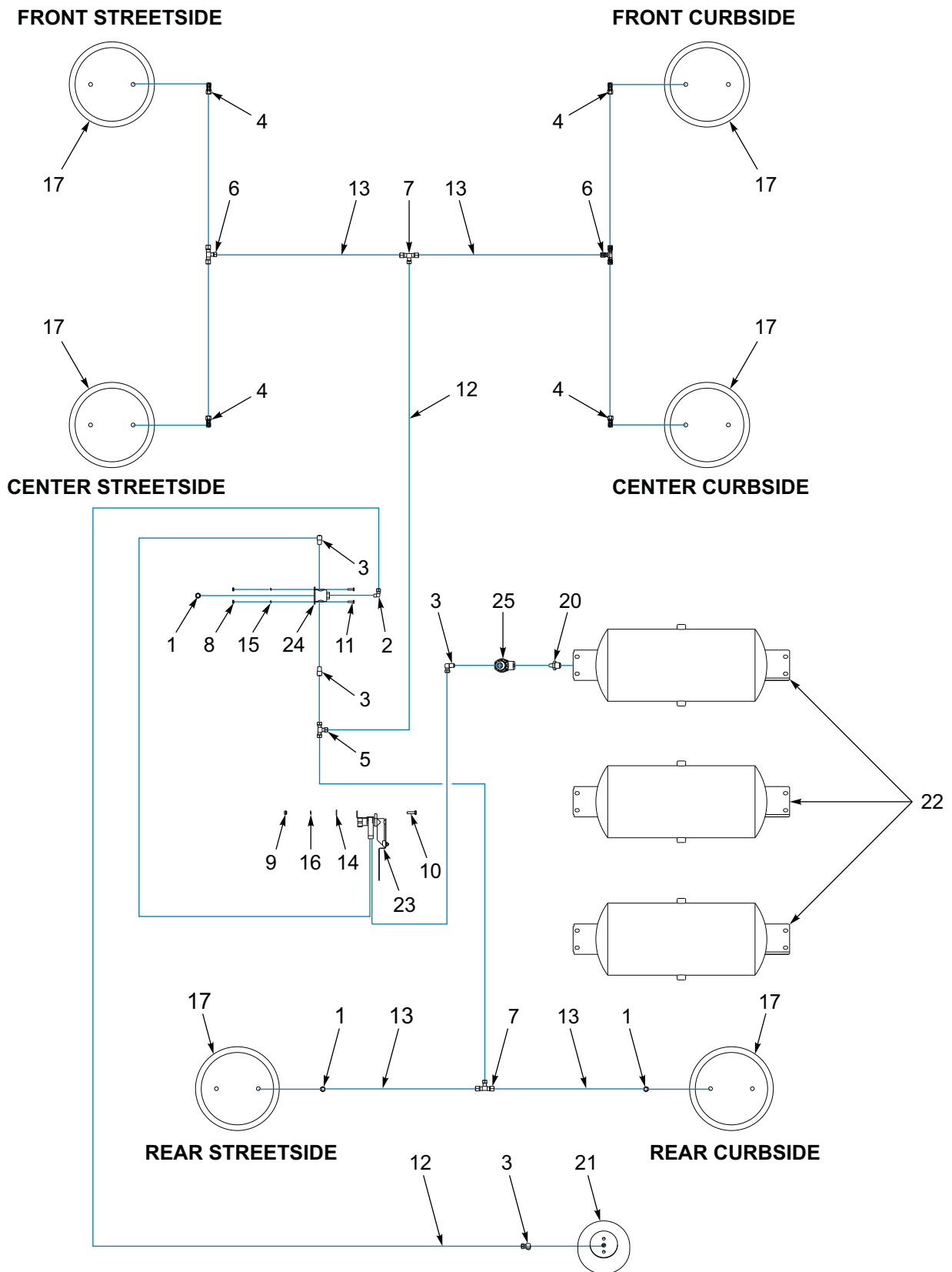
Figure 1-37: Air Ride Suspension - 950E
