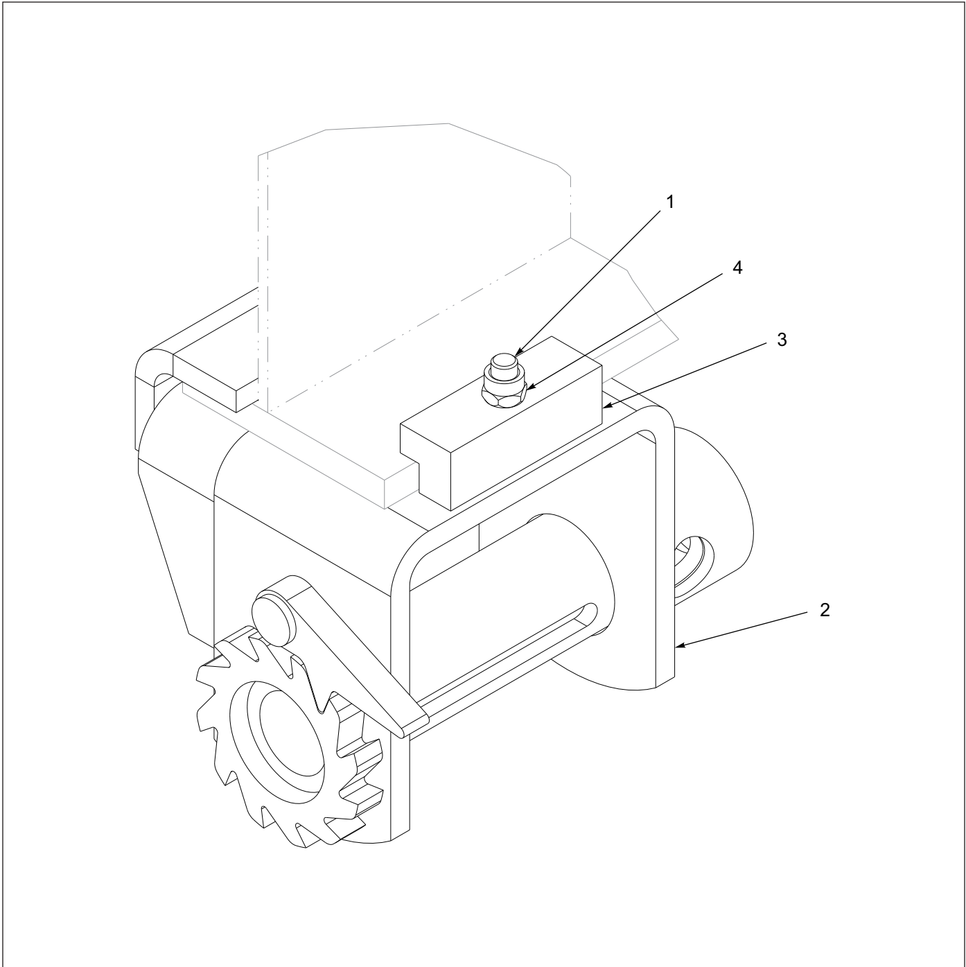
Figure 1-119: 4" Webbing Sliding Assembly
