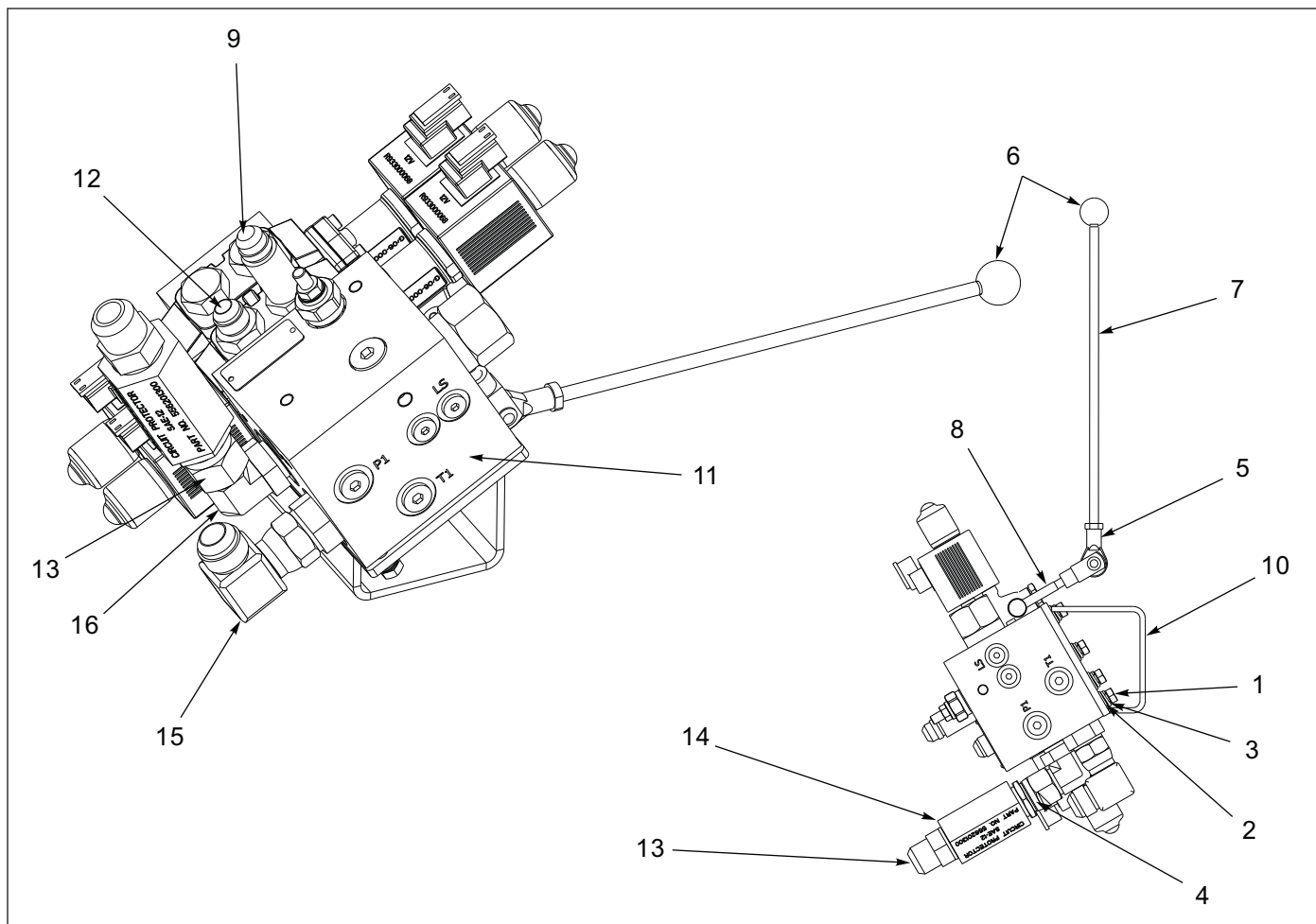
Figure 1-23: Valve Assembly - 2 Spool Control
