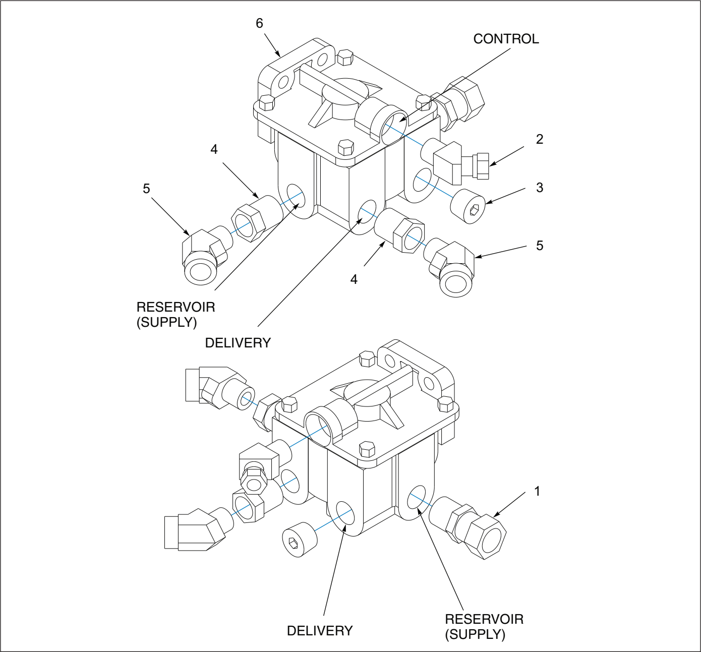
Figure 1-22: Valve Assembly - Air Booster
