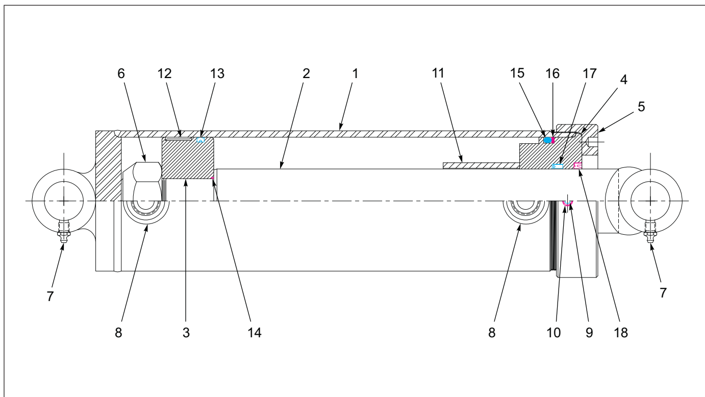
Figure 1-20: Cylinder - 5 X 60
