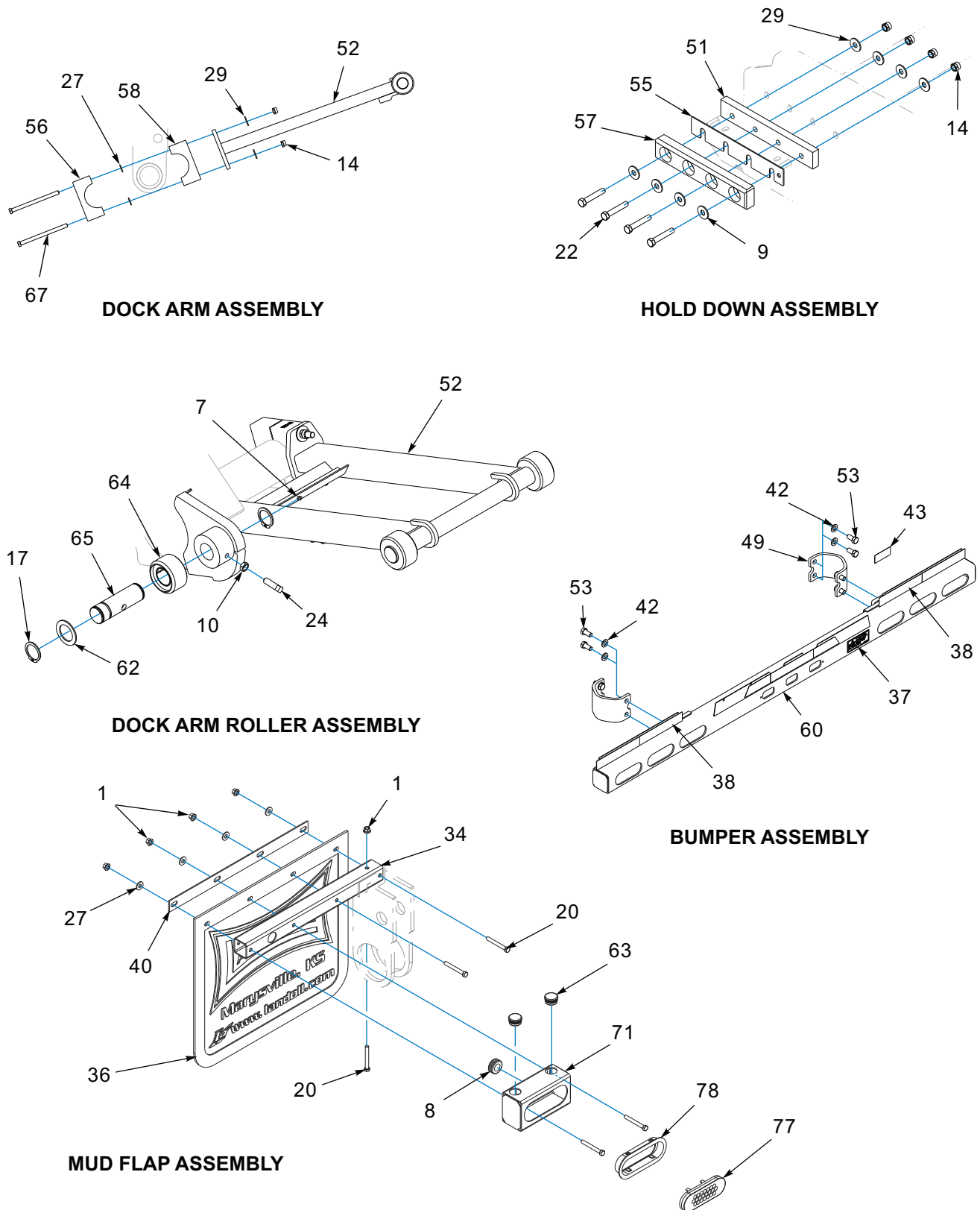
Figure 1-33: General Items - 950E (3 of 3)
