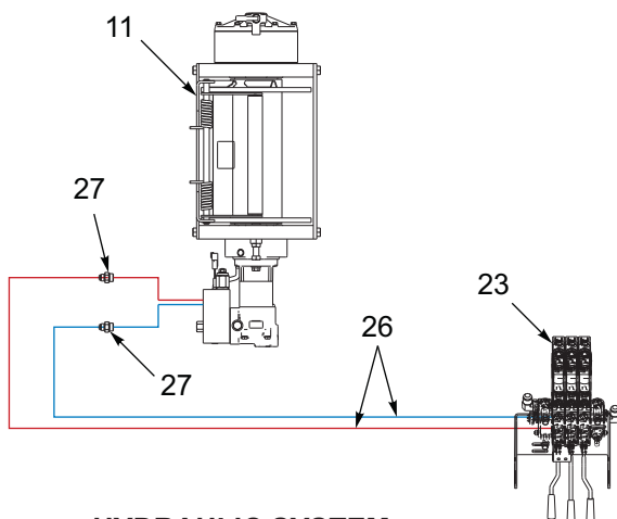
HYDRAULIC SYSTEM
