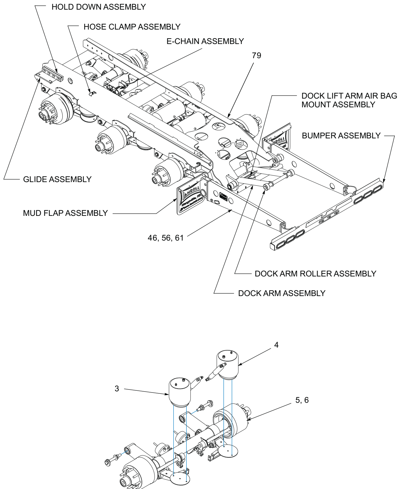
Figure 1-31: General Items - 950E (1 of 3)
