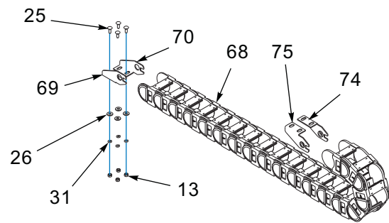
E-CHAIN ASSEMBLY
