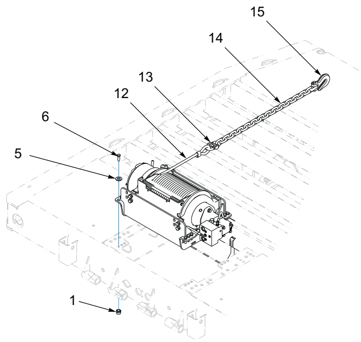
GENERAL ASSEMBLY
