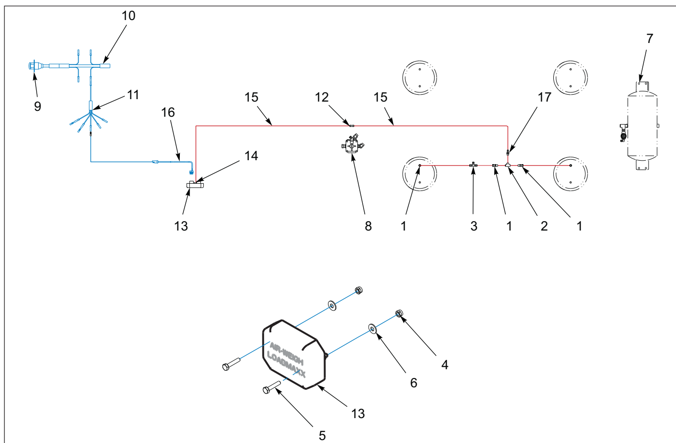
Figure 1-68: Loadmax System
