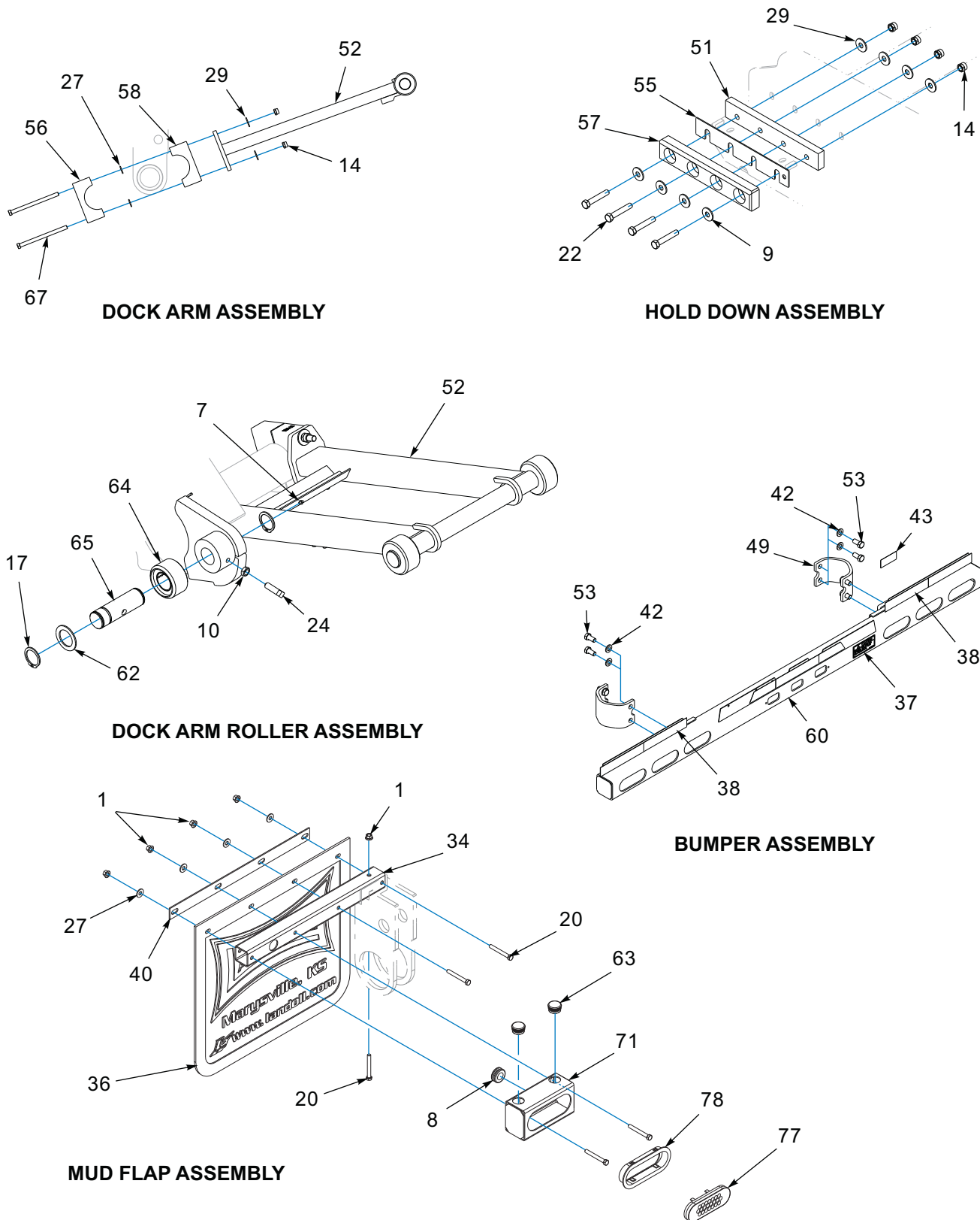
Figure 1-30: General Items - 930E (3 of 3)
