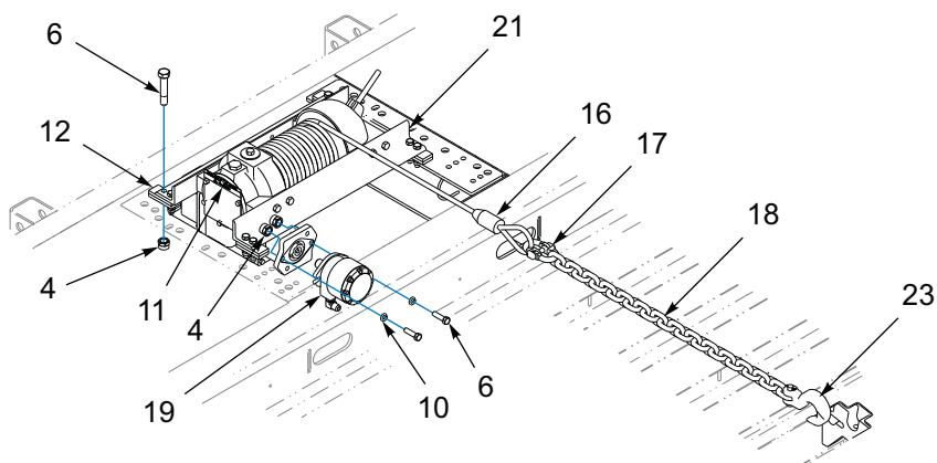
WINCH ASSEMBLY
