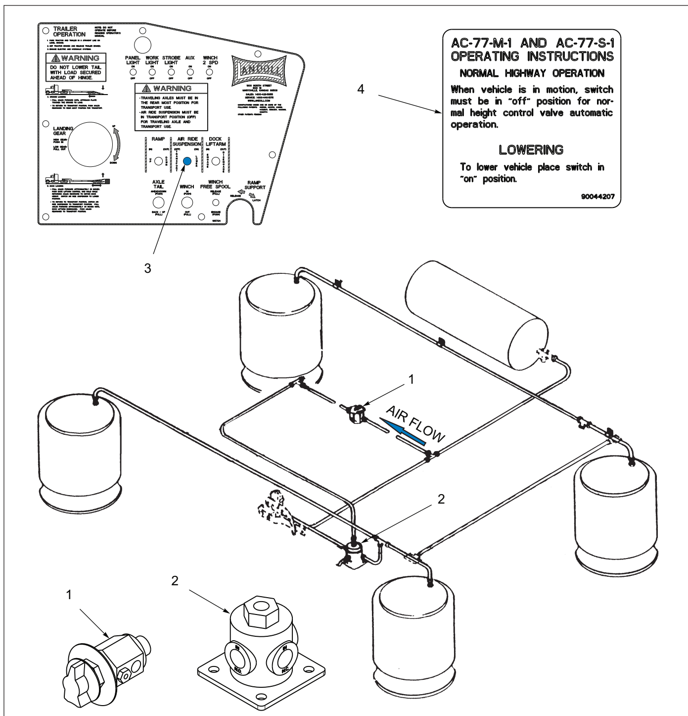
Figure 1-39: Air Control Kit - Lower Suspension
