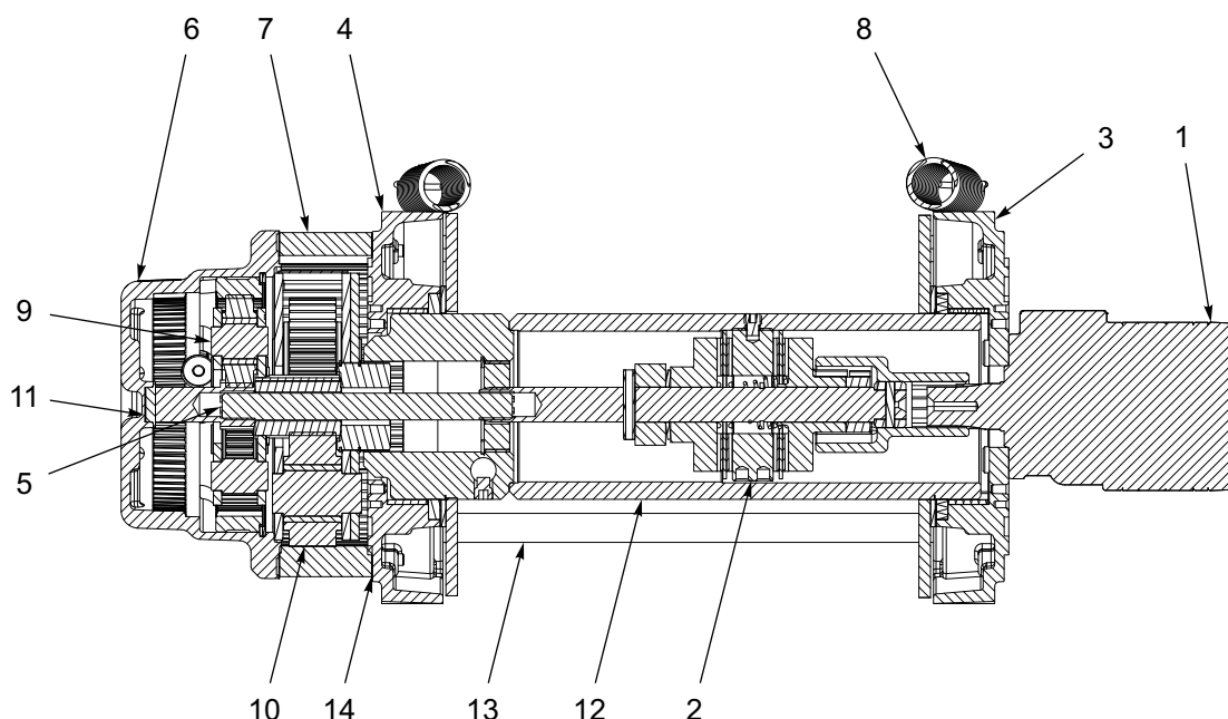
Figure 1-60: Winch Items - 12K (WARN)
