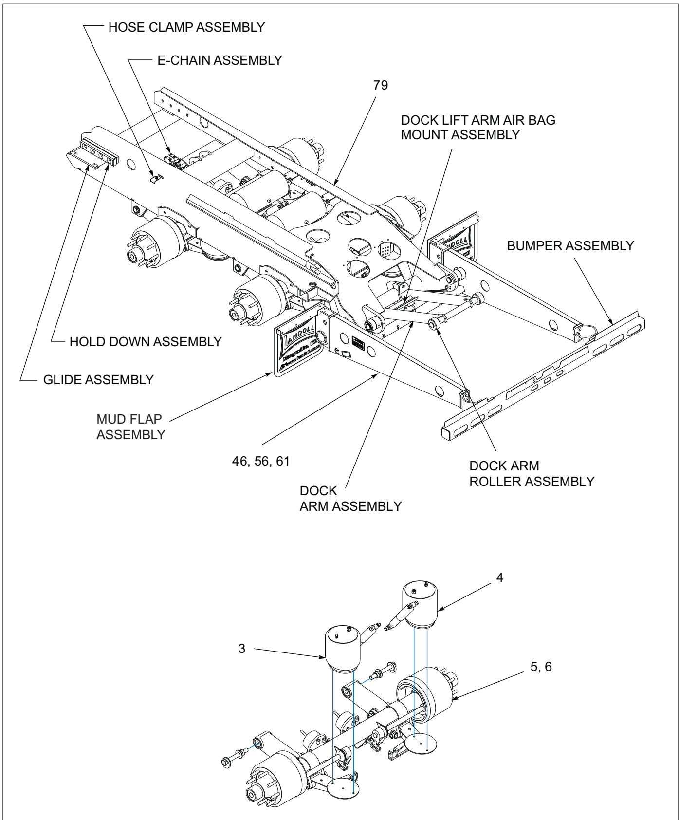
Figure 1-28: General Items - 930E (1 of 3)
