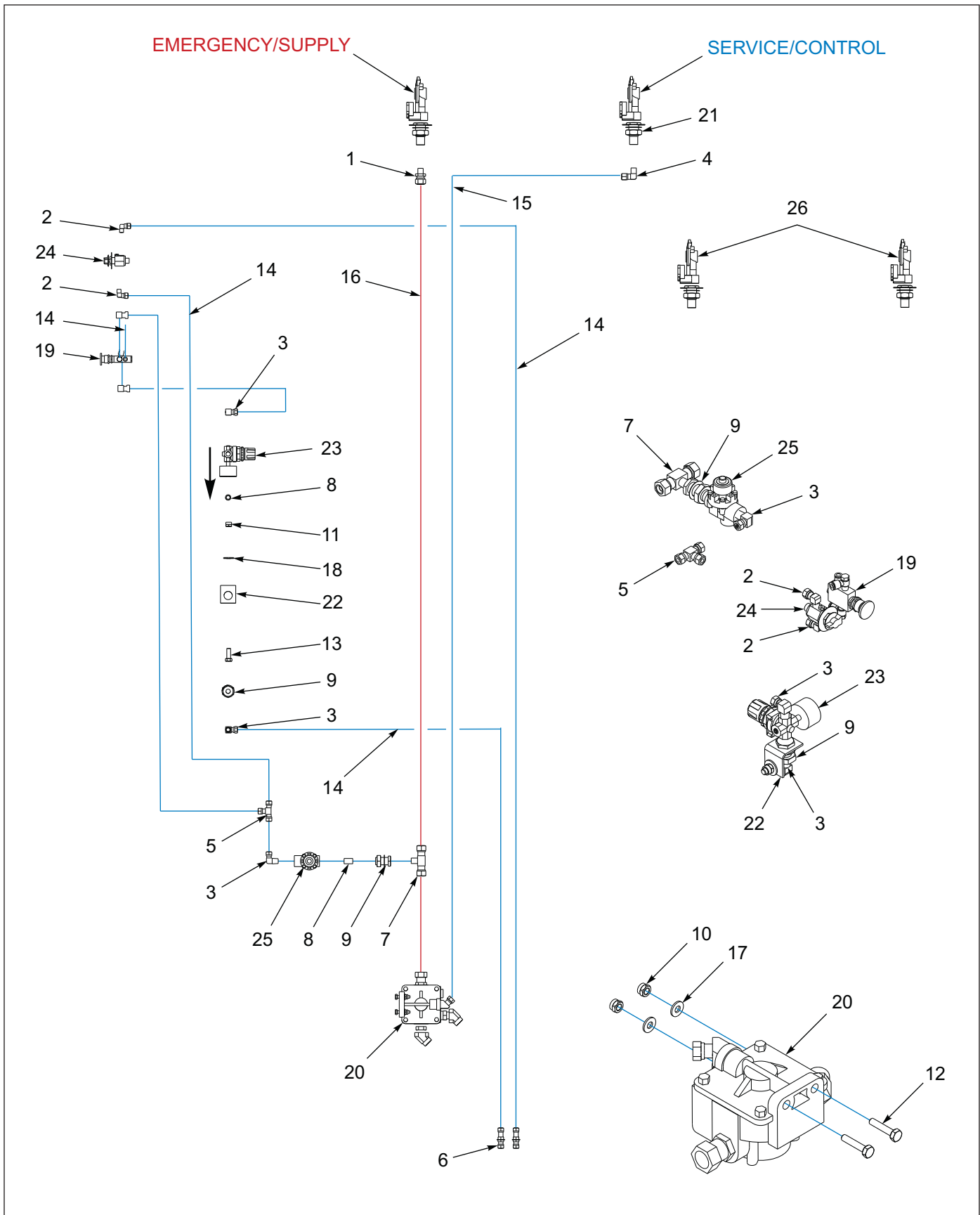
Figure 1-16: Air System
