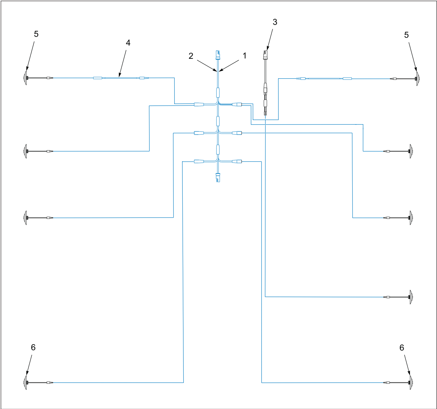
Figure 1-13: Tail Assembly - Electrical System (12', 14', 15')
