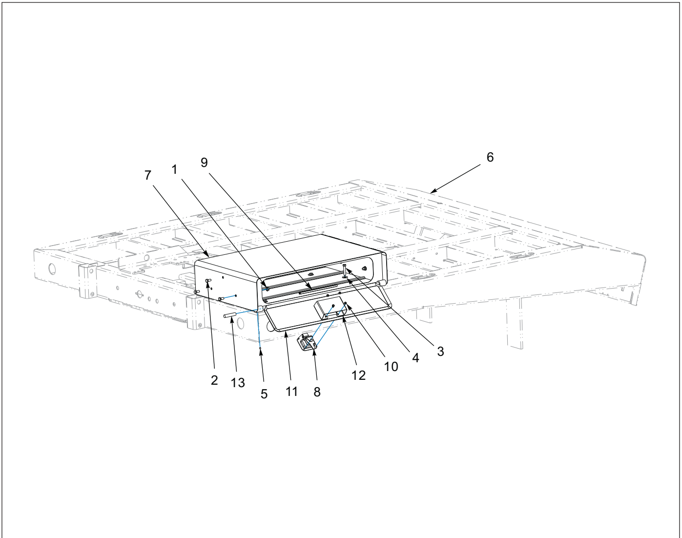
Figure 1-111: Toolbox Installation - Upper Deck
