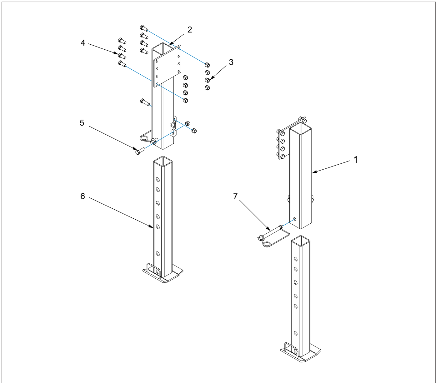
Figure 1-65: “Bolt On” Park Stand
