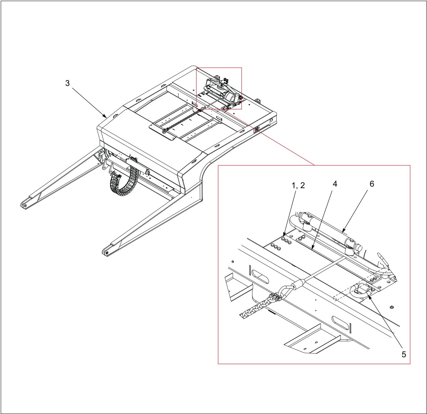
Figure 1-118: Trim Plate Installation
