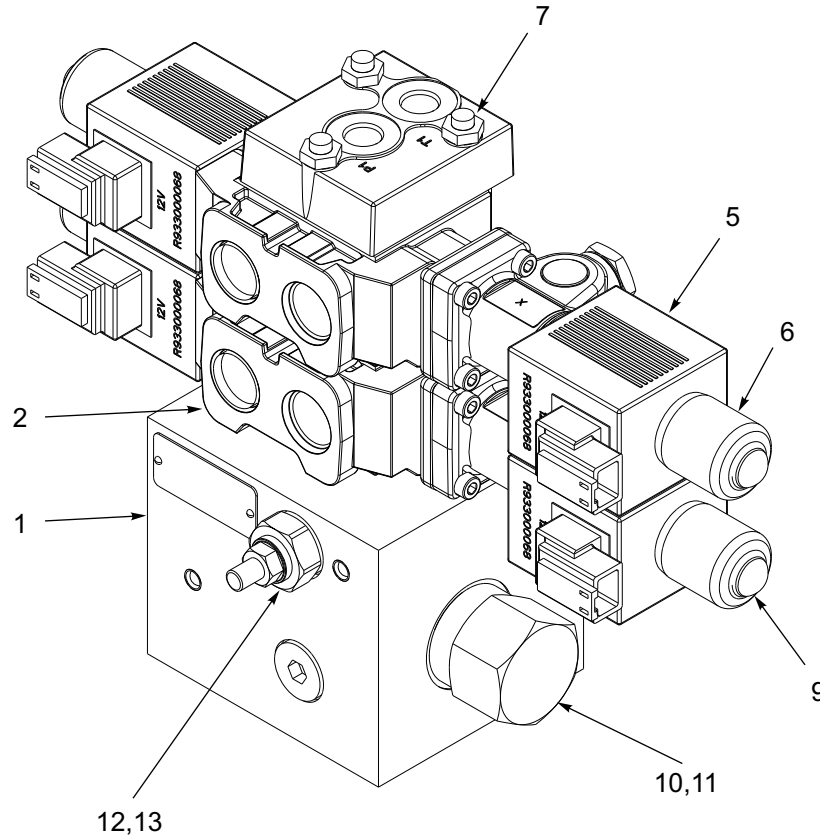
Figure 1-24: Valve Assembly - 2 Spool Solenoid
