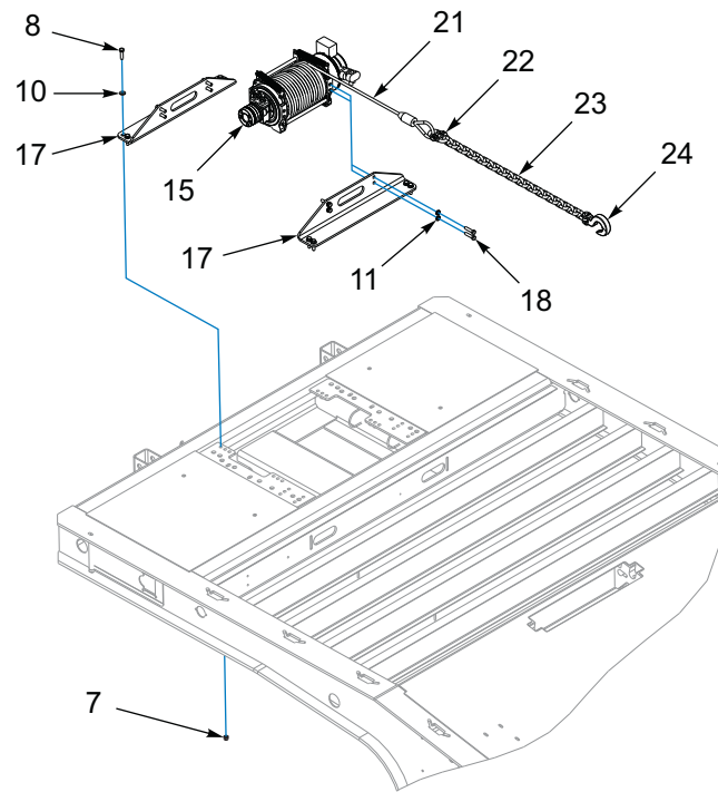
GENERAL ASSEMBLY
