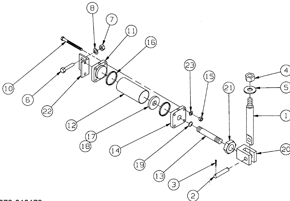
Figure 1-31 Winch Air Shift Cylinder for 20,000# Winch
