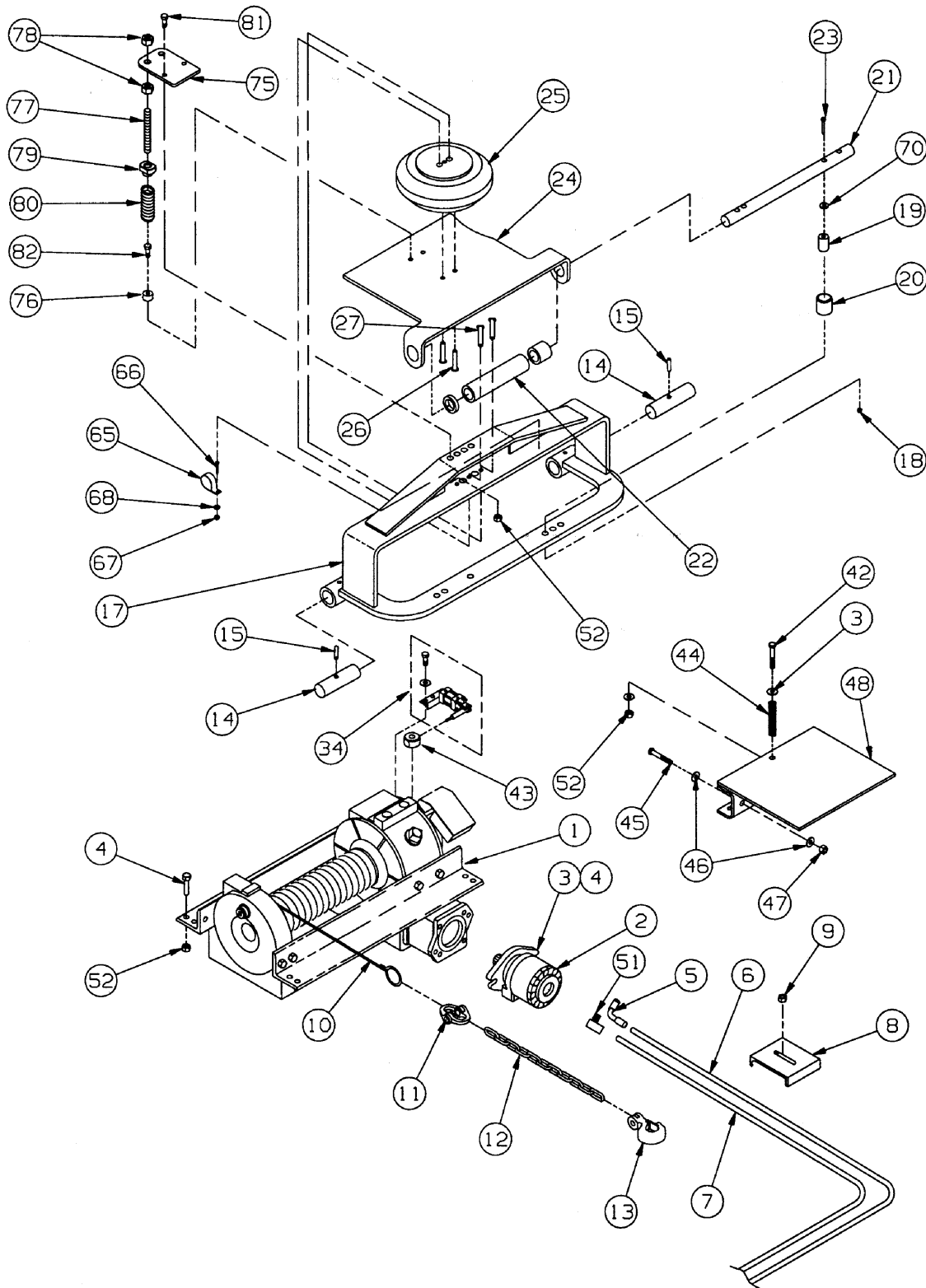
Figure 1-26 12K & 20K Upper Deck Winch (Braden) (1 of 2)
