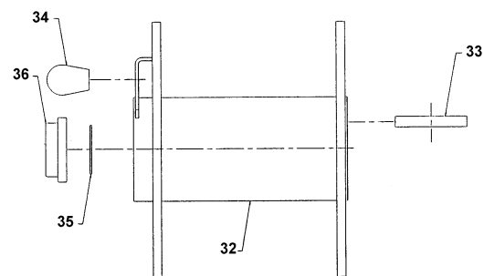
DRUM INSTALLATION
