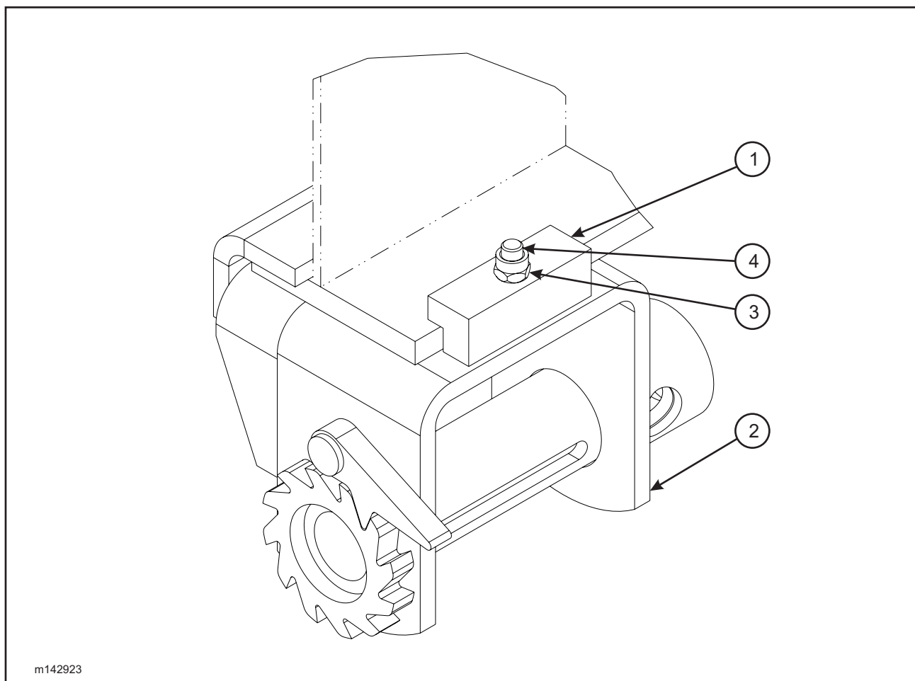
Figure 1-66 4" Webbing Sliding Winch Assembly (Option)
