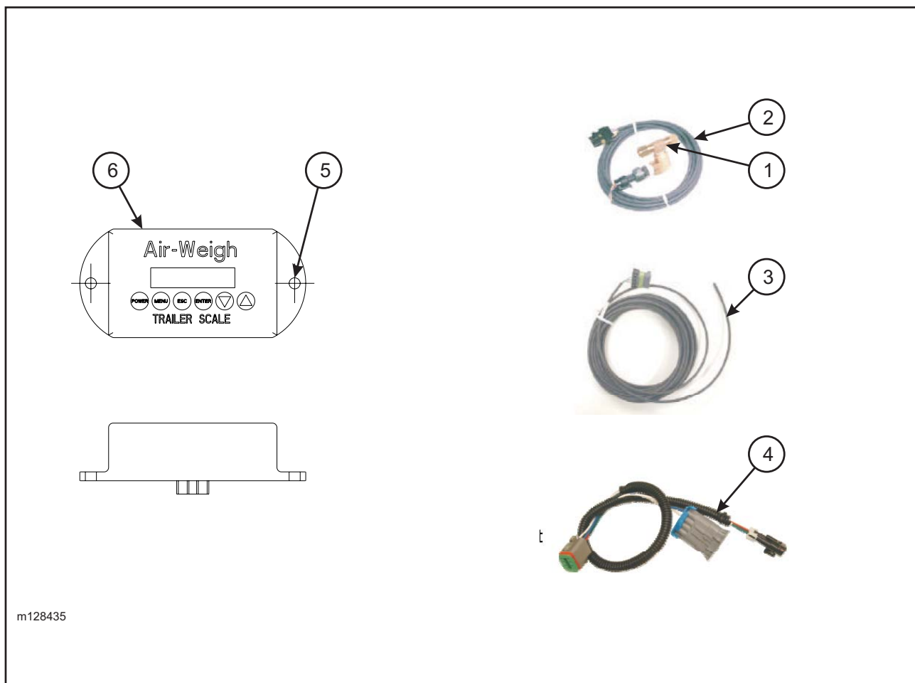
Figure 1-58 Air Digital Scale (Option)
