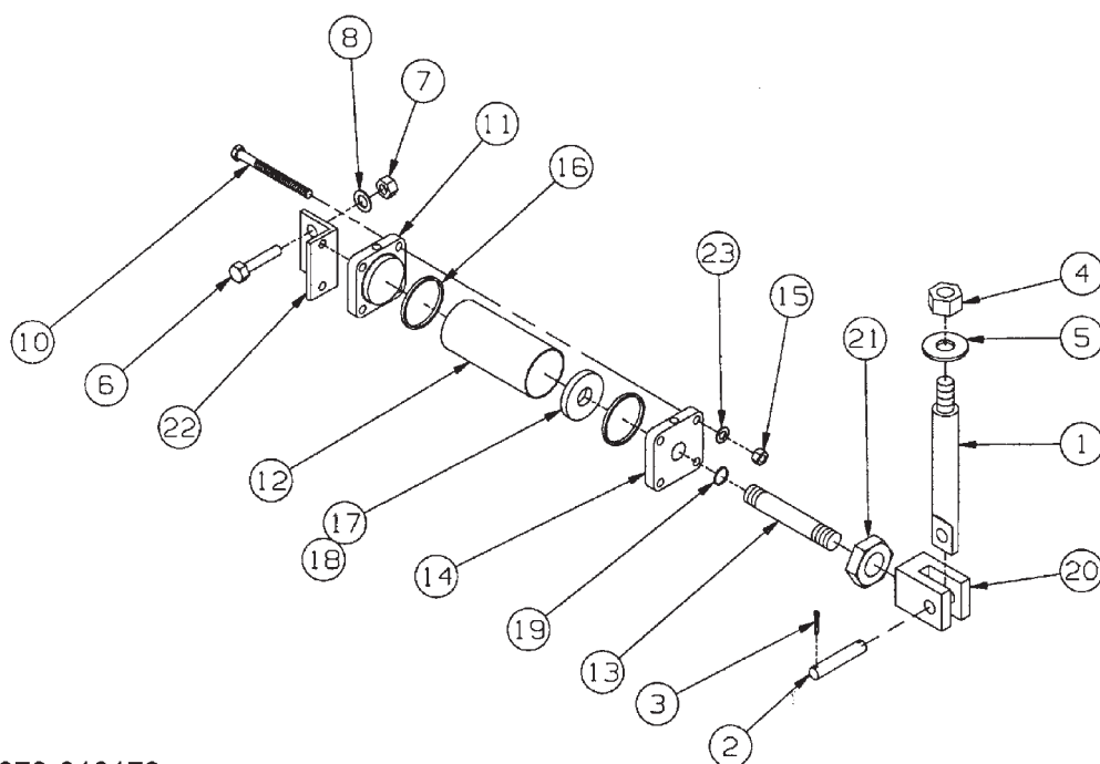
Figure 1-29 Winch Air Shift Cylinder for 20,000# Winch
