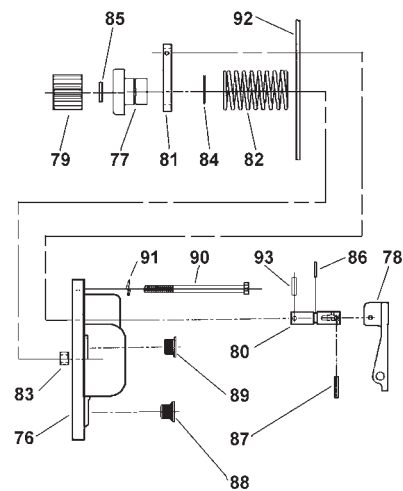
LEVER KICKOUT GEAR END COVER INSTALLATION
