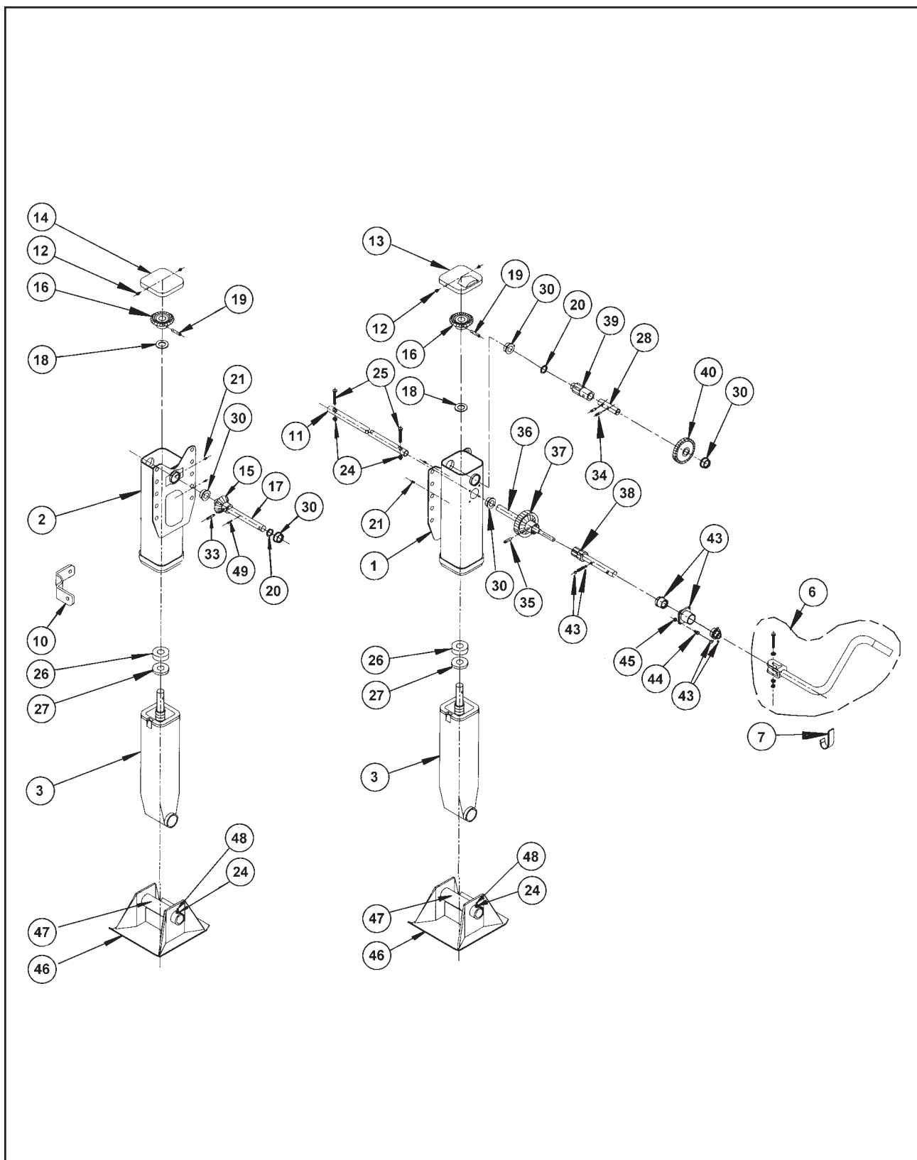
Figure 1-49 Crank Landing Gear
