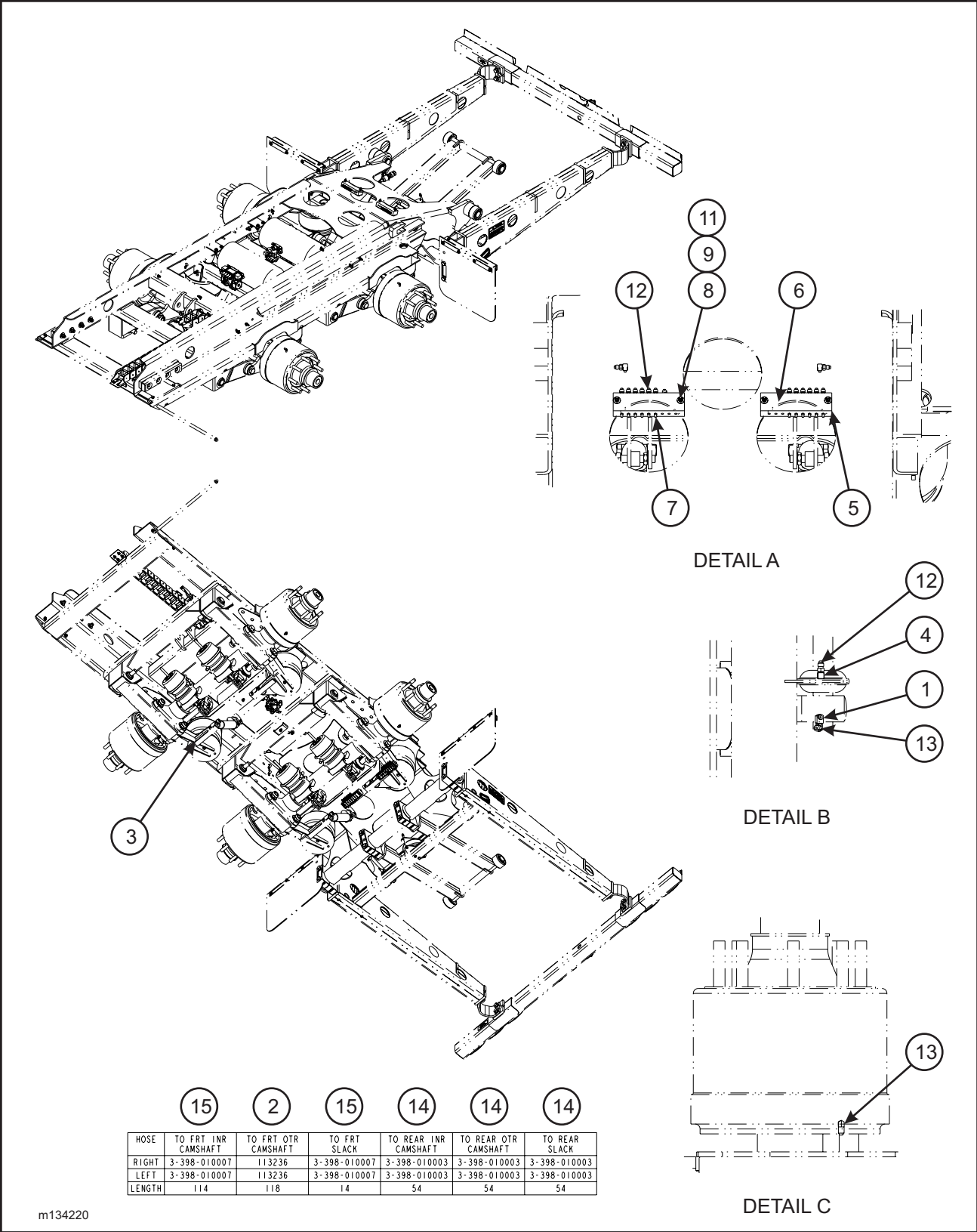
Figure 1-67 U/C Grease System (Tandem)
