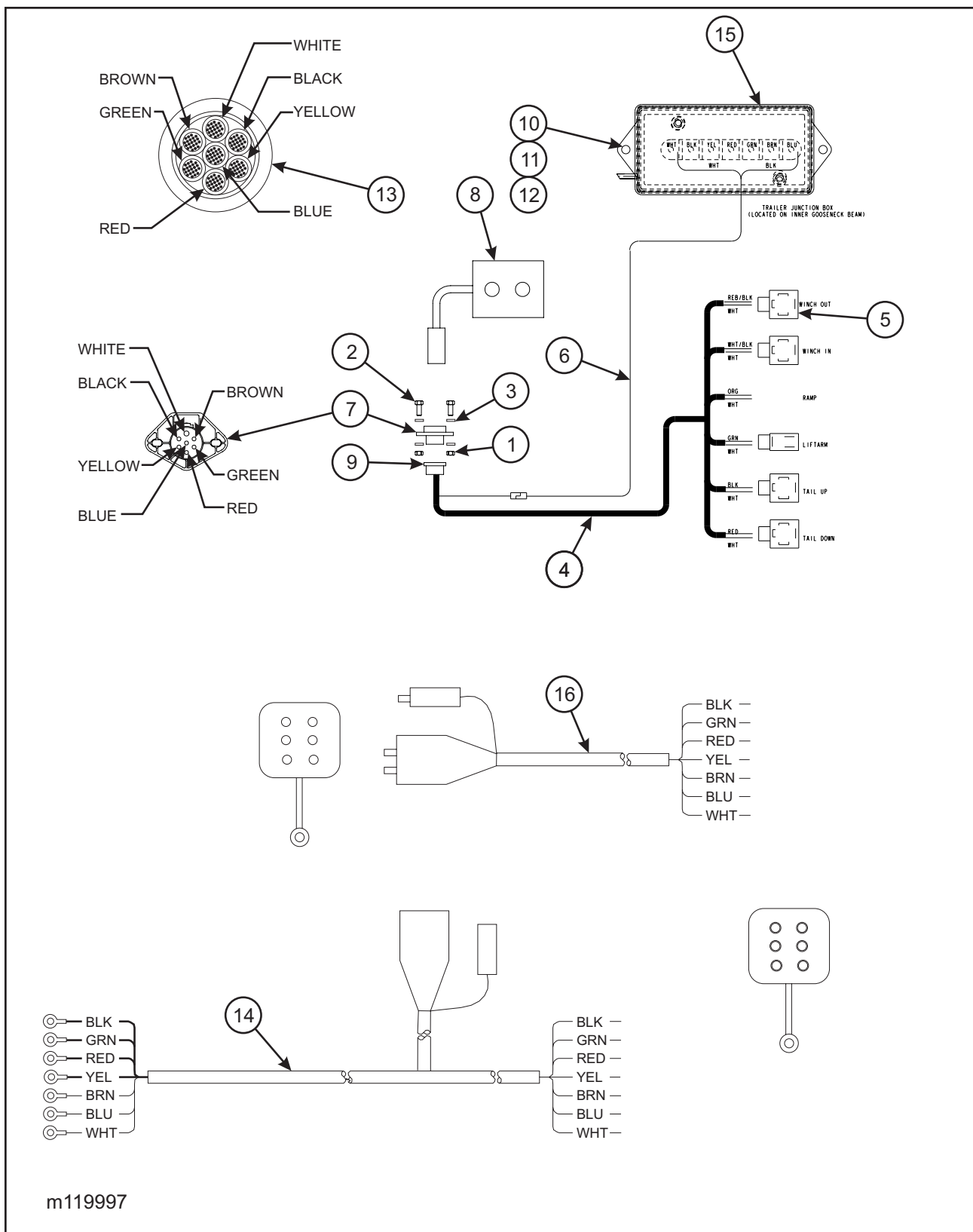
Figure 1-41 Wired Remote Control Items
