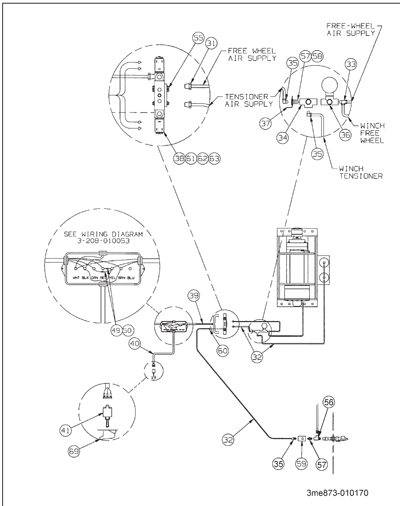
Figure 1-32 30K Upper Deck Winch (DP) (2 of 2)
