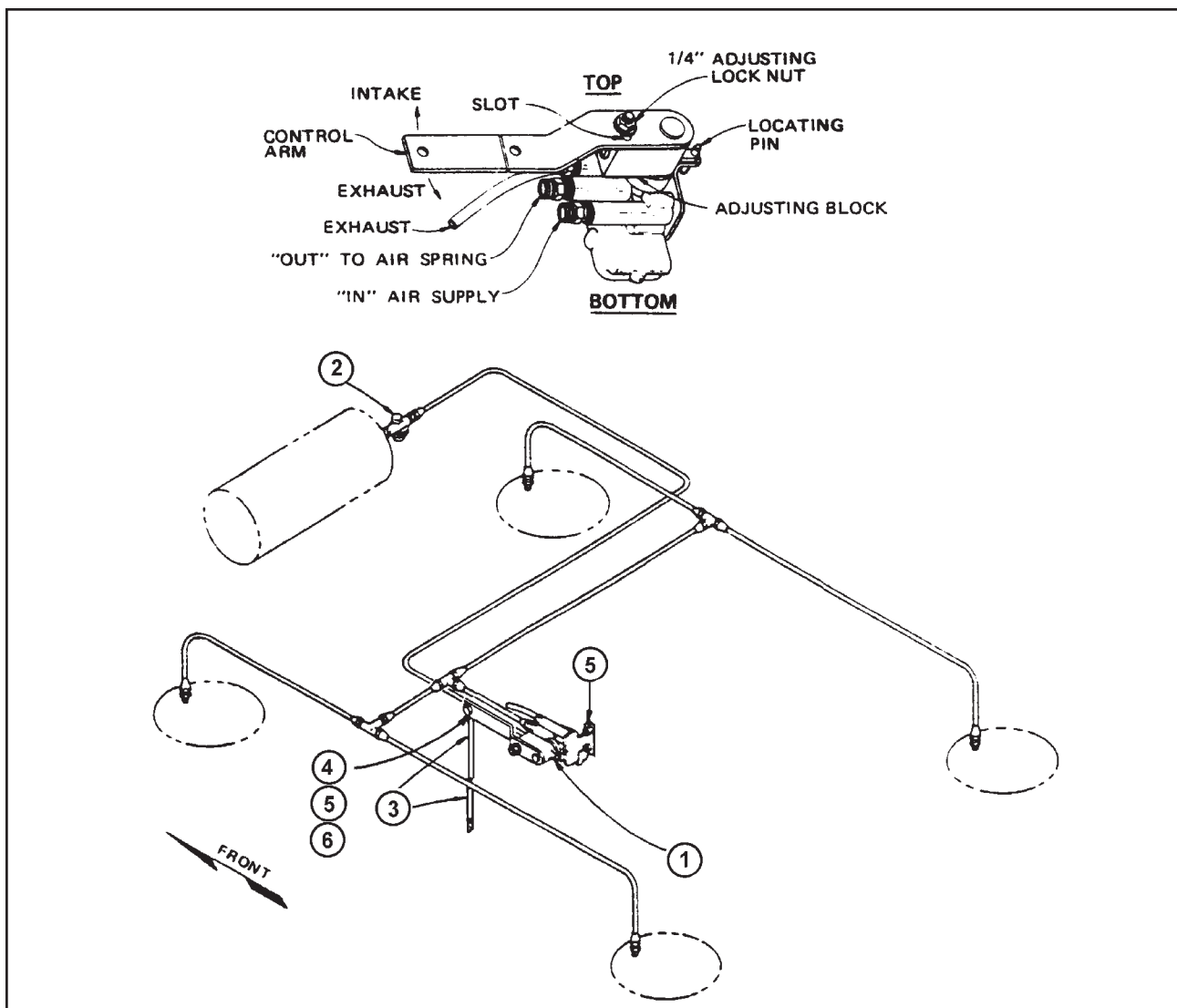
Figure 1-15 Air Control Kit
