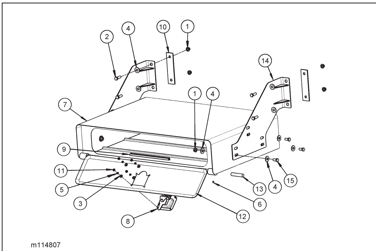
Figure 1-61 Toolbox Installation (Option)
