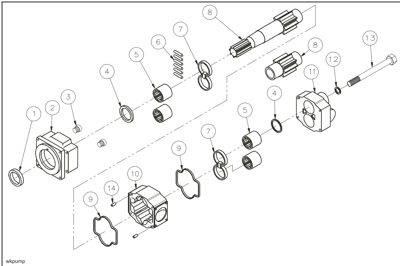
Figure 1-9 Pump, Wet Kit Hydraulic
