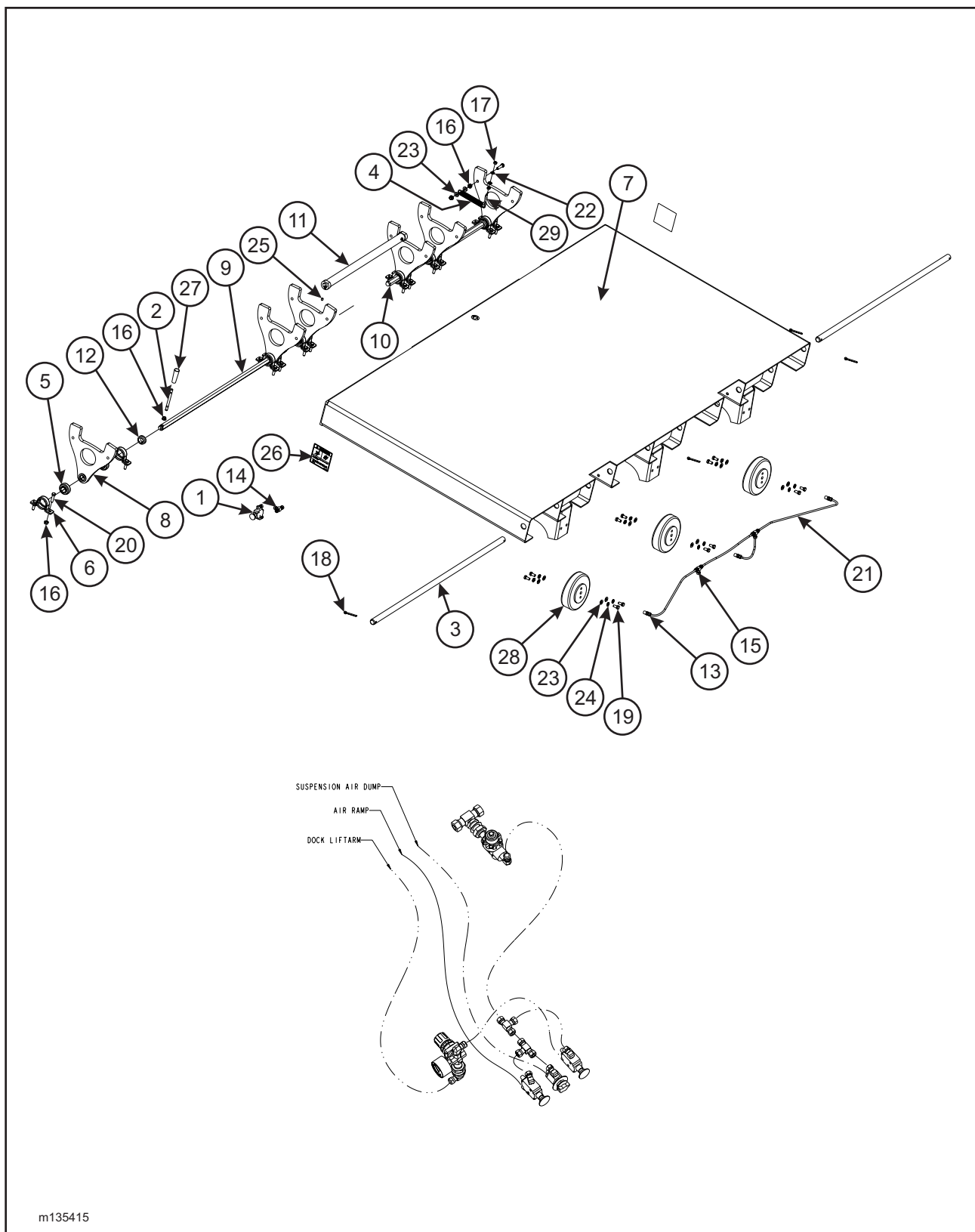
Figure 1-4 Air Ramp Assembly
