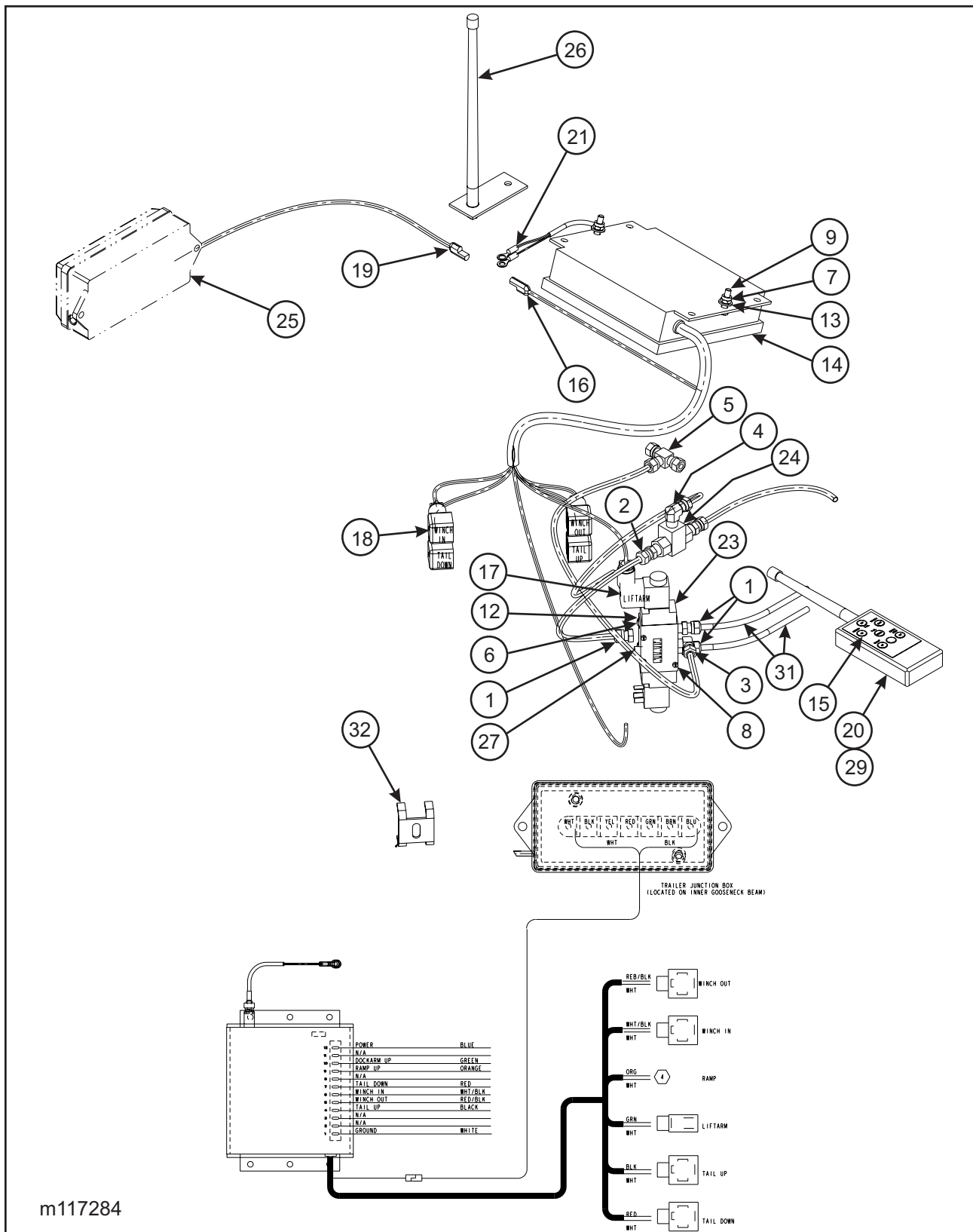
Figure 1-43 Wireless Remote Control
