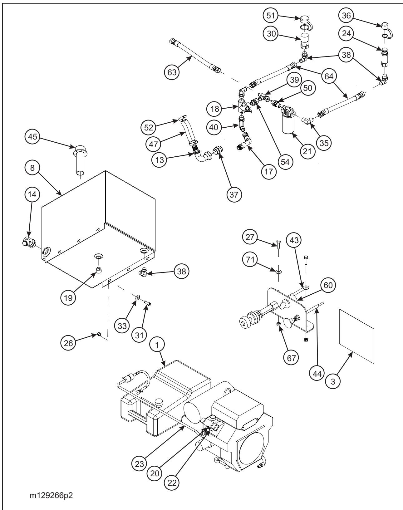
Figure 1-51 Hydraulic Engine, 27HP Upper Deck (2 of 2)
