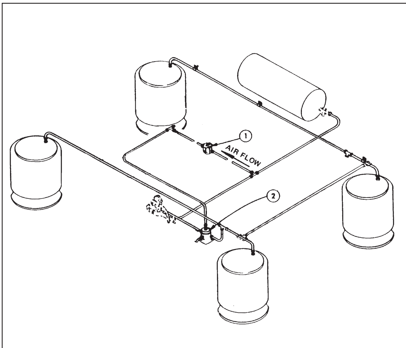
Figure 1-16 Air Control Kit
