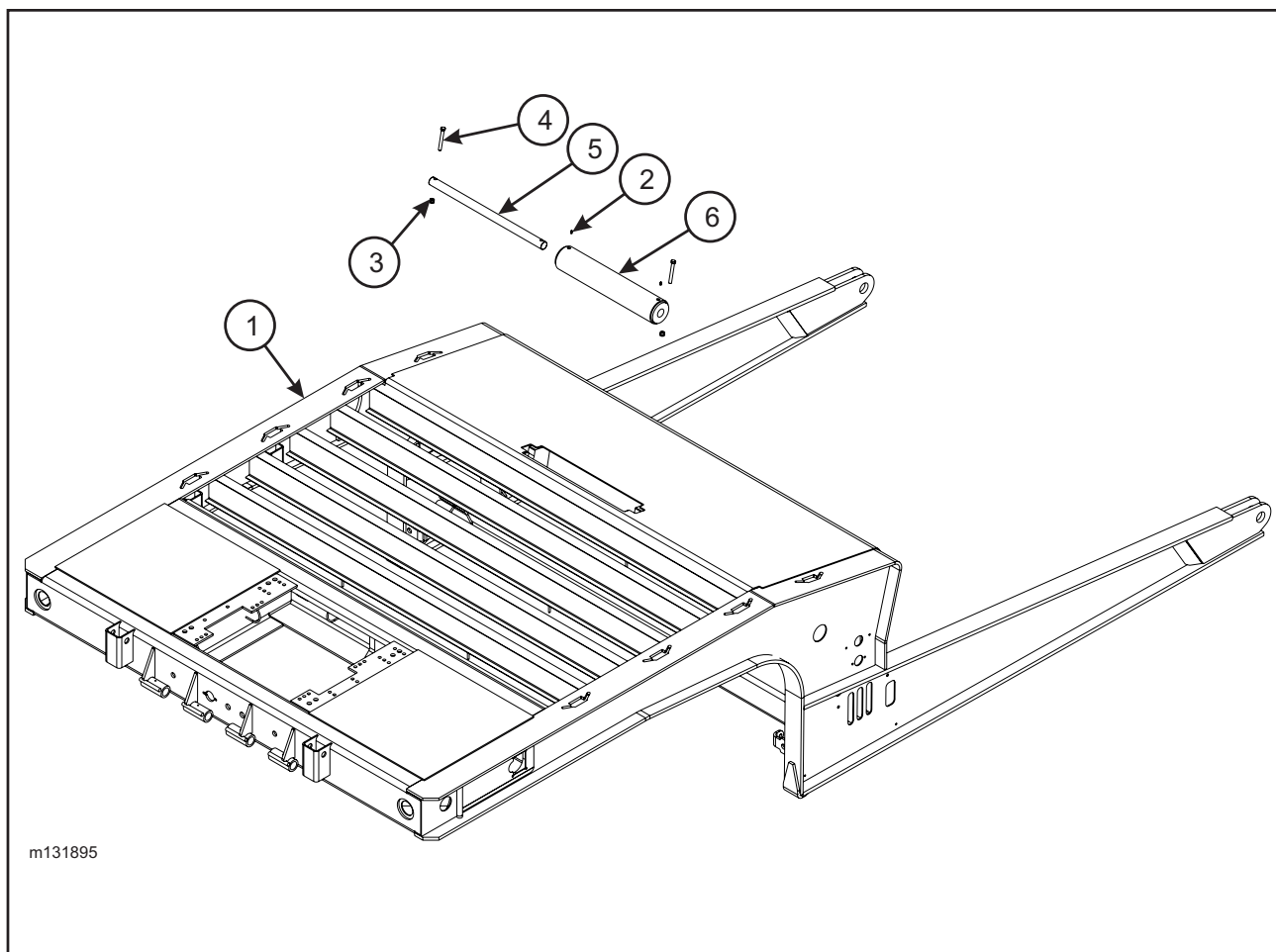
Figure 1-64 Upper Deck Roller Installation (Option)
