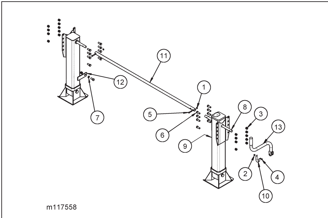
Figure 1-47 Landing Gear
