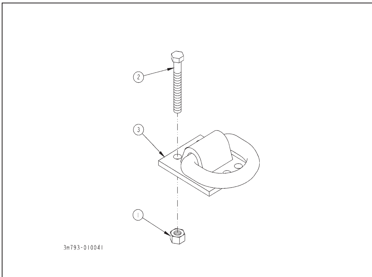
Figure 1-59 D-Ring Installations (Option)
