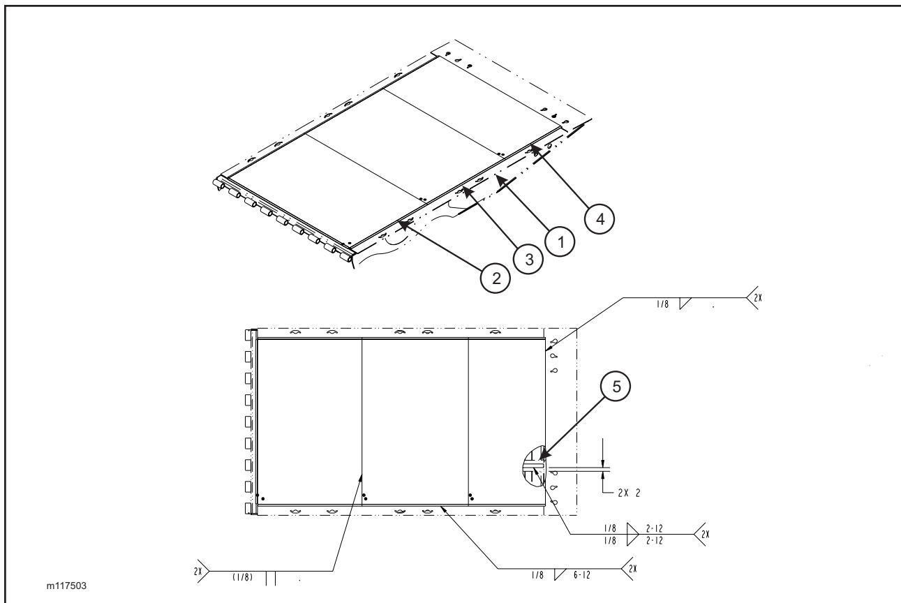
Figure 1-65 3 Deck Tread Grip/ Over Wood 15' Tail (Option)
