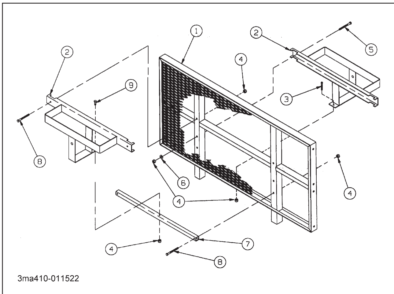
Figure 1-56 Spare Tire Carrier (Option)
