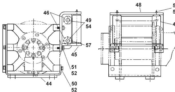
BASE INSTALLATION
