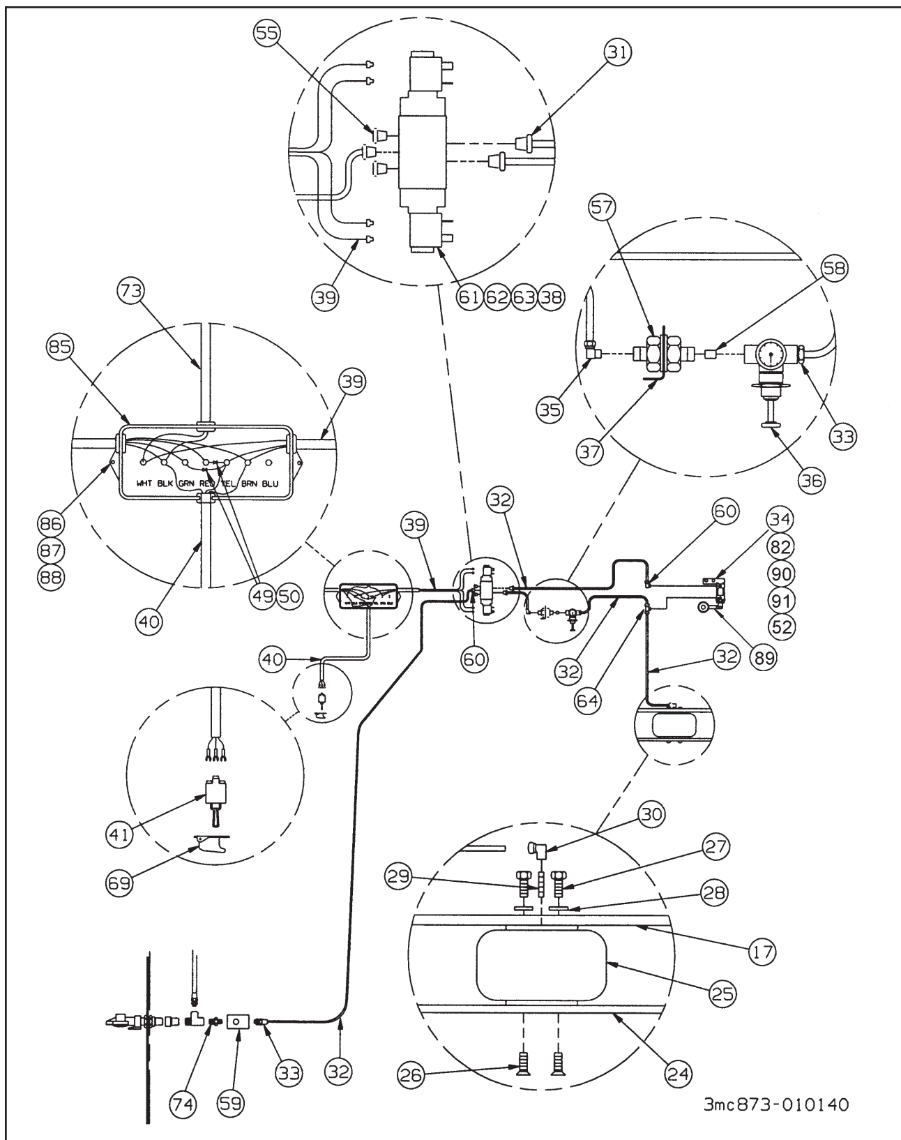
Figure 1-25 12K & 20K Upper Deck Winch (Braden) (2 of 2)
