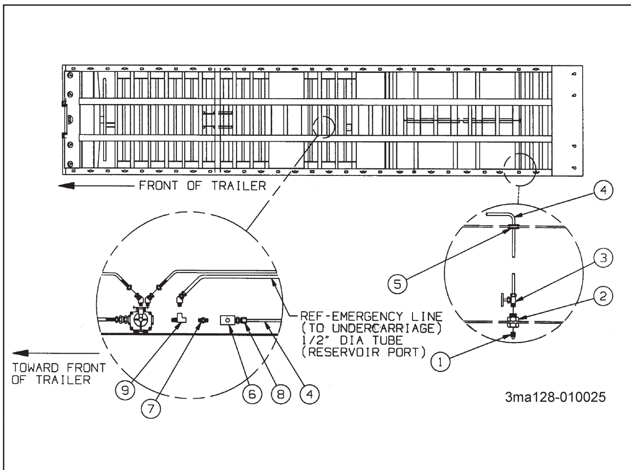
Figure 1-57 Air Outlet Assembly (Option)
