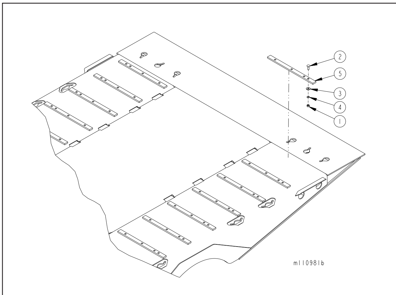
Figure 1-60 Traction Bar Assembly (Option)
