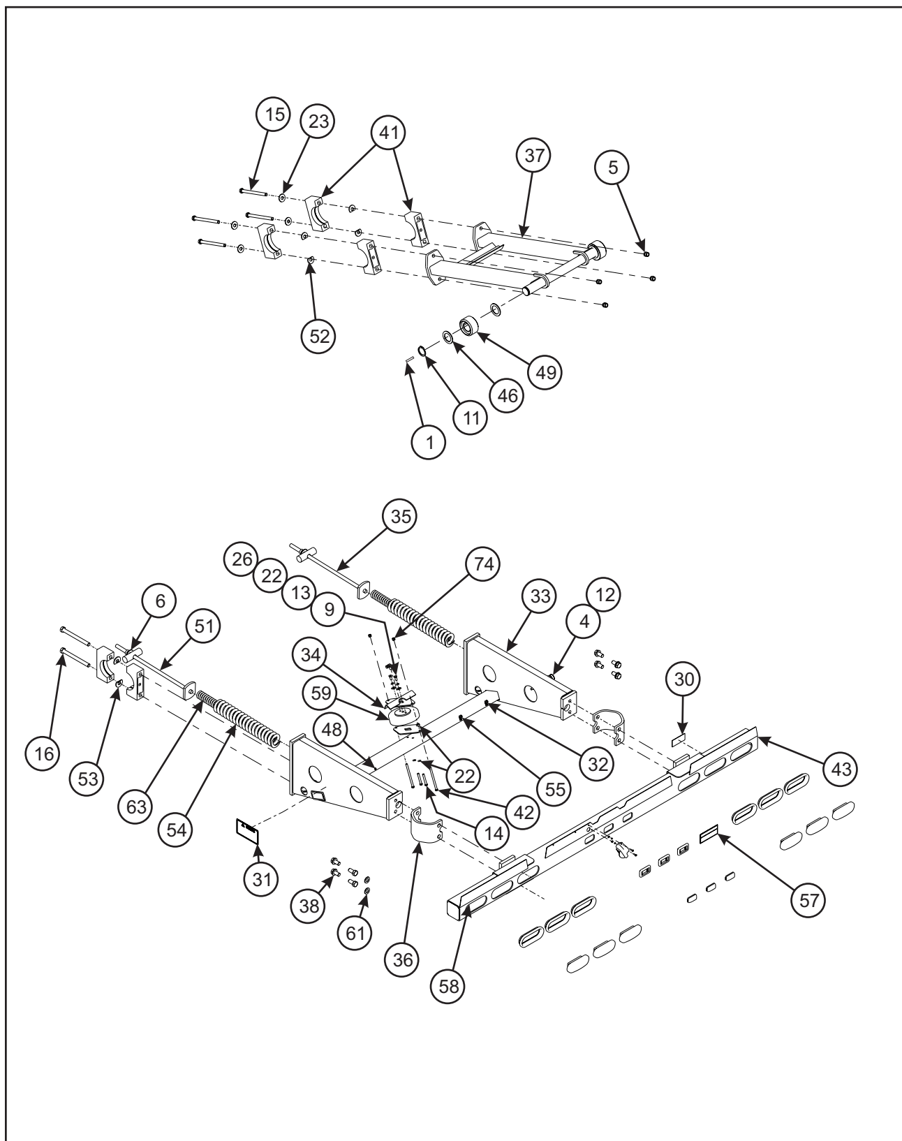
Figure 1-12 U/C Assembly, Air Ride Suspension, Tandem (2 of 2)
