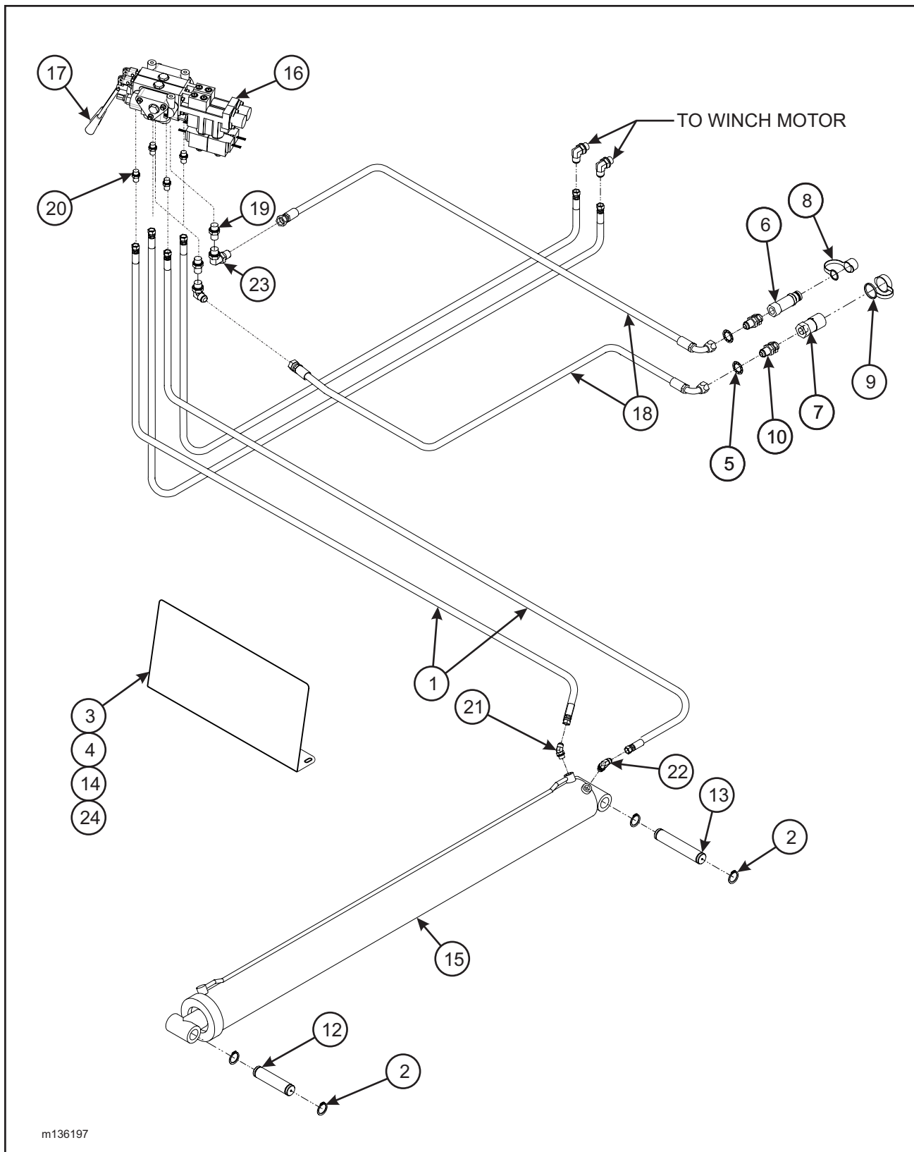
Figure 1-6 Hydraulic System Installation
