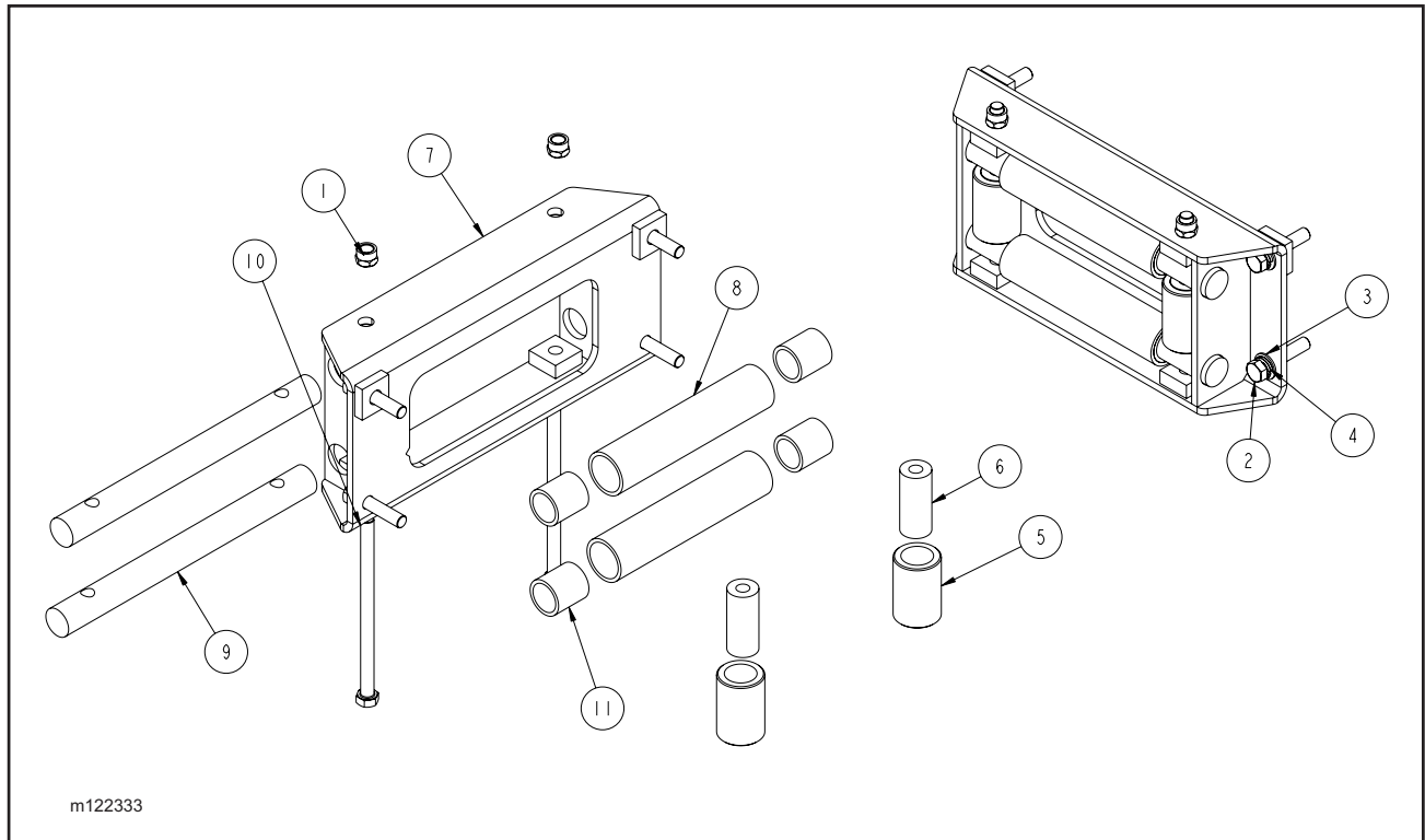
Figure 1-35 Winch Roller Guide - 30K
