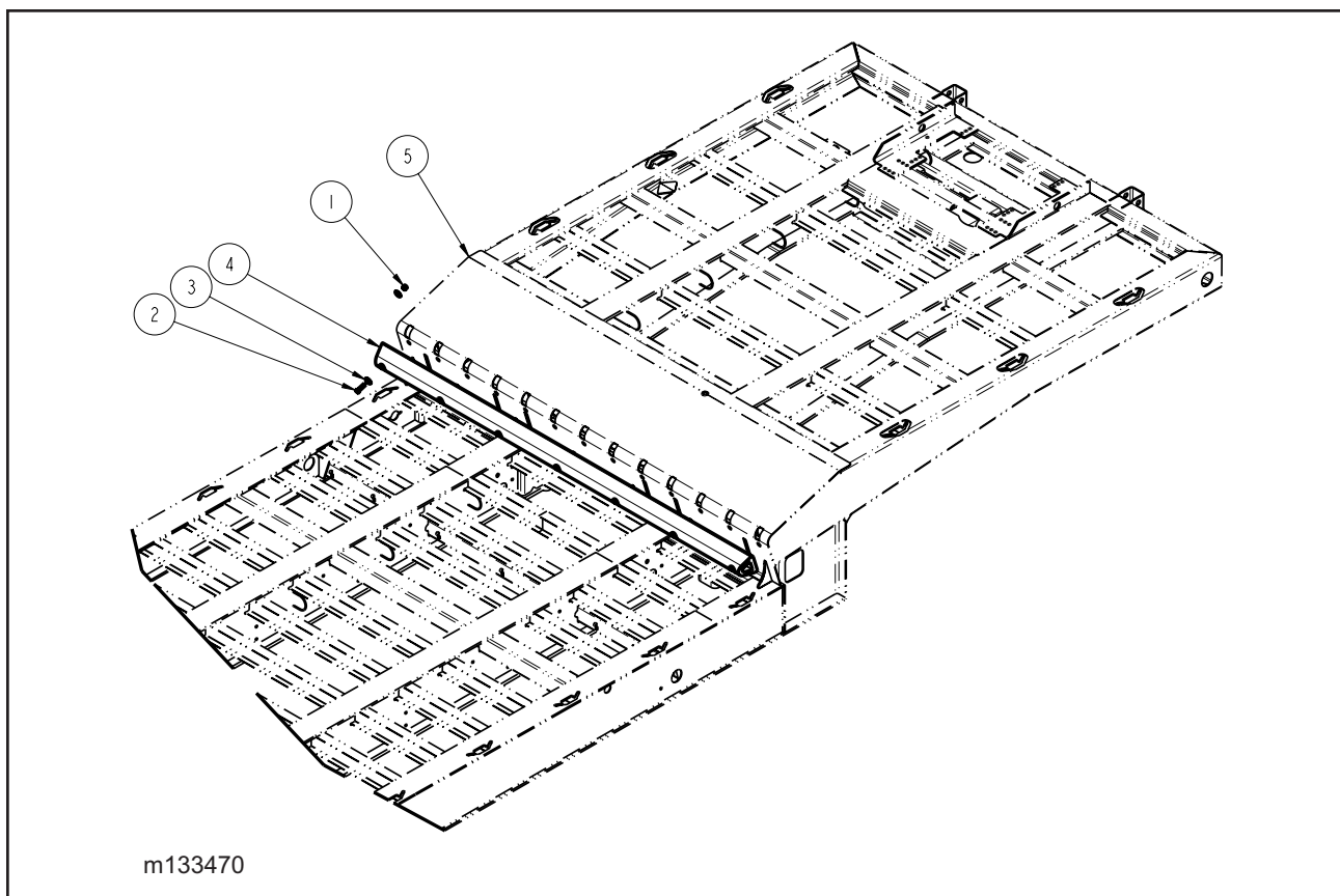
Figure 1-63 Rubber Bumper Stop (Option)
