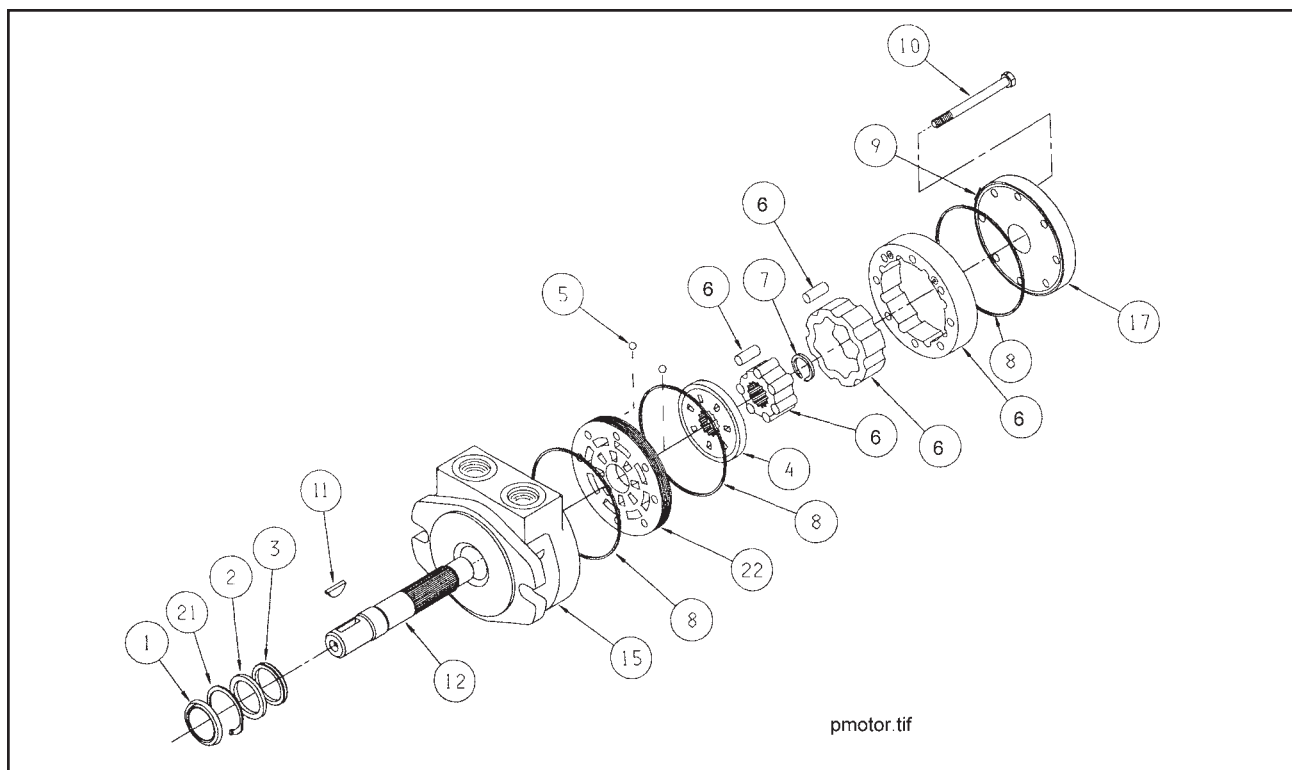
Figure 1-30 Winch Motor Assembly
