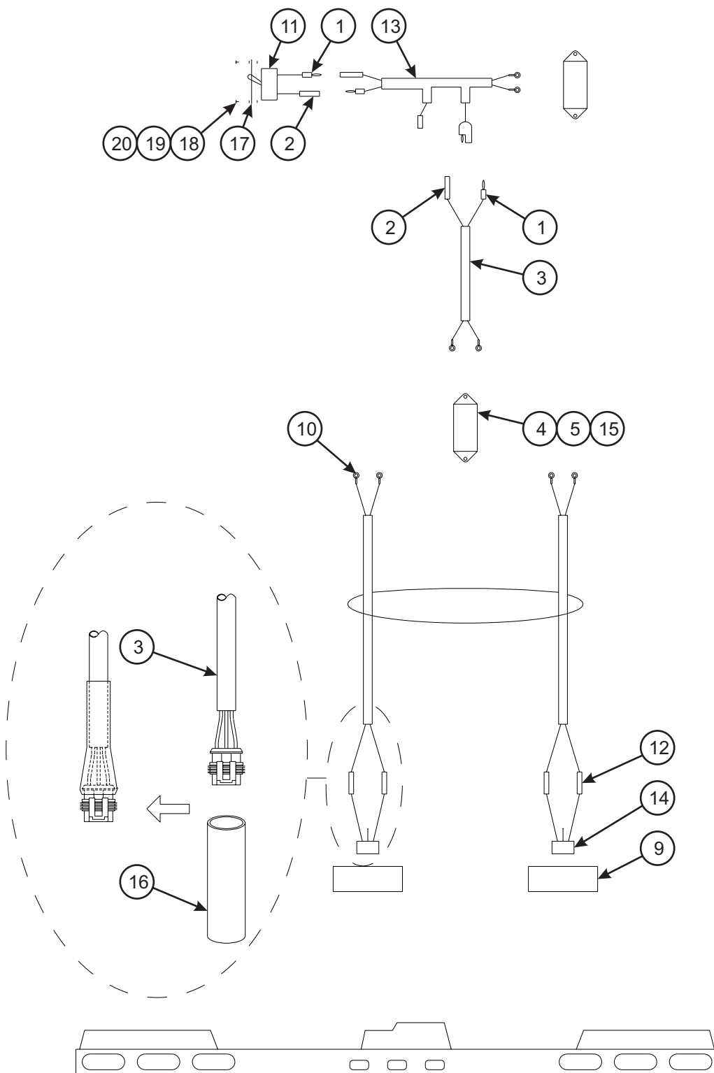
Figure 1-68 Rear Strobe Light Installation (Option)
