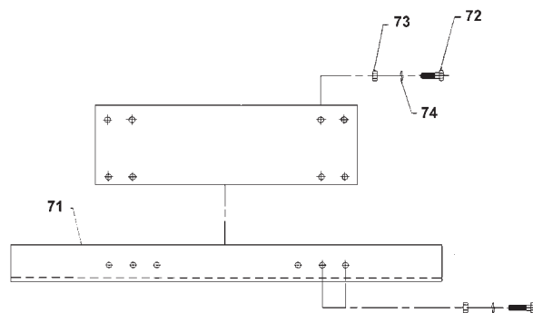
AIR/HYDRAULIC KICKOUT GEAR END COVER INSTALLATION
