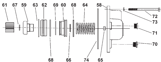
BASE INSTALLATION
