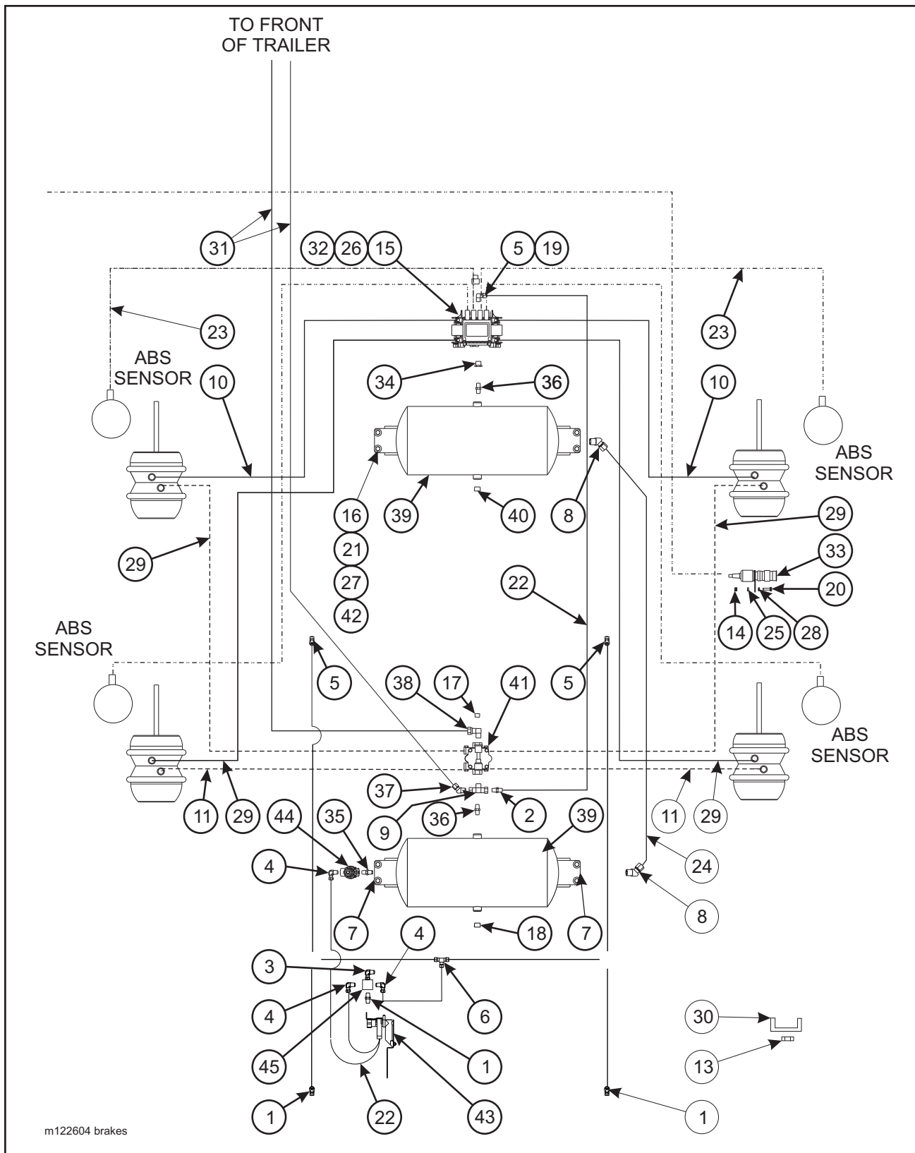
Figure 1-19 Spring Air Brake System w/ ABS, Tandem Axle
