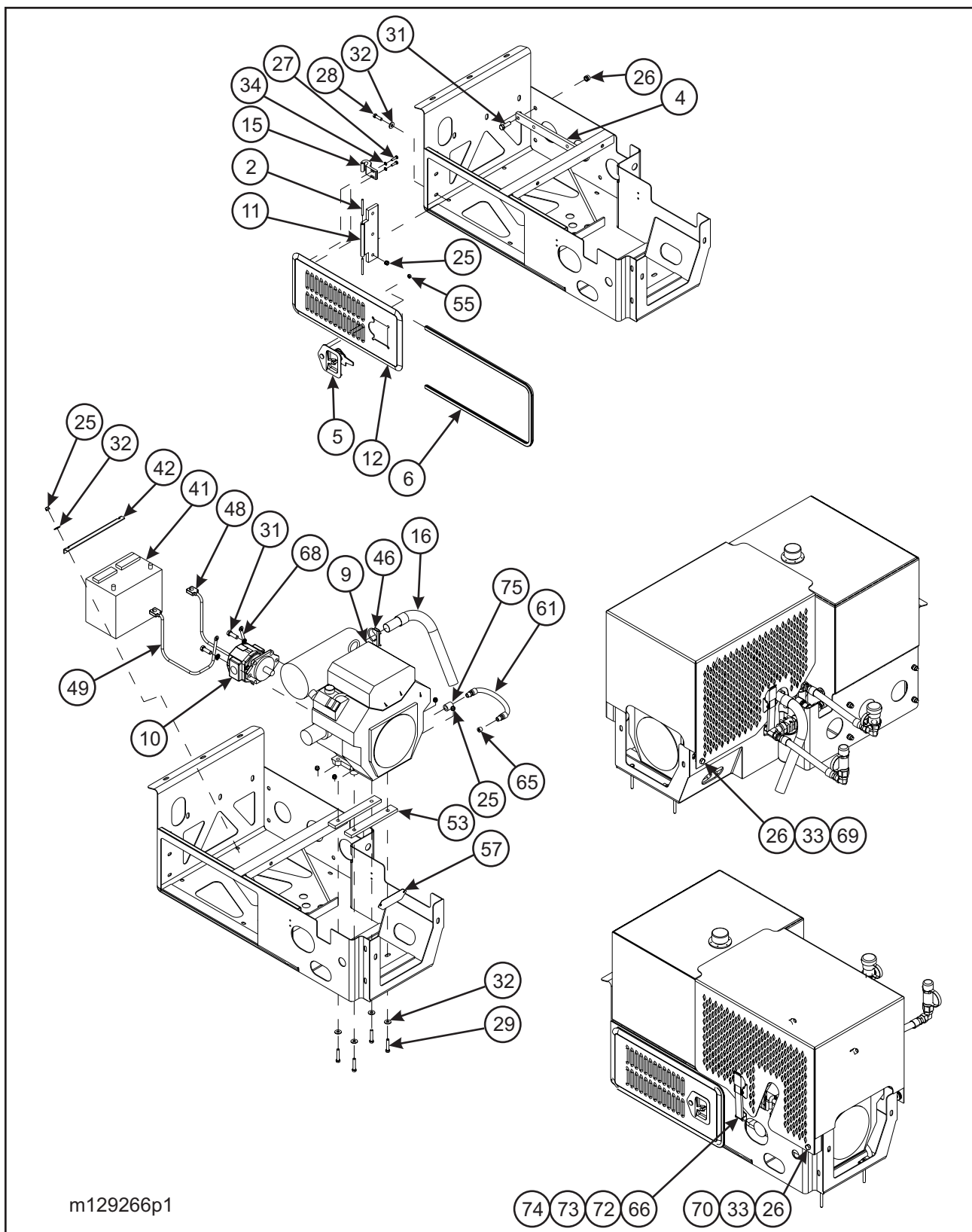
Figure 1-50 Hydraulic Engine, 27HP Upper Deck (1 of 2)
