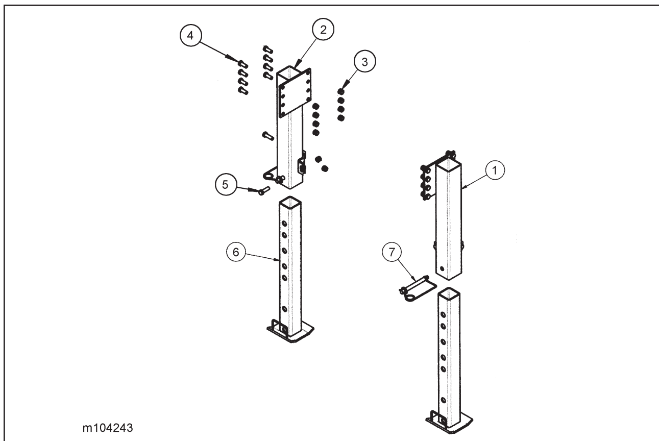
Figure 1-48 Landing Gear Installation - Bolt-on
