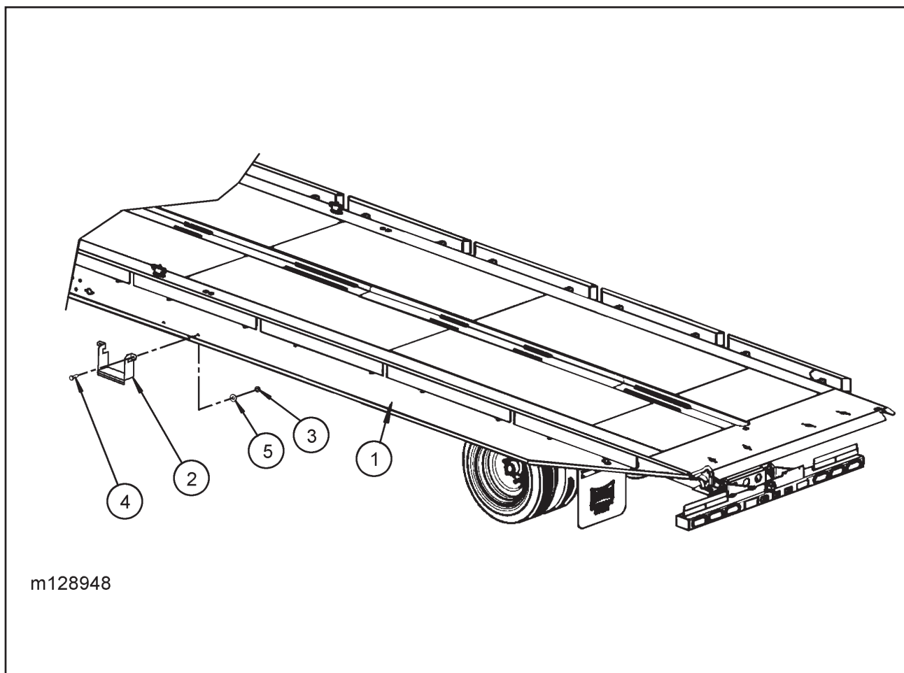
Figure 1-62 Step Assembly (Option)
