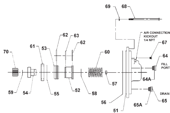
DRUM INSTALLATION
