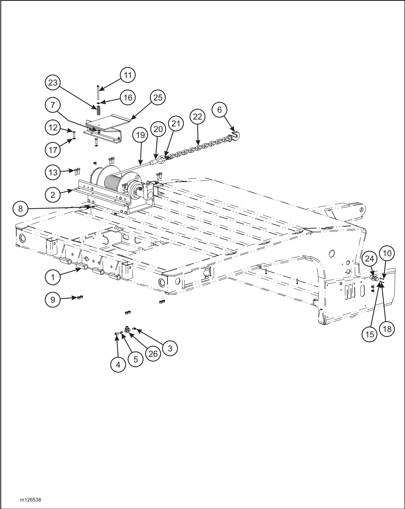
Figure 1-34 30K Upper Deck Winch (DP)
