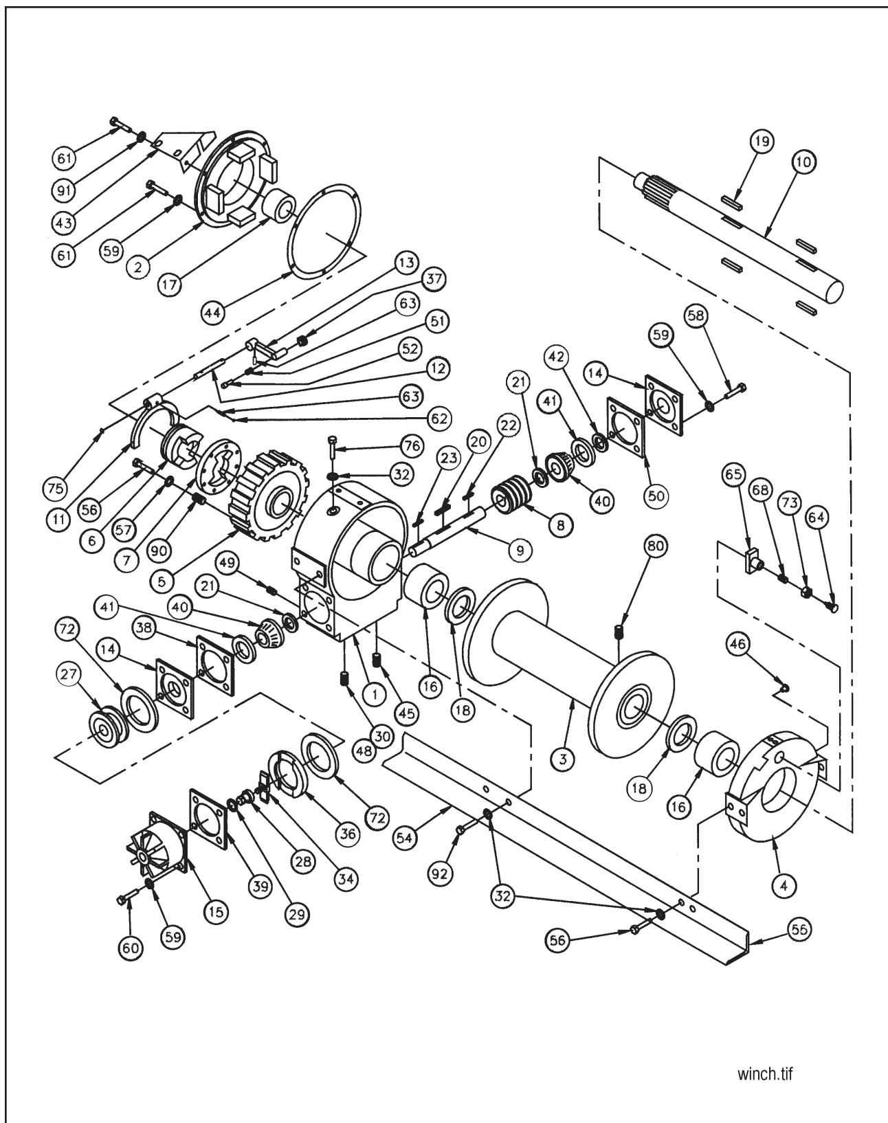
Figure 1-28 20,000# Winch Items (Braden Worm Gear)
