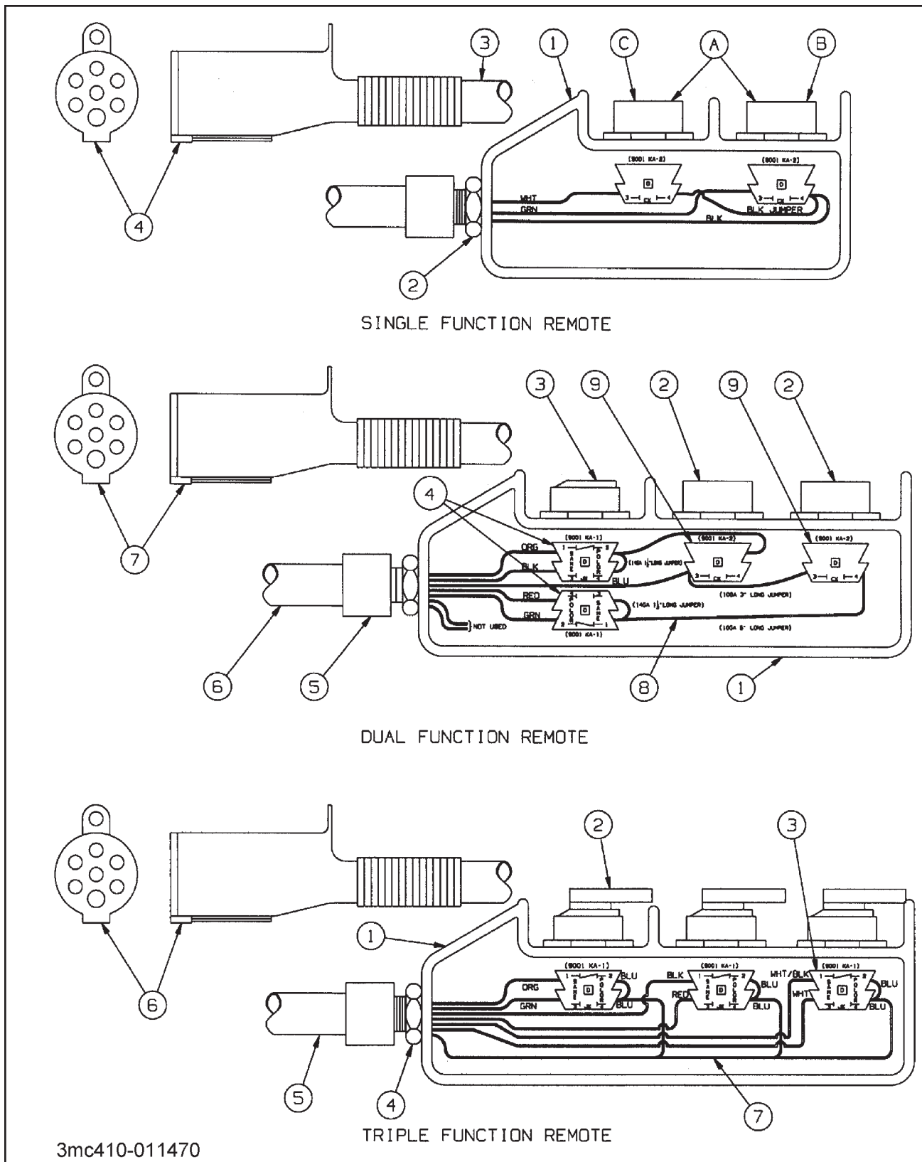
Figure 1-42 Wired Remote Control
