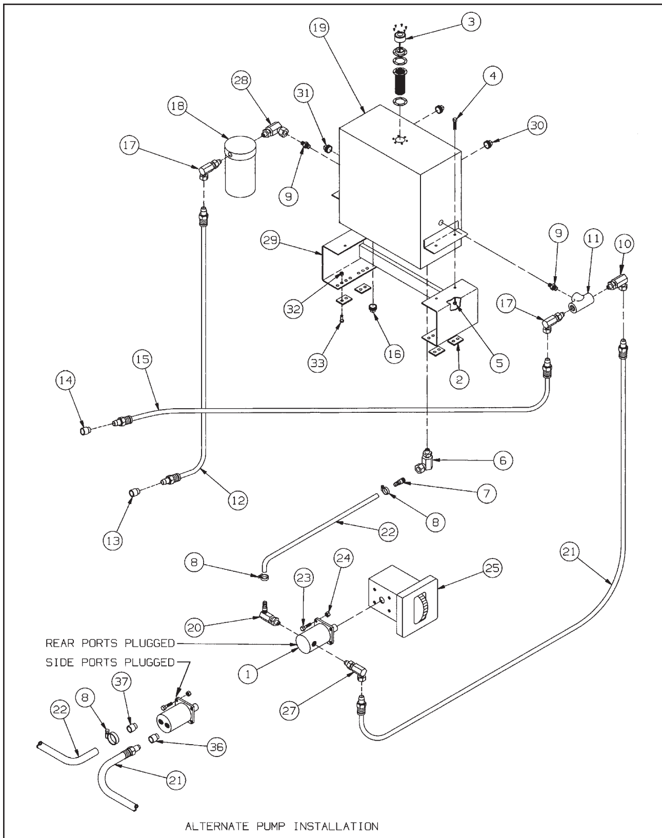
Figure 1-7 Wet Kit Assembly
