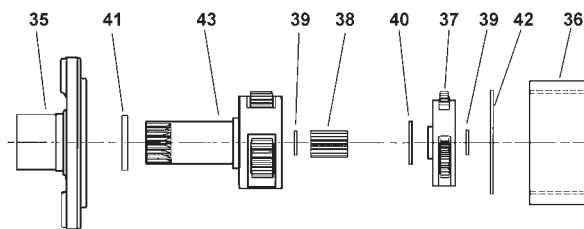
GEAR END INSTALLATION
