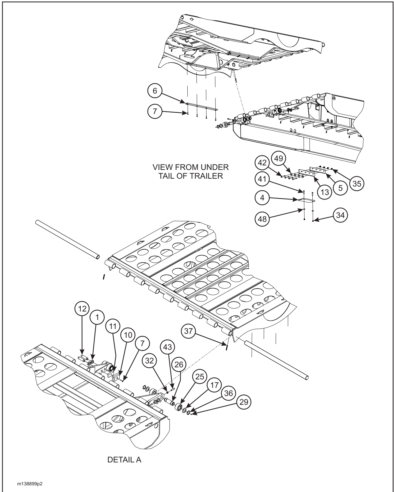
Figure 1-3 Frame Assembly (2 of 2)
