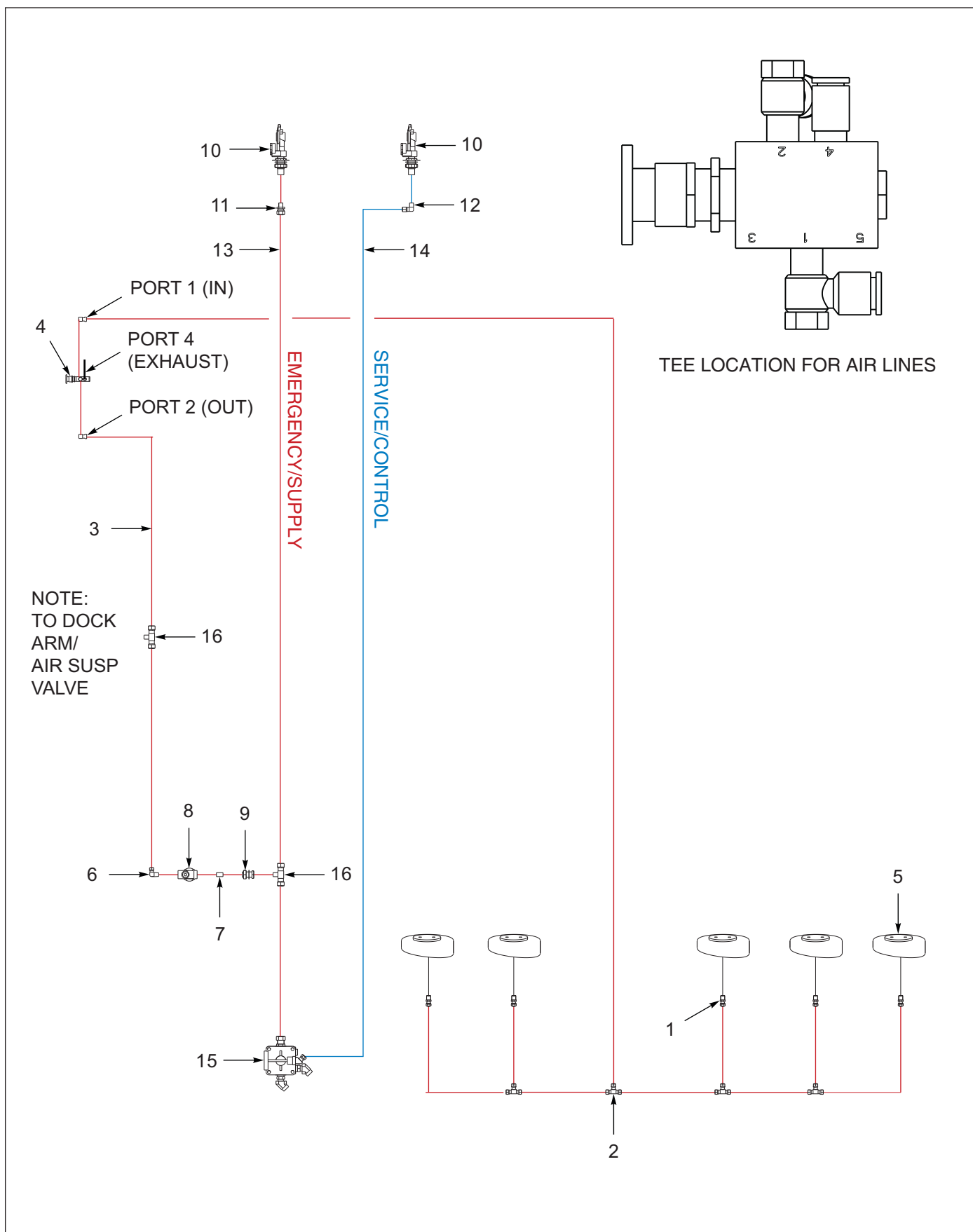
Figure 1-130: Ramp Assembly, Air System 6FT 930
