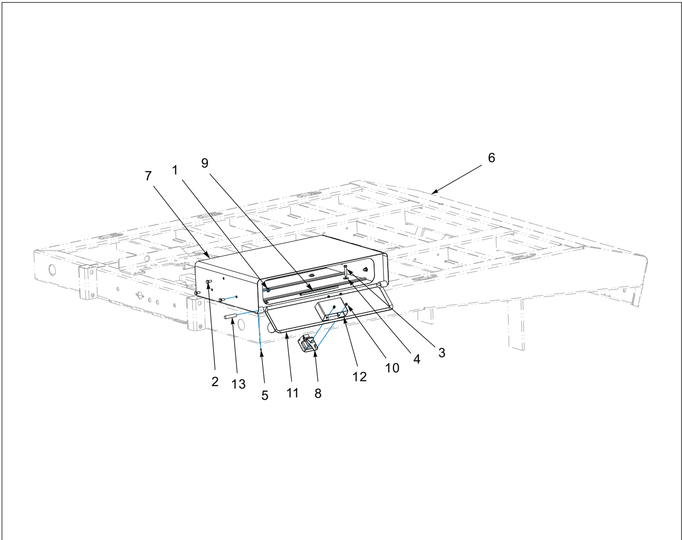
Figure 1-145: Toolbox Assembly-Upper Deck
