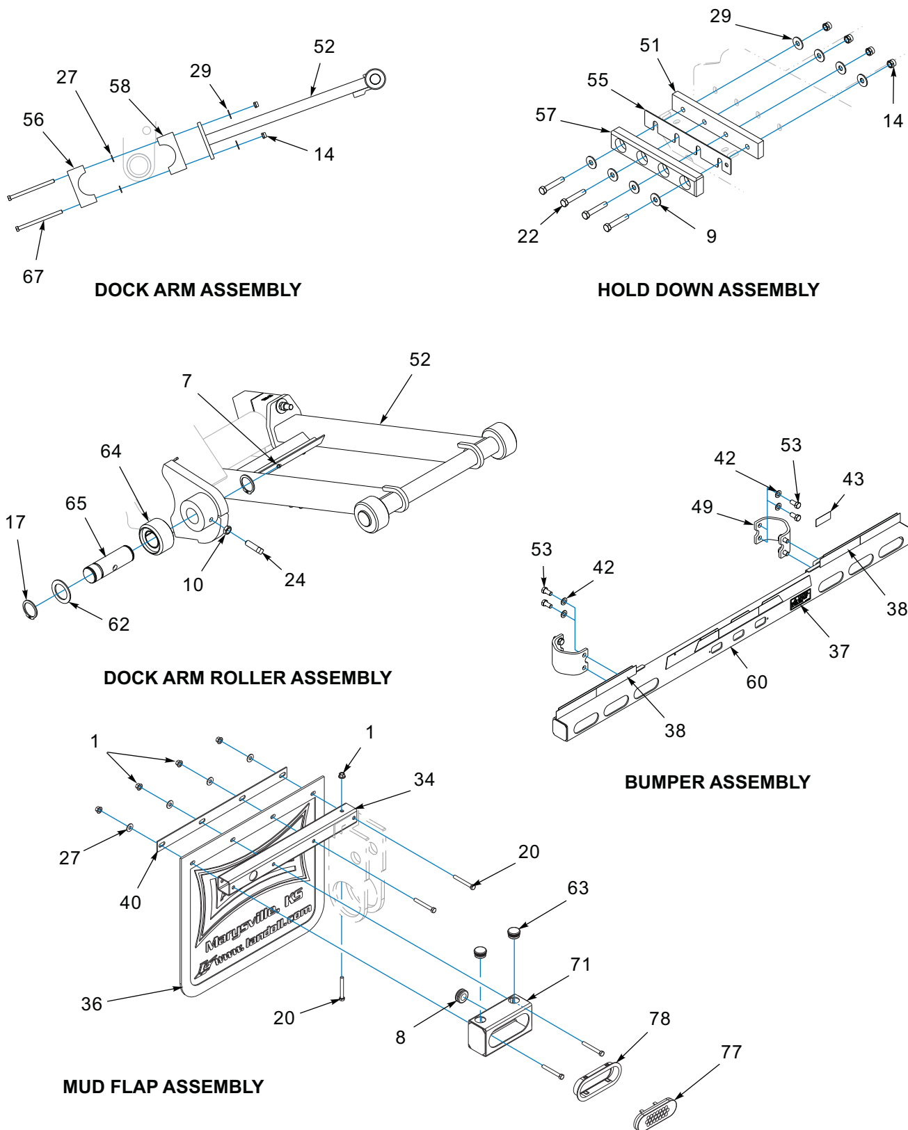
Figure 1-31: General Items - 950E (3 of 3)
