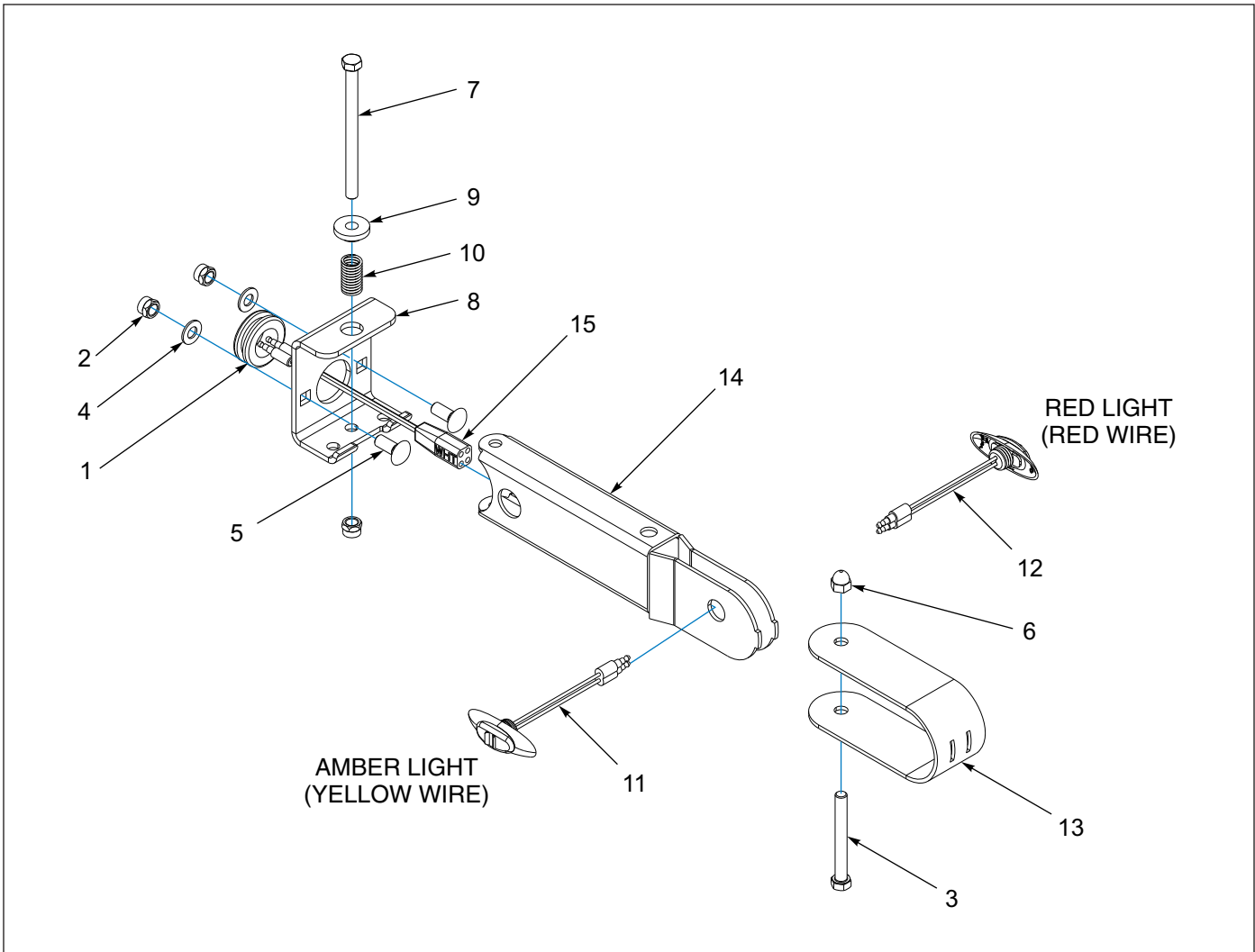
Figure 1-122: Swing-Arm Light Assembly - STREET
