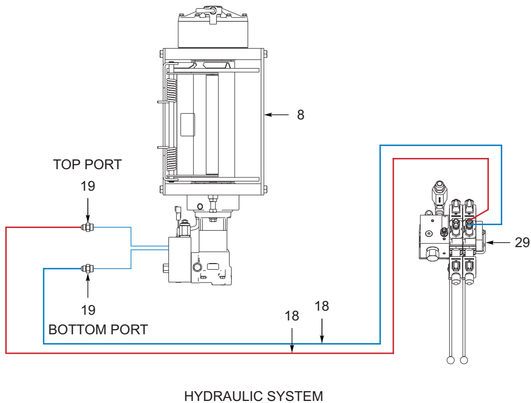
Figure 1-78: Winch Installation-20K 2 Speed (Warn) (1 of 2)
