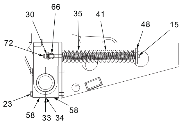
TAIL ASSEMBLY
