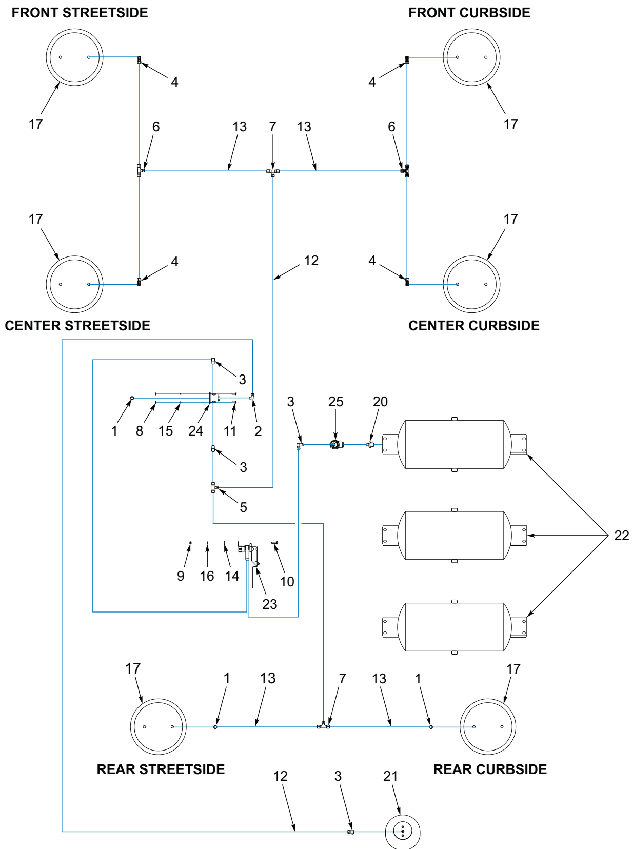
Figure 1-43: 950E-Air Ride Suspension
