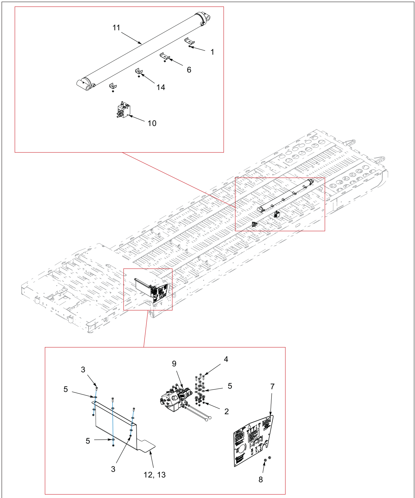
Figure 1-12: General Assembly - Hydraulic, Electric, Air
