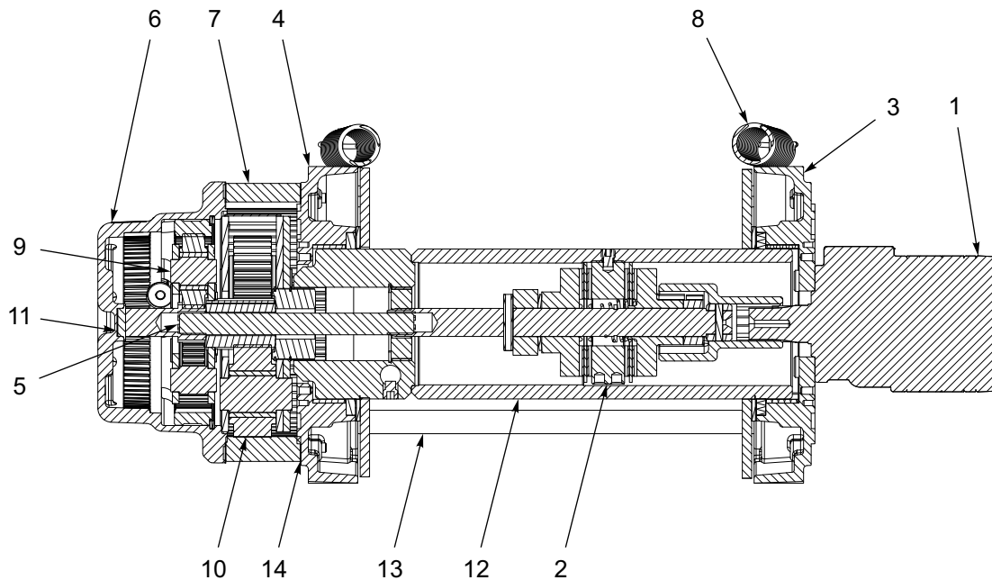
Figure 1-77: Winch Items - 12K (WARN)
