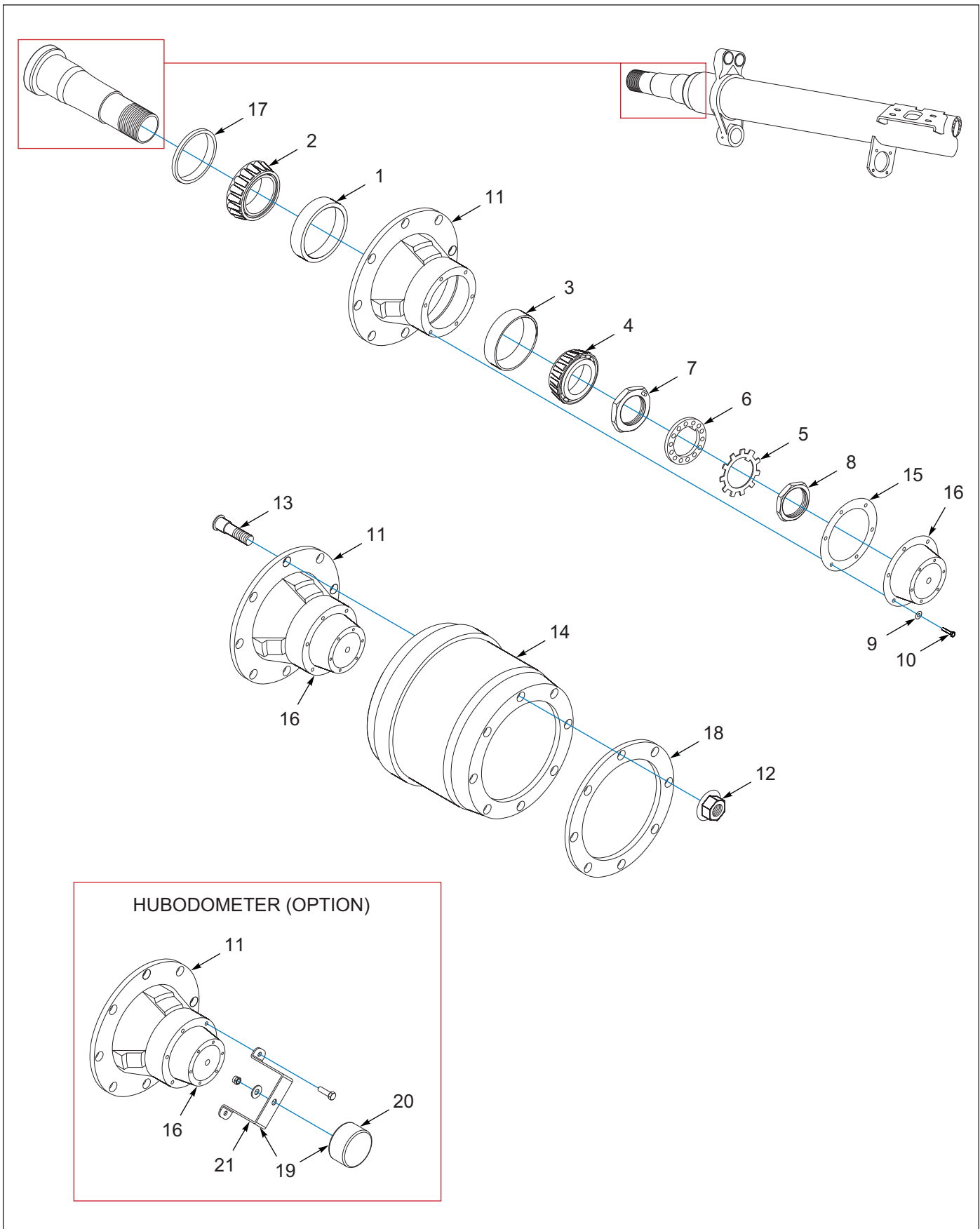
Figure 1-52: Axle 12.25 x 7.5 Drum and Hub Assembly, Dexter
