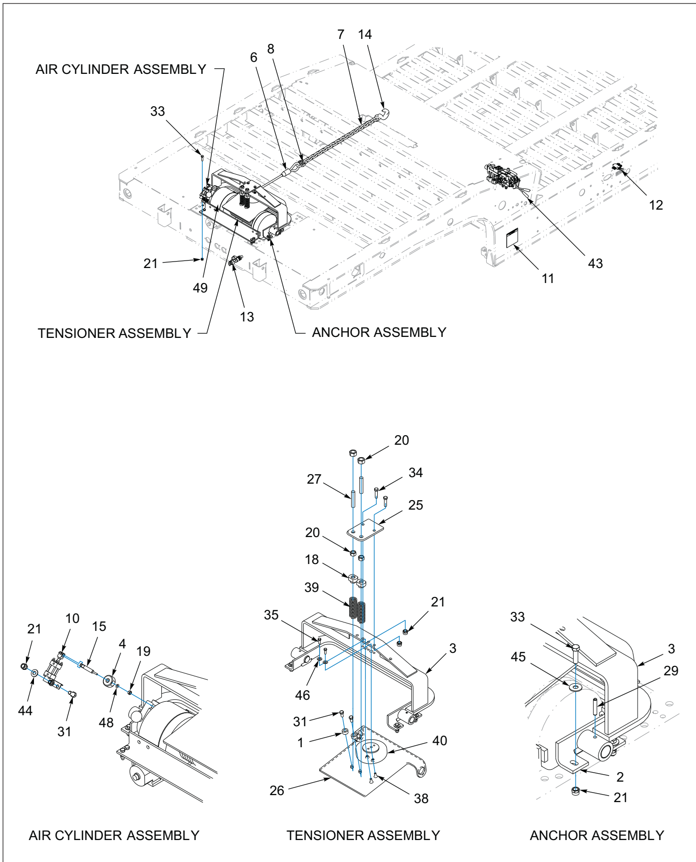
Figure 1-70: 20K Air Tension/Release (BRADEN) (1 of 3)
