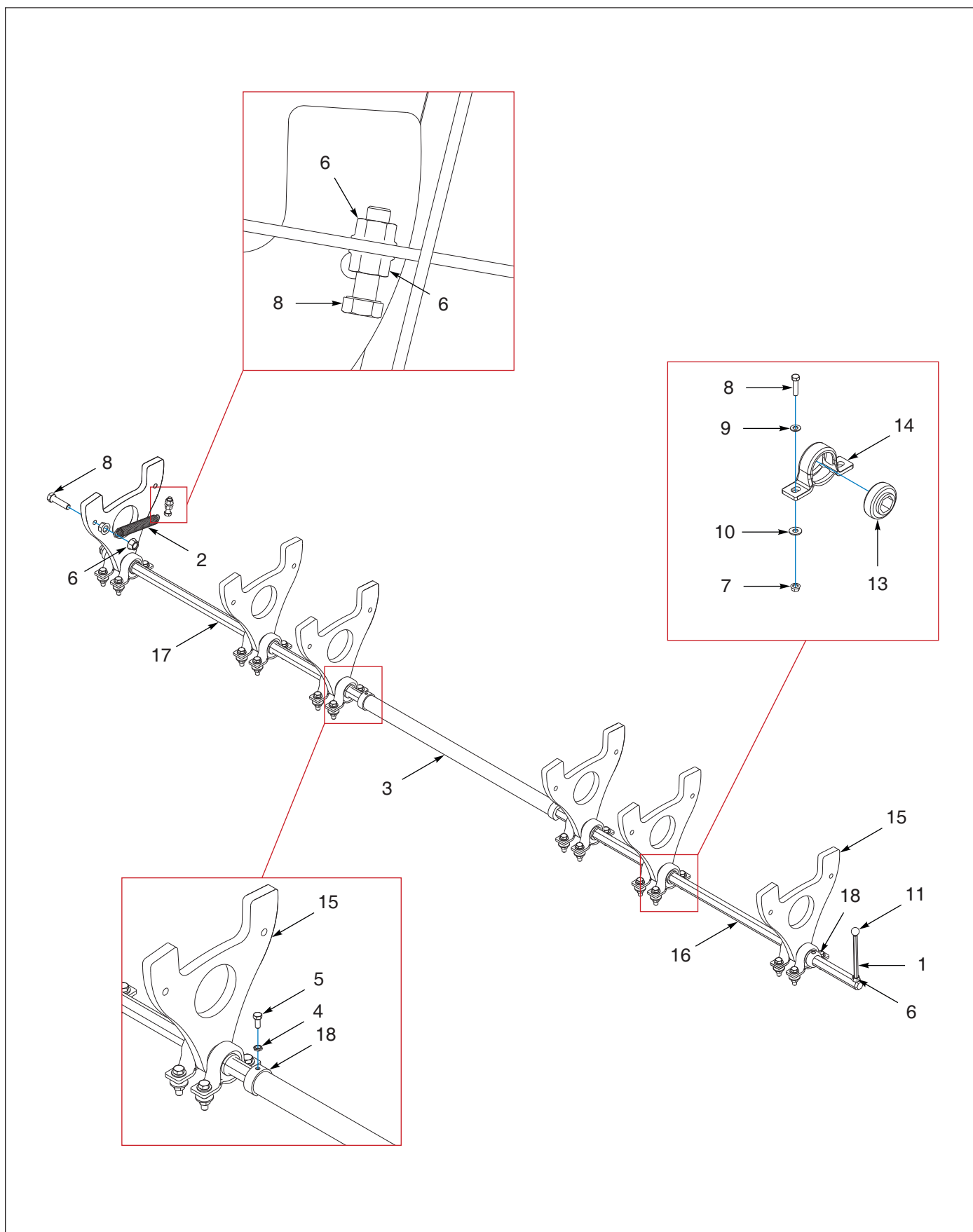
Figure 1-129: Ramp Assembly, Air 6FT 930 Support
