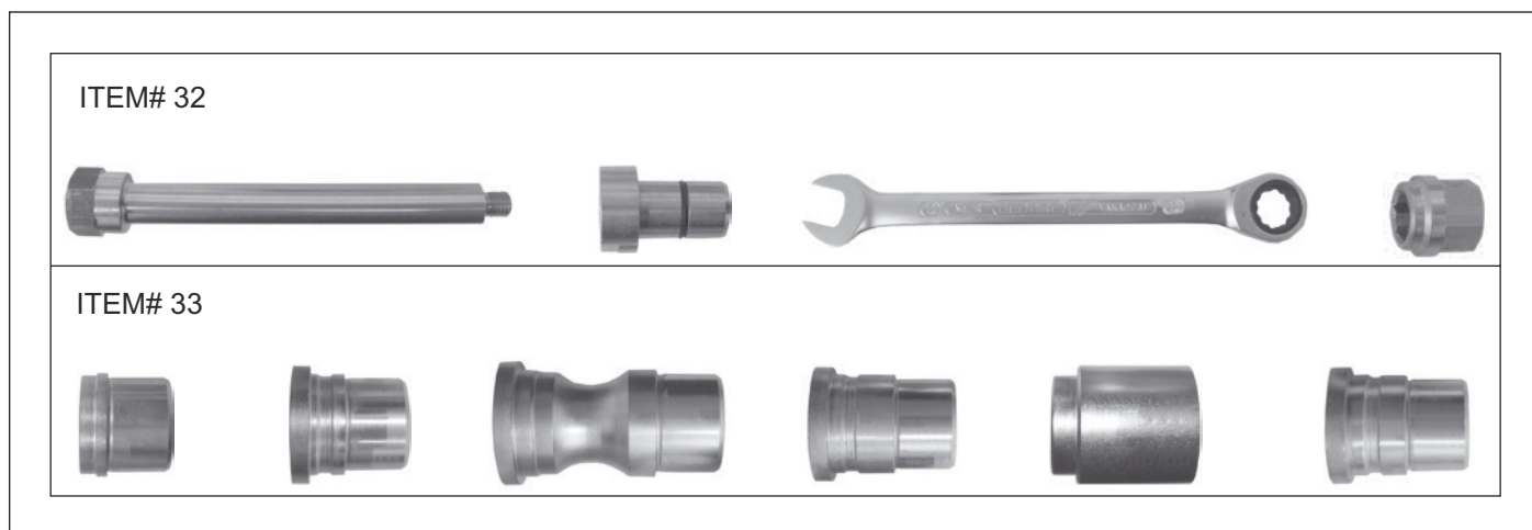
Figure 1-54: Axle 16.5 Disc Brakes &amp; Hub Assembly, Dexter (OPTION) (2 of 2)
