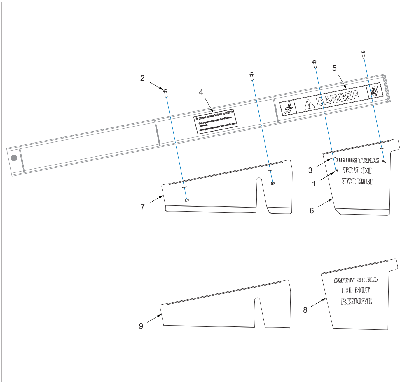
Figure 1-131: Safety Shield Assembly, Ramp
