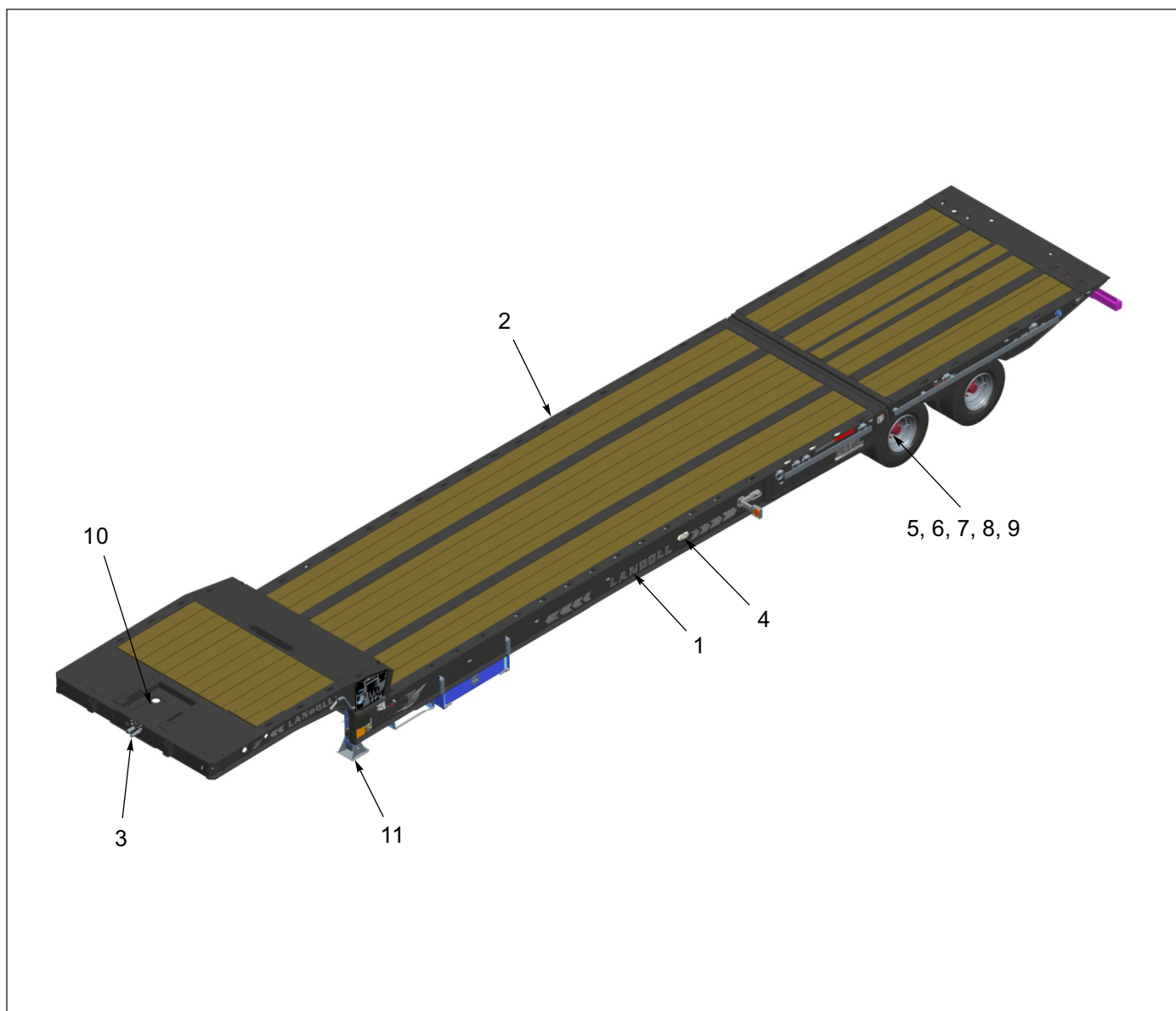
Figure 1-2: General Assembly
