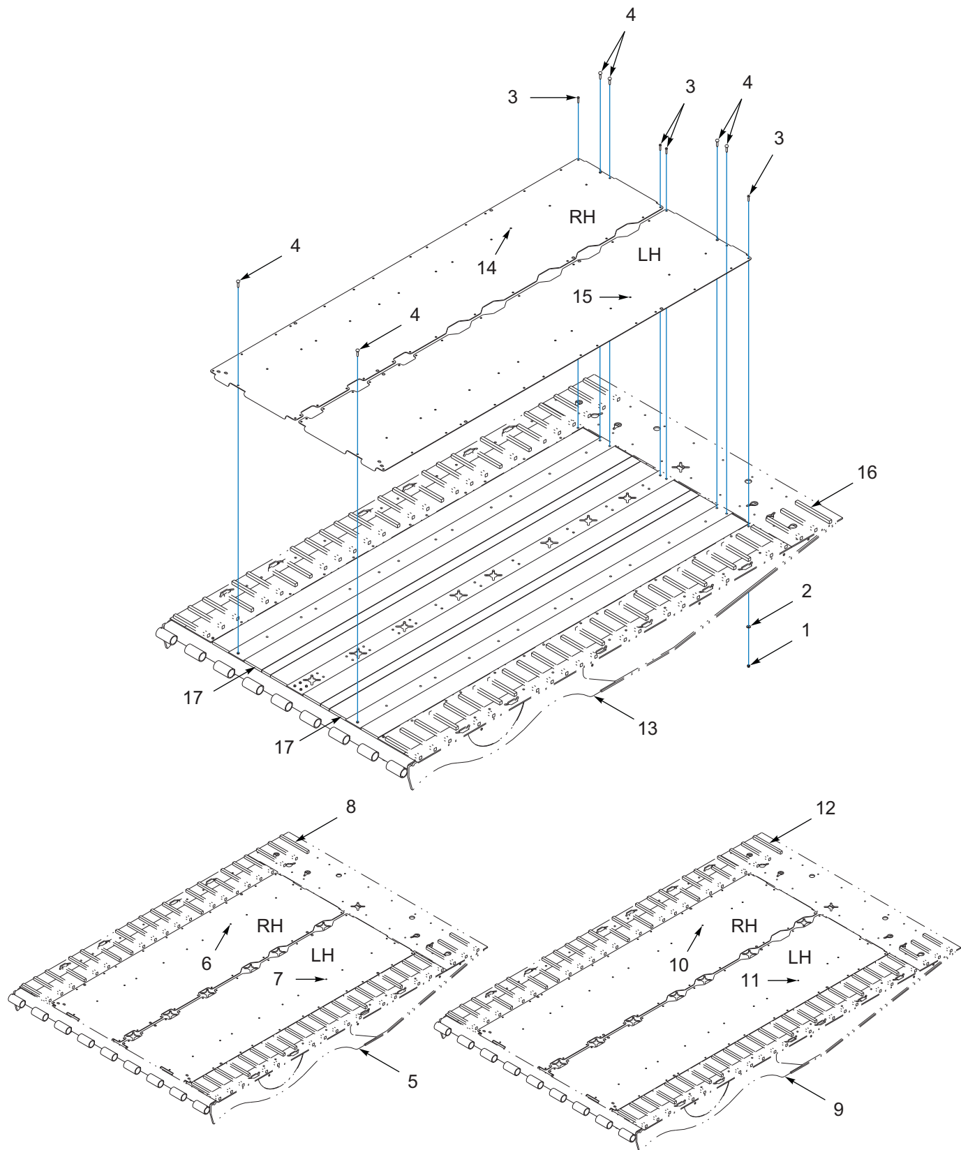
Figure 1-95: Tail Tread Grip-223036
