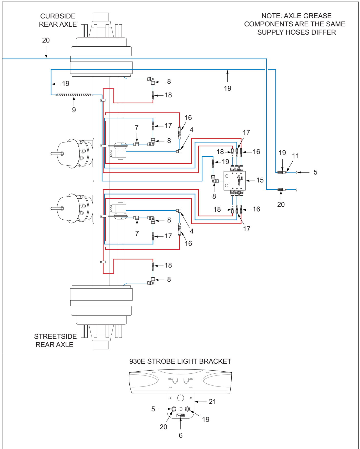
Figure 1-35: Grease System, 2 Axle (After 08/31/2020) (2 of 3)
