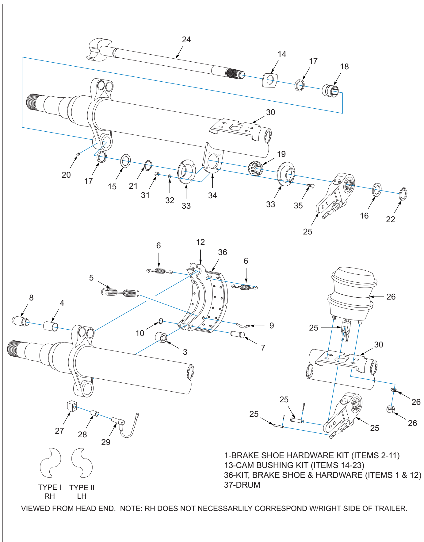
Figure 1-51: Axle 12.25 x 7.5 Drum Brakes, Dexter
