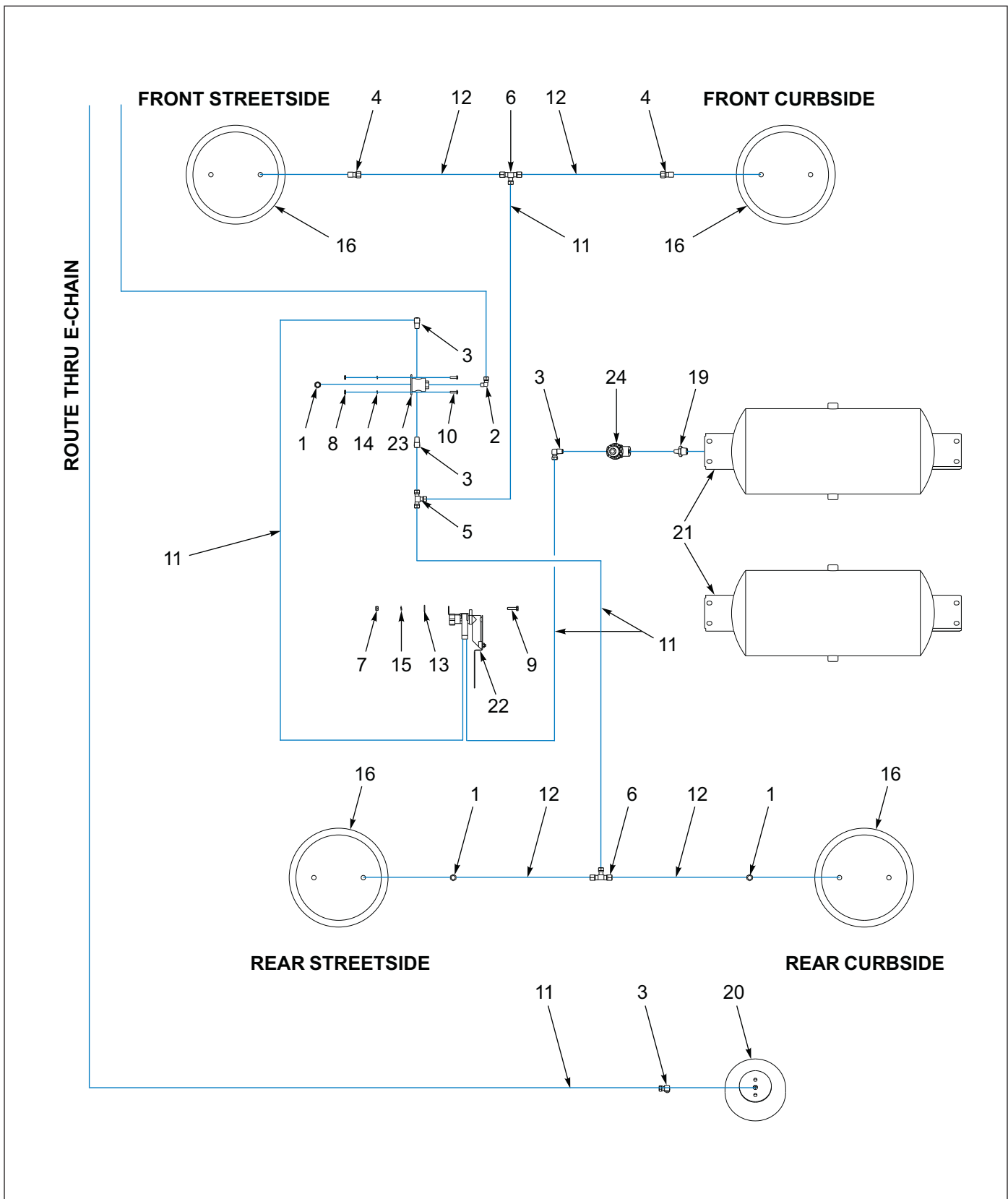
Figure 1-42: 930E-Air Ride Suspension
