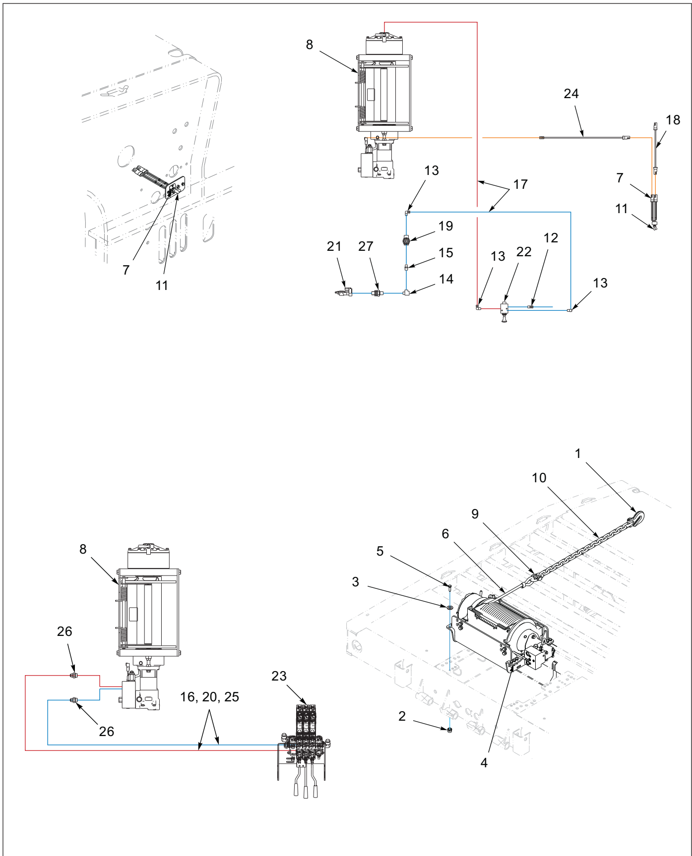
Figure 1-81: Winch Installation - 30K 2 Speed (WARN)
