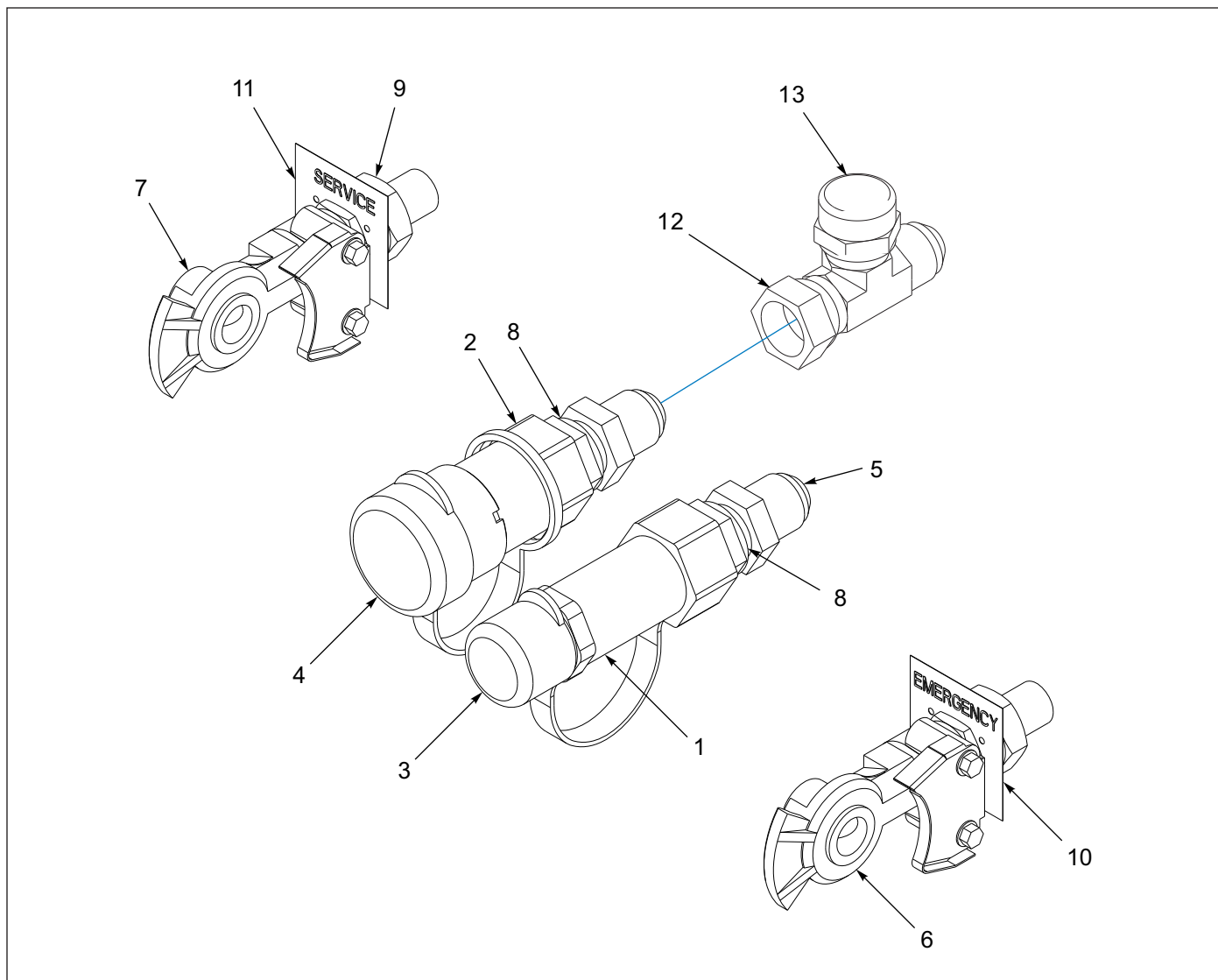
Figure 1-22: Connectors - Front Sub Assembly
