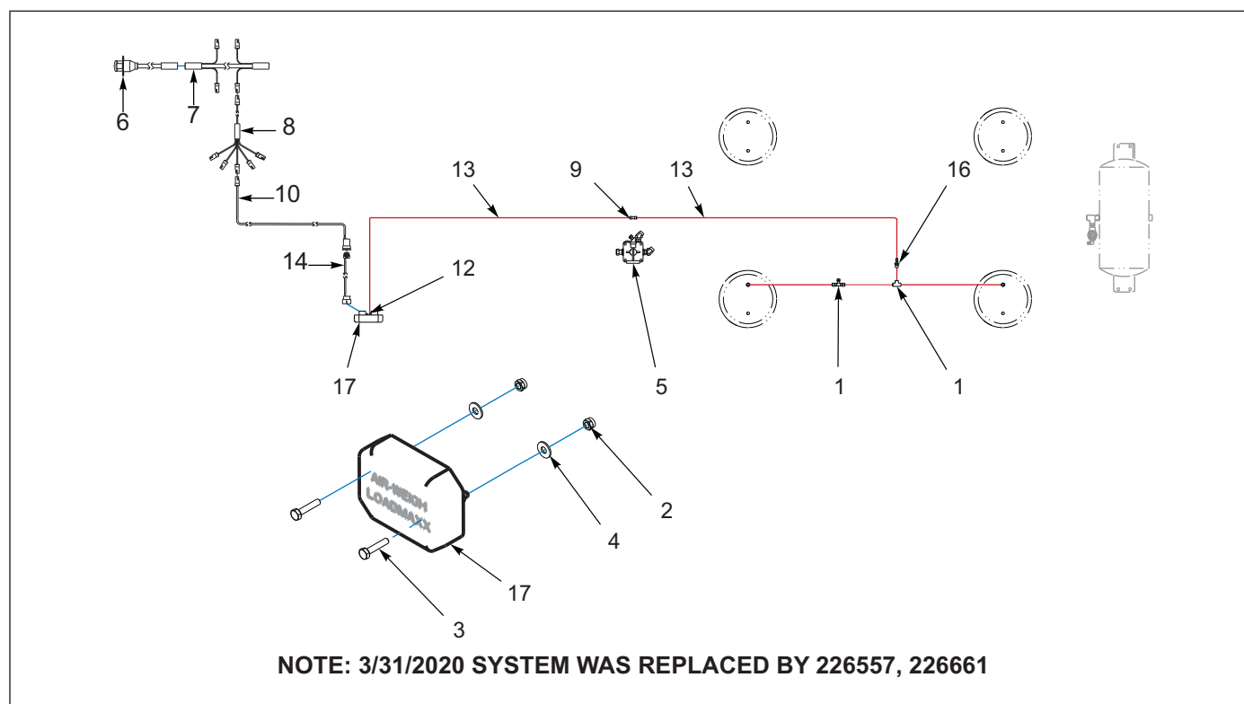
Figure 1-132: Loadmaxx (BEFORE 3/31/2020)
