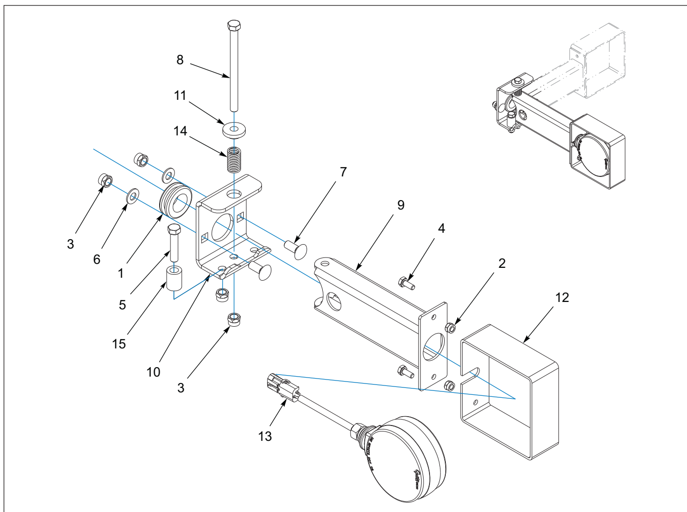
Figure 1-120: Swing-Arm Light Assembly - Turn Signal/Emergency Flasher
