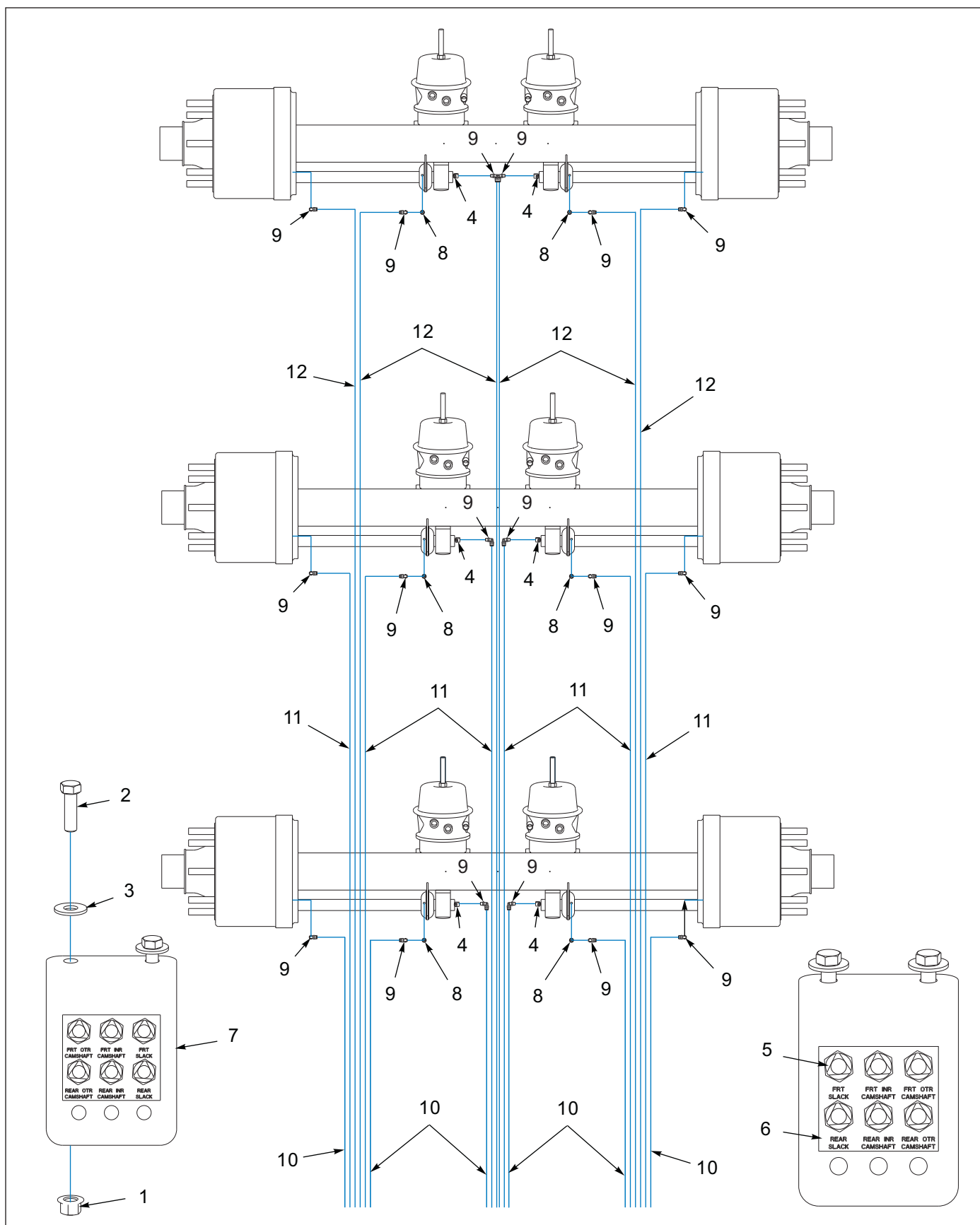
Figure 1-37: Grease System, 3 Axle (Before 11/07/2018)
