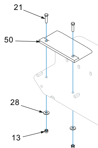
GLIDE ASSEMBLY
