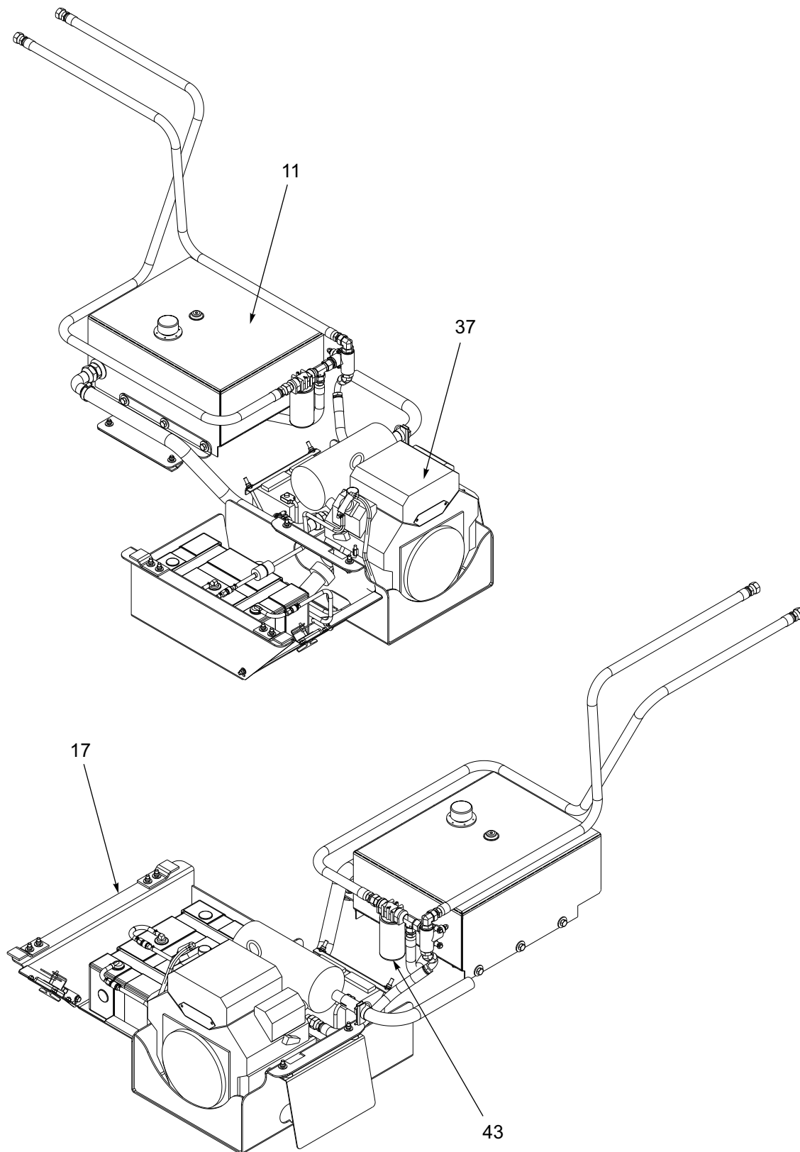
Figure 1-105: 25 HP Slope Package (1 of 4)
