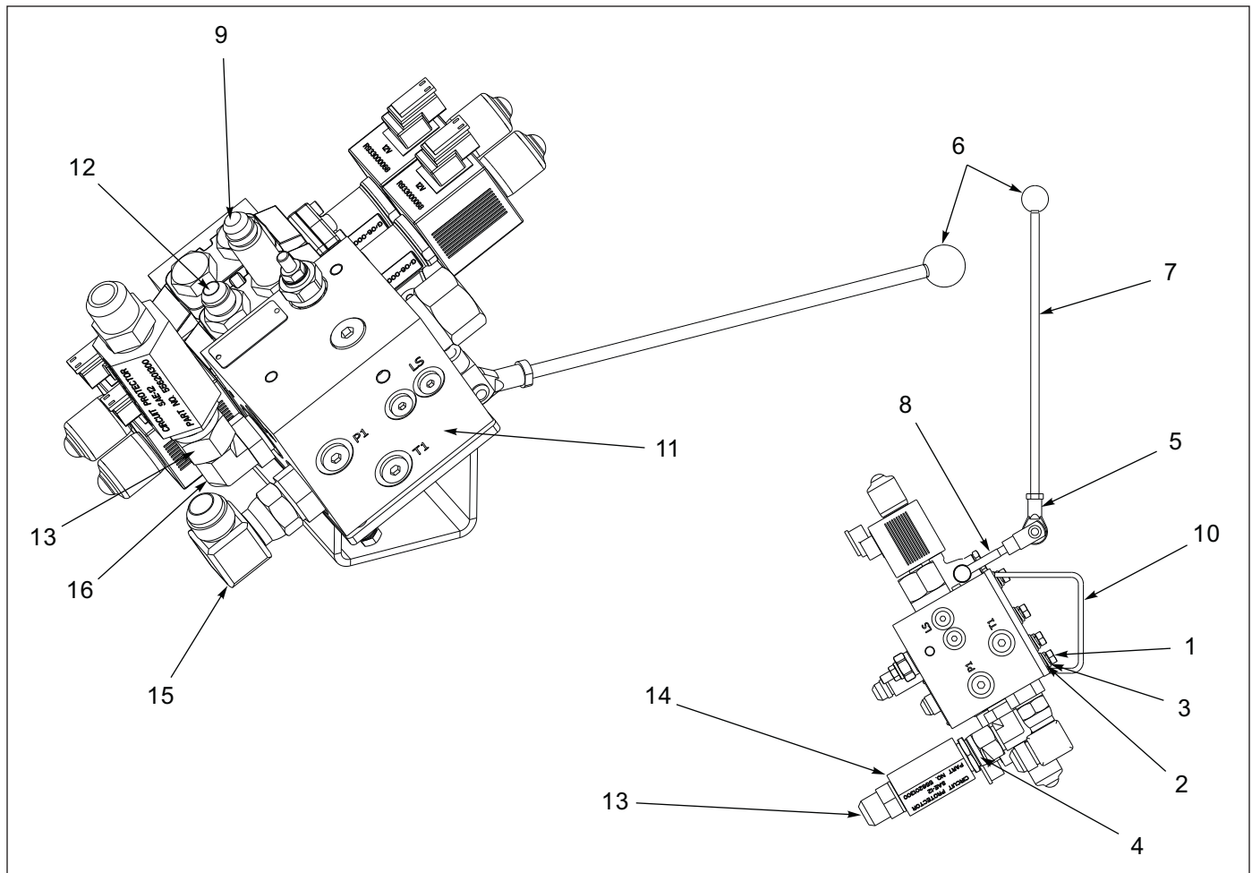
Figure 1-24: Valve Assembly - 2 Spool Control
