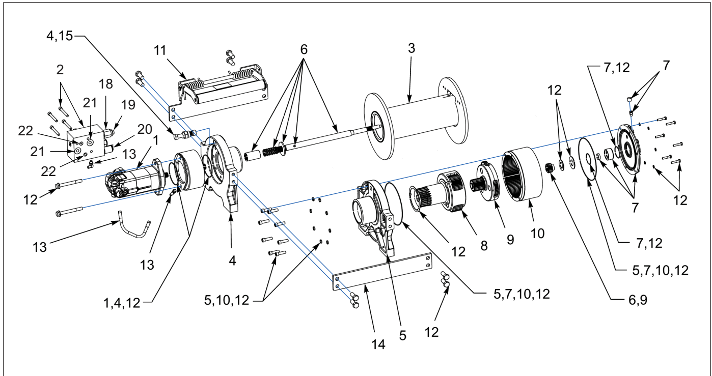
Figure 1-80: Winch Items - 20K 2 Speed (WARN)
