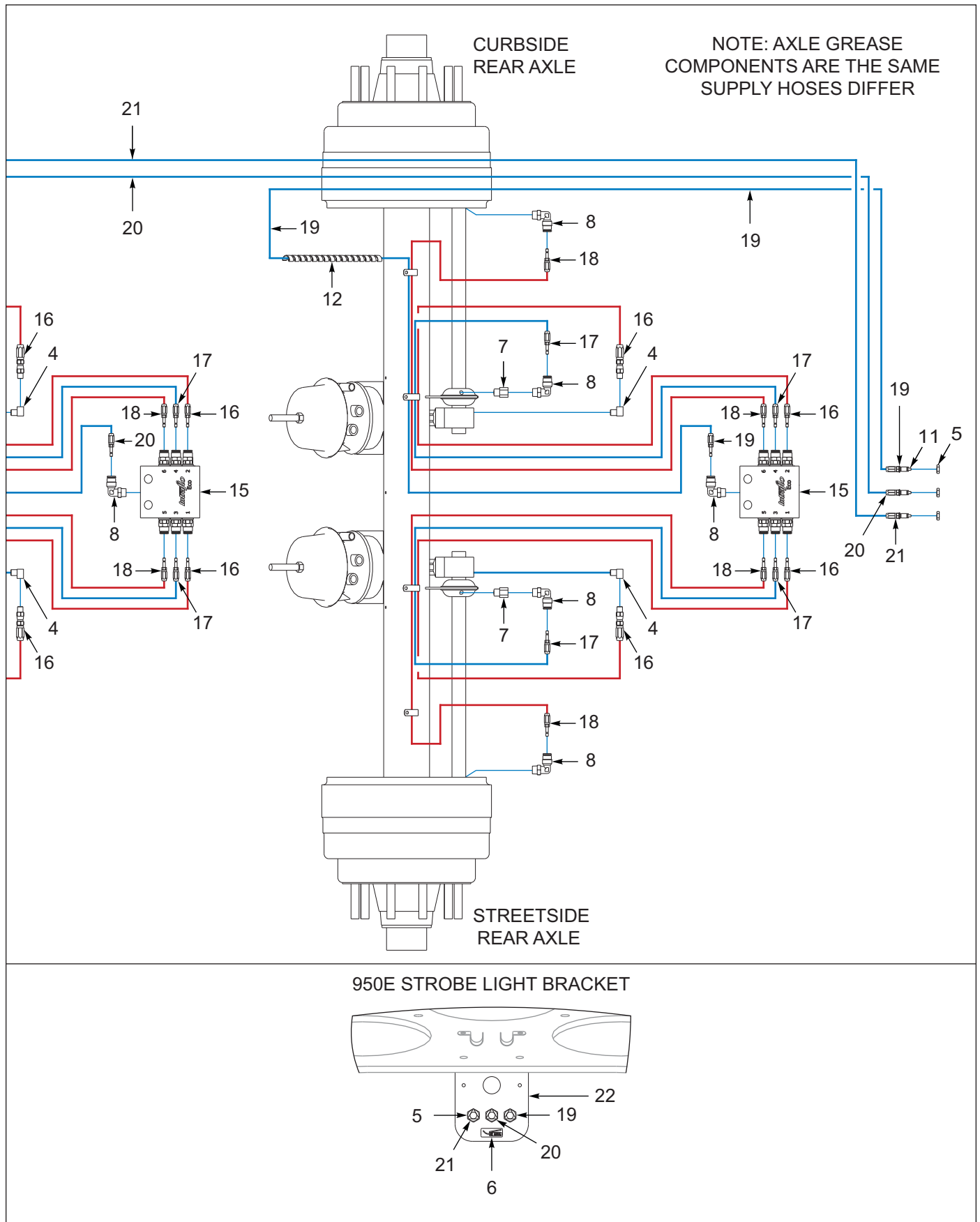
Figure 1-40: Grease System, 3 Axle (After 08/31/2020) (2 of 3)
