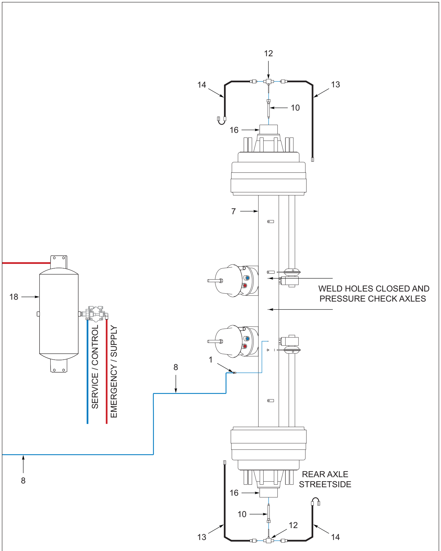
Figure 1-62: Thermalert, 2 Axle Air System (OPTION) (2 of 2)
