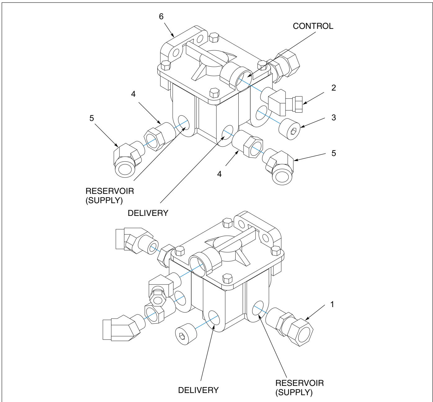
Figure 1-23: Valve Assembly - Air Booster
