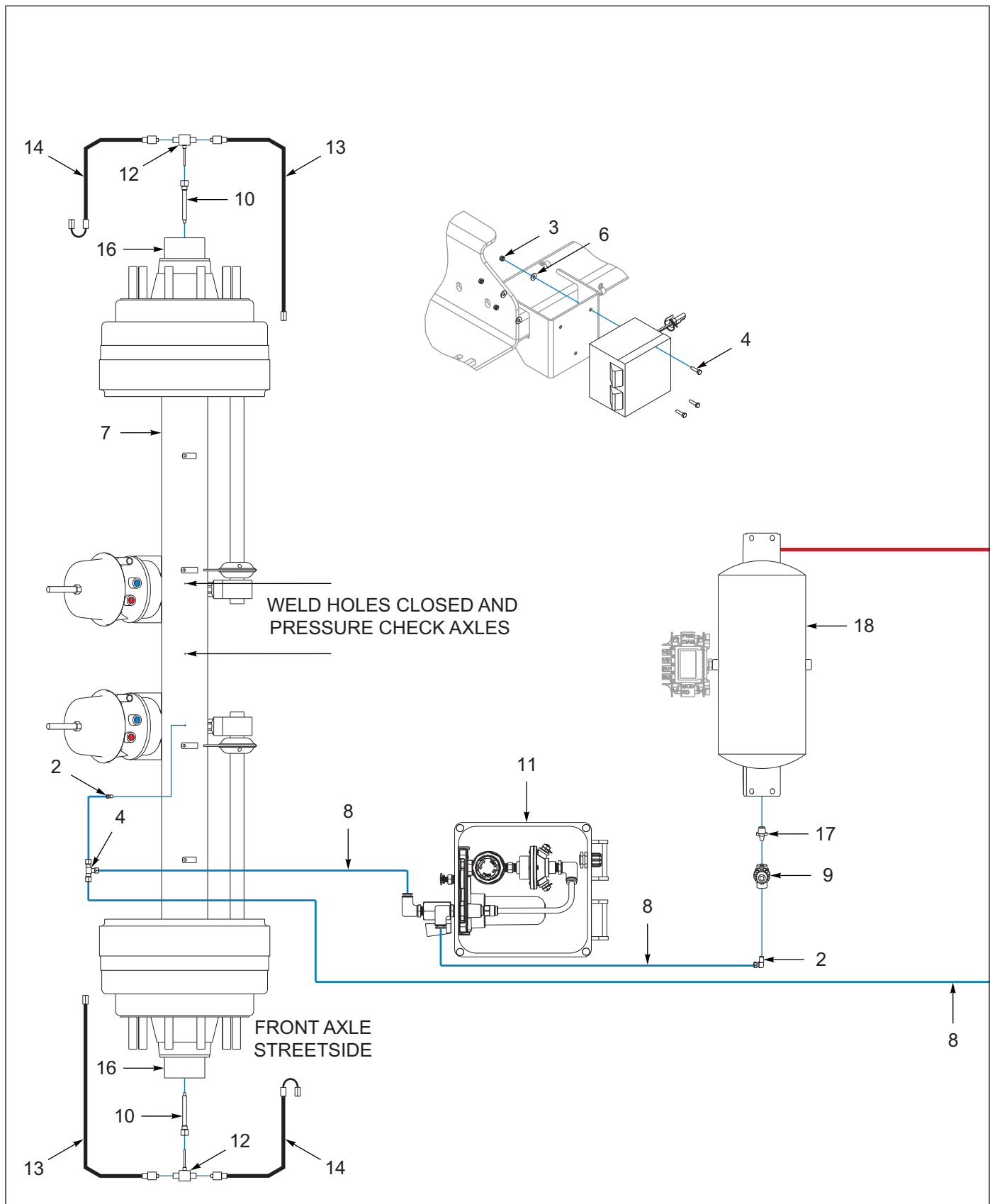
Figure 1-61: Thermalert, 2 Axle Air System (OPTION) (1 of 2)
