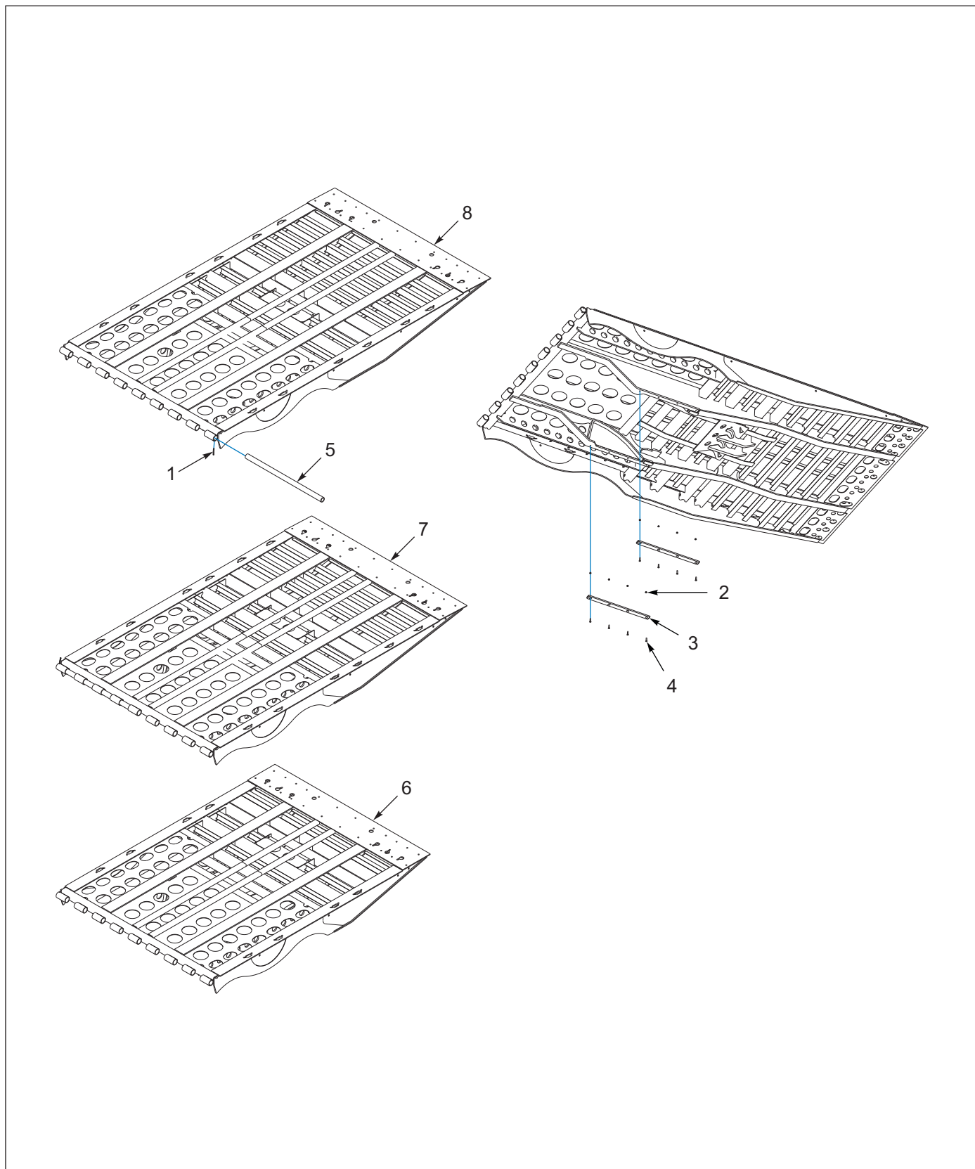
Figure 1-10: Tail Assembly, WO/Center Gotcha Plate
