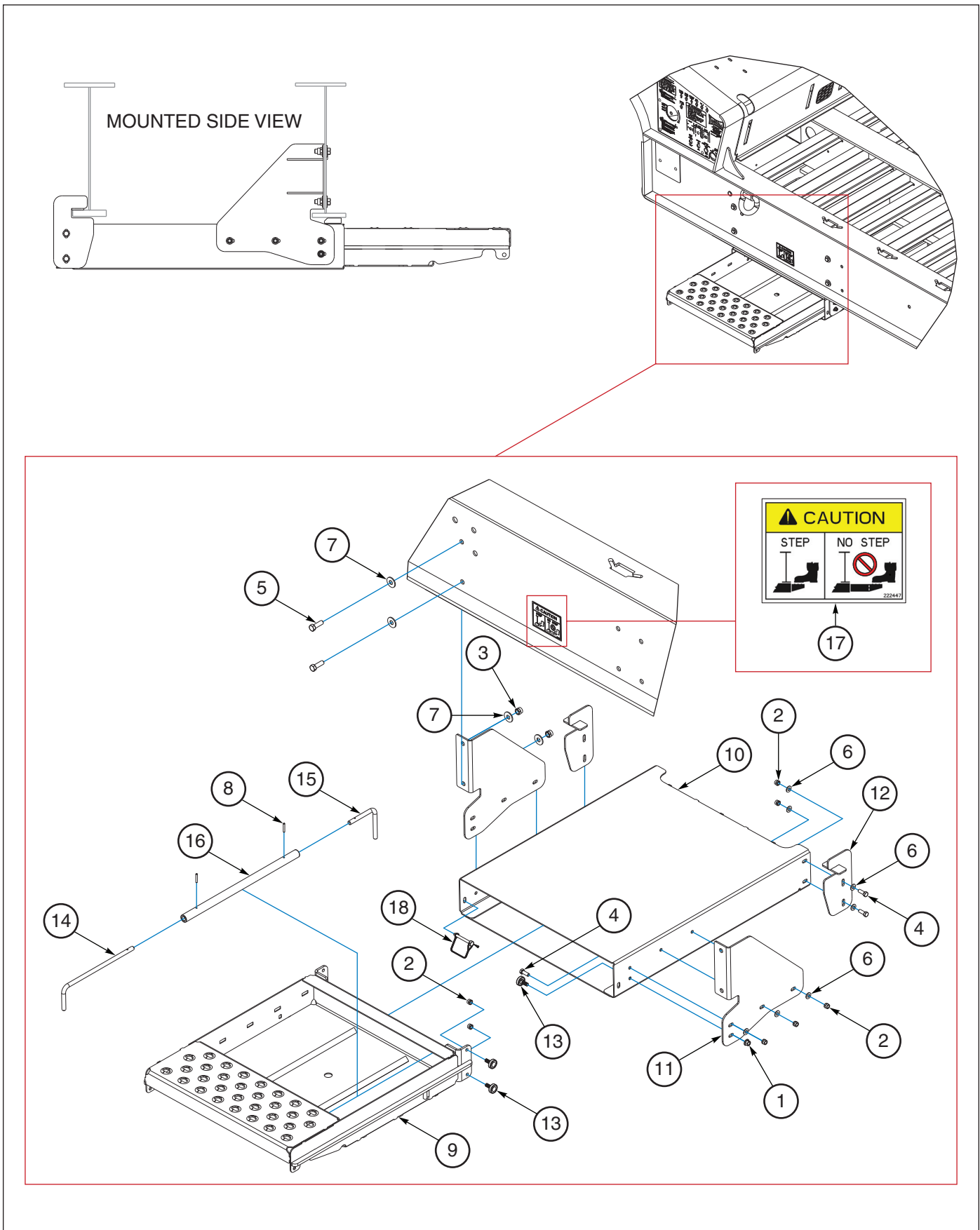
Figure 1-141: Step Drawer, Retractable Assembly
