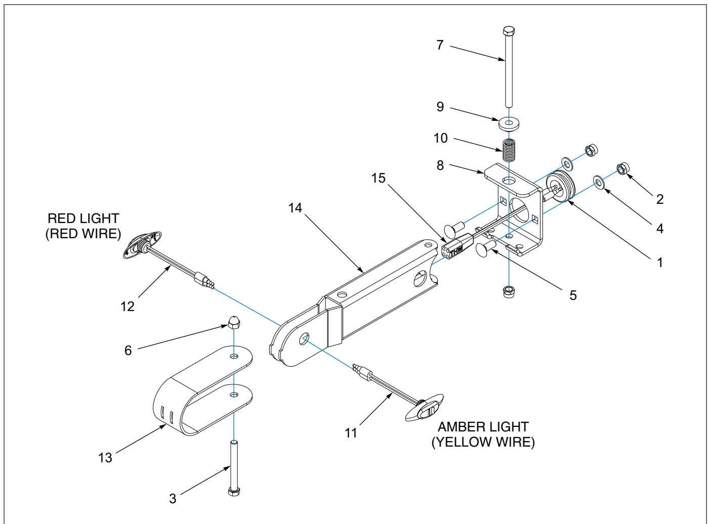
Figure 1-123: Swing-Arm Light Assembly - CURB
