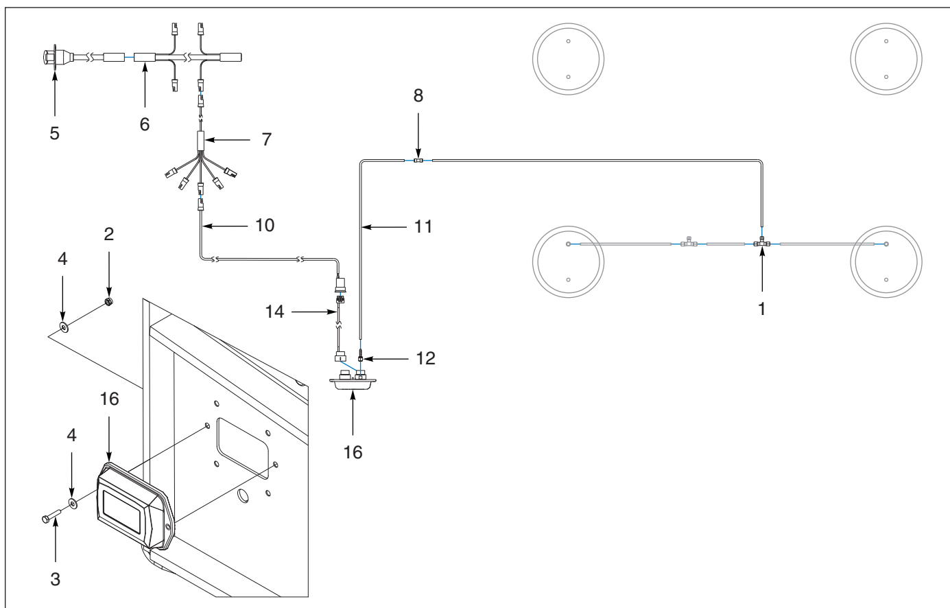
Figure 1-134: Loadmaxx Plus (AFTER 3/31/2020)
