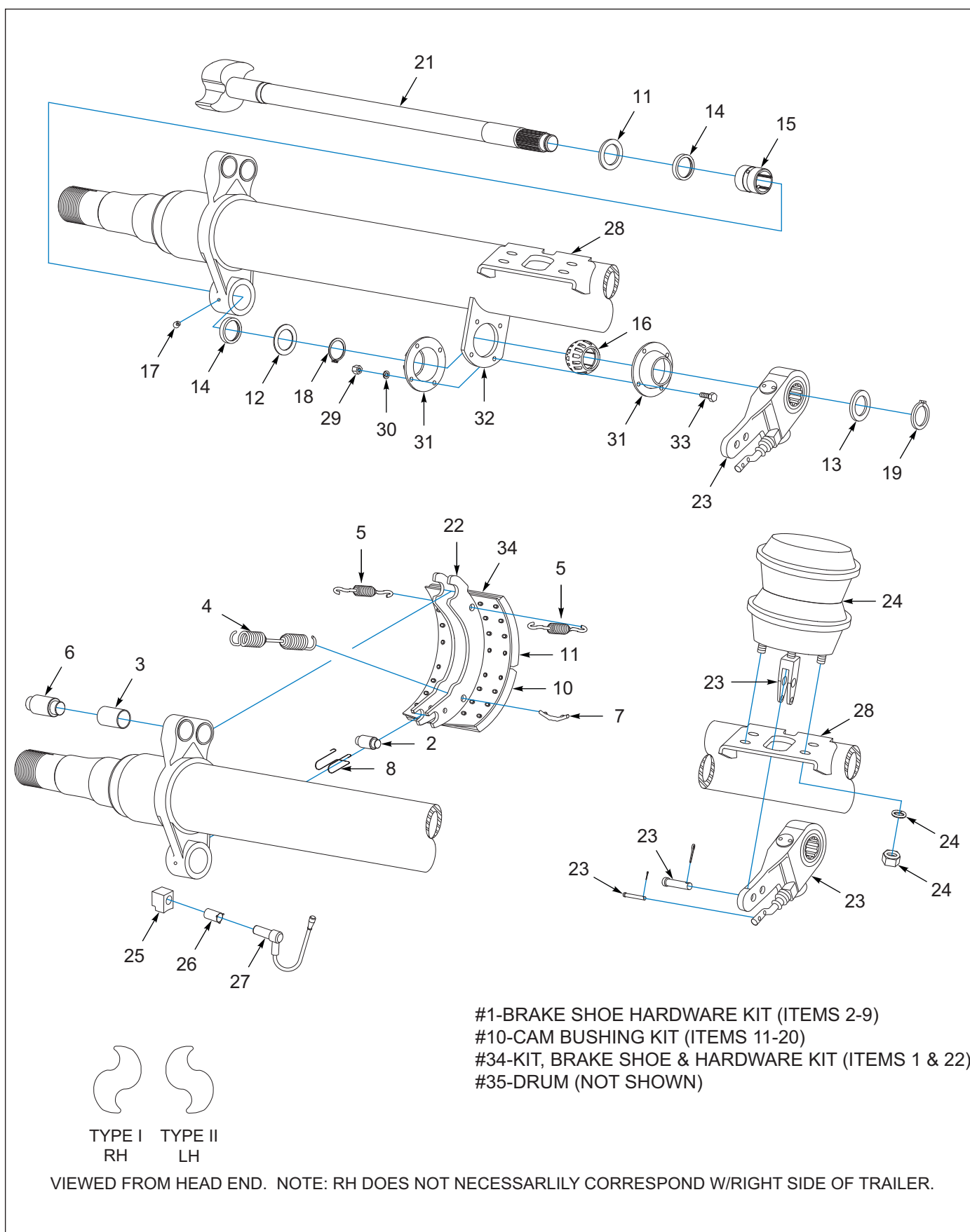
Figure 1-55: Axle 16.5 x 7 Drum Brakes, Dexter
