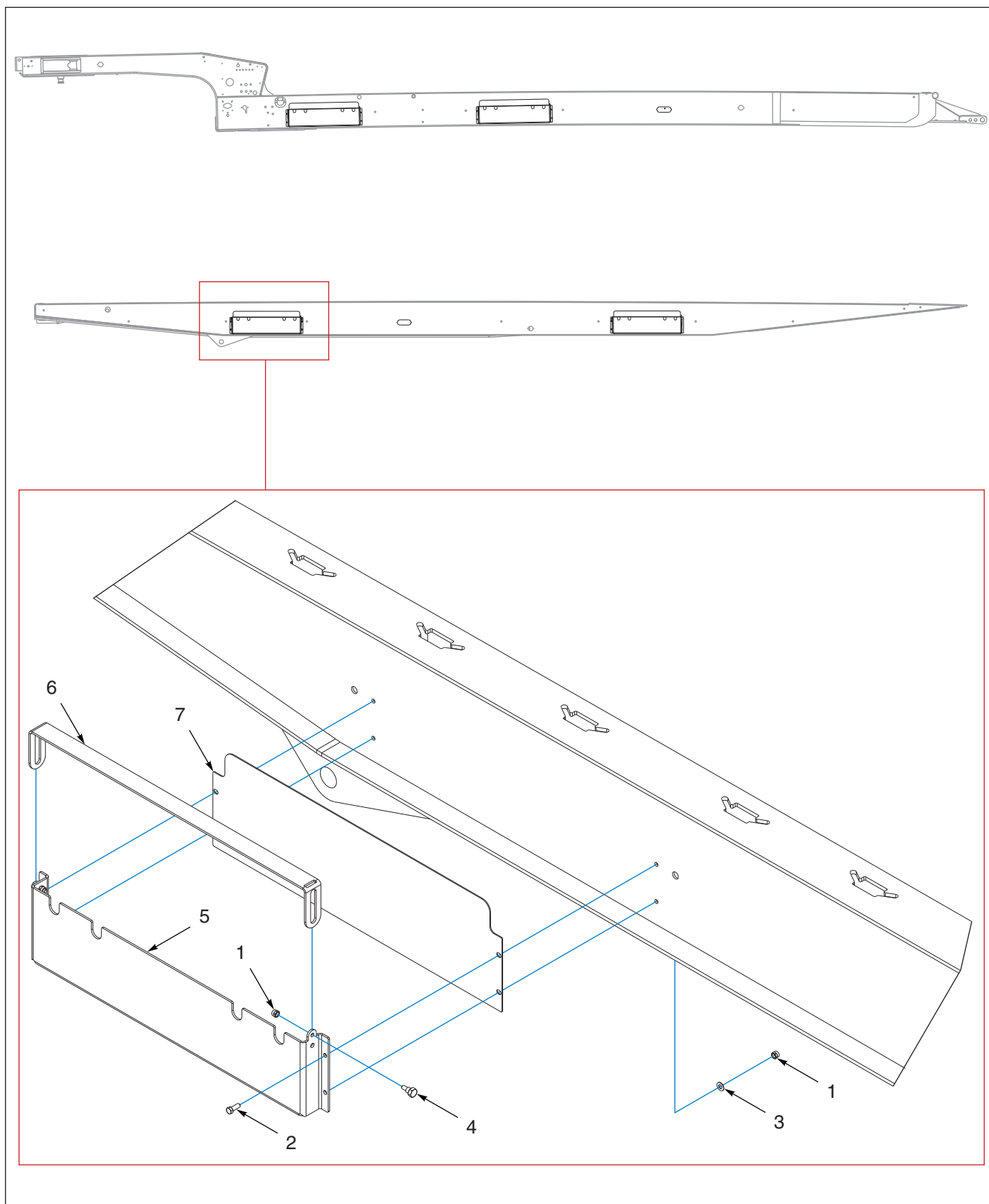
Figure 1-142: Chain Tray Assembly
