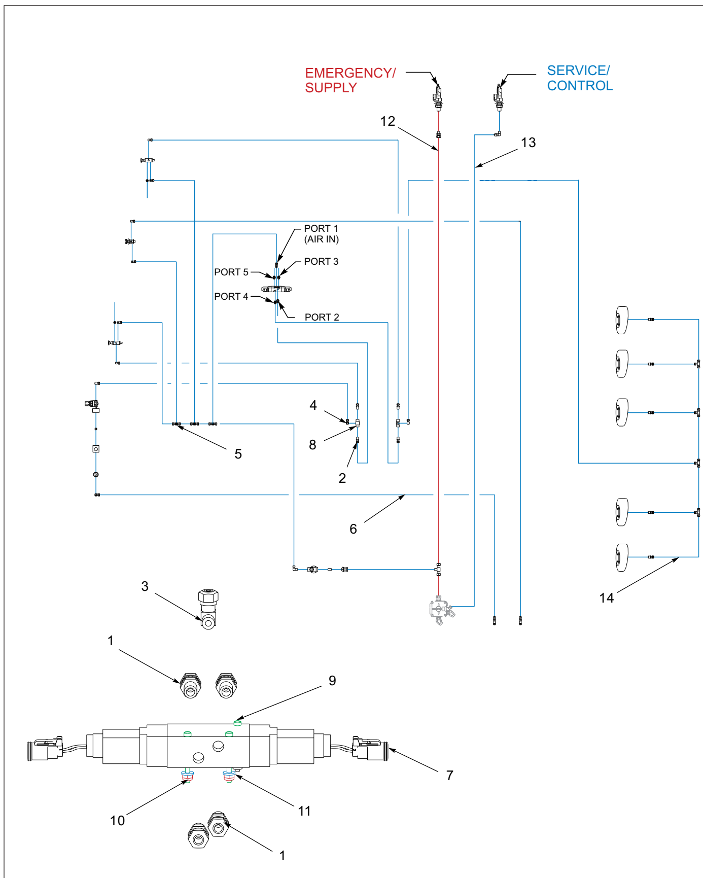
Figure 1-17: Dock & Ramp Remote Air System
