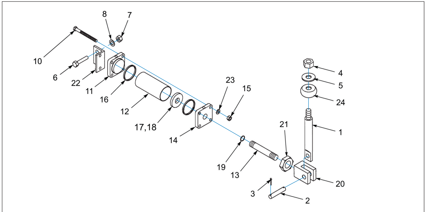
Figure 1-74: Winch - Air Shift Cylinder
