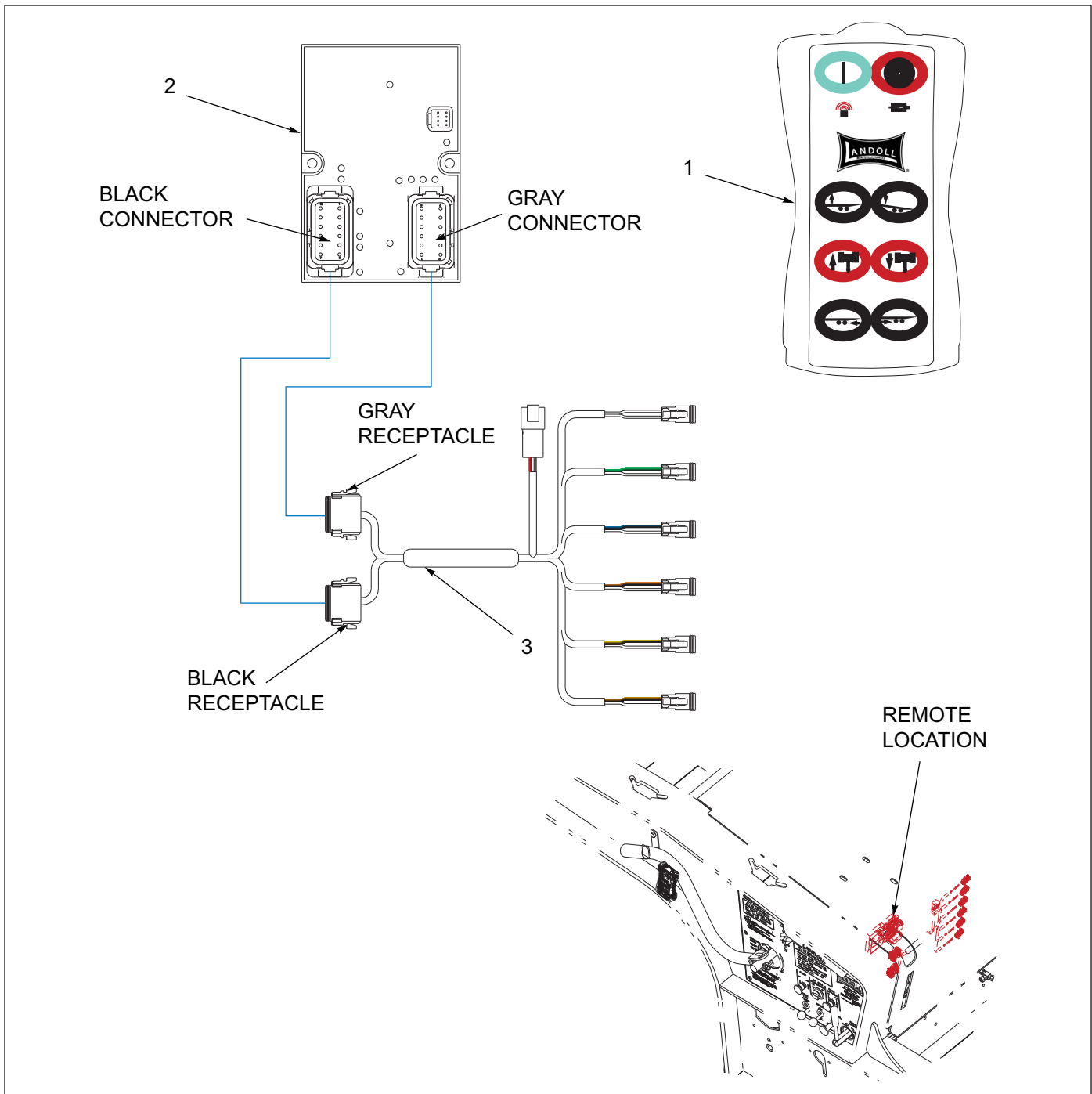
Figure 1-100: Remote - Brand 6-Function
