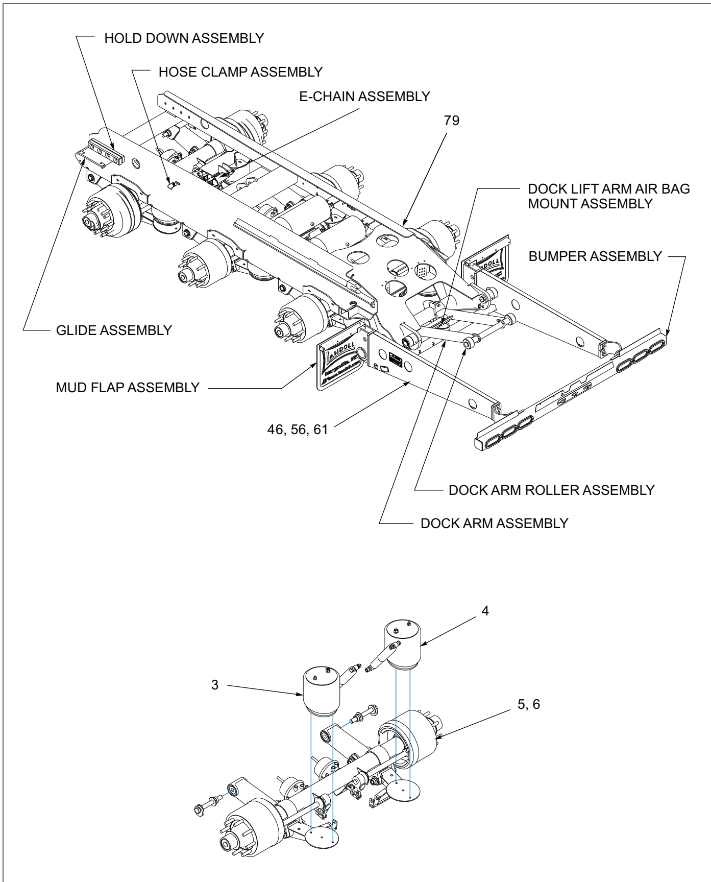
Figure 1-29: General Items - 950E (1 of 3)
