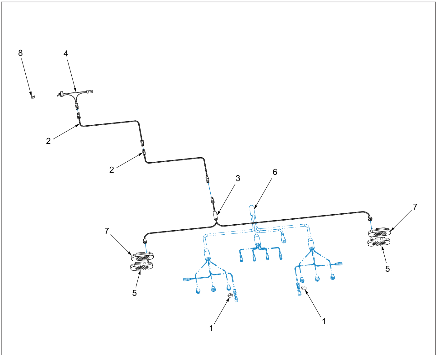
Figure 1-91: Strobe Installation
