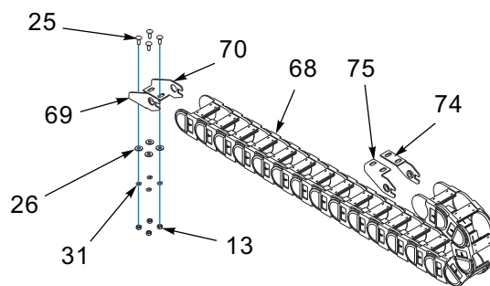
E-CHAIN ASSEMBLY
