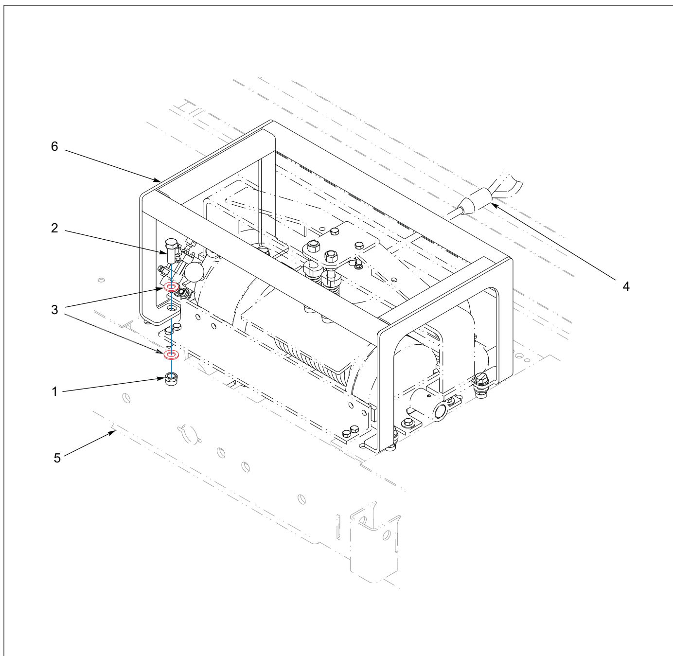
Figure 1-152: Guard Assembly, Pivot 20K
