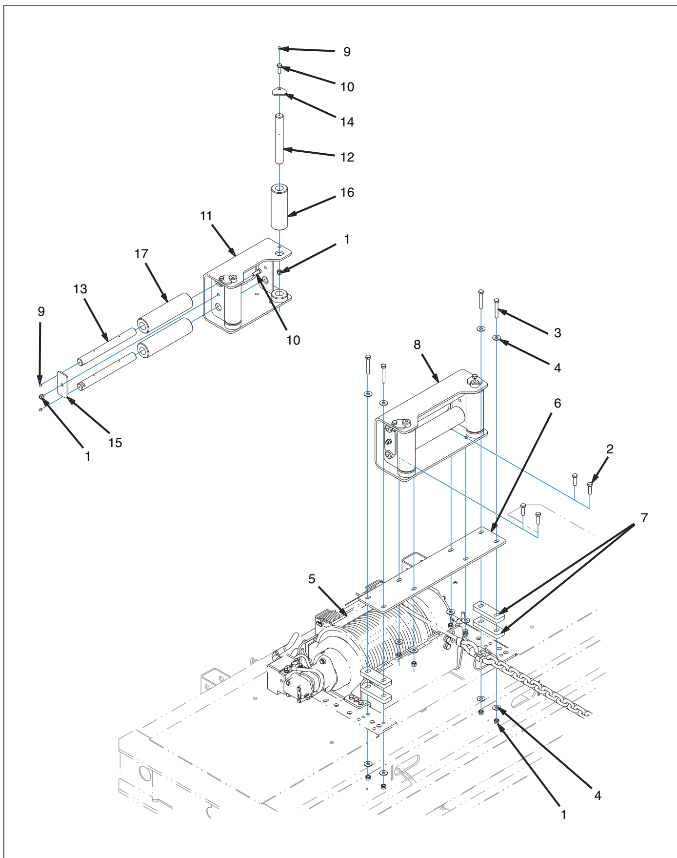
Figure 1-156: Guide Assembly, 4 Roller 20K/30K (WARN)
