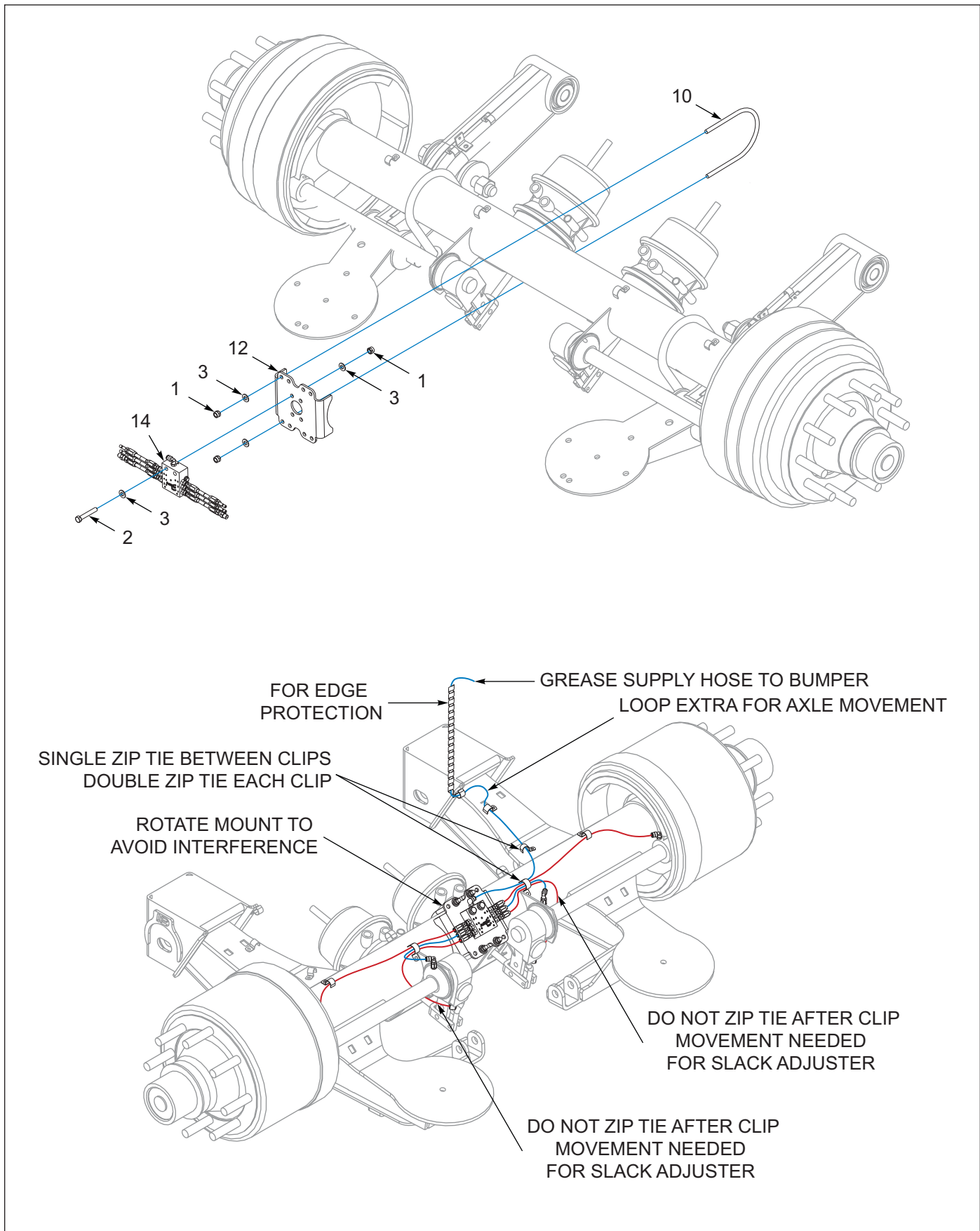
Figure 1-41: Grease System, 3 Axle (After 08/31/2020) (3 of 3)
