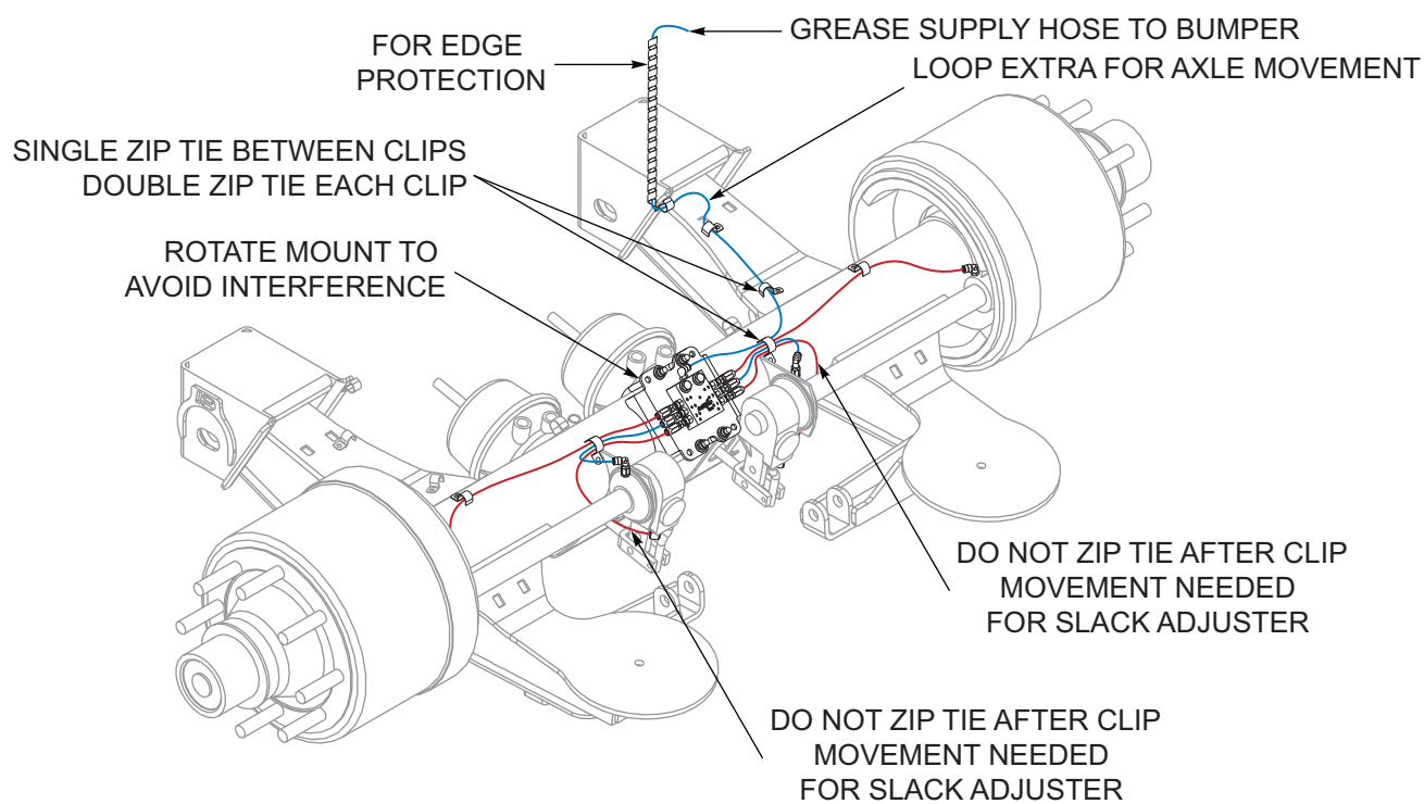
Figure 1-36: Grease System, 2 Axle (After 08/31/2020) (3 of 3)
