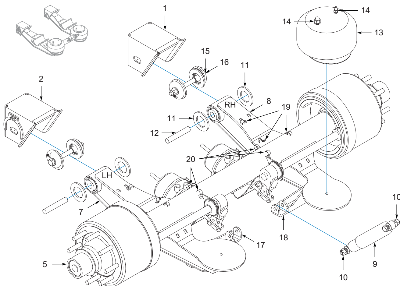
VIEW OF DRUM BRAKE ASSEMBLY
