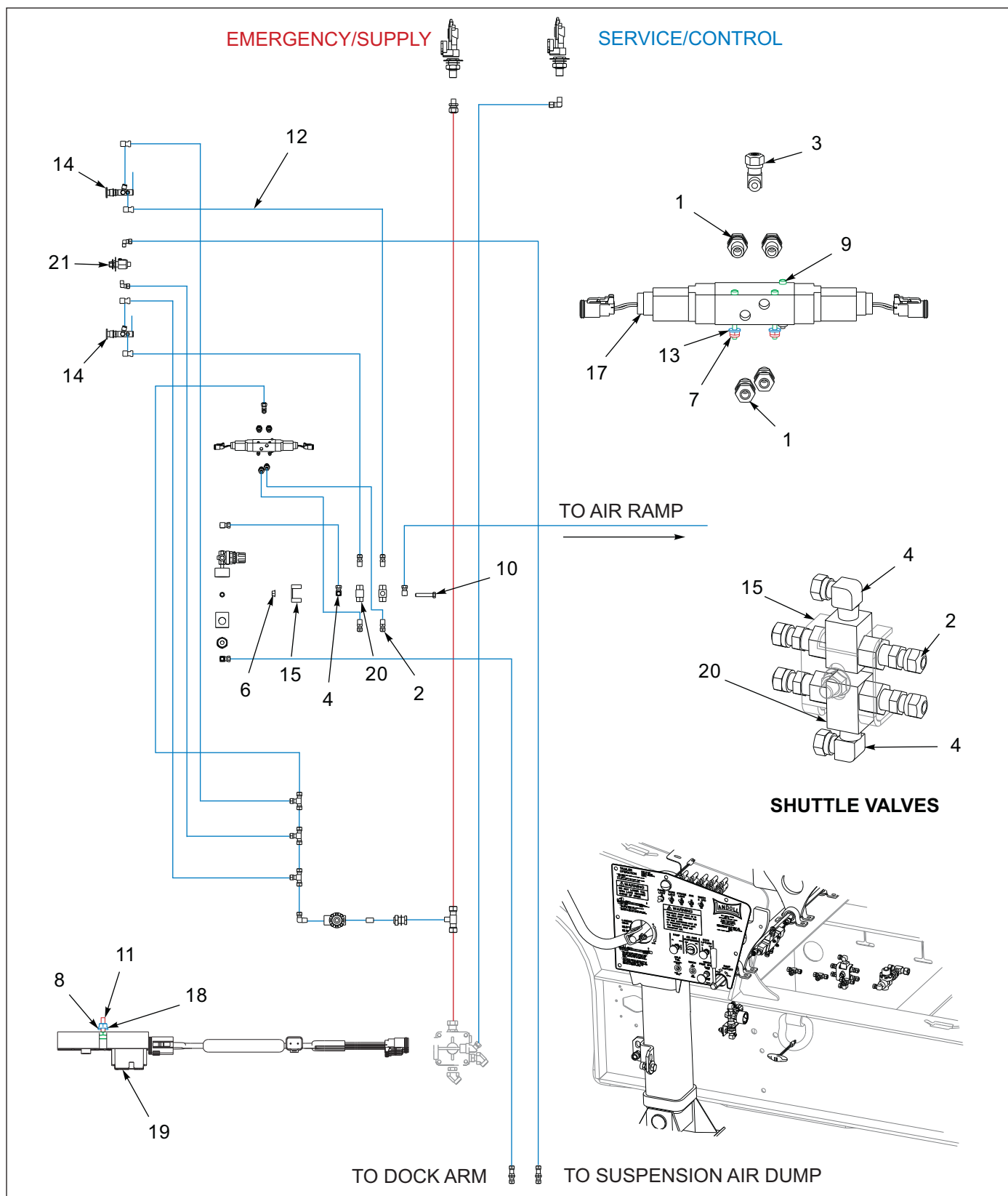
Figure 1-15: Dock &amp; Ramp Remote Air System
