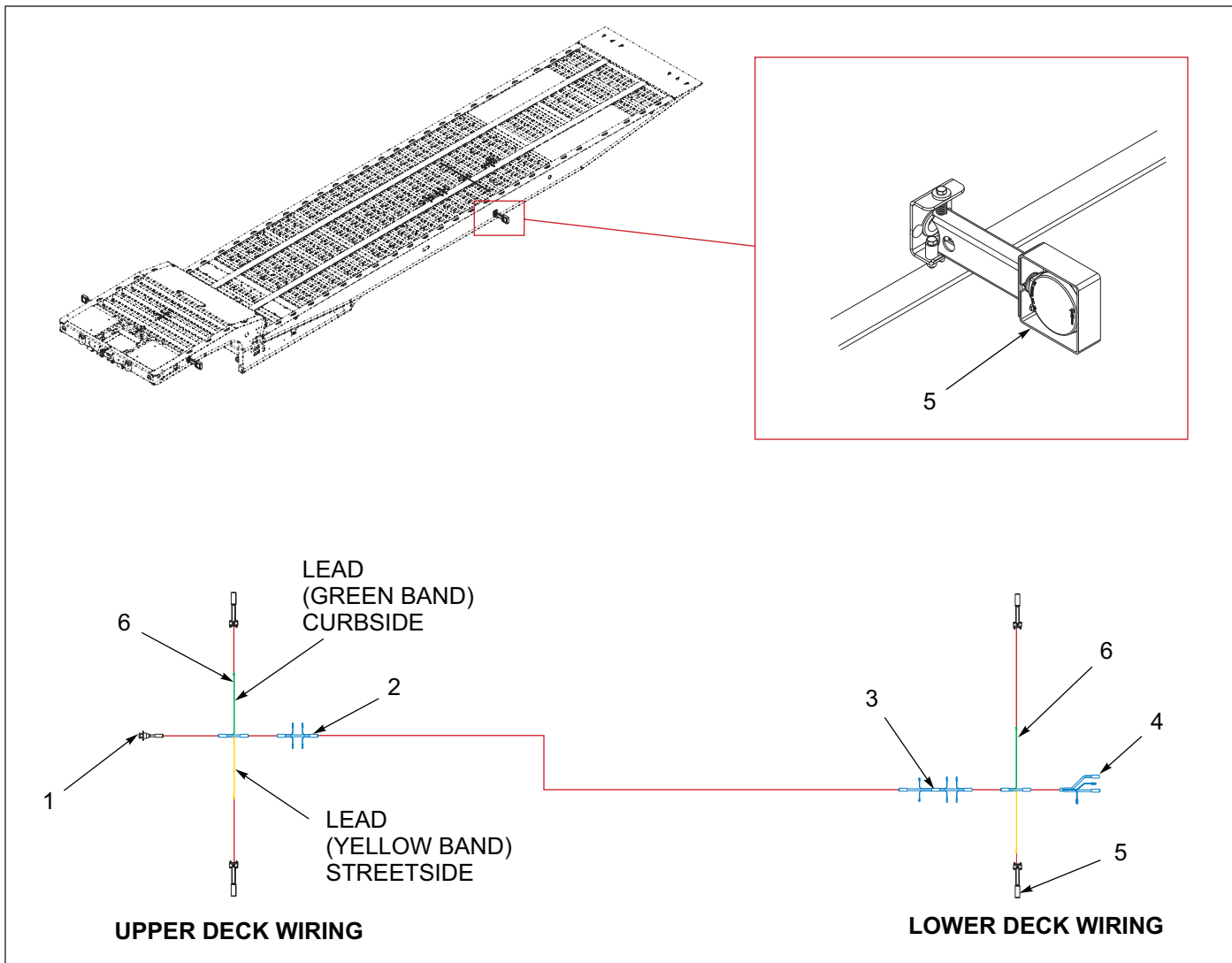
Figure 1-119: Swingout Light Installation
