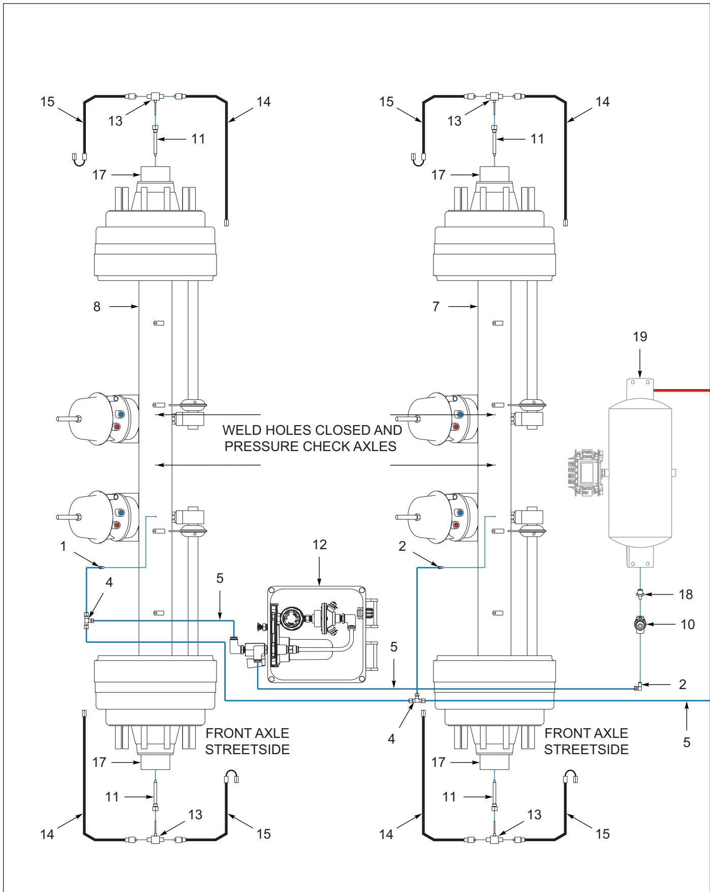
Figure 1-63: Thermalert, 3 Axle Air System (OPTION) (1 of 2)
