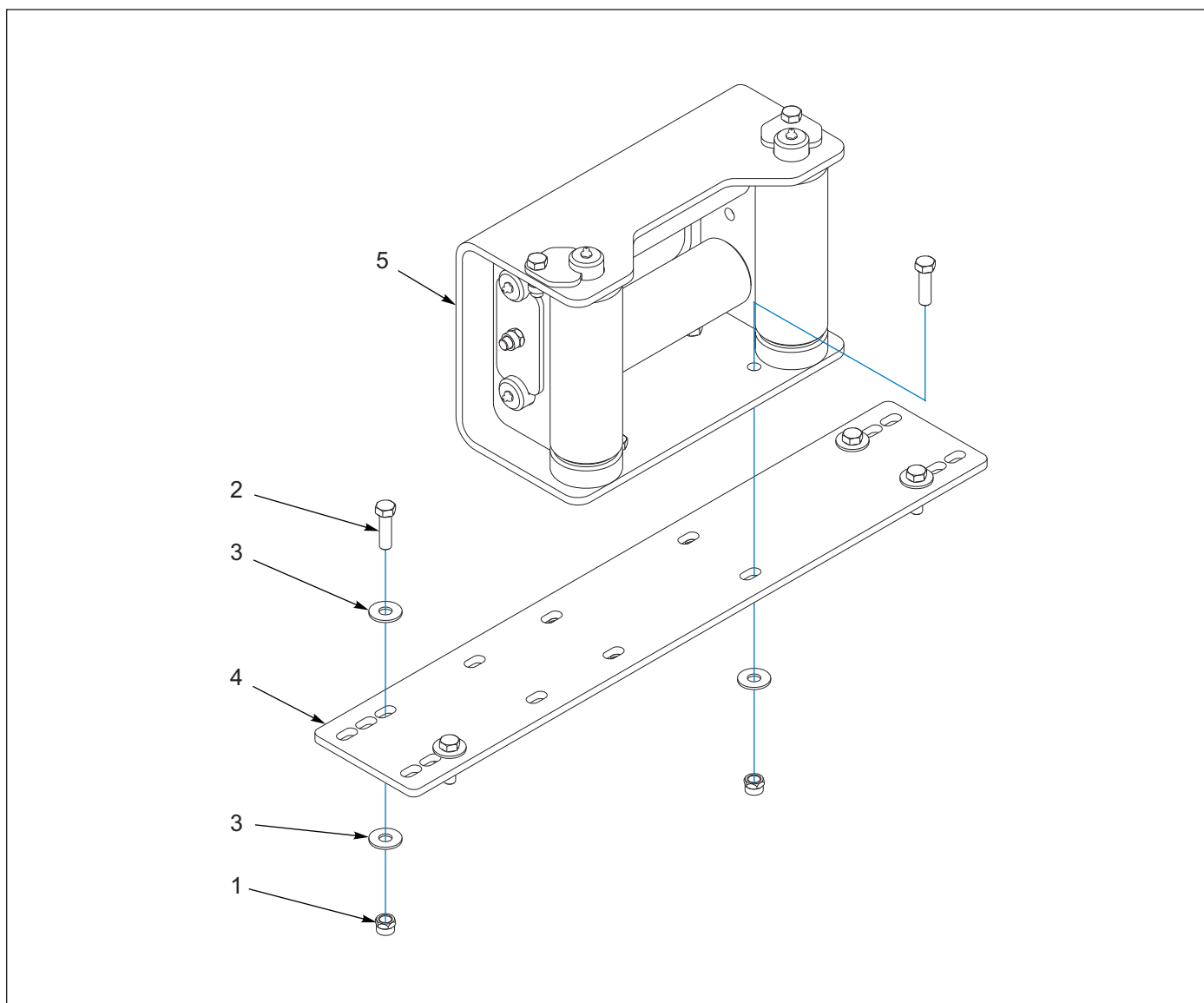
Figure 1-154: Guide Assembly, 4 Roller 12K (BRADEN) Installation
