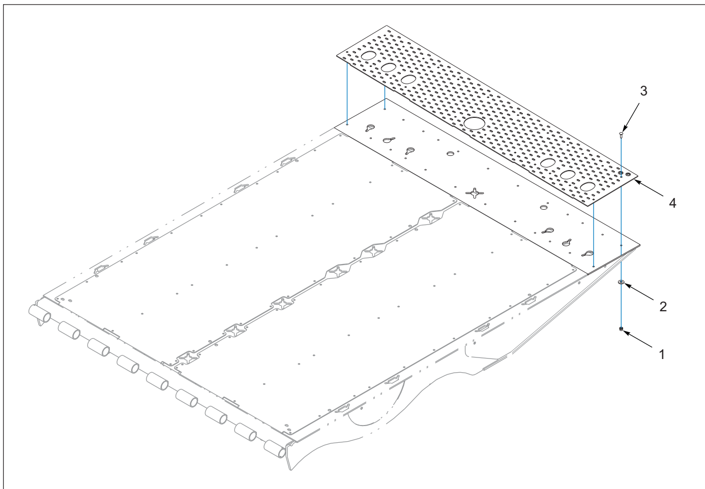
Figure 1-96: Tail Tread Grip End Plate
