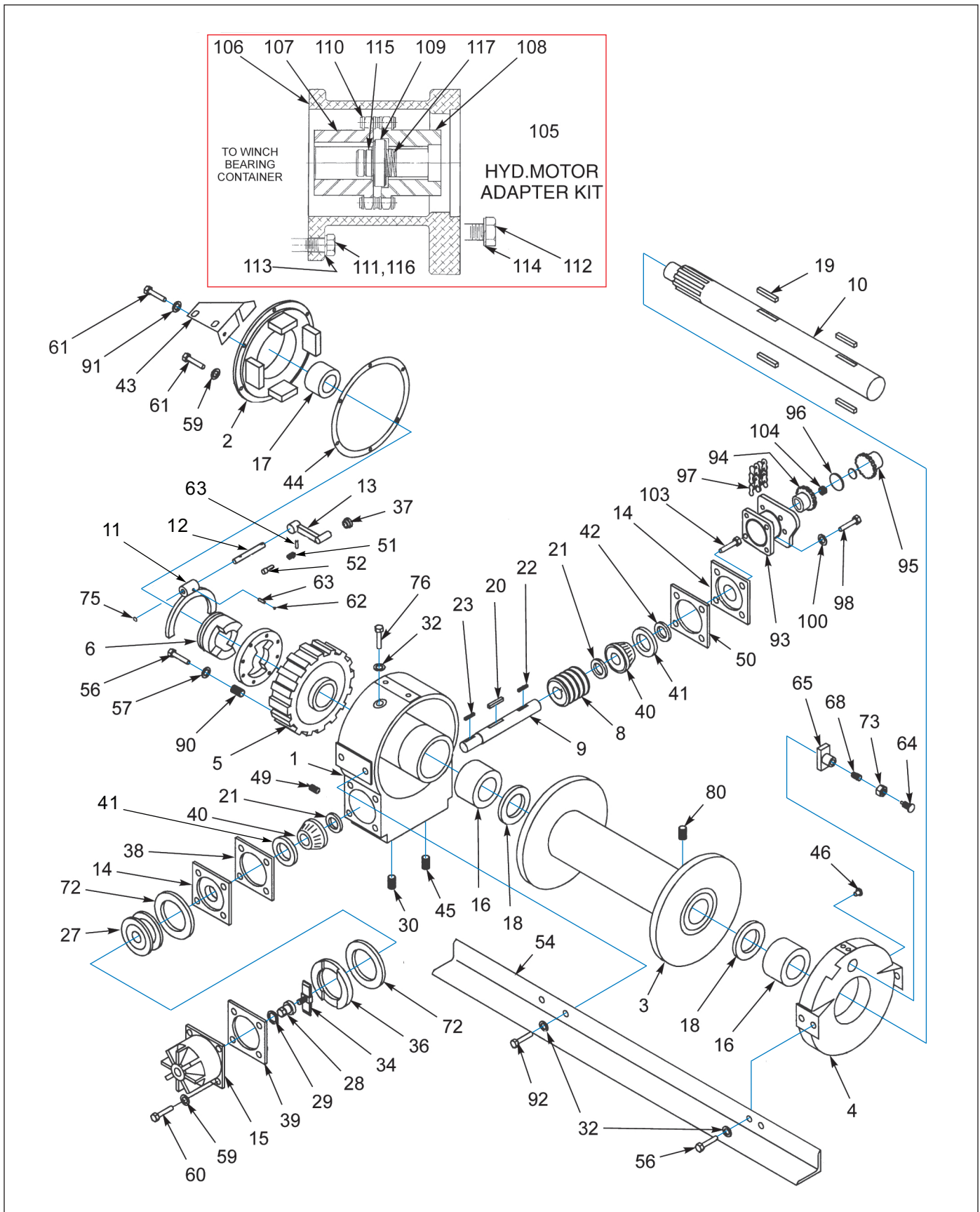
Figure 1-73: Winch Items - 20,000Lb. (BRADEN)
