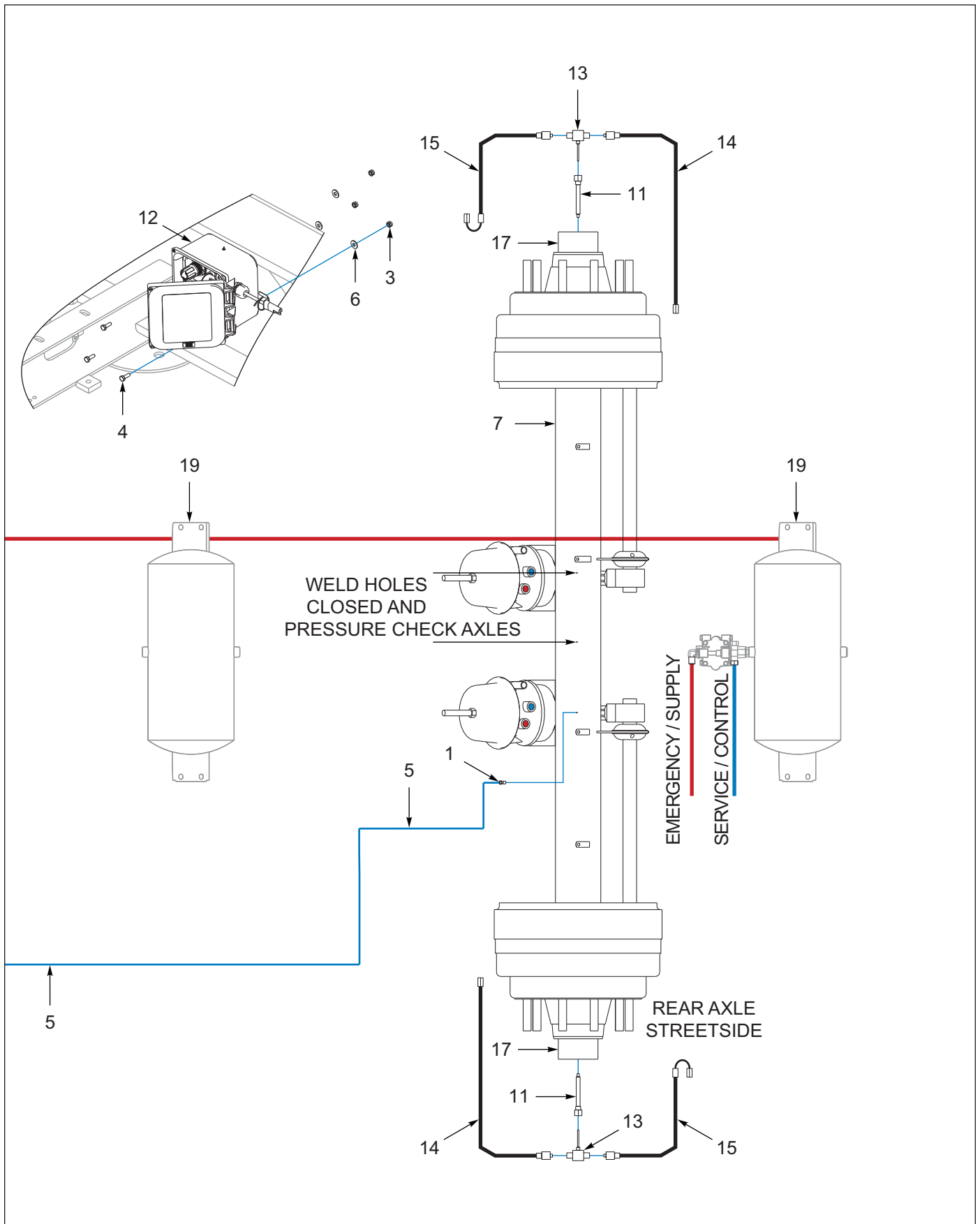
Figure 1-64: Thermalert, 3 Axle Air System (OPTION) (2 of 2)
