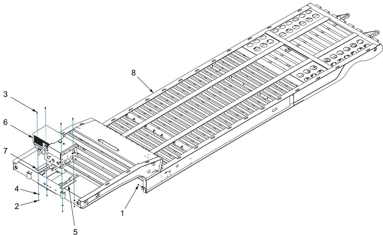
Figure 1-111: Mount Package W/O Winch
