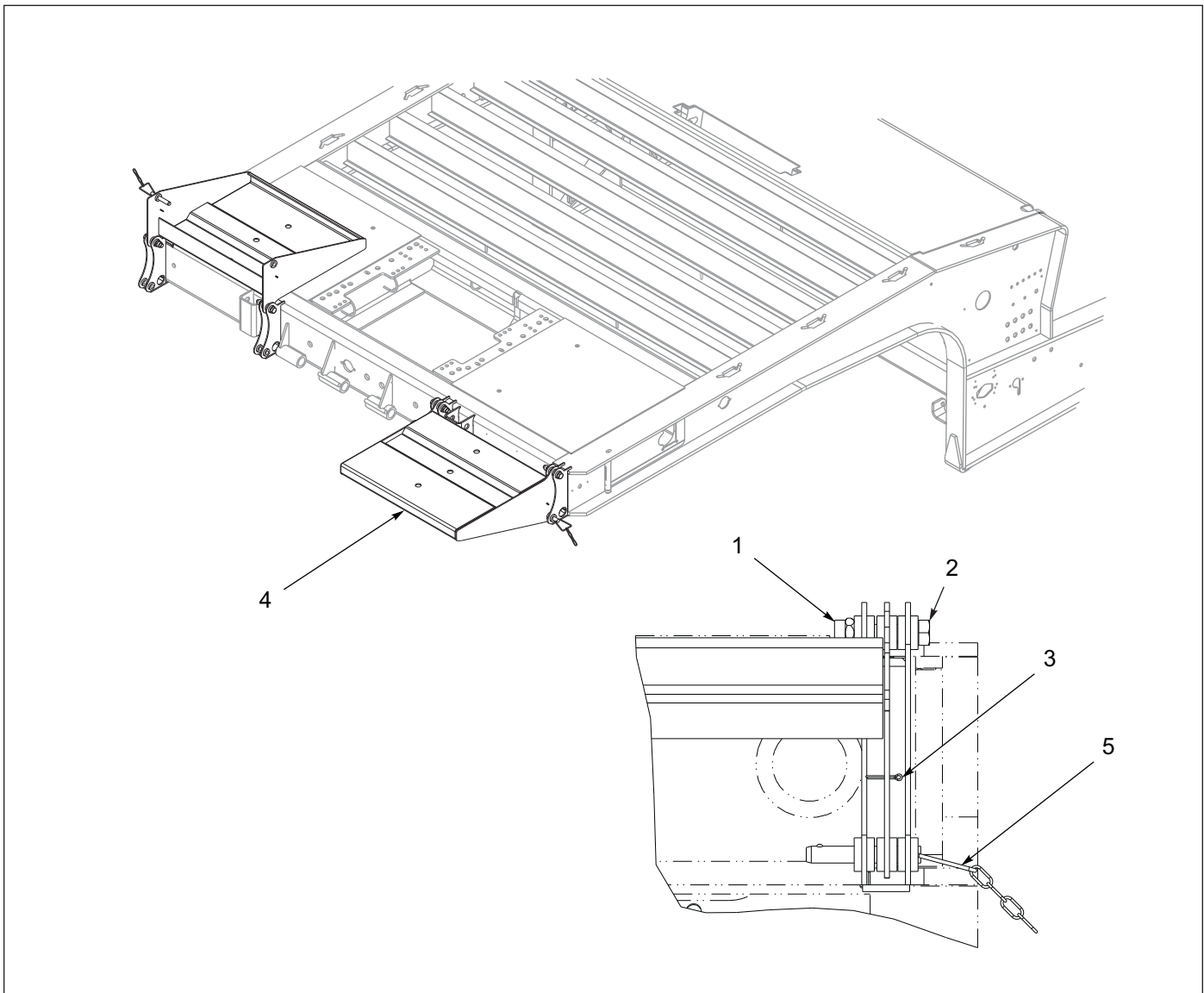
Figure 1-147: Front Flip Extension Assembly
