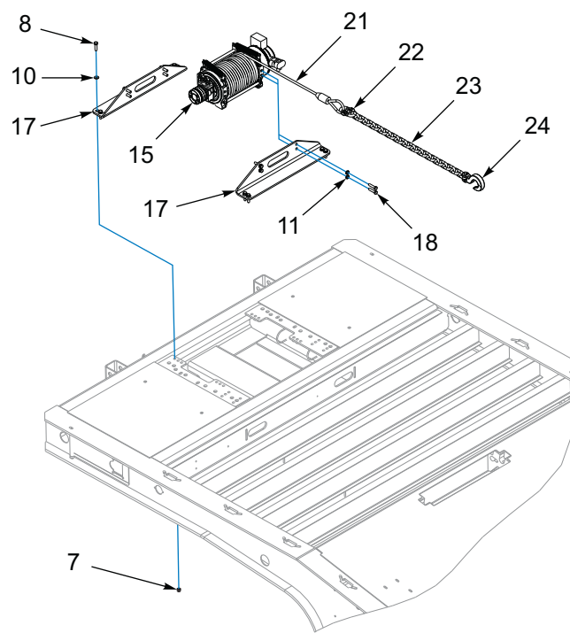
GENERAL ASSEMBLY
