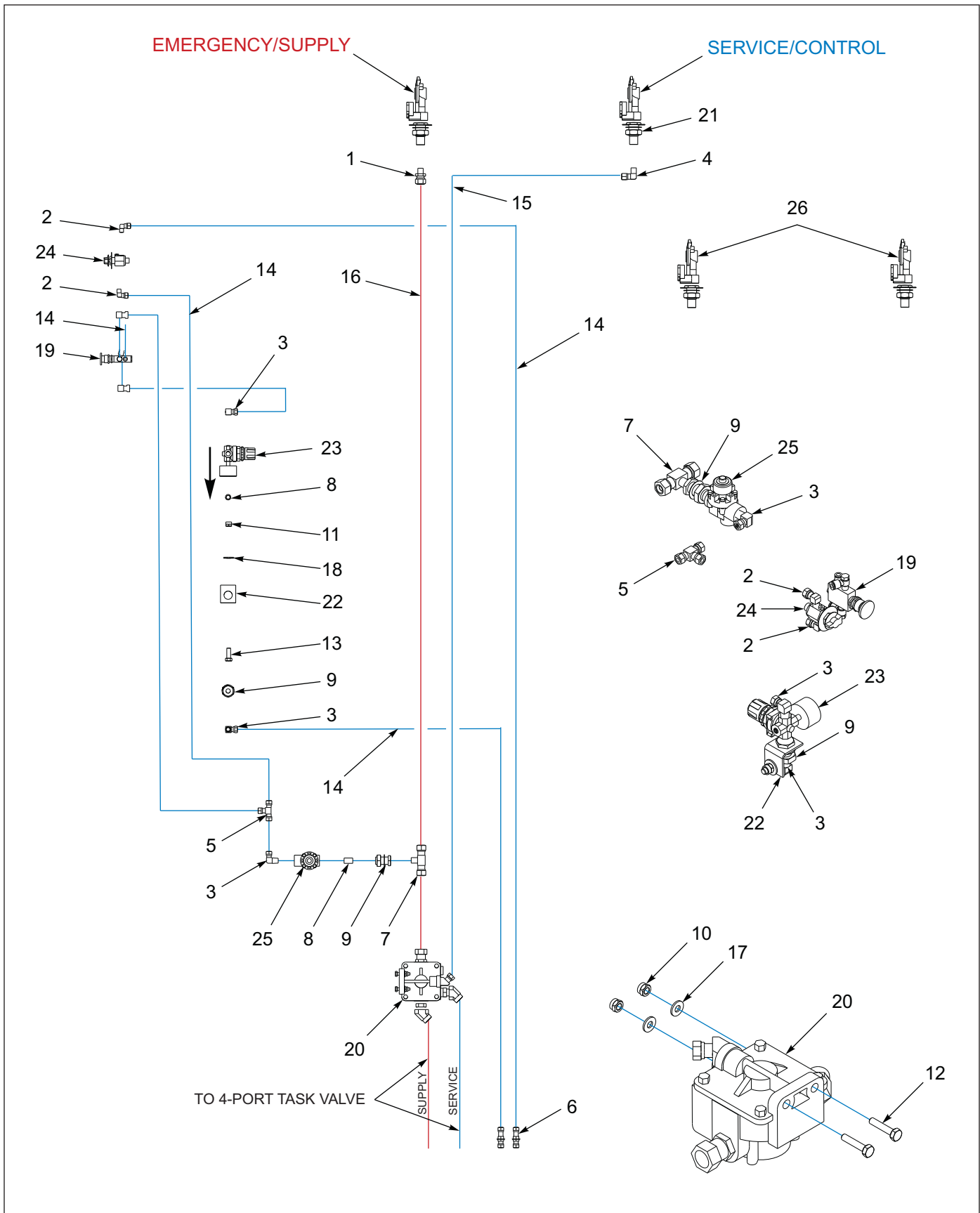
Figure 1-14: Air System
