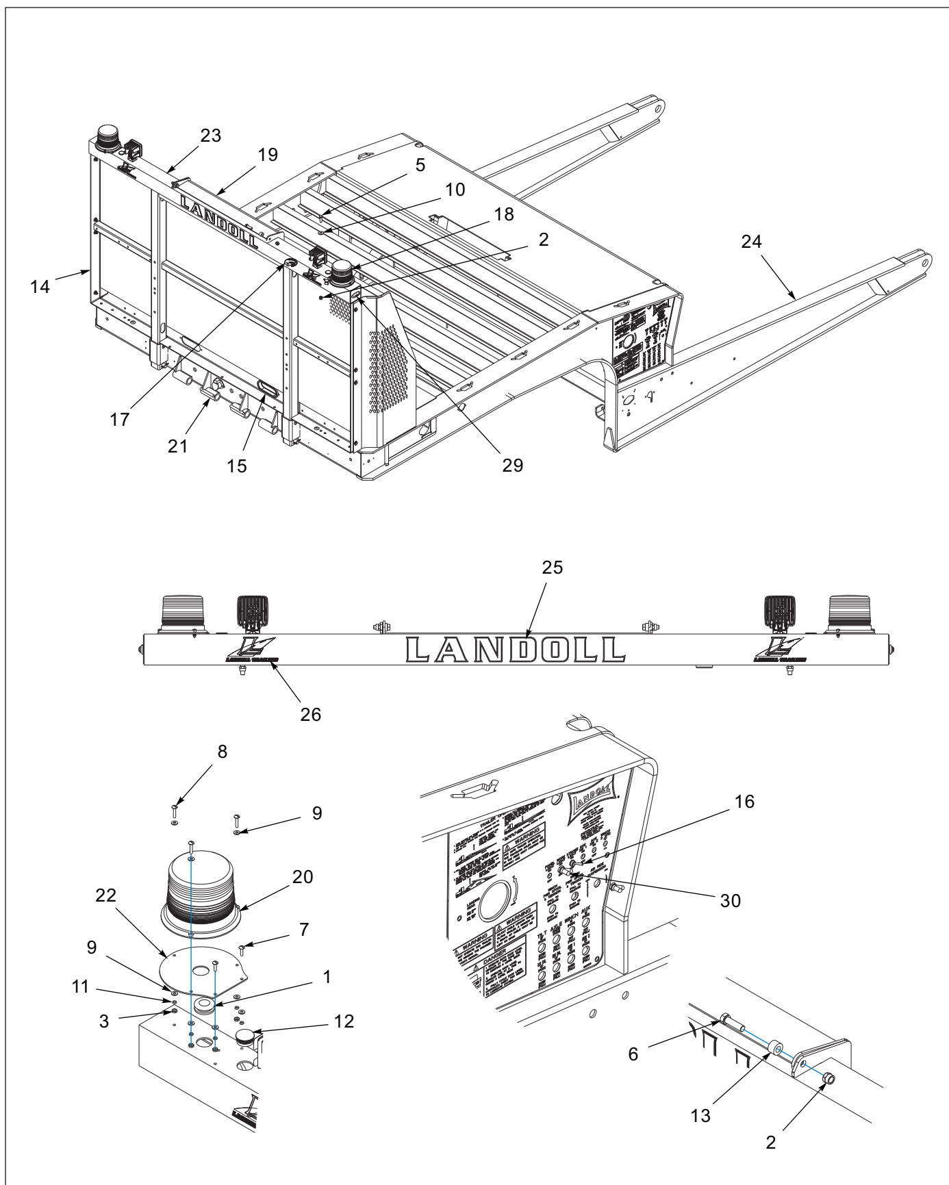
Figure 1-87: Chain Rack Lights General Assembly
