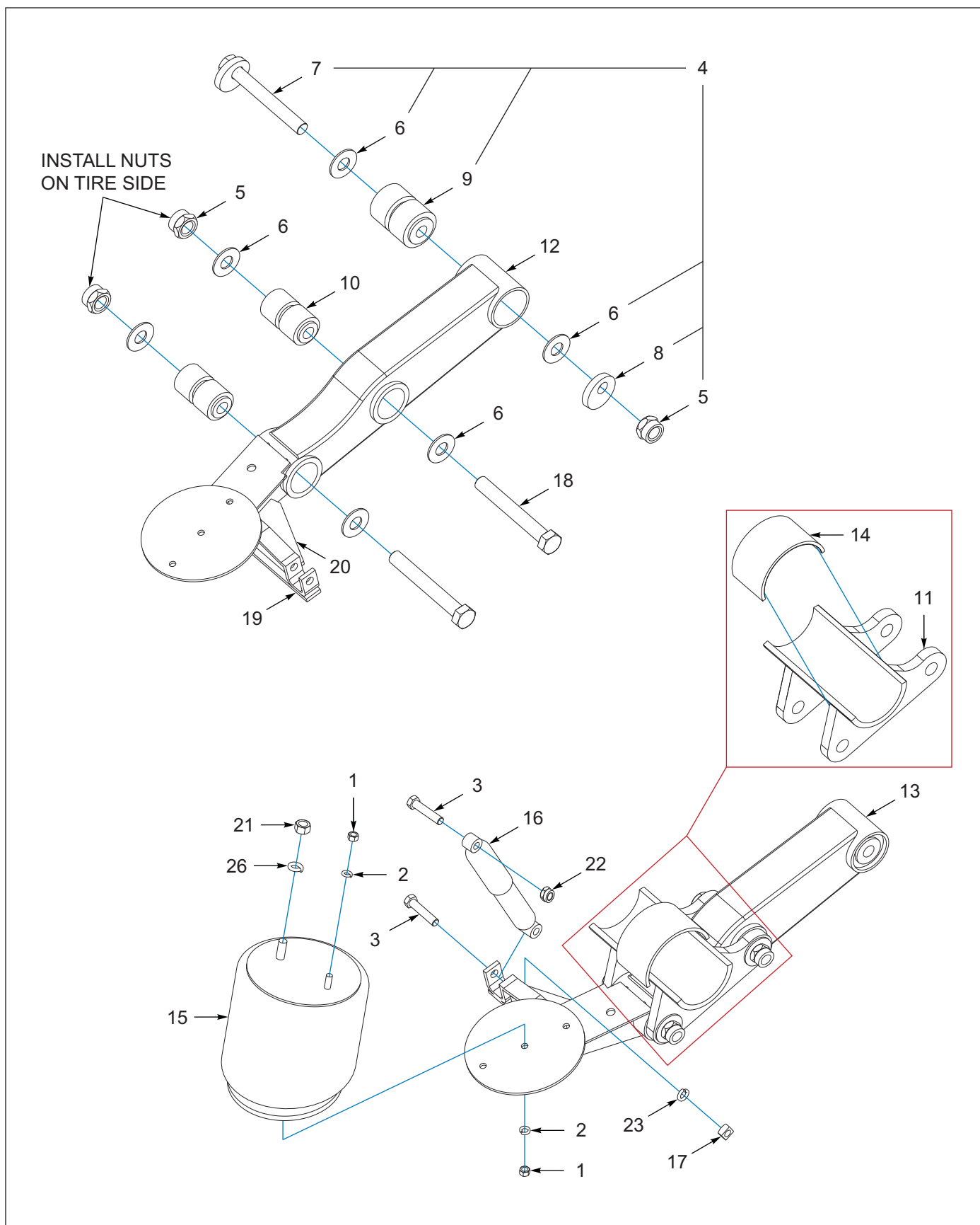
Figure 1-46: Suspension Hanger - RLU-228
