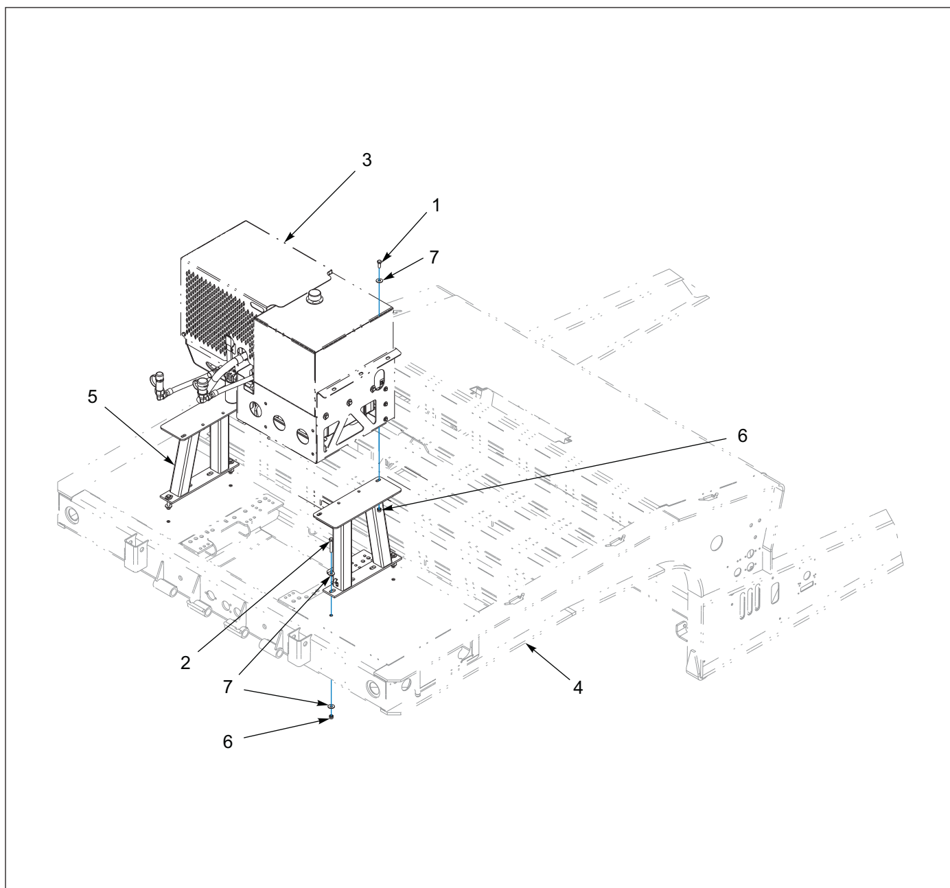
Figure 1-113: Upper Deck Stand Installation
