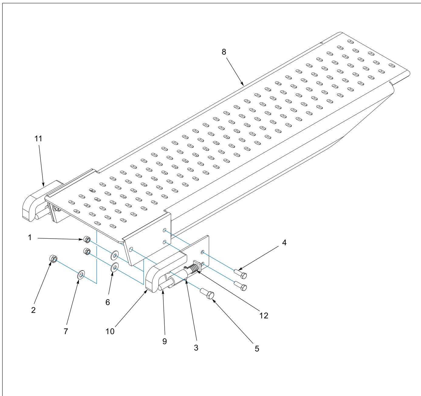
Figure 1-125: Front Slope
