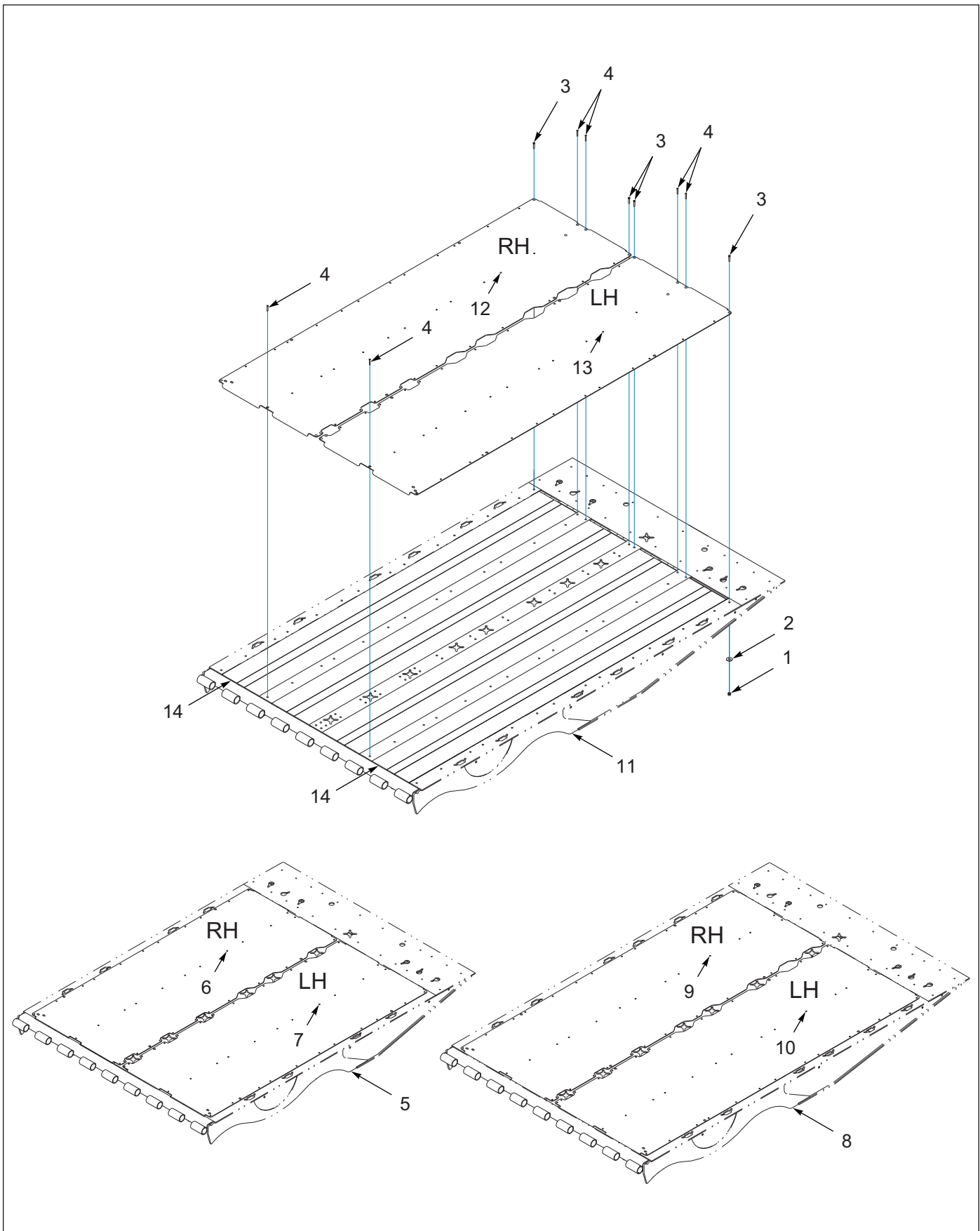
Figure 1-94: Tail Tread Grip-222967
