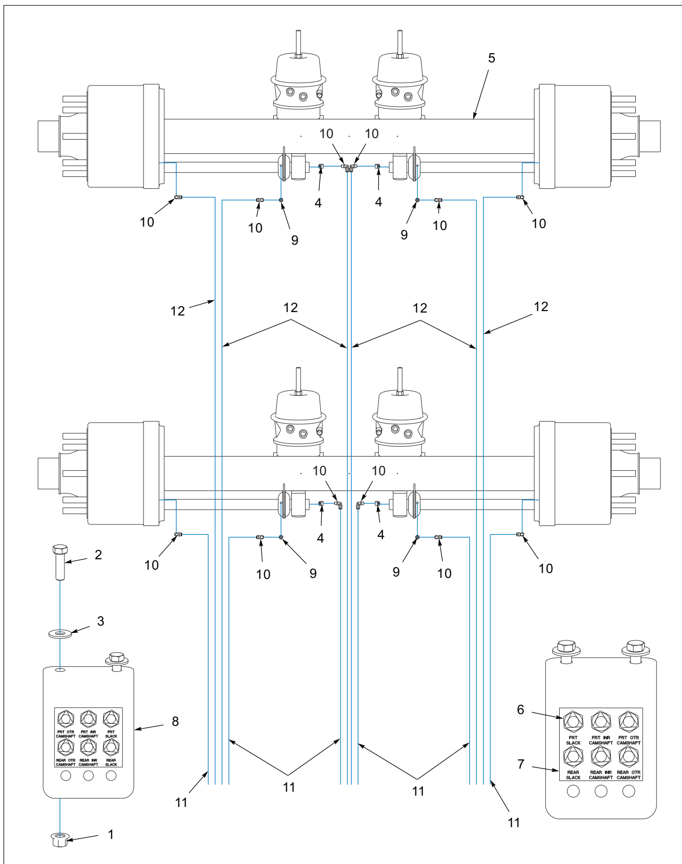
Figure 1-33: Grease System, 2 Axle (After 11/07/2018 - Before 08/31/2020)
