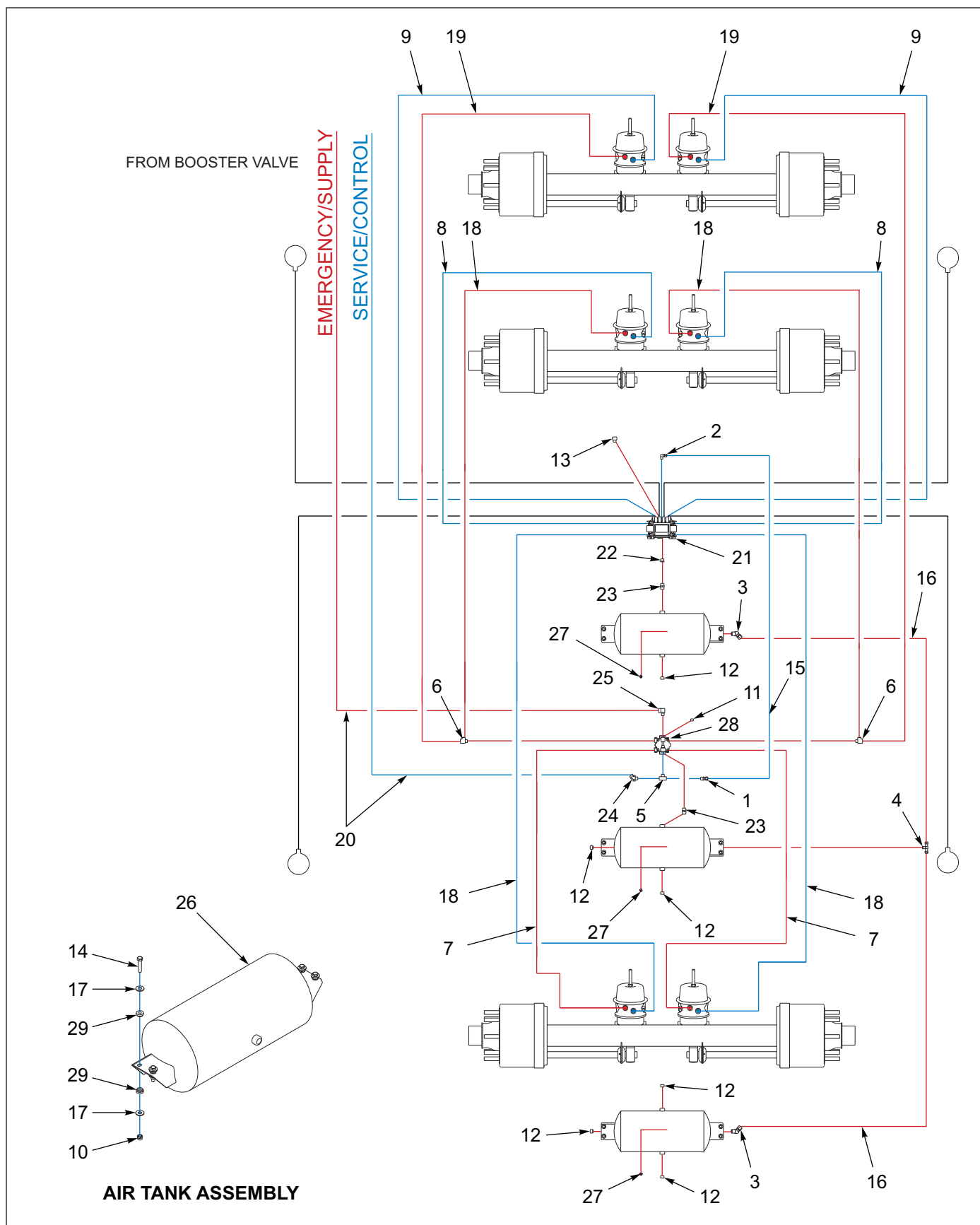
Figure 1-59: 950E-Air Brake System
