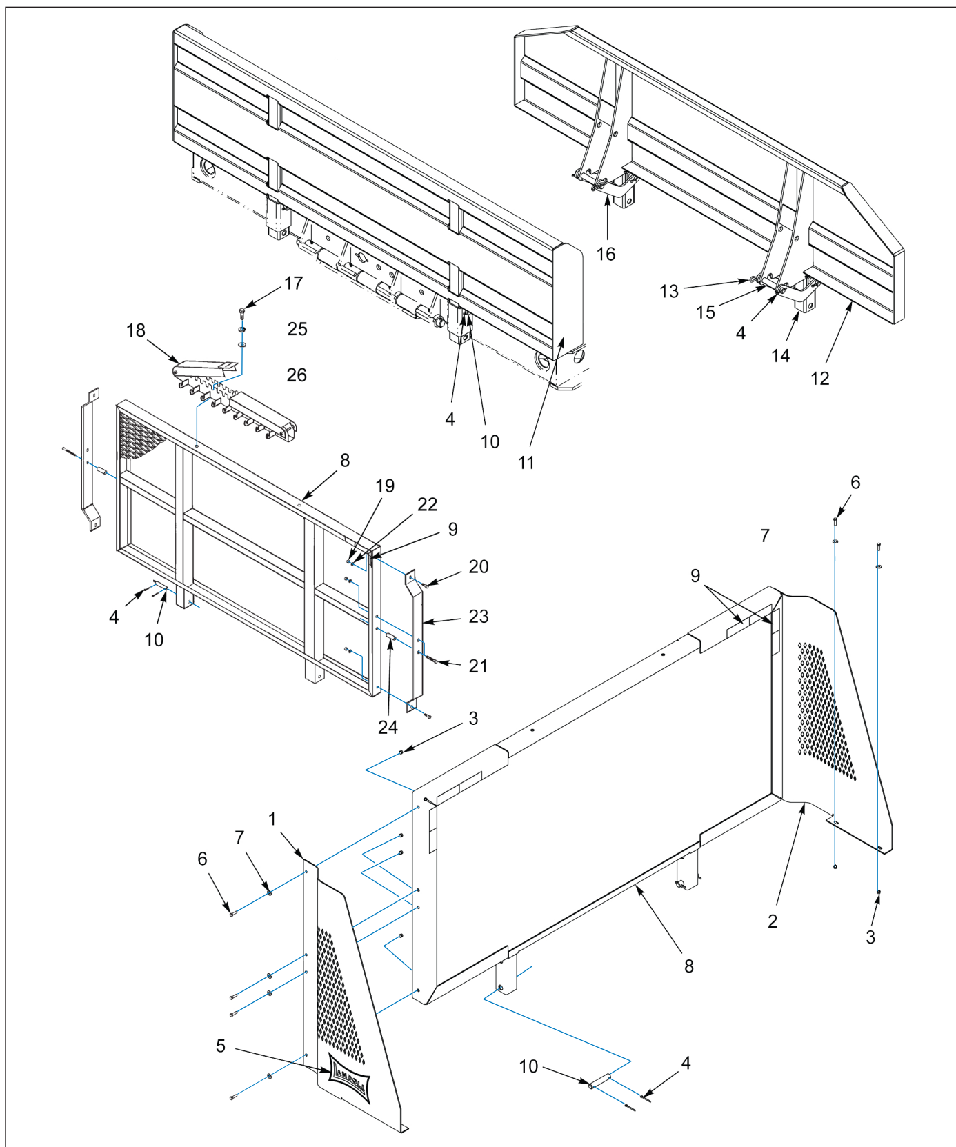
Figure 1-86: Bulkhead Assembly
