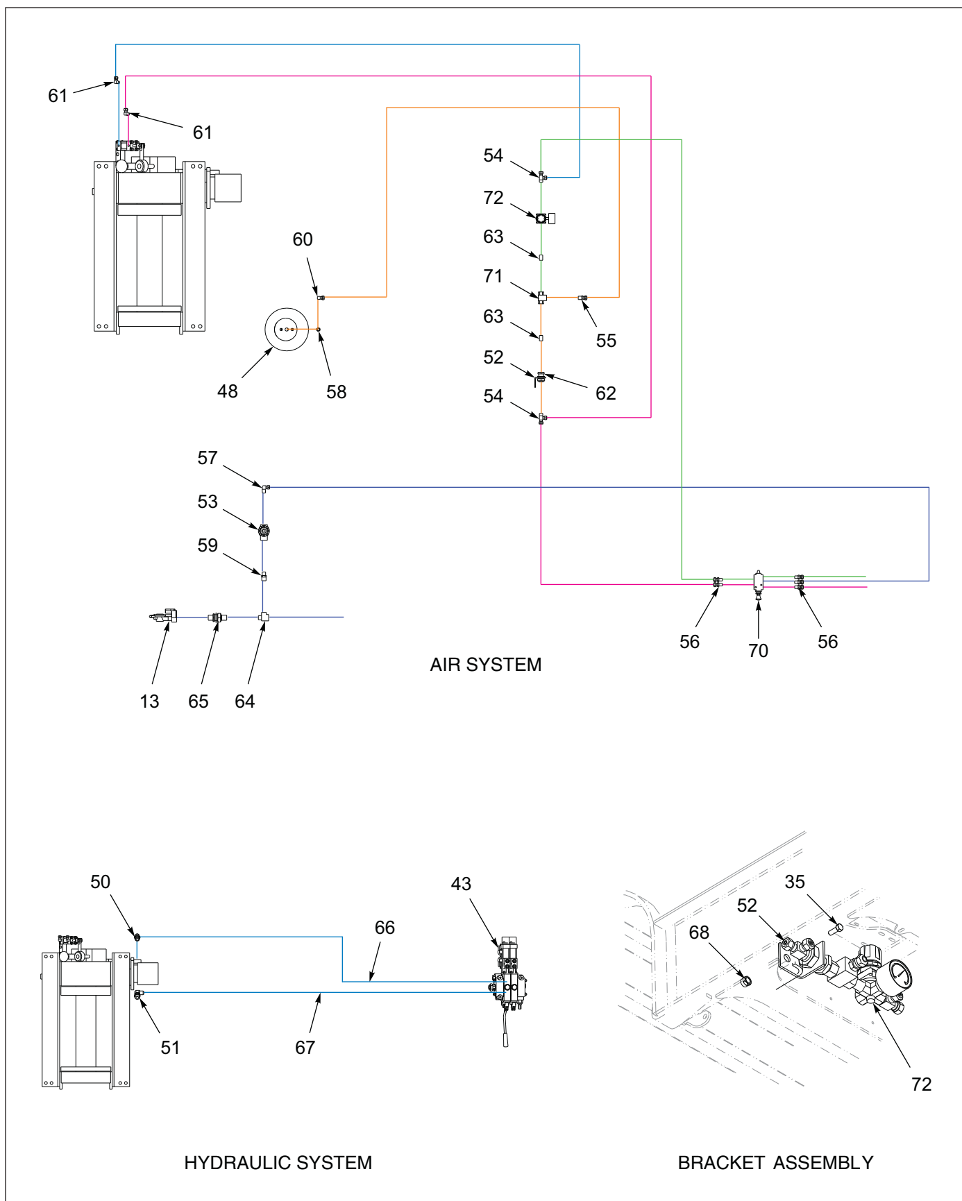
Figure 1-72: 20K Air Tension/Release (BRADEN) (3 of 3)
