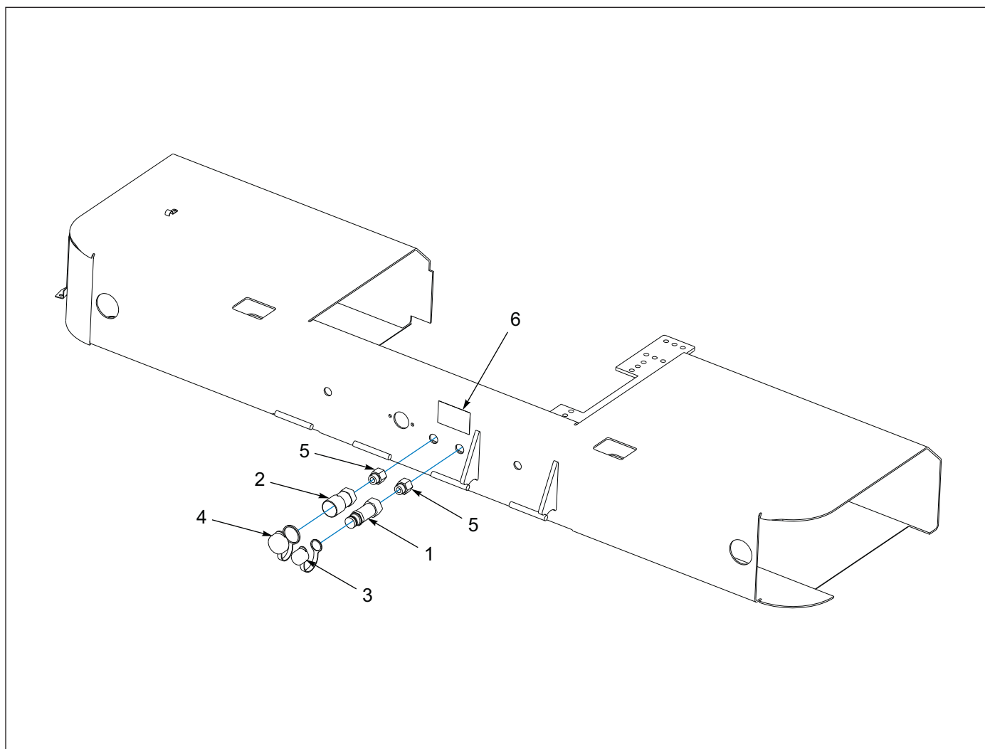
Figure 1-114: Hydraulic Conversion Kit - Ball to Flat
