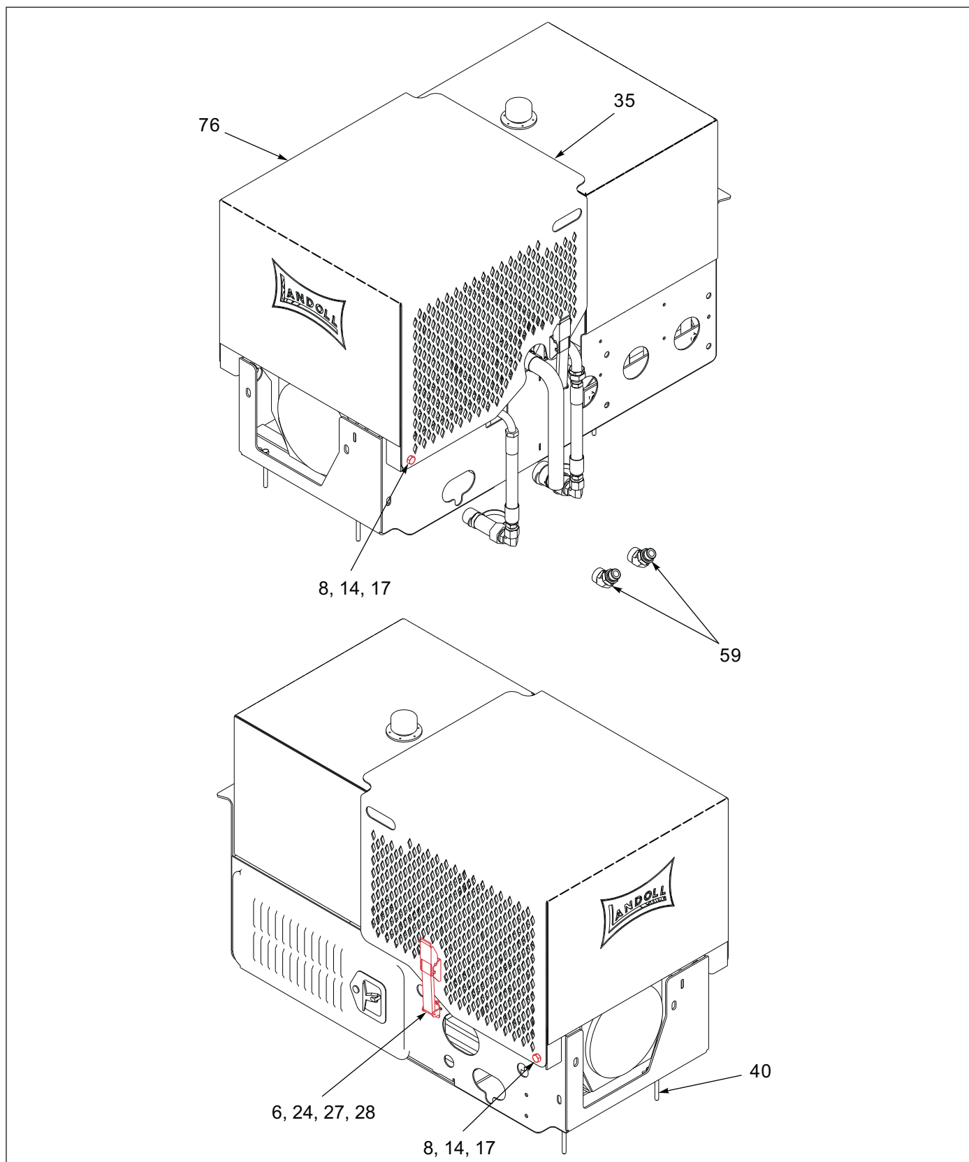
Figure 1-101: 25 HP Upper Deck Package (1 of 4)
