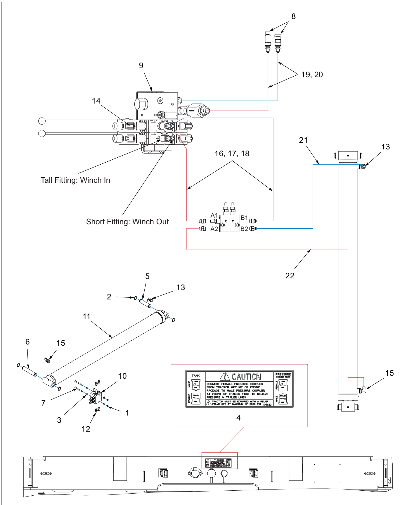
Figure 1-13: Axle Hydraulic System
