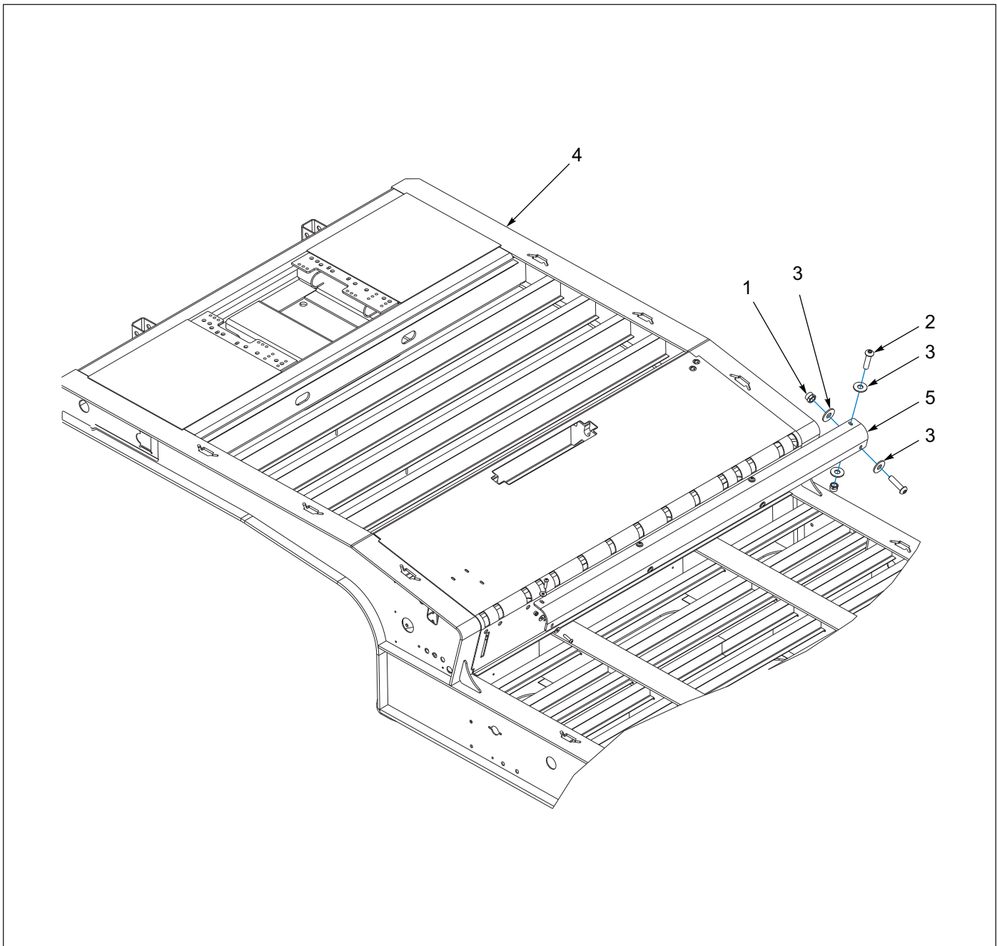
Figure 1-92: Fork Lift Plate Installation
