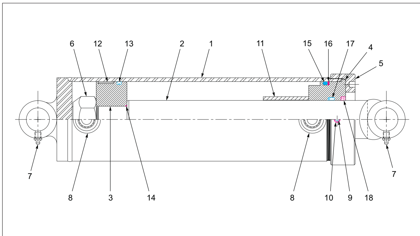
Figure 1-21: Cylinder - 5 X 60
