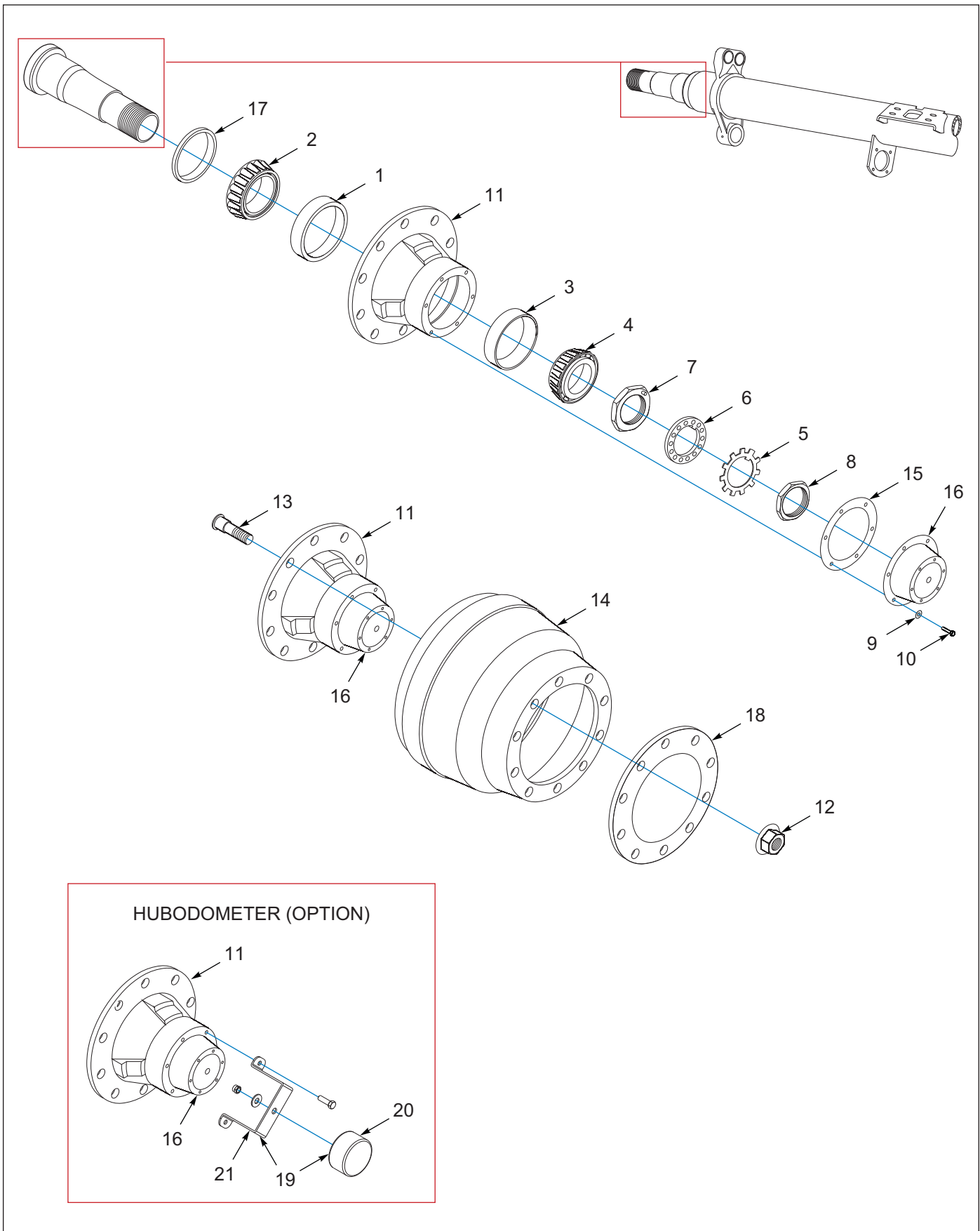
Figure 1-56: Axle 16.5 x 7 Drum and Hub Assembly, Dexter
