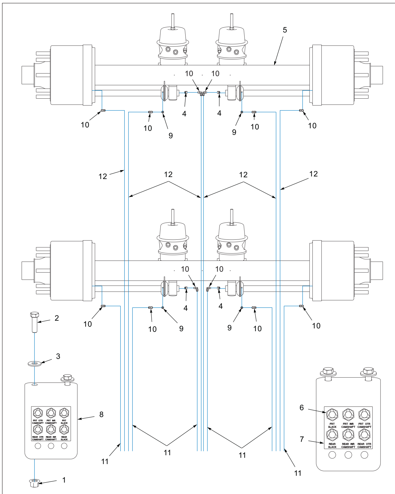
Figure 1-32: Grease System, 2 Axle (Before 11/07/2018)
