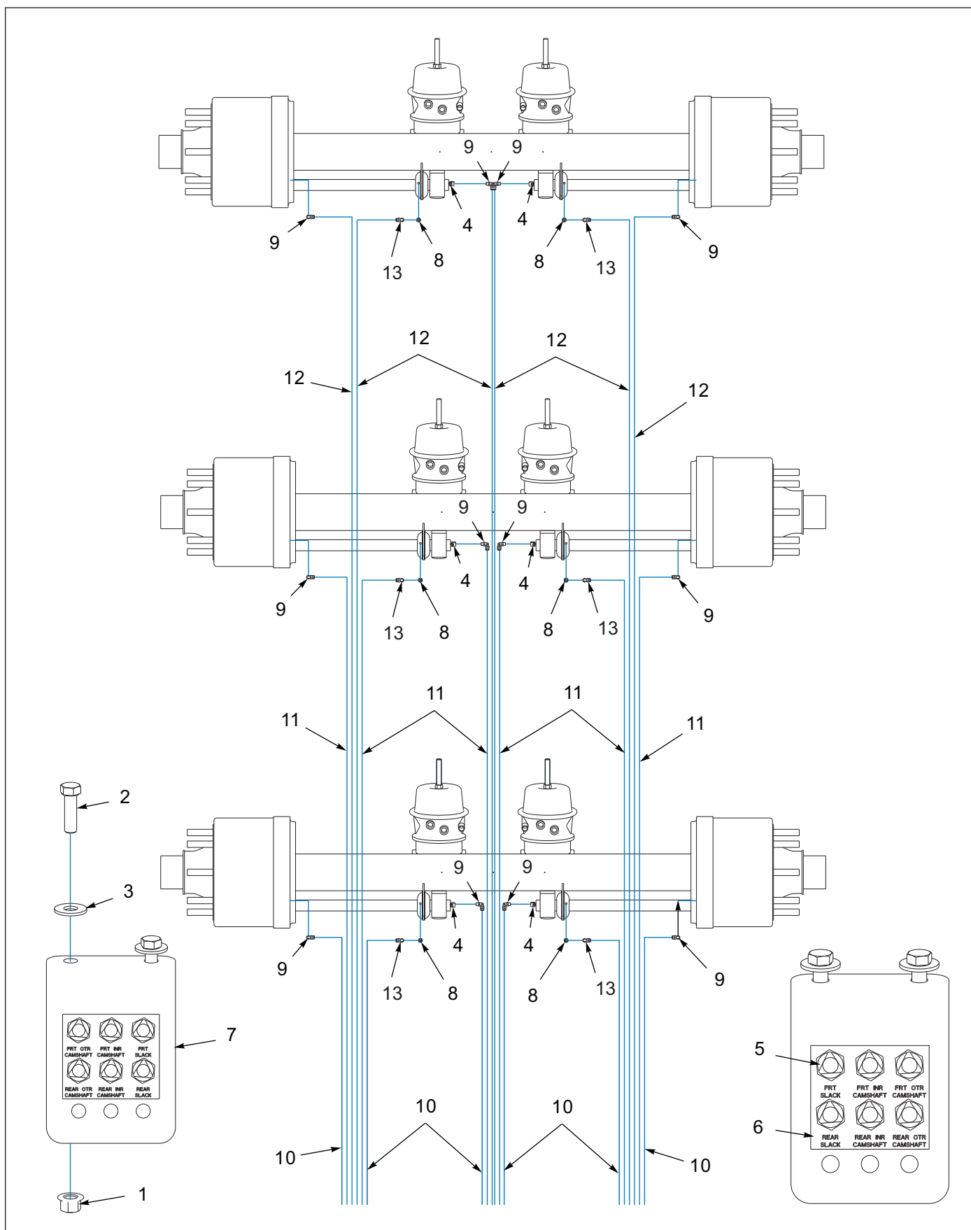
Figure 1-38: Grease System, 3 Axle (After 11/07/2018 - Before 08/31/2020)
