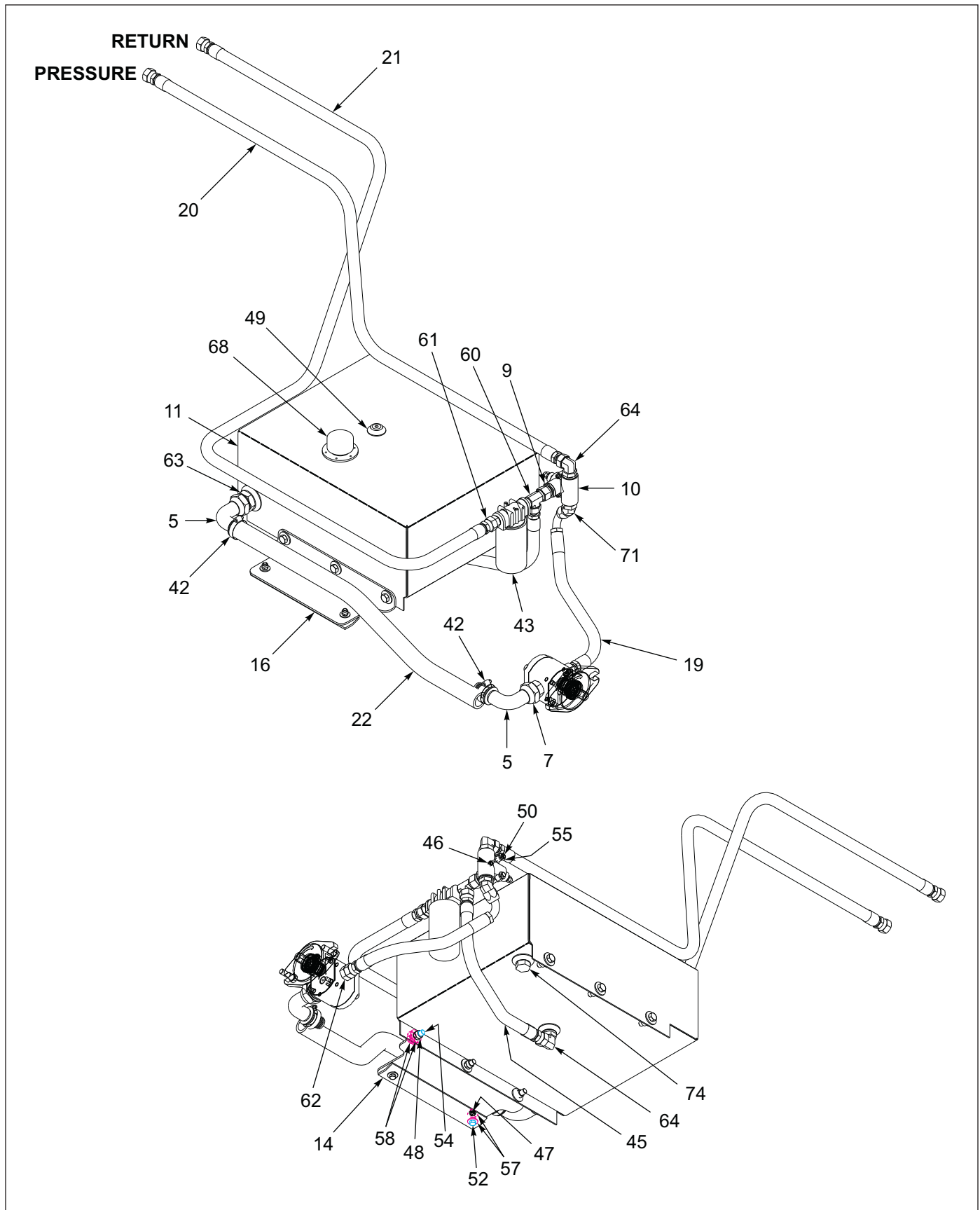
Figure 1-108: 25 HP Slope Package (4 of 4)
