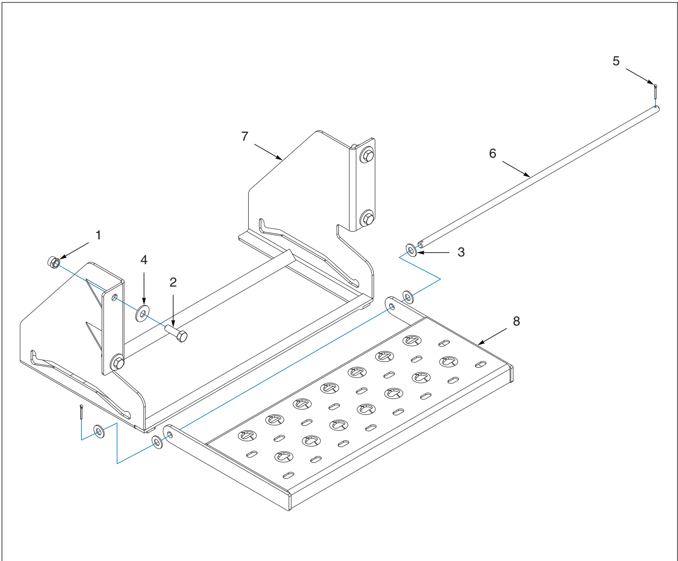
Figure 1-140: Step, Retractable Assembly
