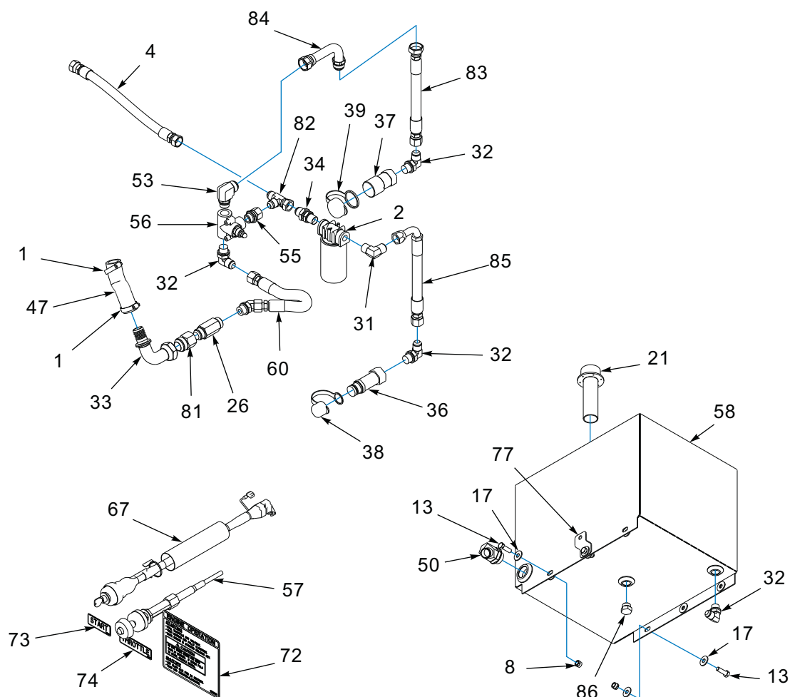
Figure 1-104: 25 HP Upper Deck Package (4 of 4)
