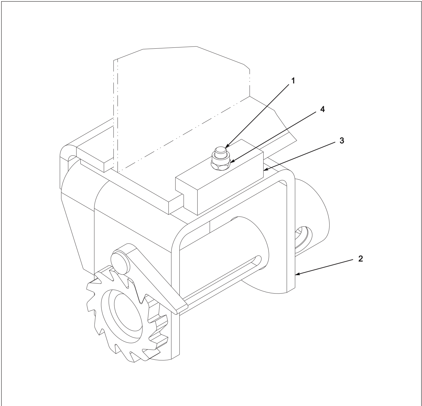
Figure 1-146: Winch Web, Sliding 4in
