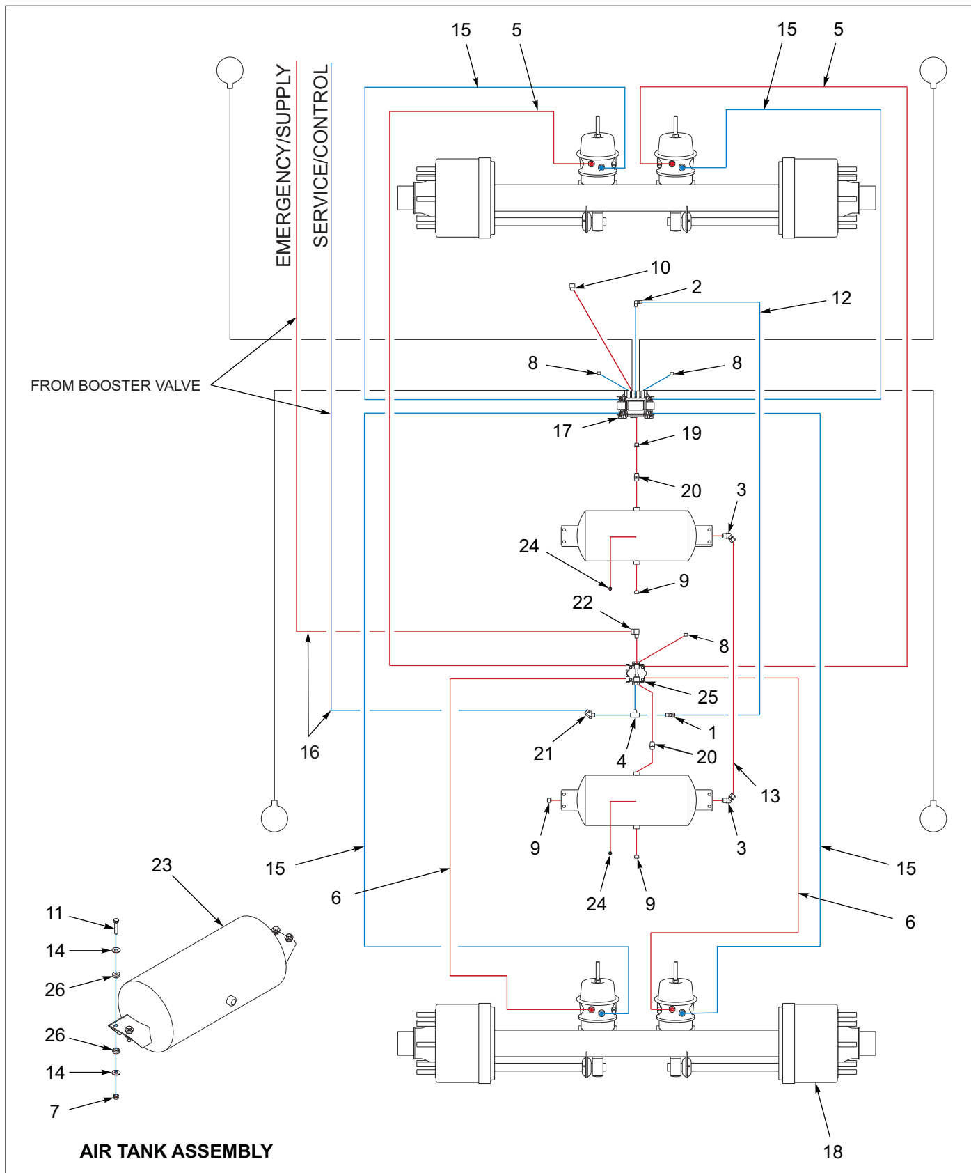
Figure 1-58: 930E-Air Brake System
