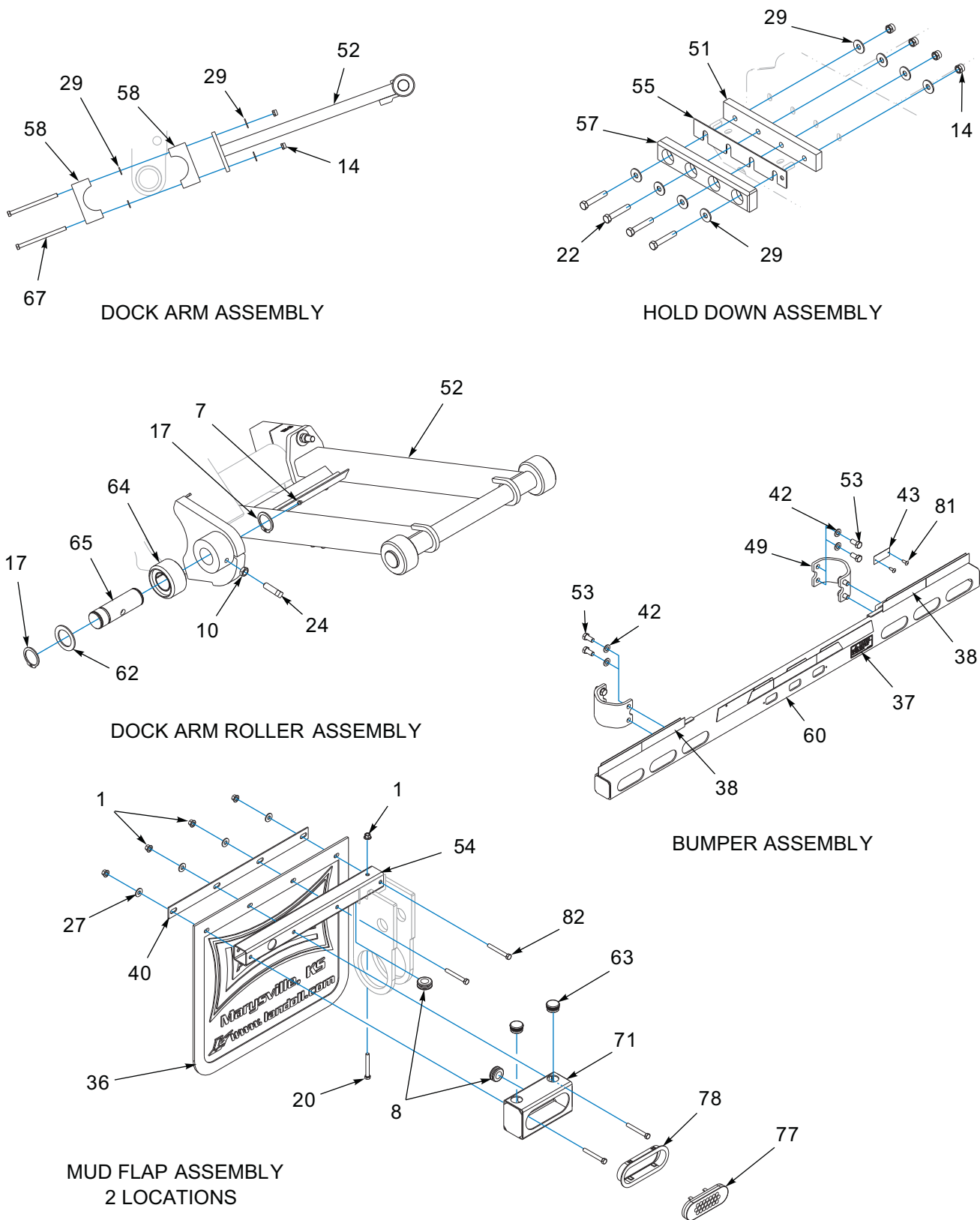
Figure 1-28: General Items - 930E (3 of 3)
