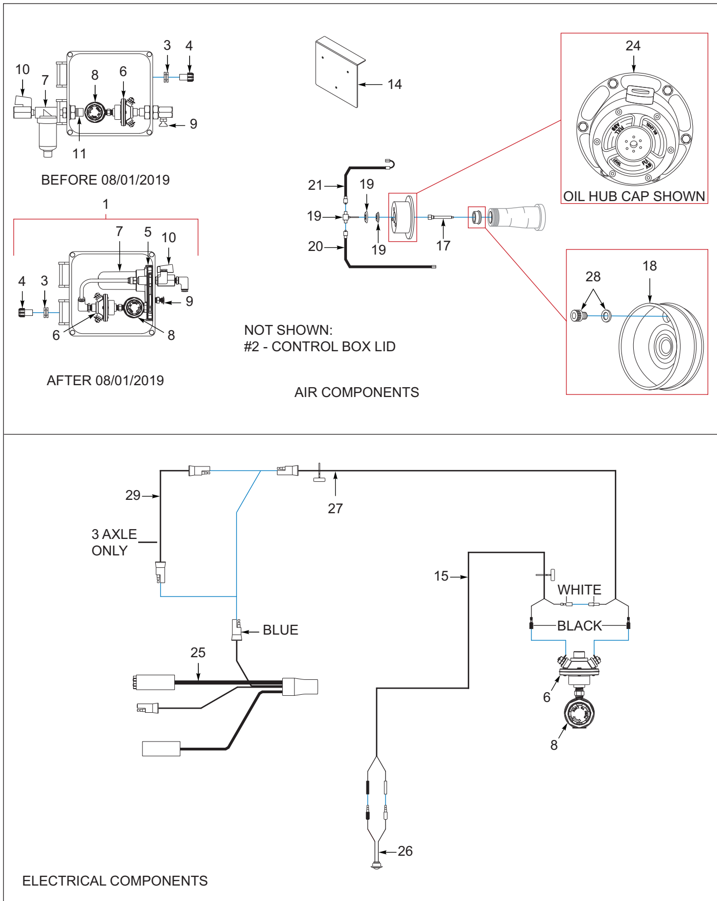
Figure 1-65: Thermalert Electrical System &amp; Components (OPTION)
