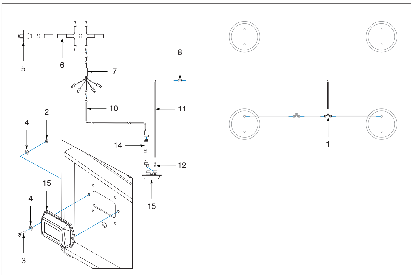
Figure 1-133: Quickload Plus (AFTER 3/31/2020)
