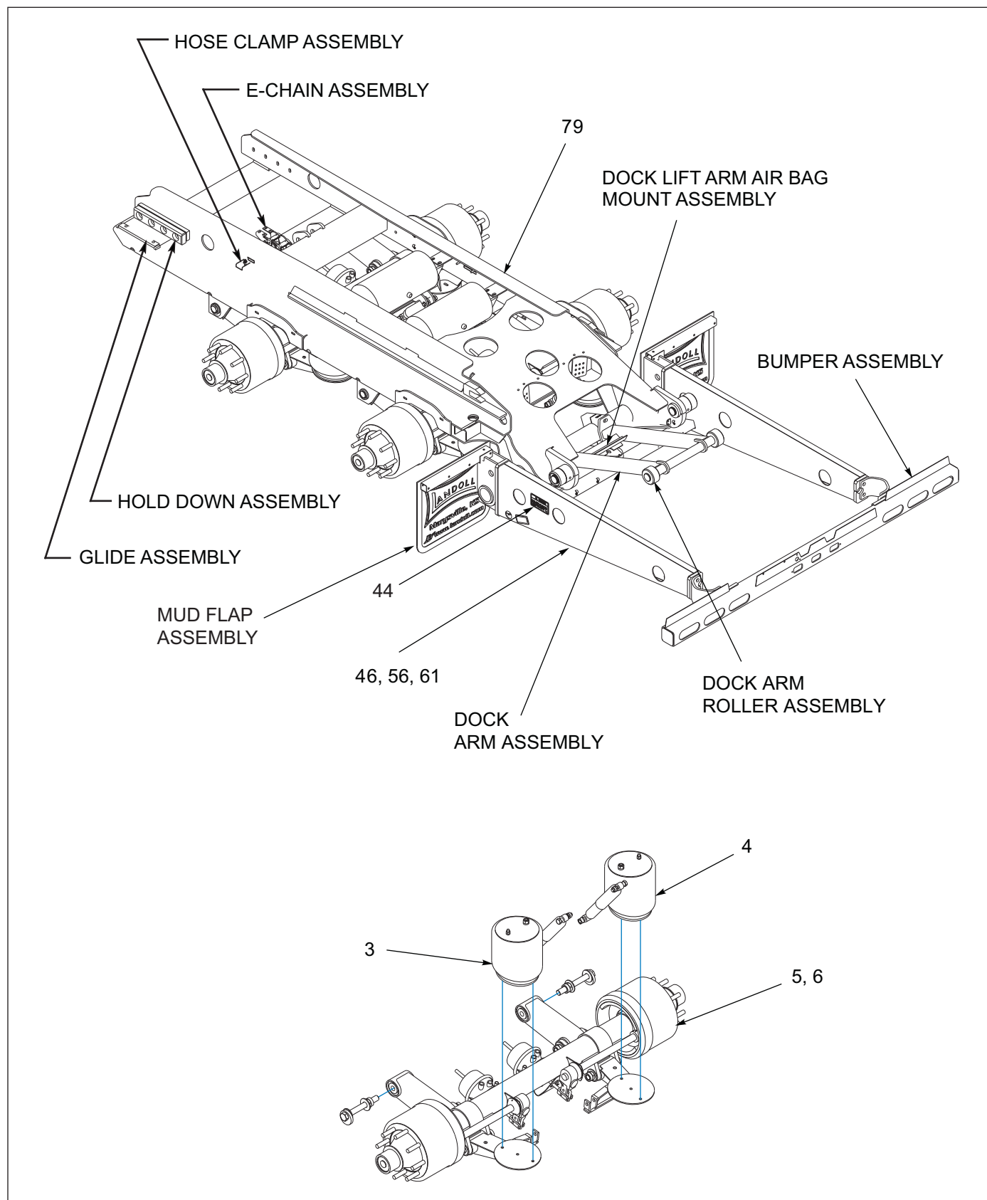
Figure 1-26: General Items - 930E (1 of 3)
