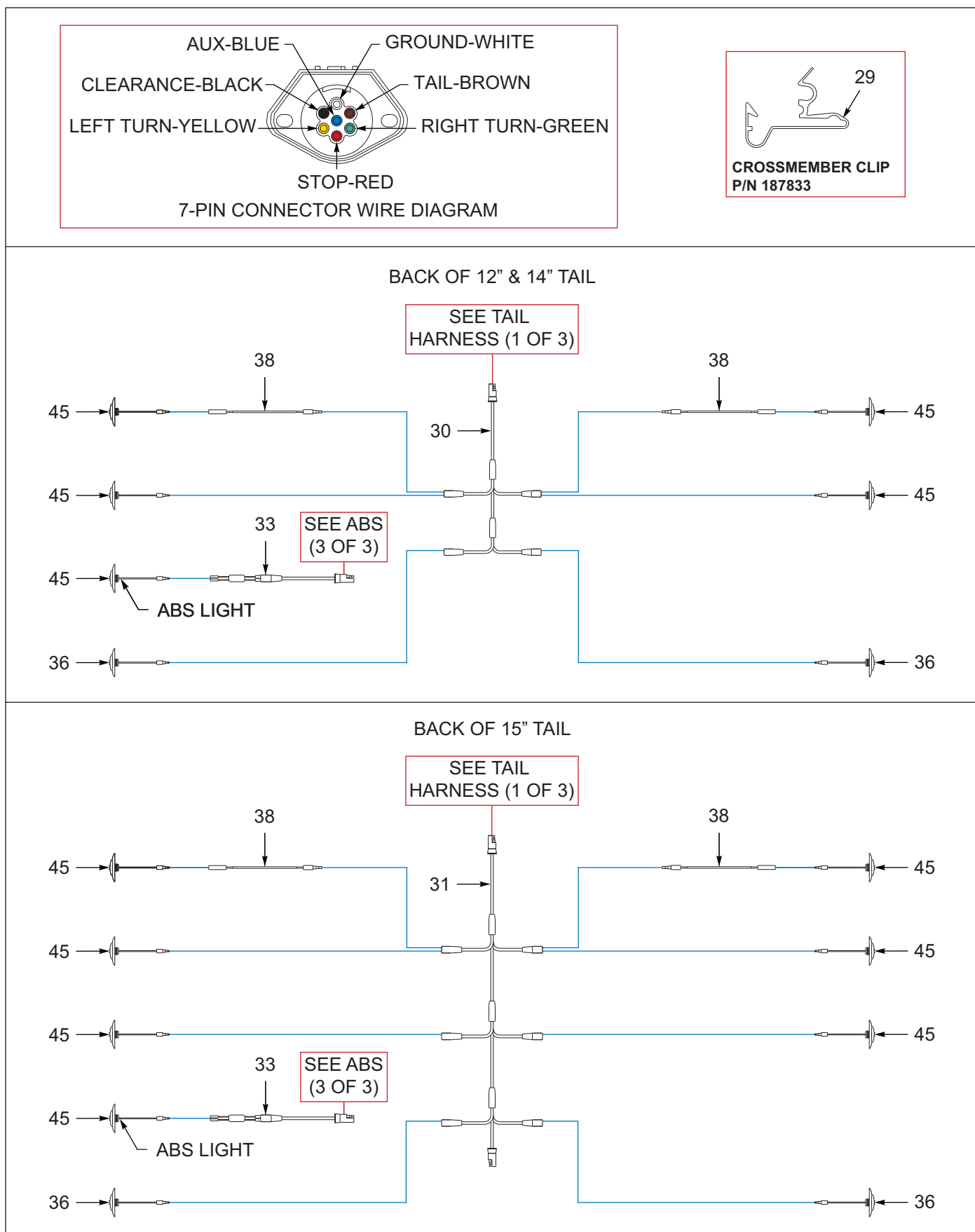
Figure 1-19: Electrical System (2 of 3)
