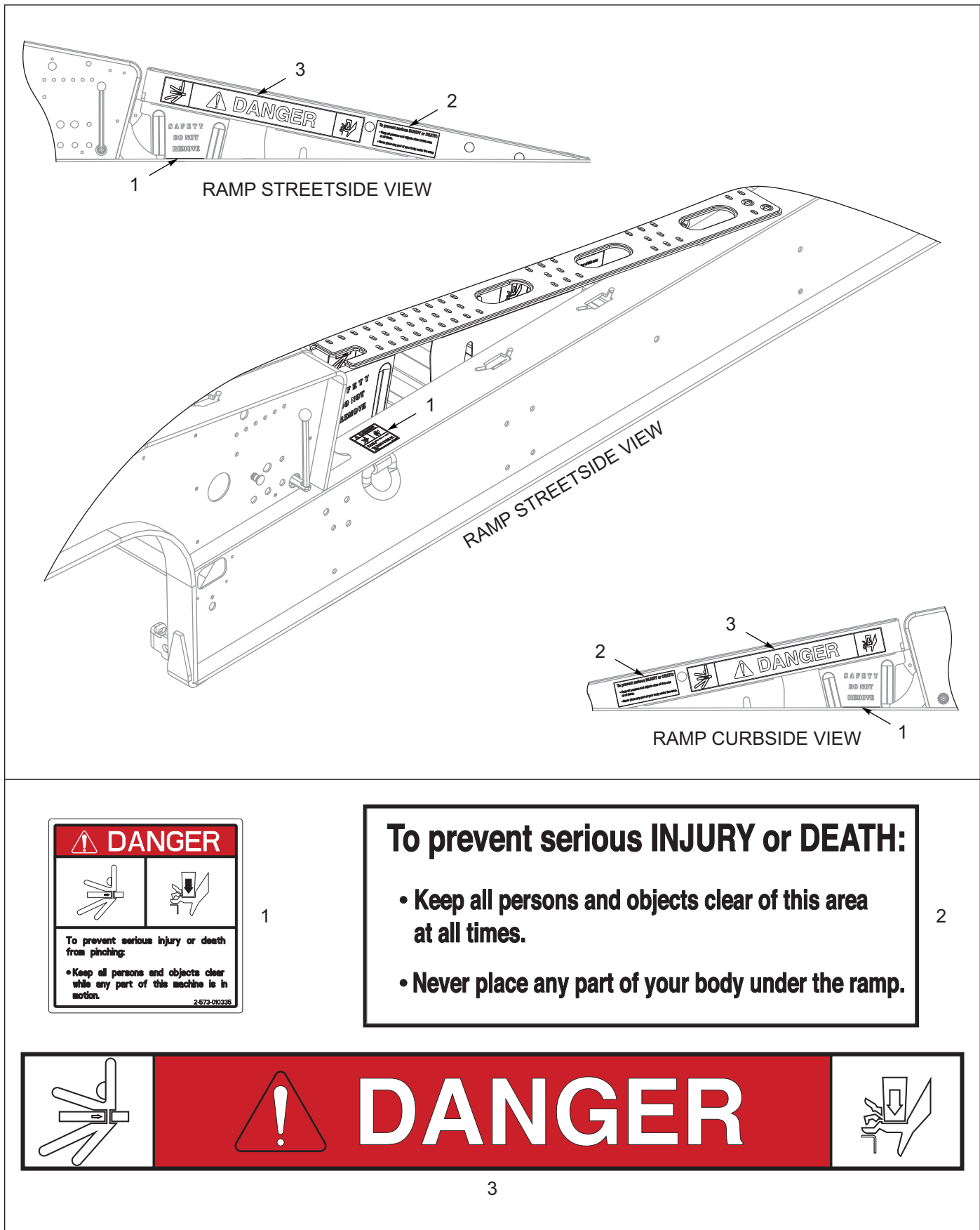
Figure 1-6: Decals, Ramp Assembly, Air 6FT
