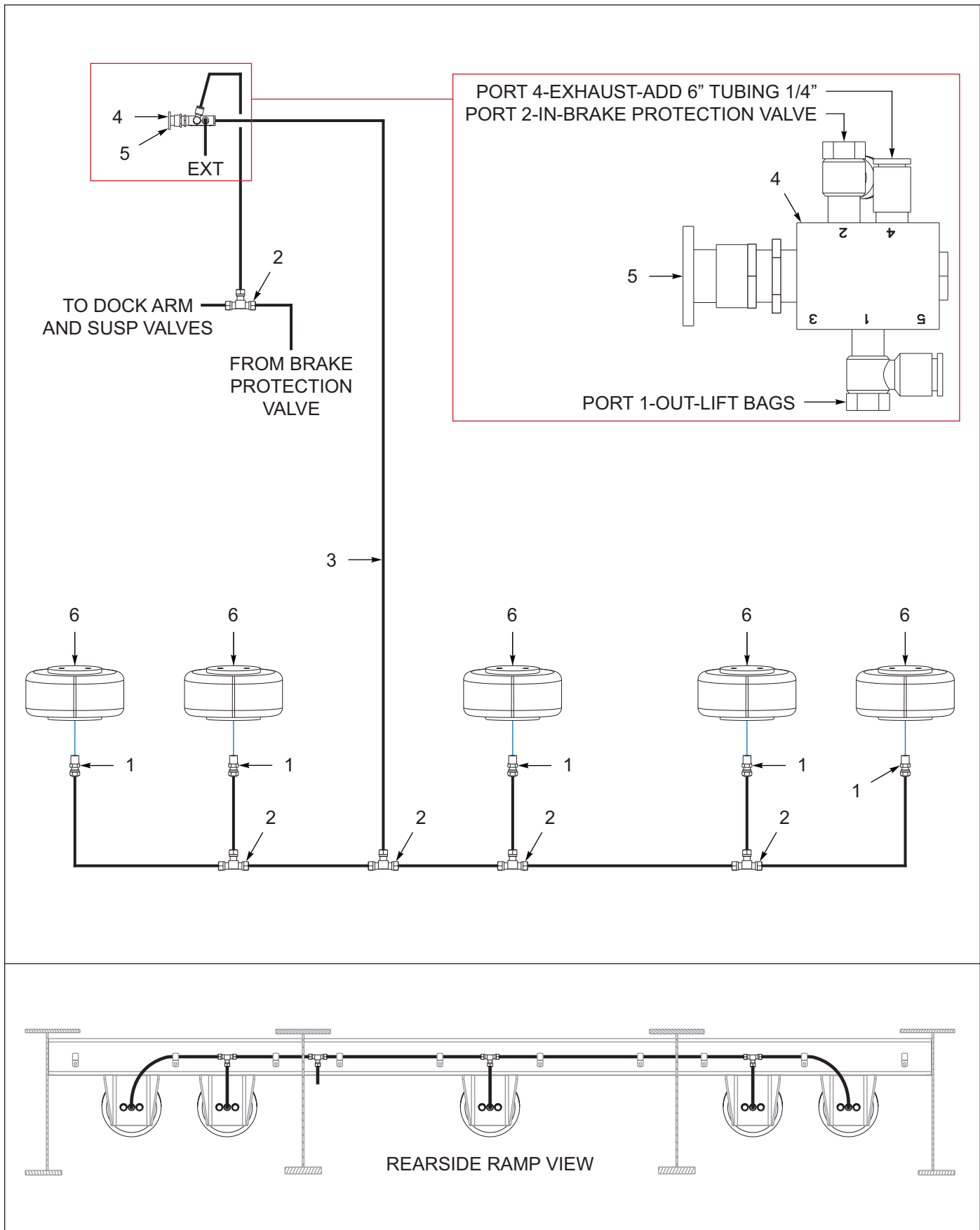
Figure 1-133: Front Slope, 6FT Air, Air System
