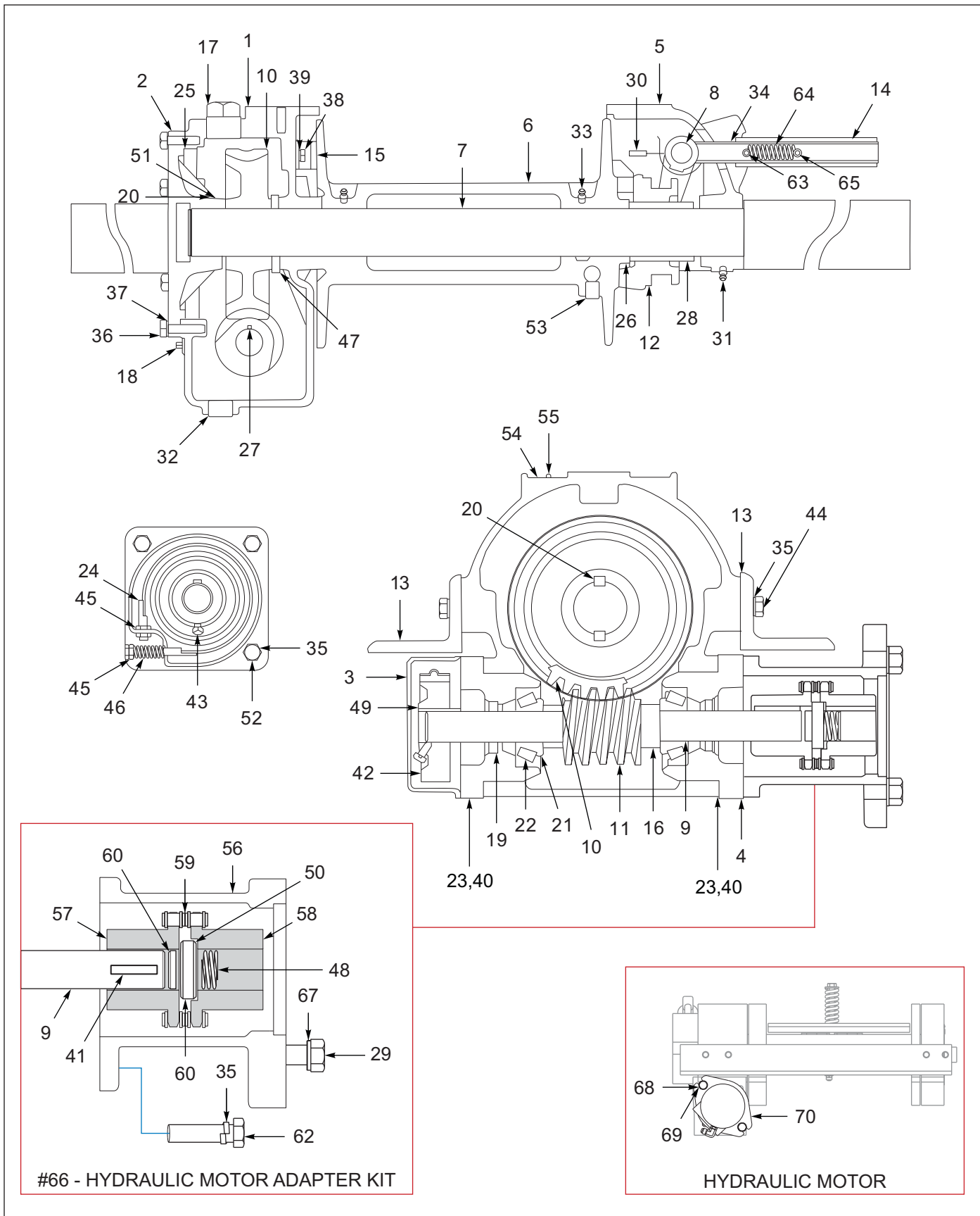
Figure 1-72: Winch Components, Braden 12K (OPTION)
