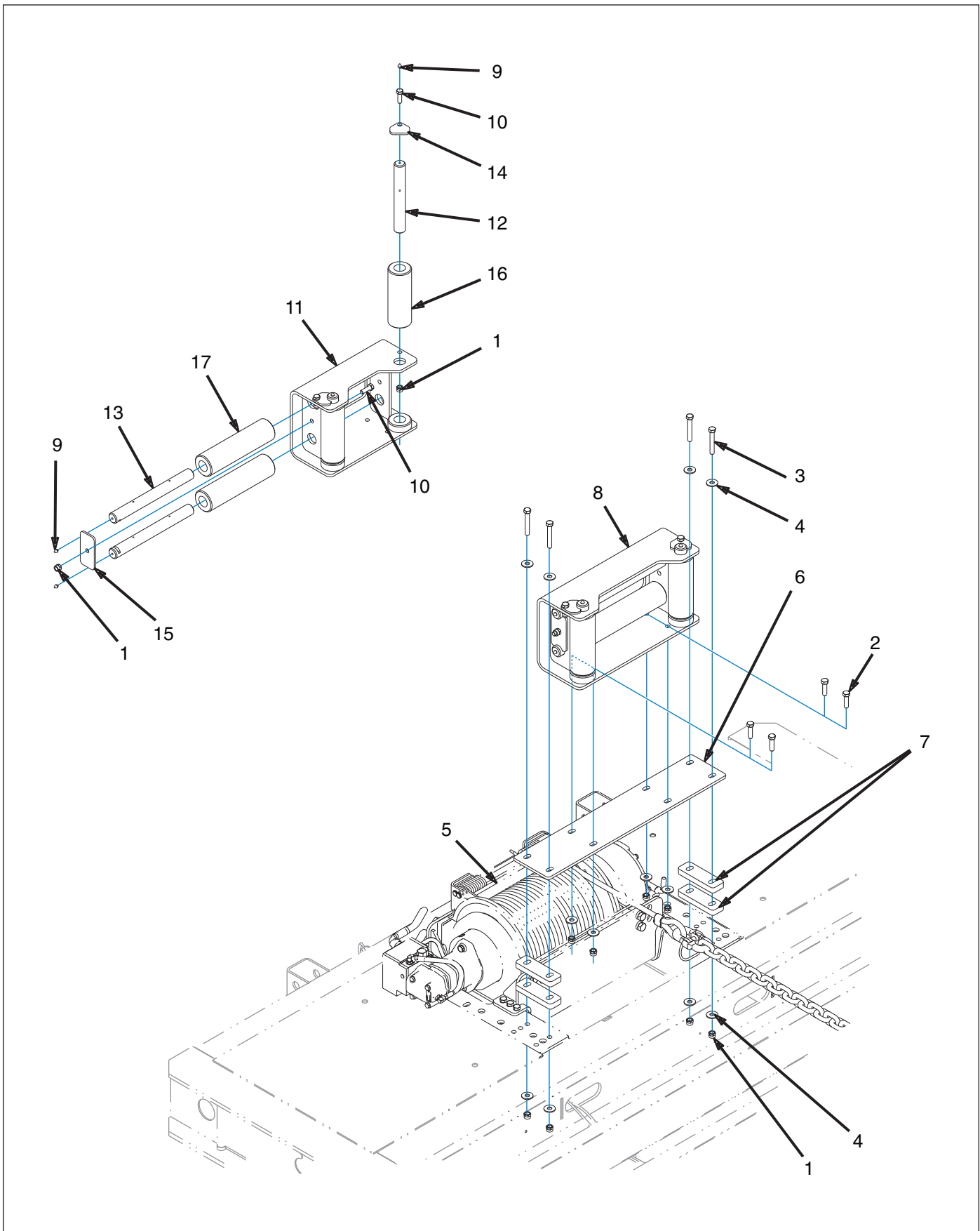
Figure 1-161: Guide Assembly, 4 Roller 20K/30K (WARN)
