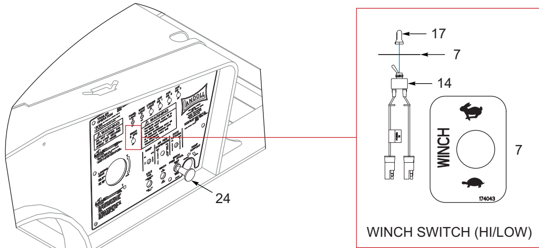
SWITCH LOCATIONS
