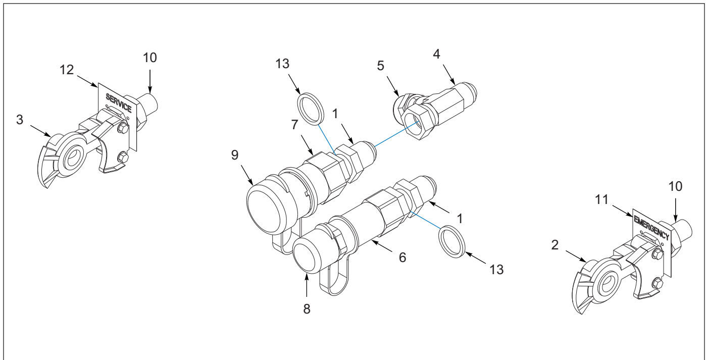
Figure 1-24: Connectors - Front Sub Assembly
