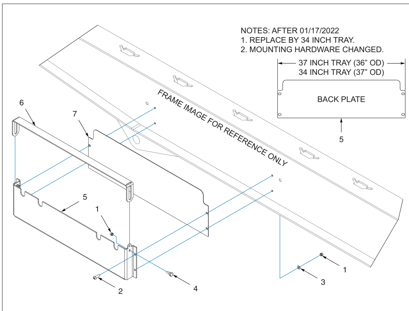
Figure 1-146: Chain Tray Assembly (BEFORE 01/17/2022)
