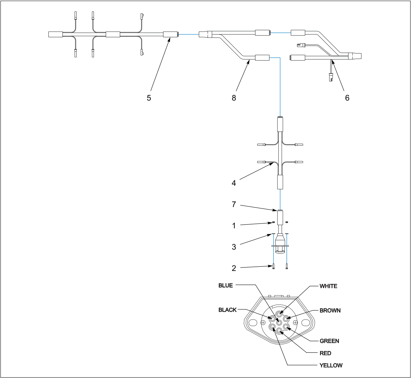
Figure 1-103: 7-Way Electrical Installation
