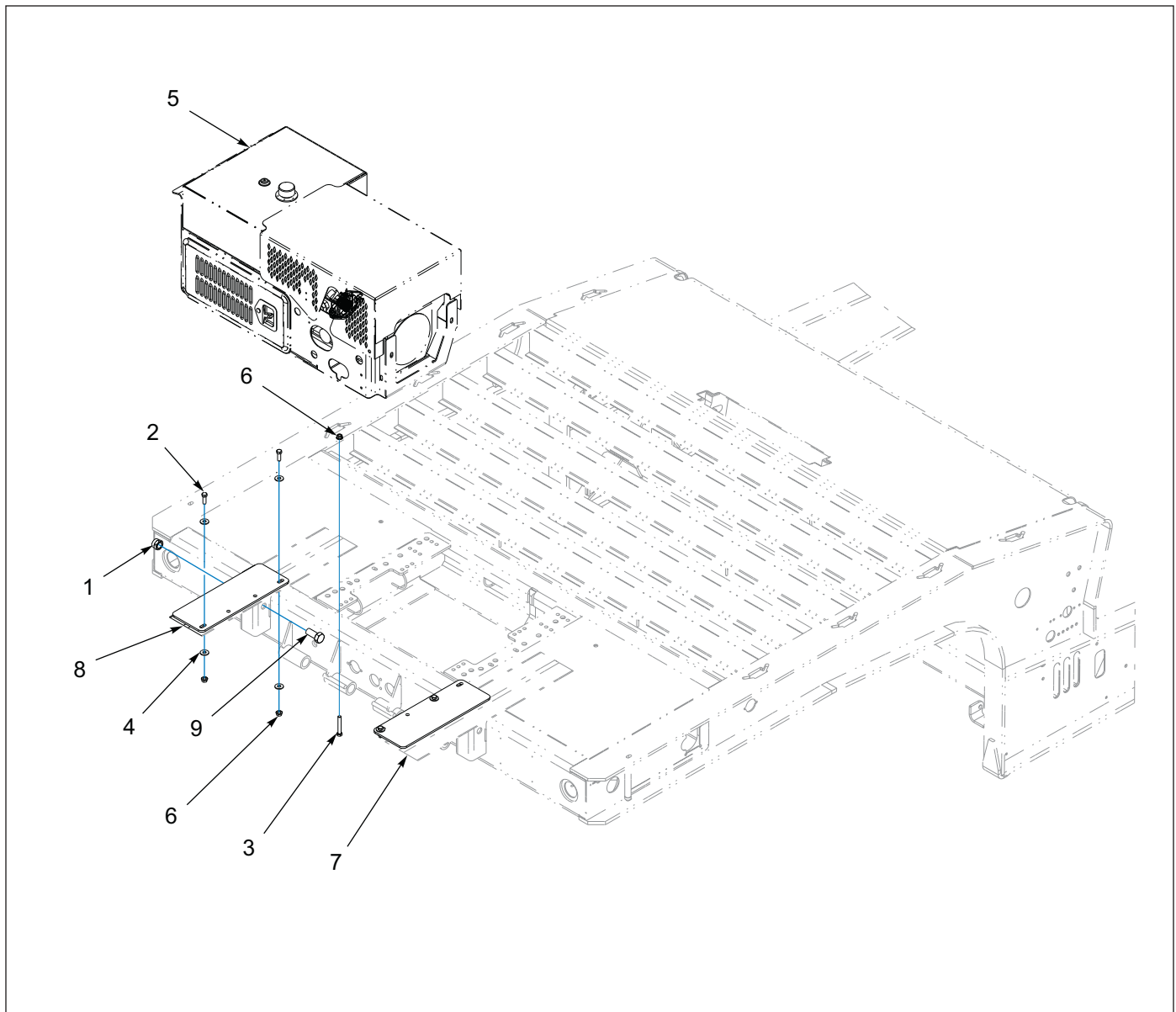
Figure 1-116: Front Mount Installation
