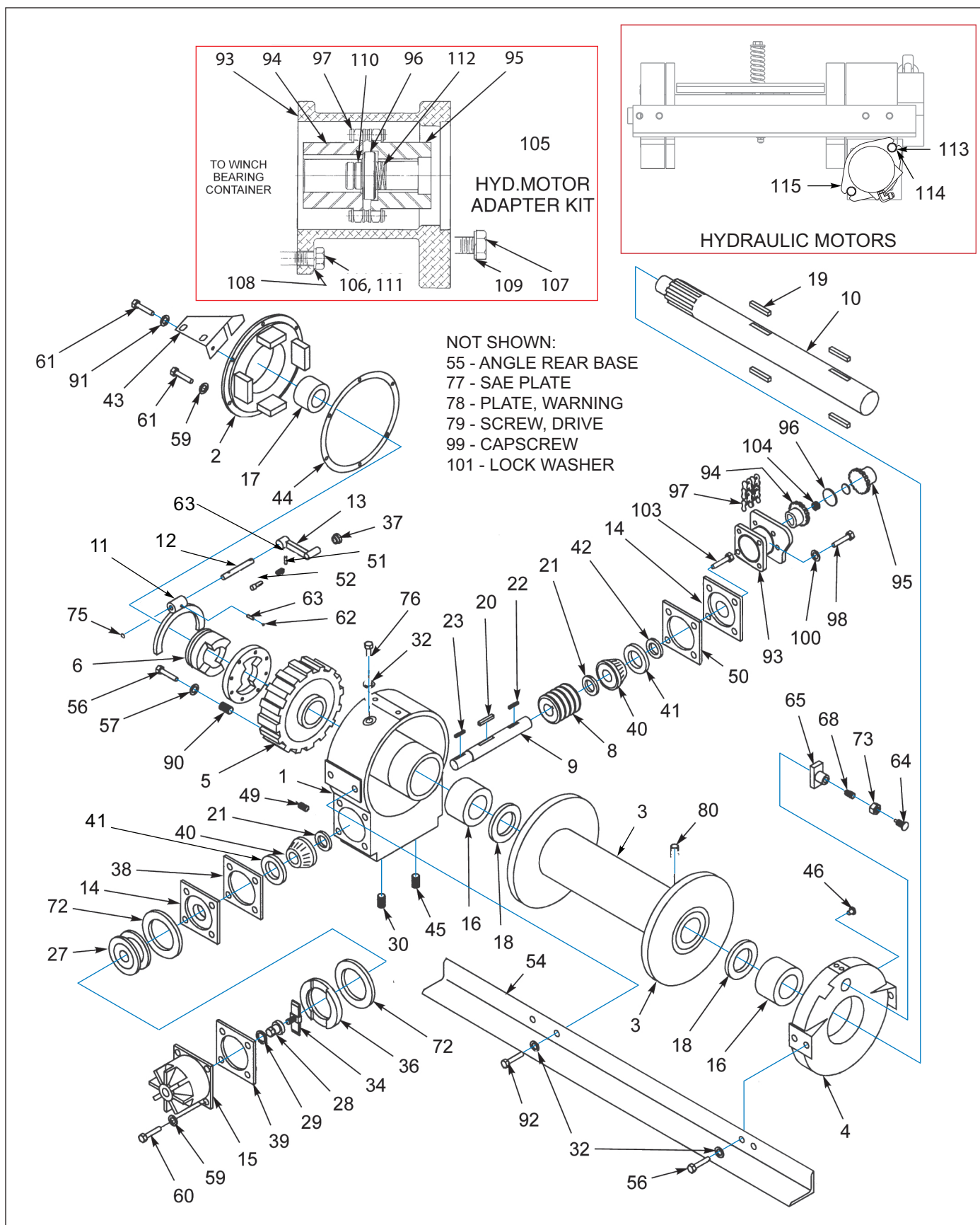
Figure 1-77: Winch Components, Braden 20K (OPTION)
