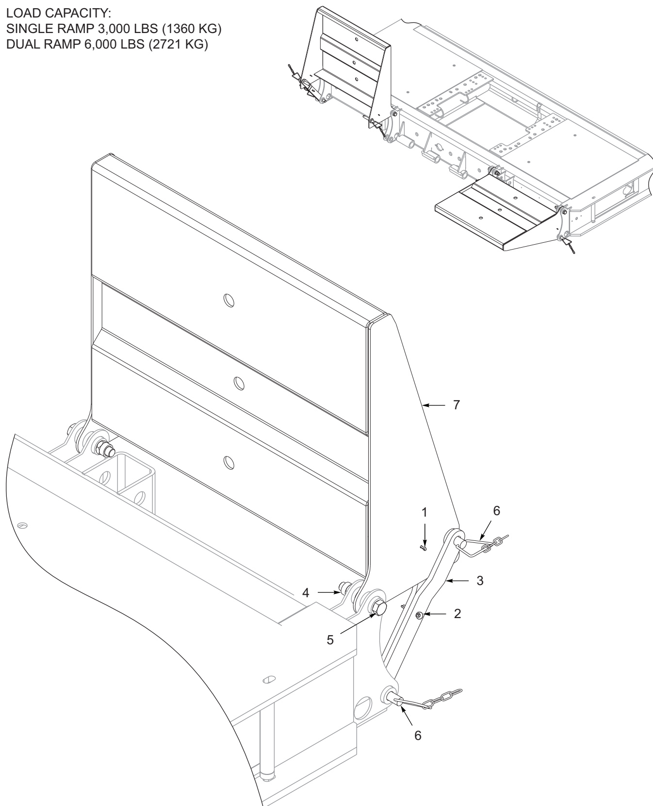
Figure 1-152: Front Flip Extension Assembly
