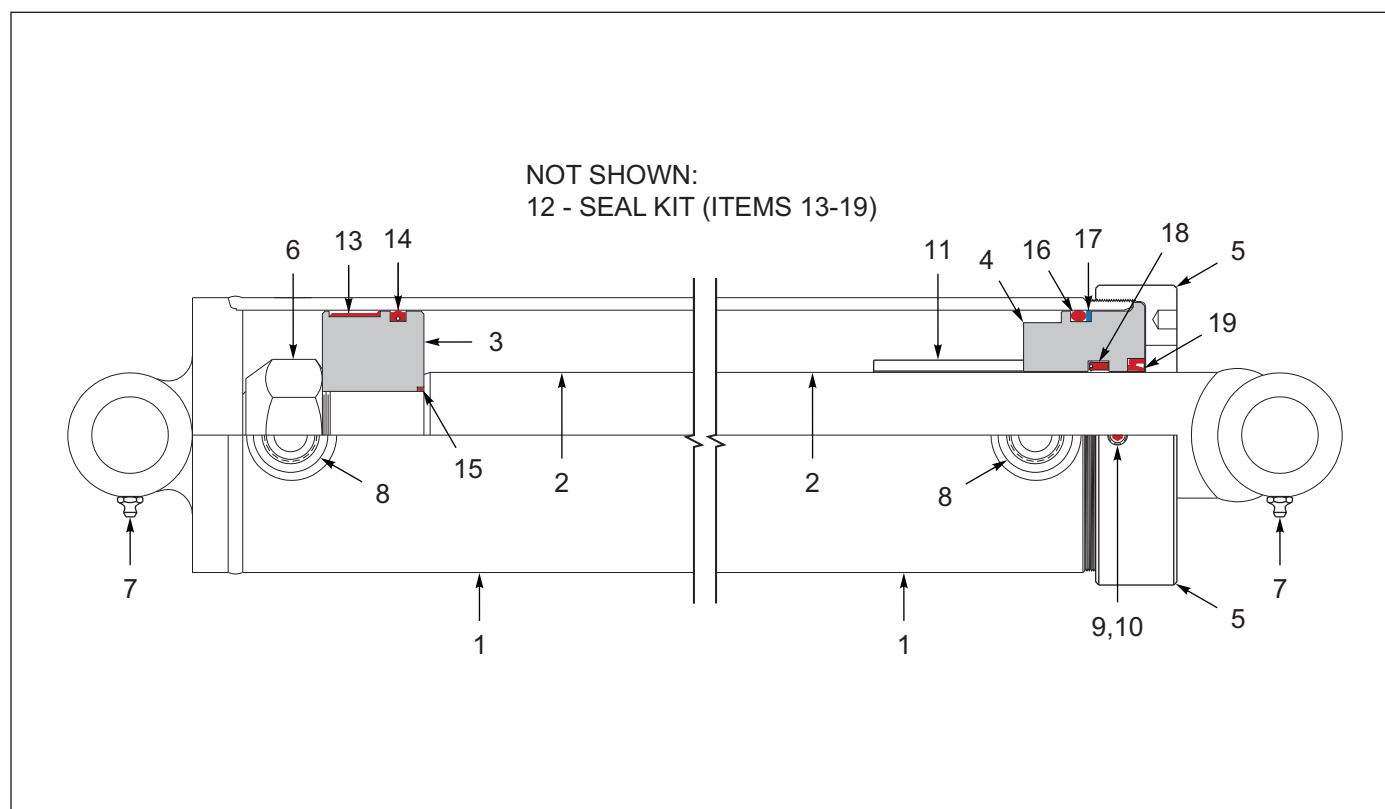
Figure 1-23: Cylinder - 5 X 60
