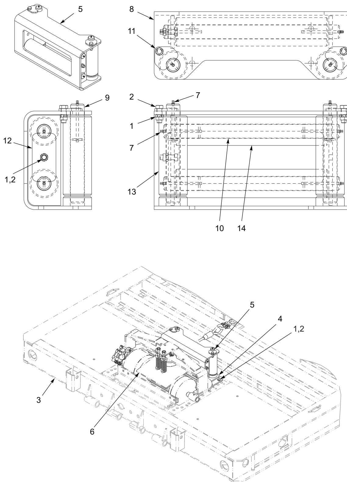
Figure 1-158: Guide Assembly, 4 Roller 20K(BRADEN)
