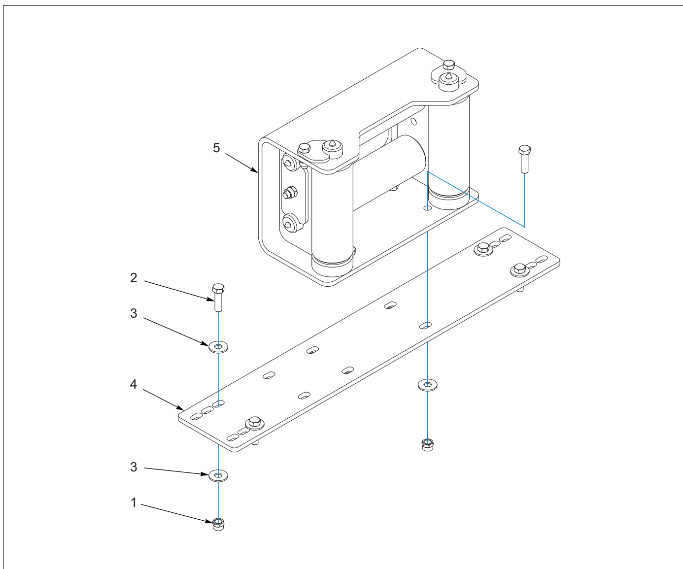
Figure 1-159: Guide Assembly, 4 Roller 12K (BRADEN) Installation
