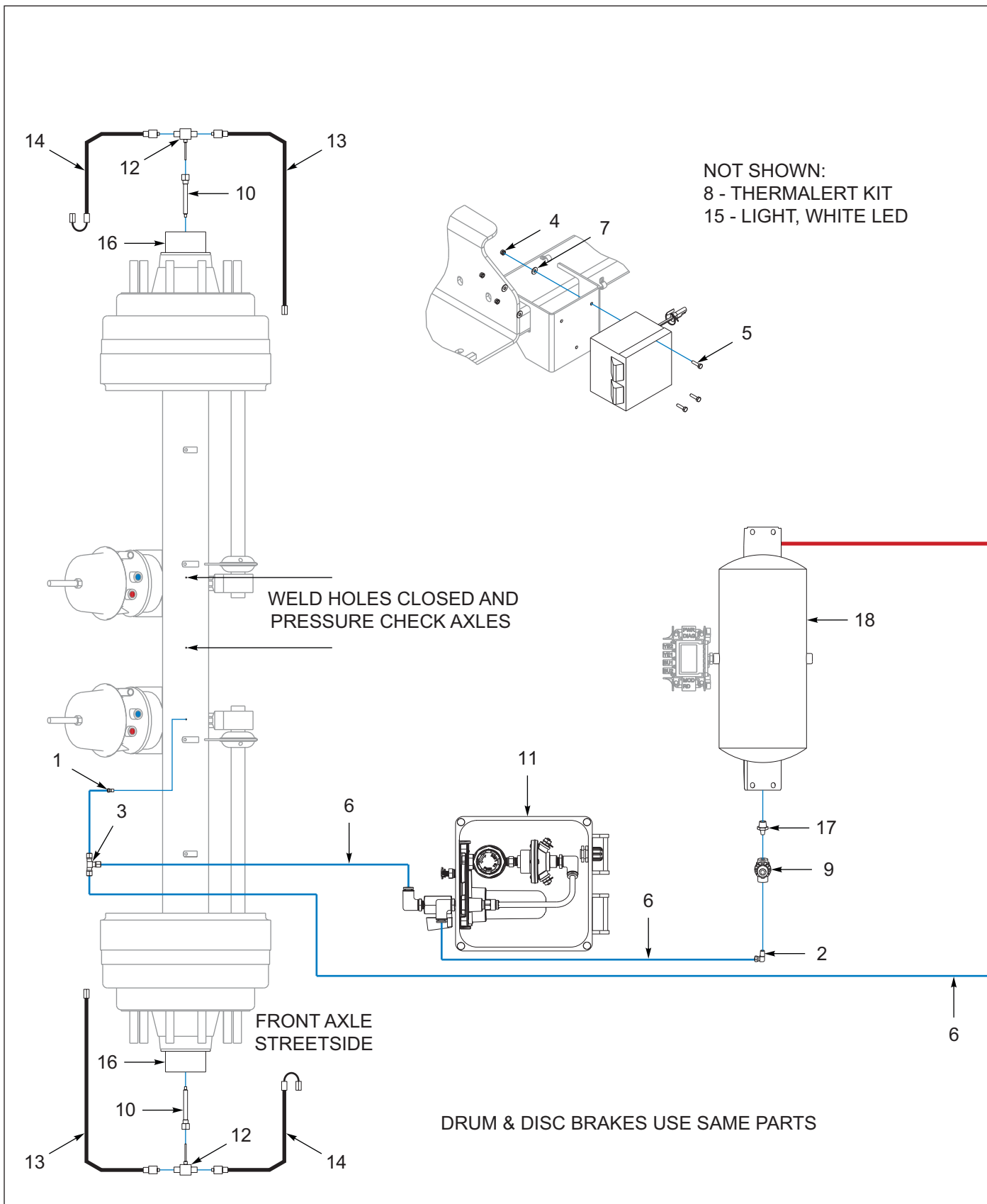
Figure 1-64: Thermalert, 2 Axle Air System (OPTION) (1 of 2)
