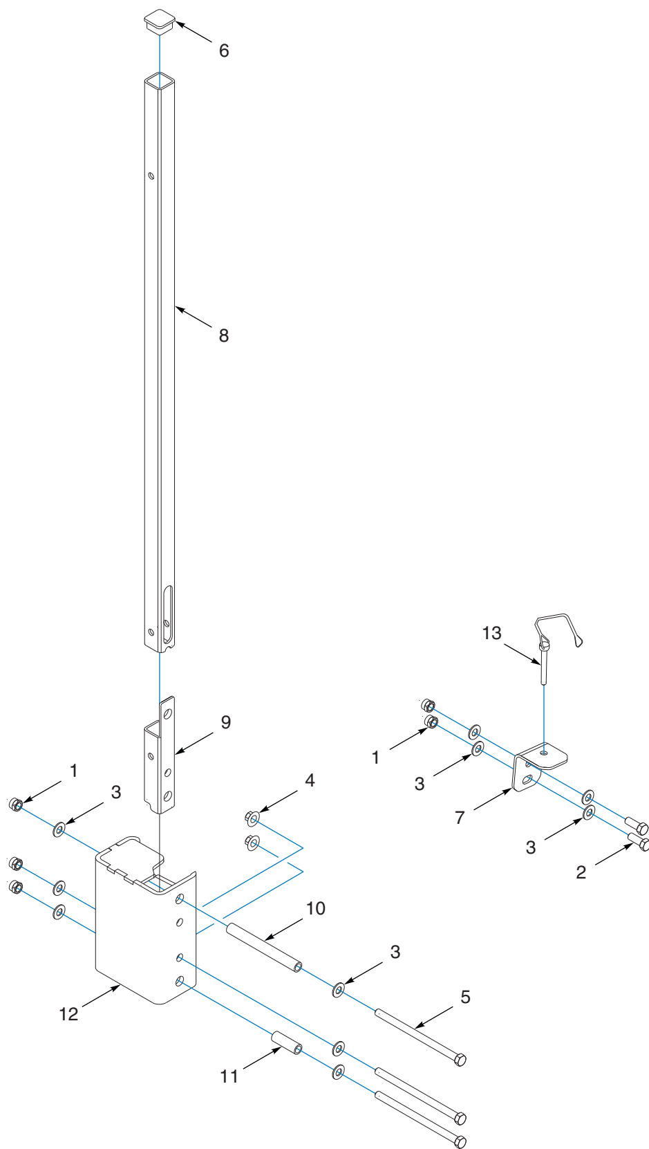
Figure 1-143: Step, Folding Handle Assembly
