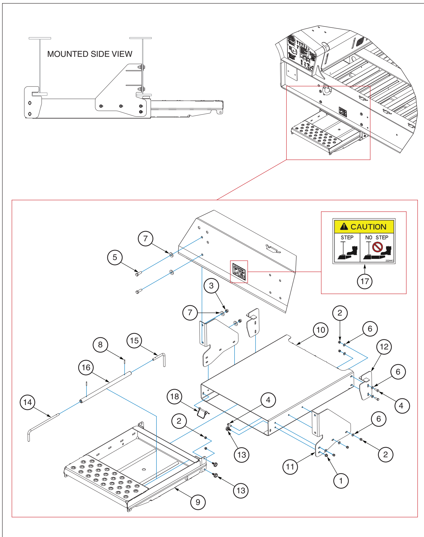
Figure 1-145: Step Drawer, Retractable Assembly
