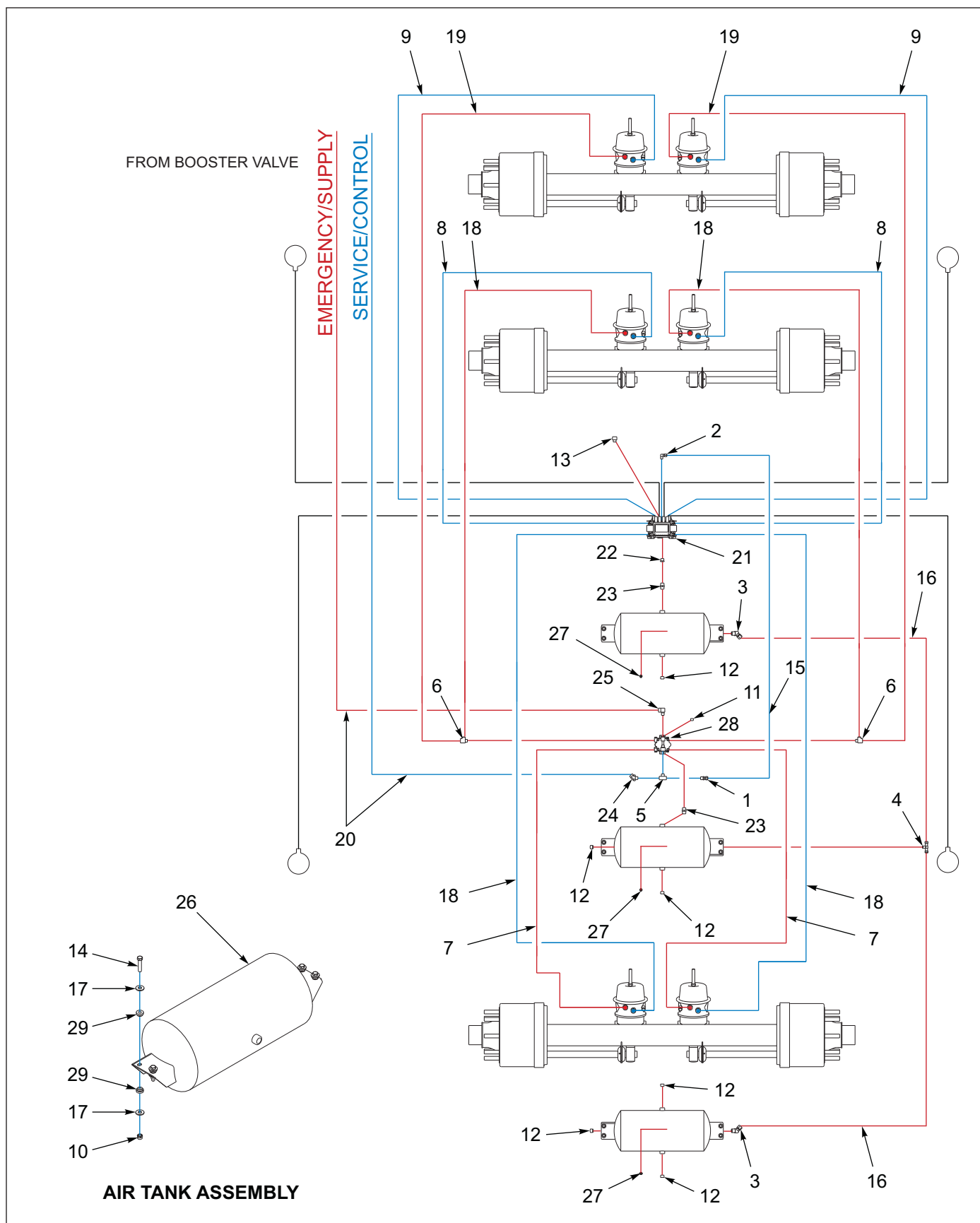
Figure 1-62: 950E-Air Brake System
