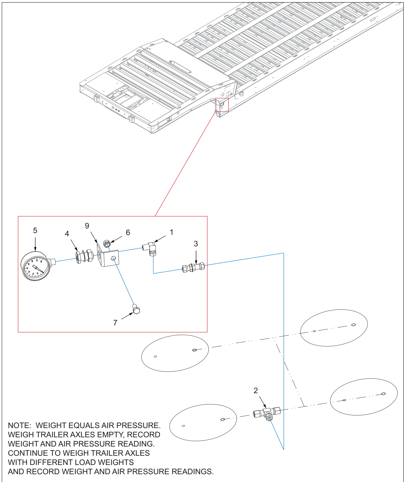
Figure 1-136: Air Pressure Gauge Assembly
