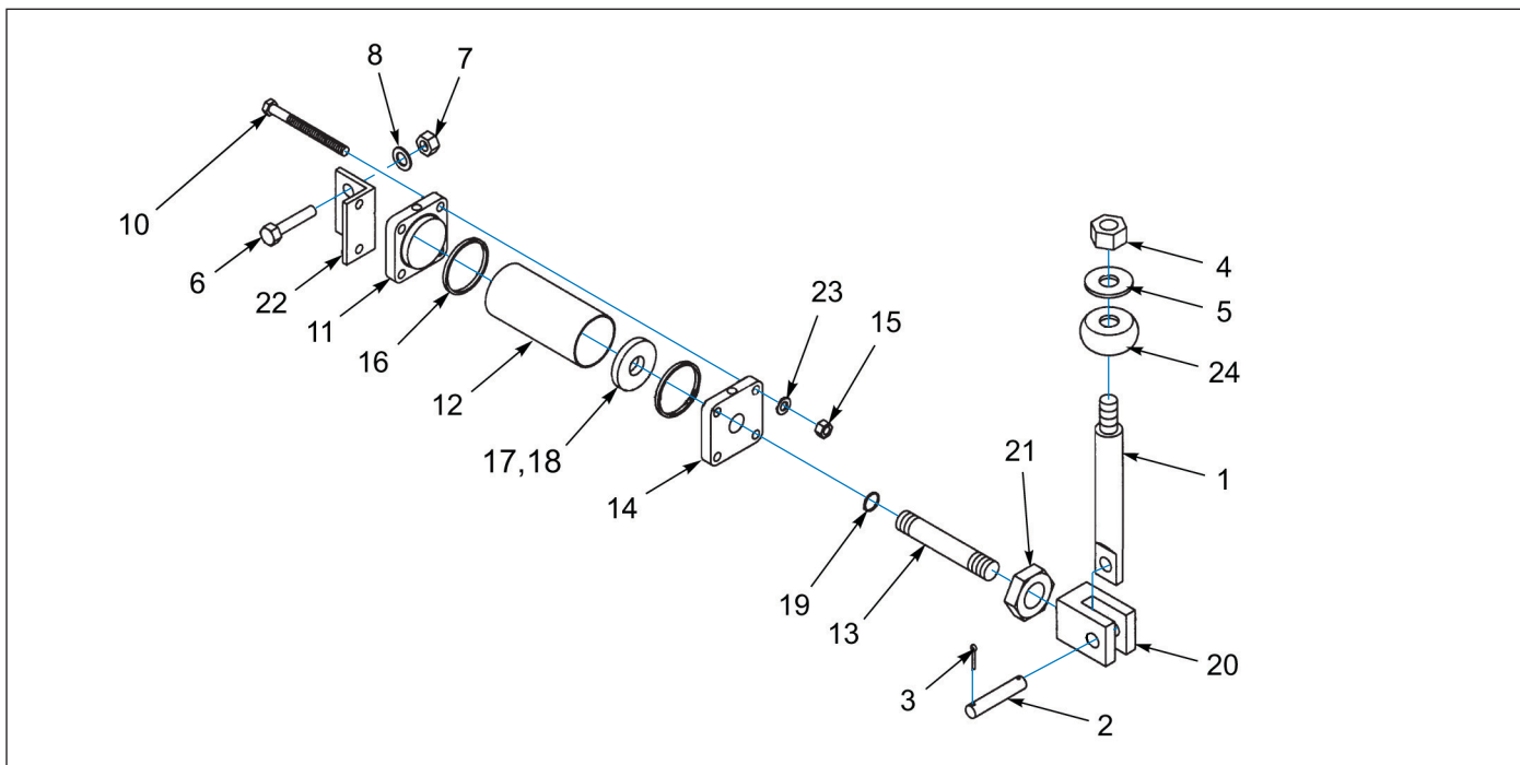
Figure 1-79: Winch Air Shift Cylinder Components, Braden 20K (OPTION)
