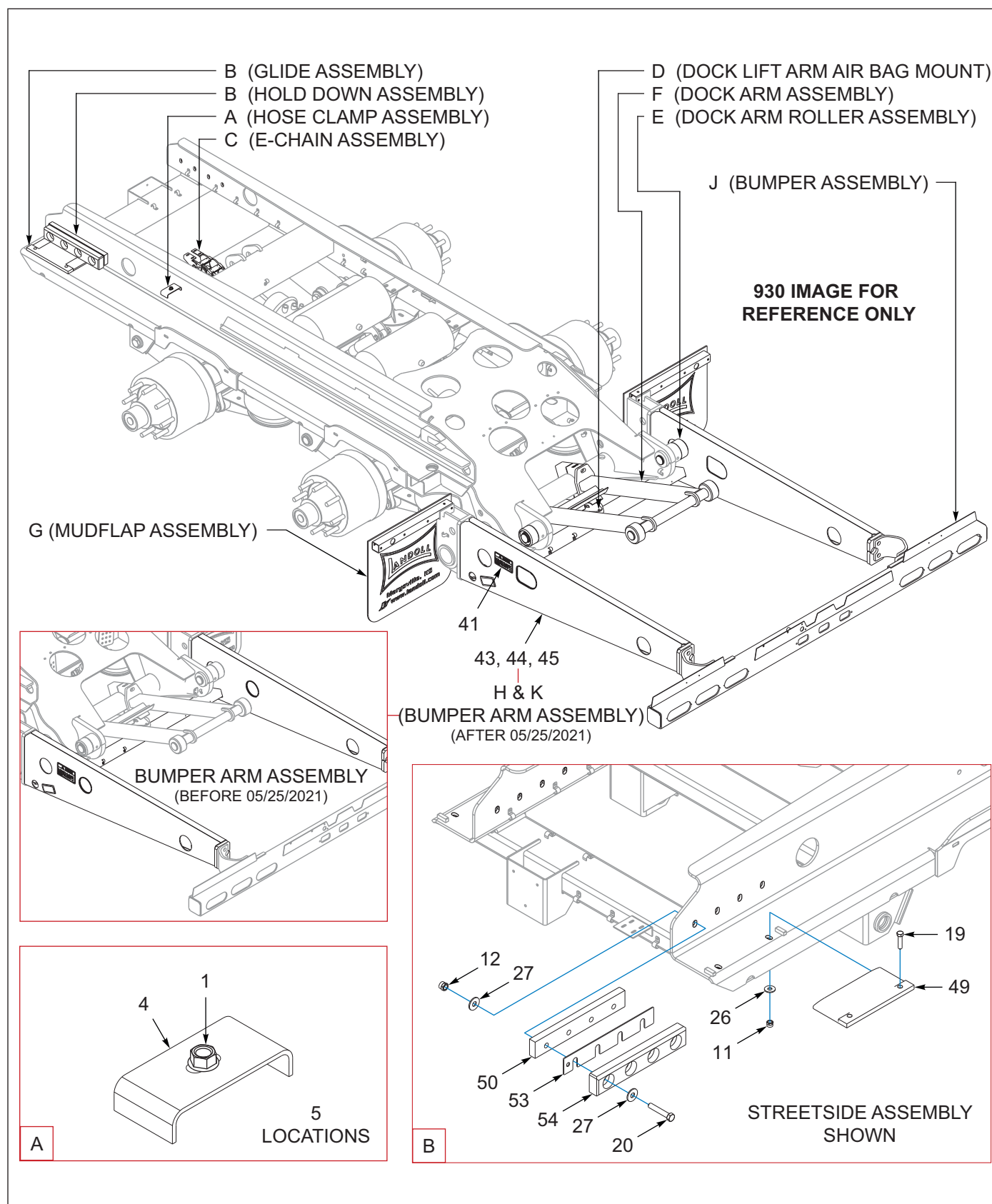
Figure 1-28: Undercarriage Components (1 of 3)
