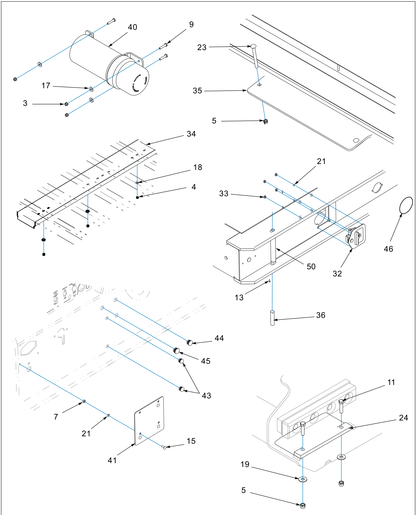
Figure 1-9: Frame Assembly (3 of 3)
