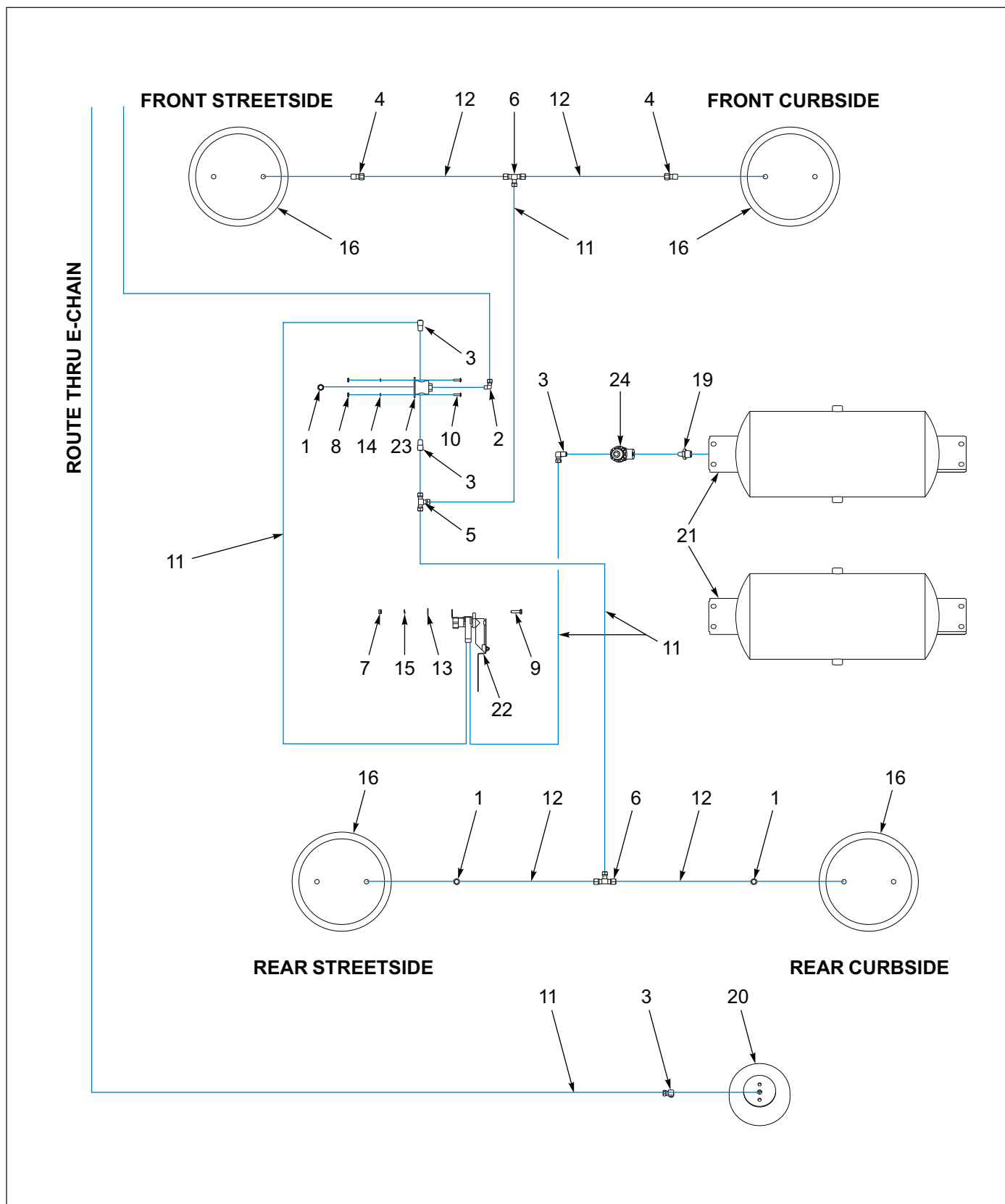
Figure 1-41: 930E-Air Ride Suspension
