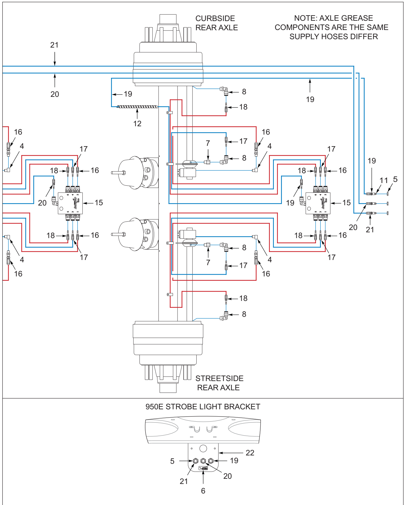
Figure 1-39: Grease System, 3 Axle (After 08/31/2020) (2 of 3)
