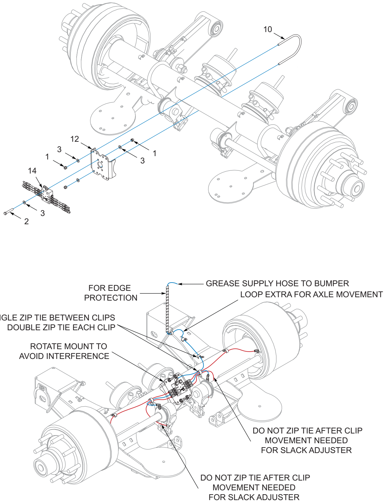
Figure 1-40: Grease System, 3 Axle (After 08/31/2020) (3 of 3)
