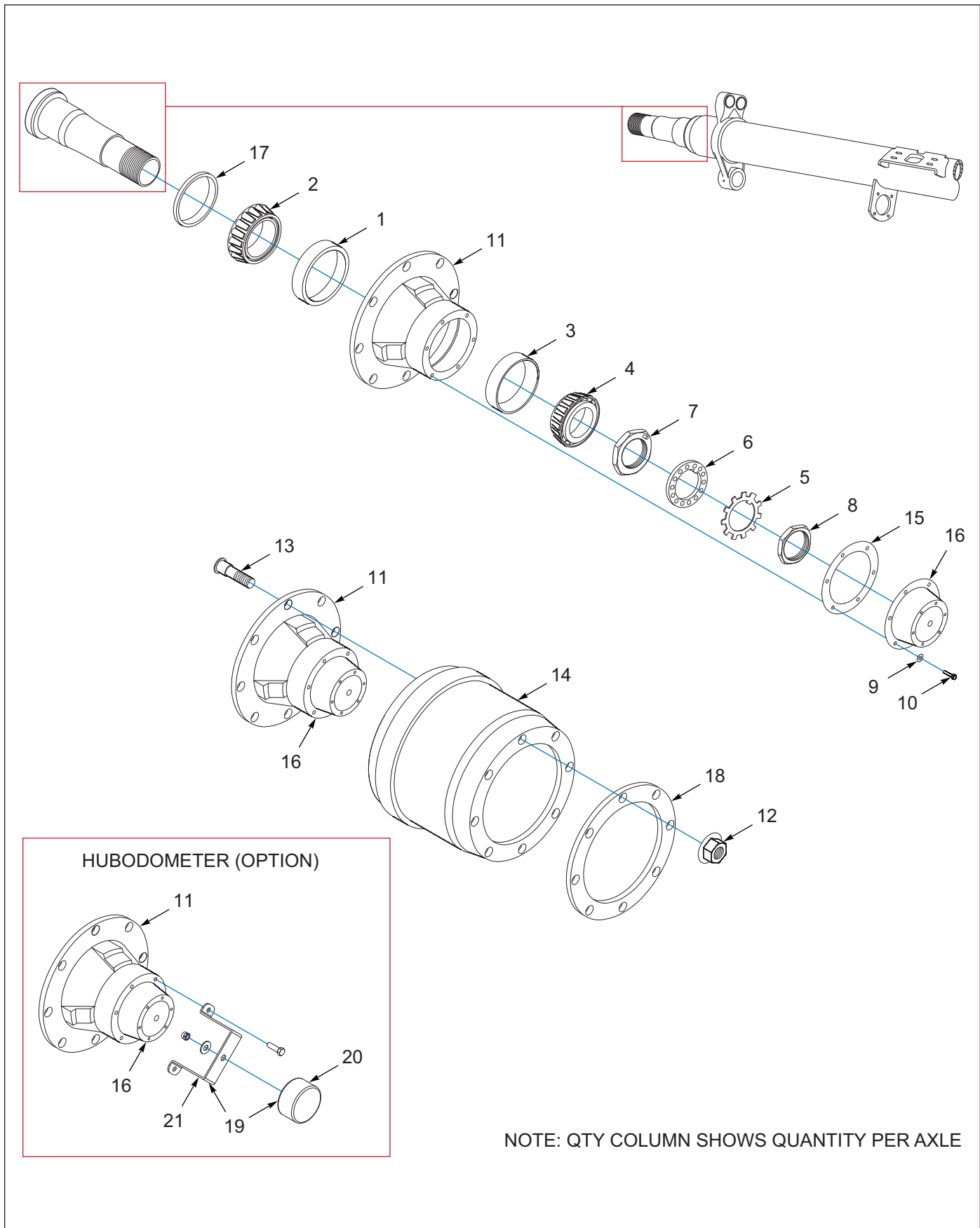
Figure 1-55: Axle 12.25 x 7.5 Drum and Hub Assembly, Dexter
