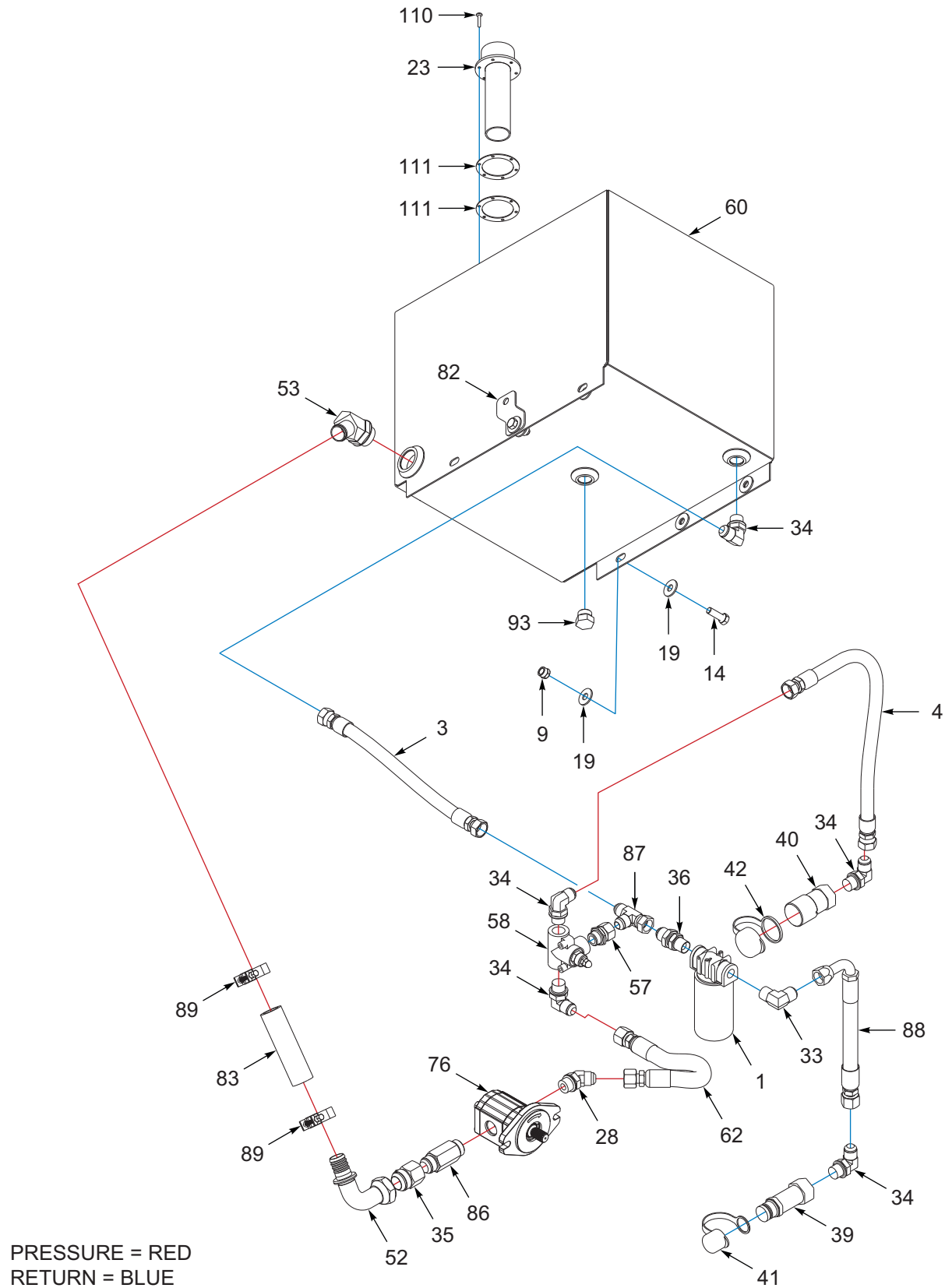
Figure 1-110: 25 HP Upper Deck Package (5 of 5)
