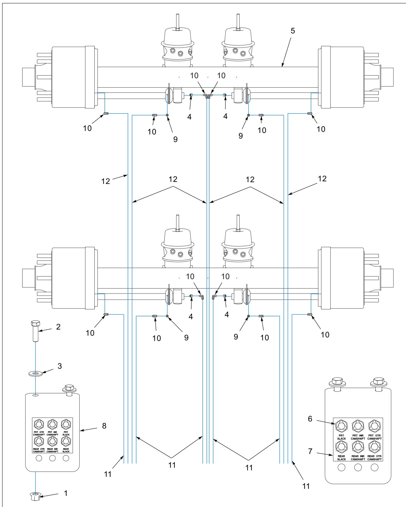
Figure 1-31: Grease System, 2 Axle (Before 11/07/2018)
