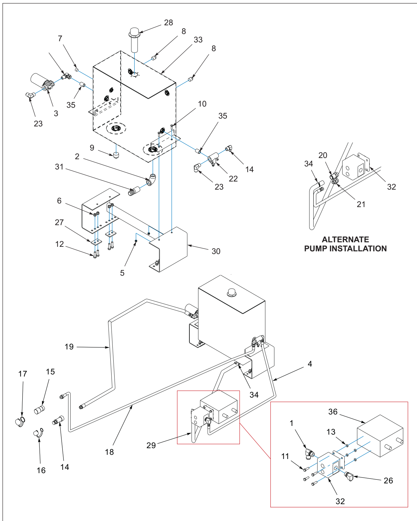
Figure 1-121: Hydraulic Wet Kit Items - 30 Gallon
