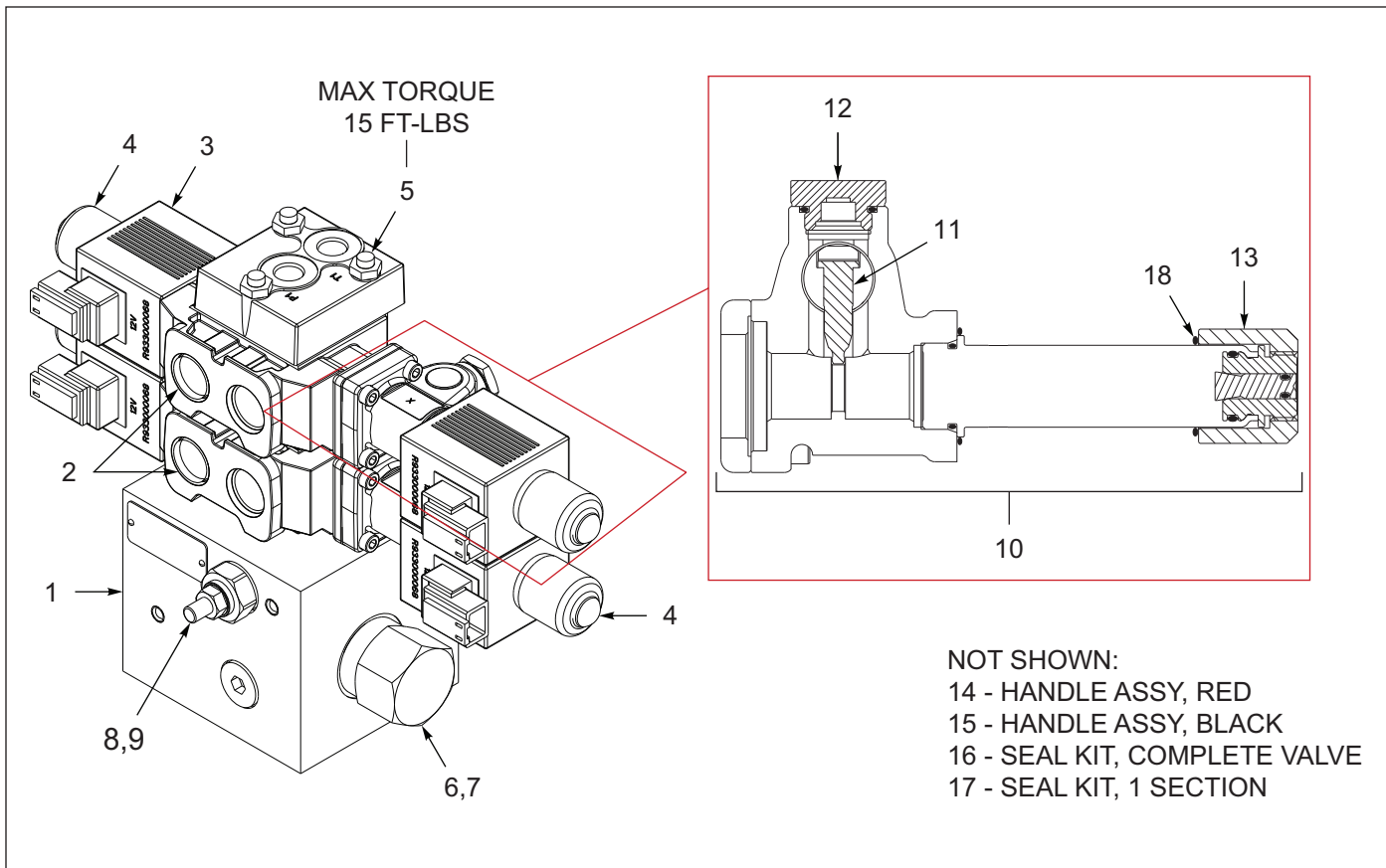
Figure 1-27: Valve Assembly - 2 Spool Solenoid
