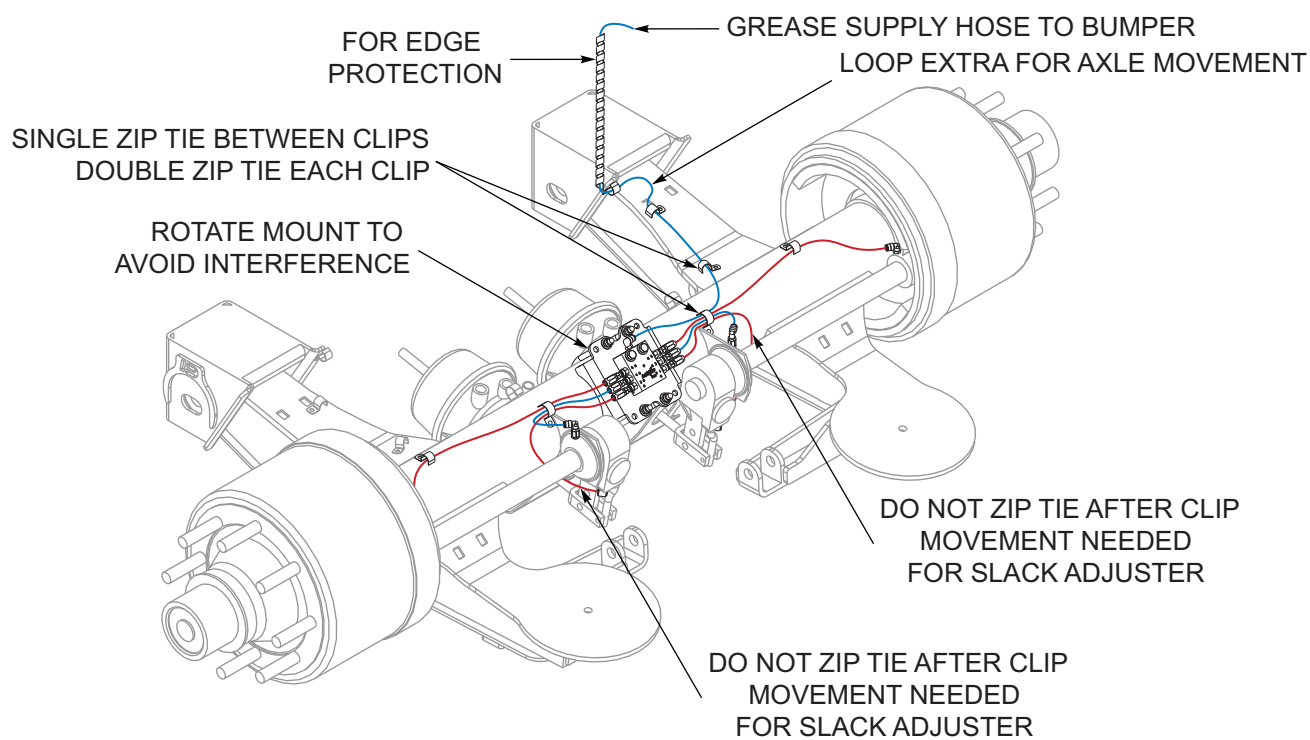
Figure 1-35: Grease System, 2 Axle (After 08/31/2020) (3 of 3)
