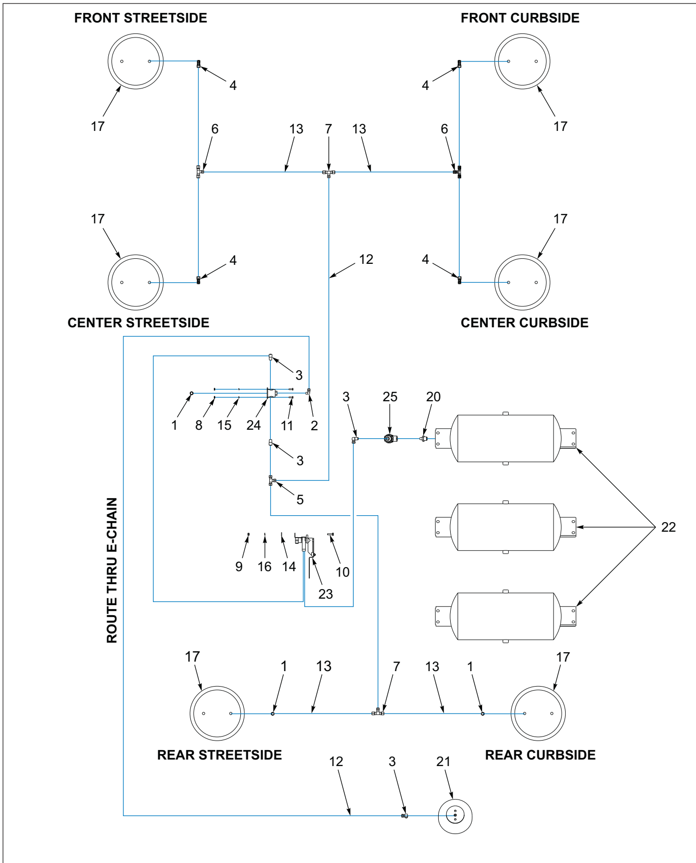
Figure 1-42: 950E-Air Ride Suspension
