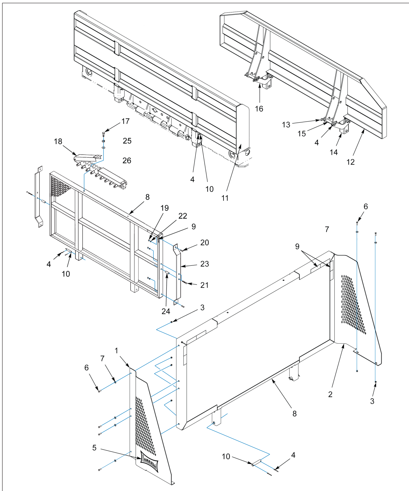
Figure 1-90: Bulkhead Assembly
