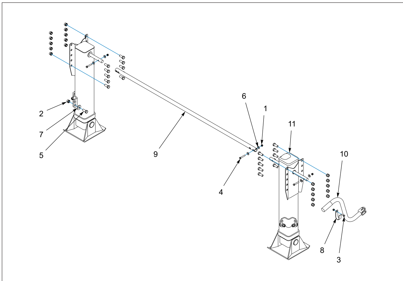
Figure 1-88: Jost 410
