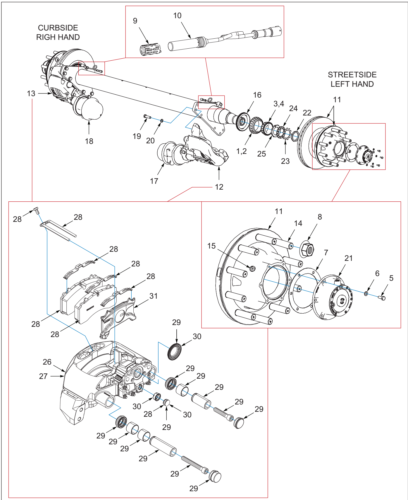
Figure 1-56: Axle 16.5 Disc Brakes & Hub Assembly, Dexter (OPTION) (1 of 2)
