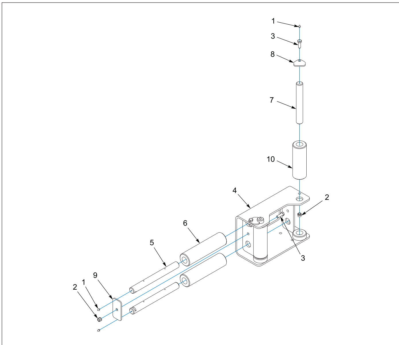
Figure 1-160: Guide Assembly, 4 Roller 12K (BRADEN) Assembly
