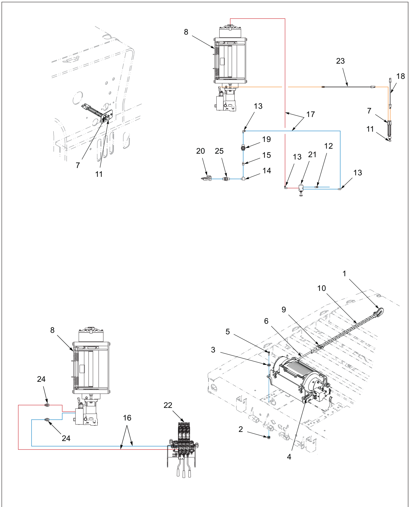
Figure 1-85: Winch Installation, Warn 30K, 2 Speed (OPTION)
