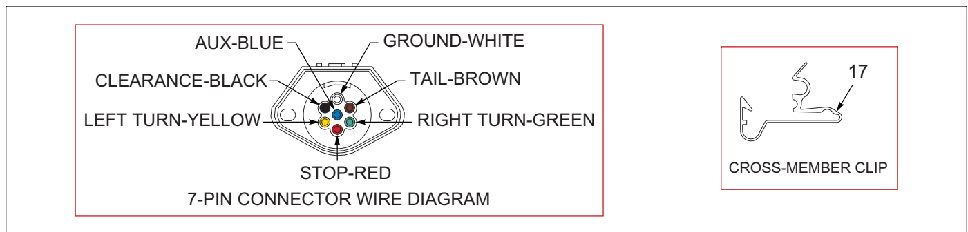
Figure 1-18: Electrical System - Trailer (Before 02/15/2022) (2 of 2)
