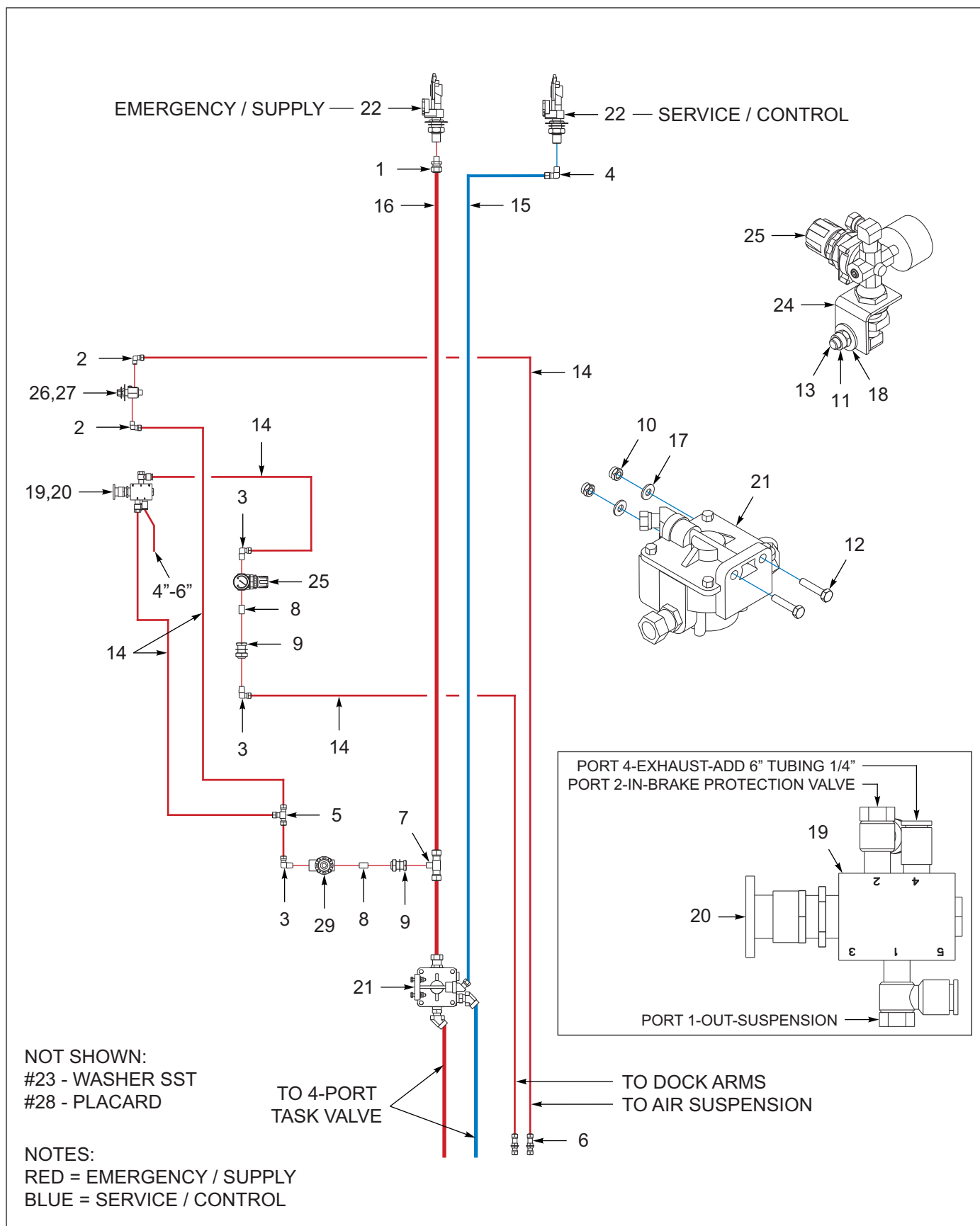
Figure 1-15: Air System - Booster Valve
