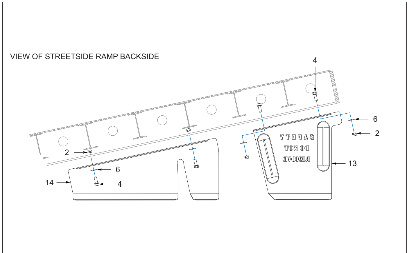
Figure 1-130: Front Slope, 6FT Air (2 of 2) (AFTER 03/11/2021)
