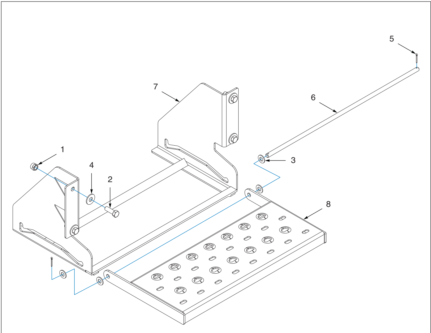
Figure 1-144: Step. Retractable Assembly
