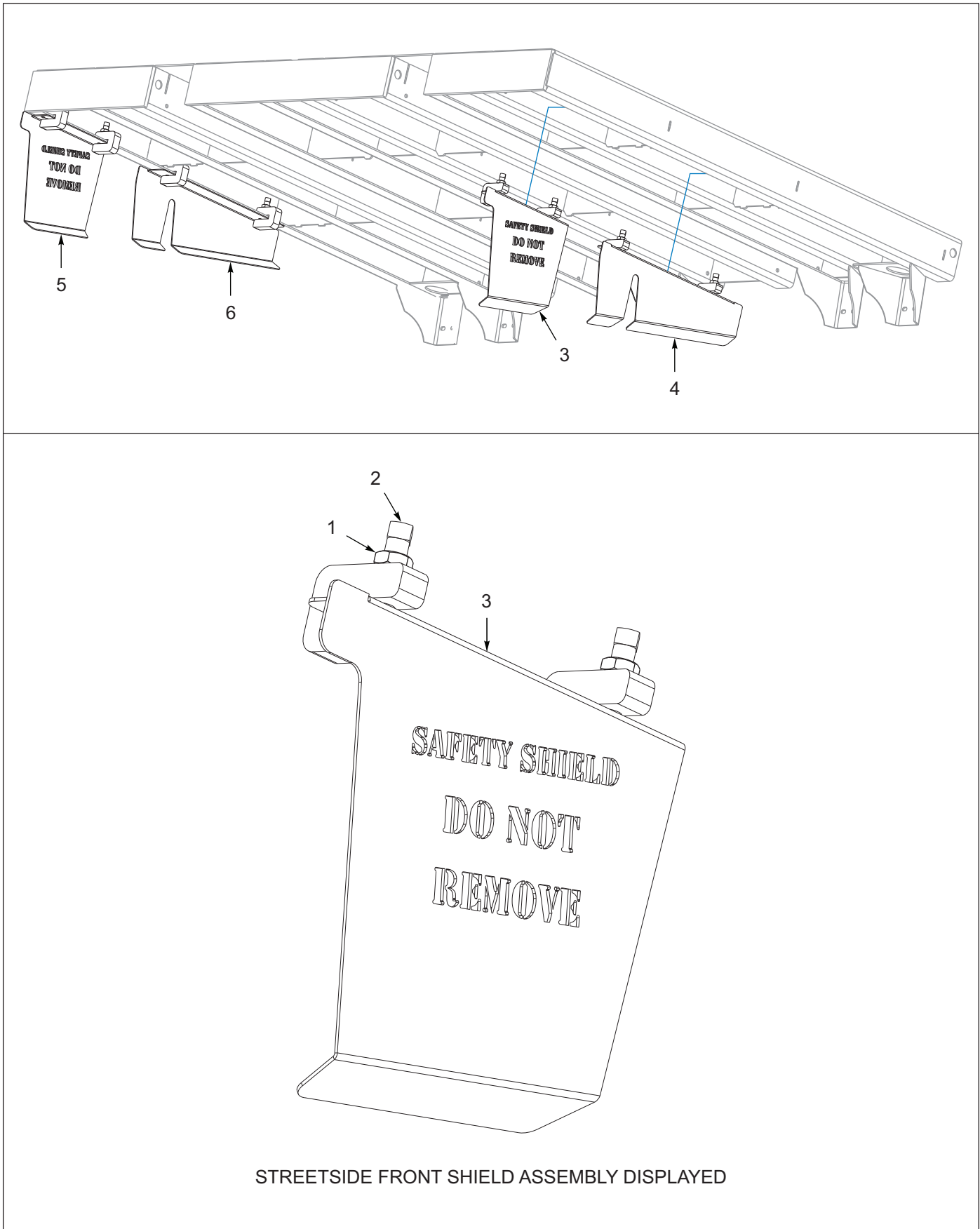
Figure 1-135: Front Slope, 6FT Air, Safety Shield Assembly, Clamp-On
