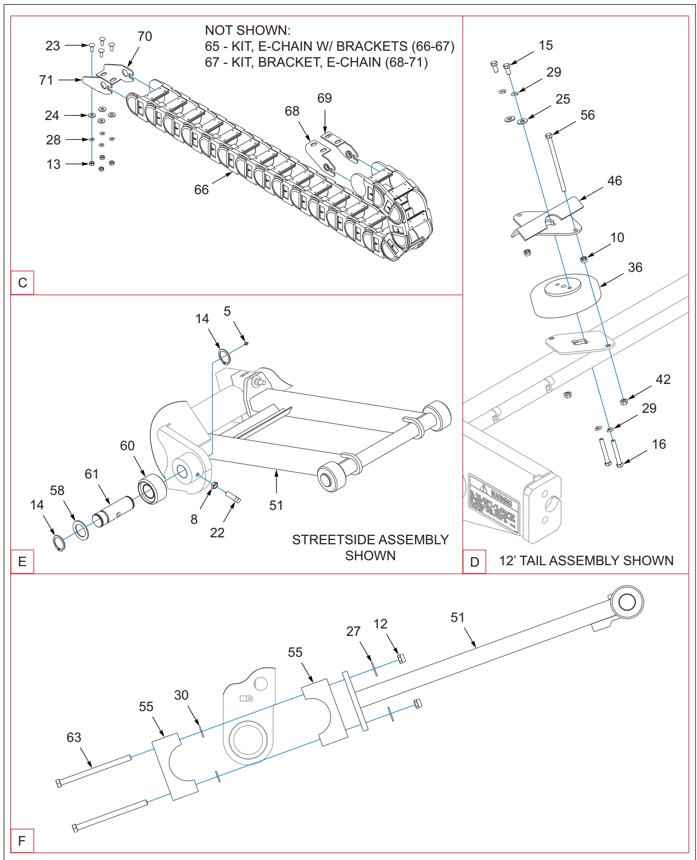
Figure 1-29: Undercarriage Components (2 of 3)
