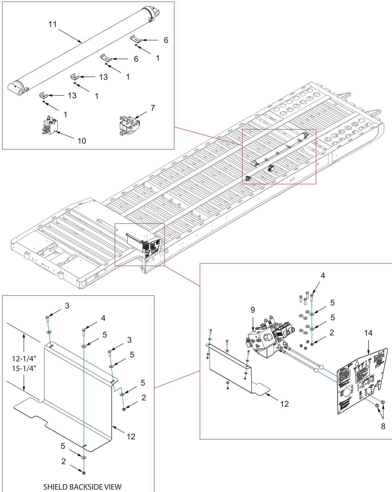
Figure 1-13: General Assembly - Hydraulic, Electric, Air
