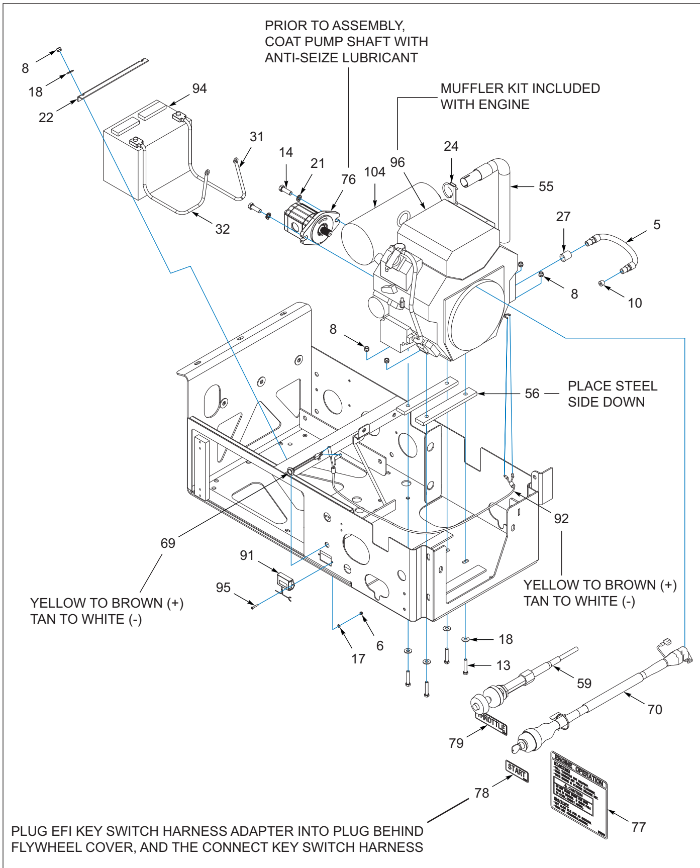
Figure 1-108: 25 HP Upper Deck Package (3 of 5)
