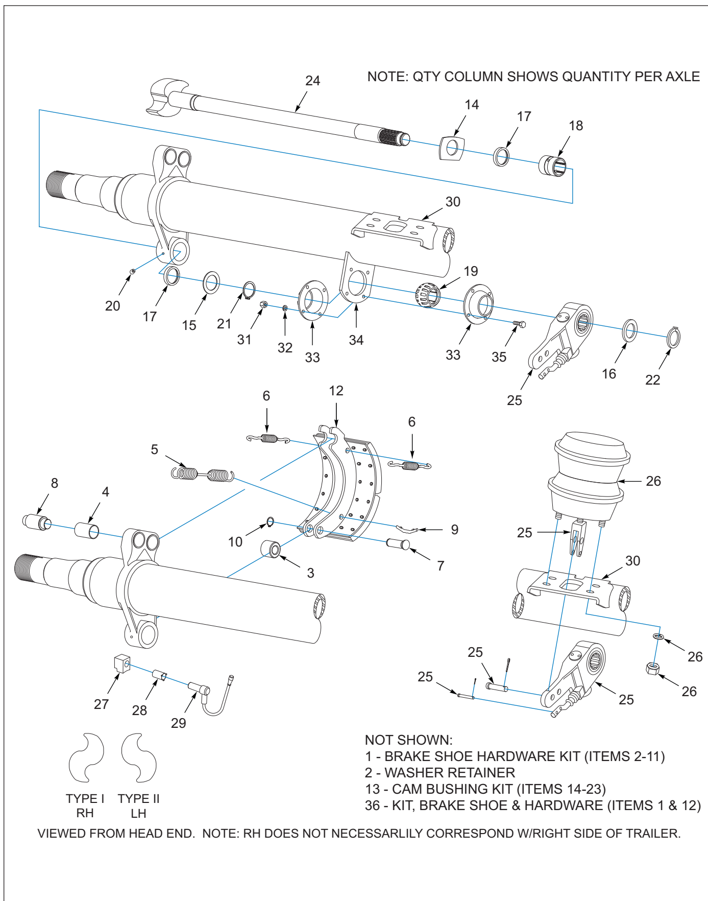
Figure 1-54: Axle 12.25 x 7.5 Drum Brakes, Dexter
