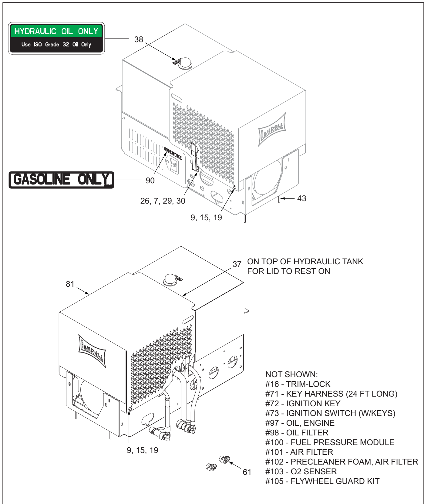
Figure 1-106: 25 HP Upper Deck Package (1 of 5)
