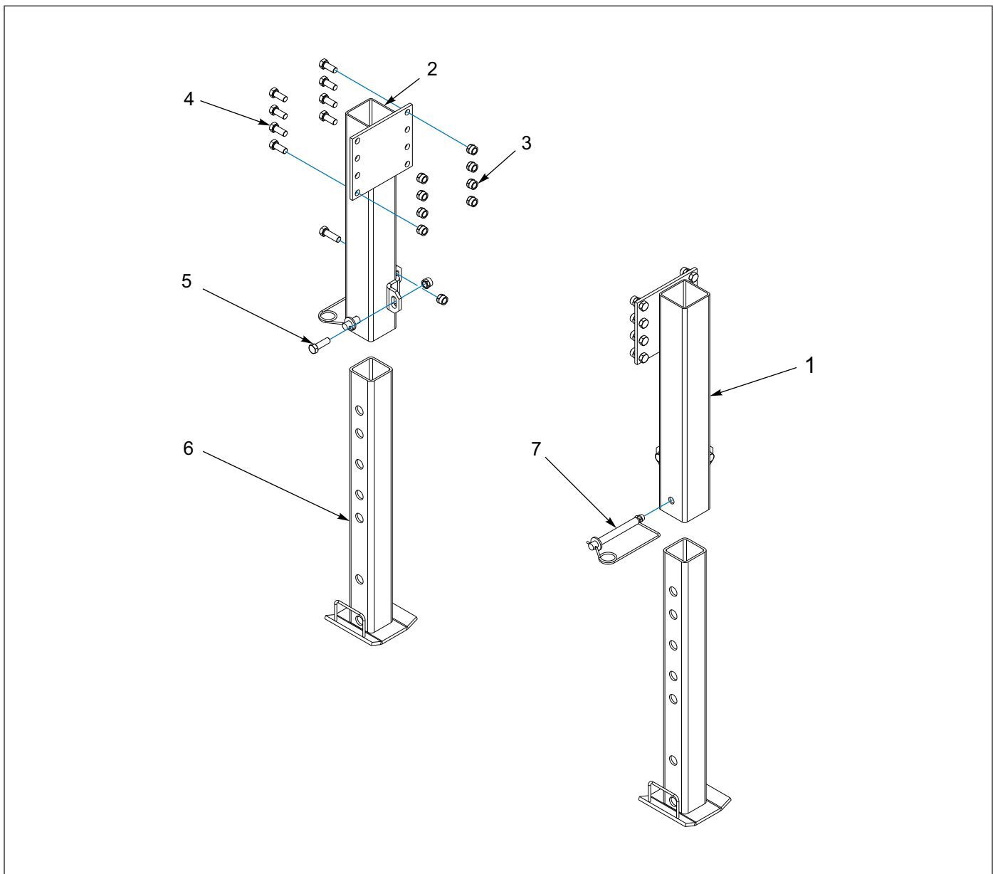
Figure 1-87: “Bolt On” Park Stand
