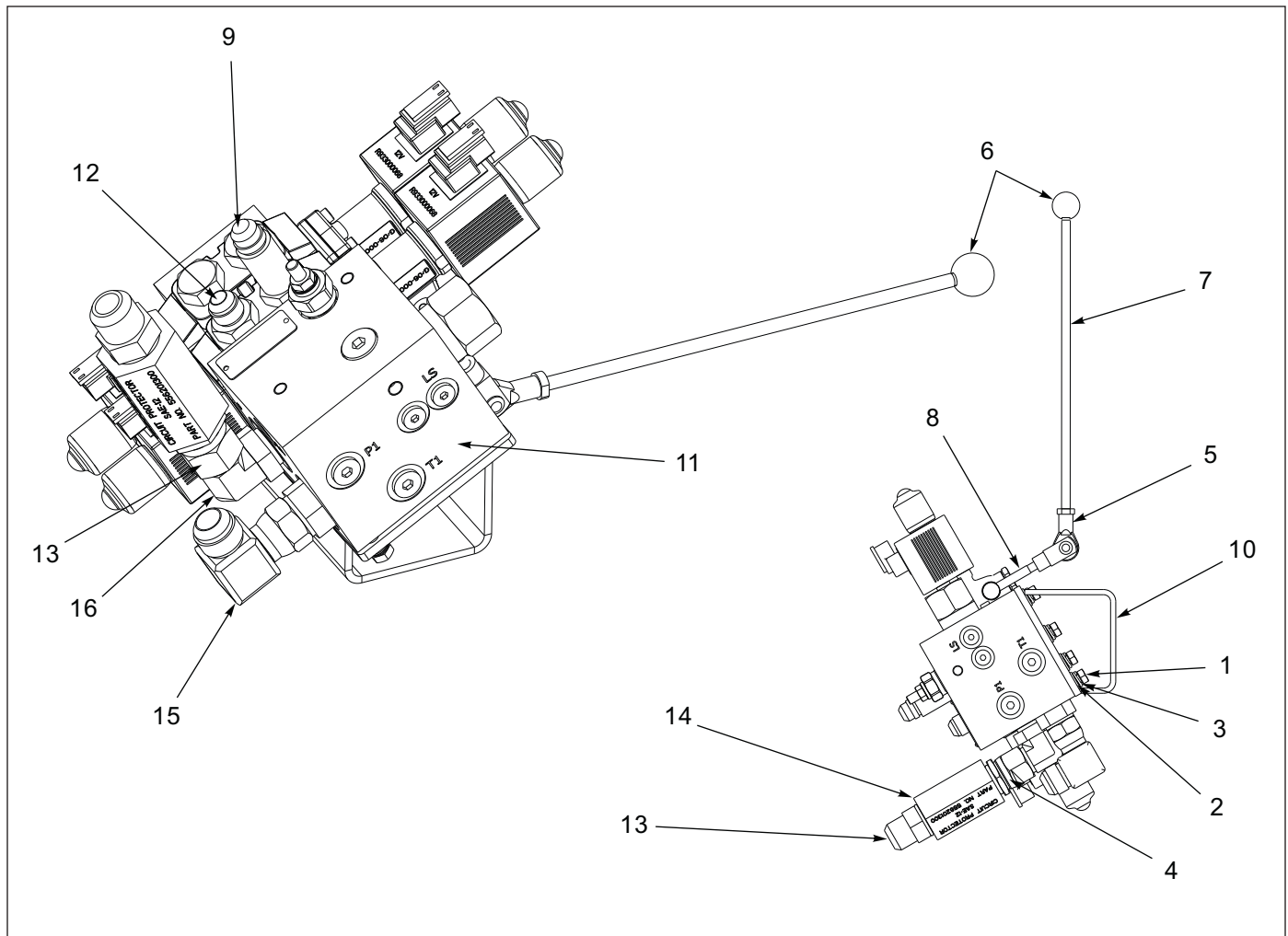
Figure 1-26: Valve Assembly - 2 Spool Control
