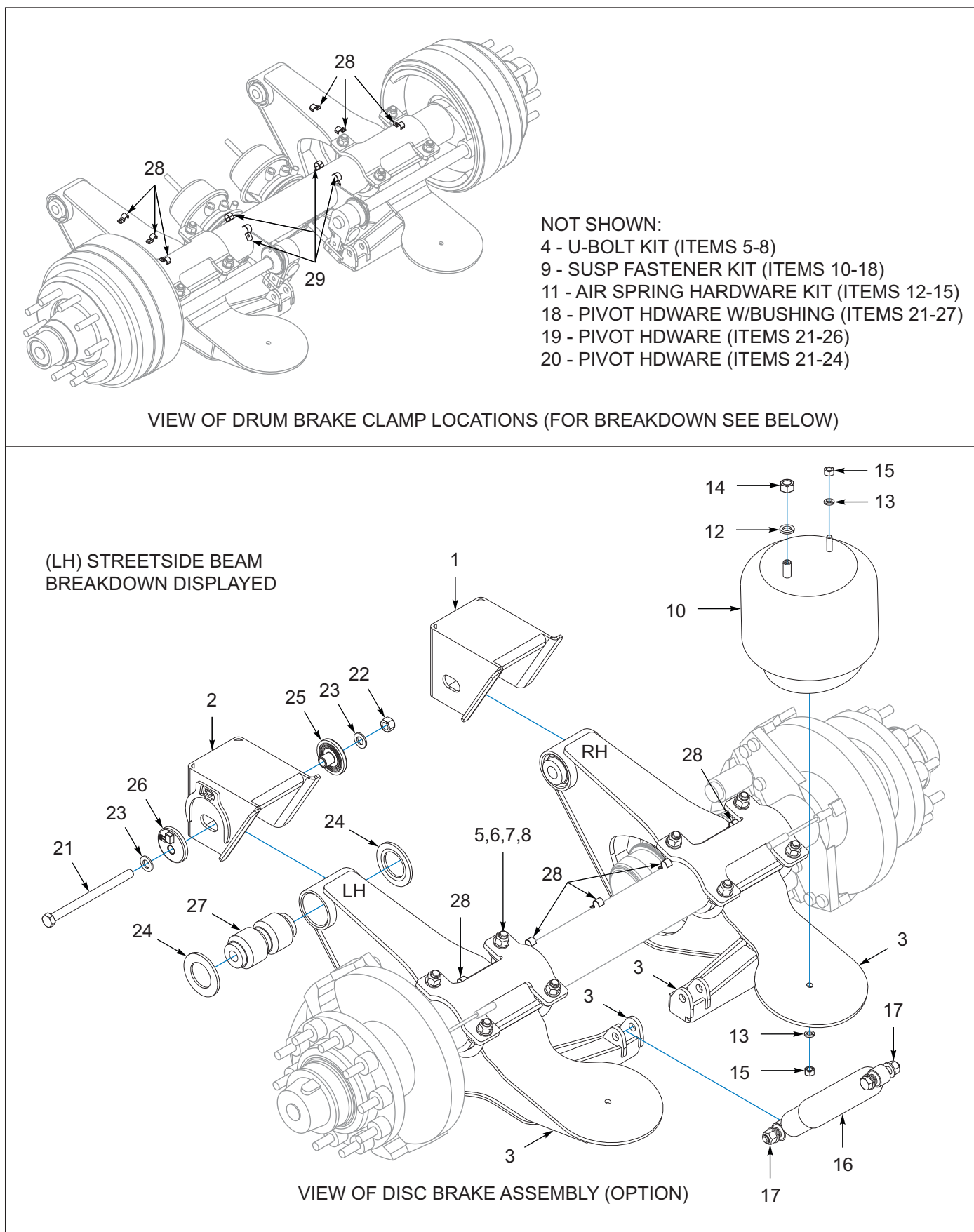
Figure 1-47: Suspension Hanger, 16.5, LSS- 25K-5.5 RLU
