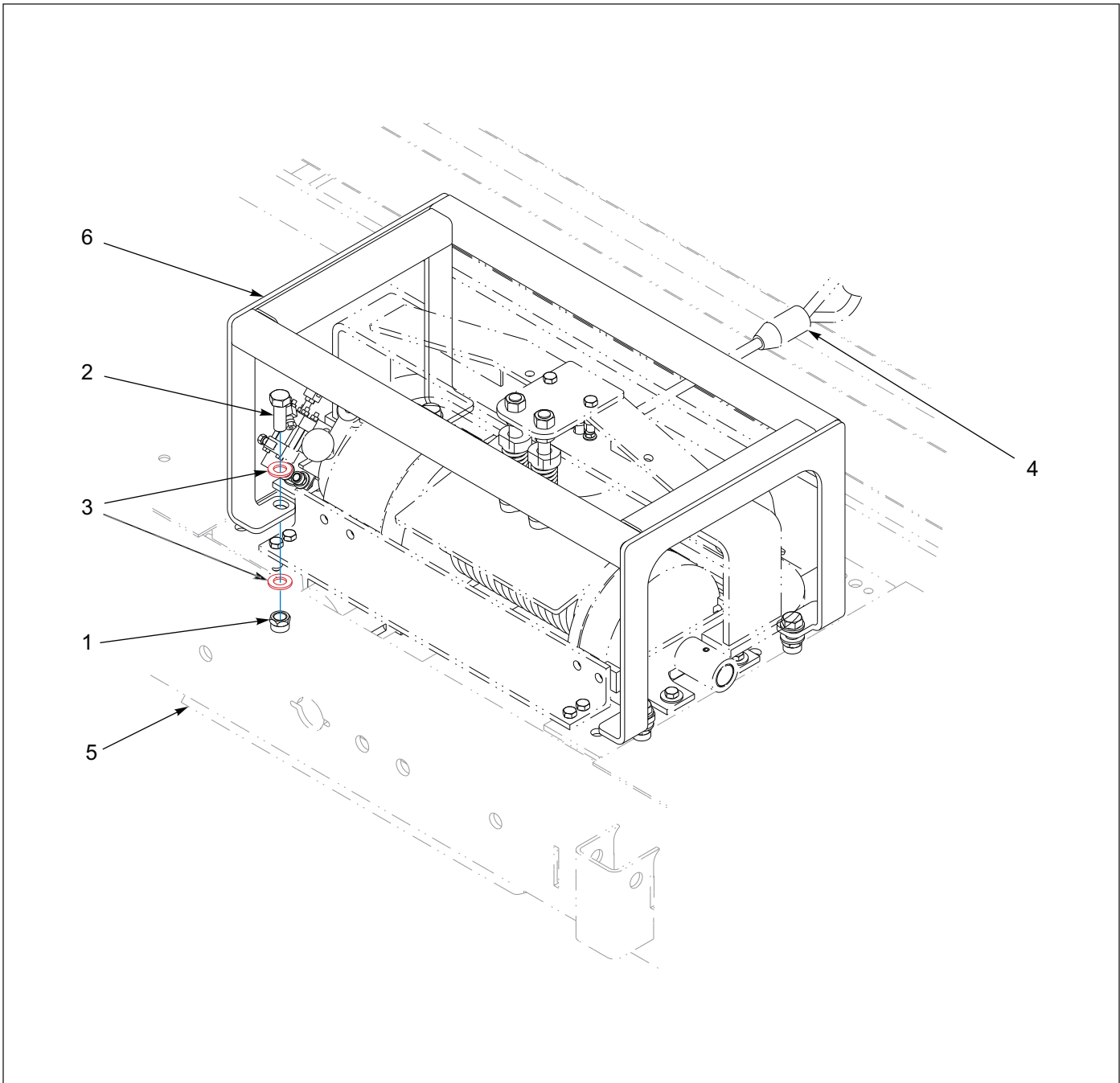
Figure 1-157: Guard Assembly, Pivot 20K
