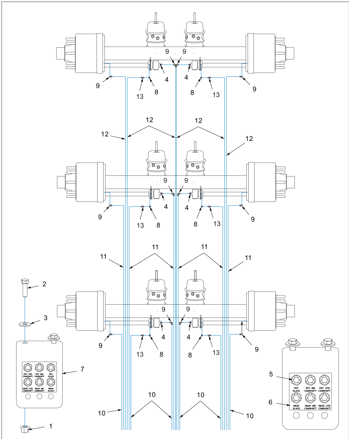
Figure 1-37: Grease System, 3 Axle (After 11/07/2018 - Before 08/31/2020)
