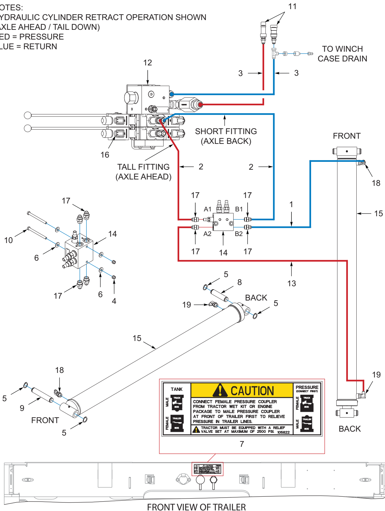
Figure 1-14: Hydraulic System - Axle / Tail Travel
