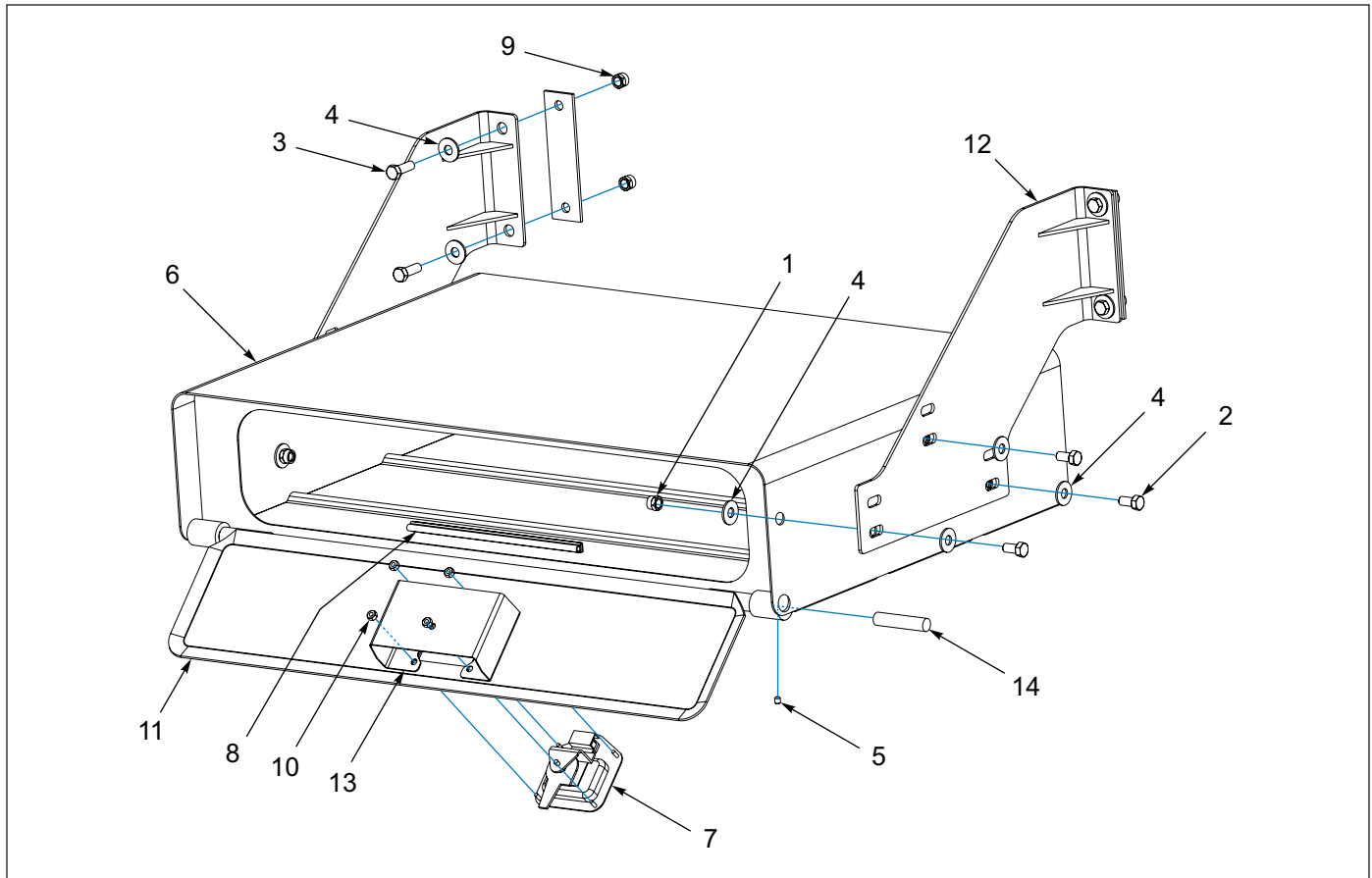
Figure 1-149: Toolbox Assembly-Steel/Aluminum Door
