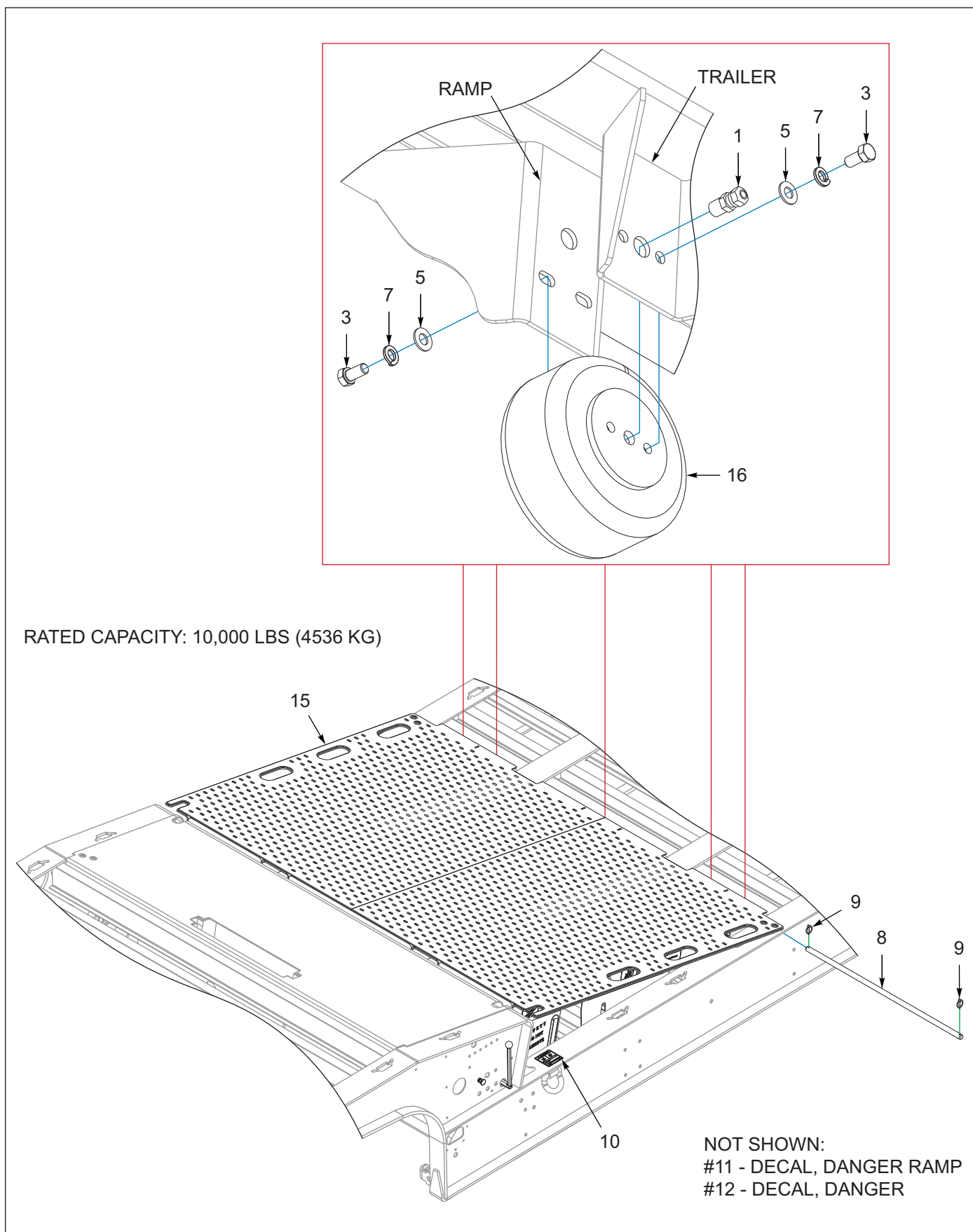
Figure 1-129: Front Slope, 6FT Air (1 of 2) (AFTER 03/11/2021)
