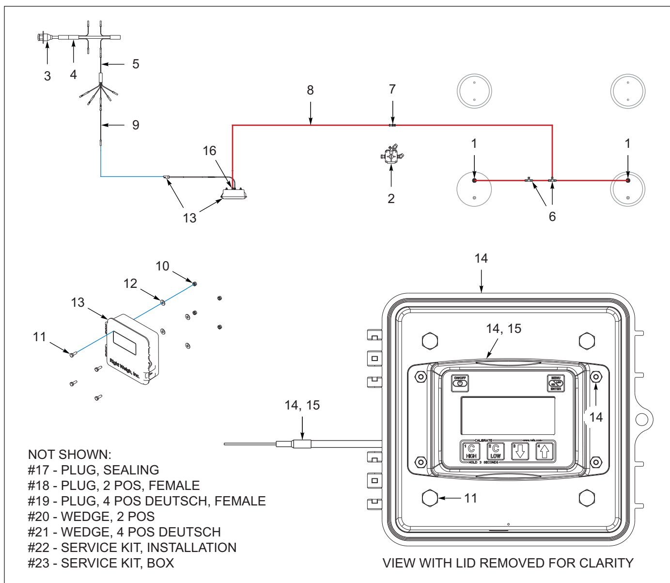
Figure 1-139: Right Weigh
