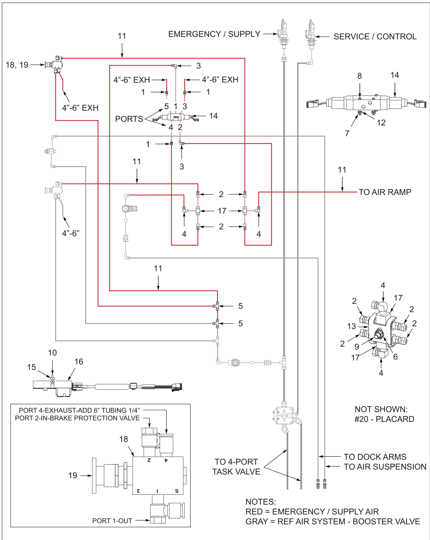
Figure 1-16: Air System - Remote, Dock Levelers & Ramp
