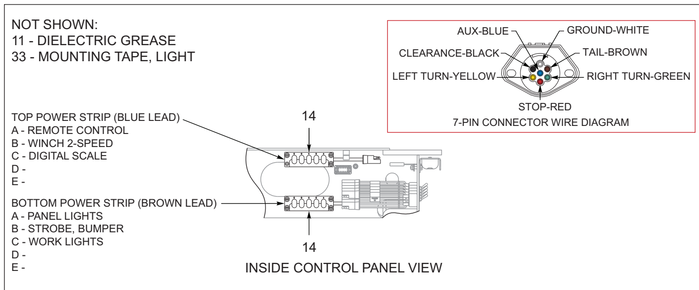
Figure 1-20: Electrical System - Trailer (After 02/15/2022) (2 of 2)
