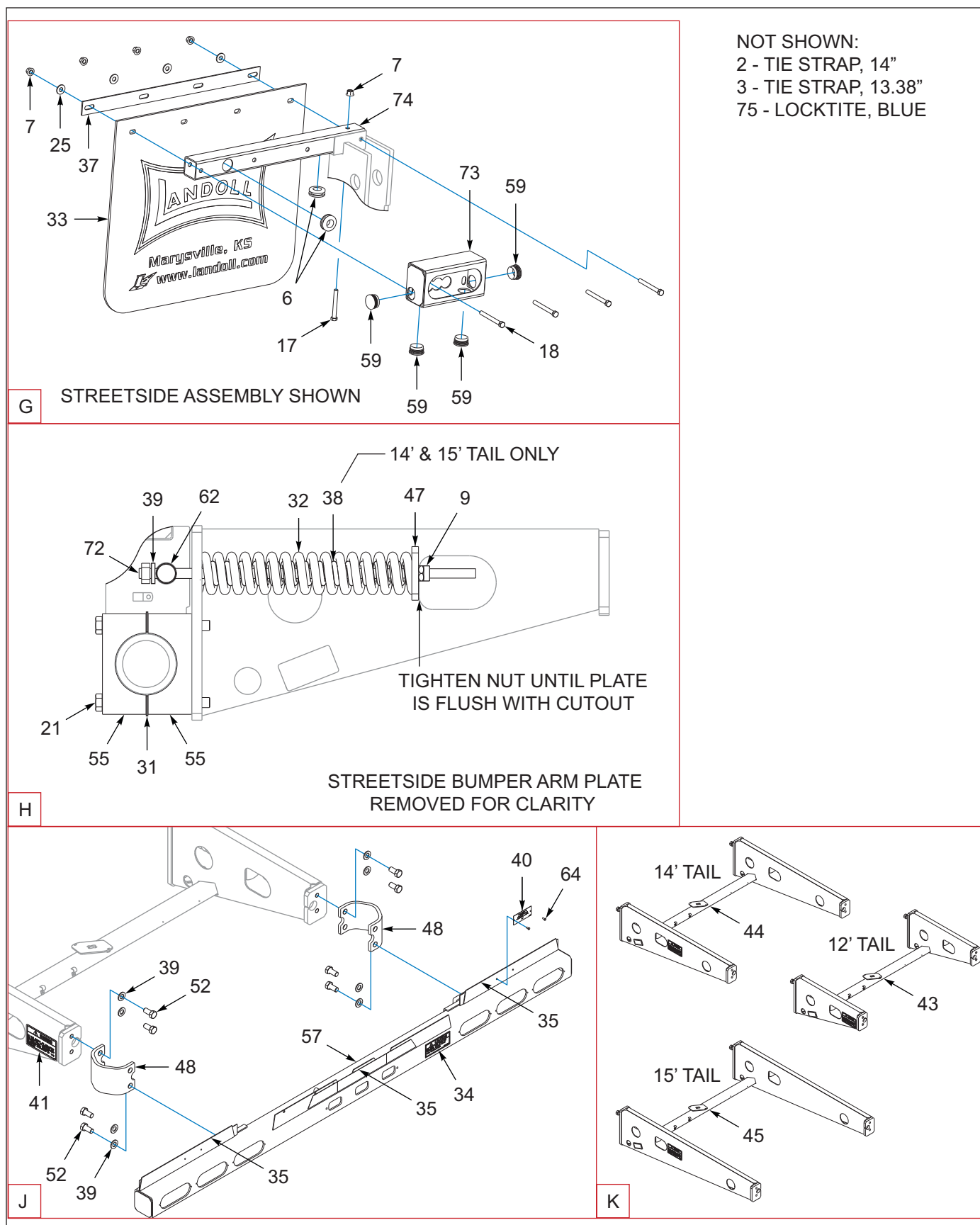
Figure 1-30: Undercarriage Components (3 of 3)
