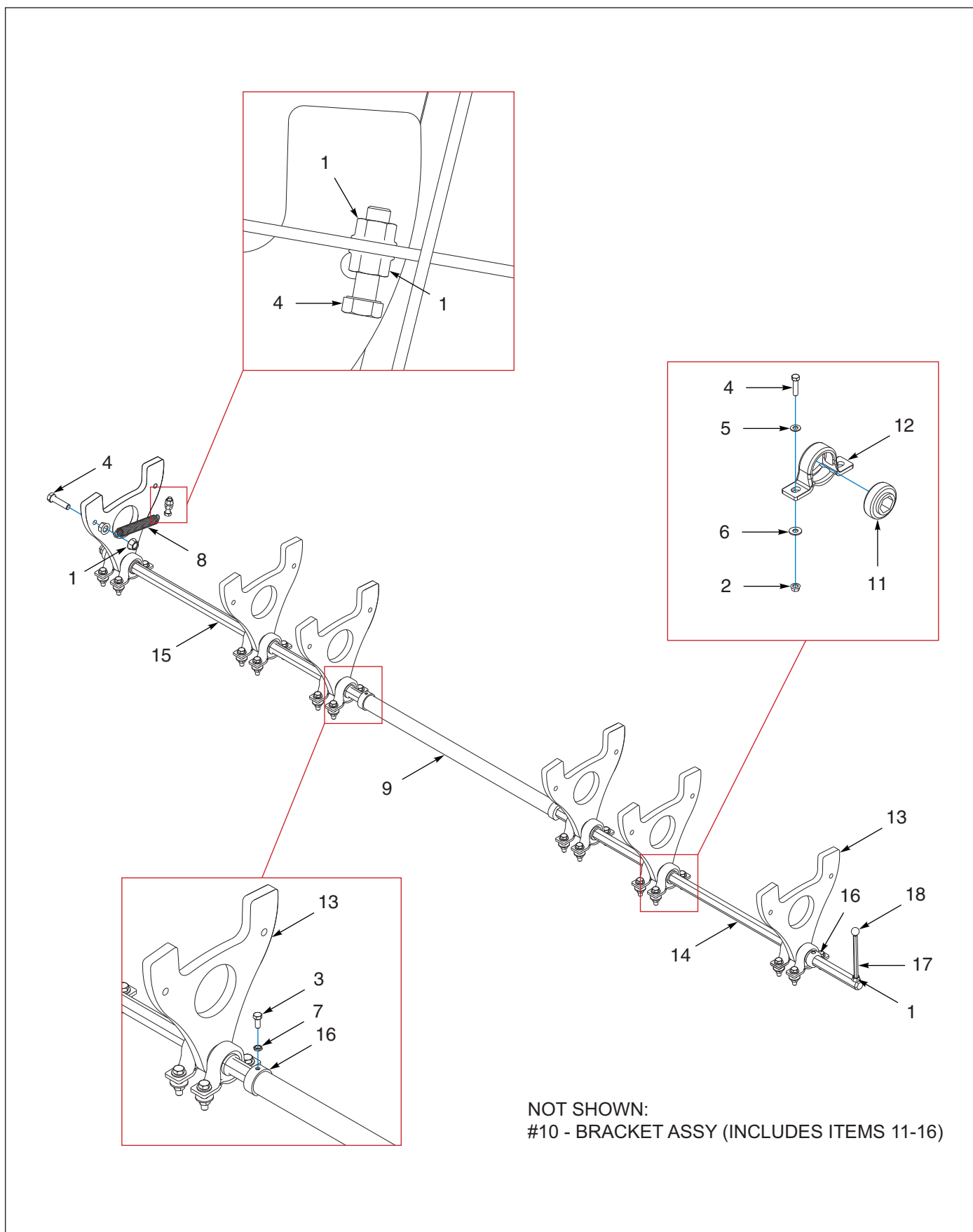
Figure 1-131: Front Slope, 6FT Air, Support (BEFORE 03/11/2021)
