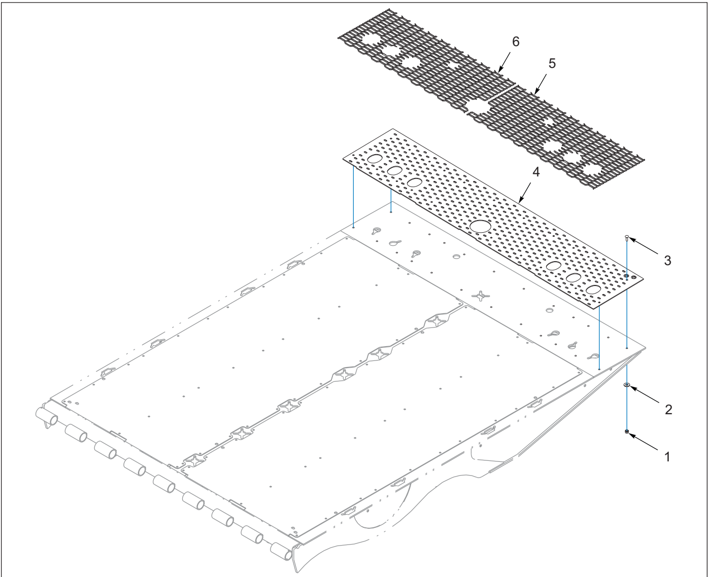
Figure 1-100: Tail Tread Grip, Approach Plate
