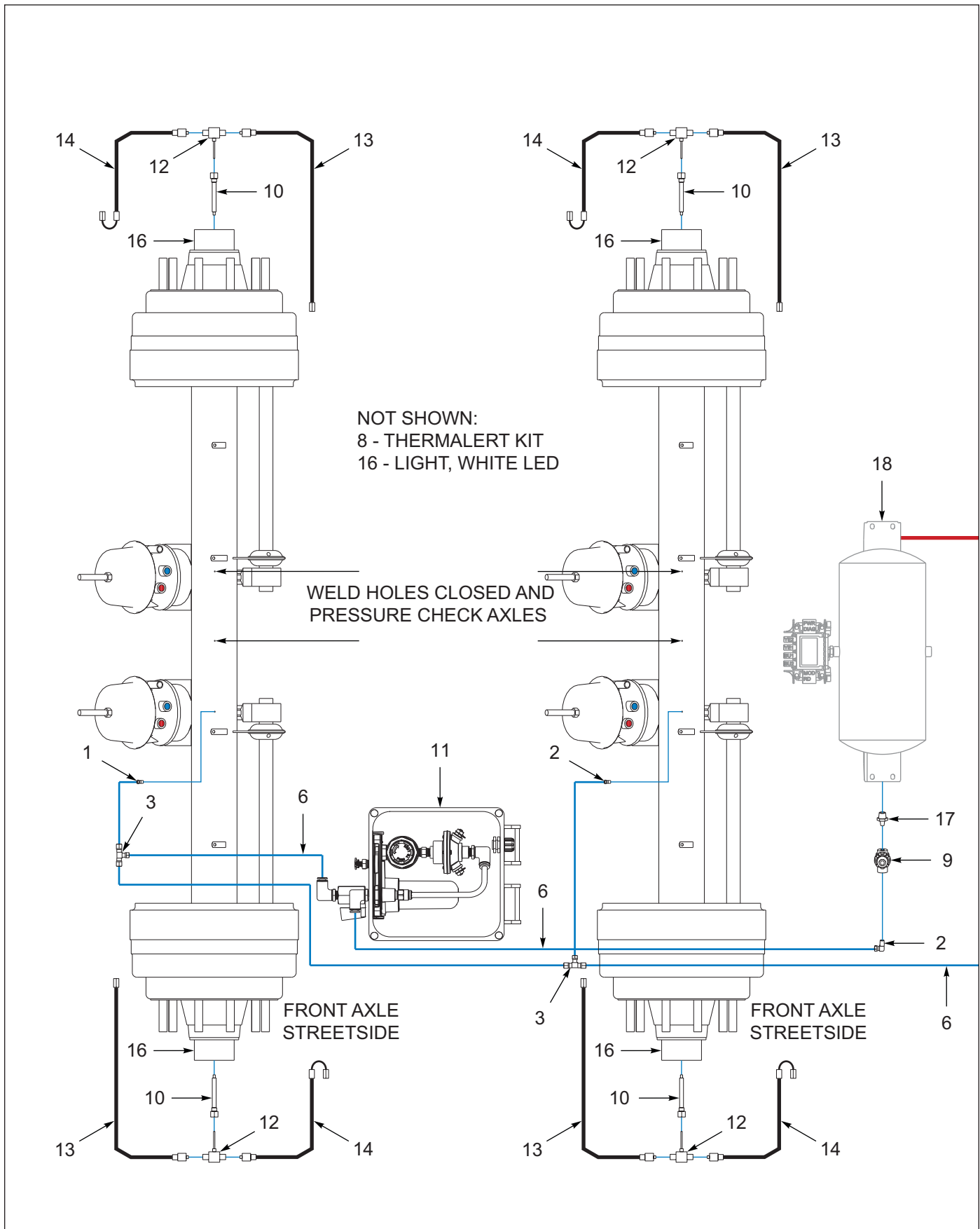
Figure 1-66: Thermalert, 3 Axle Air System (OPTION) (1 of 2)
