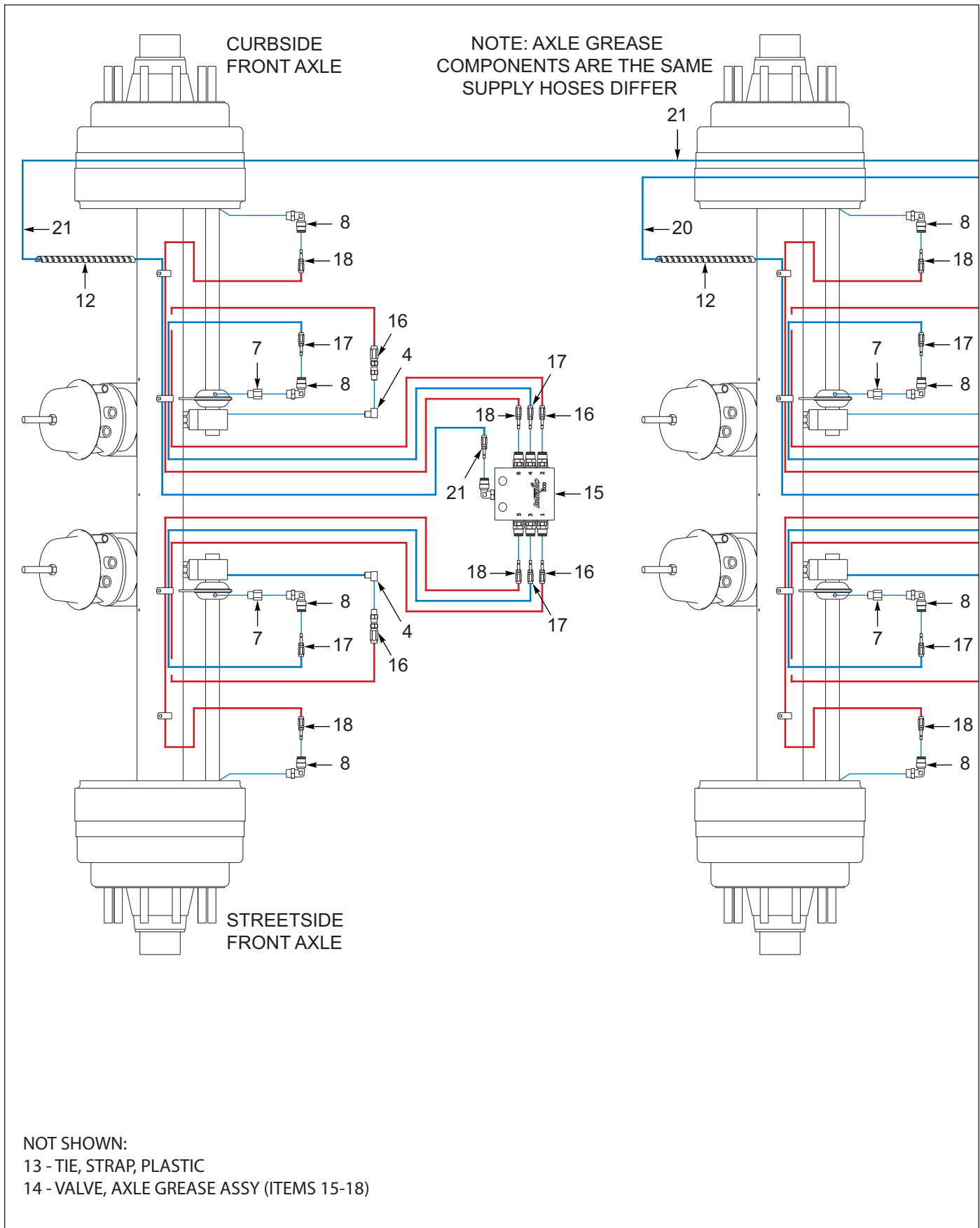
Figure 1-38: Grease System, 3 Axle (After 08/31/2020) (1 of 3)
