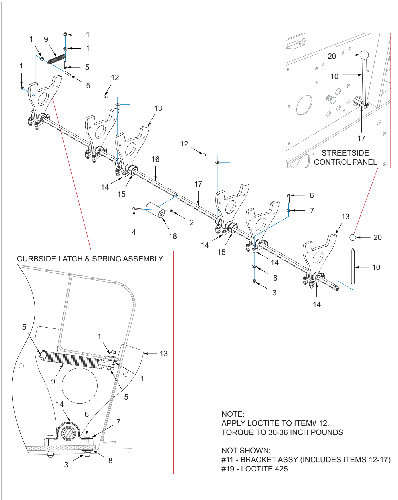
Figure 1-132: Front Slope, 6FT Air, Support (AFTER 03/11/2021)
