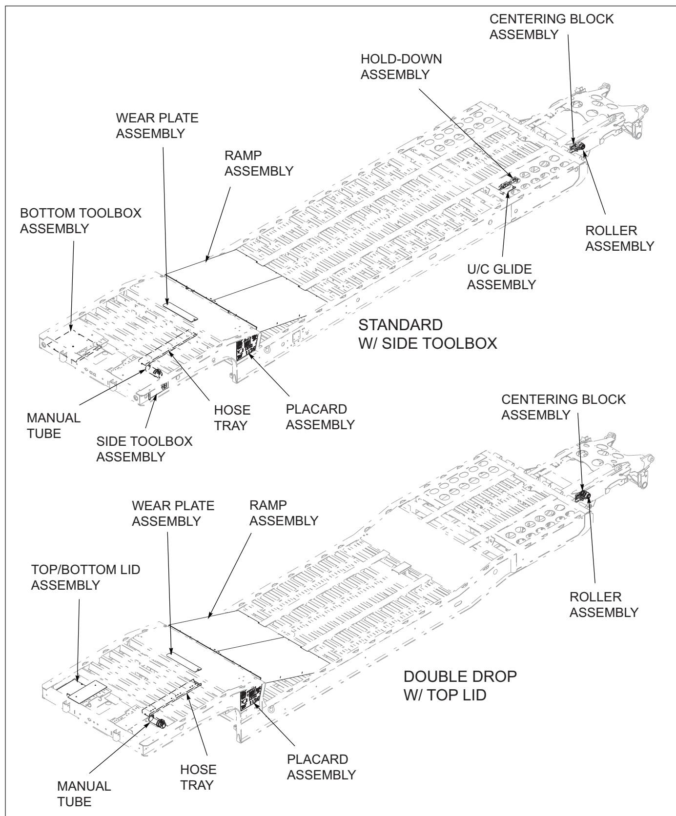
Figure 1-7: Frame Assembly (1 of 3)
