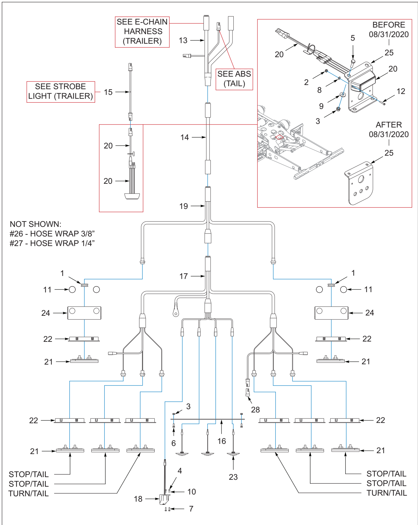
Figure 1-22: Electrical System - Bumper
