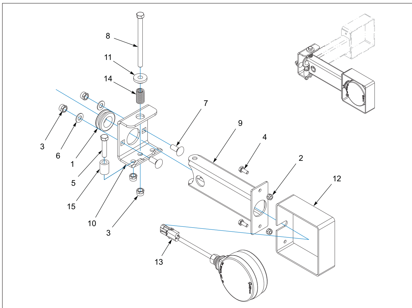
Figure 1-123: Swing-Arm Light Assembly - Turn Signal/Emergency Flasher
