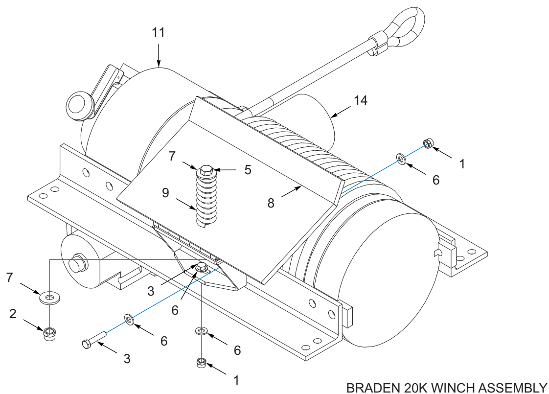
Figure 1-70: Winch Assembly, Braden 12K / 20K (OPTION)
