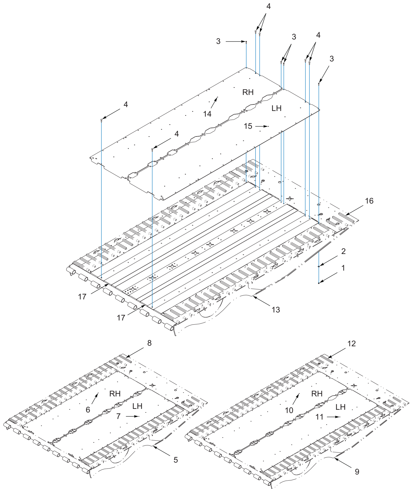
Figure 1-99: Tail Tread Grip-223036
