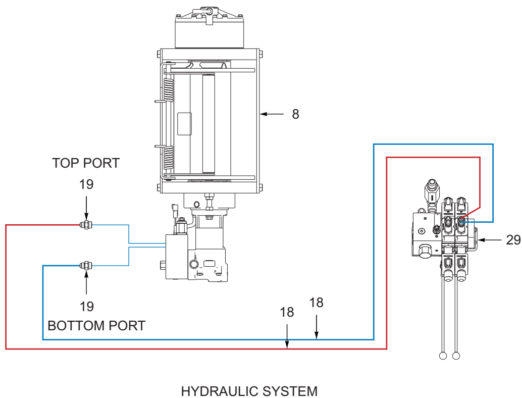
Figure 1-82: Winch Installation, Warn 20K, Speed (OPTION) (1 of 2)
