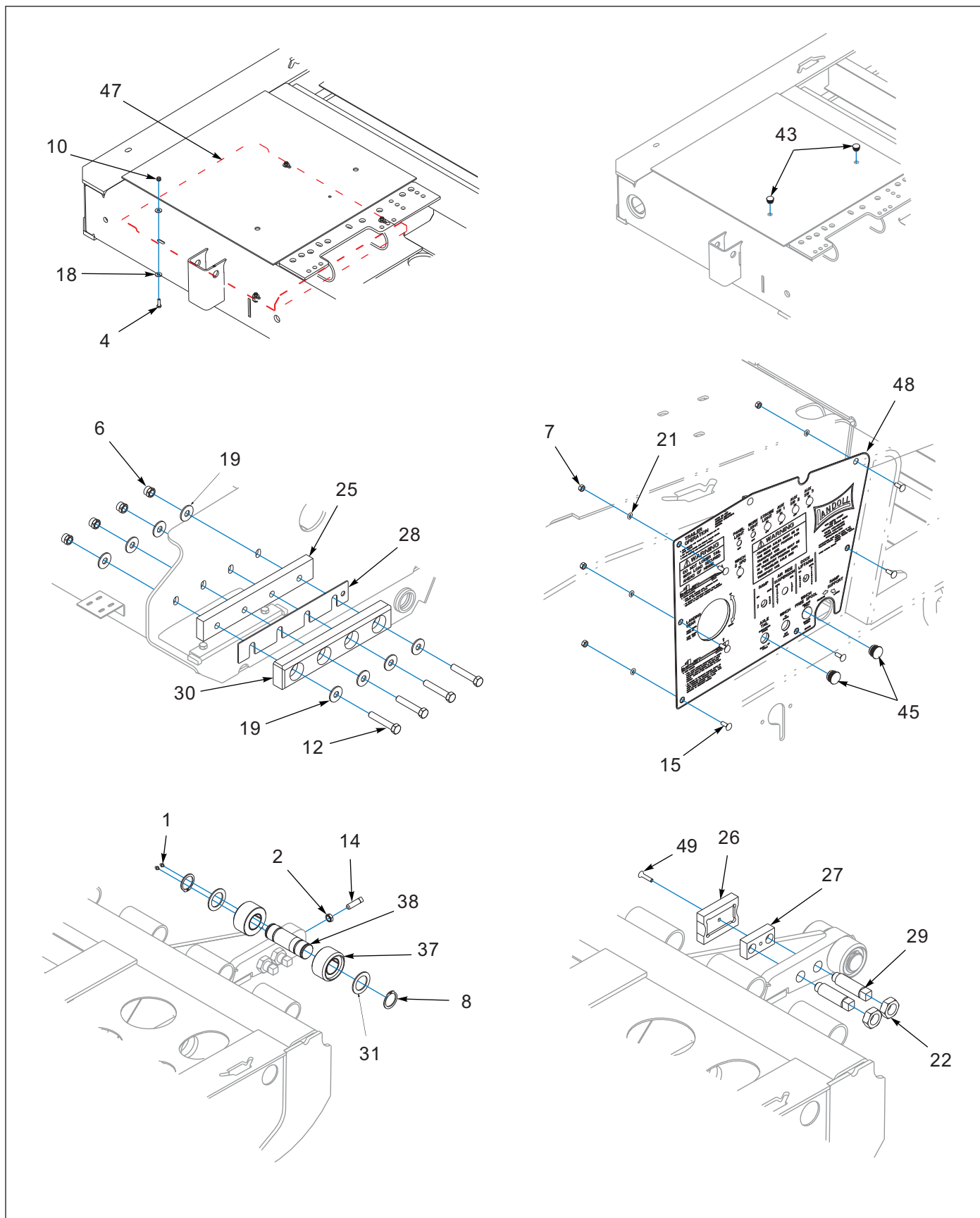
Figure 1-8: Frame Assembly (2 of 3)
