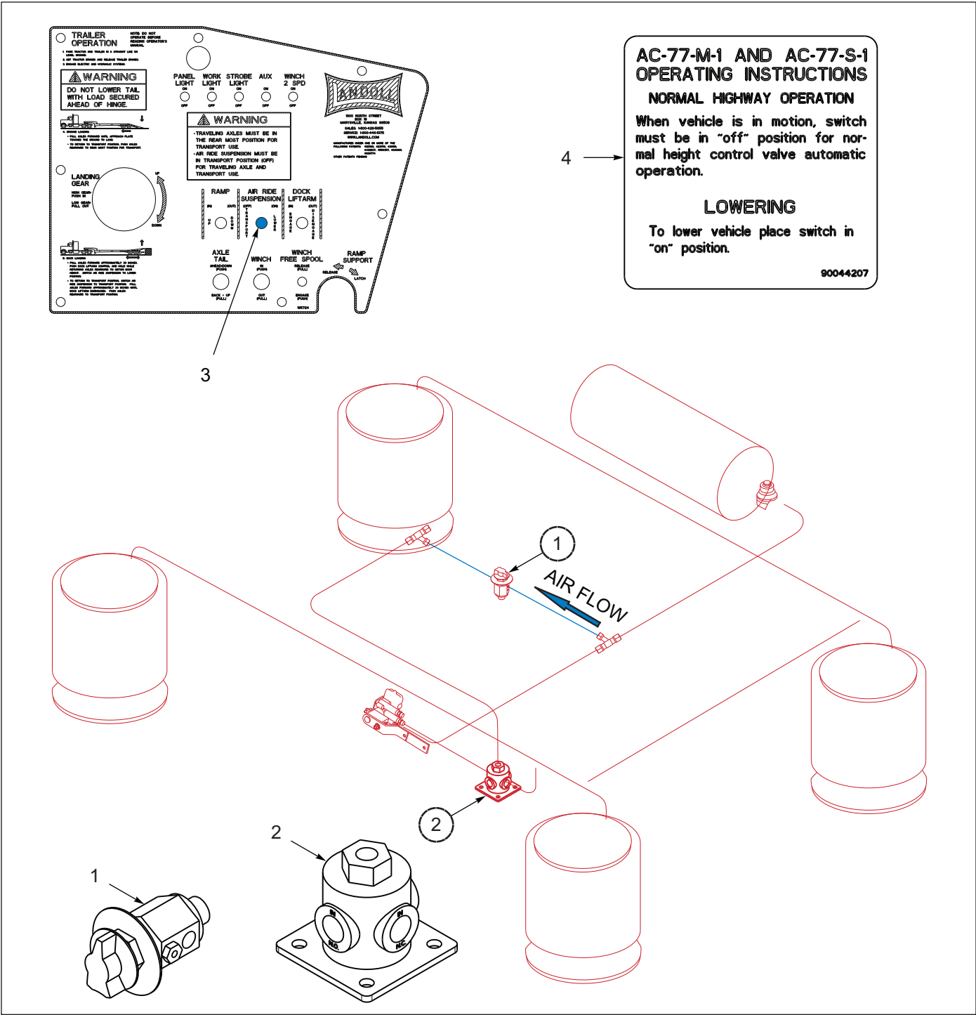
Figure 1-44: Air Control Kit - Lower Suspension
