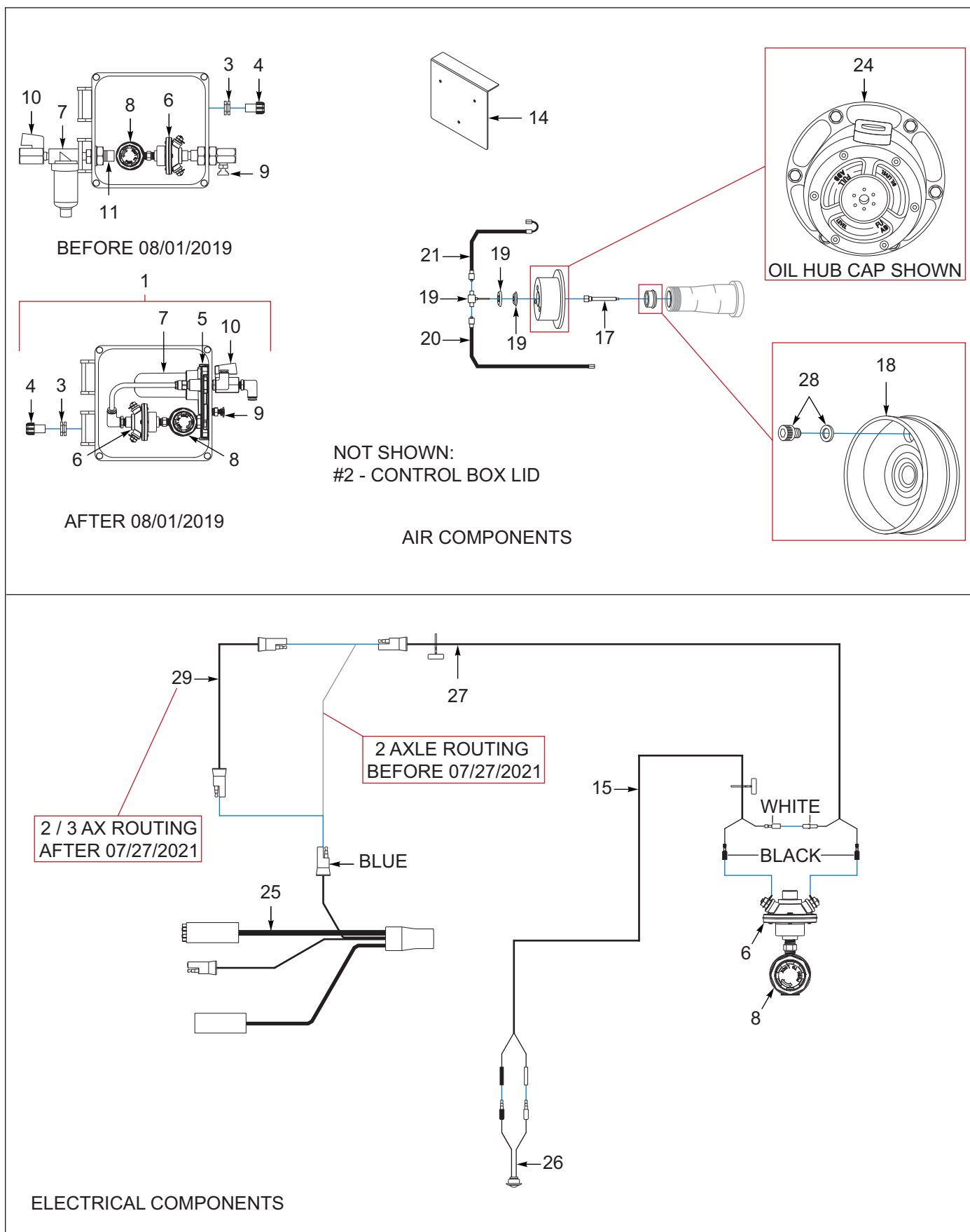
Figure 1-68: Thermalert Electrical System &amp; Components (OPTION)
