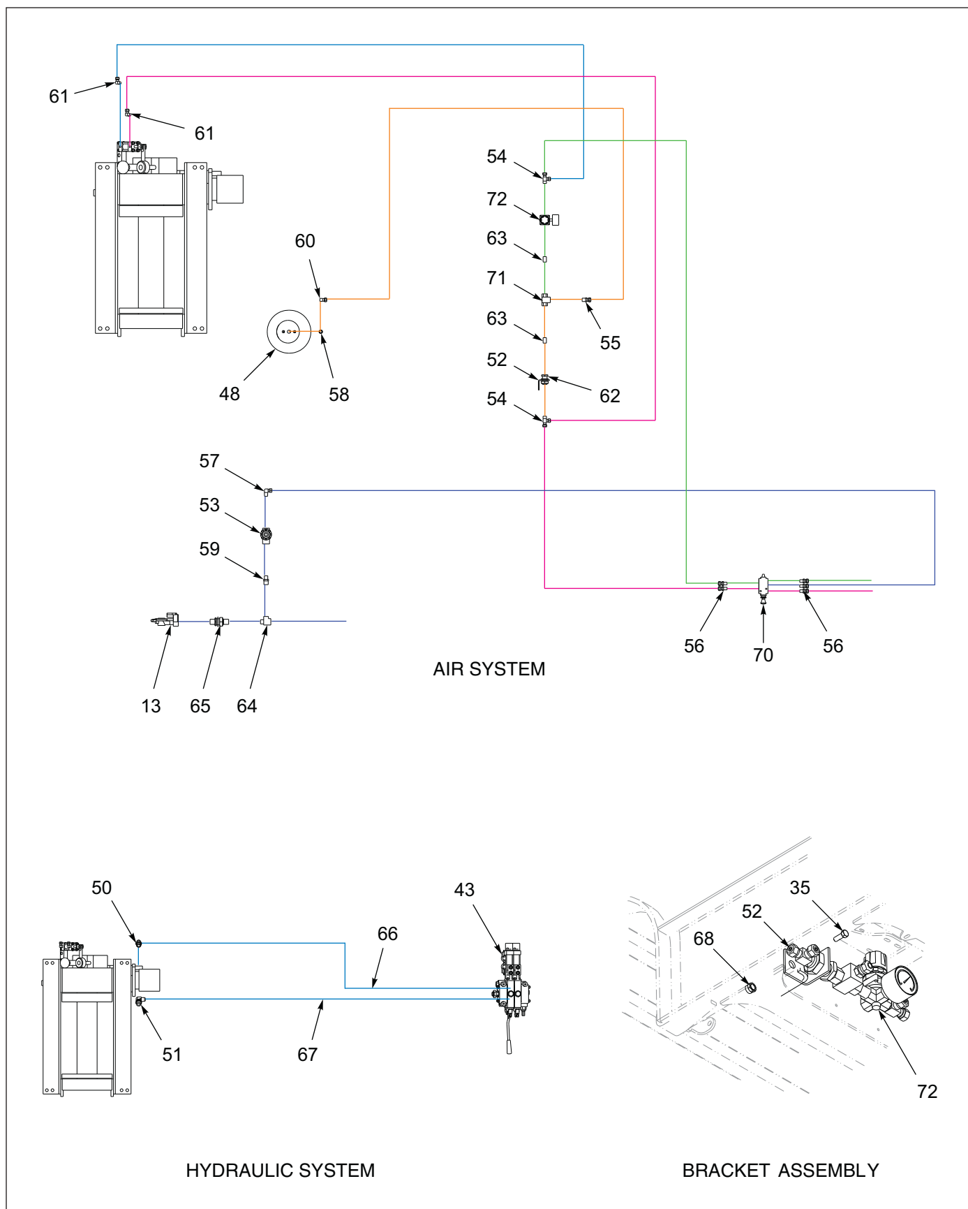
Figure 1-76: Winch Installation, Braden 20K Air Tension/Release (3 of 3)
