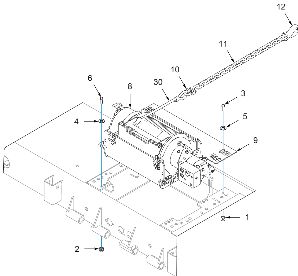
GENERAL ASSEMBLY VIEW OF TRAILER FRONT
