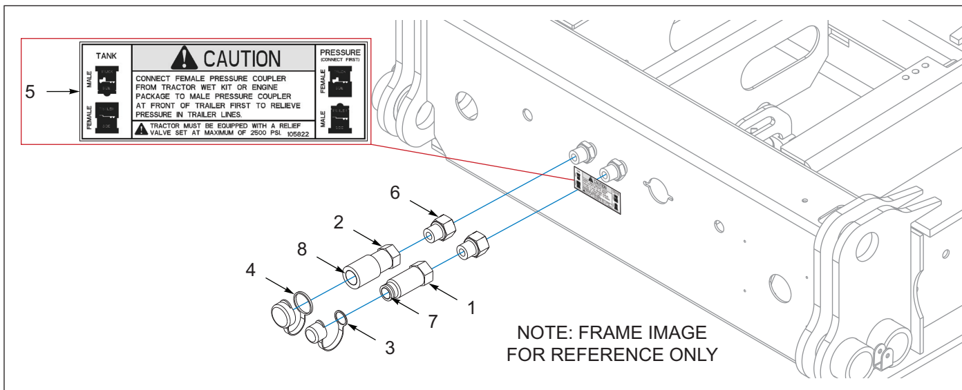
Figure 1-120: Hydraulic Conversion Kit - Ball to Flat
