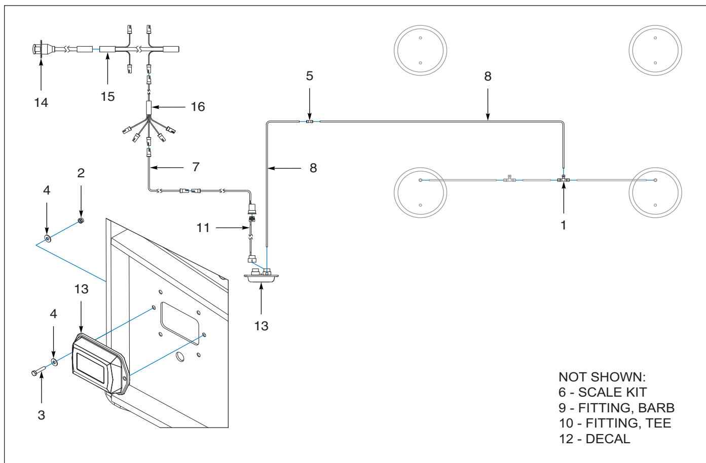
Figure 1-138: Quickload Plus & Loadmaxx Plus (AFTER 3/31/2020)
