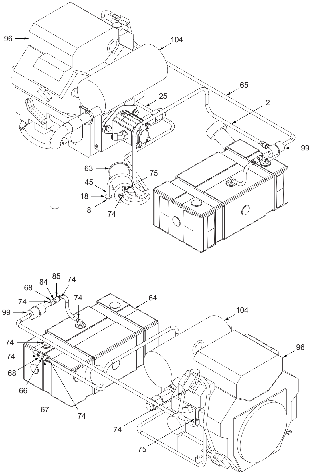
Figure 1-109: 25 HP Upper Deck Package (4 of 5)
