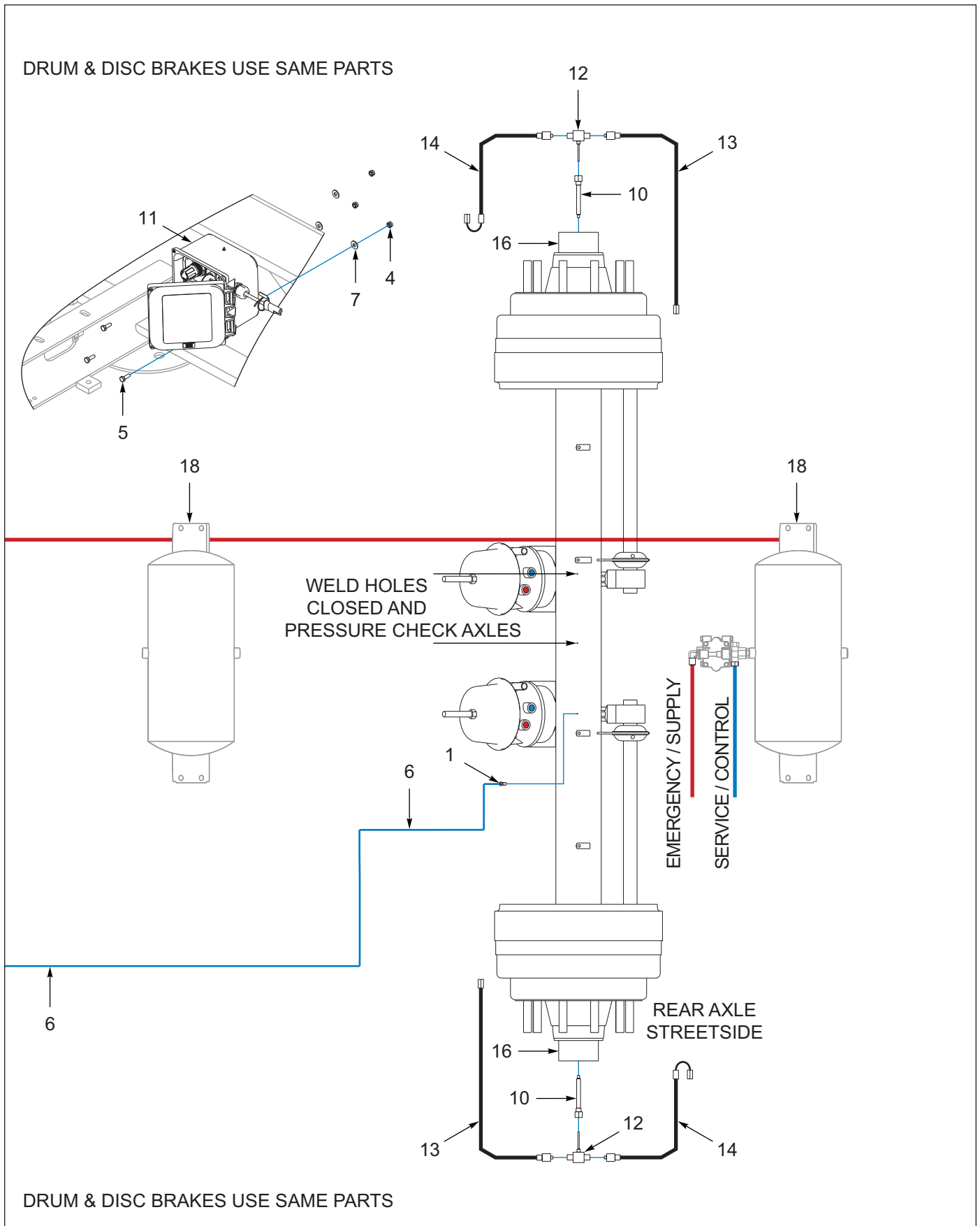
Figure 1-67: Thermalert, 3 Axle Air System (OPTION) (2 of 2)
