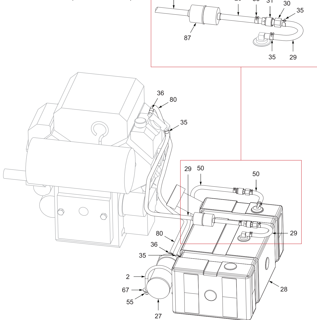
Figure 1-113: 25 HP Slope Package (3 of 4)
