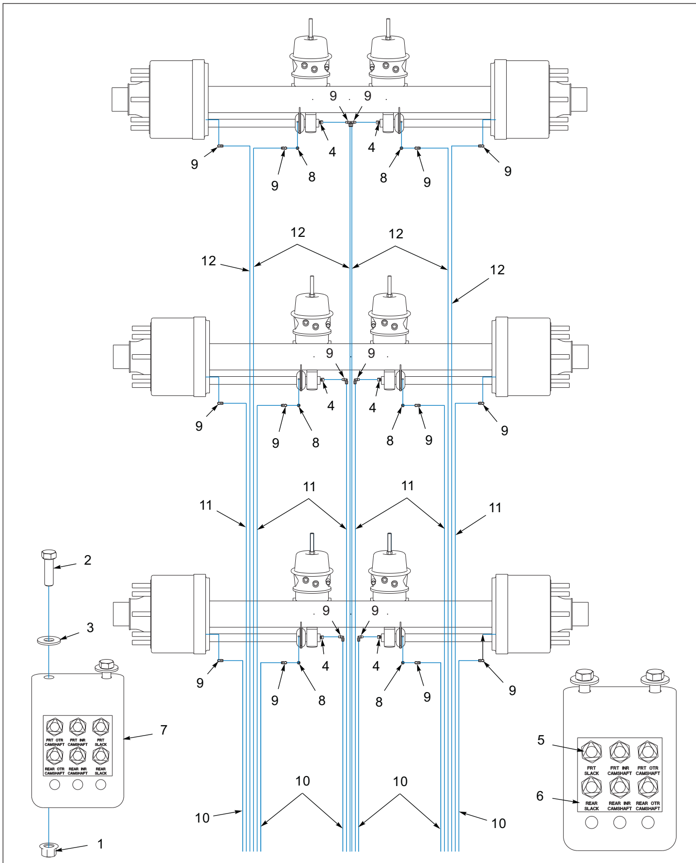
Figure 1-36: Grease System, 3 Axle (Before 11/07/2018)
