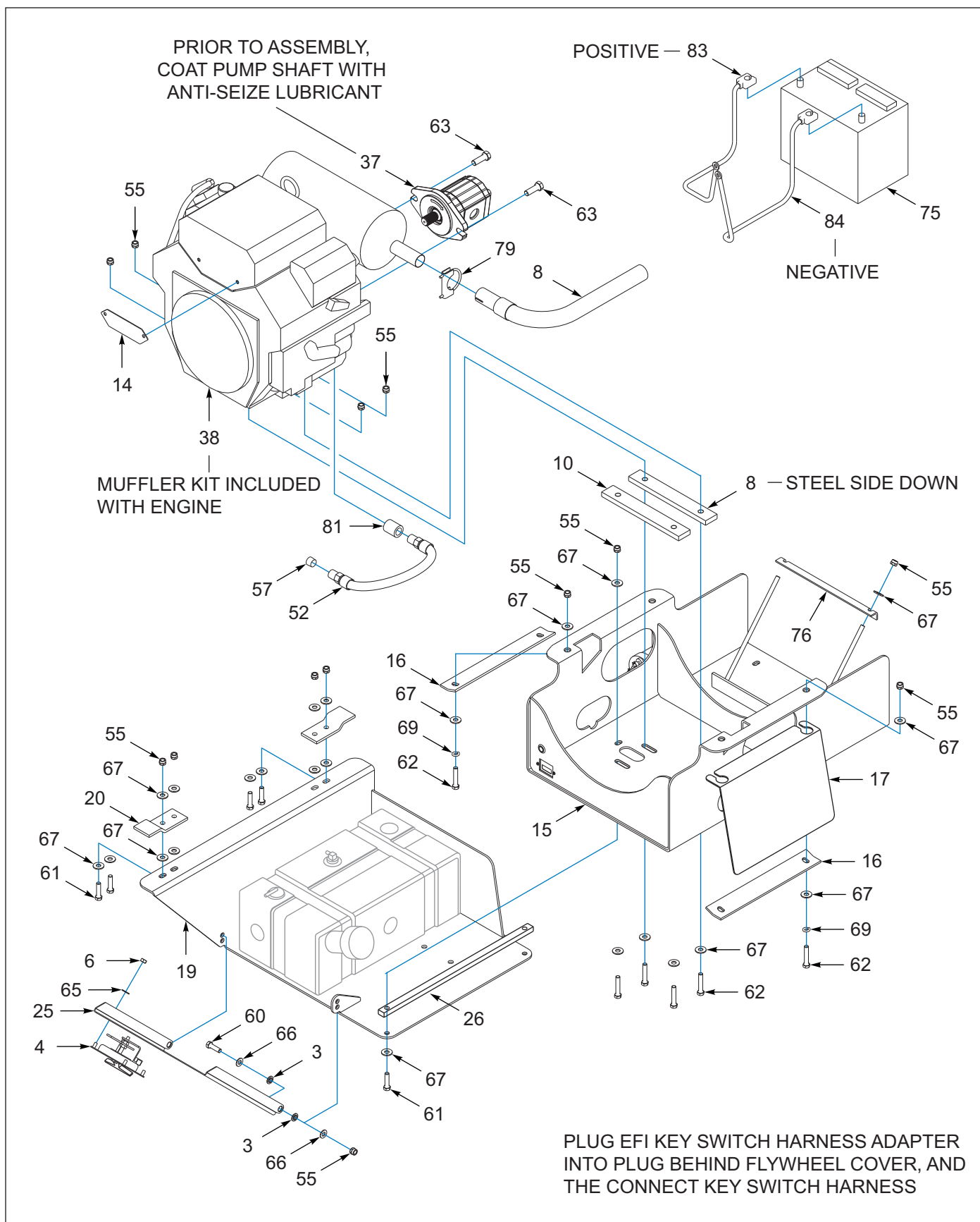
Figure 1-112: 25 HP Slope Package (2 of 4)
