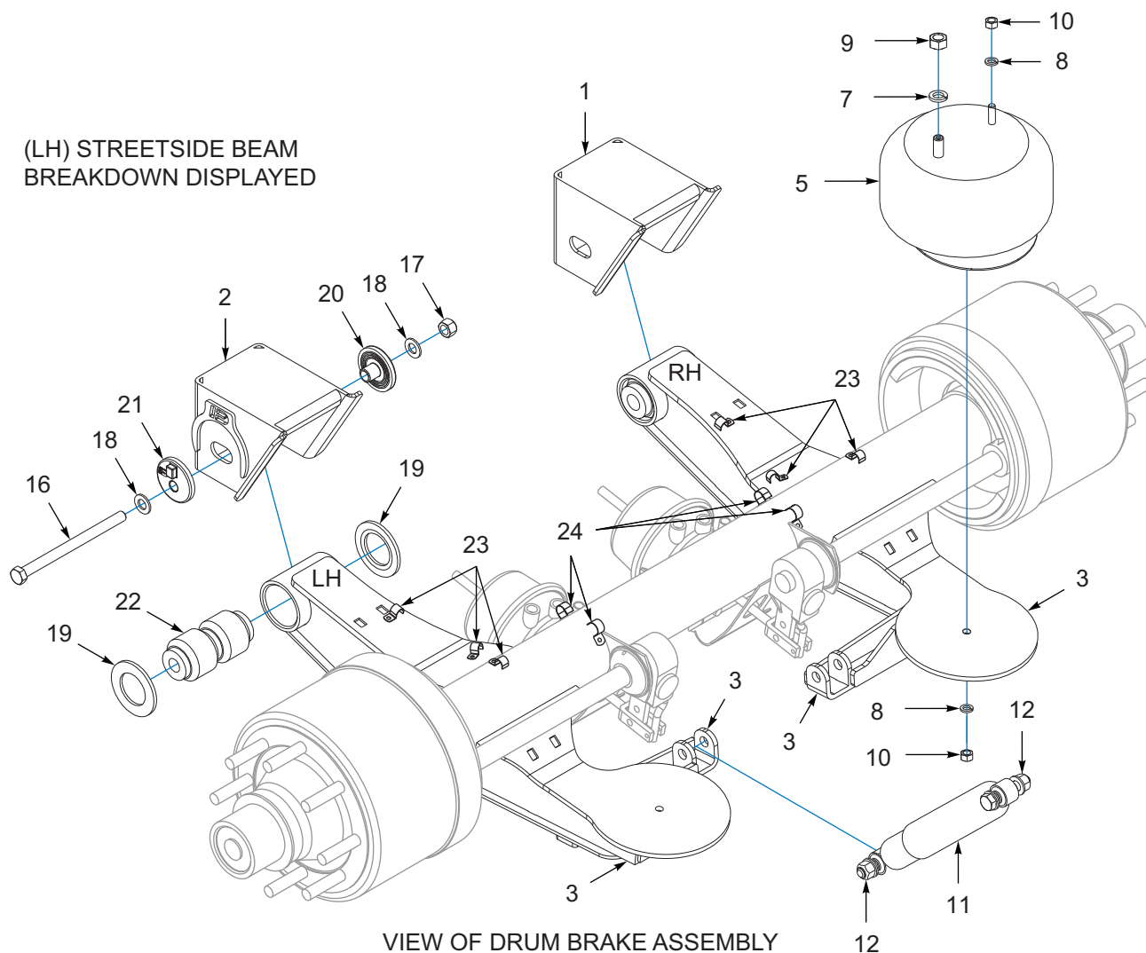
Figure 1-46: Suspension Hanger, 12.25, LSS- 25K-3.5 RLU
