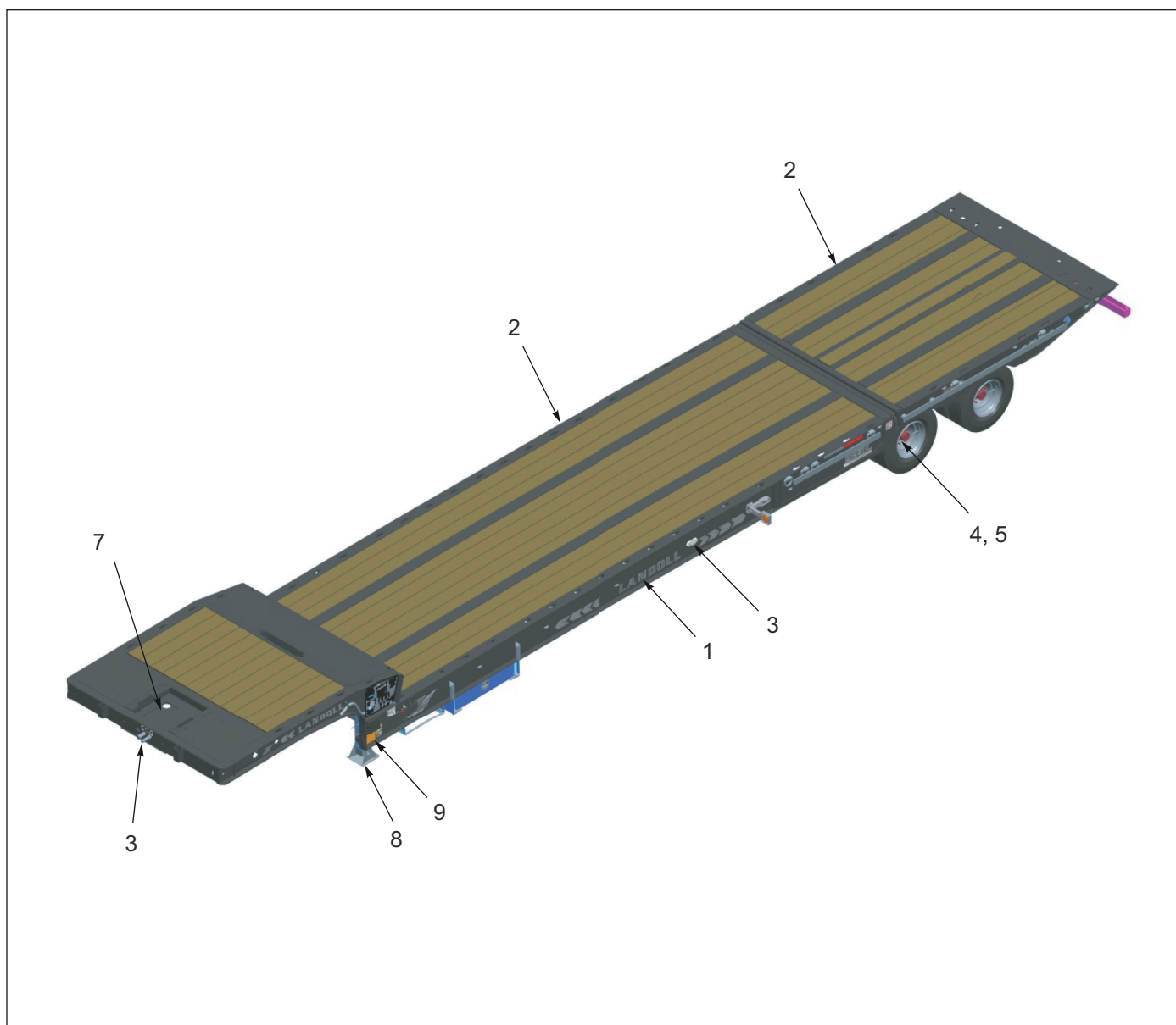
Figure 1-2: General Assembly
