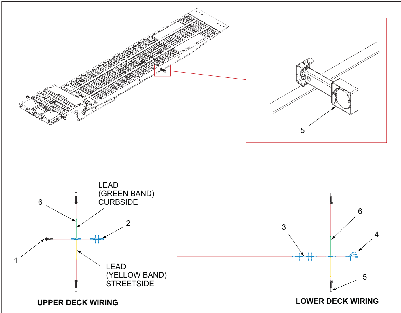
Figure 1-122: Swingout Light Installation
