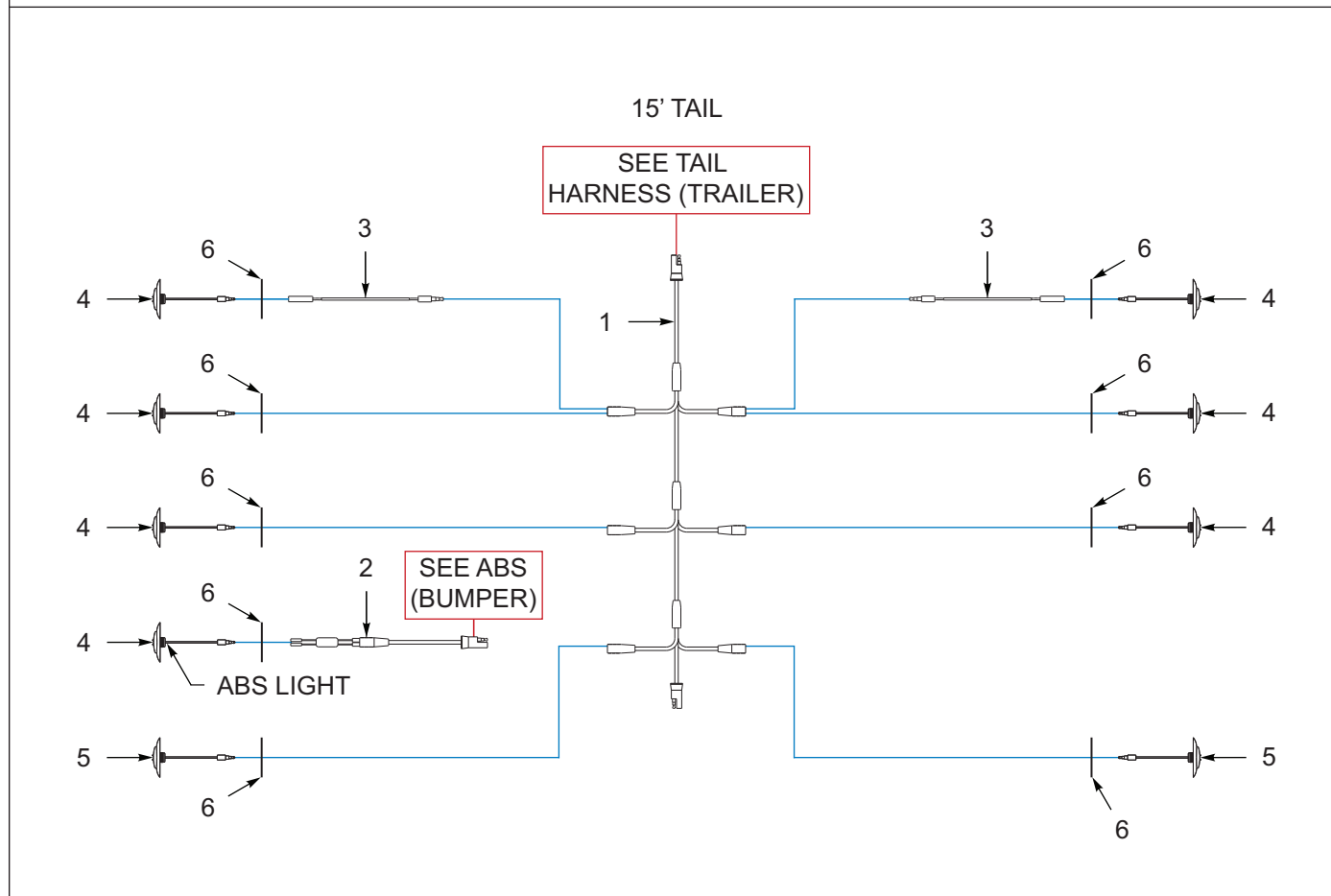
Figure 1-21: Electrical System - Tail
