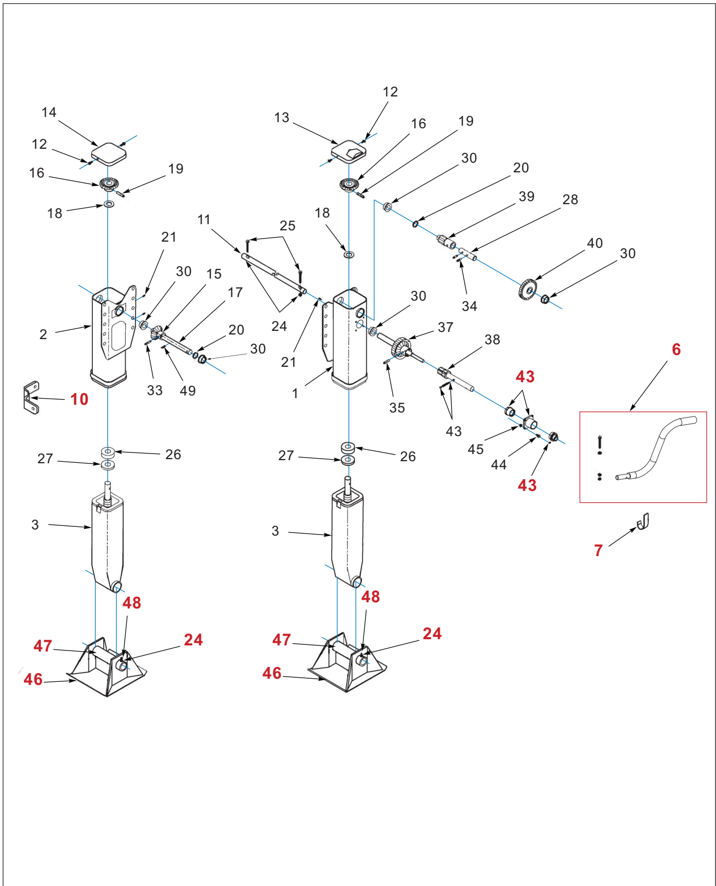
Figure 1-89: Jost #A401T19
