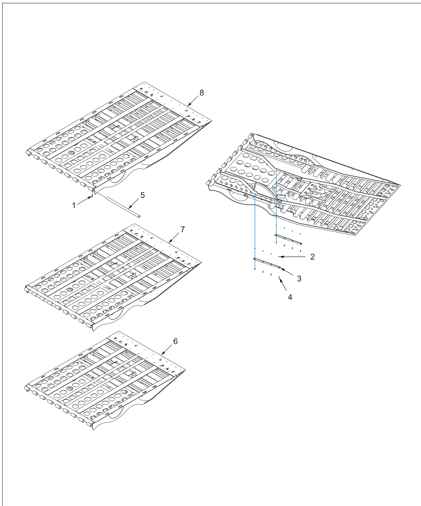
Figure 1-11: Tail Assembly, WO/Center Gotcha Plate
