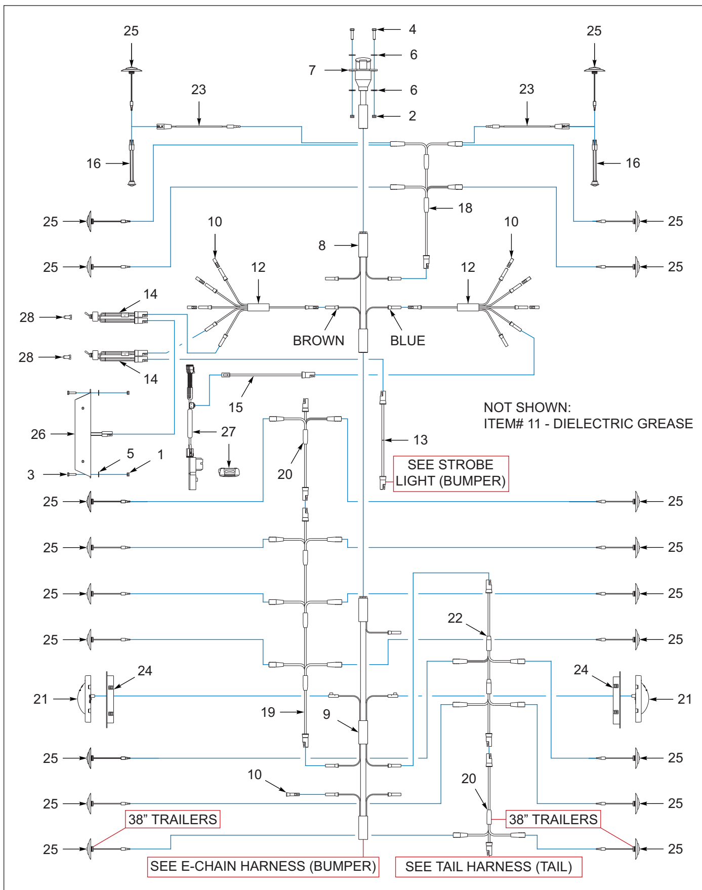
Figure 1-17: Electrical System - Trailer (Before 02/15/2022) (1 of 2)
