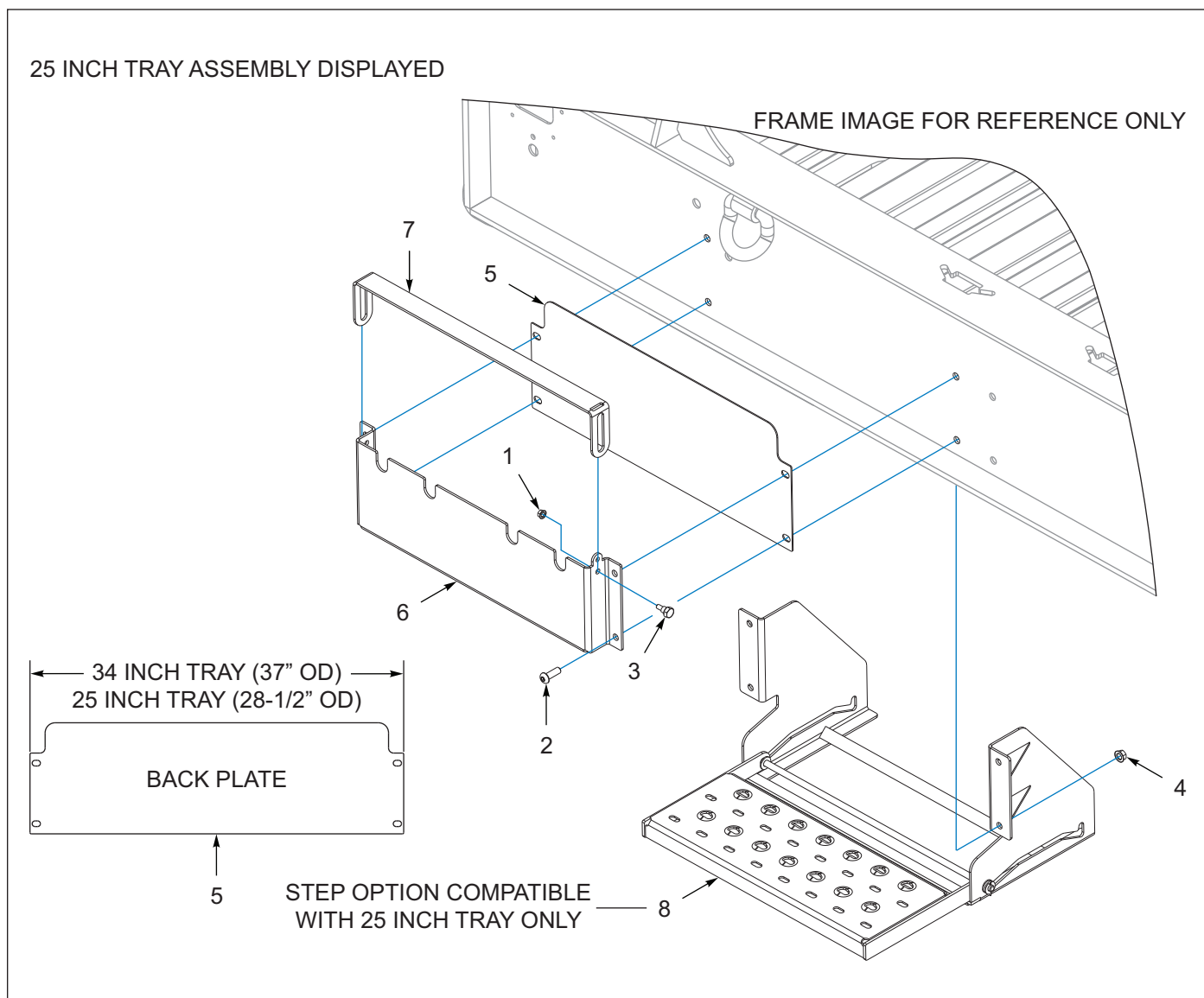
Figure 1-147: Chain Tray Assemblies (AFTER 01/17/2022)
