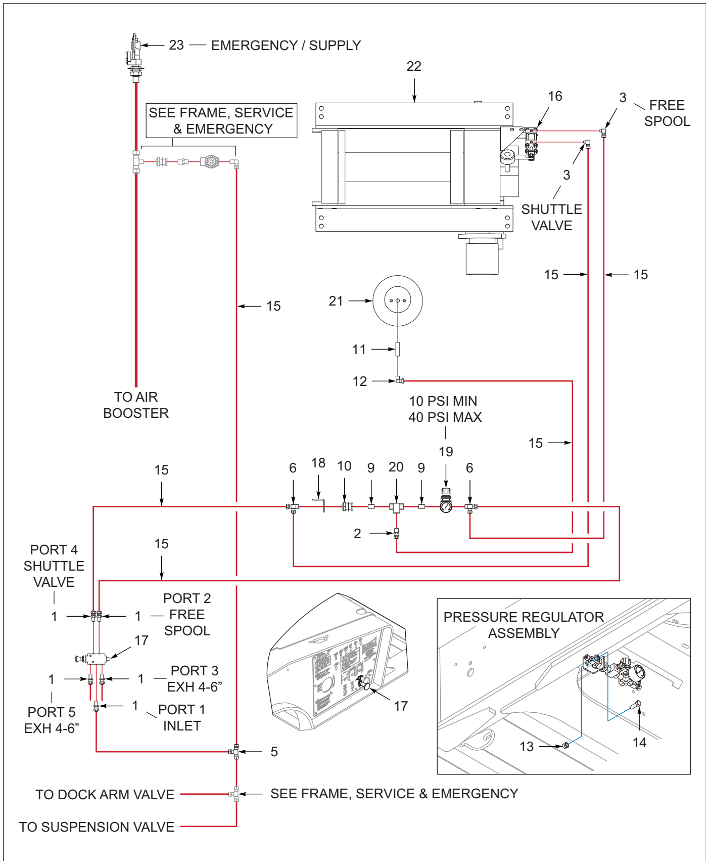
Figure 6-22: Winch Install, Braden 20K, 1 Speed, Air Tension (OPTION)
