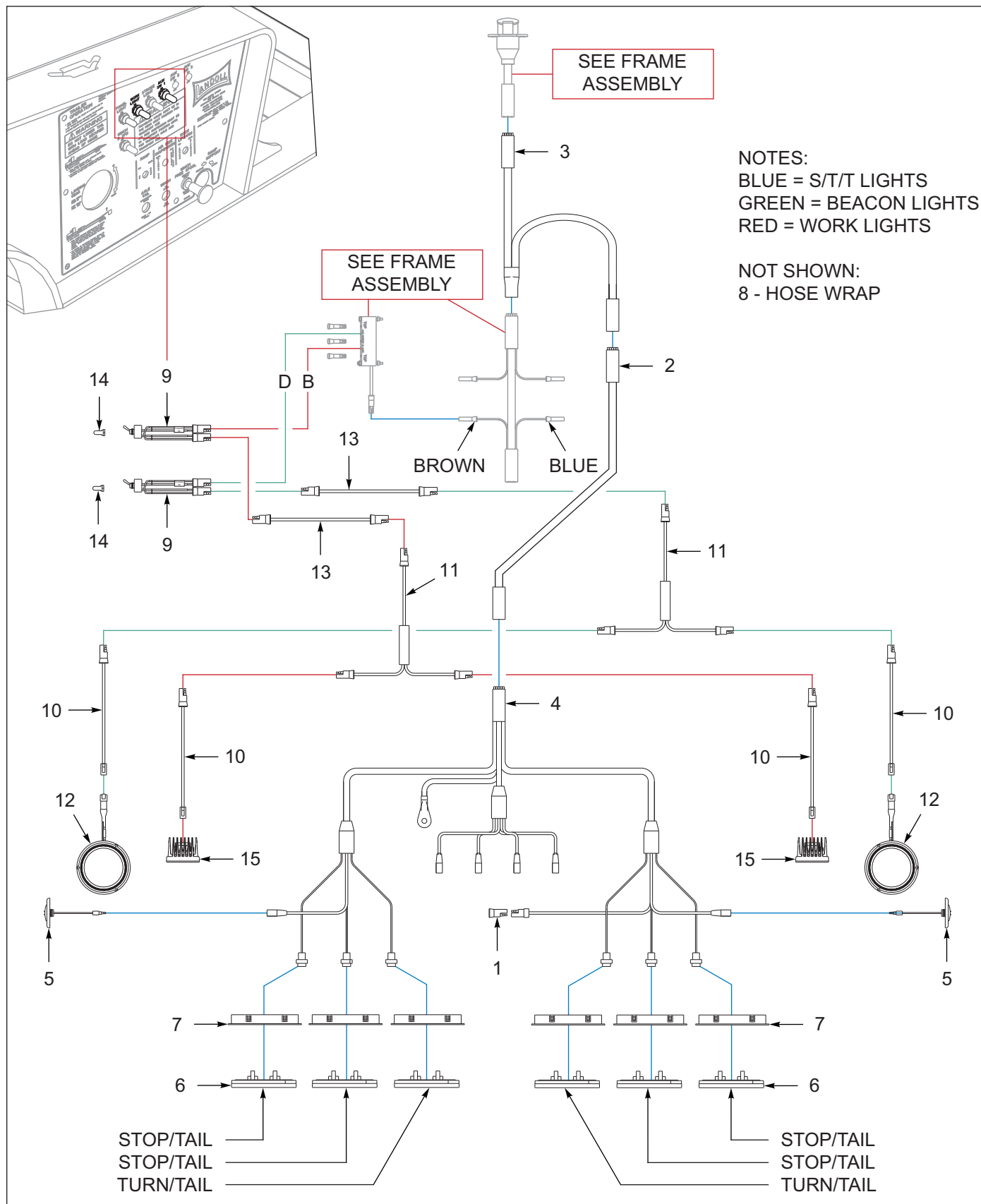
Figure 7-13: Bulkhead, Light Bar, Chain Rack (OPTIONS)
