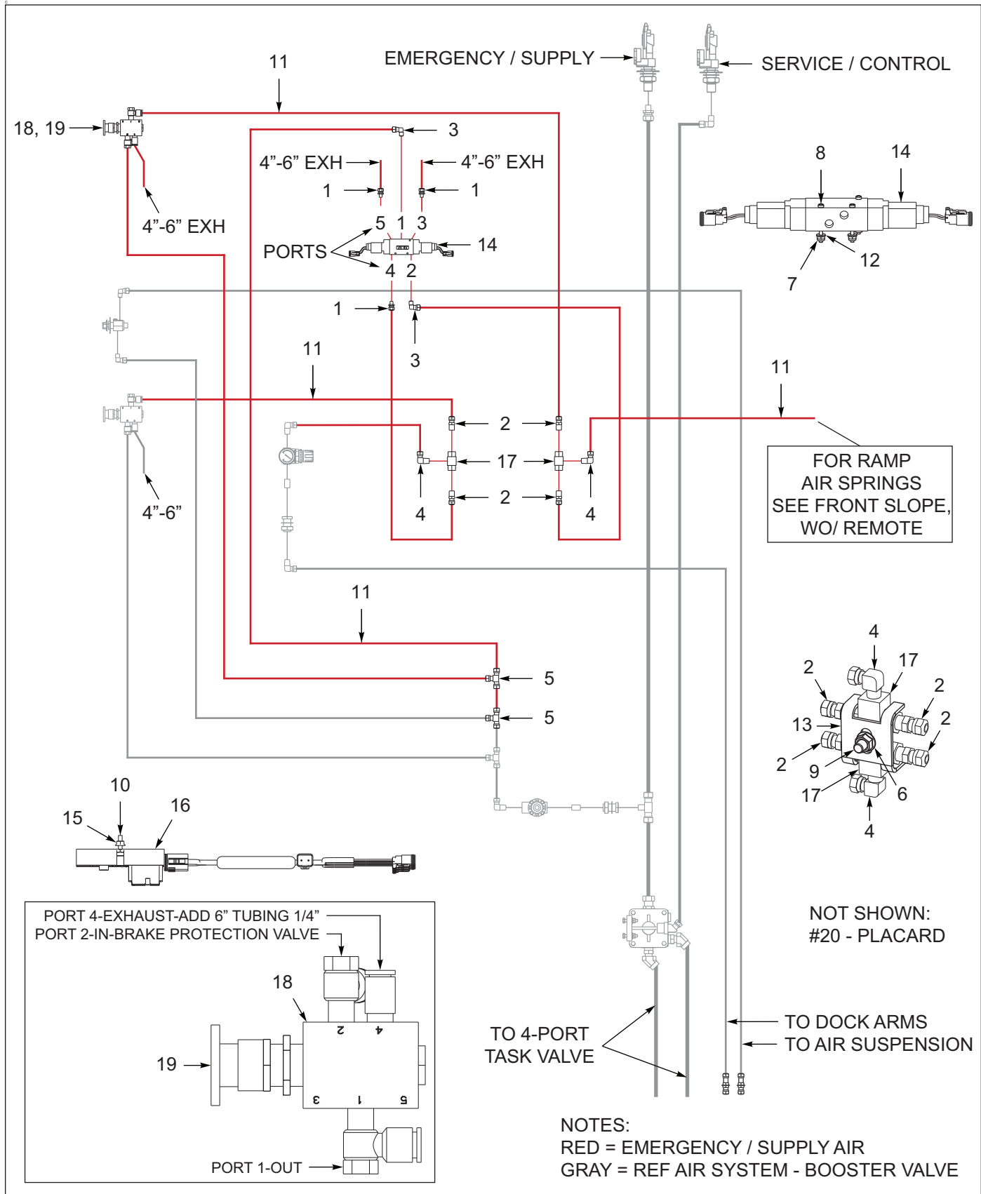
Figure 6-7: Ramp, Front Slope & Dock Arms, W/ Remote (OPTION)
