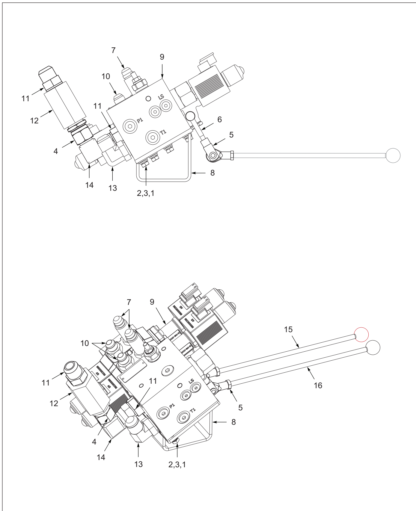
Figure 9-5: Valve Assembly, 2 Spool Solenoid
