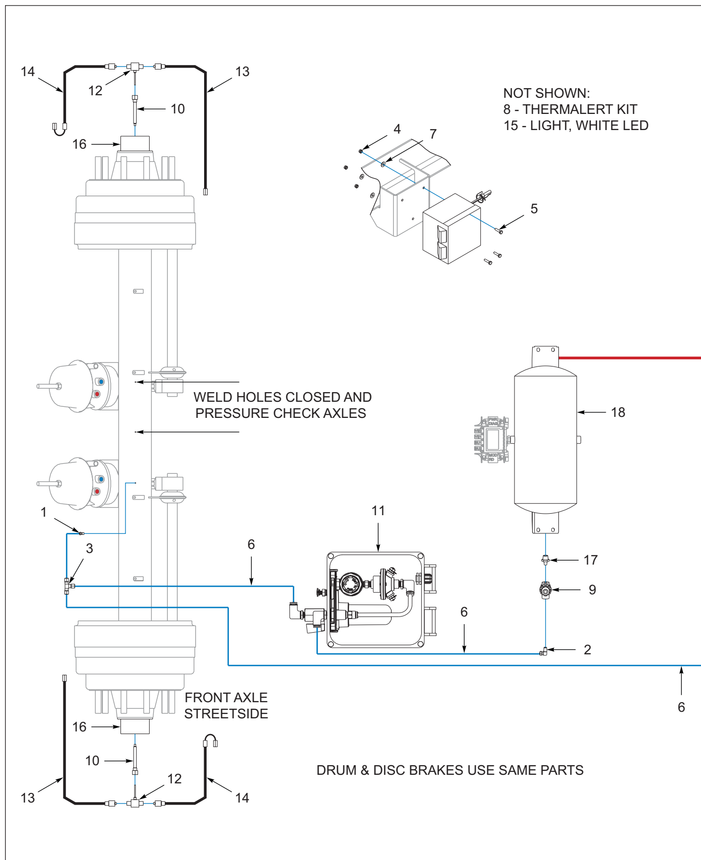
Figure 6-16: Tire Inflation, 2 Axle (OPTION) (1 of 2)
