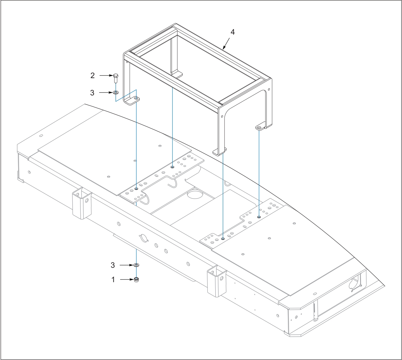
Figure 11-28: Guard, Winch W/ Cable Pivot Guide (OPTION)
