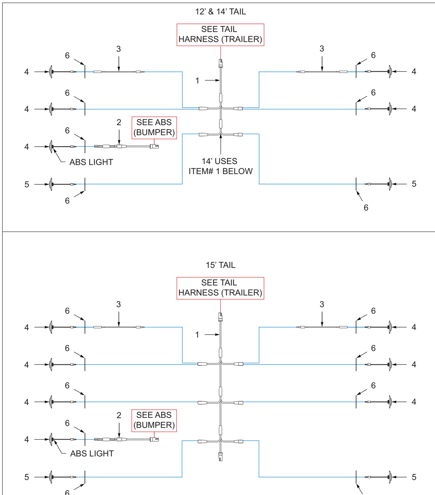
Figure 7-5: Tail Assembly
