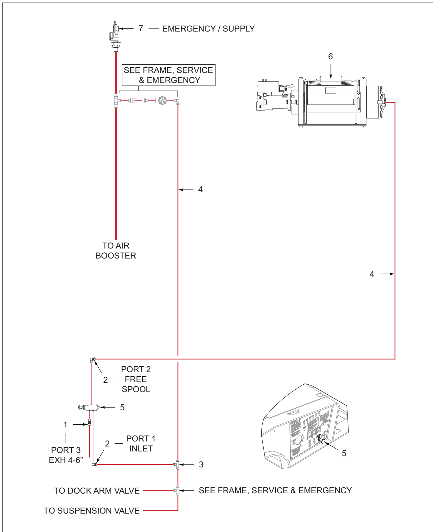
Figure 6-26: Winch Install, Warn 20K / 30K, 2 Speed, Spring Tension (OPTION)
