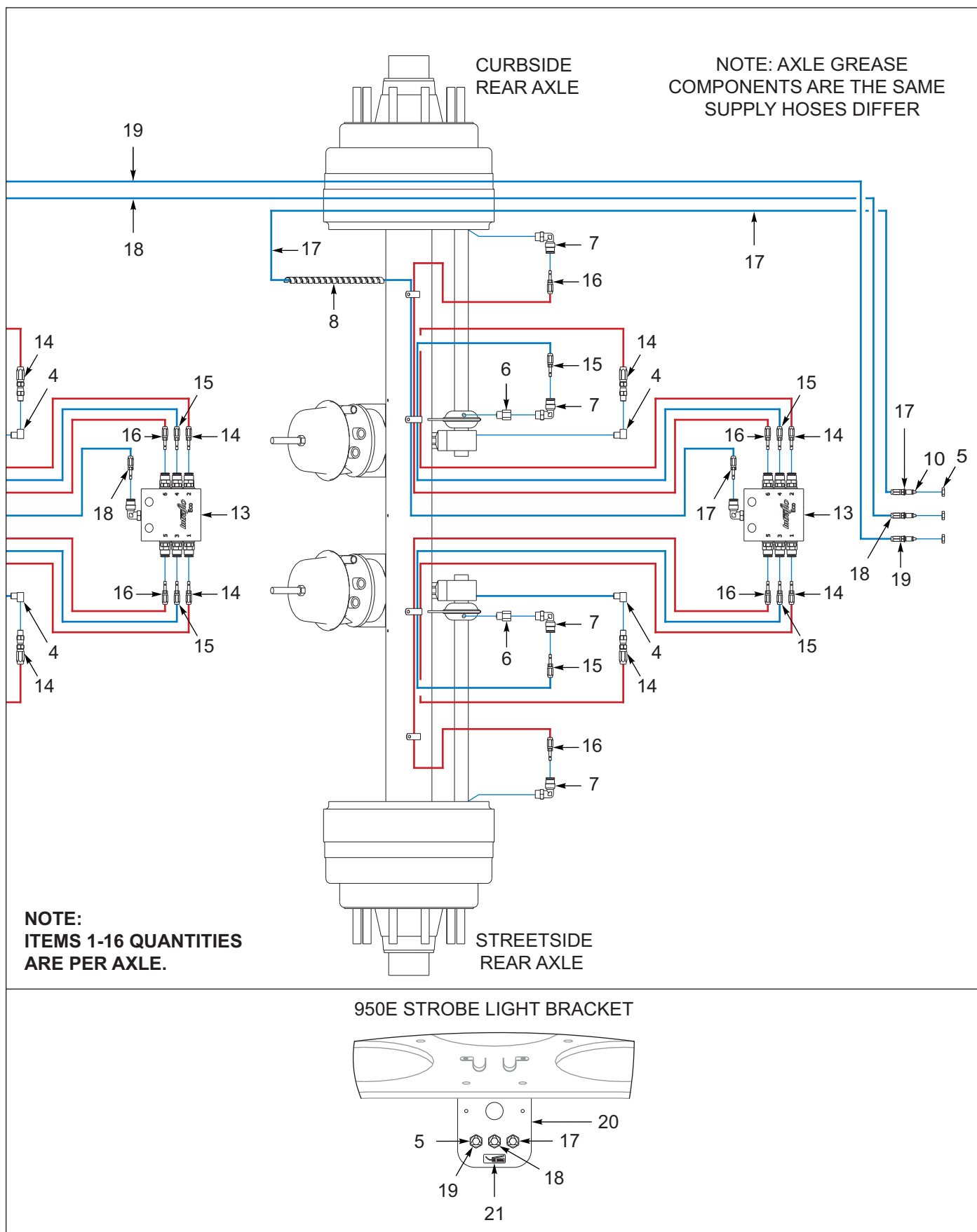
Figure 8-9: Drum Brakes, 3 Axle (After 08/31/2020) (2 of 3)
