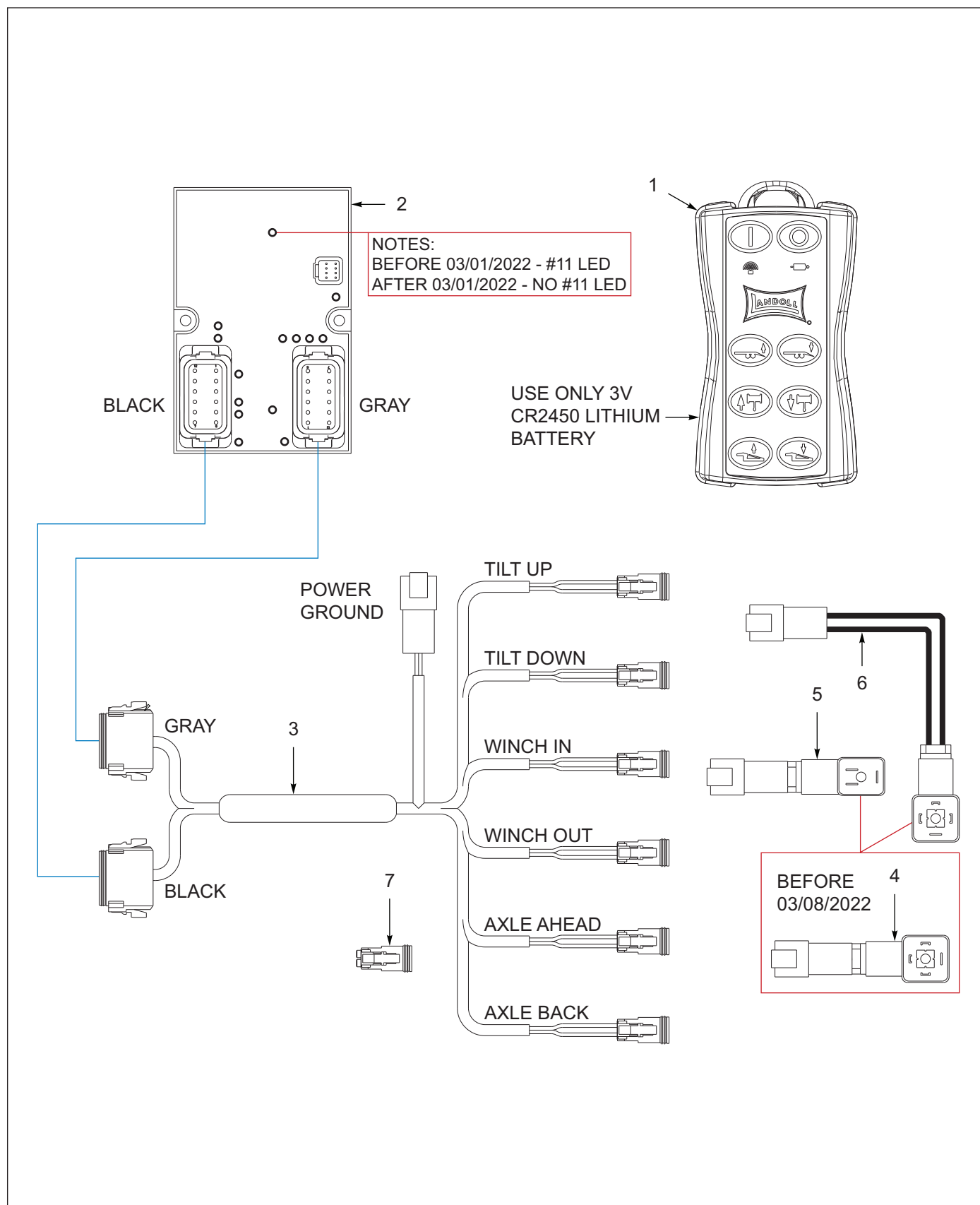
Figure 7-14: Remote Control Assembly, Wireless Brand (OPTION)
