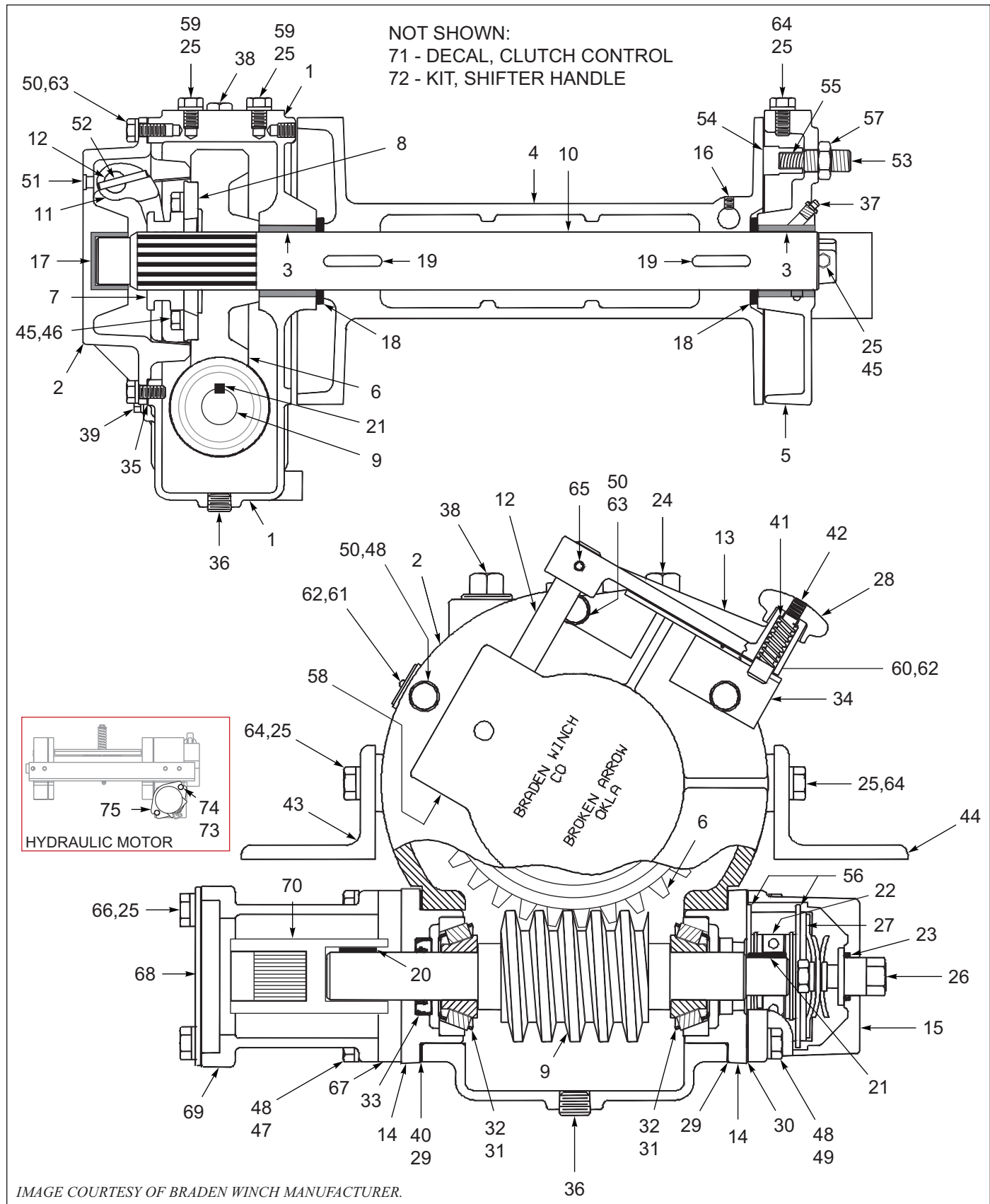
Figure 11-13: Winch Components, Braden 20K, 1 Speed (OPTION)
