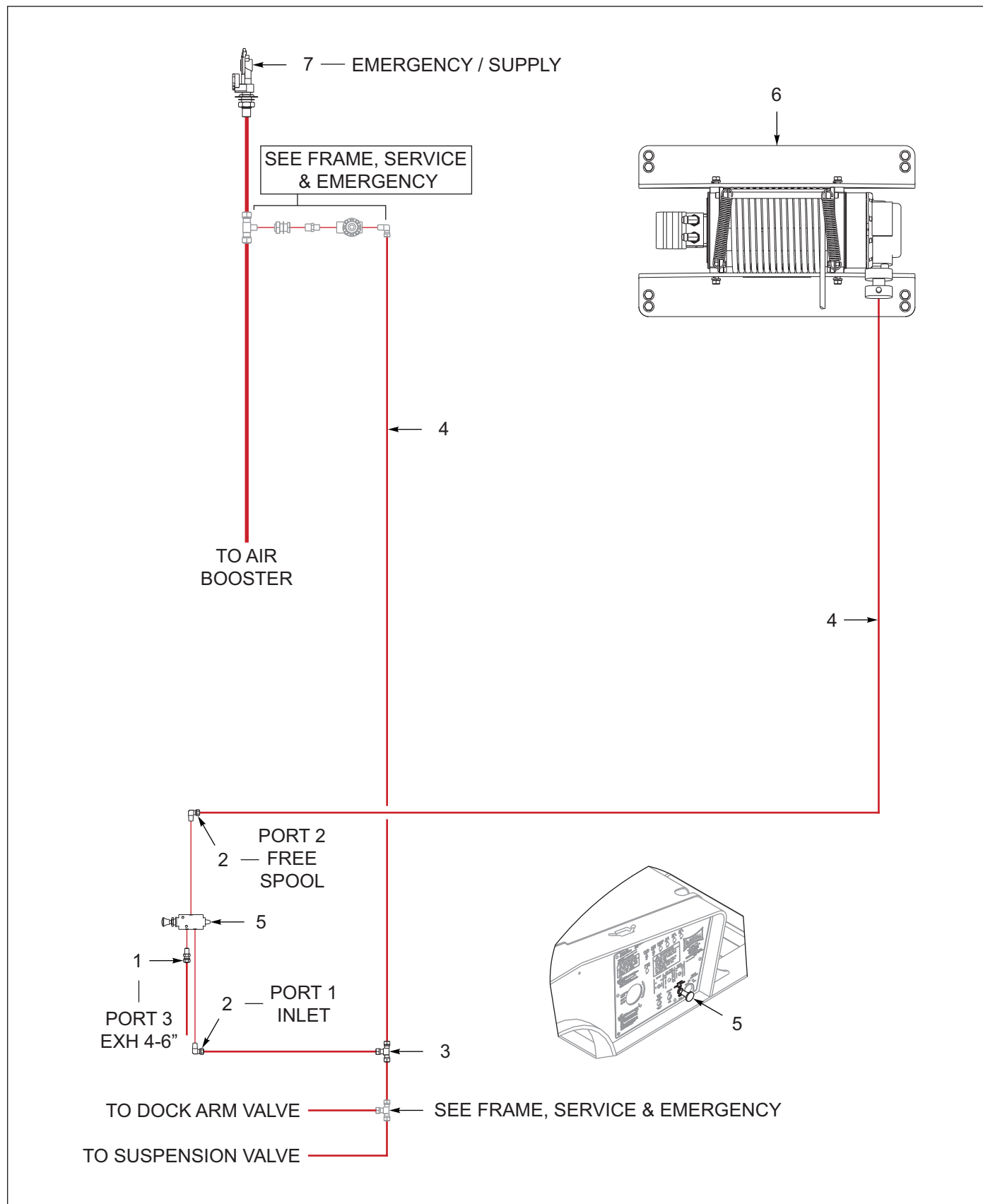
Figure 6-25: Winch Install, Warn 12K, 1 Speed, Spring Tension (OPTION)
