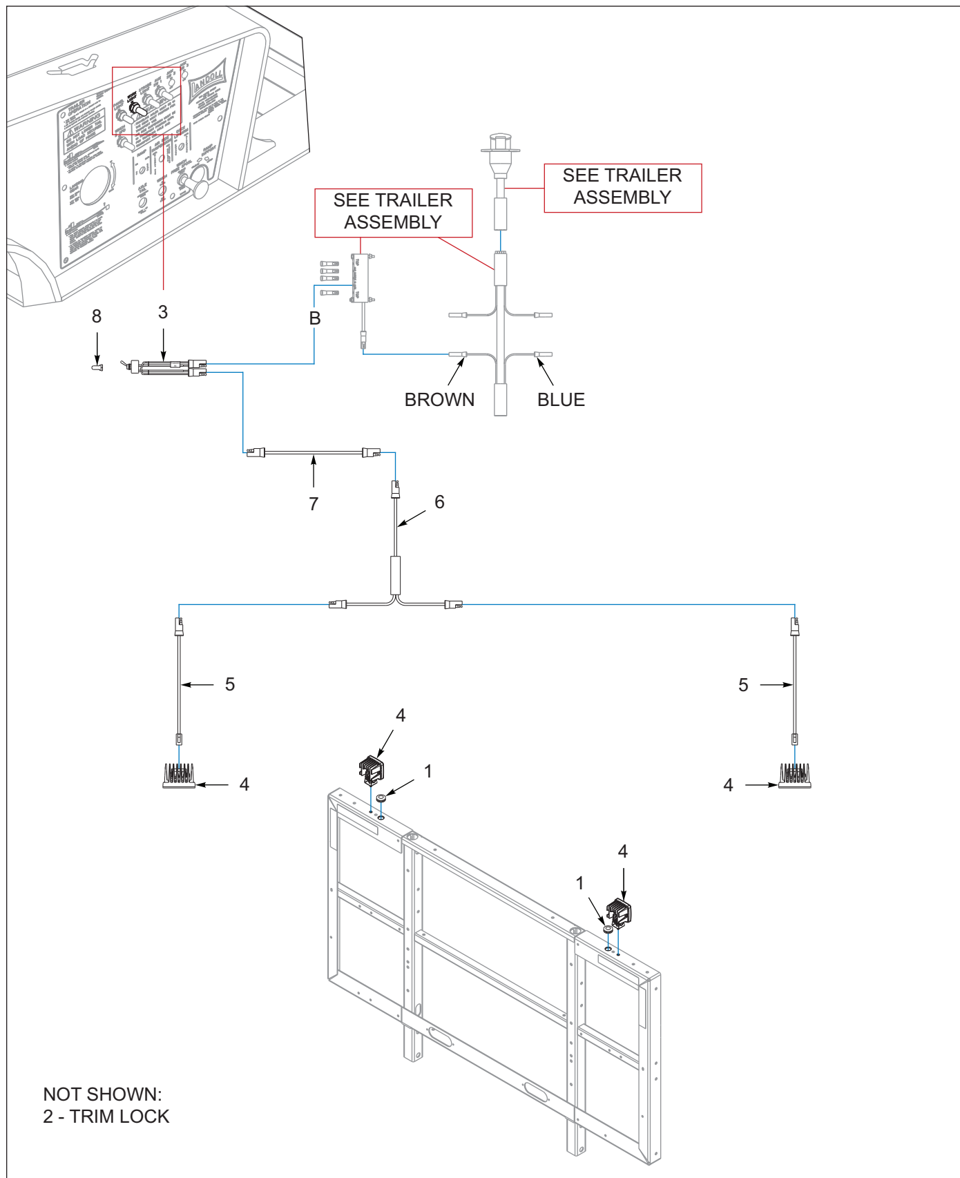
Figure 7-12: Bulkhead, Lights, Work (OPTIONS)
