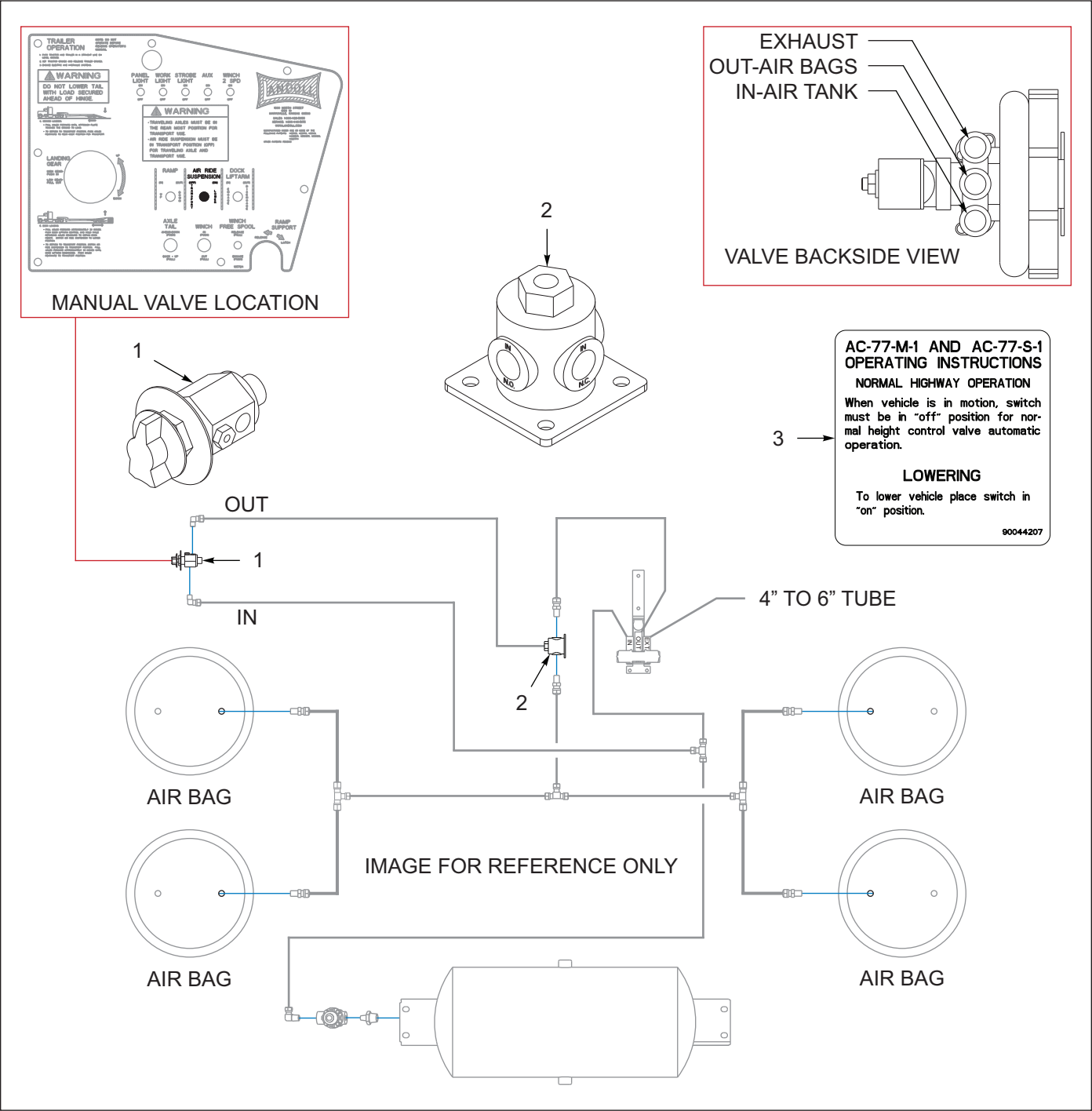
Figure 6-15: Suspension Lowering Air Control, Kit
