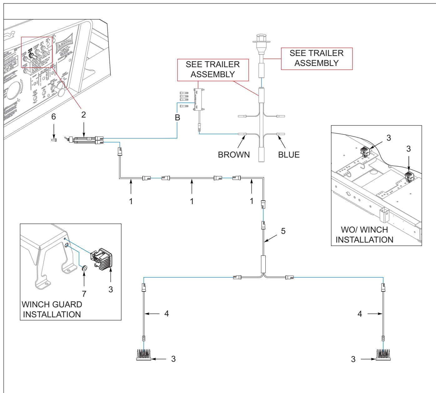
Figure 7-23: Winch Work Lights (OPTION)
