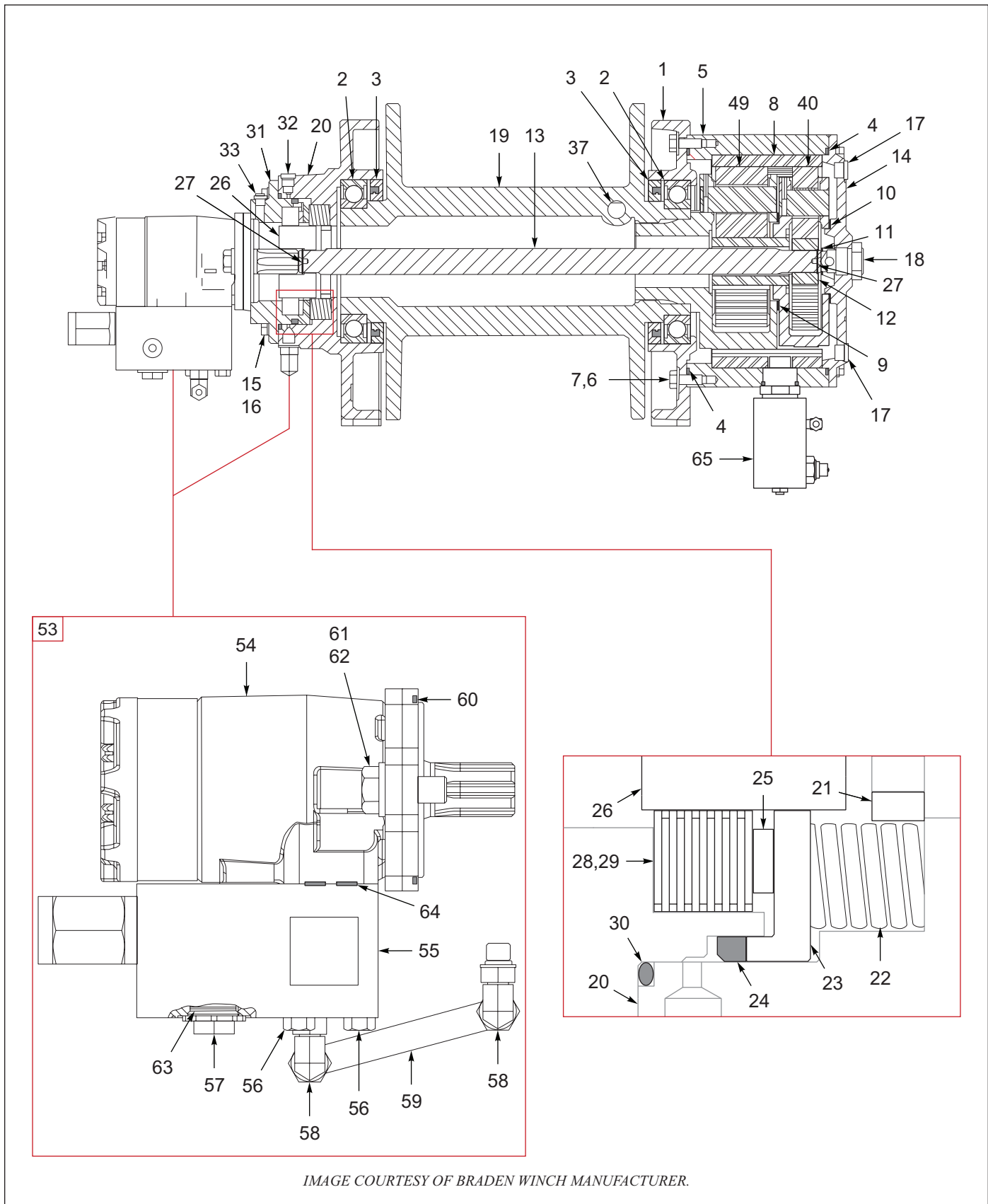
Figure 11-16: Winch Components, Braden 20K, 2 Speed (OPTION) (1 of 2)
