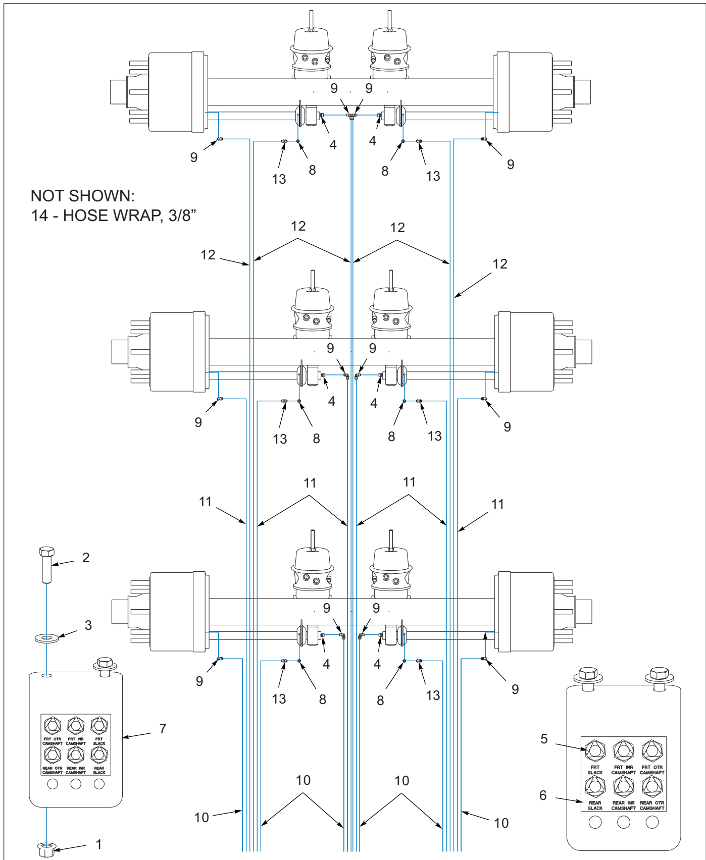
Figure 8-7: Drum Brakes, 3 Axle (After 11/07/2018 - Before 08/31/2020)
