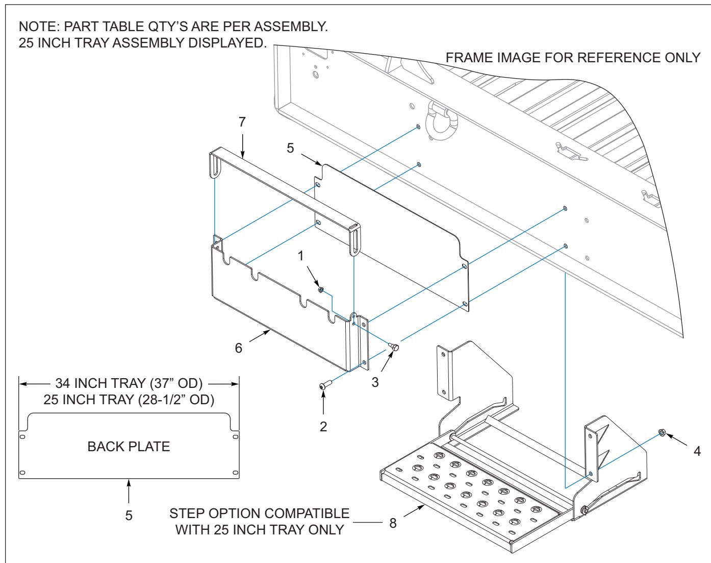
Figure 5-2: Chain Tray Assembly (AFTER 01/17/2022) (OPTIONS)
