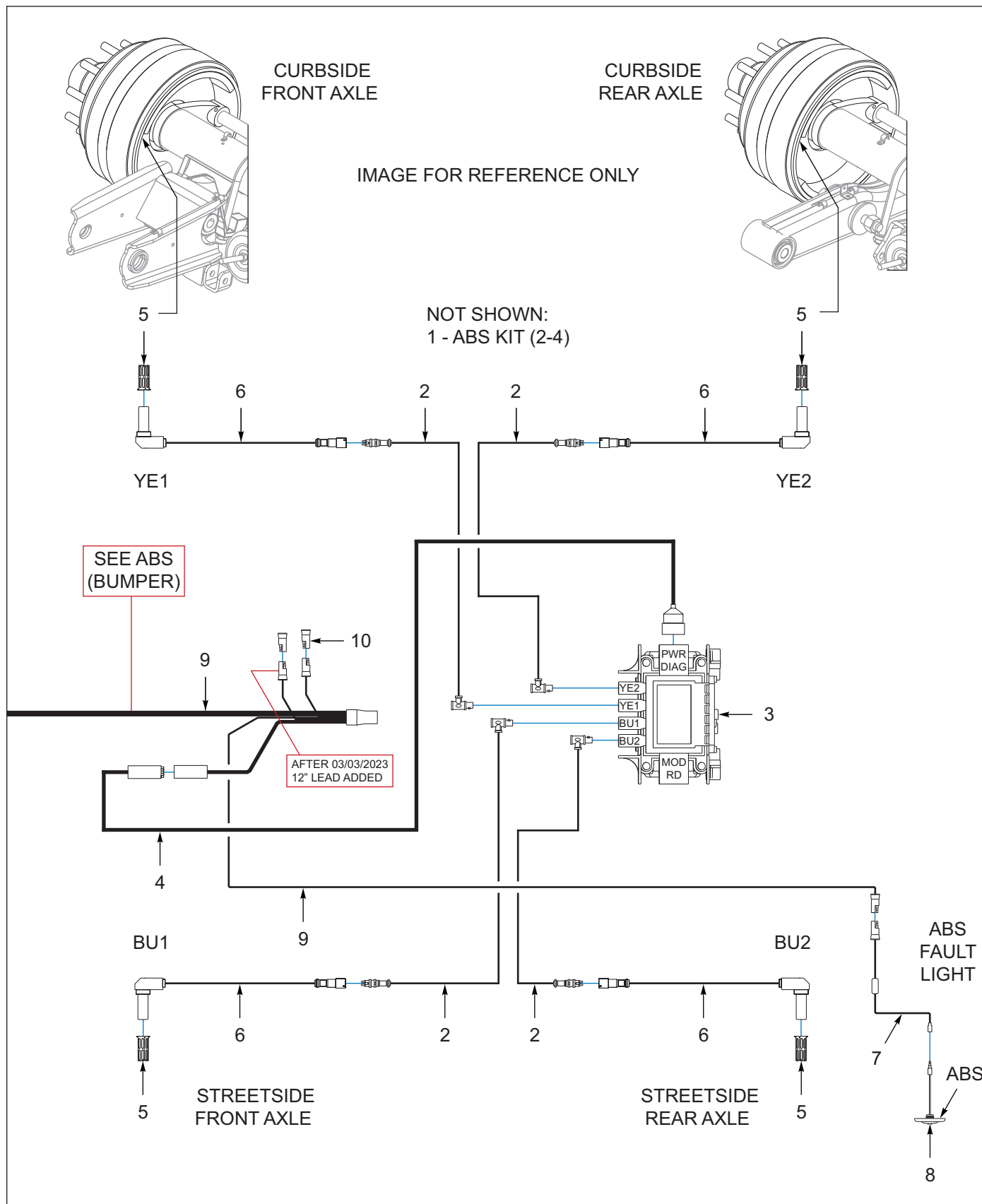
Figure 7-8: Anti-Lock Brakes, Wabco (1 of 2)
