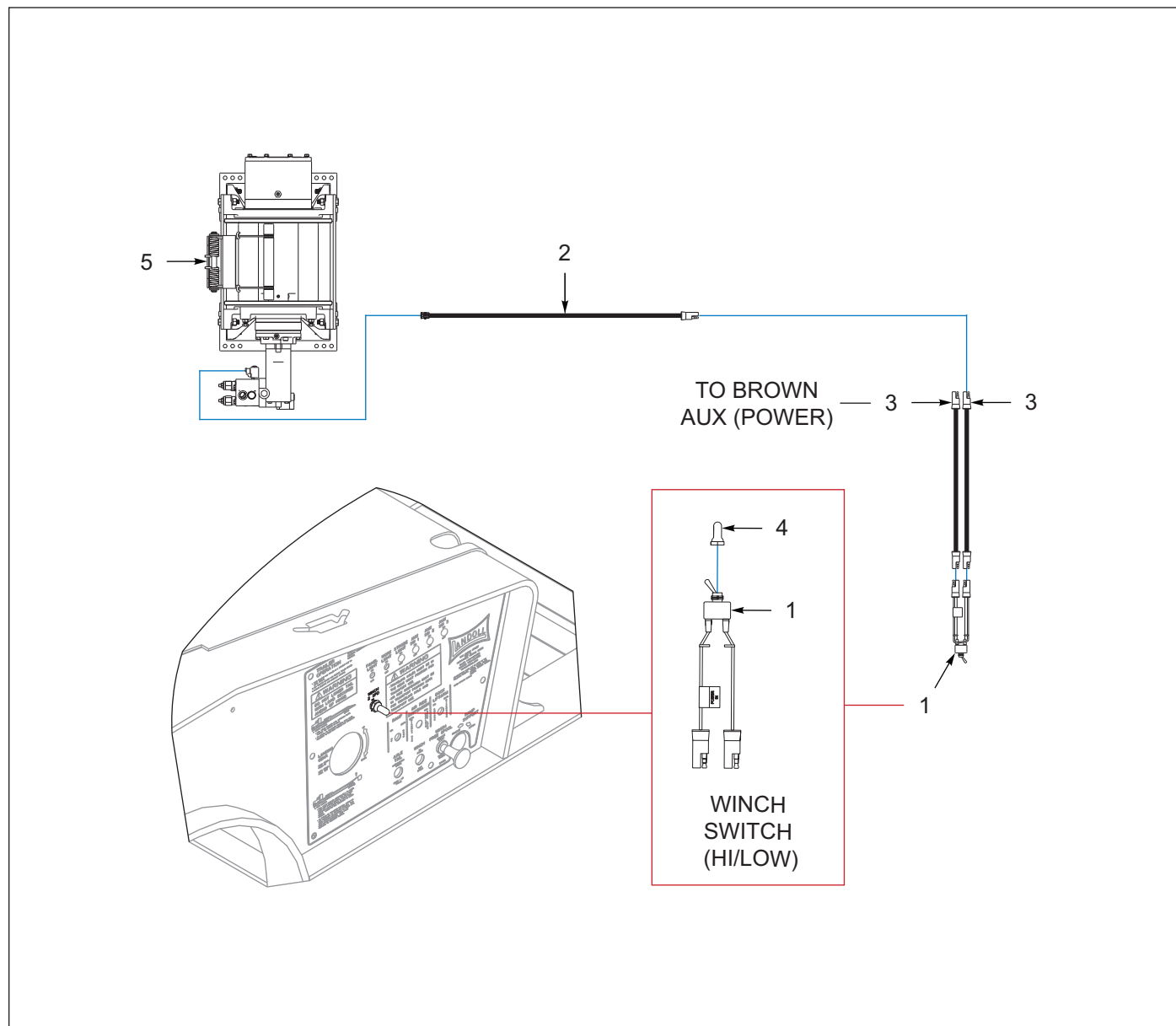
Figure 7-21: Winch Install, Ramsey 20K / 30K, 2 Speed (OPTION)
