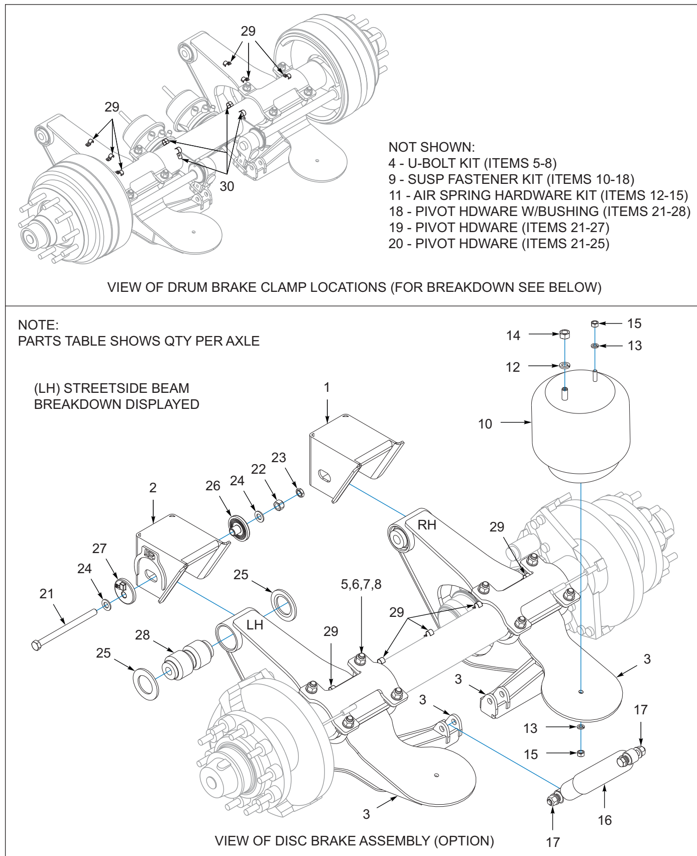
Figure 3-11: Axle Suspension, LSS-25K-5.5 RLU, 16.5
