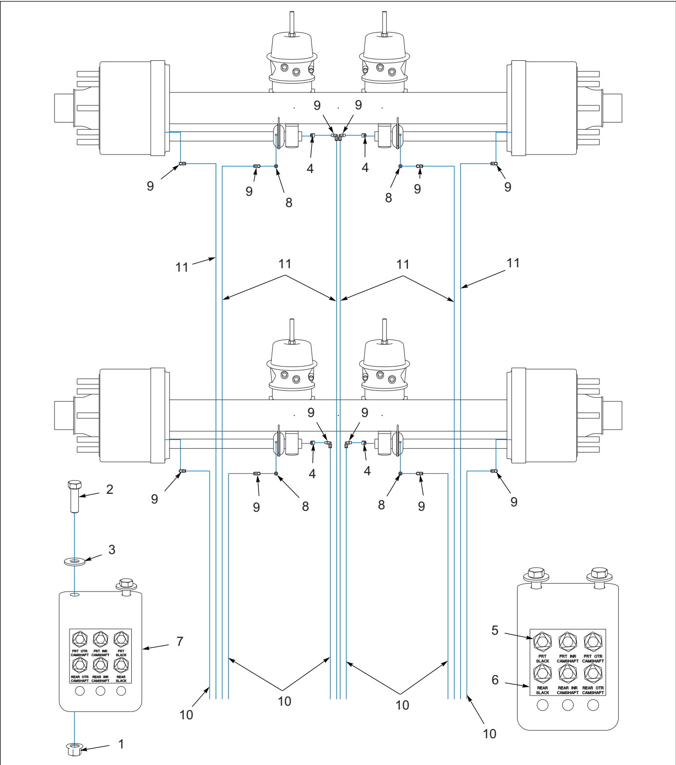
Figure 8-1: Drum Brakes, 2 Axle (Before 11/07/2018)
