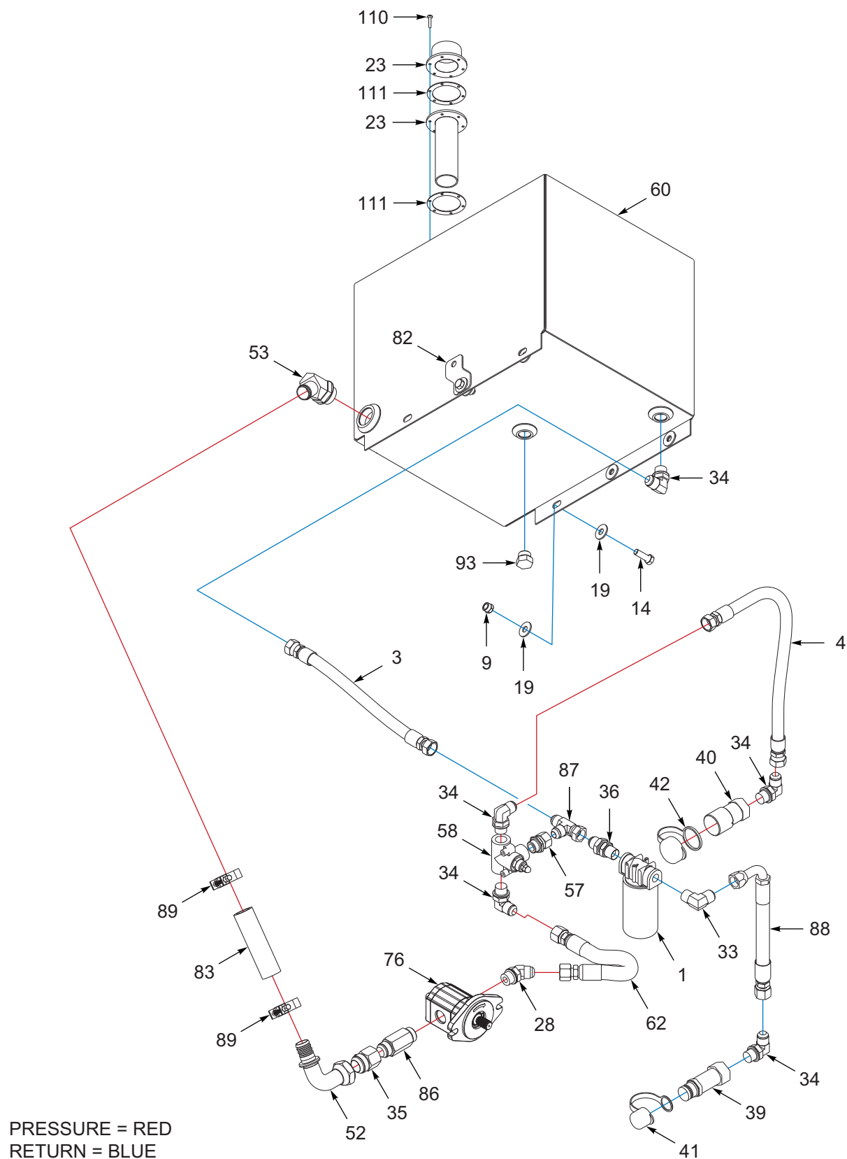
Figure 10-5: Engine, 25HP, Upper Deck Assembly (OPTION) (5 of 5)
