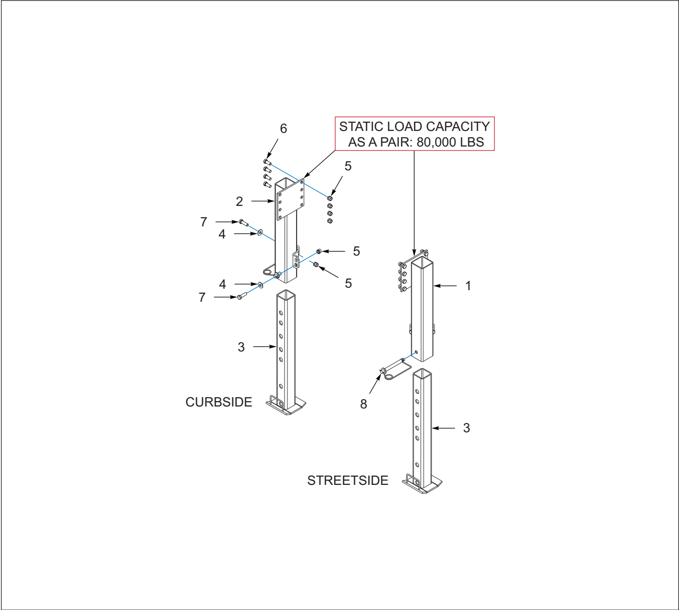
Figure 2-10: Landing Legs, Pinned (OPTION)
