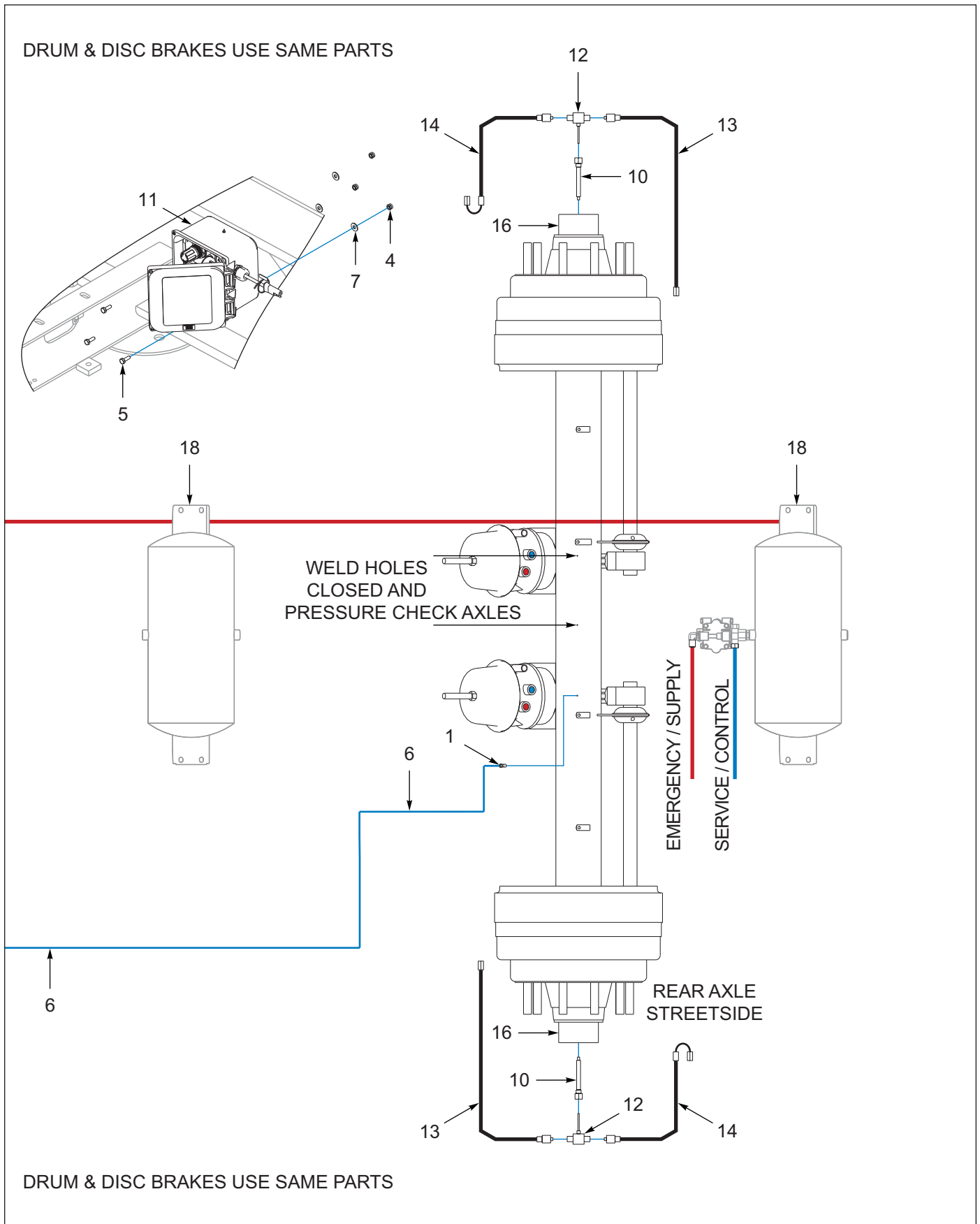
Figure 6-19: Tire Inflation, 3 Axle (OPTION) (2 of 2)
