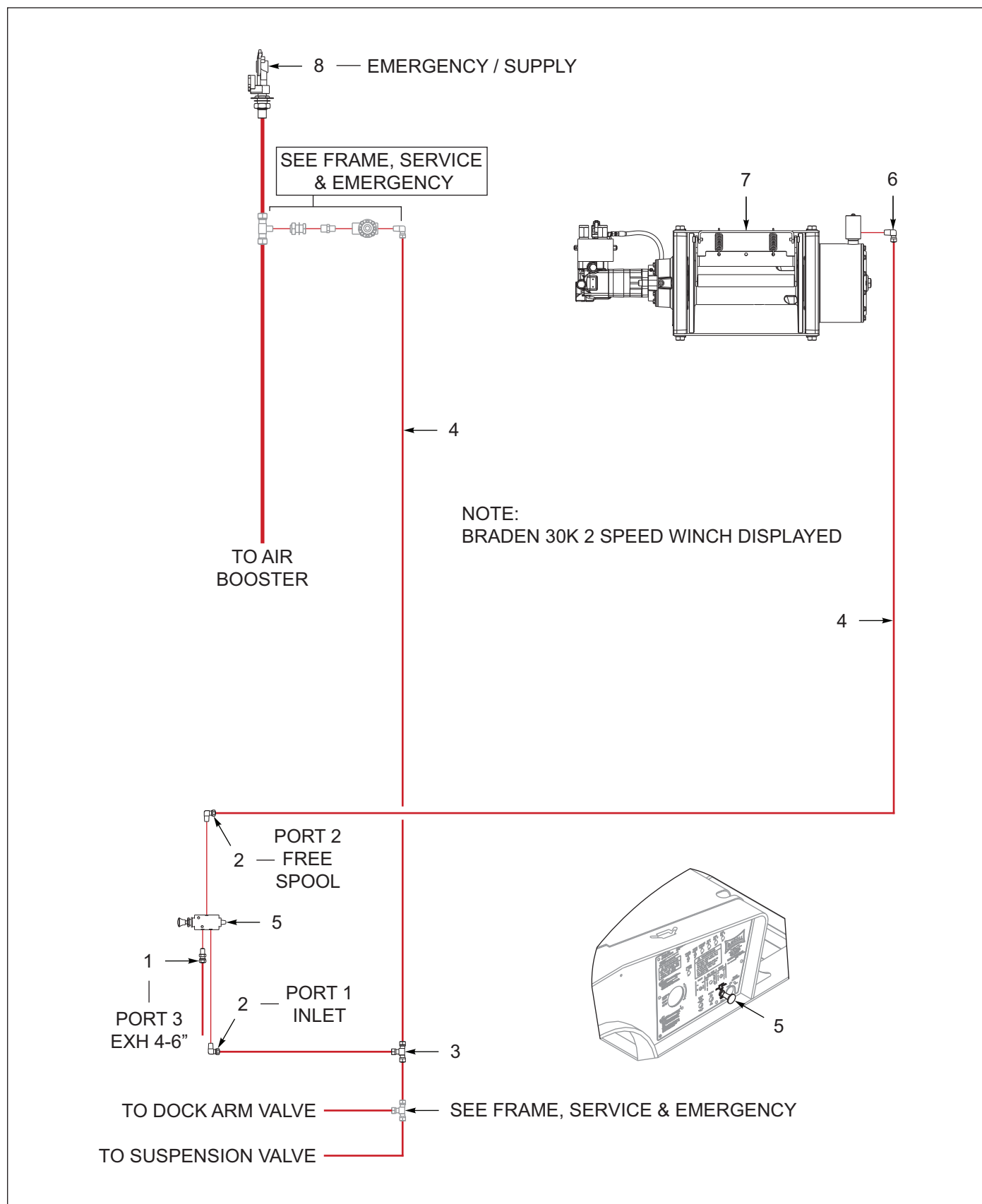
Figure 6-23: Winch Install, Braden 20K / 30K, 2 Speed (OPTION)
