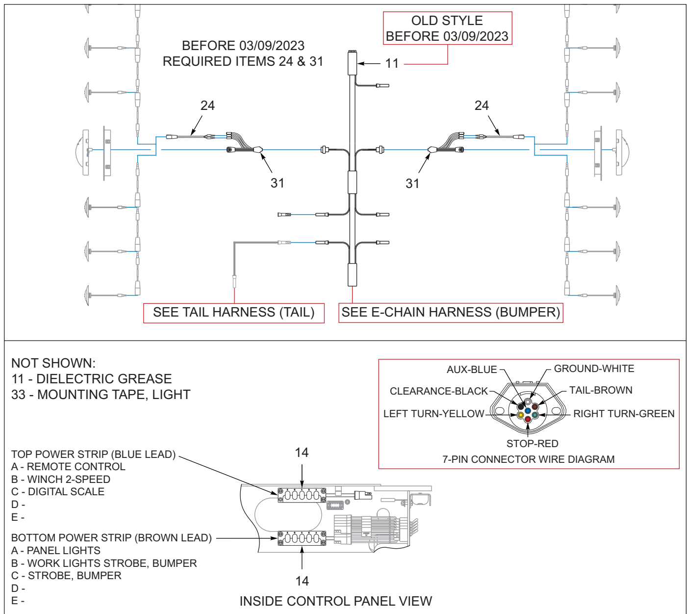
Figure 7-4: Trailer Assembly (AFTER 02/15/2022) (2 of 2)
