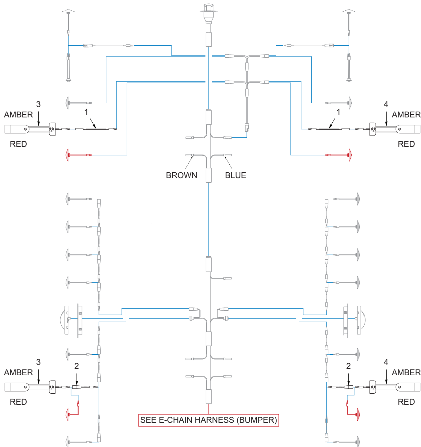
Figure 7-15: Swing Arm Light, Marker, Amber & Red (OPTION) (2 of 2)
