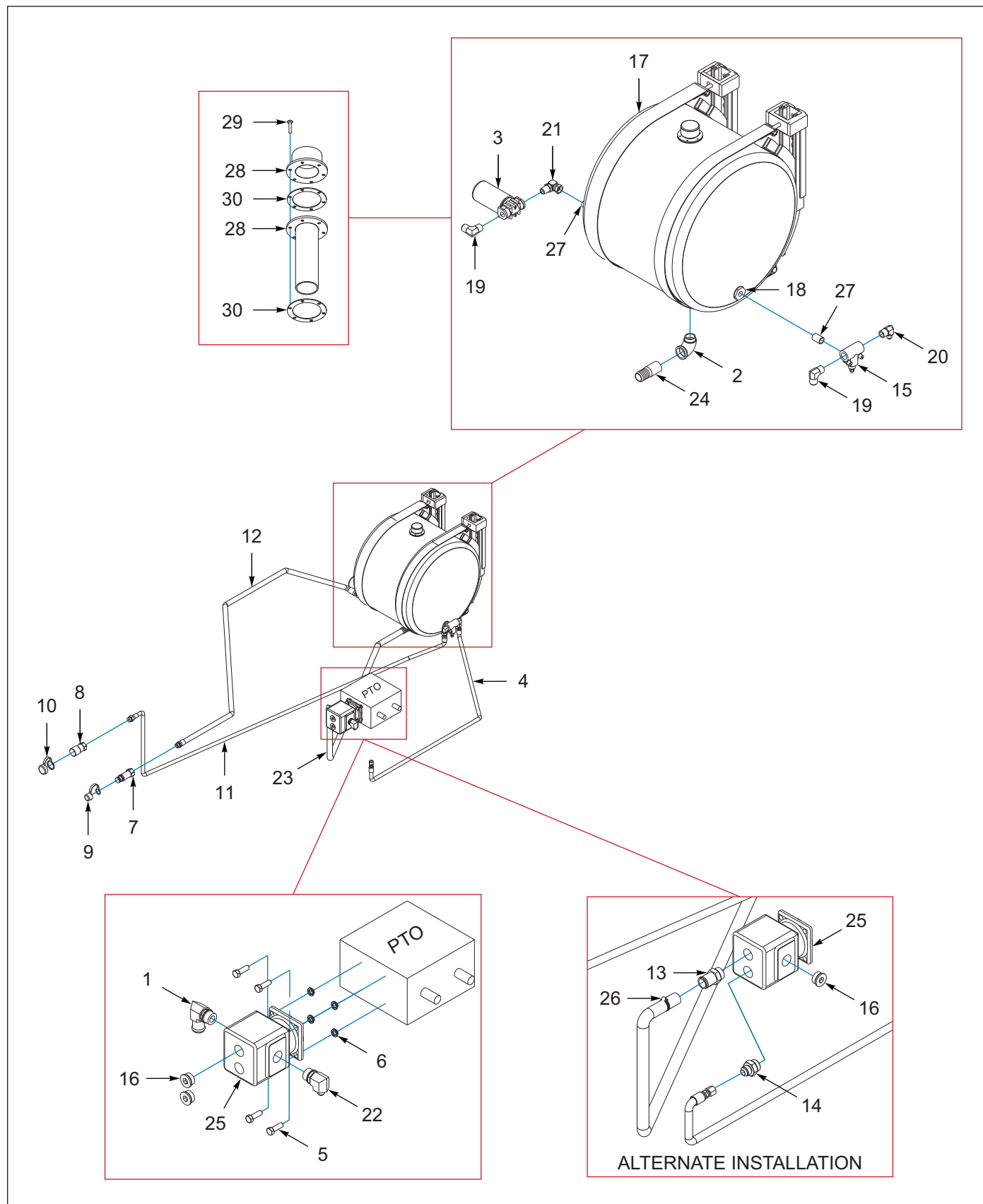
Figure 9-8: et Kit, Hydraulic (OPTION) (AFTER 03/01/2019)
