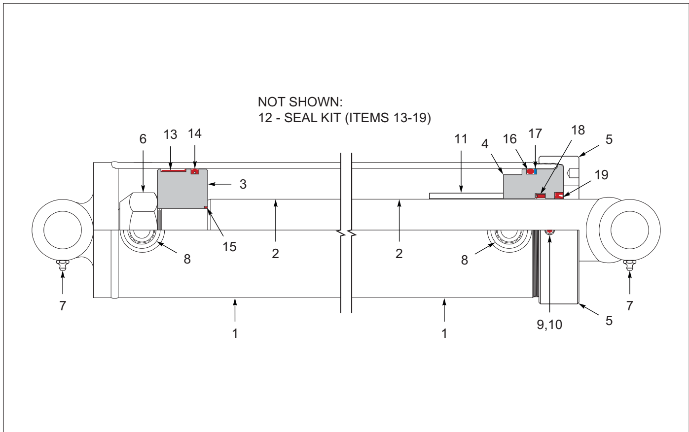
Figure 9-4: Cylinder Components, 5 x 60
