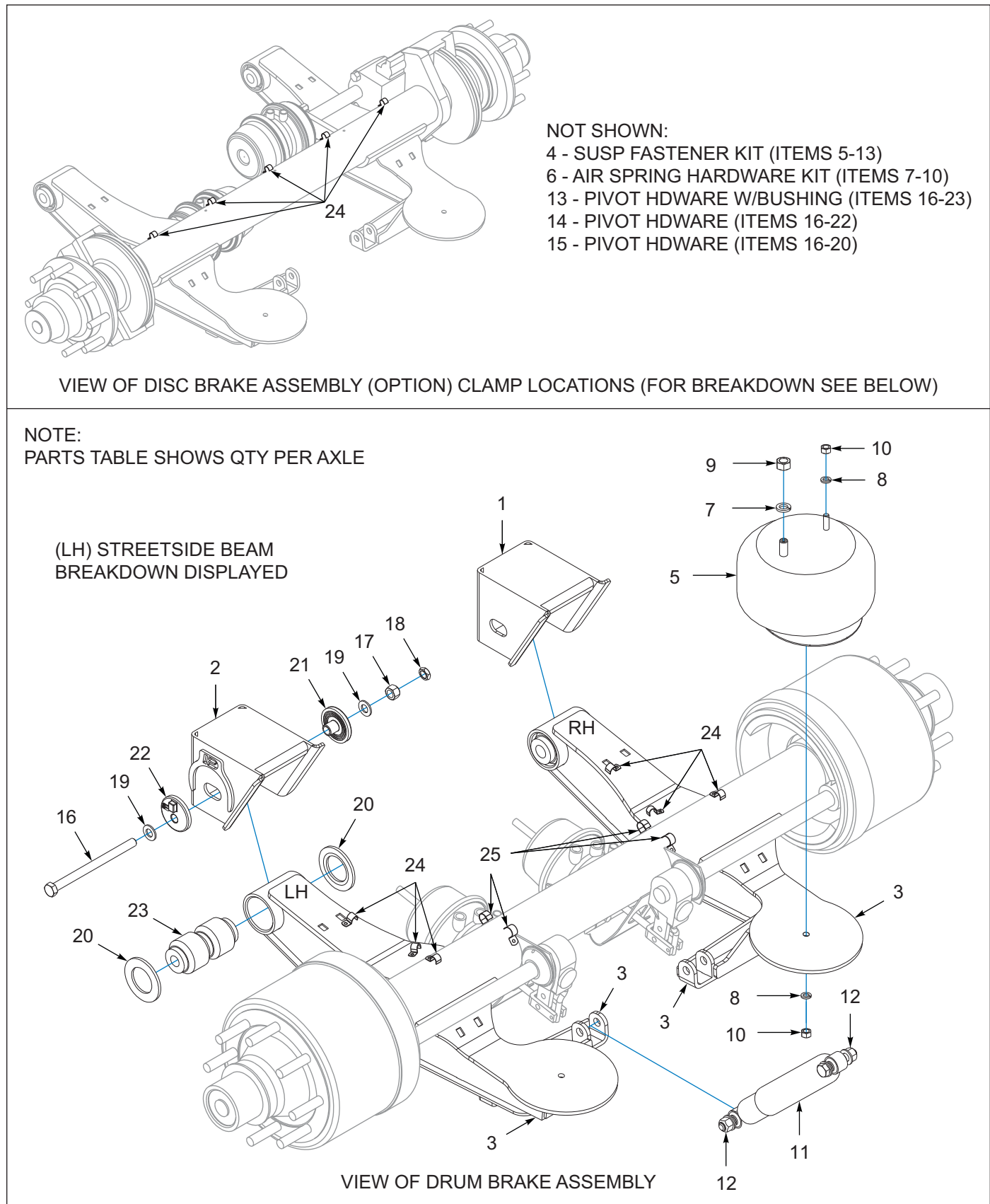
Figure 3-10: Axle Suspension, LSS-25K-3.5 RLU, 12.25
