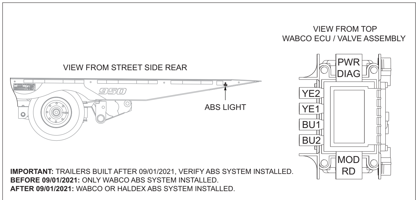
Figure 7-9: Anti-Lock Brakes, Wabco (2 of 2)
