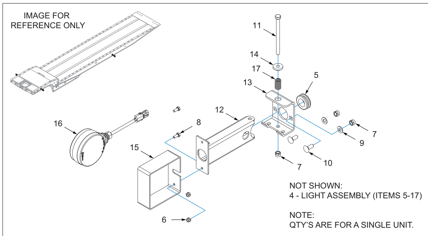
Figure 7-18: Swing Arm Light, Turn / Emergency, 4 In, Amber (OPTION) (2 of 2)
