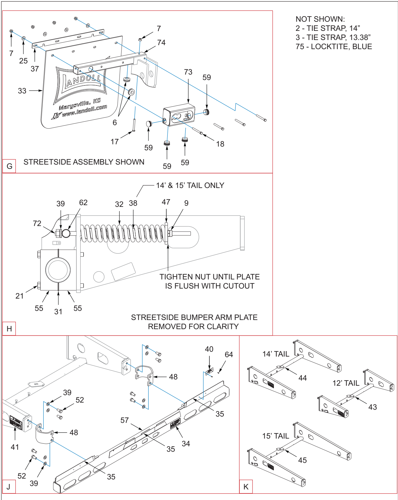
Figure 2-19: Undercarriage Components (3 of 3)
