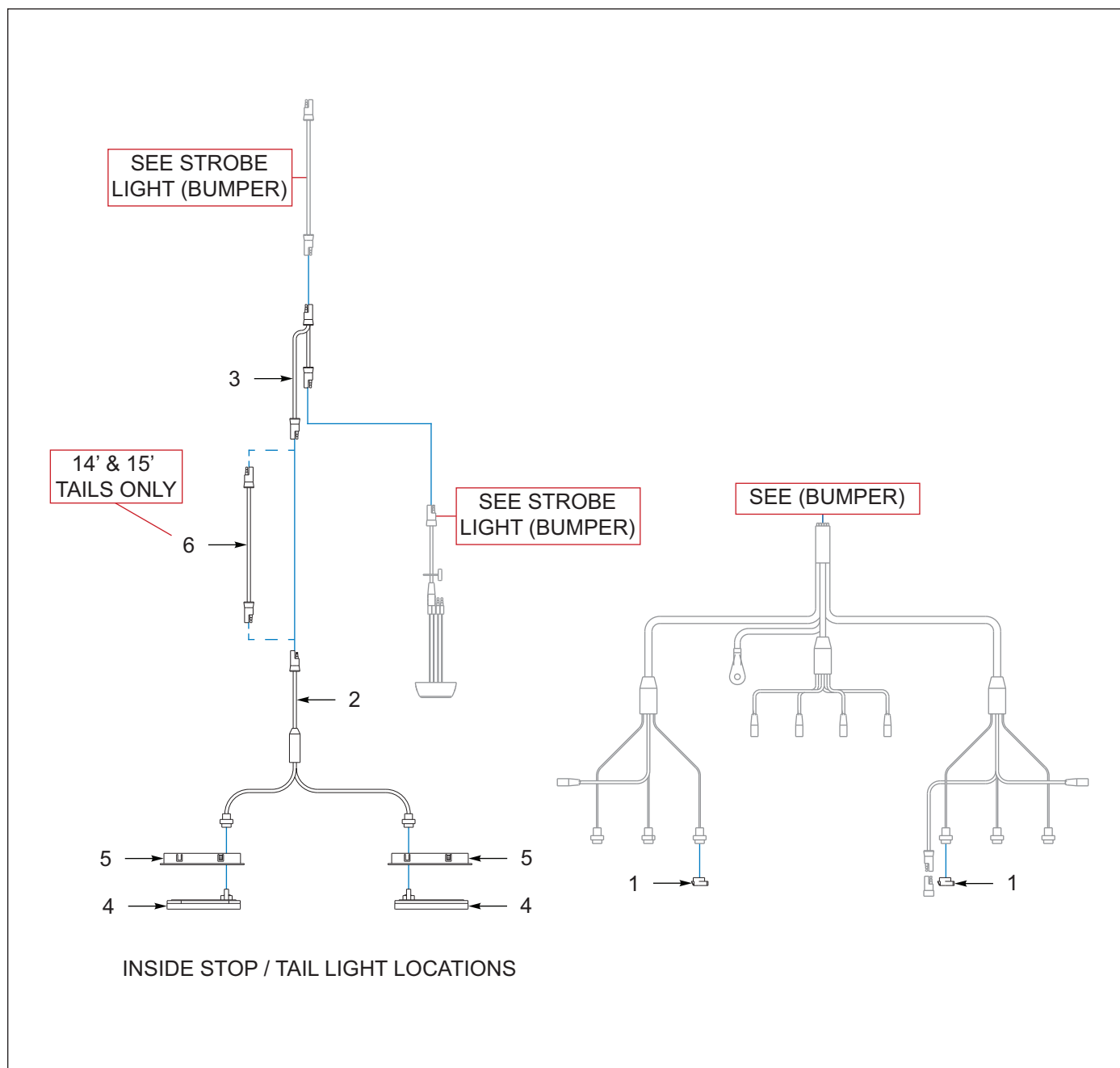
Figure 7-7: Bumper, Strobe Lights (OPTION)
