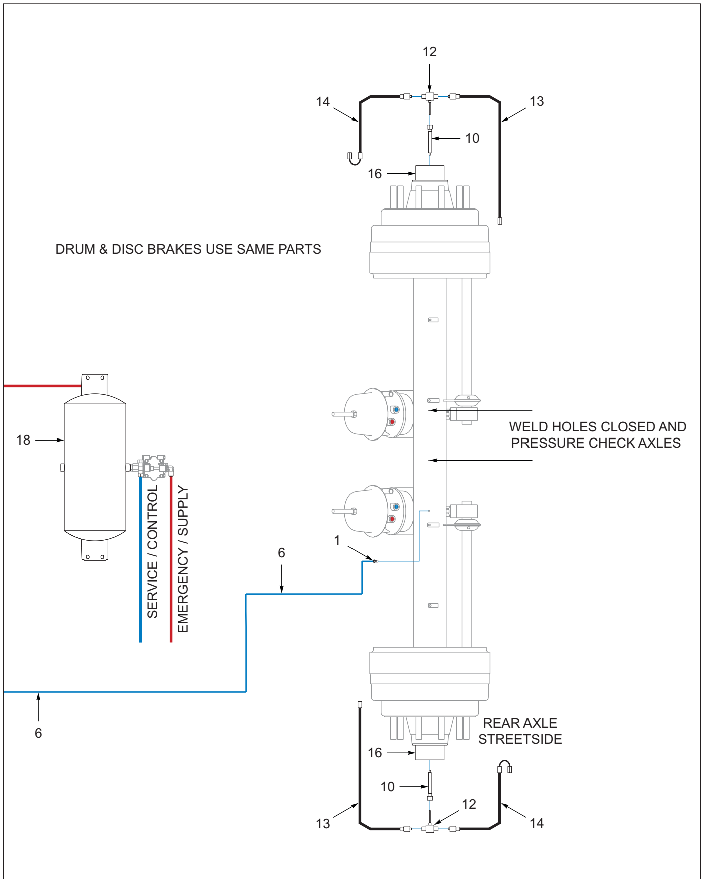
Figure 6-17: Tire Inflation, 2 Axle (OPTION) (2 of 2)
