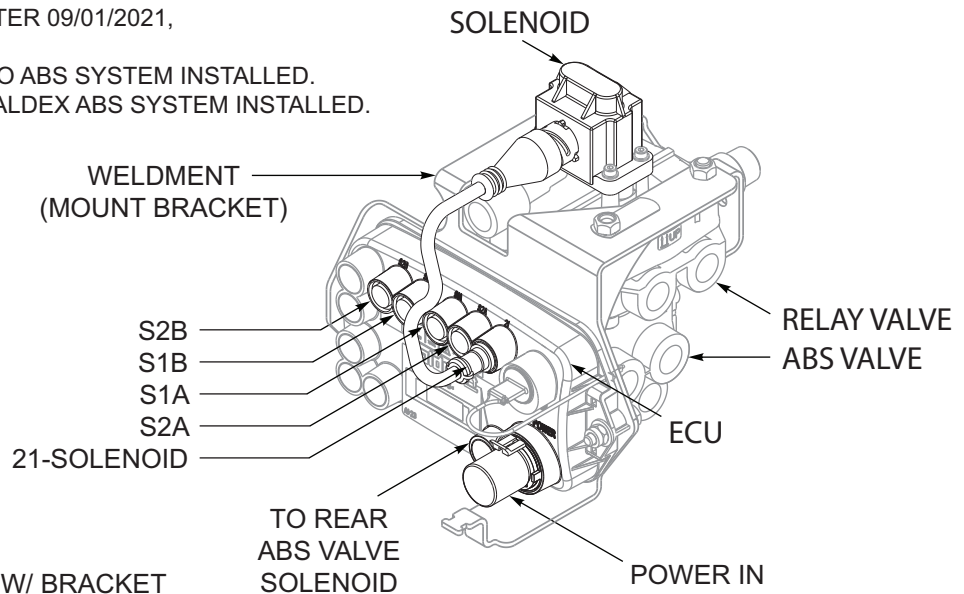
Figure 7-11: Anti-Lock Brakes, Haldex (2 of 2)
