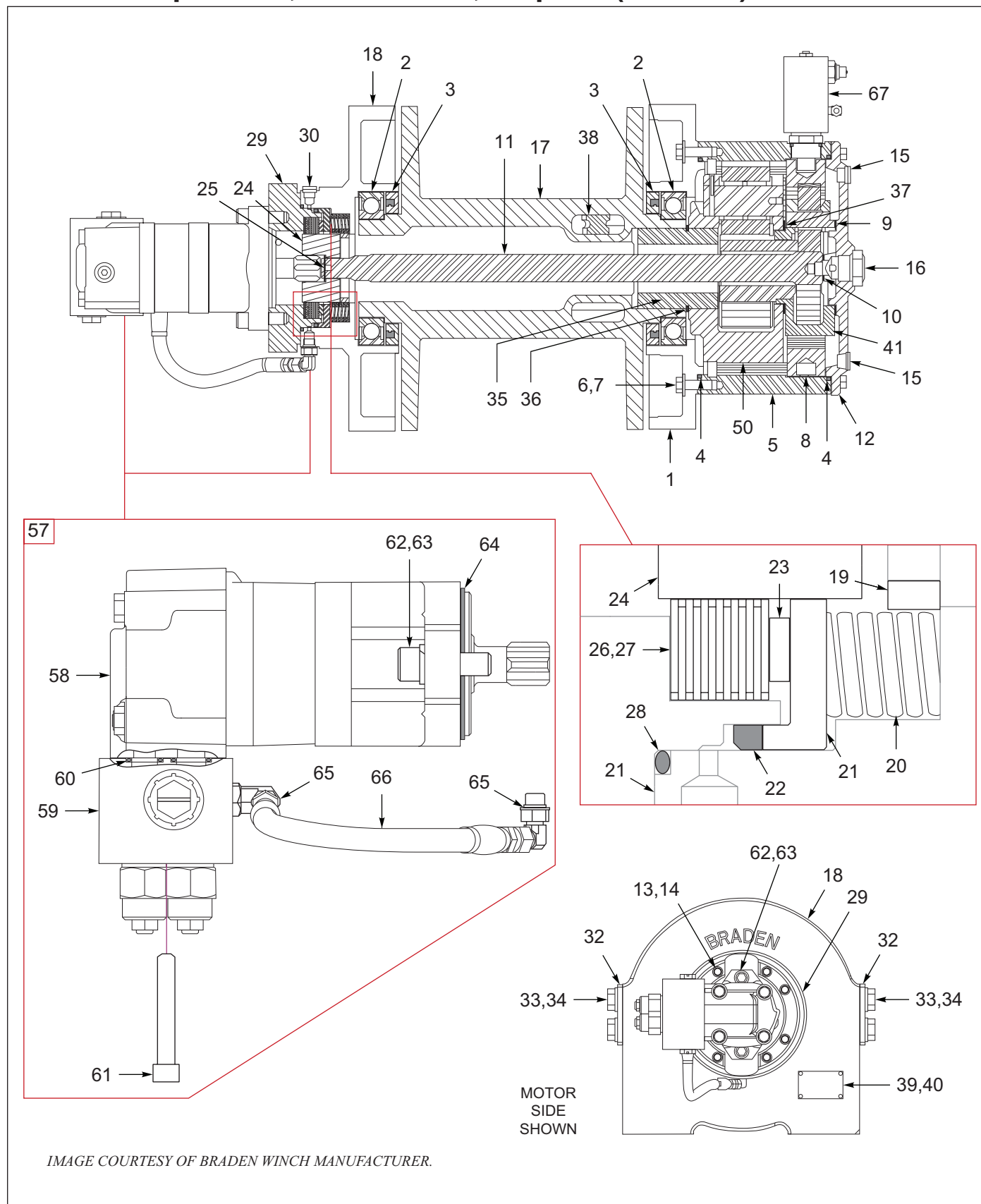
Figure 11-18: Winch Components, Braden 30K, 2 Speed (OPTION) (1 of 2)
