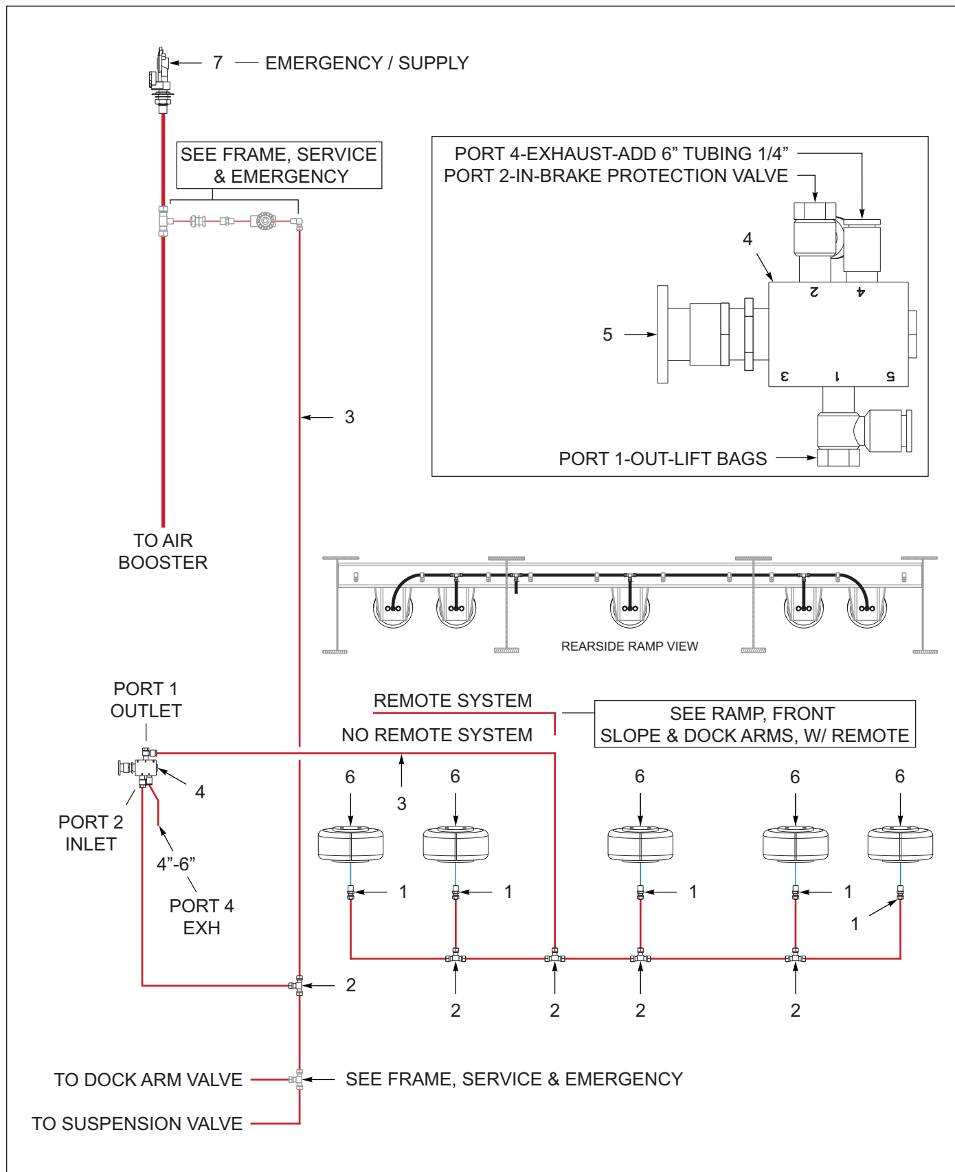
Figure 6-6: Ramp, Front Slope, WO/ Remote (OPTION)
