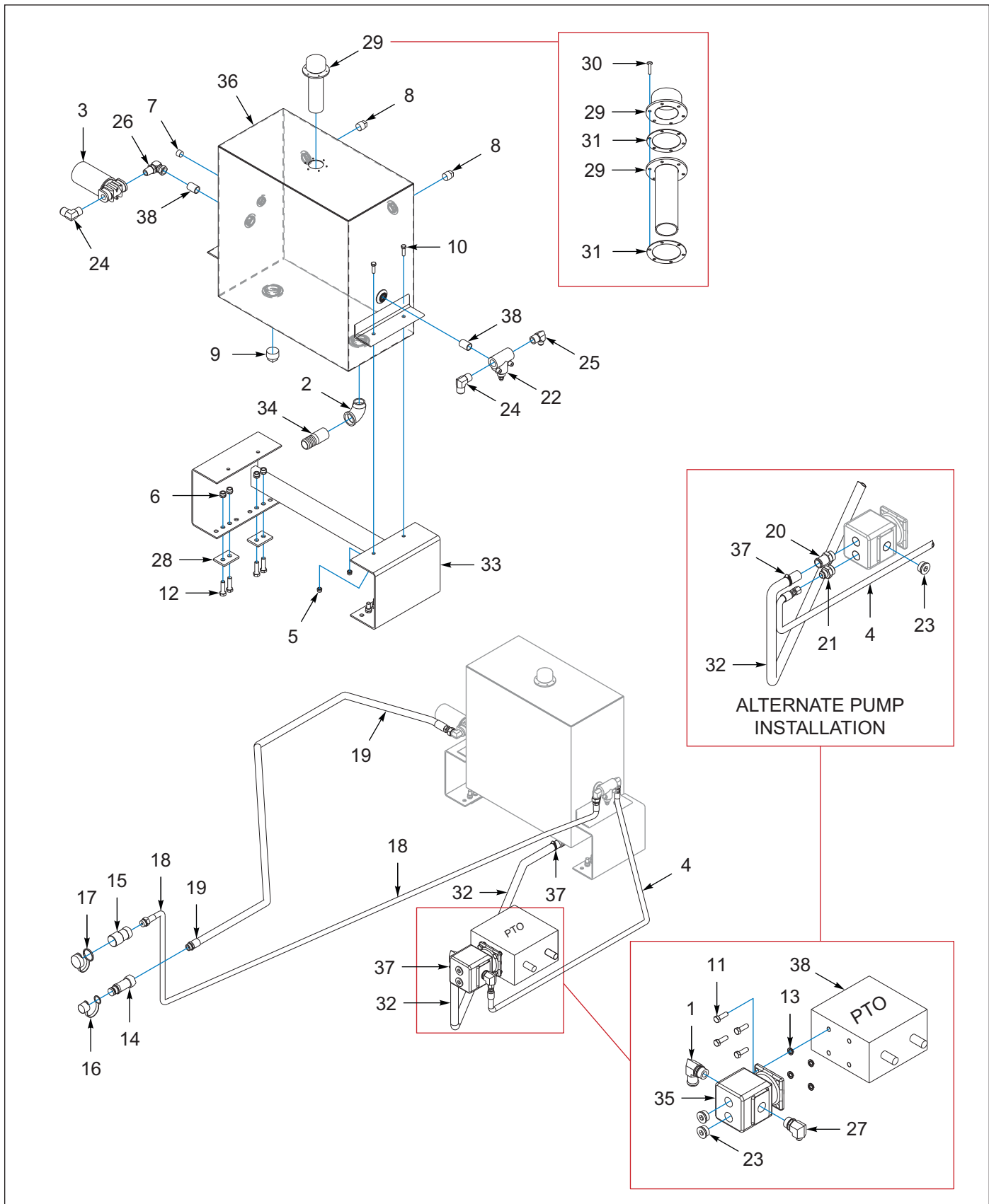
Figure 9-7: Wet Kit, Hydraulic (OPTION) (BEFORE 03/01/2019)
