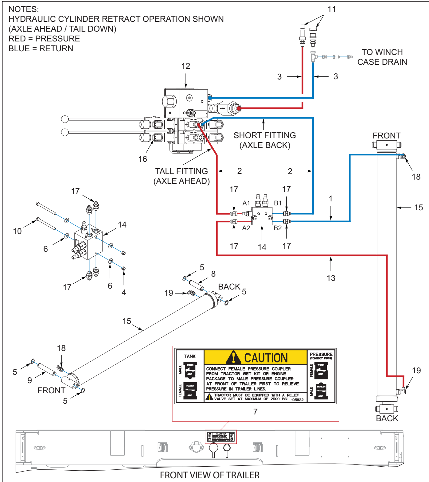
Figure 9-1: Frame Assembly, Axle / Tail Travel
