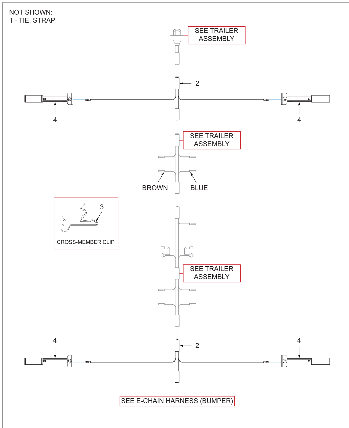
Figure 7-17: Swing Arm Light, Turn / Emergency, 4 In, Amber (OPTION) (1 of 2)
