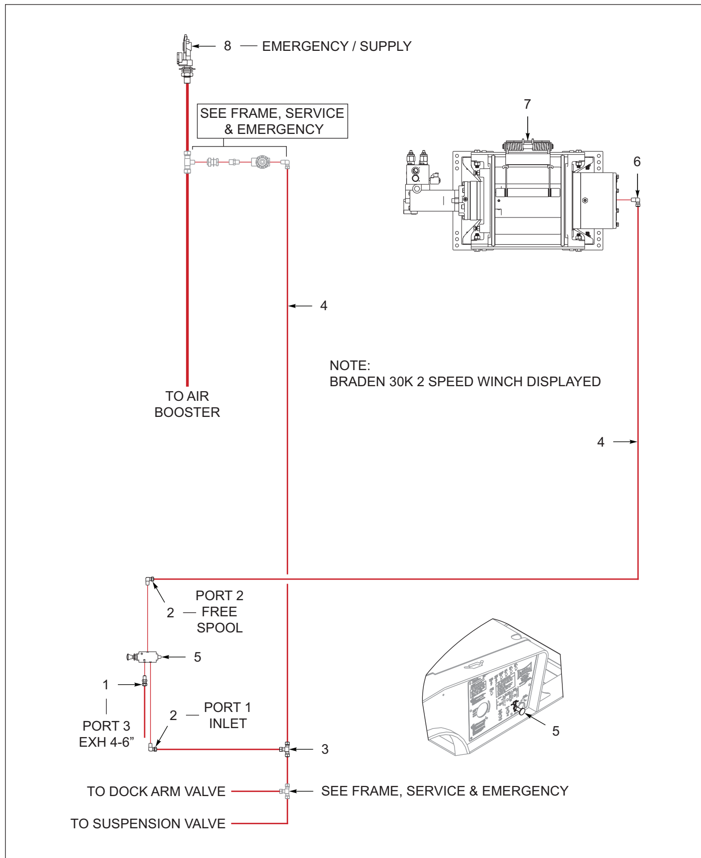
Figure 6-24: Winch Install, Ramsey 20K / 30K, 2 Speed (OPTION)
