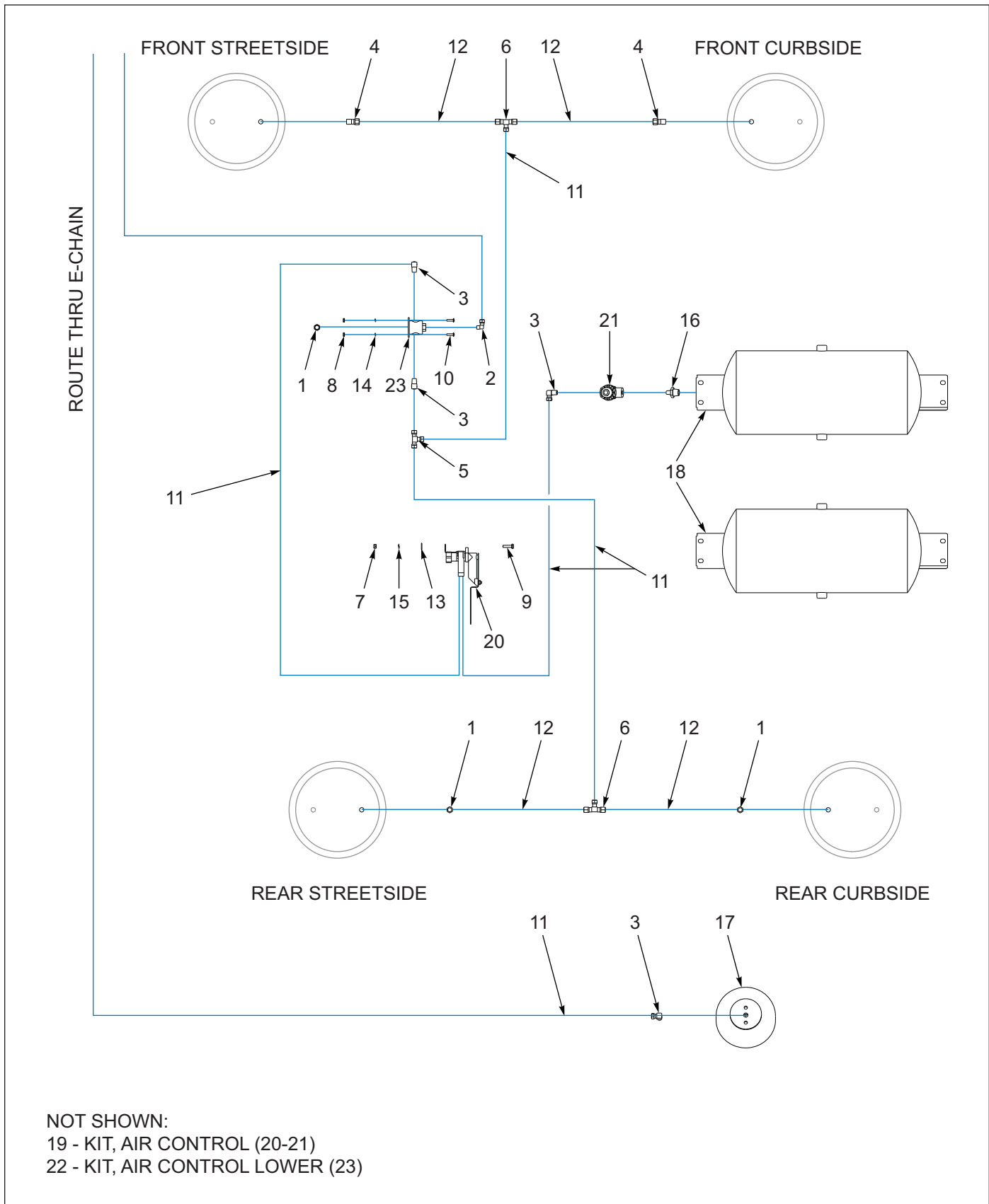
Figure 6-12: Suspension, Ride Height, 2 Axle
