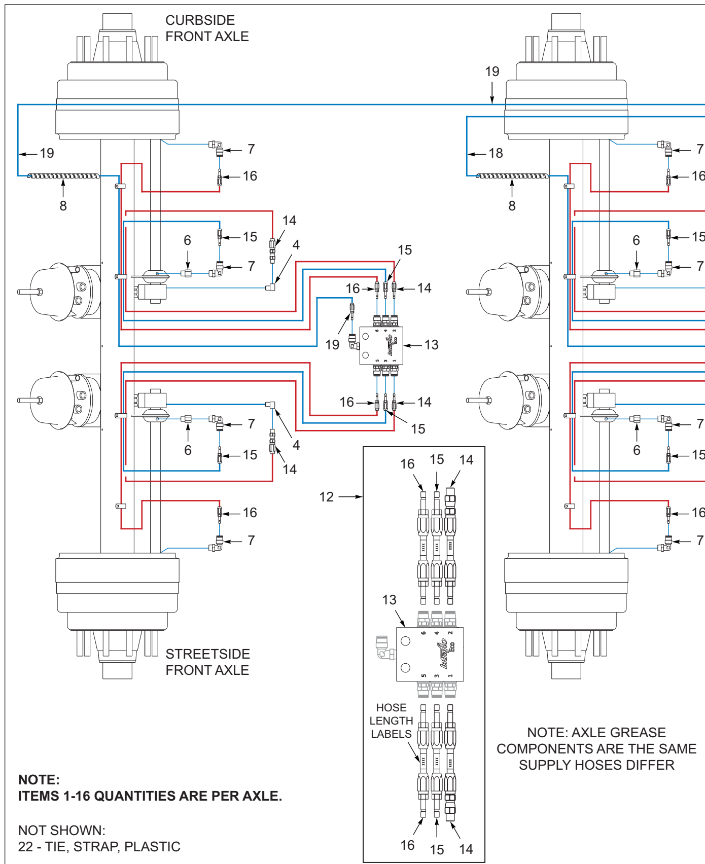
Figure 8-8: Drum Brakes, 3 Axle (After 08/31/2020) (1 of 3)
