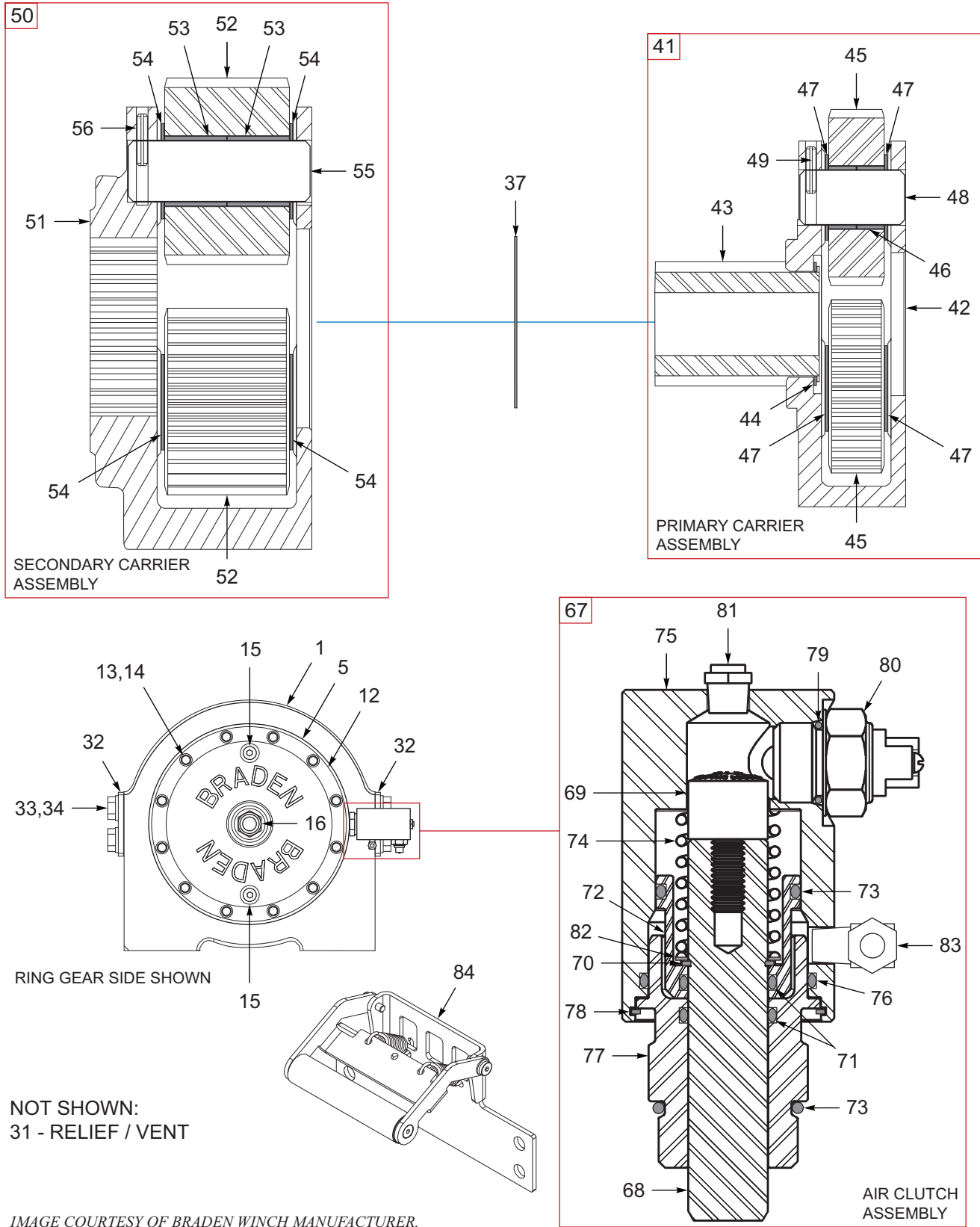
Figure 11-19: Winch Components, Braden 30K, 2 Speed (OPTION) (2 of 2)
