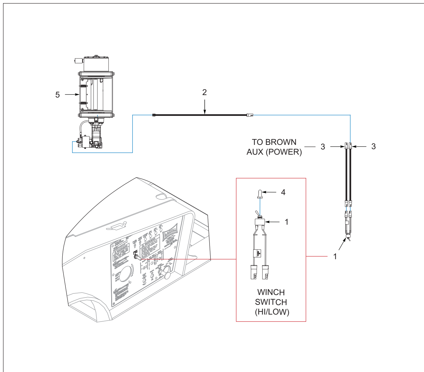
Figure 7-20: Winch Install, Braden 20K / 30K, 2 Speed (OPTION)
