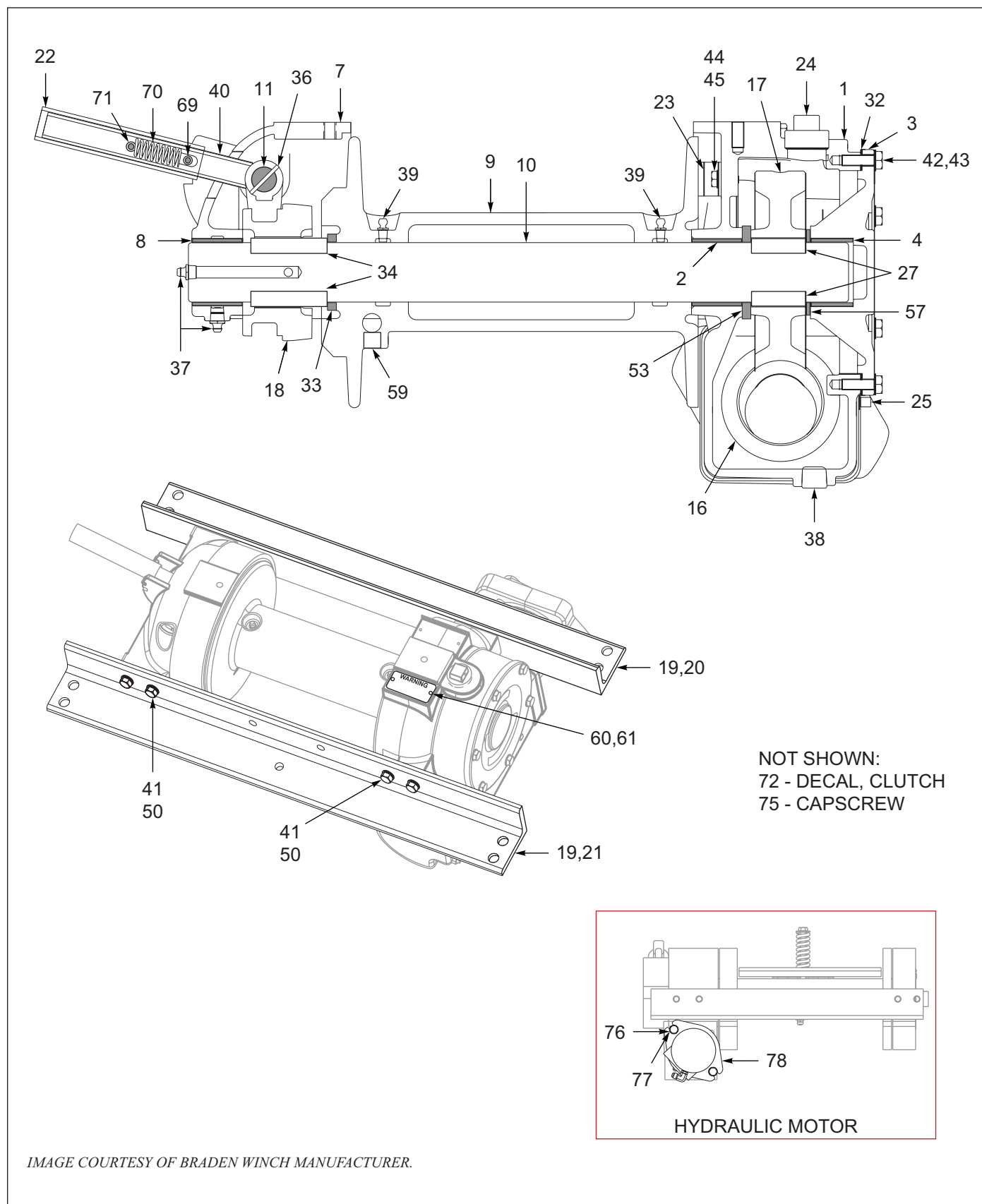
Figure 11-11: Winch Components, Braden 12K, 1 Speed (OPTION) (1 of 2)
