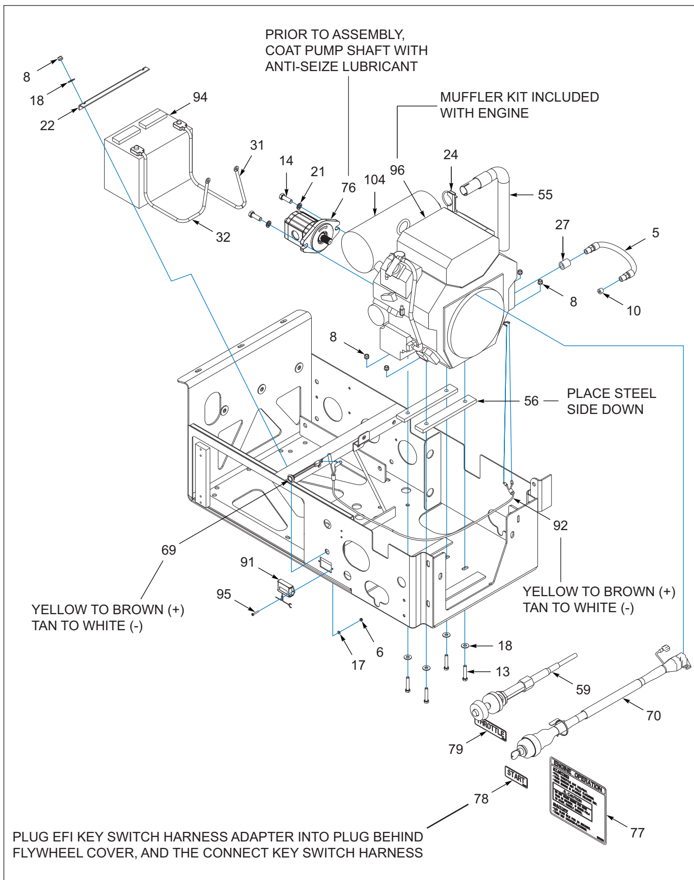
Figure 10-3: Engine, 25HP, Upper Deck Assembly (OPTION) (3 of 5)
