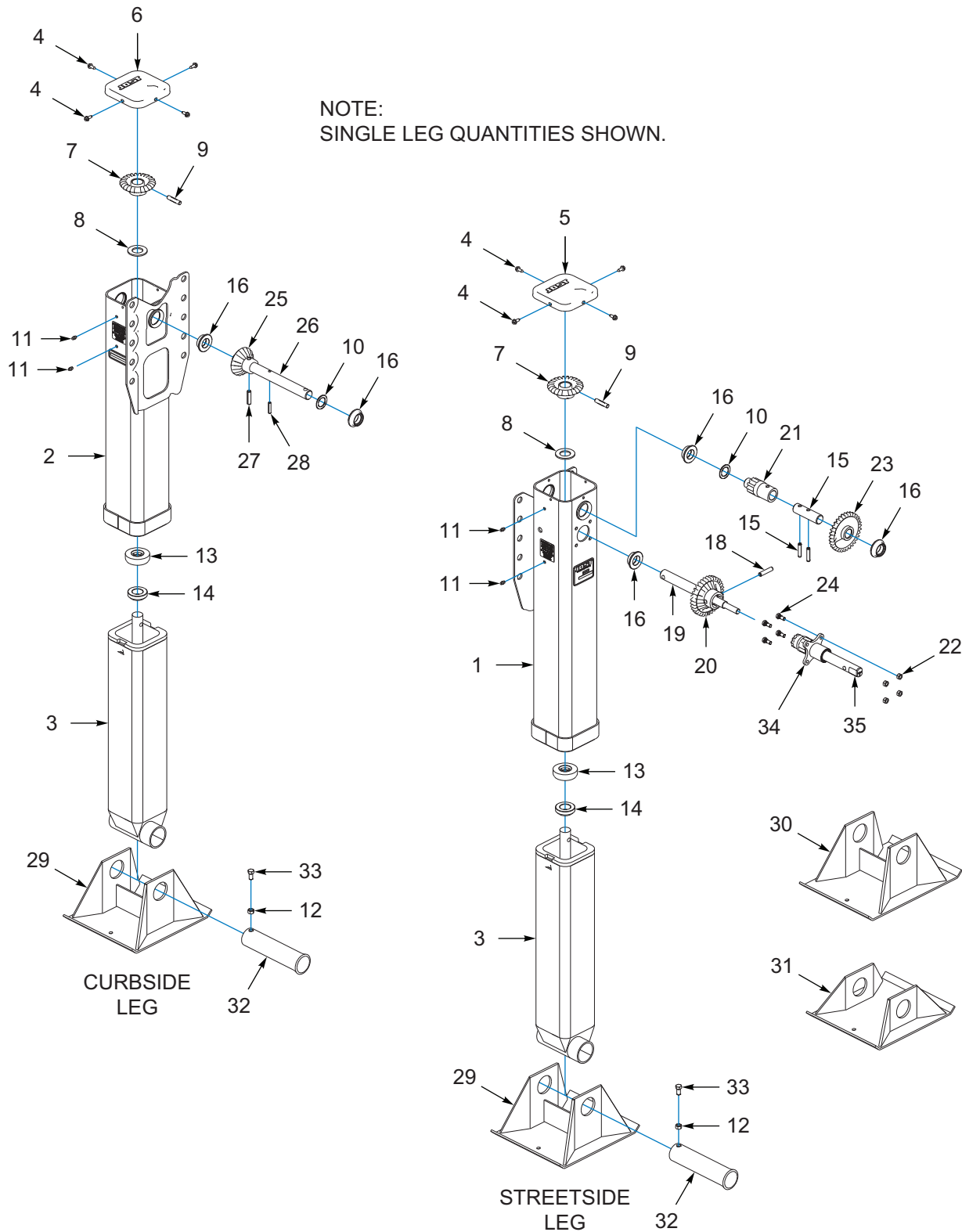
Figure 2-11: Landing Leg Components, Gear, 2 Spd
