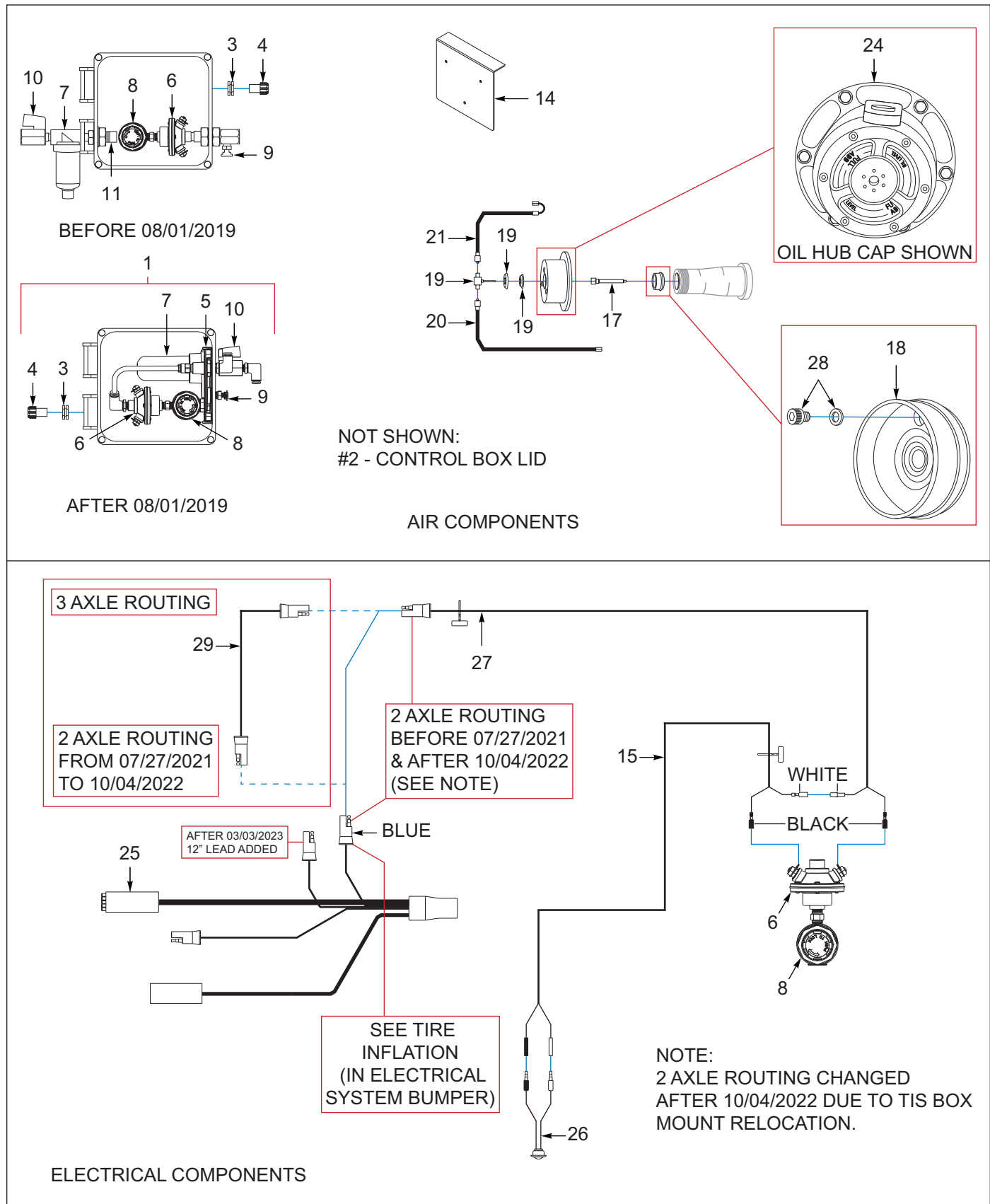
Figure 6-20: Tire Inflation Electrical System & Components (OPTION)
