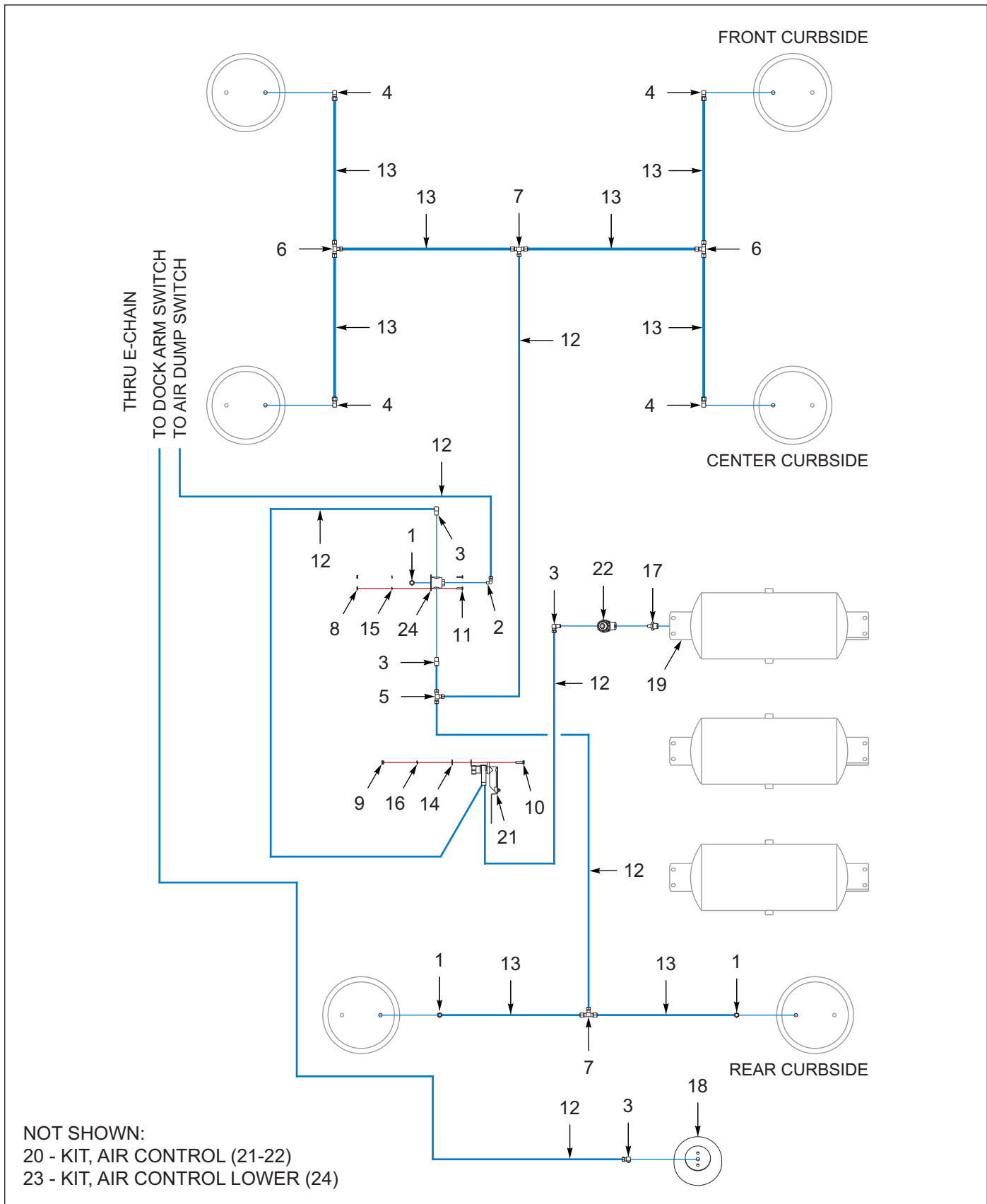
Figure 6-13: Suspension, Ride Height, 3 Axle
