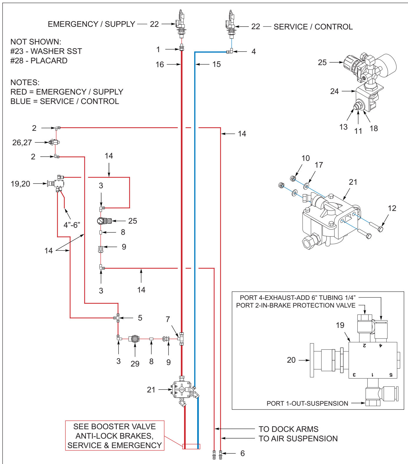
Figure 6-1: Frame, Service & Emergency
