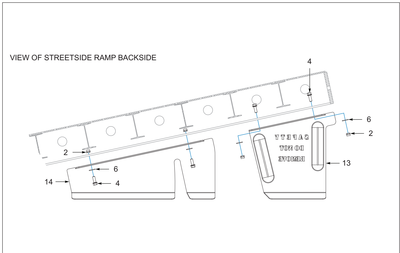
Figure 4-3: Front Slope, Deck Components (AFTER 03/11/2021) (OPTION) (2 of 2)
