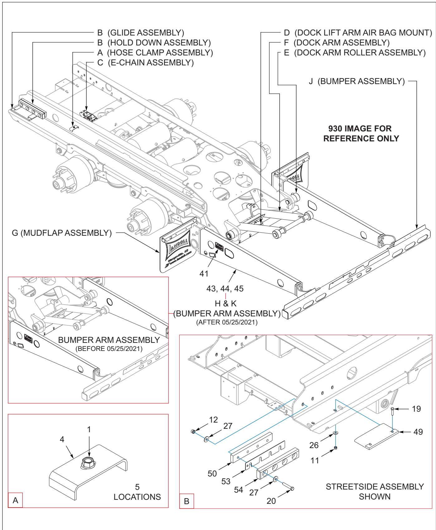
Figure 2-17: Undercarriage Components (1 of 3)
