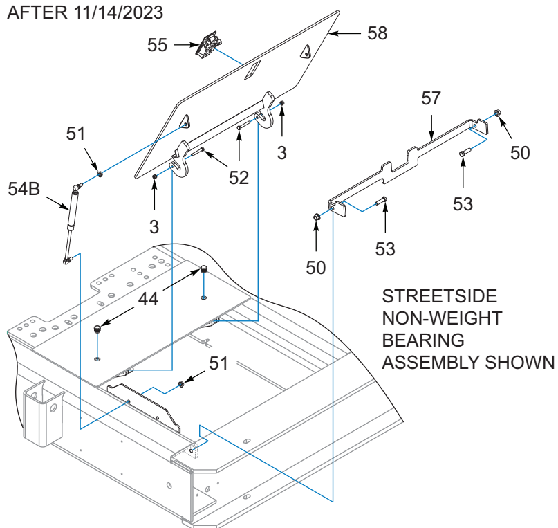
Figure 2-3: Frame Components (3 of 3)
