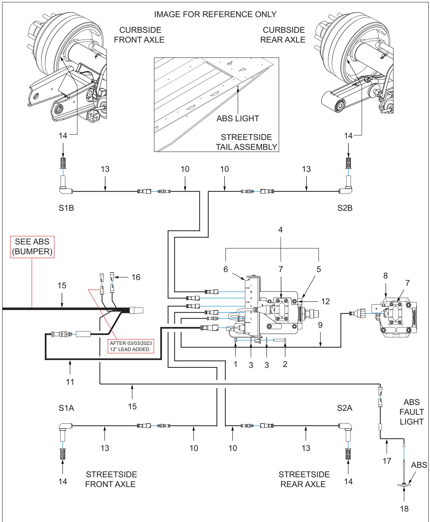
Figure 7-10: Anti-Lock Brakes, Haldex (1 of 2)
