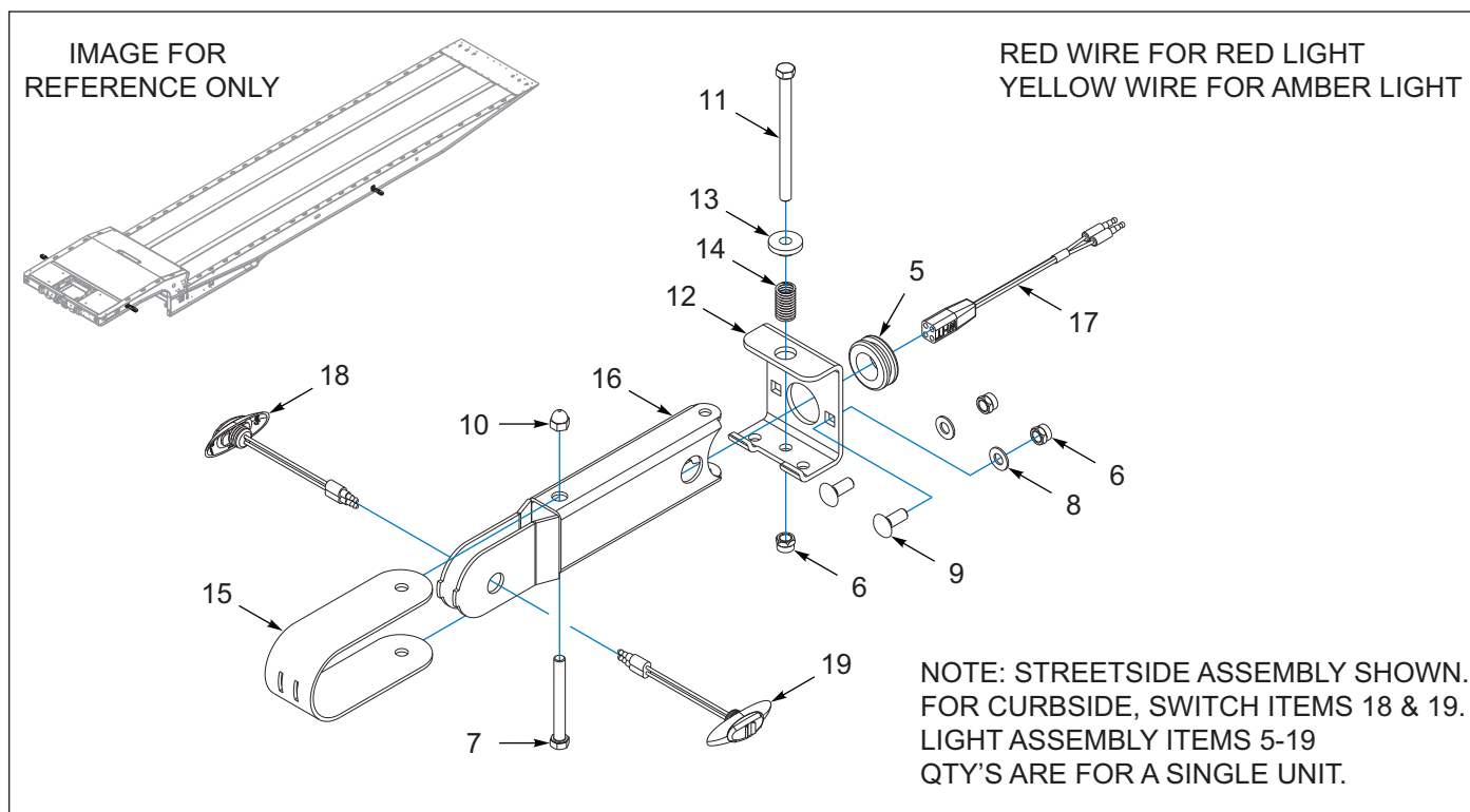
Figure 7-16: Swing Arm Light, Marker, Amber & Red (OPTION) (2 of 2)
