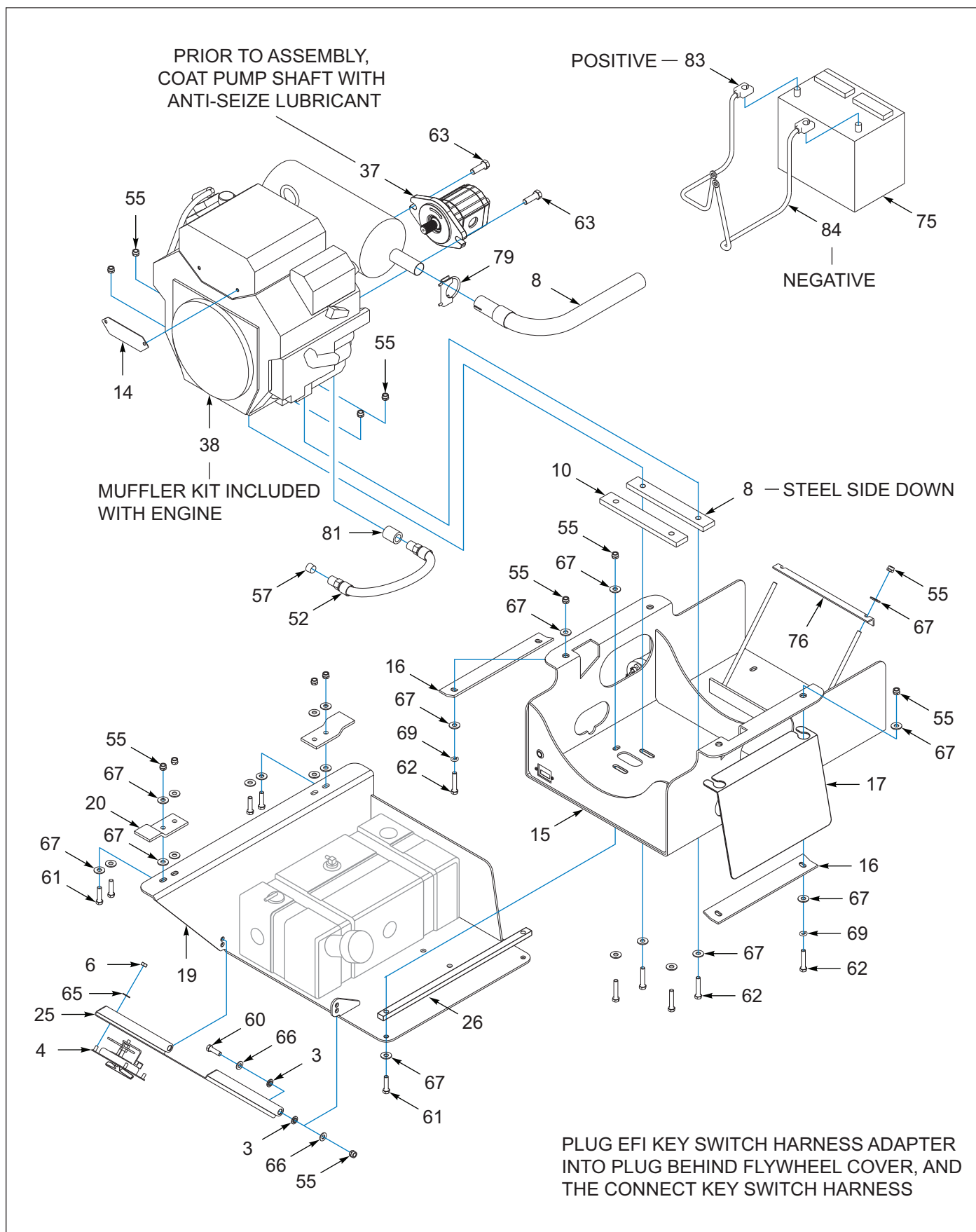
Figure 10-7: Engine, 25HP, Slope Deck Assembly (OPTION) (2 of 4)
