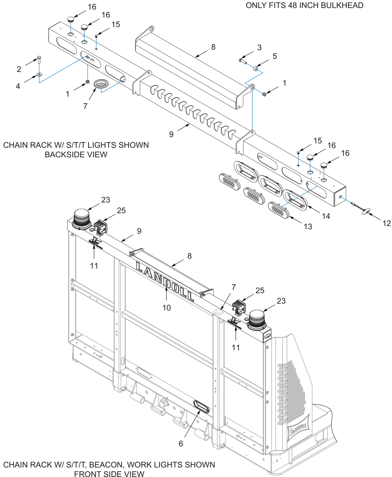
Figure 2-7: Bulkhead, Light Bar, Chain Rack (OPTIONS) (1 of 2)
