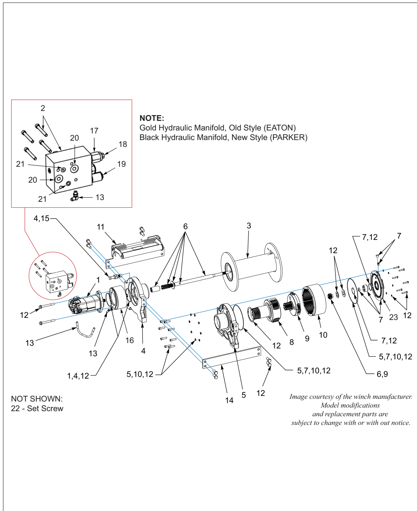
Figure 11-23: Winch Components, Warn 20K, 2 Speed (OPTION)
