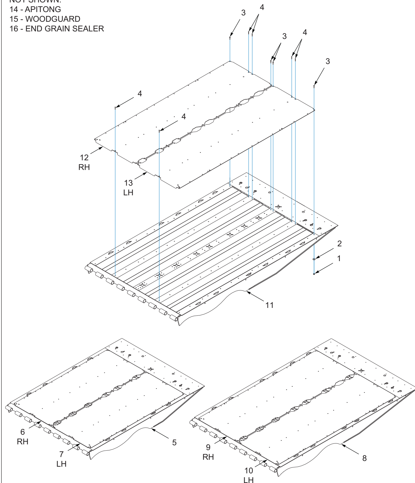
Figure 2-14: Tail Deck, Tread Grip, W/ Center Gotchas (OPTIONS)
