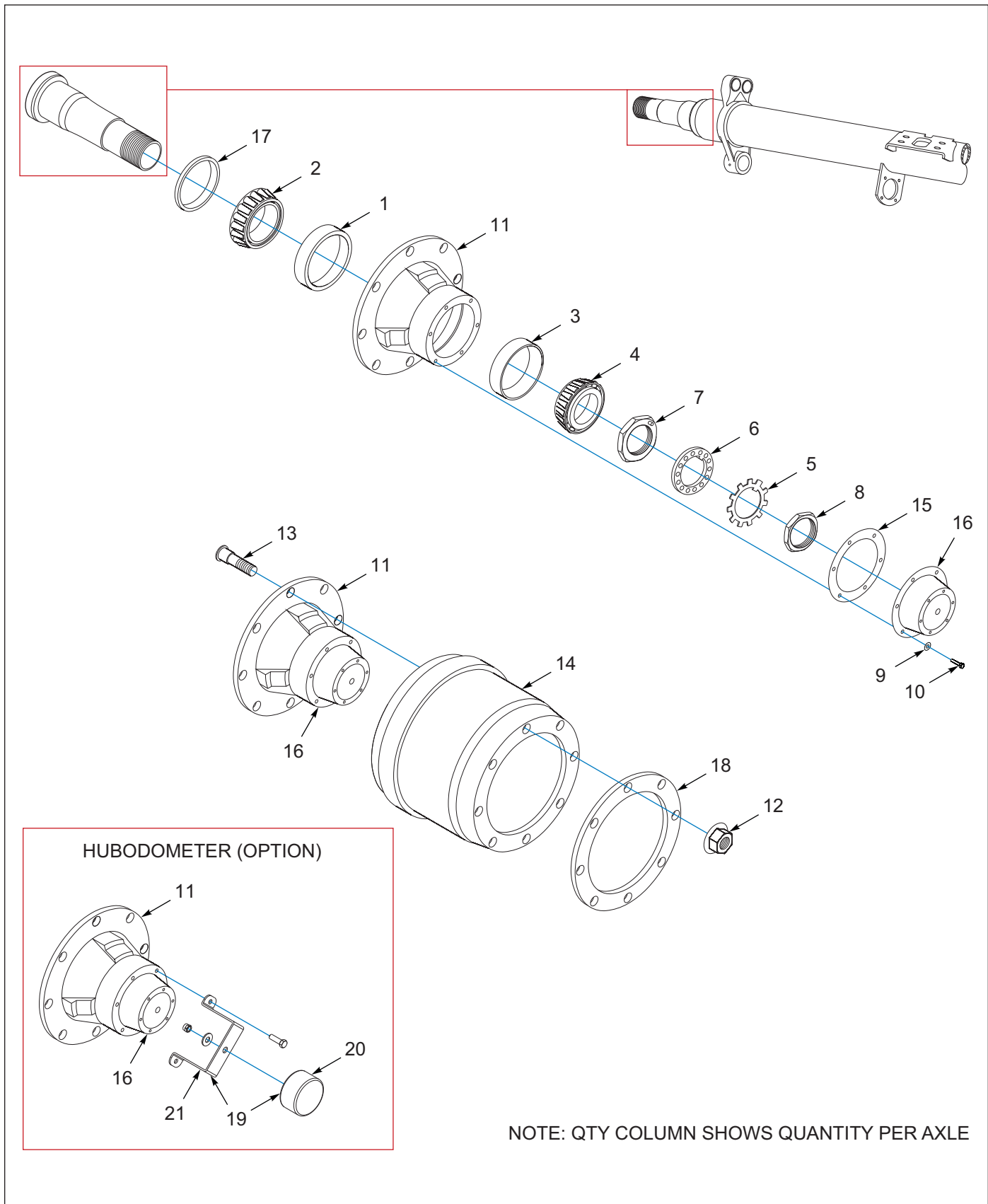
Figure 3-2: Axle 12.25 x 7.5 Drum & Hub Components
