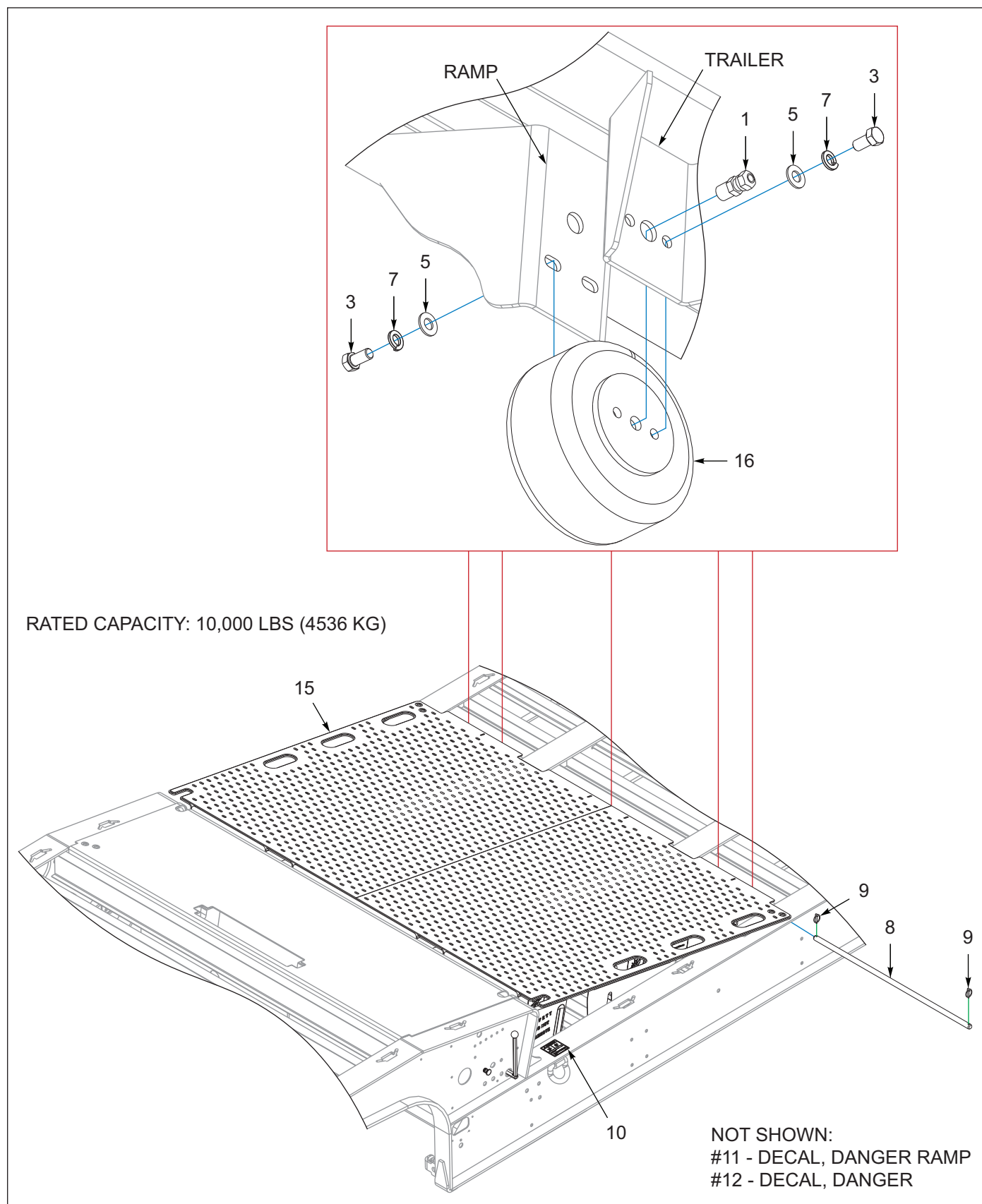
Figure 4-2: Front Slope, Deck Components (AFTER 03/11/2021) (OPTION) (1 of 2)
