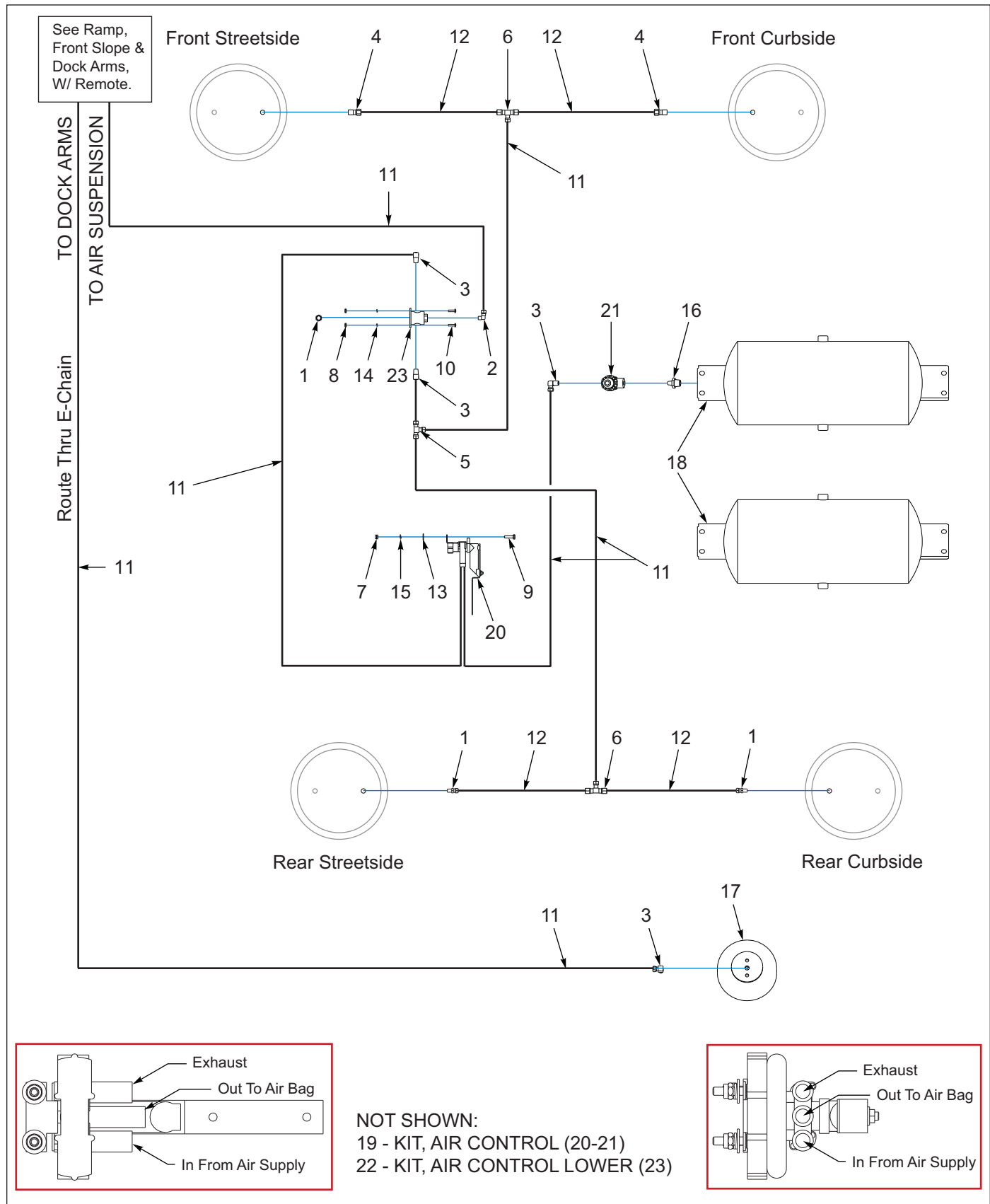
Figure 6-12: Suspension, Ride Height, 2 Axle, 1/4 in Valve, (BEFORE 06/12/2023)
