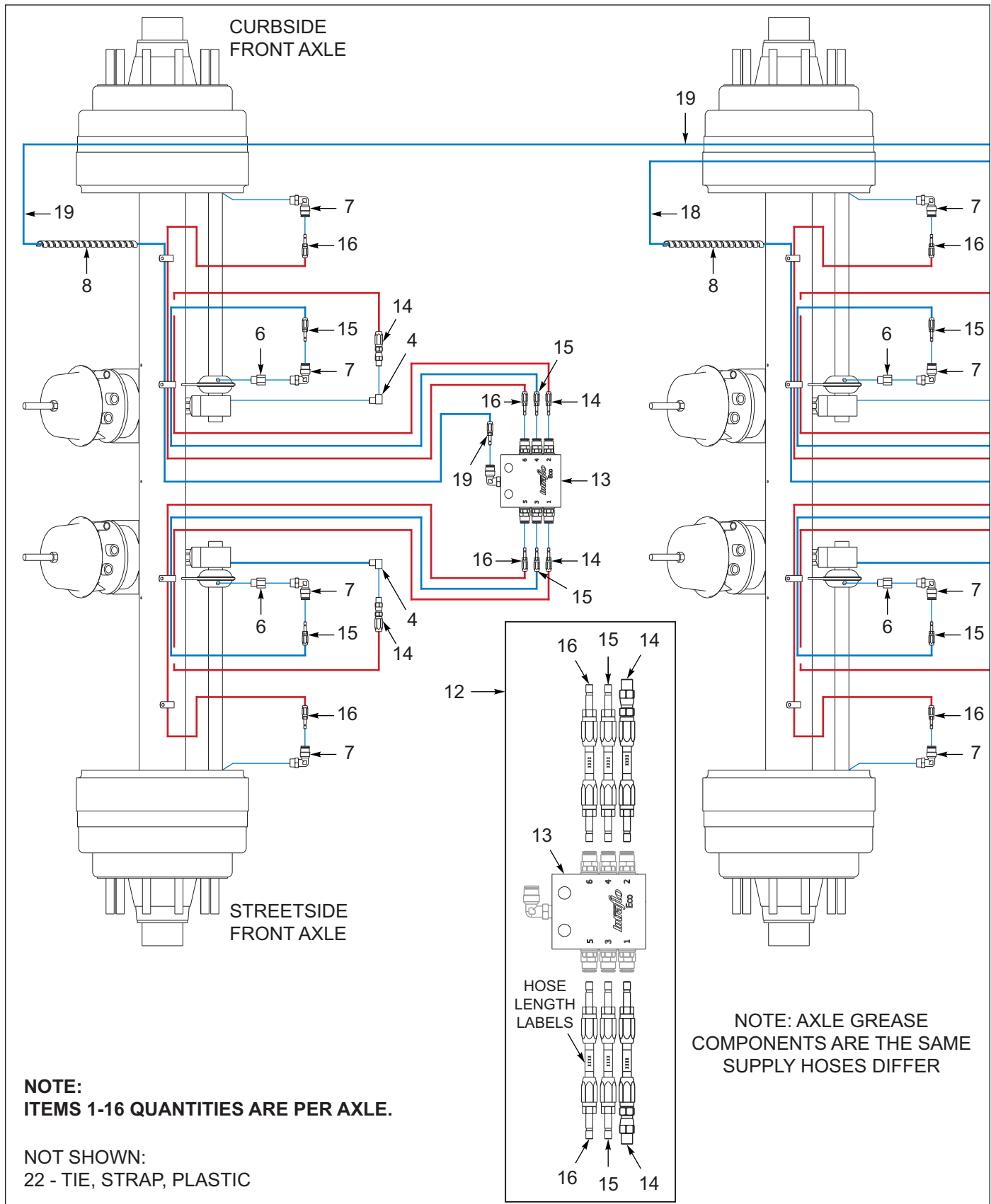
Figure 8-8: Drum Brakes, 3 Axle (After 08/31/2020) (1 of 3)
