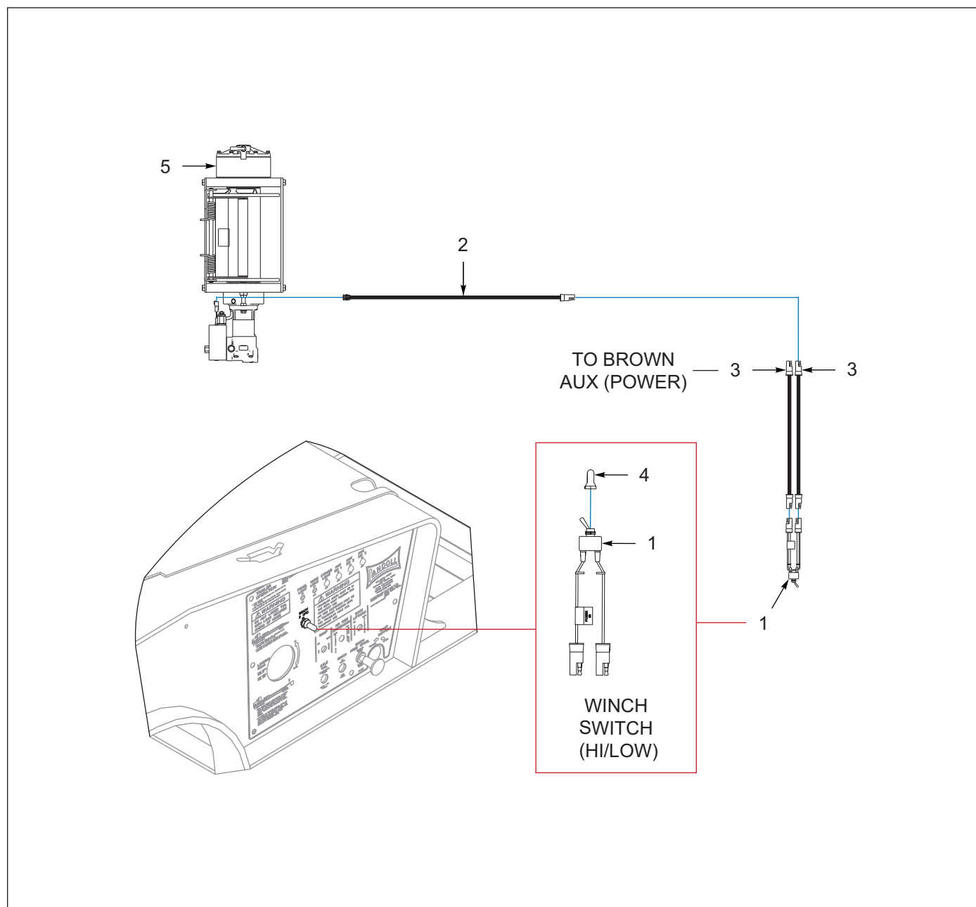
Figure 7-23: Winch Install, Warn 20K / 30K, 2 Speed, Spring Tension (OPTION)
