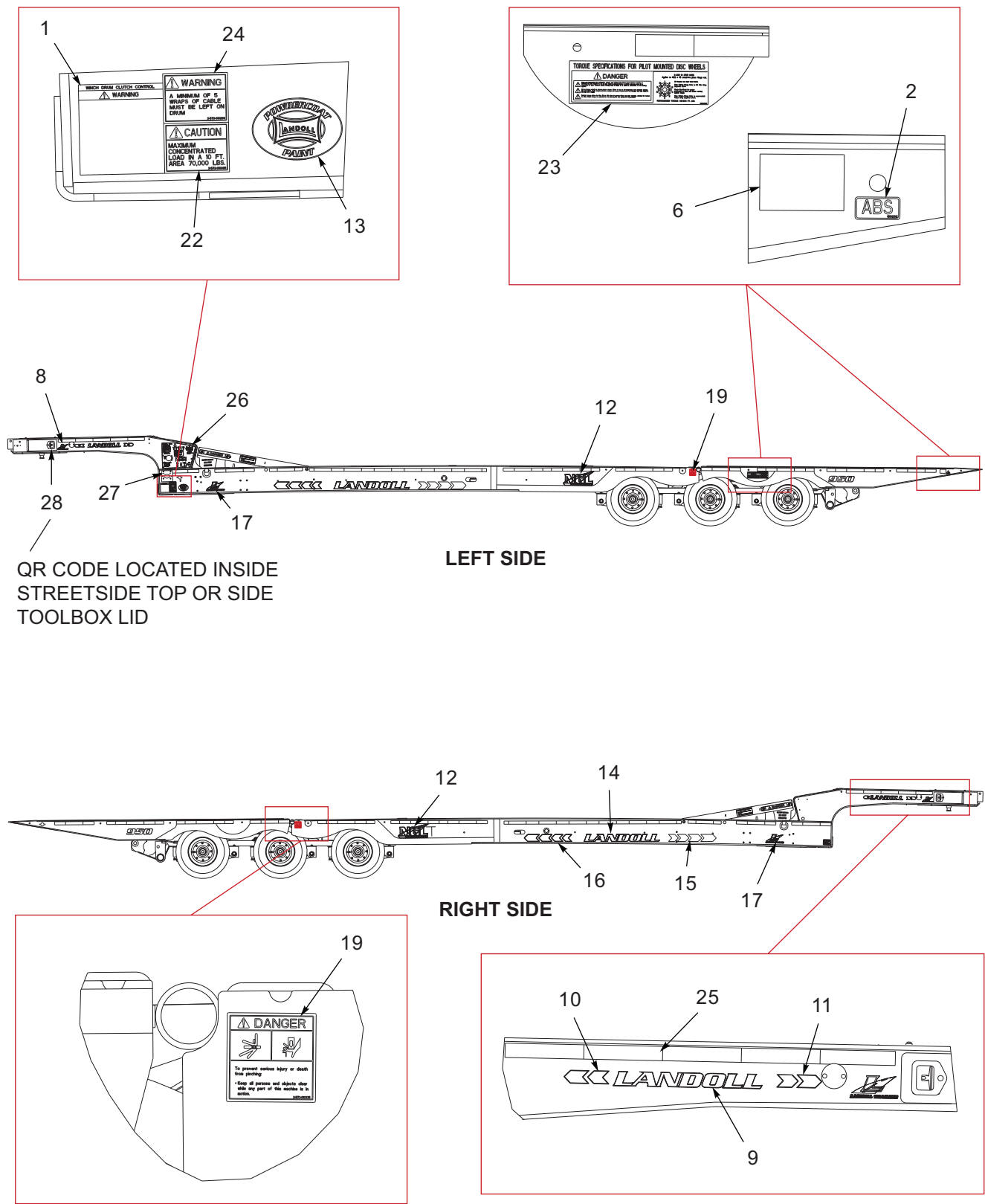
Figure 1-2: Frame Assembly (2 of 3)
