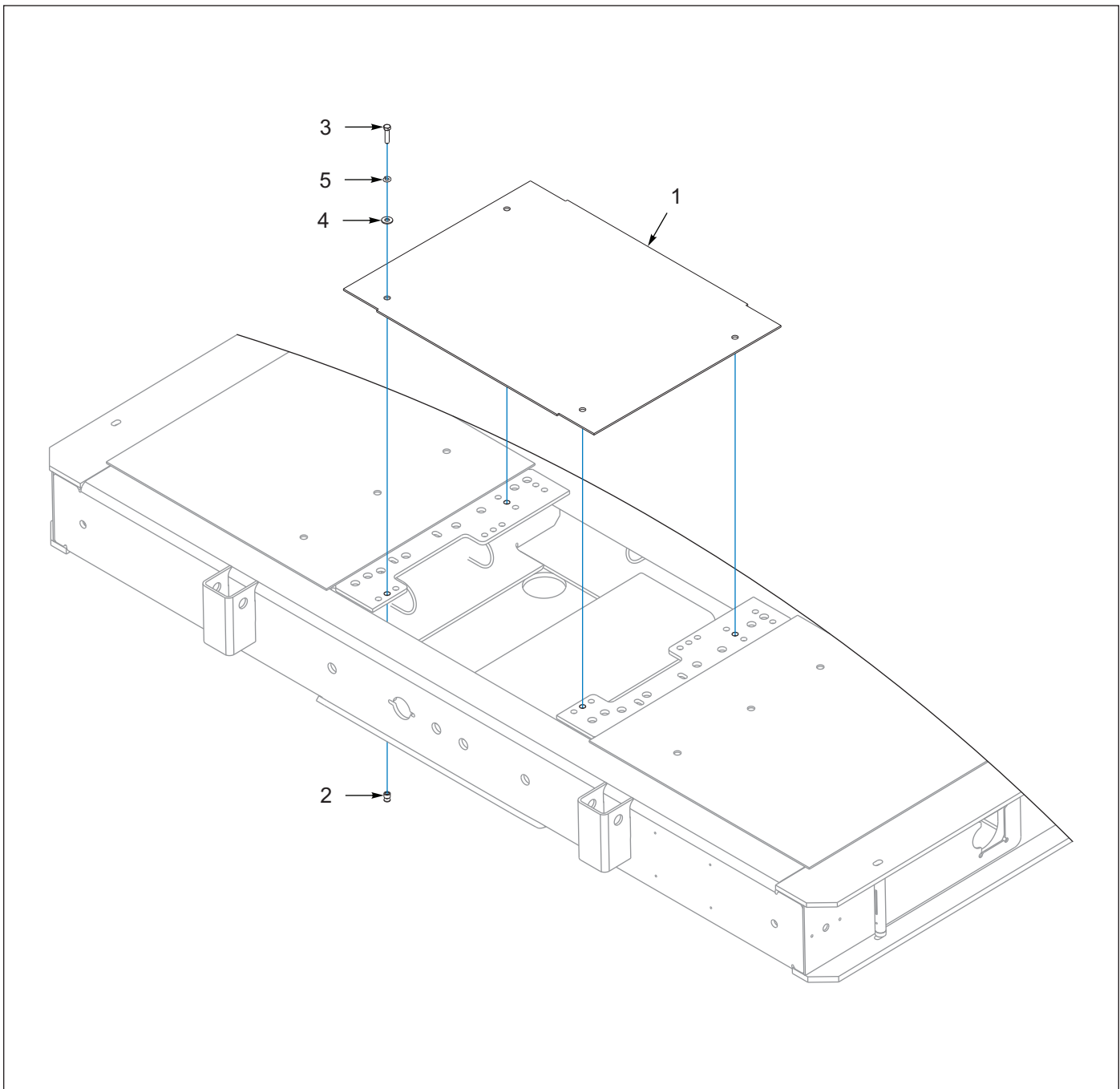
Figure 2-20: Upper Deck, Cover, Accessory (STANDARD WO/ WINCH)
