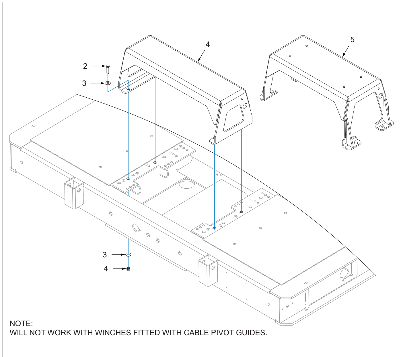
Figure 11-27: Guard, Winch WO/ Cable Pivot Guide (OPTIONS)
