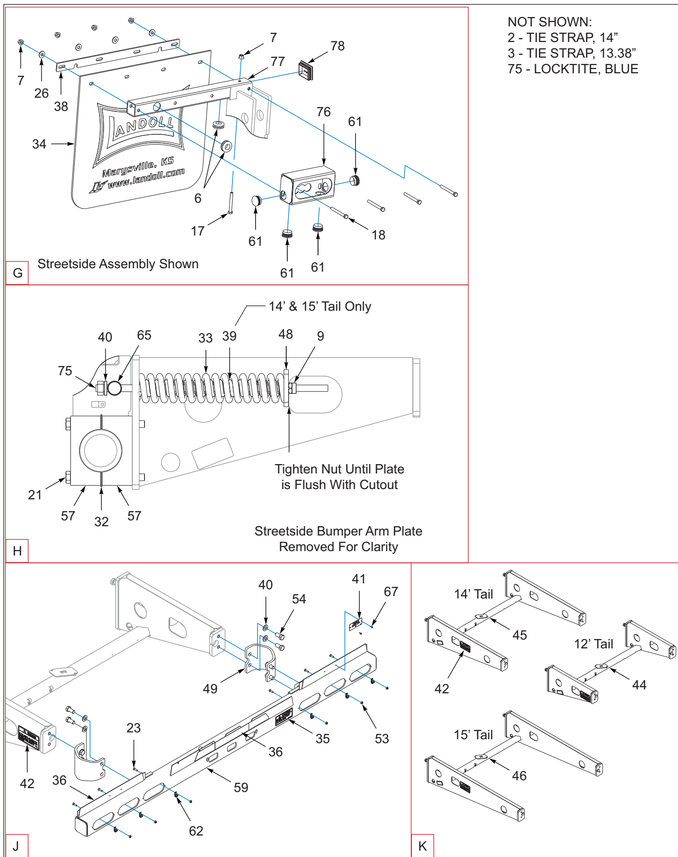
Figure 2-19: Undercarriage Components (3 of 3)
