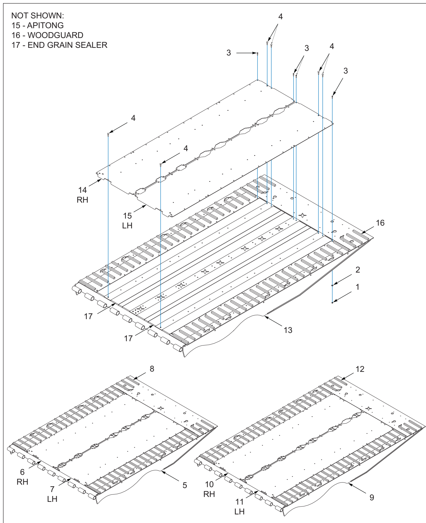
Figure 2-15: Tail Deck, Tread Grip, W/ Center Gotchas, Traction Bars (OPTIONS)
