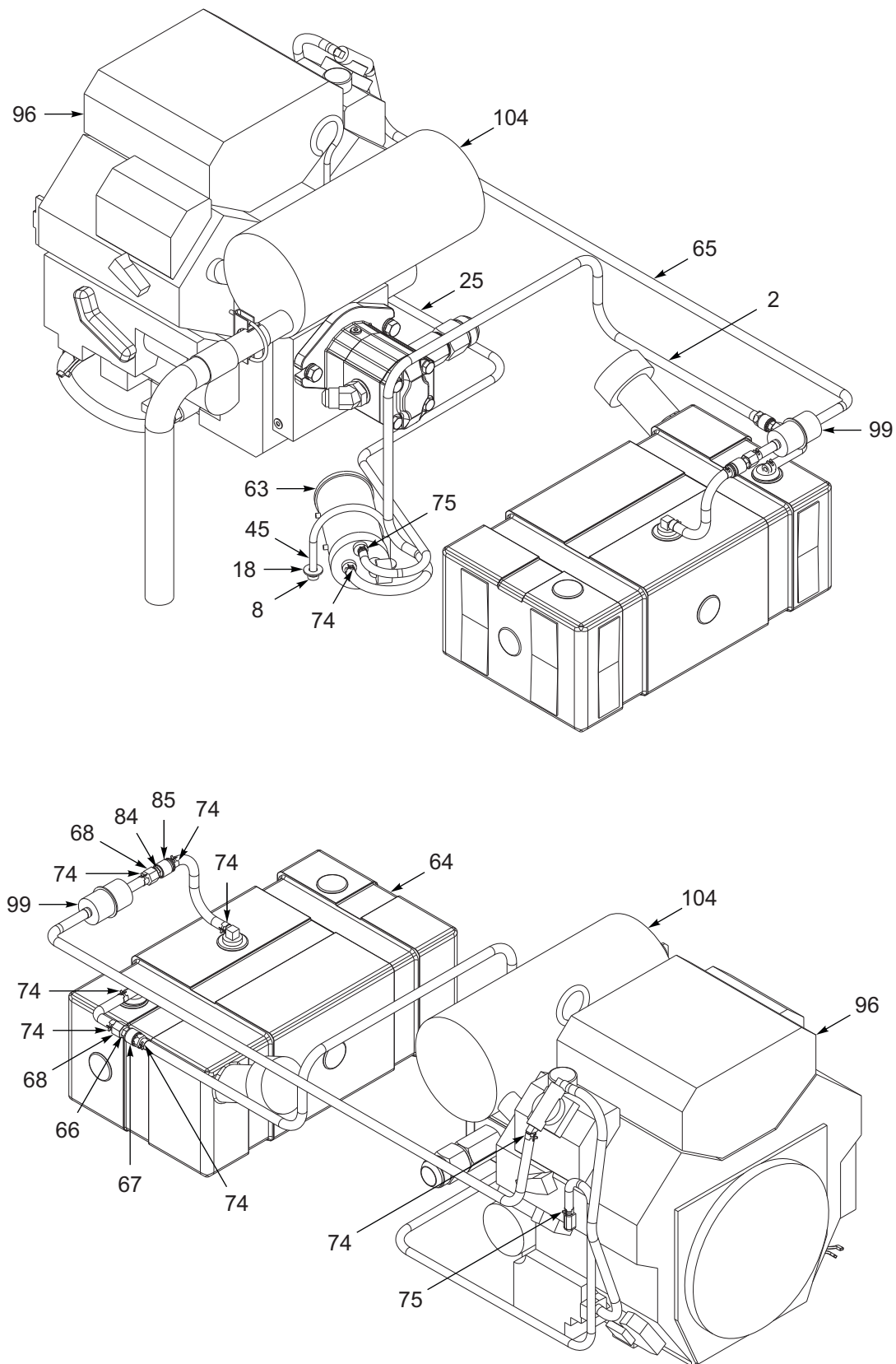
Figure 10-4: Engine, 25HP, Upper Deck Assembly (OPTION) (4 of 5)
