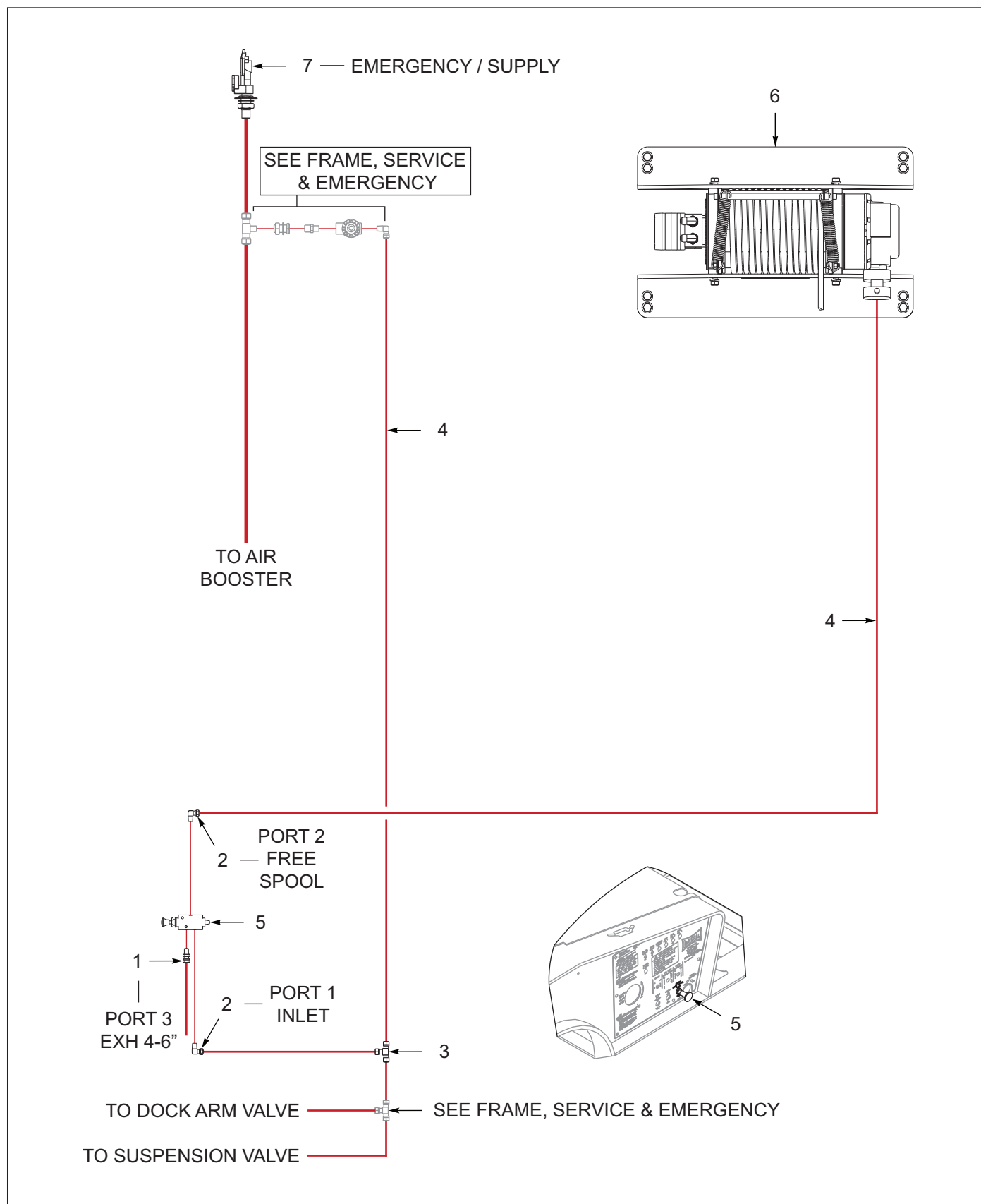
Figure 6-28: Winch Install, Warn 12K, 1 Speed, Spring Tension (OPTION)
