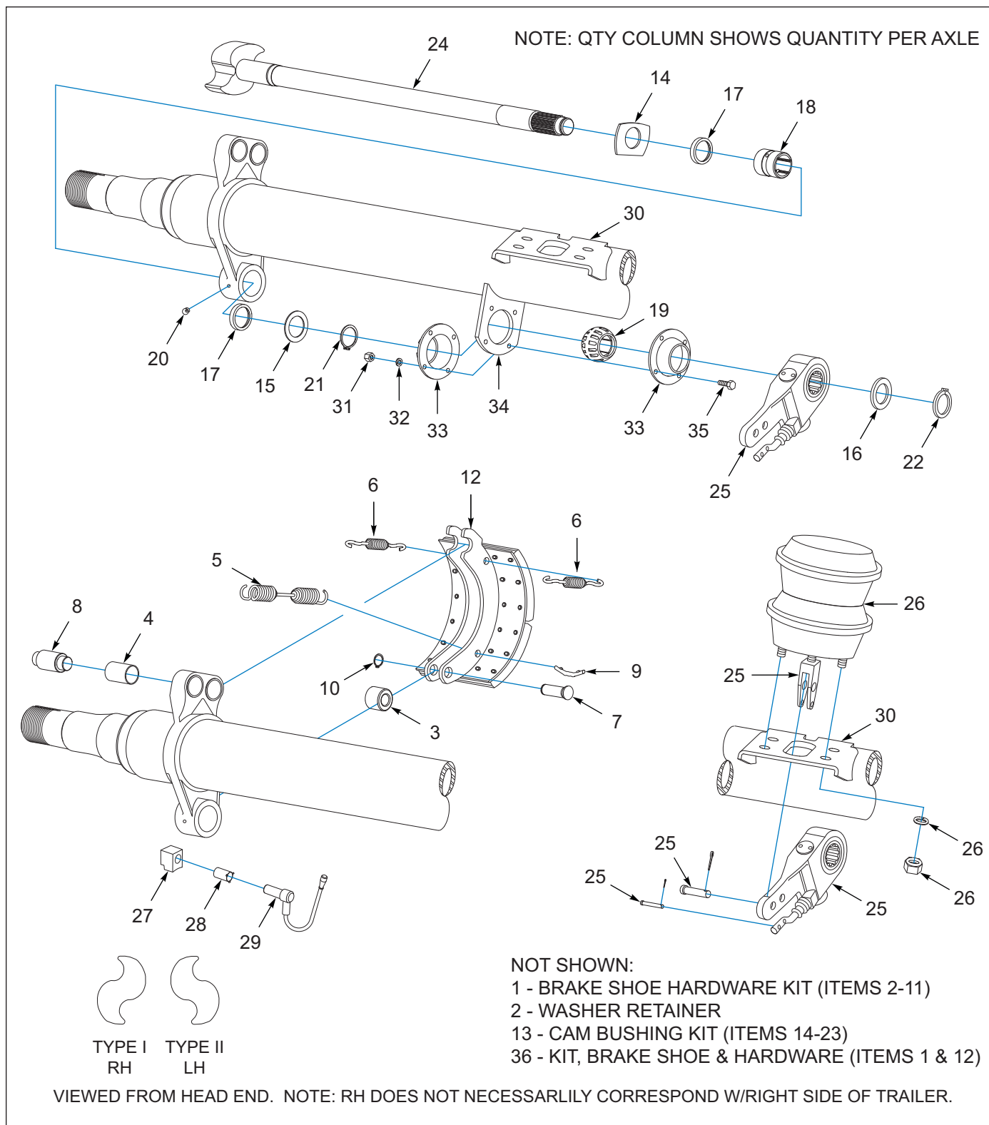
Figure 3-1: Axle 12.25 x 7.5 Drum Brake Components
