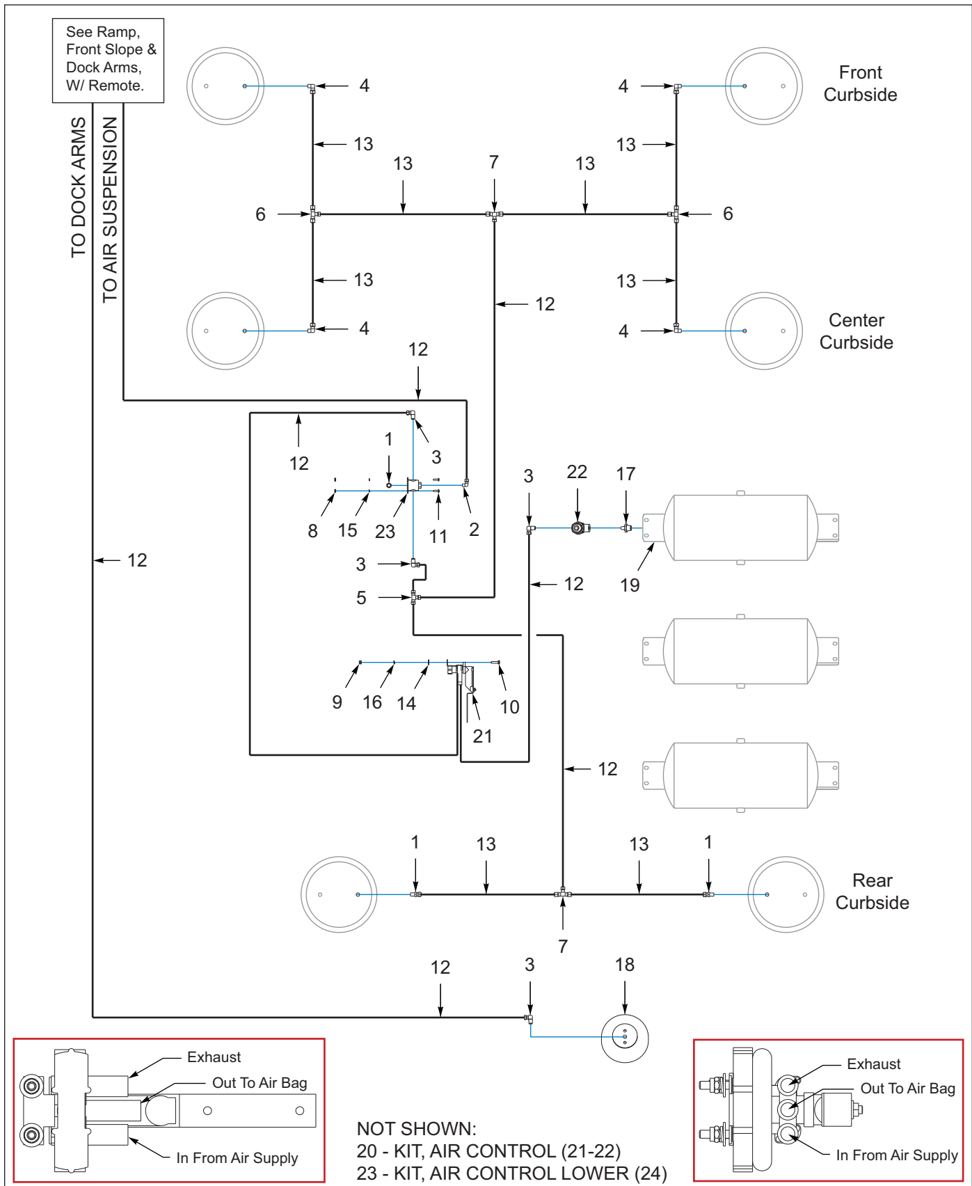
Figure 6-14: Suspension, Ride Height, 3 Axle, 1/4 in Valve, (BEFORE 06/12/2023)
