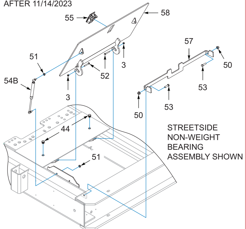
Figure 2-3: Frame Components (3 of 3)
