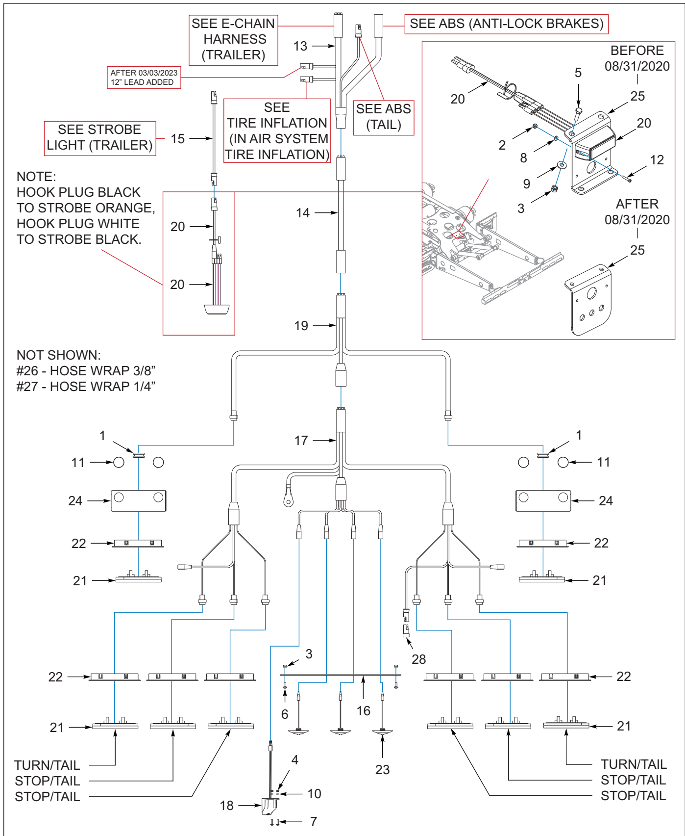
Figure 7-6: Bumper Assembly
