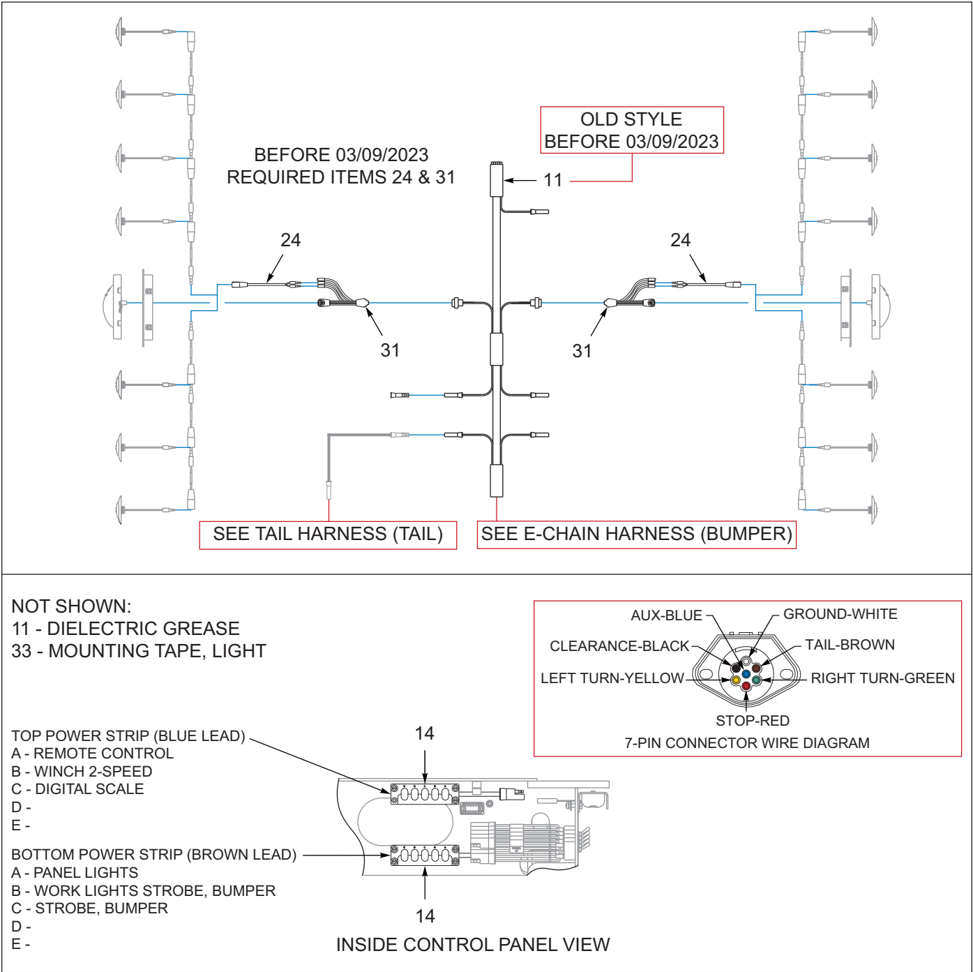
Figure 7-4: Trailer Assembly (AFTER 02/15/2022) (2 of 2)
