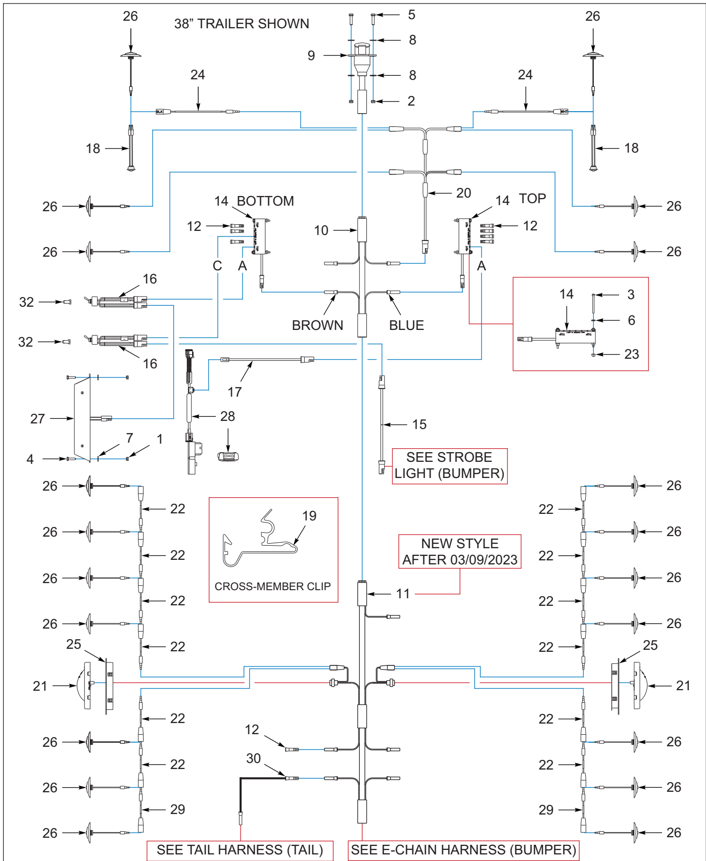
Figure 7-3: Trailer Assembly (AFTER 02/15/2022) (1 of 2)
