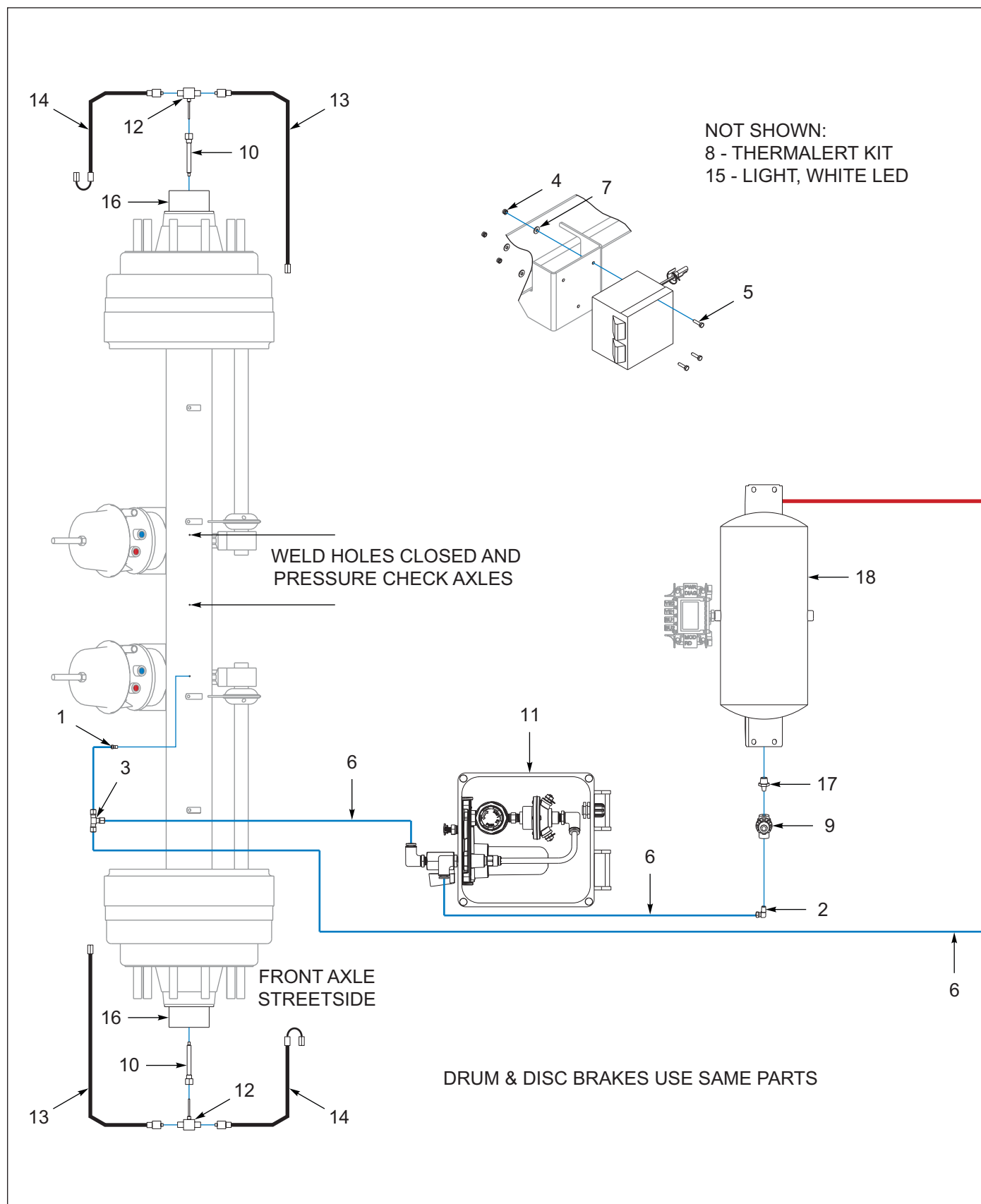
Figure 6-19: Tire Inflation, 2 Axle (OPTION) (1 of 2)
