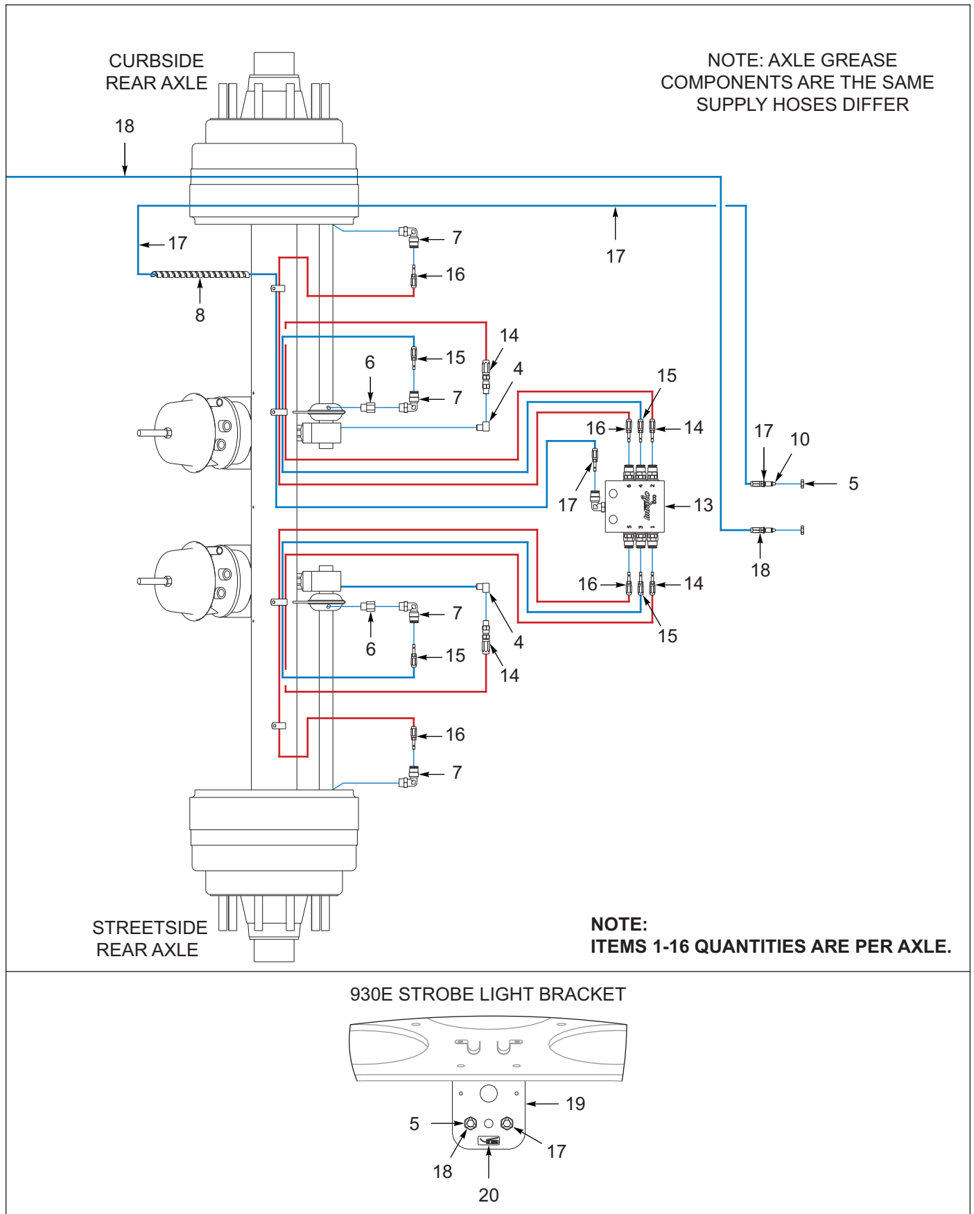
Figure 8-4: Drum Brakes, 2 Axle (After 08/31/2020) (2 of 3)
