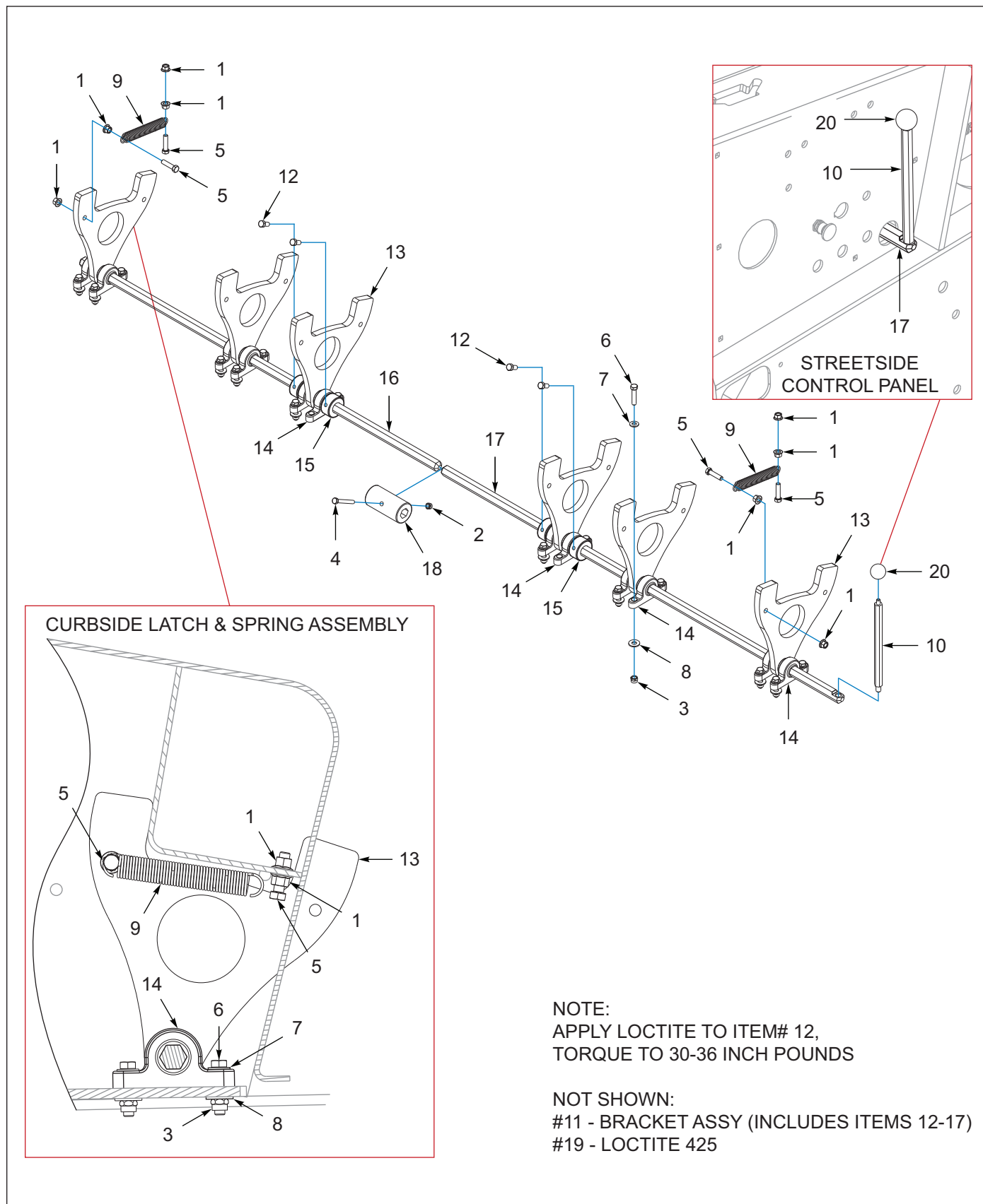
Figure 4-5: Front Slope, Support Components (AFTER 03/11/2021) (OPTION)
