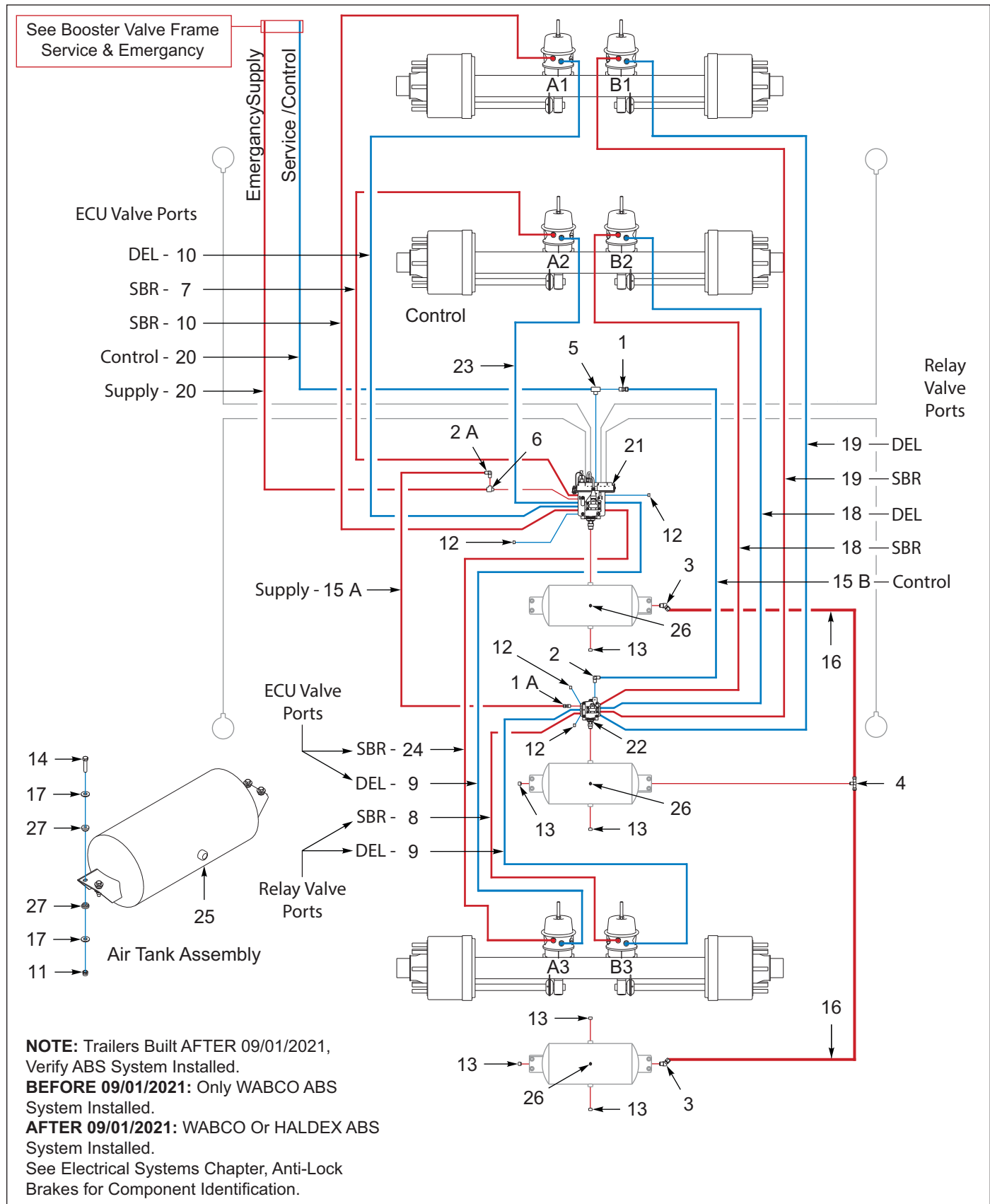
Figure 6-5: Anti-Lock Brakes, Service & Emergency, 3 Axle, Haldex
