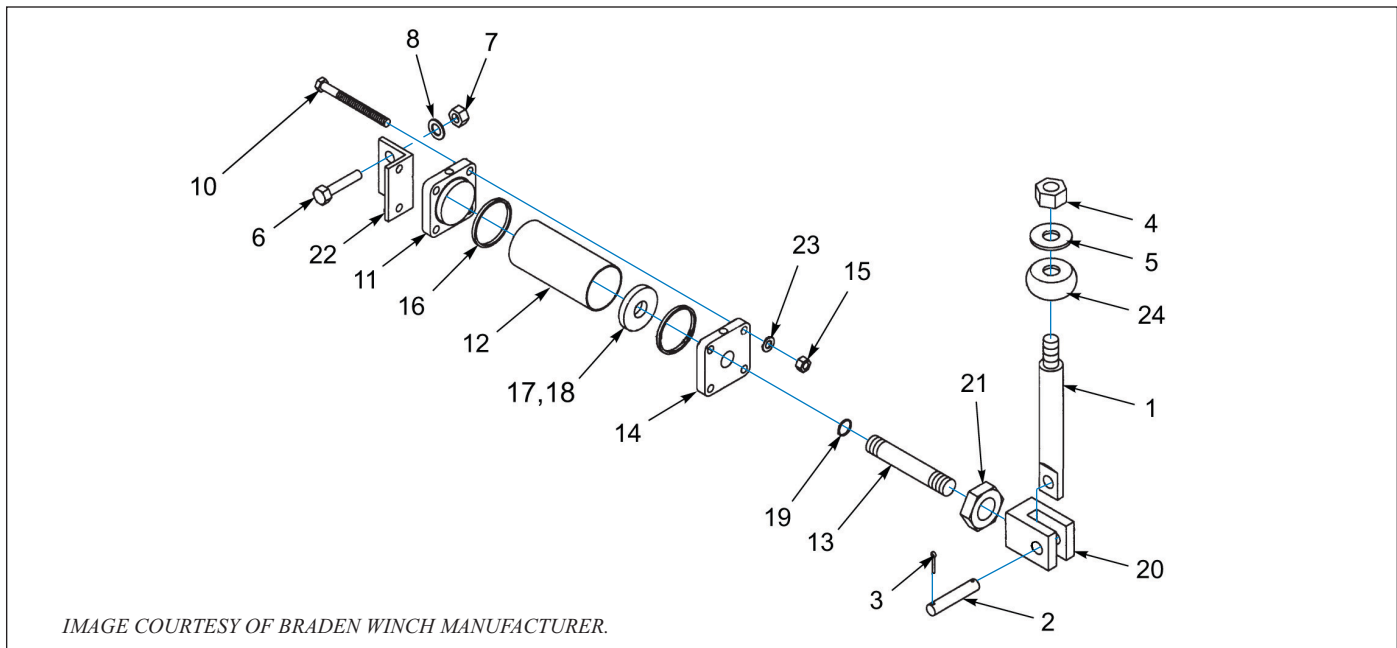
Figure 11-14: Winch Components, Braden 20K, 1 Spd, Free Spool Air Cyl (OPTION)
