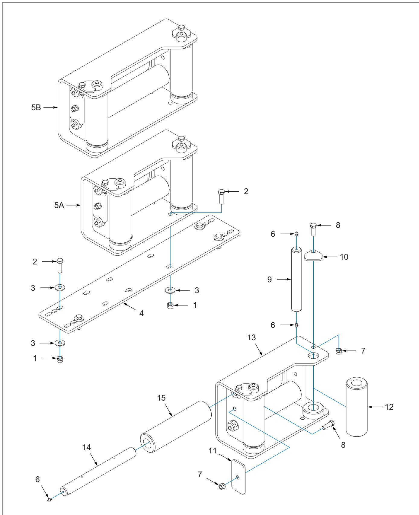
Figure 11-25: Cable Guide, 4-Roller, Braden 12K / 20K (OPTIONS)
