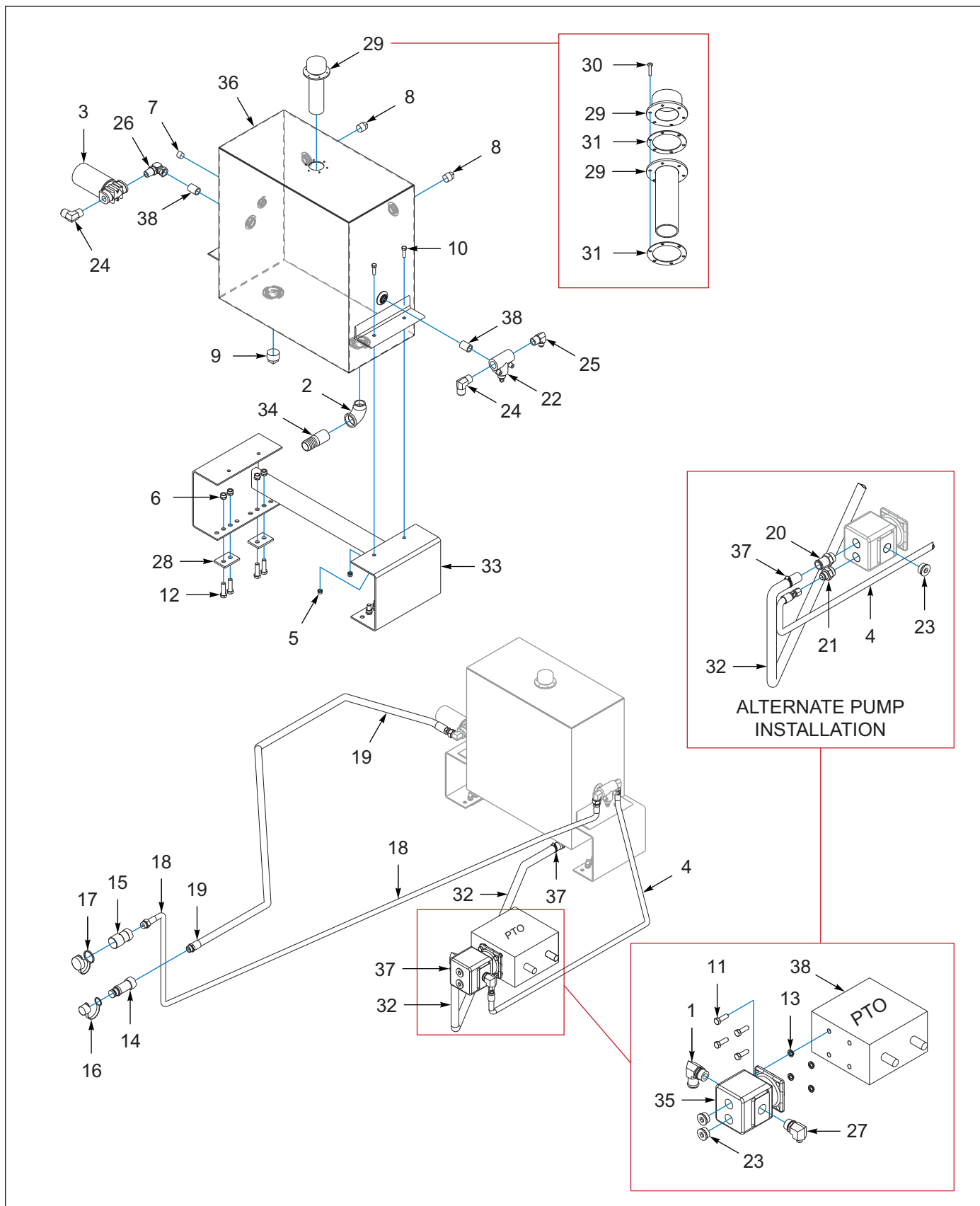
Figure 9-7: Wet Kit, Hydraulic (OPTION) (BEFORE 03/01/2019)
