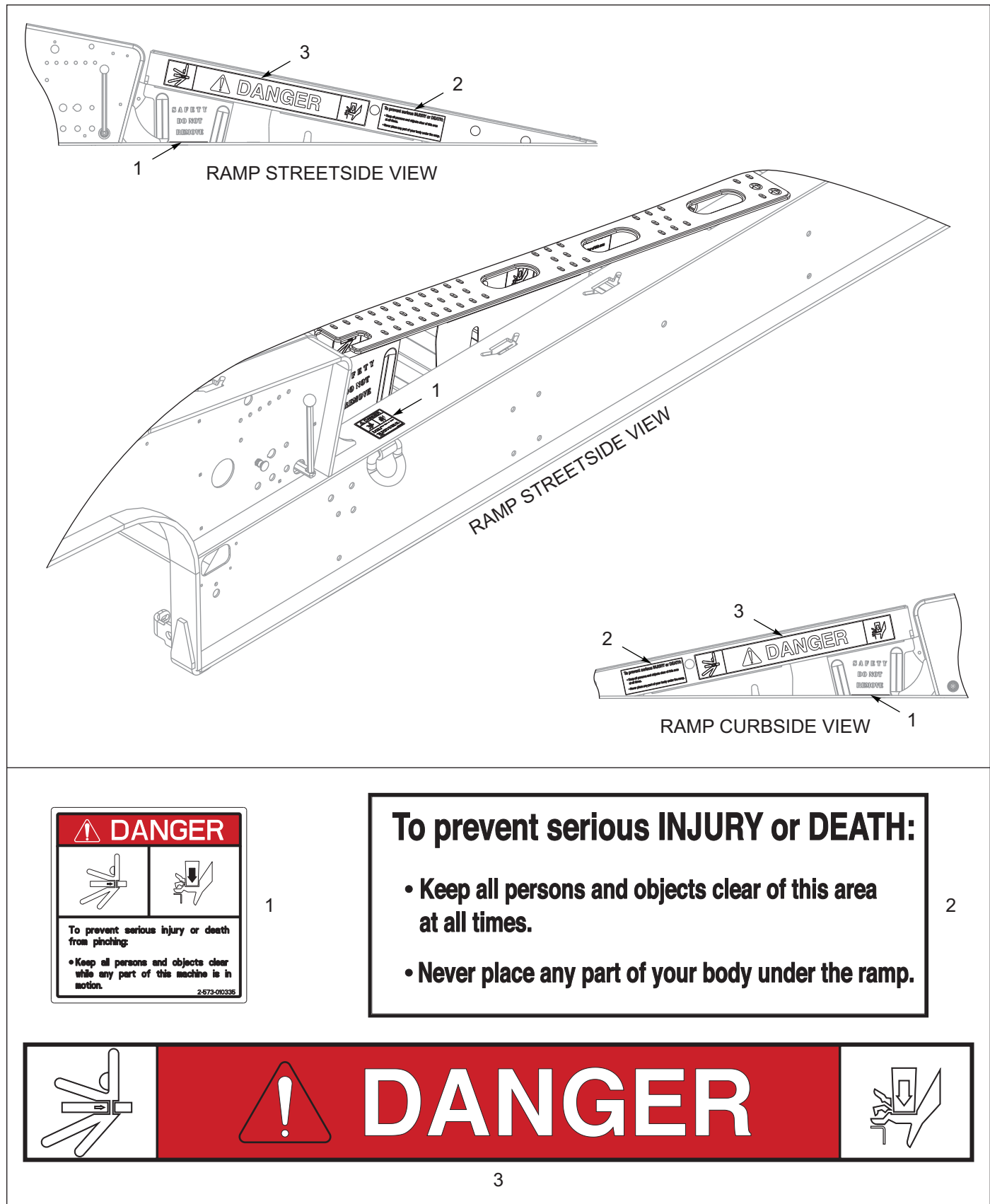
Figure 1-4: Ramp Assembly, Air 6 Feet
