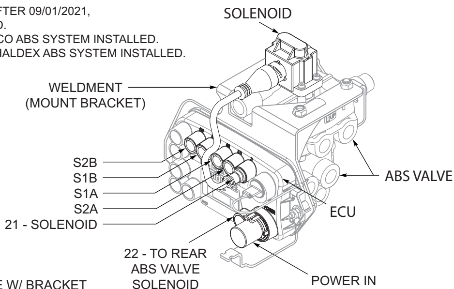
Figure 7-12: Anti-Lock Brakes, Haldex (2 of 2)
