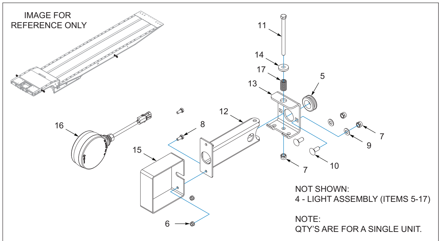
Figure 7-19: Swing Arm Light, Turn / Emergency, 4 In, Amber (OPTION) (2 of 2)
