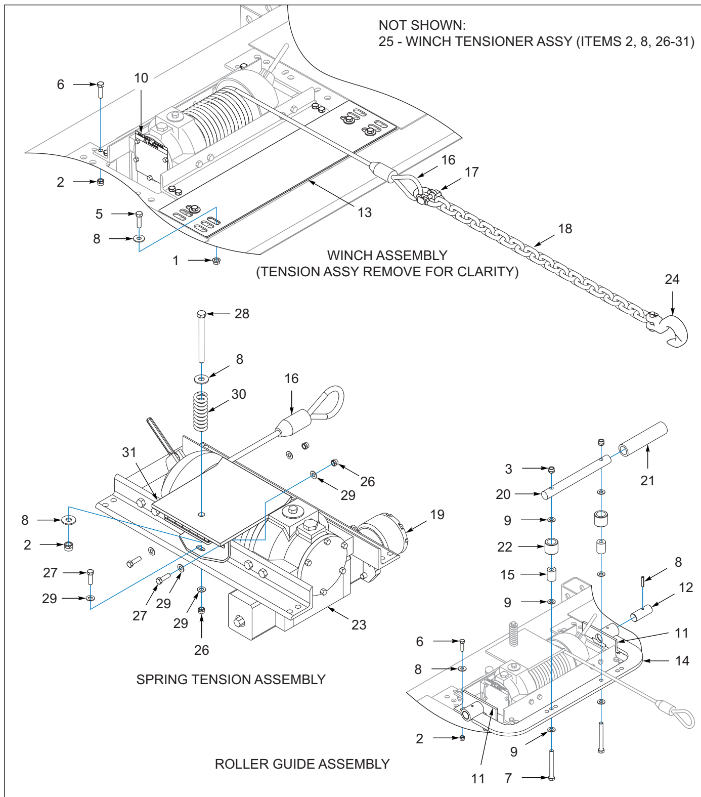
Figure 11-1: Winch Install, Braden 12K, 1 Speed, Spring Tension (OPTION)
