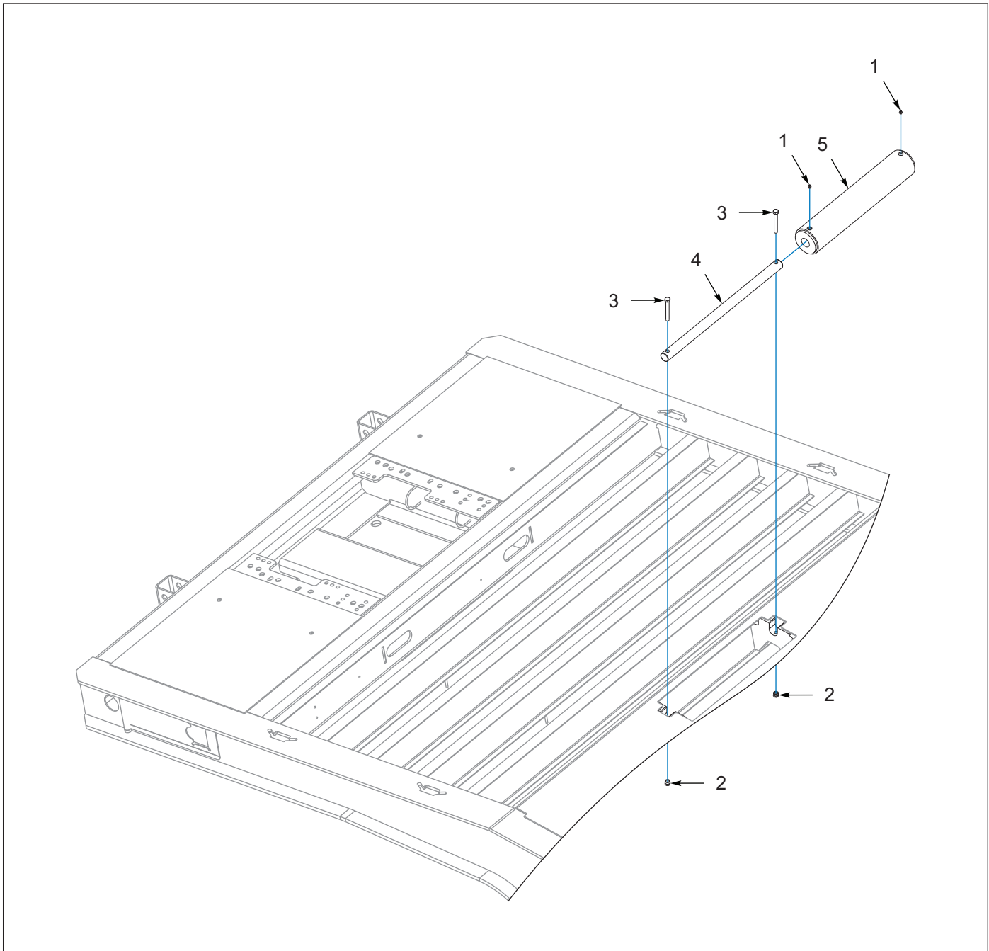
Figure 11-29: Upper Deck, Slope Roller (OPTIONS)
