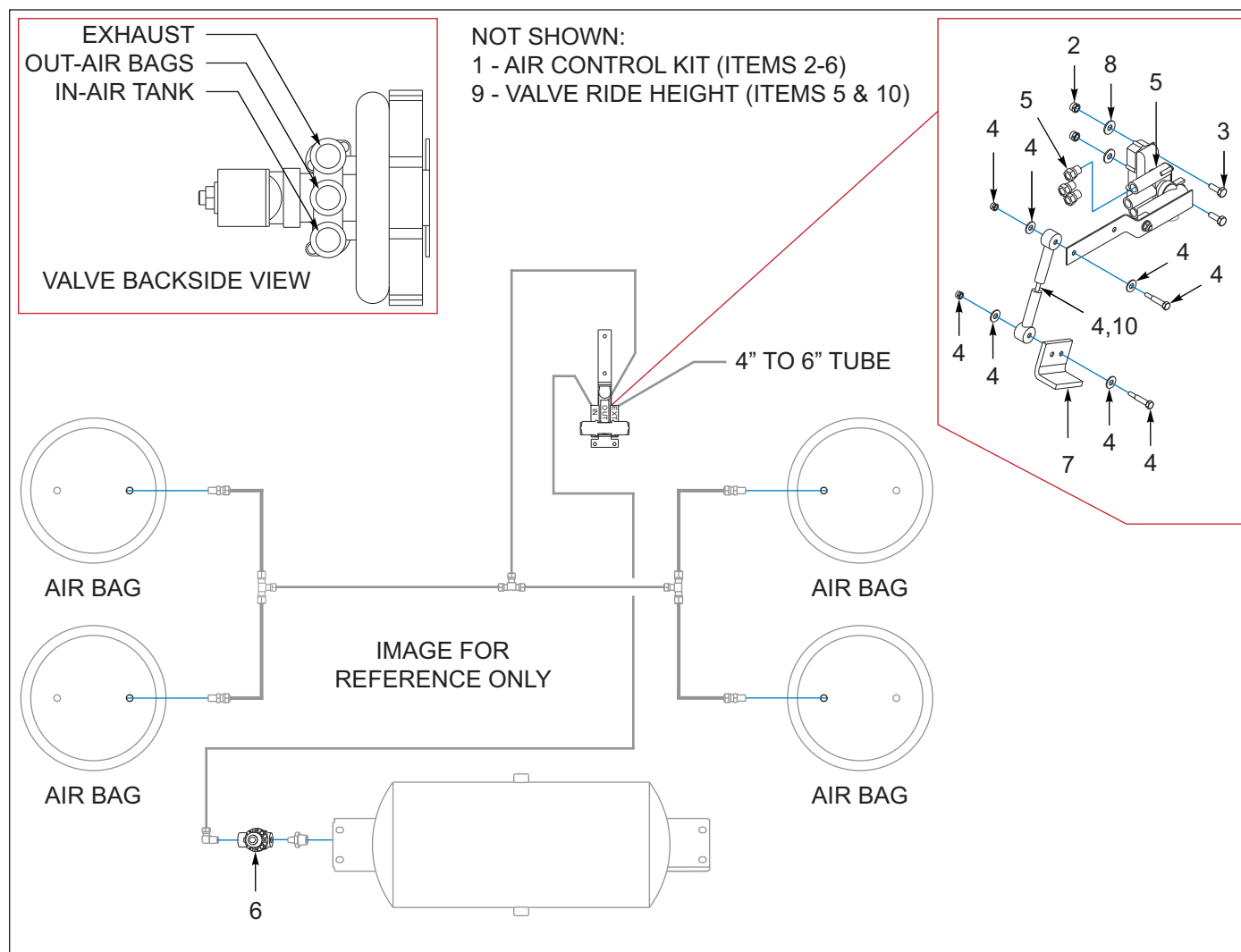
Figure 6-16: Suspension Air Control, Kit, Neway
