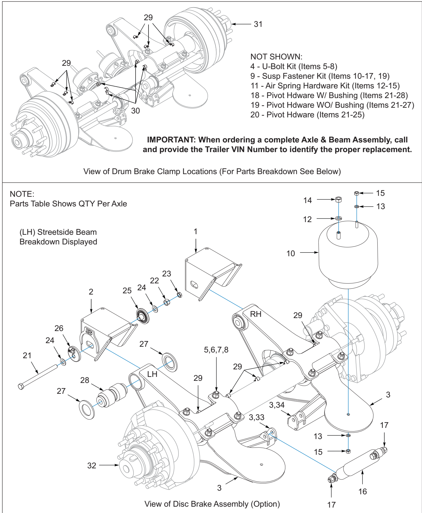
Figure 3-12: Axle Suspension, LSS-25K-5.5 RLU, 16.5
