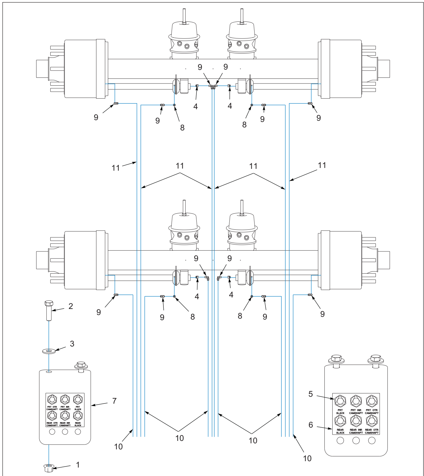
Figure 8-1: Drum Brakes, 2 Axle (Before 11/07/2018)
