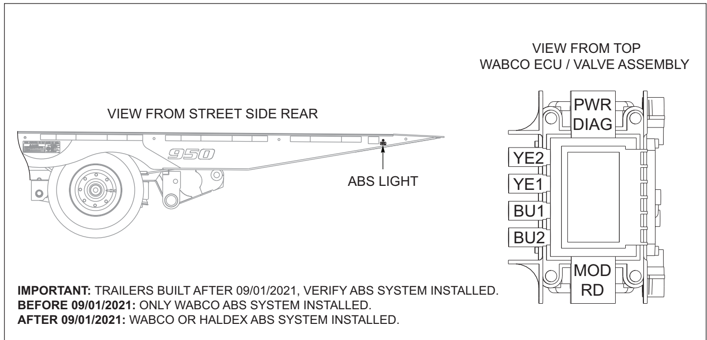
Figure 7-10: Anti-Lock Brakes, Wabco (2 of 2)
