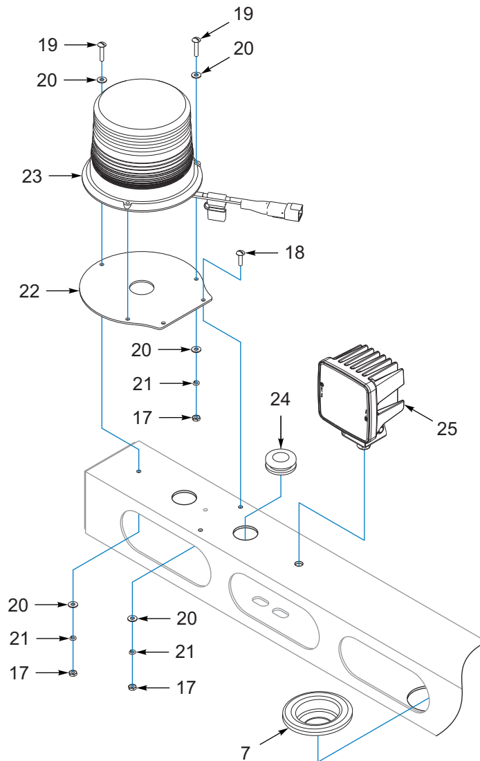
CHAIN RACK W/ S/T/T, BEACON, WORK LIGHTS SHOWN BACKSIDE VIEW
