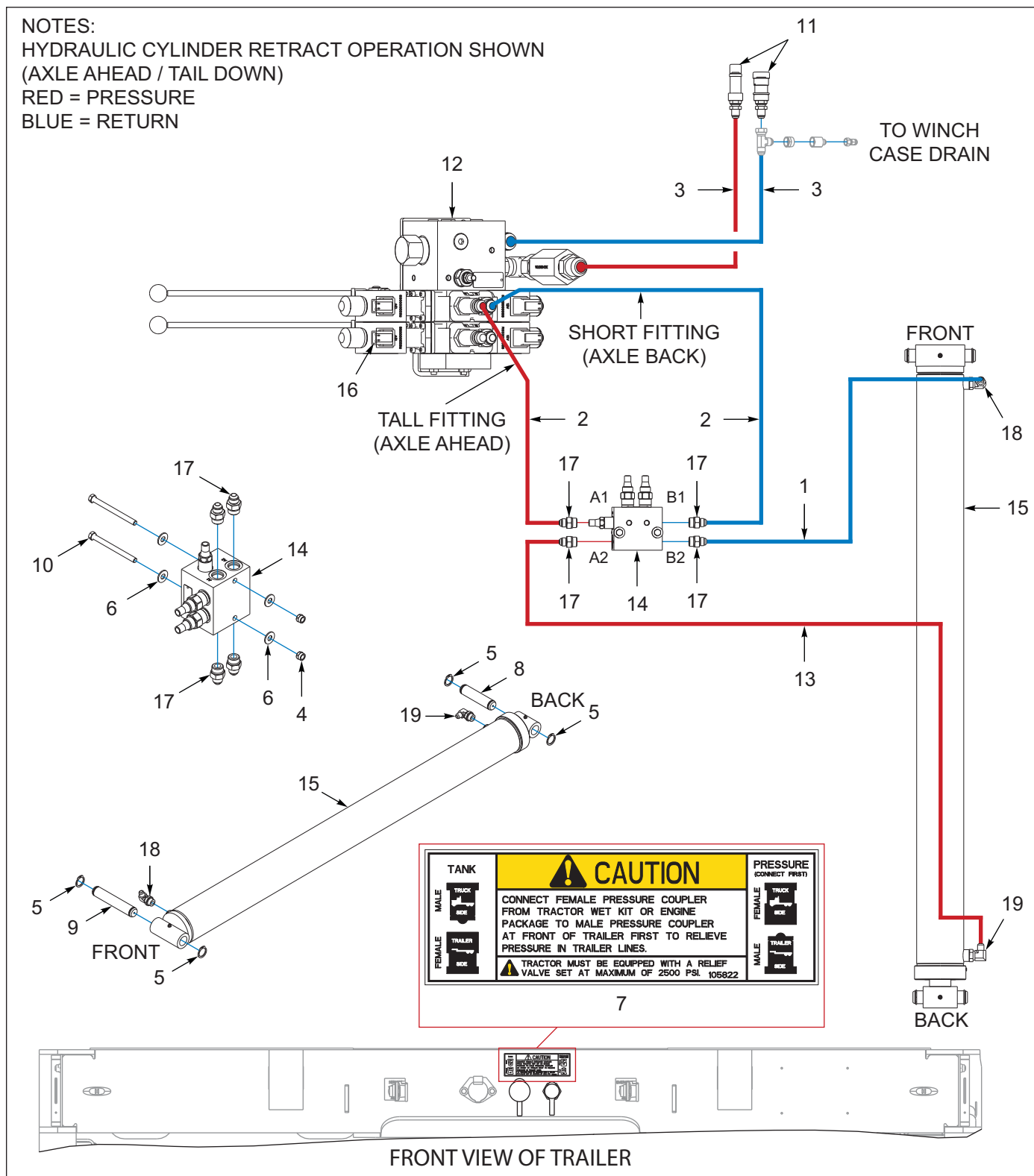
Figure 9-1: Frame Assembly, Axle / Tail Travel
