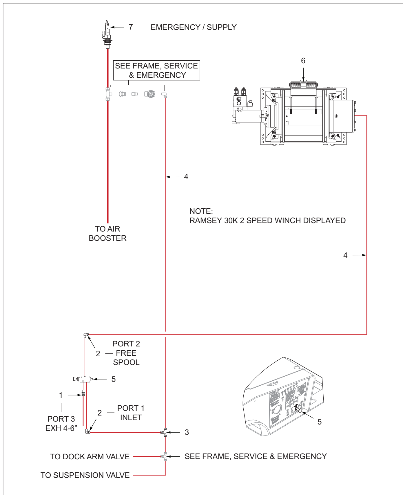
Figure 6-27: Winch Install, Ramsey 20K / 30K, 2 Speed (OPTION)
