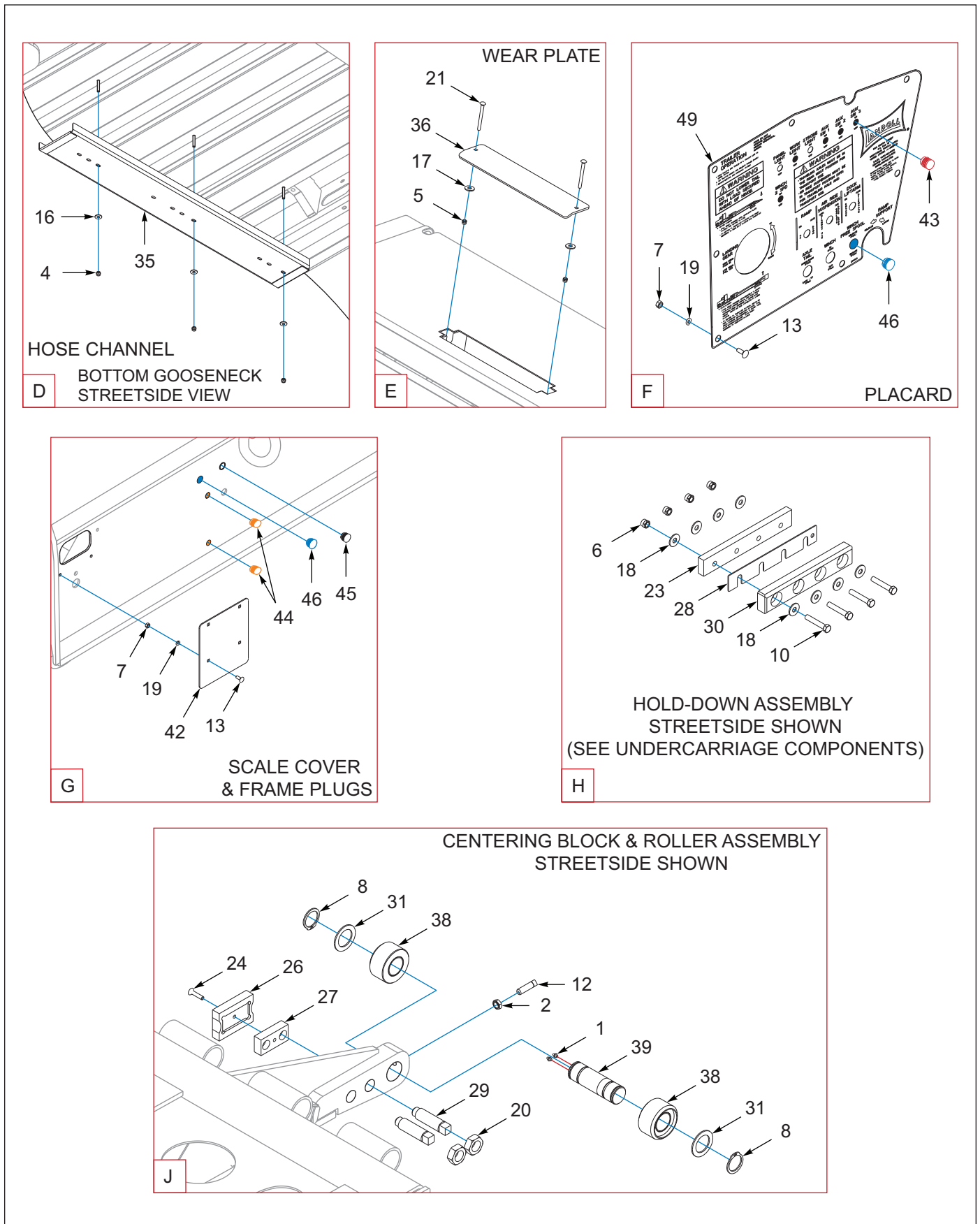
Figure 2-2: Frame Components (2 of 3)
