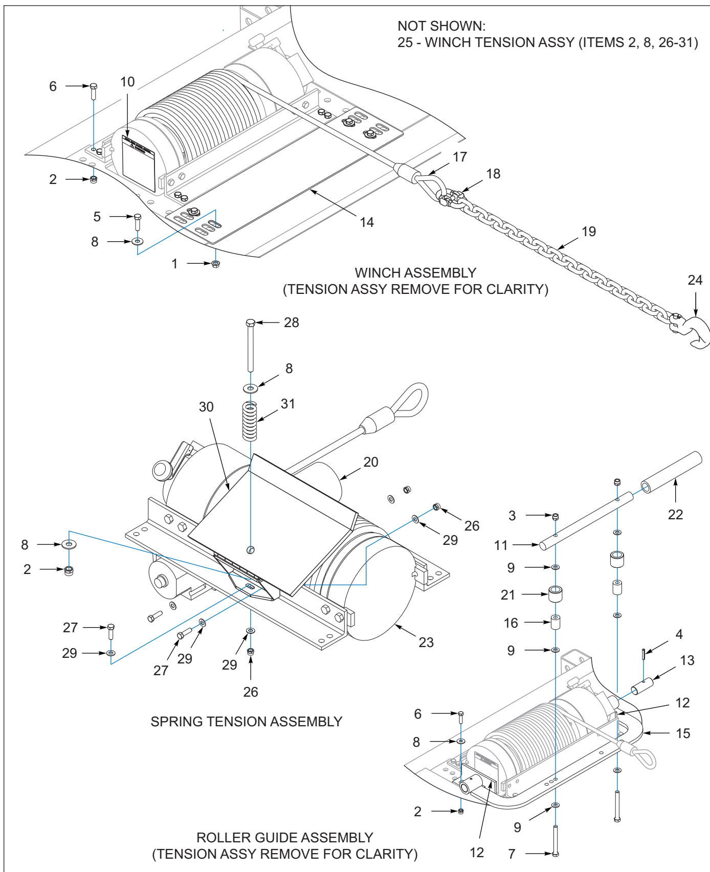
Figure 11-2: Winch Install, Braden 20K, 1 Speed, Spring Tension (OPTION)
