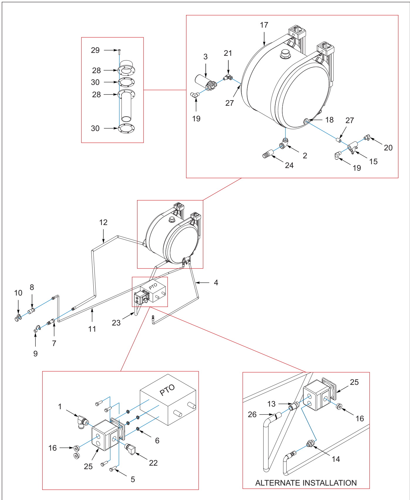
Figure 9-8: et Kit, Hydraulic (OPTION) (AFTER 03/01/2019)
