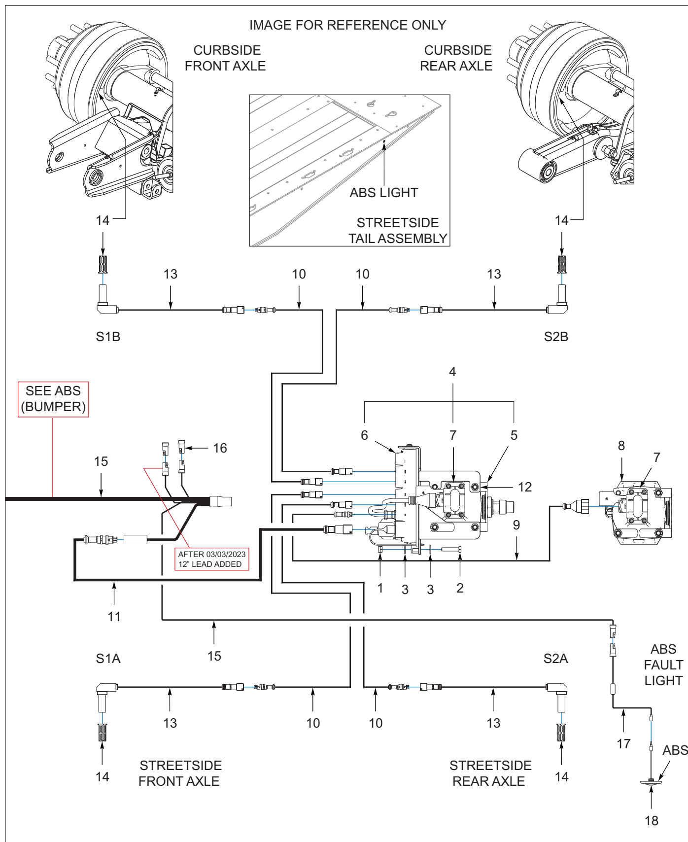
Figure 7-11: Anti-Lock Brakes, Haldex (1 of 2)
