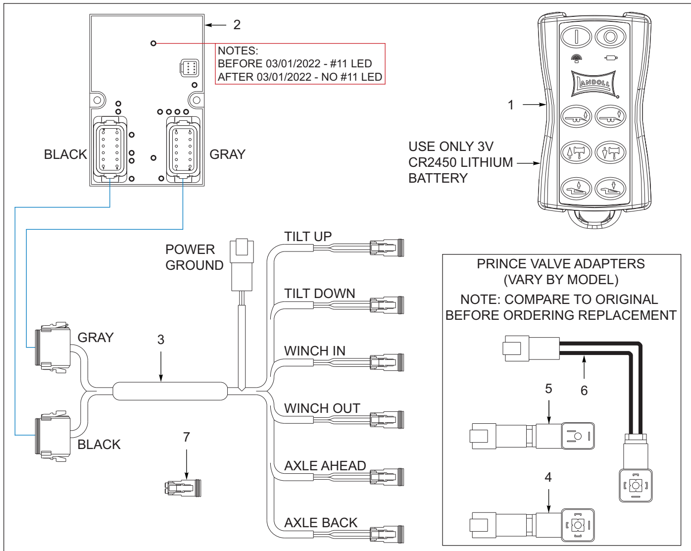
Figure 7-15: Remote Control Assembly, Wireless Brand (OPTION)
