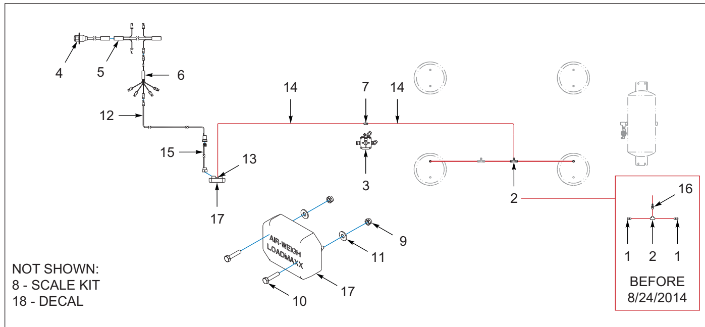
Figure 6-9: Scale, Quickload (BEFORE 03/31/2020) (OPTION)
