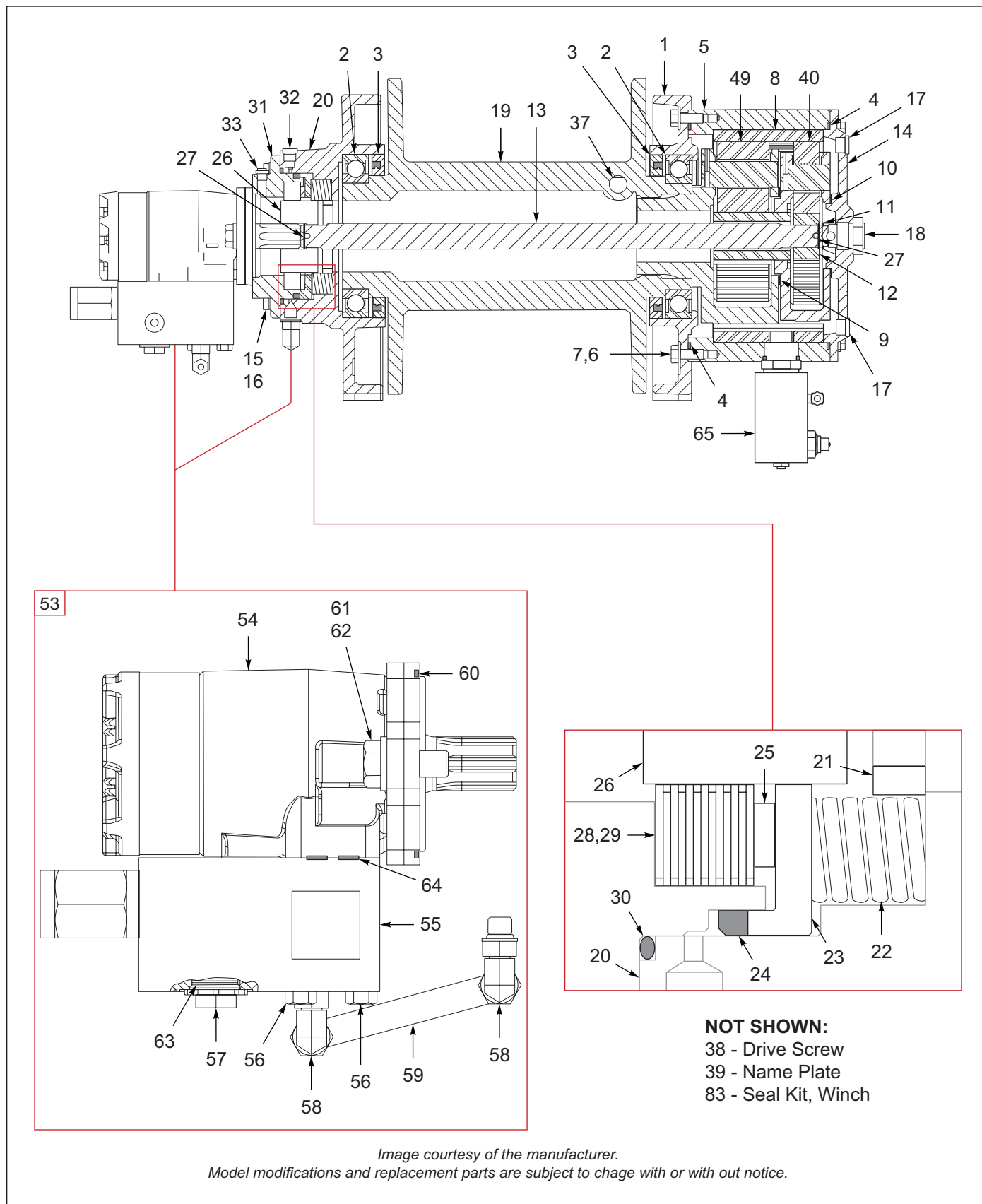
Figure 11-16: Winch Components, Braden 20K, 2 Speed (OPTION) (1 of 2)
