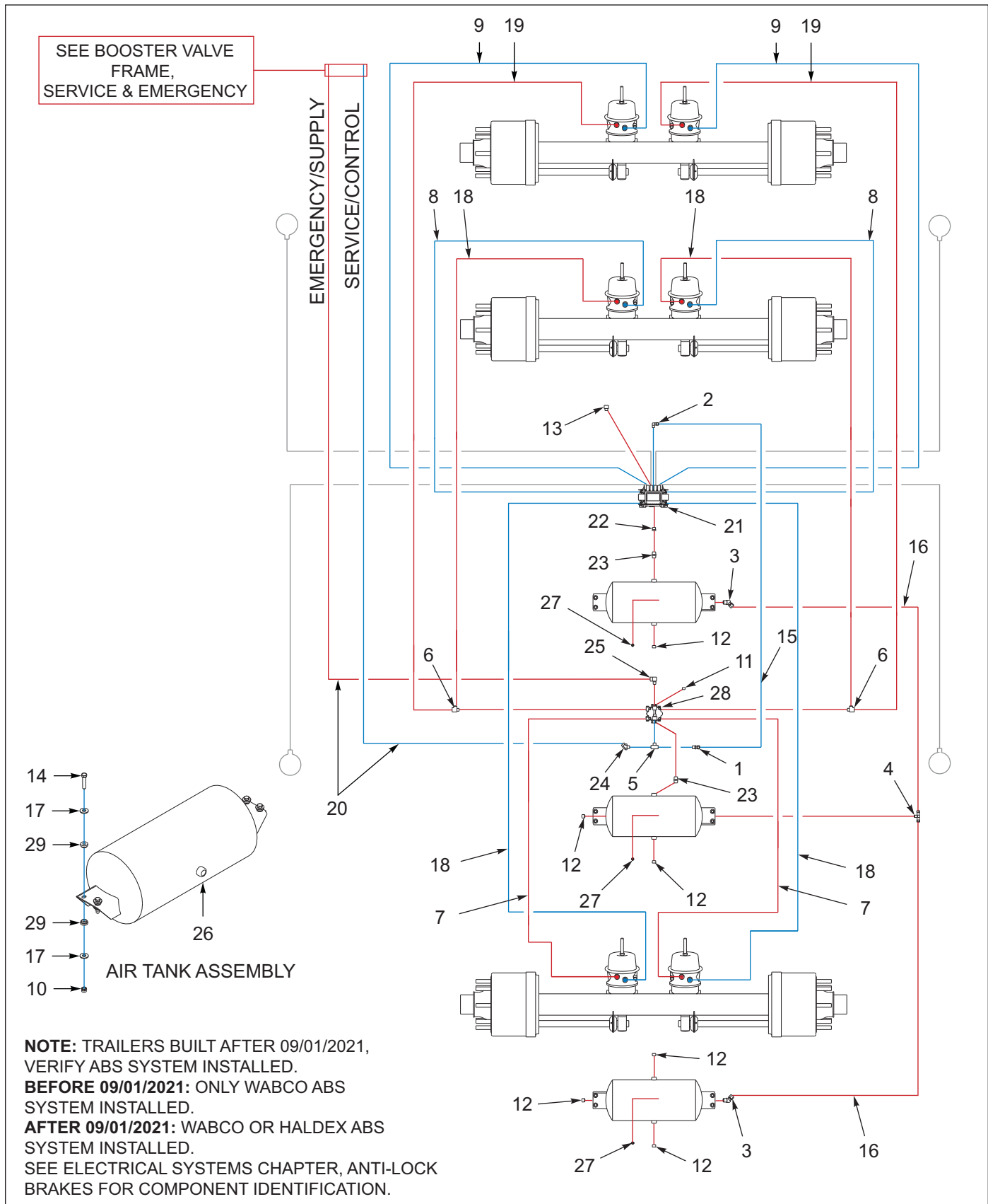
Figure 6-4: Anti-Lock Brakes, Service & Emergency, 3 Axle, Wabco
