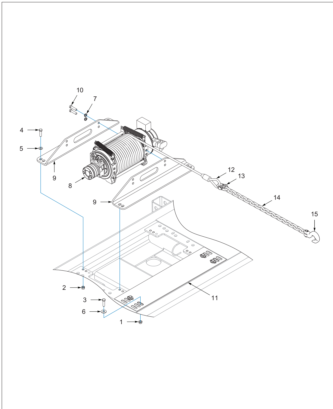
Figure 11-7: Winch Install, Warn 12K, 1 Speed, Spring Tension (OPTION)
