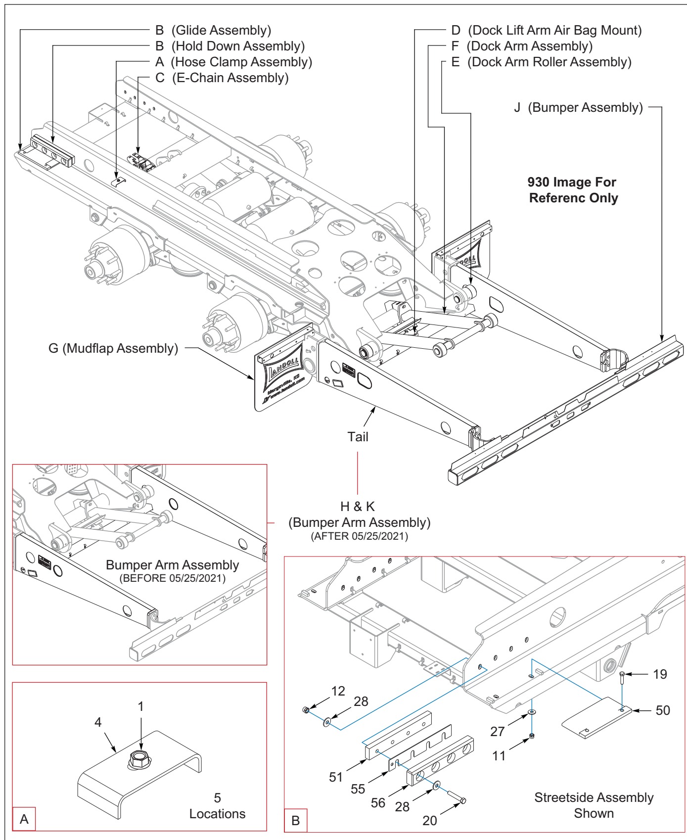
Figure 2-17: Undercarriage Components (1 of 3)
