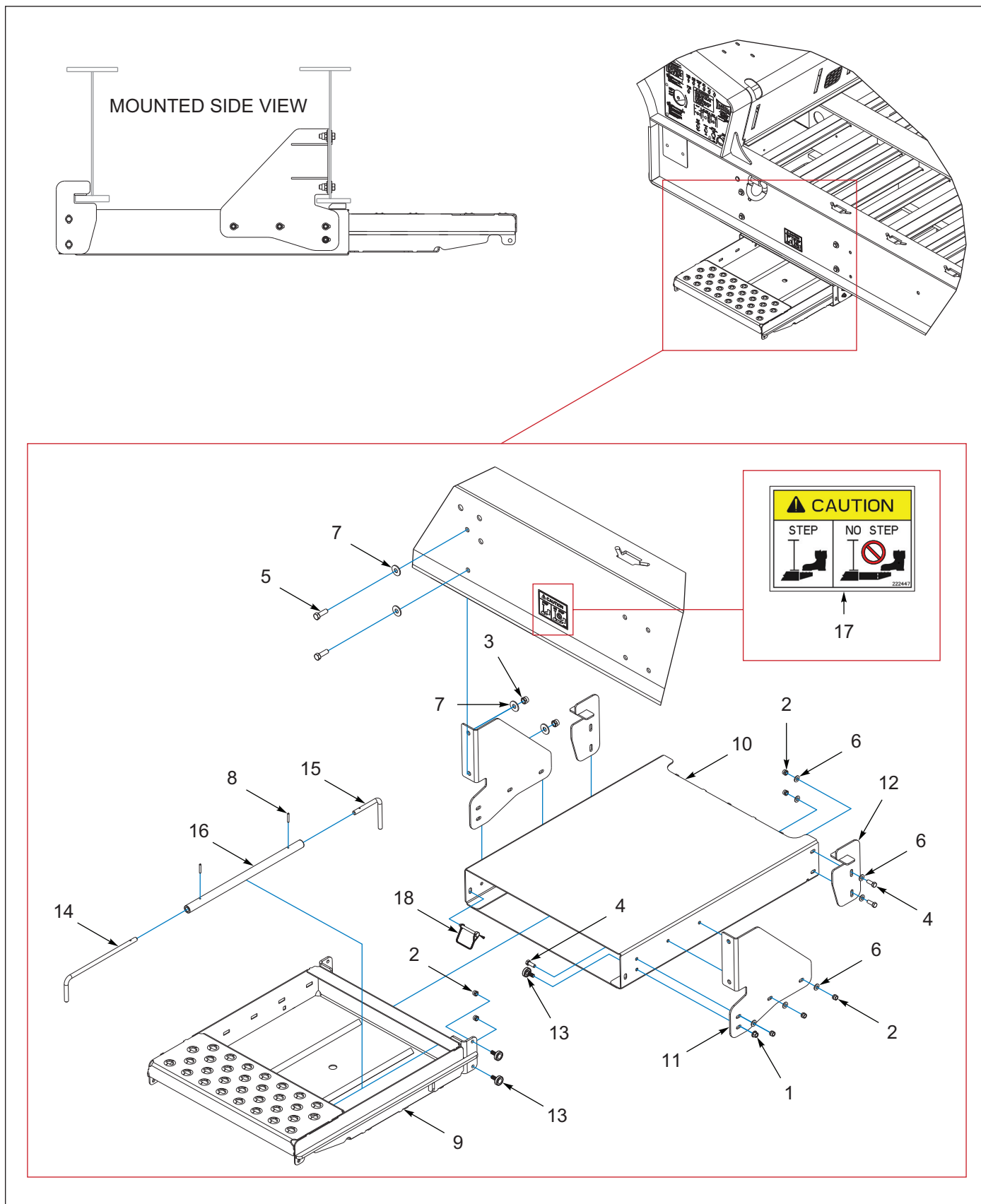
Figure 5-8: Step, Retractable Drawer Assembly (OPTIONS)
