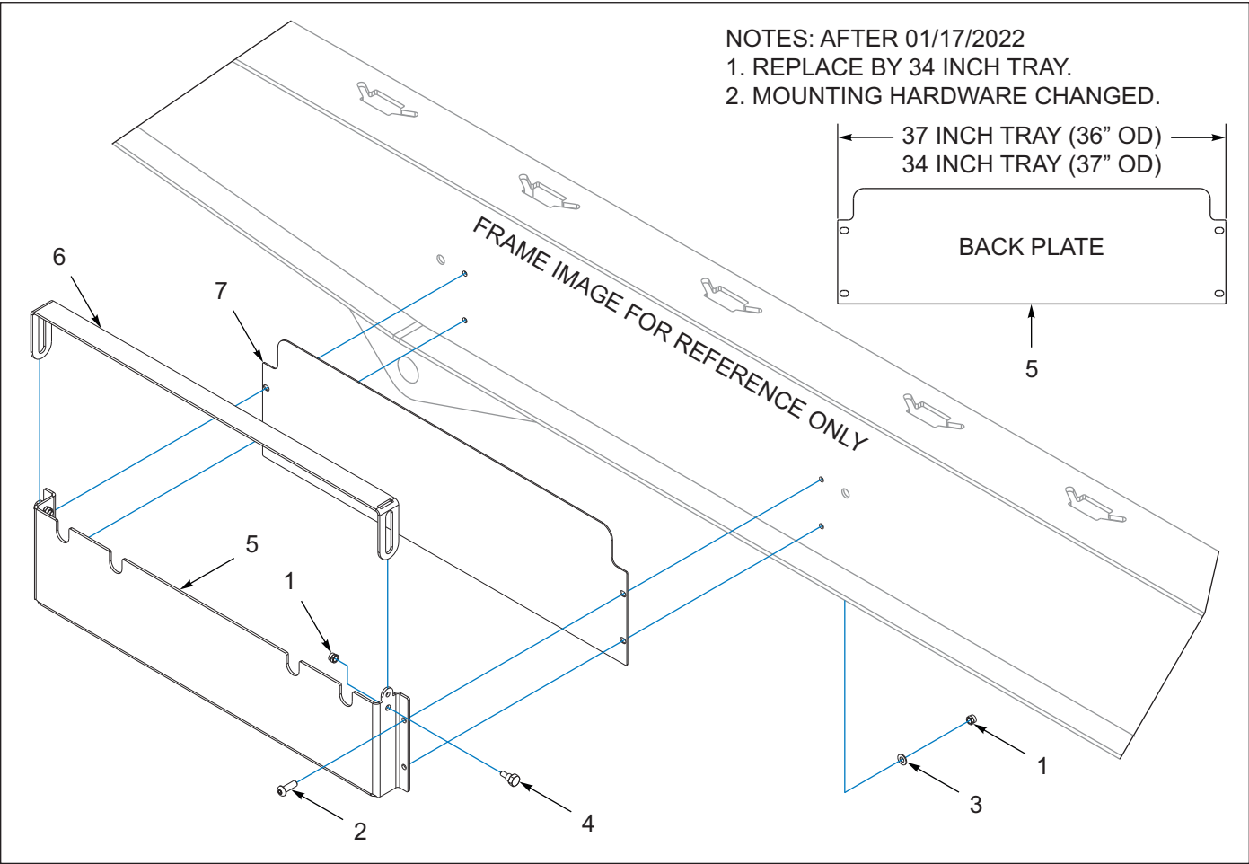
Figure 5-1: Chain Tray Assembly (BEFORE 01/17/2022) (OPTIONS)
