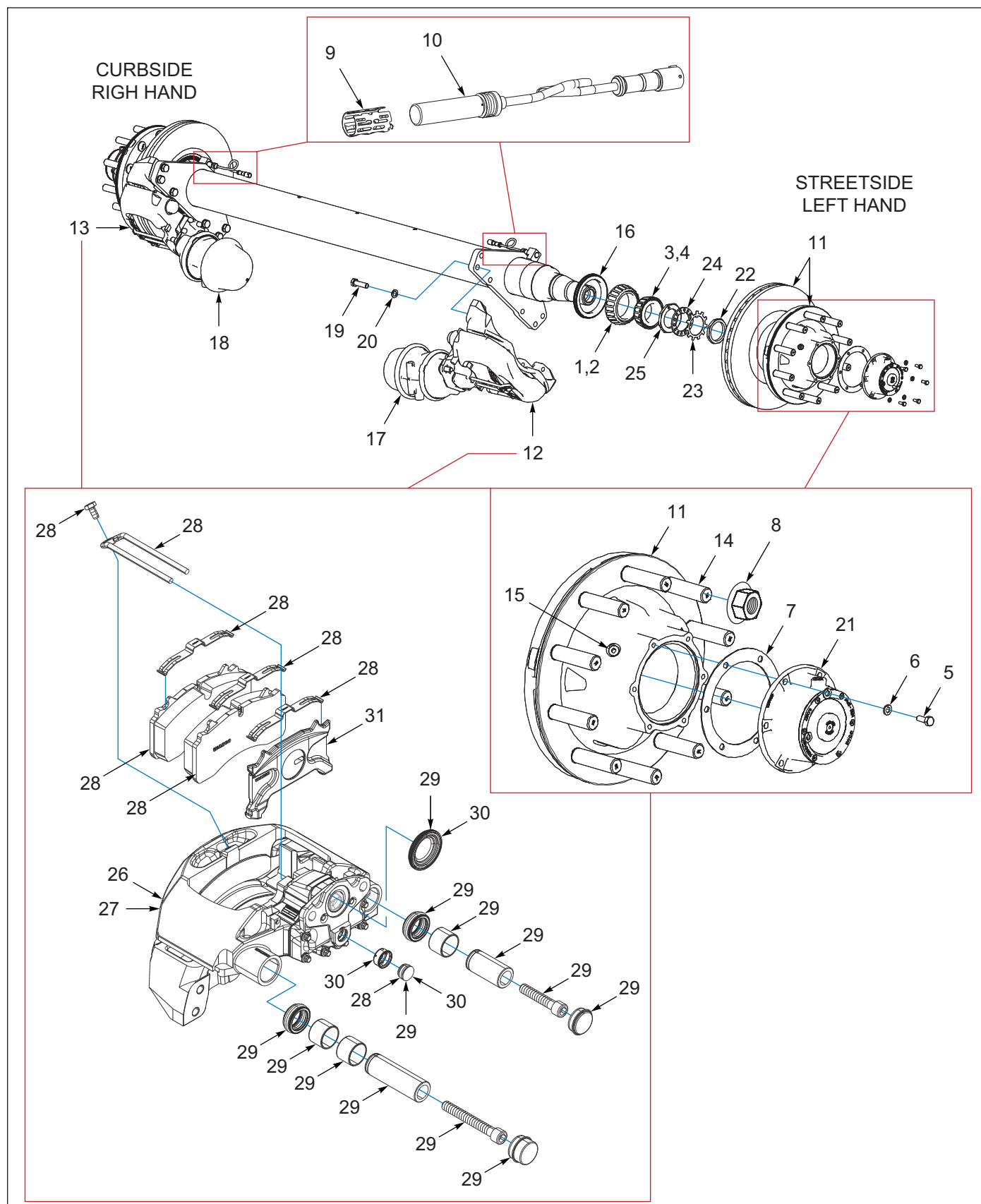
Figure 3-7: Axle 16.5 Disc Brake & Hub Components (OPTION) (1 of 2)
