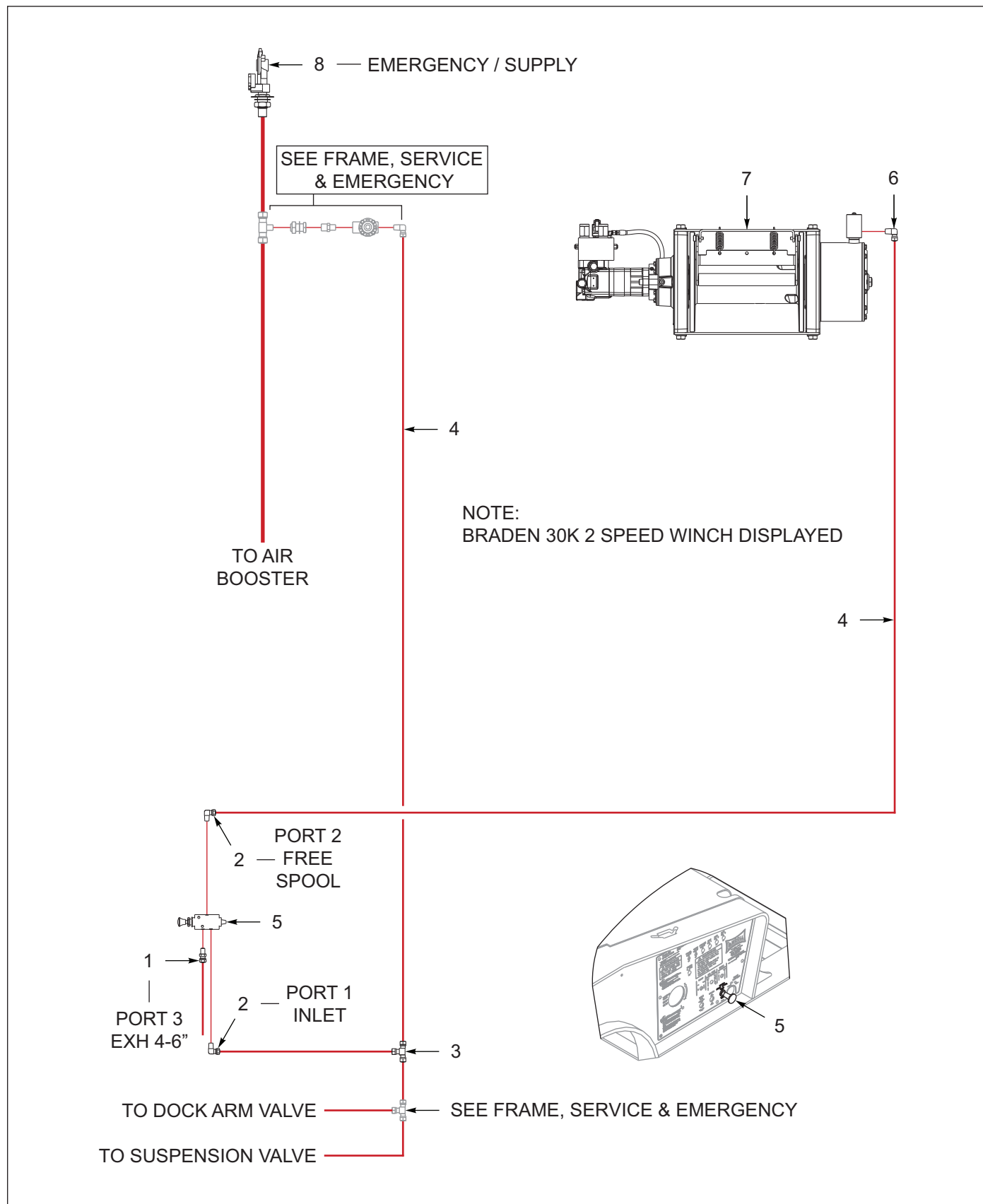
Figure 6-26: Winch Install, Braden 20K / 30K, 2 Speed (OPTION)
