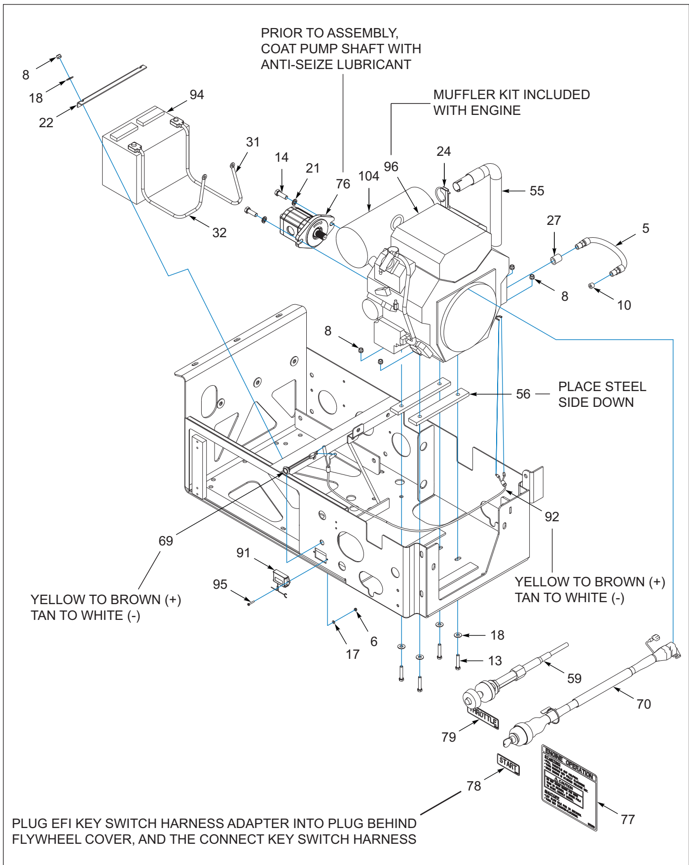
Figure 10-3: Engine, 25HP, Upper Deck Assembly (OPTION) (3 of 5)
