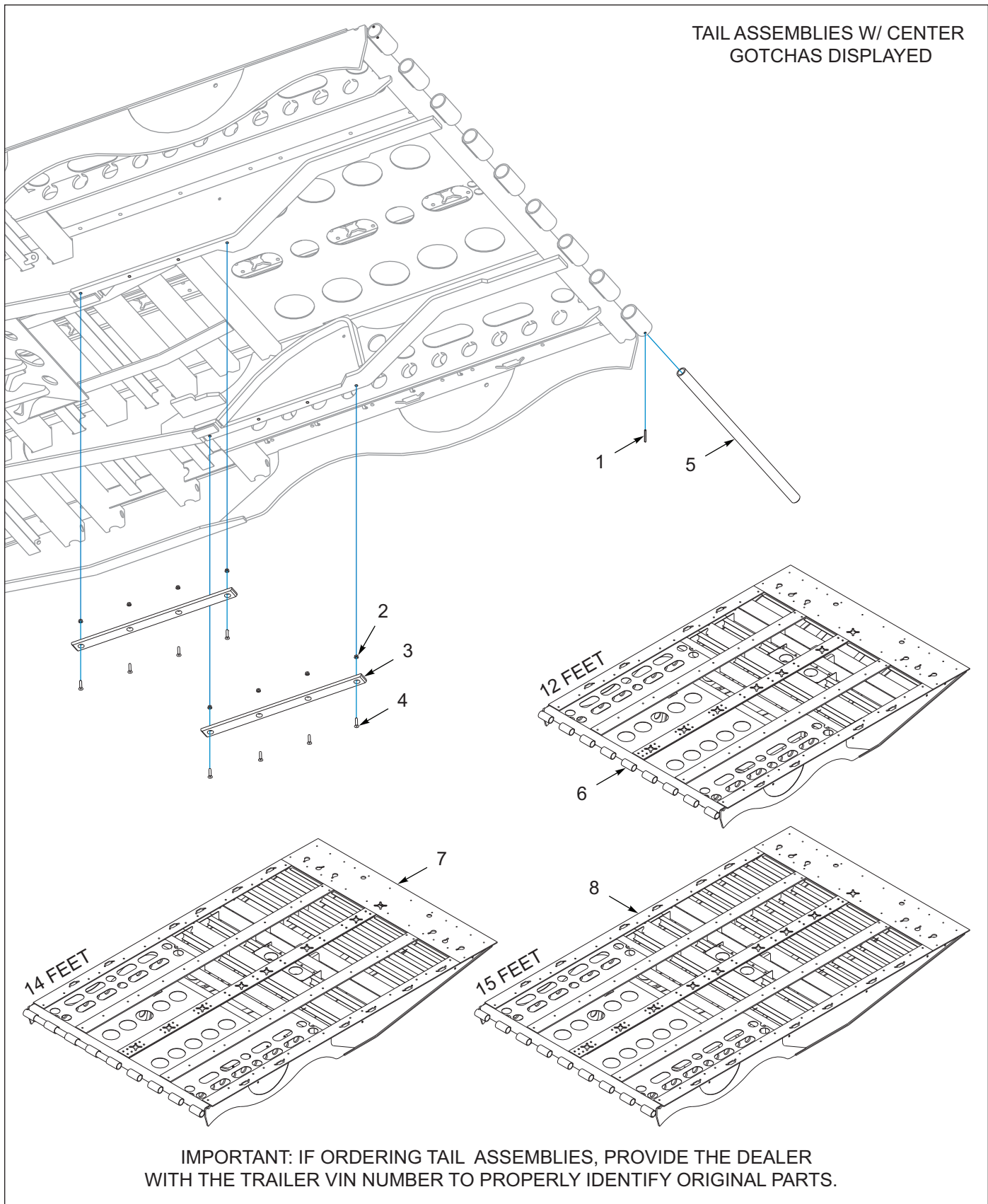
Figure 2-12: Tail Assembly, General Components
