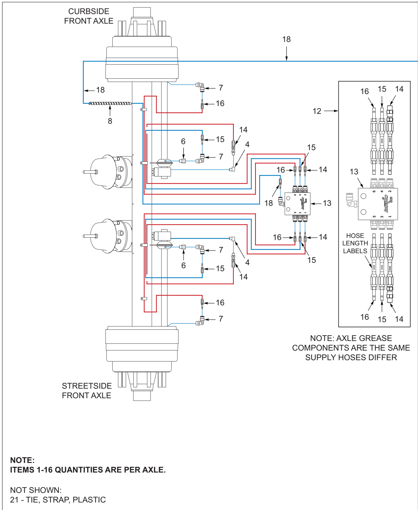
Figure 8-3: Drum Brakes, 2 Axle (After 08/31/2020) (1 of 3)
