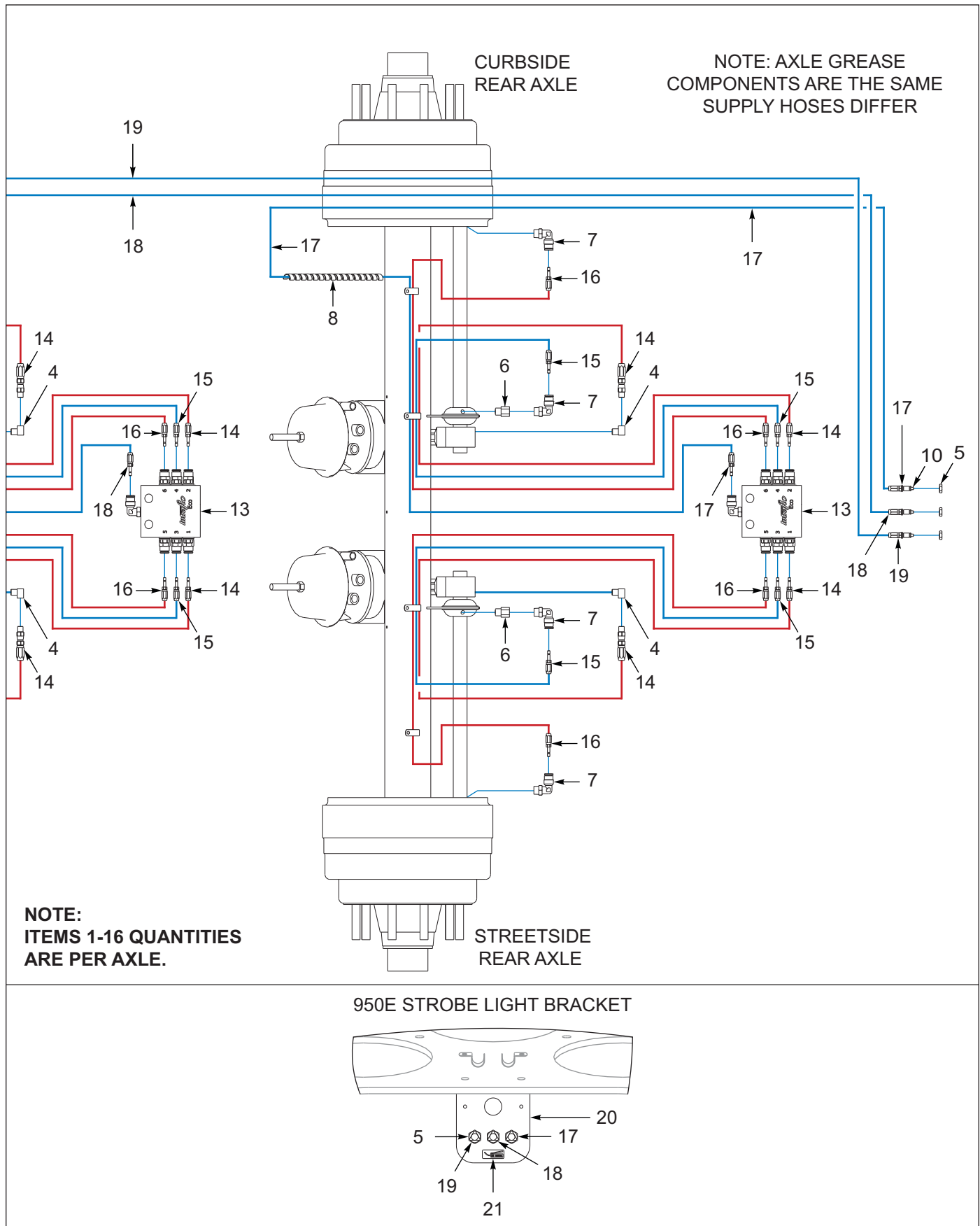
Figure 8-9: Drum Brakes, 3 Axle (After 08/31/2020) (2 of 3)
