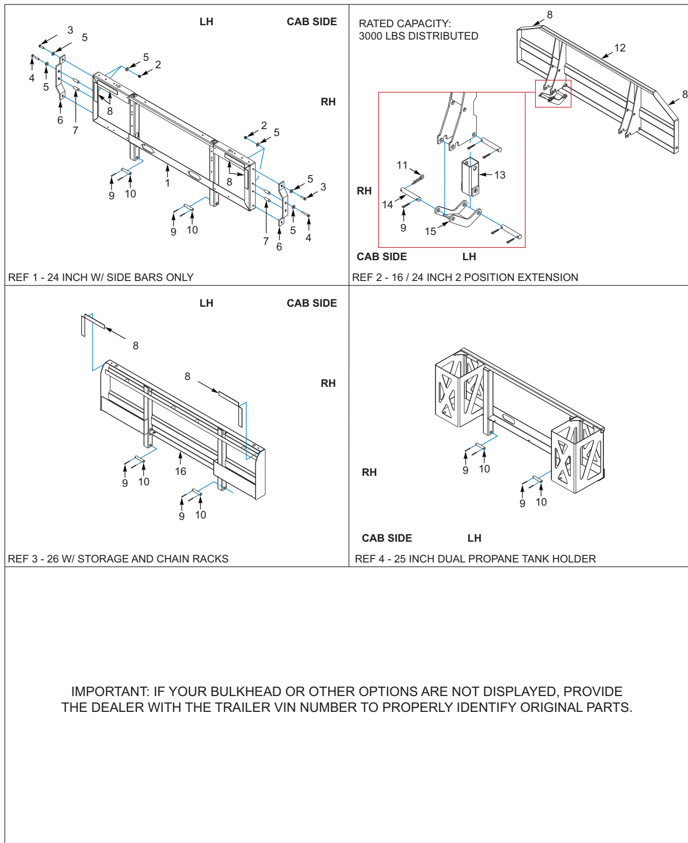
Figure 2-5: Bulkhead Components, 24, 25 & 26 x 102 (OPTIONS)
