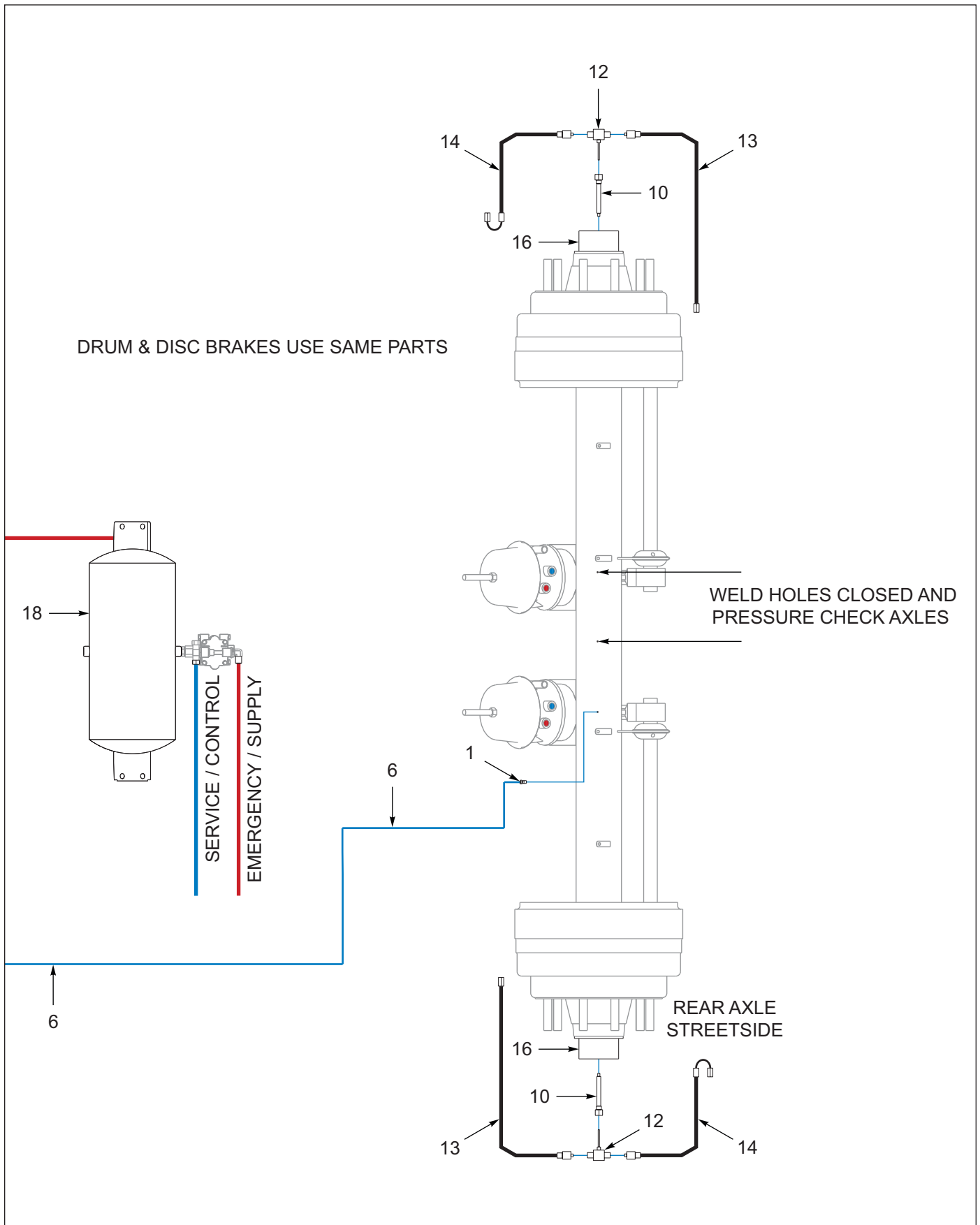
Figure 6-20: Tire Inflation, 2 Axle (OPTION) (2 of 2)
