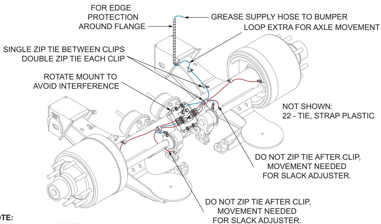
Figure 8-10: Drum Brakes, 3 Axle (After 08/31/2020) (3 of 3)
