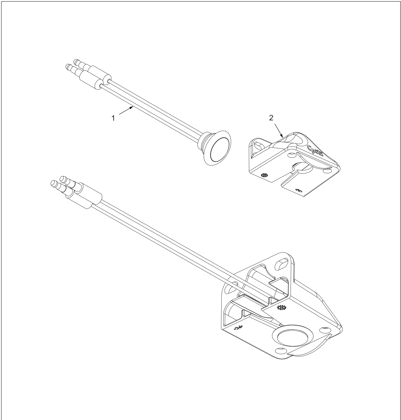
Figure 7-7: License Plate Light Assembly
