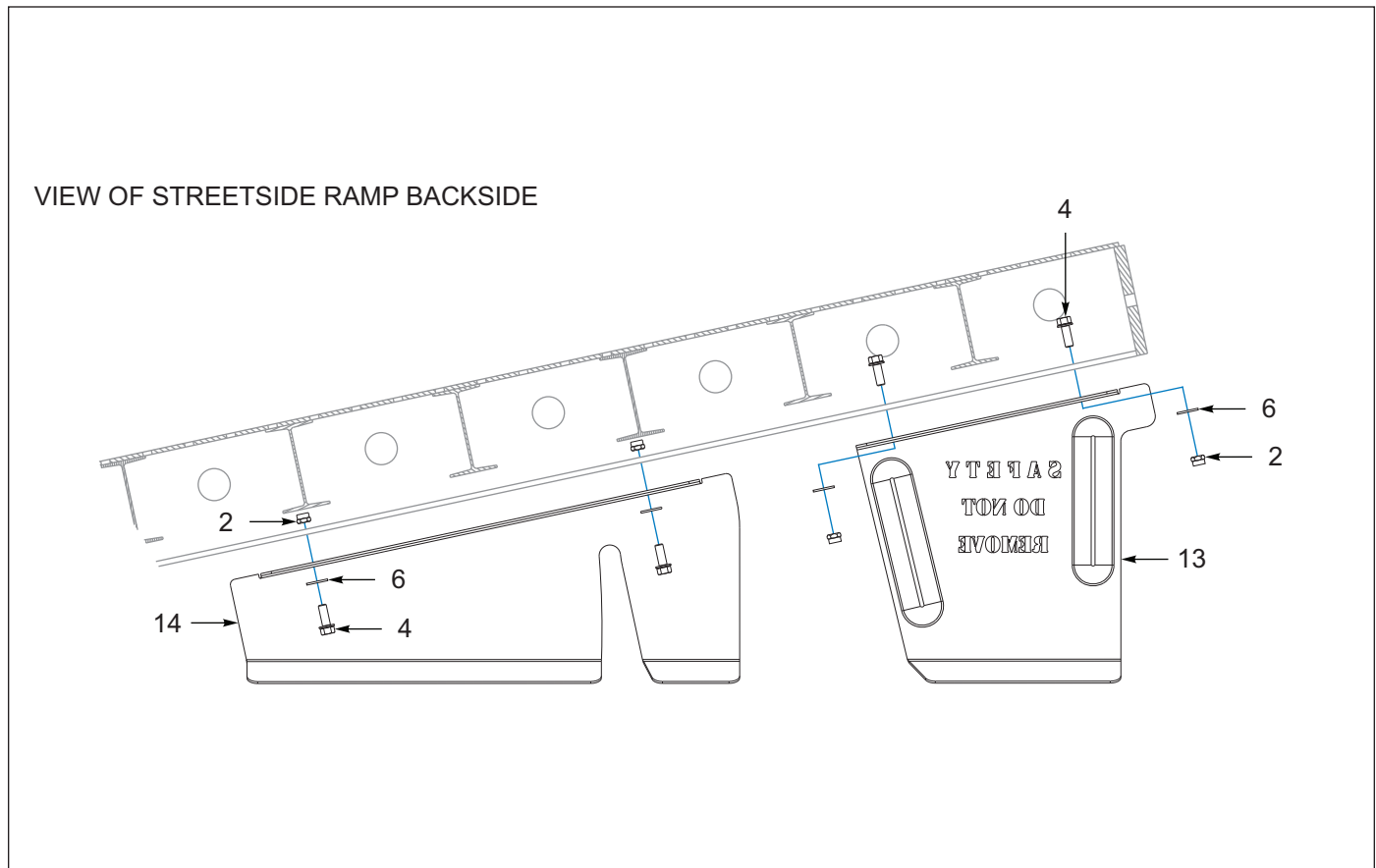
Figure 4-3: Front Slope, Deck Components (AFTER 03/11/2021) (OPTION) (2 of 2)
