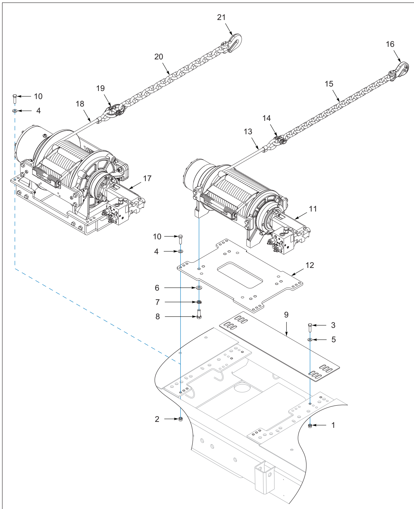
Figure 11-6: Winch Install, Ramsey 20K / 30K, 2 Speed (OPTION)
