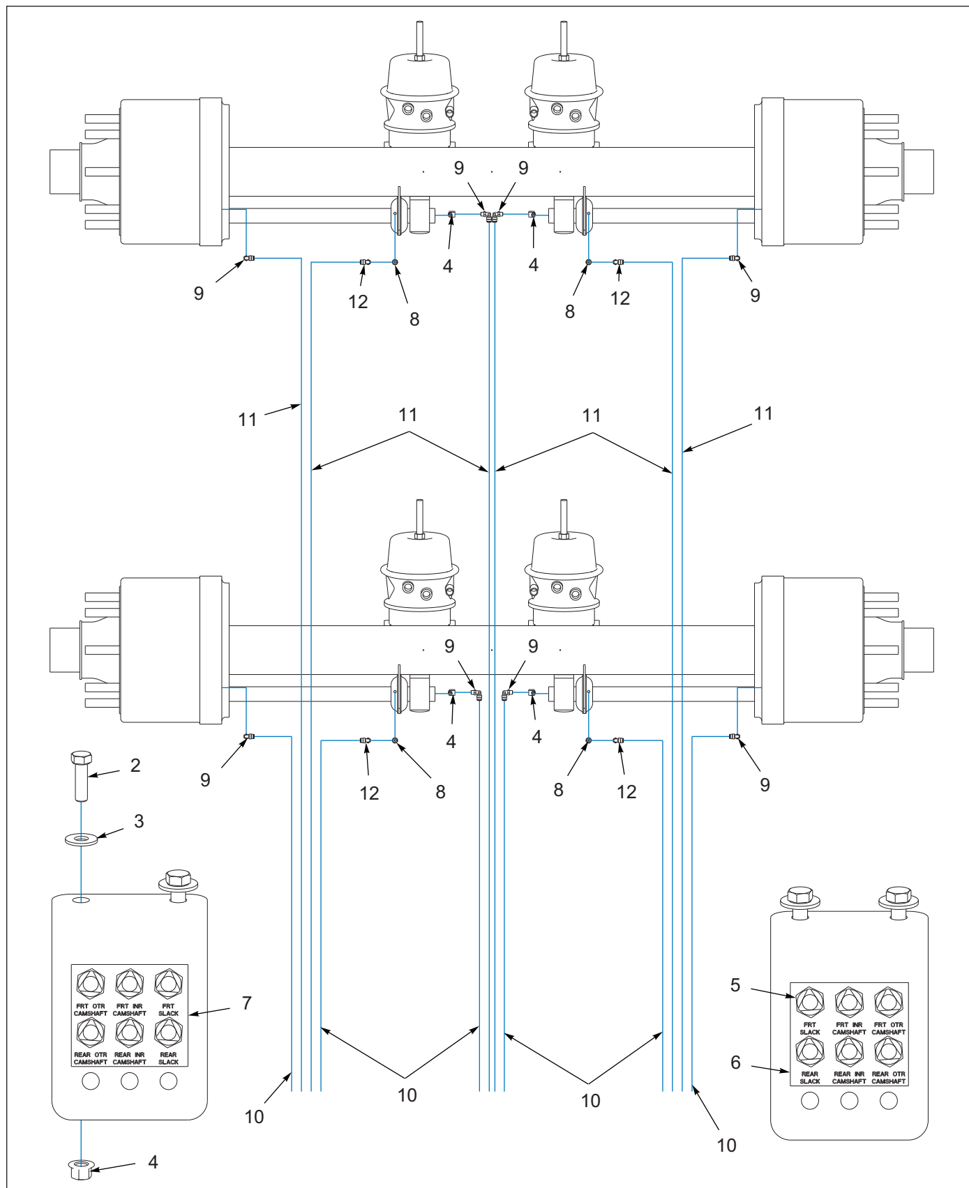
Figure 8-2: Drum Brakes, 2 Axle (After 11/07/2018 - Before 08/31/2020)
