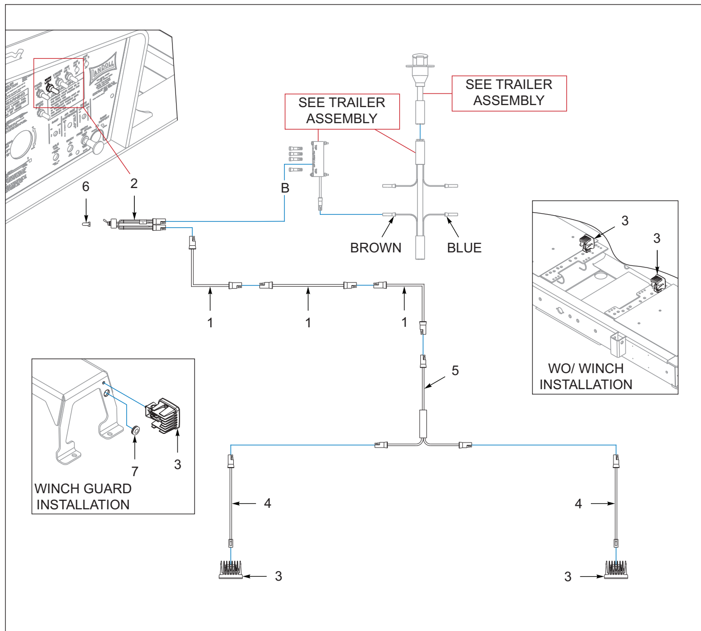
Figure 7-24: Winch Work Lights (OPTION)
