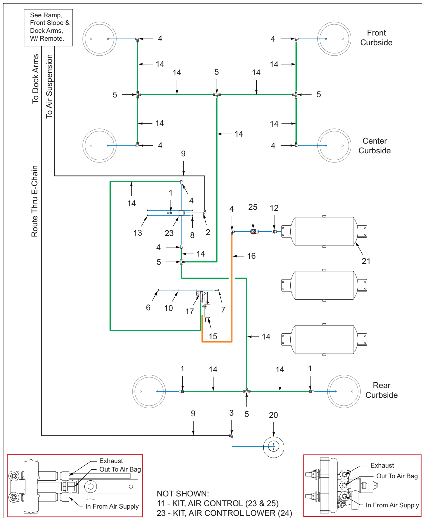
Figure 6-15: Suspension, Ride Height, 3 Axle, 3/8 in Valve, (AFTER 06/12/2023)
