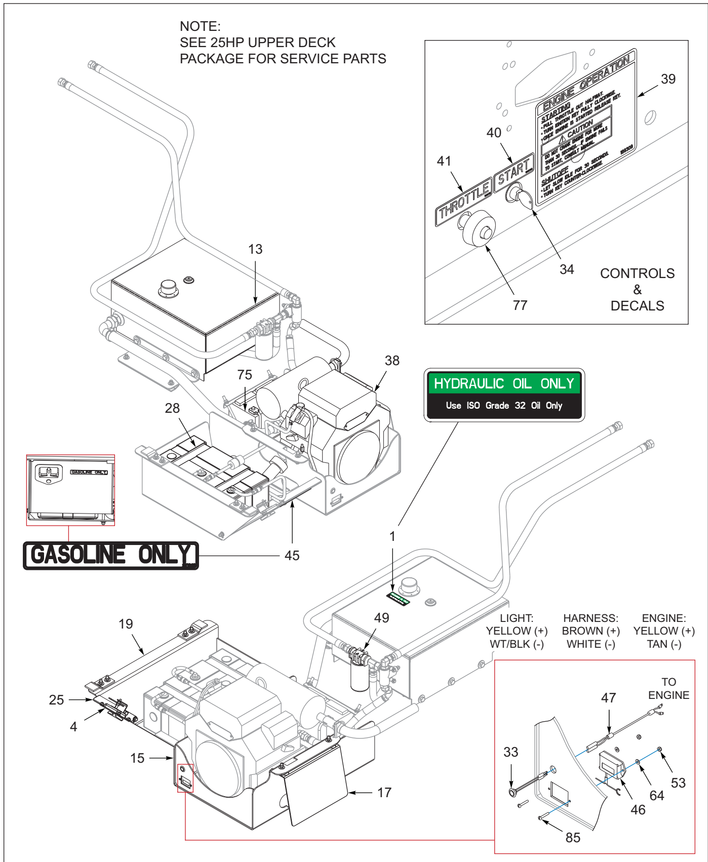
Figure 10-6: Engine, 25HP, Slope Deck Assembly (OPTION) (1 of 4)
