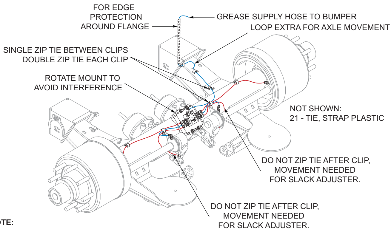
Figure 8-5: Drum Brakes, 2 Axle (After 08/31/2020) (3 of 3)
