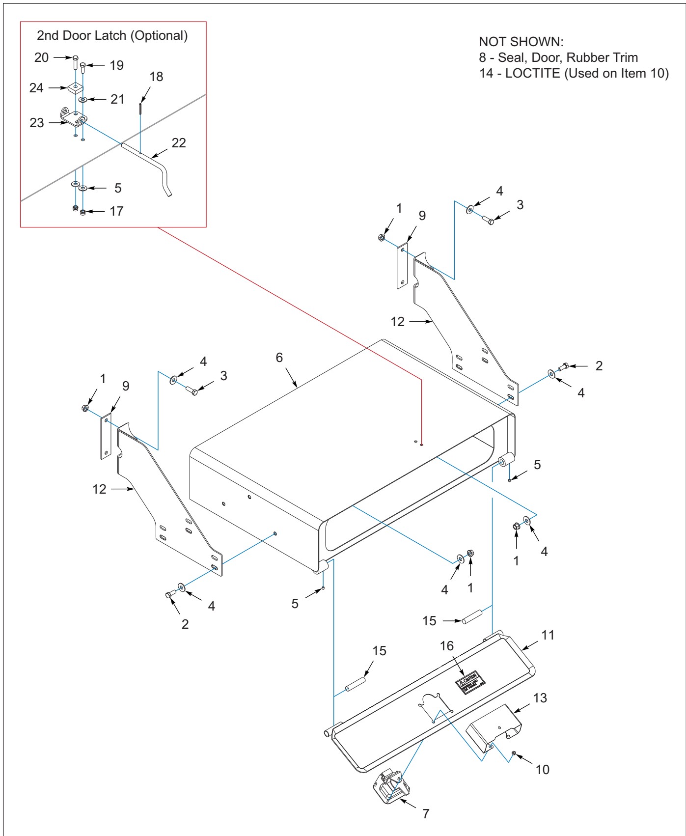
Figure 5-10: Toolbox, Bolt-On, 42"W X 28"D X 9"H (OPTIONS)
