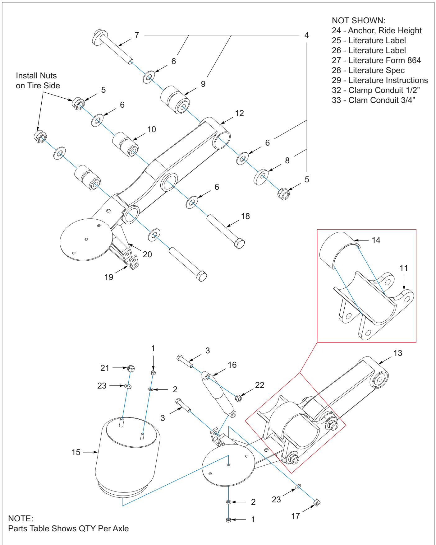
Figure 3-10: Axle Suspension, RLU-228, 12.25 & 16.5 (2 of 2)
