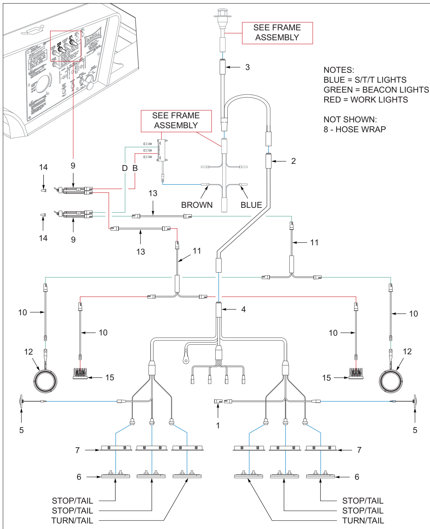
Figure 7-14: Bulkhead, Light Bar, Chain Rack (OPTIONS)
