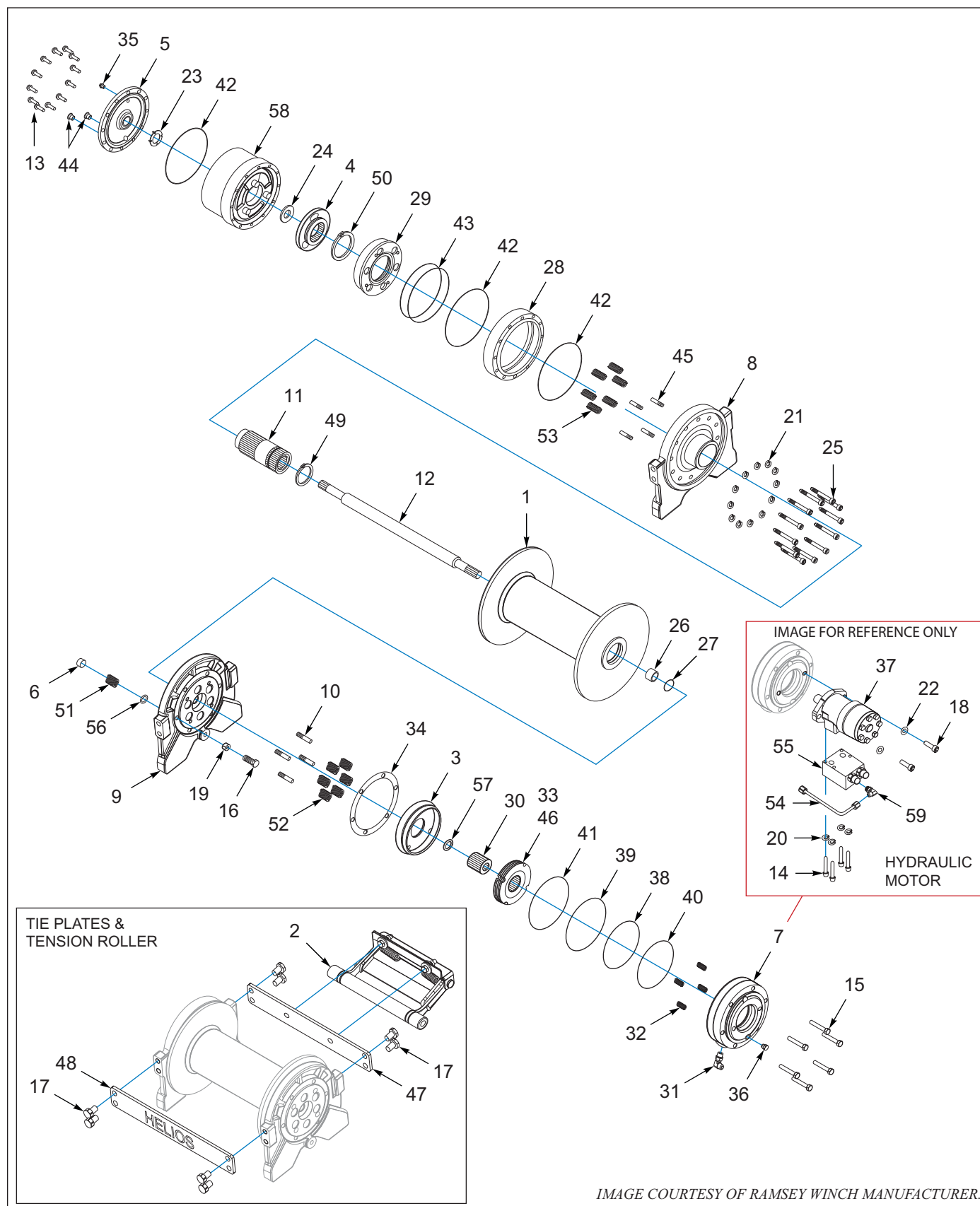
Figure 11-20: Winch Components, Ramsey 20K, 2 Speed (OPTION)
