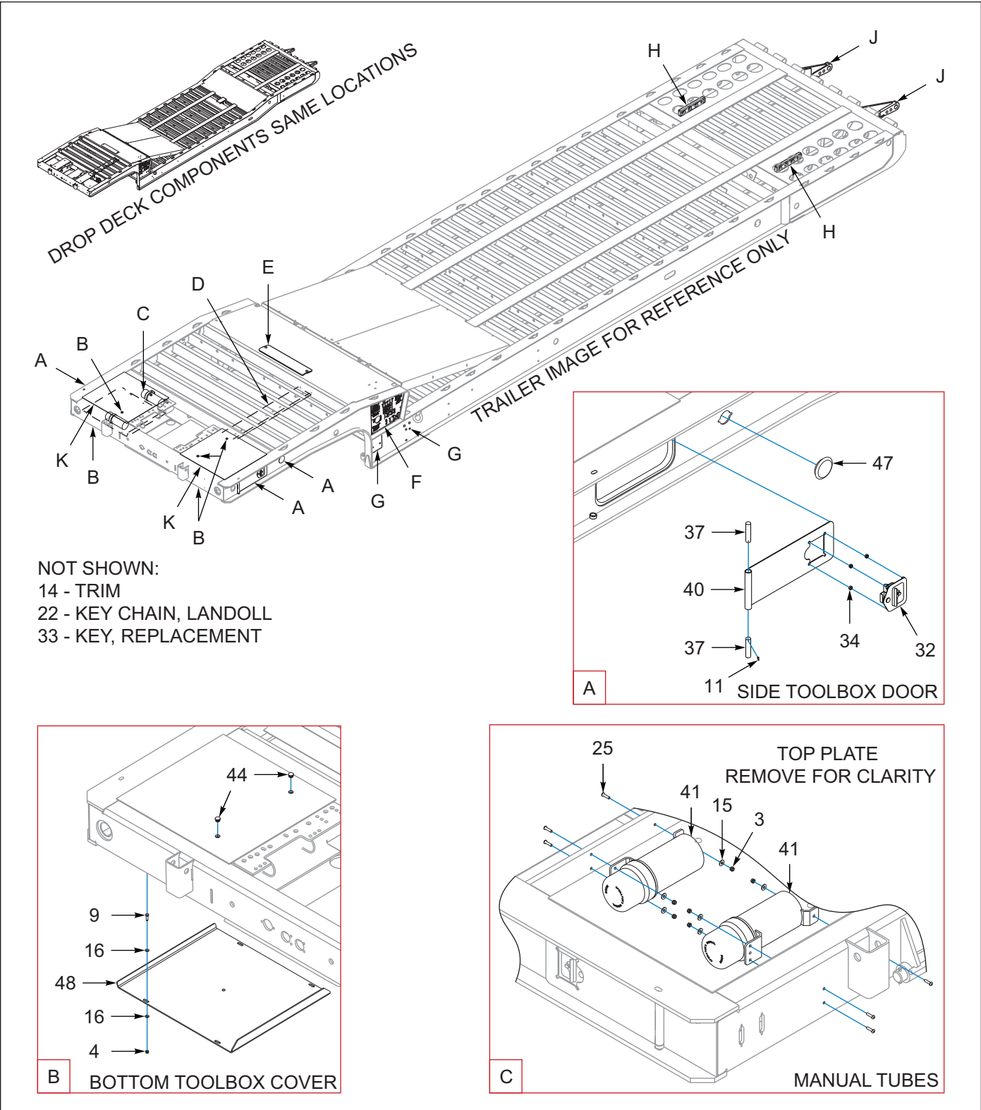
Figure 2-1: Frame Components (1 of 3)
