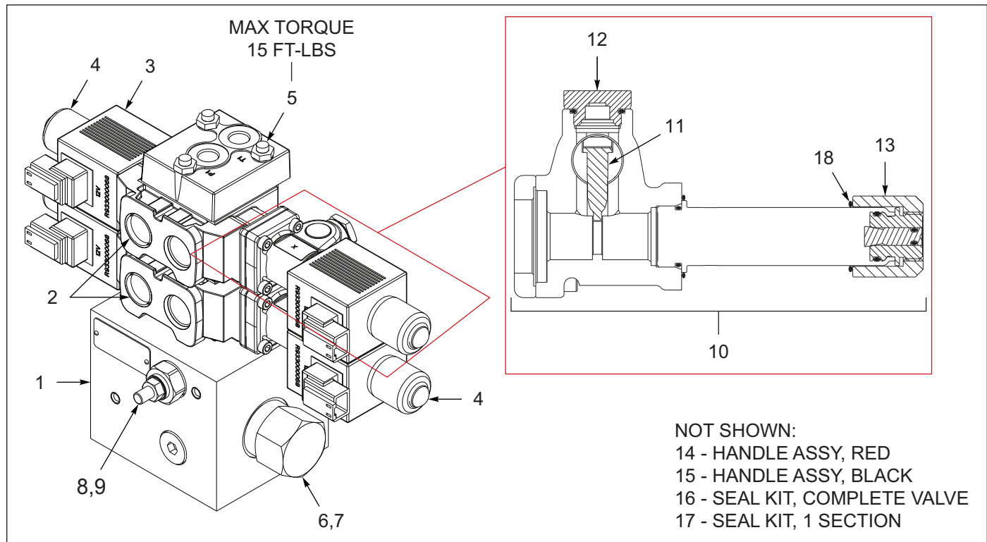
Figure 9-6: Valve Components, 2 Spool Solenoid
