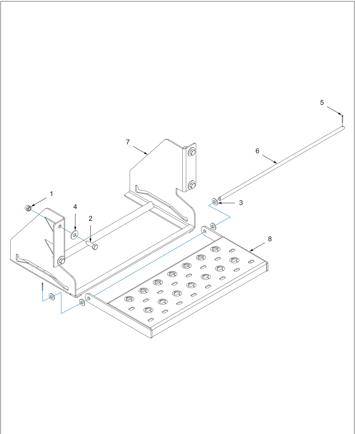
Figure 5-7: Step, Retractable Assembly (OPTIONS)
