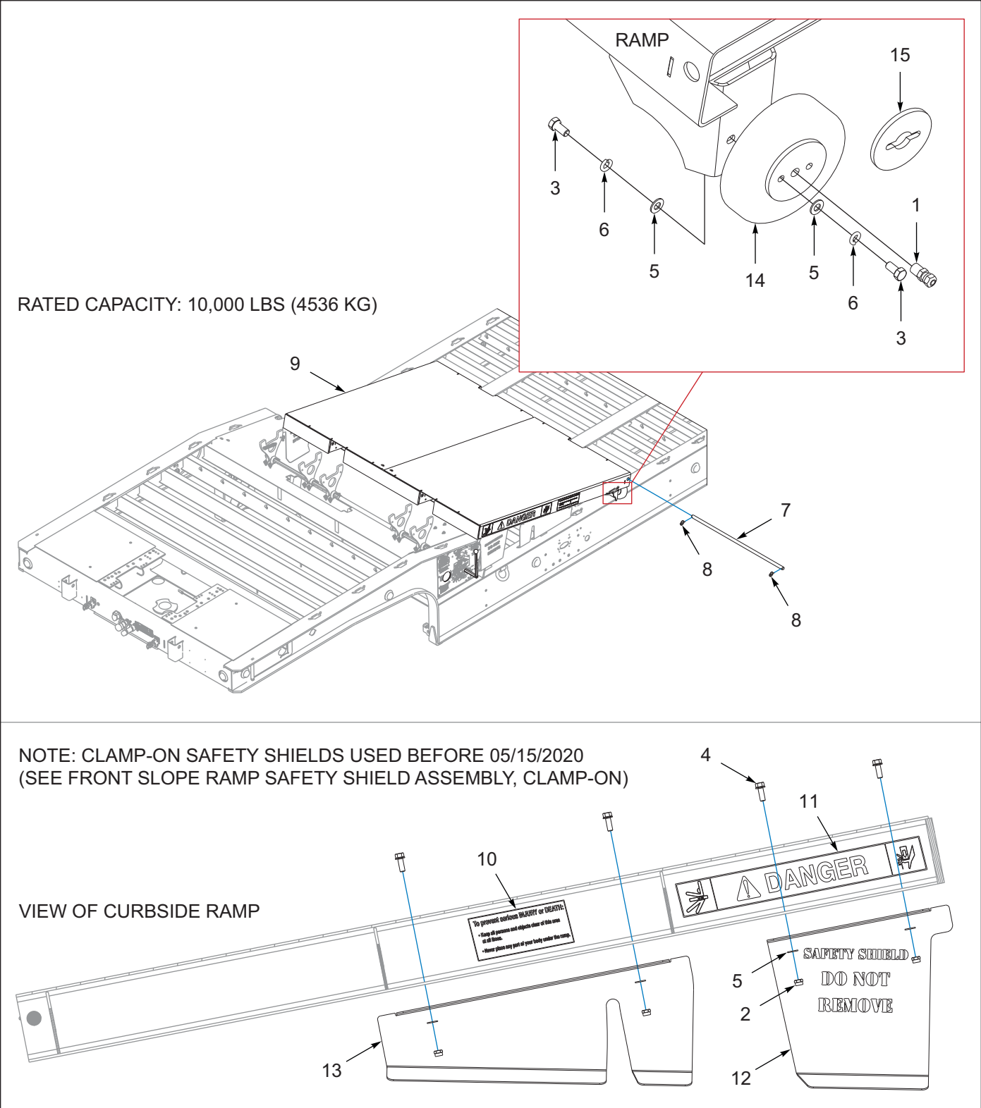
Figure 4-1: Front Slope, Deck Components (BEFORE 03/11/2021) (OPTION)
