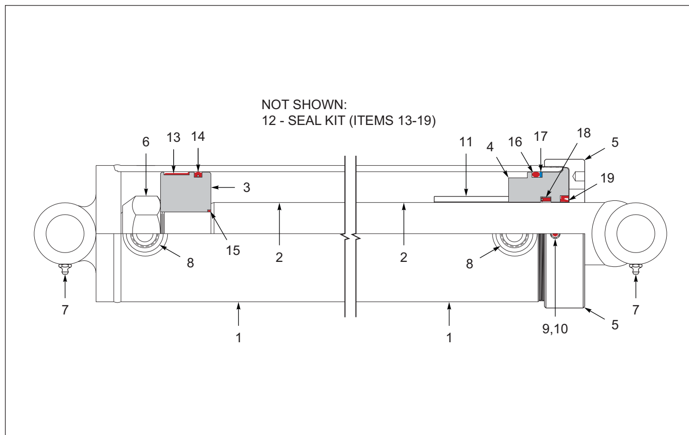
Figure 9-4: Cylinder Components, 5 x 60
