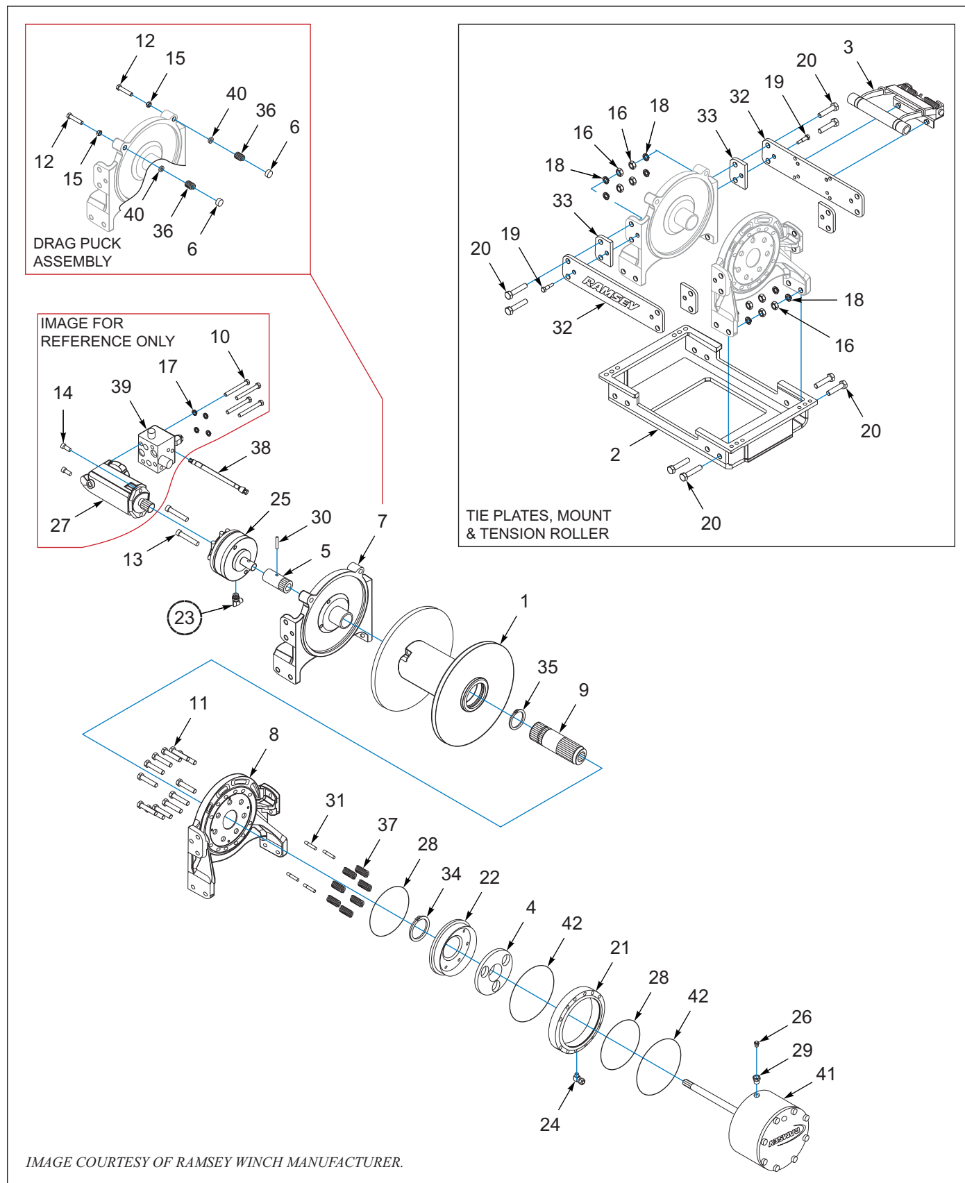
Figure 11-21: Winch Components, Ramsey 30K, 2 Speed (OPTION)
