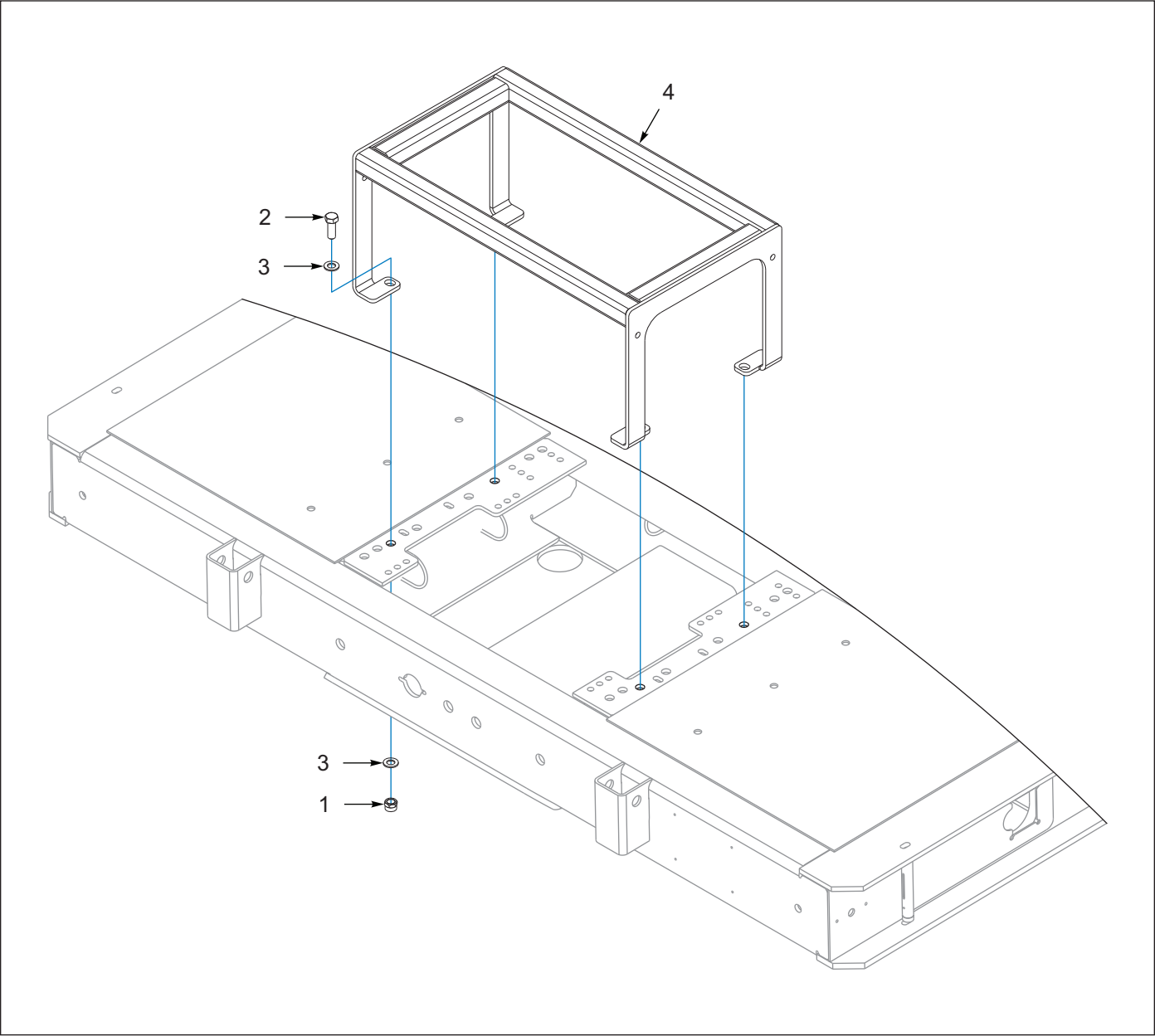
Figure 11-28: Guard, Winch W/ Cable Pivot Guide (OPTION)
