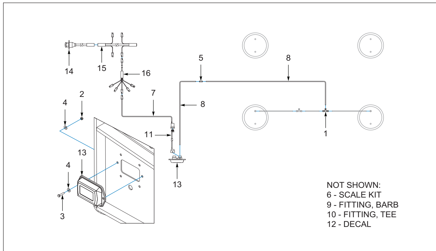
Figure 6-10: Scale, Quickload & Loadmaxx (AFTER 03/31/2020) (OPTIONS)
