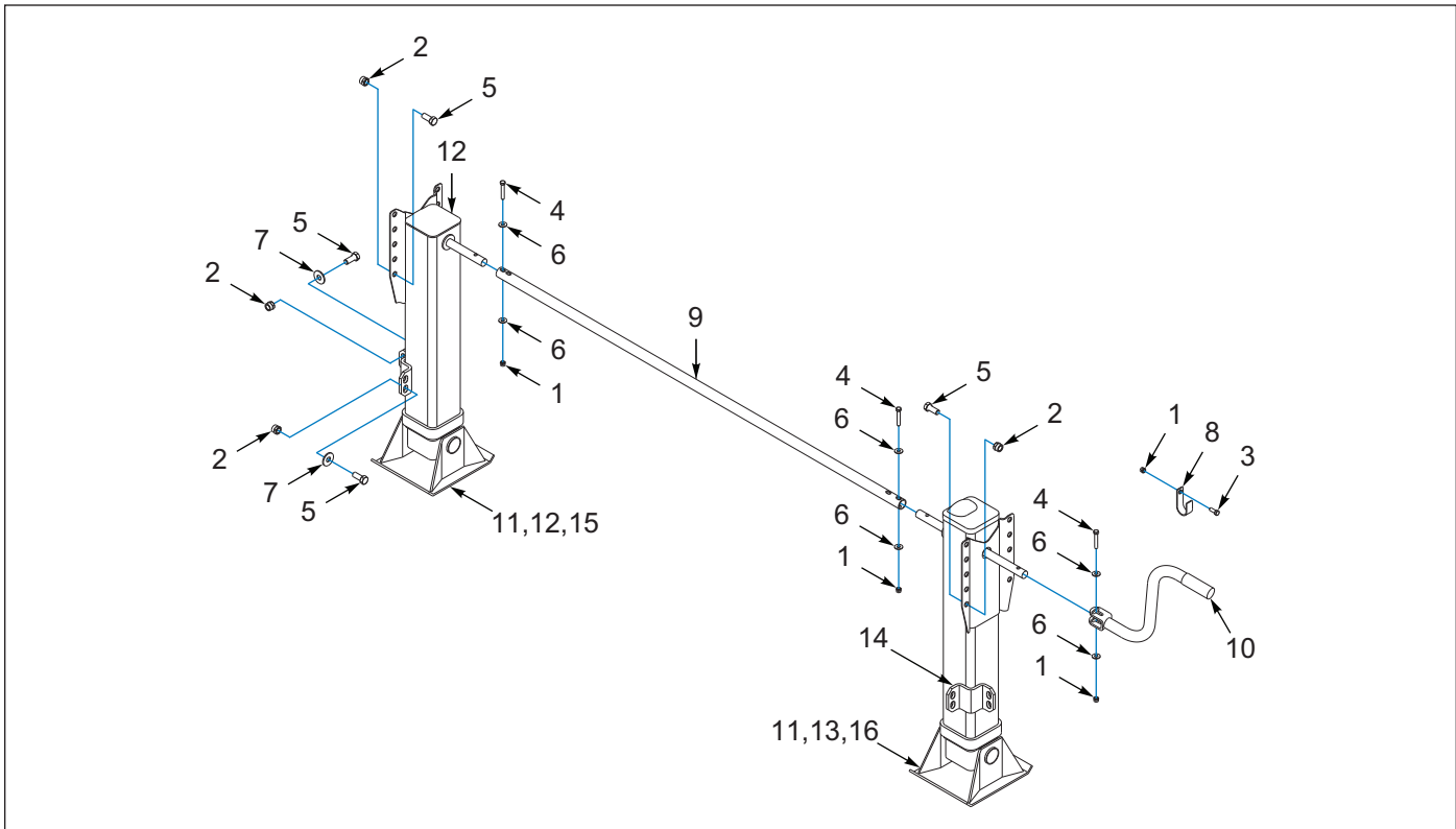
Figure 2-9: Landing Legs, Gear, 2 Spd, Flip Crank, Front Interior Low Mt Bkt
