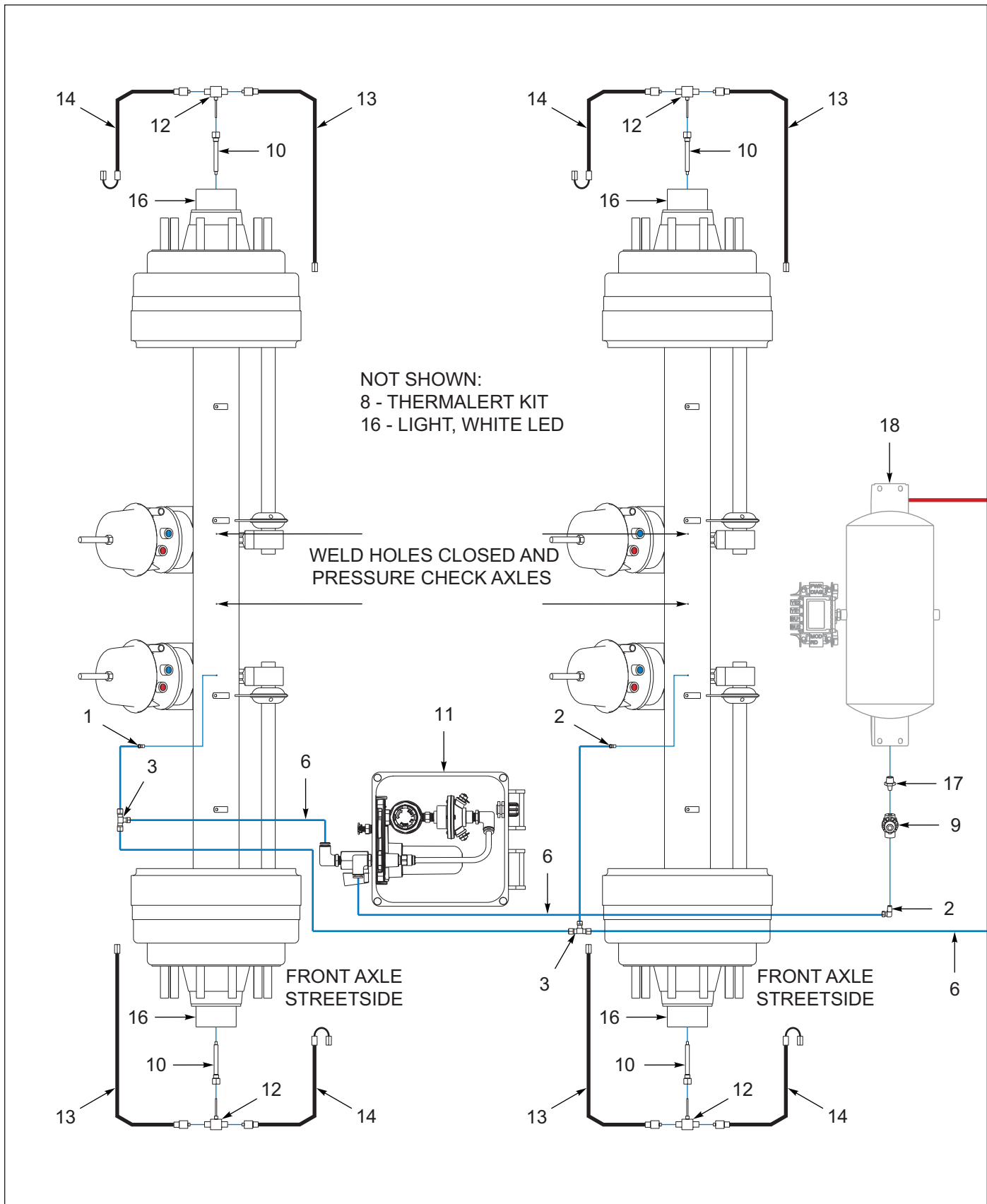
Figure 6-21: Tire Inflation, 3 Axle (OPTION) (1 of 2)
