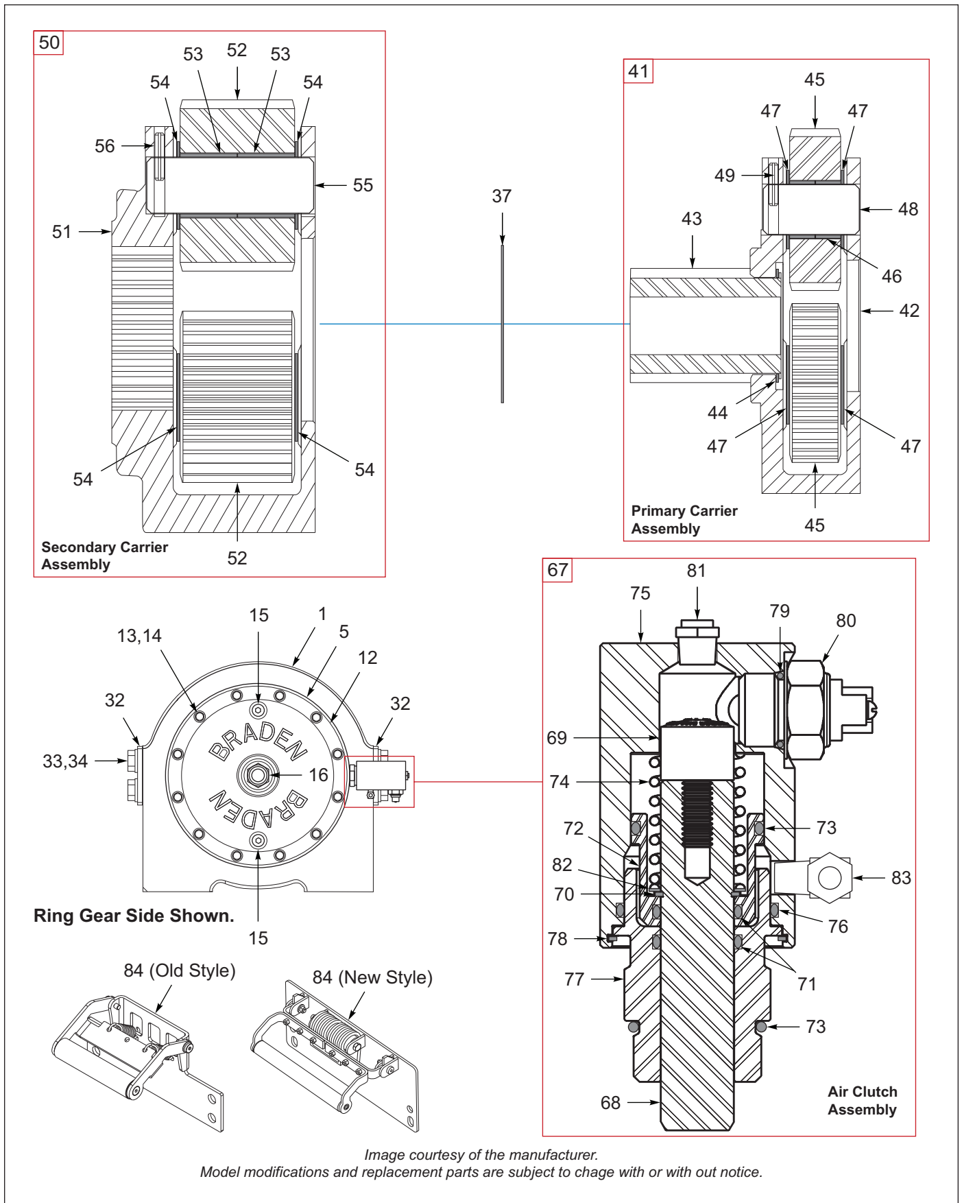
Figure 11-19: Winch Components, Braden 30K, 2 Speed (OPTION) (2 of 2)
