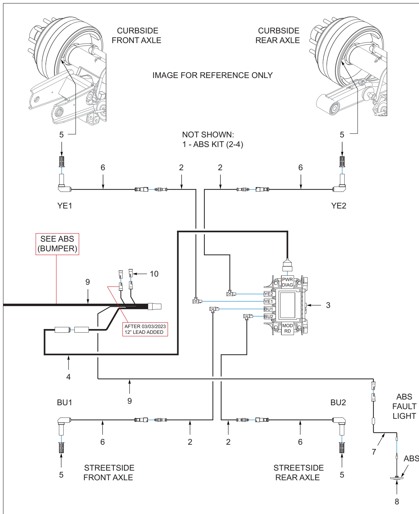
Figure 7-9: Anti-Lock Brakes, Wabco (1 of 2)
