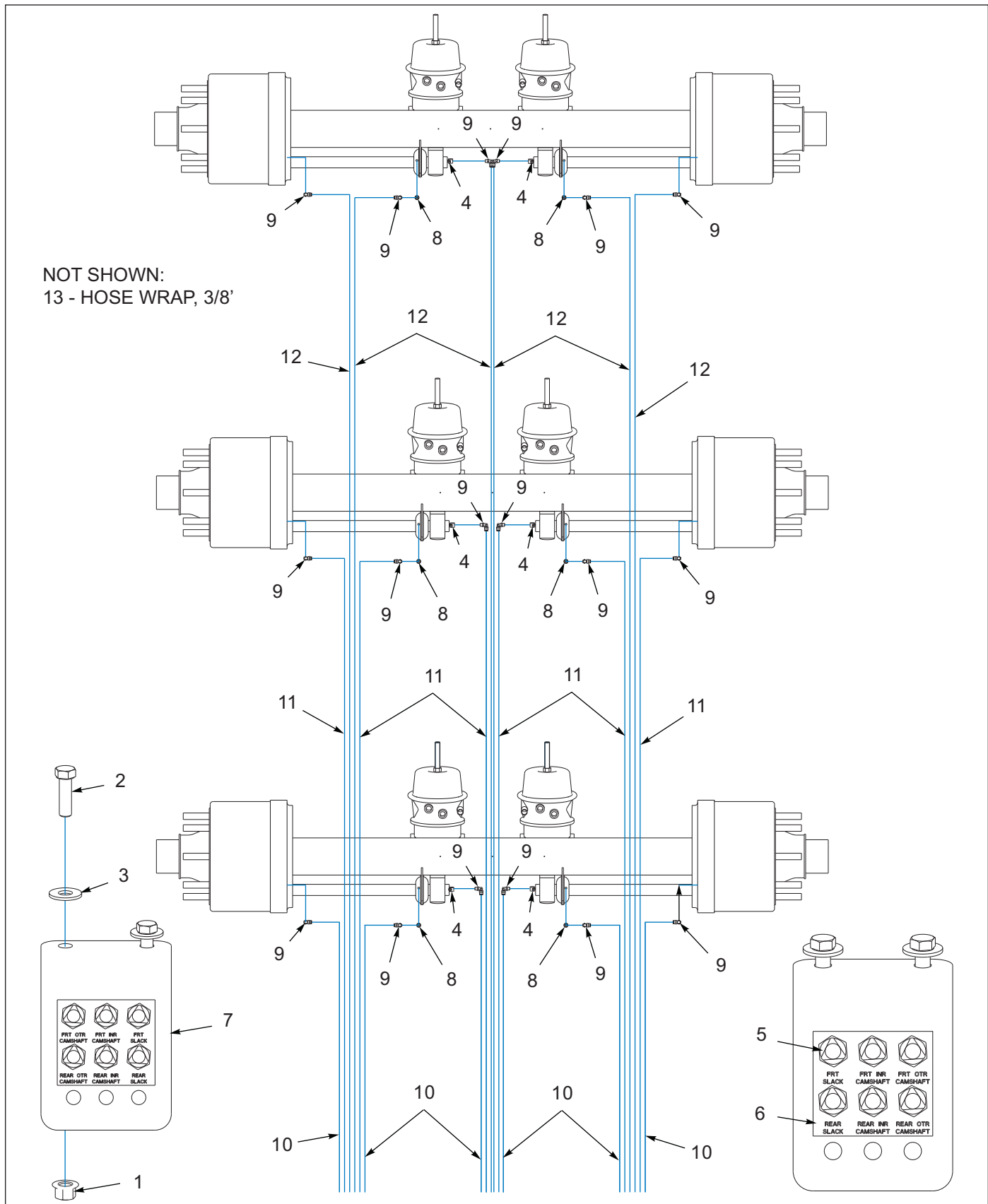
Figure 8-6: Drum Brakes, 3 Axle (Before 11/07/2018)
