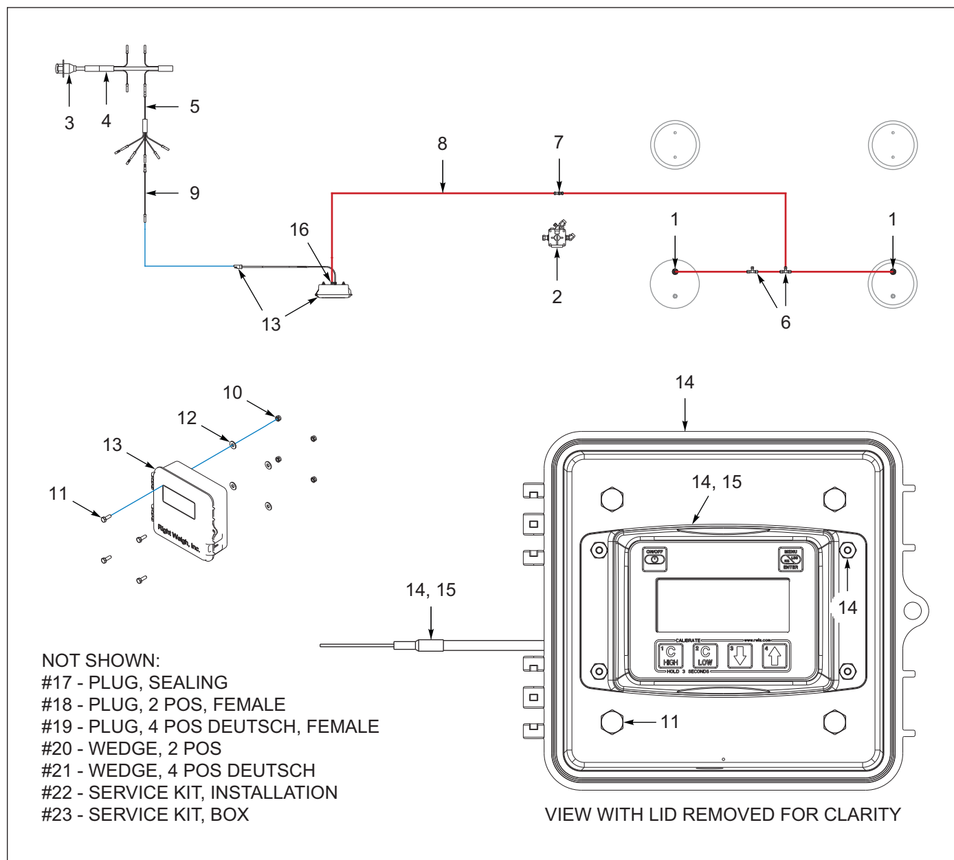
Figure 6-11: Scale, Right Weigh
