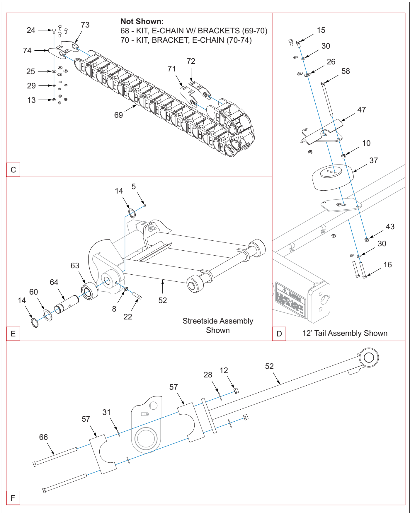
Figure 2-18: Undercarriage Components (2 of 3)
