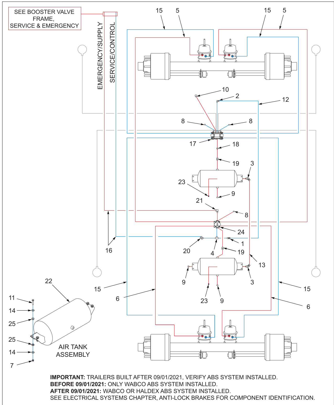
Figure 6-2: Anti-Lock Brakes, Service & Emergency, 2 Axle, Wabco
