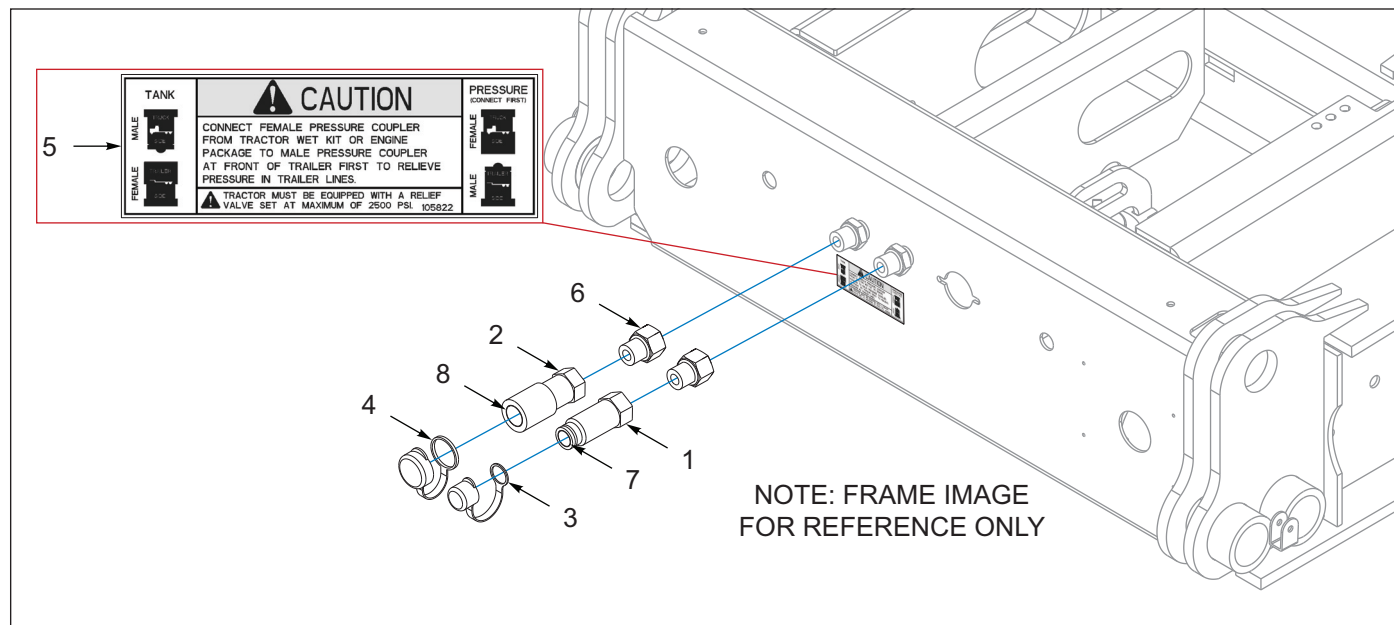
Figure 9-3: Couplers Kit, Hydraulic Conversion & Repair
