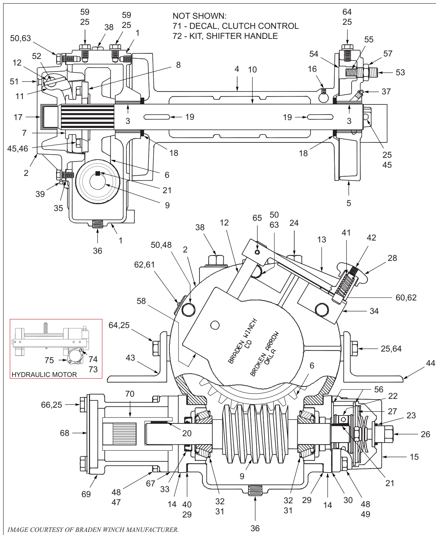
Figure 11-13: Winch Components, Braden 20K, 1 Speed (OPTION)
