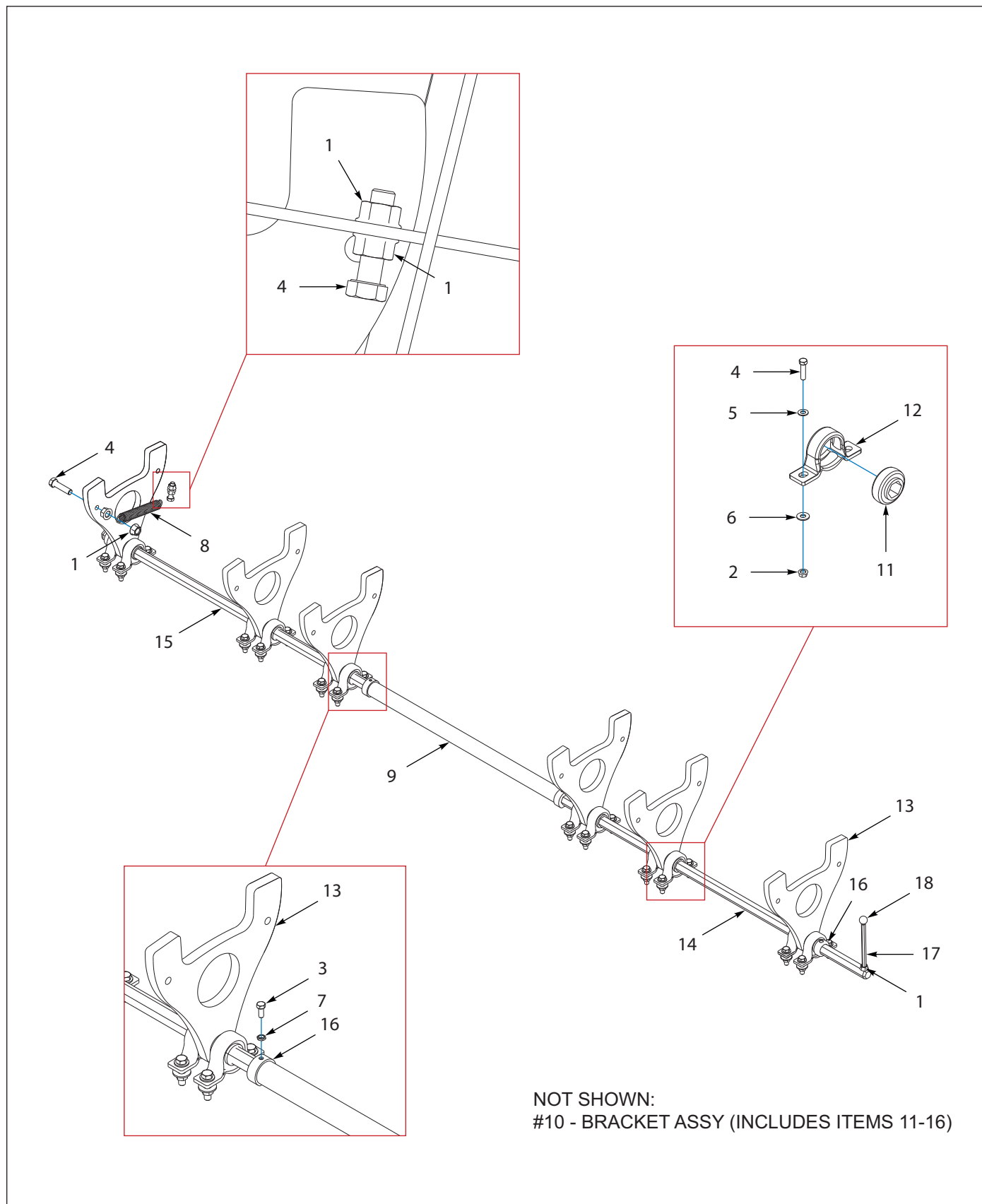
Figure 4-4: Front Slope, Support Components (BEFORE 03/11/2021) (OPTION)
