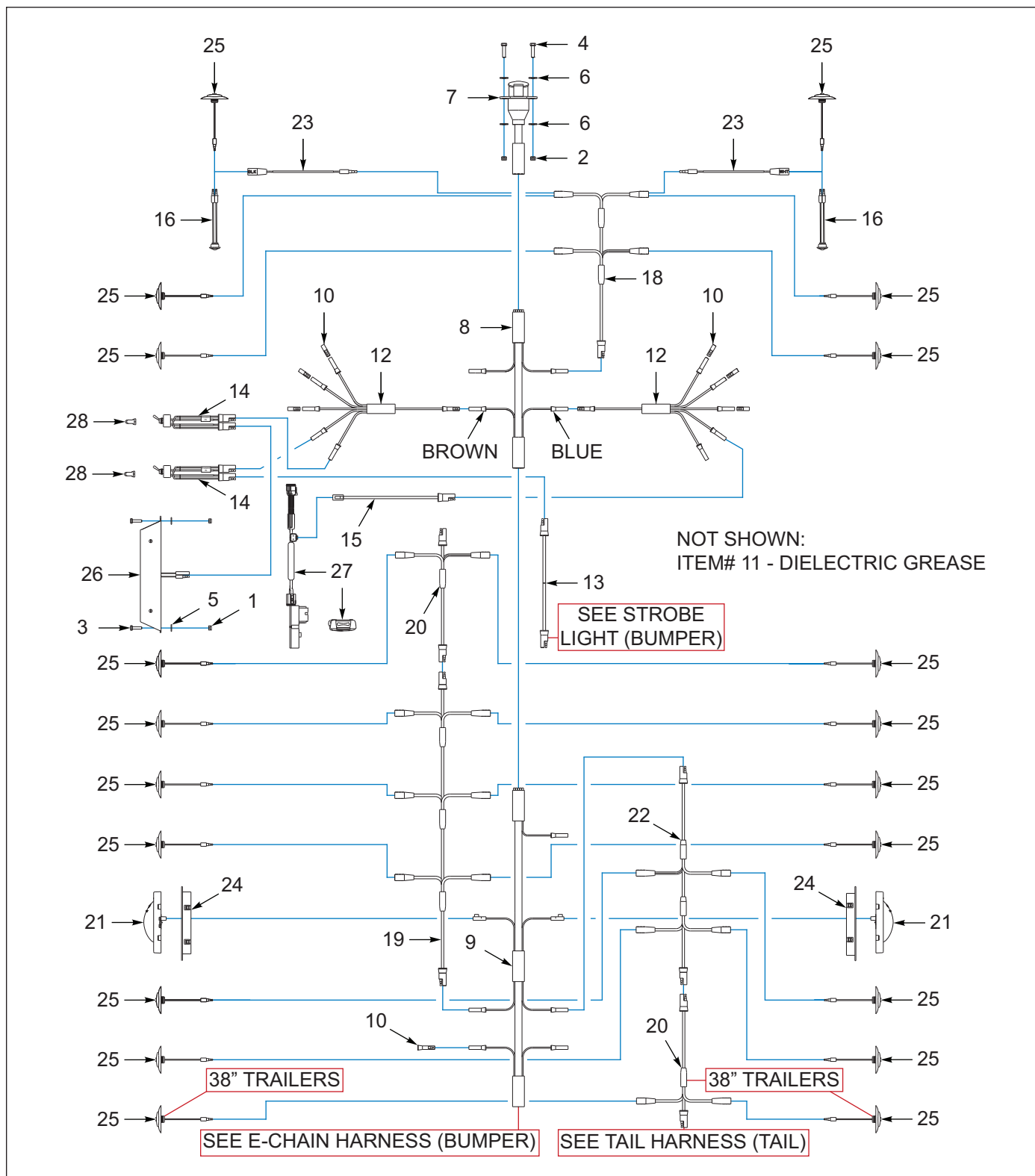
Figure 7-1: Trailer Assembly (BEFORE 02/15/2022) (1 of 2)
