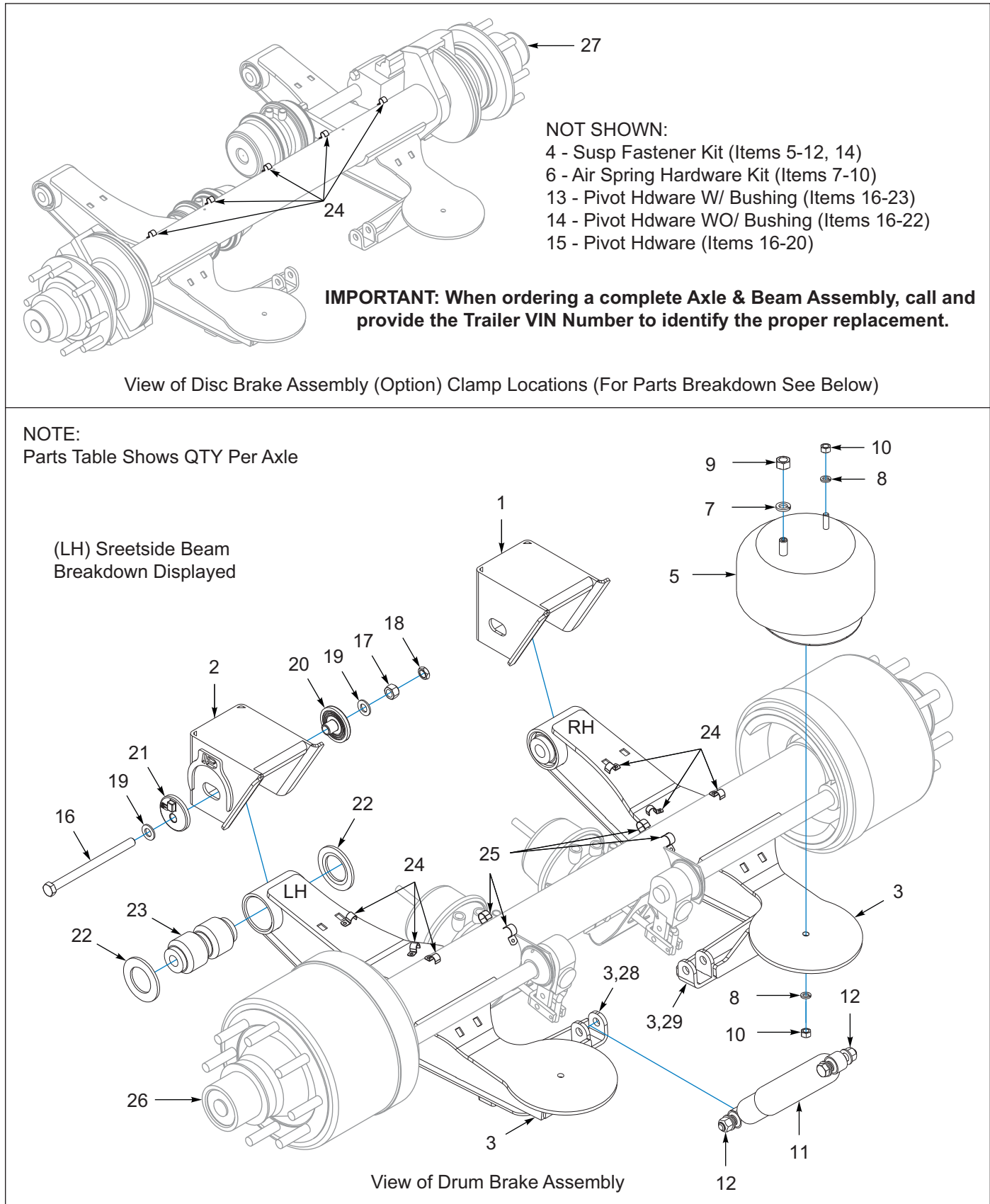
Figure 3-11: Axle Suspension, LSS-25K-3.5 RLU, 12.25
