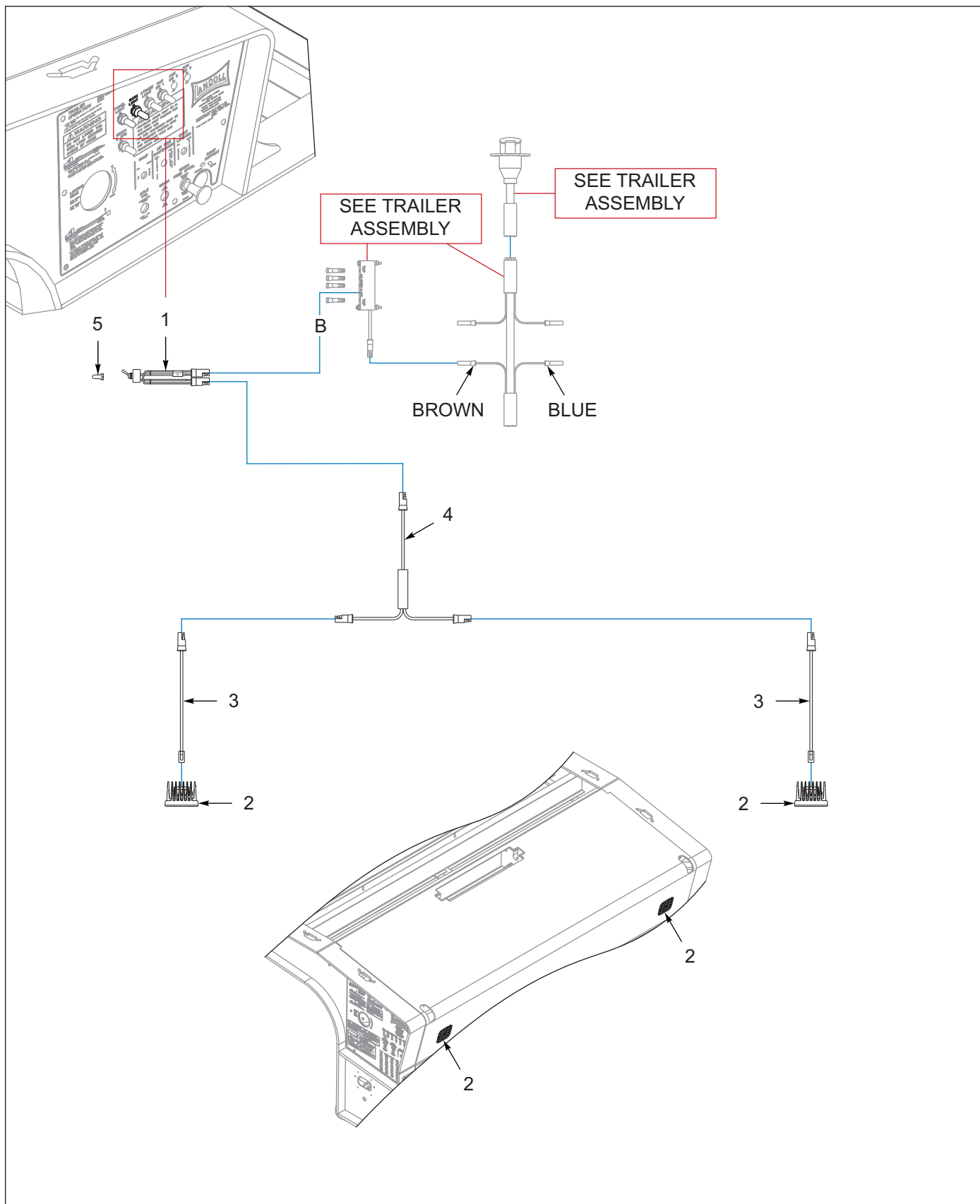
Figure 7-20: Upper Deck, Slope, Work Lights (OPTION)
