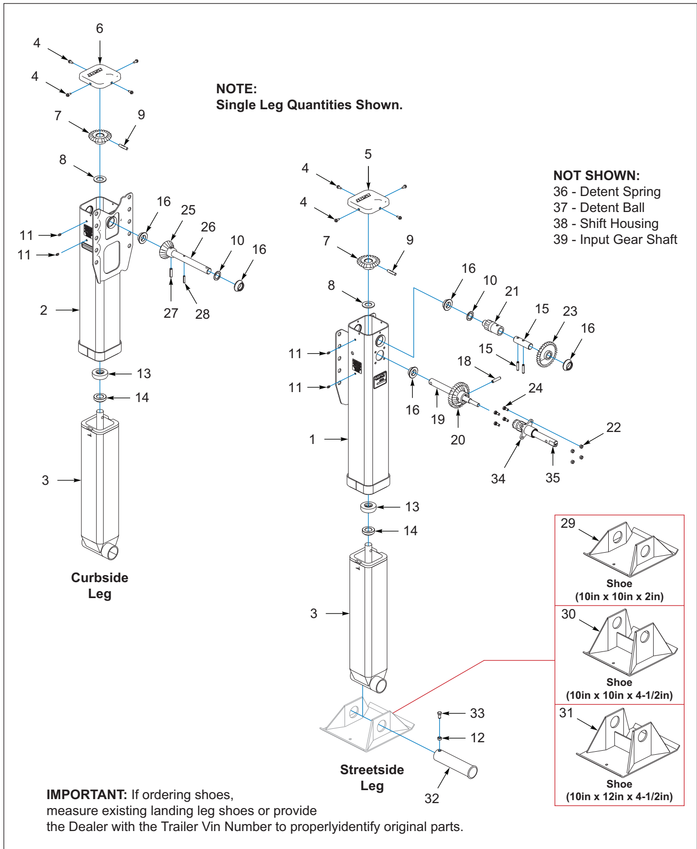
Figure 2-11: Landing Leg Components, Gear, 2 Spd
