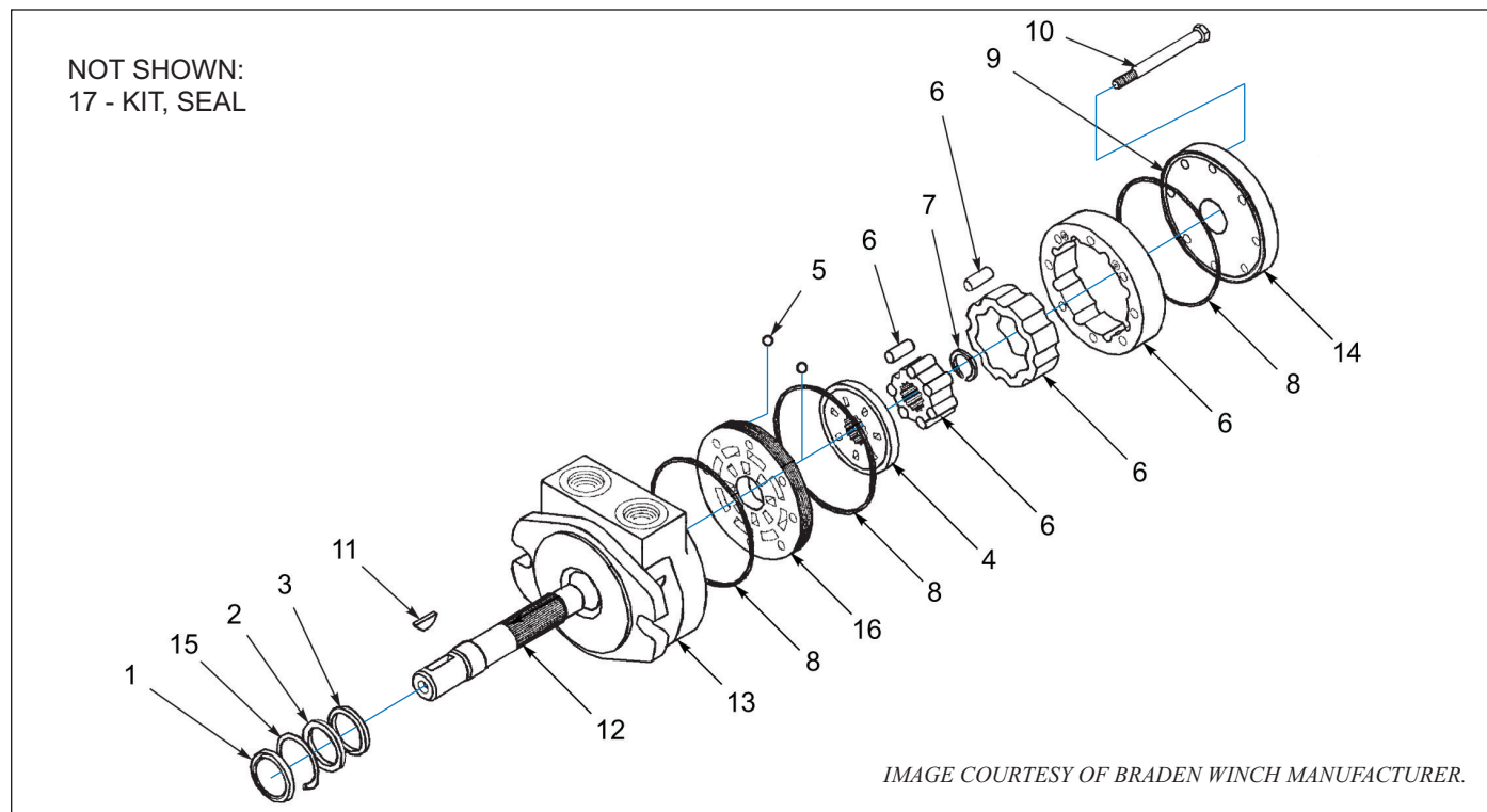
Figure 11-15: Winch Components, Braden 12K / 20K, 1 Speed, Motor (OPTION)
