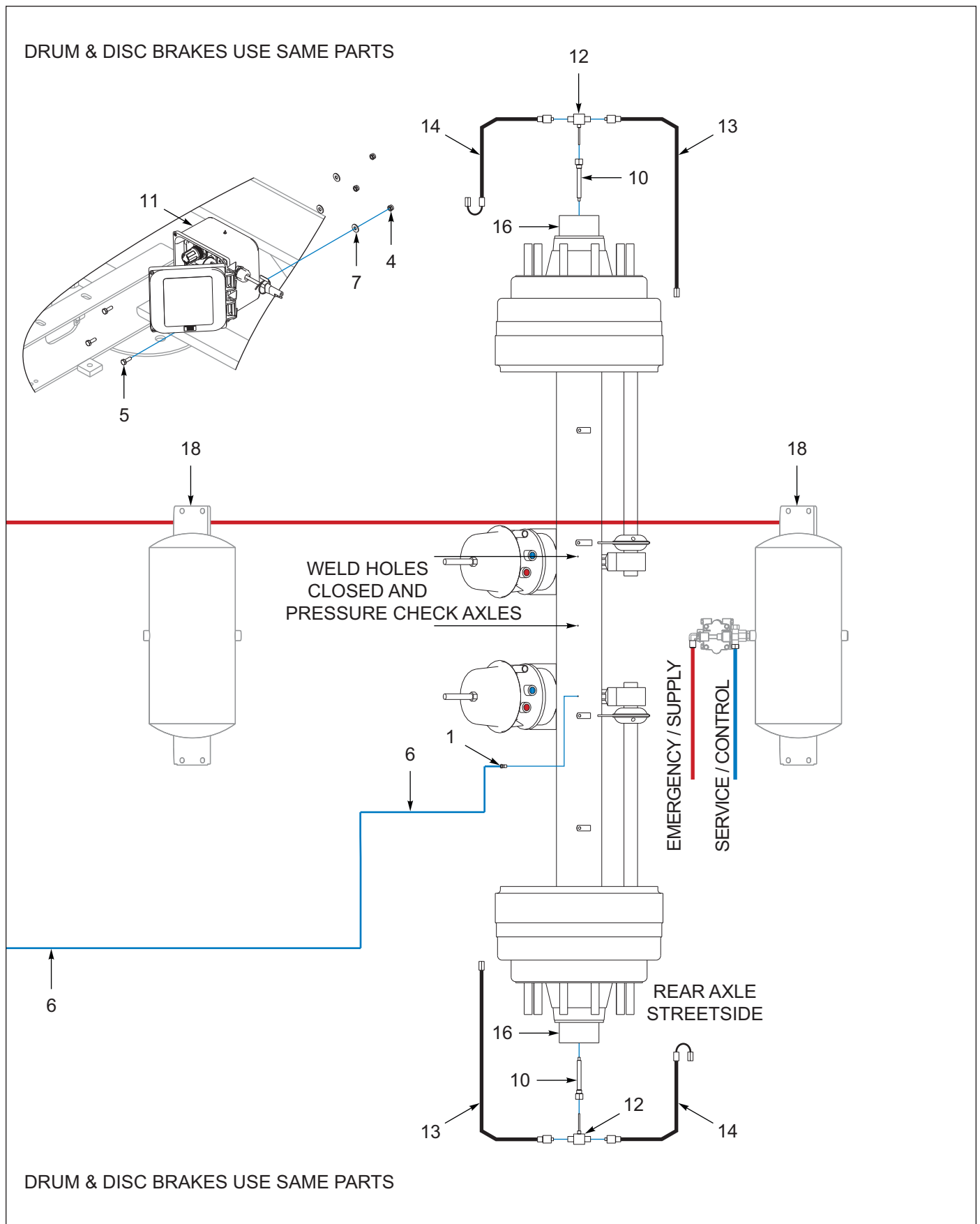
Figure 6-22: Tire Inflation, 3 Axle (OPTION) (2 of 2)
