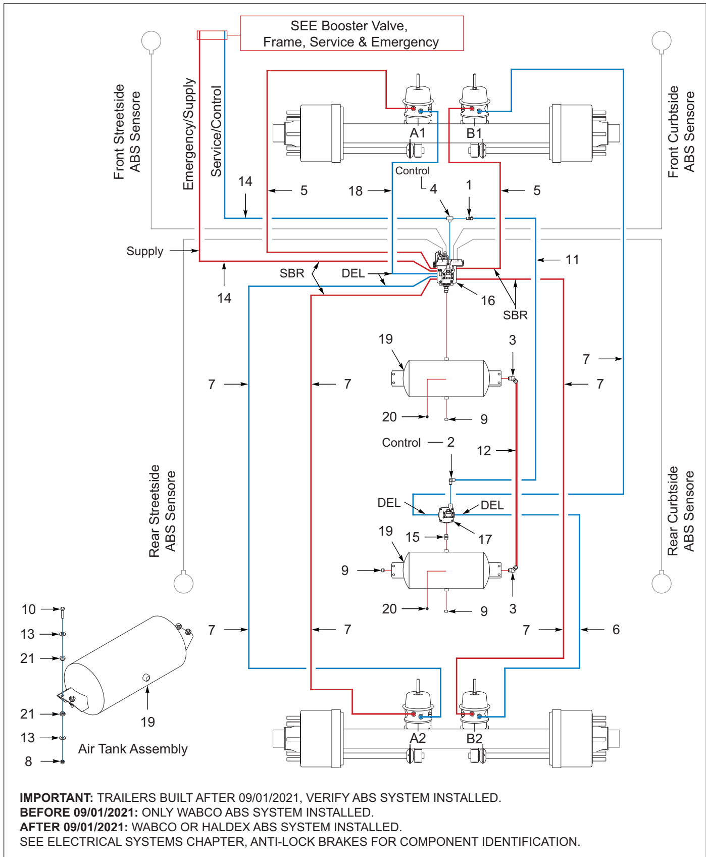
Figure 6-3: Anti-Lock Brakes, Service & Emergency, 2 Axle, Haldex
