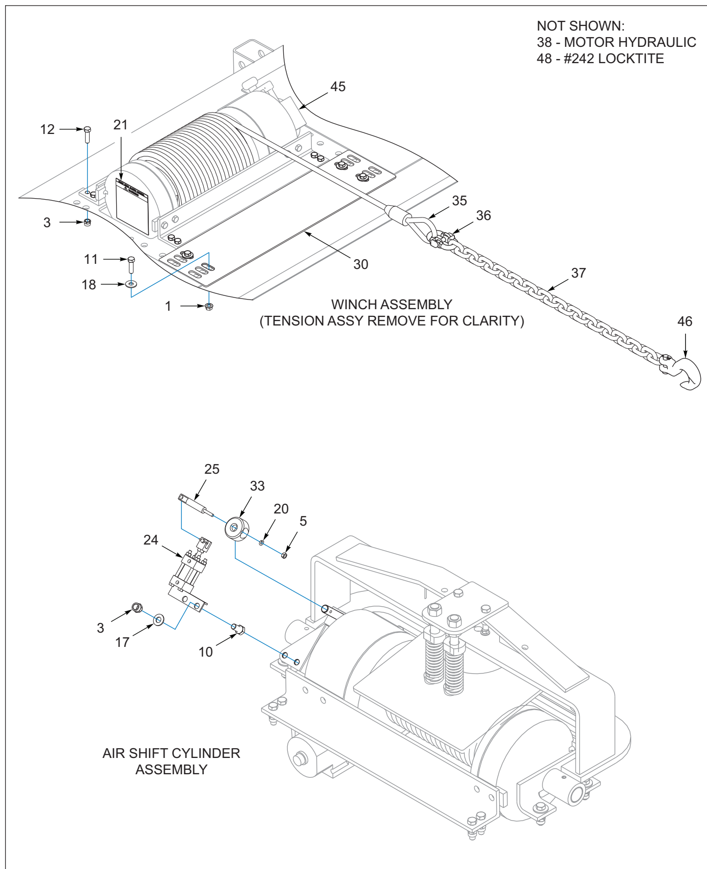
Figure 11-3: Winch Install, Braden 20K, 1 Speed, Air Tension (OPTION) (1 of 2)
