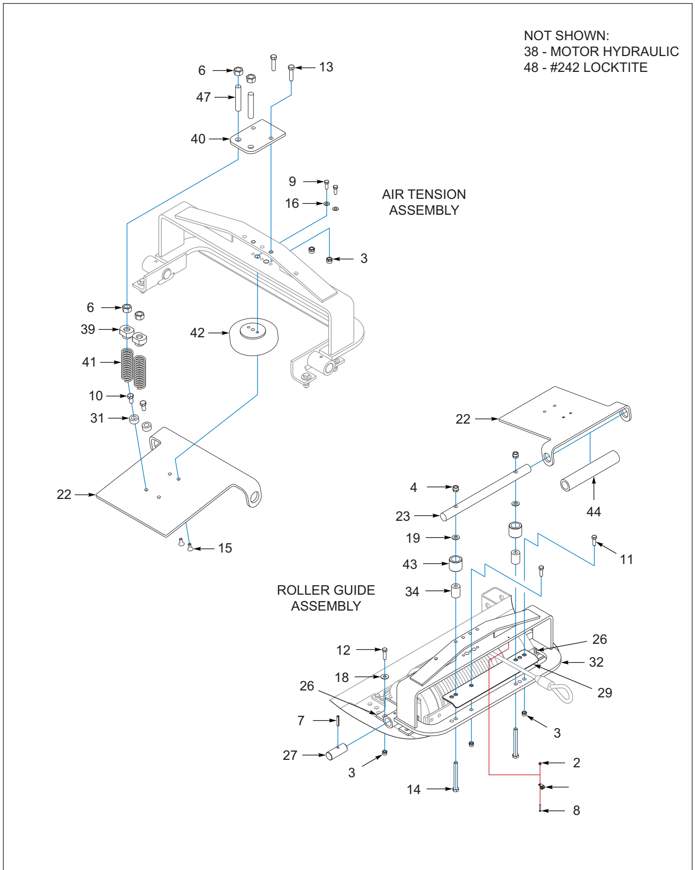
Figure 11-4: Winch Install, Braden 20K, 1 Speed, Air Tension (OPTION) (2 of 2)
