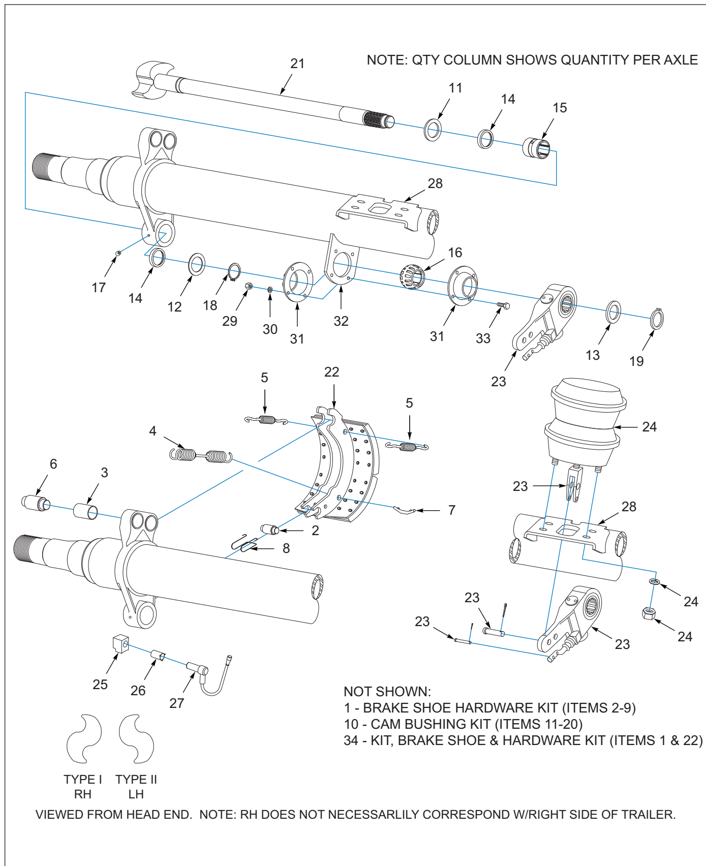
Figure 3-5: Axle 16.5 x 7 Drum Brake Components
