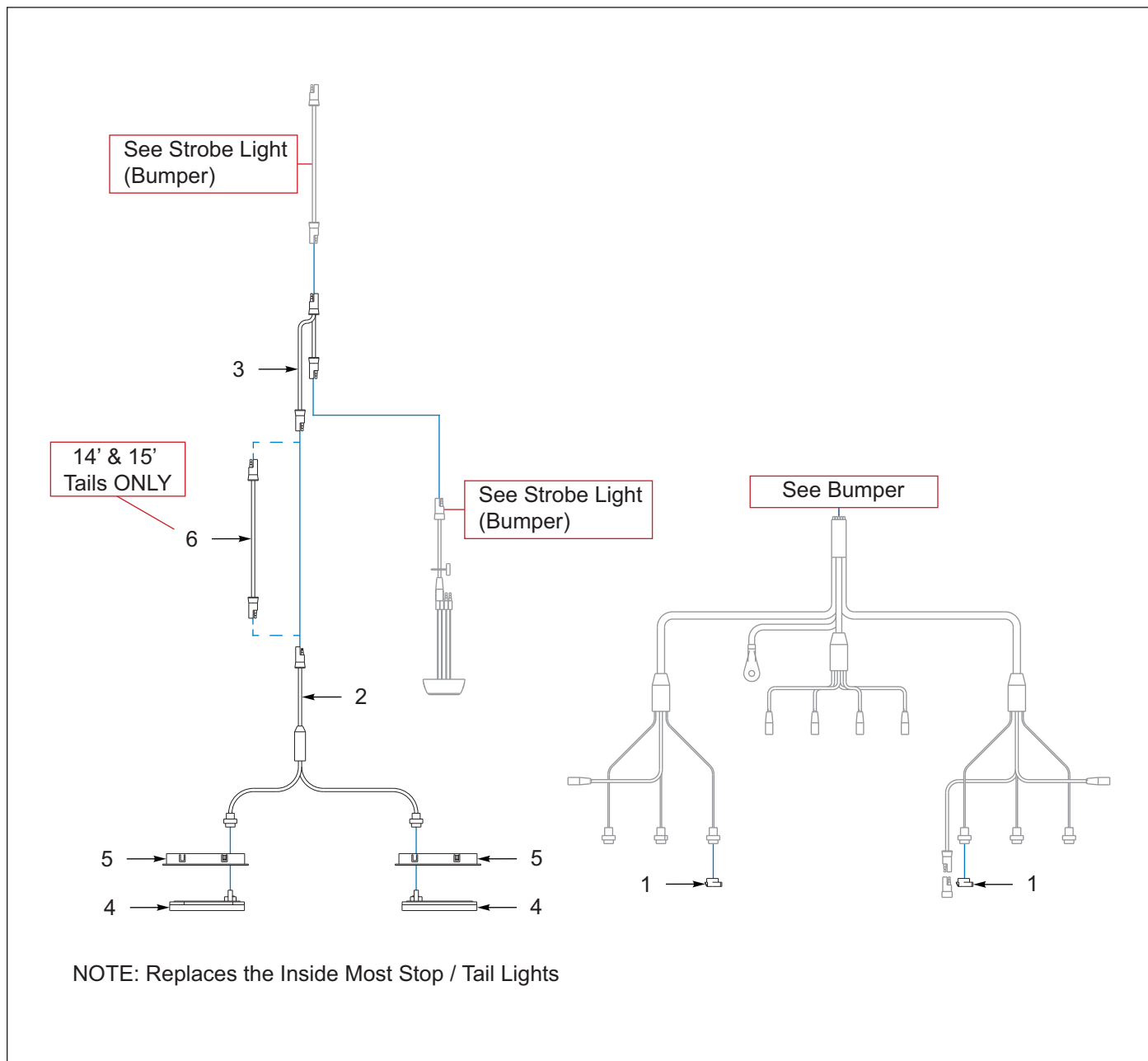
Figure 7-8: Bumper, Strobe Lights (OPTION)
