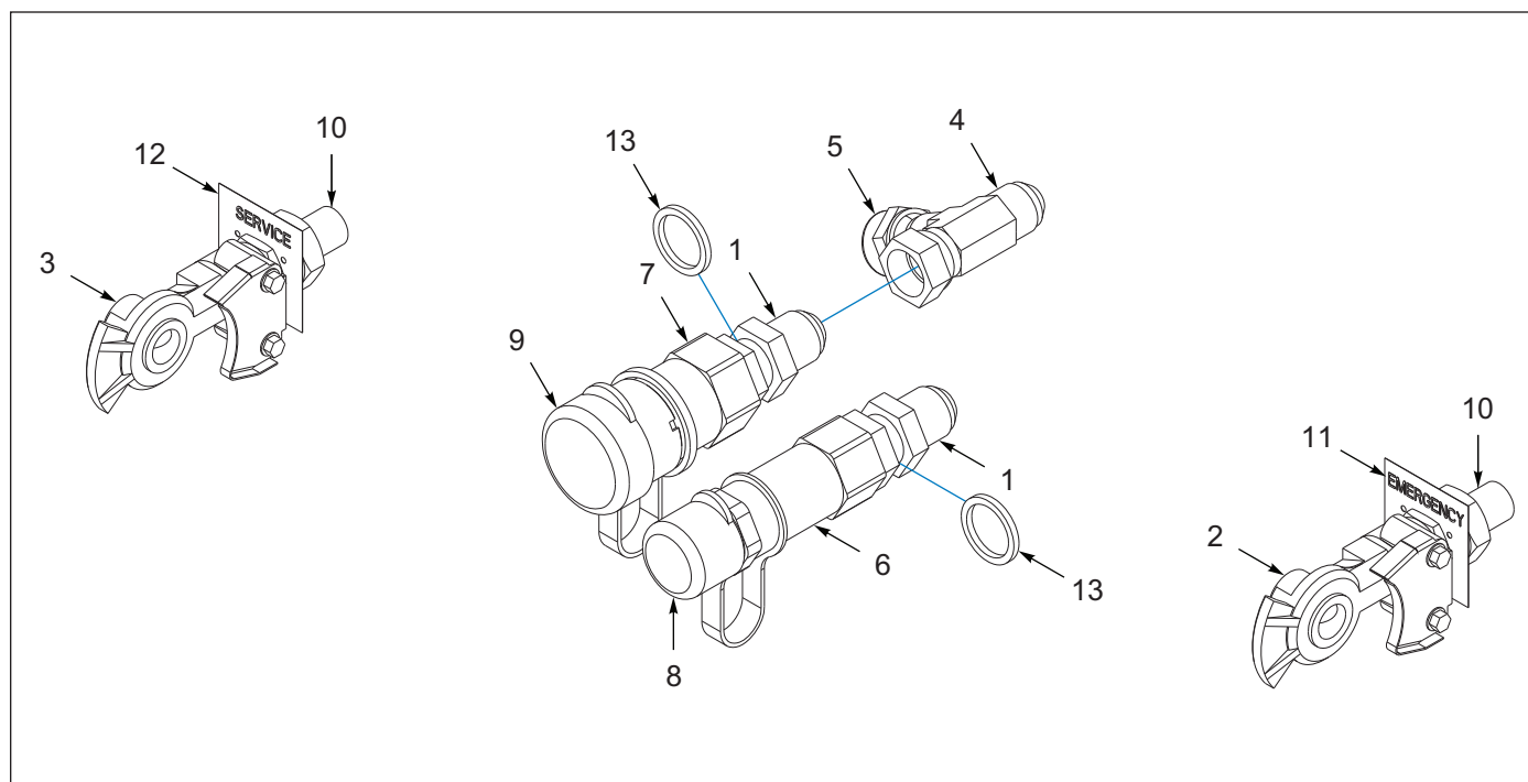
Figure 9-2: Connectors Kit, Front Sub-Assembly
