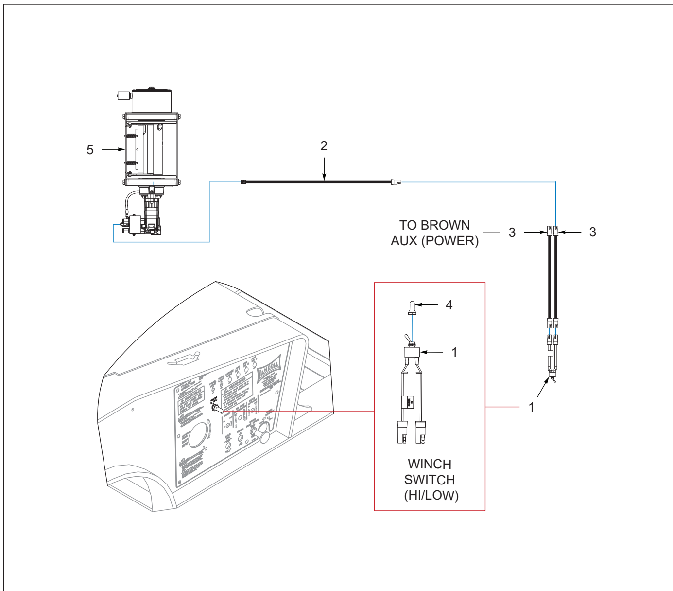
Figure 7-21: Winch Install, Braden 20K / 30K, 2 Speed (OPTION)
