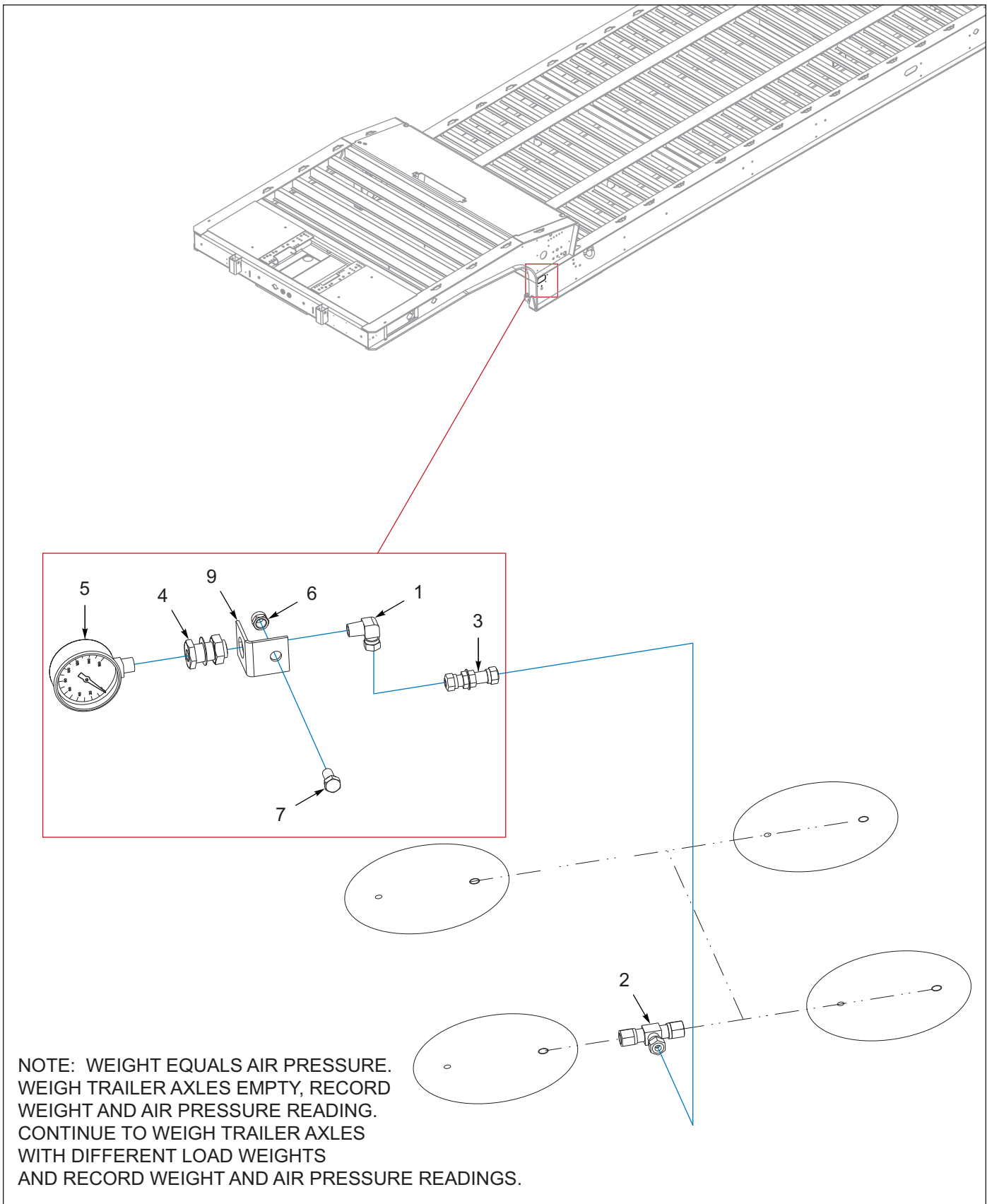
Figure 6-8: Scale, Air Pressure Gauge Assembly (OPTION)
