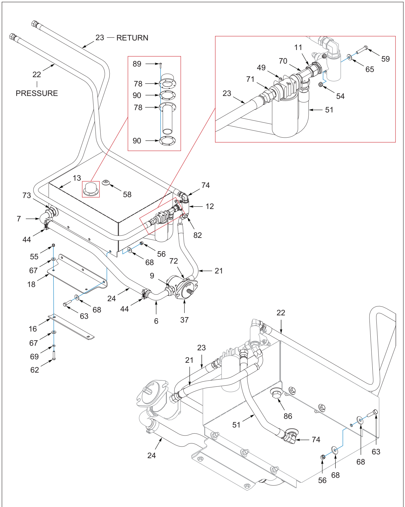
Figure 10-9: Engine, 25HP, Slope Deck Assembly (OPTION) (4 of 4)
