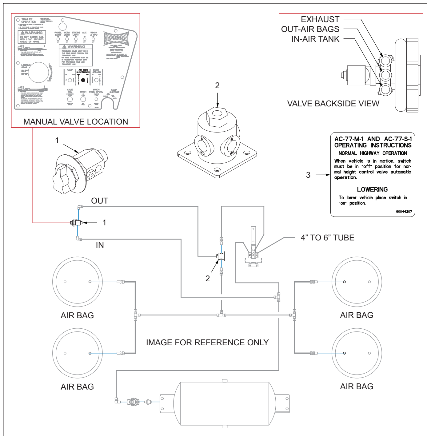
Figure 6-18: Suspension Lowering Air Control, Kit
