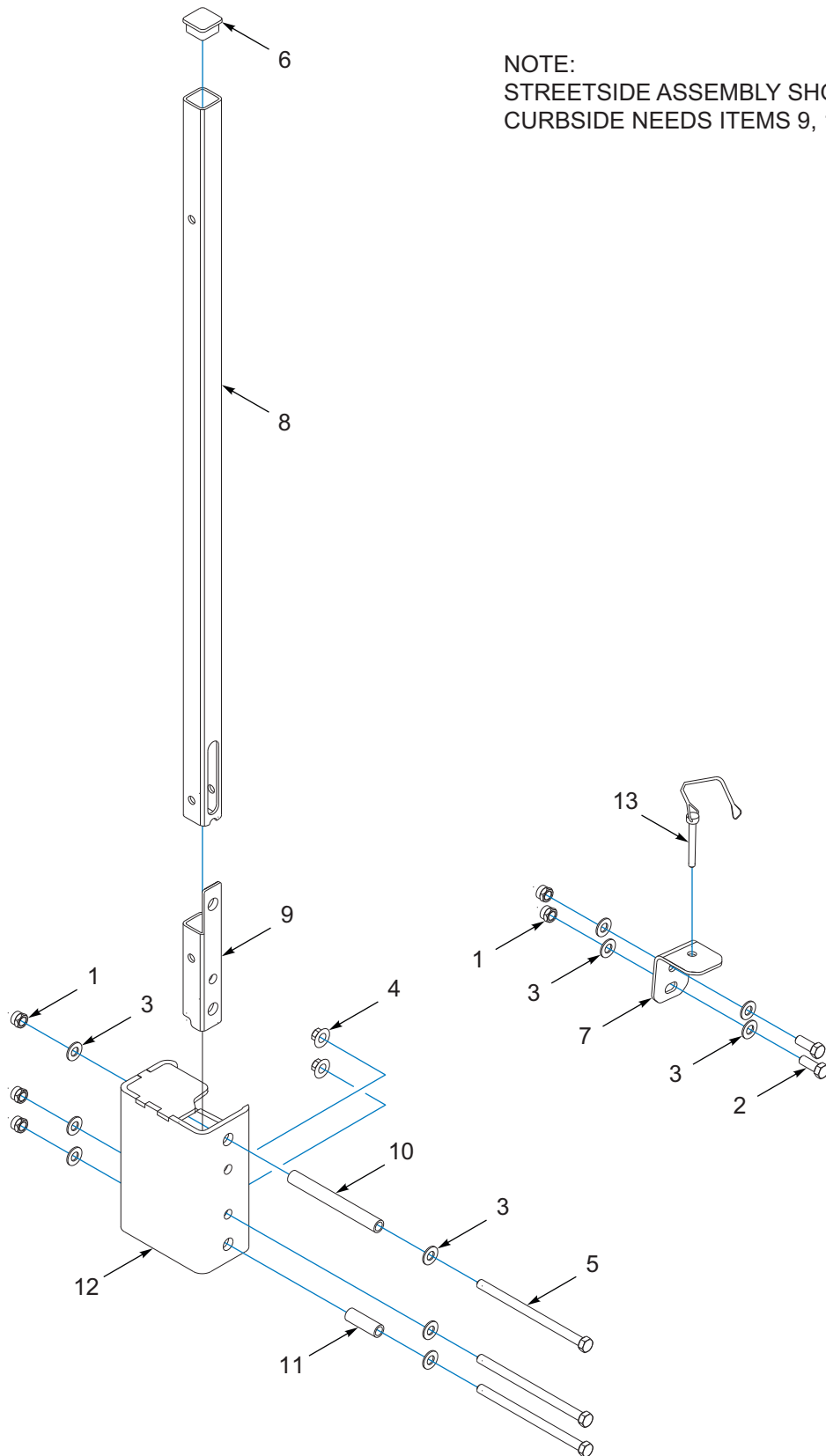
Figure 5-6: Step, Folding Handle Assembly (OPTIONS)
