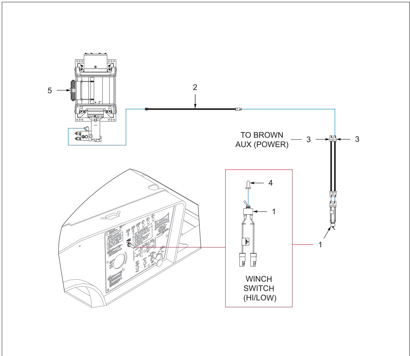
Figure 7-22: Winch Install, Ramsey 20K / 30K, 2 Speed (OPTION)
