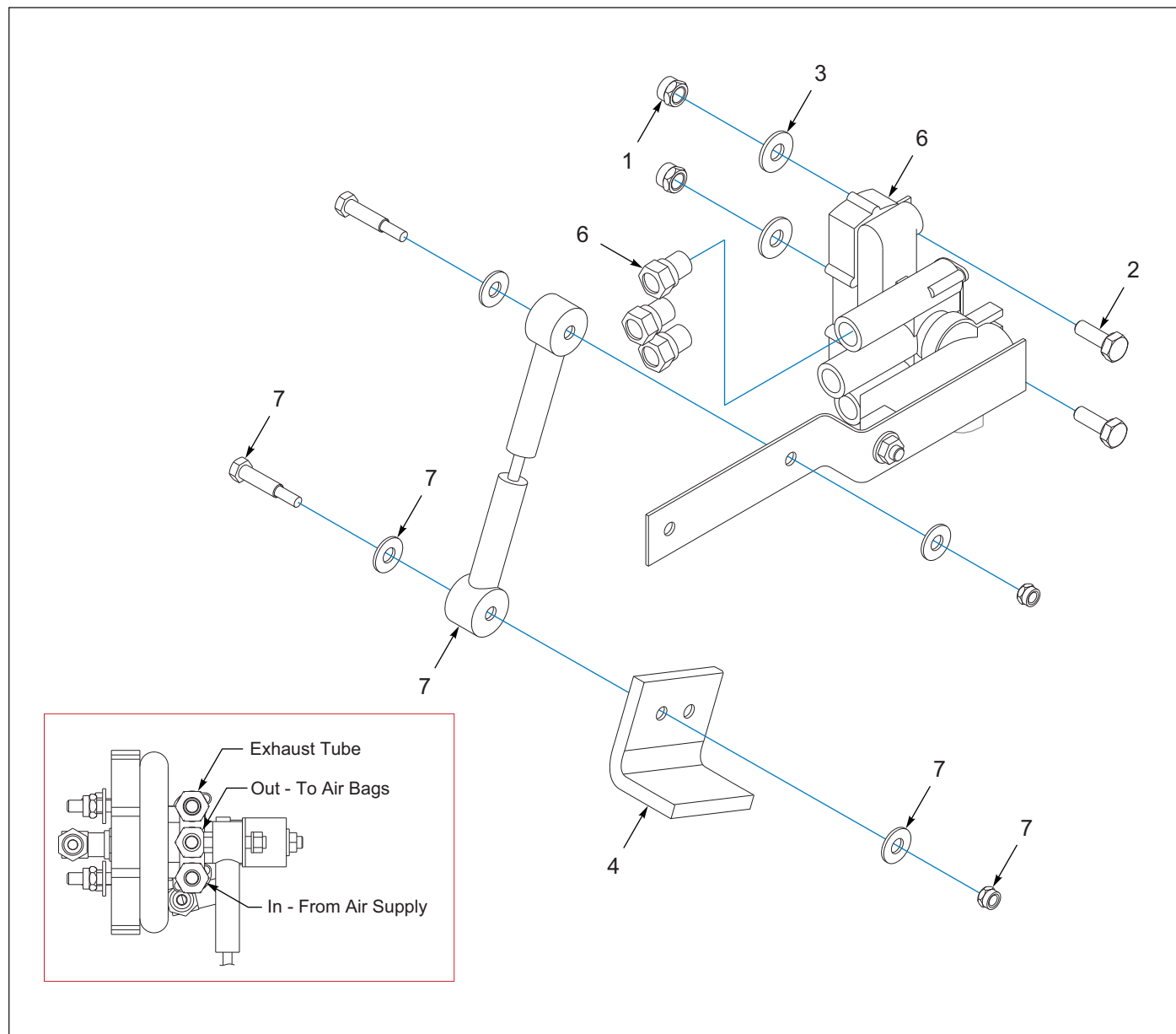
Figure 6-17: Suspension Air Control, Kit, Haldex
