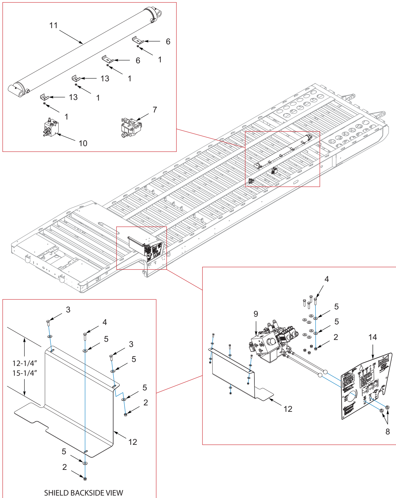
Figure 2-4: Frame Assembly, Components, Air & Hydraulic
