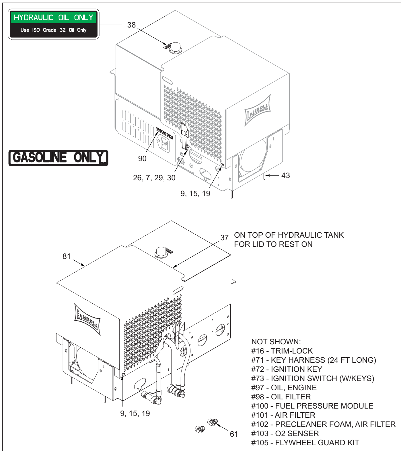
Figure 10-1: Engine, 25HP, Upper Deck Assembly (OPTION) (1 of 5)
