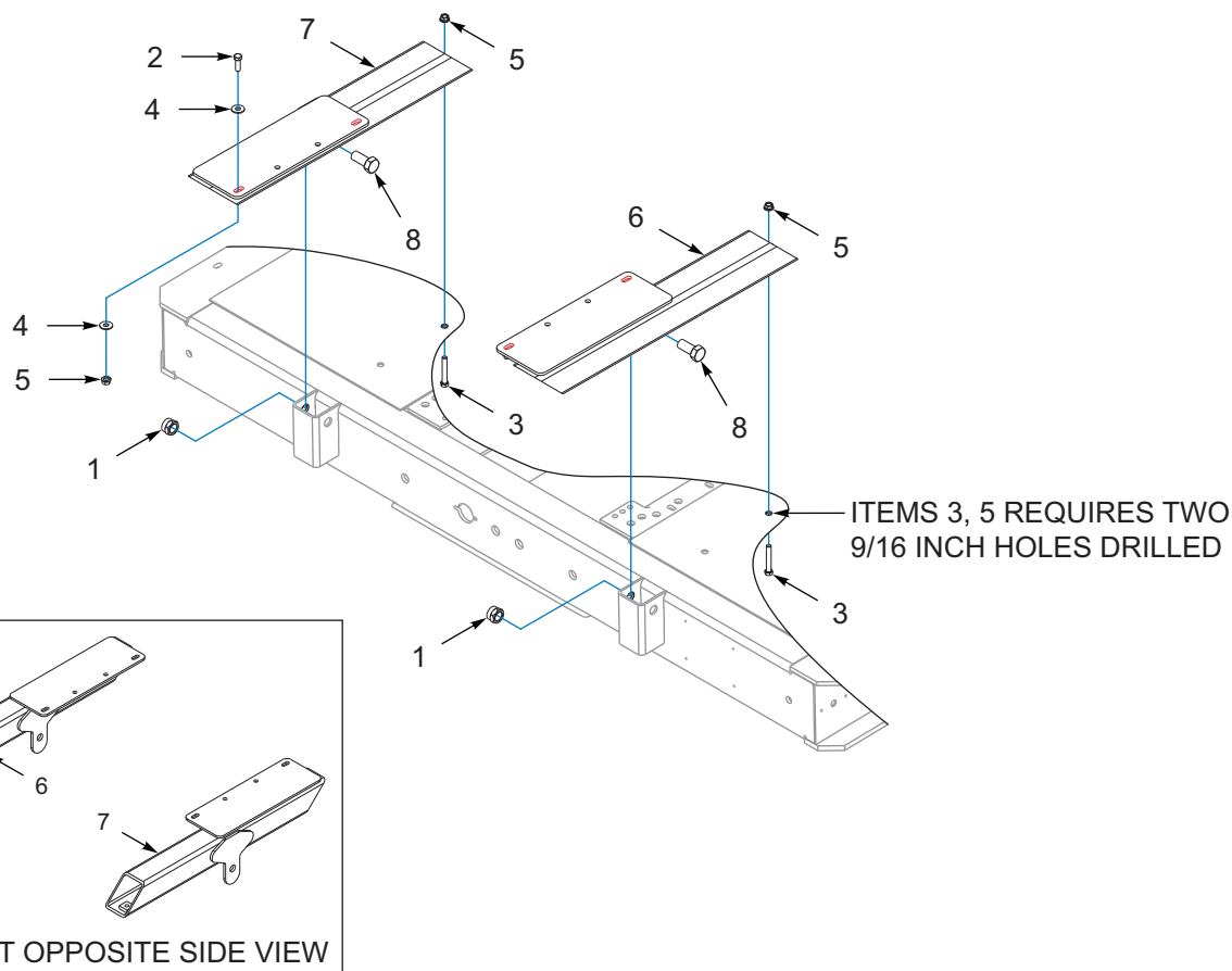
Figure 10-11: Mount, Front, Extension, Bolt-On (OPTION)
