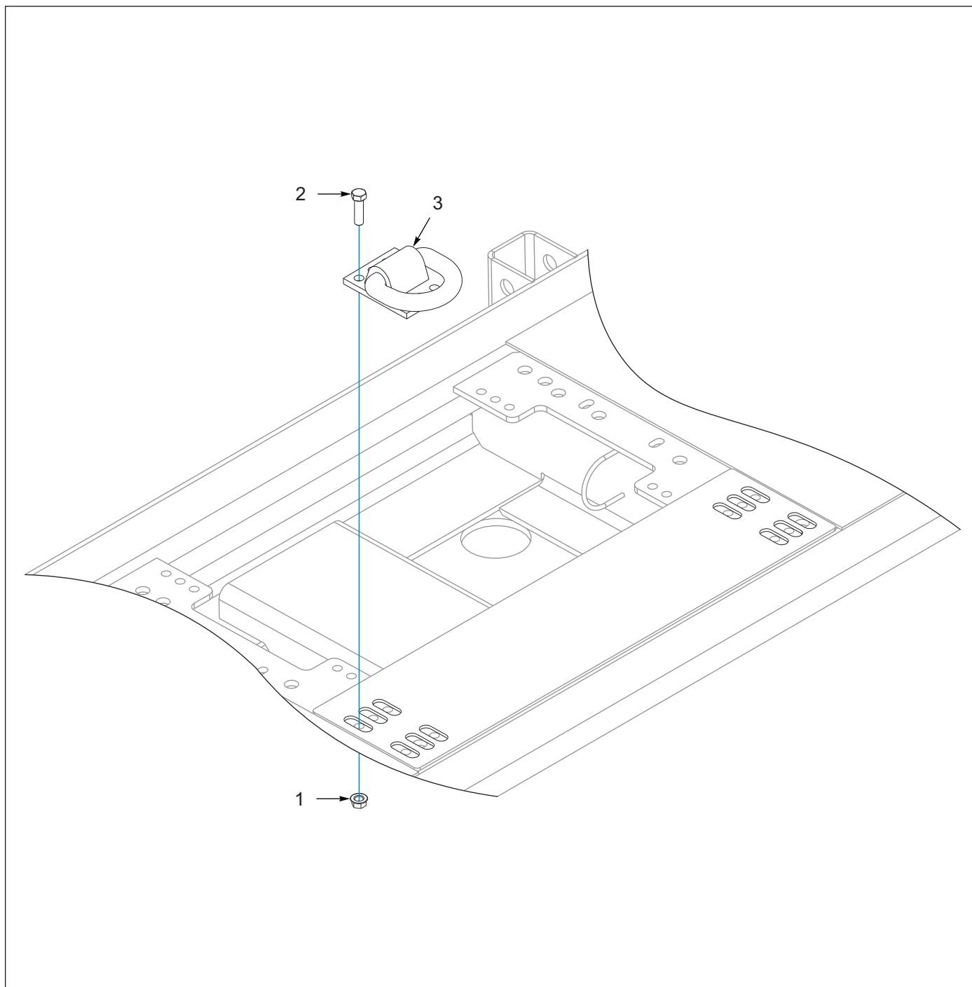
Figure 5-9: Tie Down, D-Ring, Bolt-On, Winch (OPTION)
