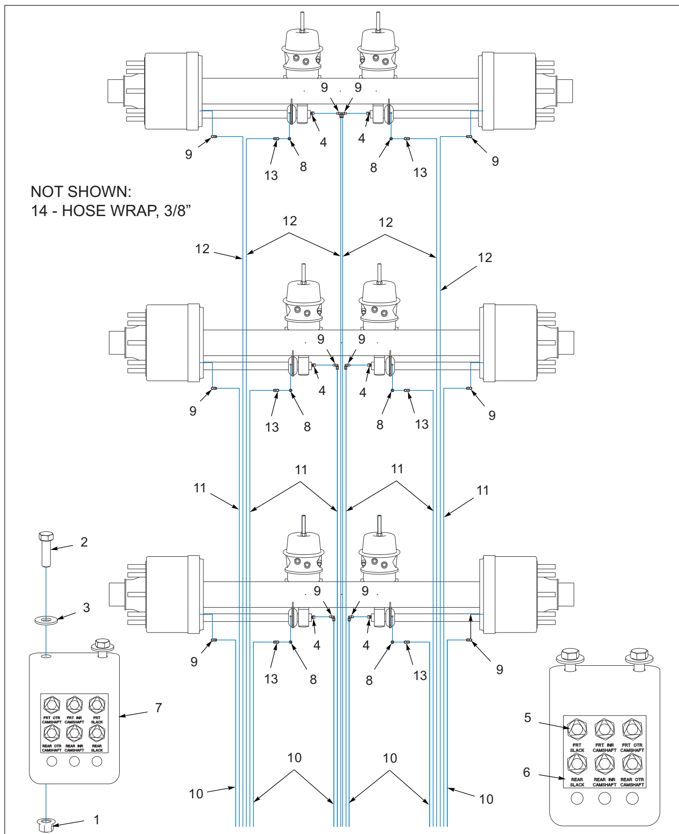
Figure 8-7: Drum Brakes, 3 Axle (After 11/07/2018 - Before 08/31/2020)
