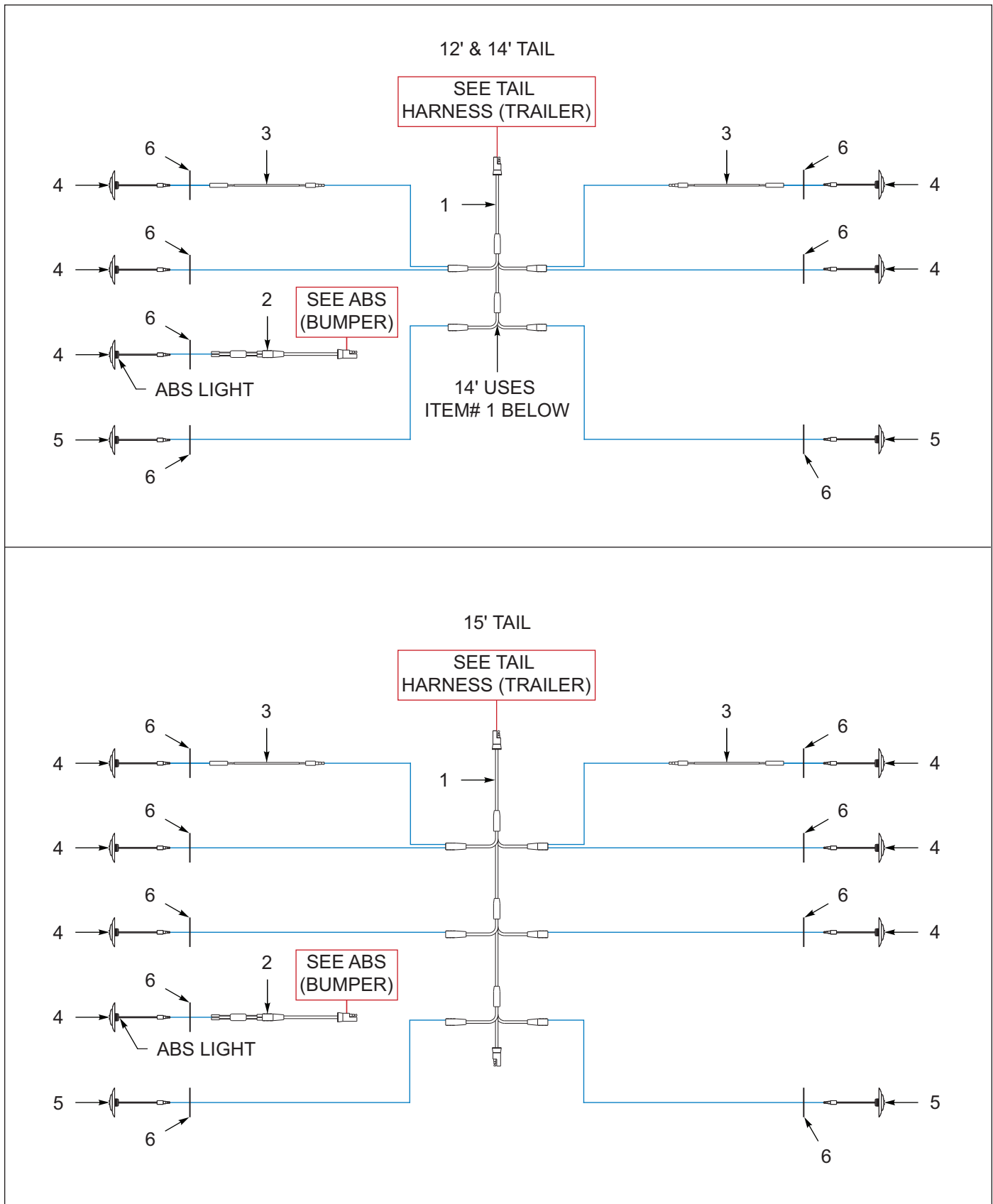
Figure 7-5: Tail Assembly
