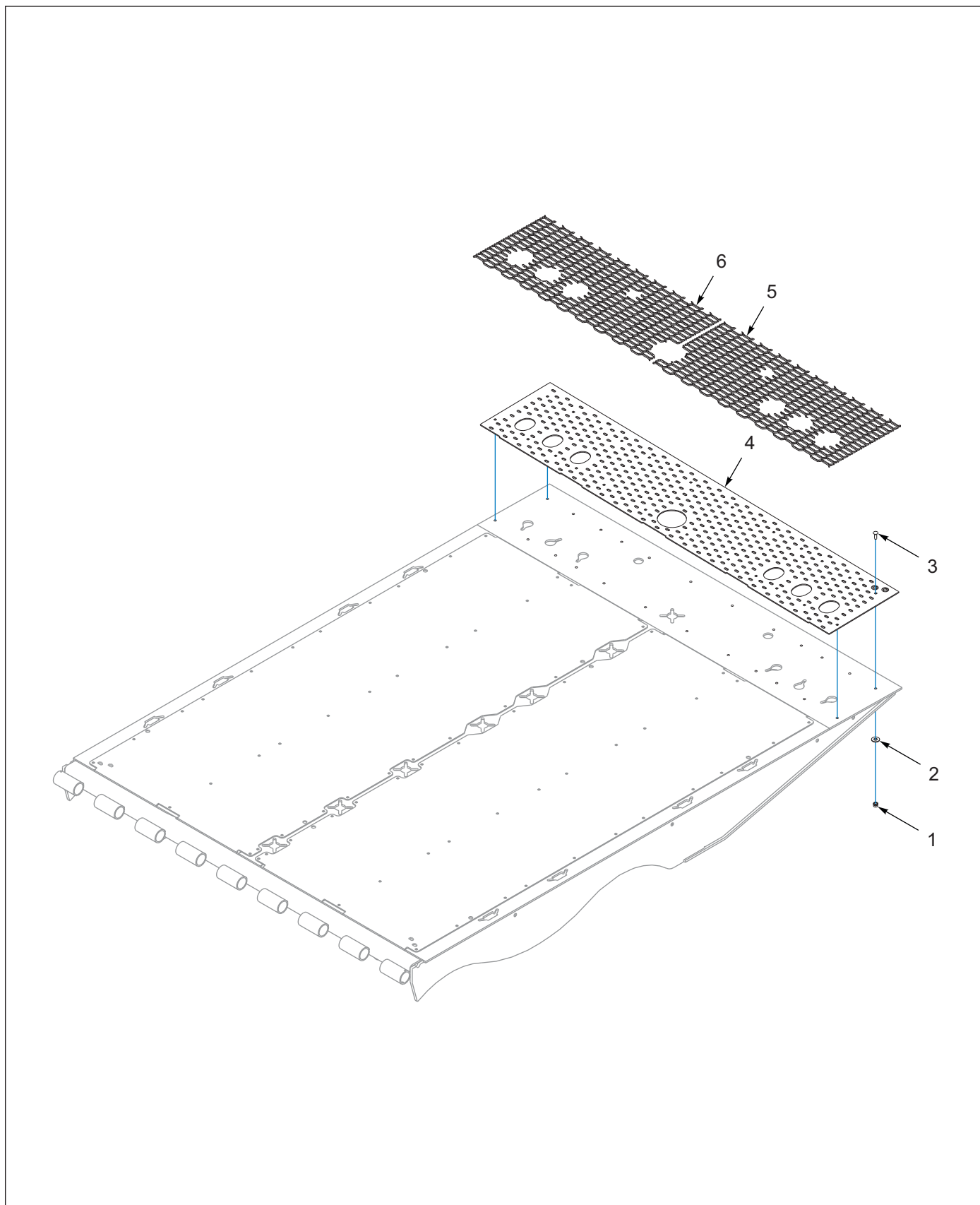
Figure 2-13: Tail Approach Plate, Tread Grip (OPTIONS)
