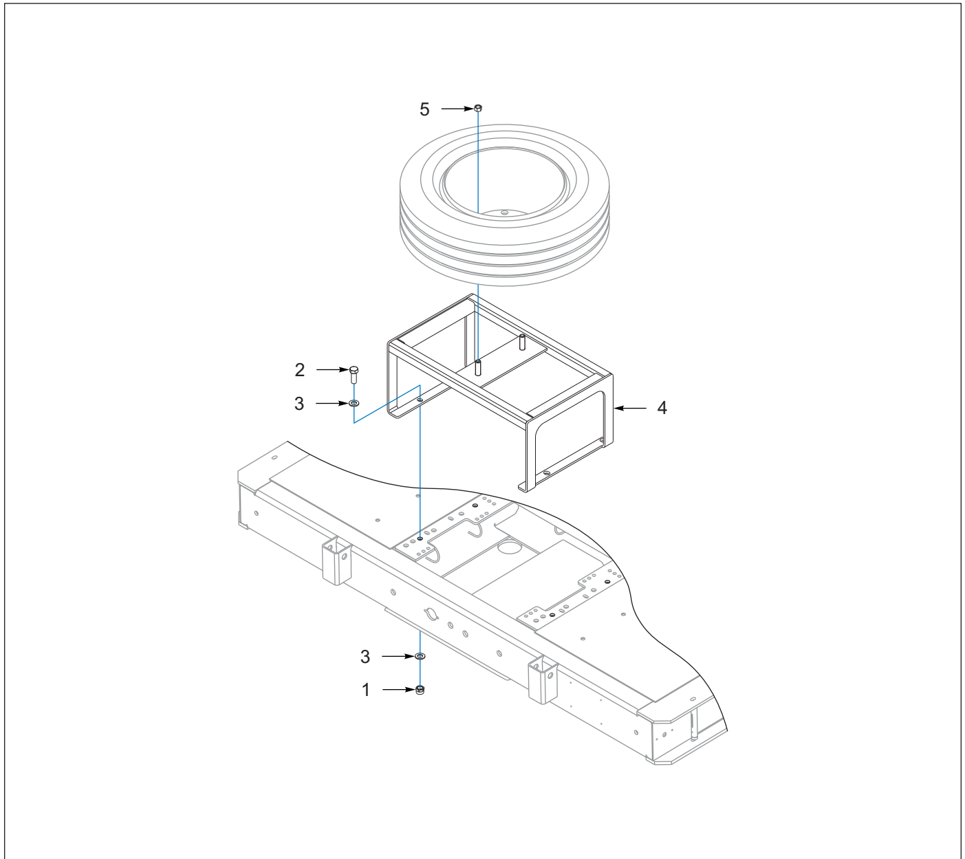
Figure 5-4: Spare Tire Mount, Upper Deck (OPTION)
