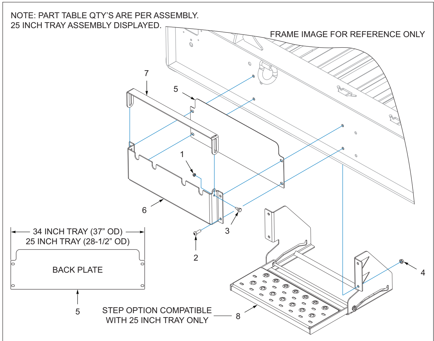
Figure 5-2: Chain Tray Assembly (AFTER 01/17/2022) (OPTIONS)
